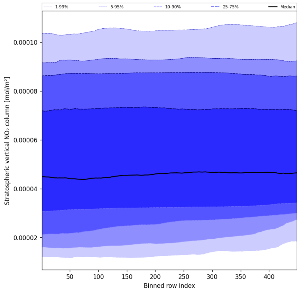
Figure 51: Along track statistics of “Stratospheric vertical NO 2 column” for 2024-12-14 to 2024-12-14
