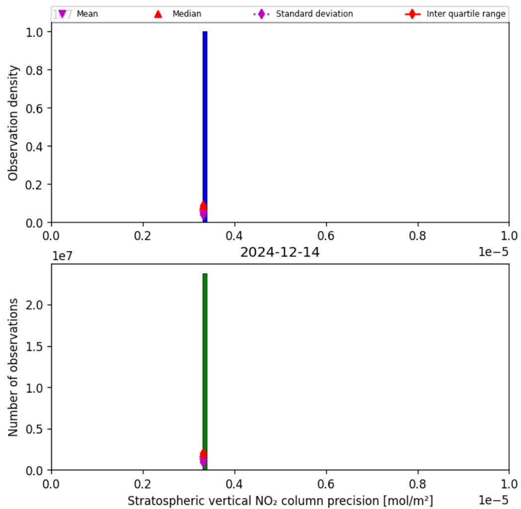
Figure 35: Histogram of “Stratospheric vertical NO 2 column precision” for 2024-12-14 to 2024-12-14
