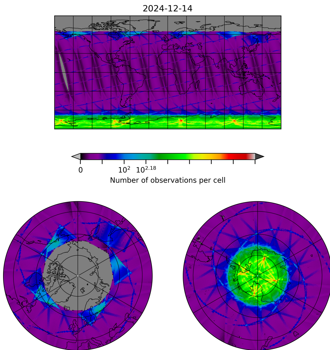
Figure 8: Map of the number of observations for 2024-12-14 to 2024-12-14
