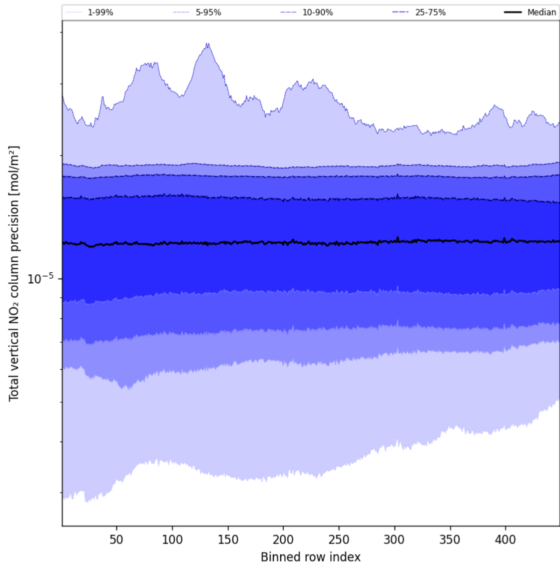
Figure 54: Along track statistics of “Total vertical NO 2 column precision” for 2024-12-14 to 2024-12-14
