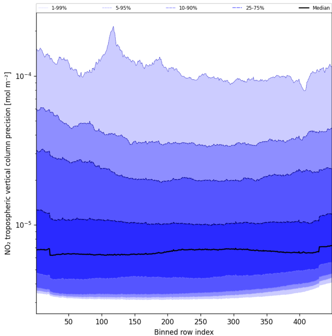
Figure 45: Along track statistics of “NO 2 tropospheric vertical column precision” for 2024-12-14 to 2024-12-14
