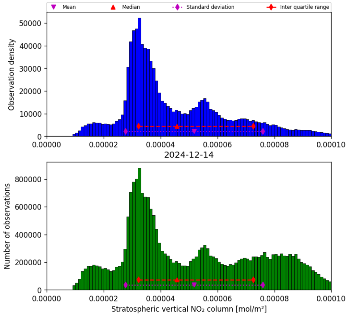
Figure 34: Histogram of “Stratospheric vertical NO 2 column” for 2024-12-14 to 2024-12-14
