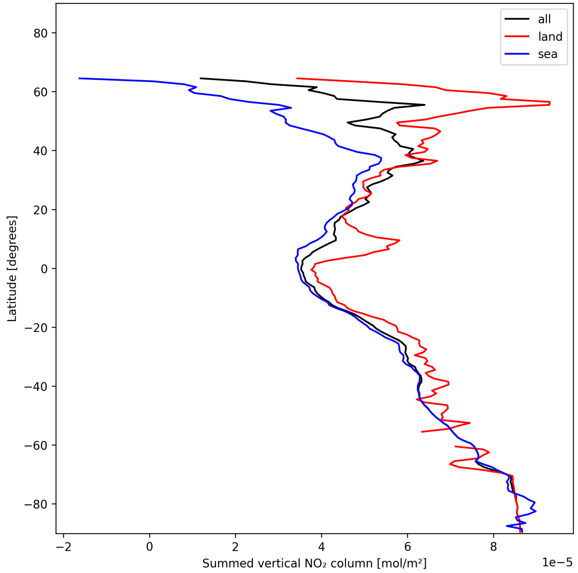
Figure 21: Zonal average of “Summed vertical NO 2 column” for 2024-12-14 to 2024-12-14.
