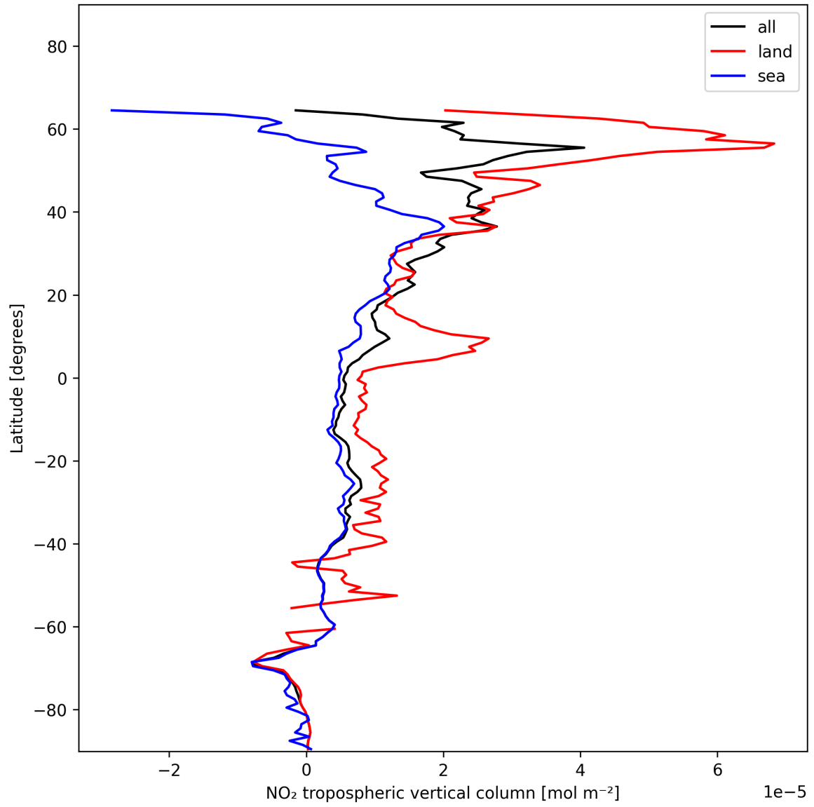
Figure 10: Zonal average of “NO 2 tropospheric vertical column” for 2024-12-14 to 2024-12-14.
