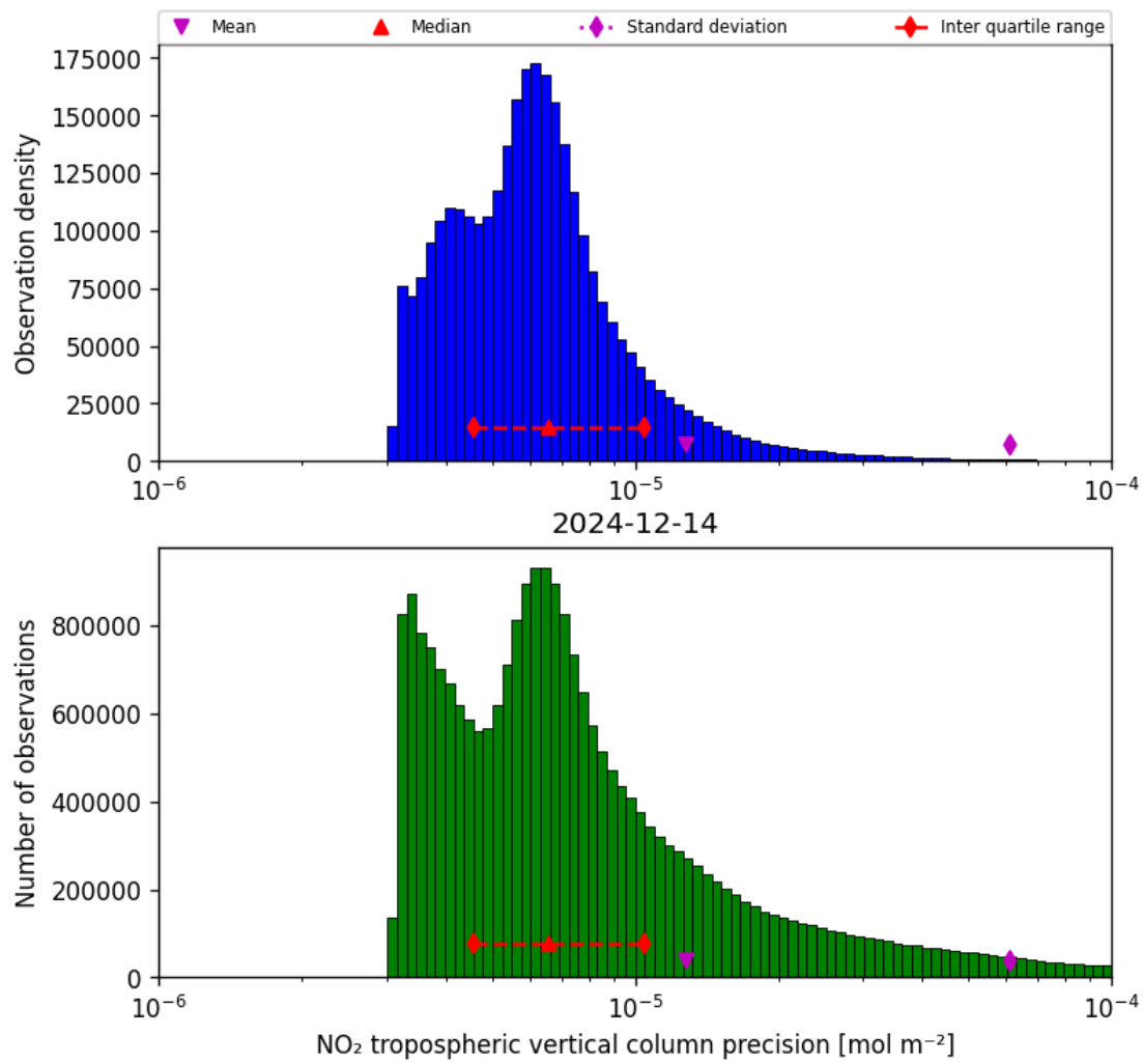
Figure 28: Histogram of “NO 2 tropospheric vertical column precision” for 2024-12-14 to 2024-12-14
