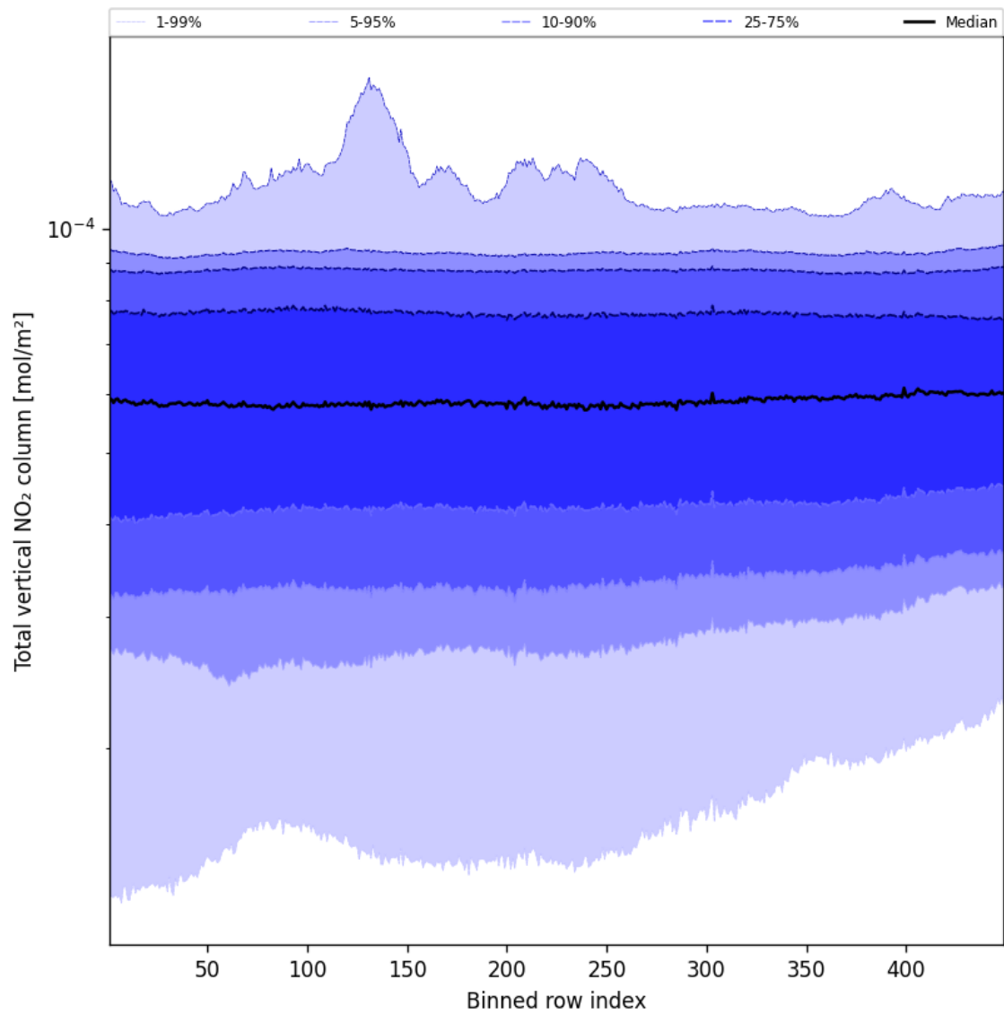
Figure 53: Along track statistics of “Total vertical NO 2 column” for 2024-12-14 to 2024-12-14
