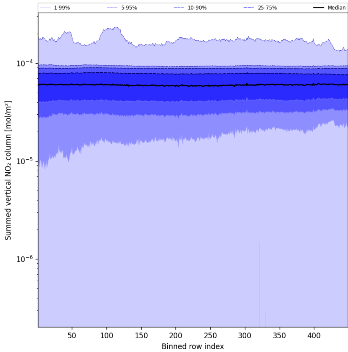
Figure 55: Along track statistics of “Summed vertical NO 2 column” for 2024-12-14 to 2024-12-14
