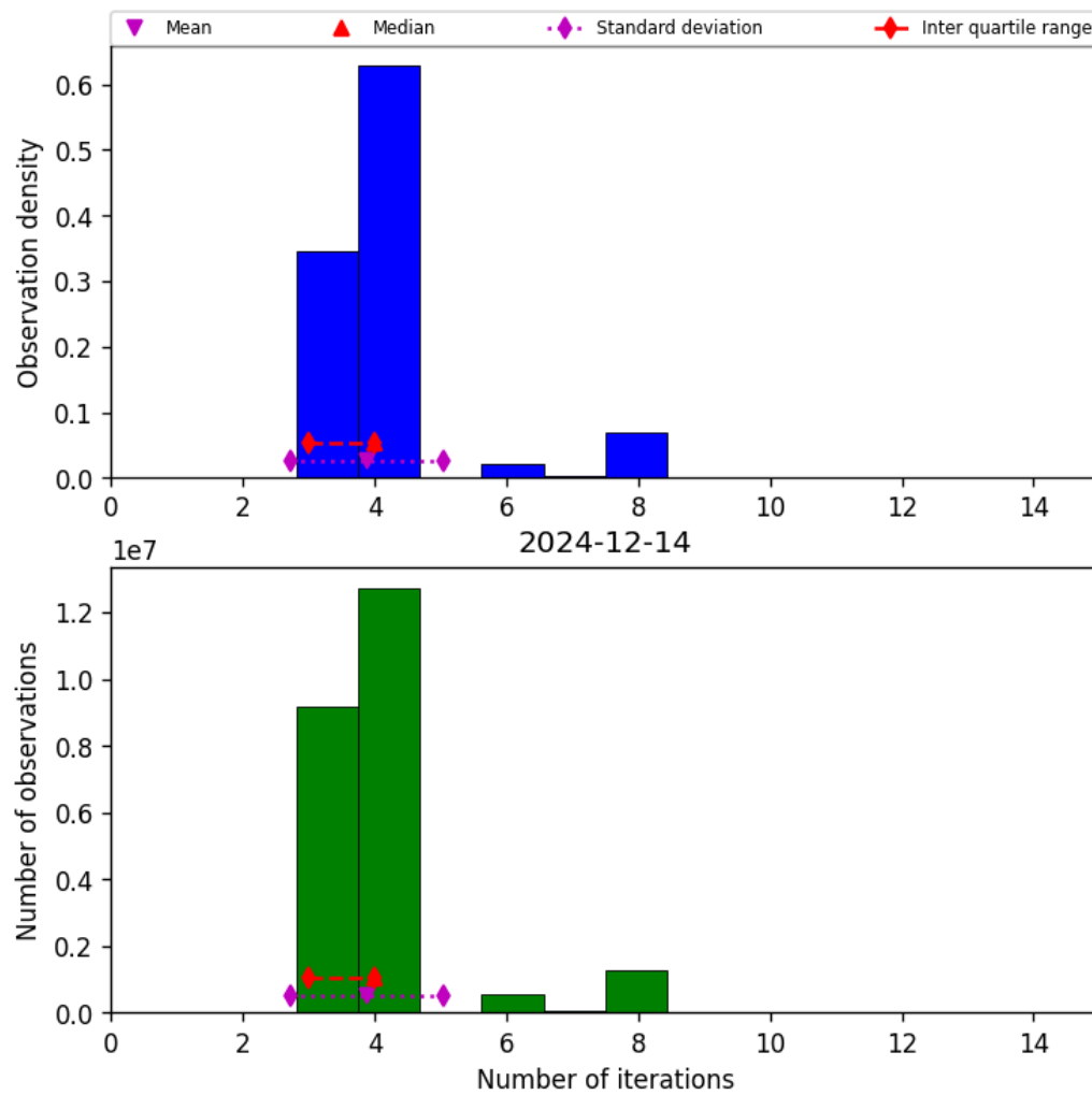
Figure 32: Histogram of “Number of iterations” for 2024-12-14 to 2024-12-14
