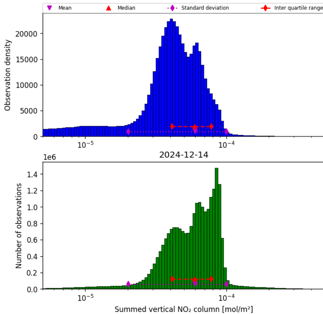
Figure 38: Histogram of “Summed vertical NO 2 column” for 2024-12-14 to 2024-12-14
