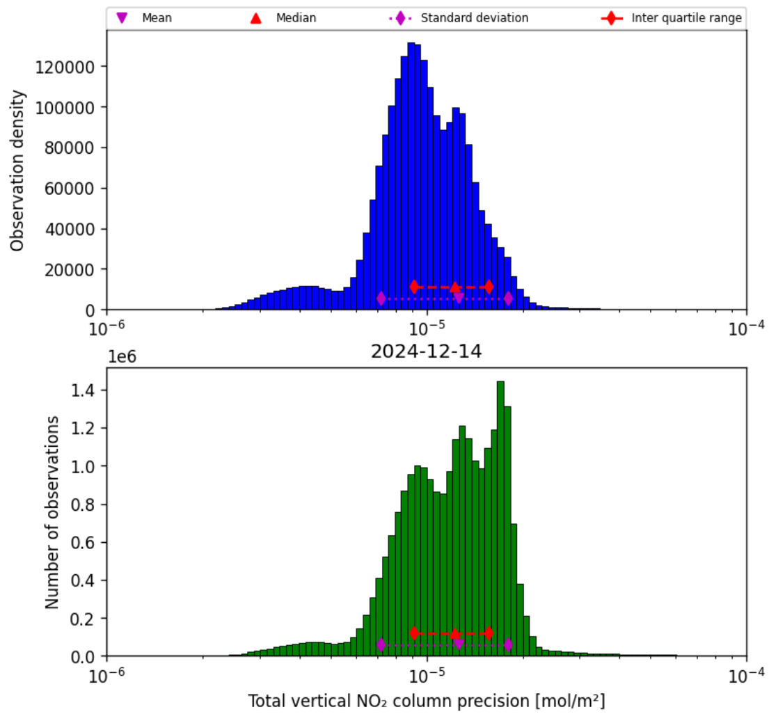
Figure 37: Histogram of “Total vertical NO 2 column precision” for 2024-12-14 to 2024-12-14
