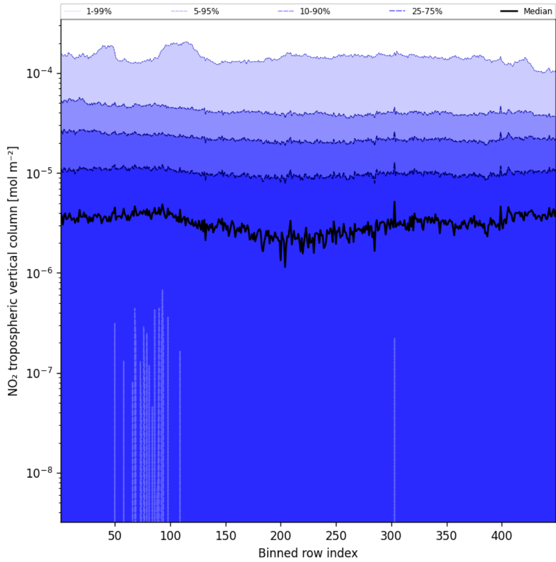
Figure 44: Along track statistics of “NO 2 tropospheric vertical column” for 2024-12-14 to 2024-12-14
