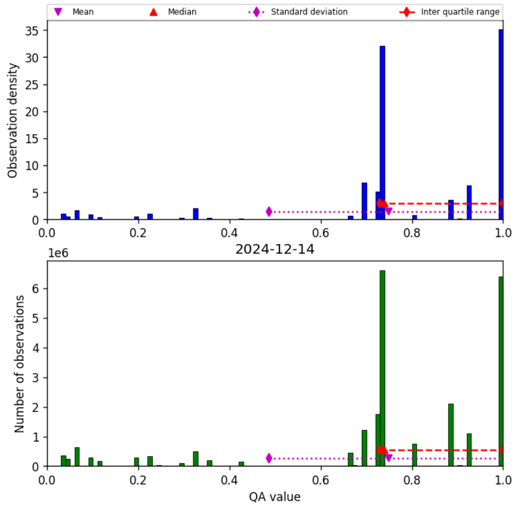
Figure 26: Histogram of “QA value” for 2024-12-14 to 2024-12-14
