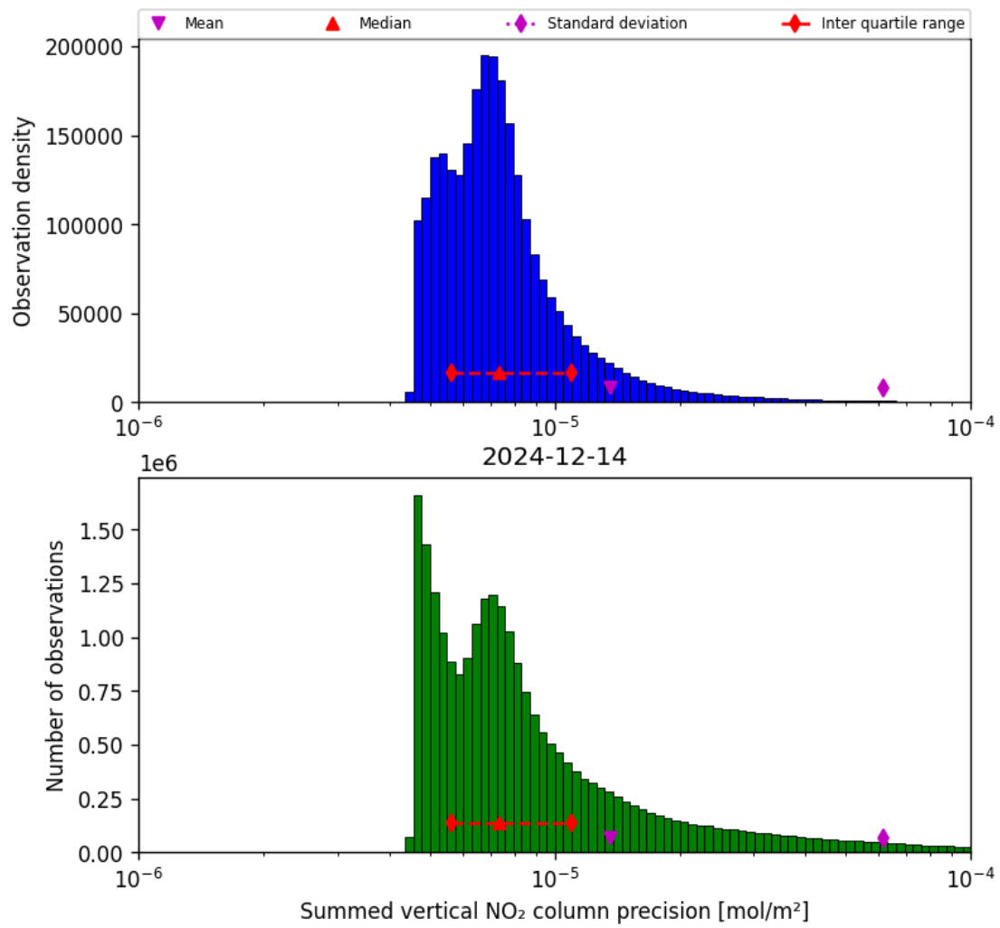
Figure 39: Histogram of “Summed vertical NO 2 column precision” for 2024-12-14 to 2024-12-14
