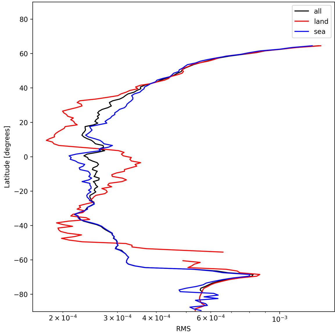
Figure 24: Zonal average of “RMS” for 2024-12-14 to 2024-12-14.
