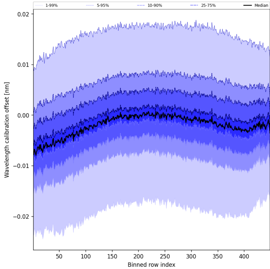
Figure 50: Along track statistics of “Wavelength calibration offset” for 2024-12-14 to 2024-12-14
