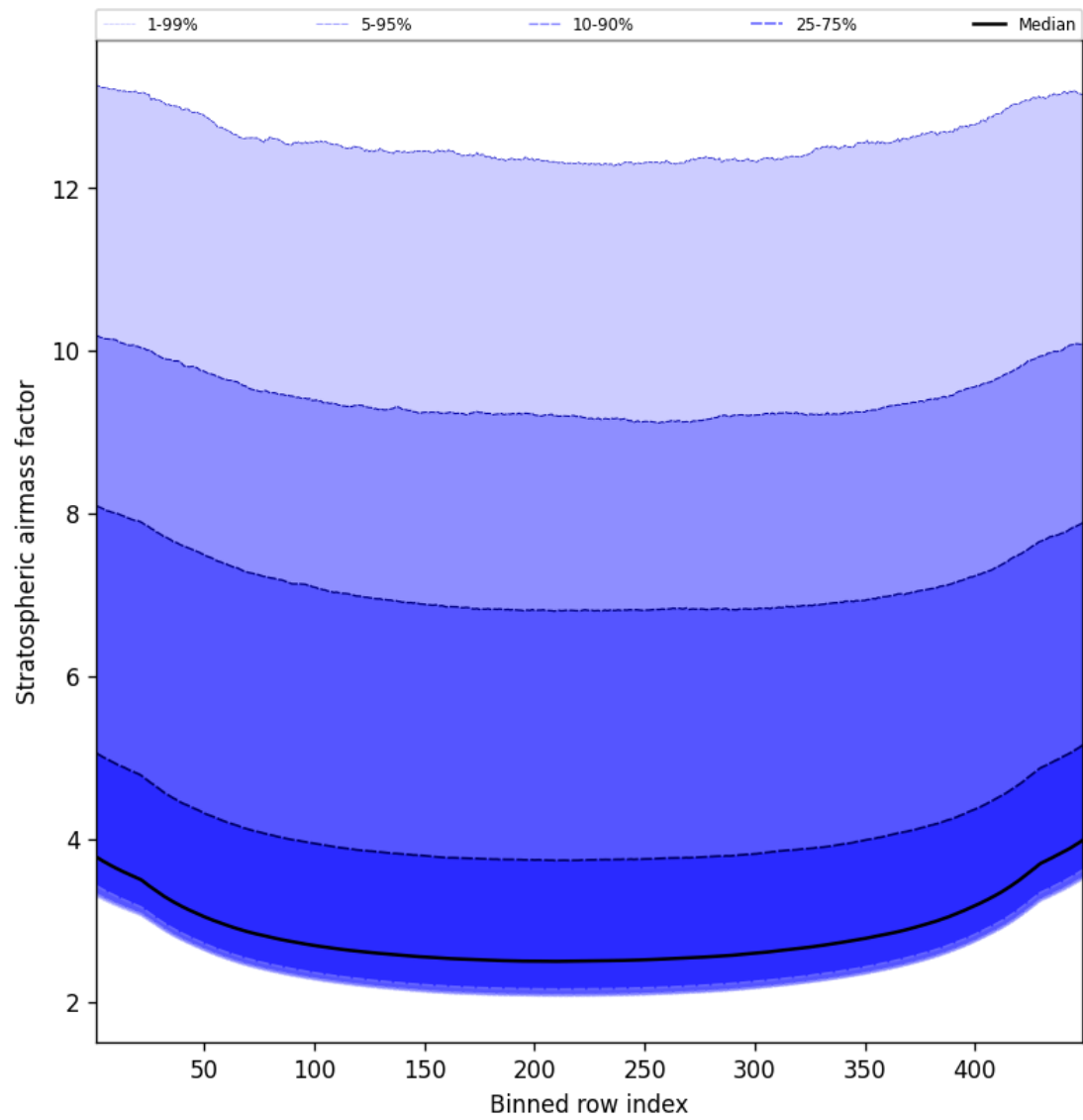
Figure 59: Along track statistics of “Stratospheric airmass factor” for 2024-12-14 to 2024-12-14
