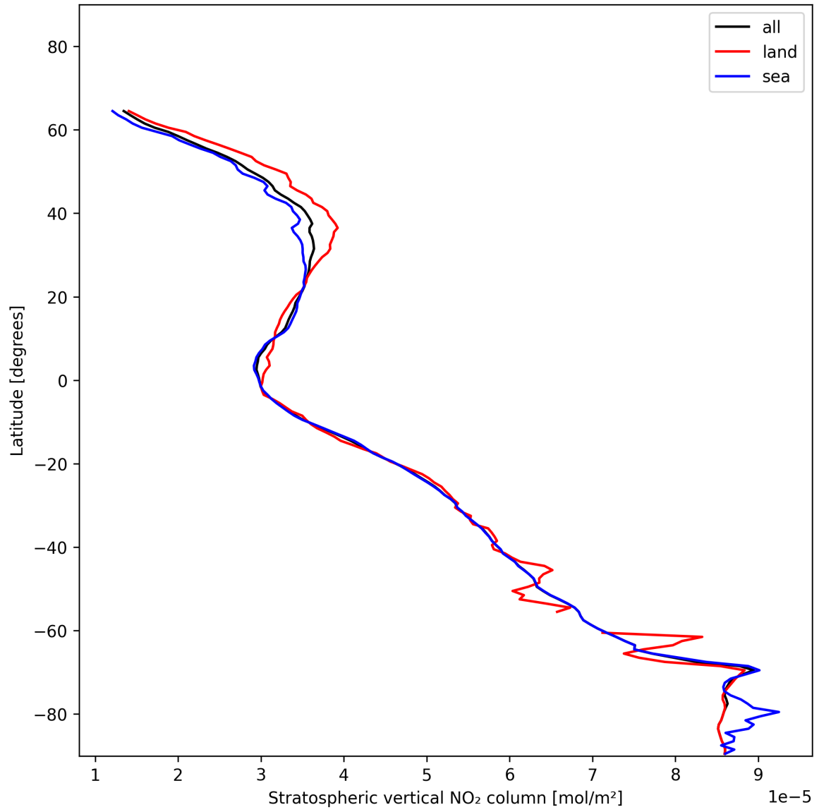
Figure 17: Zonal average of “Stratospheric vertical NO 2 column” for 2024-12-14 to 2024-12-14.
