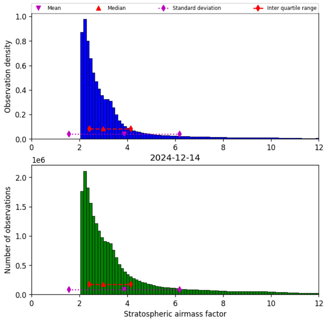
Figure 42: Histogram of “Stratospheric airmass factor” for 2024-12-14 to 2024-12-14
