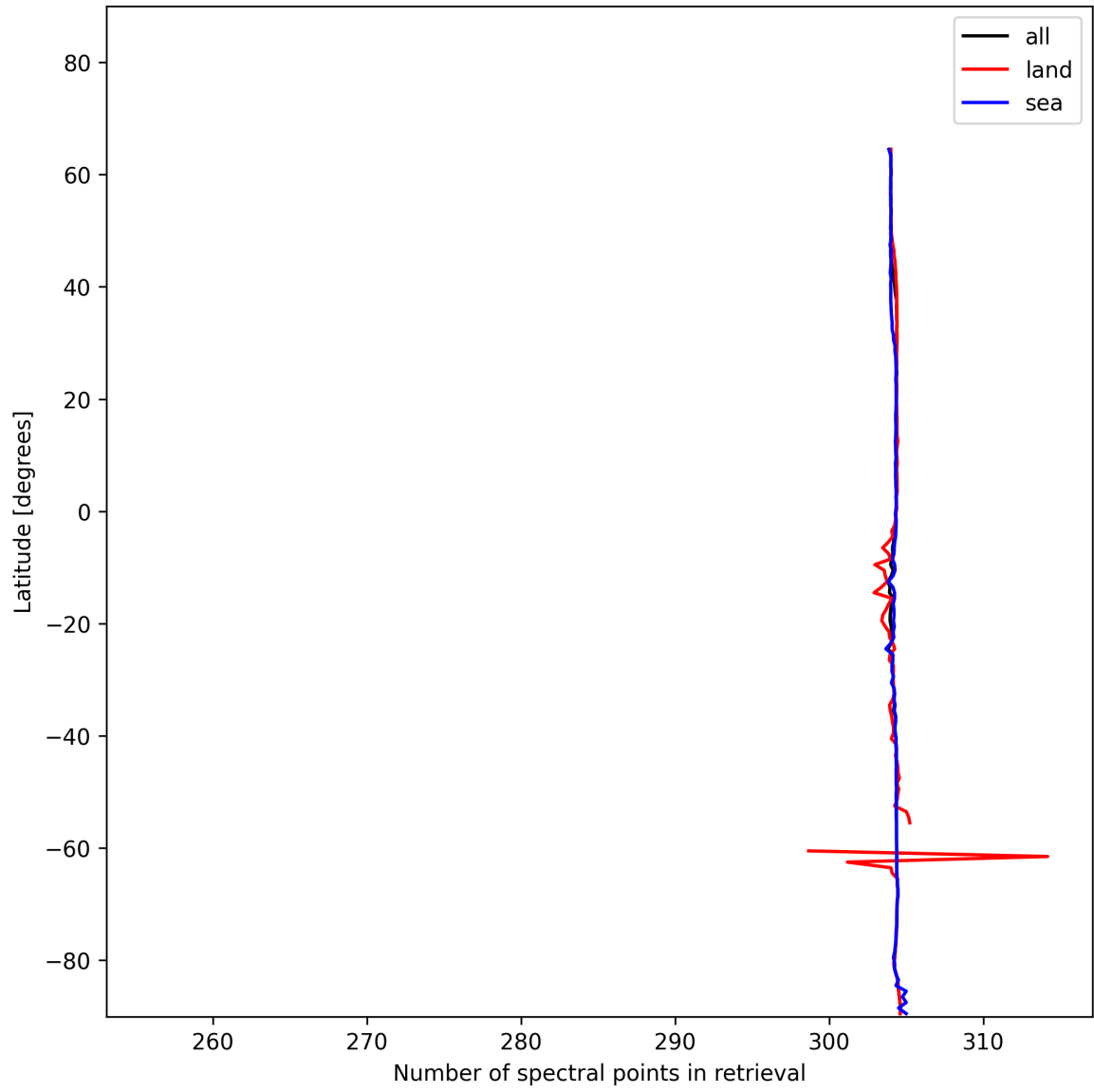
Figure 14: Zonal average of “Number of spectral points in retrieval” for 2024-12-14 to 2024-12-14.
