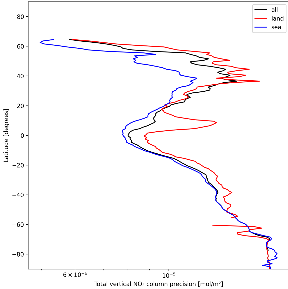
Figure 20: Zonal average of “Total vertical NO 2 column precision” for 2024-12-14 to 2024-12-14.
