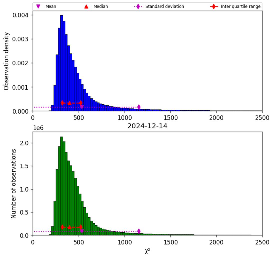
Figure 40: Histogram of “ \chi^2 ” for 2024-12-14 to 2024-12-14
