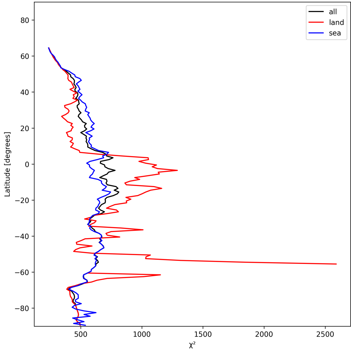
Figure 23: Zonal average of “ \chi^2 ” for 2024-12-14 to 2024-12-14.
