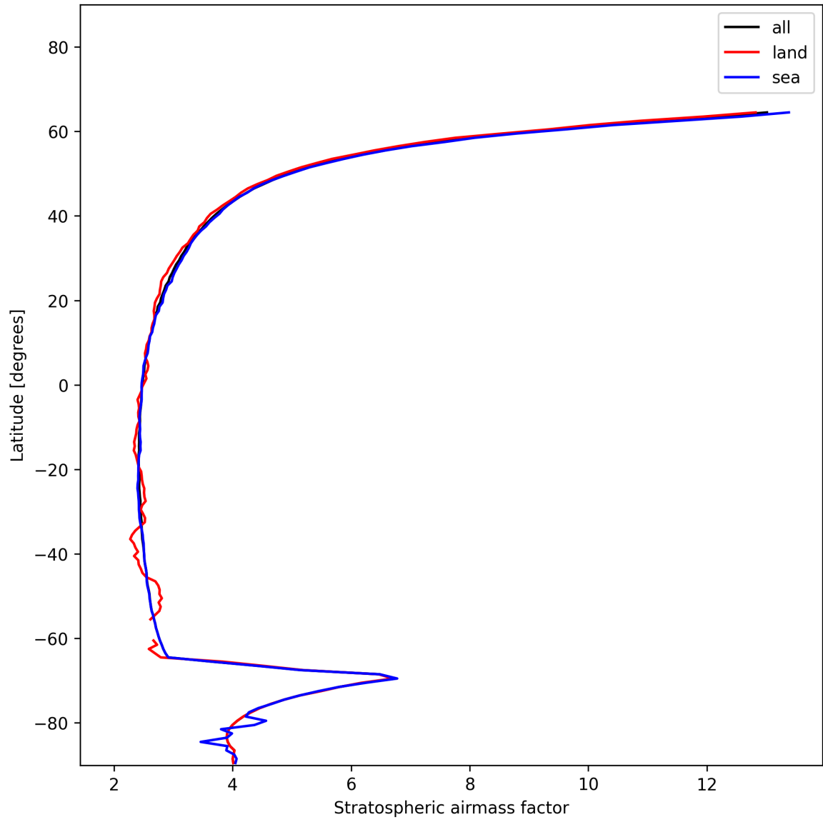
Figure 25: Zonal average of “Stratospheric airmass factor” for 2024-12-14 to 2024-12-14.
