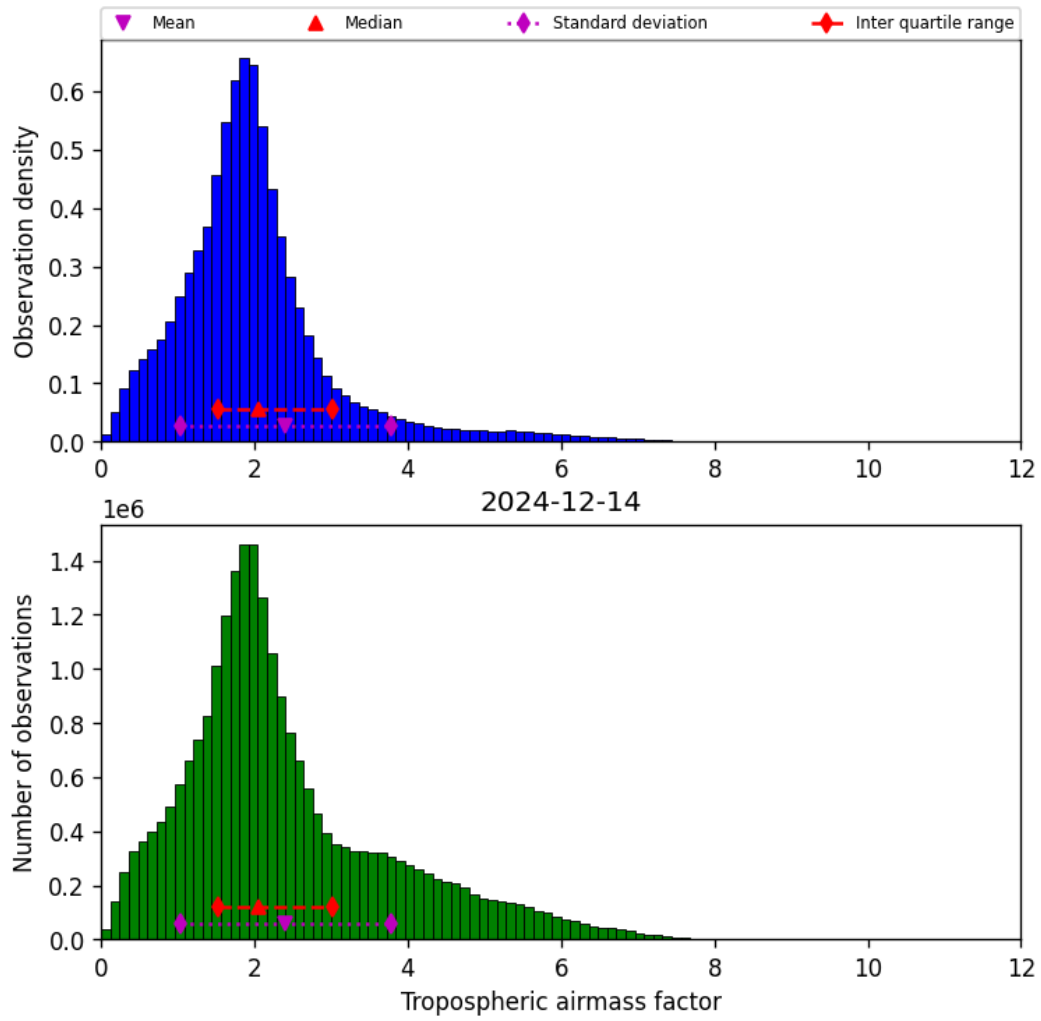
Figure 29: Histogram of “Tropospheric airmass factor” for 2024-12-14 to 2024-12-14
