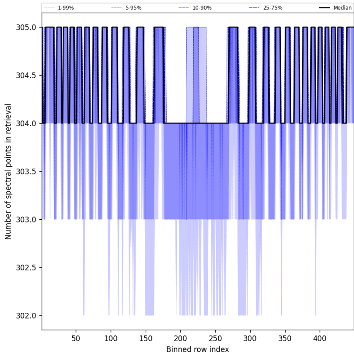
Figure 48: Along track statistics of “Number of spectral points in retrieval” for 2024-12-14 to 2024-12-14
