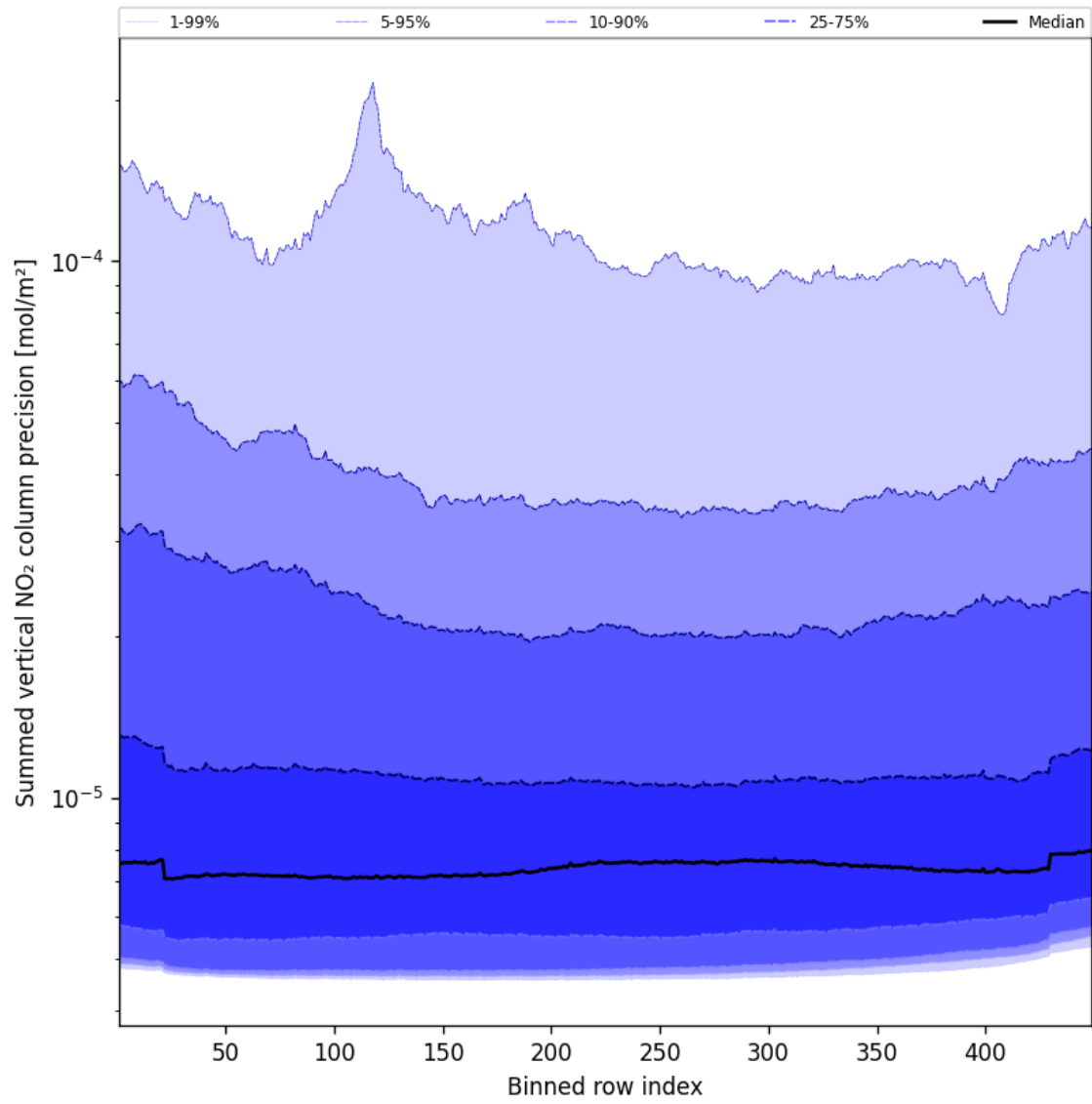
Figure 56: Along track statistics of “Summed vertical NO 2 column precision” for 2024-12-14 to 2024-12-14
