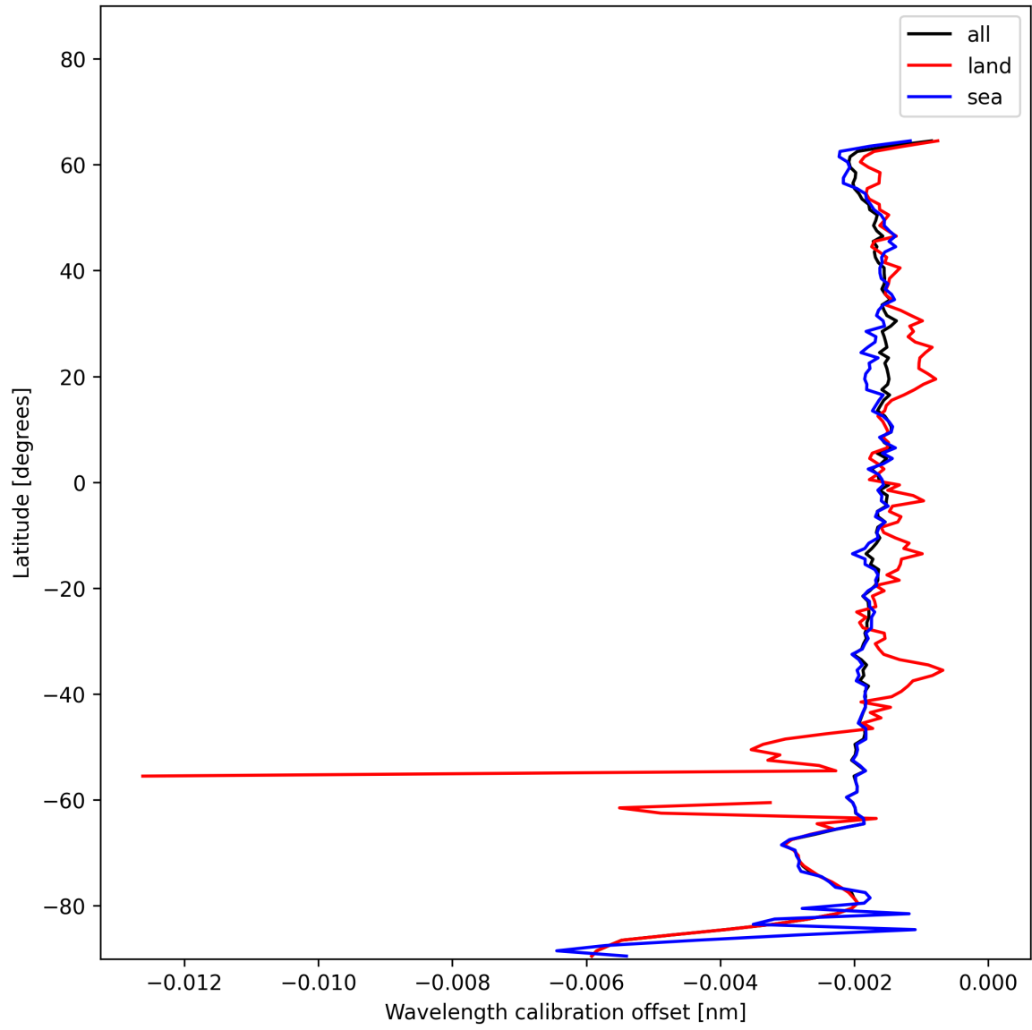
Figure 16: Zonal average of “Wavelength calibration offset” for 2024-12-14 to 2024-12-14.
