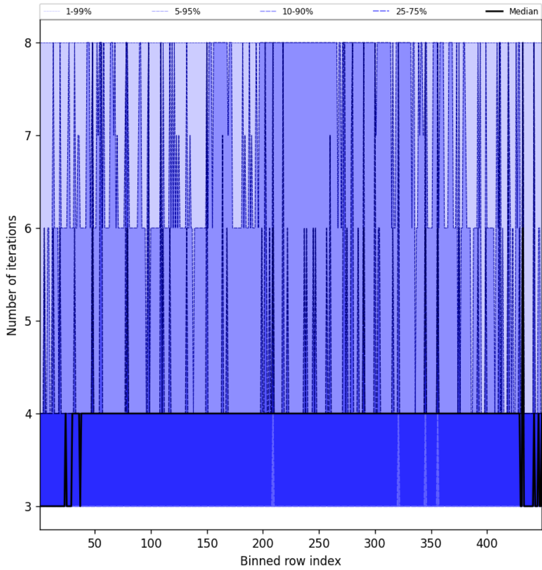
Figure 49: Along track statistics of “Number of iterations” for 2024-12-14 to 2024-12-14
