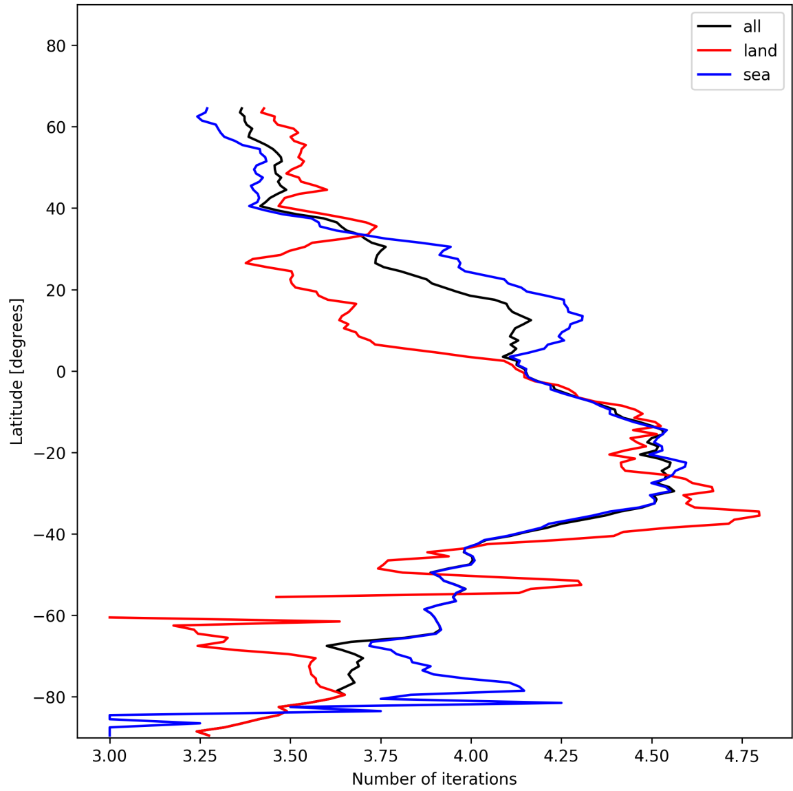
Figure 15: Zonal average of “Number of iterations” for 2024-12-14 to 2024-12-14.
