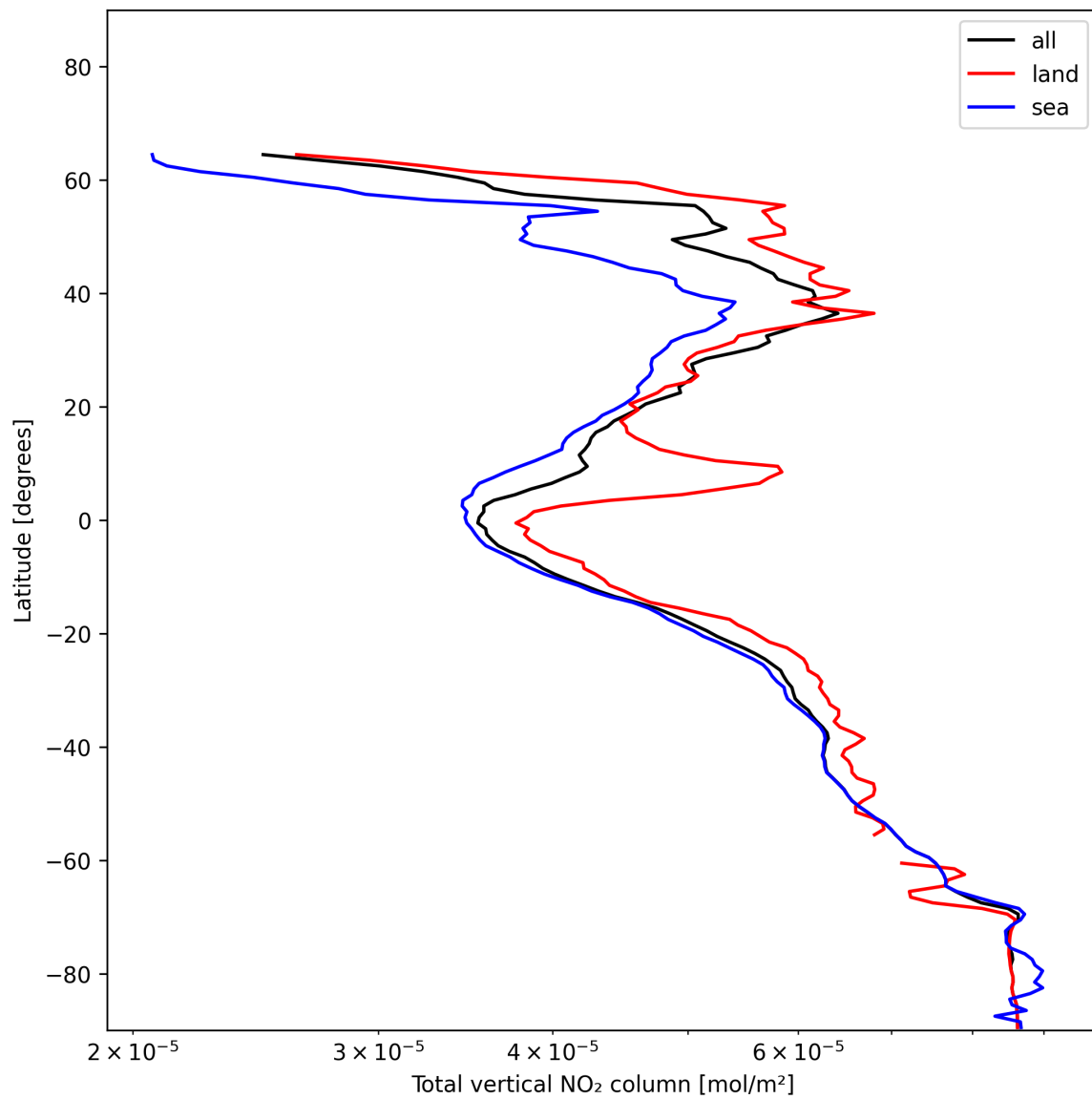
Figure 19: Zonal average of “Total vertical NO 2 column” for 2024-12-14 to 2024-12-14.
