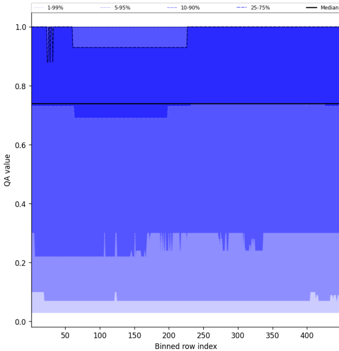
Figure 43: Along track statistics of “QA value” for 2024-12-14 to 2024-12-14
