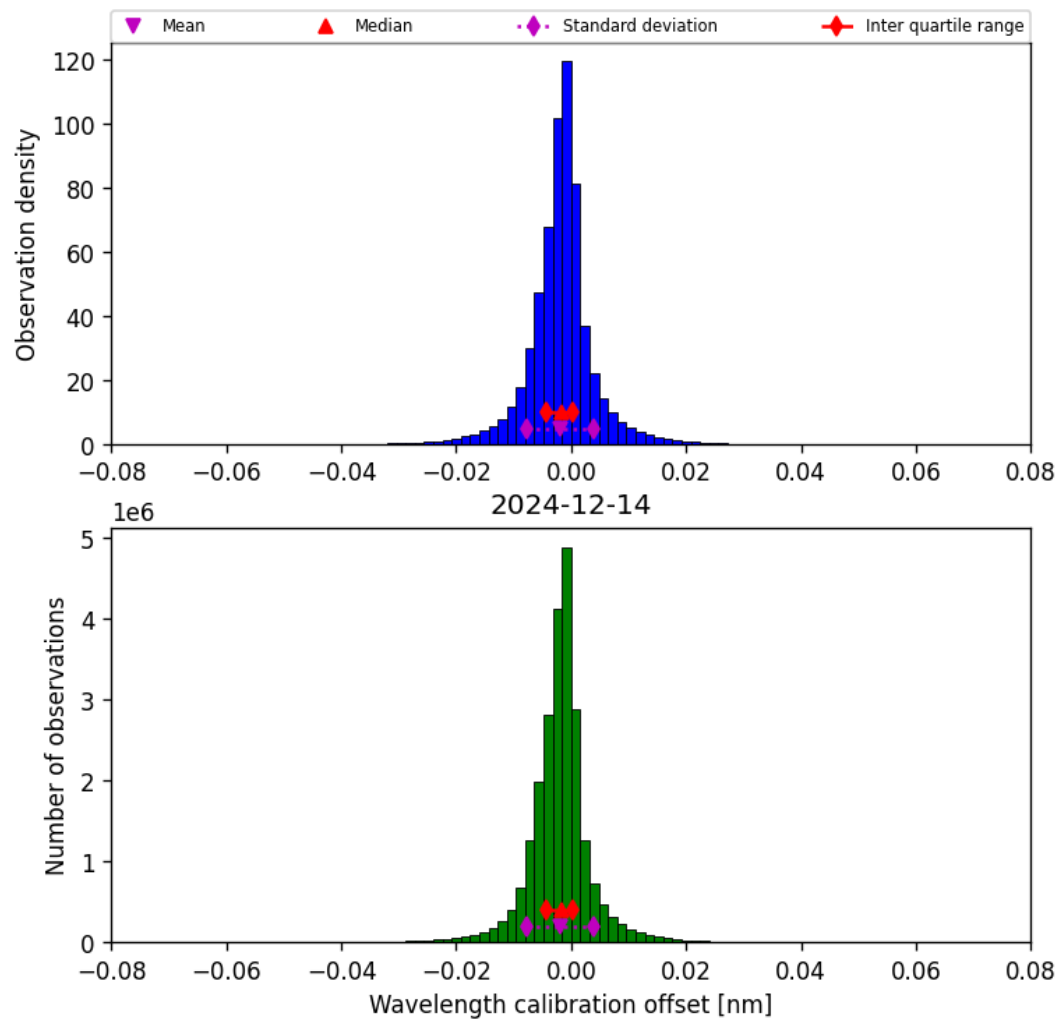
Figure 33: Histogram of “Wavelength calibration offset” for 2024-12-14 to 2024-12-14
