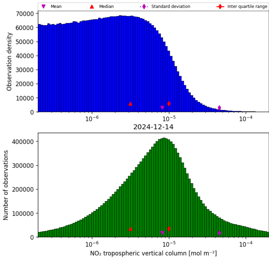
Figure 27: Histogram of “NO 2 tropospheric vertical column” for 2024-12-14 to 2024-12-14
