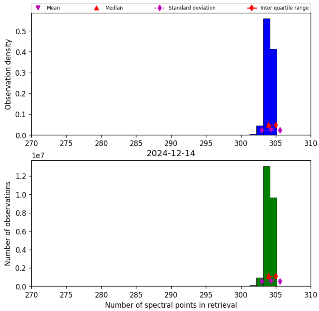
Figure 31: Histogram of “Number of spectral points in retrieval” for 2024-12-14 to 2024-12-14
