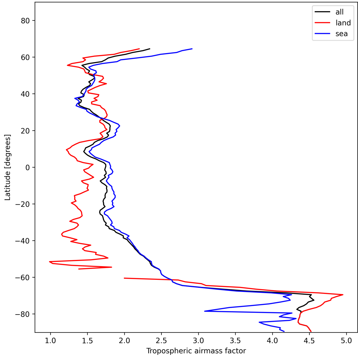
Figure 12: Zonal average of “Tropospheric airmass factor” for 2024-12-14 to 2024-12-14.
