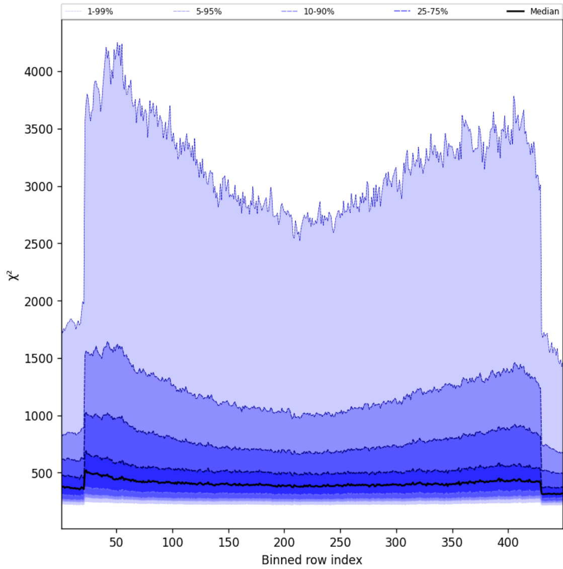
Figure 57: Along track statistics of “ \chi^2 ” for 2024-12-14 to 2024-12-14
