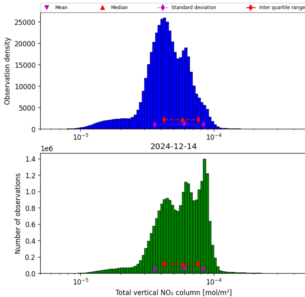
Figure 36: Histogram of “Total vertical NO 2 column” for 2024-12-14 to 2024-12-14
