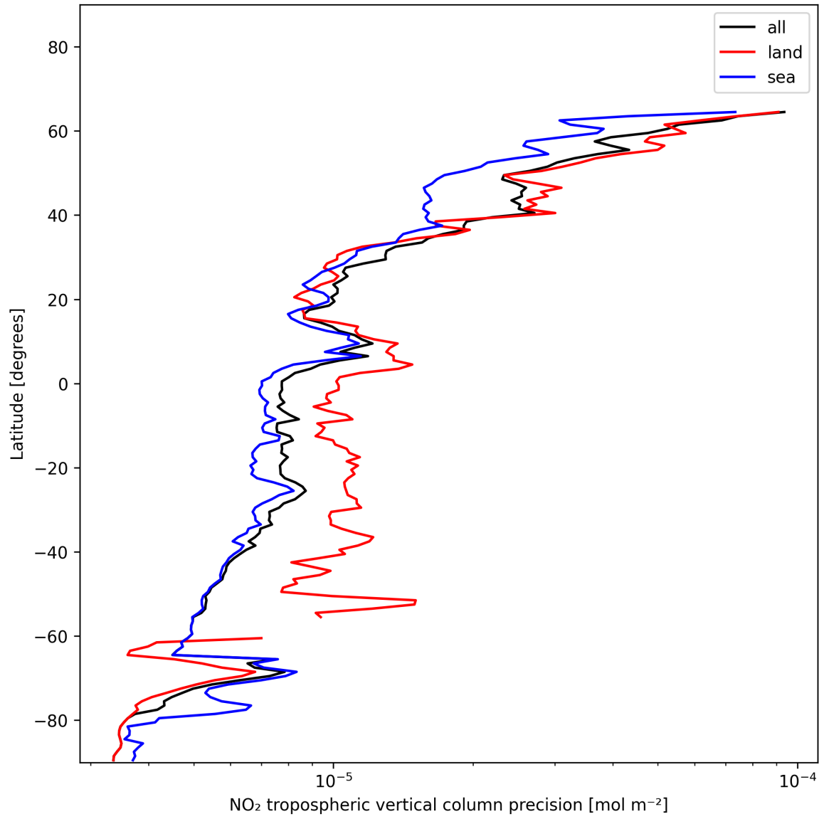
Figure 11: Zonal average of “NO 2 tropospheric vertical column precision” for 2024-12-14 to 2024-12-14.
