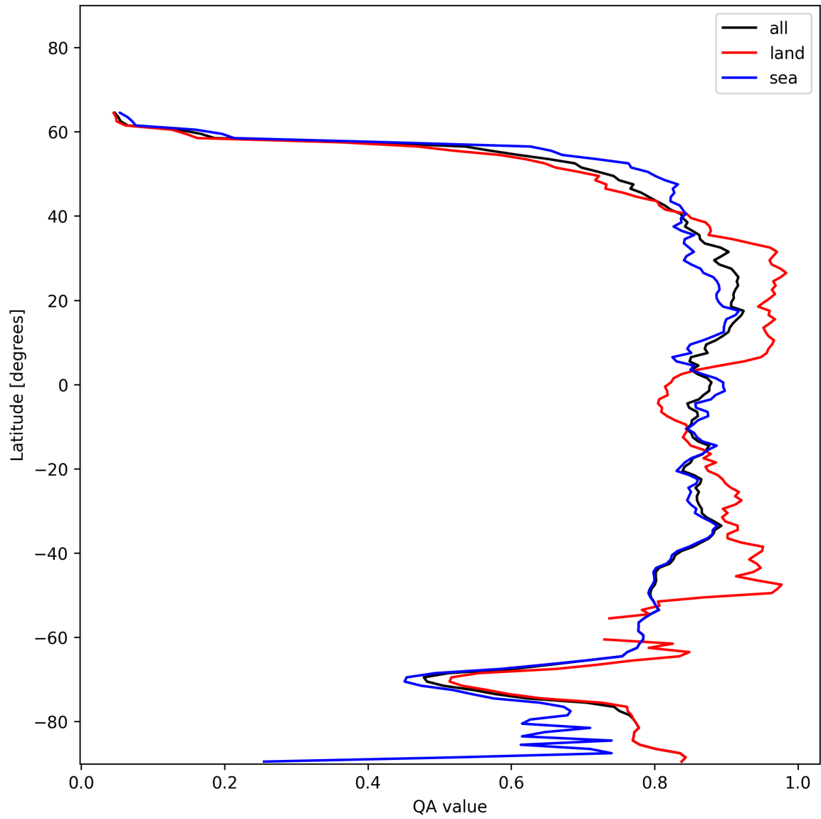
Figure 9: Zonal average of “QA value” for 2024-12-14 to 2024-12-14.
