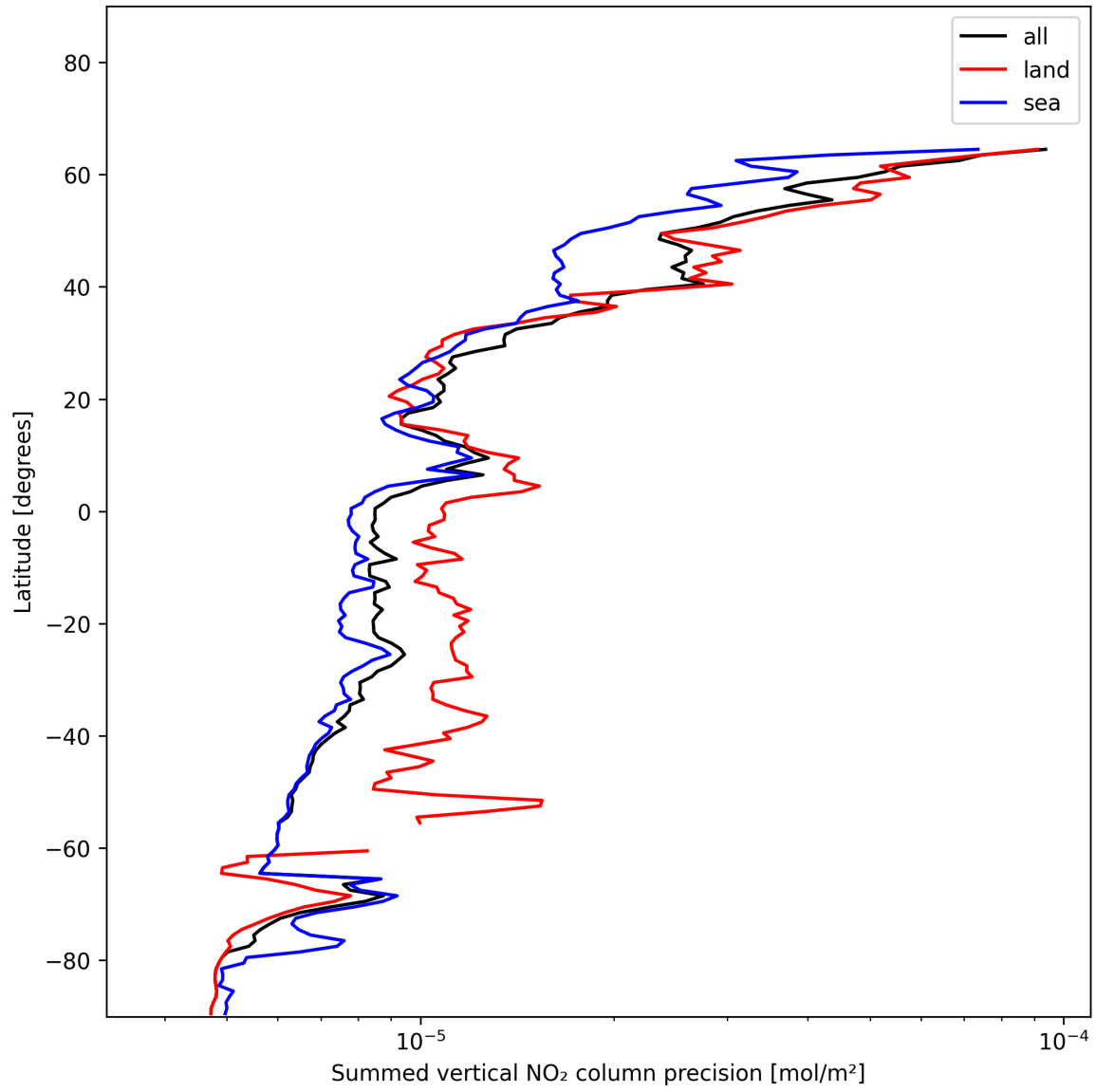
Figure 22: Zonal average of “Summed vertical NO 2 column precision” for 2024-12-14 to 2024-12-14.
