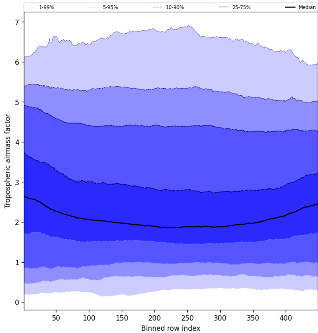
Figure 46: Along track statistics of “Tropospheric air mass factor” for 2024-12-14 to 2024-12-14
