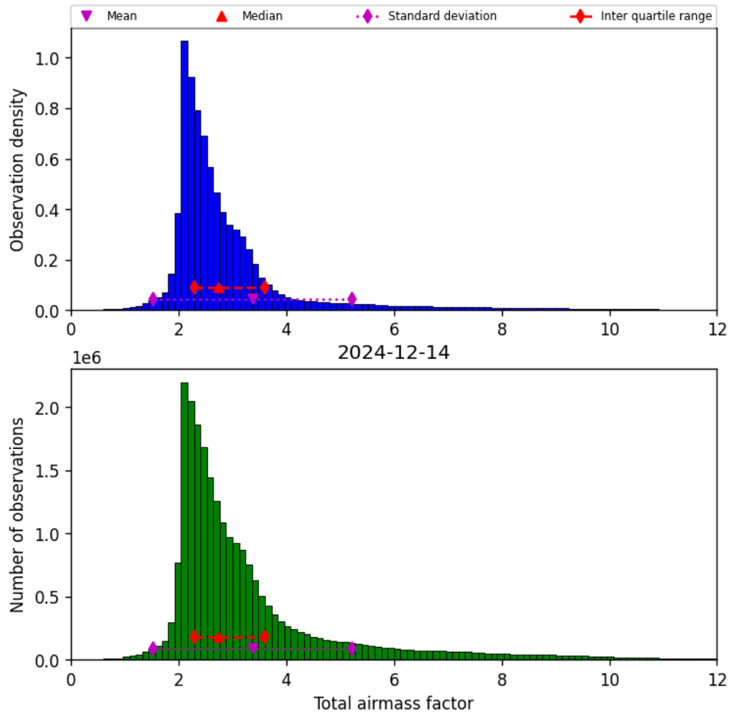
Figure 30: Histogram of “Total airmass factor” for 2024-12-14 to 2024-12-14
