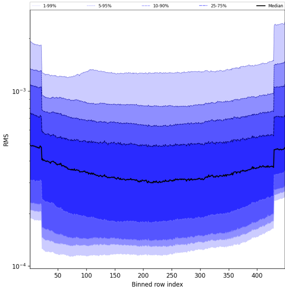
Figure 58: Along track statistics of “RMS” for 2024-12-14 to 2024-12-14
