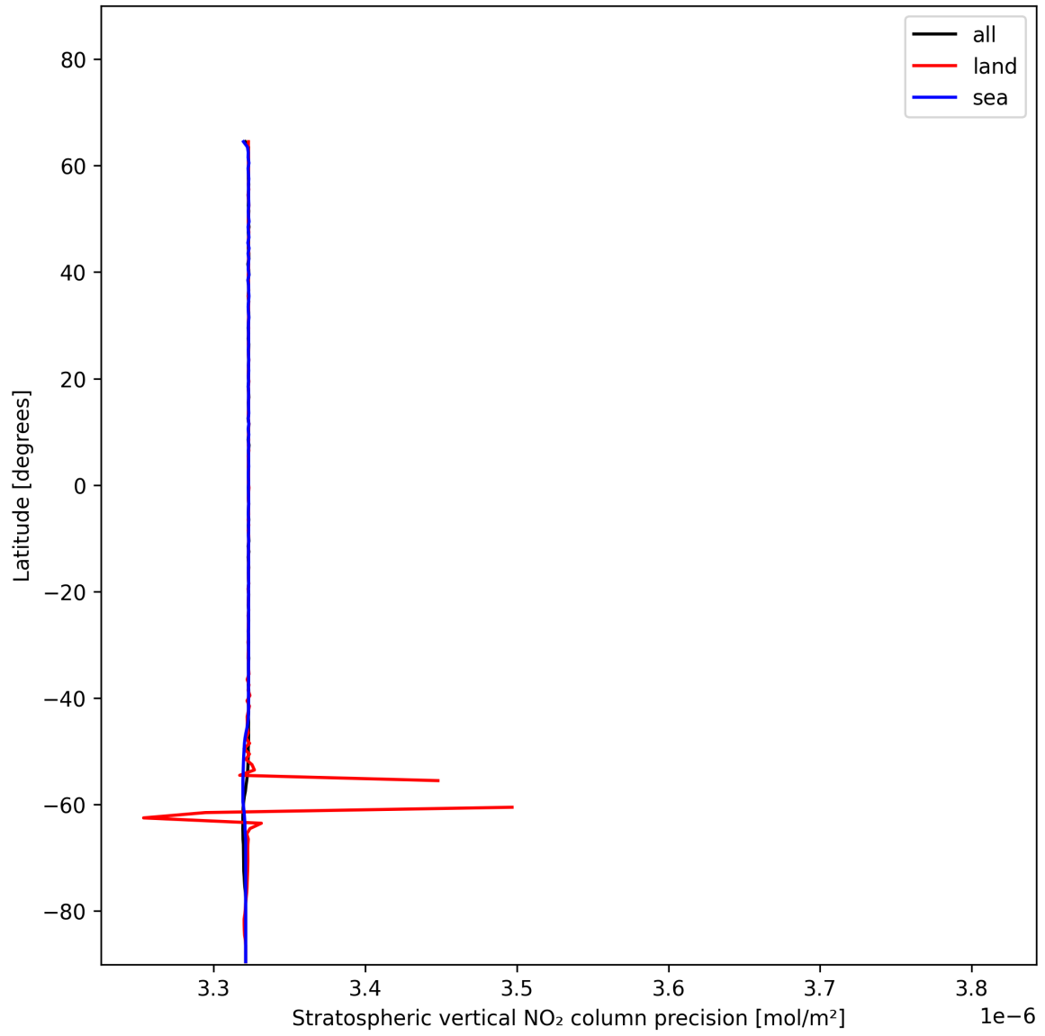
Figure 18: Zonal average of “Stratospheric vertical NO 2 column precision” for 2024-12-14 to 2024-12-14.
