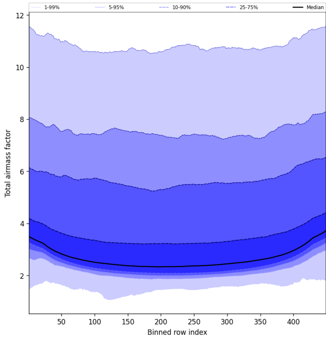
Figure 47: Along track statistics of “Total airmass factor” for 2024-12-14 to 2024-12-14
