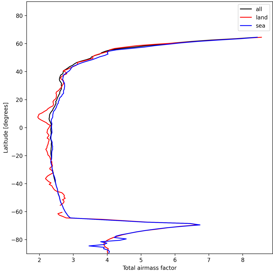
Figure 13: Zonal average of “Total airmass factor” for 2024-12-14 to 2024-12-14.
