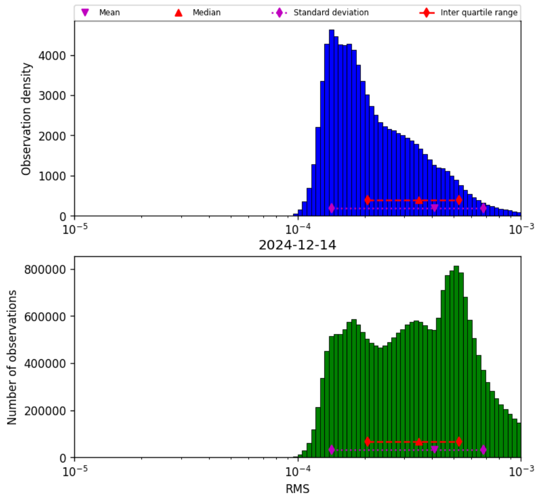
Figure 41: Histogram of “RMS” for 2024-12-14 to 2024-12-14
