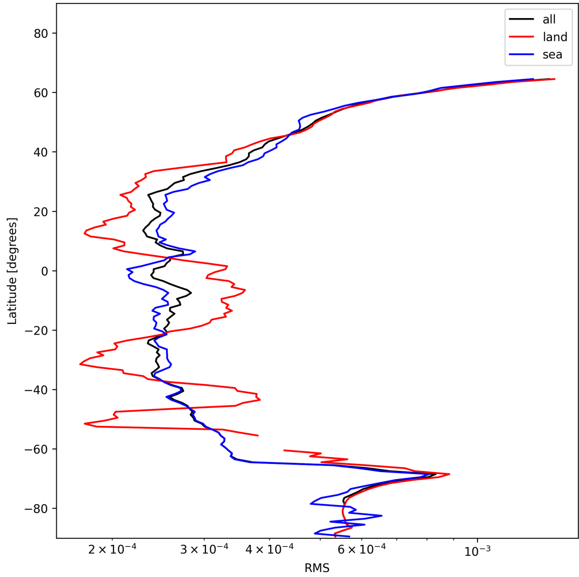
Figure 24: Zonal average of “RMS” for 2024-12-16 to 2024-12-17.
