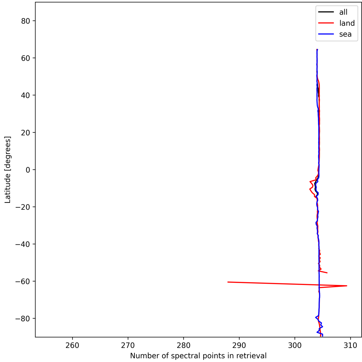
Figure 14: Zonal average of “Number of spectral points in retrieval” for 2024-12-16 to 2024-12-17.
