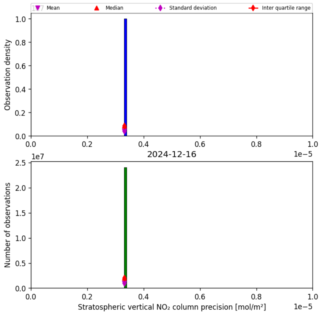
Figure 35: Histogram of “Stratospheric vertical NO 2 column precision” for 2024-12-16 to 2024-12-17
