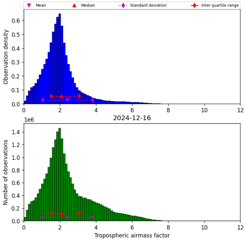
Figure 29: Histogram of “Tropospheric airmass factor” for 2024-12-16 to 2024-12-17
