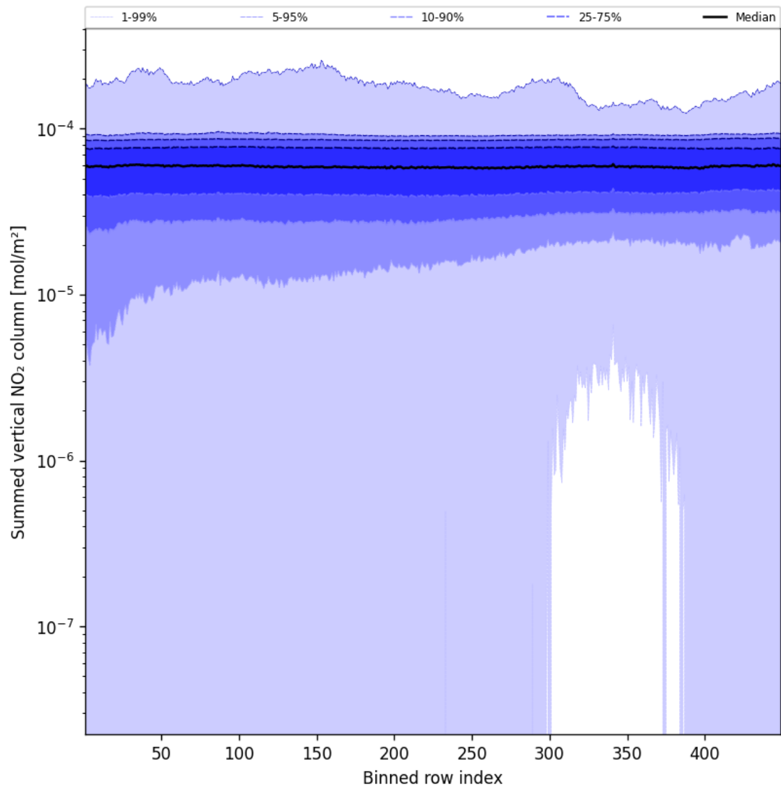
Figure 55: Along track statistics of “Summed vertical NO 2 column” for 2024-12-16 to 2024-12-17
