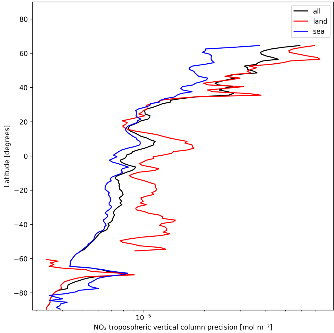
Figure 11: Zonal average of “NO 2 tropospheric vertical column precision” for 2024-12-16 to 2024-12-17.
