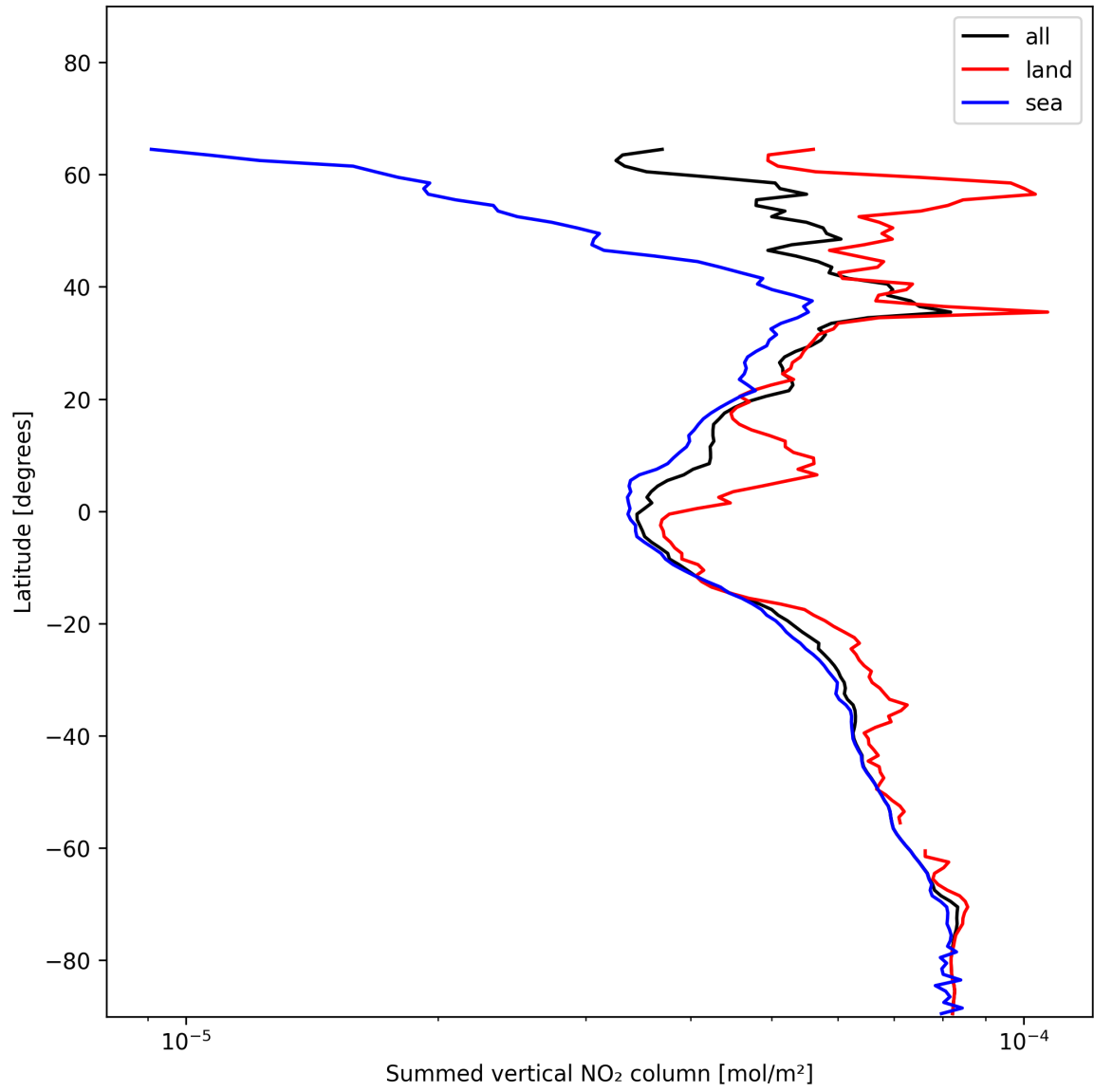
Figure 21: Zonal average of “Summed vertical NO 2 column” for 2024-12-16 to 2024-12-17.
