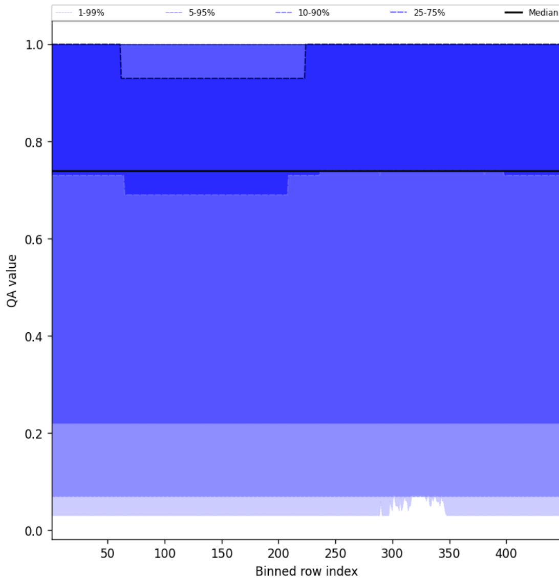
Figure 43: Along track statistics of “QA value” for 2024-12-16 to 2024-12-17
