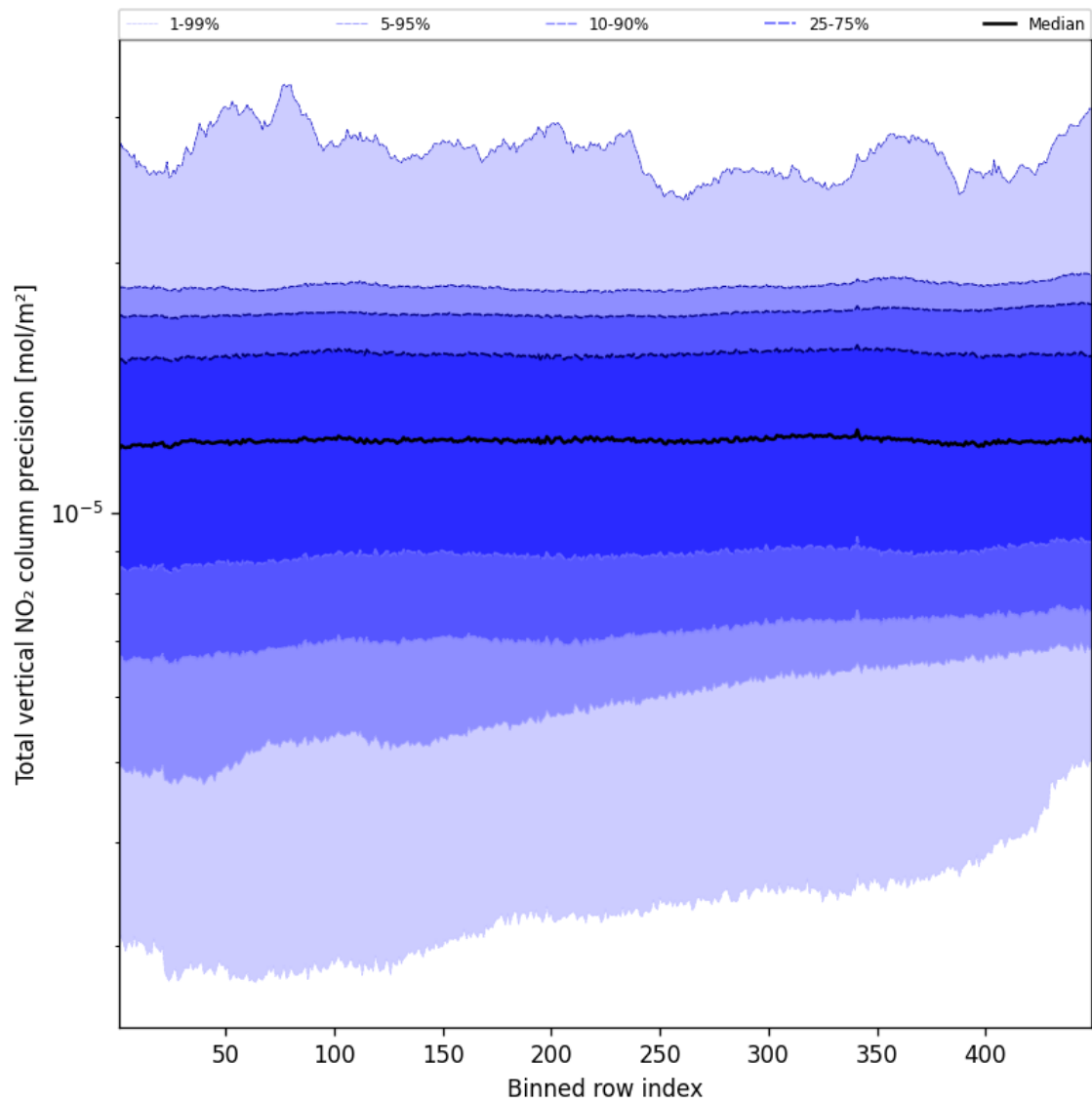
Figure 54: Along track statistics of “Total vertical NO 2 column precision” for 2024-12-16 to 2024-12-17
