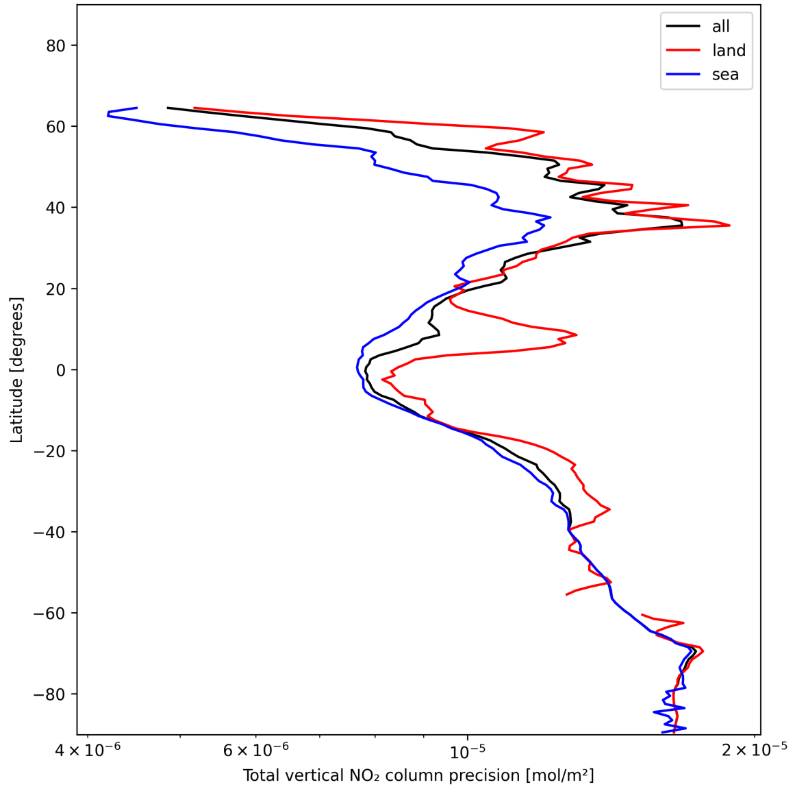
Figure 20: Zonal average of “Total vertical NO 2 column precision” for 2024-12-16 to 2024-12-17.
