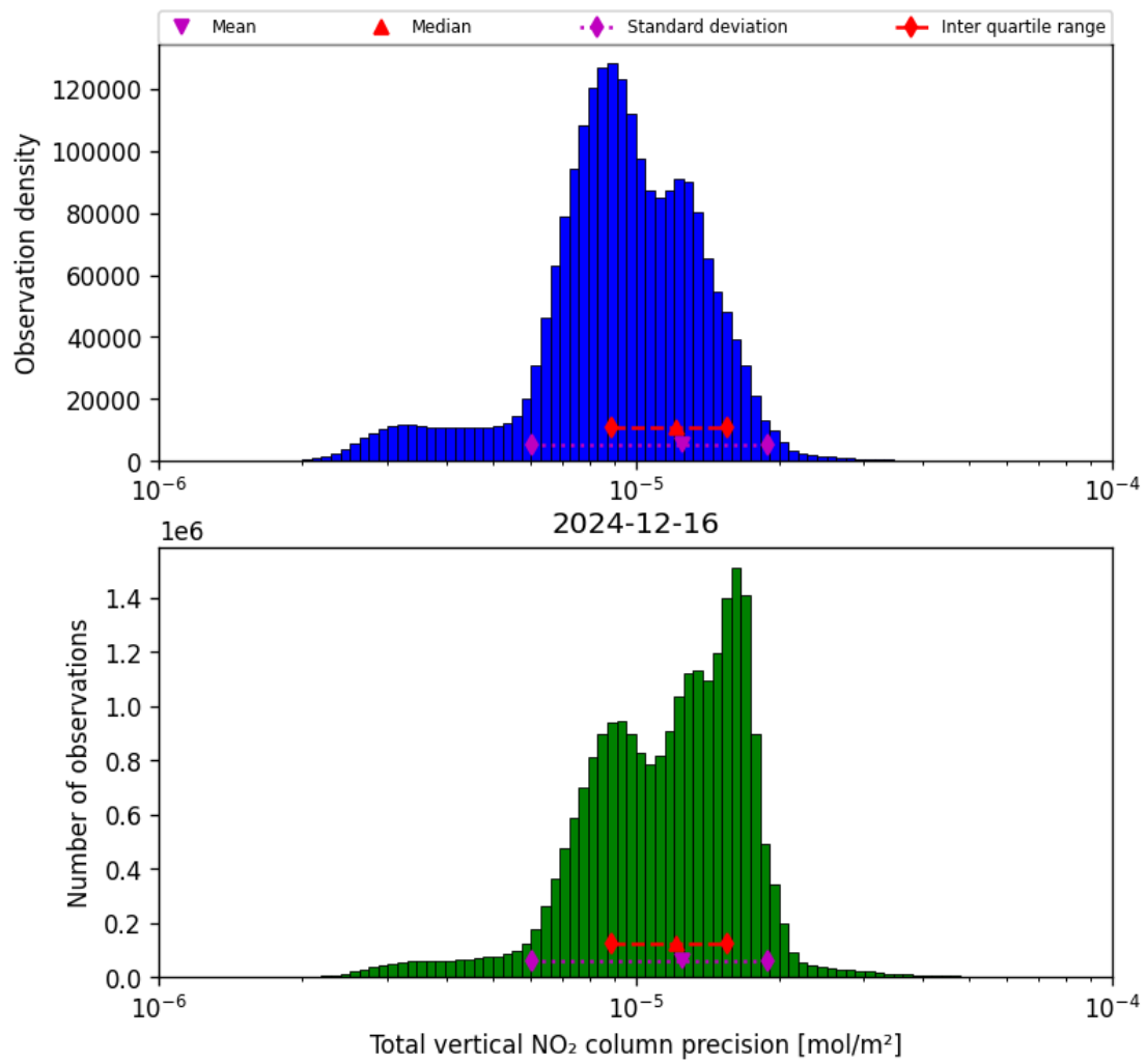
Figure 37: Histogram of “Total vertical NO 2 column precision” for 2024-12-16 to 2024-12-17
