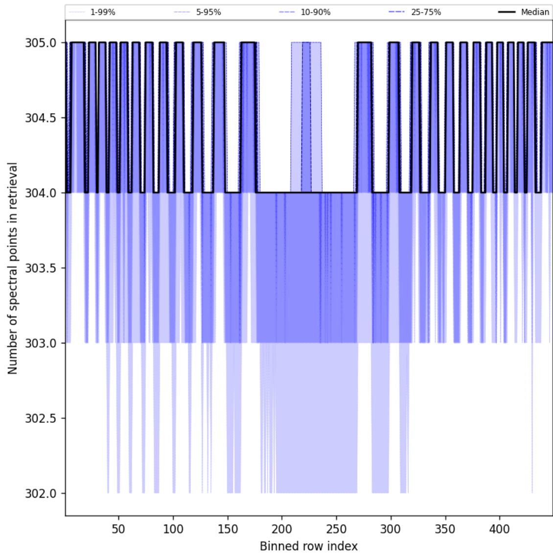
Figure 48: Along track statistics of “Number of spectral points in retrieval” for 2024-12-16 to 2024-12-17
