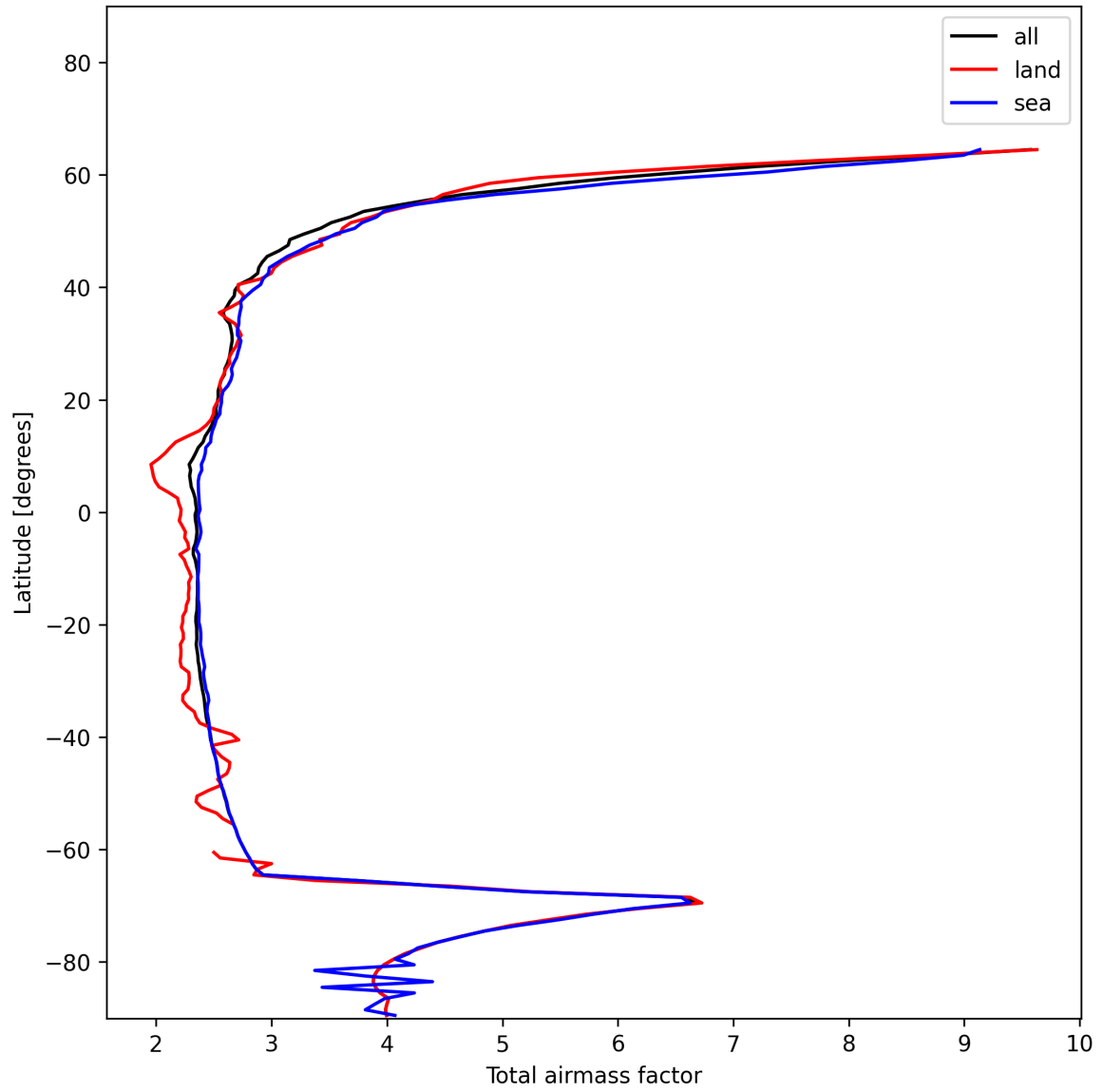
Figure 13: Zonal average of “Total airmass factor” for 2024-12-16 to 2024-12-17.
