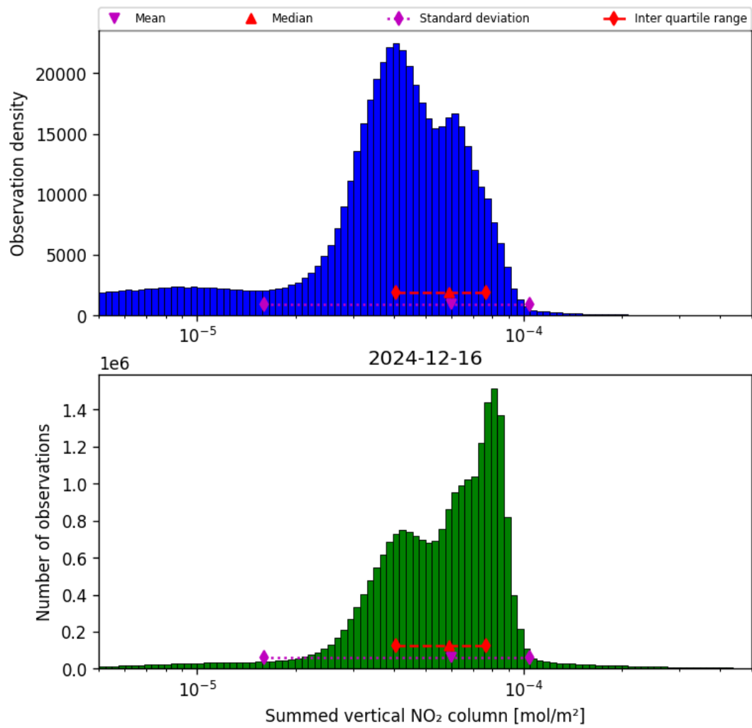
Figure 38: Histogram of “Summed vertical NO 2 column” for 2024-12-16 to 2024-12-17
