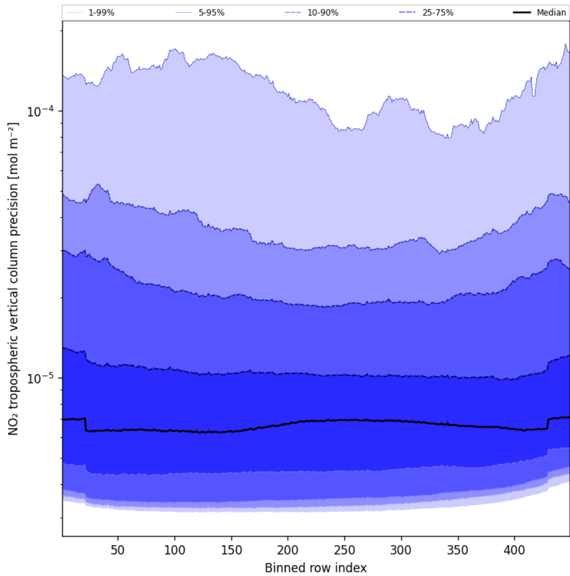
Figure 45: Along track statistics of “NO 2 tropospheric vertical column precision” for 2024-12-16 to 2024-12-17
