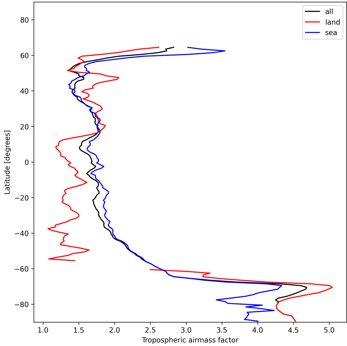
Figure 12: Zonal average of “Tropospheric airmass factor” for 2024-12-16 to 2024-12-17.
