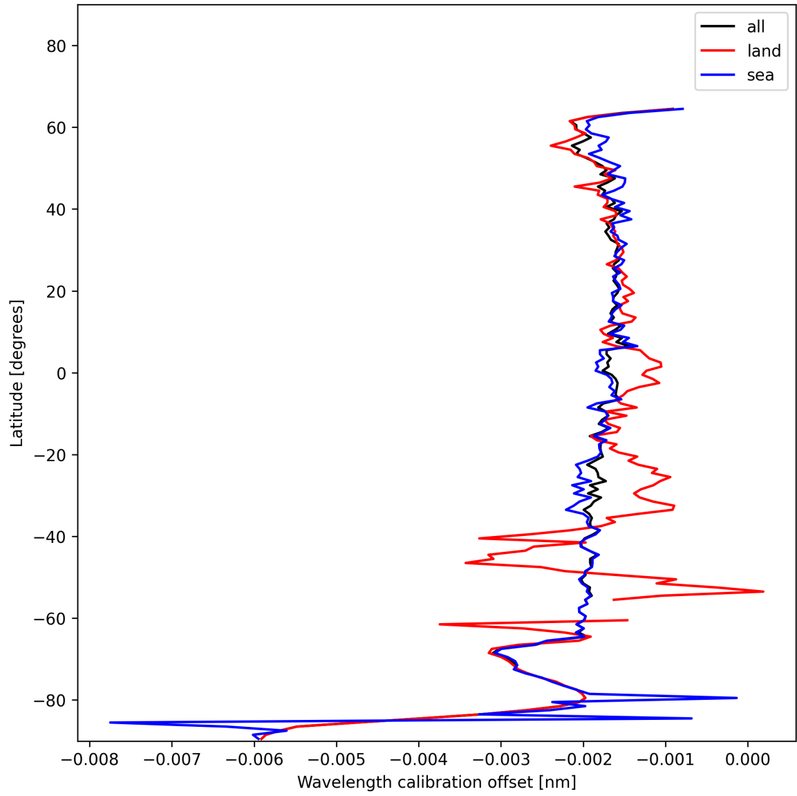
Figure 16: Zonal average of “Wavelength calibration offset” for 2024-12-16 to 2024-12-17.
