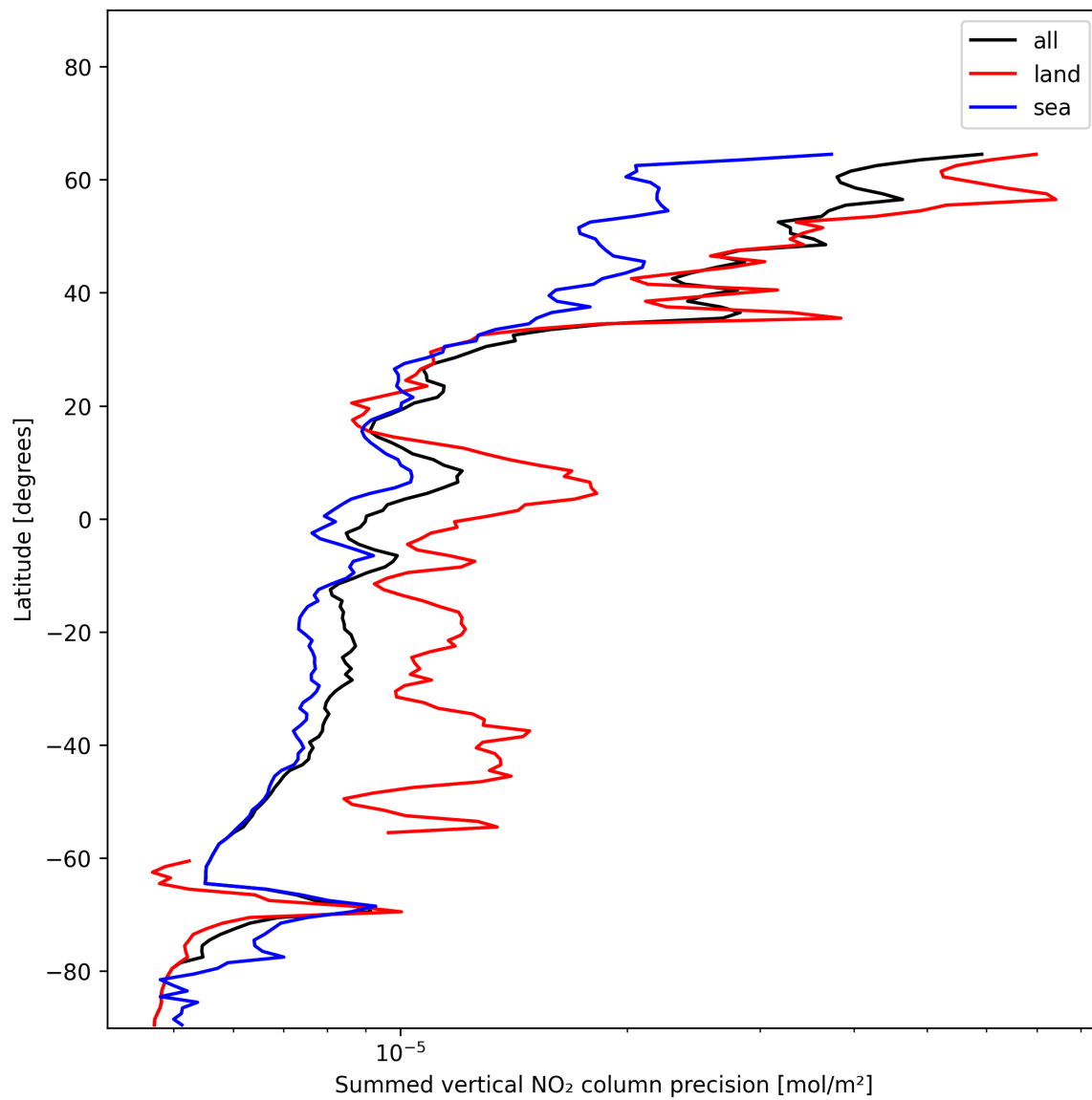
Figure 22: Zonal average of “Summed vertical NO 2 column precision” for 2024-12-16 to 2024-12-17.
