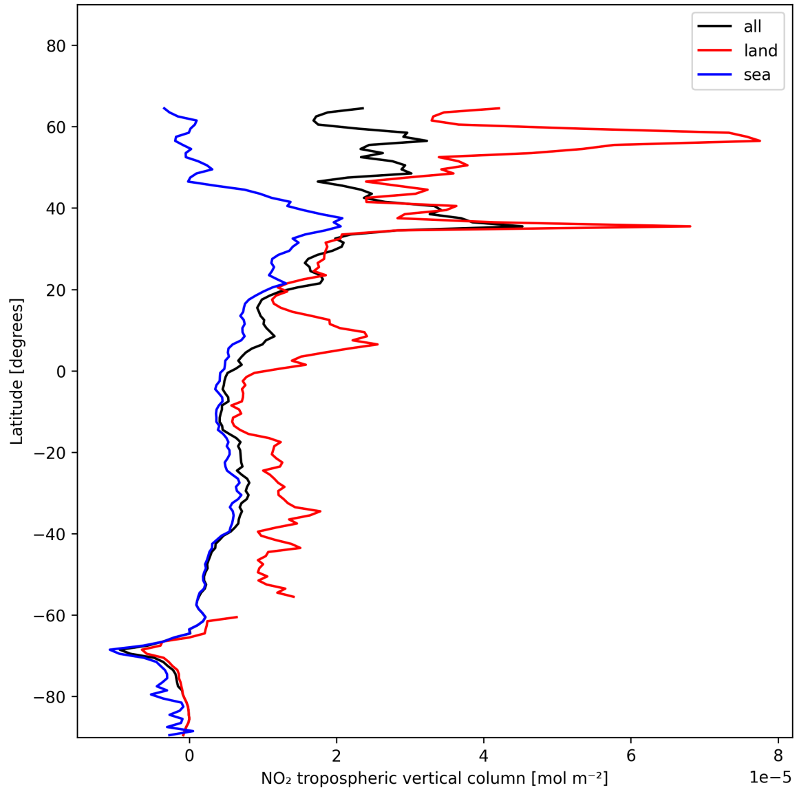
Figure 10: Zonal average of “NO 2 tropospheric vertical column” for 2024-12-16 to 2024-12-17.
