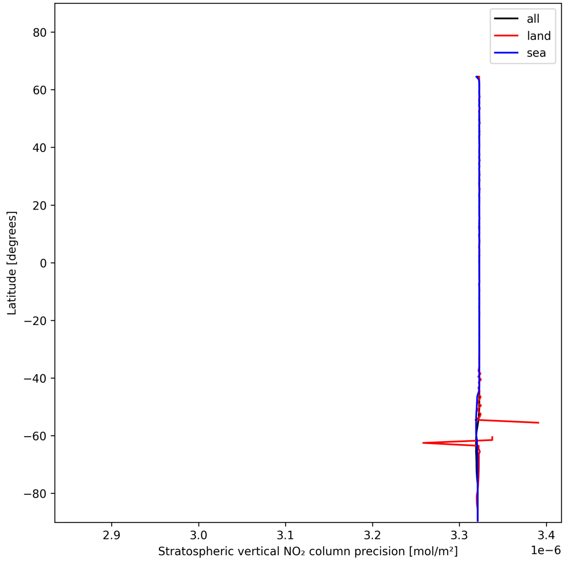
Figure 18: Zonal average of “Stratospheric vertical NO 2 column precision” for 2024-12-16 to 2024-12-17.
