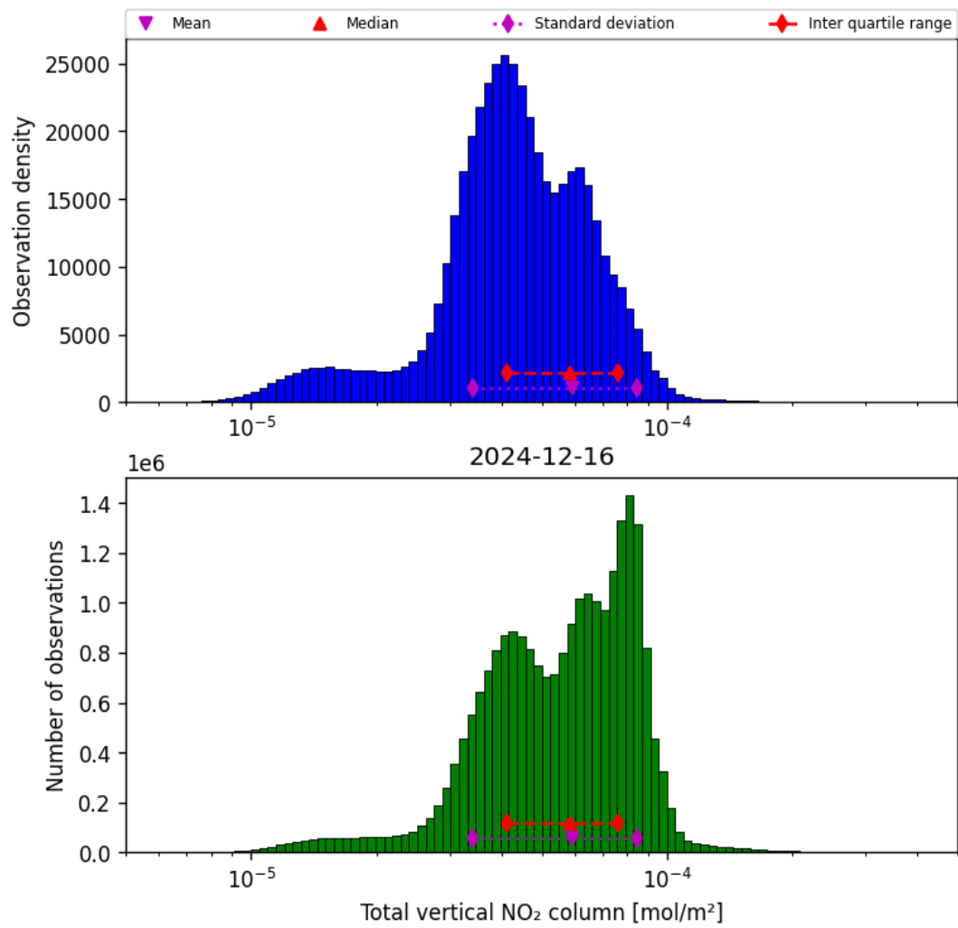
Figure 36: Histogram of “Total vertical NO 2 column” for 2024-12-16 to 2024-12-17
