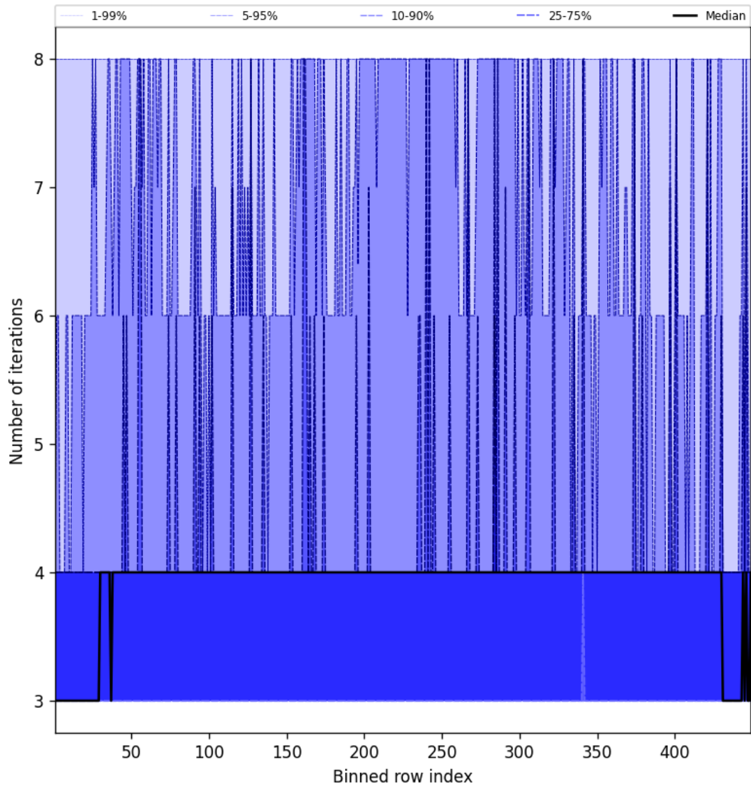
Figure 49: Along track statistics of “Number of iterations” for 2024-12-16 to 2024-12-17
