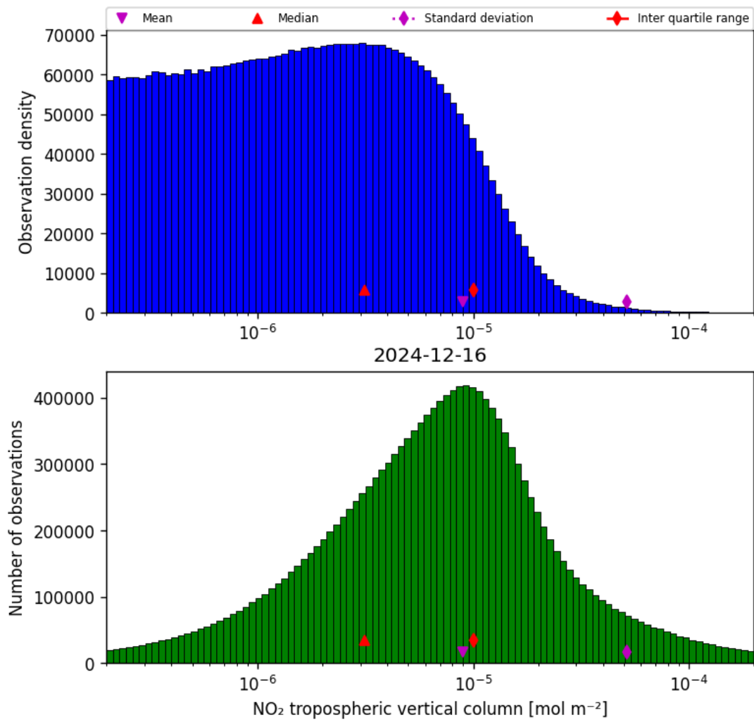
Figure 27: Histogram of “NO 2 tropospheric vertical column” for 2024-12-16 to 2024-12-17
