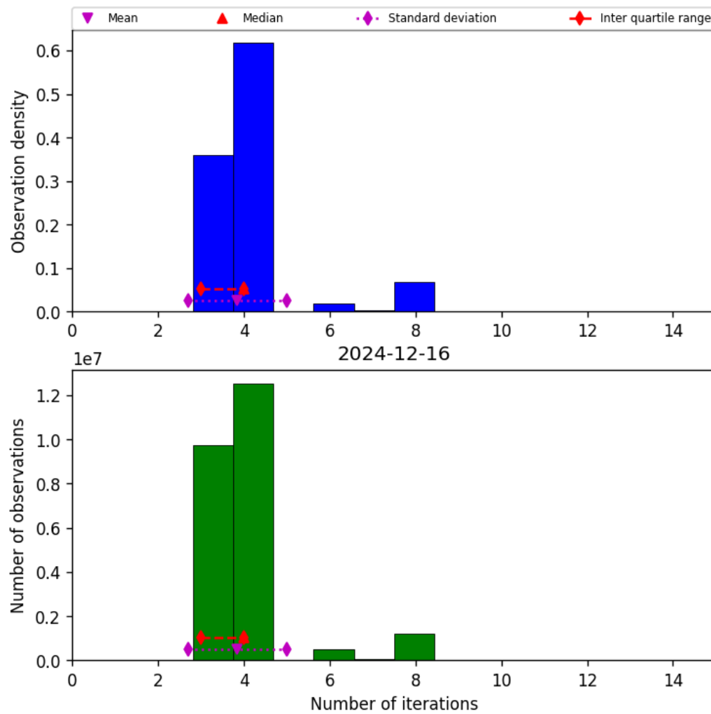
Figure 32: Histogram of “Number of iterations” for 2024-12-16 to 2024-12-17
