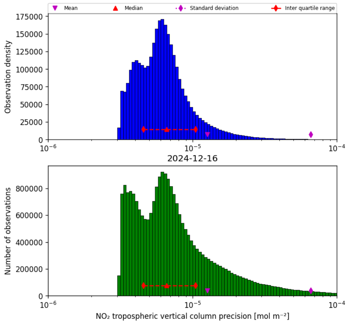
Figure 28: Histogram of “NO 2 tropospheric vertical column precision” for 2024-12-16 to 2024-12-17
