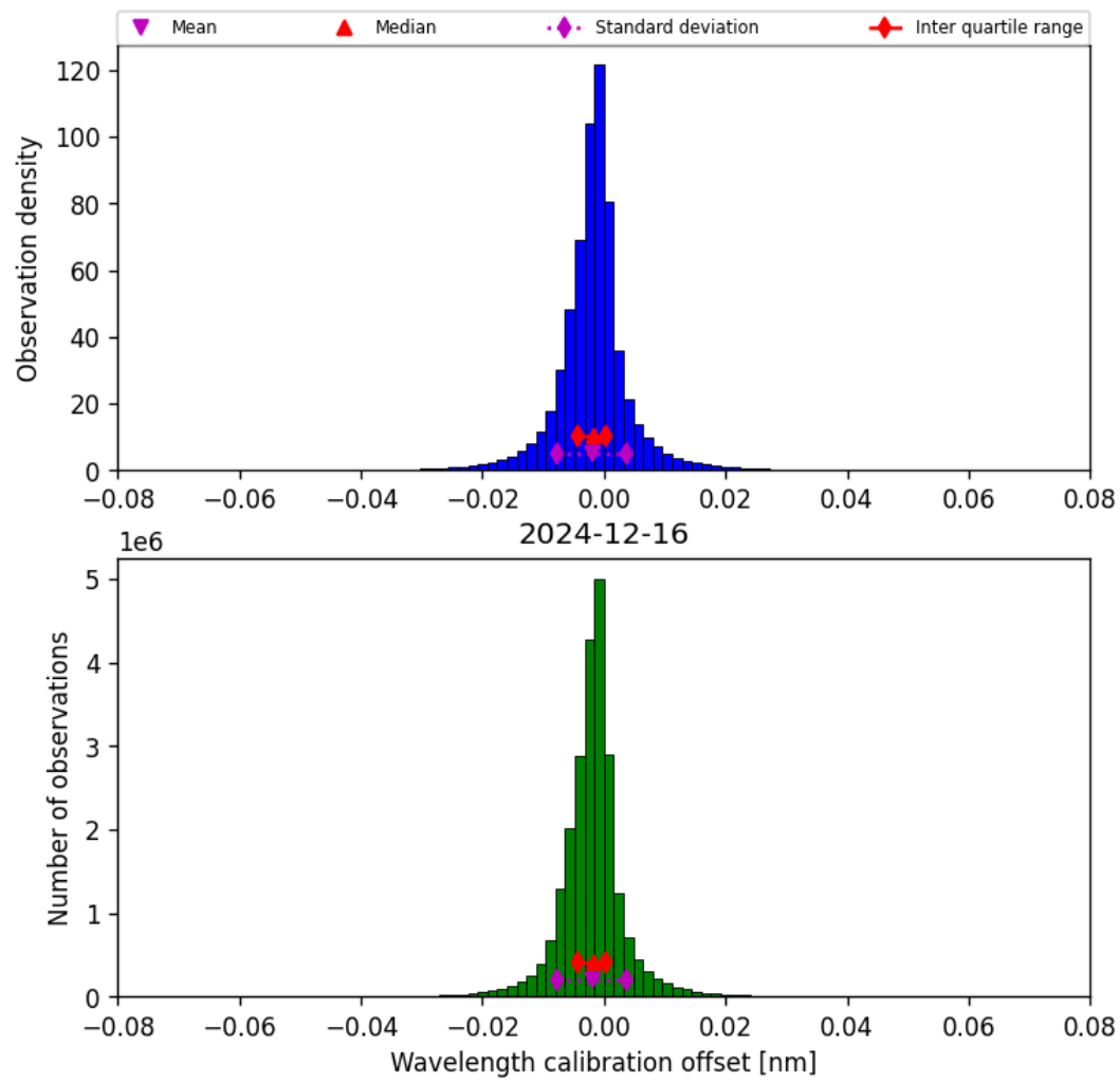
Figure 33: Histogram of “Wavelength calibration offset” for 2024-12-16 to 2024-12-17
