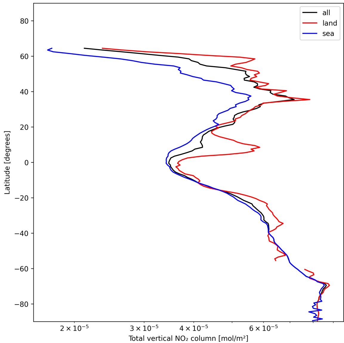
Figure 19: Zonal average of “Total vertical NO 2 column” for 2024-12-16 to 2024-12-17.
