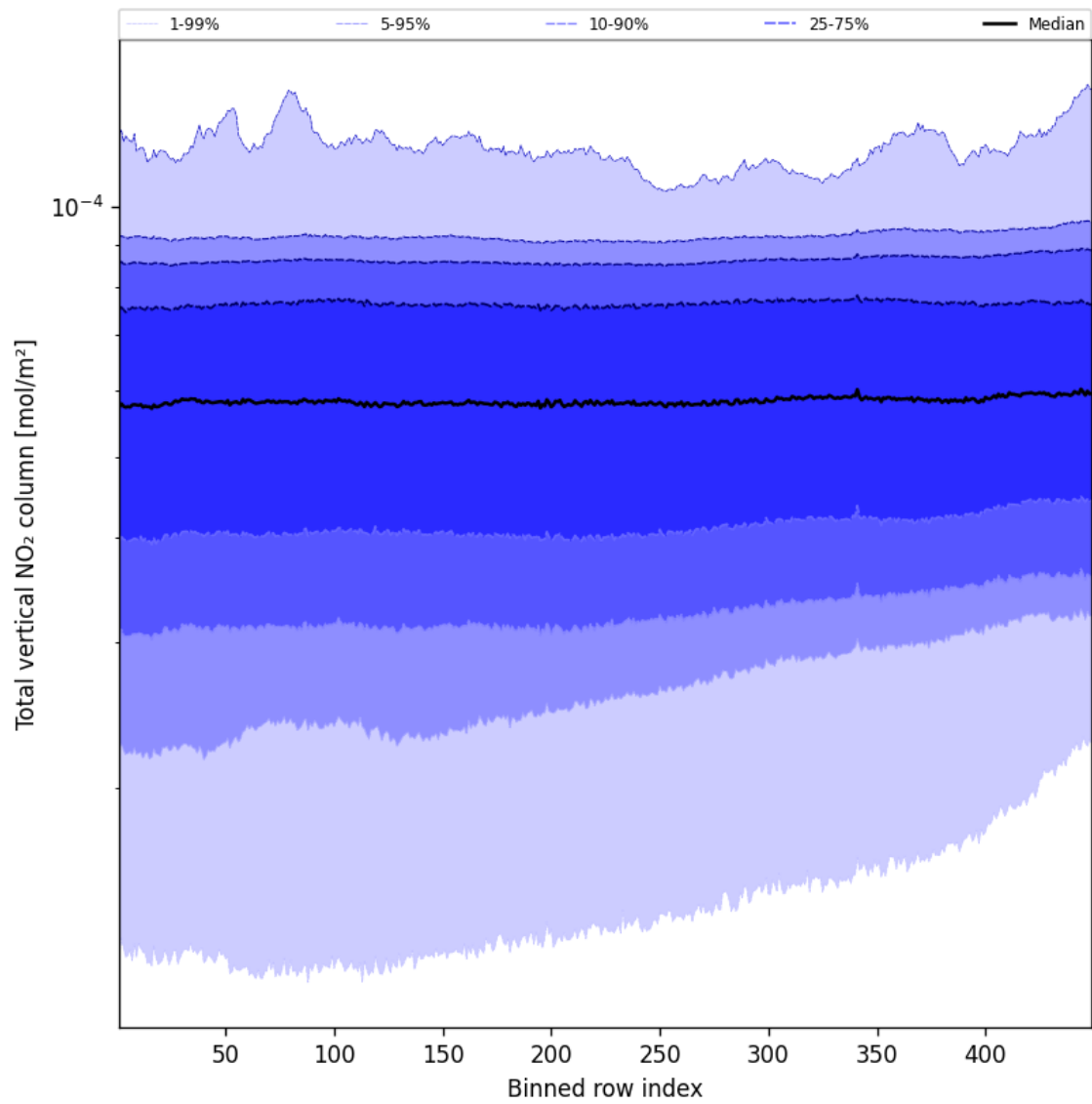
Figure 53: Along track statistics of “Total vertical NO 2 column” for 2024-12-16 to 2024-12-17
