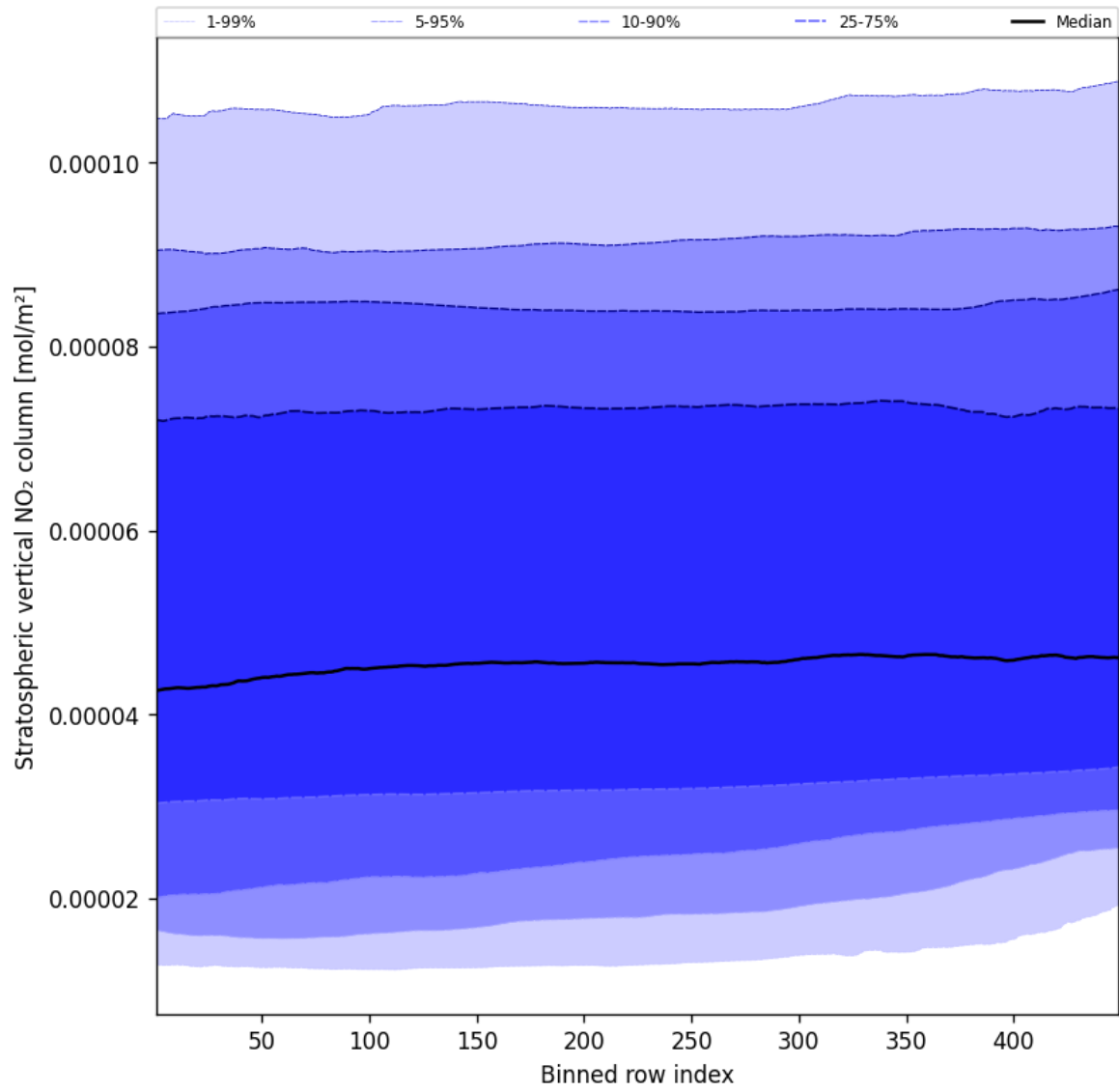
Figure 51: Along track statistics of “Stratospheric vertical NO 2 column” for 2024-12-16 to 2024-12-17
