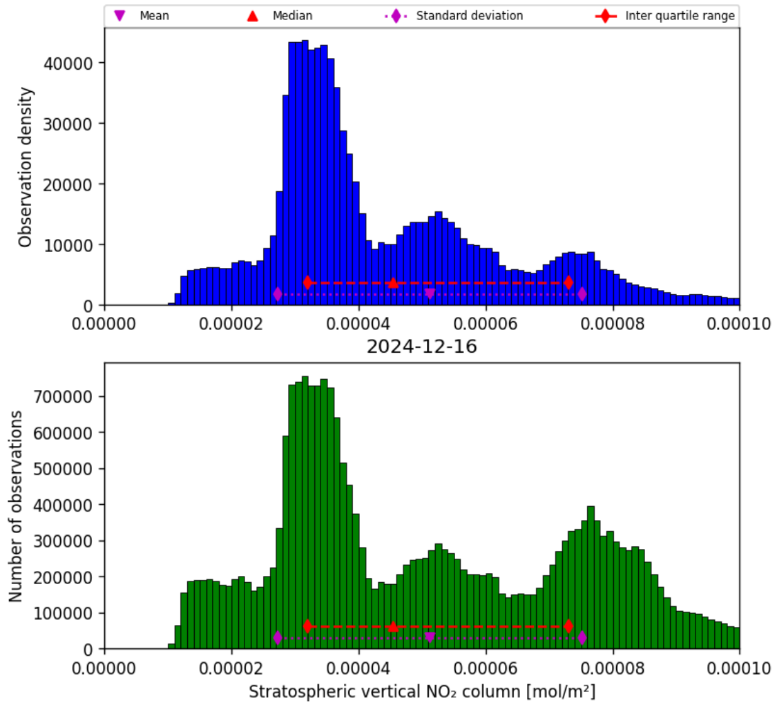
Figure 34: Histogram of “Stratospheric vertical NO 2 column” for 2024-12-16 to 2024-12-17
