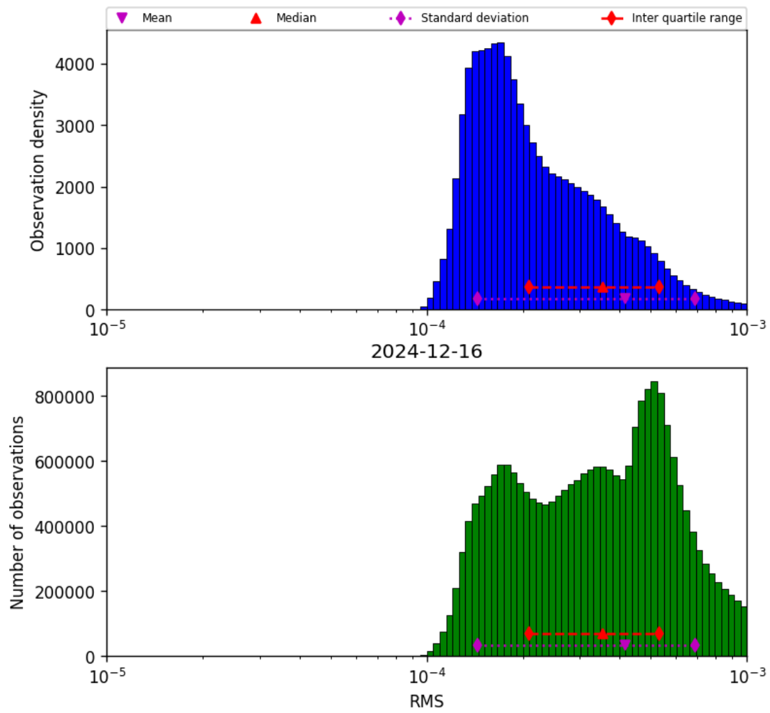
Figure 41: Histogram of “RMS” for 2024-12-16 to 2024-12-17
