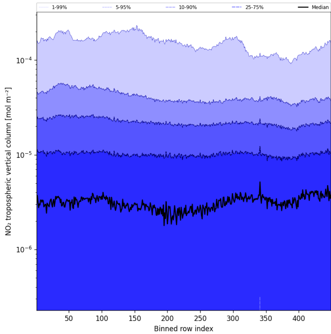
Figure 44: Along track statistics of “NO 2 tropospheric vertical column” for 2024-12-16 to 2024-12-17
