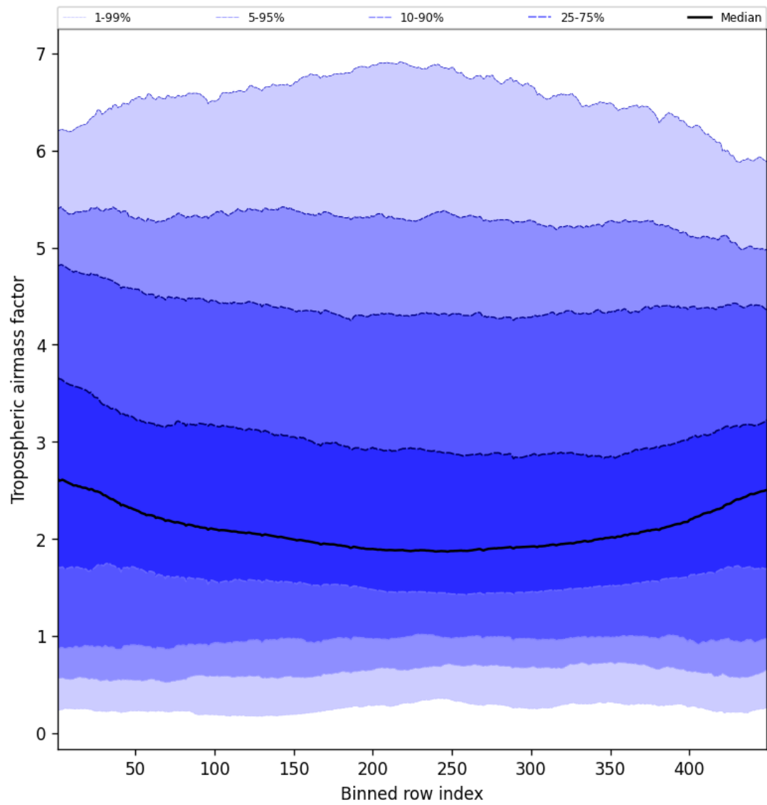
Figure 46: Along track statistics of “Tropospheric airmass factor” for 2024-12-16 to 2024-12-17
