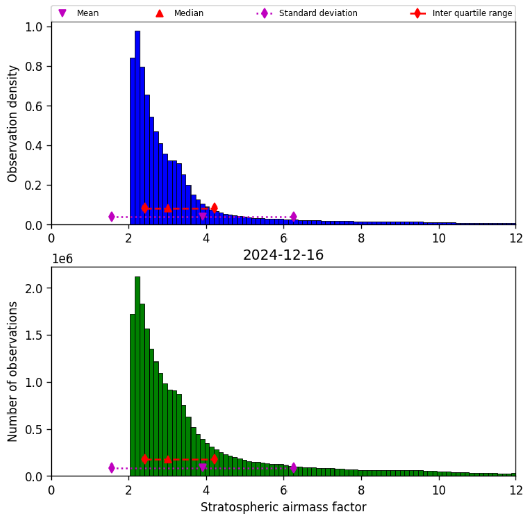
Figure 42: Histogram of “Stratospheric airmass factor” for 2024-12-16 to 2024-12-17
