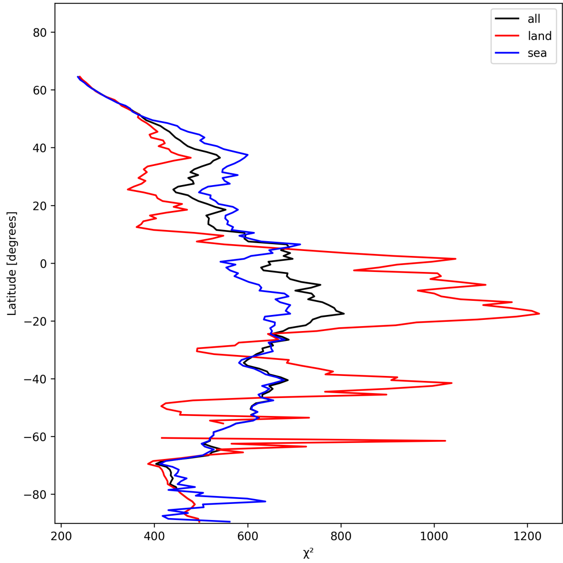
Figure 23: Zonal average of “ \chi^2 ” for 2024-12-16 to 2024-12-17.
