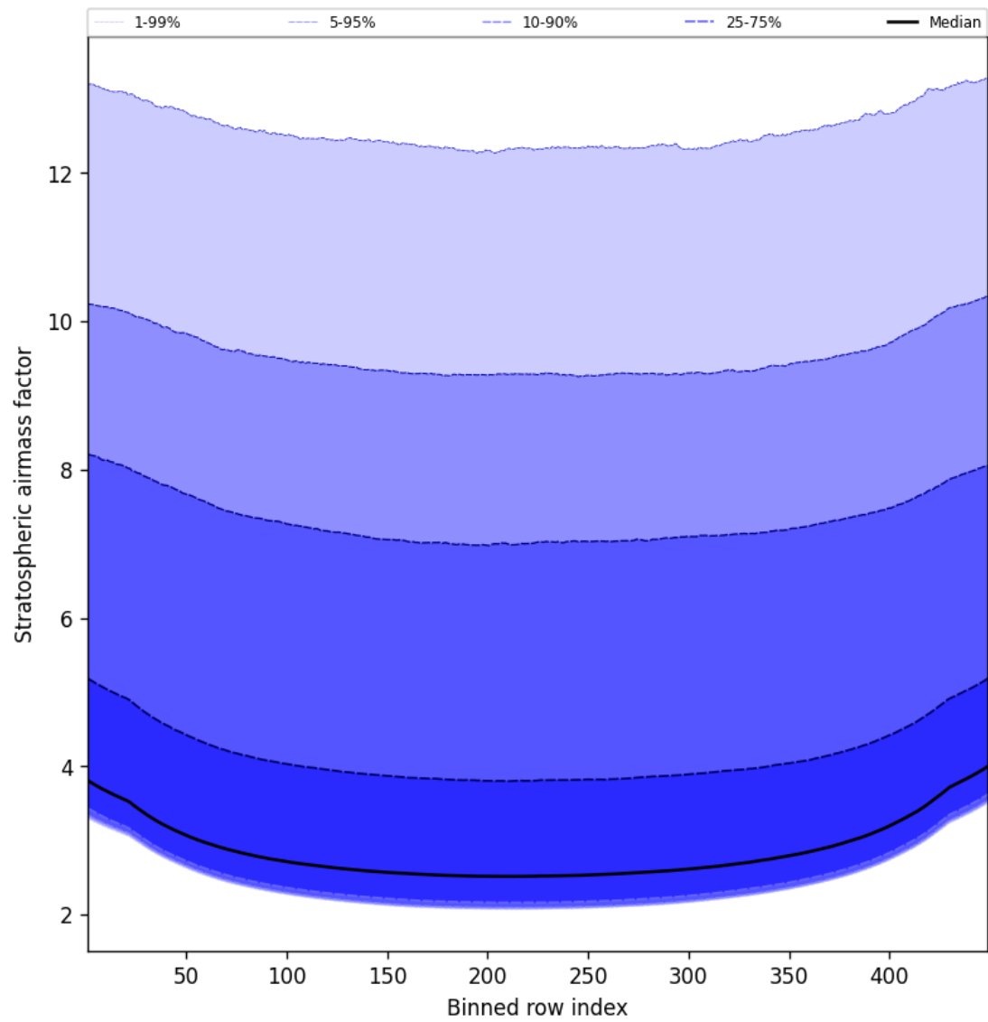
Figure 59: Along track statistics of “Stratospheric airmass factor” for 2024-12-16 to 2024-12-17
