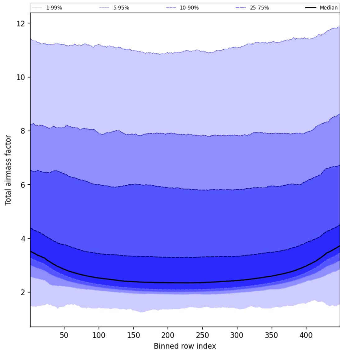
Figure 47: Along track statistics of “Total airmass factor” for 2024-12-16 to 2024-12-17
