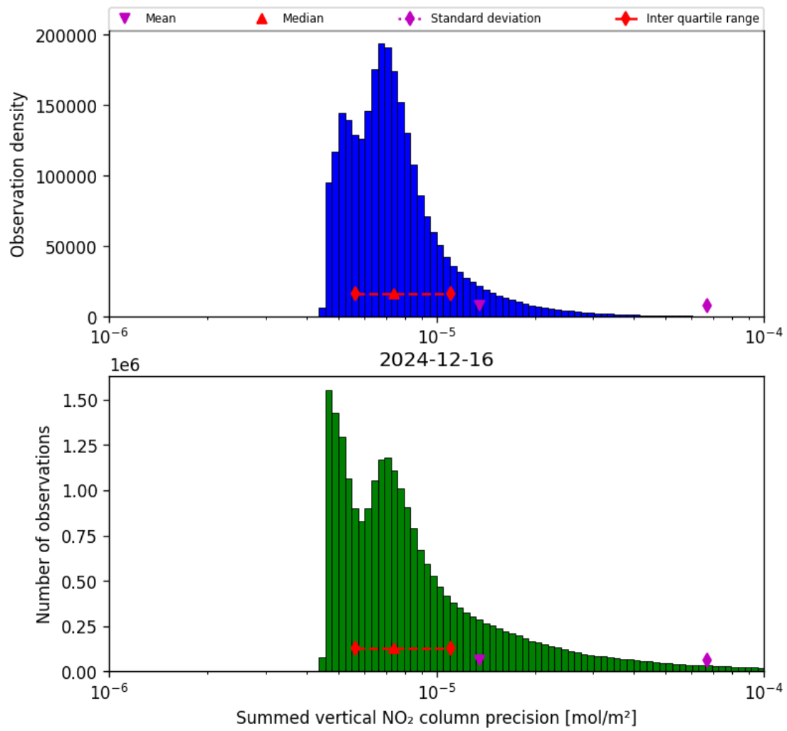
Figure 39: Histogram of “Summed vertical NO 2 column precision” for 2024-12-16 to 2024-12-17
