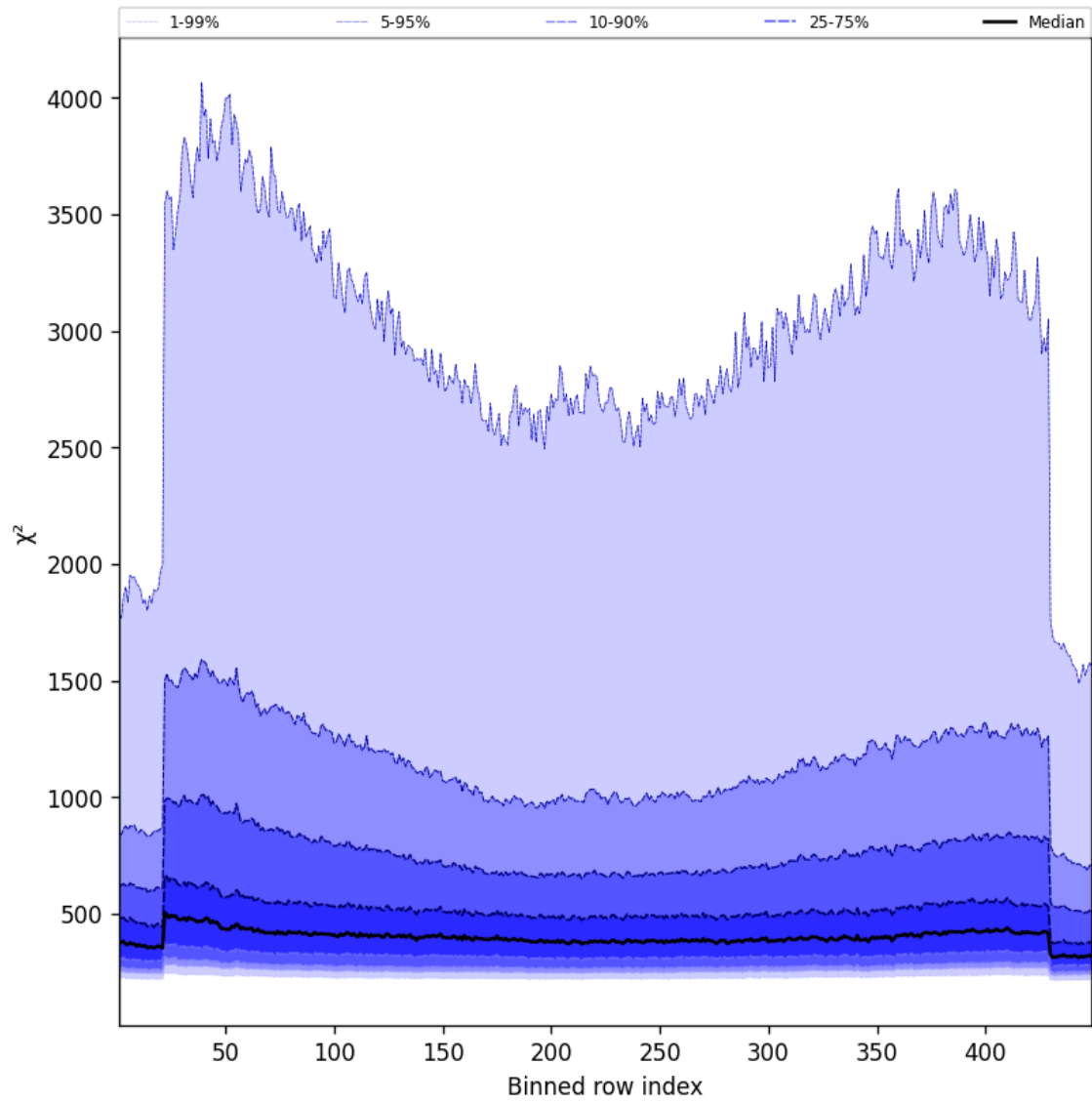
Figure 57: Along track statistics of “ \chi^2 ” for 2024-12-16 to 2024-12-17
