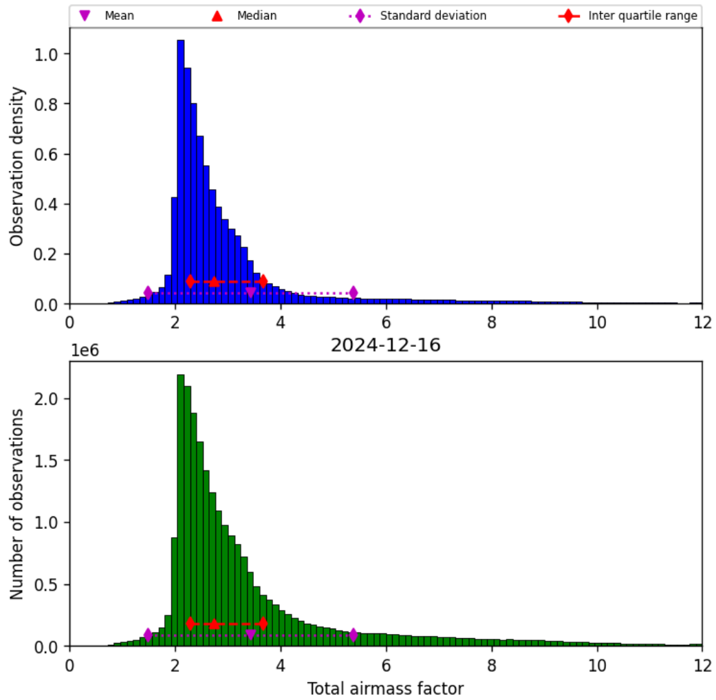
Figure 30: Histogram of “Total airmass factor” for 2024-12-16 to 2024-12-17
