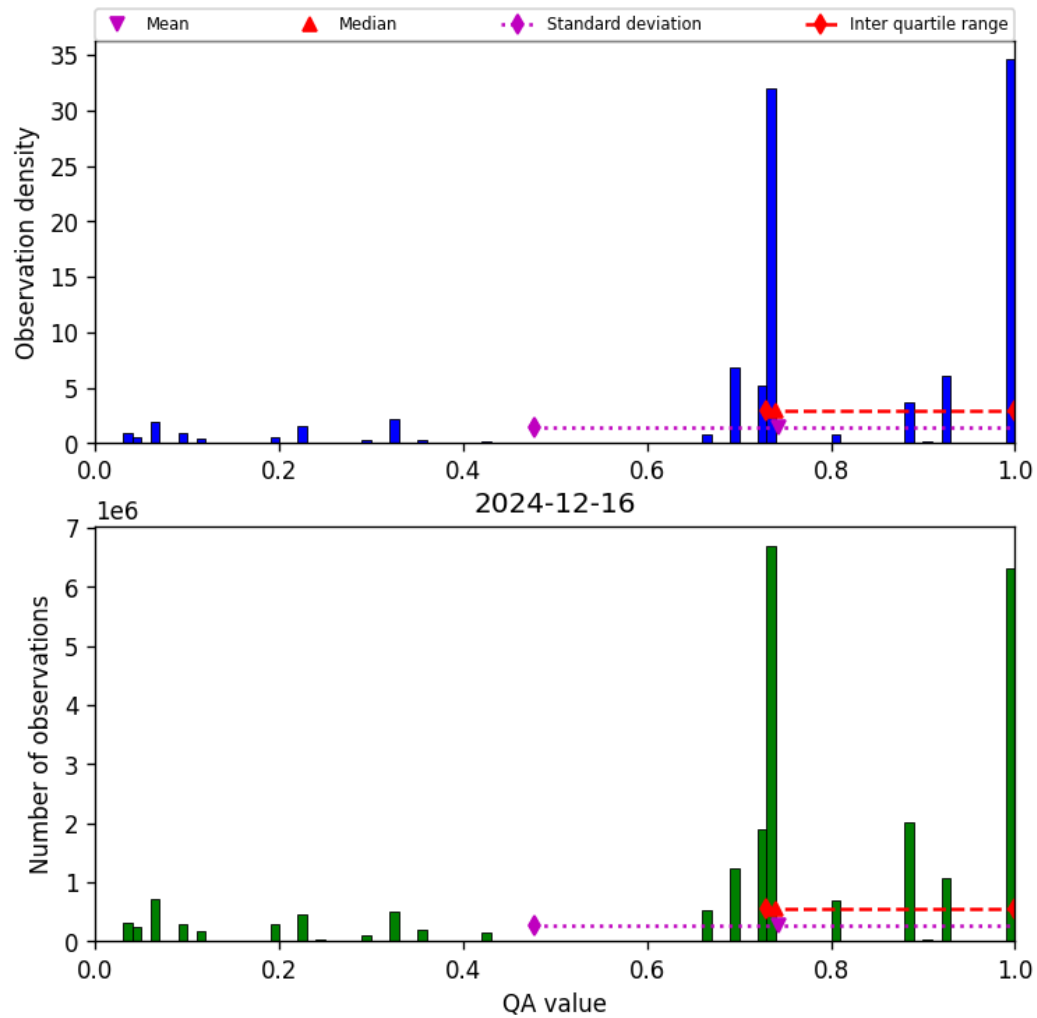
Figure 26: Histogram of “QA value” for 2024-12-16 to 2024-12-17
