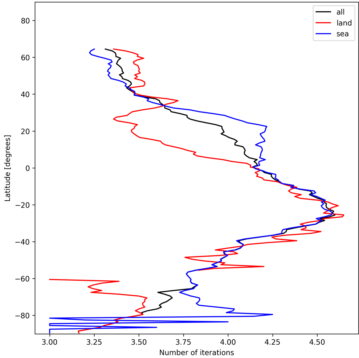
Figure 15: Zonal average of “Number of iterations” for 2024-12-16 to 2024-12-17.
