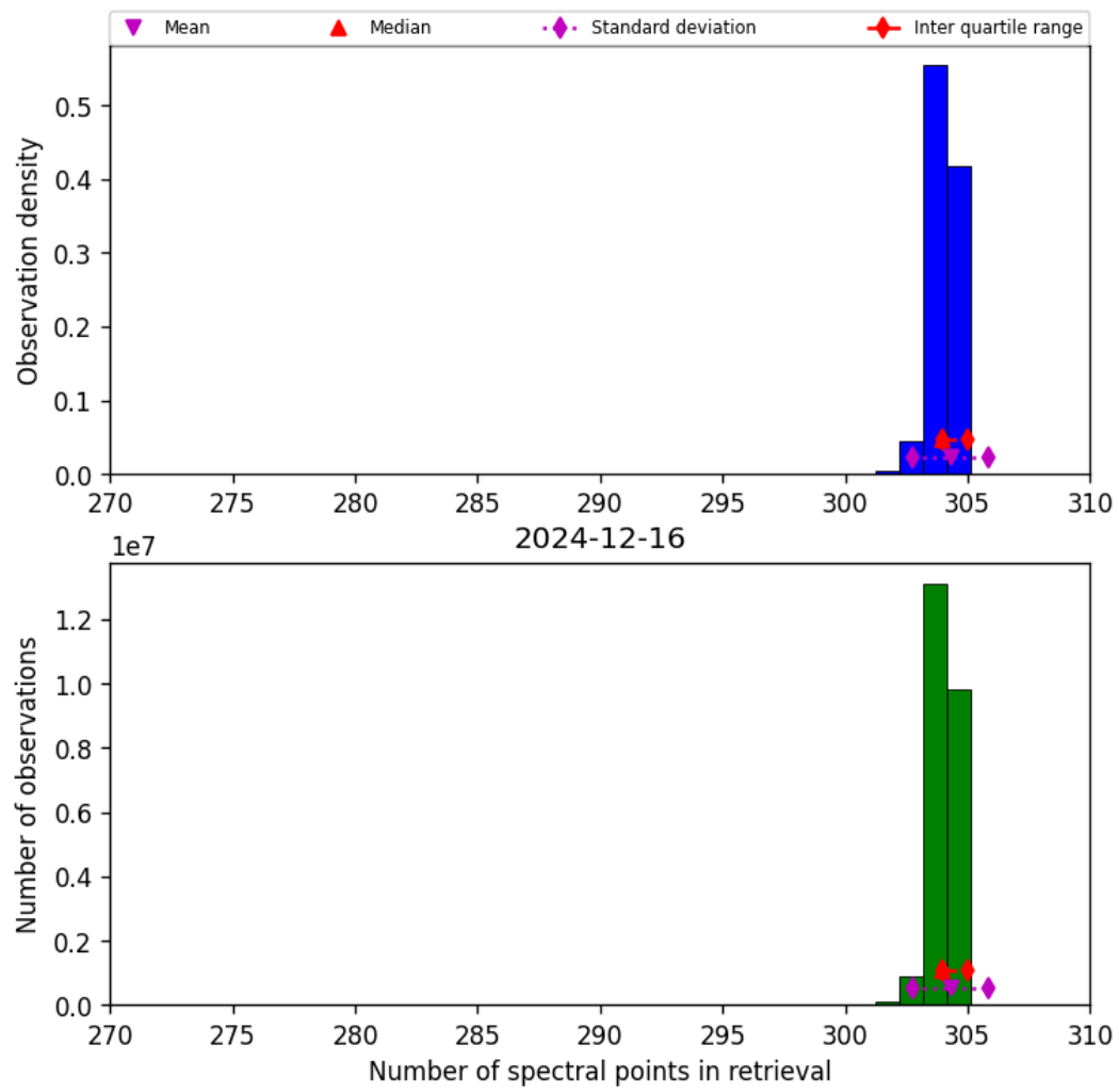
Figure 31: Histogram of “Number of spectral points in retrieval” for 2024-12-16 to 2024-12-17
