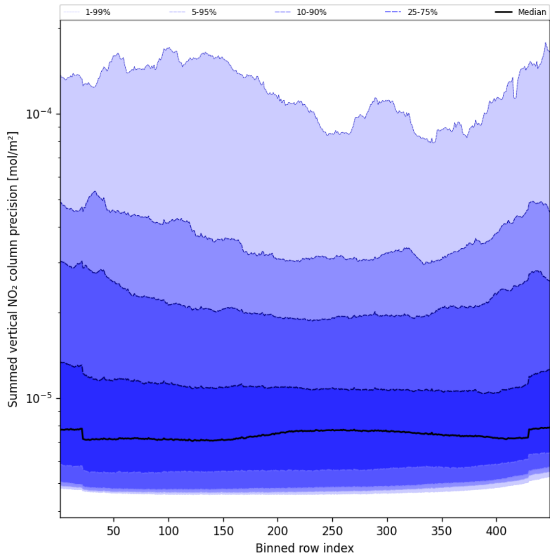
Figure 56: Along track statistics of “Summed vertical NO 2 column precision” for 2024-12-16 to 2024-12-17
