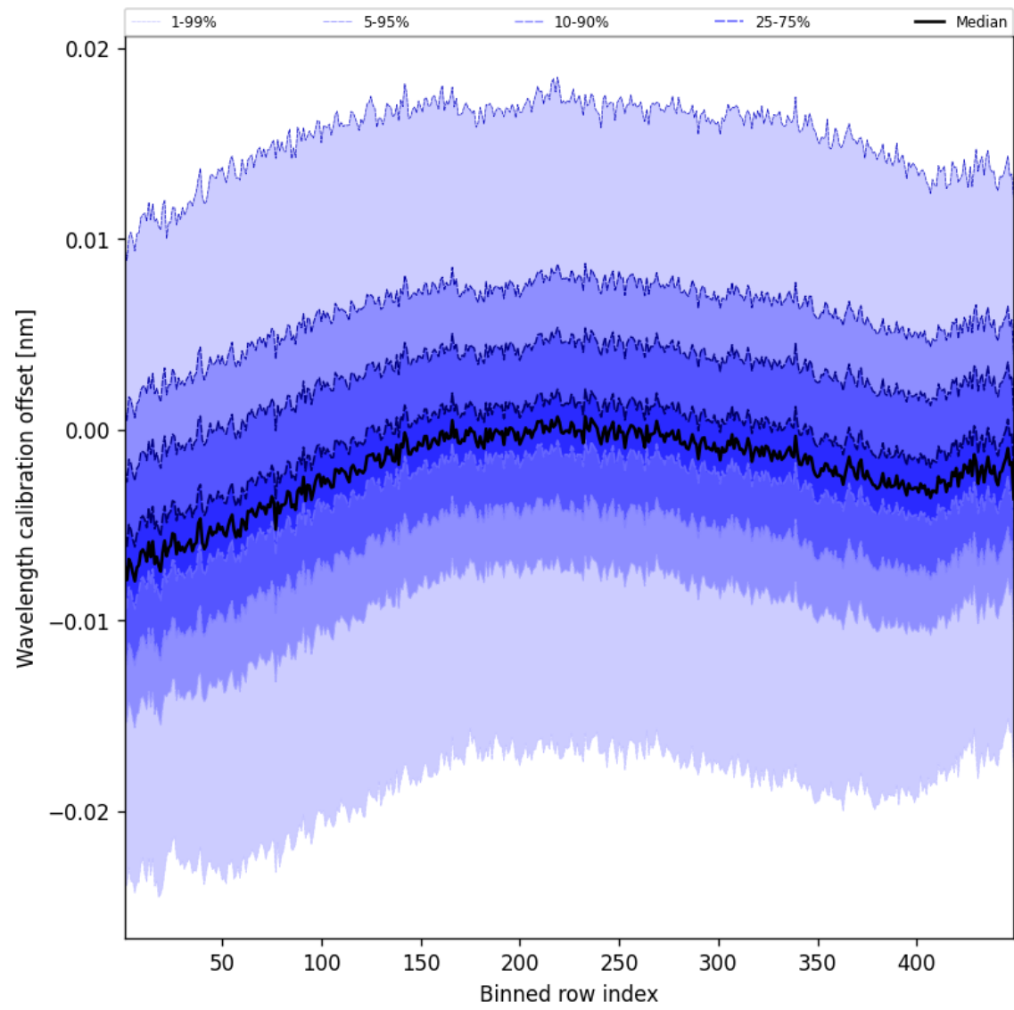
Figure 50: Along track statistics of “Wavelength calibration offset” for 2024-12-16 to 2024-12-17
