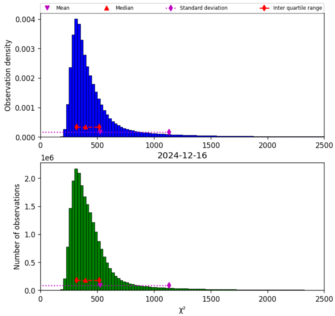
Figure 40: Histogram of “ \chi^2 ” for 2024-12-16 to 2024-12-17
