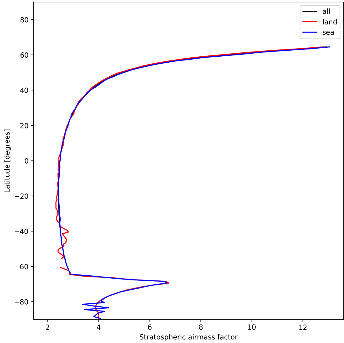
Figure 25: Zonal average of “Stratospheric airmass factor” for 2024-12-16 to 2024-12-17.
