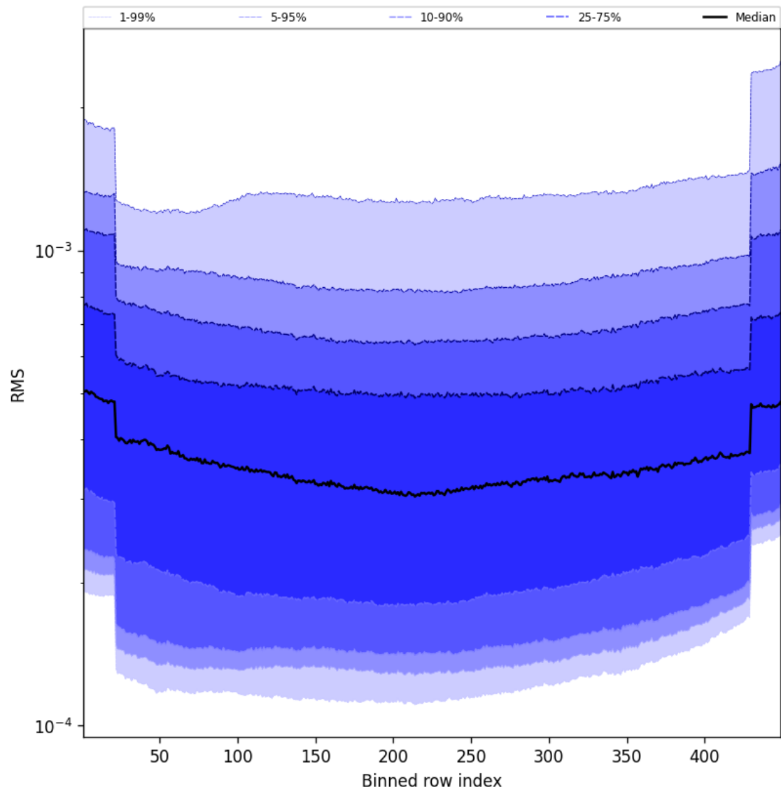
Figure 58: Along track statistics of “RMS” for 2024-12-16 to 2024-12-17
