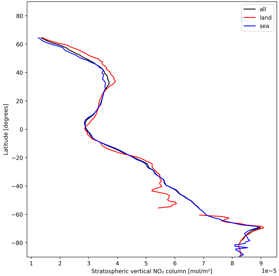
Figure 17: Zonal average of “Stratospheric vertical NO 2 column” for 2024-12-16 to 2024-12-17.
