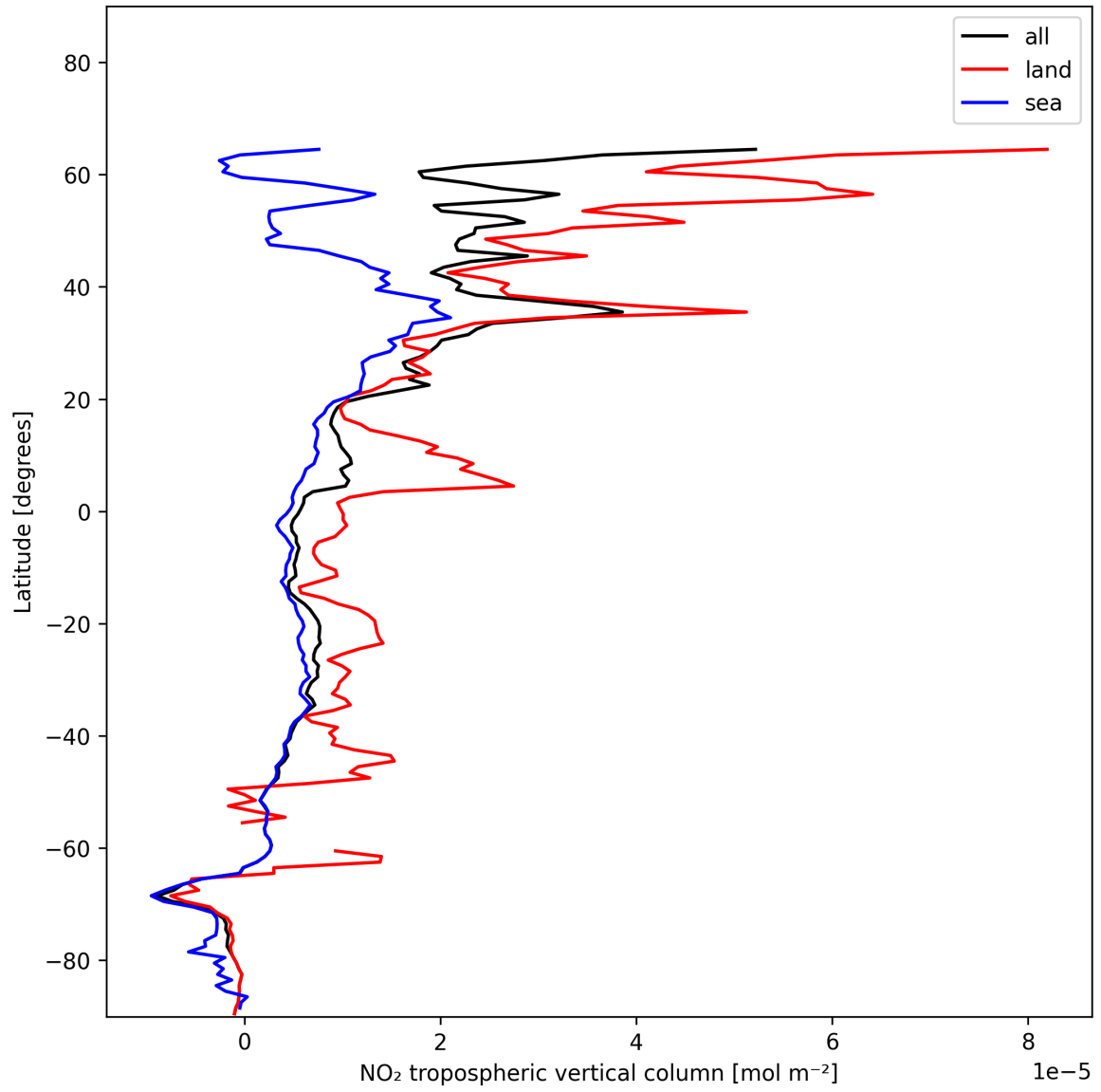
Figure 10: Zonal average of “NO 2 tropospheric vertical column” for 2024-12-17 to 2024-12-18.
