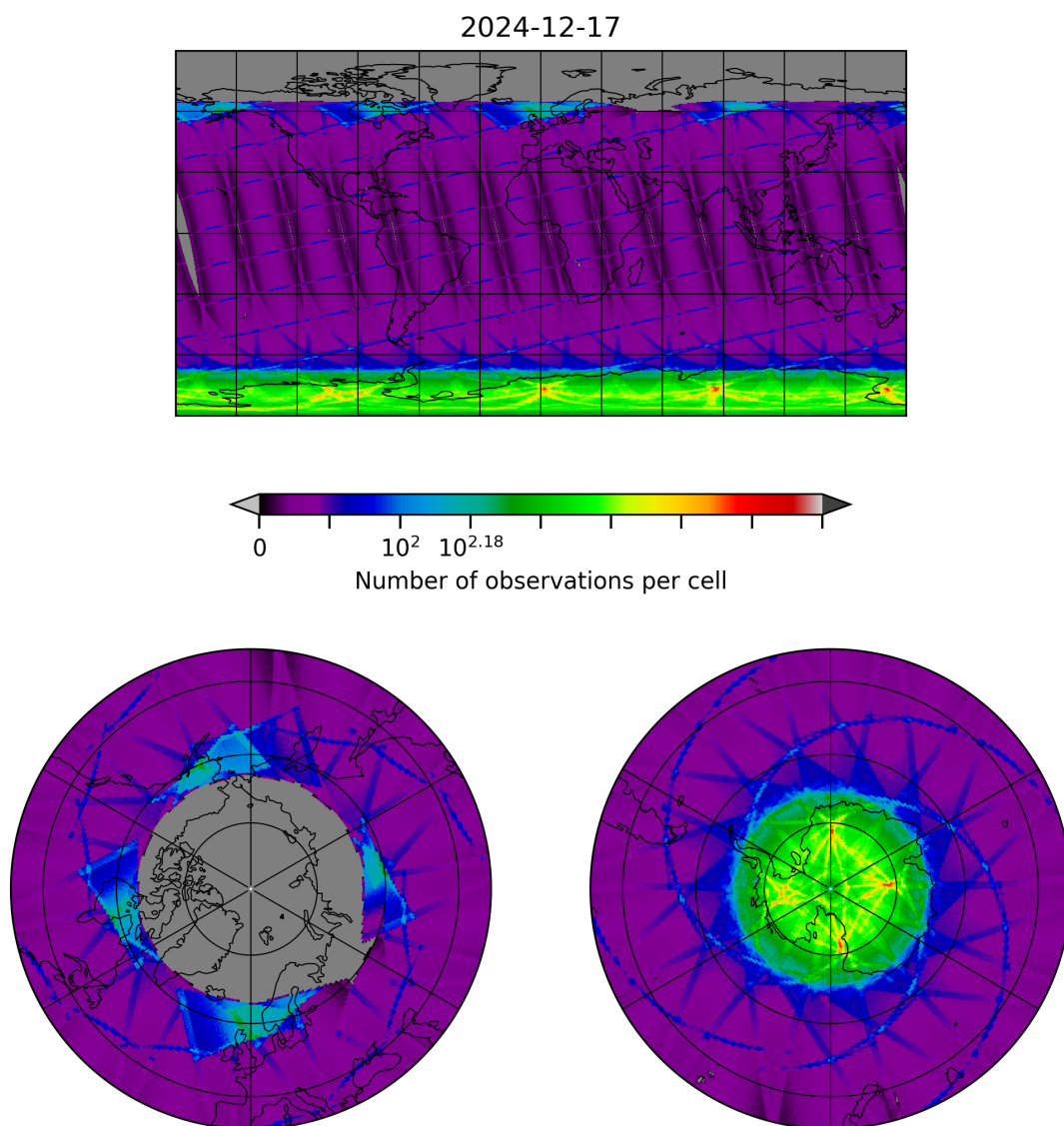
Figure 8: Map of the number of observations for 2024-12-17 to 2024-12-18
