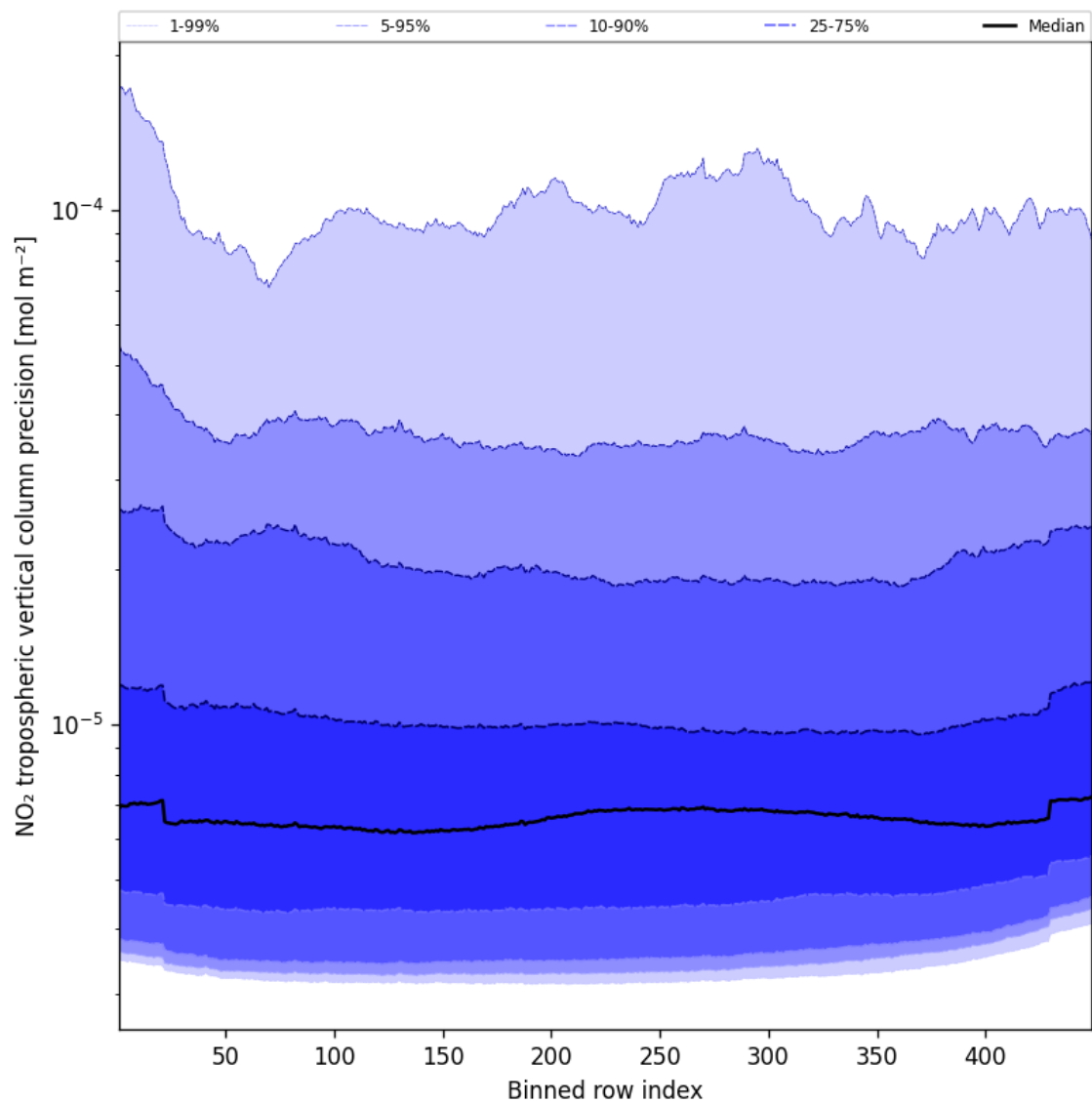
Figure 45: Along track statistics of “NO 2 tropospheric vertical column precision” for 2024-12-17 to 2024-12-18
