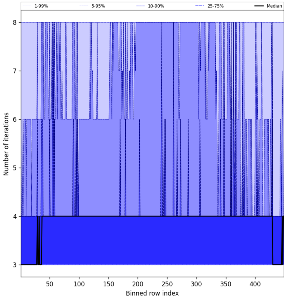
Figure 49: Along track statistics of “Number of iterations” for 2024-12-17 to 2024-12-18
