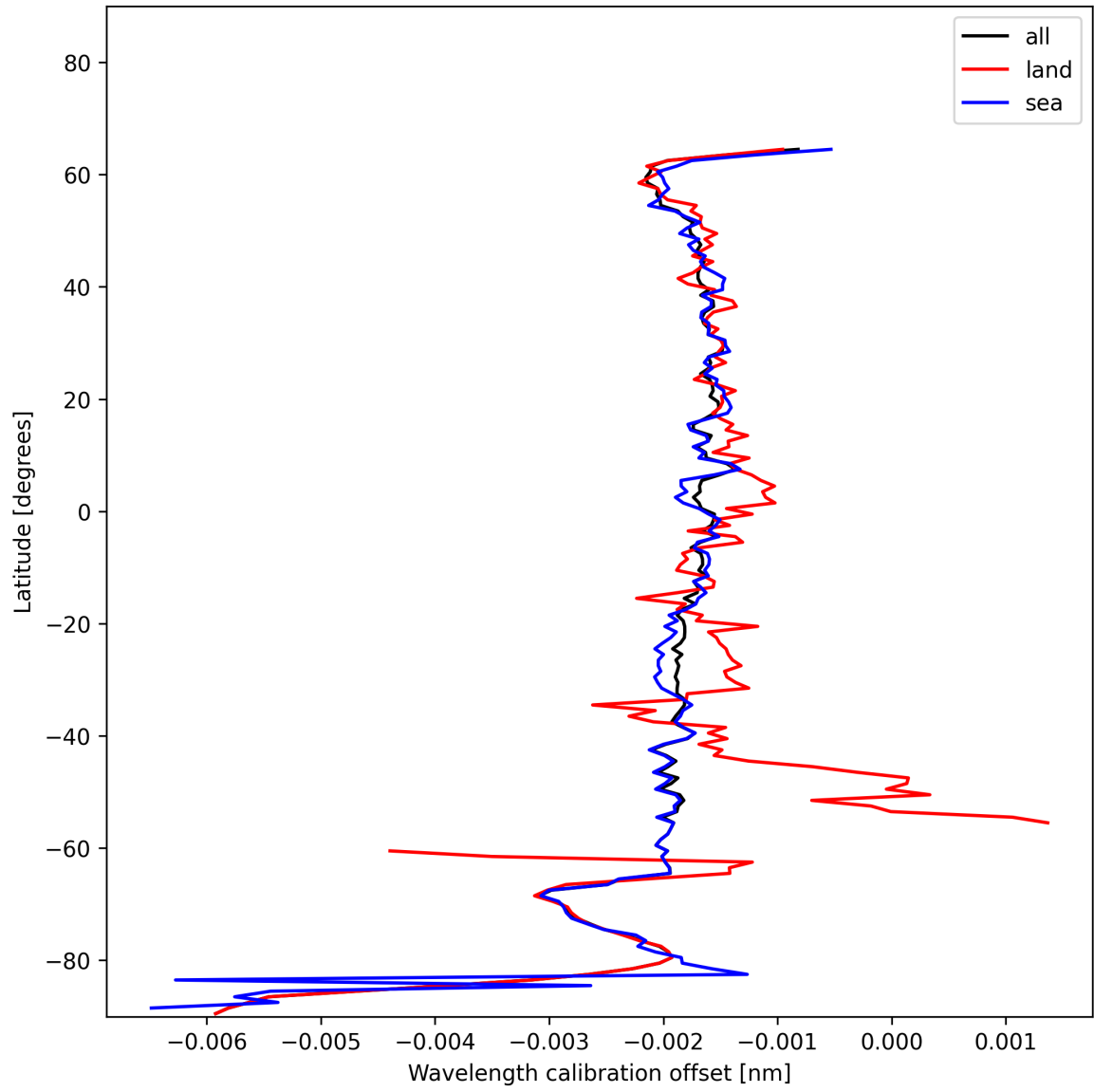
Figure 16: Zonal average of “Wavelength calibration offset” for 2024-12-17 to 2024-12-18.
