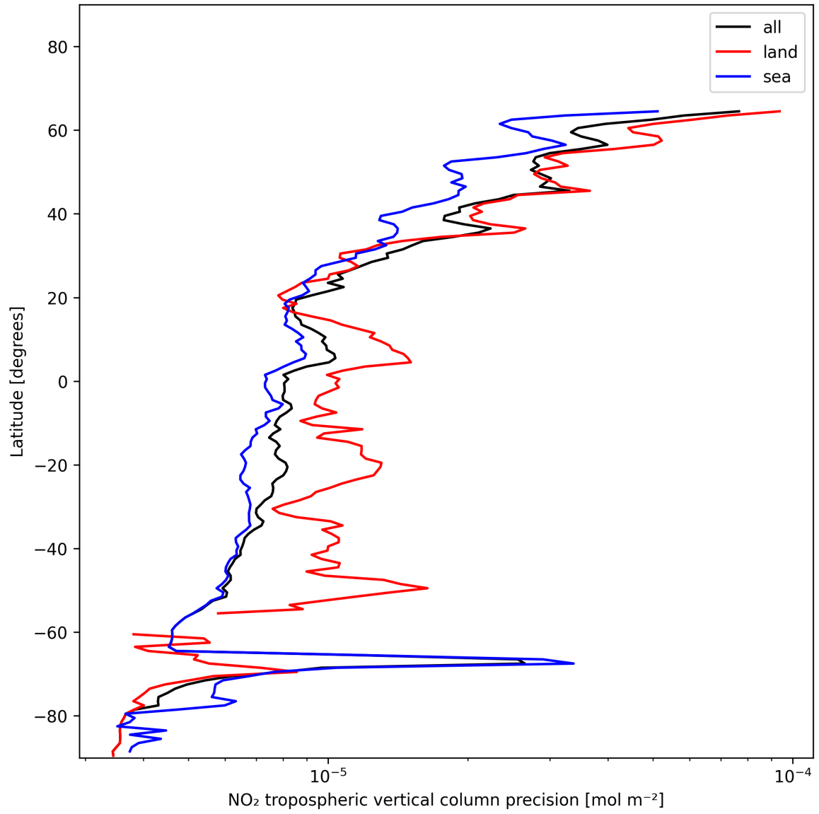
Figure 11: Zonal average of “NO 2 tropospheric vertical column precision” for 2024-12-17 to 2024-12-18.
