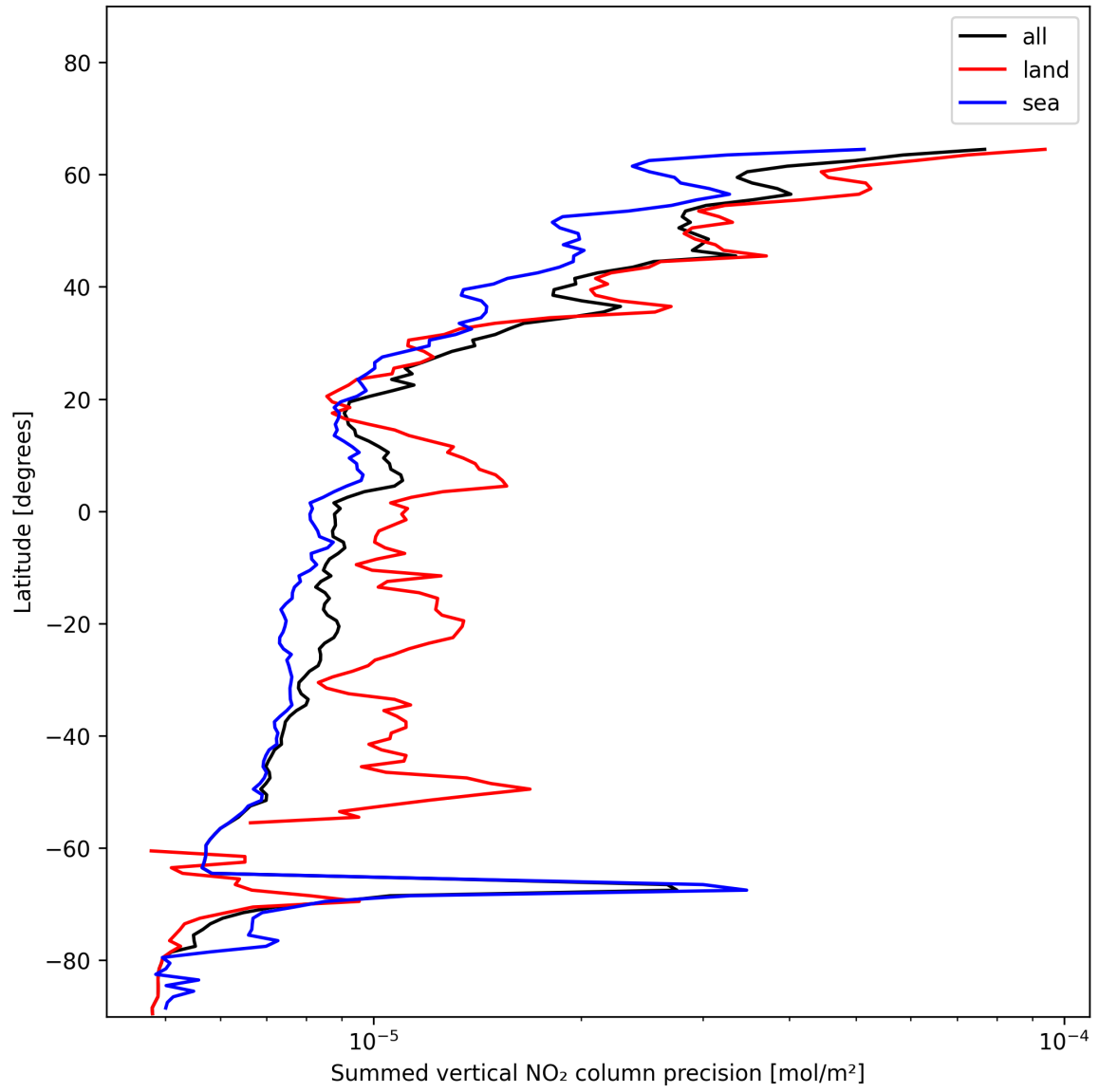
Figure 22: Zonal average of “Summed vertical NO 2 column precision” for 2024-12-17 to 2024-12-18.
