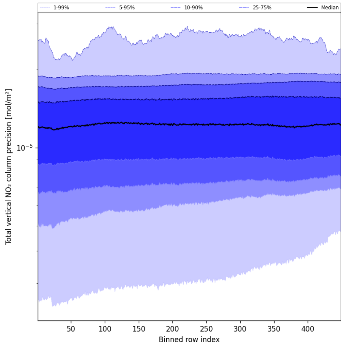
Figure 54: Along track statistics of “Total vertical NO 2 column precision” for 2024-12-17 to 2024-12-18
