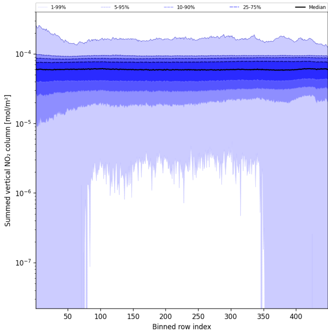
Figure 55: Along track statistics of “Summed vertical NO 2 column” for 2024-12-17 to 2024-12-18
