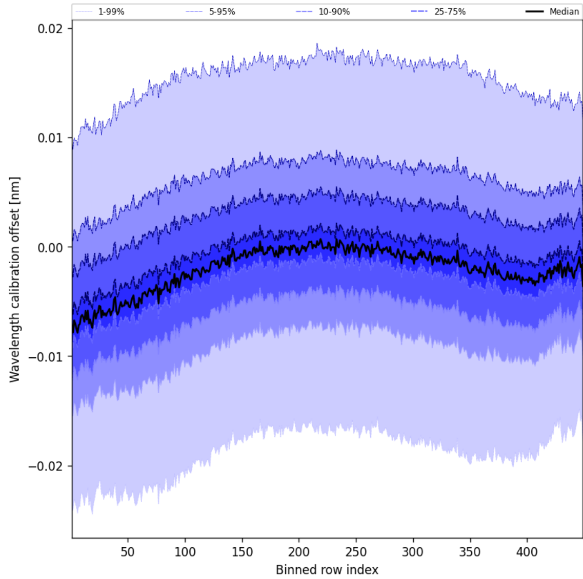
Figure 50: Along track statistics of “Wavelength calibration offset” for 2024-12-17 to 2024-12-18
