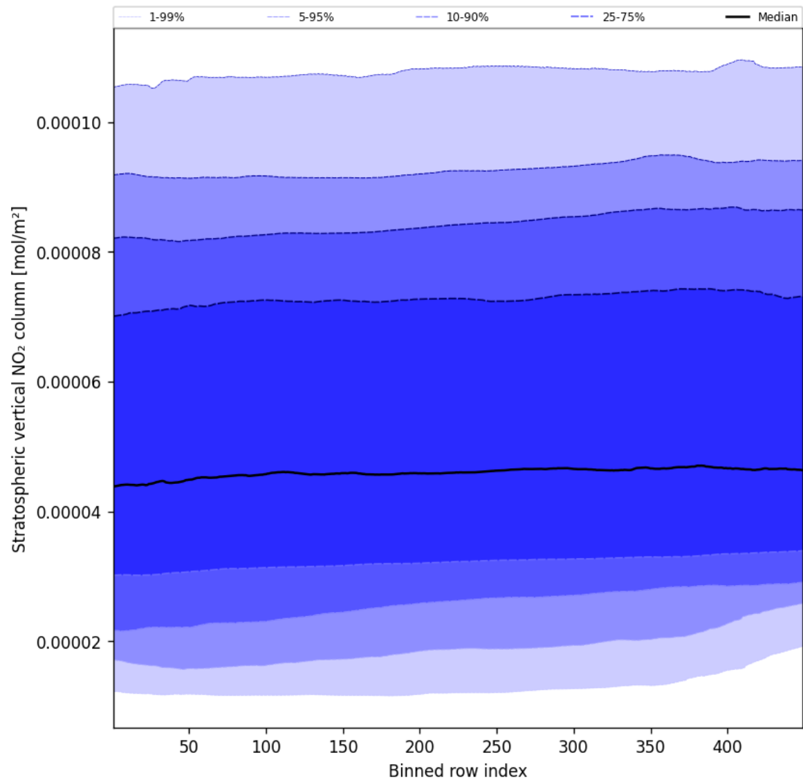
Figure 51: Along track statistics of “Stratospheric vertical NO 2 column” for 2024-12-17 to 2024-12-18
