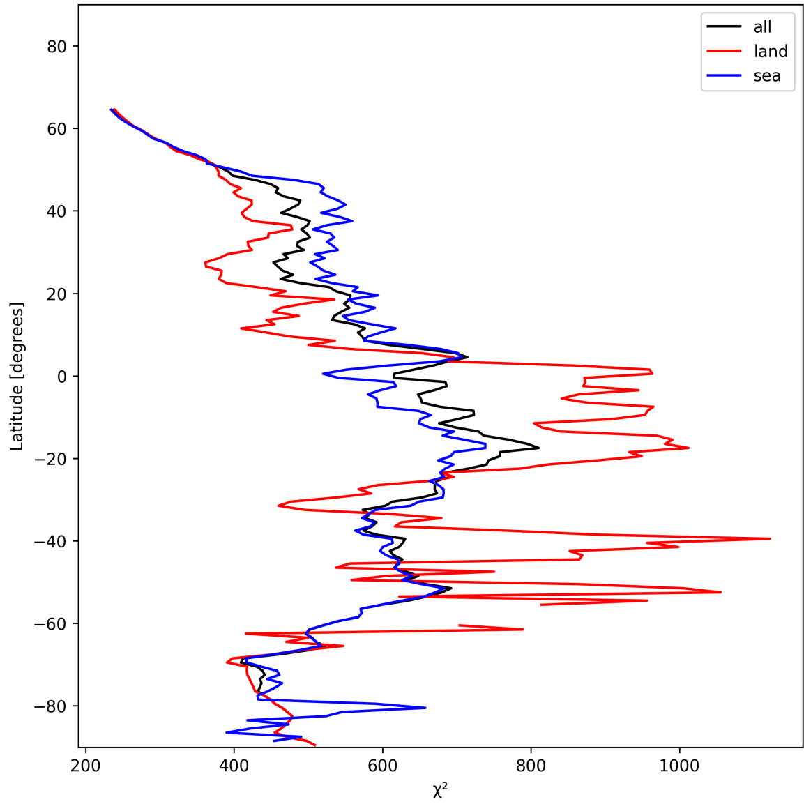
Figure 23: Zonal average of “ \chi^2 ” for 2024-12-17 to 2024-12-18.
