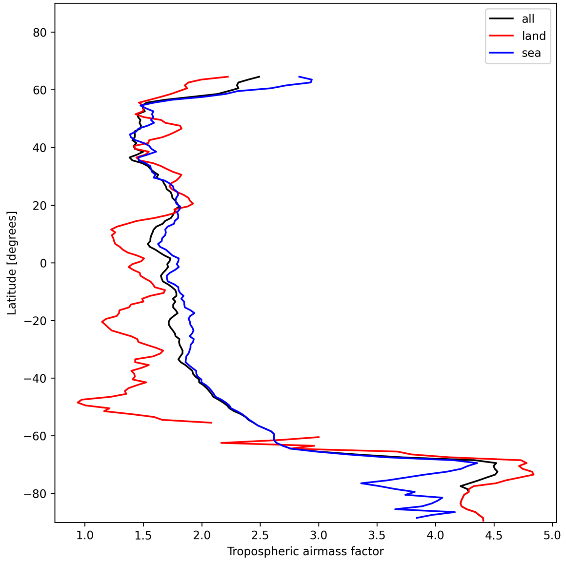
Figure 12: Zonal average of “Tropospheric airmass factor” for 2024-12-17 to 2024-12-18.
