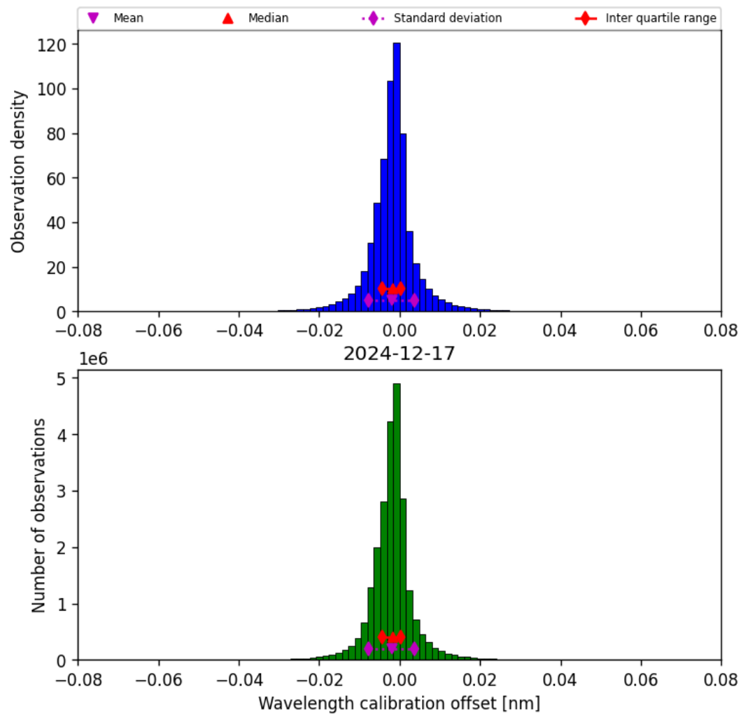
Figure 33: Histogram of “Wavelength calibration offset” for 2024-12-17 to 2024-12-18
