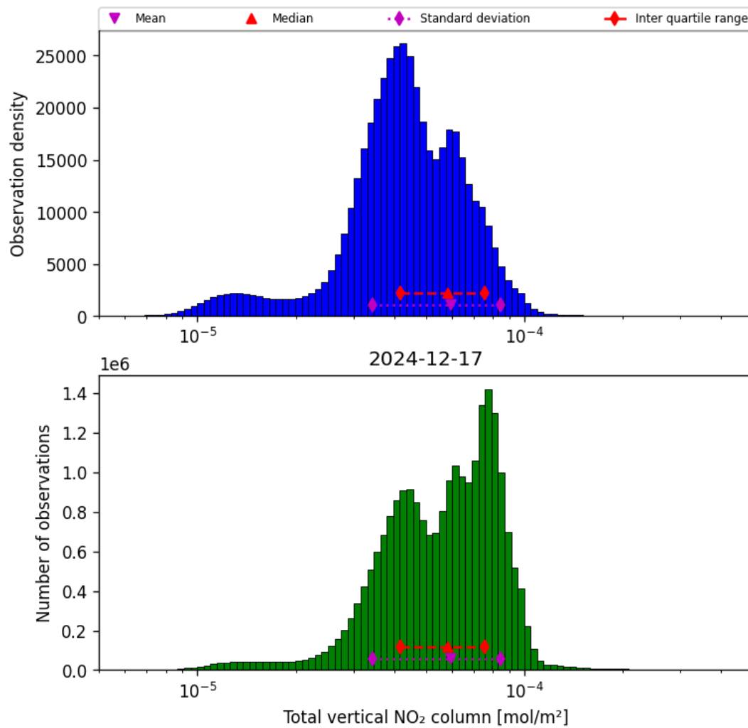
Figure 36: Histogram of “Total vertical NO 2 column” for 2024-12-17 to 2024-12-18
