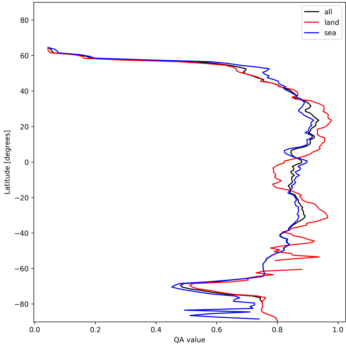
Figure 9: Zonal average of “QA value” for 2024-12-17 to 2024-12-18.
