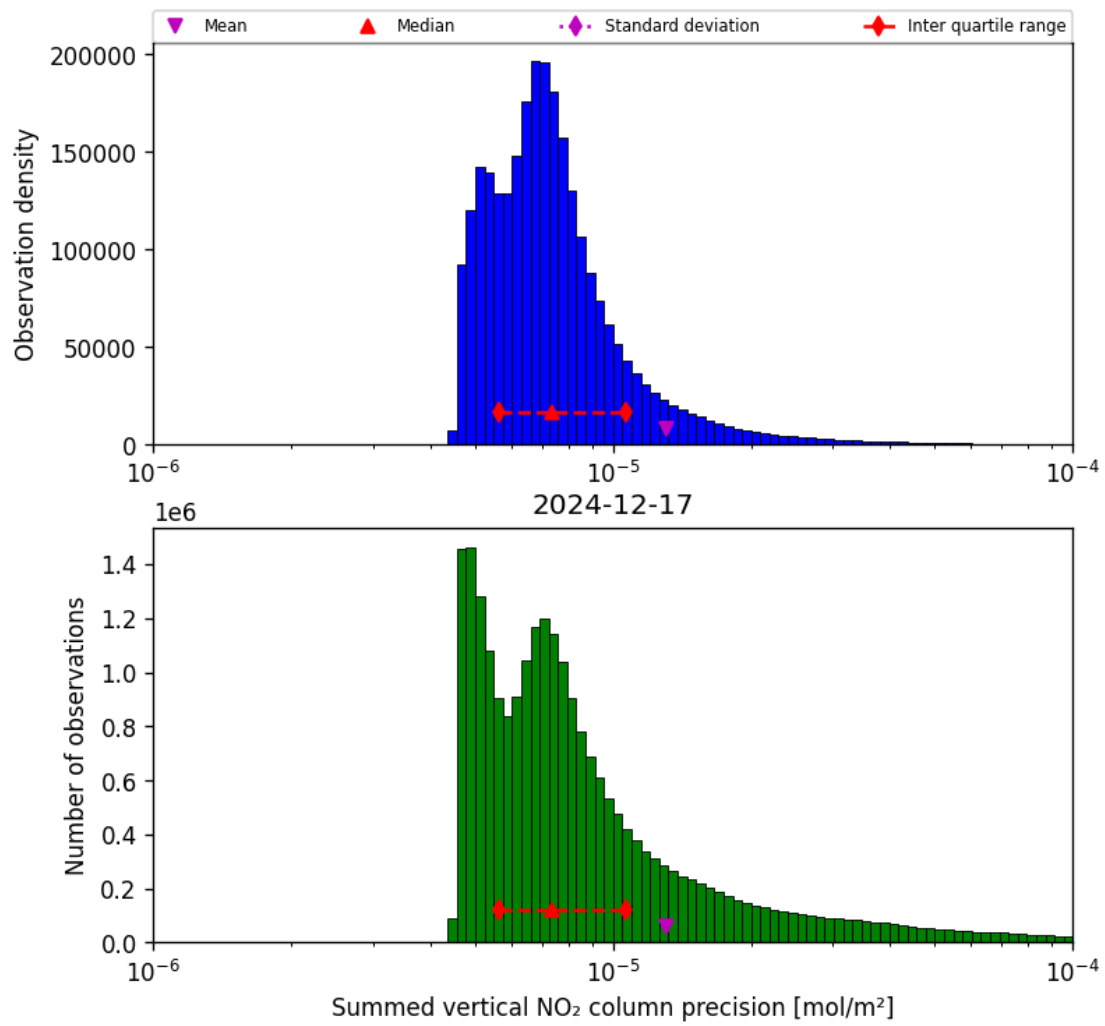
Figure 39: Histogram of “Summed vertical NO 2 column precision” for 2024-12-17 to 2024-12-18
