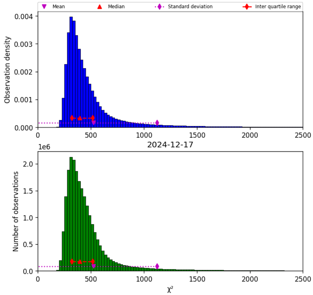
Figure 40: Histogram of “ \chi^2 ” for 2024-12-17 to 2024-12-18
