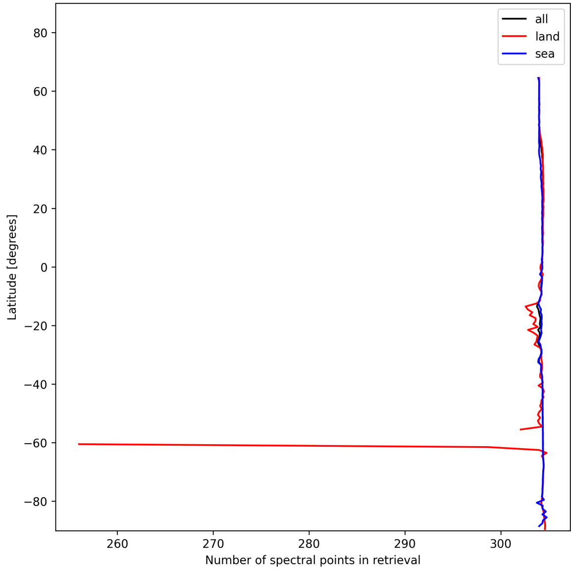
Figure 14: Zonal average of “Number of spectral points in retrieval” for 2024-12-17 to 2024-12-18.
