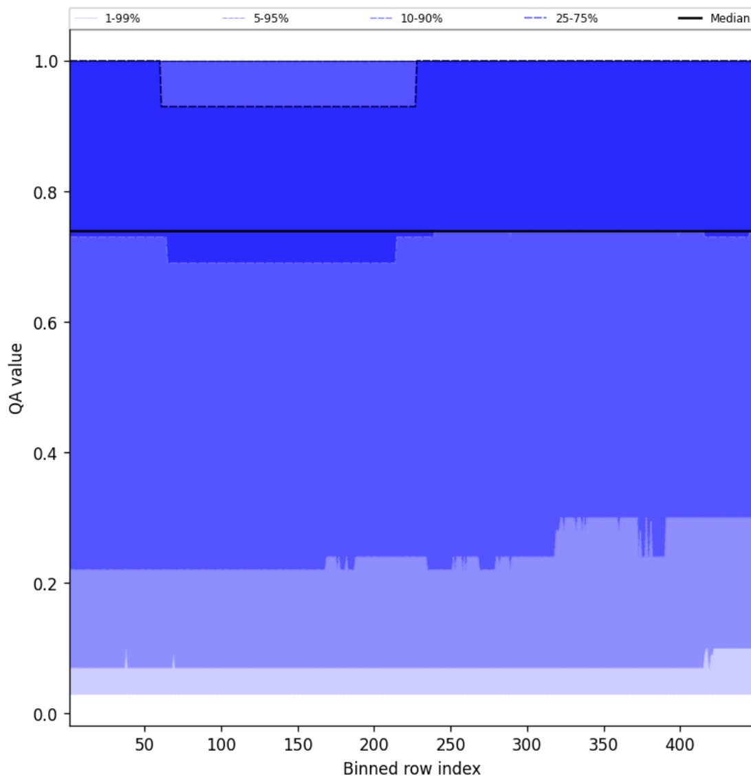
Figure 43: Along track statistics of “QA value” for 2024-12-17 to 2024-12-18
