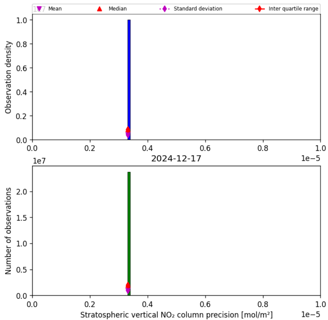
Figure 35: Histogram of “Stratospheric vertical NO 2 column precision” for 2024-12-17 to 2024-12-18
