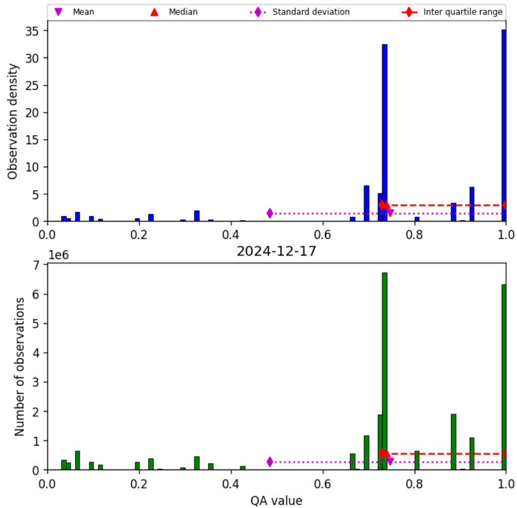
Figure 26: Histogram of “QA value” for 2024-12-17 to 2024-12-18
