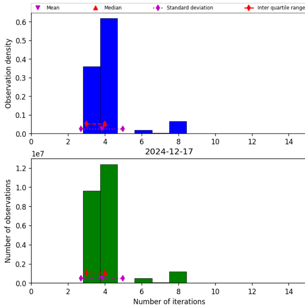
Figure 32: Histogram of “Number of iterations” for 2024-12-17 to 2024-12-18
