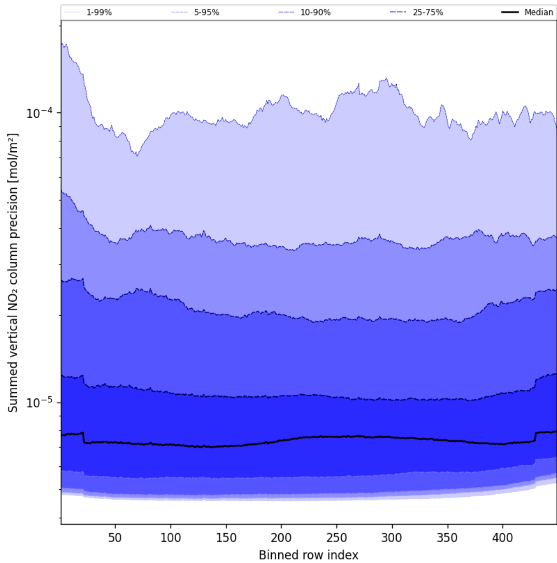
Figure 56: Along track statistics of “Summed vertical NO 2 column precision” for 2024-12-17 to 2024-12-18
