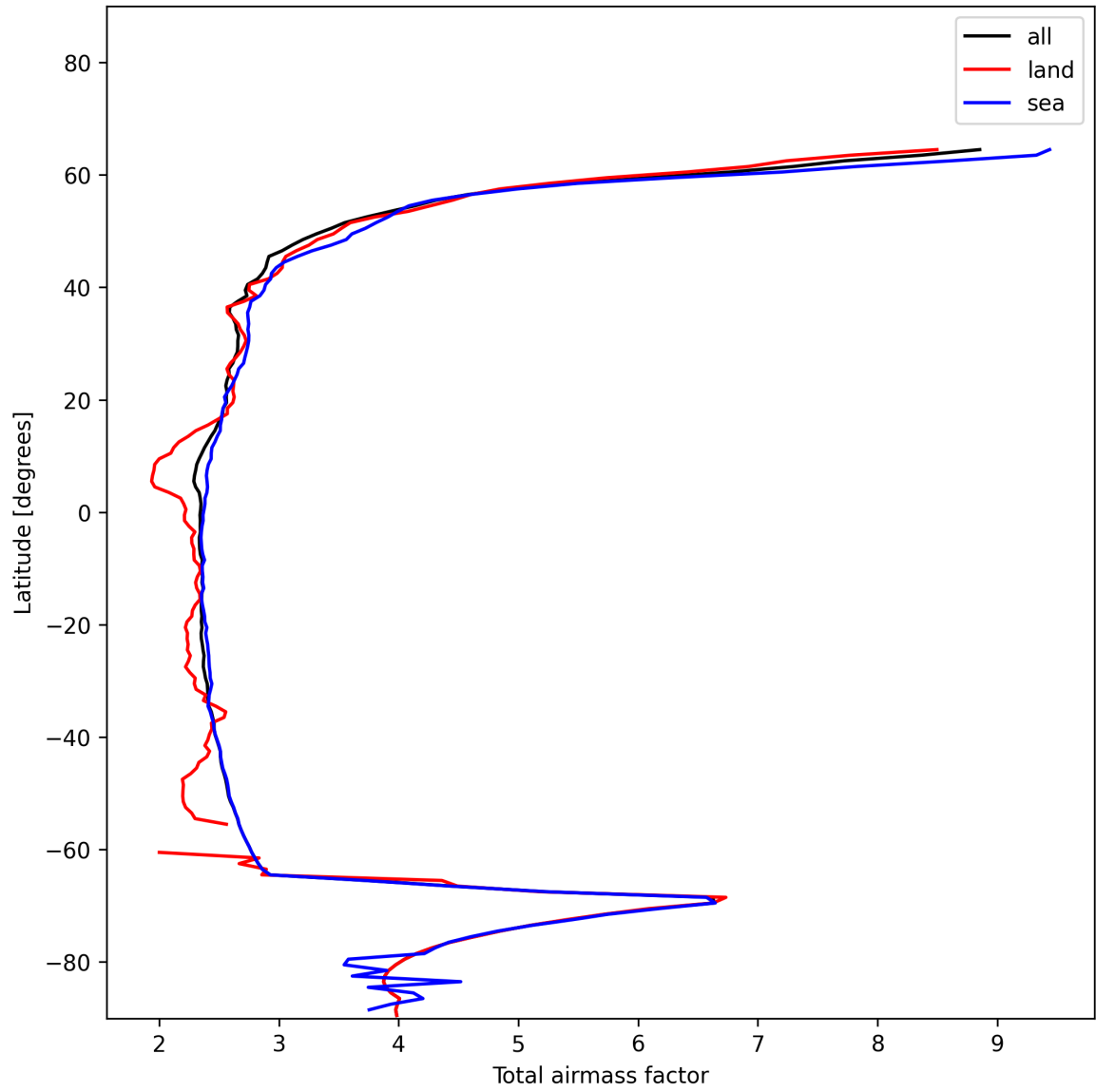
Figure 13: Zonal average of “Total airmass factor” for 2024-12-17 to 2024-12-18.
