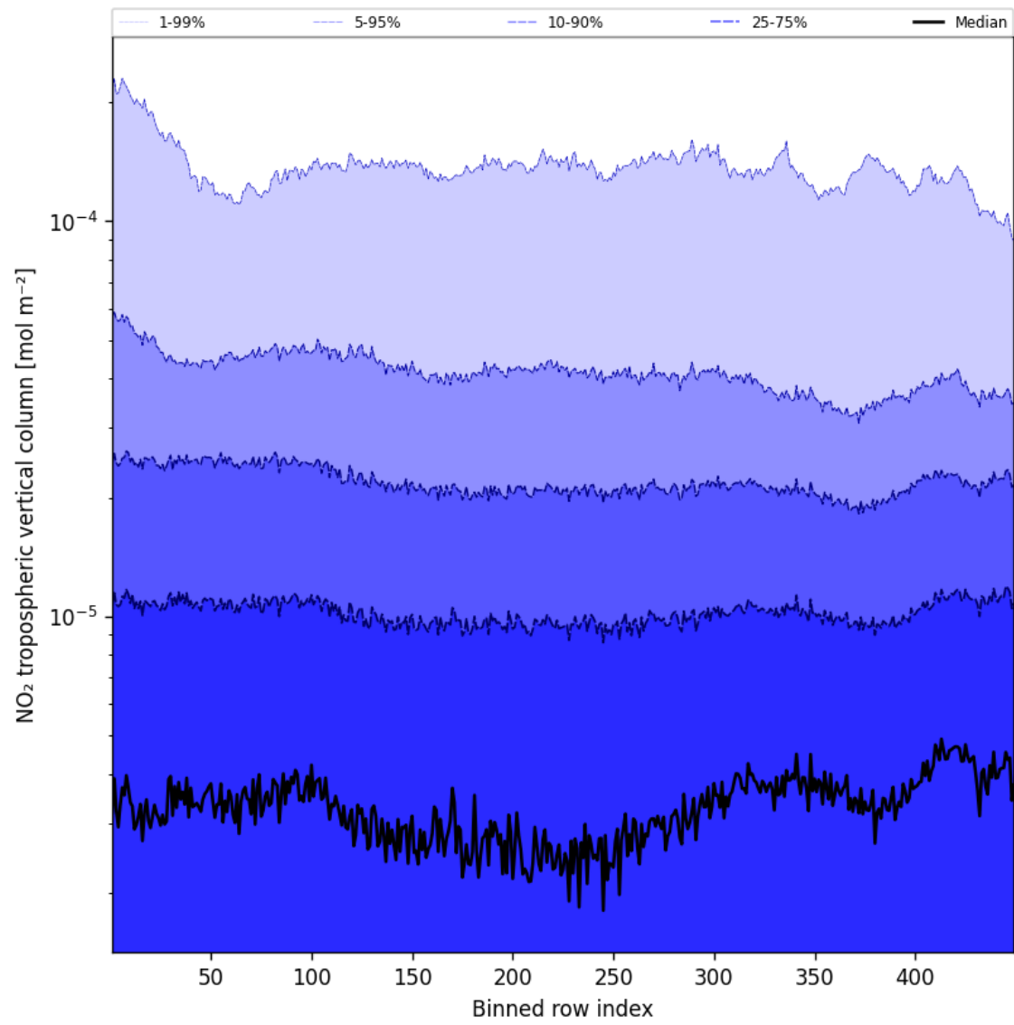
Figure 44: Along track statistics of “NO 2 tropospheric vertical column” for 2024-12-17 to 2024-12-18
