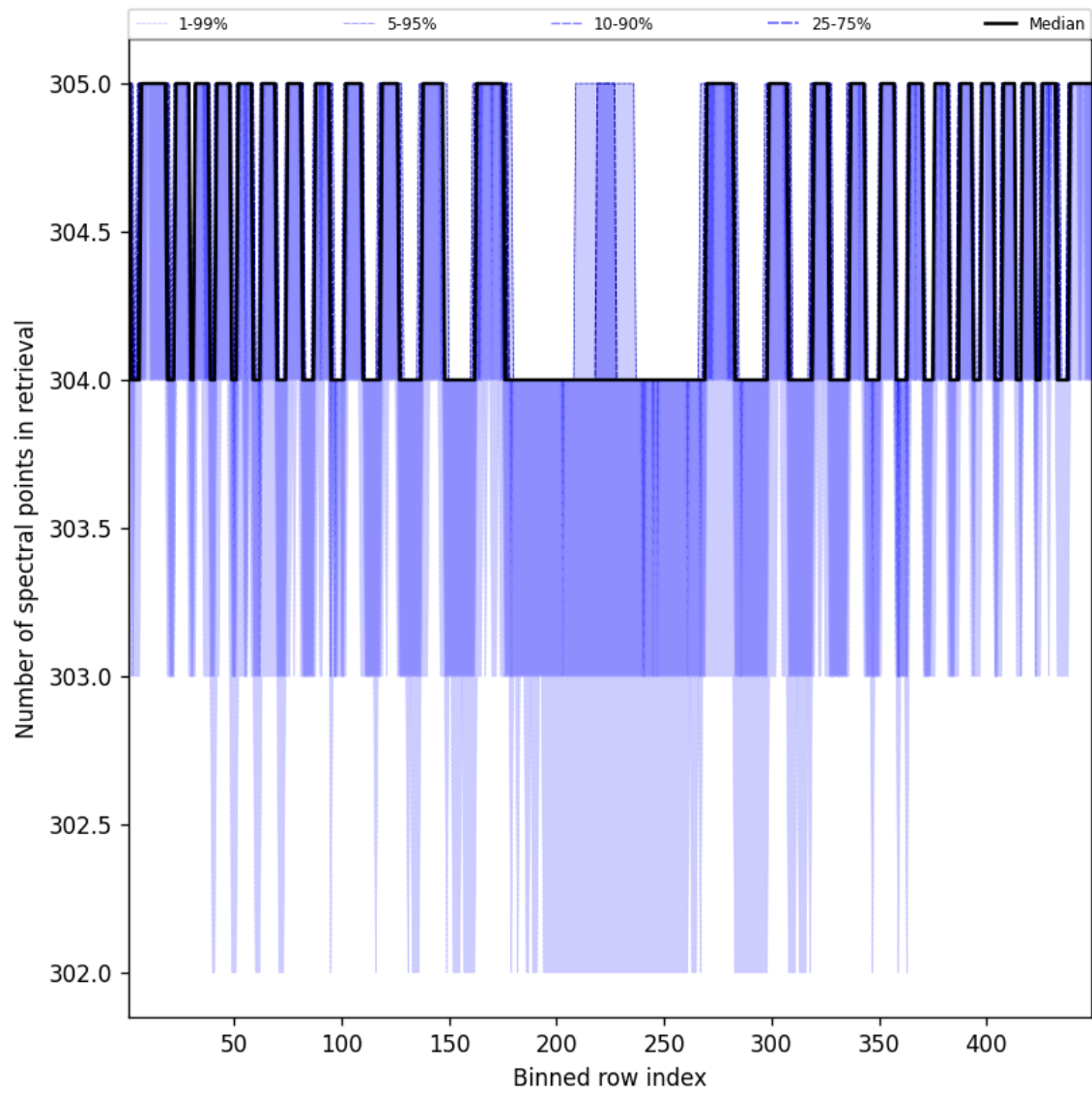
Figure 48: Along track statistics of “Number of spectral points in retrieval” for 2024-12-17 to 2024-12-18
