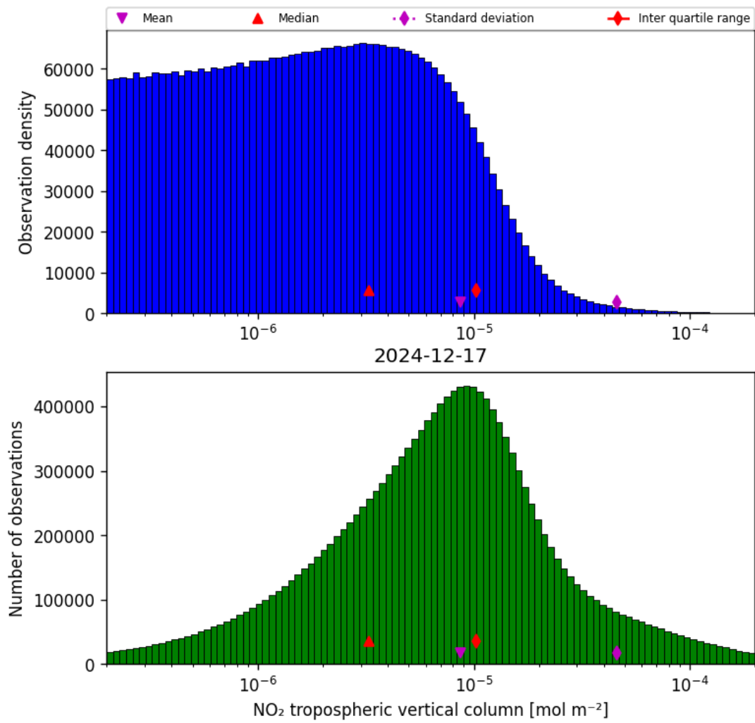
Figure 27: Histogram of “NO 2 tropospheric vertical column” for 2024-12-17 to 2024-12-18
