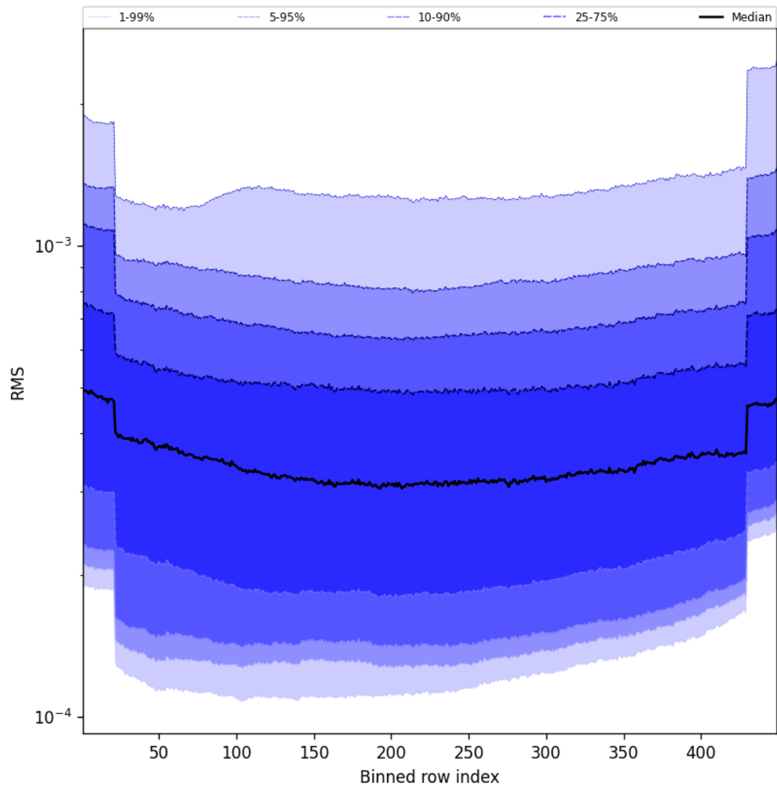
Figure 58: Along track statistics of “RMS” for 2024-12-17 to 2024-12-18
