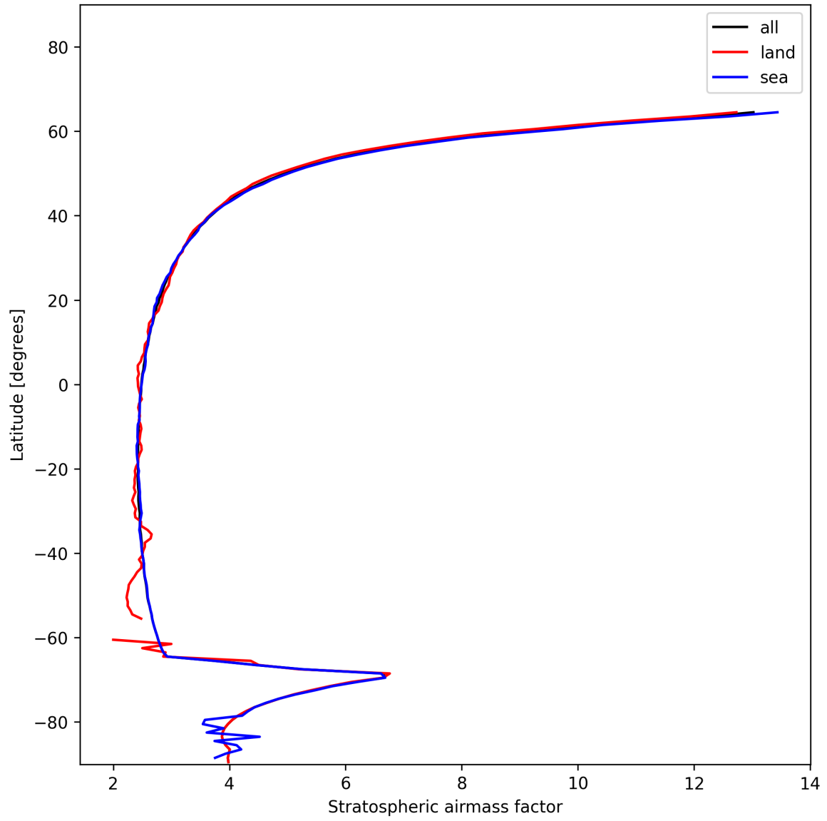
Figure 25: Zonal average of “Stratospheric airmass factor” for 2024-12-17 to 2024-12-18.
