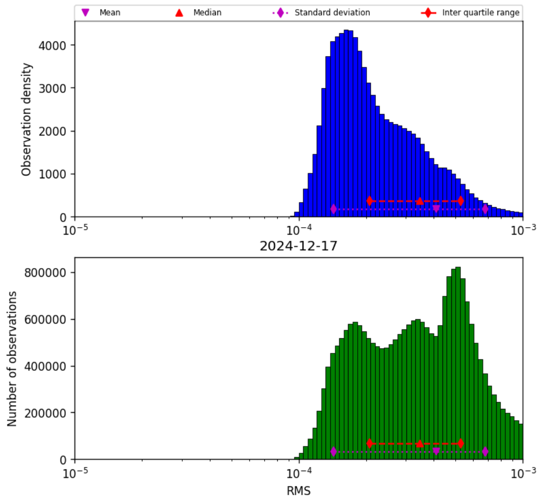
Figure 41: Histogram of “RMS” for 2024-12-17 to 2024-12-18
