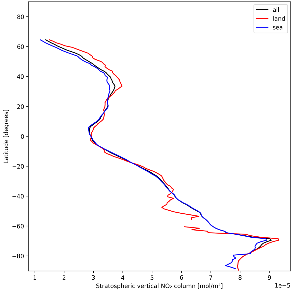
Figure 17: Zonal average of “Stratospheric vertical NO 2 column” for 2024-12-17 to 2024-12-18.
