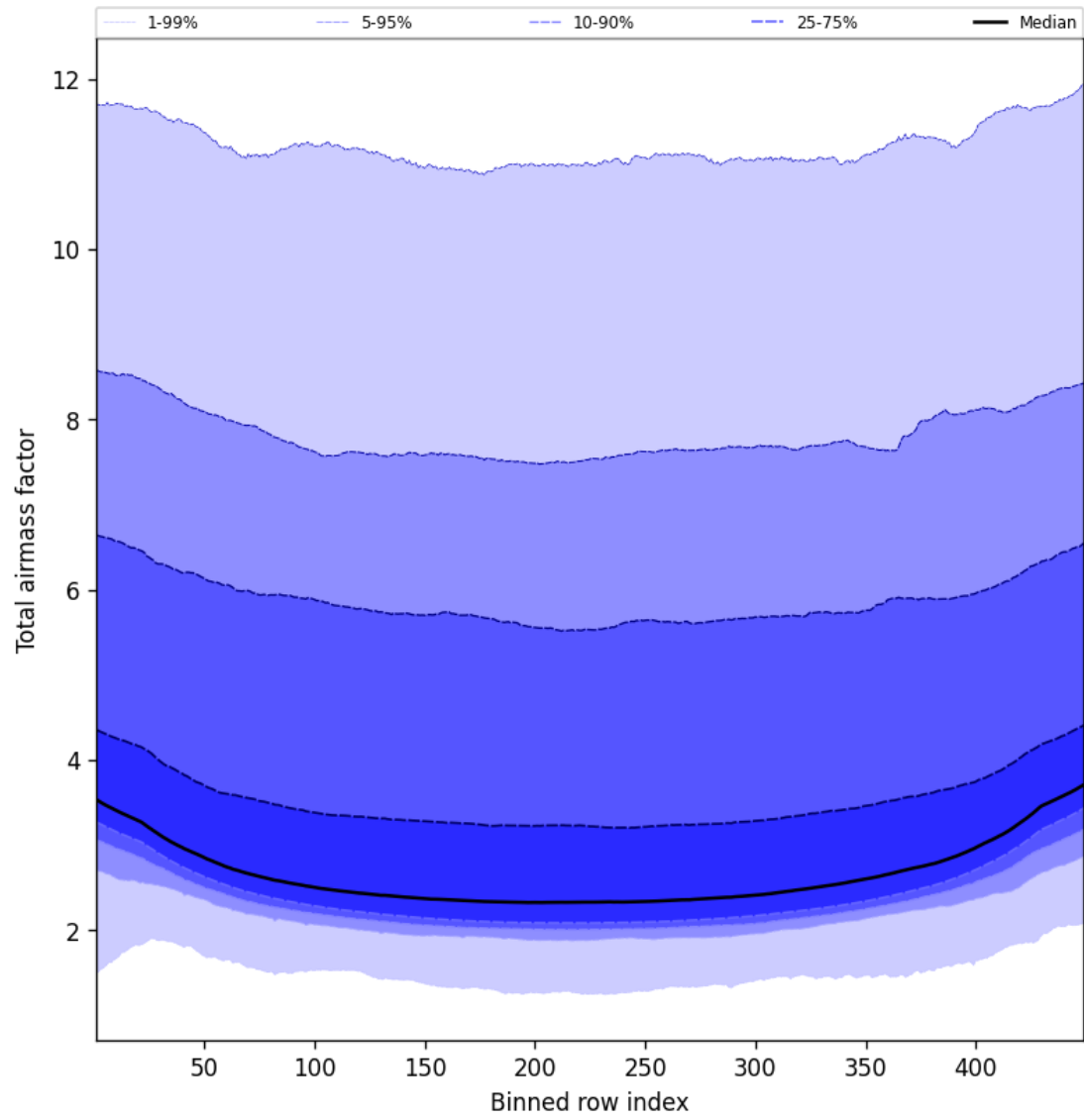
Figure 47: Along track statistics of “Total airmass factor” for 2024-12-17 to 2024-12-18
