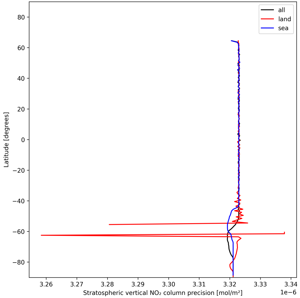
Figure 18: Zonal average of “Stratospheric vertical NO 2 column precision” for 2024-12-17 to 2024-12-18.
