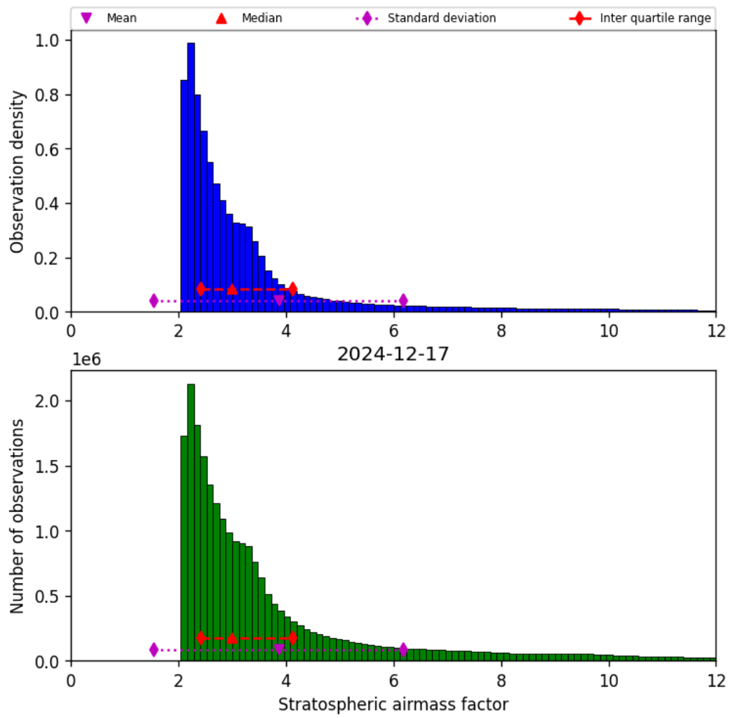
Figure 42: Histogram of “Stratospheric airmass factor” for 2024-12-17 to 2024-12-18
