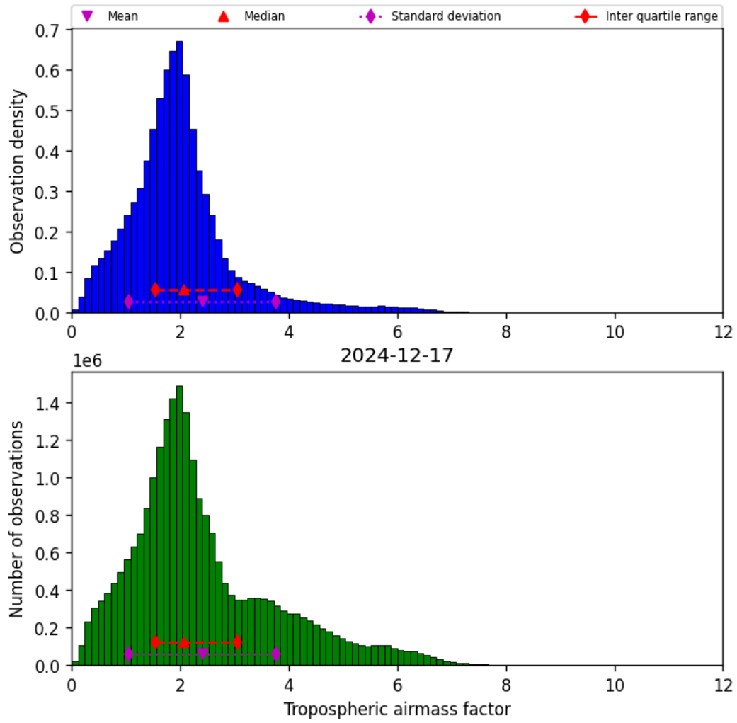
Figure 29: Histogram of “Tropospheric airmass factor” for 2024-12-17 to 2024-12-18
