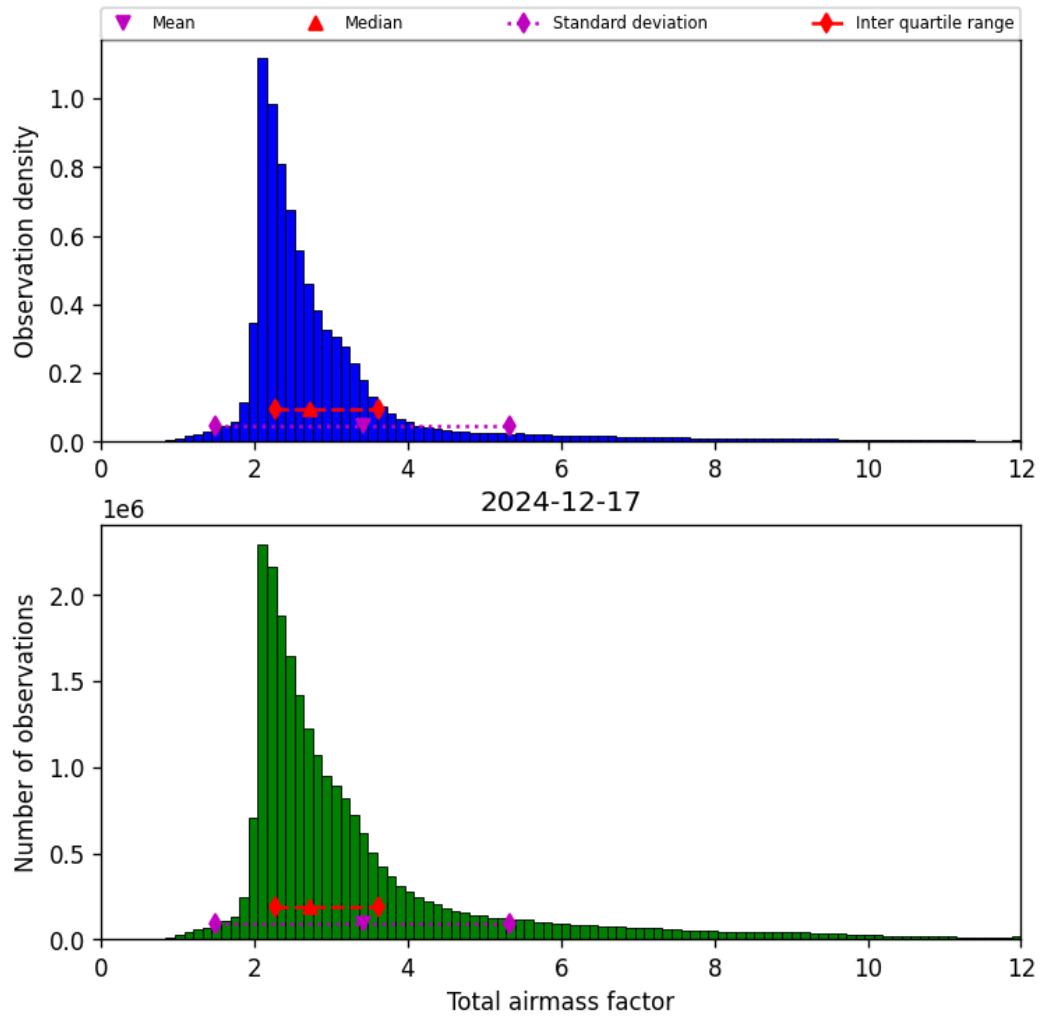
Figure 30: Histogram of “Total airmass factor” for 2024-12-17 to 2024-12-18
