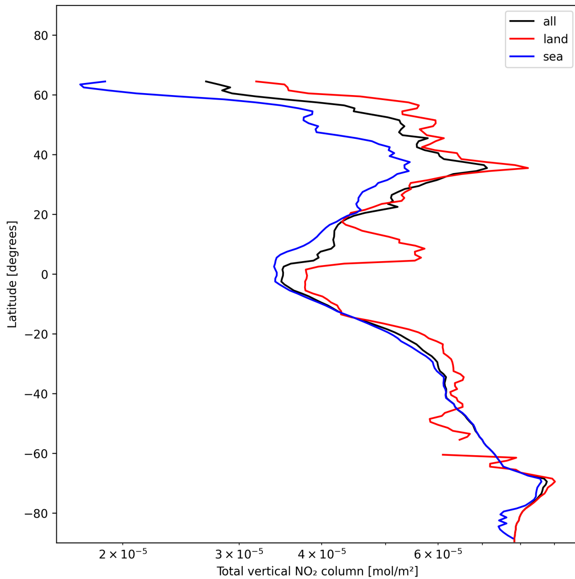
Figure 19: Zonal average of “Total vertical NO 2 column” for 2024-12-17 to 2024-12-18.
