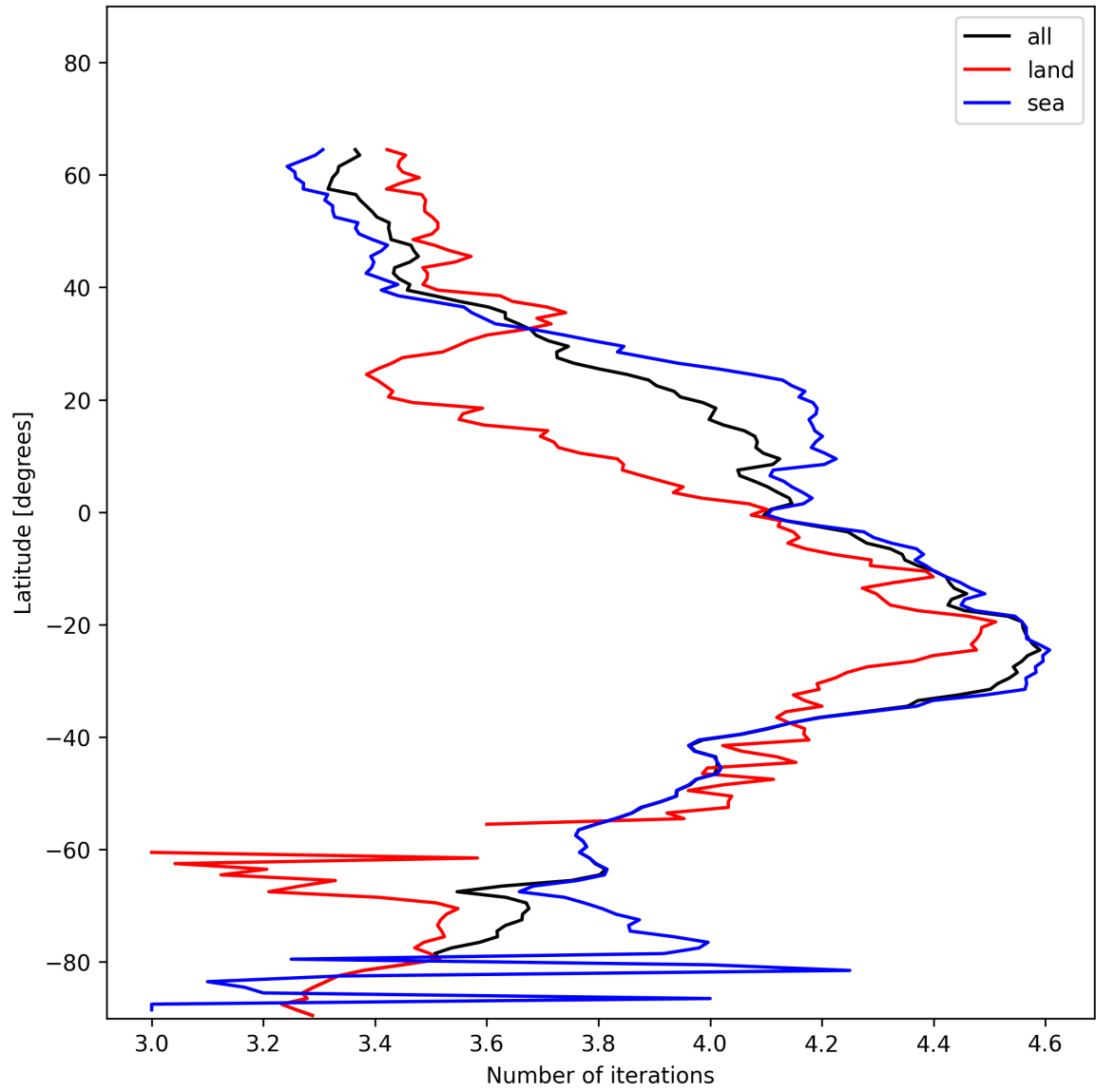
Figure 15: Zonal average of “Number of iterations” for 2024-12-17 to 2024-12-18.
