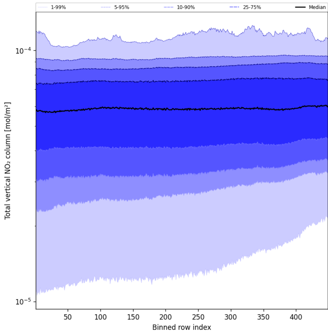
Figure 53: Along track statistics of “Total vertical NO 2 column” for 2024-12-17 to 2024-12-18
