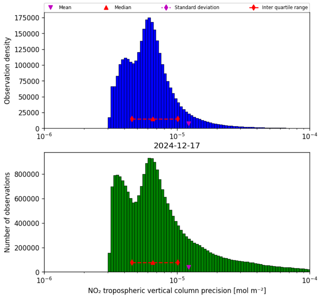
Figure 28: Histogram of “NO 2 tropospheric vertical column precision” for 2024-12-17 to 2024-12-18
