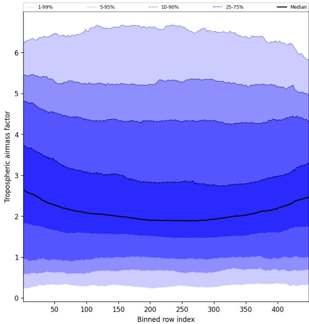
Figure 46: Along track statistics of “Tropospheric airmass factor” for 2024-12-17 to 2024-12-18
