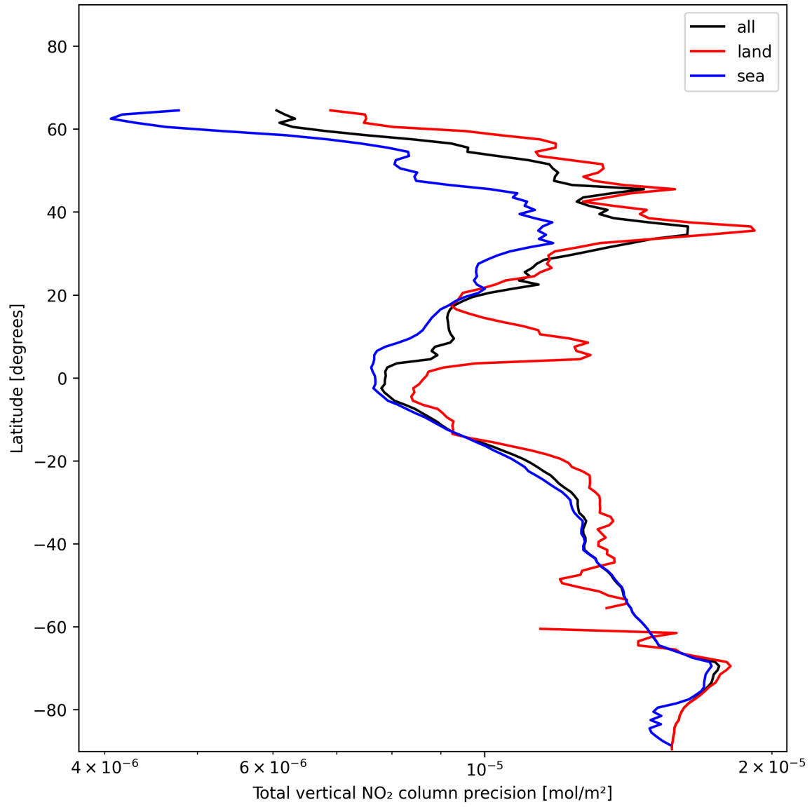
Figure 20: Zonal average of “Total vertical NO 2 column precision” for 2024-12-17 to 2024-12-18.
