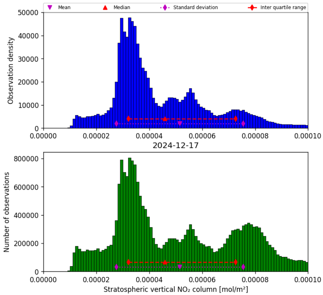
Figure 34: Histogram of “Stratospheric vertical NO 2 column” for 2024-12-17 to 2024-12-18
