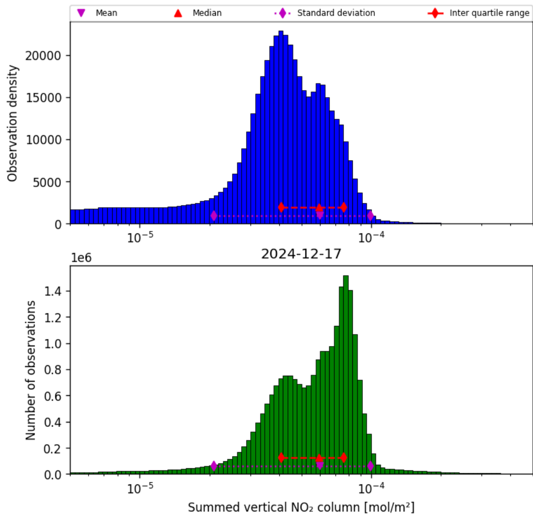
Figure 38: Histogram of “Summed vertical NO 2 column” for 2024-12-17 to 2024-12-18
