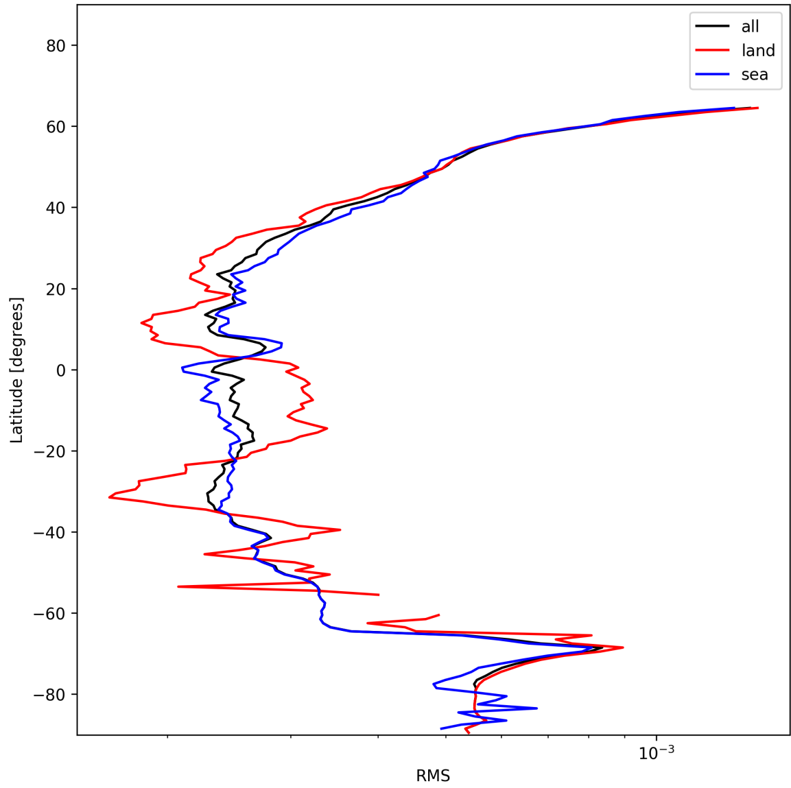
Figure 24: Zonal average of “RMS” for 2024-12-17 to 2024-12-18.
