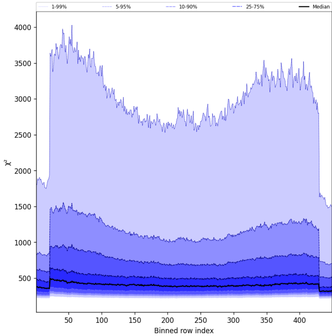
Figure 57: Along track statistics of “ \chi^2 ” for 2024-12-17 to 2024-12-18
