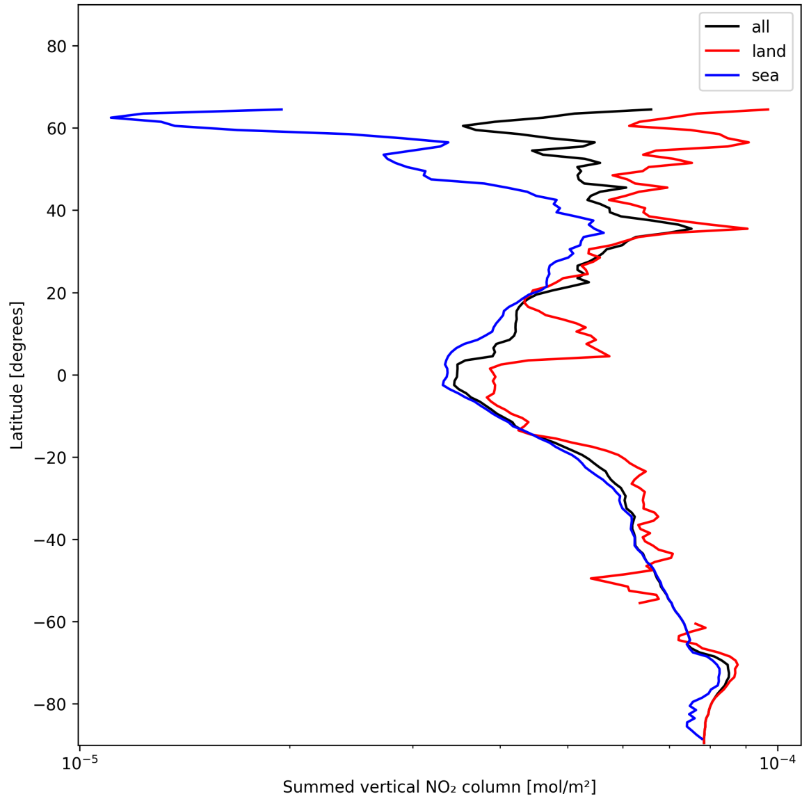
Figure 21: Zonal average of “Summed vertical NO 2 column” for 2024-12-17 to 2024-12-18.
