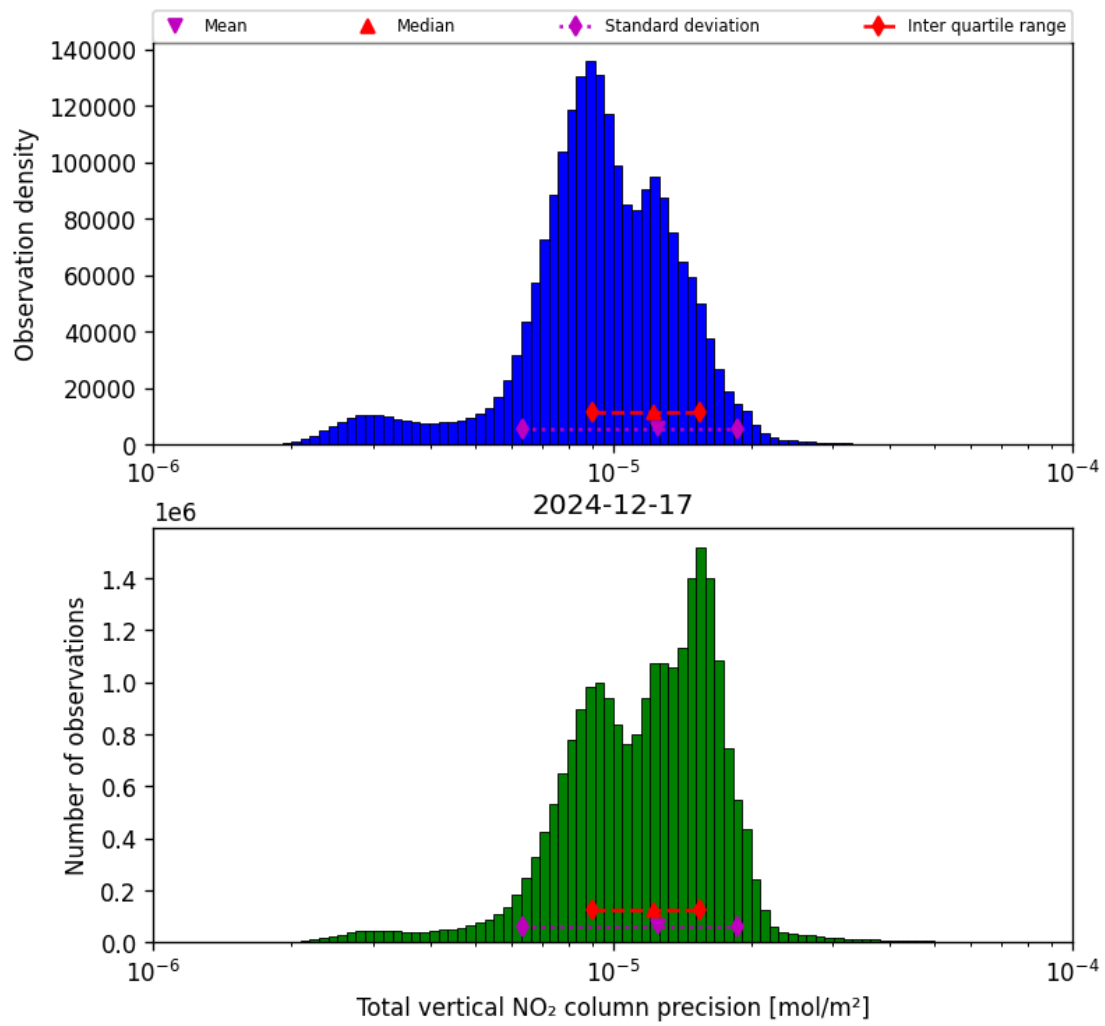
Figure 37: Histogram of “Total vertical NO 2 column precision” for 2024-12-17 to 2024-12-18
