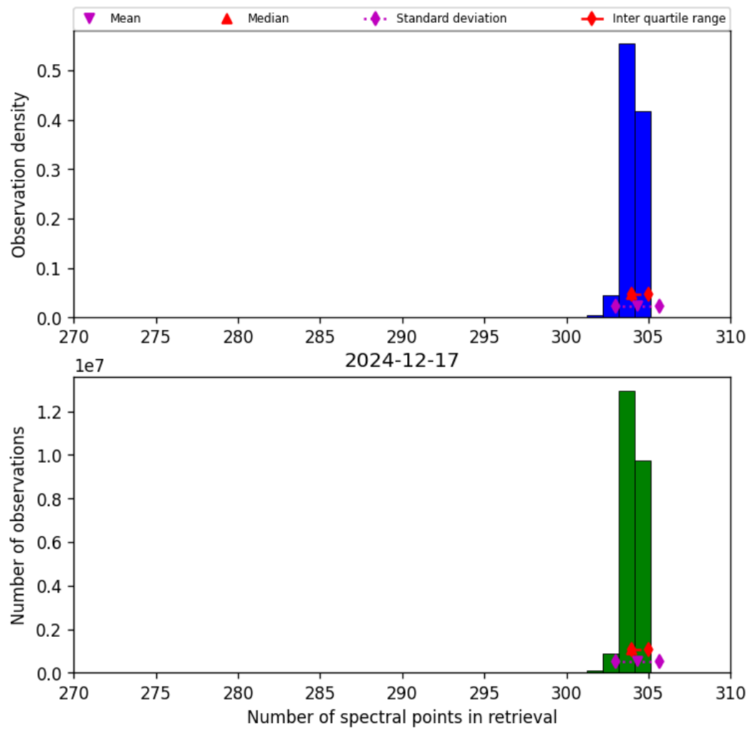
Figure 31: Histogram of “Number of spectral points in retrieval” for 2024-12-17 to 2024-12-18
