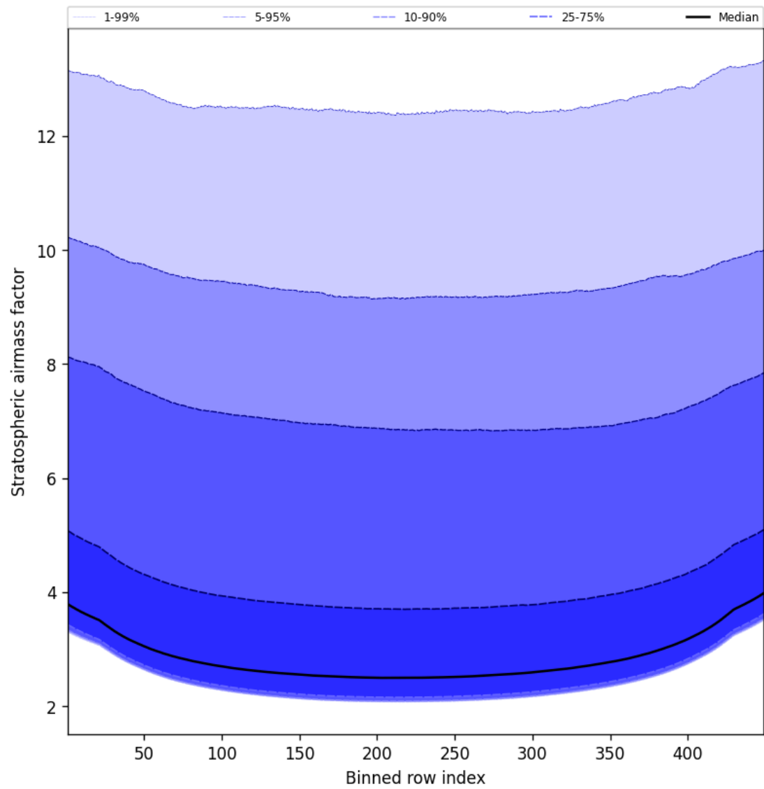
Figure 59: Along track statistics of “Stratospheric airmass factor” for 2024-12-17 to 2024-12-18
