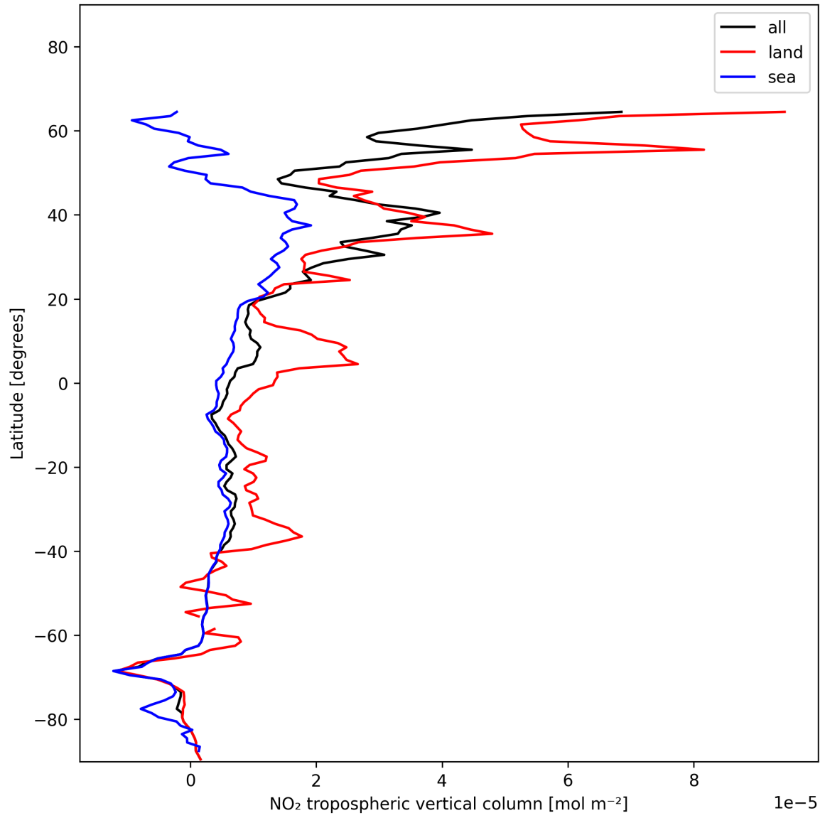
Figure 10: Zonal average of “NO 2 tropospheric vertical column” for 2024-12-18 to 2024-12-19.
