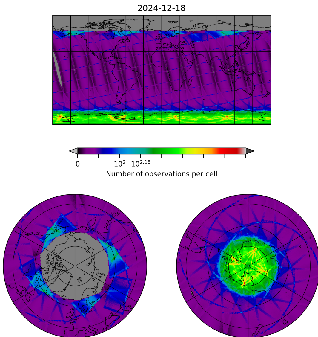
Figure 8: Map of the number of observations for 2024-12-18 to 2024-12-19
