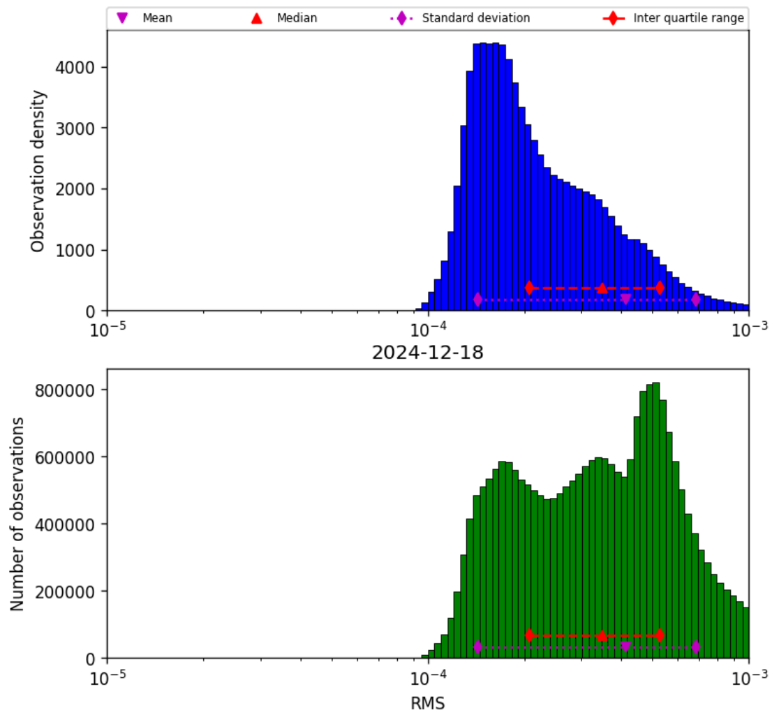
Figure 41: Histogram of “RMS” for 2024-12-18 to 2024-12-19
