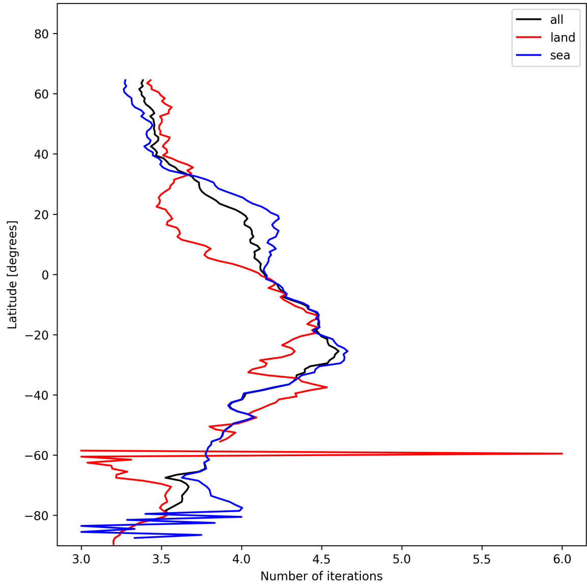
Figure 15: Zonal average of “Number of iterations” for 2024-12-18 to 2024-12-19.
