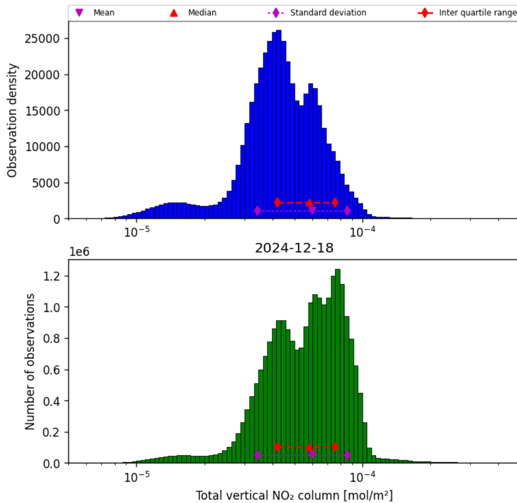
Figure 36: Histogram of “Total vertical NO 2 column” for 2024-12-18 to 2024-12-19
