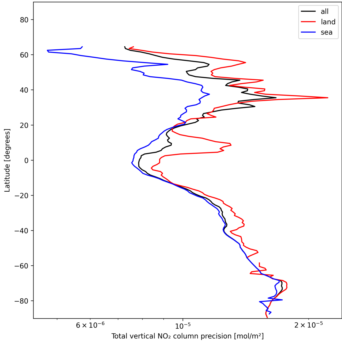
Figure 20: Zonal average of “Total vertical NO 2 column precision” for 2024-12-18 to 2024-12-19.
