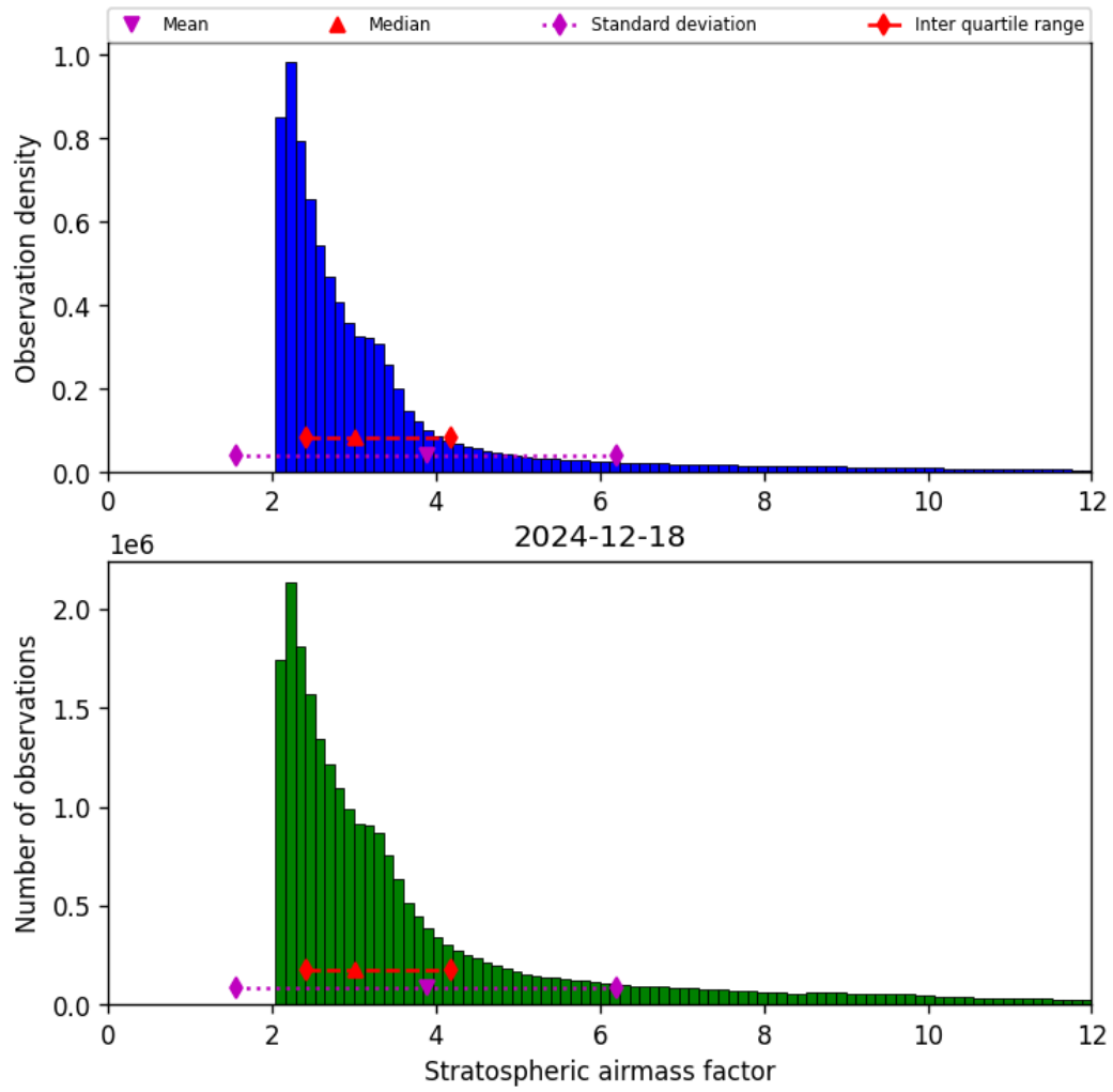
Figure 42: Histogram of “Stratospheric airmass factor” for 2024-12-18 to 2024-12-19
