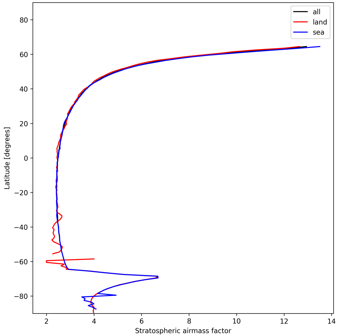
Figure 25: Zonal average of “Stratospheric airmass factor” for 2024-12-18 to 2024-12-19.
