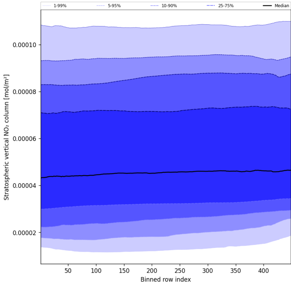
Figure 51: Along track statistics of “Stratospheric vertical NO 2 column” for 2024-12-18 to 2024-12-19
