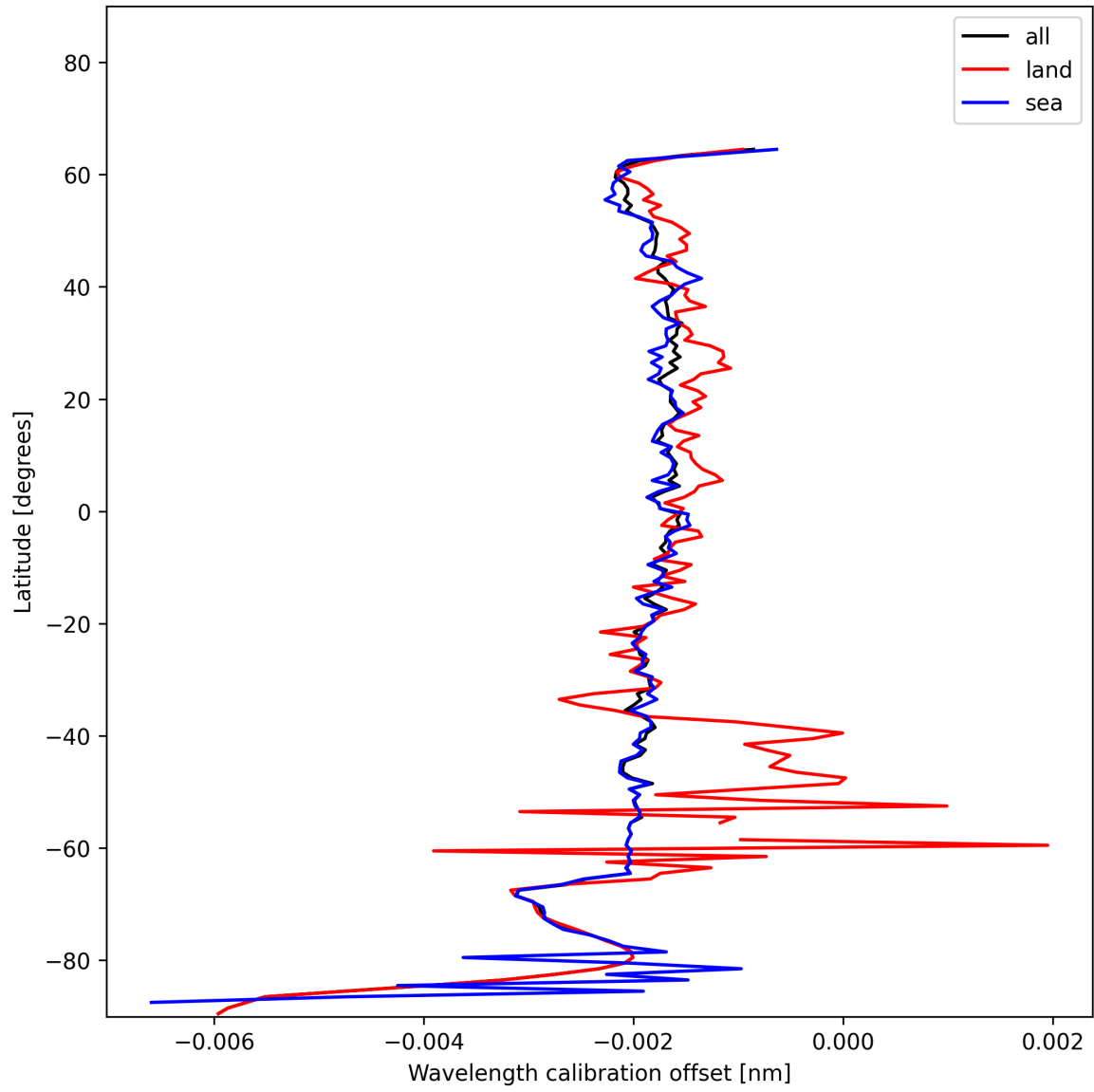
Figure 16: Zonal average of “Wavelength calibration offset” for 2024-12-18 to 2024-12-19.
