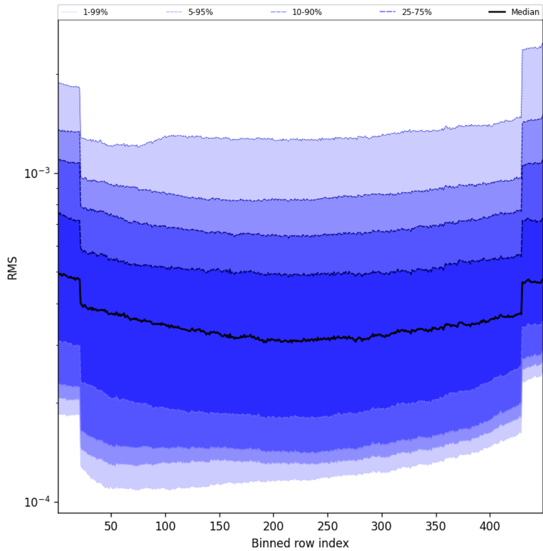
Figure 58: Along track statistics of “RMS” for 2024-12-18 to 2024-12-19
