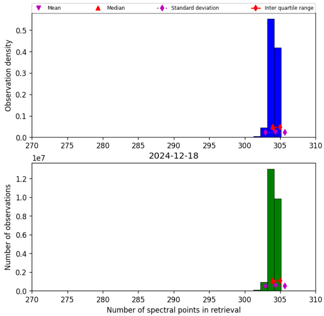
Figure 31: Histogram of “Number of spectral points in retrieval” for 2024-12-18 to 2024-12-19
