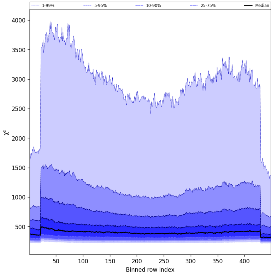
Figure 57: Along track statistics of “ \chi^2 ” for 2024-12-18 to 2024-12-19
