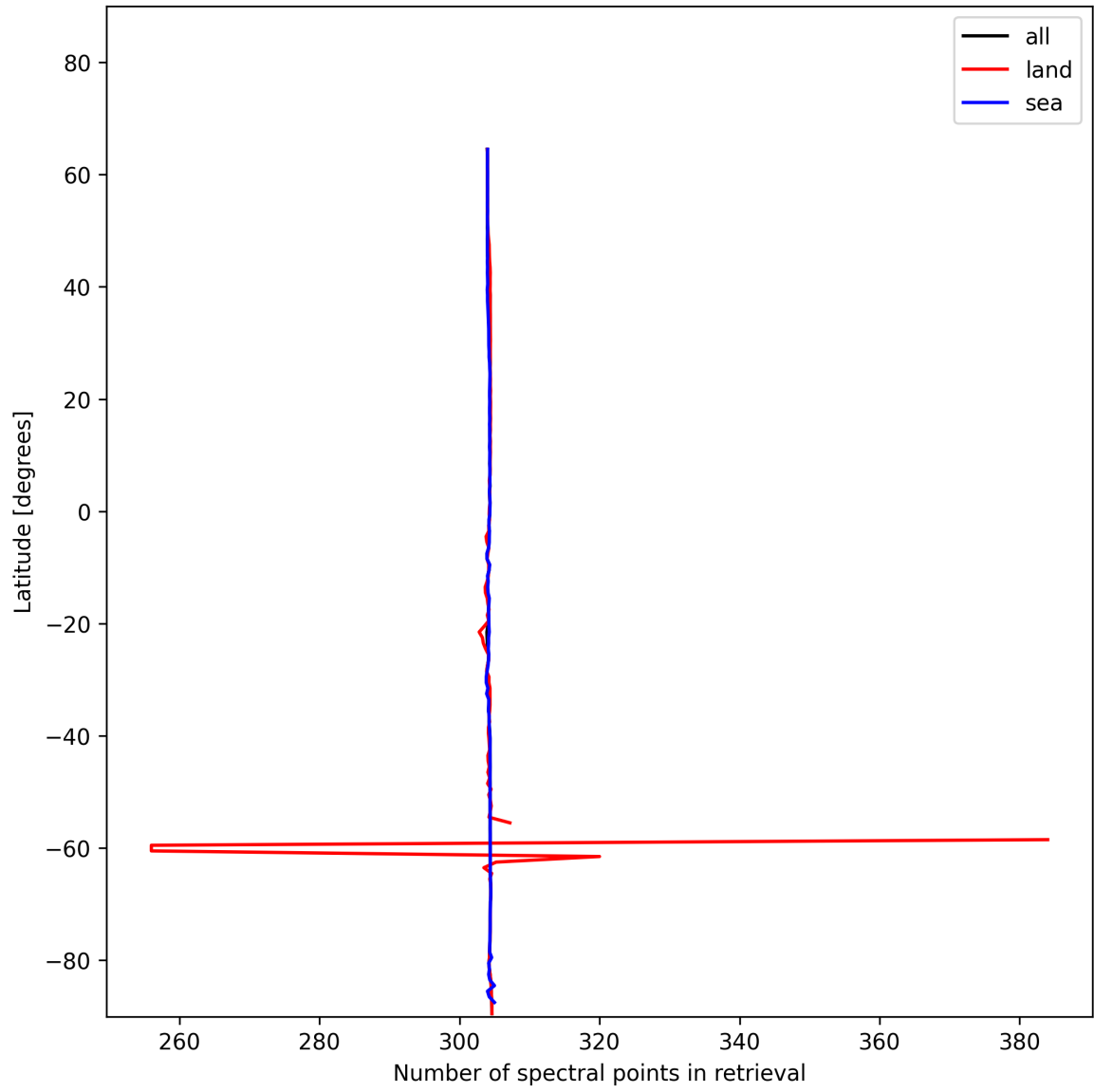
Figure 14: Zonal average of “Number of spectral points in retrieval” for 2024-12-18 to 2024-12-19.
