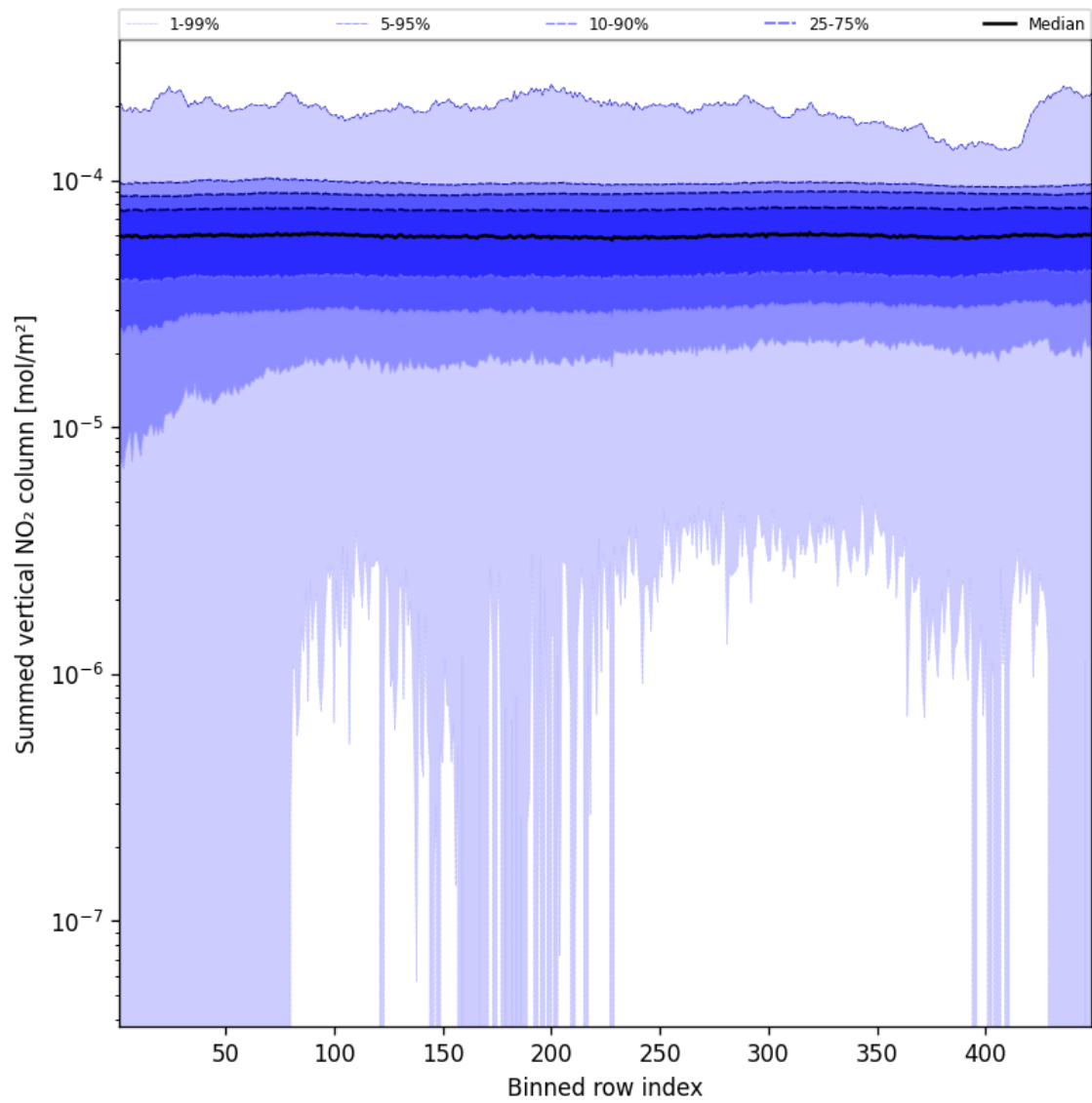
Figure 55: Along track statistics of “Summed vertical NO 2 column” for 2024-12-18 to 2024-12-19
