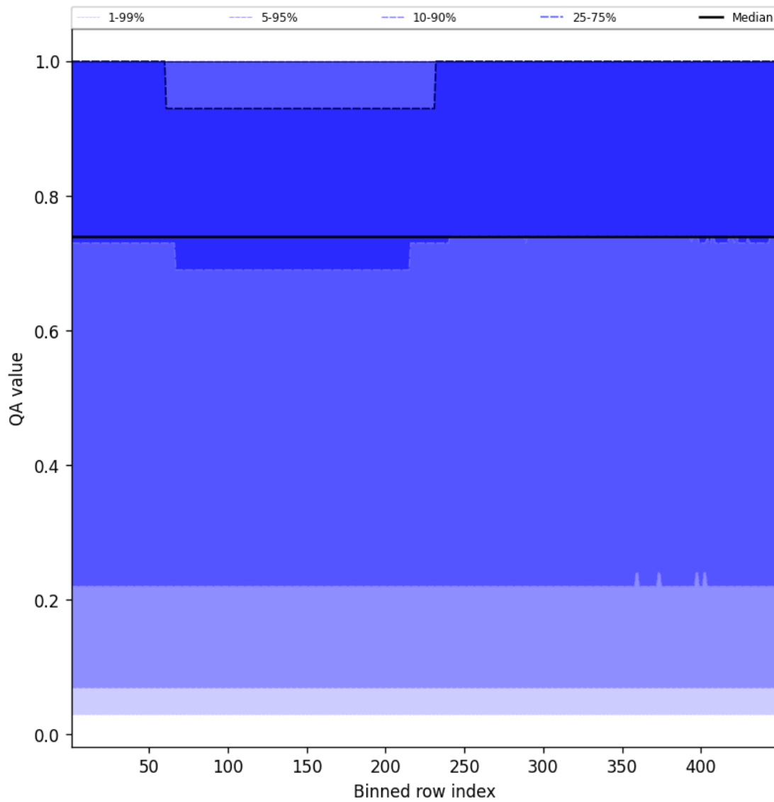
Figure 43: Along track statistics of “QA value” for 2024-12-18 to 2024-12-19
