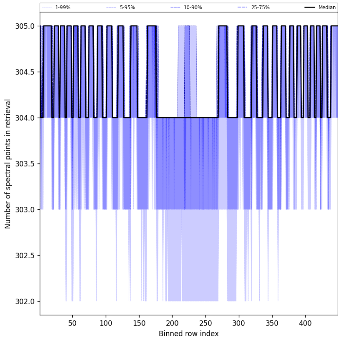
Figure 48: Along track statistics of “Number of spectral points in retrieval” for 2024-12-18 to 2024-12-19
