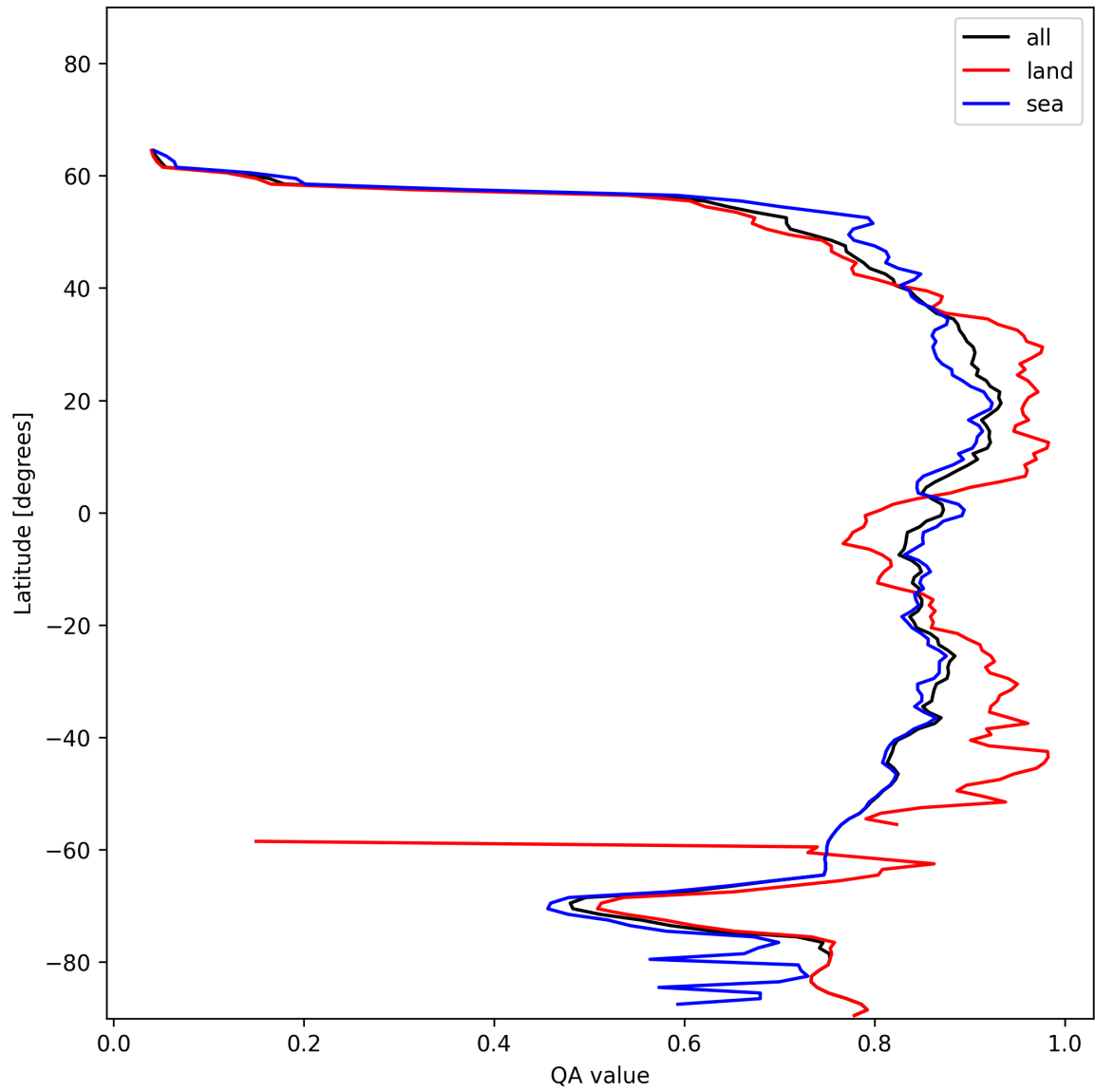
Figure 9: Zonal average of “QA value” for 2024-12-18 to 2024-12-19.
