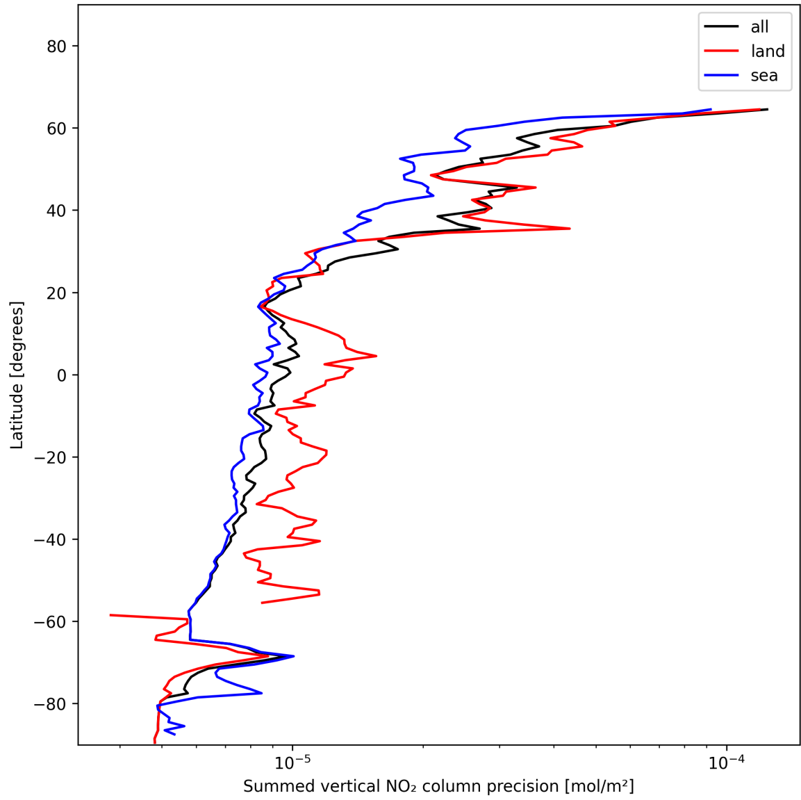
Figure 22: Zonal average of “Summed vertical NO 2 column precision” for 2024-12-18 to 2024-12-19.
