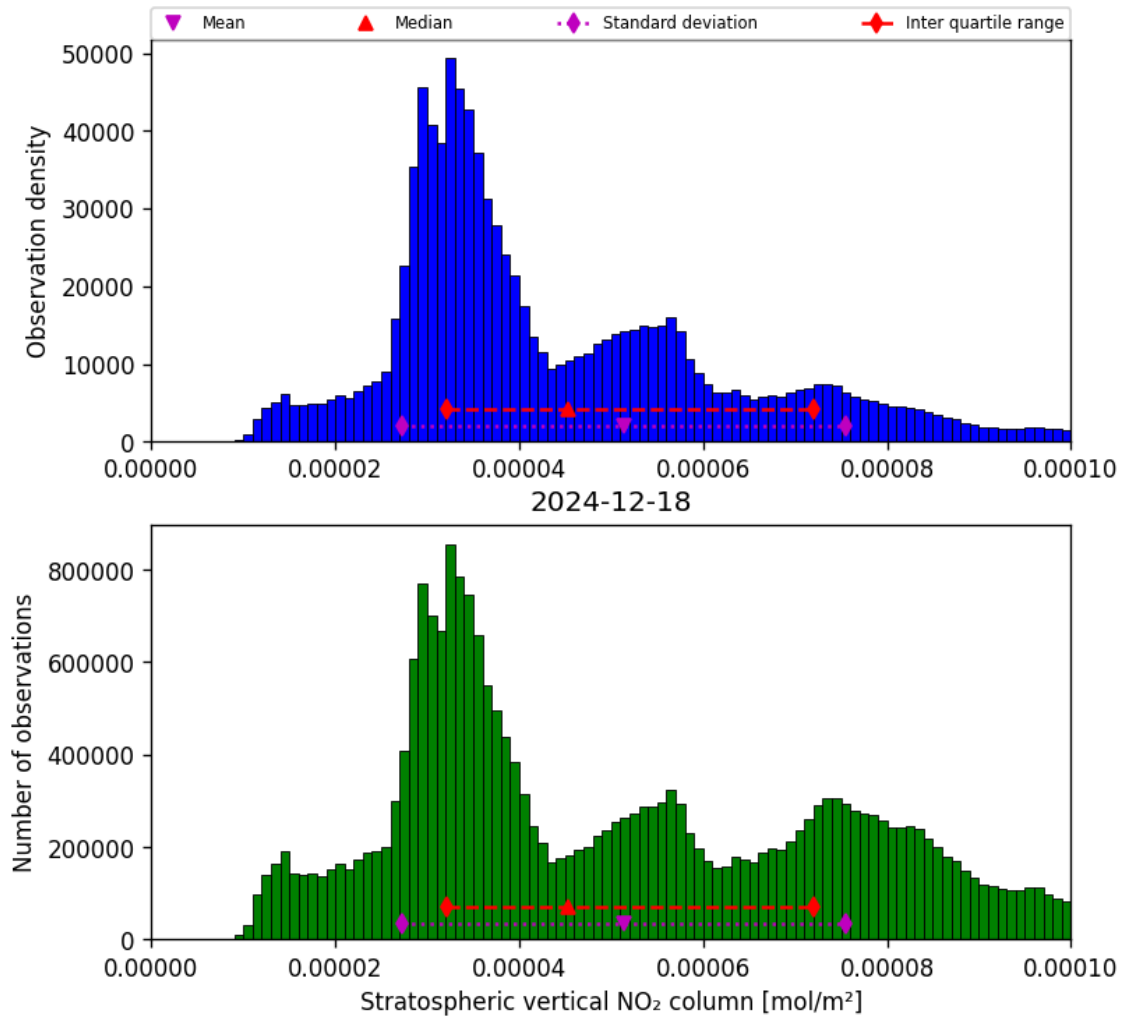
Figure 34: Histogram of “Stratospheric vertical NO 2 column” for 2024-12-18 to 2024-12-19
