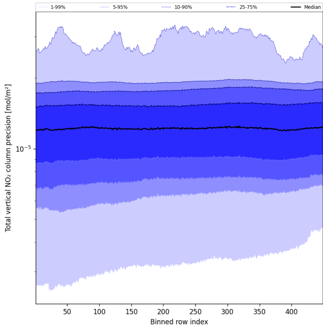
Figure 54: Along track statistics of “Total vertical NO 2 column precision” for 2024-12-18 to 2024-12-19
