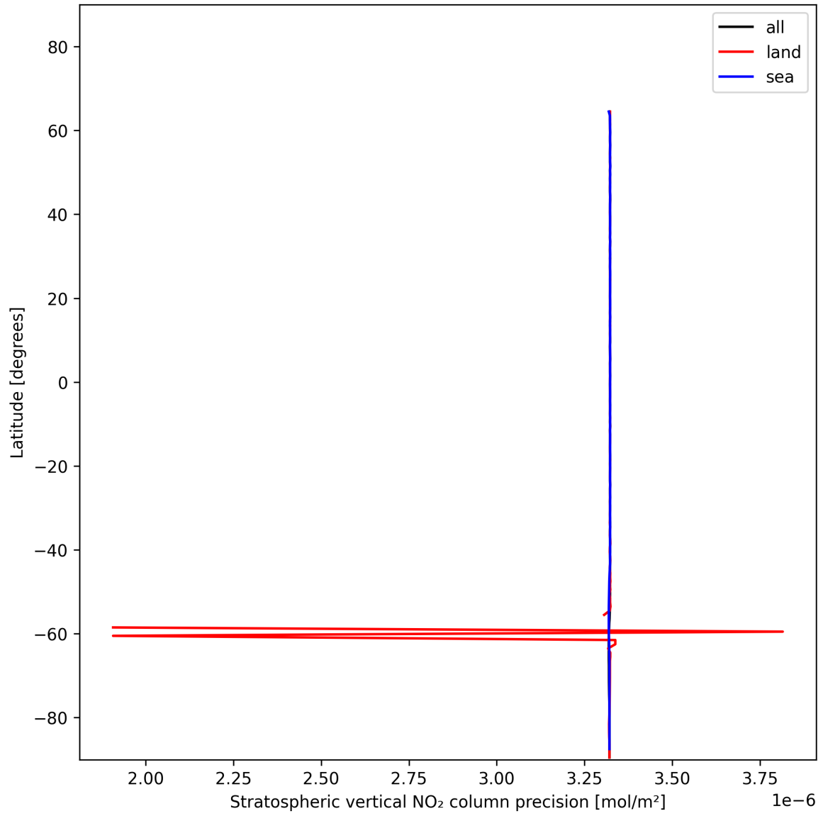
Figure 18: Zonal average of “Stratospheric vertical NO 2 column precision” for 2024-12-18 to 2024-12-19.
