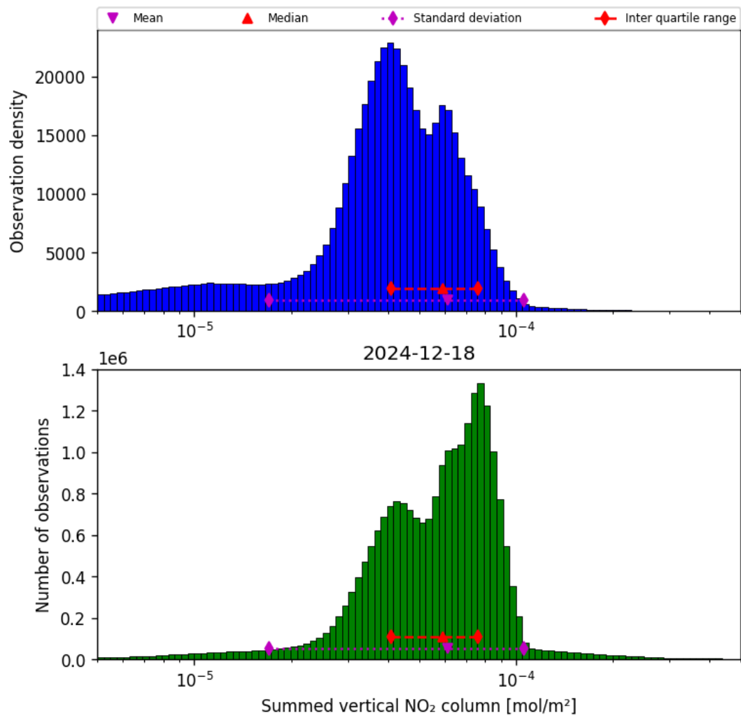
Figure 38: Histogram of “Summed vertical NO 2 column” for 2024-12-18 to 2024-12-19
