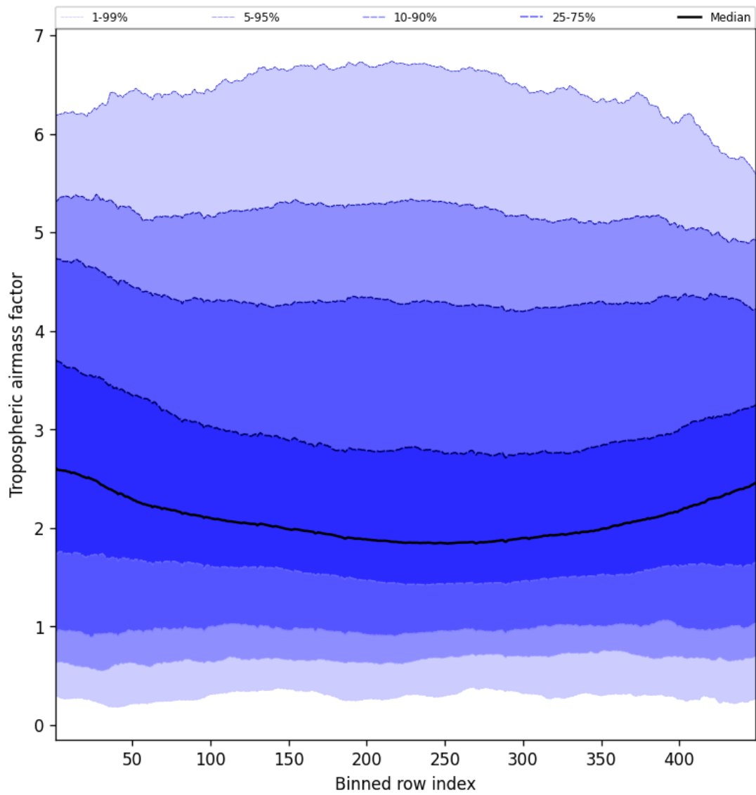
Figure 46: Along track statistics of “Tropospheric airmass factor” for 2024-12-18 to 2024-12-19
