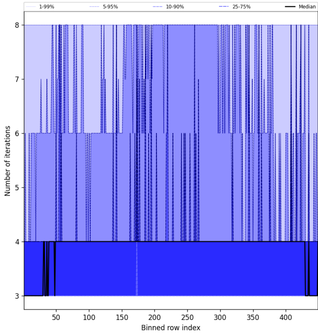
Figure 49: Along track statistics of “Number of iterations” for 2024-12-18 to 2024-12-19
