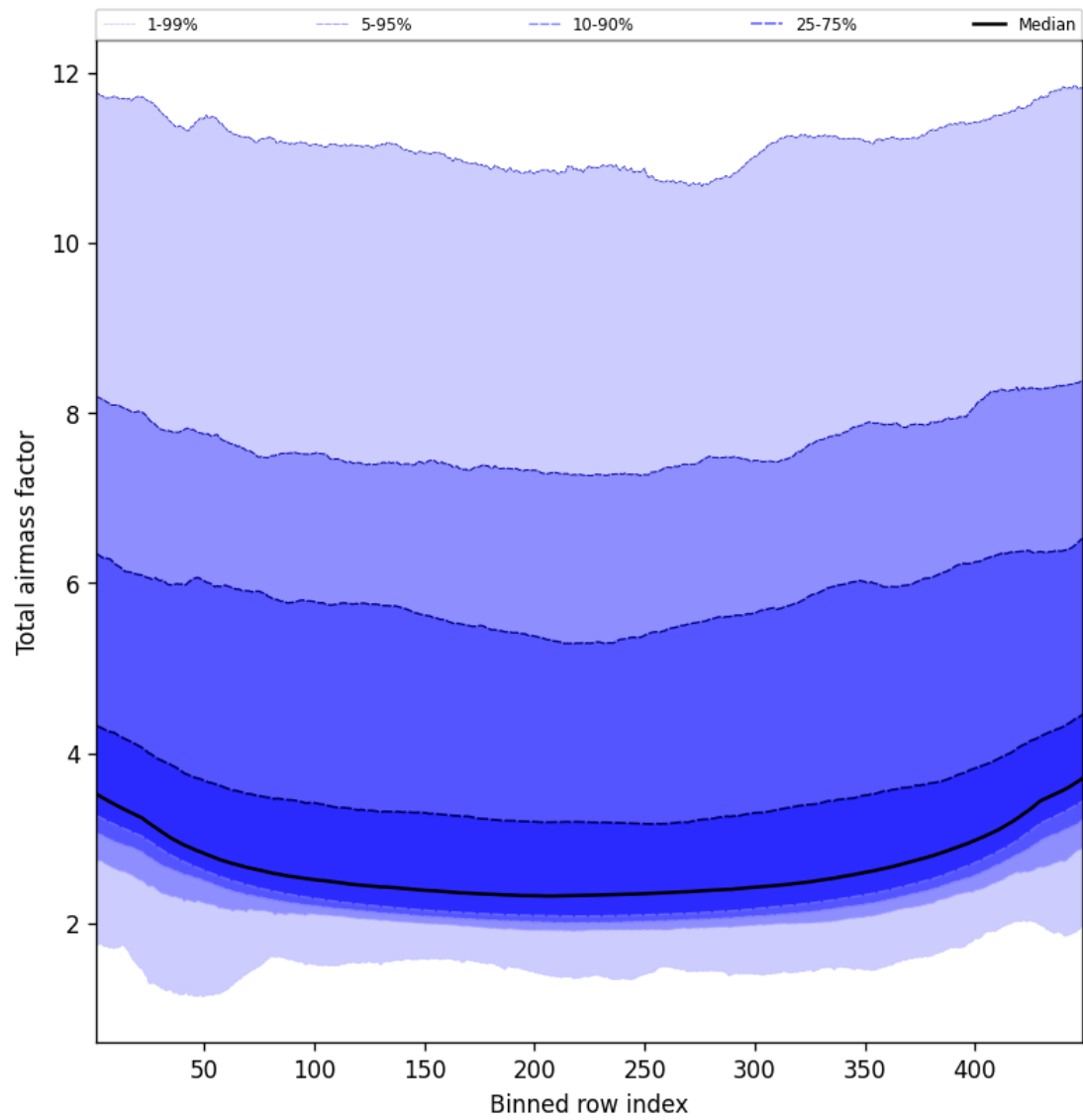
Figure 47: Along track statistics of “Total airmass factor” for 2024-12-18 to 2024-12-19
