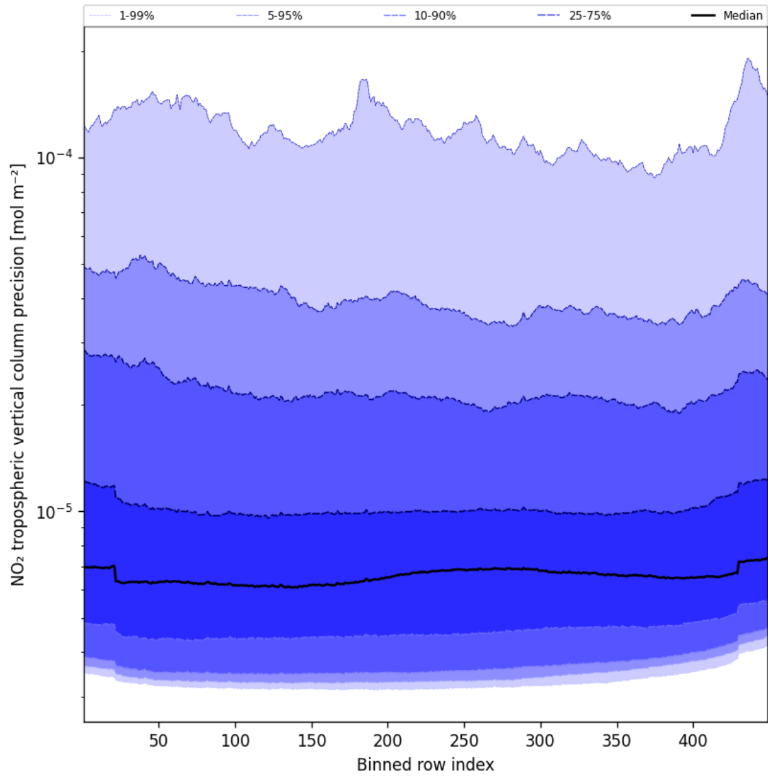
Figure 45: Along track statistics of “NO 2 tropospheric vertical column precision” for 2024-12-18 to 2024-12-19
