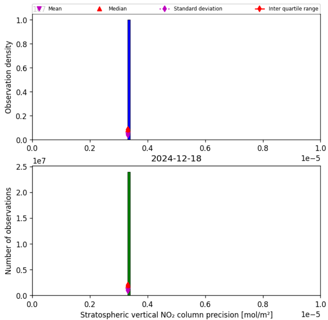
Figure 35: Histogram of “Stratospheric vertical NO 2 column precision” for 2024-12-18 to 2024-12-19
