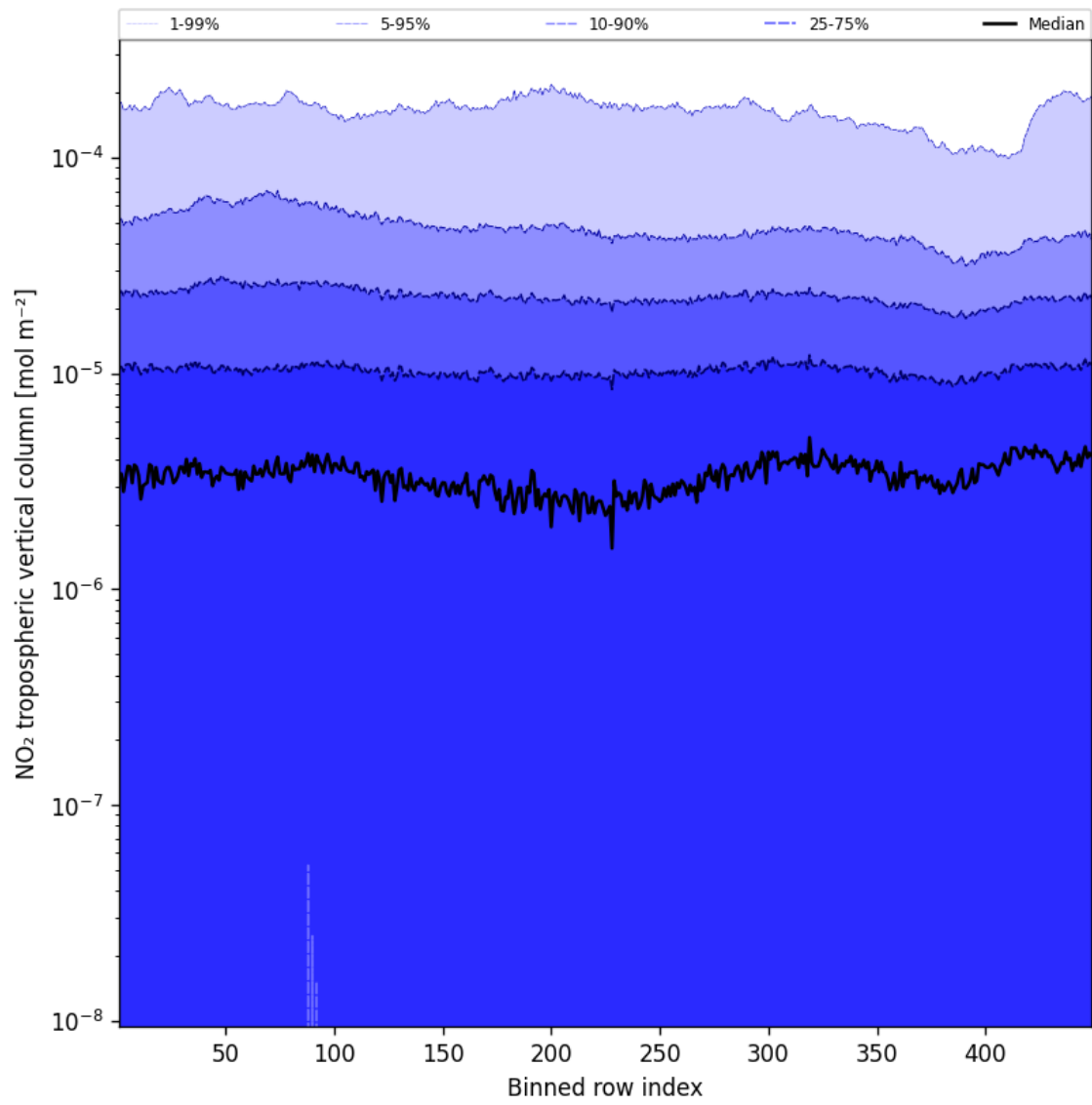
Figure 44: Along track statistics of “NO 2 tropospheric vertical column” for 2024-12-18 to 2024-12-19
