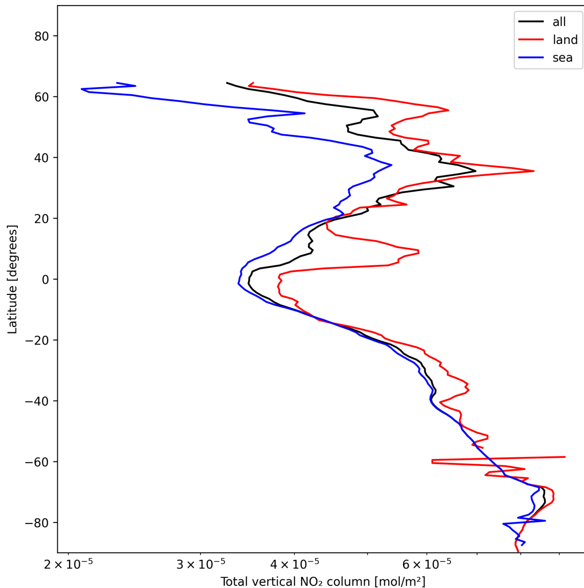
Figure 19: Zonal average of “Total vertical NO 2 column” for 2024-12-18 to 2024-12-19.
