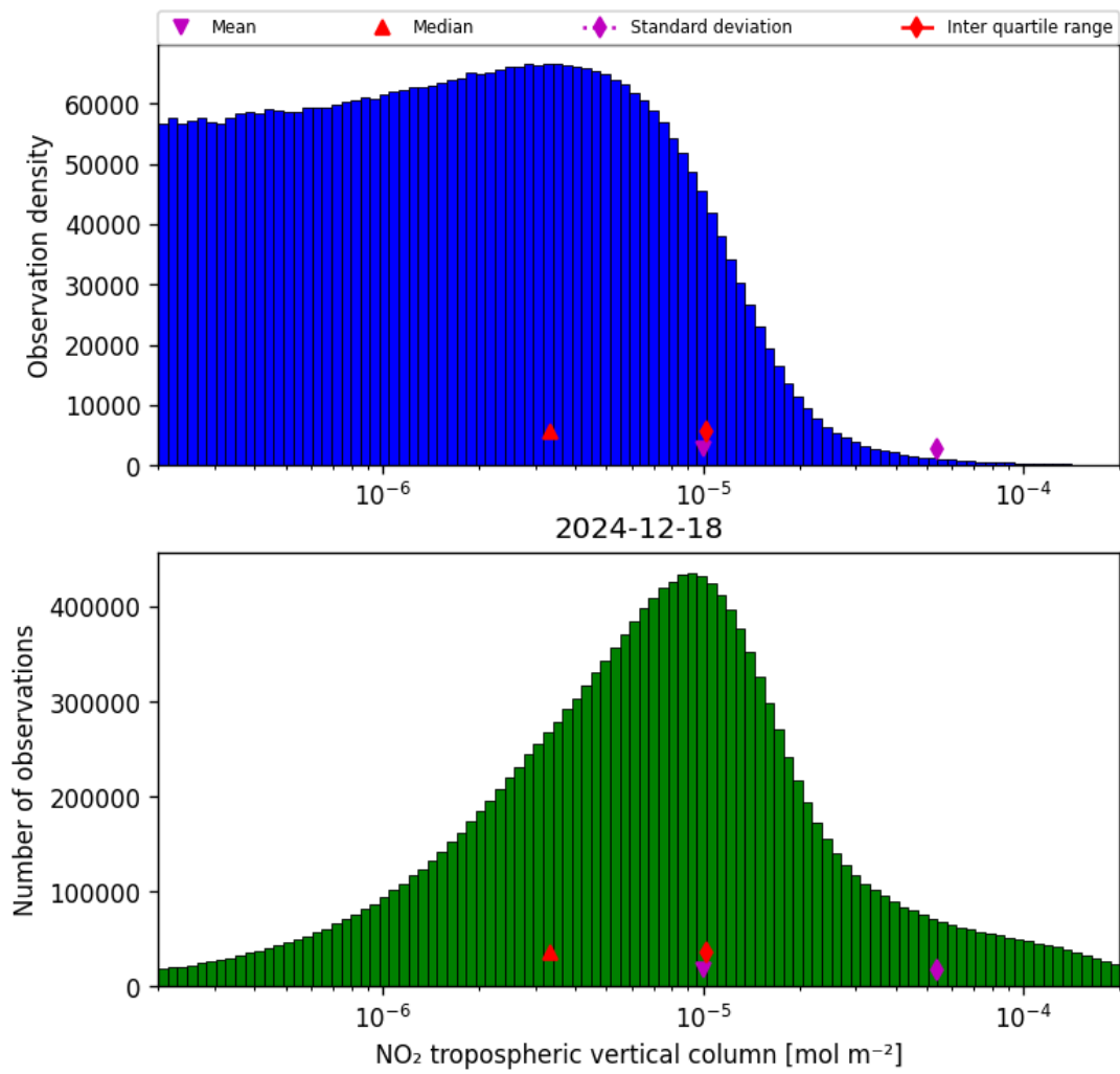
Figure 27: Histogram of “NO 2 tropospheric vertical column” for 2024-12-18 to 2024-12-19
