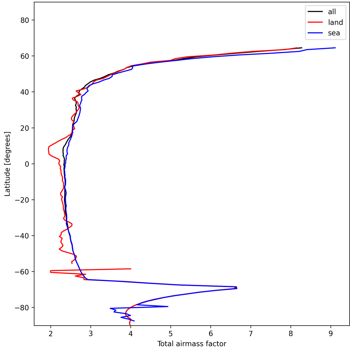
Figure 13: Zonal average of “Total airmass factor” for 2024-12-18 to 2024-12-19.
