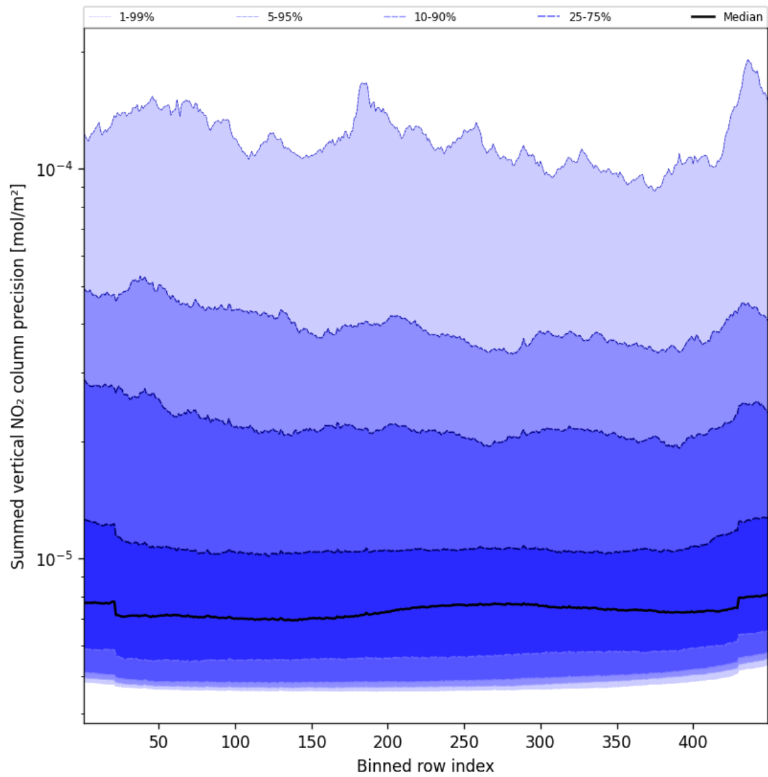
Figure 56: Along track statistics of “Summed vertical NO 2 column precision” for 2024-12-18 to 2024-12-19
