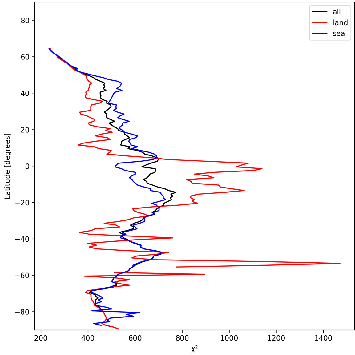
Figure 23: Zonal average of “ \chi^2 ” for 2024-12-18 to 2024-12-19.
