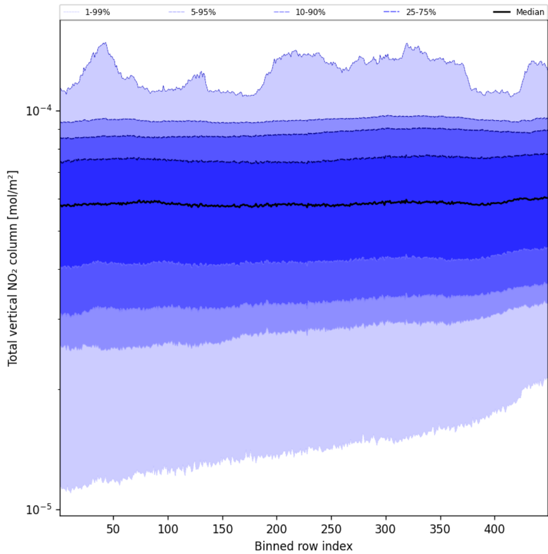
Figure 53: Along track statistics of “Total vertical NO 2 column” for 2024-12-18 to 2024-12-19
