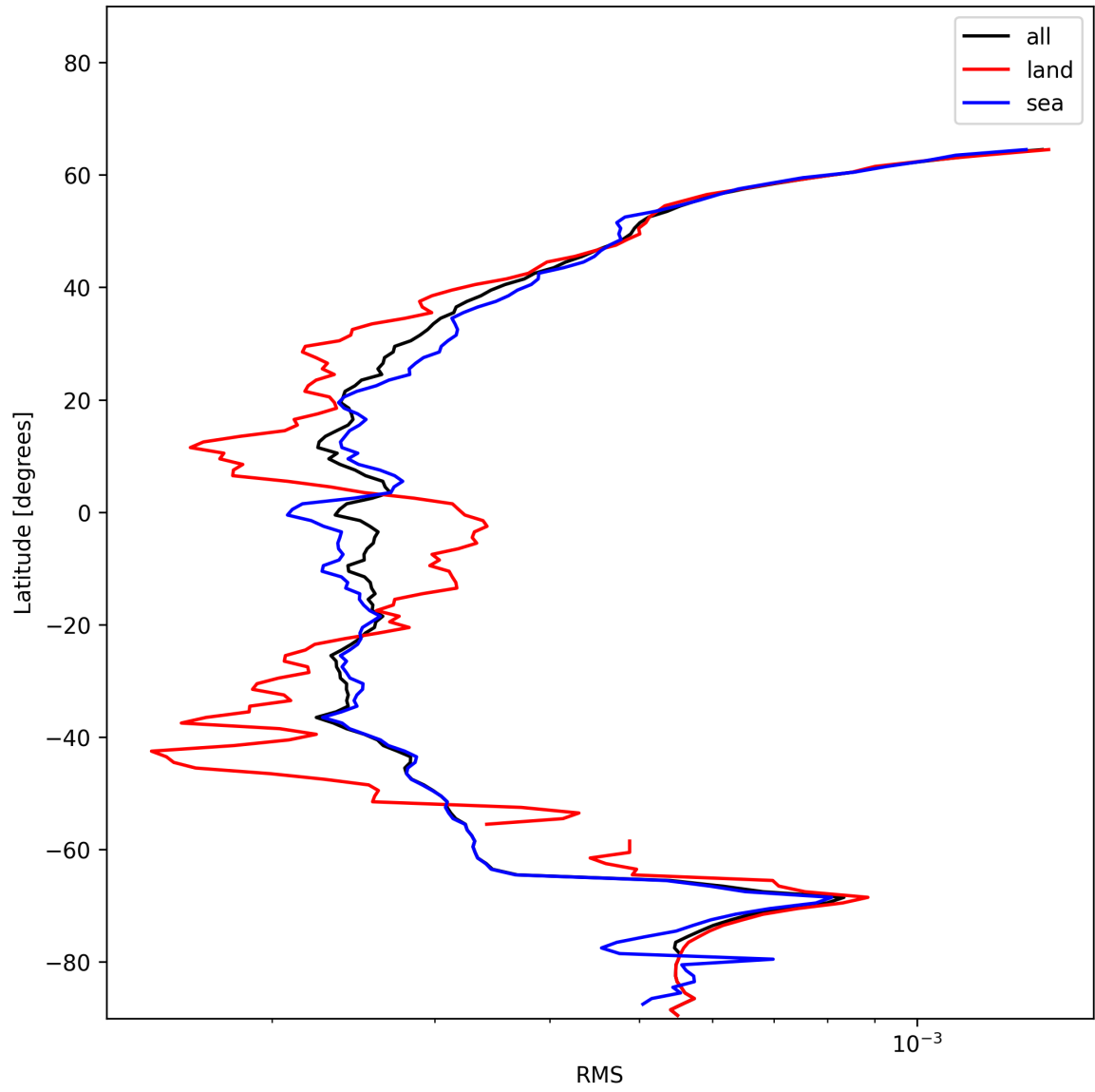
Figure 24: Zonal average of “RMS” for 2024-12-18 to 2024-12-19.
