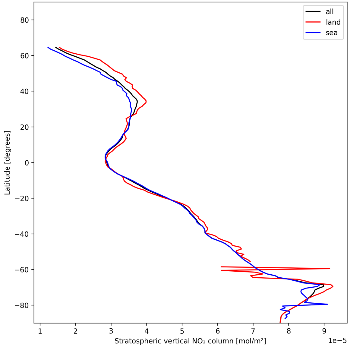
Figure 17: Zonal average of “Stratospheric vertical NO 2 column” for 2024-12-18 to 2024-12-19.
