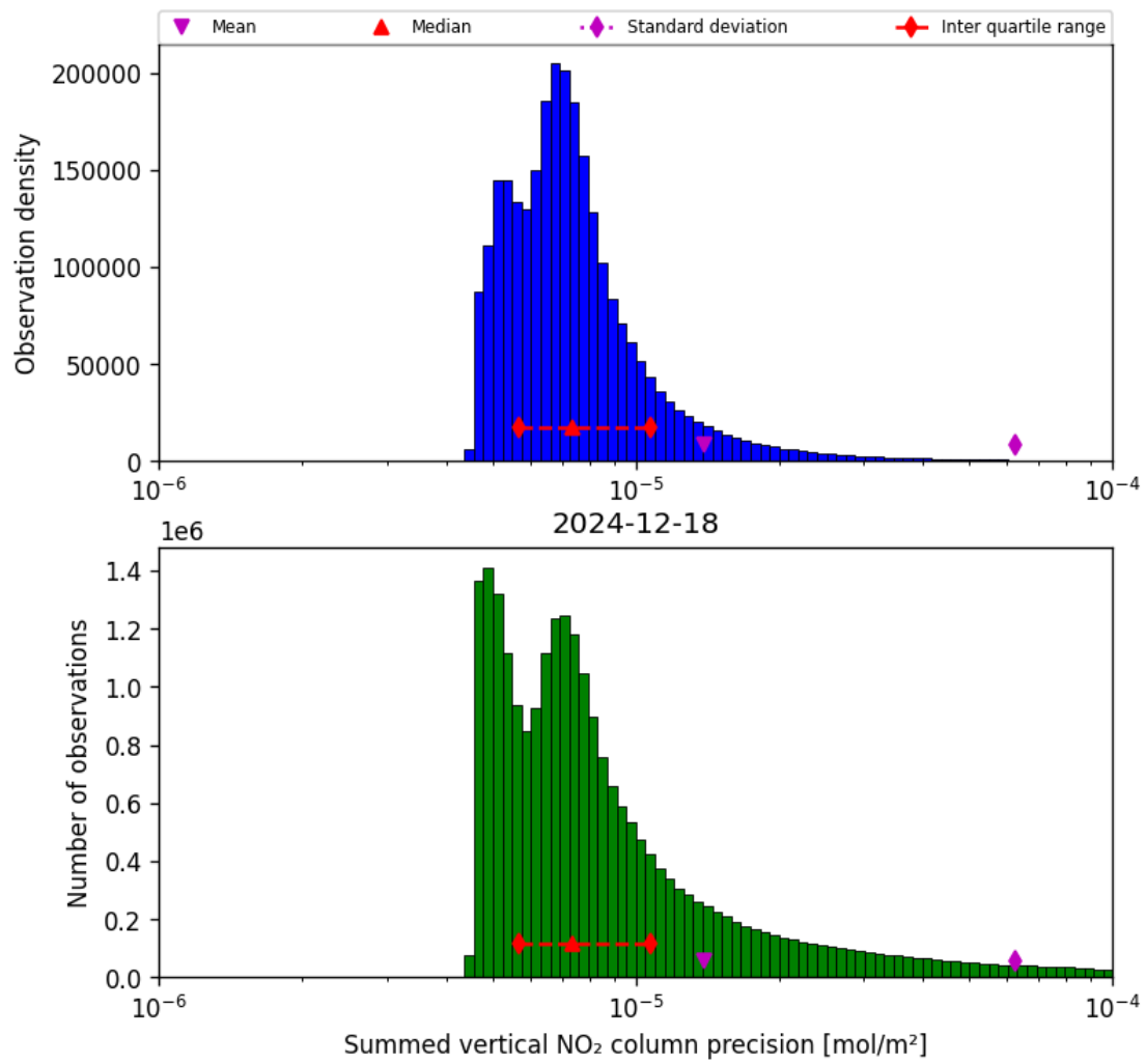
Figure 39: Histogram of “Summed vertical NO 2 column precision” for 2024-12-18 to 2024-12-19
