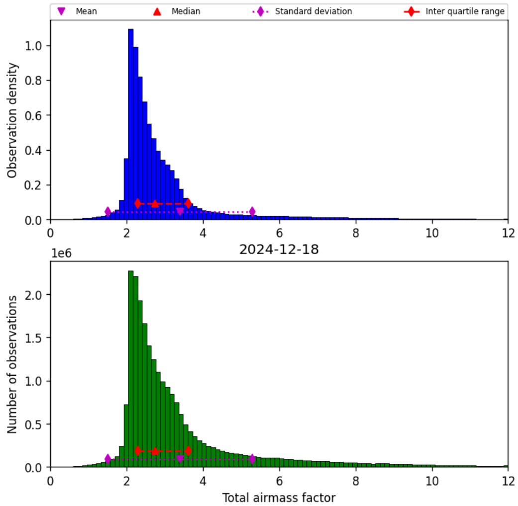
Figure 30: Histogram of “Total airmass factor” for 2024-12-18 to 2024-12-19
