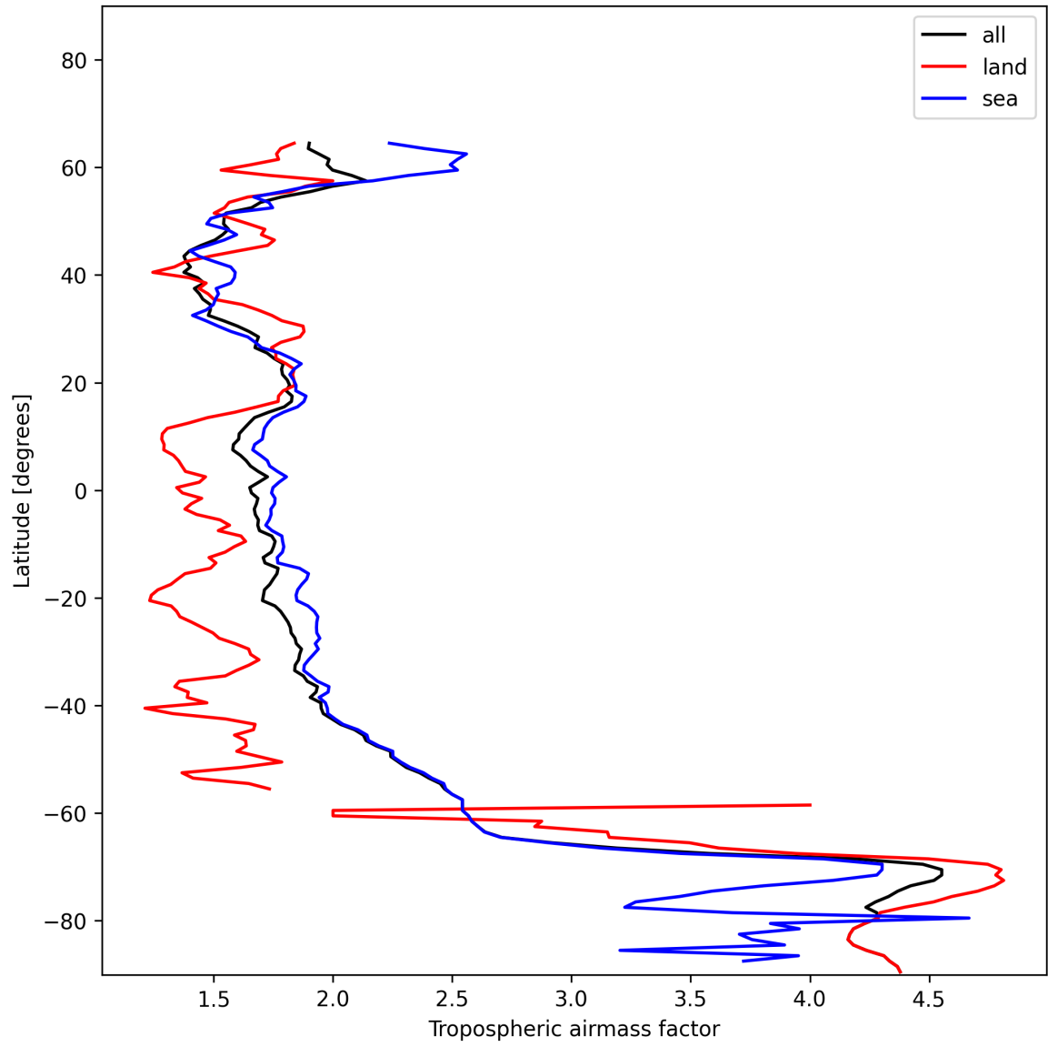
Figure 12: Zonal average of “Tropospheric airmass factor” for 2024-12-18 to 2024-12-19.
