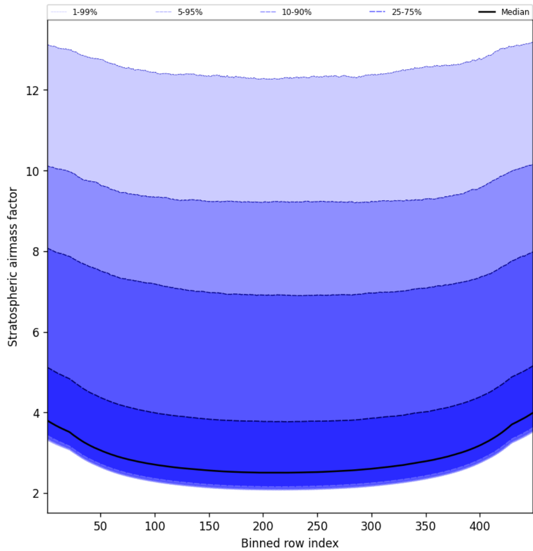
Figure 59: Along track statistics of “Stratospheric airmass factor” for 2024-12-18 to 2024-12-19
