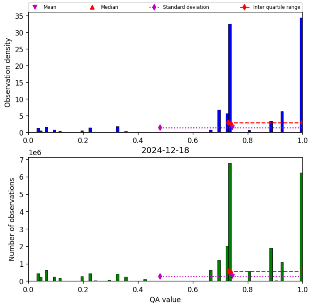
Figure 26: Histogram of “QA value” for 2024-12-18 to 2024-12-19
