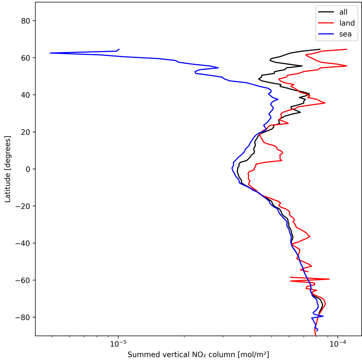
Figure 21: Zonal average of “Summed vertical NO 2 column” for 2024-12-18 to 2024-12-19.
