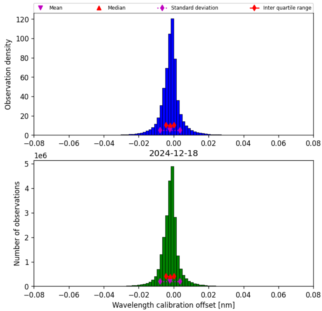
Figure 33: Histogram of “Wavelength calibration offset” for 2024-12-18 to 2024-12-19
