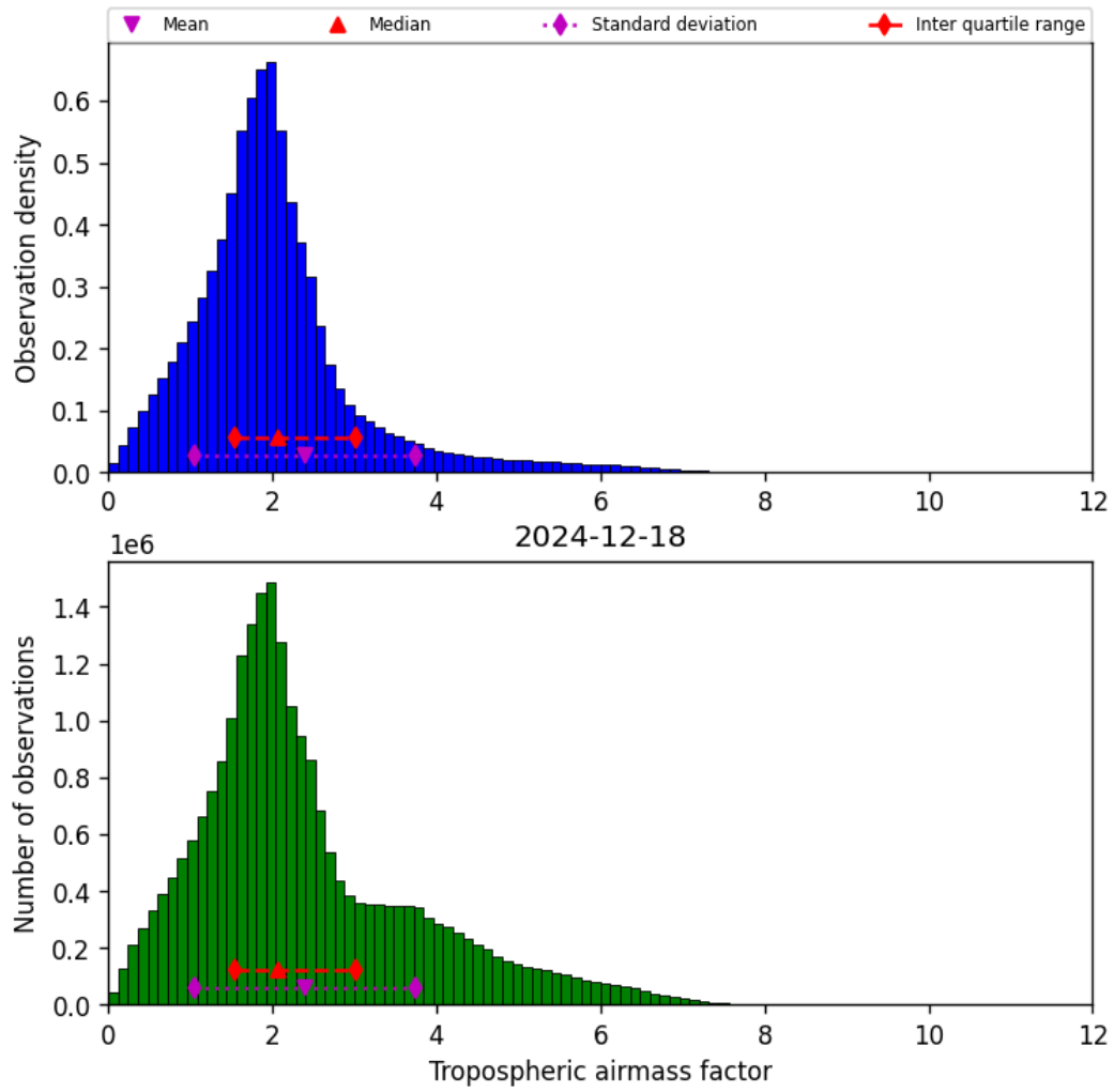
Figure 29: Histogram of “Tropospheric airmass factor” for 2024-12-18 to 2024-12-19
