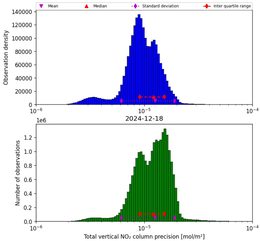
Figure 37: Histogram of “Total vertical NO 2 column precision” for 2024-12-18 to 2024-12-19
