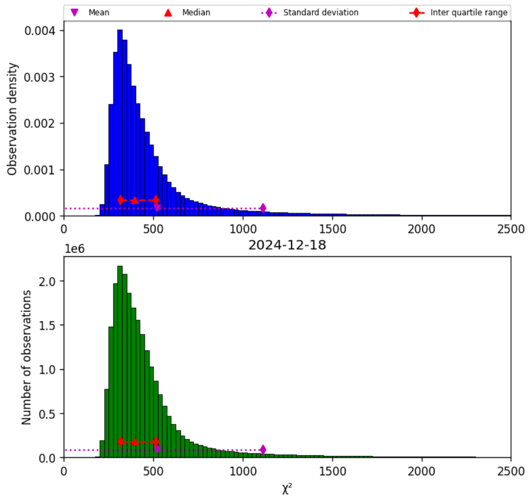
Figure 40: Histogram of “ \chi^2 ” for 2024-12-18 to 2024-12-19
