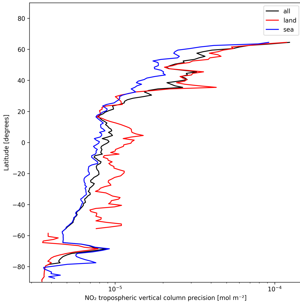
Figure 11: Zonal average of “NO 2 tropospheric vertical column precision” for 2024-12-18 to 2024-12-19.
