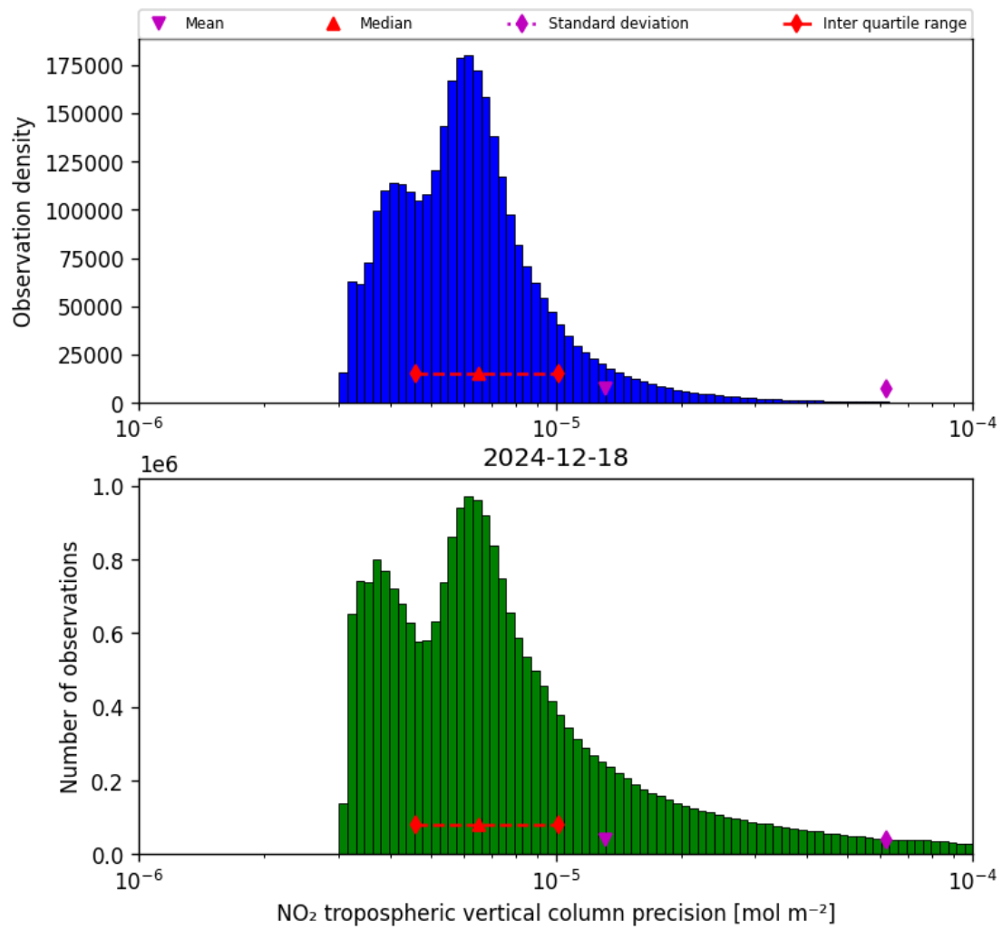
Figure 28: Histogram of “NO 2 tropospheric vertical column precision” for 2024-12-18 to 2024-12-19
