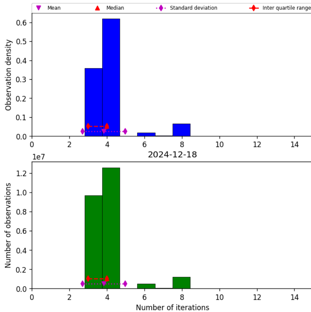
Figure 32: Histogram of “Number of iterations” for 2024-12-18 to 2024-12-19
