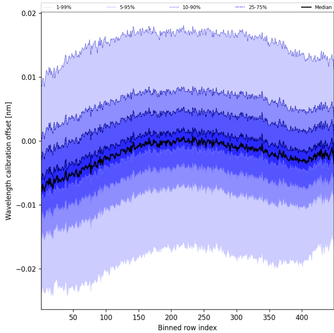
Figure 50: Along track statistics of “Wavelength calibration offset” for 2024-12-18 to 2024-12-19
