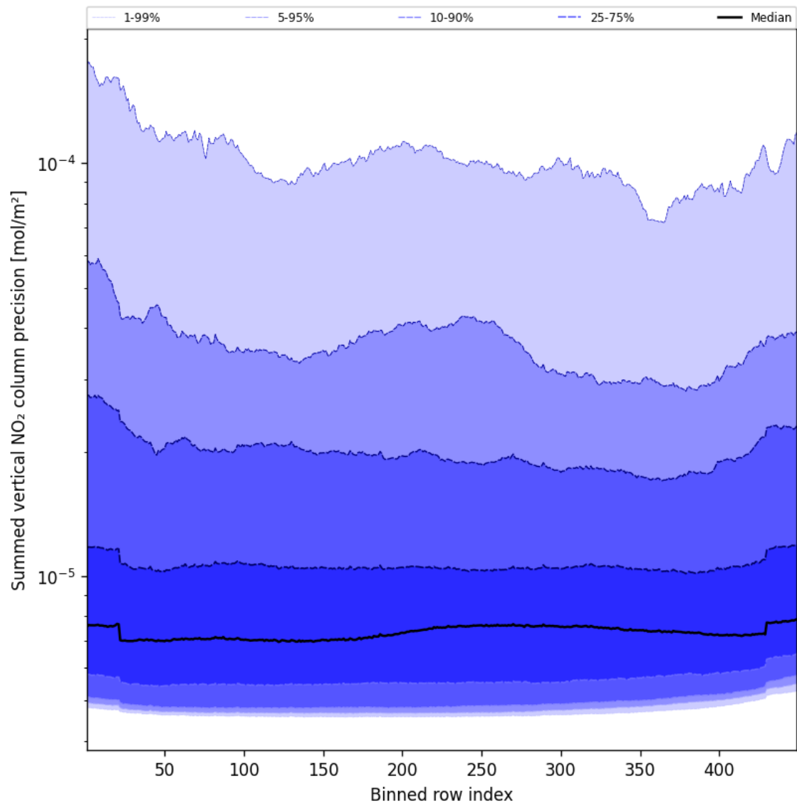
Figure 56: Along track statistics of “Summed vertical NO 2 column precision” for 2024-12-19 to 2024-12-19
