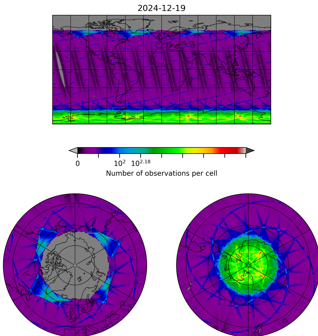
Figure 8: Map of the number of observations for 2024-12-19 to 2024-12-19
