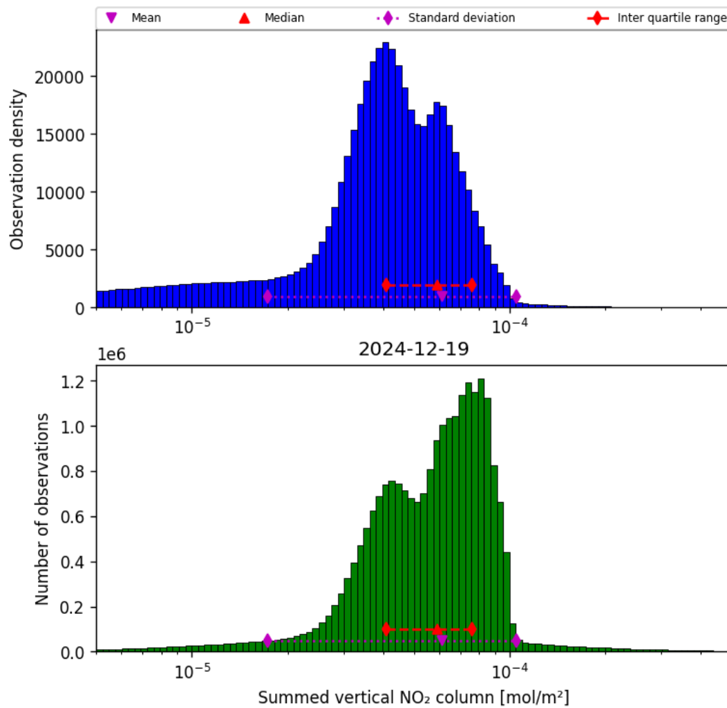
Figure 38: Histogram of “Summed vertical NO 2 column” for 2024-12-19 to 2024-12-19
