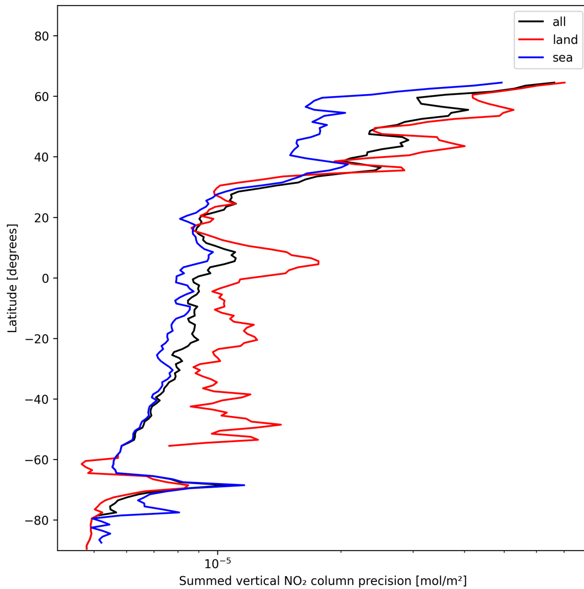
Figure 22: Zonal average of “Summed vertical NO 2 column precision” for 2024-12-19 to 2024-12-19.
