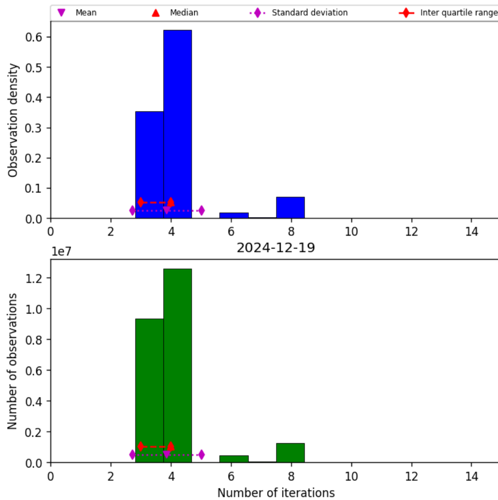
Figure 32: Histogram of “Number of iterations” for 2024-12-19 to 2024-12-19
