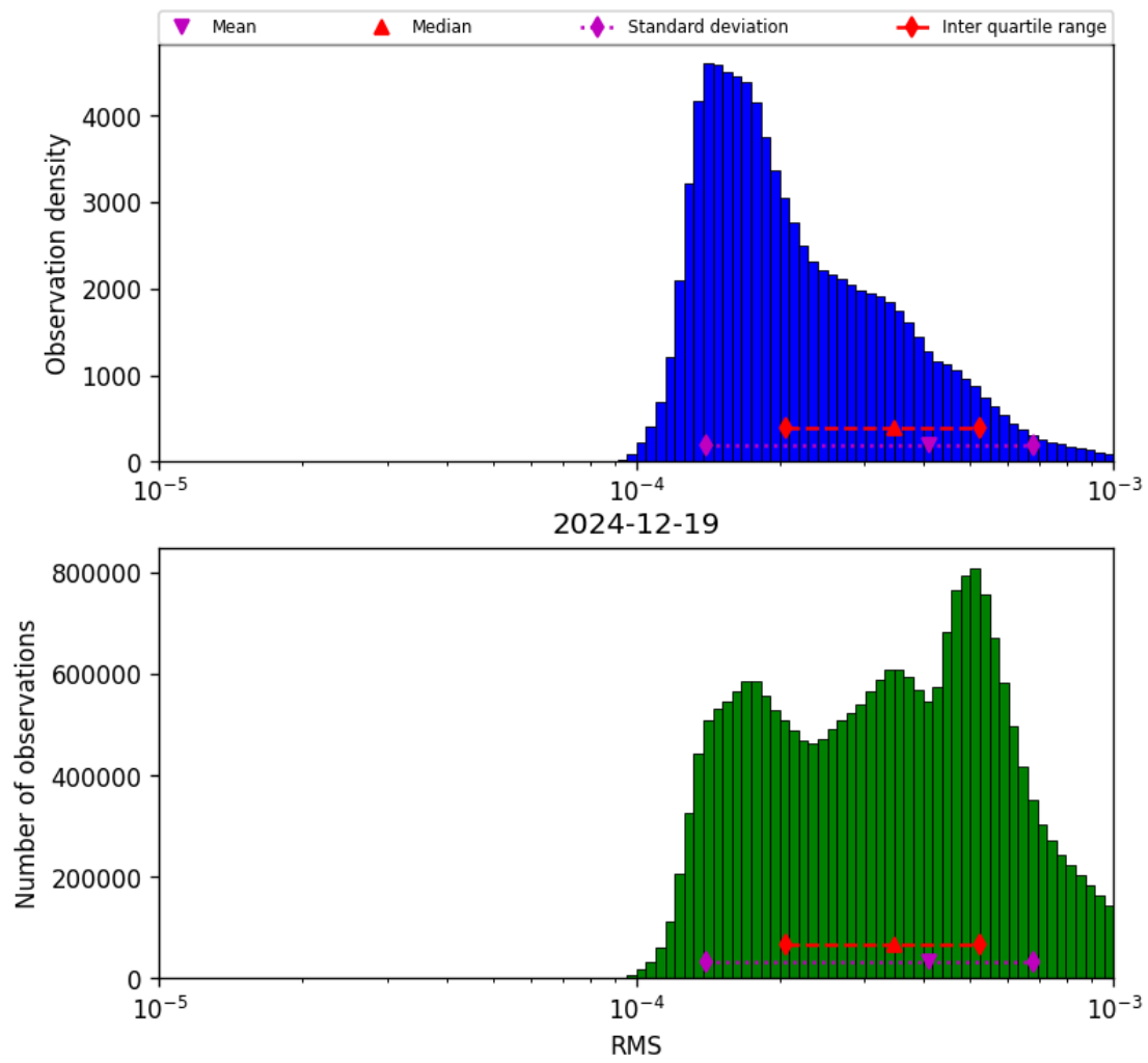
Figure 41: Histogram of “RMS” for 2024-12-19 to 2024-12-19
