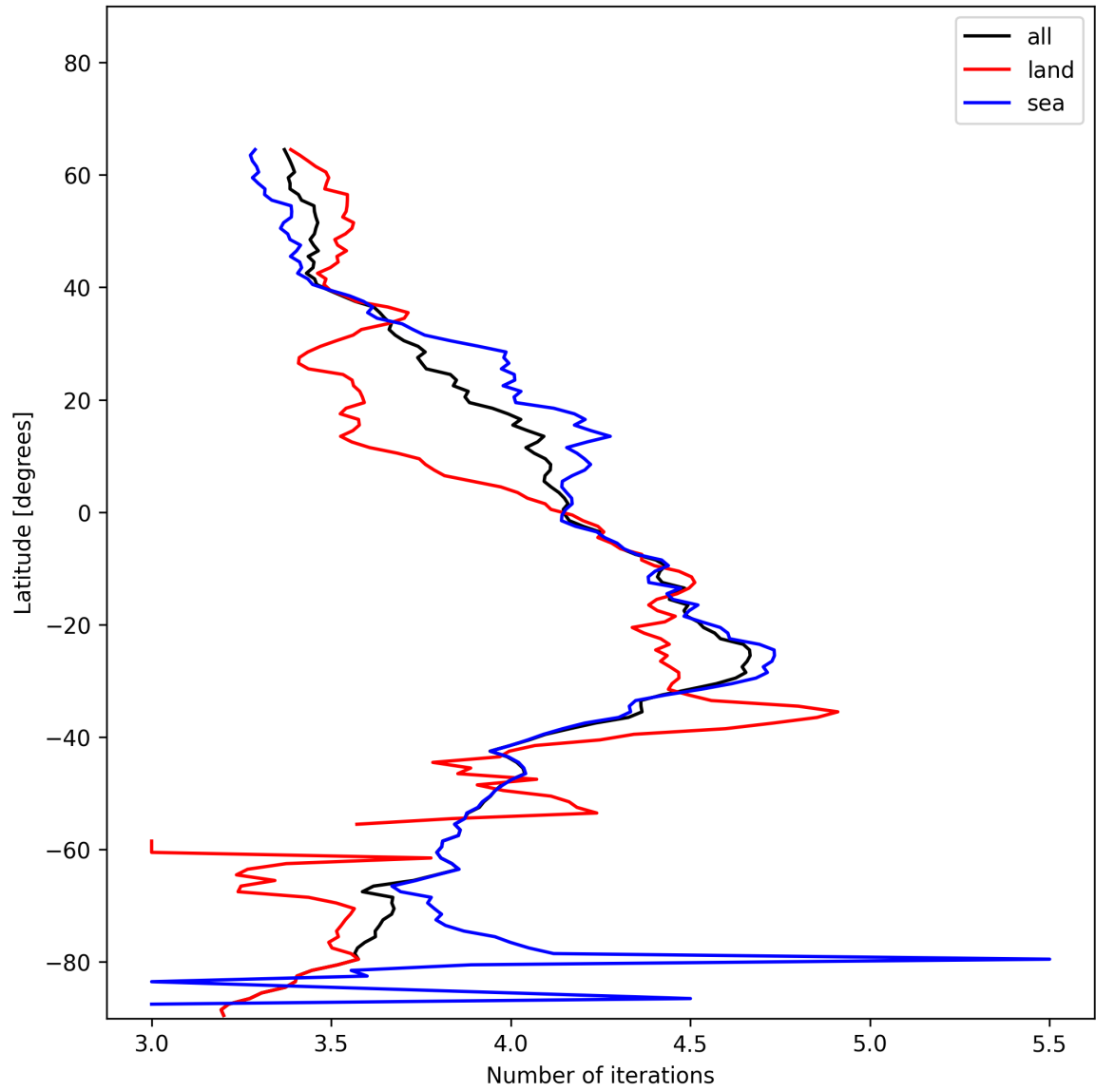
Figure 15: Zonal average of “Number of iterations” for 2024-12-19 to 2024-12-19.
