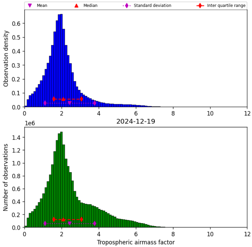
Figure 29: Histogram of “Tropospheric airmass factor” for 2024-12-19 to 2024-12-19
