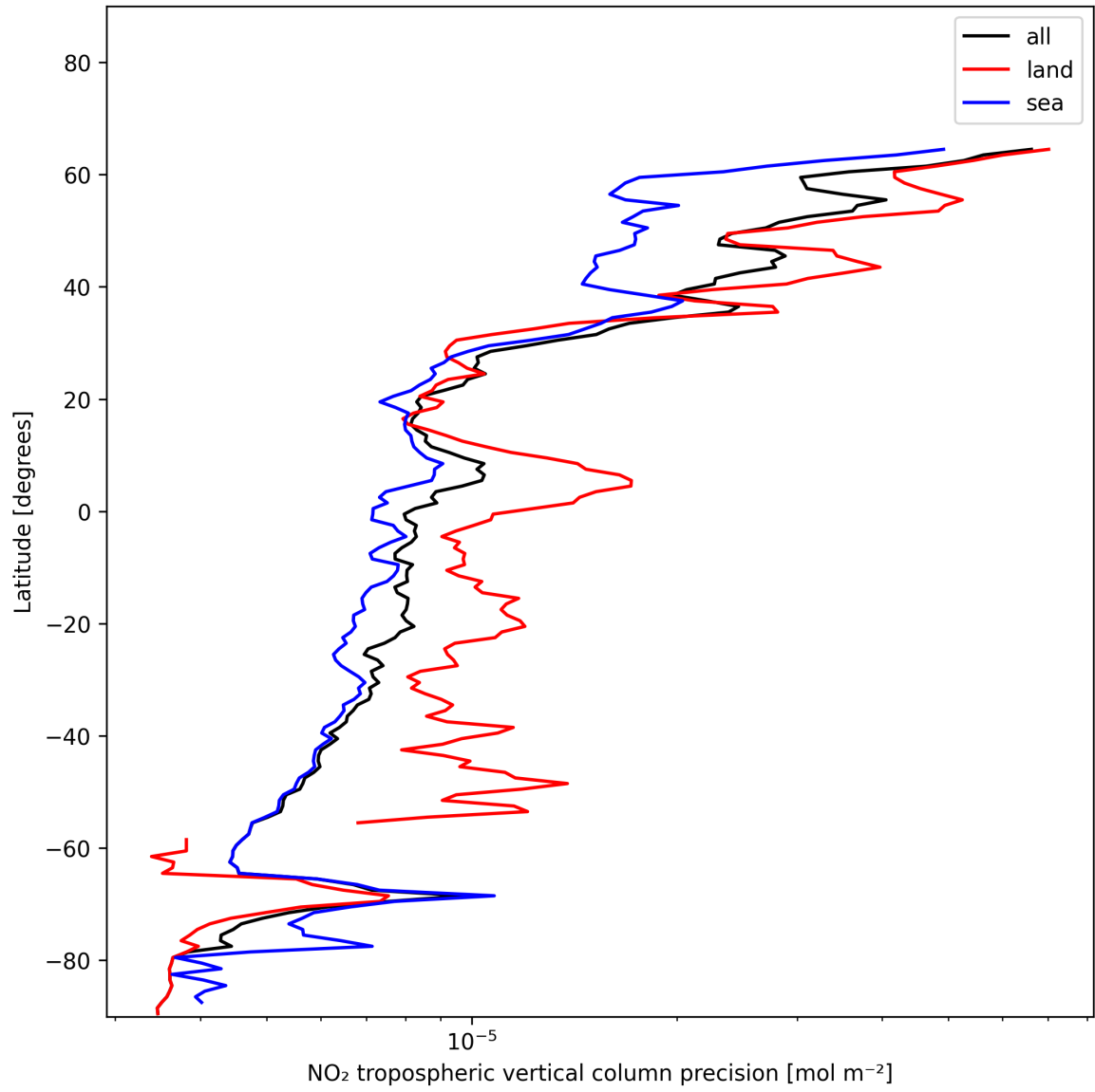
Figure 11: Zonal average of “NO 2 tropospheric vertical column precision” for 2024-12-19 to 2024-12-19.
