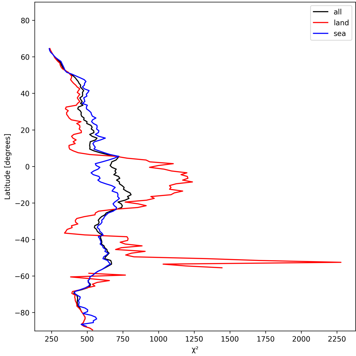
Figure 23: Zonal average of “ \chi^2 ” for 2024-12-19 to 2024-12-19.
