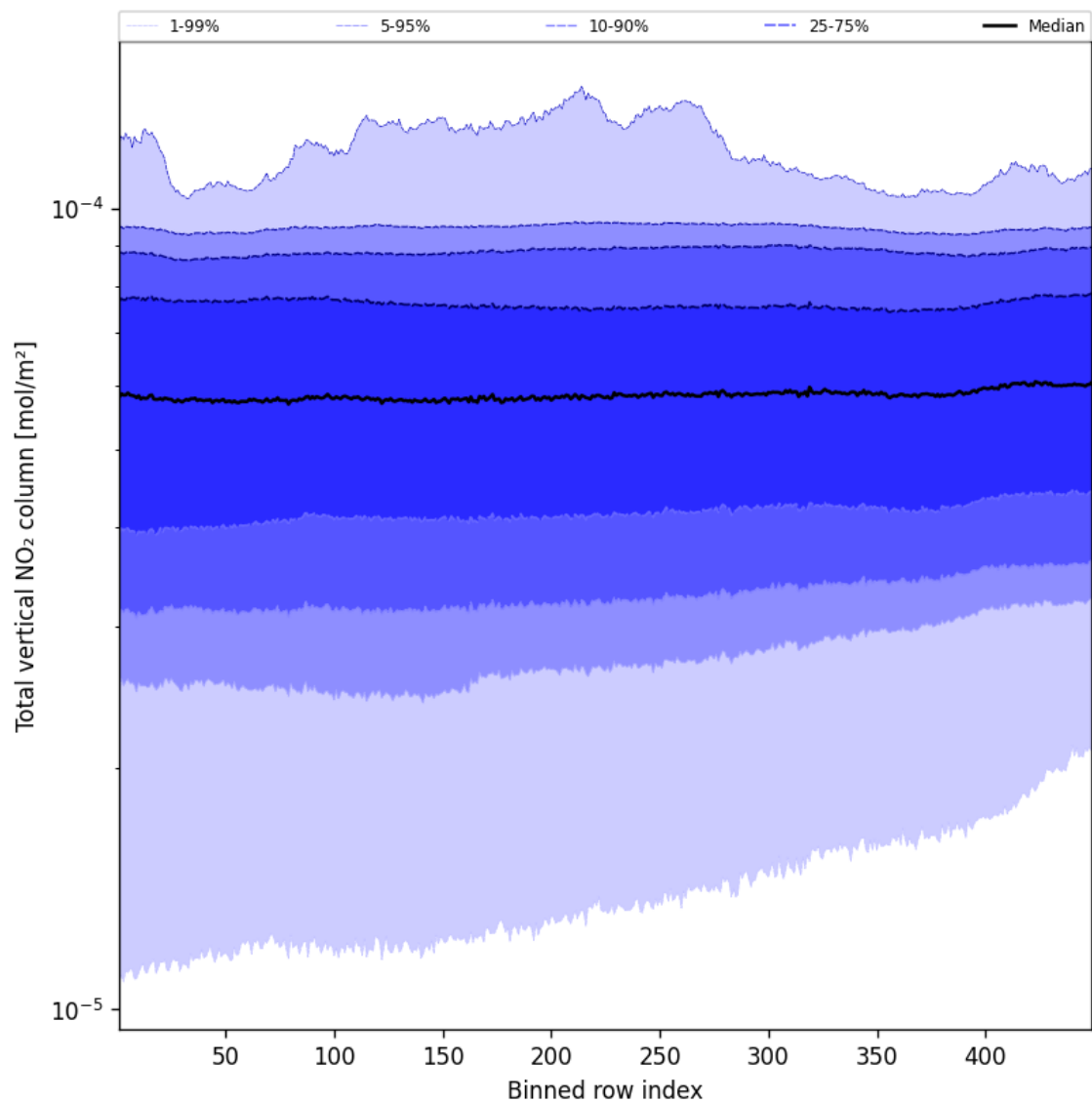
Figure 53: Along track statistics of “Total vertical NO 2 column” for 2024-12-19 to 2024-12-19
