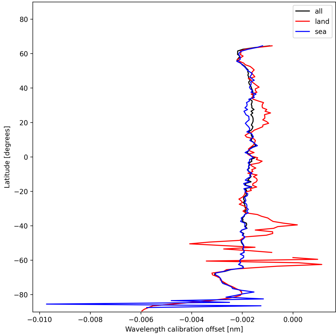
Figure 16: Zonal average of “Wavelength calibration offset” for 2024-12-19 to 2024-12-19.
