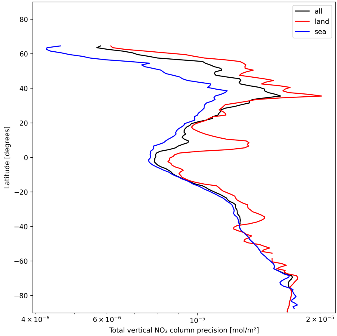
Figure 20: Zonal average of “Total vertical NO 2 column precision” for 2024-12-19 to 2024-12-19.
