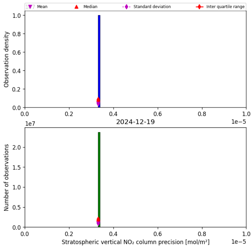
Figure 35: Histogram of “Stratospheric vertical NO 2 column precision” for 2024-12-19 to 2024-12-19
