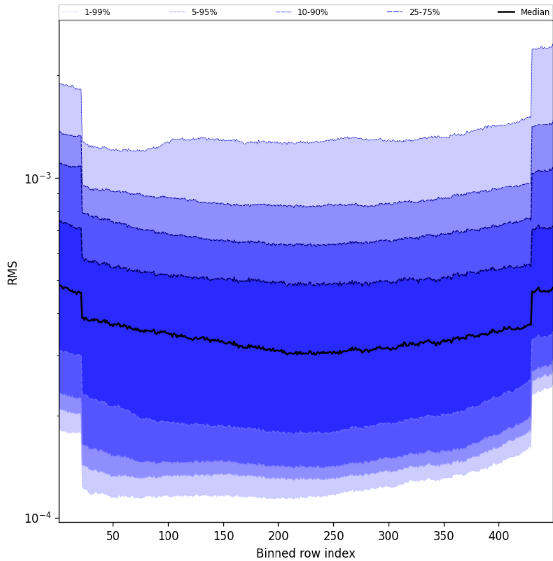
Figure 58: Along track statistics of “RMS” for 2024-12-19 to 2024-12-19
