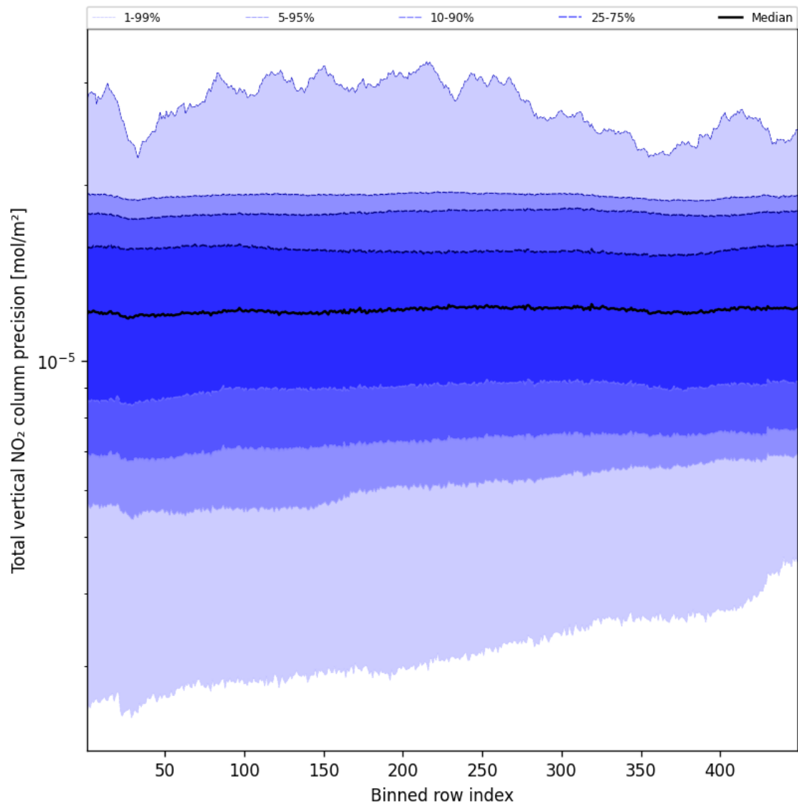
Figure 54: Along track statistics of “Total vertical NO 2 column precision” for 2024-12-19 to 2024-12-19
