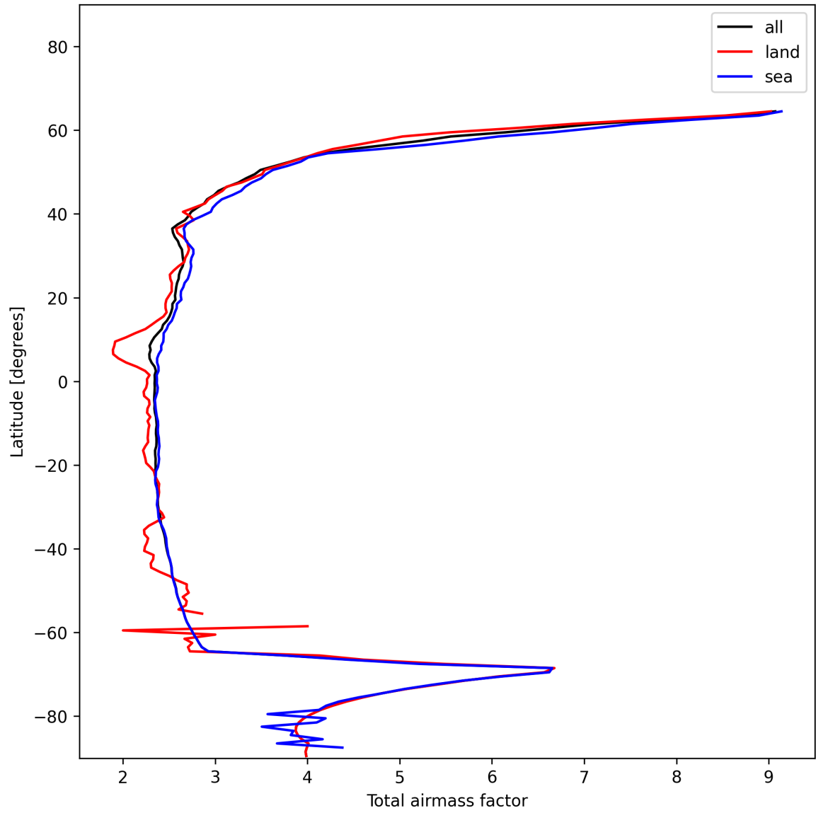
Figure 13: Zonal average of “Total airmass factor” for 2024-12-19 to 2024-12-19.
