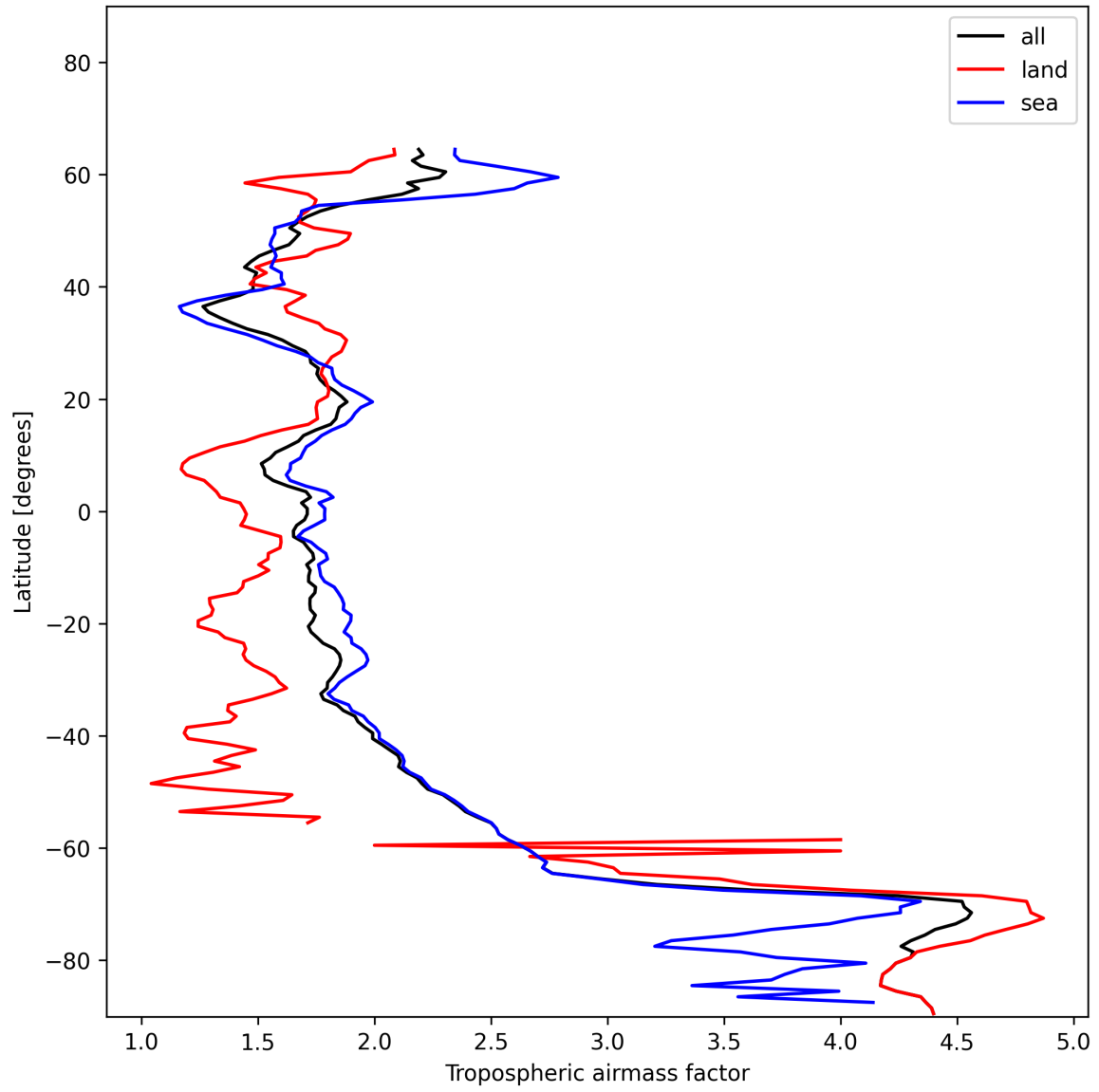
Figure 12: Zonal average of “Tropospheric airmass factor” for 2024-12-19 to 2024-12-19.
