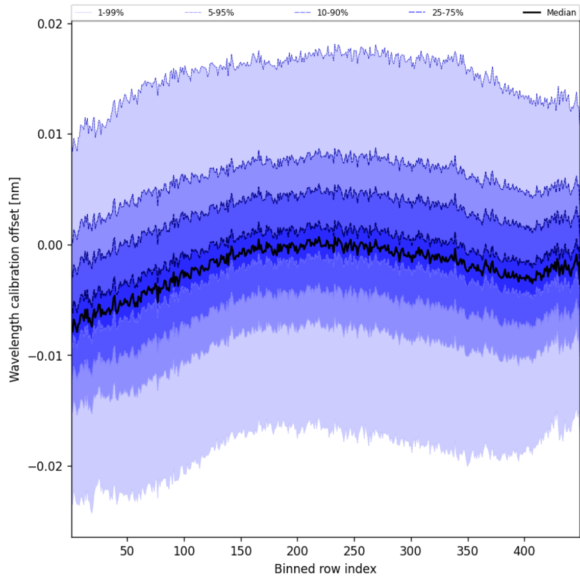
Figure 50: Along track statistics of “Wavelength calibration offset” for 2024-12-19 to 2024-12-19
