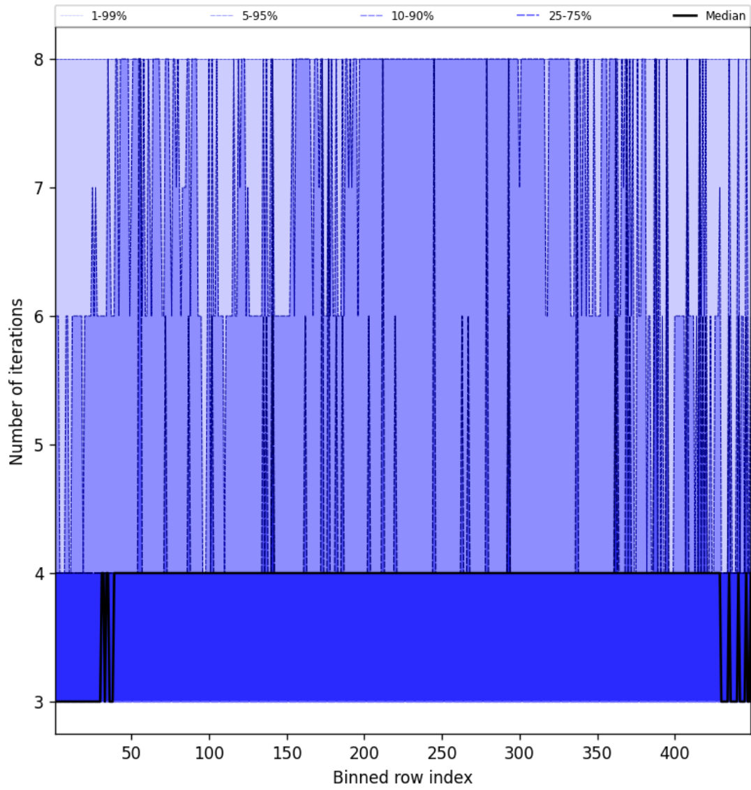
Figure 49: Along track statistics of “Number of iterations” for 2024-12-19 to 2024-12-19
