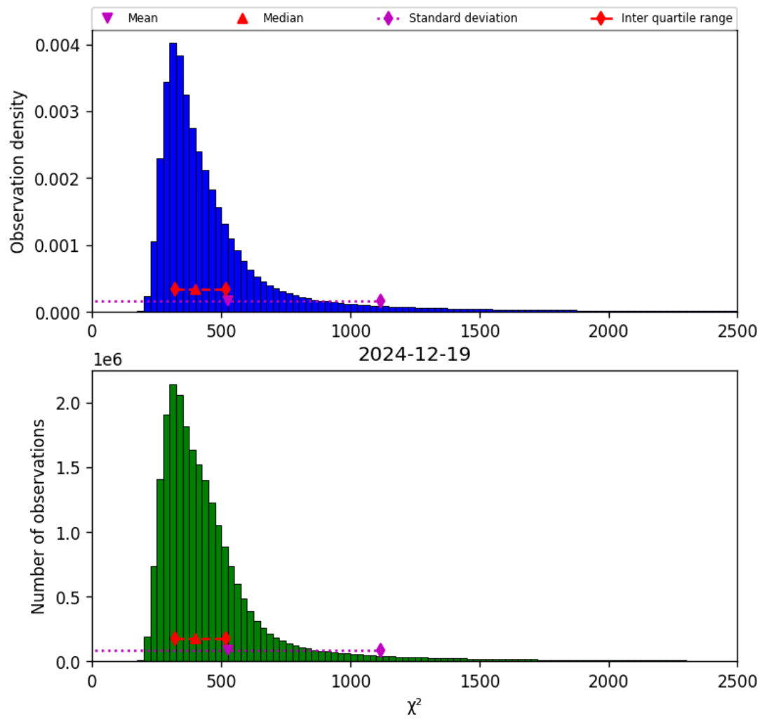
Figure 40: Histogram of “ \chi^2 ” for 2024-12-19 to 2024-12-19
