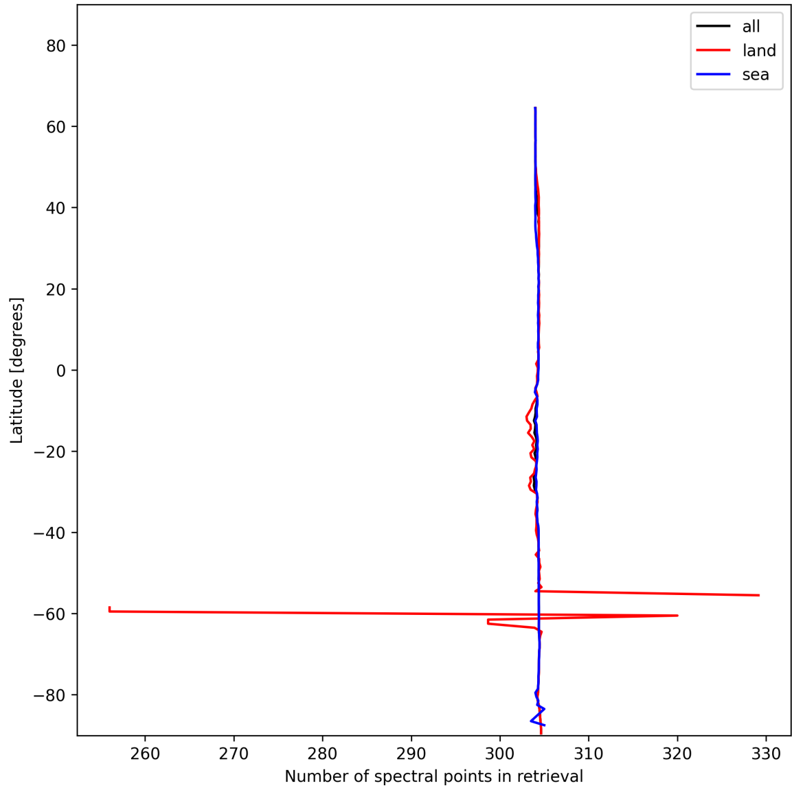
Figure 14: Zonal average of “Number of spectral points in retrieval” for 2024-12-19 to 2024-12-19.
