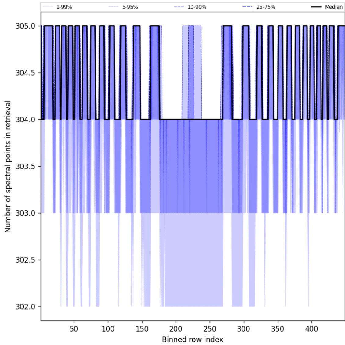
Figure 48: Along track statistics of “Number of spectral points in retrieval” for 2024-12-19 to 2024-12-19
