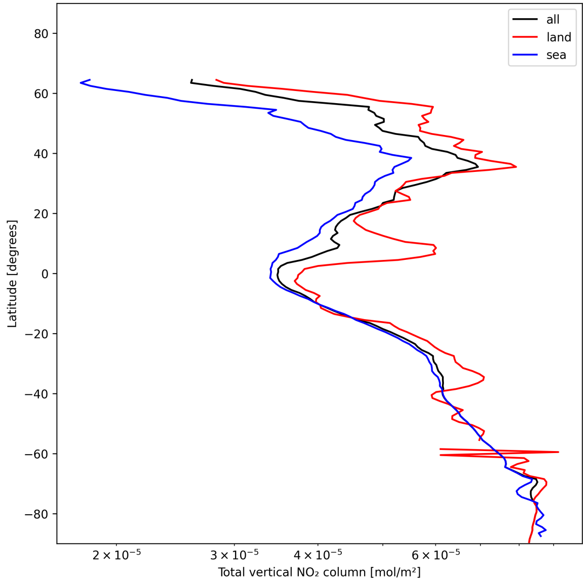
Figure 19: Zonal average of “Total vertical NO 2 column” for 2024-12-19 to 2024-12-19.
