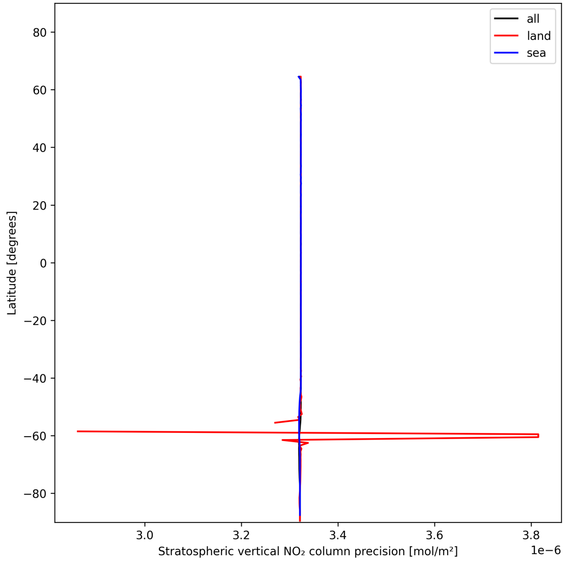
Figure 18: Zonal average of “Stratospheric vertical NO 2 column precision” for 2024-12-19 to 2024-12-19.
