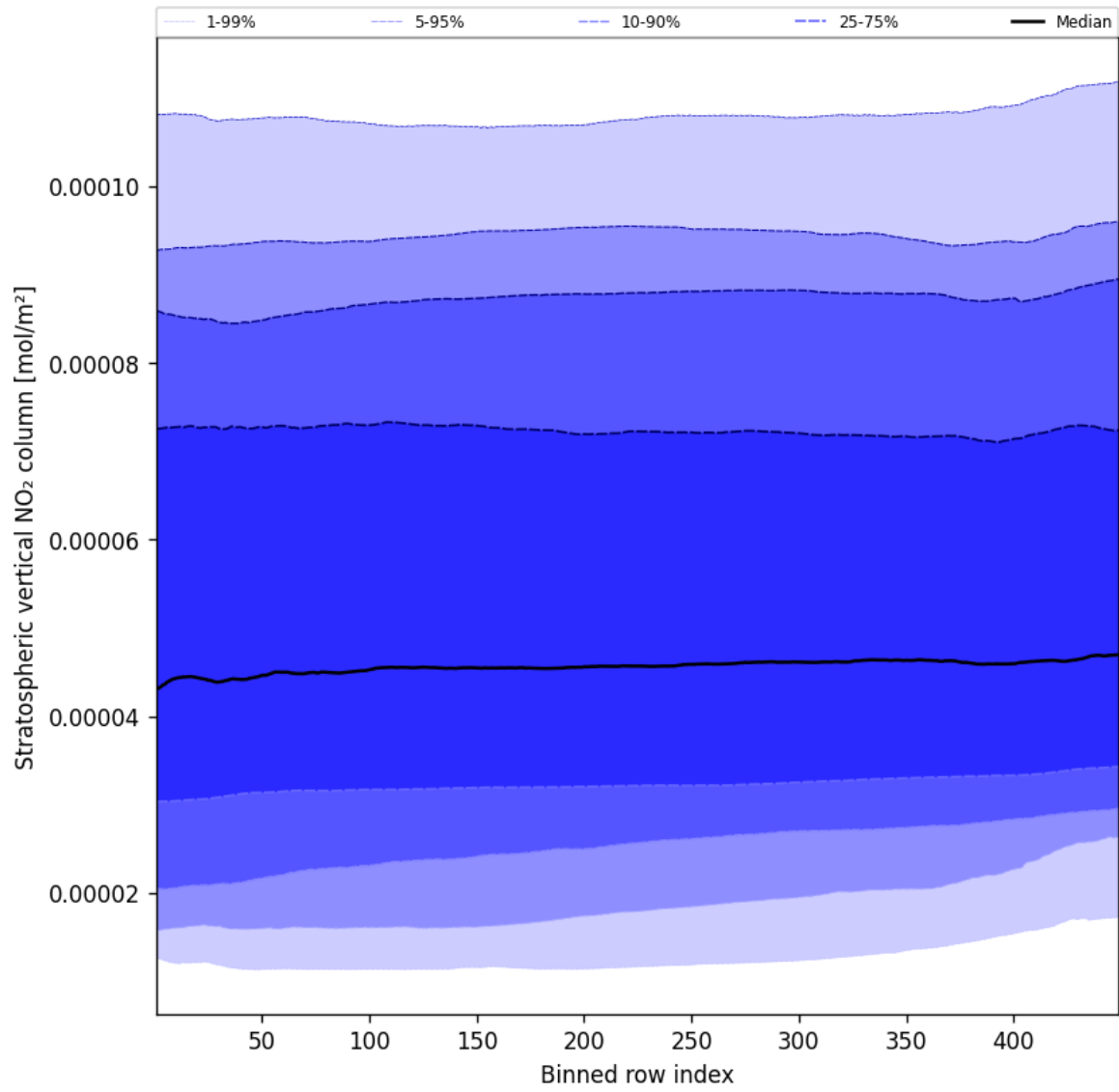
Figure 51: Along track statistics of “Stratospheric vertical NO 2 column” for 2024-12-19 to 2024-12-19
