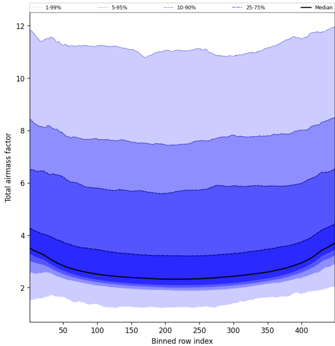
Figure 47: Along track statistics of “Total airmass factor” for 2024-12-19 to 2024-12-19
