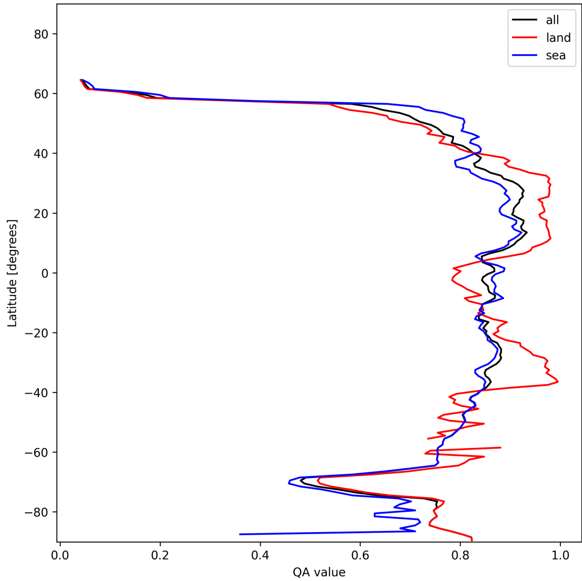
Figure 9: Zonal average of “QA value” for 2024-12-19 to 2024-12-19.
