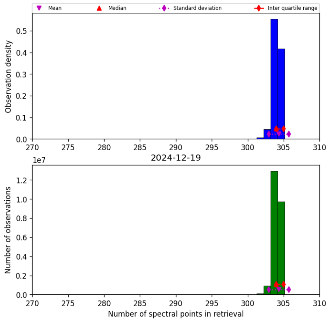
Figure 31: Histogram of “Number of spectral points in retrieval” for 2024-12-19 to 2024-12-19
