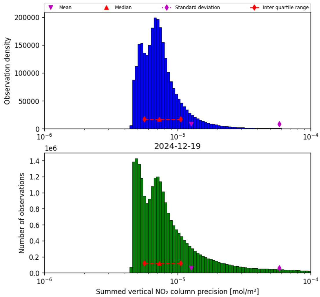
Figure 39: Histogram of “Summed vertical NO 2 column precision” for 2024-12-19 to 2024-12-19
