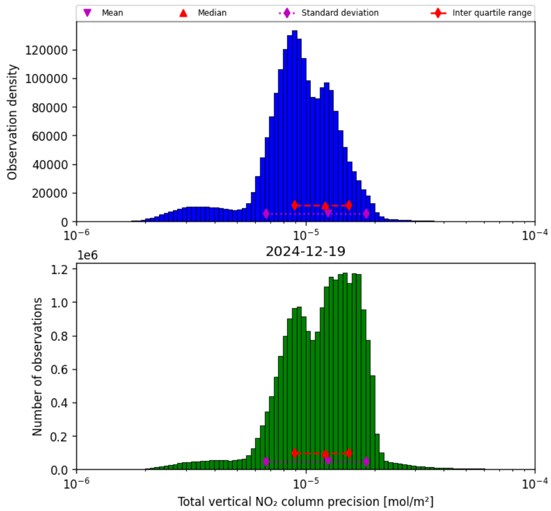
Figure 37: Histogram of "Total vertical NO 2 column precision" for 2024-12-19 to 2024-12-19
