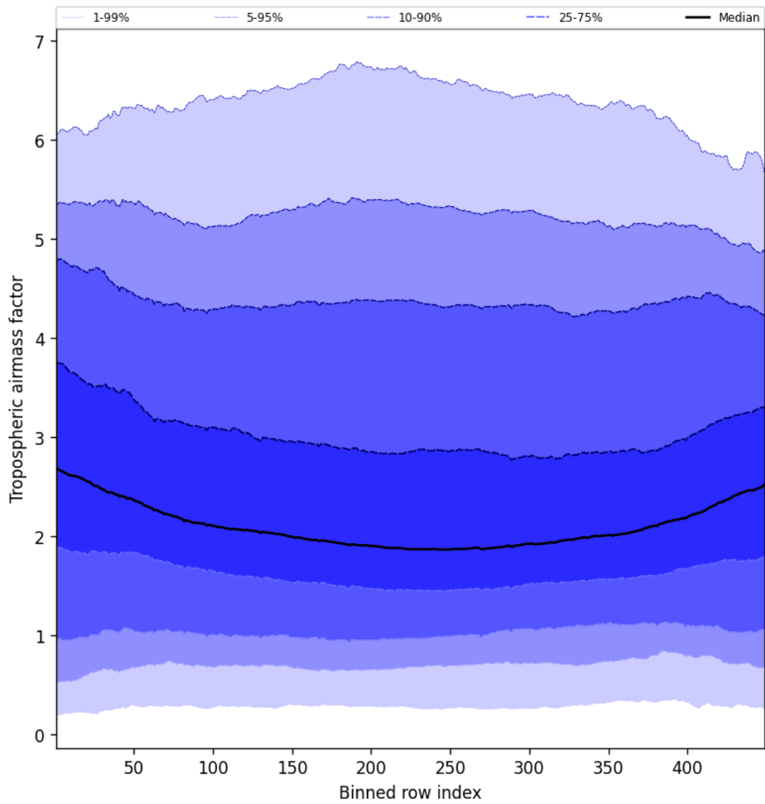
Figure 46: Along track statistics of “Tropospheric air mass factor” for 2024-12-19 to 2024-12-19
