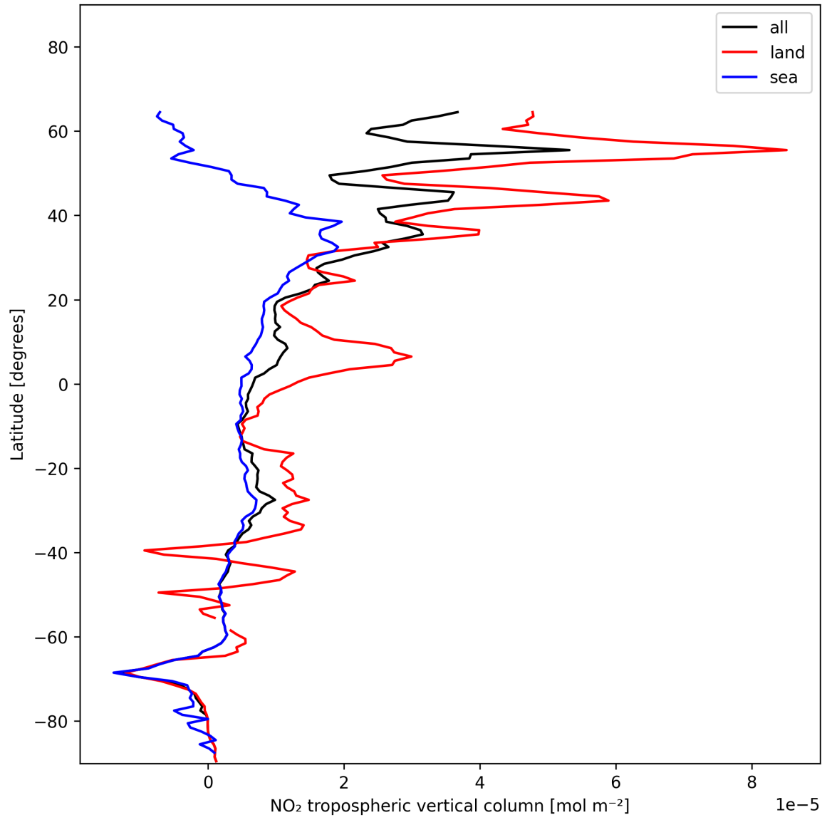
Figure 10: Zonal average of “NO 2 tropospheric vertical column” for 2024-12-19 to 2024-12-19.
