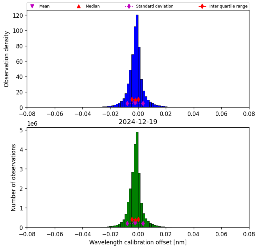
Figure 33: Histogram of “Wavelength calibration offset” for 2024-12-19 to 2024-12-19
