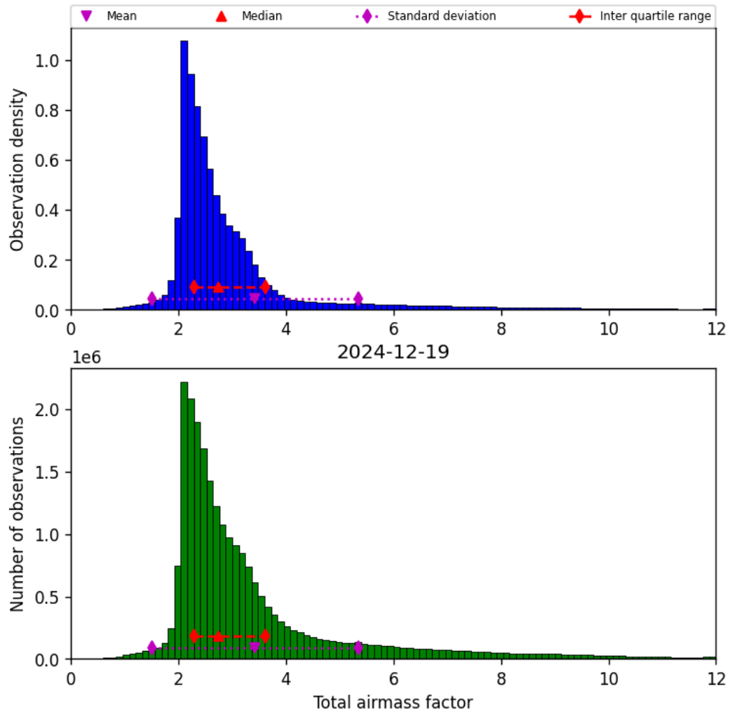
Figure 30: Histogram of “Total airmass factor” for 2024-12-19 to 2024-12-19
