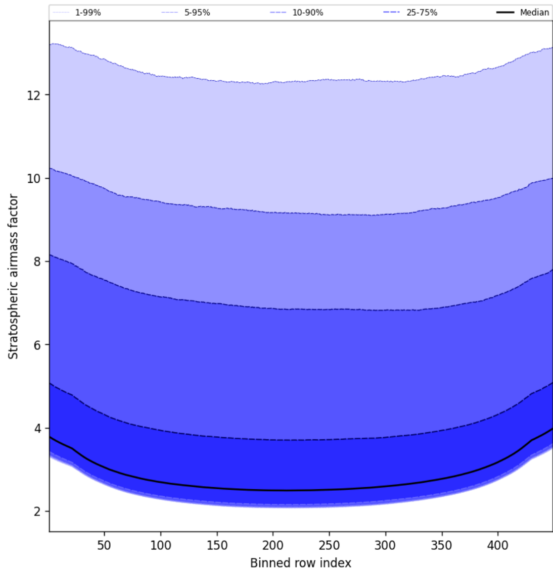
Figure 59: Along track statistics of “Stratospheric airmass factor” for 2024-12-19 to 2024-12-19
