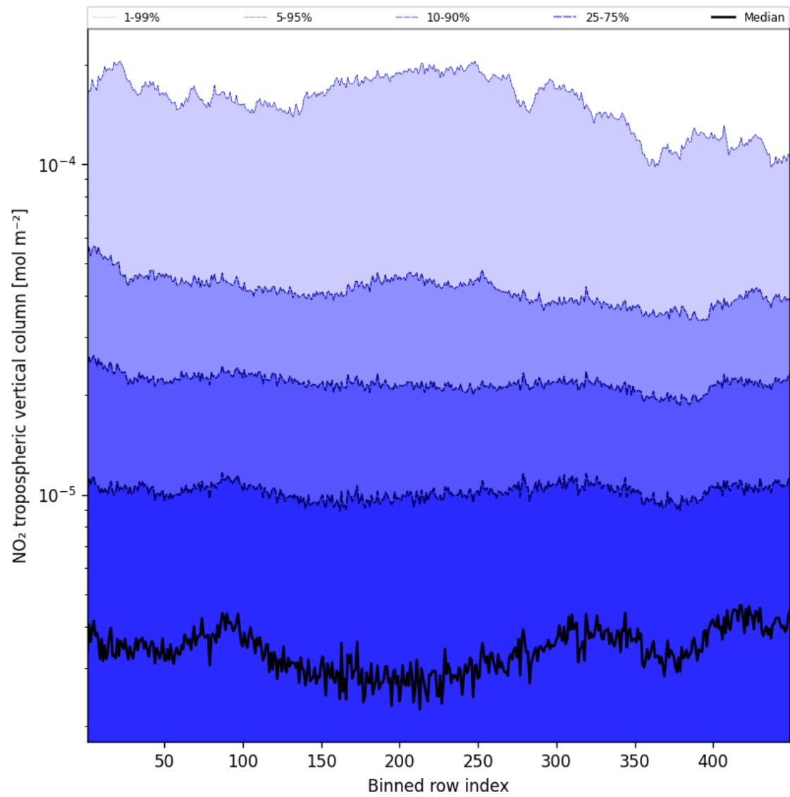
Figure 44: Along track statistics of “NO 2 tropospheric vertical column” for 2024-12-19 to 2024-12-19
