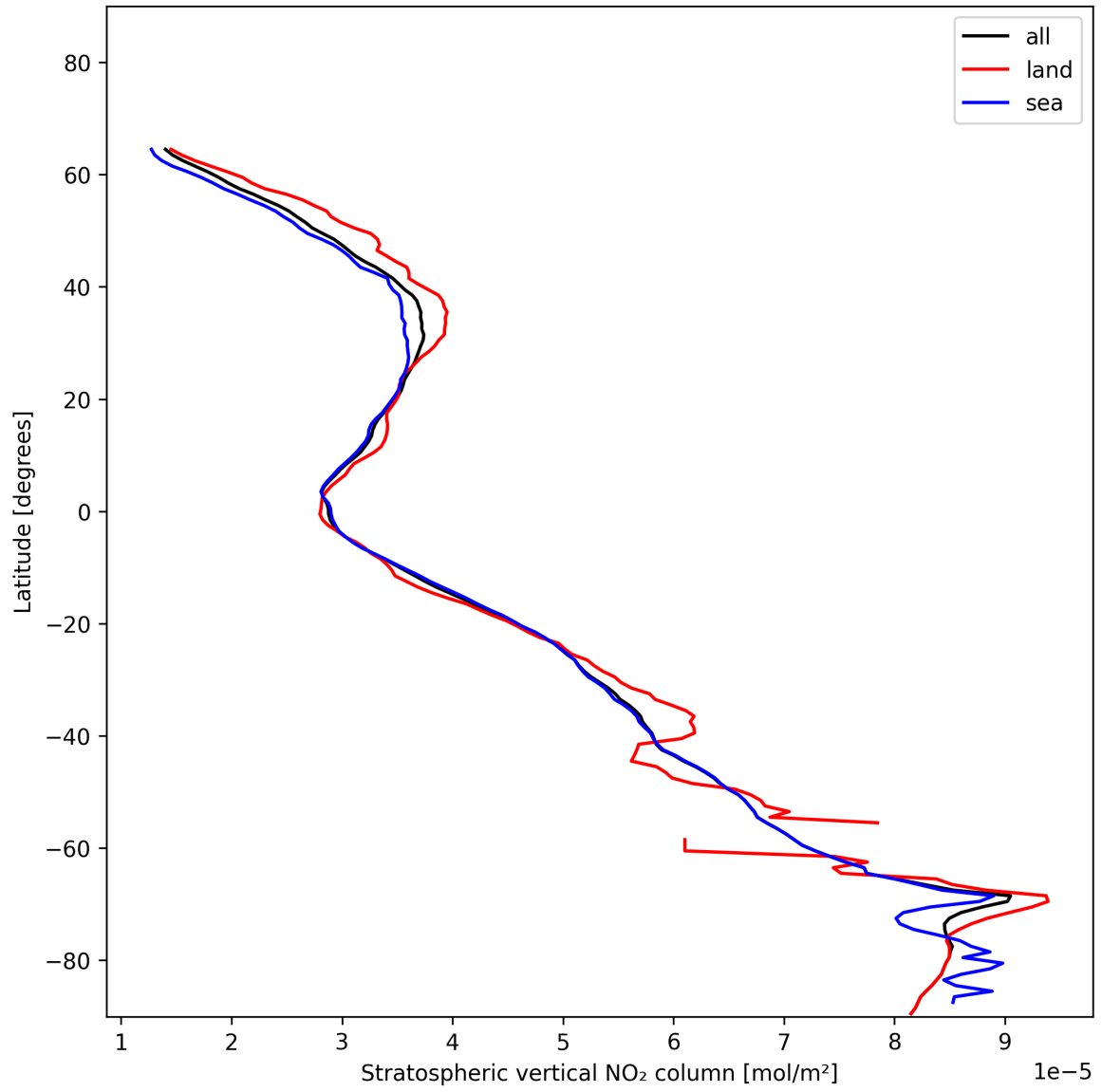
Figure 17: Zonal average of “Stratospheric vertical NO 2 column” for 2024-12-19 to 2024-12-19.
