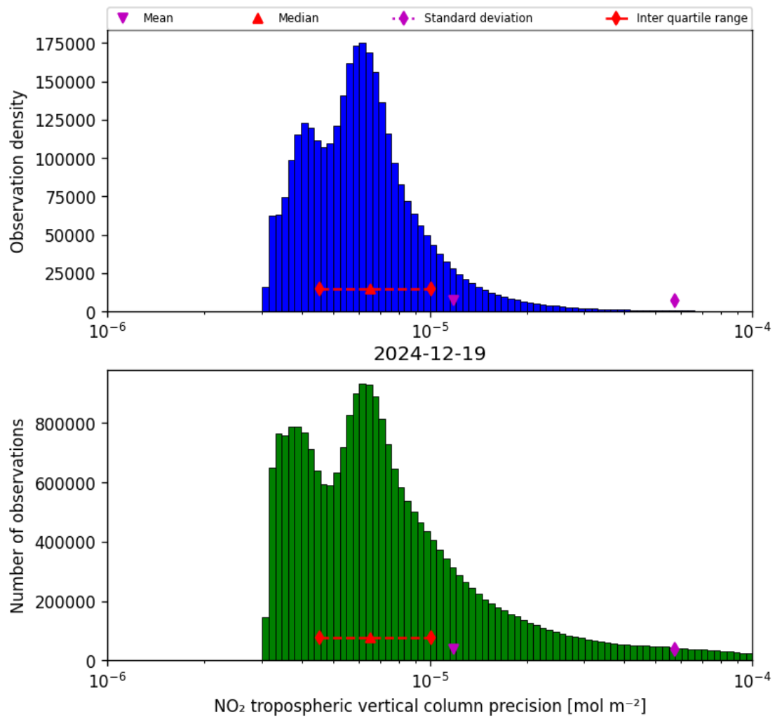
Figure 28: Histogram of “NO 2 tropospheric vertical column precision” for 2024-12-19 to 2024-12-19
