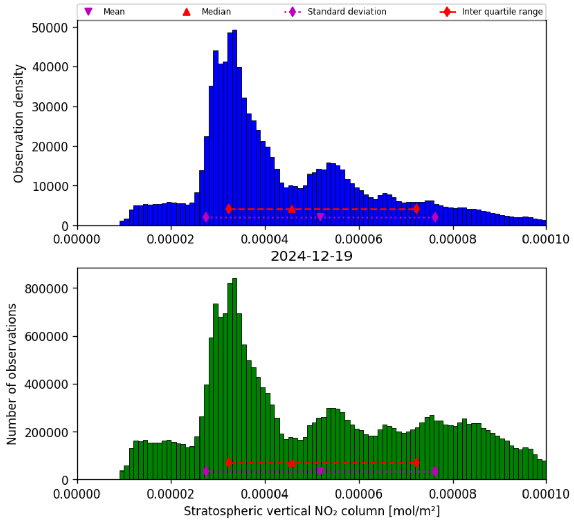
Figure 34: Histogram of “Stratospheric vertical NO 2 column” for 2024-12-19 to 2024-12-19
