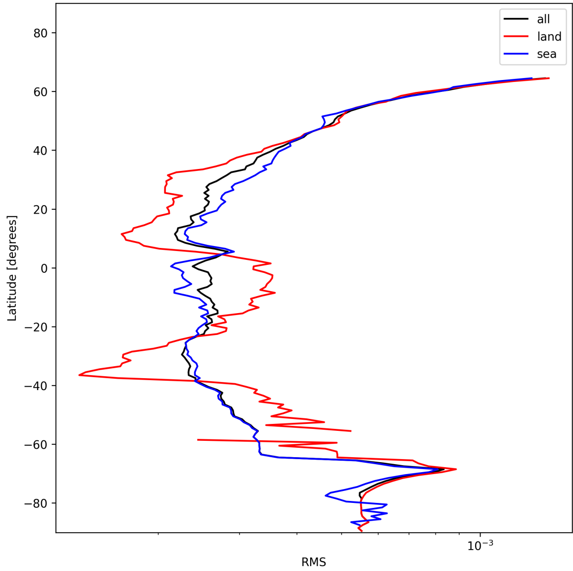
Figure 24: Zonal average of “RMS” for 2024-12-19 to 2024-12-19.
