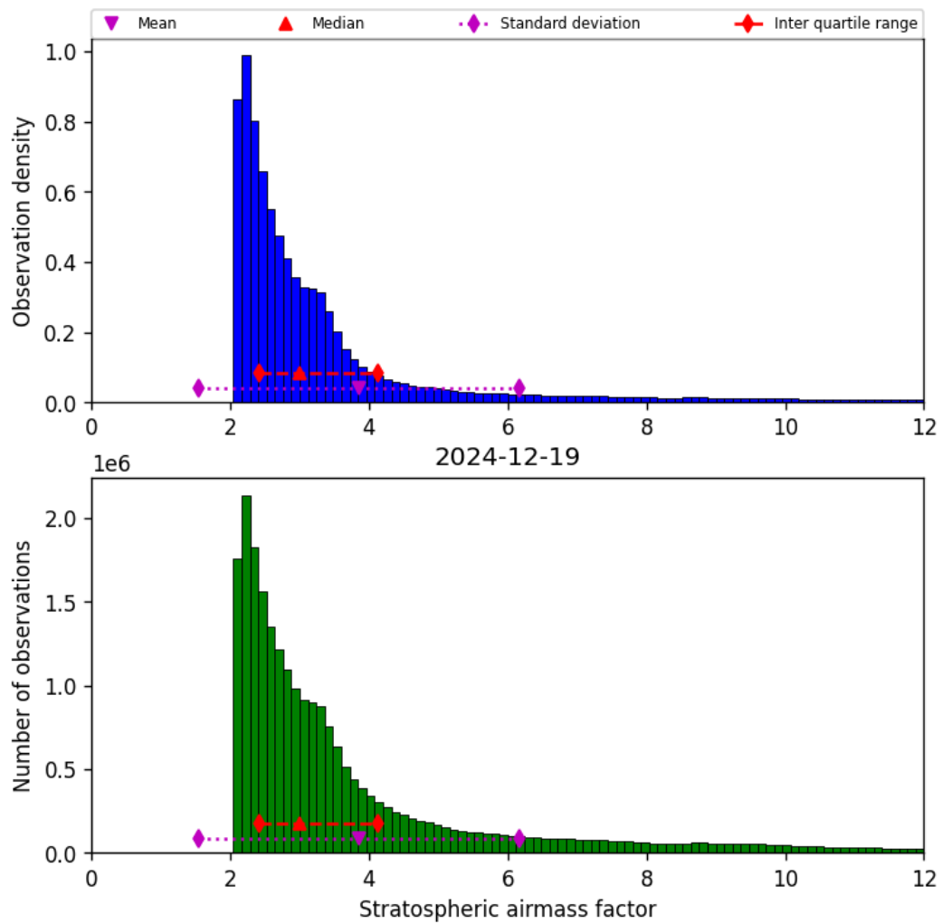
Figure 42: Histogram of “Stratospheric airmass factor” for 2024-12-19 to 2024-12-19
