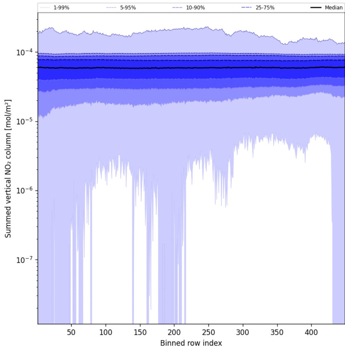
Figure 55: Along track statistics of “Summed vertical NO 2 column” for 2024-12-19 to 2024-12-19
