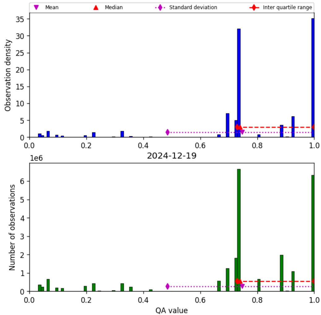
Figure 26: Histogram of “QA value” for 2024-12-19 to 2024-12-19
