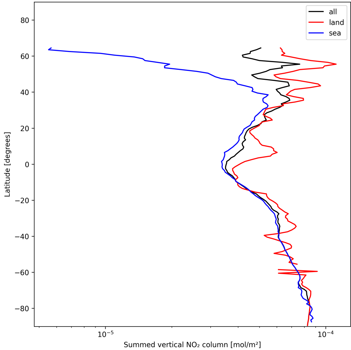
Figure 21: Zonal average of “Summed vertical NO 2 column” for 2024-12-19 to 2024-12-19.
