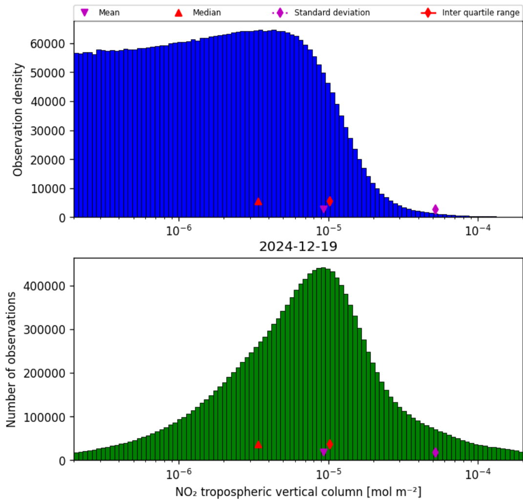
Figure 27: Histogram of “ \text{NO}_2 tropospheric vertical column” for 2024-12-19 to 2024-12-19
