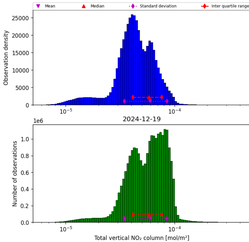
Figure 36: Histogram of "Total vertical NO 2 column" for 2024-12-19 to 2024-12-19
