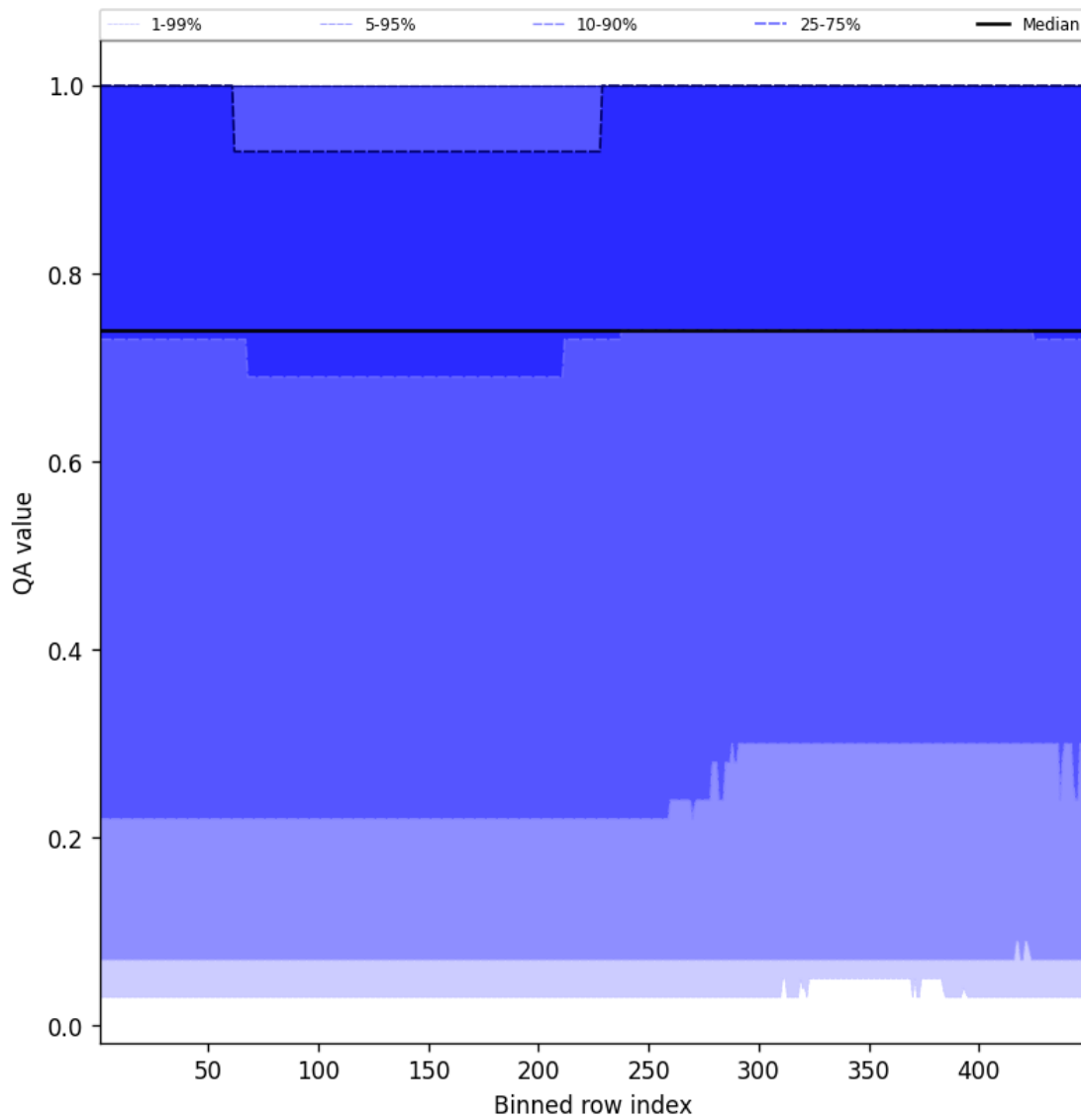
Figure 43: Along track statistics of “QA value” for 2024-12-19 to 2024-12-19
