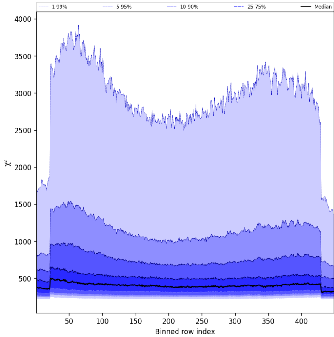
Figure 57: Along track statistics of “ \chi^2 ” for 2024-12-19 to 2024-12-19
