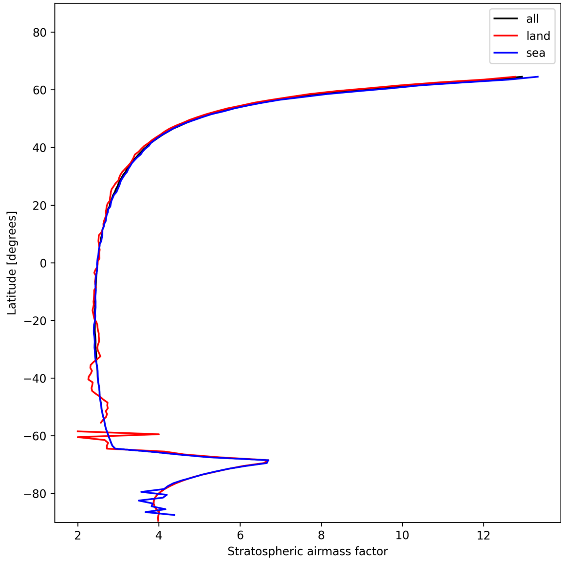
Figure 25: Zonal average of “Stratospheric airmass factor” for 2024-12-19 to 2024-12-19.
