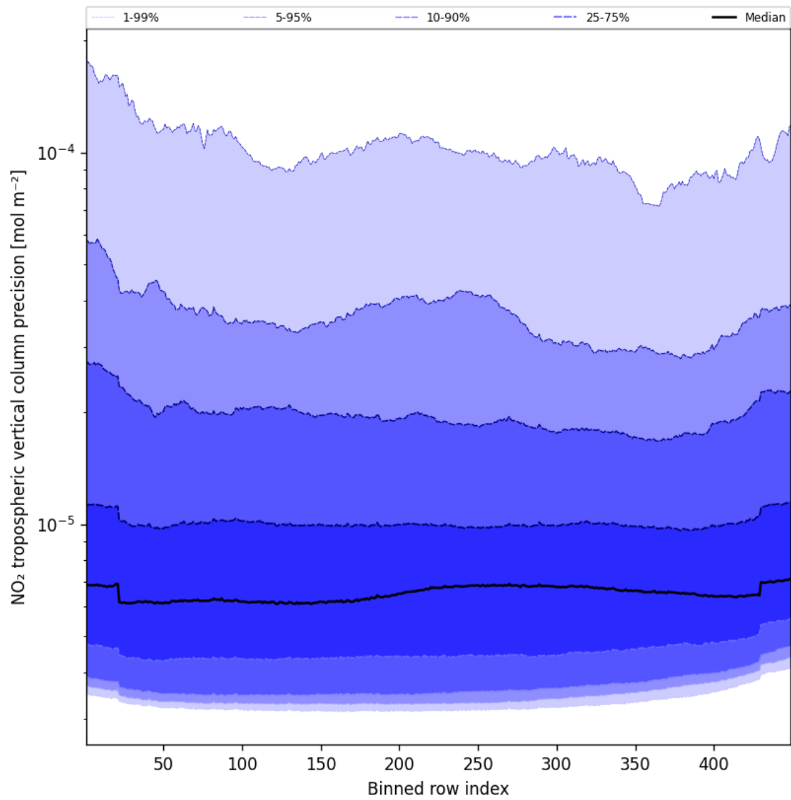
Figure 45: Along track statistics of “NO 2 tropospheric vertical column precision” for 2024-12-19 to 2024-12-19
