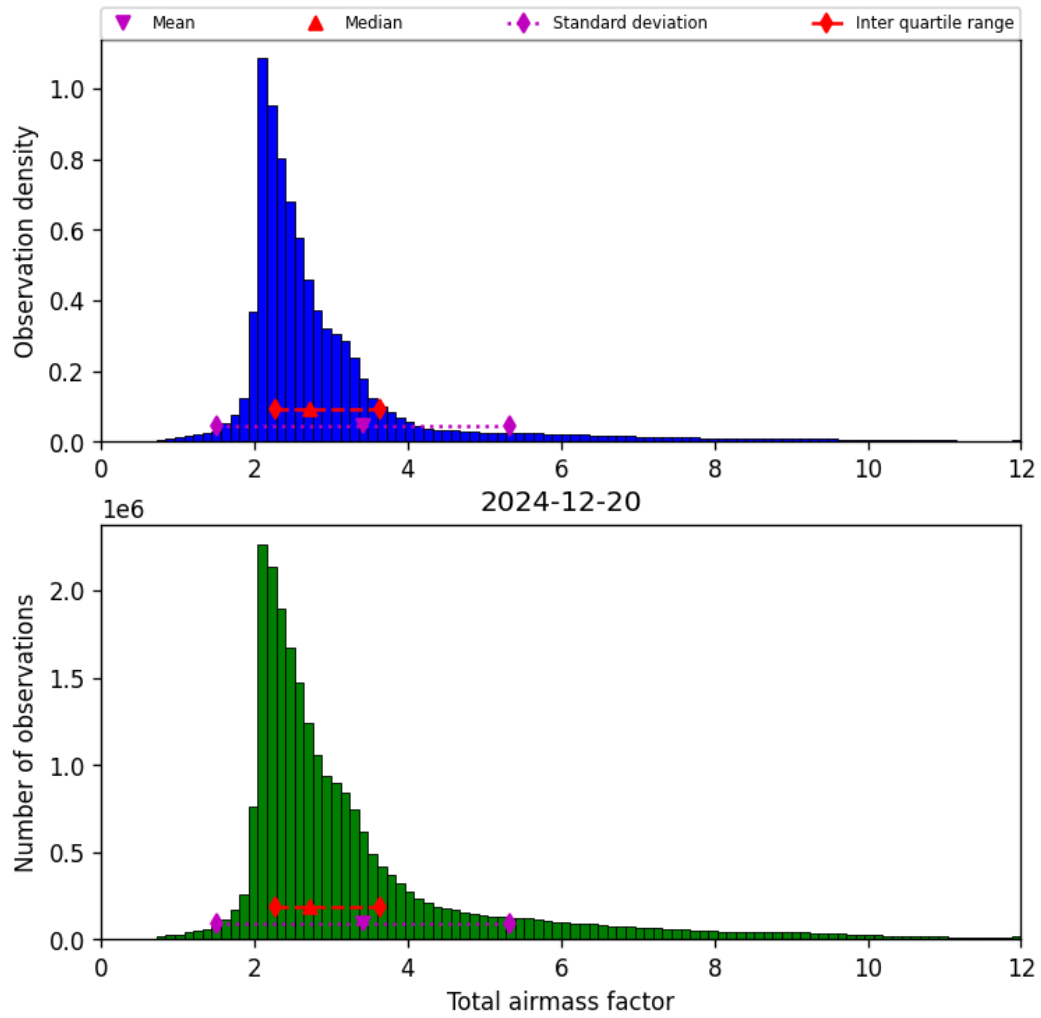
Figure 30: Histogram of “Total airmass factor” for 2024-12-20 to 2024-12-20
