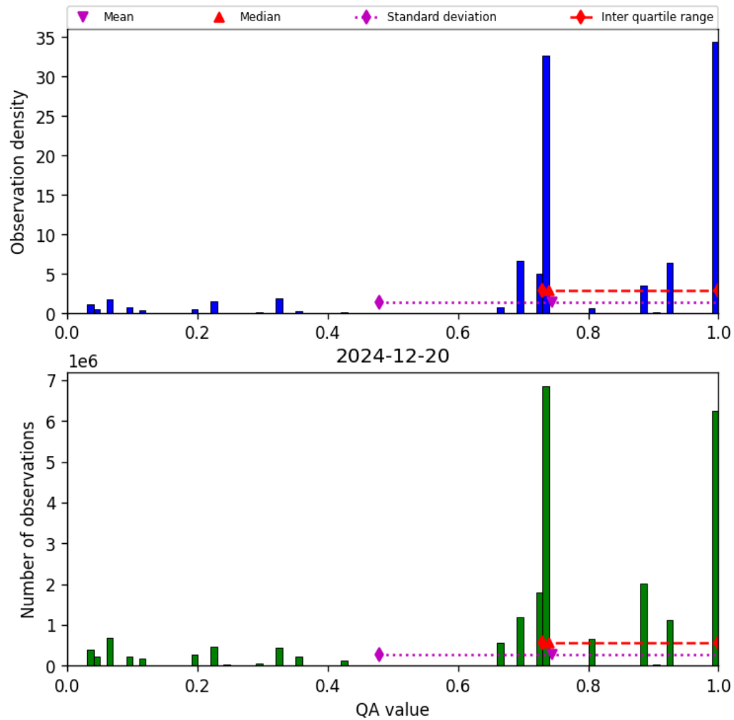
Figure 26: Histogram of “QA value” for 2024-12-20 to 2024-12-20
