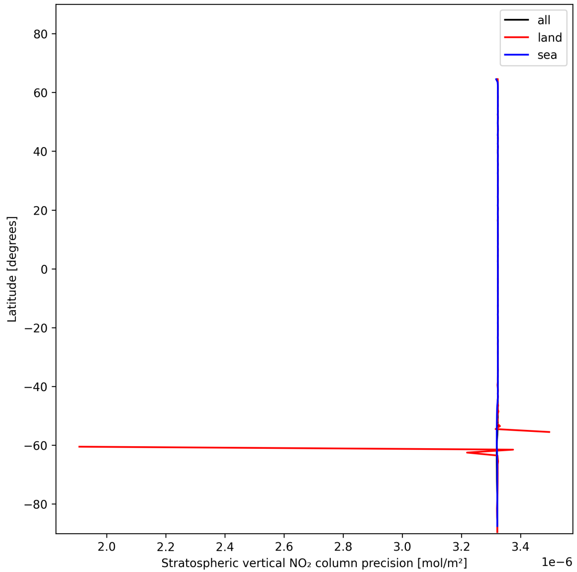
Figure 18: Zonal average of “Stratospheric vertical NO 2 column precision” for 2024-12-20 to 2024-12-20.
