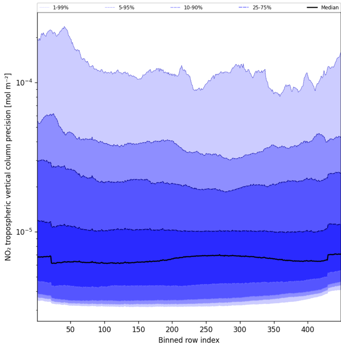
Figure 45: Along track statistics of “NO 2 tropospheric vertical column precision” for 2024-12-20 to 2024-12-20
