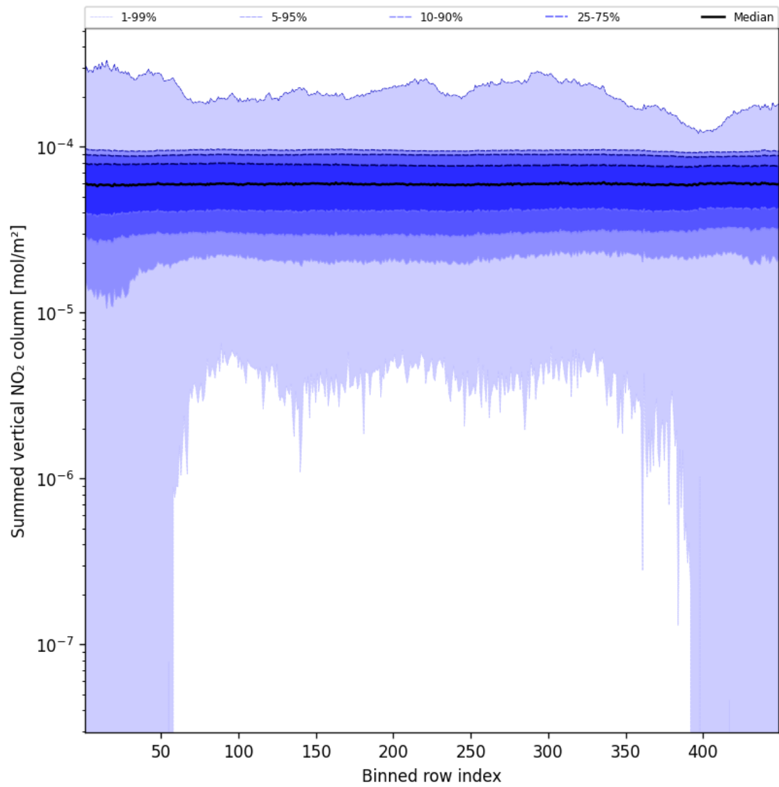
Figure 55: Along track statistics of “Summed vertical NO 2 column” for 2024-12-20 to 2024-12-20
