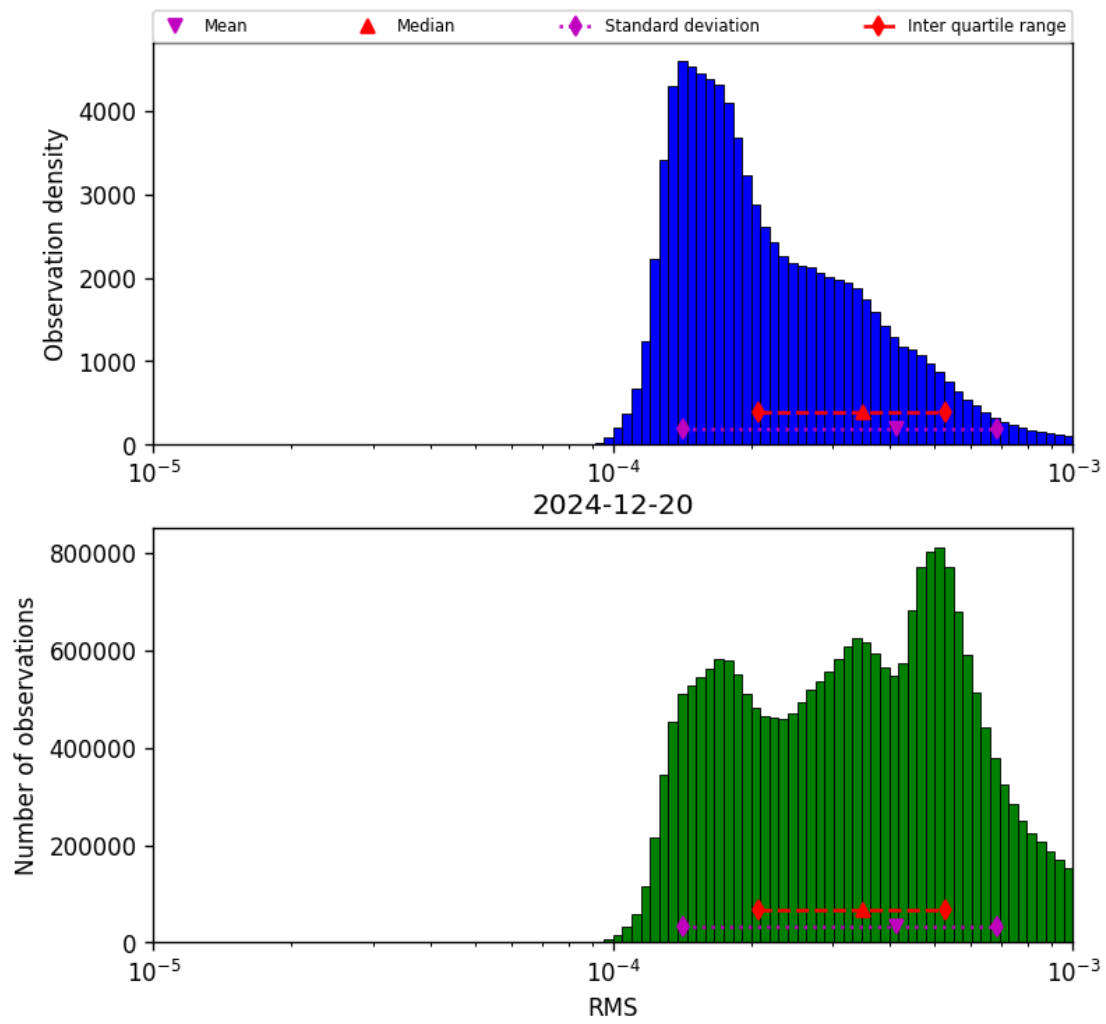
Figure 41: Histogram of “RMS” for 2024-12-20 to 2024-12-20
