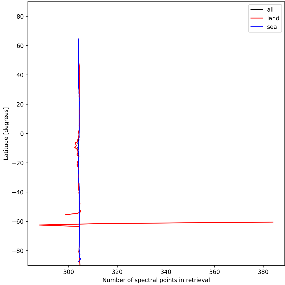
Figure 14: Zonal average of “Number of spectral points in retrieval” for 2024-12-20 to 2024-12-20.
