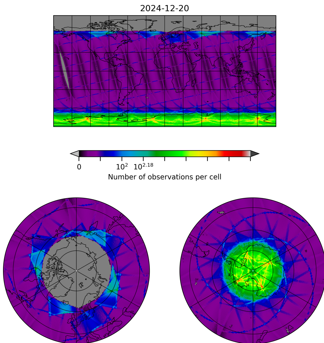
Figure 8: Map of the number of observations for 2024-12-20 to 2024-12-20
