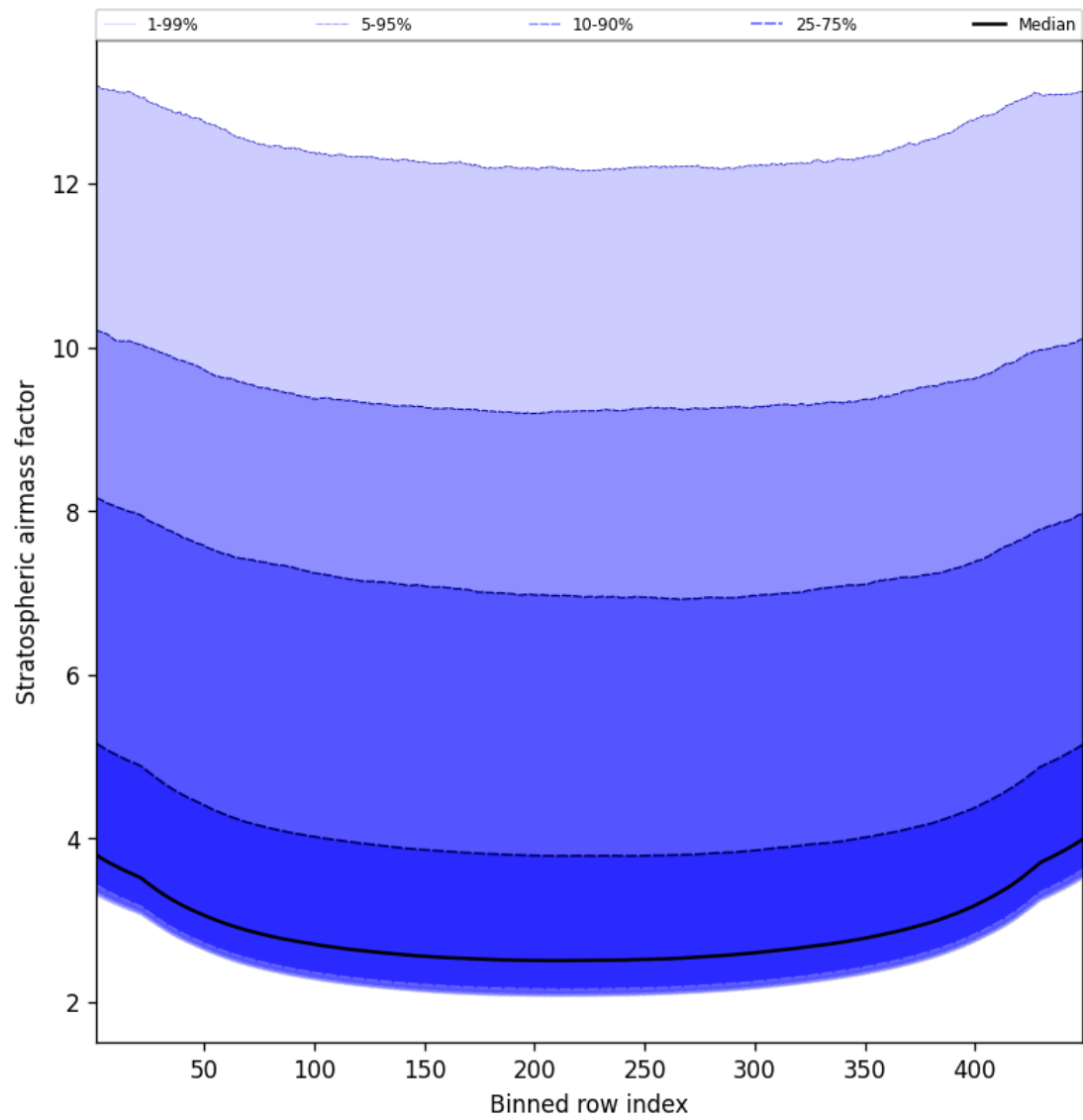
Figure 59: Along track statistics of “Stratospheric airmass factor” for 2024-12-20 to 2024-12-20
