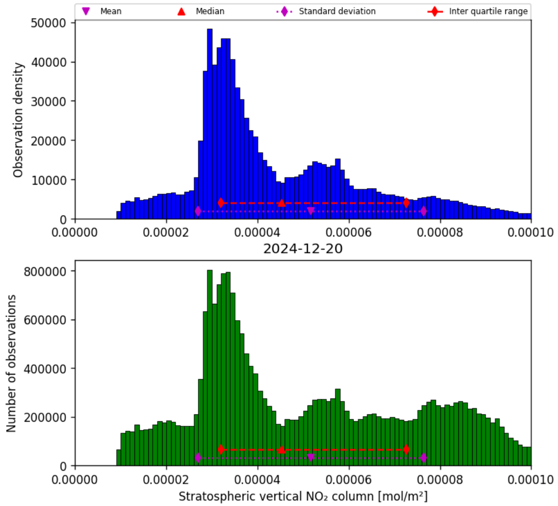
Figure 34: Histogram of “Stratospheric vertical NO 2 column” for 2024-12-20 to 2024-12-20
