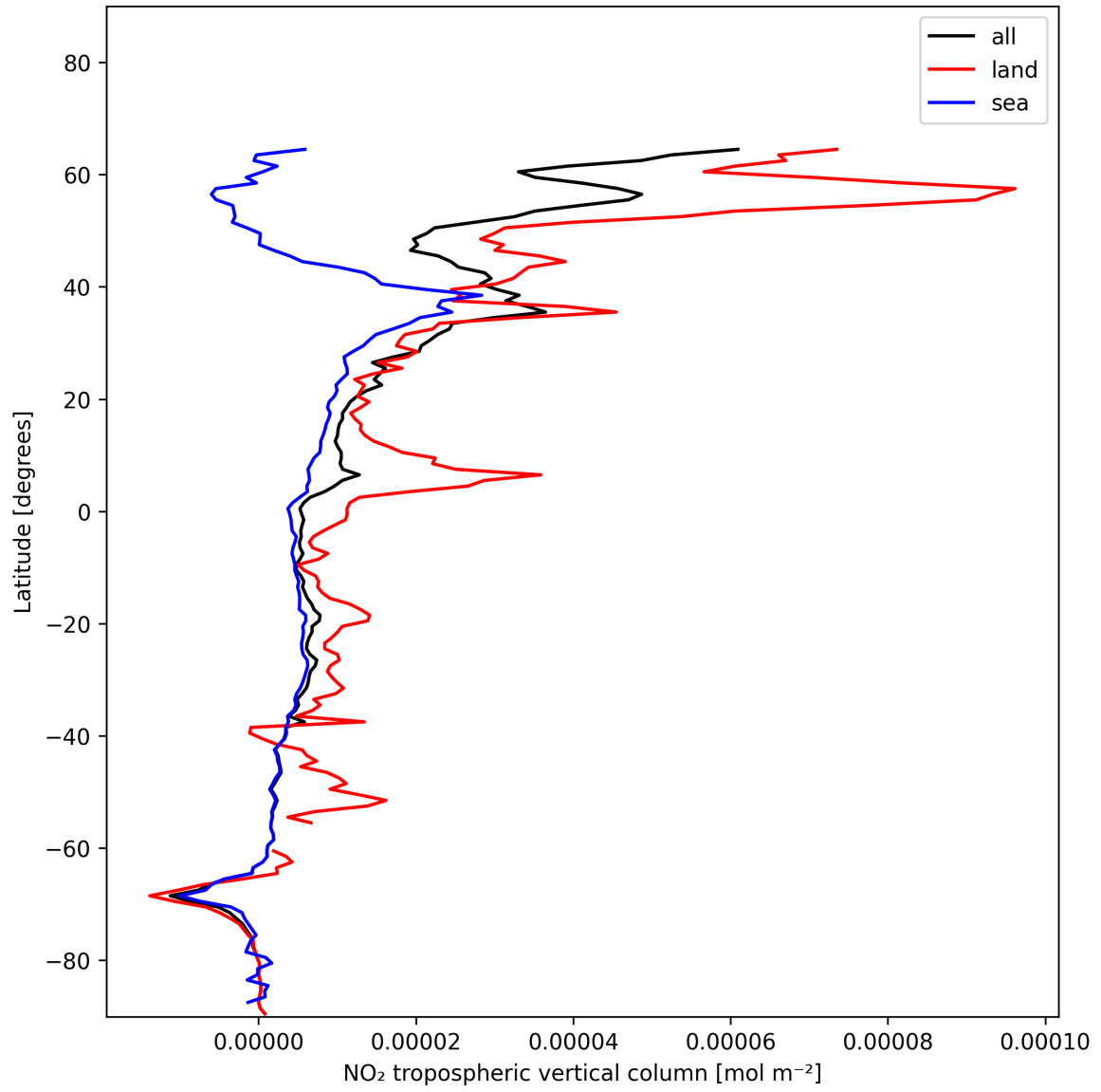
Figure 10: Zonal average of “NO 2 tropospheric vertical column” for 2024-12-20 to 2024-12-20.
