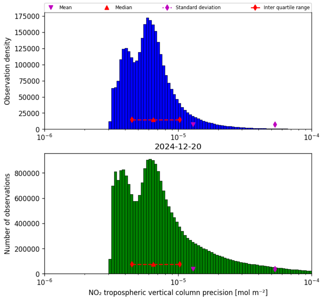
Figure 28: Histogram of “NO 2 tropospheric vertical column precision” for 2024-12-20 to 2024-12-20
