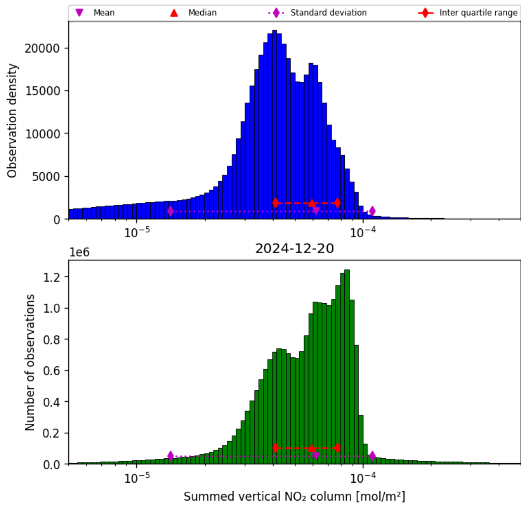
Figure 38: Histogram of “Summed vertical NO 2 column” for 2024-12-20 to 2024-12-20
