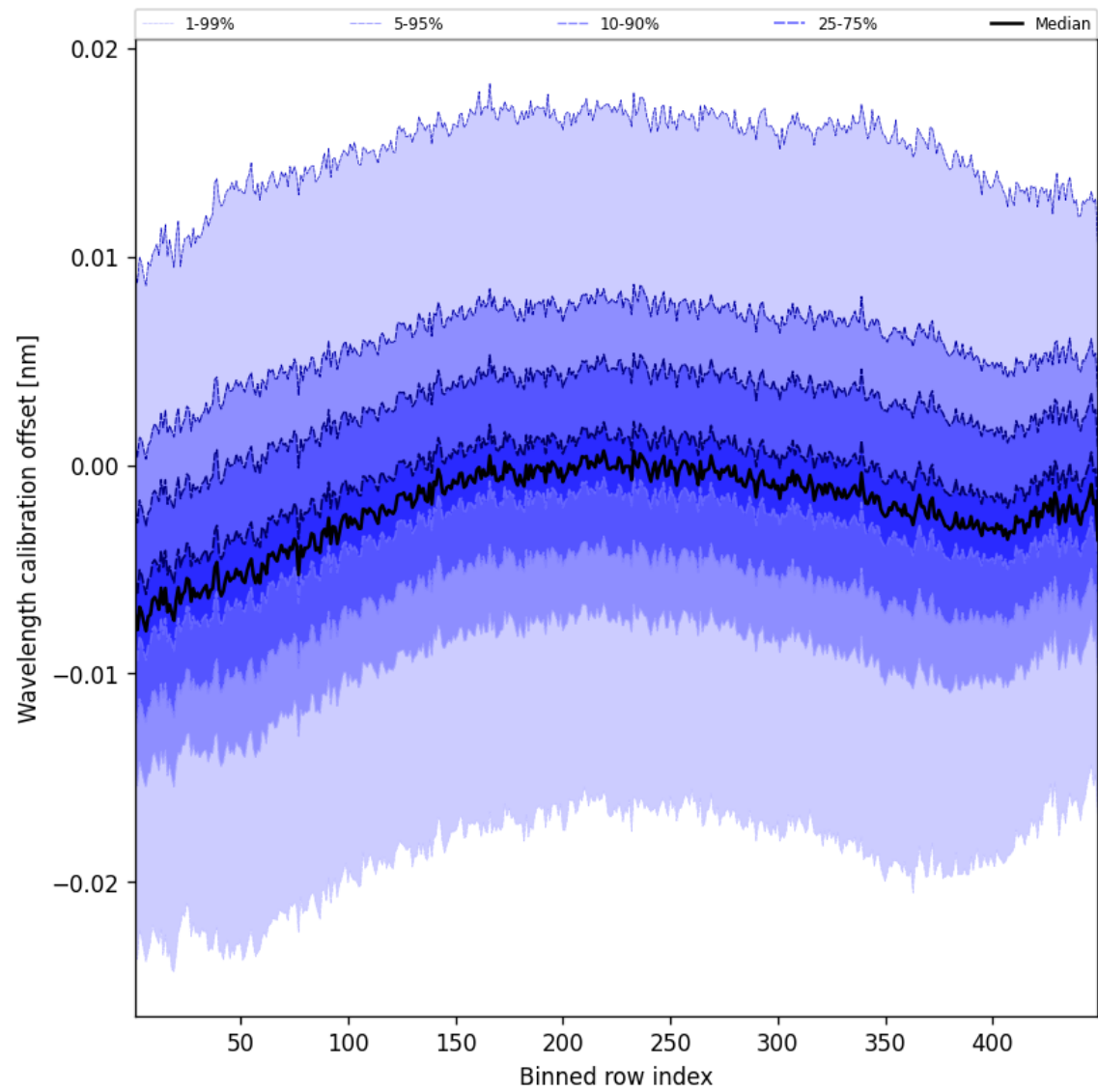
Figure 50: Along track statistics of “Wavelength calibration offset” for 2024-12-20 to 2024-12-20
