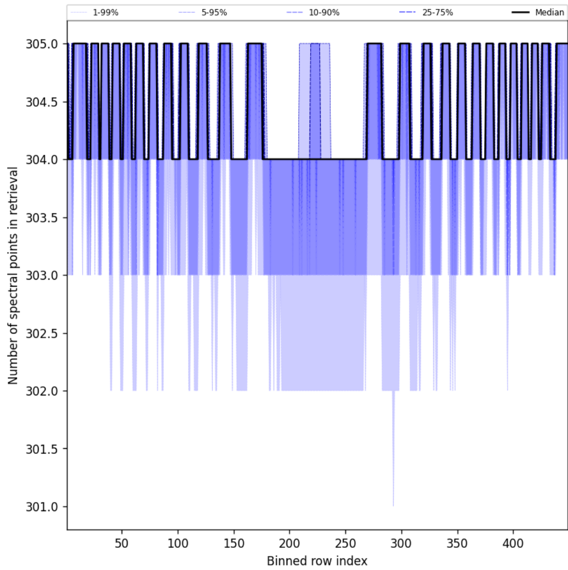
Figure 48: Along track statistics of “Number of spectral points in retrieval” for 2024-12-20 to 2024-12-20
