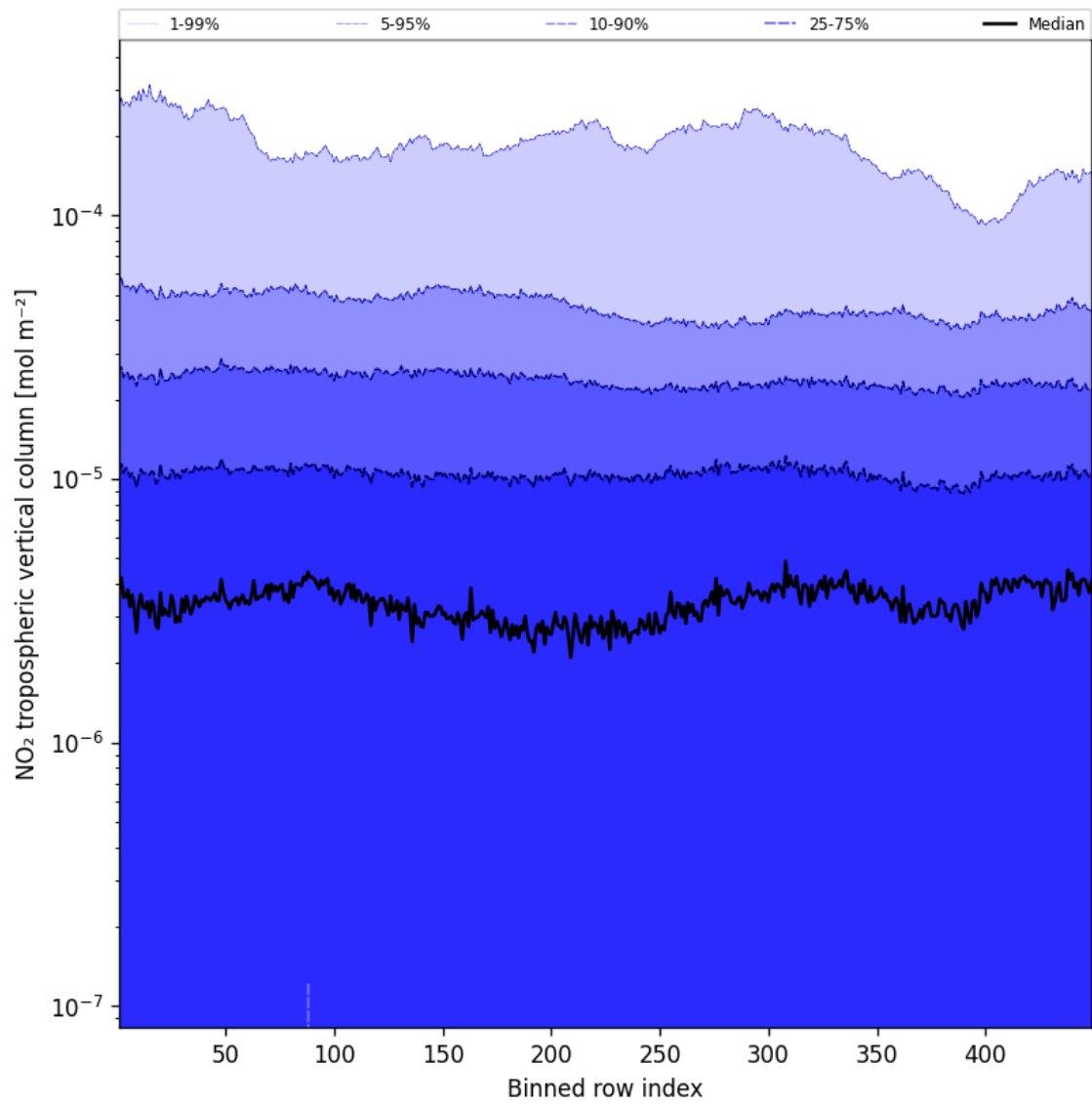
Figure 44: Along track statistics of “NO 2 tropospheric vertical column” for 2024-12-20 to 2024-12-20
