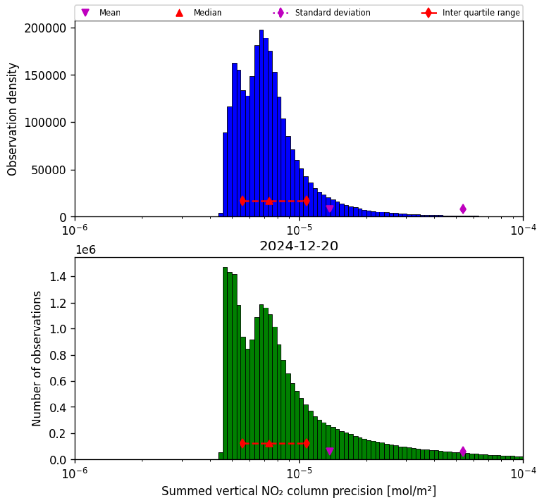
Figure 39: Histogram of "Summed vertical NO 2 column precision" for 2024-12-20 to 2024-12-20
