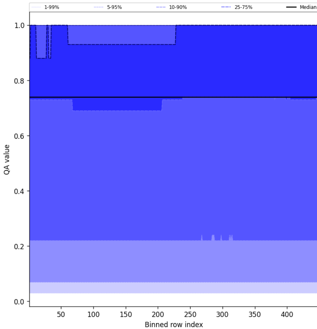
Figure 43: Along track statistics of "QA value" for 2024-12-20 to 2024-12-20
