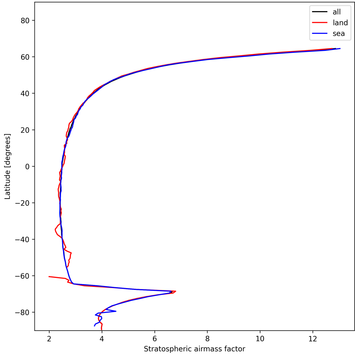
Figure 25: Zonal average of “Stratospheric airmass factor” for 2024-12-20 to 2024-12-20.
