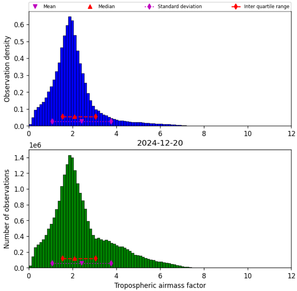
Figure 29: Histogram of “Tropospheric airmass factor” for 2024-12-20 to 2024-12-20
