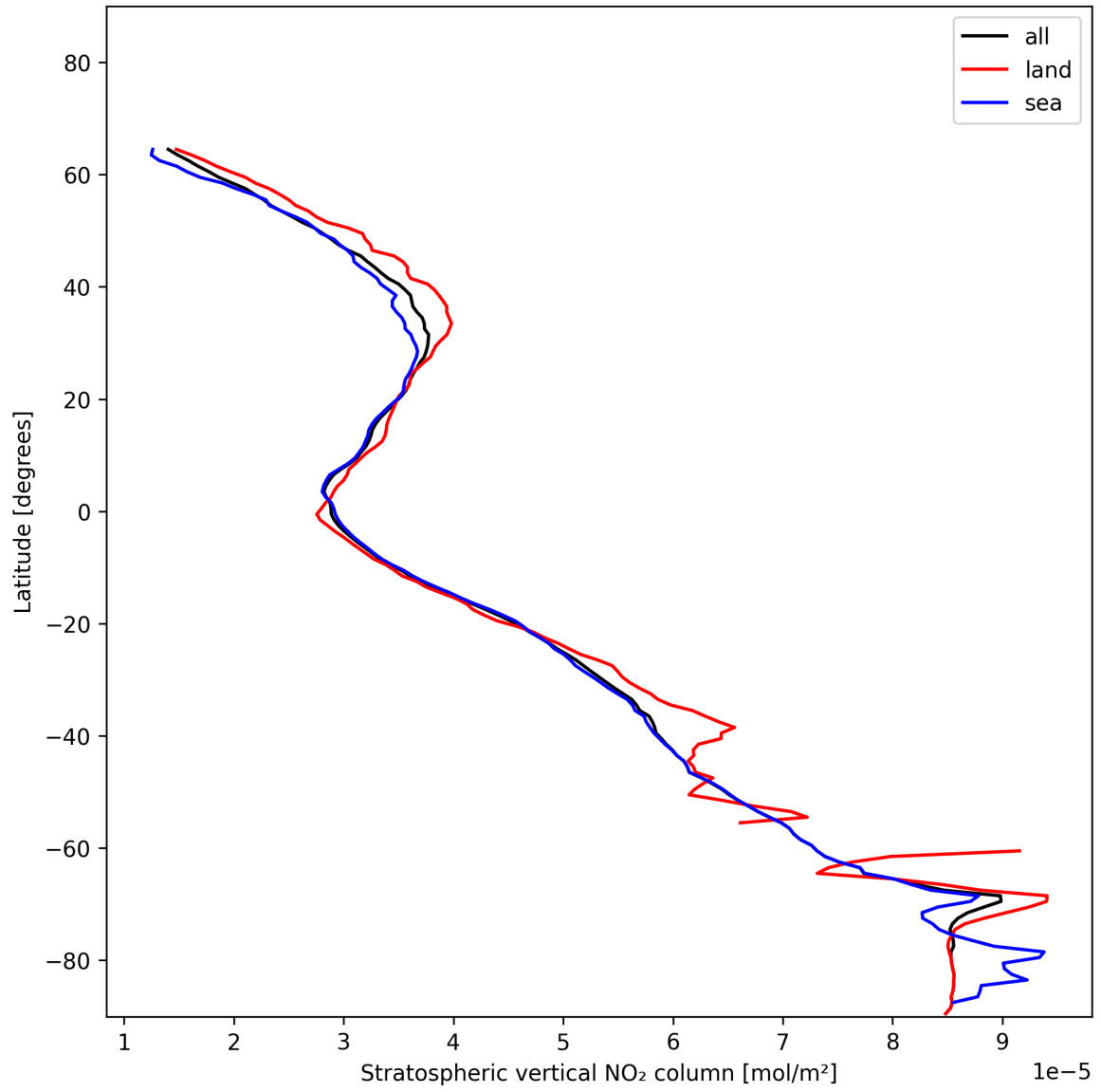
Figure 17: Zonal average of “Stratospheric vertical NO 2 column” for 2024-12-20 to 2024-12-20.
