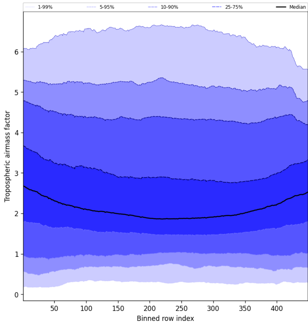
Figure 46: Along track statistics of “Tropospheric airmass factor” for 2024-12-20 to 2024-12-20
