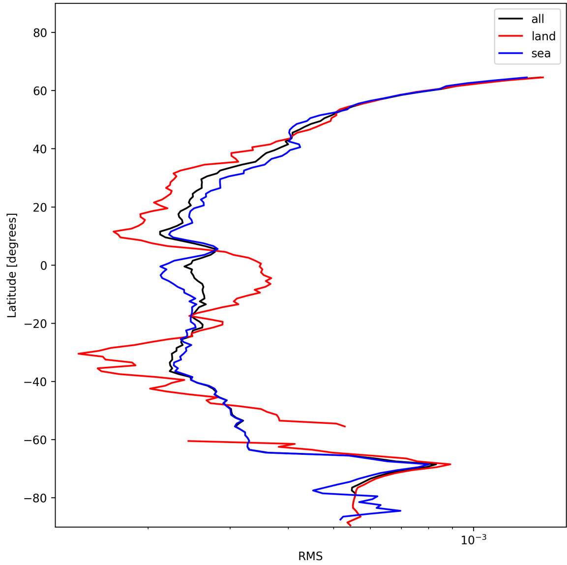
Figure 24: Zonal average of “RMS” for 2024-12-20 to 2024-12-20.
