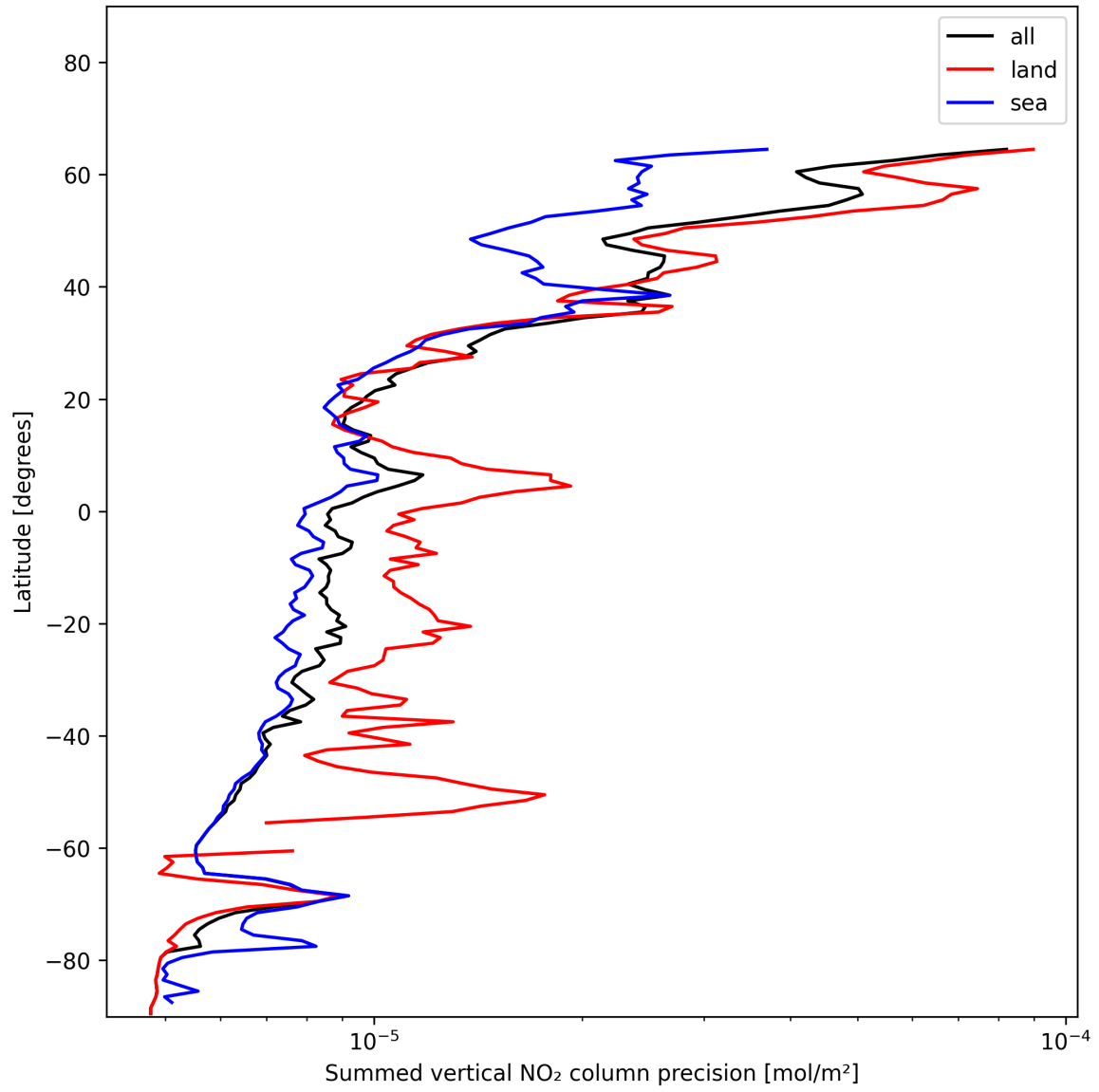
Figure 22: Zonal average of “Summed vertical NO 2 column precision” for 2024-12-20 to 2024-12-20.
