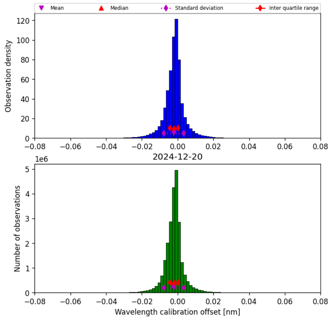
Figure 33: Histogram of “Wavelength calibration offset” for 2024-12-20 to 2024-12-20
