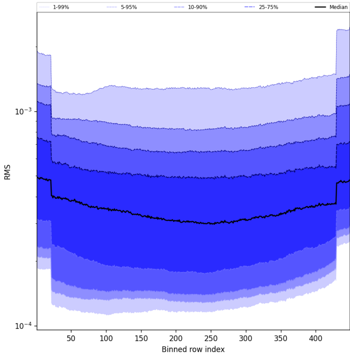
Figure 58: Along track statistics of “RMS” for 2024-12-20 to 2024-12-20
