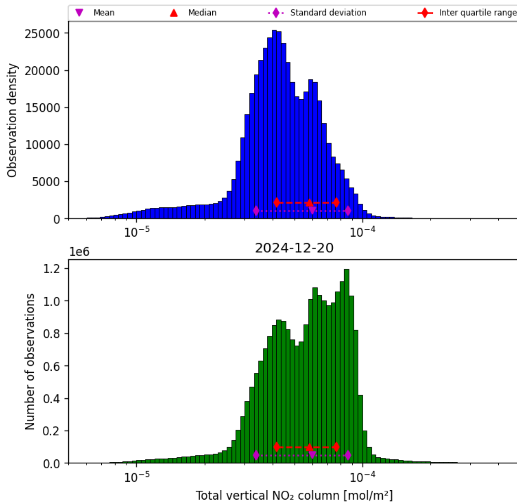
Figure 36: Histogram of "Total vertical NO 2 column" for 2024-12-20 to 2024-12-20
