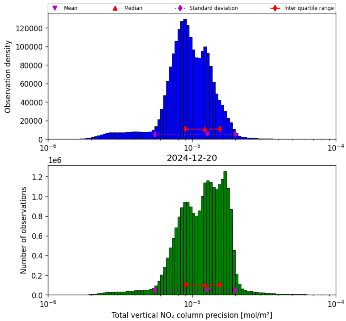
Figure 37: Histogram of "Total vertical NO 2 column precision" for 2024-12-20 to 2024-12-20
