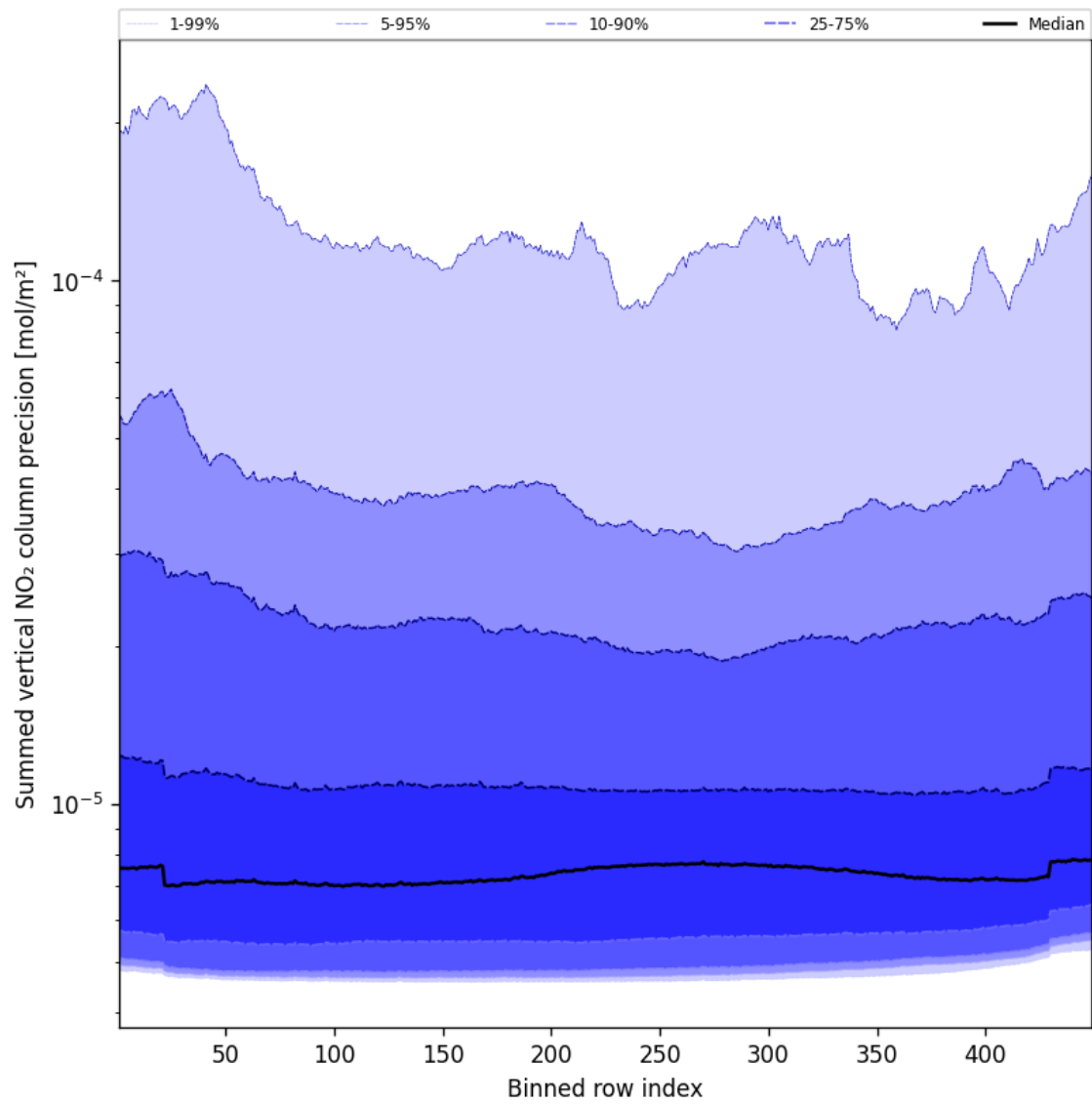
Figure 56: Along track statistics of “Summed vertical NO 2 column precision” for 2024-12-20 to 2024-12-20
