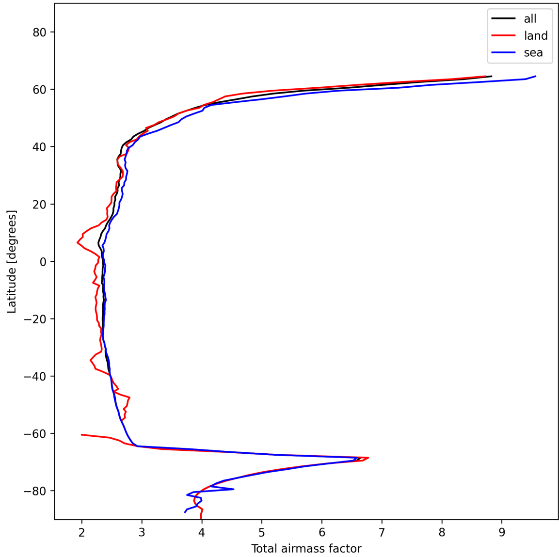
Figure 13: Zonal average of “Total airmass factor” for 2024-12-20 to 2024-12-20.
