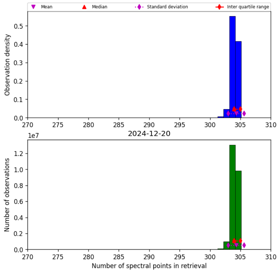
Figure 31: Histogram of “Number of spectral points in retrieval” for 2024-12-20 to 2024-12-20
