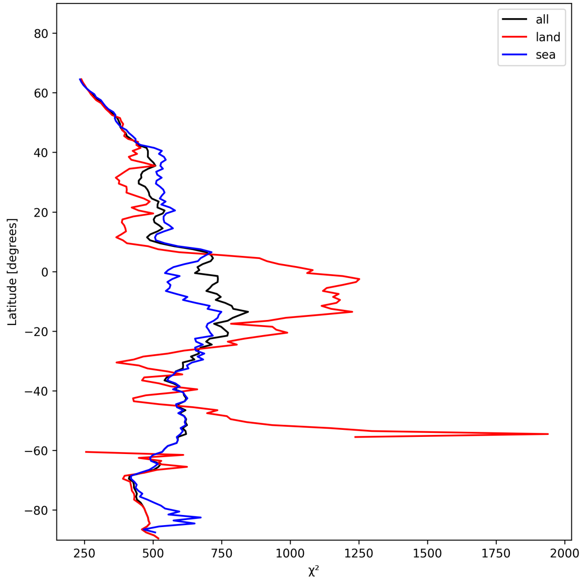
Figure 23: Zonal average of “ \chi^2 ” for 2024-12-20 to 2024-12-20.
