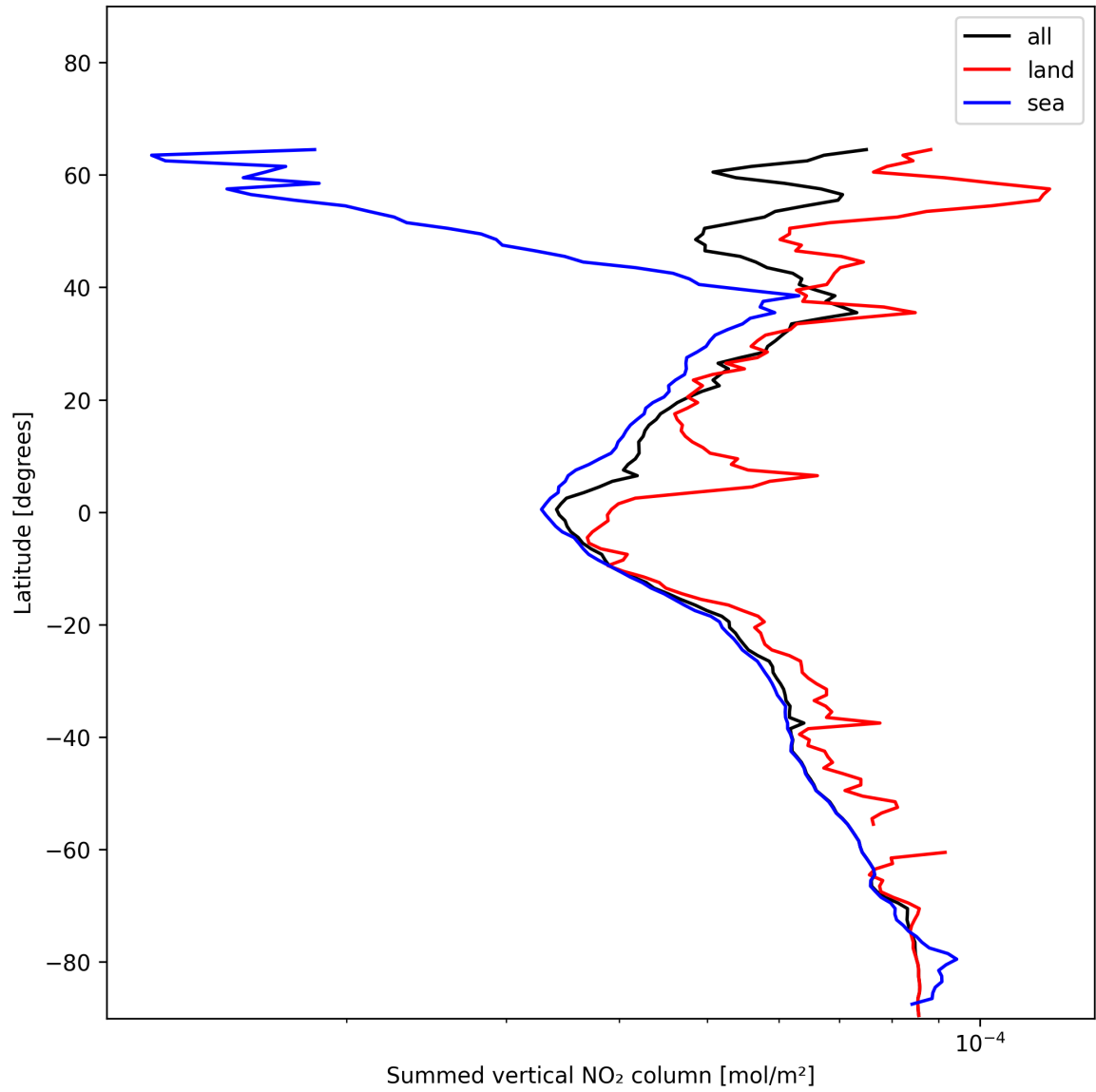
Figure 21: Zonal average of “Summed vertical NO 2 column” for 2024-12-20 to 2024-12-20.
