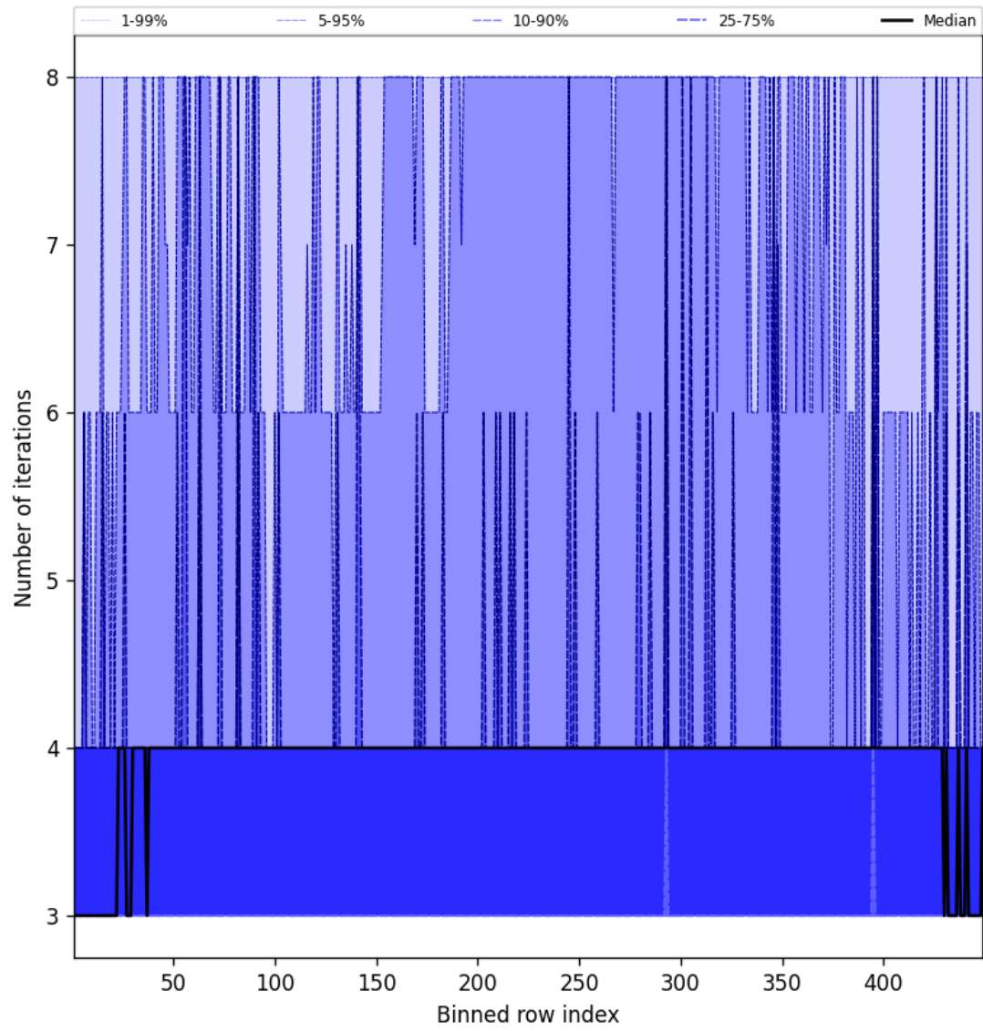
Figure 49: Along track statistics of “Number of iterations” for 2024-12-20 to 2024-12-20
