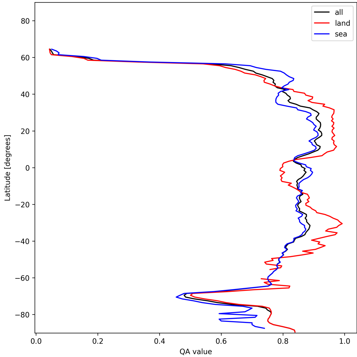
Figure 9: Zonal average of “QA value” for 2024-12-20 to 2024-12-20.
