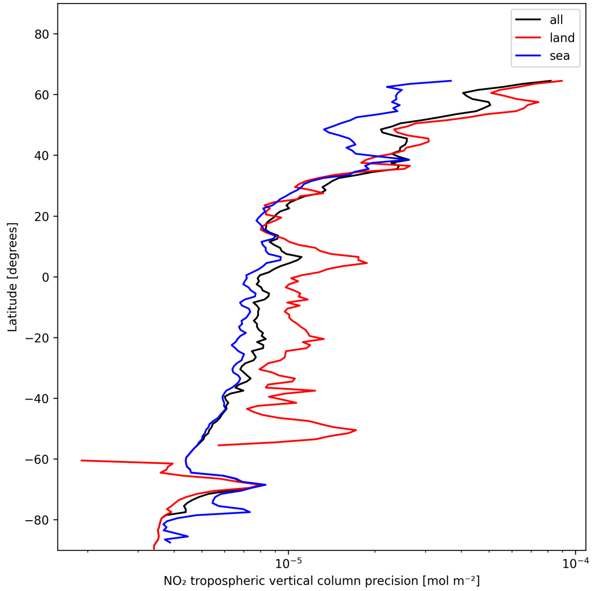
Figure 11: Zonal average of “NO 2 tropospheric vertical column precision” for 2024-12-20 to 2024-12-20.
