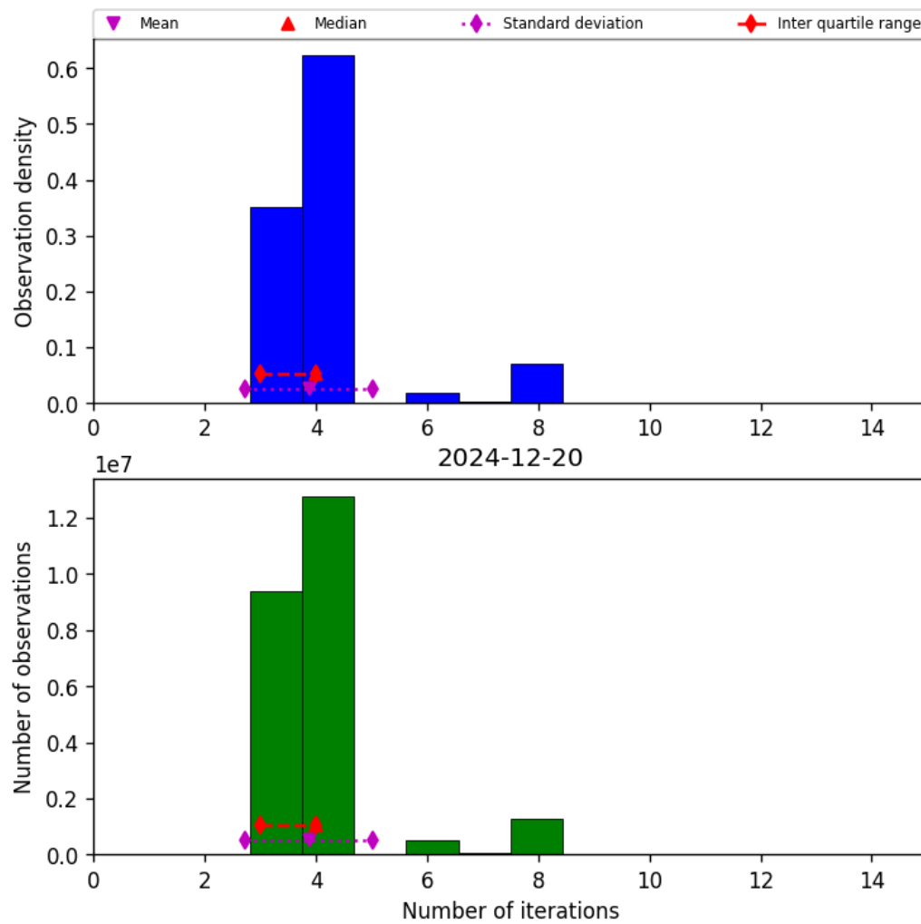
Figure 32: Histogram of “Number of iterations” for 2024-12-20 to 2024-12-20
