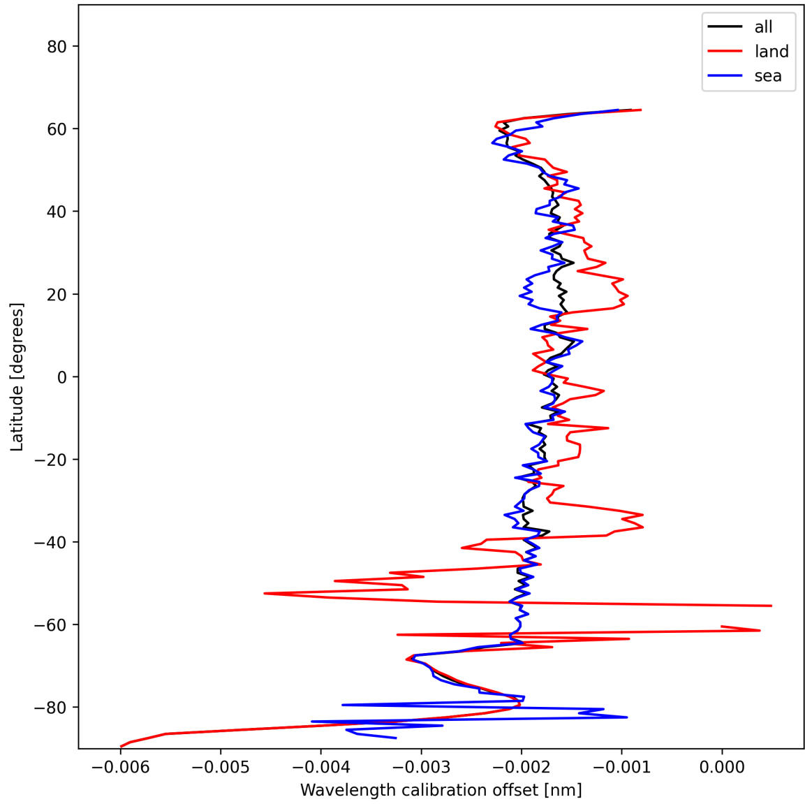
Figure 16: Zonal average of “Wavelength calibration offset” for 2024-12-20 to 2024-12-20.
