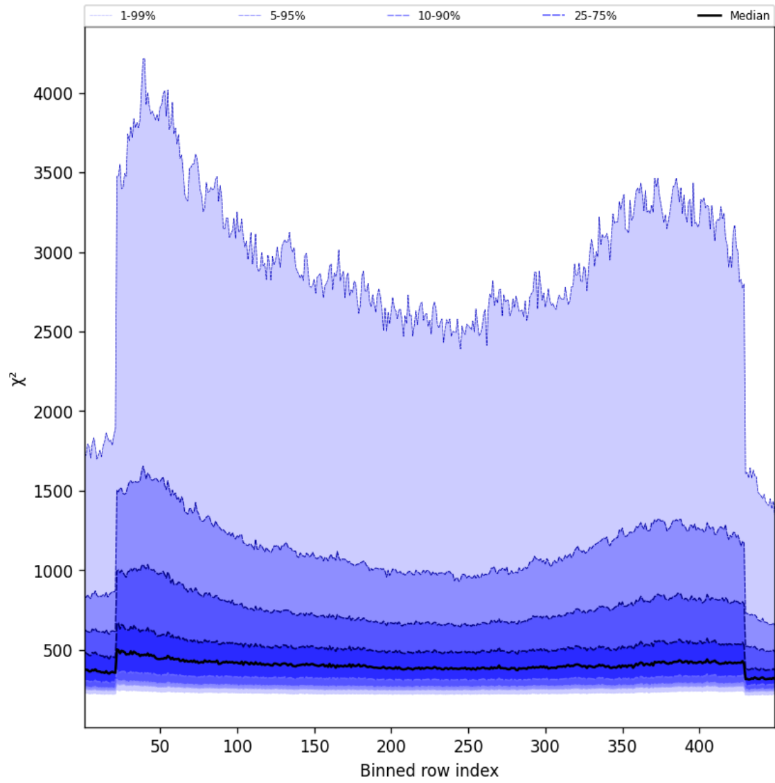
Figure 57: Along track statistics of “ \chi^2 ” for 2024-12-20 to 2024-12-20
