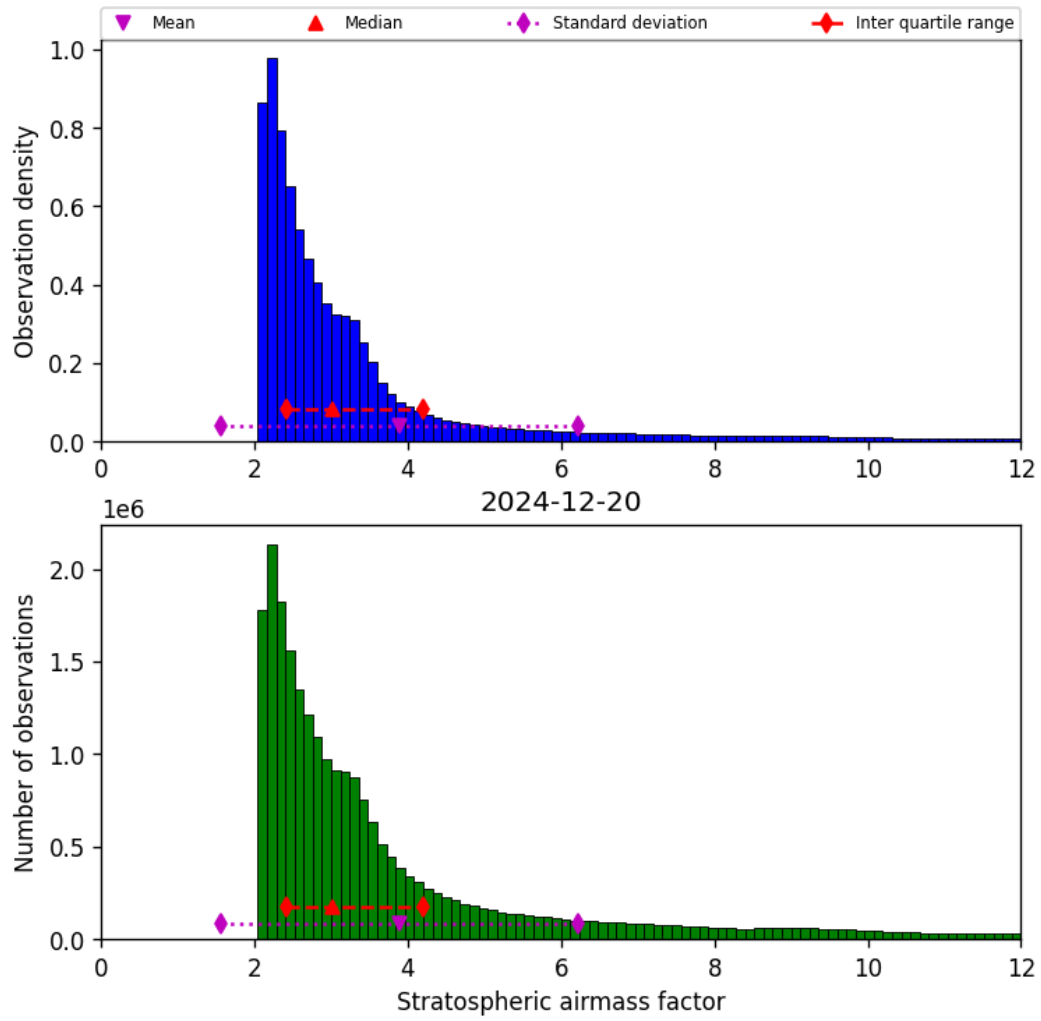
Figure 42: Histogram of “Stratospheric airmass factor” for 2024-12-20 to 2024-12-20
