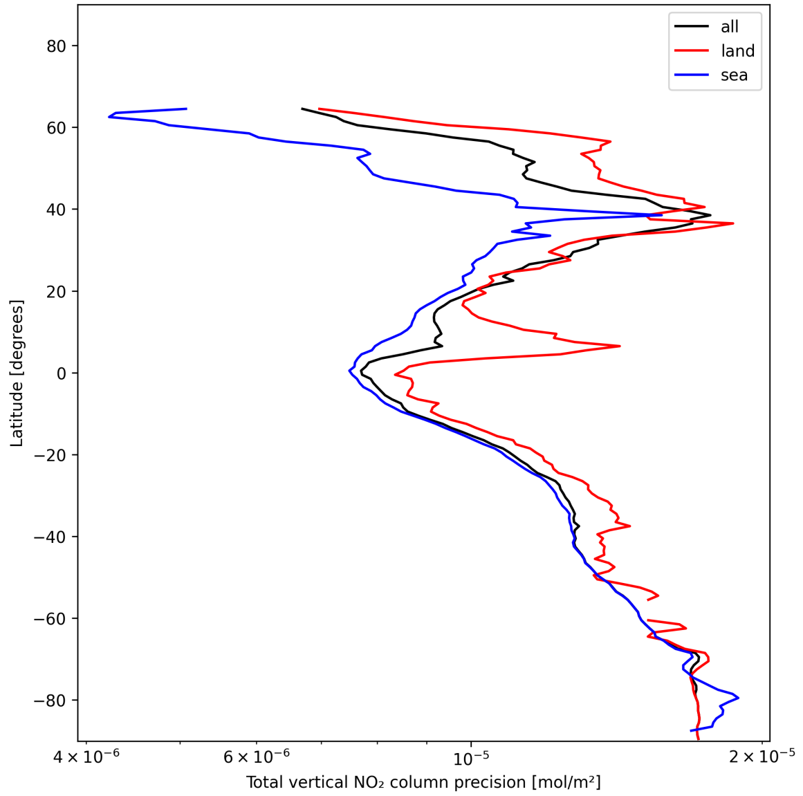
Figure 20: Zonal average of “Total vertical NO 2 column precision” for 2024-12-20 to 2024-12-20.
