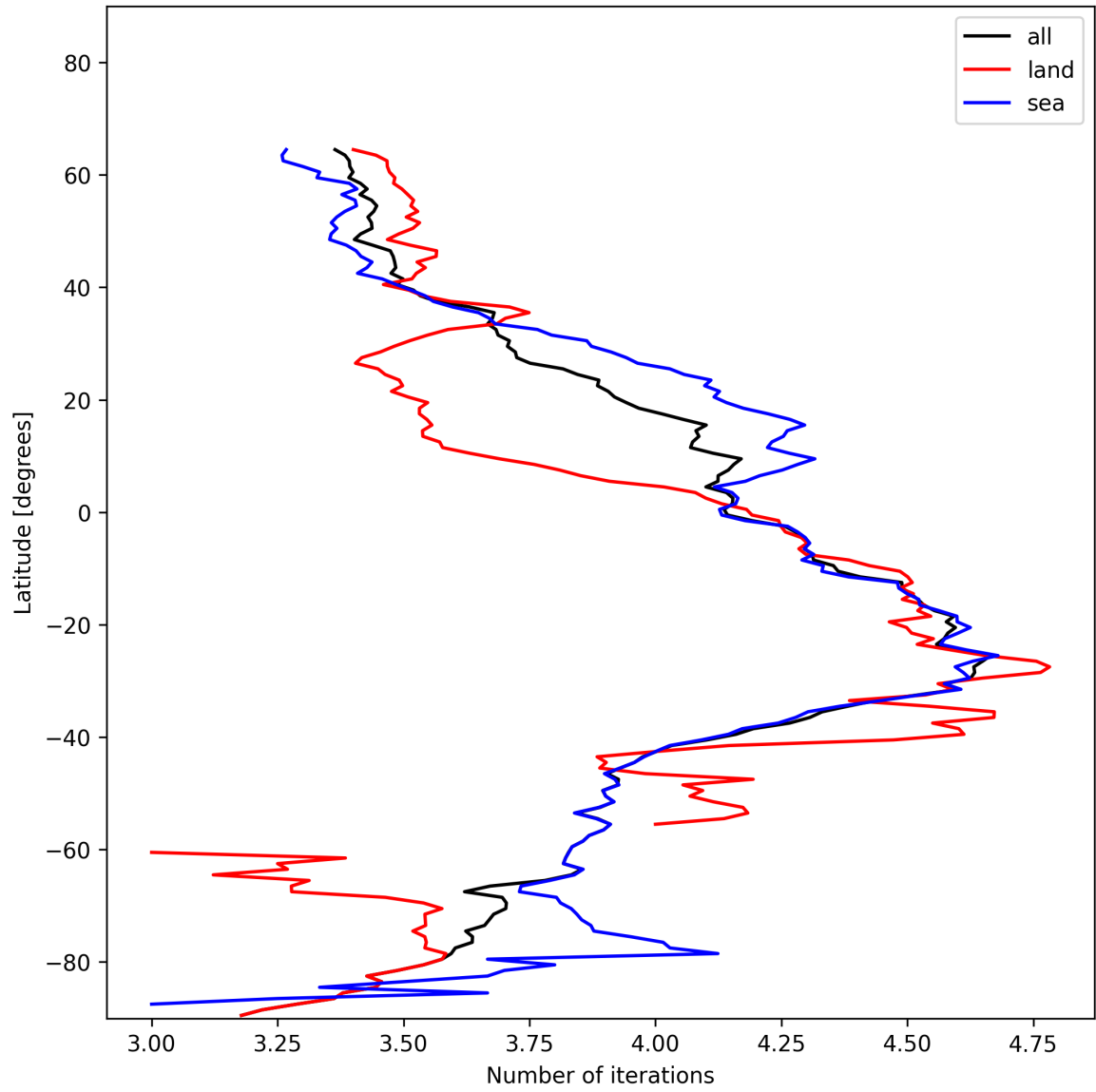
Figure 15: Zonal average of “Number of iterations” for 2024-12-20 to 2024-12-20.
