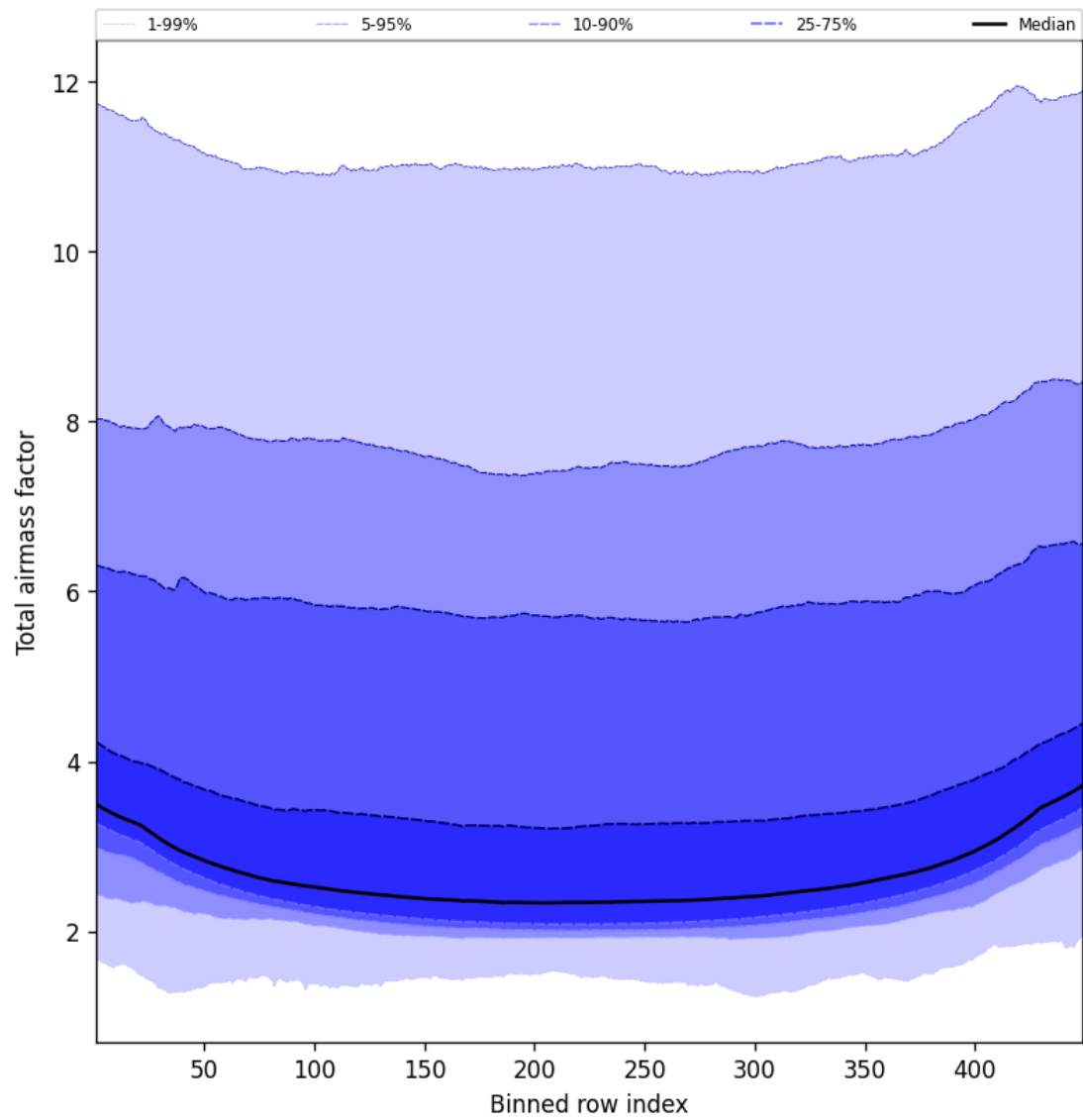
Figure 47: Along track statistics of “Total airmass factor” for 2024-12-20 to 2024-12-20
