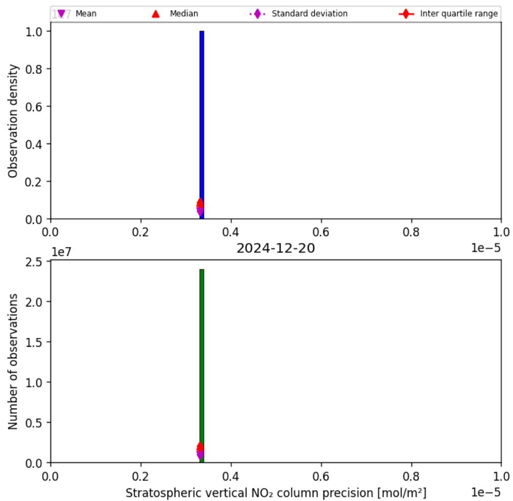
Figure 35: Histogram of “Stratospheric vertical NO 2 column precision” for 2024-12-20 to 2024-12-20
