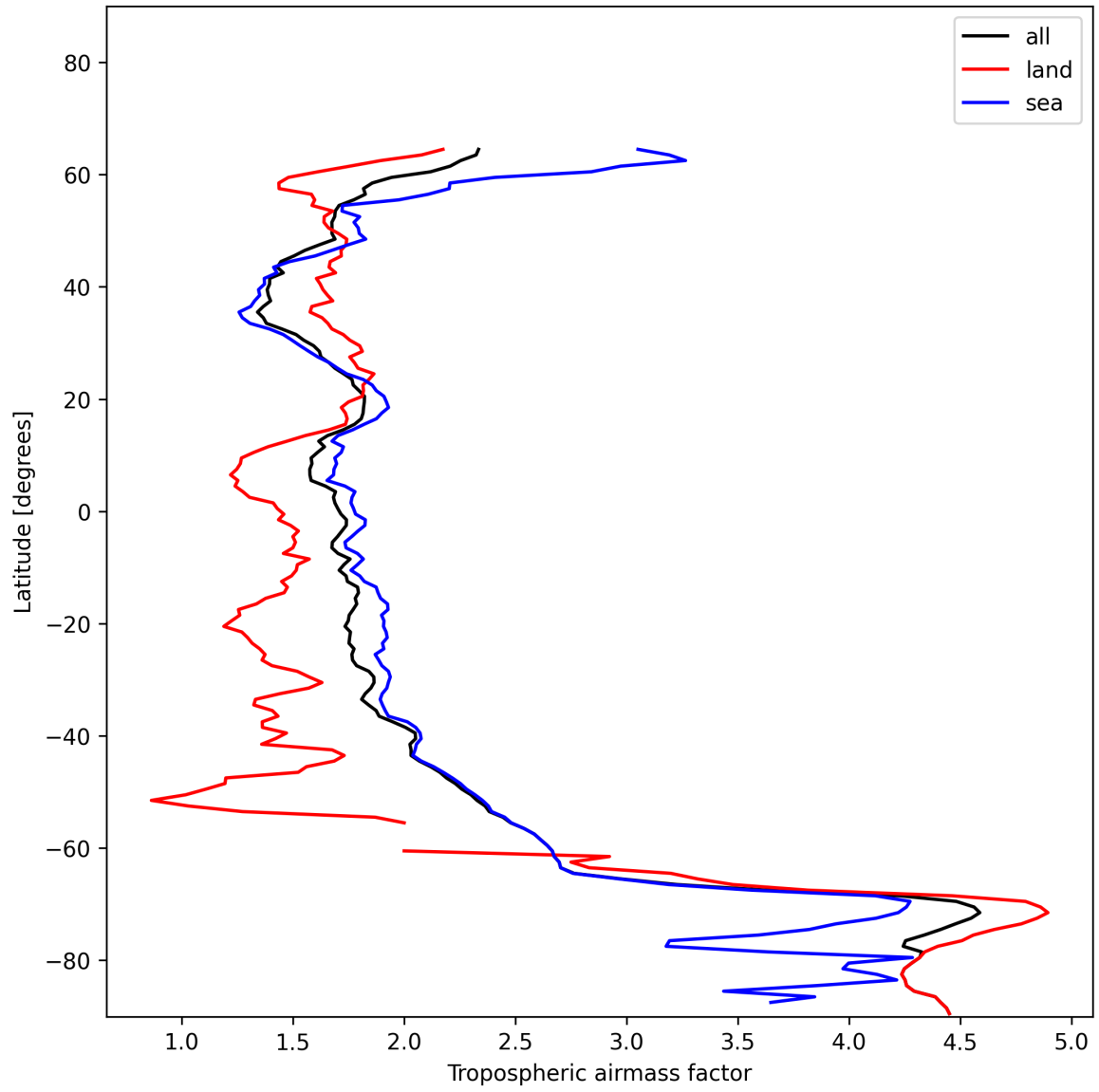
Figure 12: Zonal average of “Tropospheric airmass factor” for 2024-12-20 to 2024-12-20.
