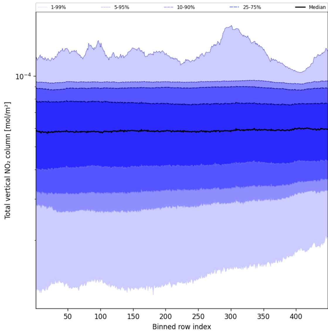
Figure 53: Along track statistics of “Total vertical NO 2 column” for 2024-12-20 to 2024-12-20
