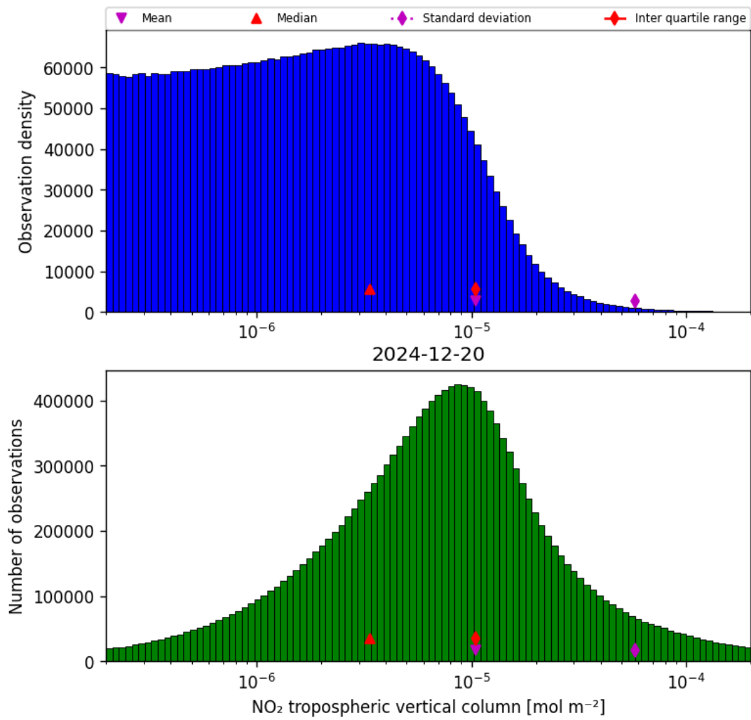
Figure 27: Histogram of “NO 2 tropospheric vertical column” for 2024-12-20 to 2024-12-20
