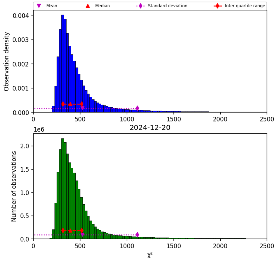
Figure 40: Histogram of “ \chi^2 ” for 2024-12-20 to 2024-12-20
