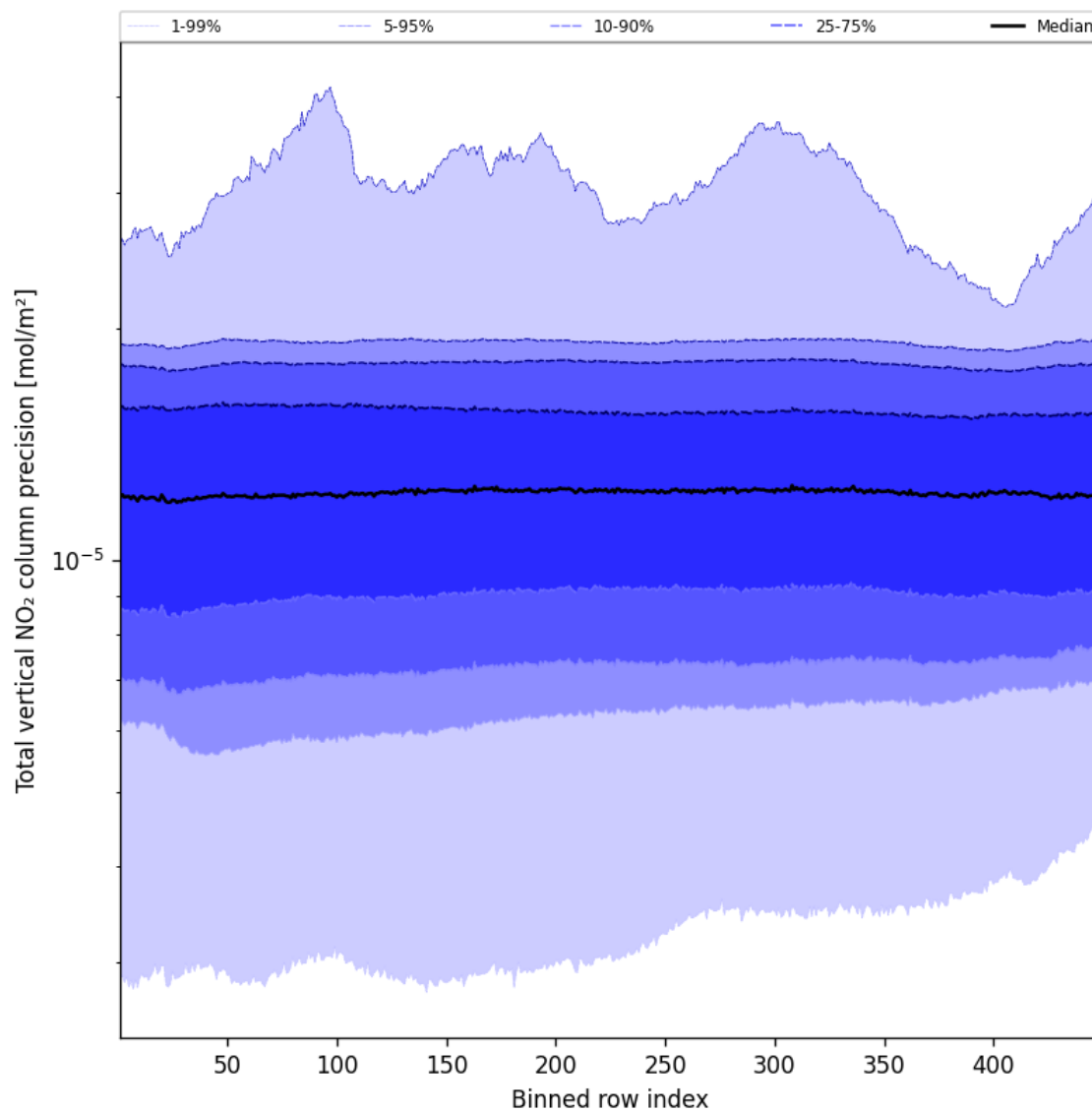
Figure 54: Along track statistics of “Total vertical NO 2 column precision” for 2024-12-20 to 2024-12-20
