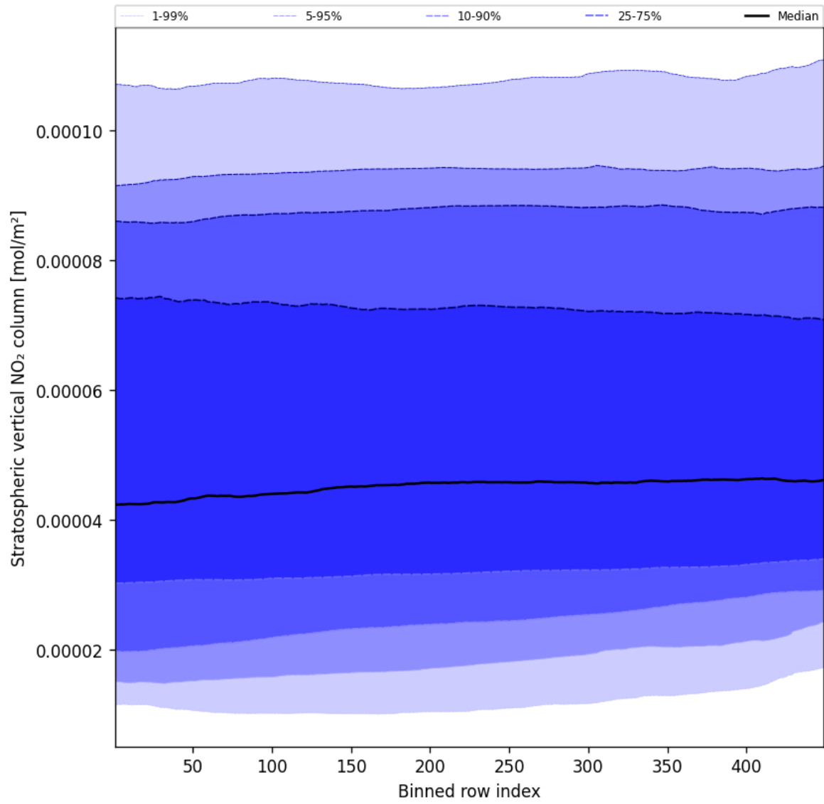
Figure 51: Along track statistics of “Stratospheric vertical NO 2 column” for 2024-12-20 to 2024-12-20
