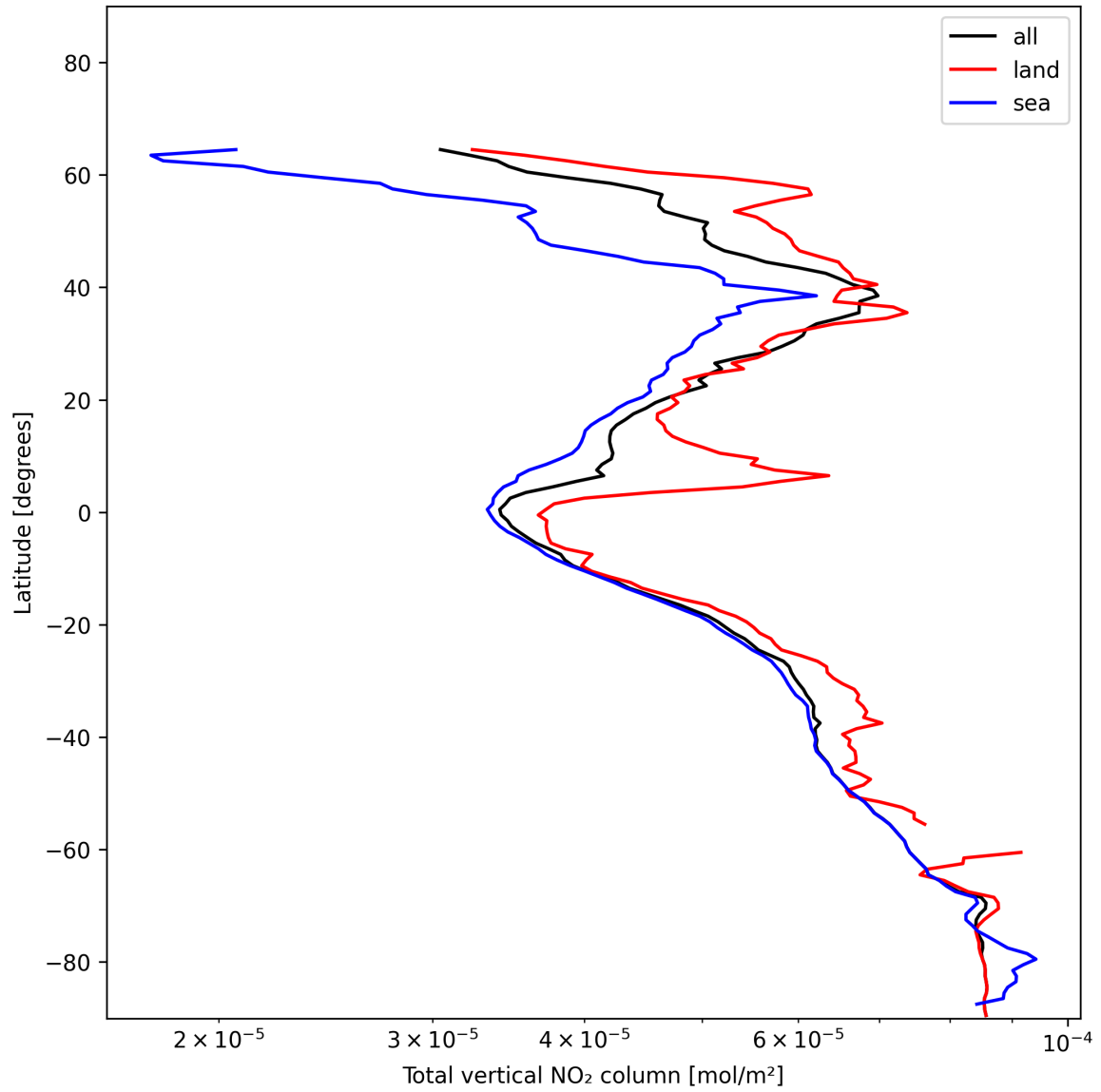
Figure 19: Zonal average of “Total vertical NO 2 column” for 2024-12-20 to 2024-12-20.
