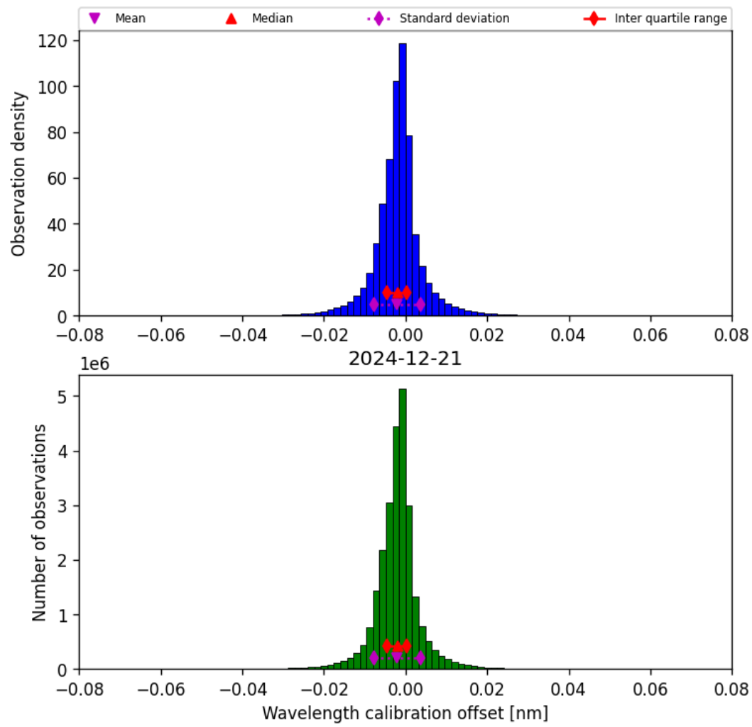
Figure 33: Histogram of “Wavelength calibration offset” for 2024-12-21 to 2024-12-22
