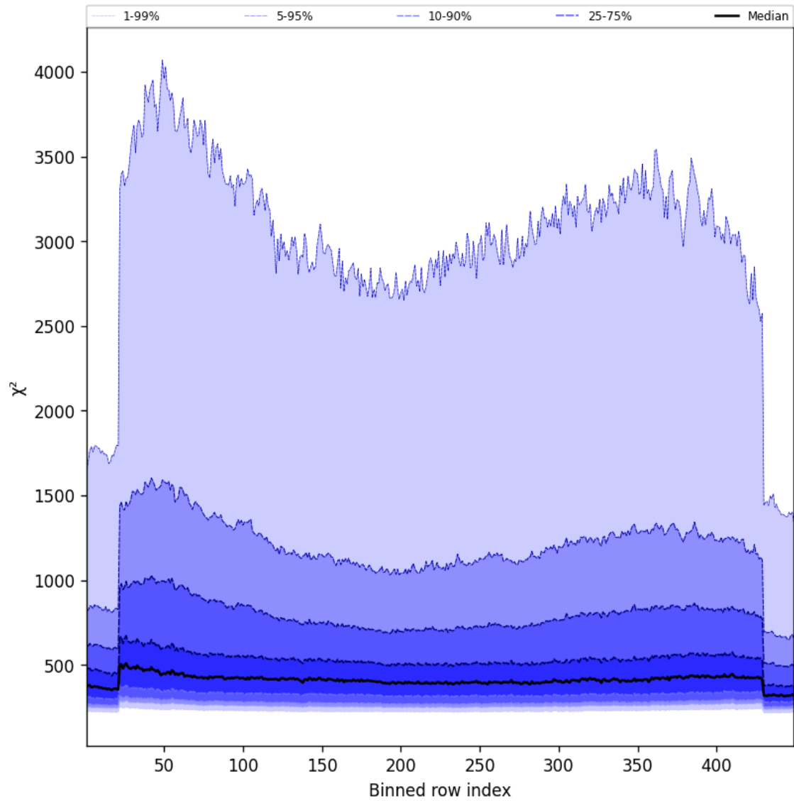
Figure 57: Along track statistics of “ \chi^2 ” for 2024-12-21 to 2024-12-22
