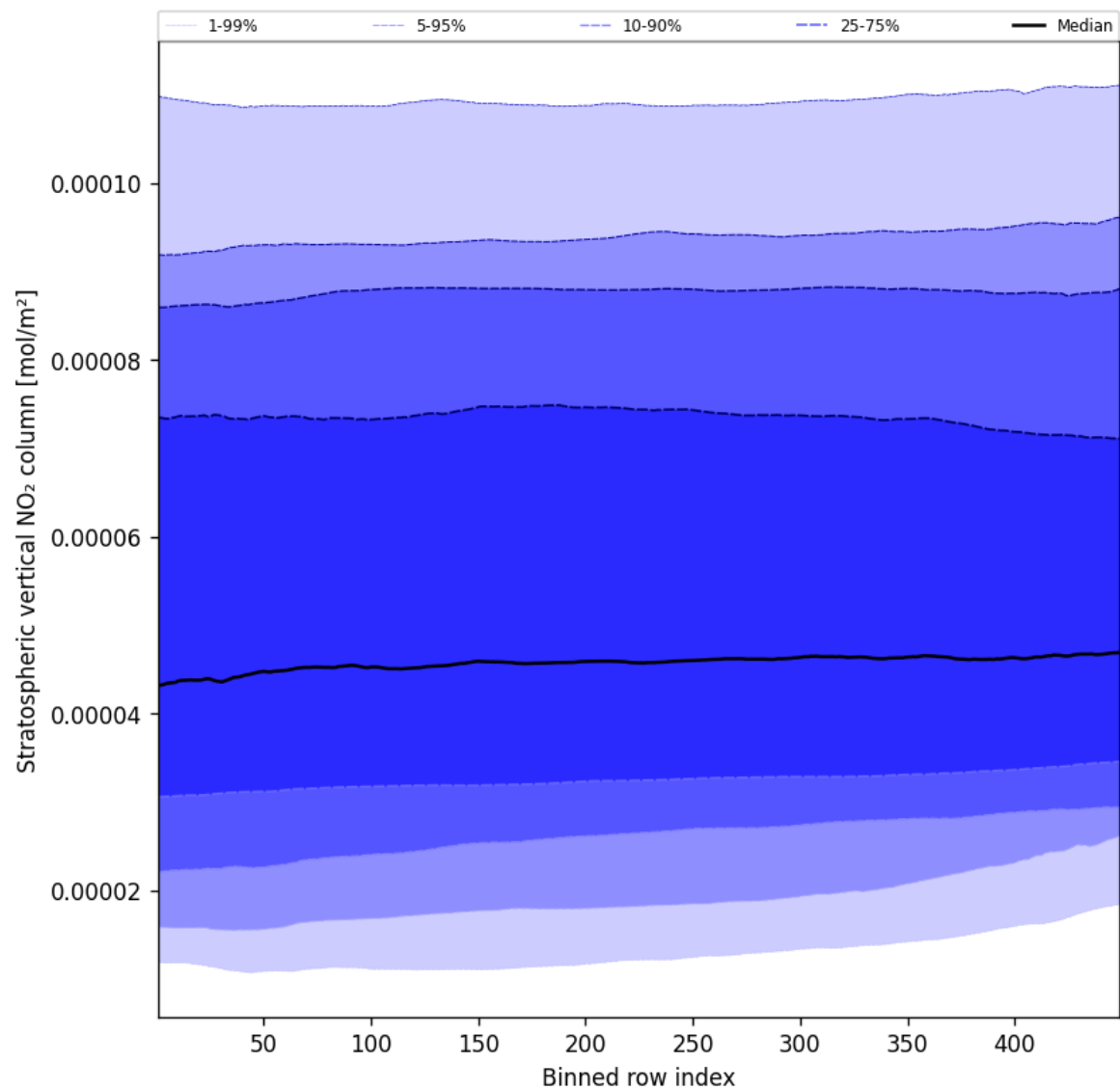
Figure 51: Along track statistics of “Stratospheric vertical NO 2 column” for 2024-12-21 to 2024-12-22
