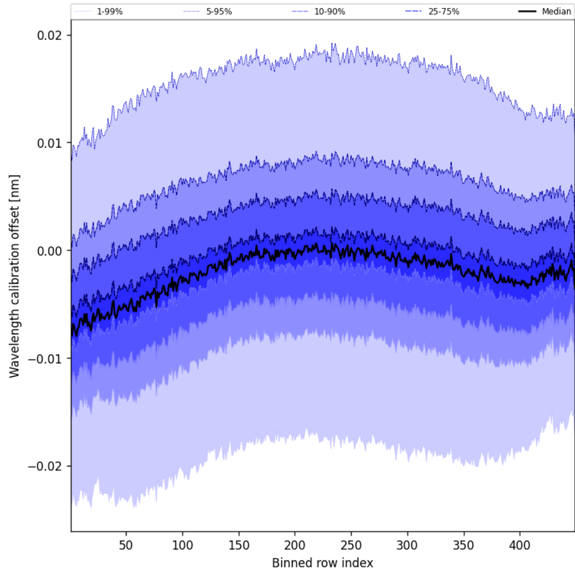
Figure 50: Along track statistics of “Wavelength calibration offset” for 2024-12-21 to 2024-12-22
