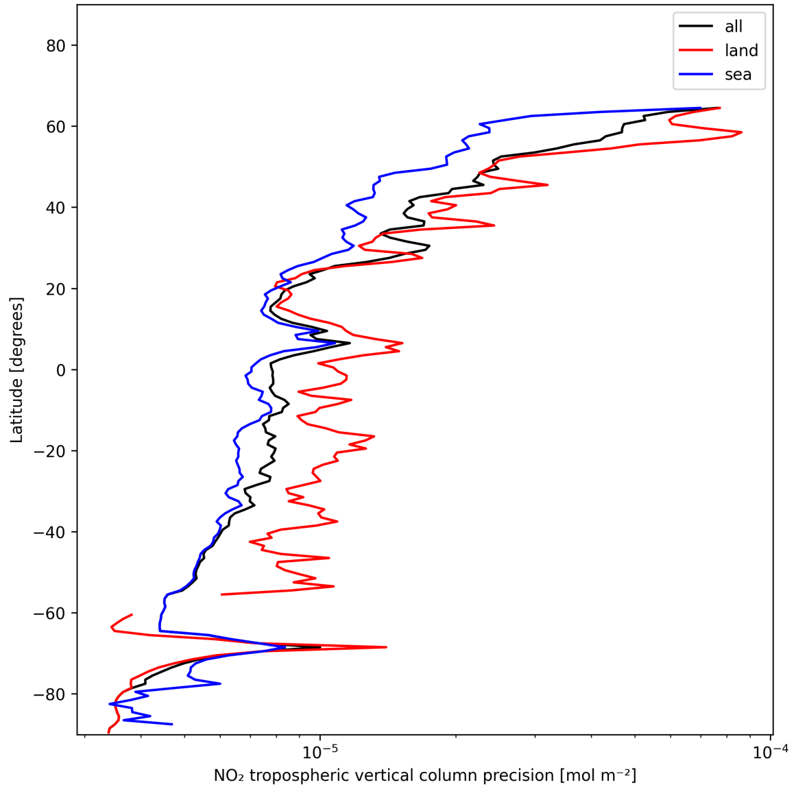
Figure 11: Zonal average of “NO 2 tropospheric vertical column precision” for 2024-12-21 to 2024-12-22.
