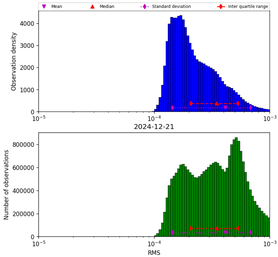
Figure 41: Histogram of “RMS” for 2024-12-21 to 2024-12-22
