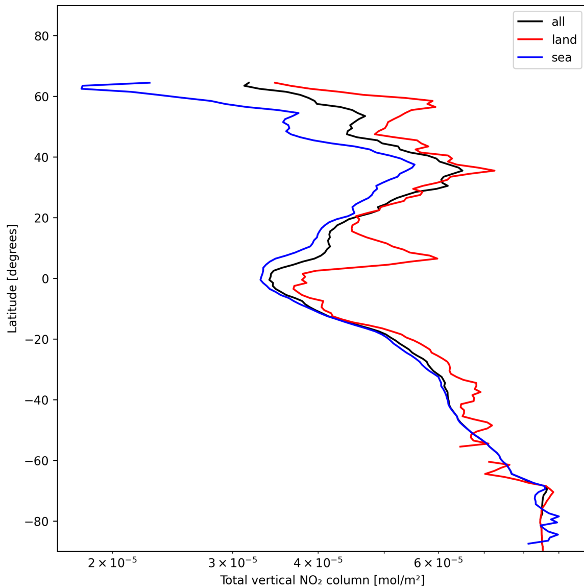
Figure 19: Zonal average of “Total vertical NO 2 column” for 2024-12-21 to 2024-12-22.
