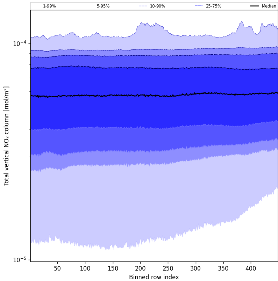
Figure 53: Along track statistics of “Total vertical NO 2 column” for 2024-12-21 to 2024-12-22
