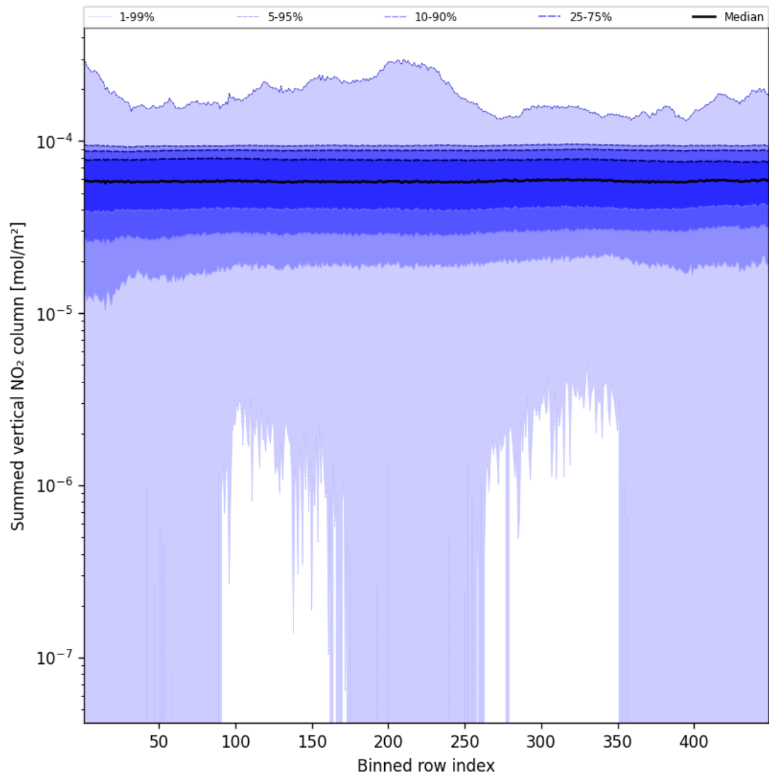
Figure 55: Along track statistics of "Summed vertical NO 2 column" for 2024-12-21 to 2024-12-22
