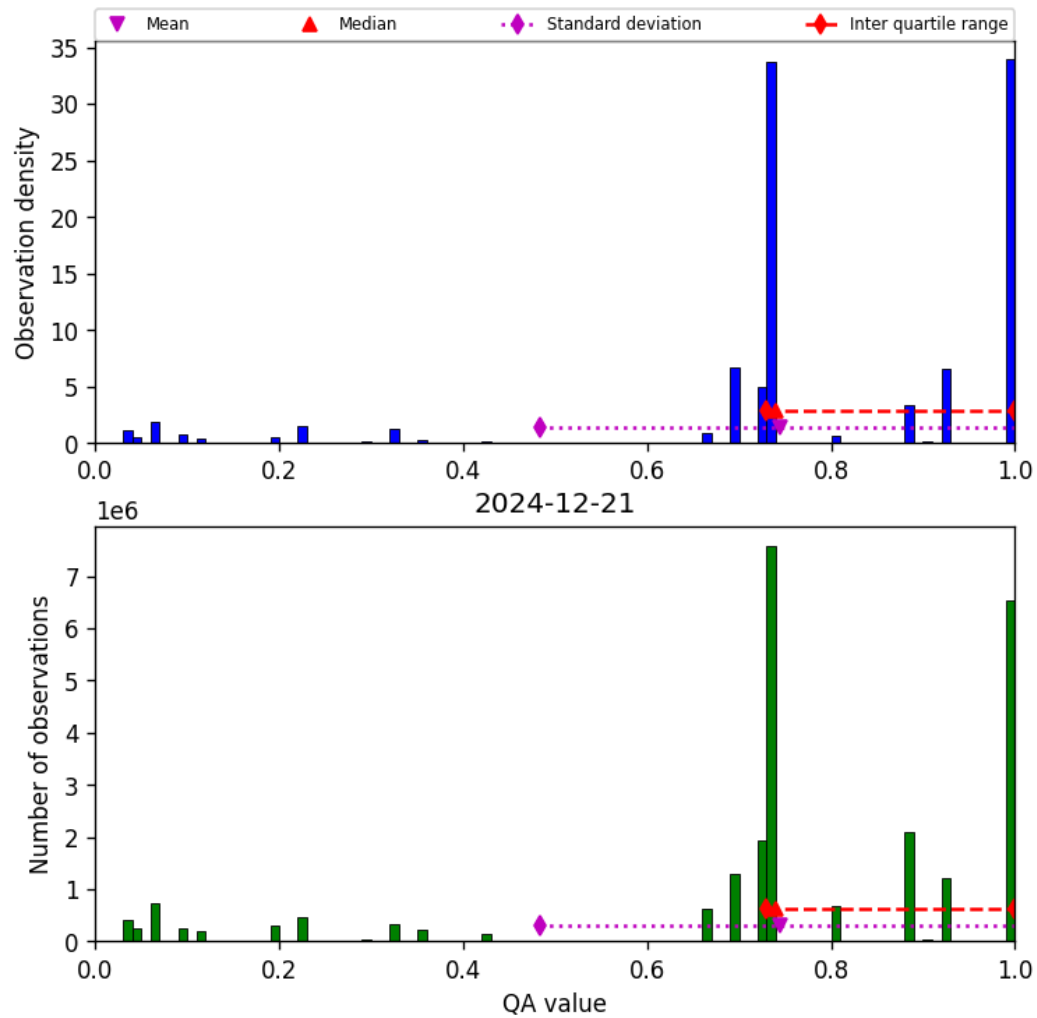
Figure 26: Histogram of “QA value” for 2024-12-21 to 2024-12-22
