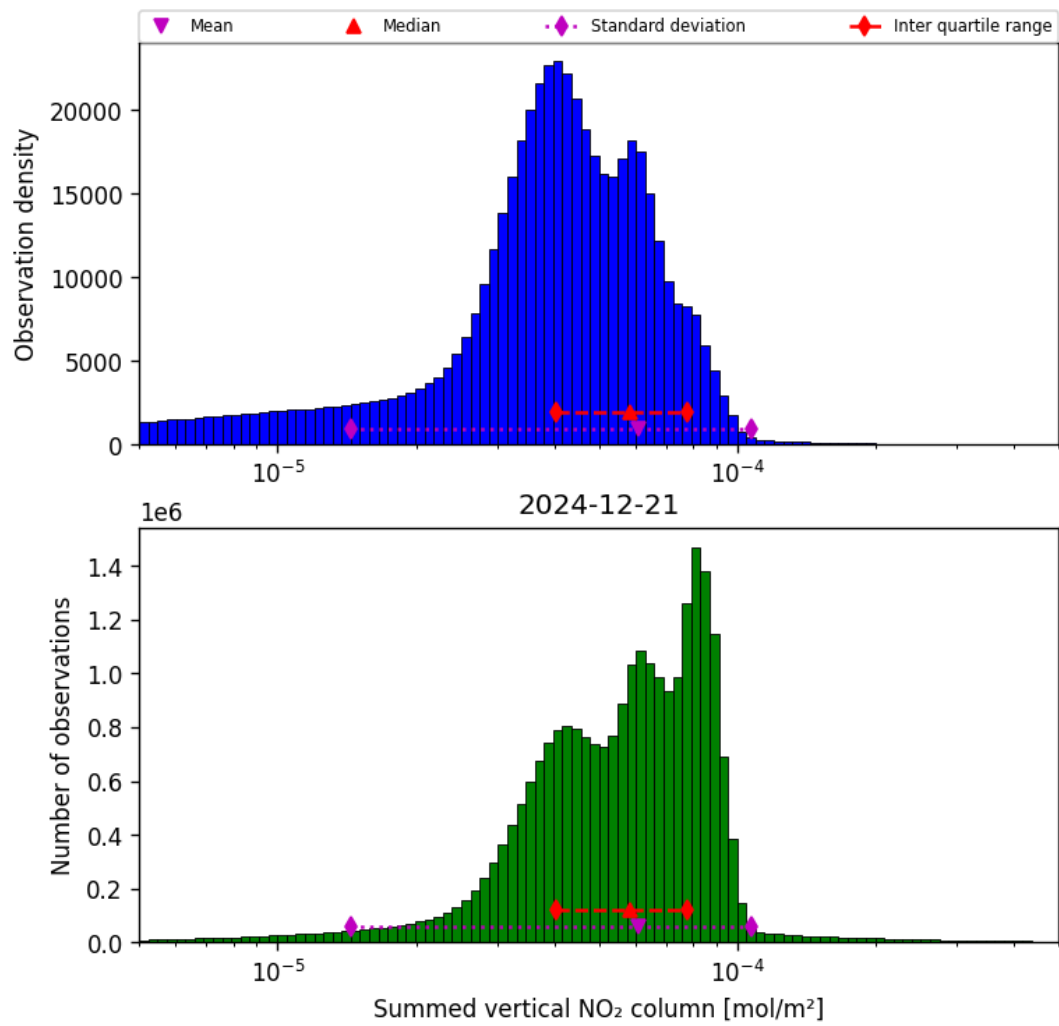
Figure 38: Histogram of “Summed vertical NO 2 column” for 2024-12-21 to 2024-12-22
