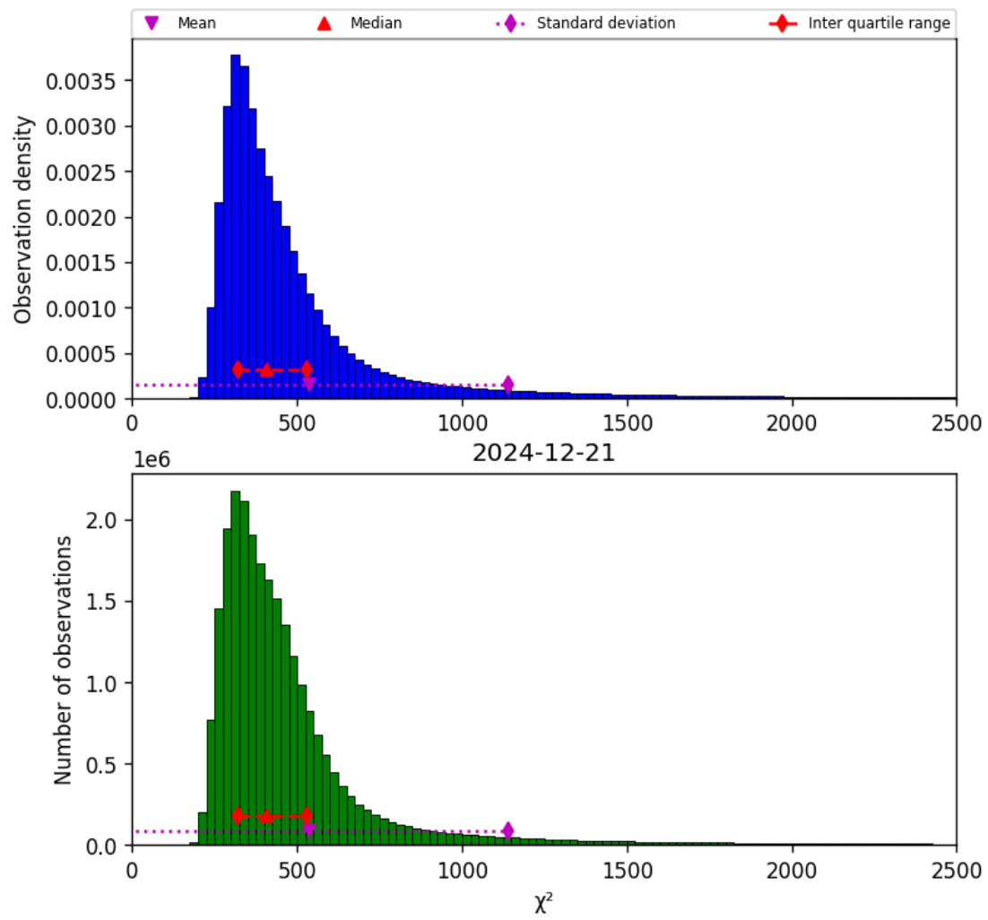
Figure 40: Histogram of “ \chi^2 ” for 2024-12-21 to 2024-12-22
