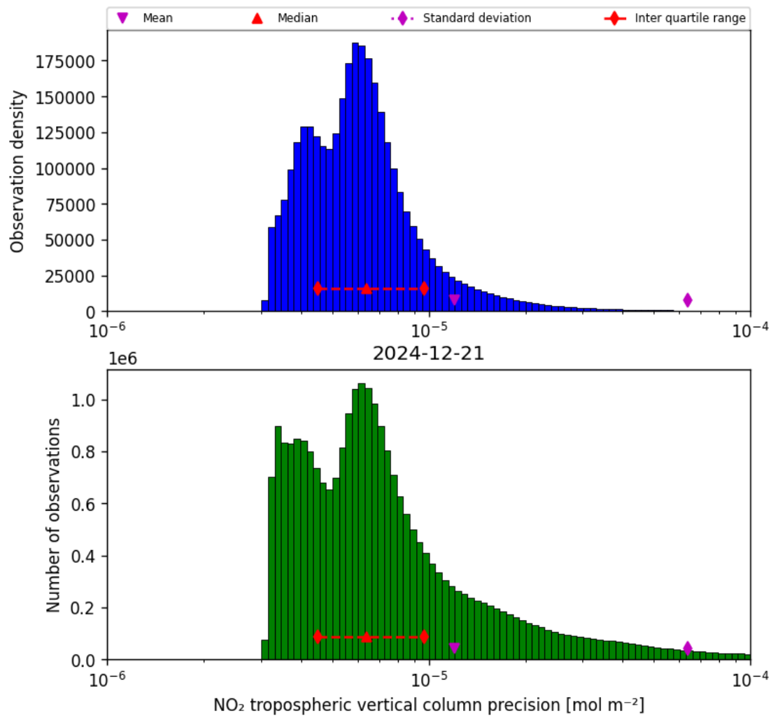
Figure 28: Histogram of “NO 2 tropospheric vertical column precision” for 2024-12-21 to 2024-12-22
