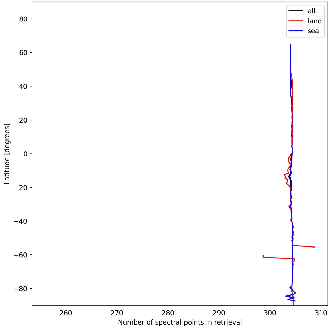
Figure 14: Zonal average of “Number of spectral points in retrieval” for 2024-12-21 to 2024-12-22.
