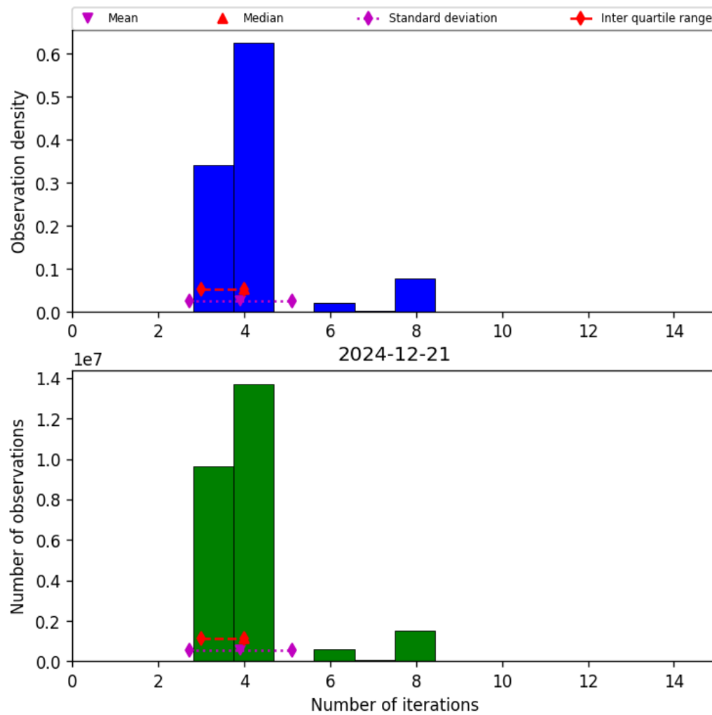
Figure 32: Histogram of “Number of iterations” for 2024-12-21 to 2024-12-22
