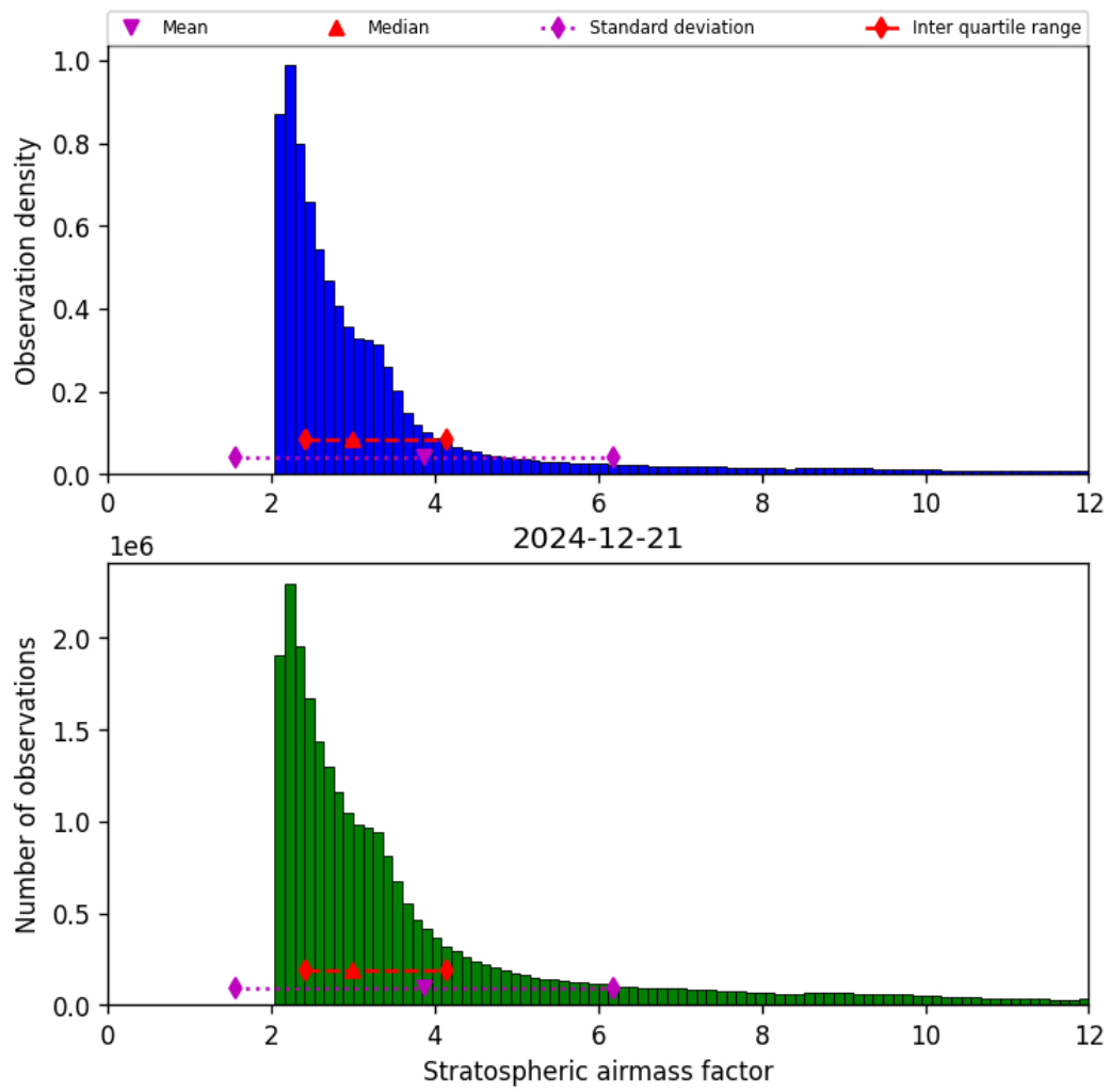
Figure 42: Histogram of “Stratospheric airmass factor” for 2024-12-21 to 2024-12-22
