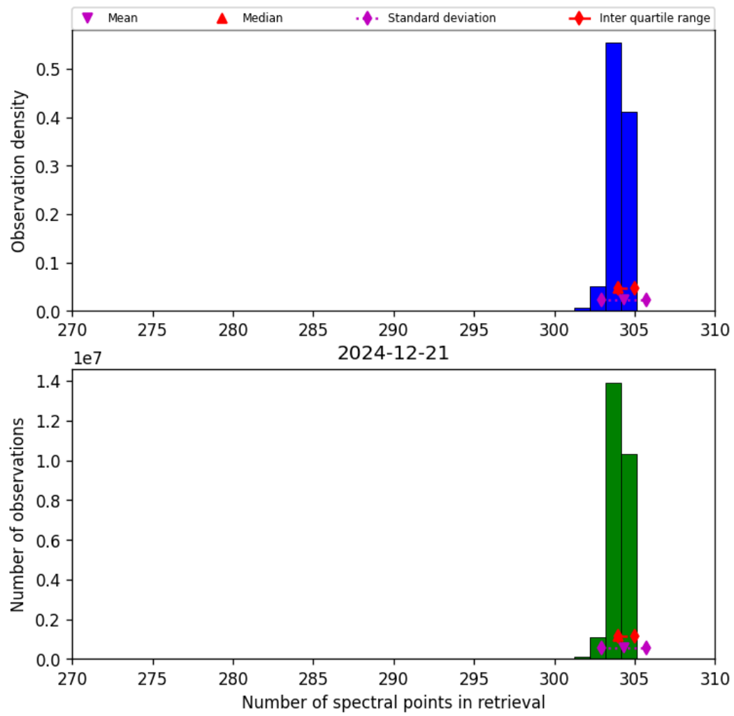
Figure 31: Histogram of “Number of spectral points in retrieval” for 2024-12-21 to 2024-12-22
