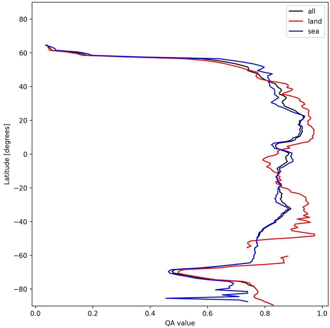
Figure 9: Zonal average of “QA value” for 2024-12-21 to 2024-12-22.
