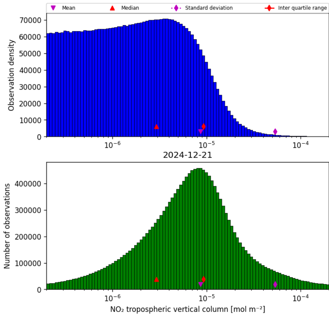
Figure 27: Histogram of “NO 2 tropospheric vertical column” for 2024-12-21 to 2024-12-22
