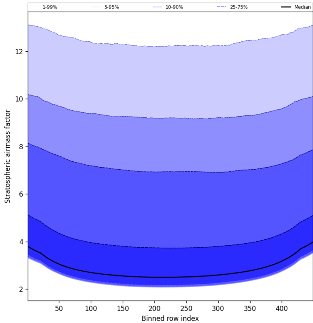
Figure 59: Along track statistics of “Stratospheric airmass factor” for 2024-12-21 to 2024-12-22
