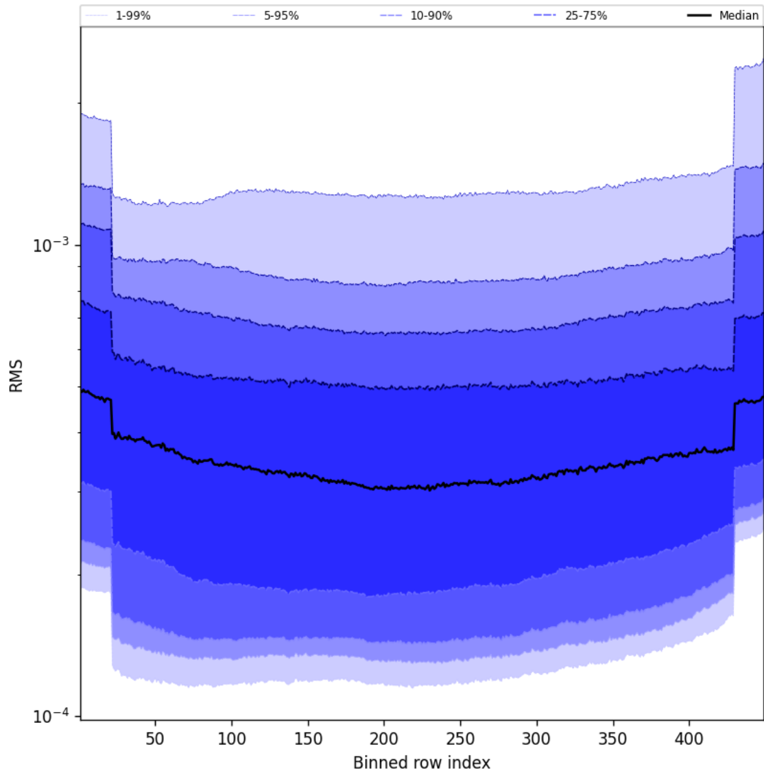
Figure 58: Along track statistics of “RMS” for 2024-12-21 to 2024-12-22
