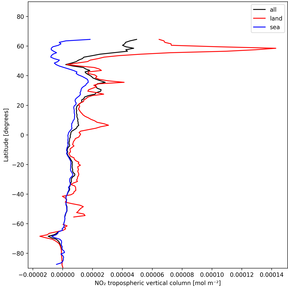
Figure 10: Zonal average of “NO 2 tropospheric vertical column” for 2024-12-21 to 2024-12-22.
