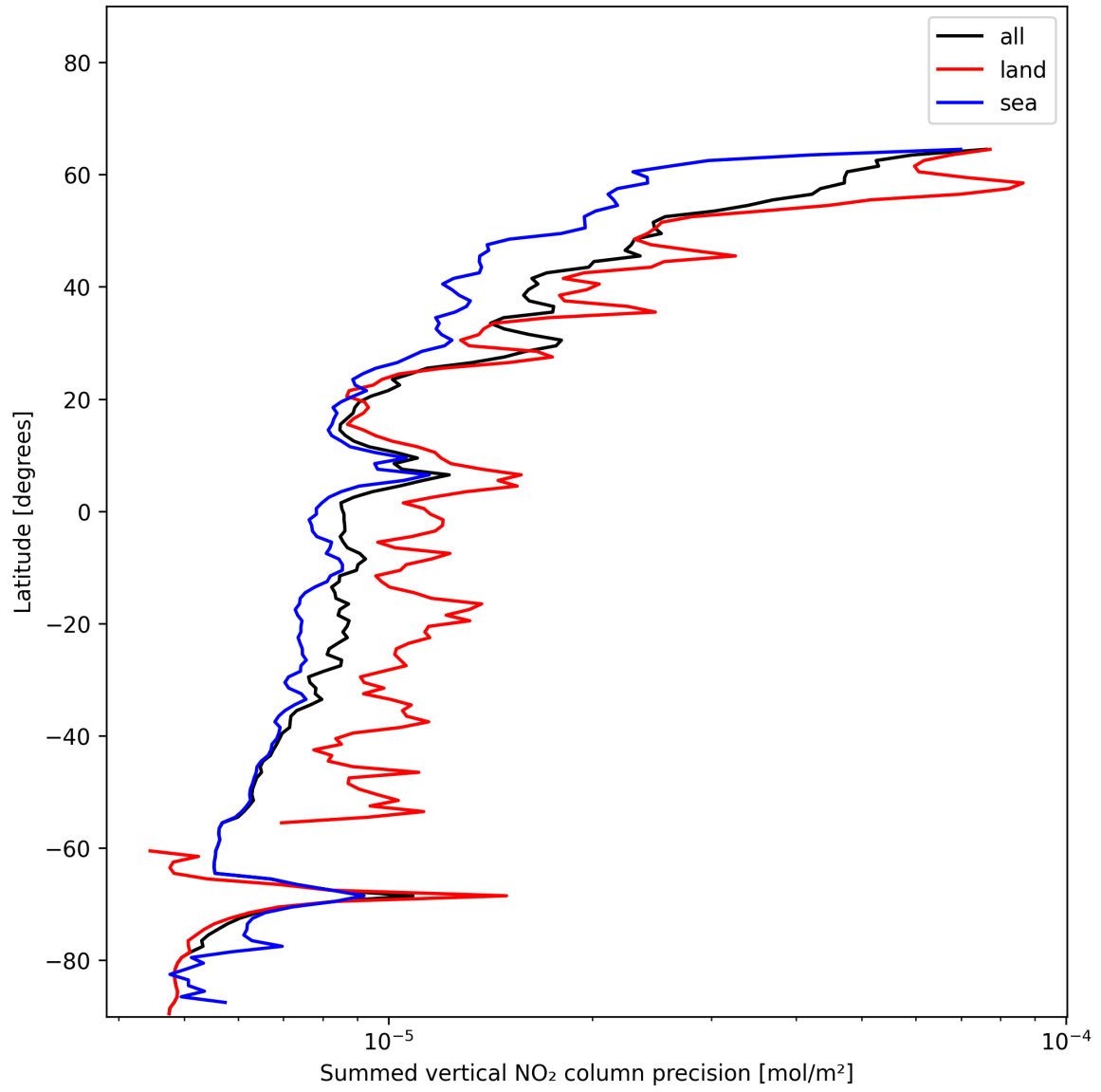
Figure 22: Zonal average of “Summed vertical NO 2 column precision” for 2024-12-21 to 2024-12-22.
