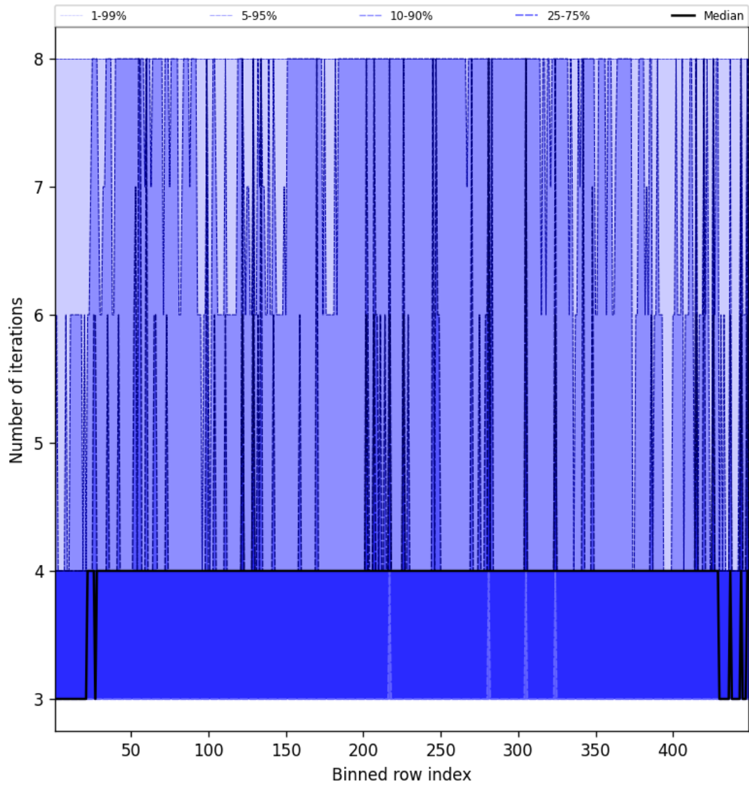
Figure 49: Along track statistics of “Number of iterations” for 2024-12-21 to 2024-12-22
