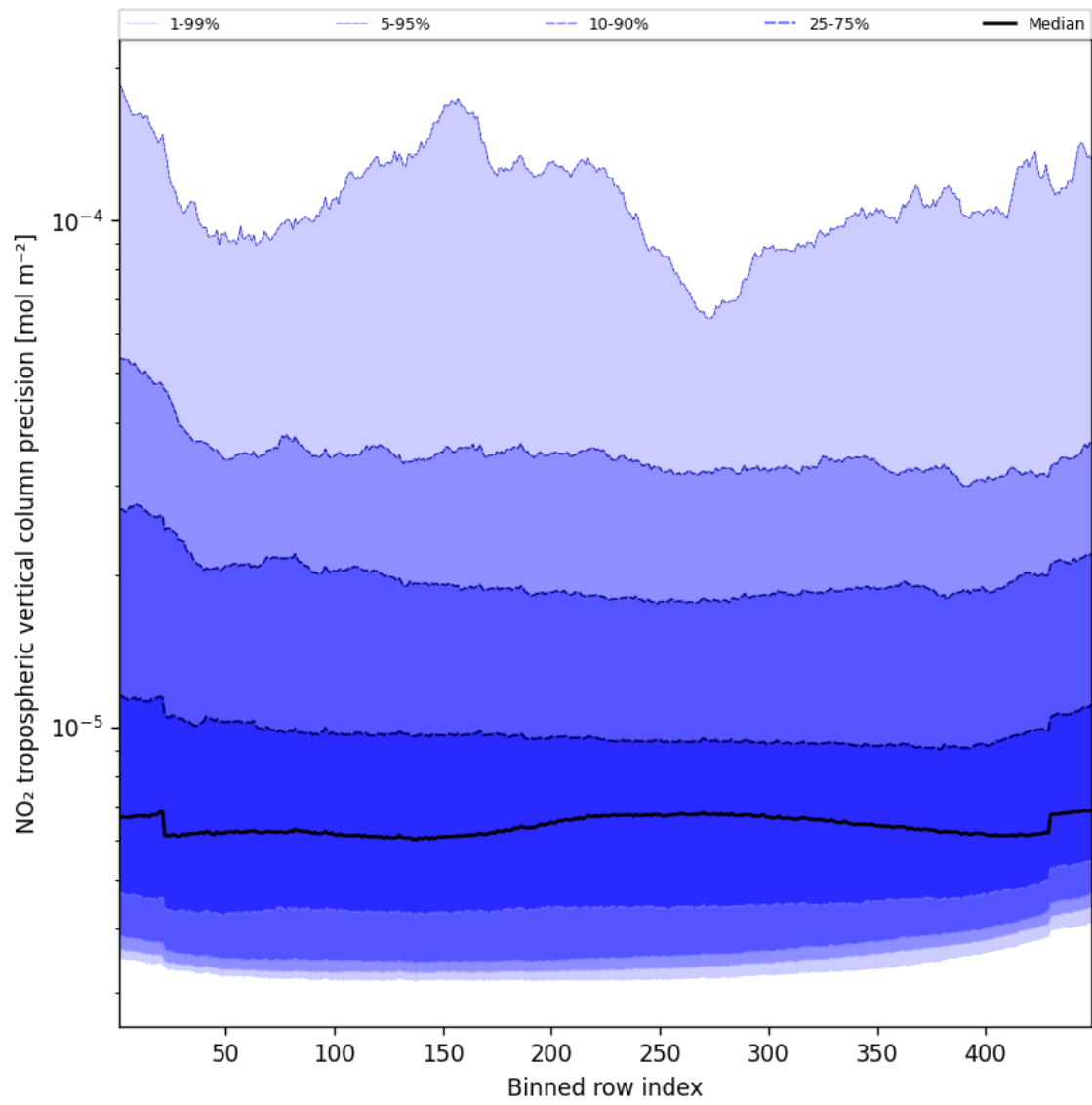
Figure 45: Along track statistics of “NO 2 tropospheric vertical column precision” for 2024-12-21 to 2024-12-22
