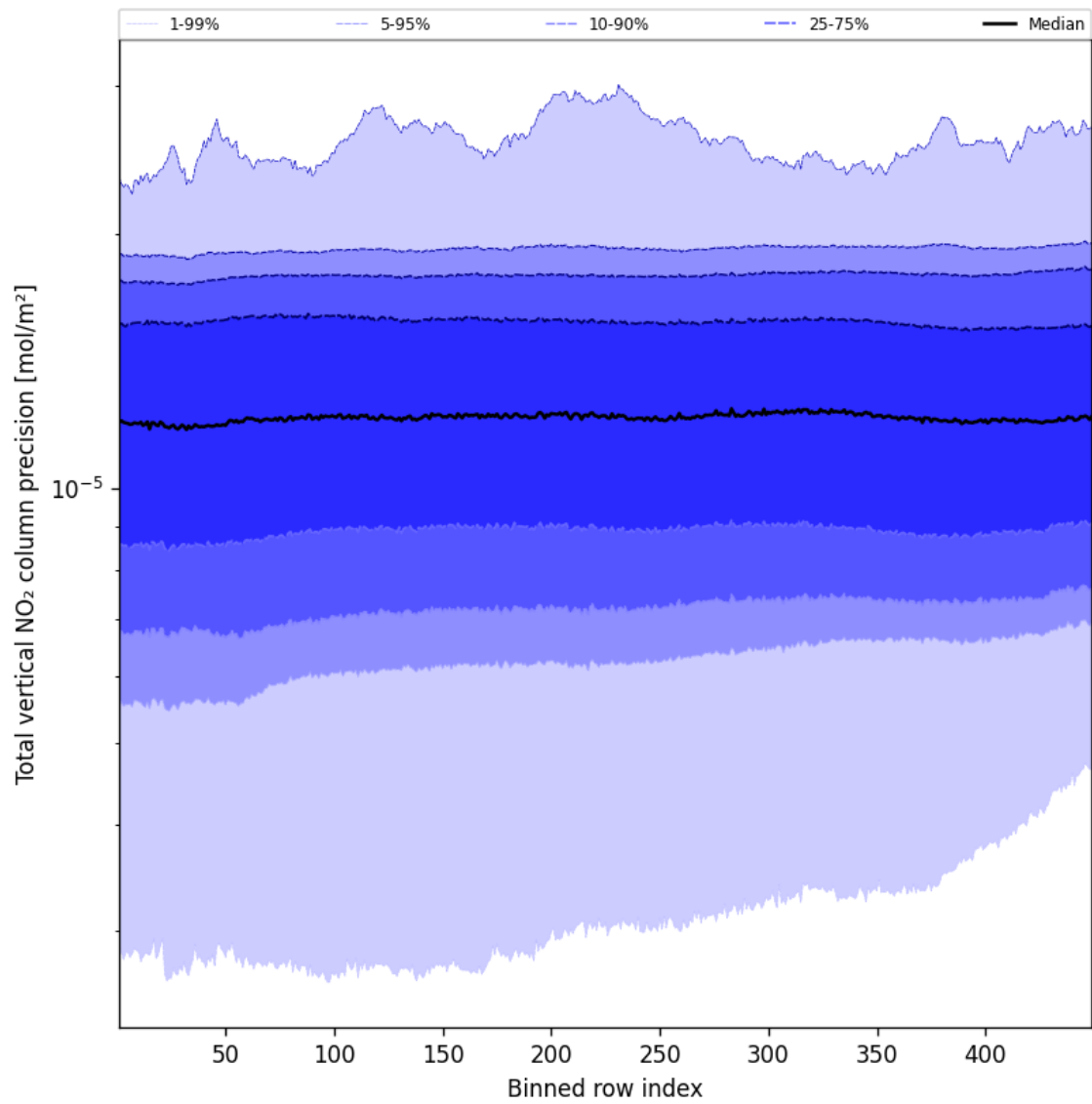
Figure 54: Along track statistics of “Total vertical NO 2 column precision” for 2024-12-21 to 2024-12-22
