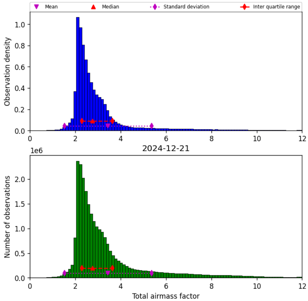
Figure 30: Histogram of “Total airmass factor” for 2024-12-21 to 2024-12-22
