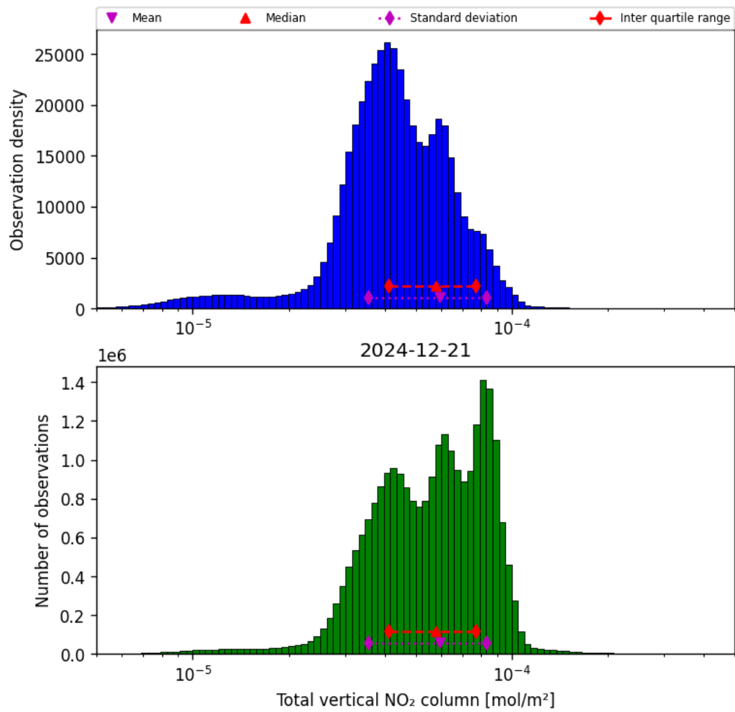
Figure 36: Histogram of “Total vertical NO 2 column” for 2024-12-21 to 2024-12-22
