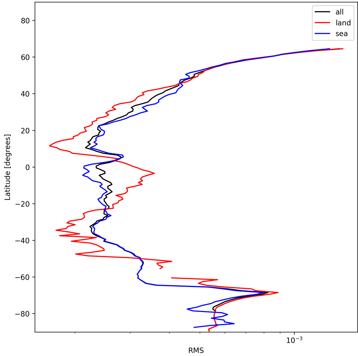
Figure 24: Zonal average of “RMS” for 2024-12-21 to 2024-12-22.
