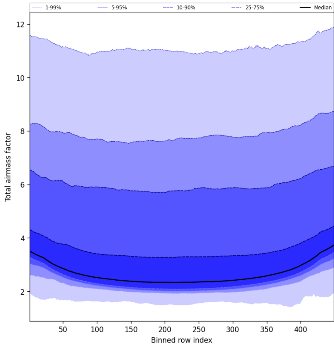
Figure 47: Along track statistics of “Total airmass factor” for 2024-12-21 to 2024-12-22
