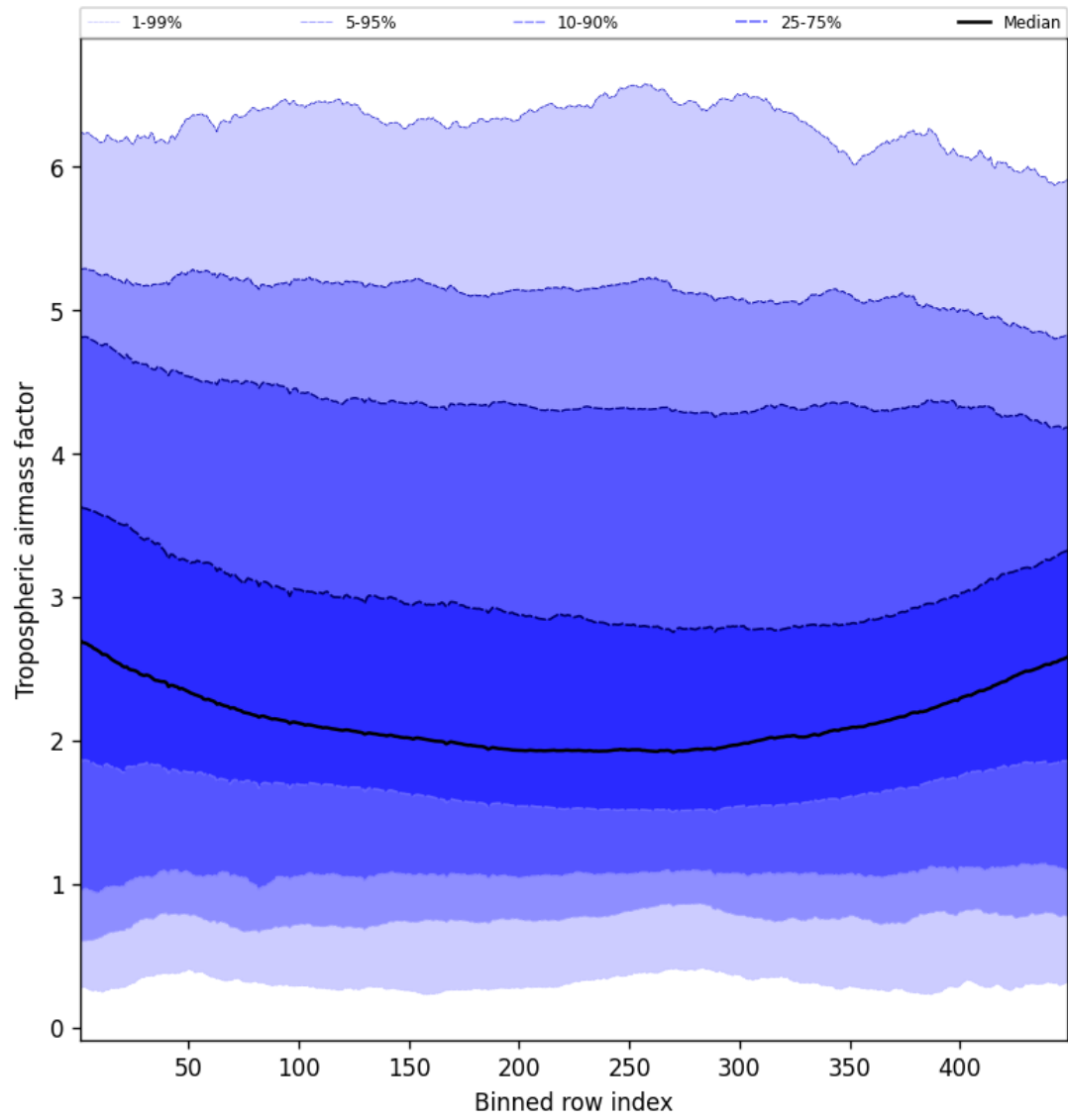
Figure 46: Along track statistics of “Tropospheric airmass factor” for 2024-12-21 to 2024-12-22
