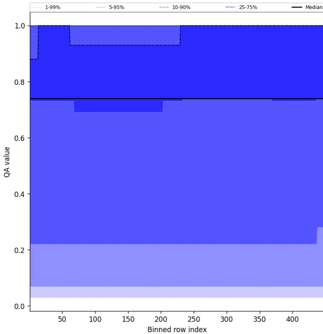
Figure 43: Along track statistics of “QA value” for 2024-12-21 to 2024-12-22
