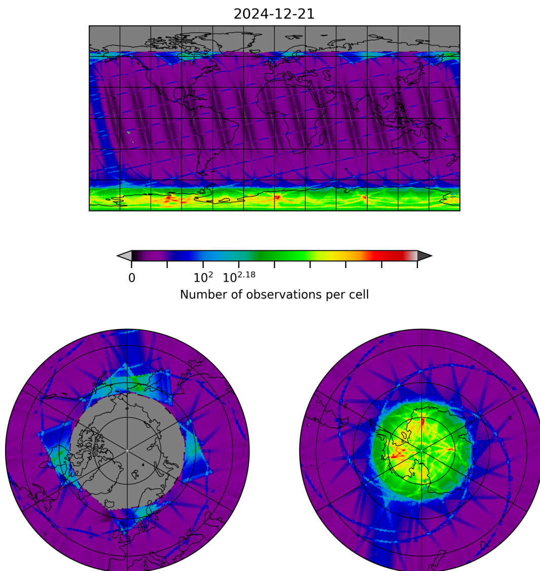
Figure 8: Map of the number of observations for 2024-12-21 to 2024-12-22
