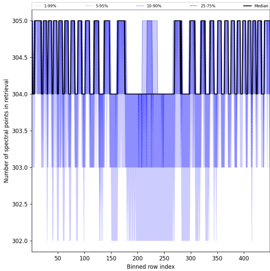
Figure 48: Along track statistics of “Number of spectral points in retrieval” for 2024-12-21 to 2024-12-22
