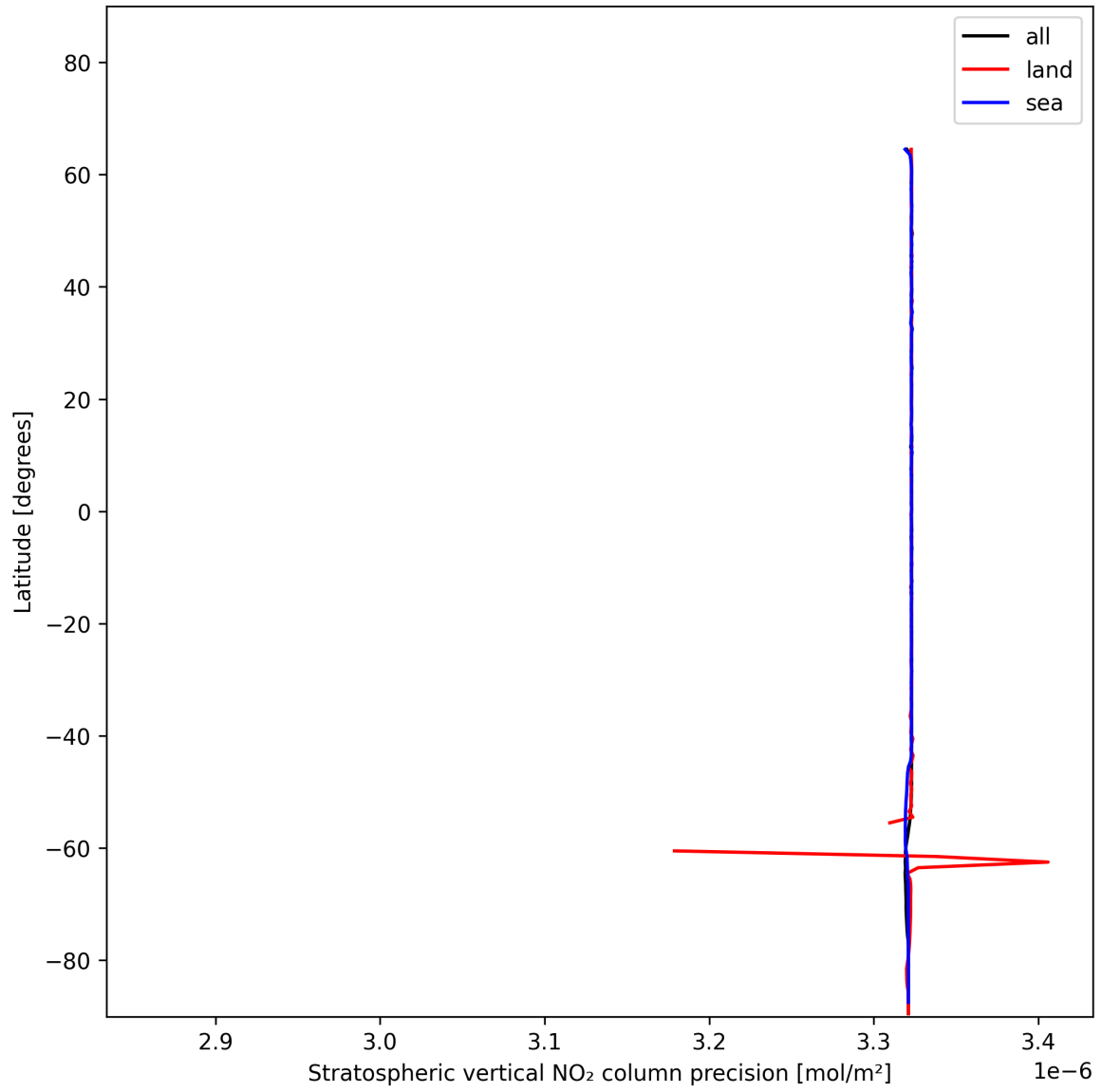
Figure 18: Zonal average of “Stratospheric vertical NO 2 column precision” for 2024-12-21 to 2024-12-22.
