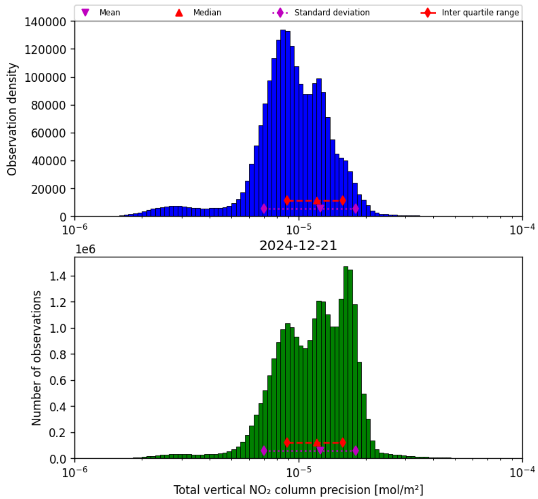
Figure 37: Histogram of “Total vertical NO 2 column precision” for 2024-12-21 to 2024-12-22
