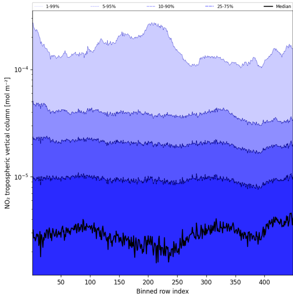
Figure 44: Along track statistics of “NO 2 tropospheric vertical column” for 2024-12-21 to 2024-12-22
