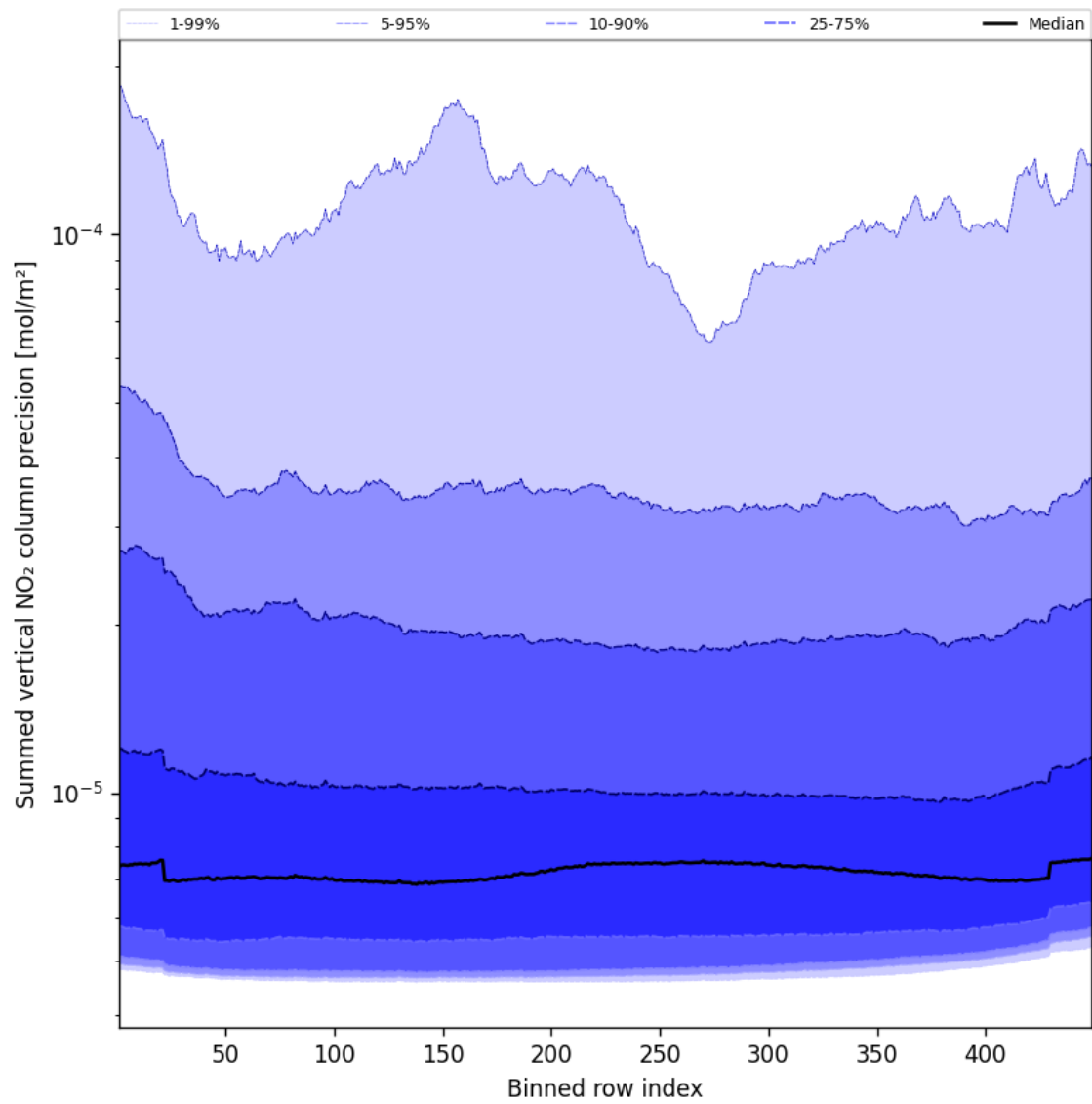
Figure 56: Along track statistics of “Summed vertical NO 2 column precision” for 2024-12-21 to 2024-12-22
