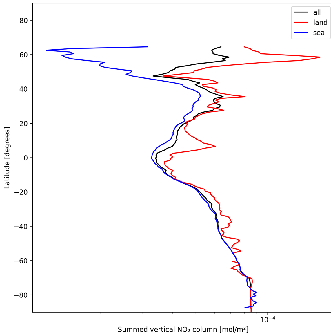
Figure 21: Zonal average of “Summed vertical NO 2 column” for 2024-12-21 to 2024-12-22.
