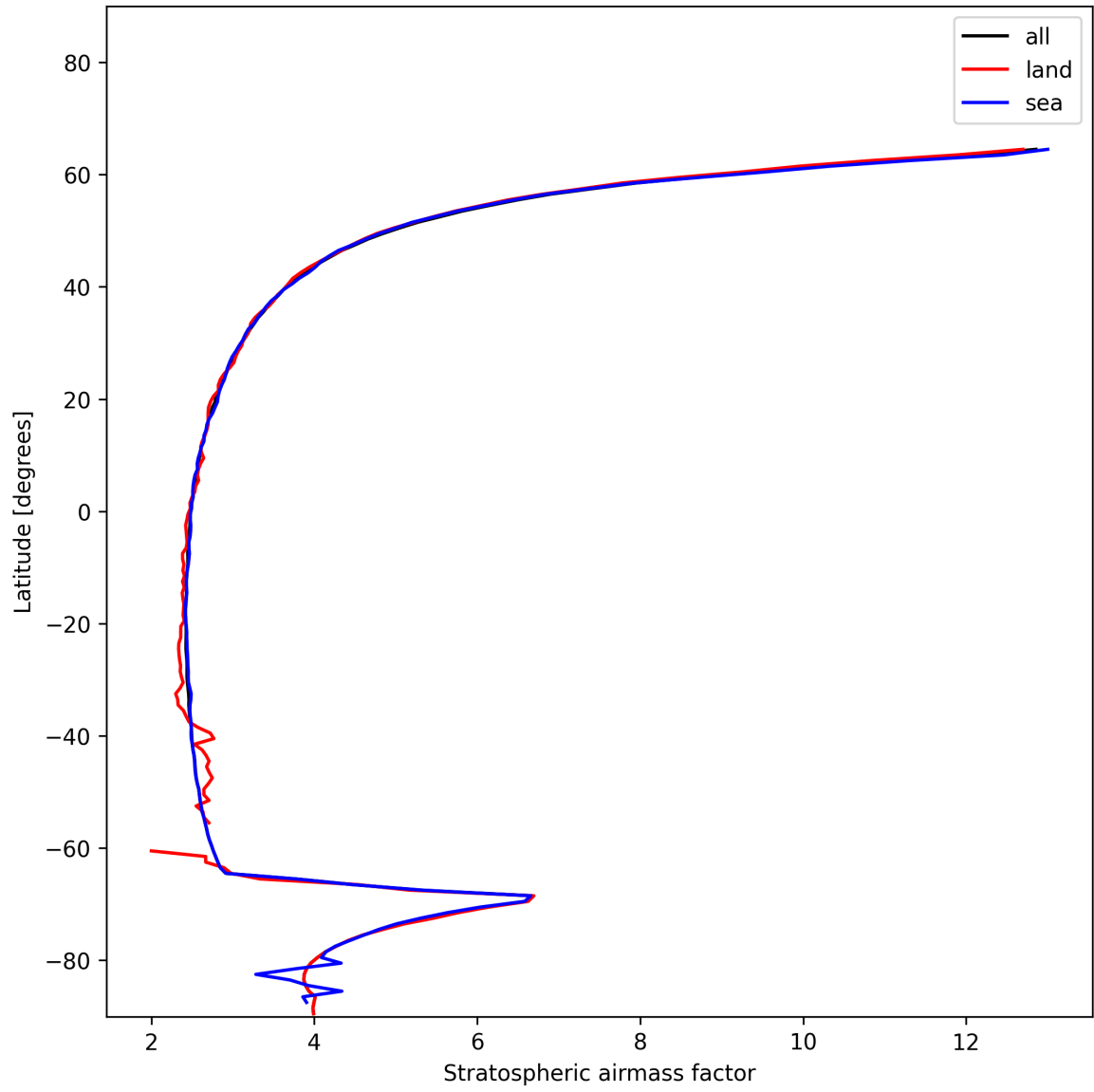
Figure 25: Zonal average of “Stratospheric airmass factor” for 2024-12-21 to 2024-12-22.
