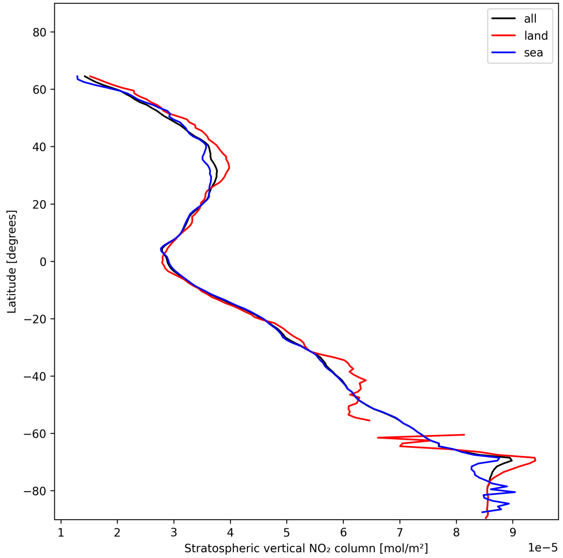
Figure 17: Zonal average of “Stratospheric vertical NO 2 column” for 2024-12-21 to 2024-12-22.
