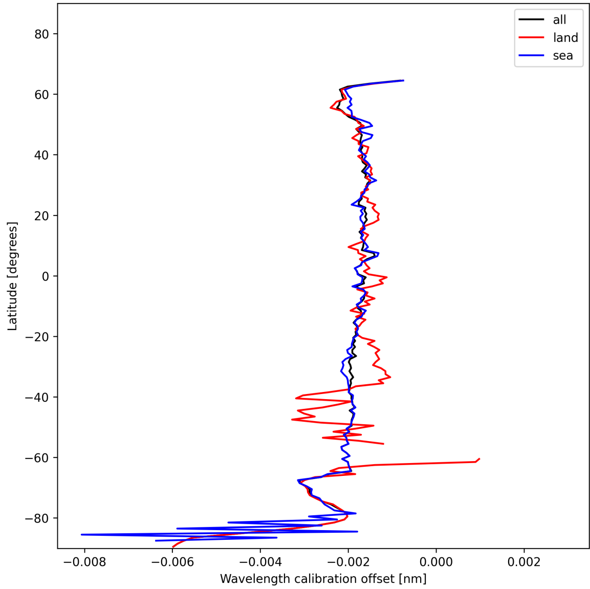
Figure 16: Zonal average of “Wavelength calibration offset” for 2024-12-21 to 2024-12-22.
