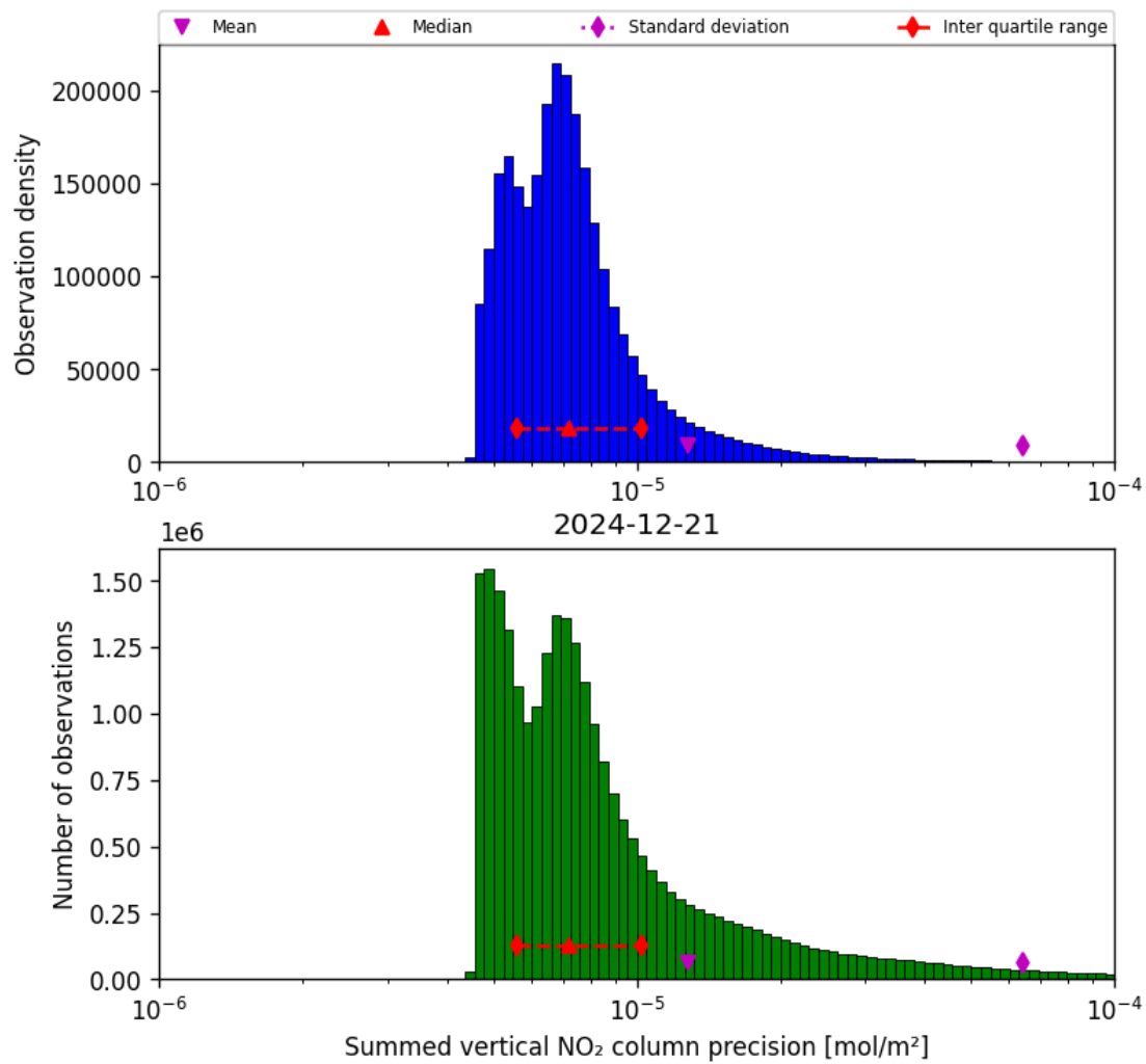
Figure 39: Histogram of “Summed vertical NO 2 column precision” for 2024-12-21 to 2024-12-22
