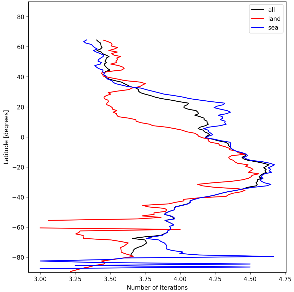
Figure 15: Zonal average of “Number of iterations” for 2024-12-21 to 2024-12-22.
