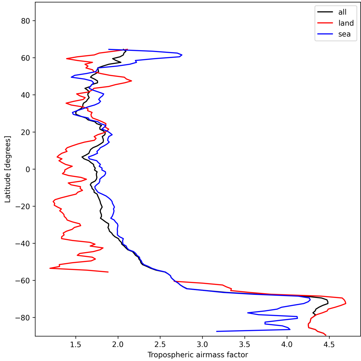
Figure 12: Zonal average of “Tropospheric airmass factor” for 2024-12-21 to 2024-12-22.
