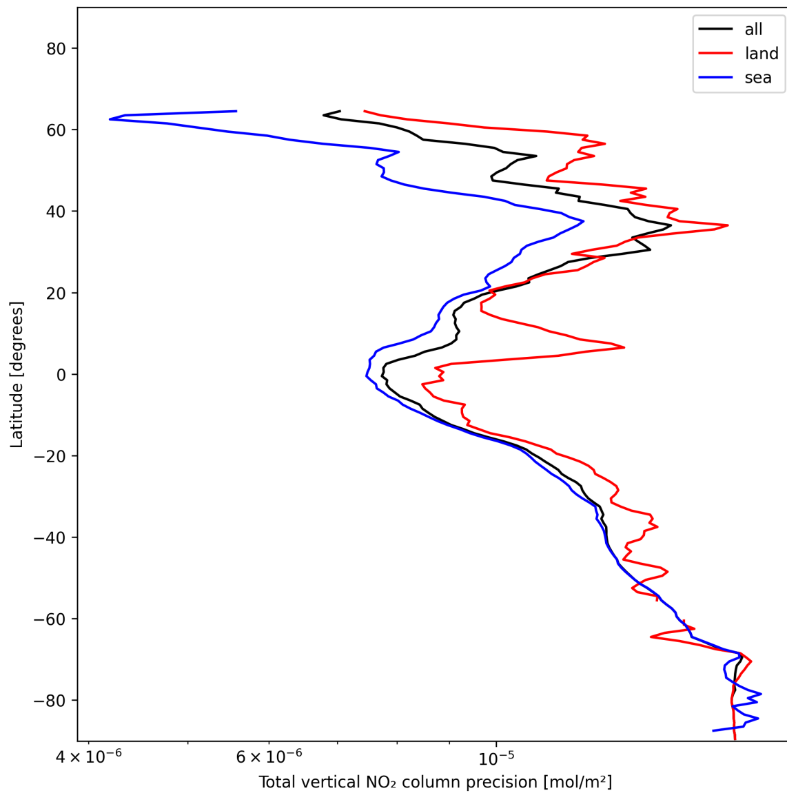
Figure 20: Zonal average of “Total vertical NO 2 column precision” for 2024-12-21 to 2024-12-22.
