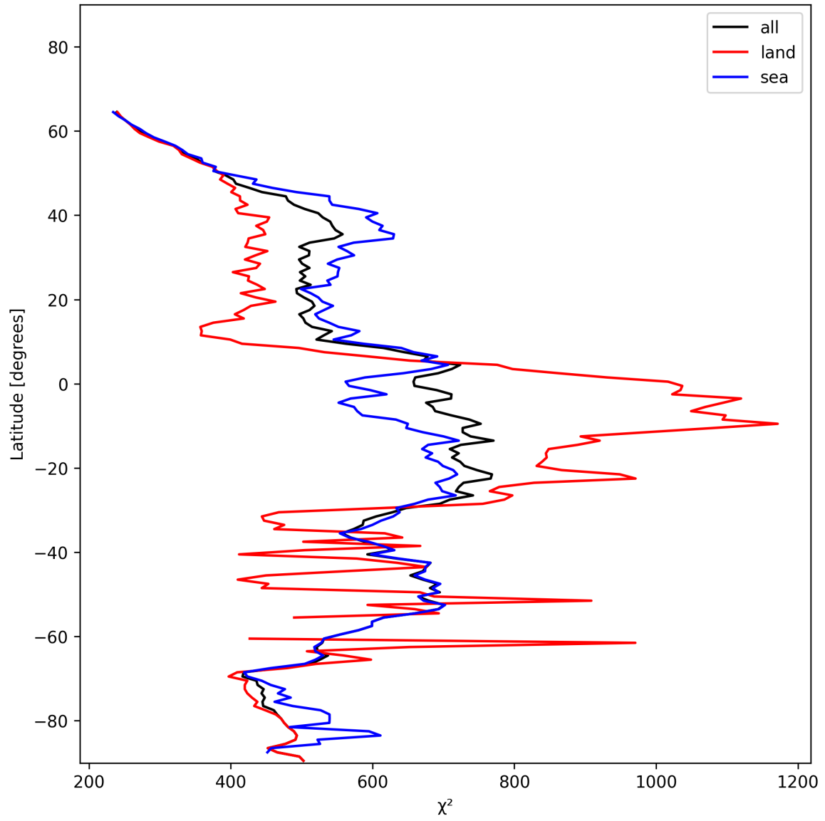
Figure 23: Zonal average of “ \chi^2 ” for 2024-12-21 to 2024-12-22.
