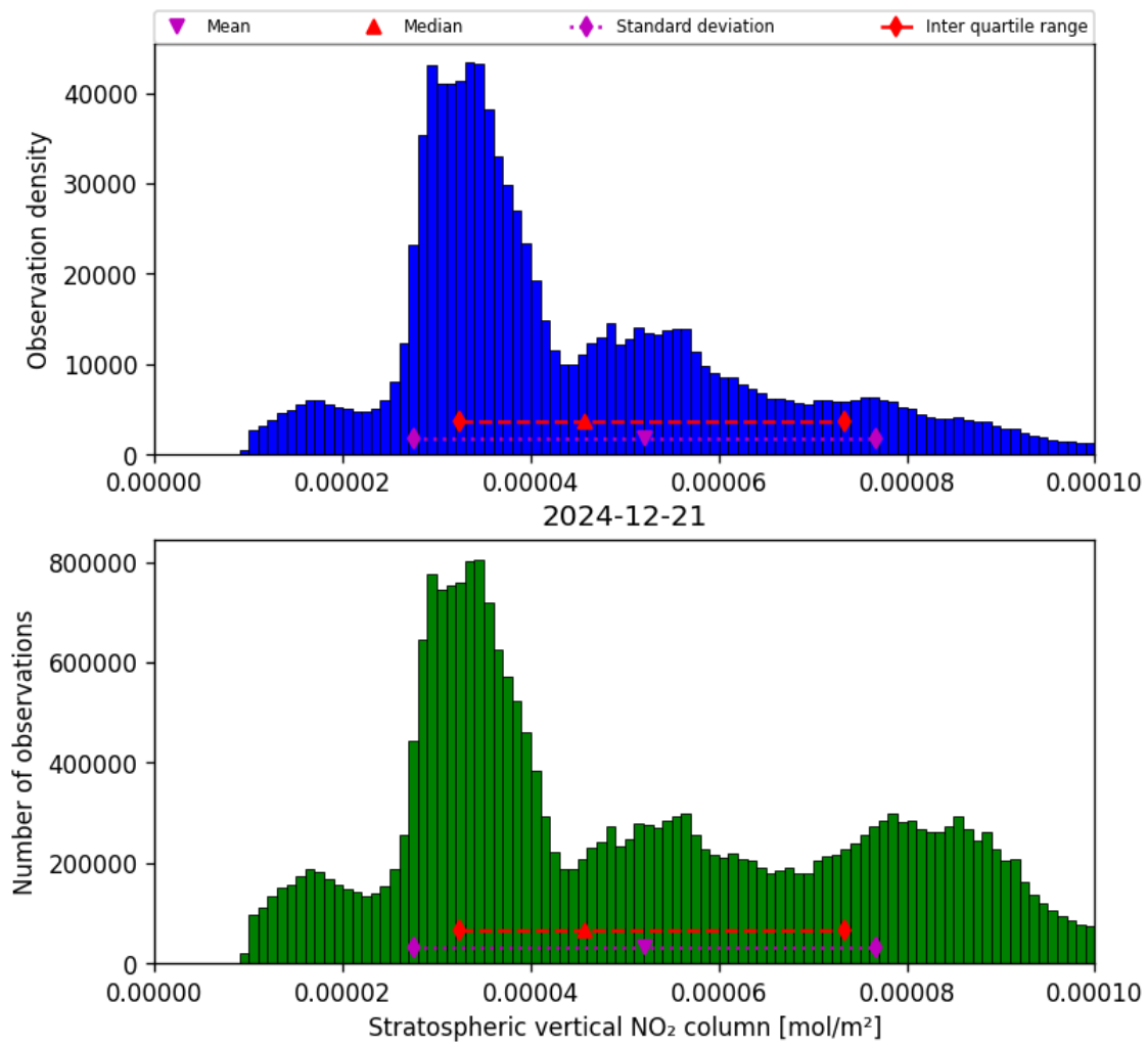
Figure 34: Histogram of “Stratospheric vertical NO 2 column” for 2024-12-21 to 2024-12-22
