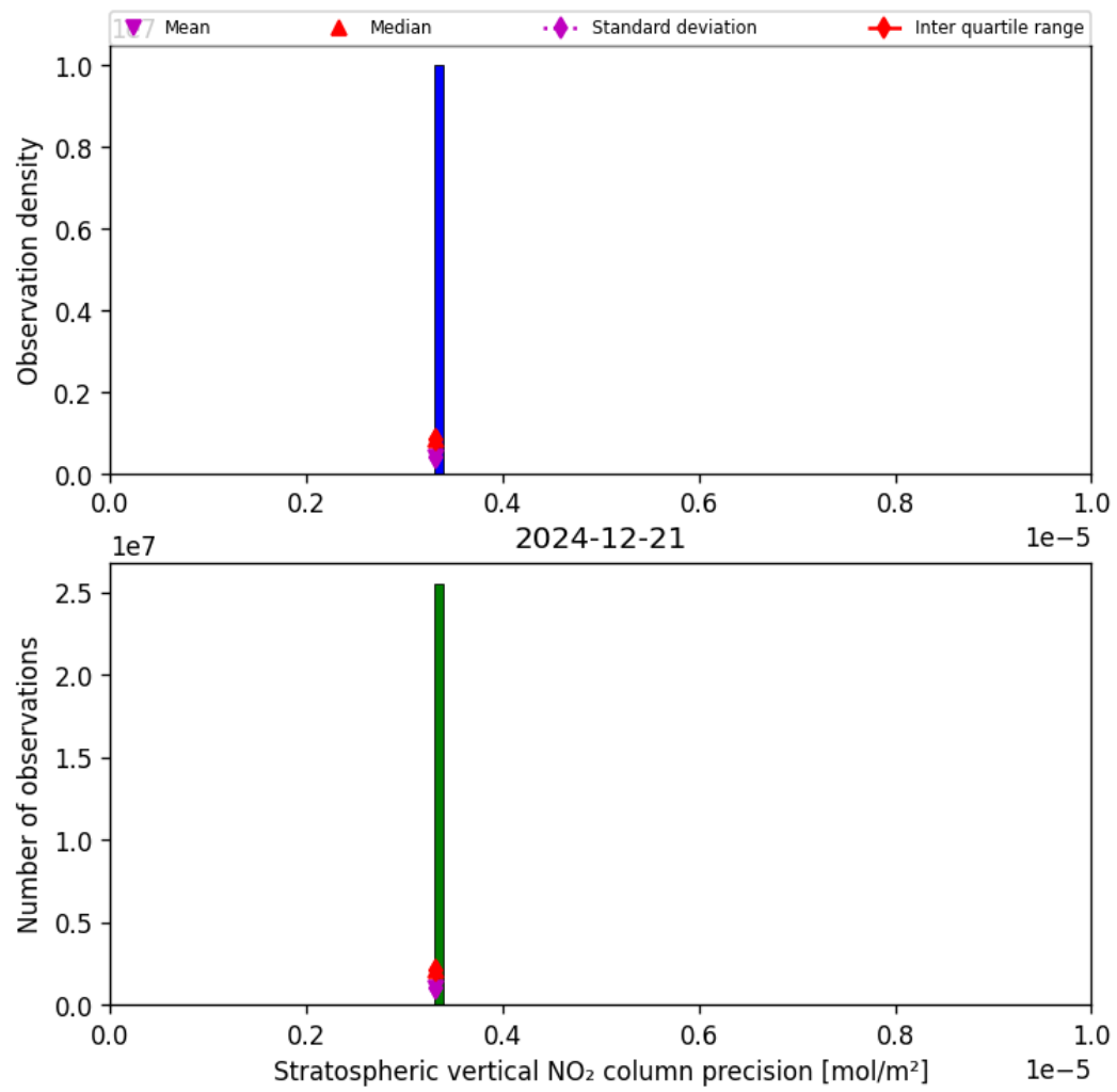
Figure 35: Histogram of “Stratospheric vertical NO 2 column precision” for 2024-12-21 to 2024-12-22
