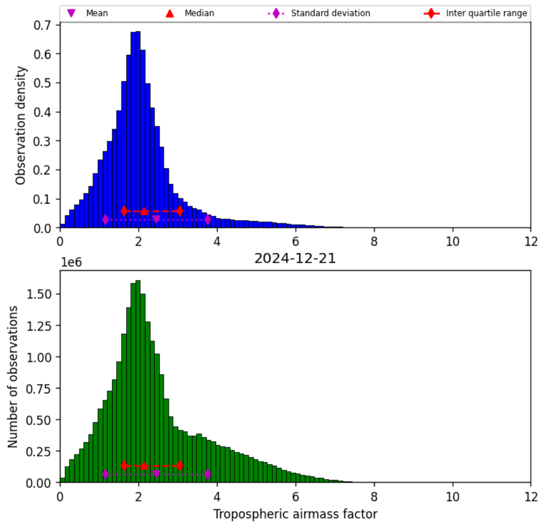
Figure 29: Histogram of “Tropospheric airmass factor” for 2024-12-21 to 2024-12-22
