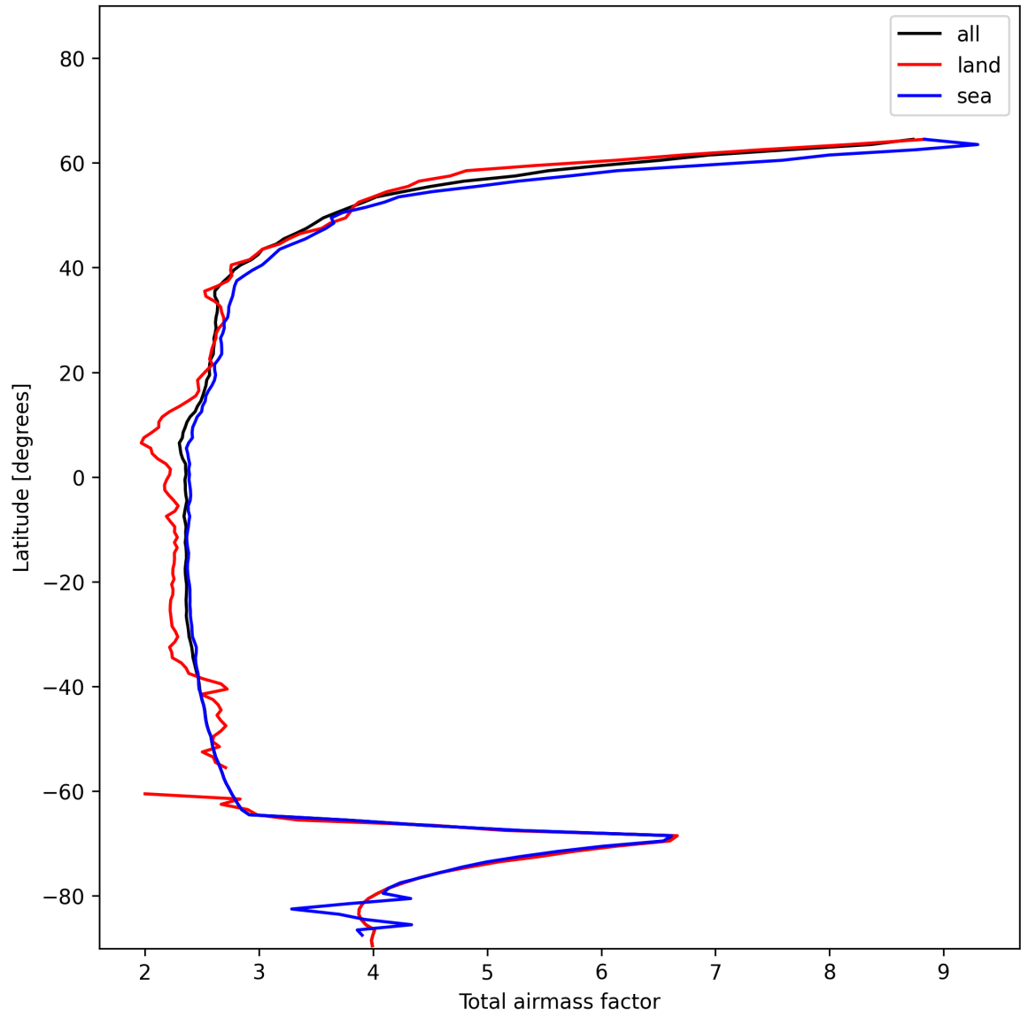
Figure 13: Zonal average of “Total airmass factor” for 2024-12-21 to 2024-12-22.
