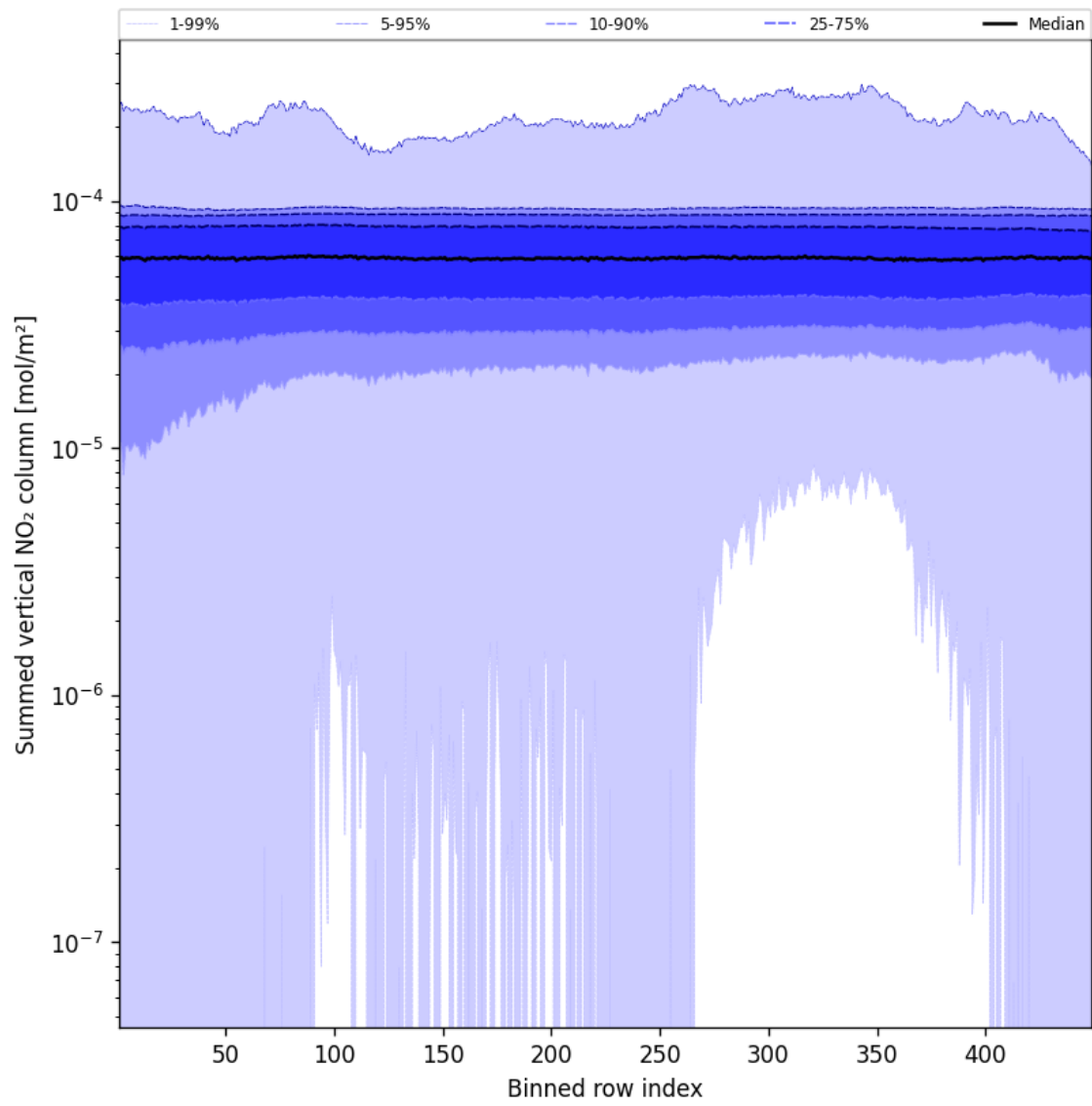
Figure 55: Along track statistics of “Summed vertical NO 2 column” for 2024-12-22 to 2024-12-23
