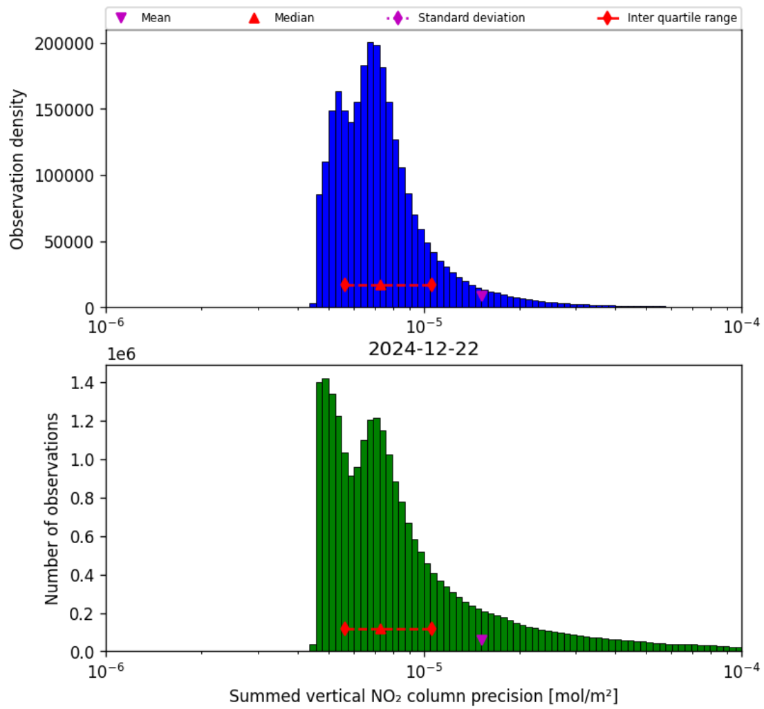
Figure 39: Histogram of “Summed vertical NO 2 column precision” for 2024-12-22 to 2024-12-23
