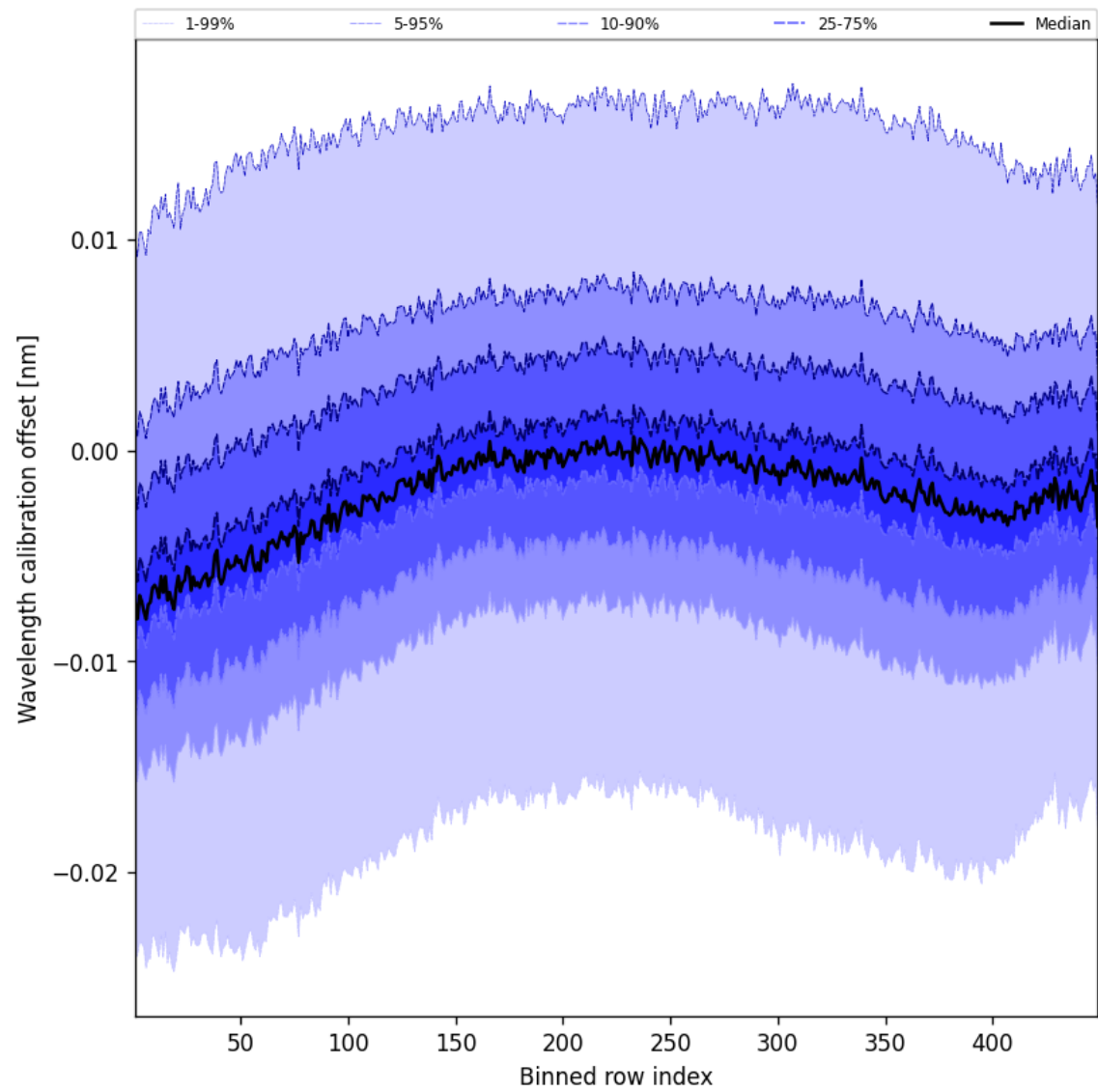
Figure 50: Along track statistics of “Wavelength calibration offset” for 2024-12-22 to 2024-12-23
