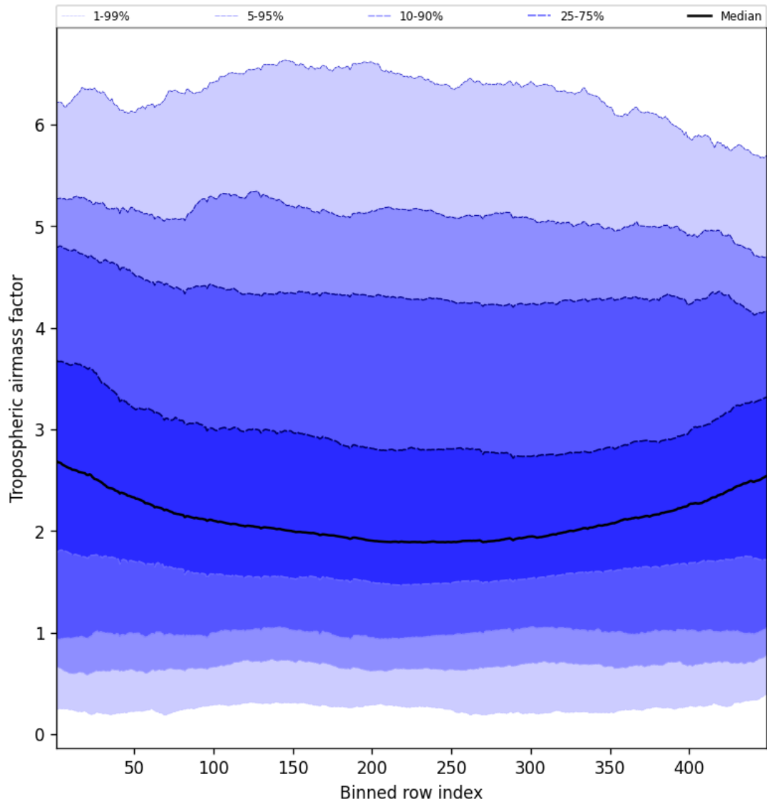
Figure 46: Along track statistics of “Tropospheric airmass factor” for 2024-12-22 to 2024-12-23
