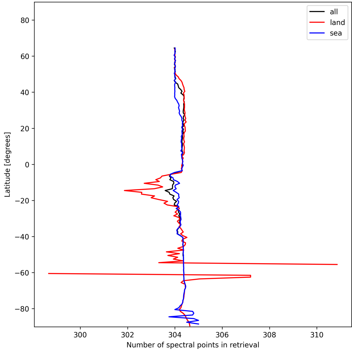
Figure 14: Zonal average of “Number of spectral points in retrieval” for 2024-12-22 to 2024-12-23.
