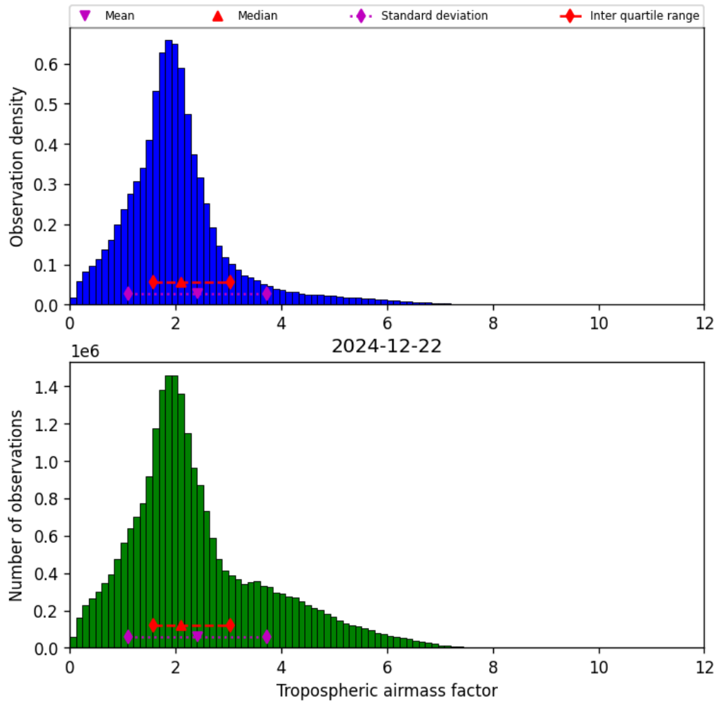
Figure 29: Histogram of “Tropospheric airmass factor” for 2024-12-22 to 2024-12-23
