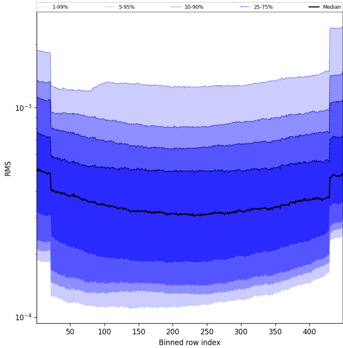
Figure 58: Along track statistics of “RMS” for 2024-12-22 to 2024-12-23
