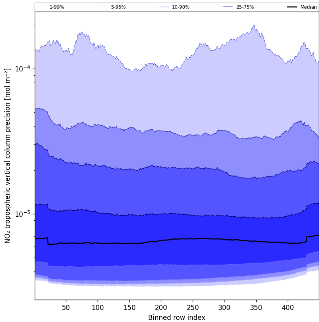
Figure 45: Along track statistics of “NO 2 tropospheric vertical column precision” for 2024-12-22 to 2024-12-23
