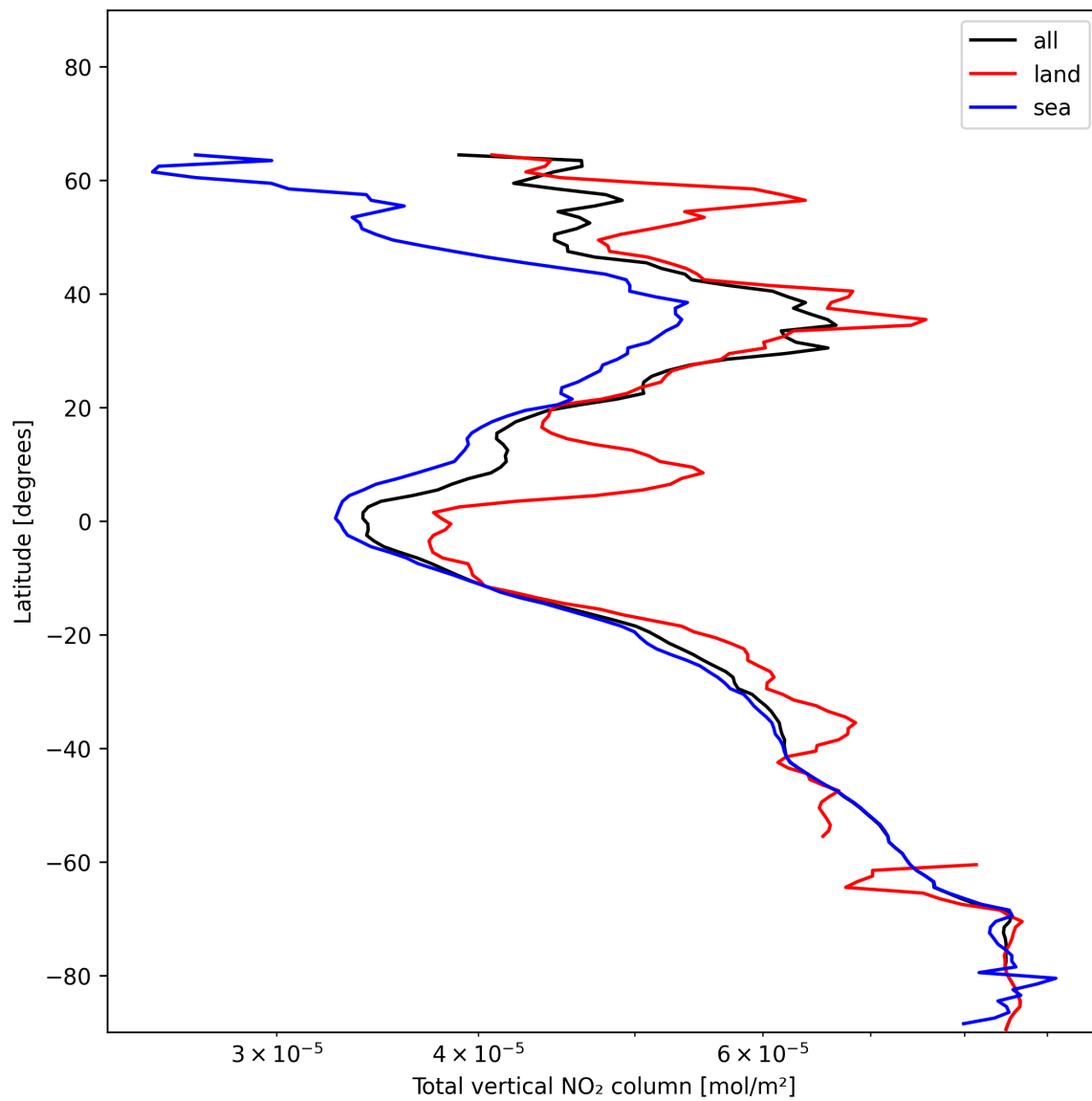
Figure 19: Zonal average of “Total vertical NO 2 column” for 2024-12-22 to 2024-12-23.
