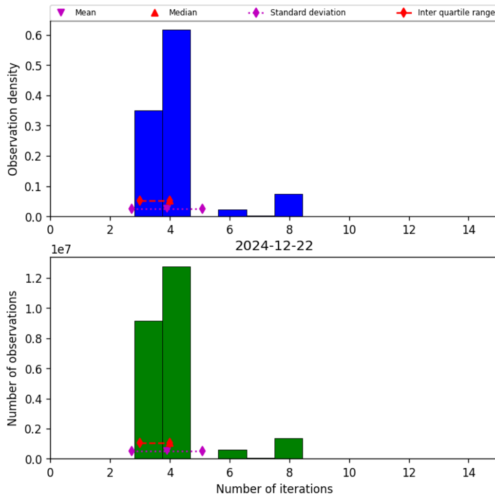
Figure 32: Histogram of “Number of iterations” for 2024-12-22 to 2024-12-23
