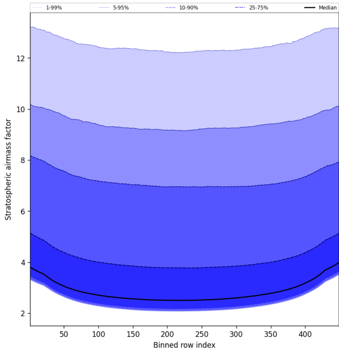
Figure 59: Along track statistics of “Stratospheric airmass factor” for 2024-12-22 to 2024-12-23
