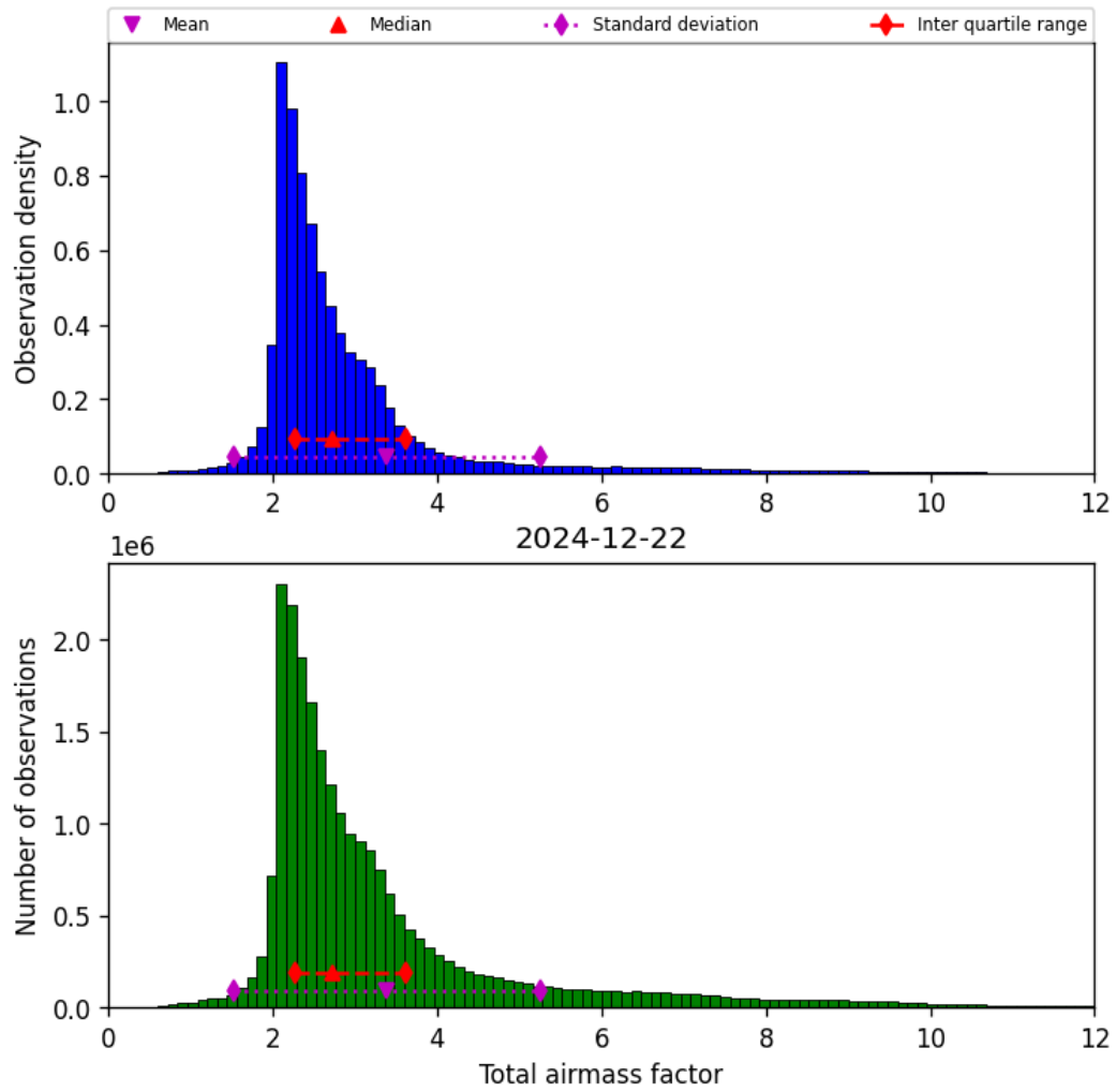
Figure 30: Histogram of “Total airmass factor” for 2024-12-22 to 2024-12-23
