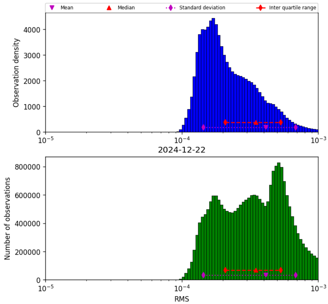
Figure 41: Histogram of “RMS” for 2024-12-22 to 2024-12-23
