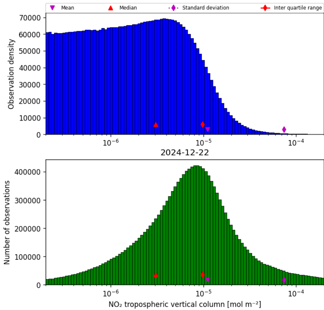
Figure 27: Histogram of “NO 2 tropospheric vertical column” for 2024-12-22 to 2024-12-23
