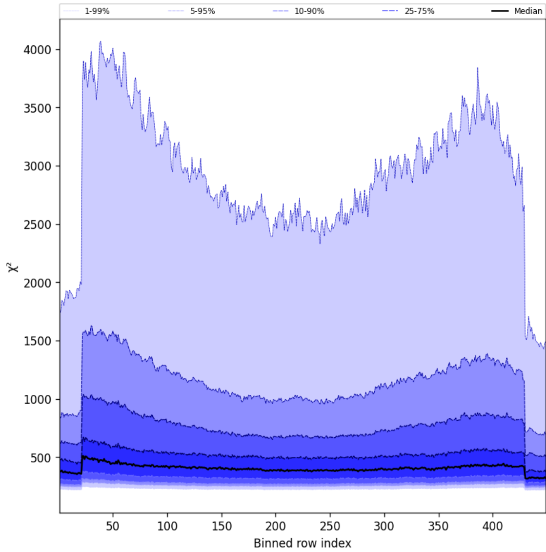
Figure 57: Along track statistics of “ \chi^2 ” for 2024-12-22 to 2024-12-23
