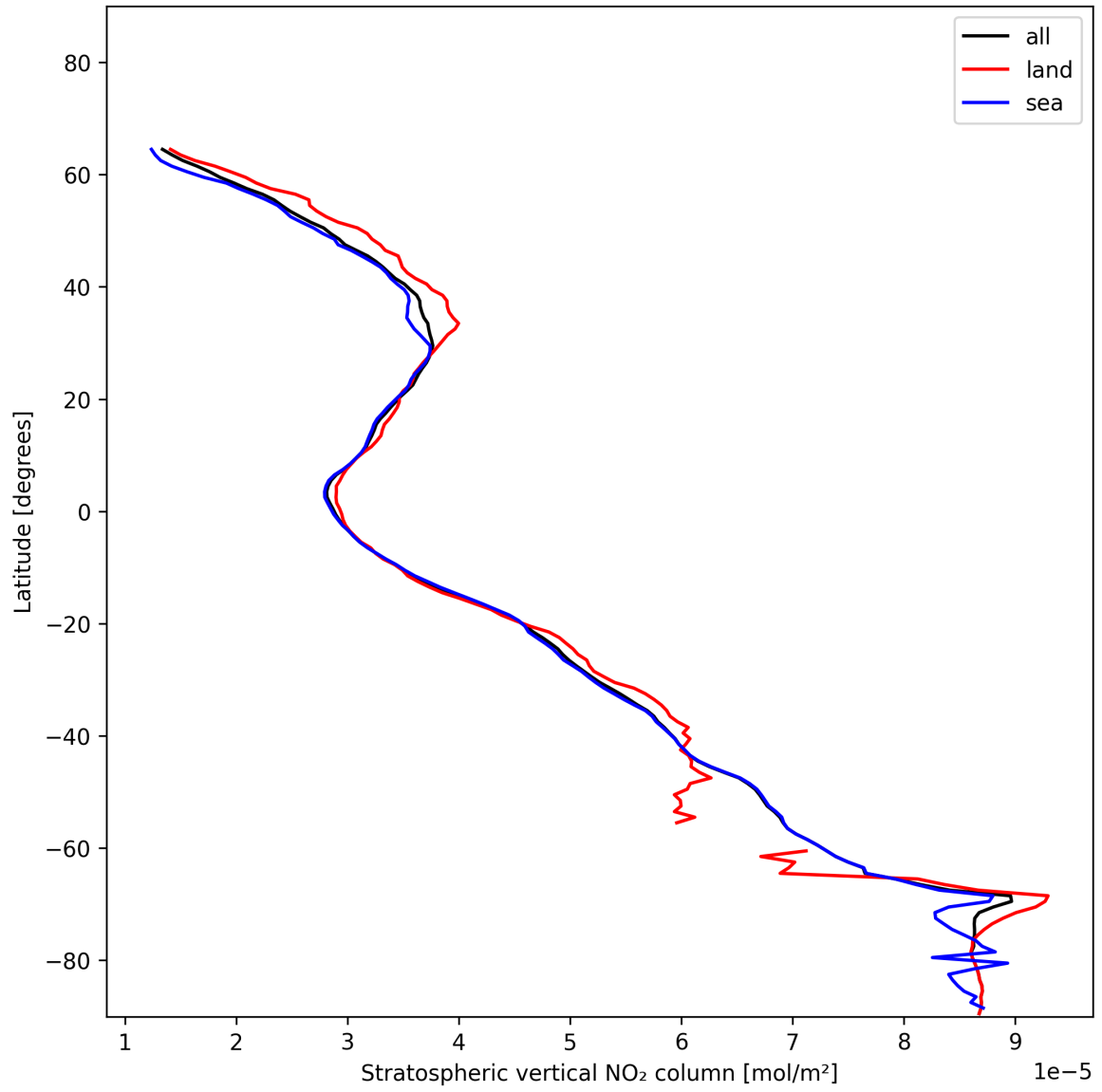
Figure 17: Zonal average of “Stratospheric vertical NO 2 column” for 2024-12-22 to 2024-12-23.
