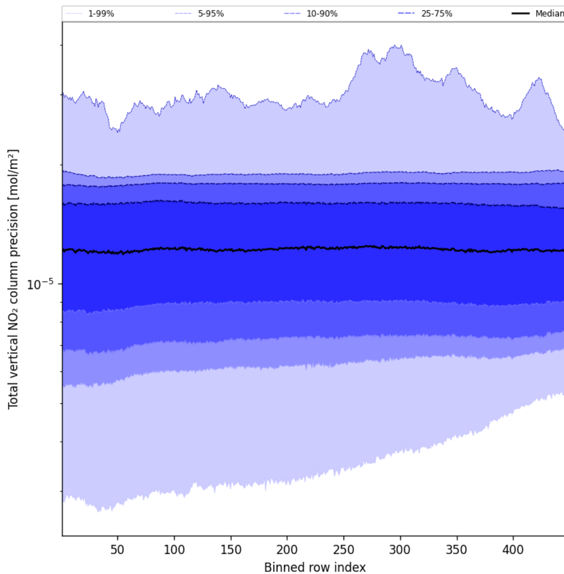
Figure 54: Along track statistics of “Total vertical NO 2 column precision” for 2024-12-22 to 2024-12-23
