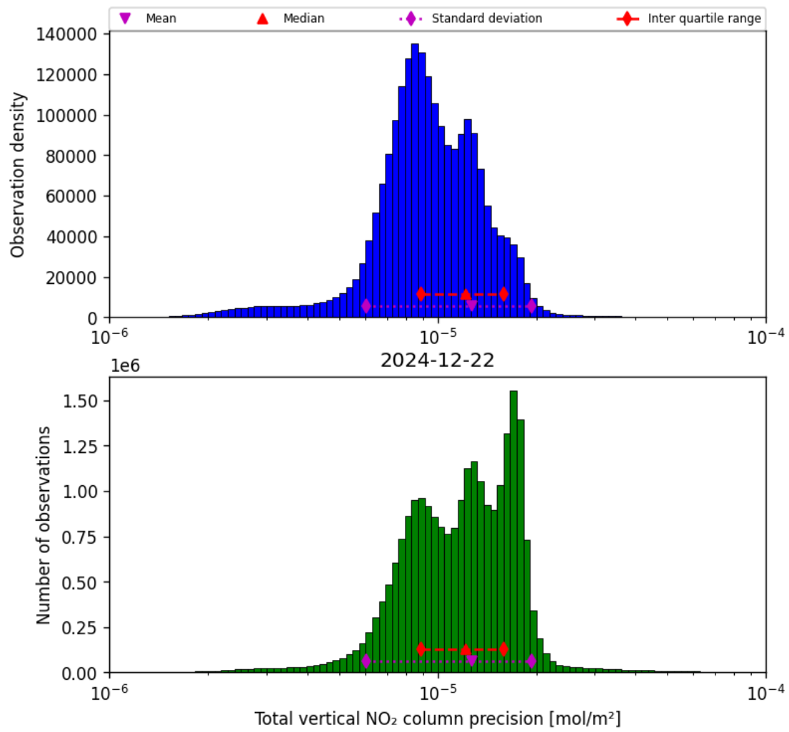
Figure 37: Histogram of “Total vertical NO 2 column precision” for 2024-12-22 to 2024-12-23
