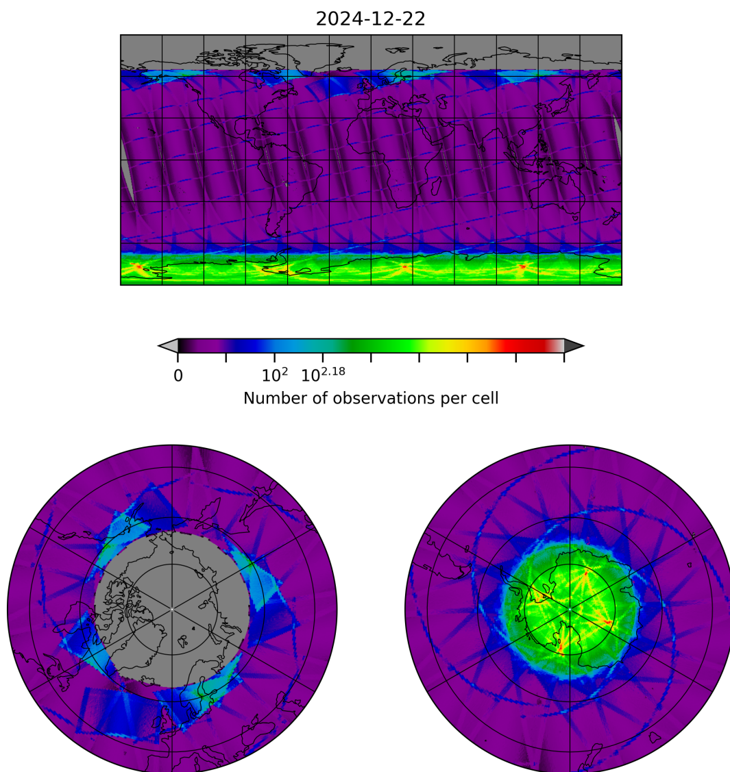
Figure 8: Map of the number of observations for 2024-12-22 to 2024-12-23
