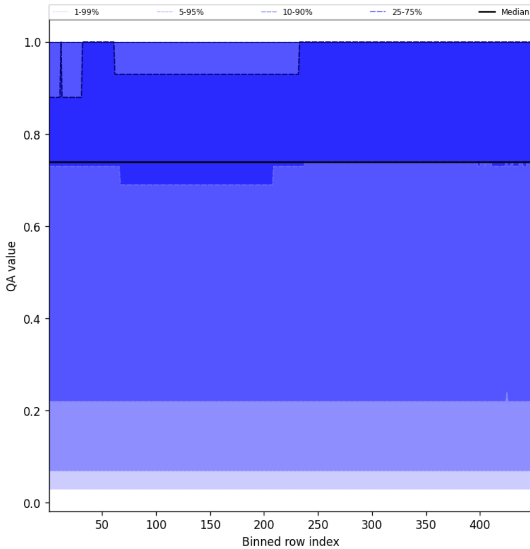
Figure 43: Along track statistics of “QA value” for 2024-12-22 to 2024-12-23
