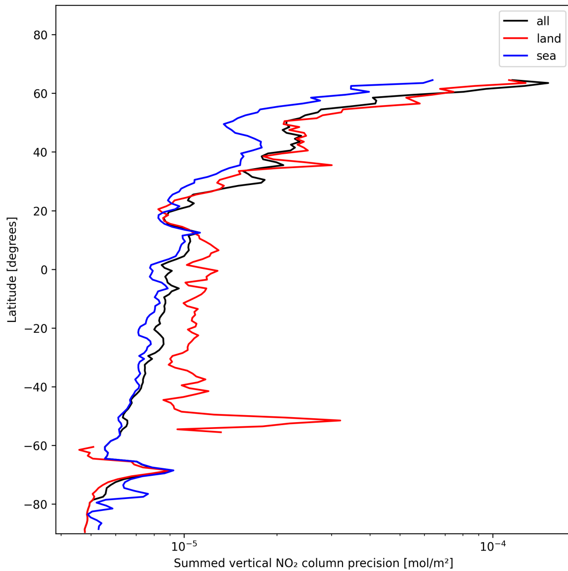
Figure 22: Zonal average of “Summed vertical NO 2 column precision” for 2024-12-22 to 2024-12-23.
