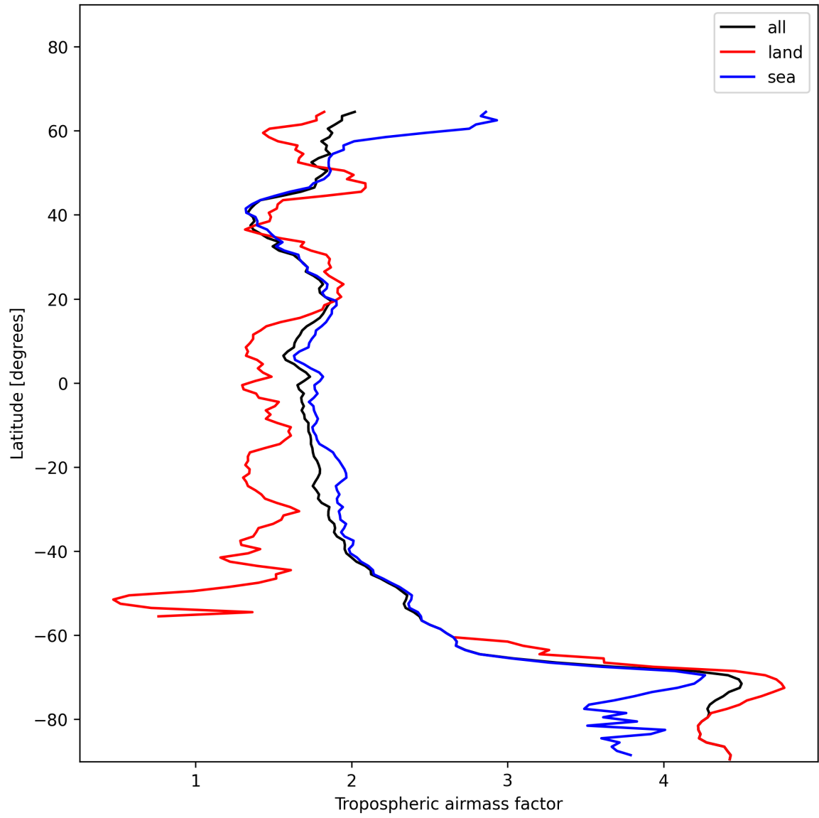
Figure 12: Zonal average of “Tropospheric airmass factor” for 2024-12-22 to 2024-12-23.
