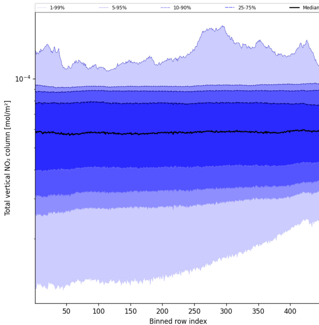
Figure 53: Along track statistics of “Total vertical NO 2 column” for 2024-12-22 to 2024-12-23
