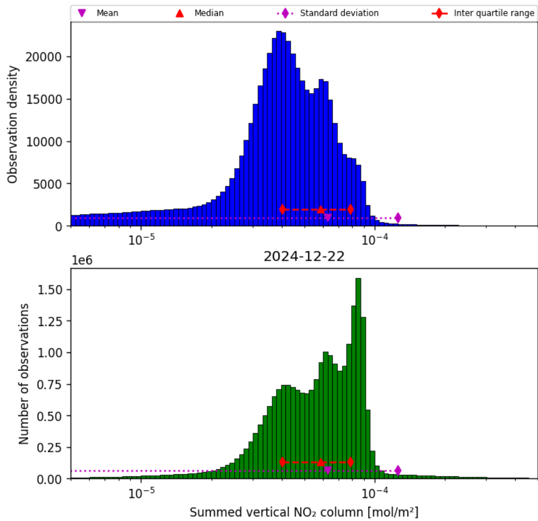
Figure 38: Histogram of “Summed vertical NO 2 column” for 2024-12-22 to 2024-12-23
