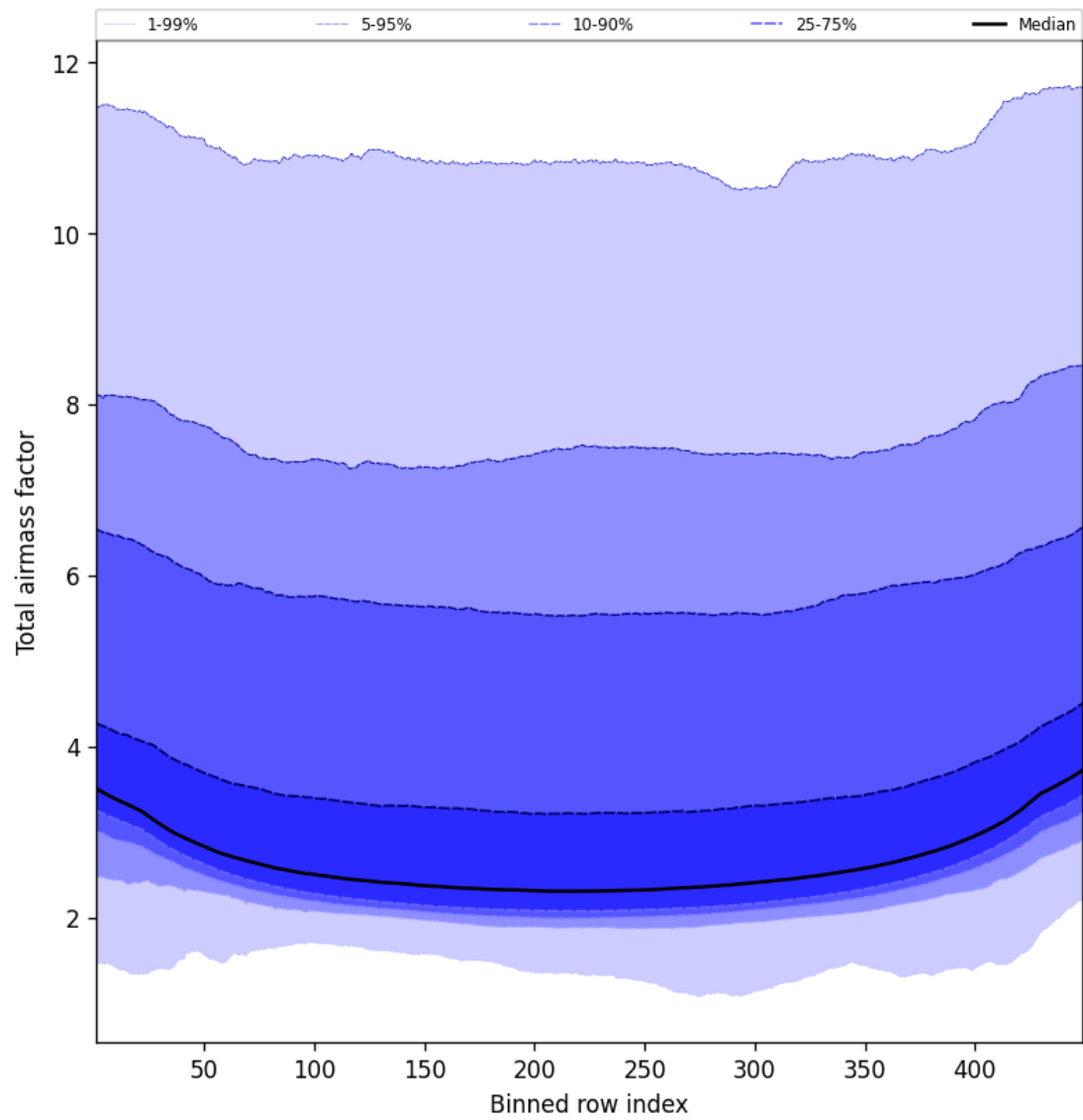
Figure 47: Along track statistics of “Total airmass factor” for 2024-12-22 to 2024-12-23
