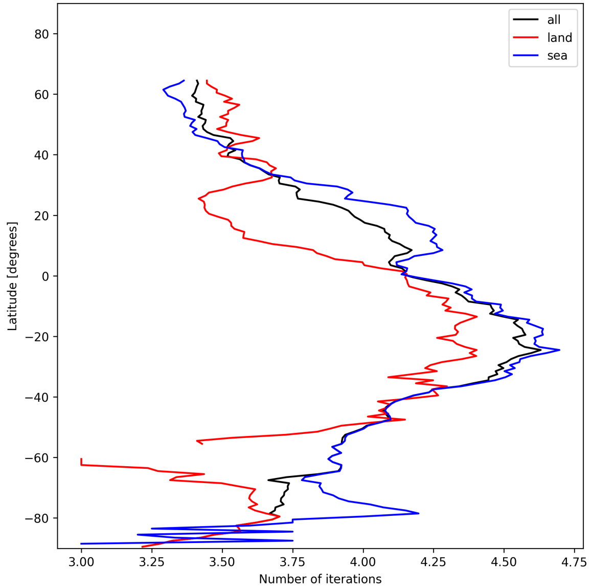
Figure 15: Zonal average of “Number of iterations” for 2024-12-22 to 2024-12-23.
