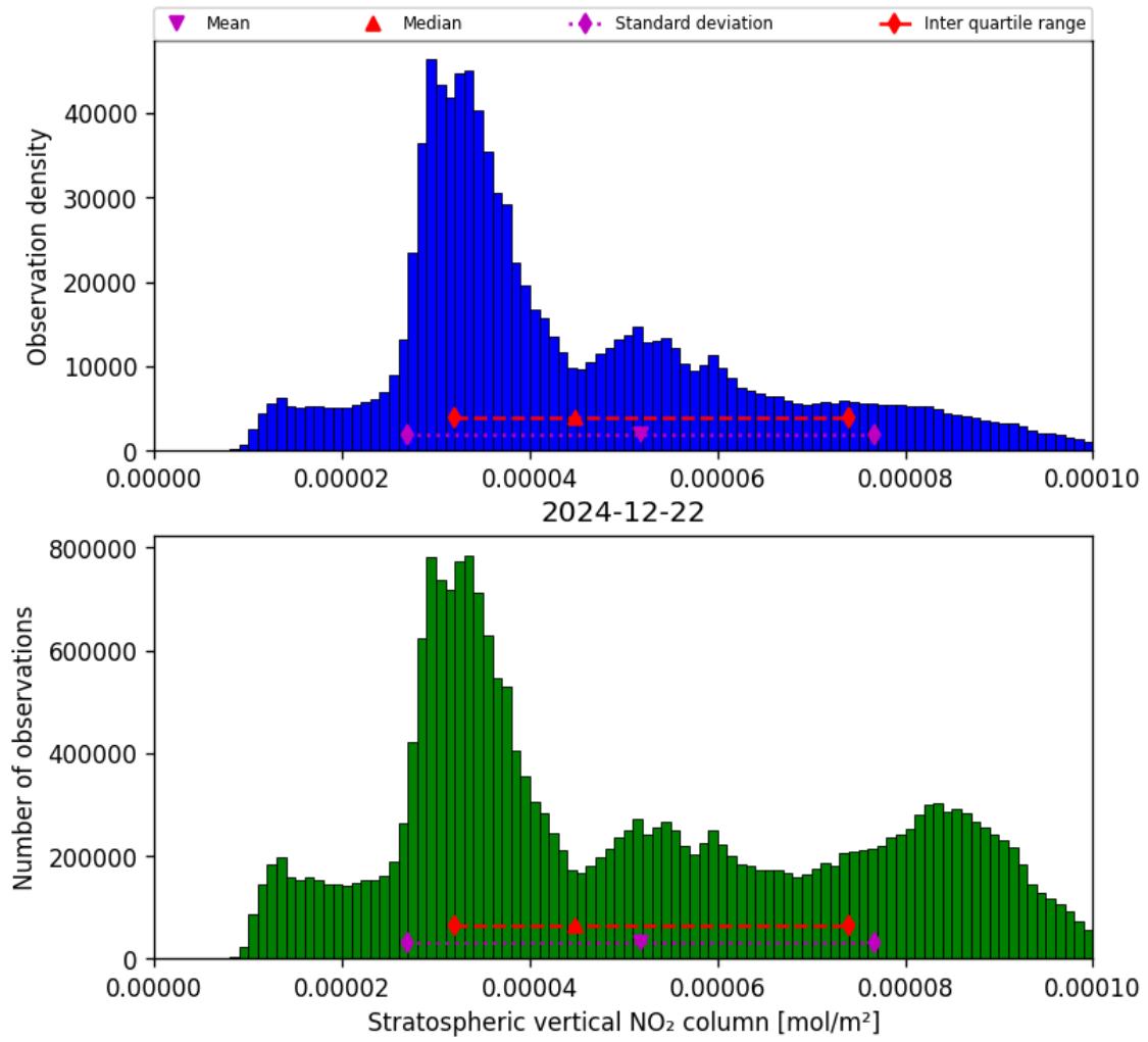
Figure 34: Histogram of “Stratospheric vertical NO 2 column” for 2024-12-22 to 2024-12-23
