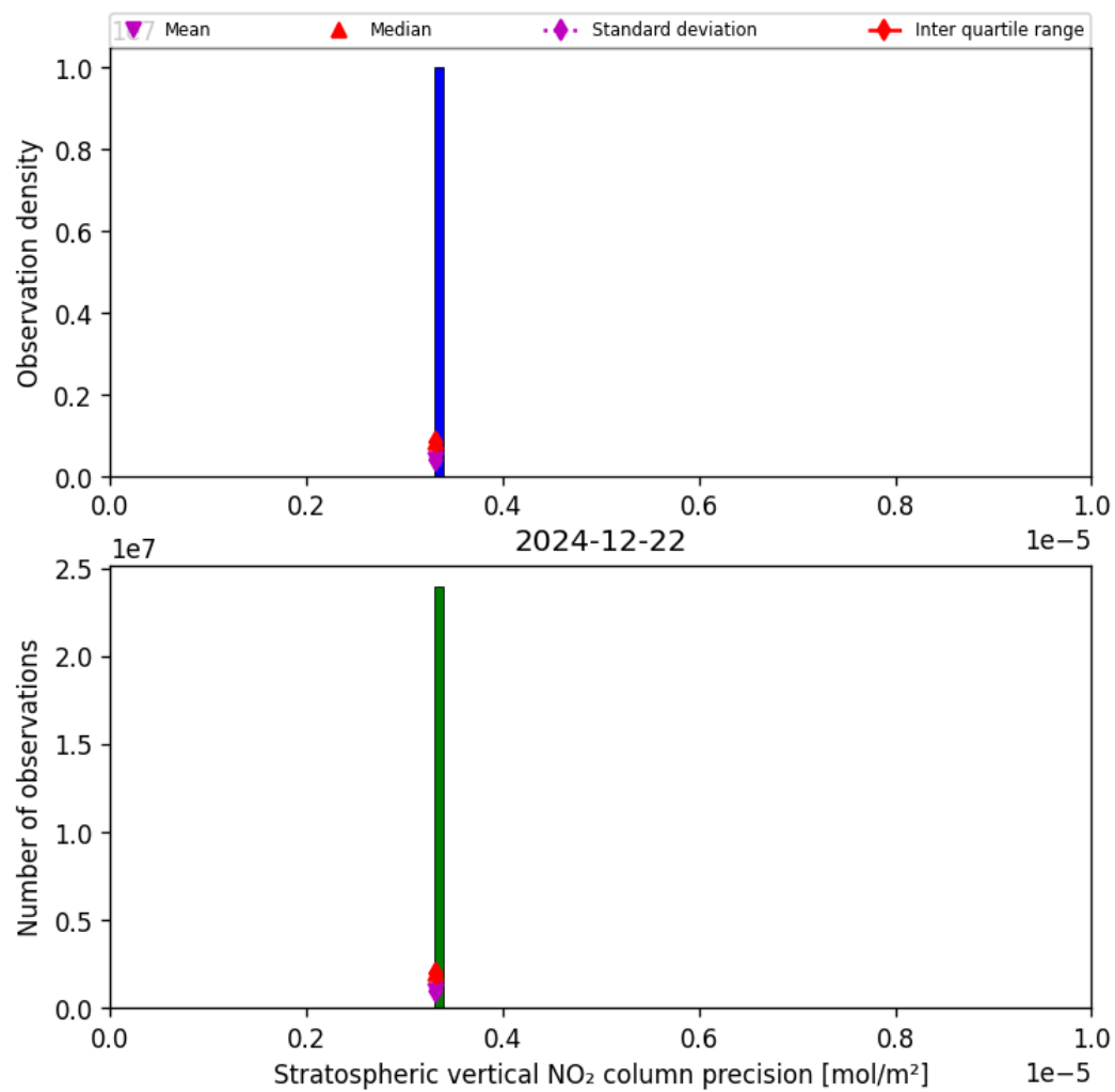
Figure 35: Histogram of “Stratospheric vertical NO 2 column precision” for 2024-12-22 to 2024-12-23
