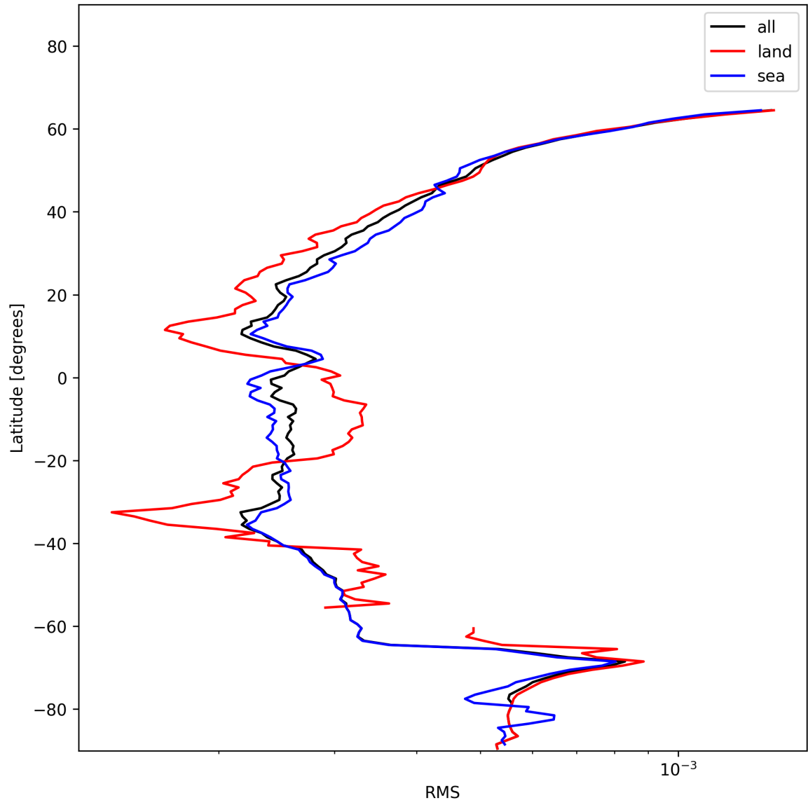
Figure 24: Zonal average of “RMS” for 2024-12-22 to 2024-12-23.
