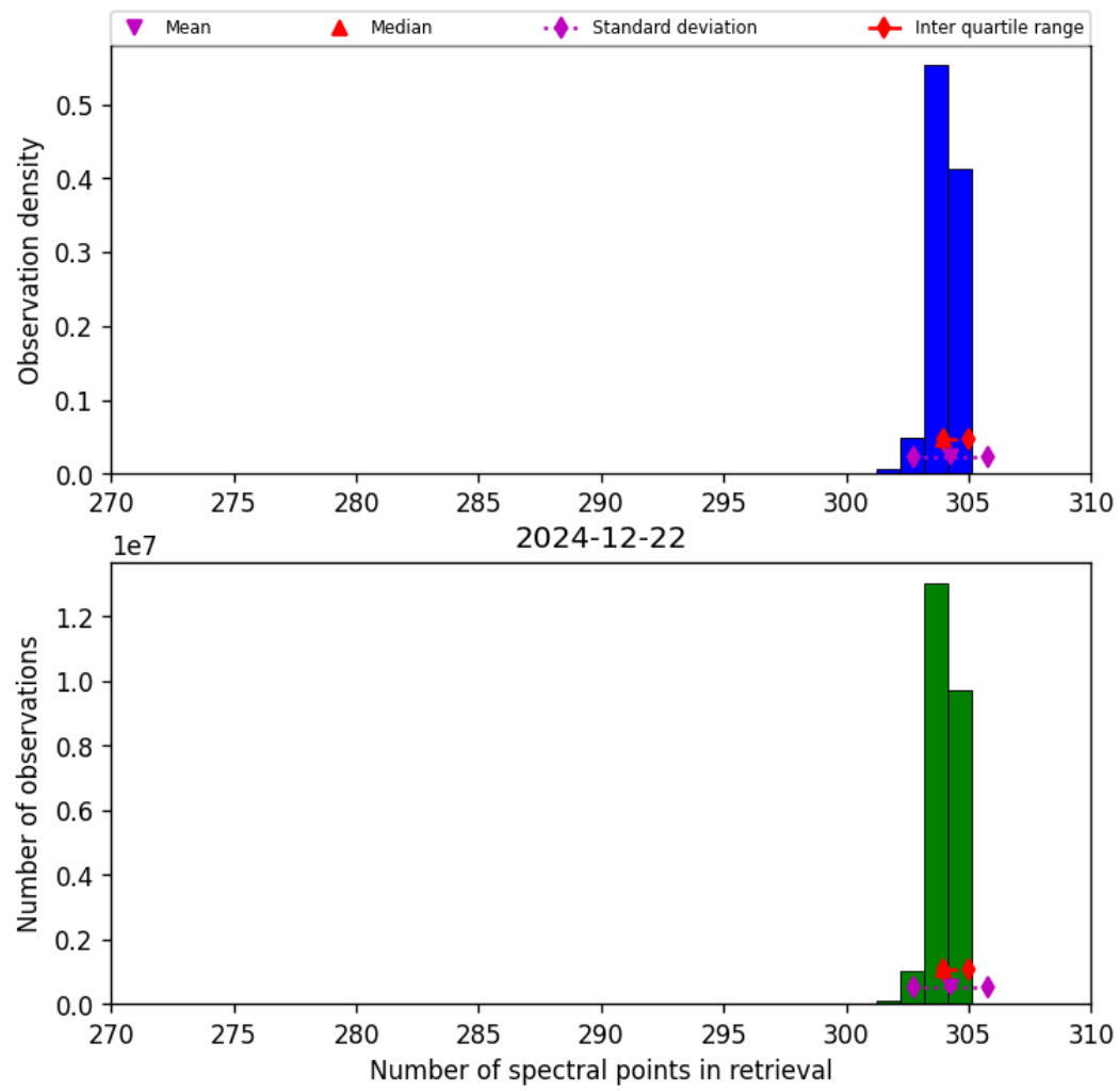
Figure 31: Histogram of “Number of spectral points in retrieval” for 2024-12-22 to 2024-12-23
