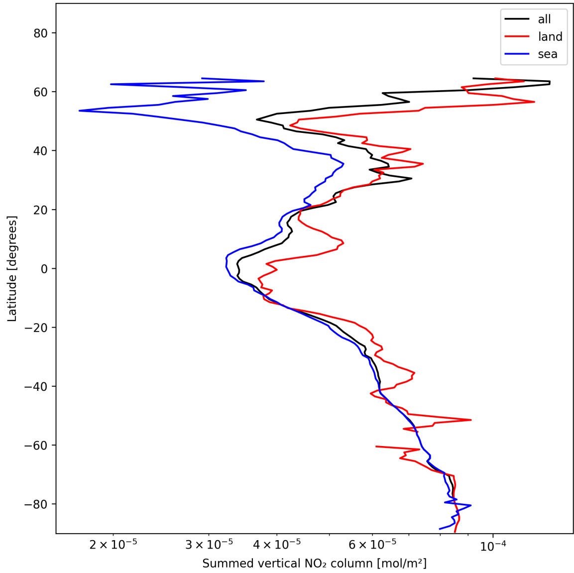
Figure 21: Zonal average of “Summed vertical NO 2 column” for 2024-12-22 to 2024-12-23.
