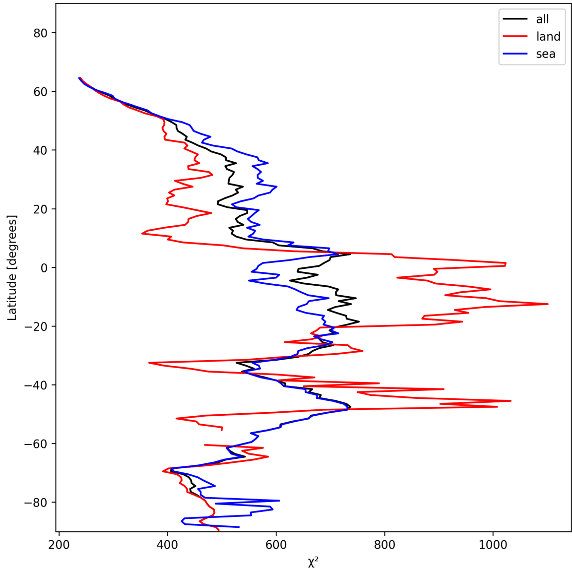
Figure 23: Zonal average of “ \chi^2 ” for 2024-12-22 to 2024-12-23.
