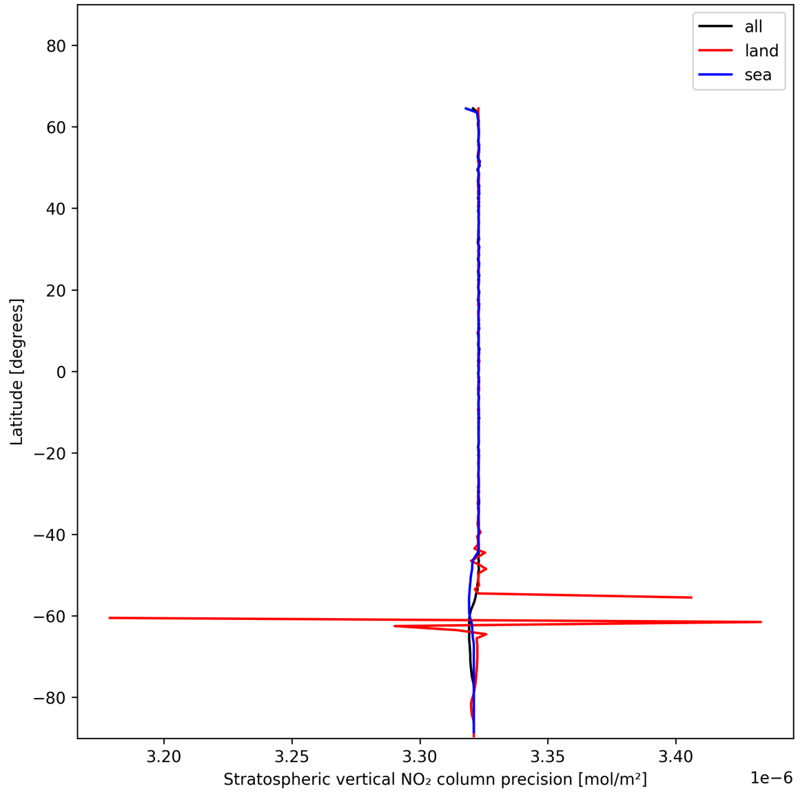
Figure 18: Zonal average of “Stratospheric vertical NO 2 column precision” for 2024-12-22 to 2024-12-23.
