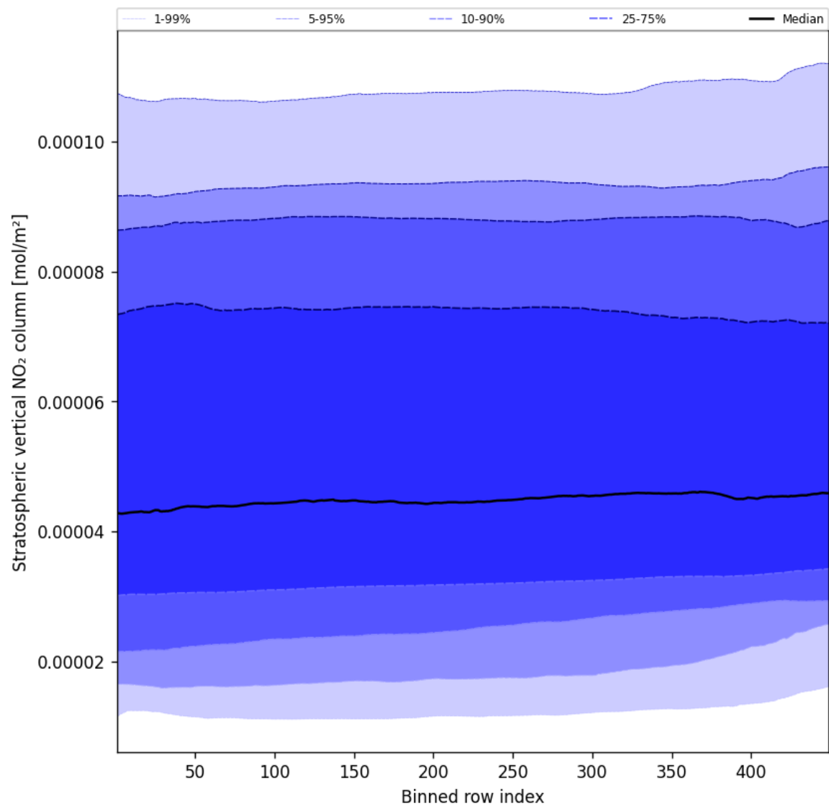
Figure 51: Along track statistics of “Stratospheric vertical NO 2 column” for 2024-12-22 to 2024-12-23
