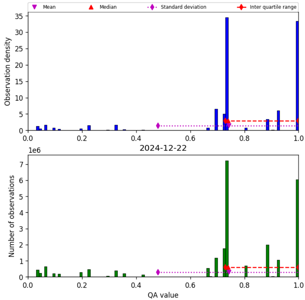
Figure 26: Histogram of “QA value” for 2024-12-22 to 2024-12-23
