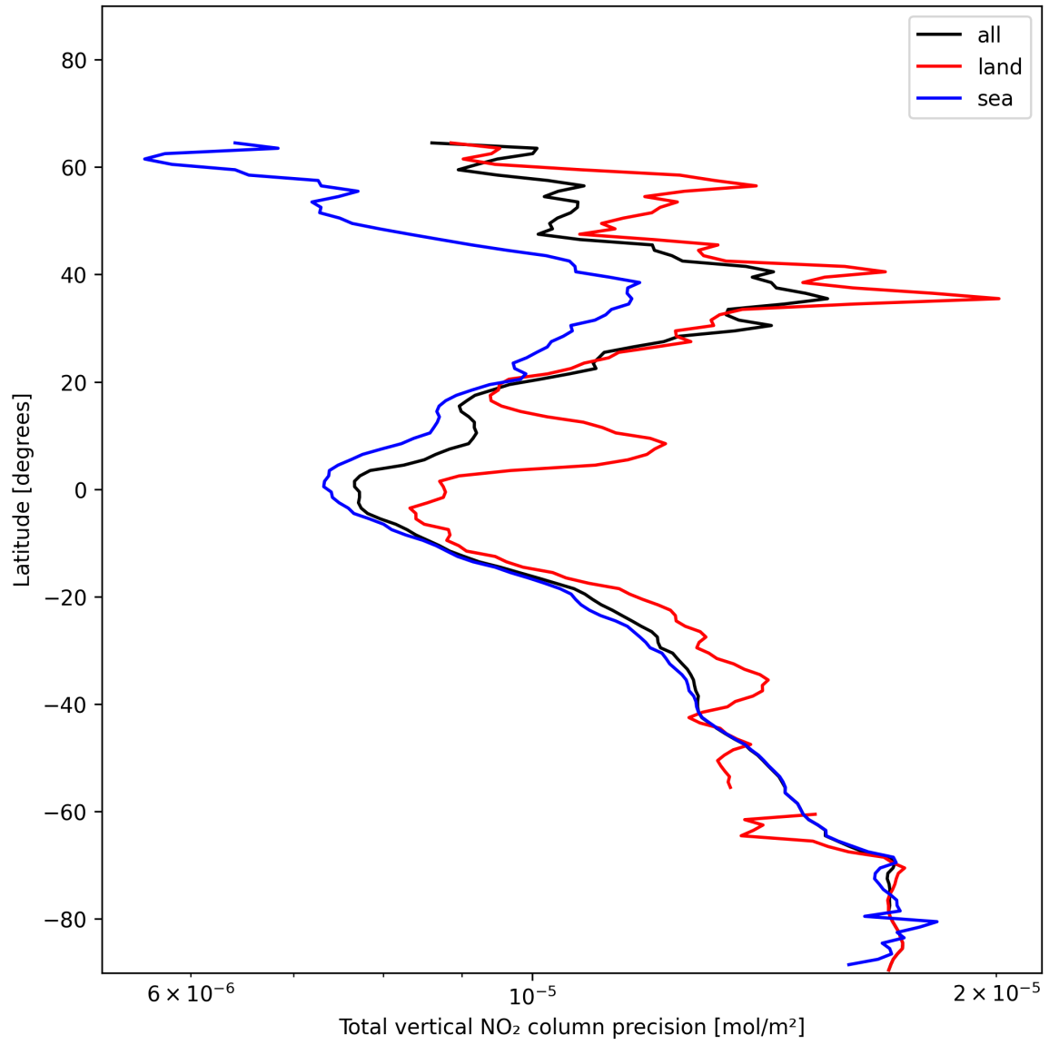
Figure 20: Zonal average of “Total vertical NO 2 column precision” for 2024-12-22 to 2024-12-23.
