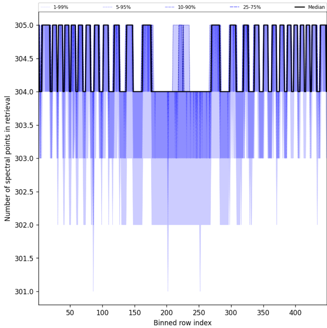
Figure 48: Along track statistics of “Number of spectral points in retrieval” for 2024-12-22 to 2024-12-23
