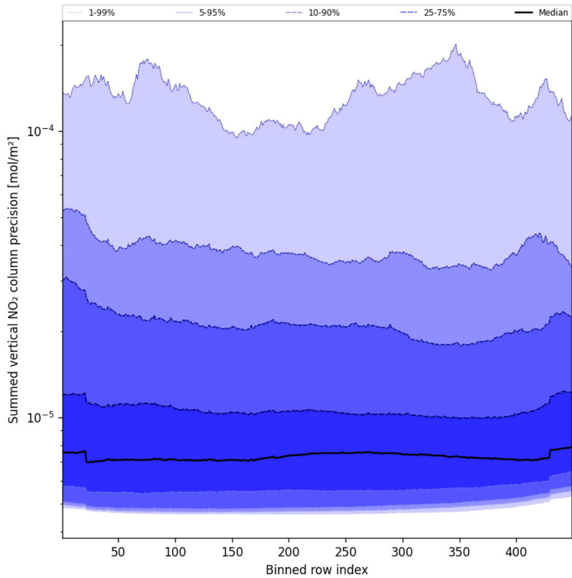
Figure 56: Along track statistics of “Summed vertical NO 2 column precision” for 2024-12-22 to 2024-12-23
