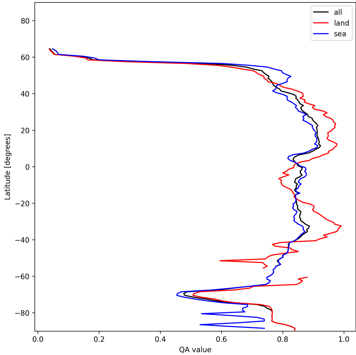
Figure 9: Zonal average of “QA value” for 2024-12-22 to 2024-12-23.
