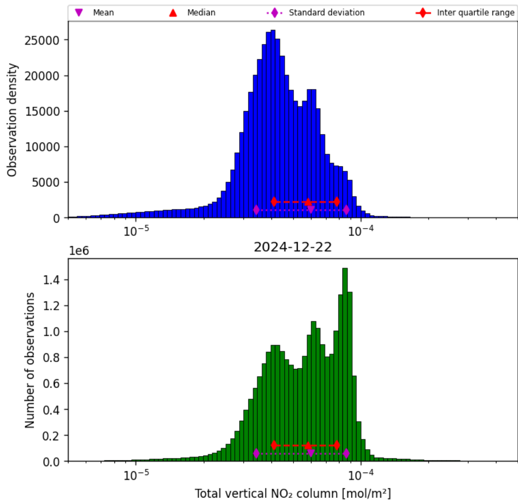
Figure 36: Histogram of “Total vertical NO 2 column” for 2024-12-22 to 2024-12-23
