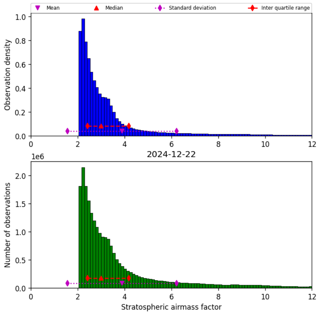
Figure 42: Histogram of “Stratospheric airmass factor” for 2024-12-22 to 2024-12-23
