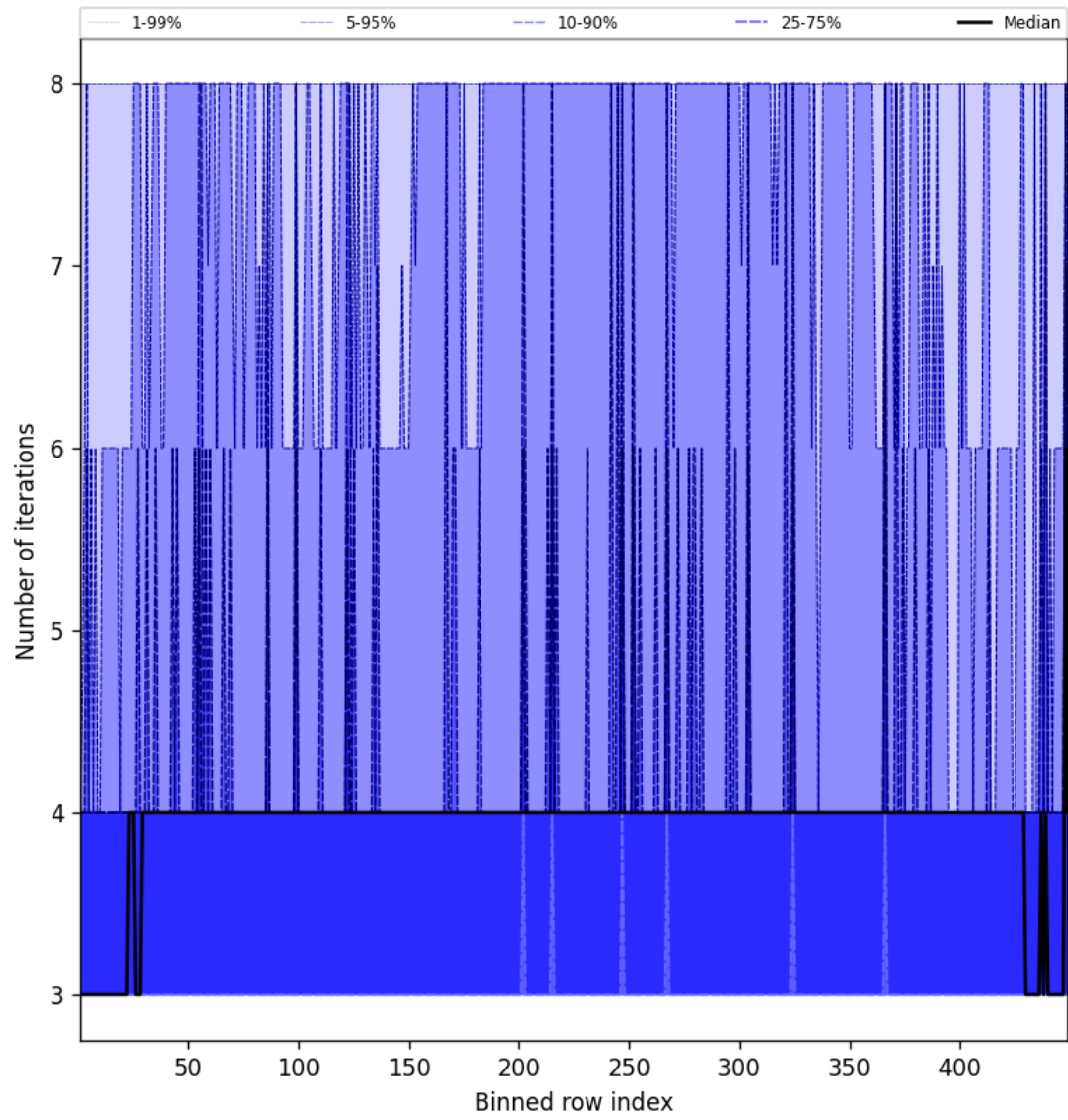
Figure 49: Along track statistics of “Number of iterations” for 2024-12-22 to 2024-12-23
