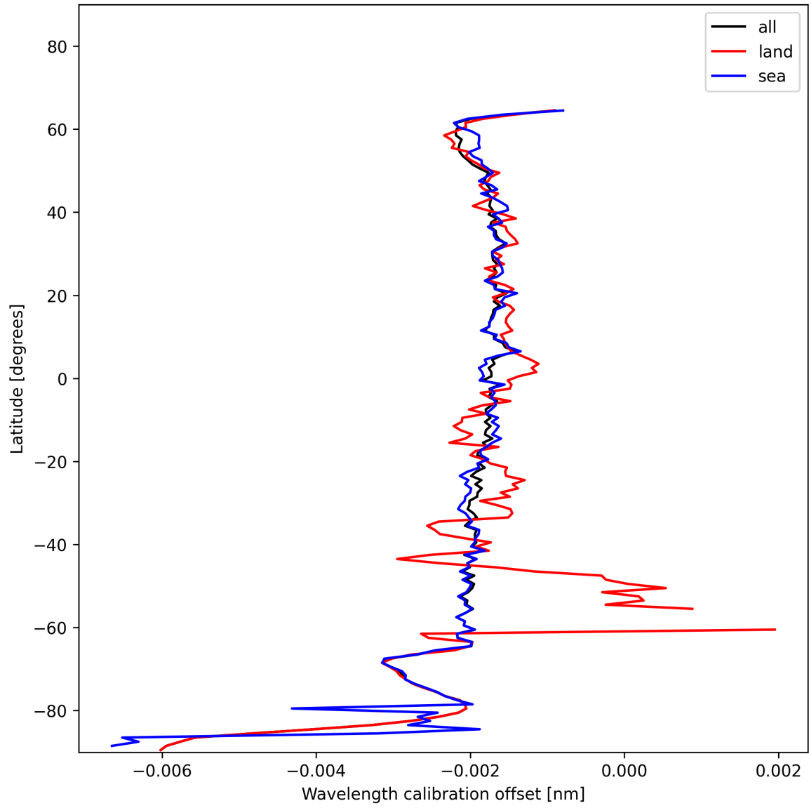
Figure 16: Zonal average of “Wavelength calibration offset” for 2024-12-22 to 2024-12-23.
