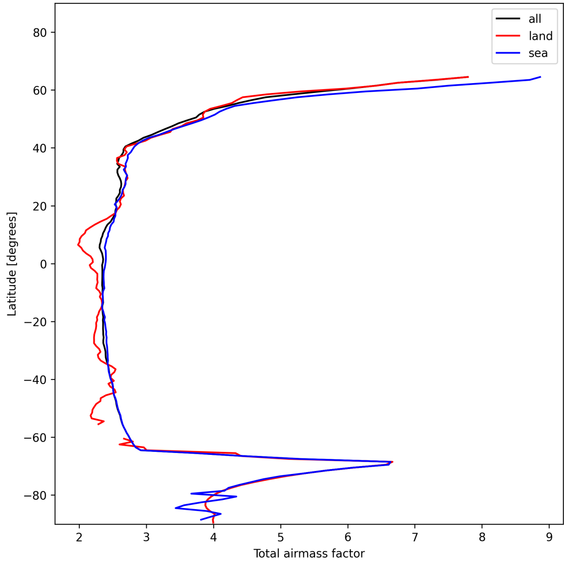
Figure 13: Zonal average of “Total airmass factor” for 2024-12-22 to 2024-12-23.
