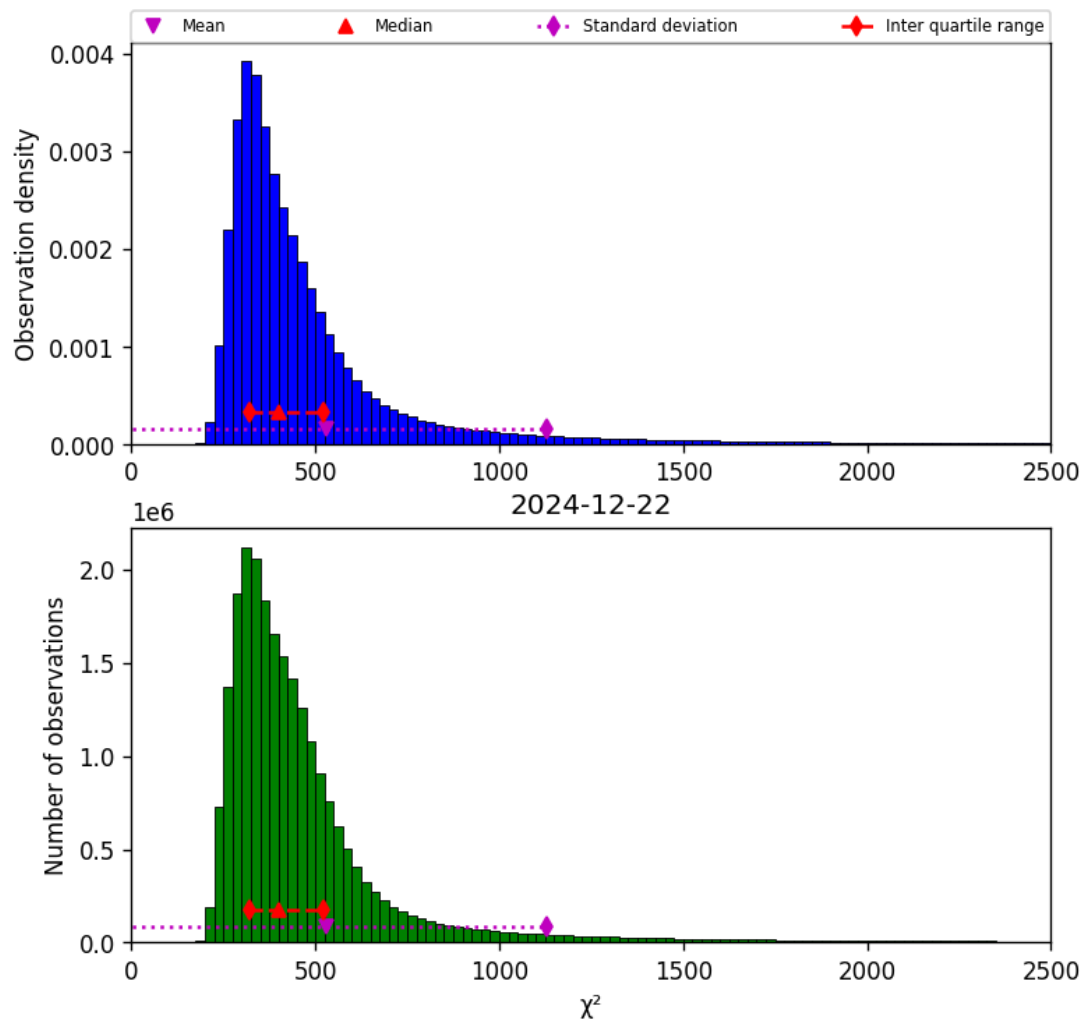
Figure 40: Histogram of “ \chi^2 ” for 2024-12-22 to 2024-12-23
