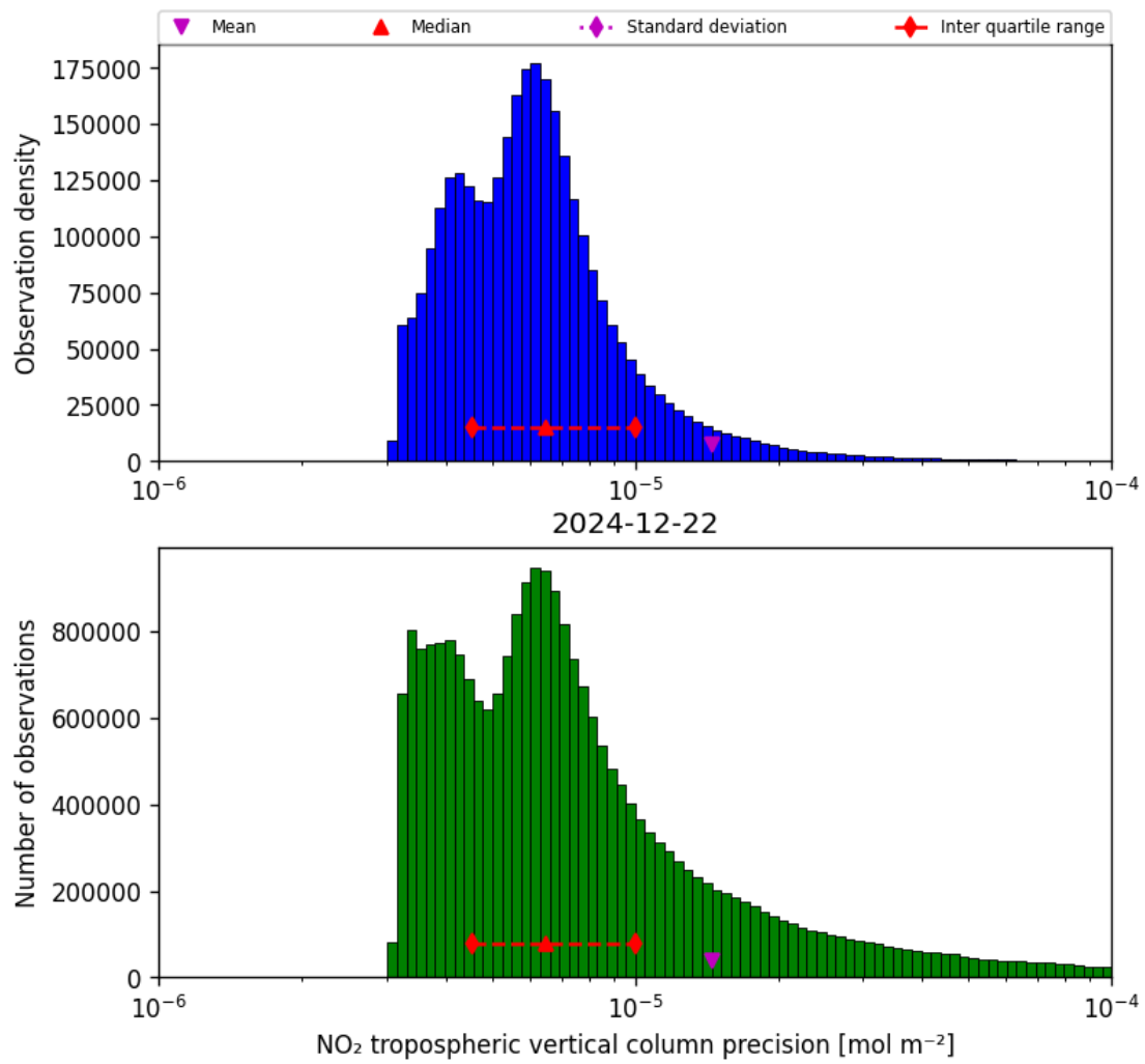
Figure 28: Histogram of “NO 2 tropospheric vertical column precision” for 2024-12-22 to 2024-12-23
