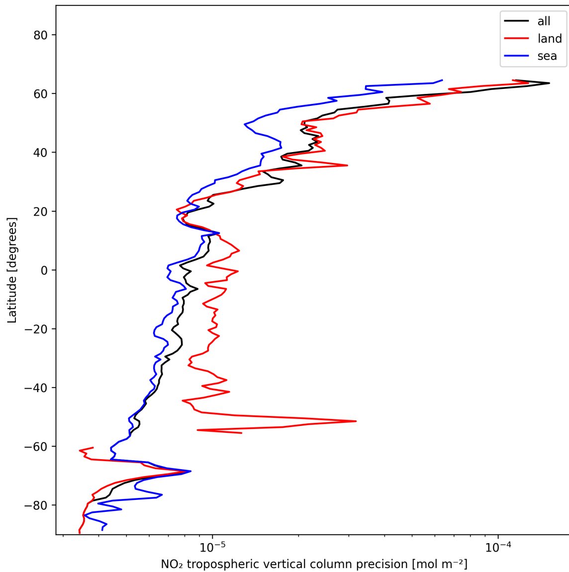
Figure 11: Zonal average of “NO 2 tropospheric vertical column precision” for 2024-12-22 to 2024-12-23.
