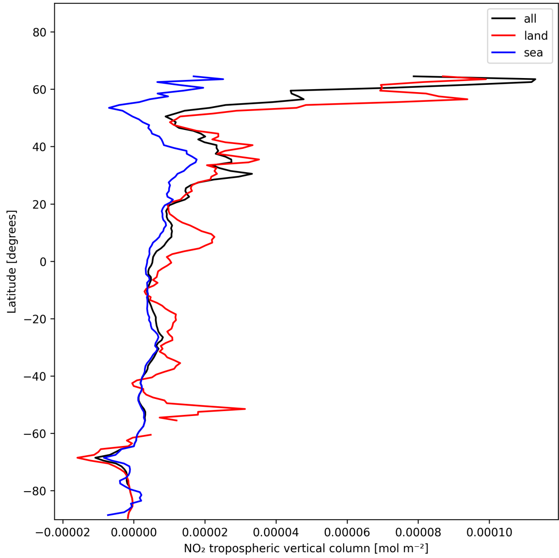
Figure 10: Zonal average of “NO 2 tropospheric vertical column” for 2024-12-22 to 2024-12-23.
