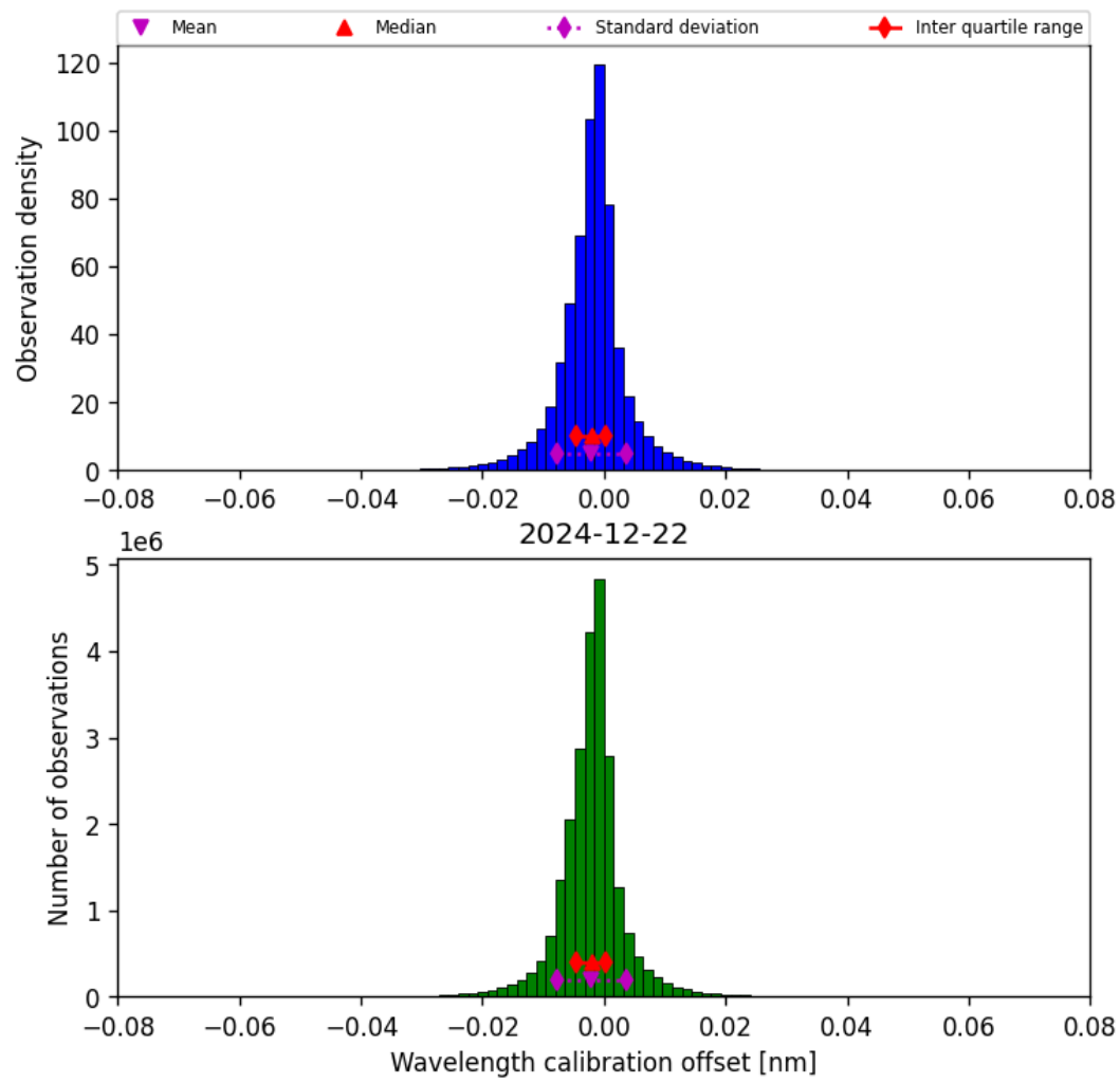
Figure 33: Histogram of “Wavelength calibration offset” for 2024-12-22 to 2024-12-23
