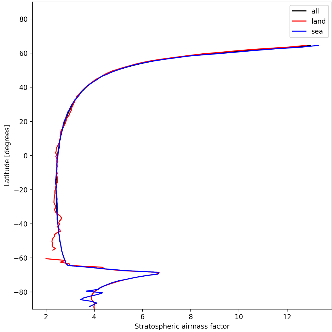
Figure 25: Zonal average of “Stratospheric airmass factor” for 2024-12-22 to 2024-12-23.
