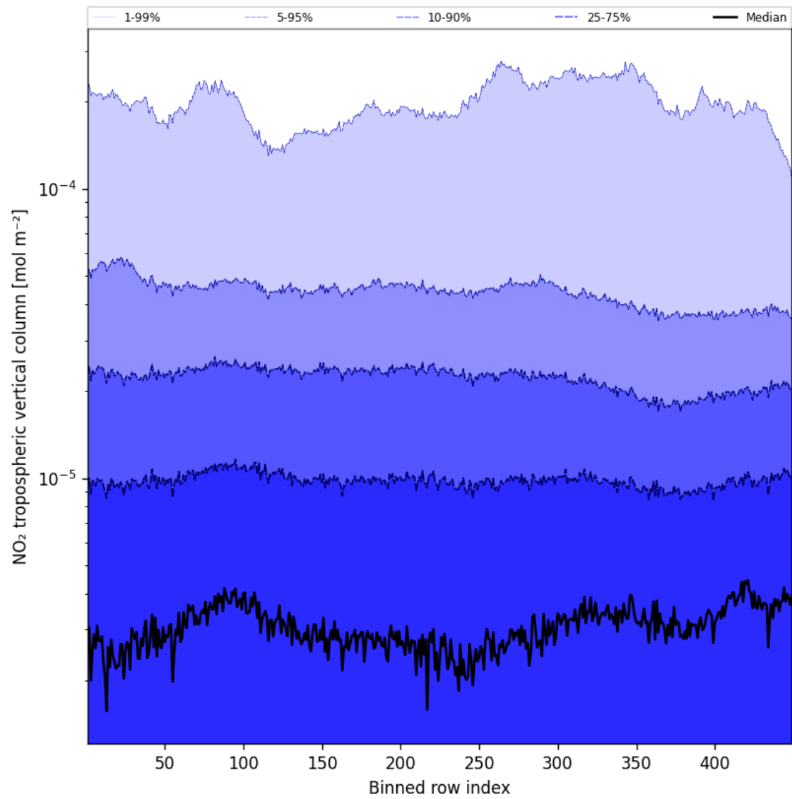
Figure 44: Along track statistics of “NO 2 tropospheric vertical column” for 2024-12-22 to 2024-12-23
