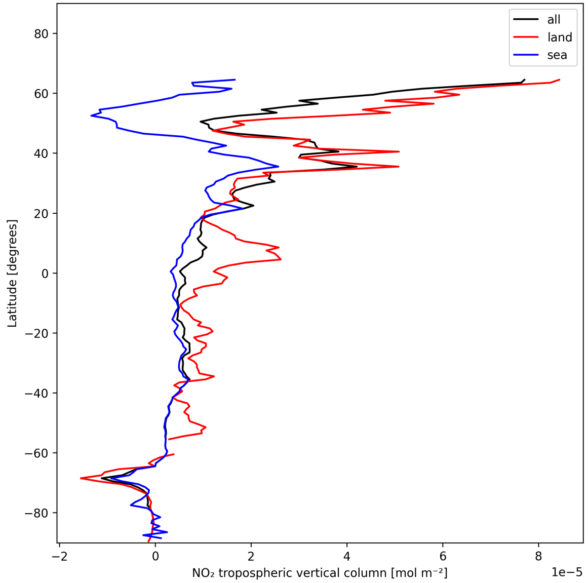
Figure 10: Zonal average of “NO 2 tropospheric vertical column” for 2024-12-23 to 2024-12-24.
