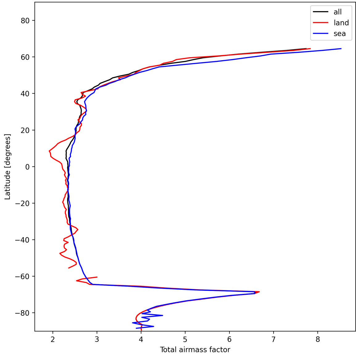
Figure 13: Zonal average of “Total airmass factor” for 2024-12-23 to 2024-12-24.
