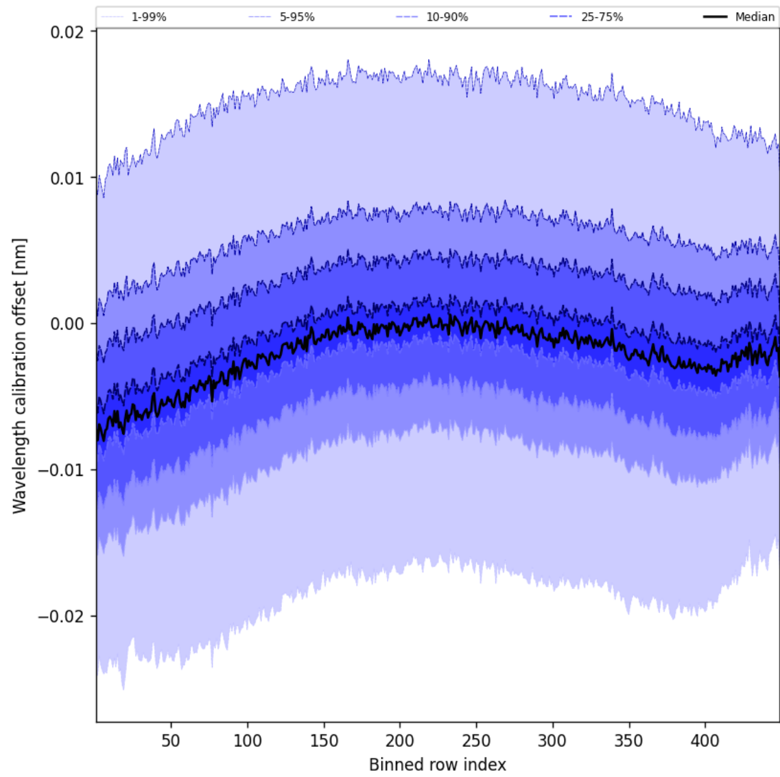
Figure 50: Along track statistics of “Wavelength calibration offset” for 2024-12-23 to 2024-12-24
