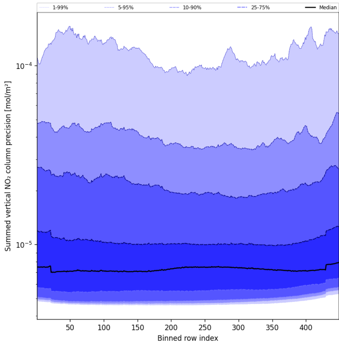
Figure 56: Along track statistics of “Summed vertical NO 2 column precision” for 2024-12-23 to 2024-12-24
