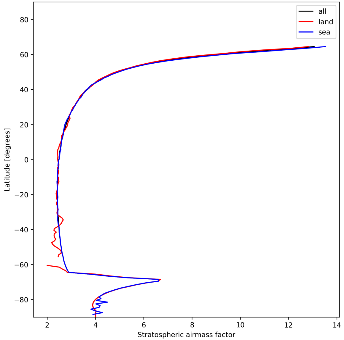
Figure 25: Zonal average of “Stratospheric airmass factor” for 2024-12-23 to 2024-12-24.
