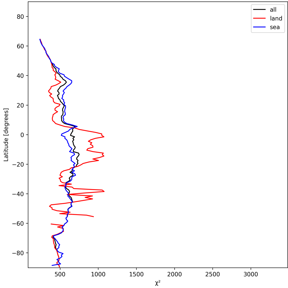
Figure 23: Zonal average of “ \chi^2 ” for 2024-12-23 to 2024-12-24.
