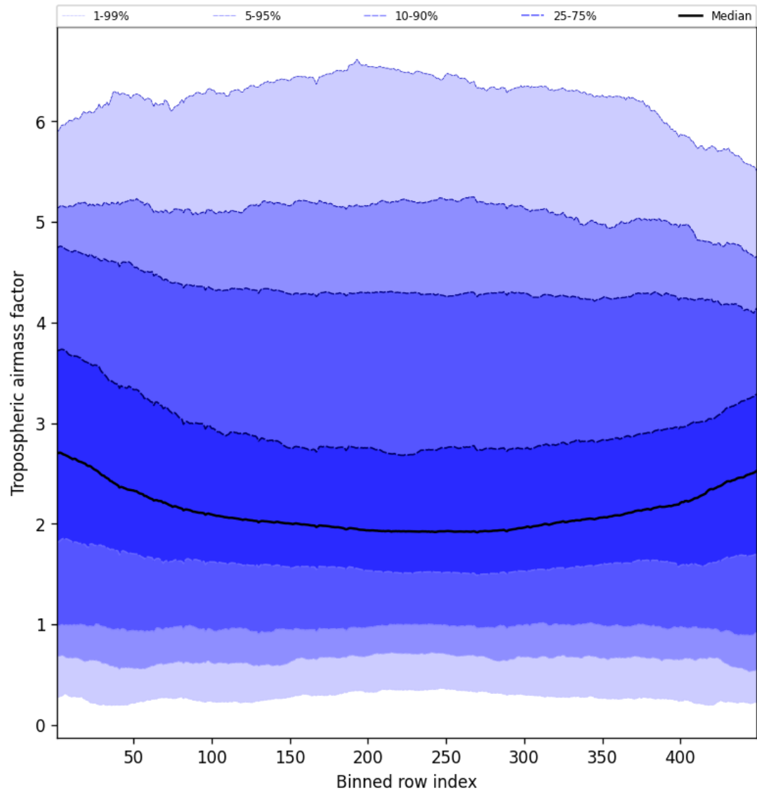
Figure 46: Along track statistics of “Tropospheric air mass factor” for 2024-12-23 to 2024-12-24
