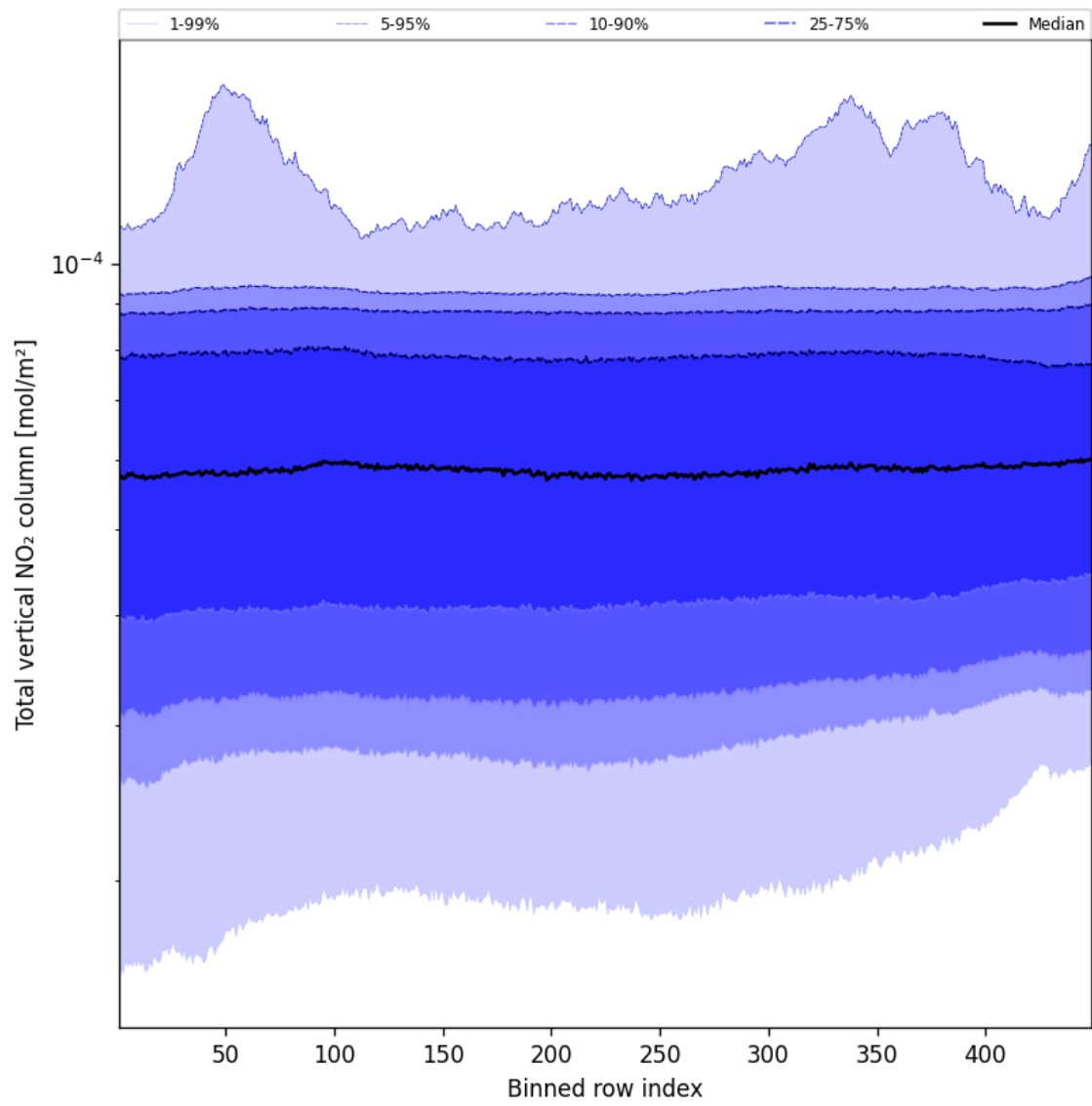
Figure 53: Along track statistics of “Total vertical NO 2 column” for 2024-12-23 to 2024-12-24
