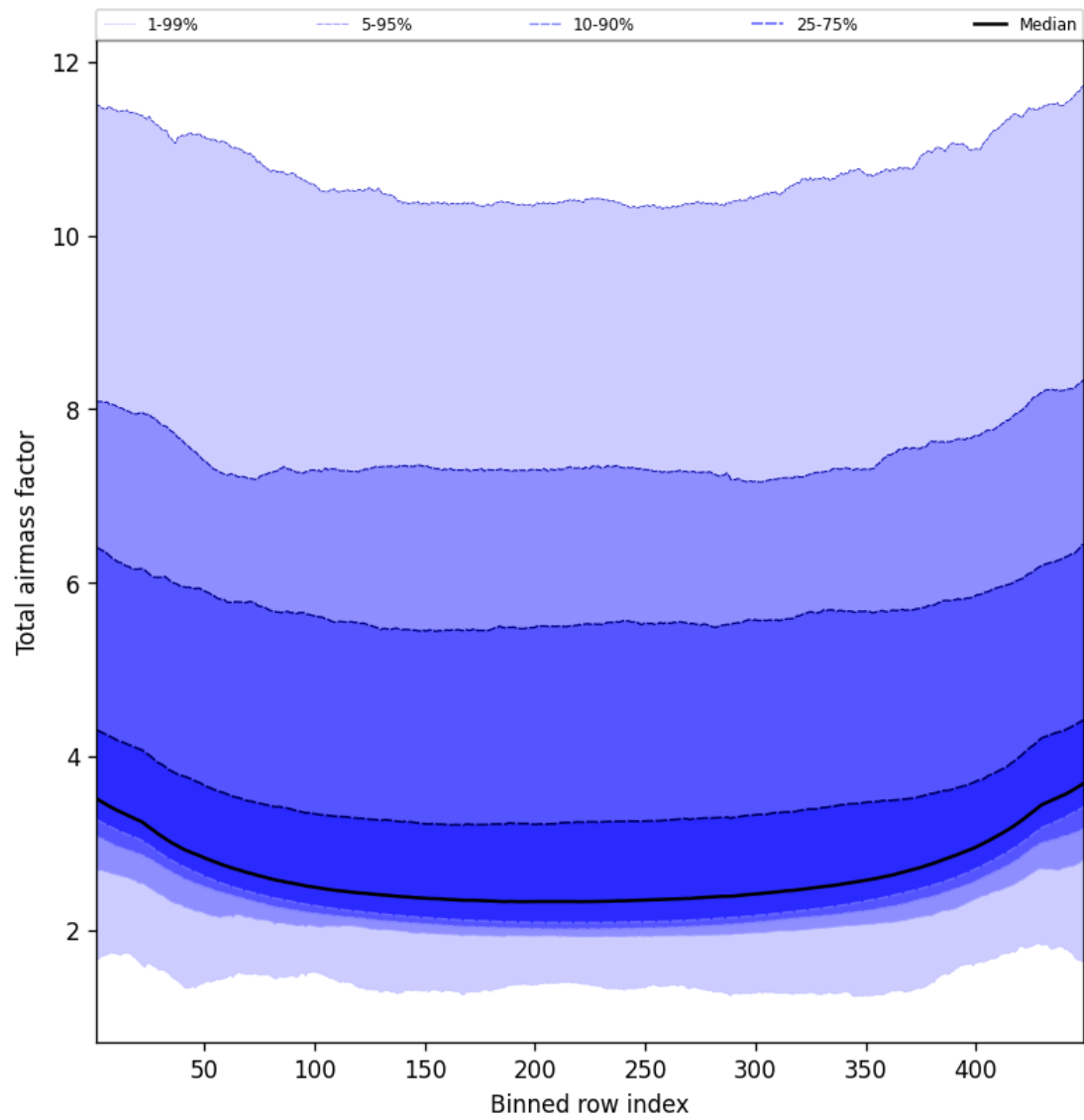
Figure 47: Along track statistics of “Total airmass factor” for 2024-12-23 to 2024-12-24
