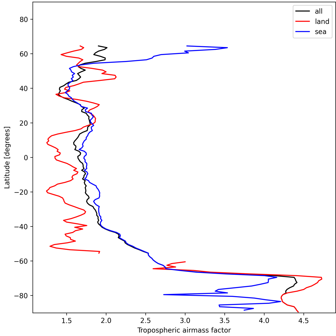
Figure 12: Zonal average of “Tropospheric airmass factor” for 2024-12-23 to 2024-12-24.
