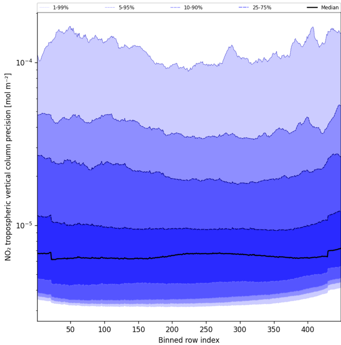
Figure 45: Along track statistics of “NO 2 tropospheric vertical column precision” for 2024-12-23 to 2024-12-24
