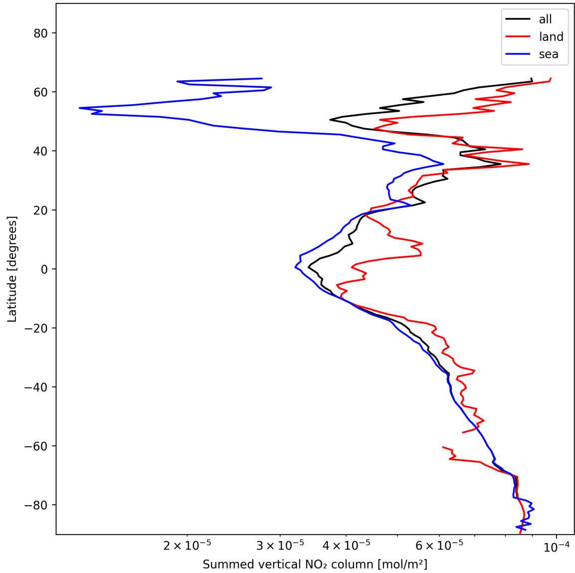
Figure 21: Zonal average of “Summed vertical NO 2 column” for 2024-12-23 to 2024-12-24.
