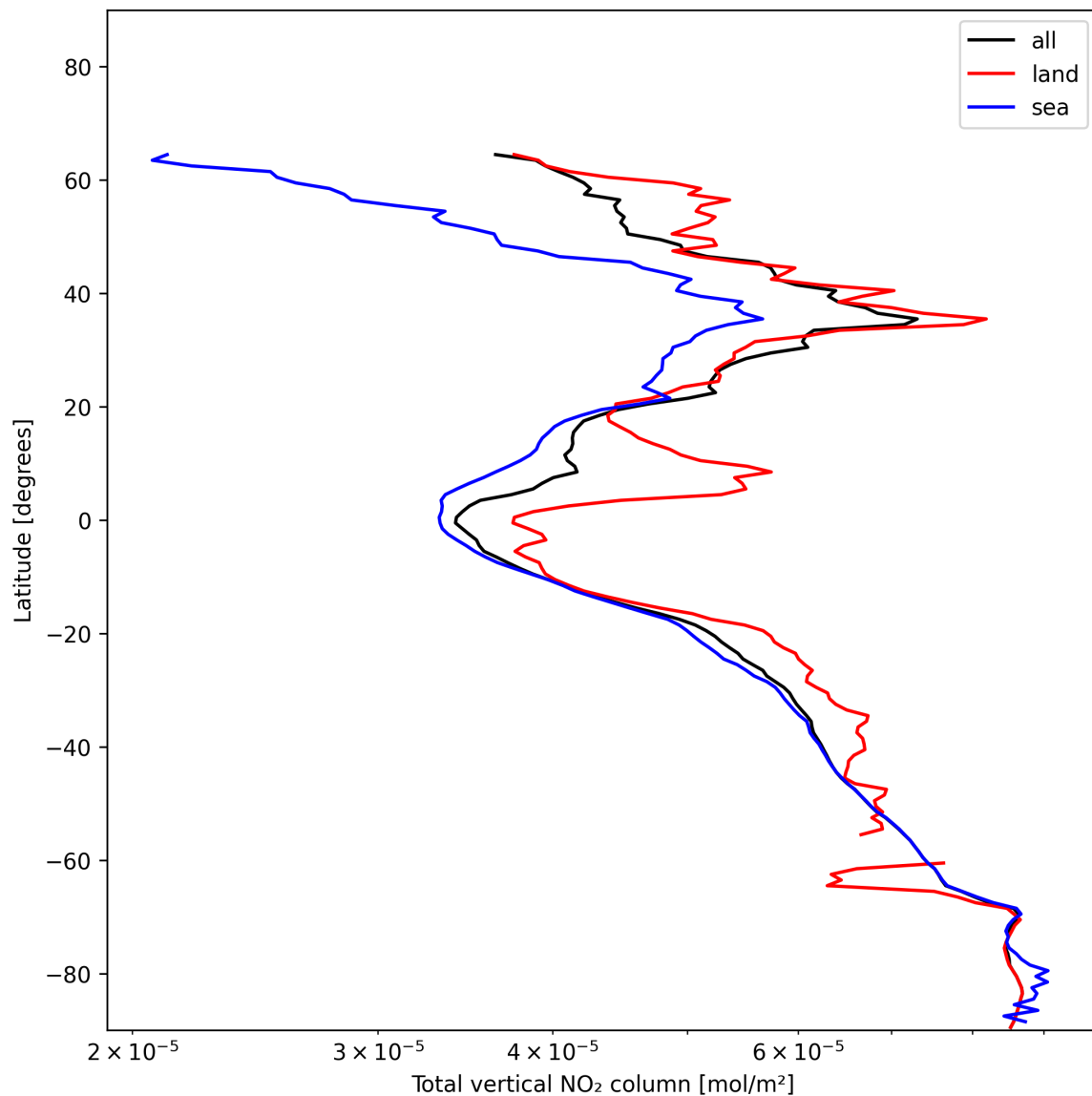
Figure 19: Zonal average of “Total vertical NO 2 column” for 2024-12-23 to 2024-12-24.
