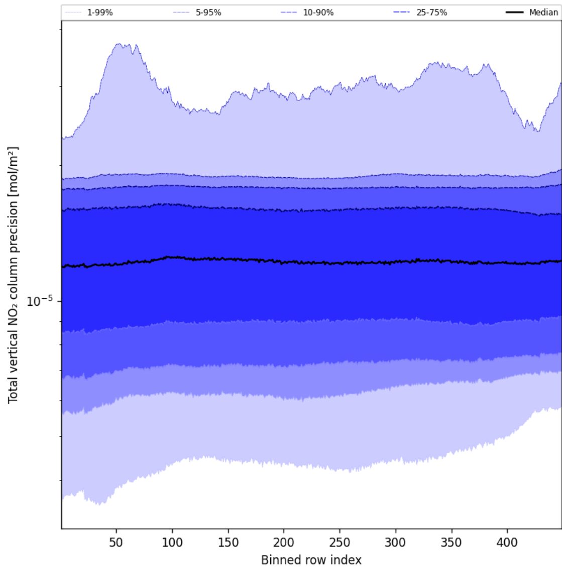
Figure 54: Along track statistics of “Total vertical NO 2 column precision” for 2024-12-23 to 2024-12-24
