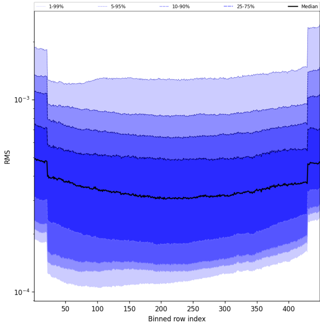
Figure 58: Along track statistics of “RMS” for 2024-12-23 to 2024-12-24
