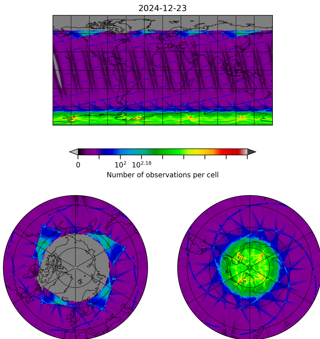
Figure 8: Map of the number of observations for 2024-12-23 to 2024-12-24
