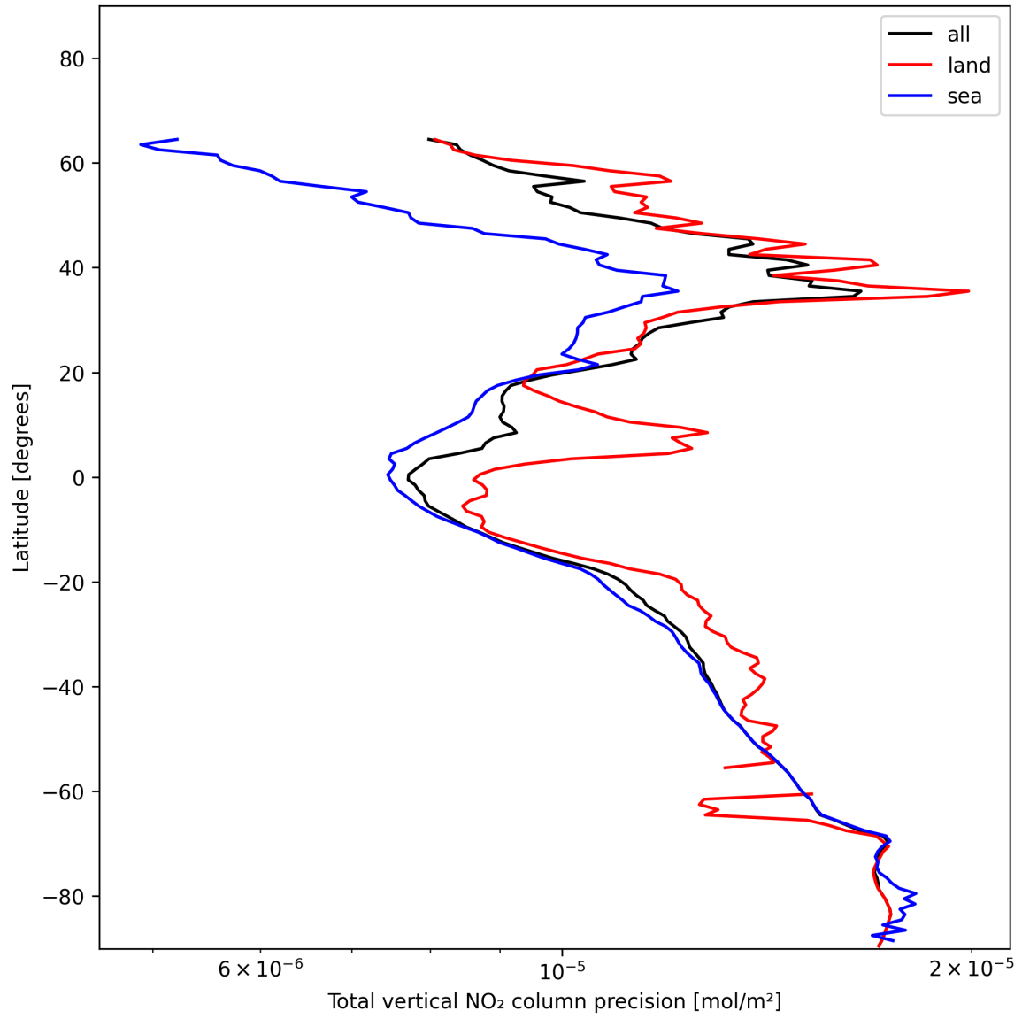
Figure 20: Zonal average of "Total vertical NO 2 column precision" for 2024-12-23 to 2024-12-24.
