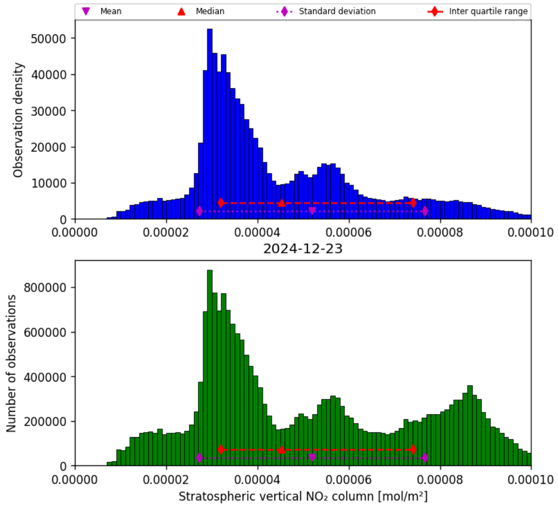
Figure 34: Histogram of “Stratospheric vertical NO 2 column” for 2024-12-23 to 2024-12-24
