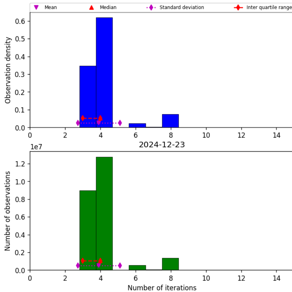
Figure 32: Histogram of “Number of iterations” for 2024-12-23 to 2024-12-24
