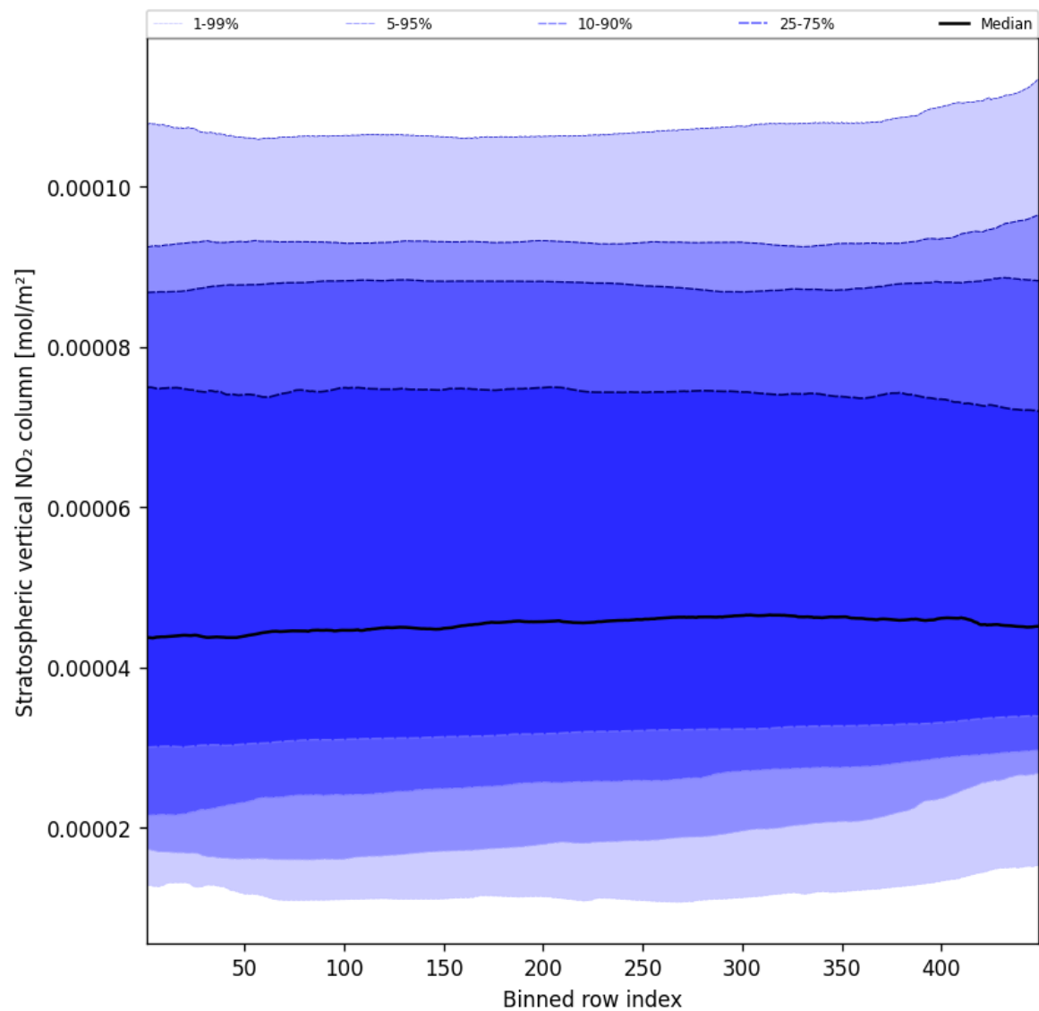
Figure 51: Along track statistics of “Stratospheric vertical NO 2 column” for 2024-12-23 to 2024-12-24
