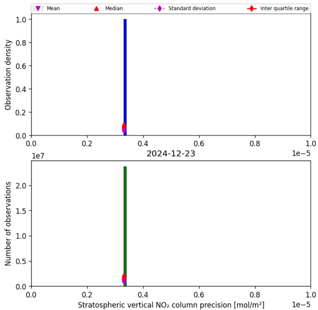
Figure 35: Histogram of “Stratospheric vertical NO 2 column precision” for 2024-12-23 to 2024-12-24
