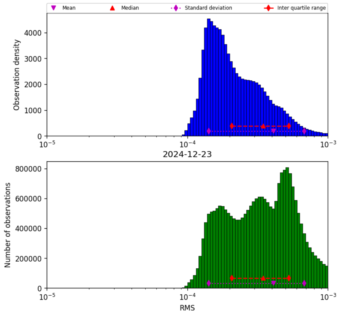
Figure 41: Histogram of “RMS” for 2024-12-23 to 2024-12-24
