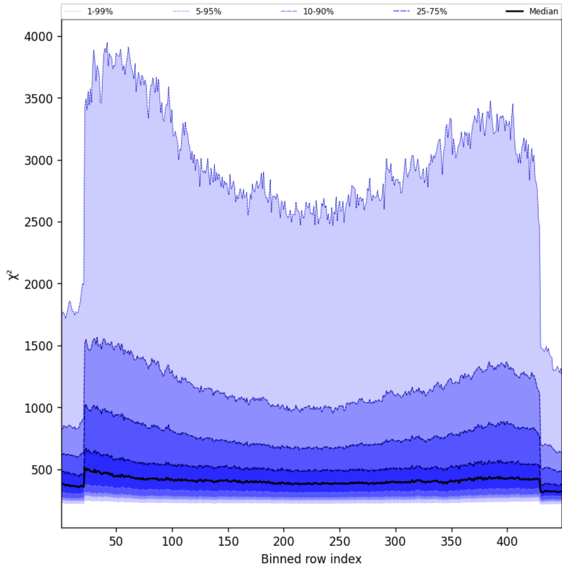
Figure 57: Along track statistics of “ \chi^2 ” for 2024-12-23 to 2024-12-24
