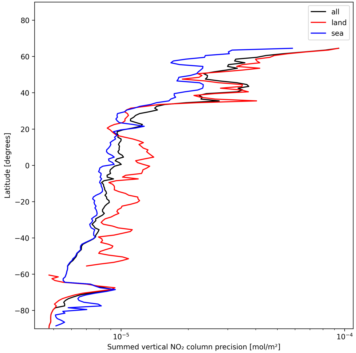
Figure 22: Zonal average of “Summed vertical NO 2 column precision” for 2024-12-23 to 2024-12-24.
