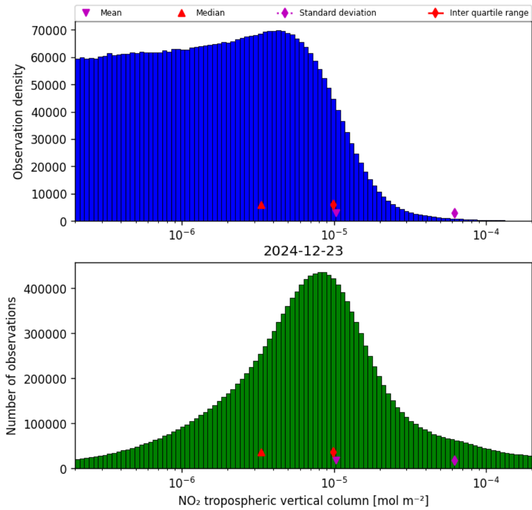
Figure 27: Histogram of “NO 2 tropospheric vertical column” for 2024-12-23 to 2024-12-24
