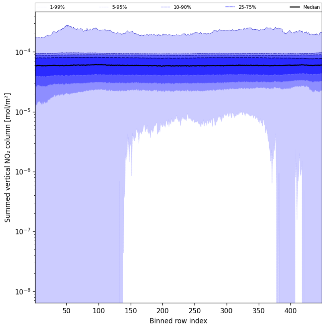
Figure 55: Along track statistics of “Summed vertical NO 2 column” for 2024-12-23 to 2024-12-24
