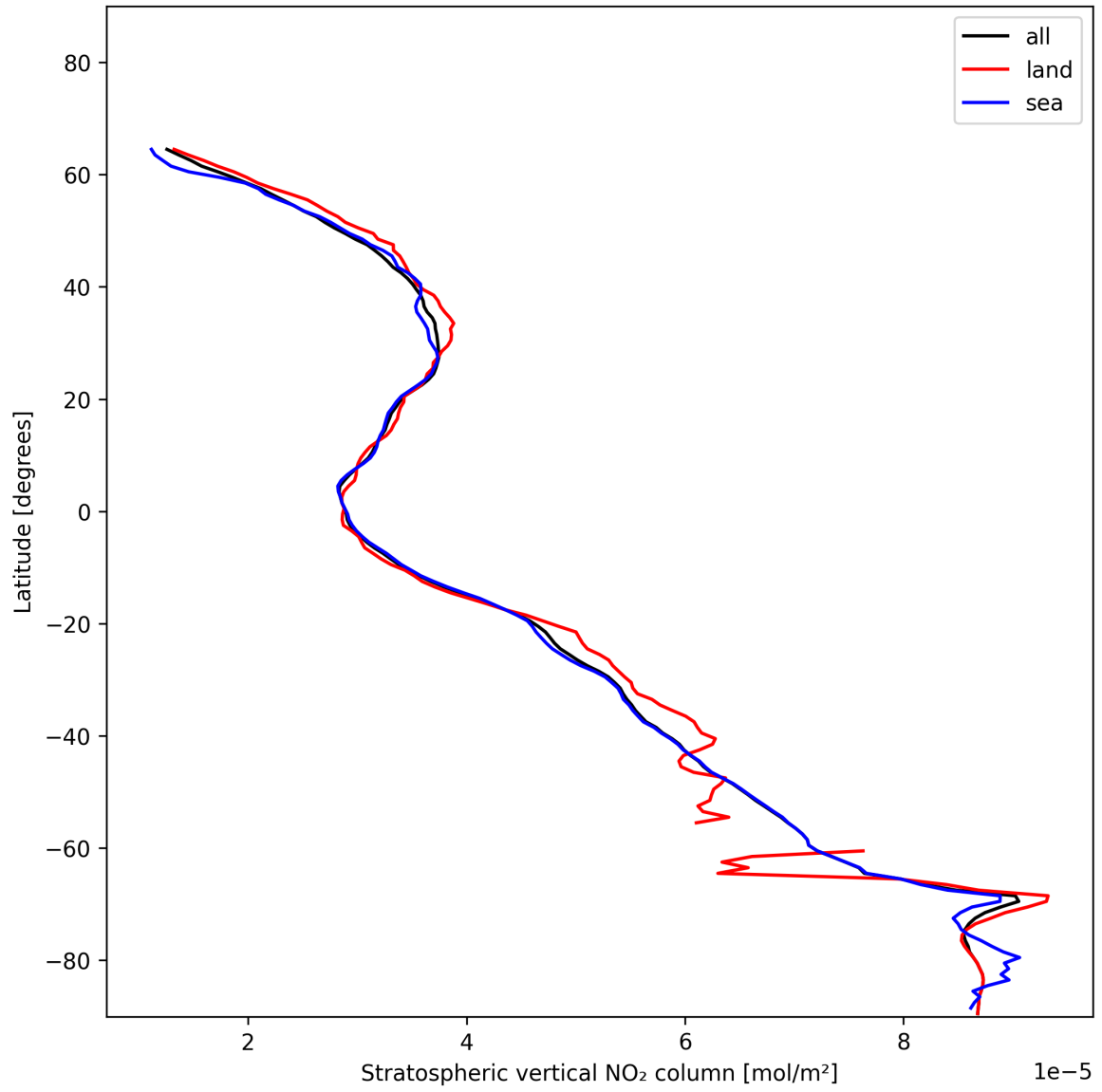
Figure 17: Zonal average of “Stratospheric vertical NO 2 column” for 2024-12-23 to 2024-12-24.
