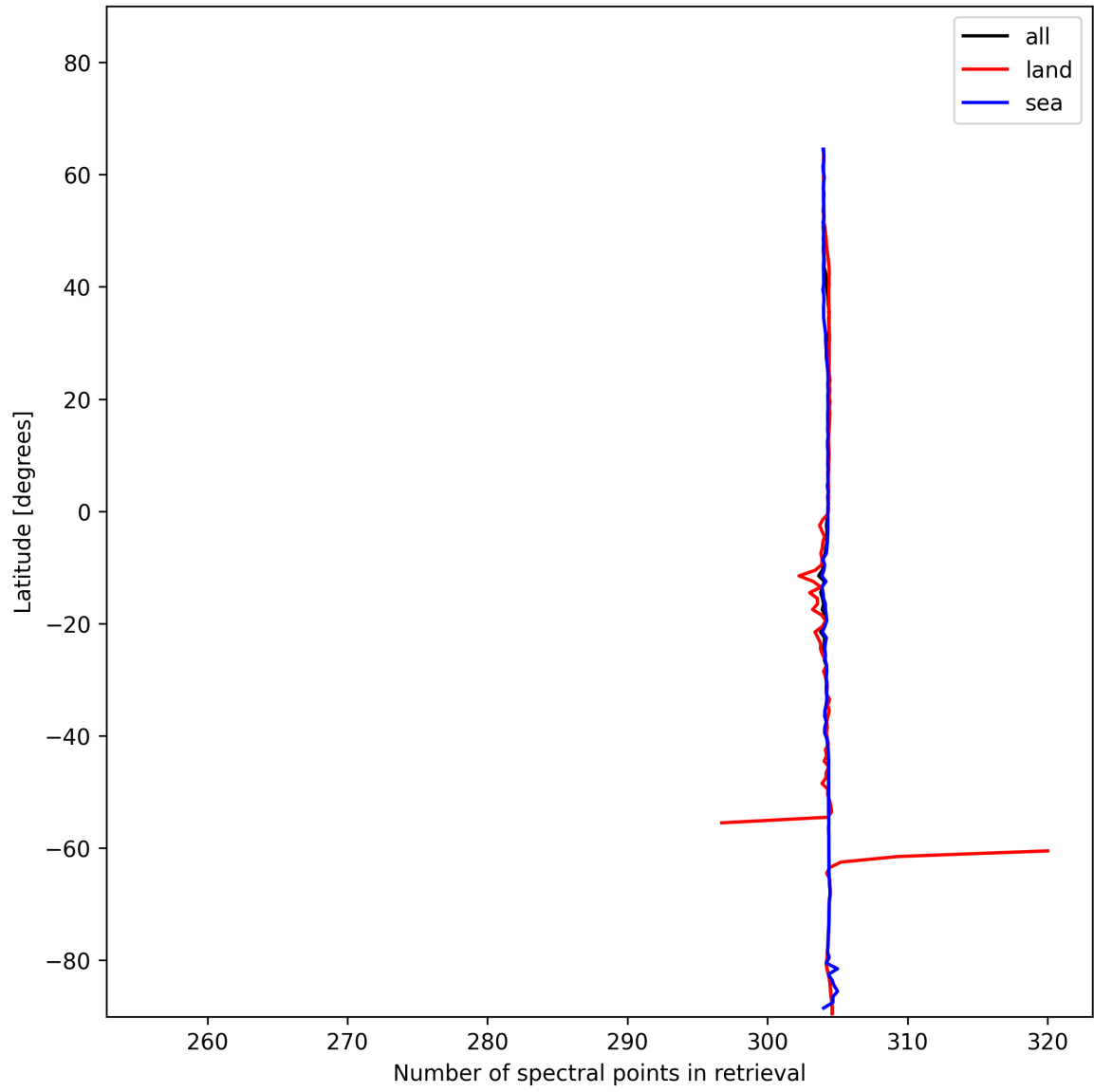
Figure 14: Zonal average of “Number of spectral points in retrieval” for 2024-12-23 to 2024-12-24.
