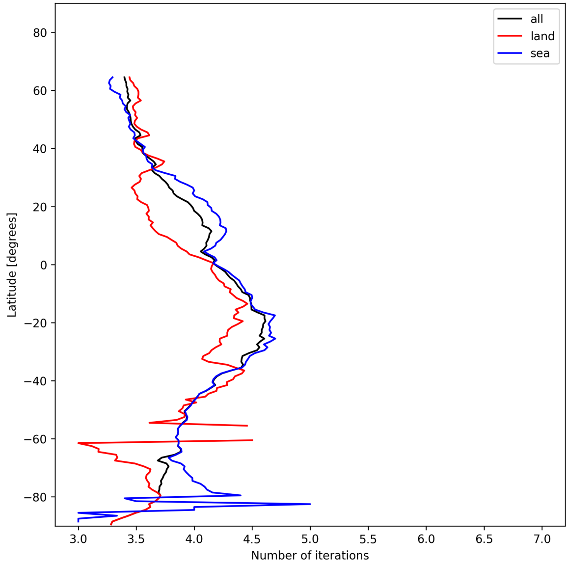
Figure 15: Zonal average of “Number of iterations” for 2024-12-23 to 2024-12-24.
