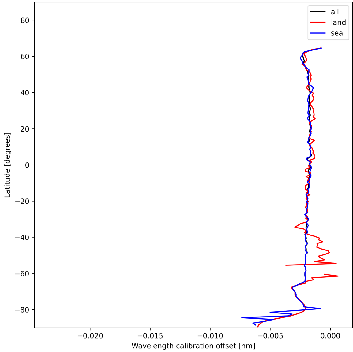
Figure 16: Zonal average of “Wavelength calibration offset” for 2024-12-23 to 2024-12-24.
