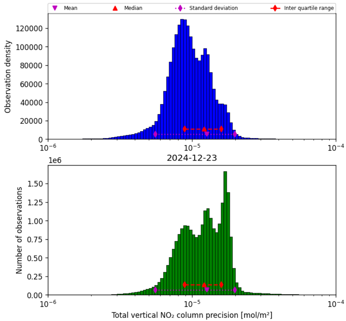
Figure 37: Histogram of “Total vertical NO 2 column precision” for 2024-12-23 to 2024-12-24
