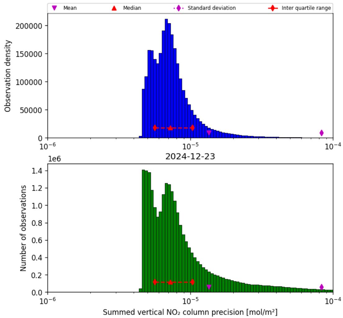
Figure 39: Histogram of “Summed vertical NO 2 column precision” for 2024-12-23 to 2024-12-24
