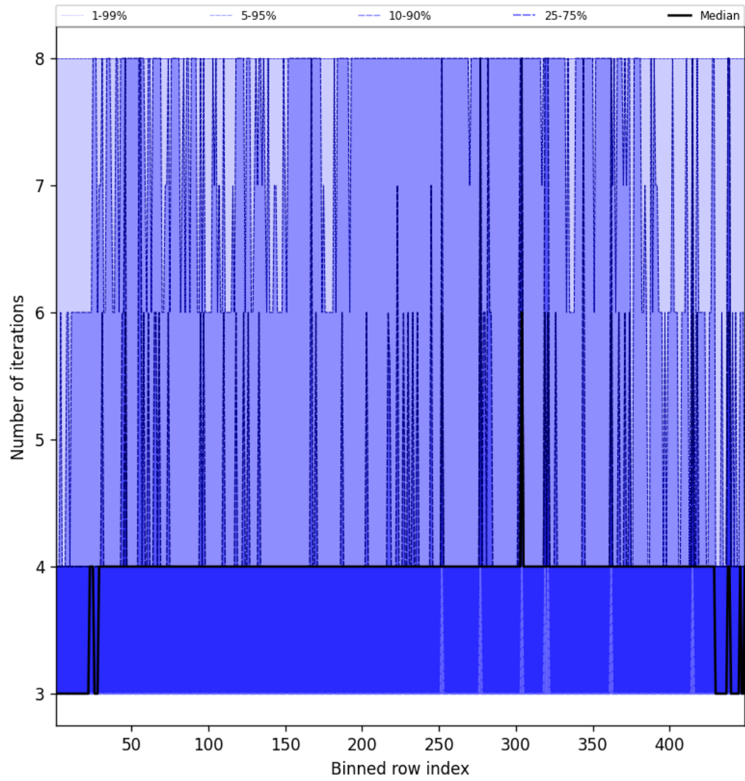
Figure 49: Along track statistics of “Number of iterations” for 2024-12-23 to 2024-12-24
