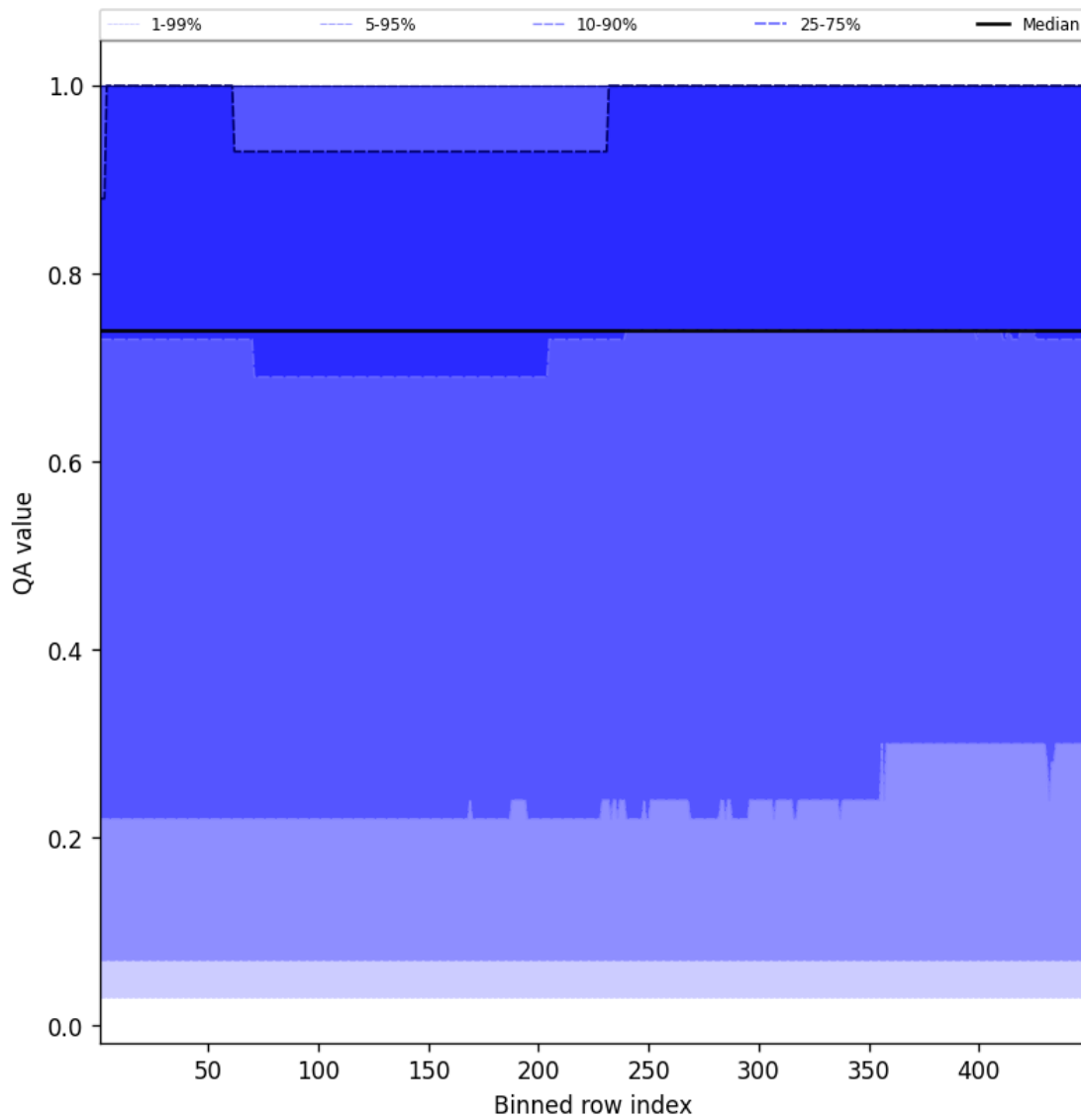
Figure 43: Along track statistics of “QA value” for 2024-12-23 to 2024-12-24
