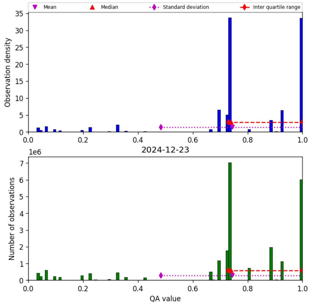
Figure 26: Histogram of “QA value” for 2024-12-23 to 2024-12-24
