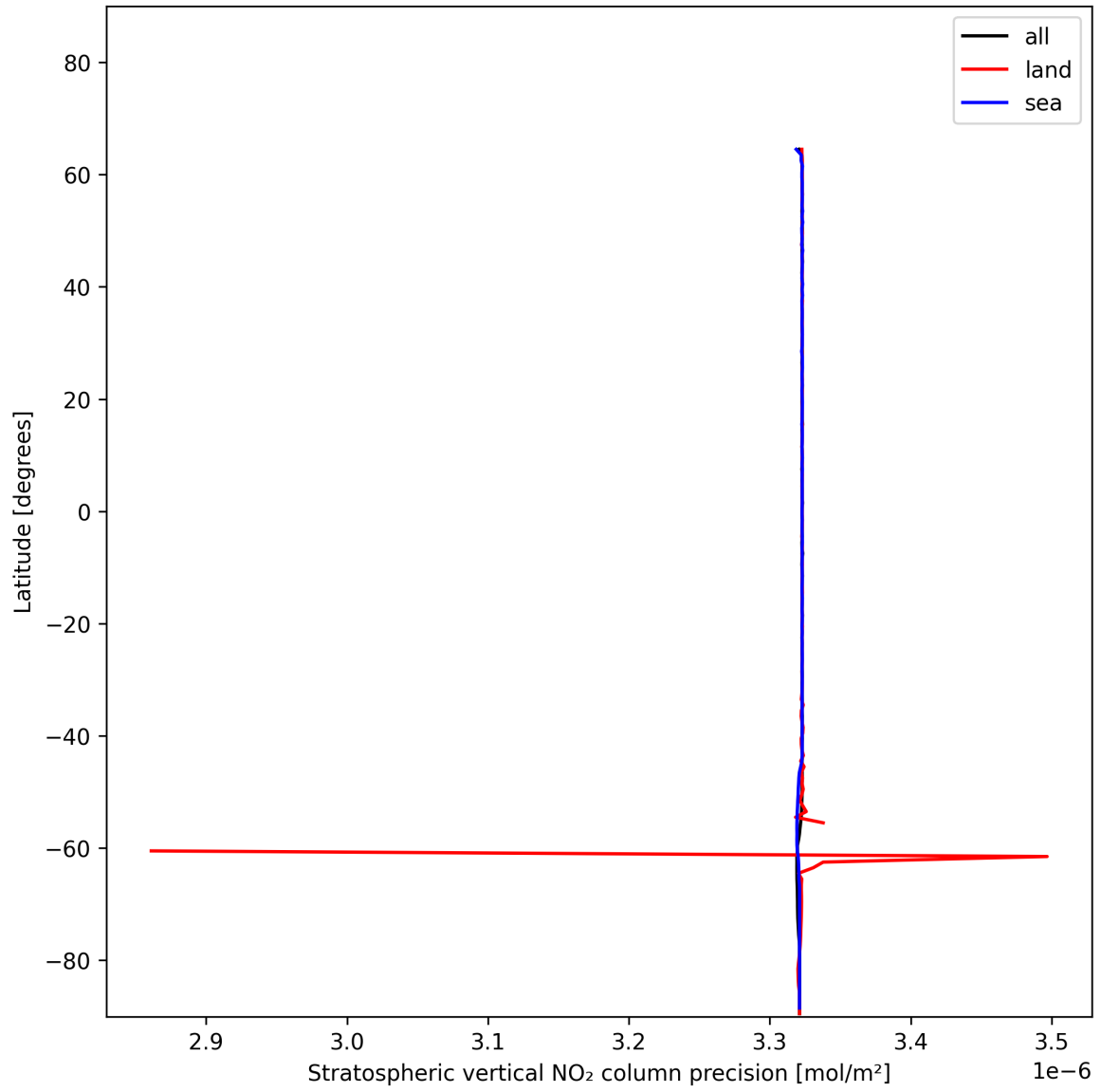
Figure 18: Zonal average of “Stratospheric vertical NO 2 column precision” for 2024-12-23 to 2024-12-24.
