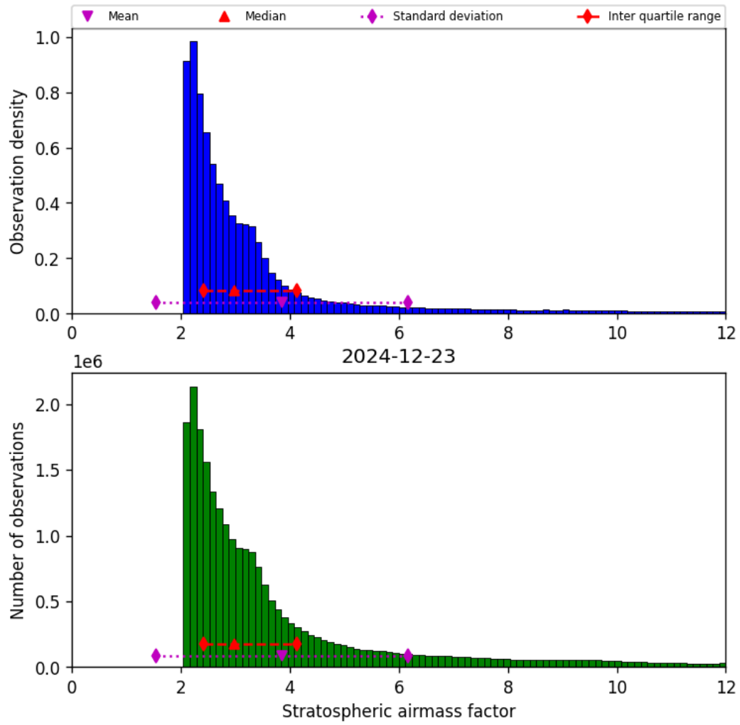
Figure 42: Histogram of “Stratospheric airmass factor” for 2024-12-23 to 2024-12-24
