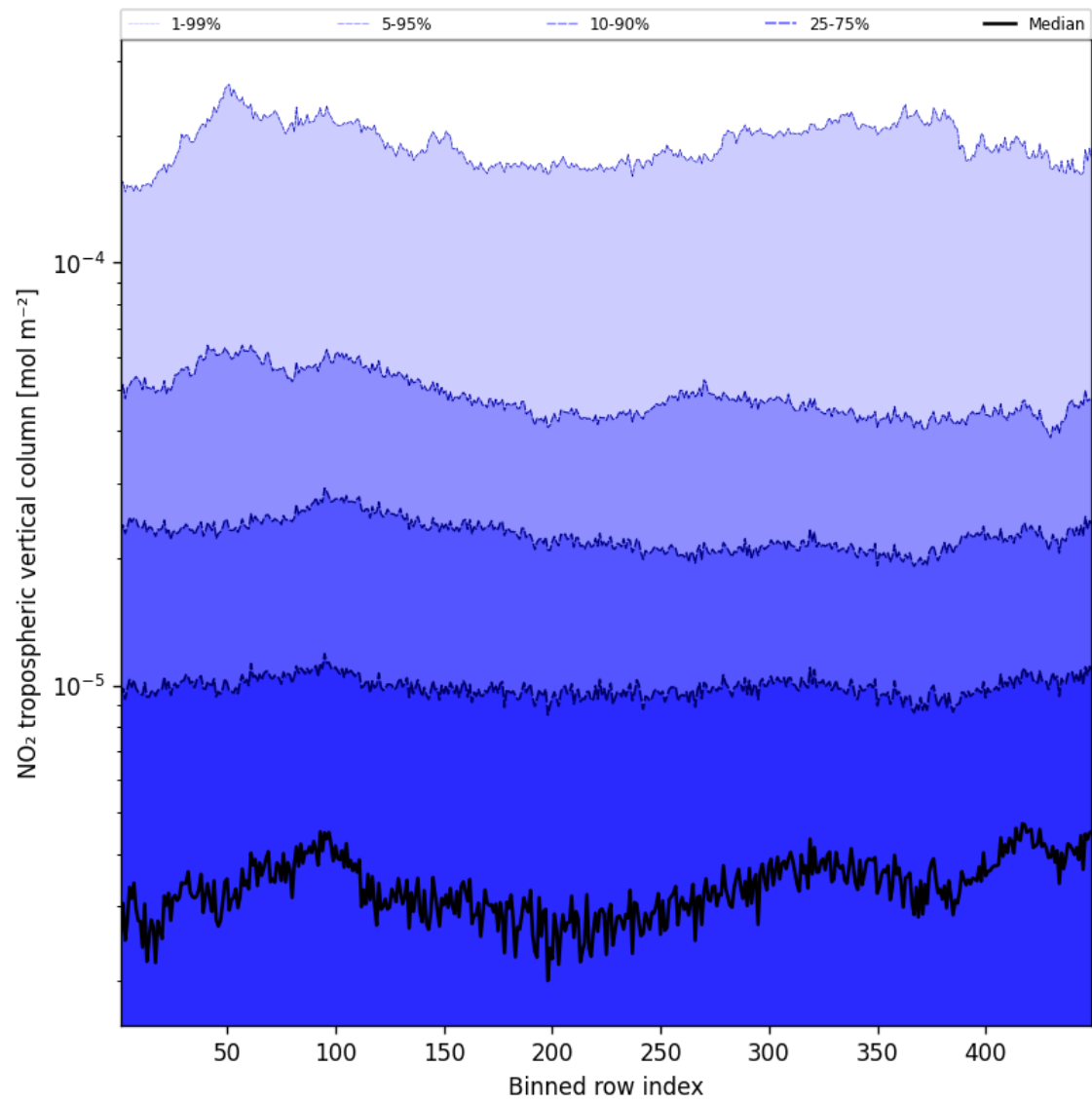
Figure 44: Along track statistics of “NO 2 tropospheric vertical column” for 2024-12-23 to 2024-12-24
