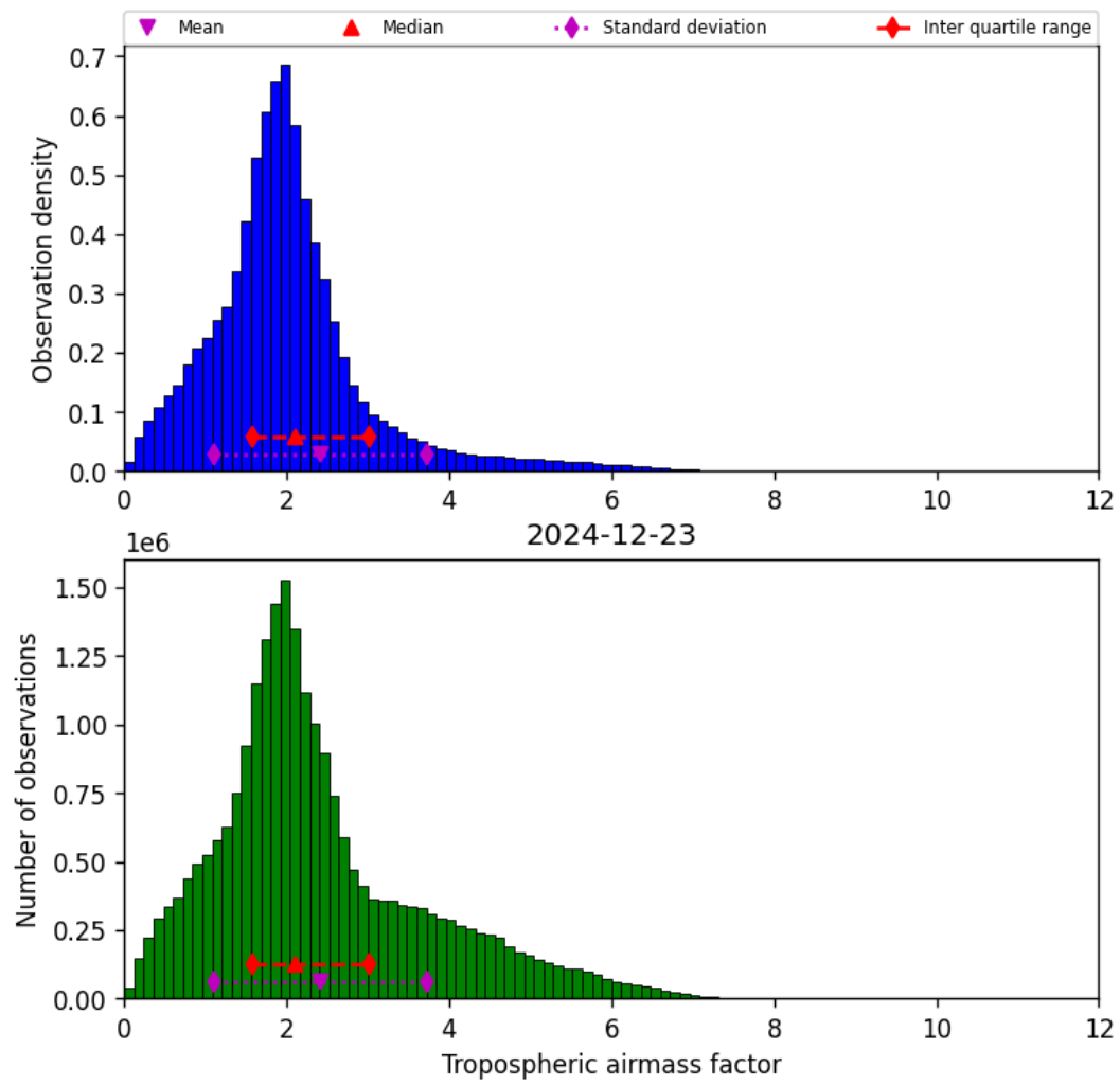
Figure 29: Histogram of “Tropospheric airmass factor” for 2024-12-23 to 2024-12-24
