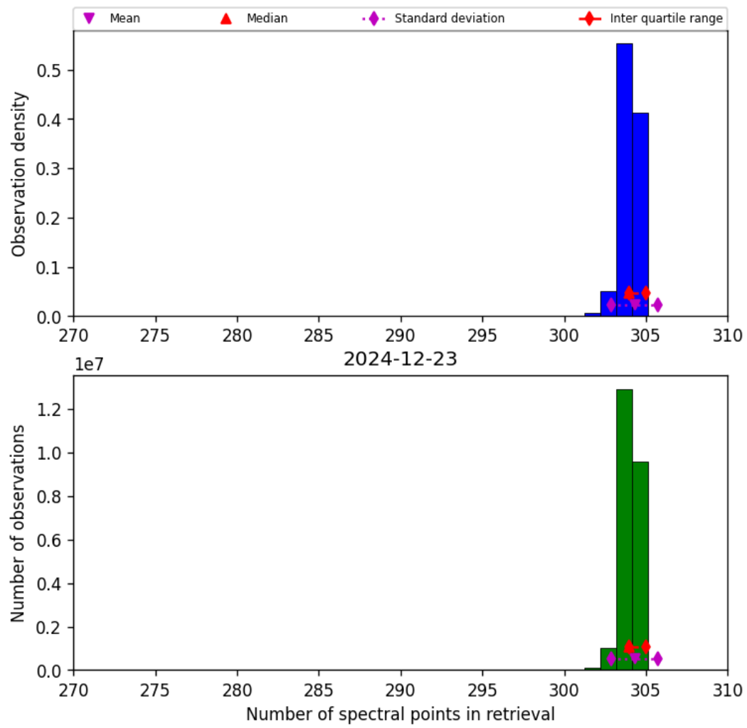
Figure 31: Histogram of “Number of spectral points in retrieval” for 2024-12-23 to 2024-12-24
