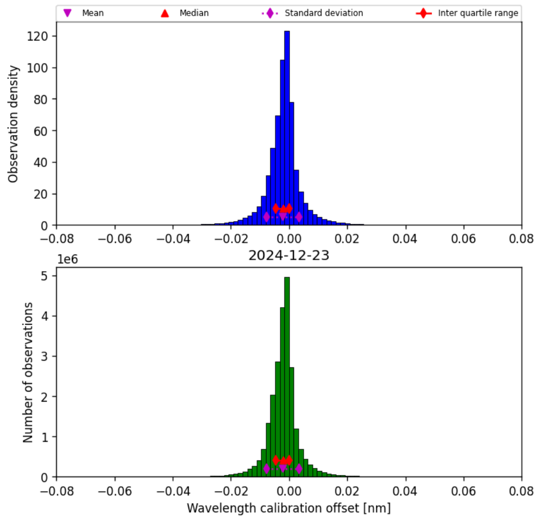
Figure 33: Histogram of “Wavelength calibration offset” for 2024-12-23 to 2024-12-24
