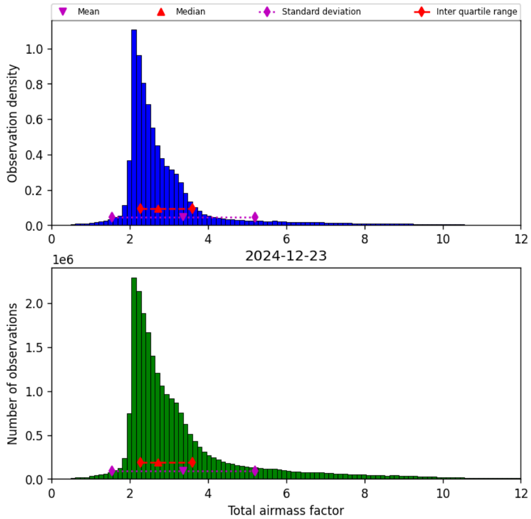
Figure 30: Histogram of “Total airmass factor” for 2024-12-23 to 2024-12-24
