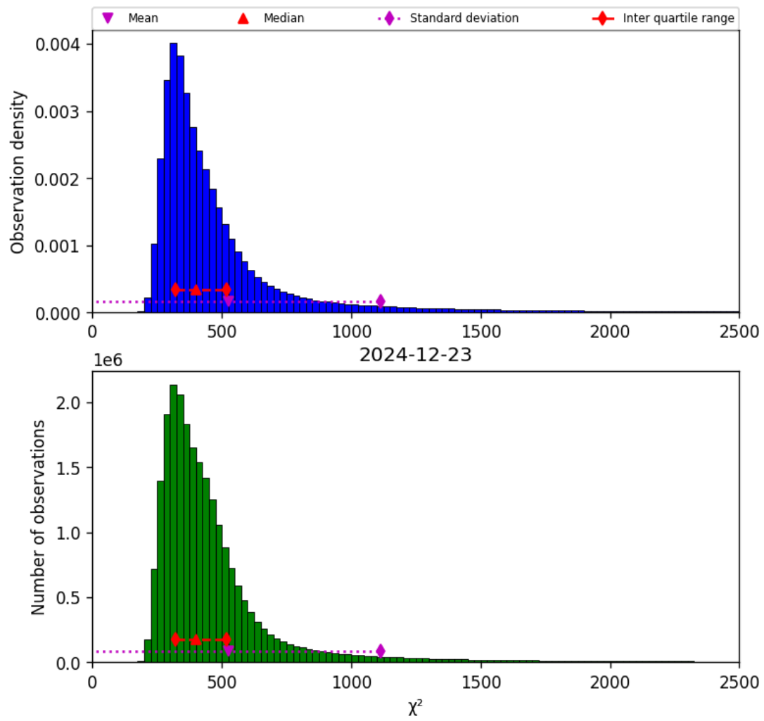
Figure 40: Histogram of “ \chi^2 ” for 2024-12-23 to 2024-12-24
