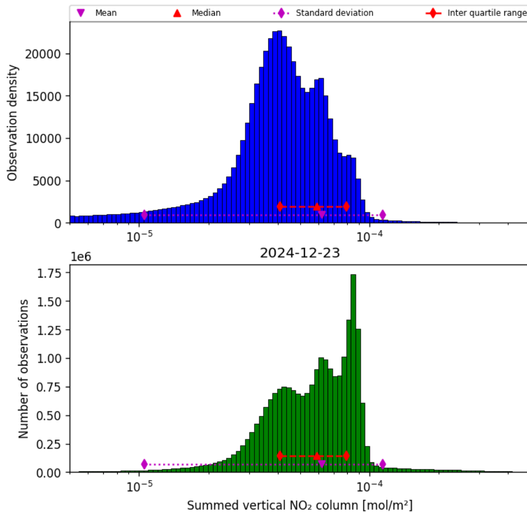
Figure 38: Histogram of “Summed vertical NO 2 column” for 2024-12-23 to 2024-12-24
