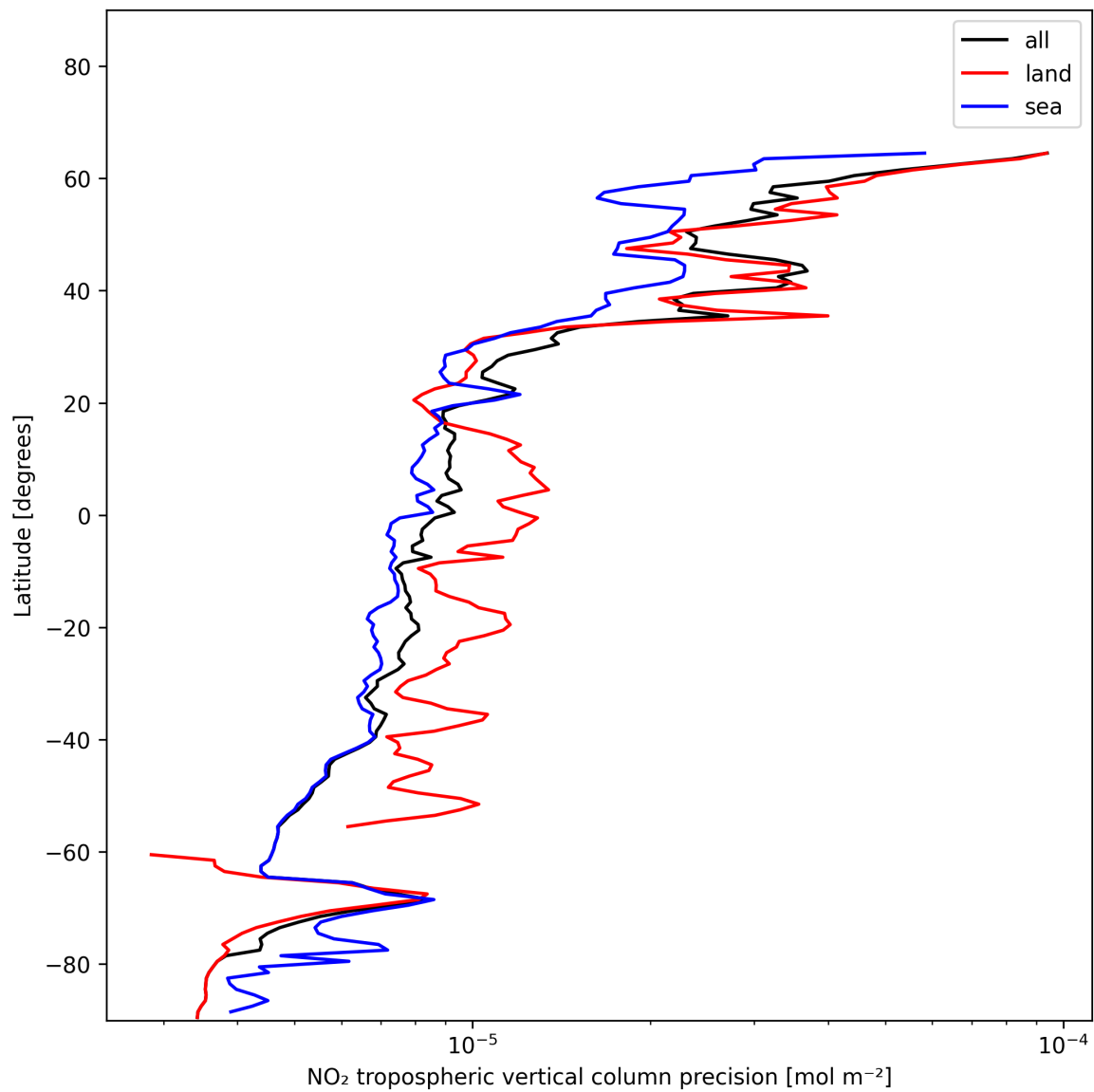
Figure 11: Zonal average of “NO 2 tropospheric vertical column precision” for 2024-12-23 to 2024-12-24.
