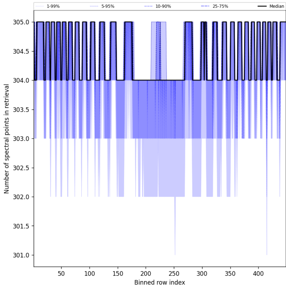
Figure 48: Along track statistics of “Number of spectral points in retrieval” for 2024-12-23 to 2024-12-24
