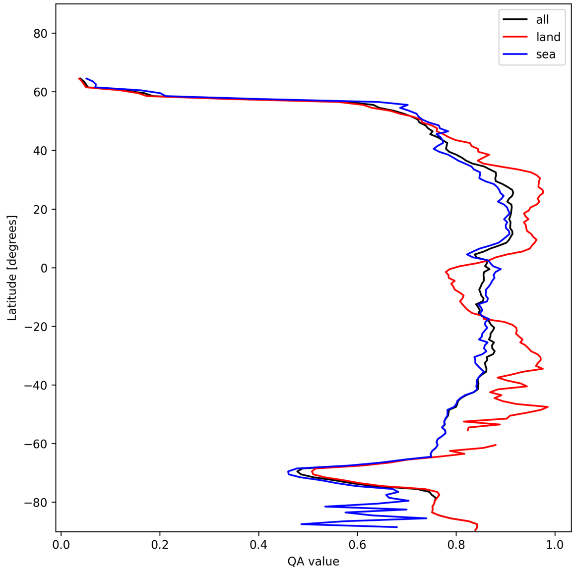
Figure 9: Zonal average of “QA value” for 2024-12-23 to 2024-12-24.
