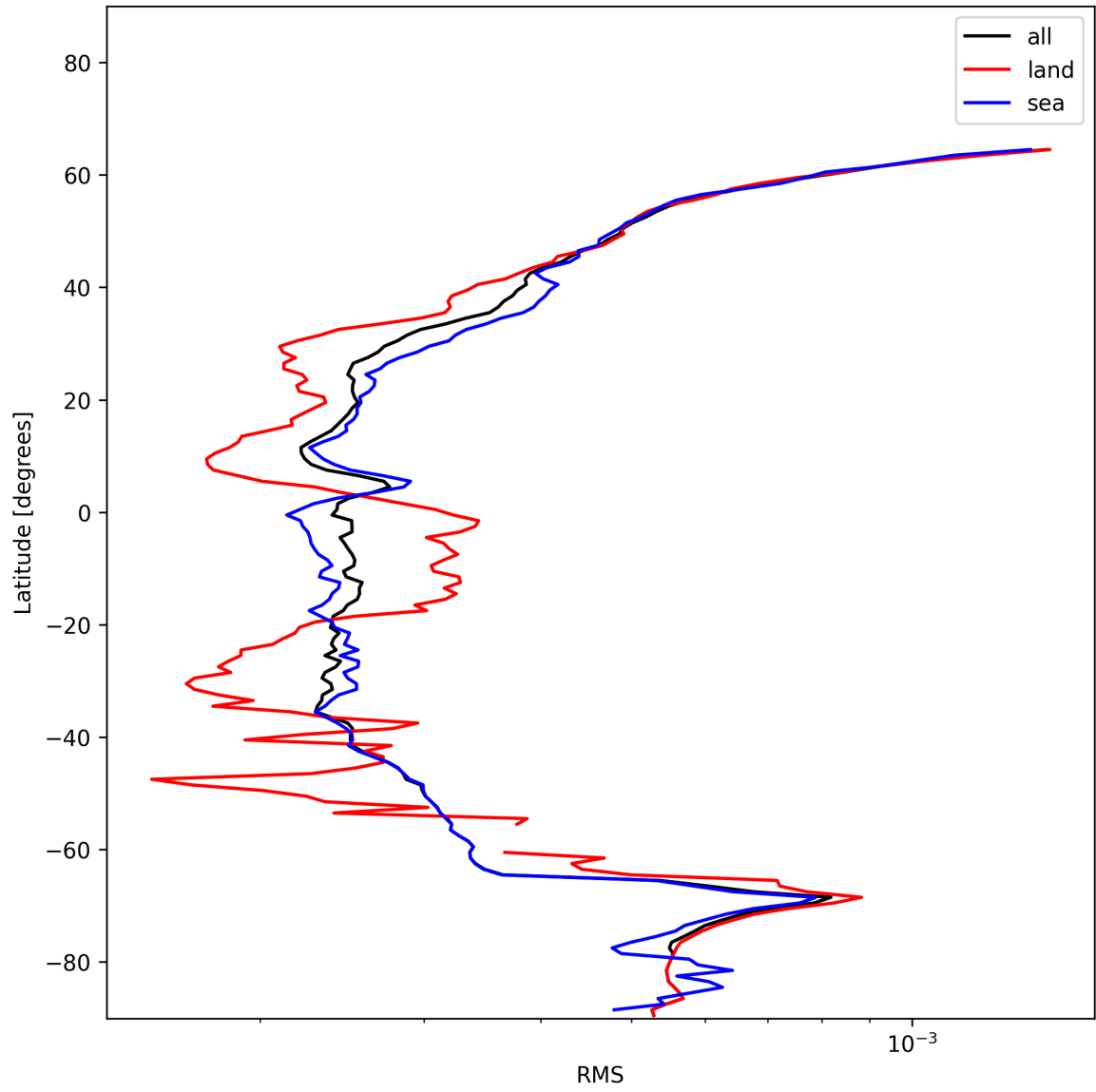
Figure 24: Zonal average of “RMS” for 2024-12-23 to 2024-12-24.
