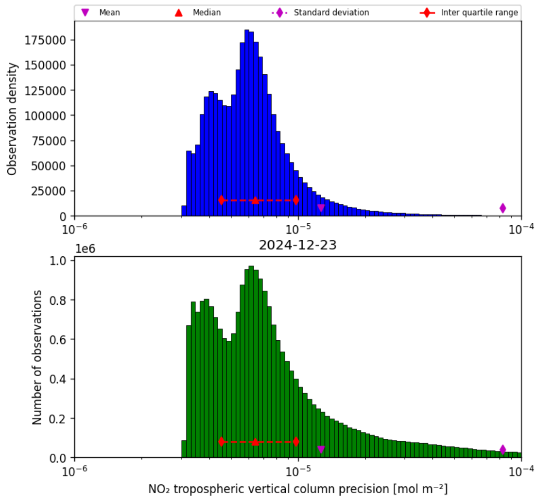
Figure 28: Histogram of “NO 2 tropospheric vertical column precision” for 2024-12-23 to 2024-12-24
