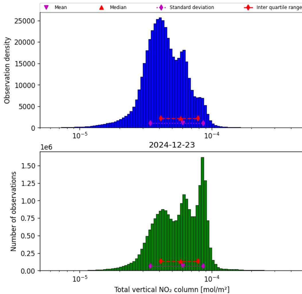
Figure 36: Histogram of “Total vertical NO 2 column” for 2024-12-23 to 2024-12-24
