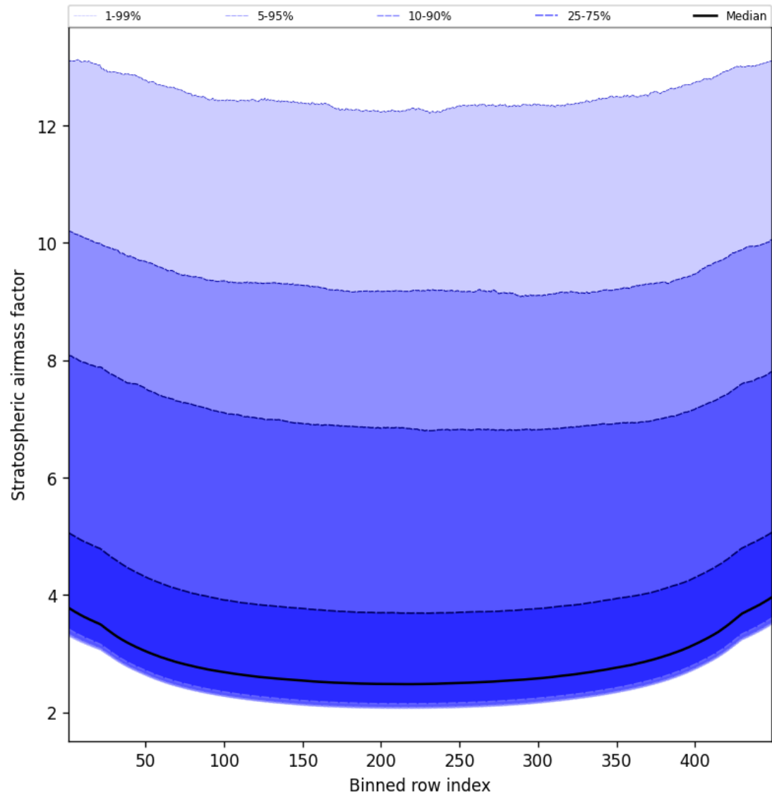
Figure 59: Along track statistics of “Stratospheric airmass factor” for 2024-12-23 to 2024-12-24
