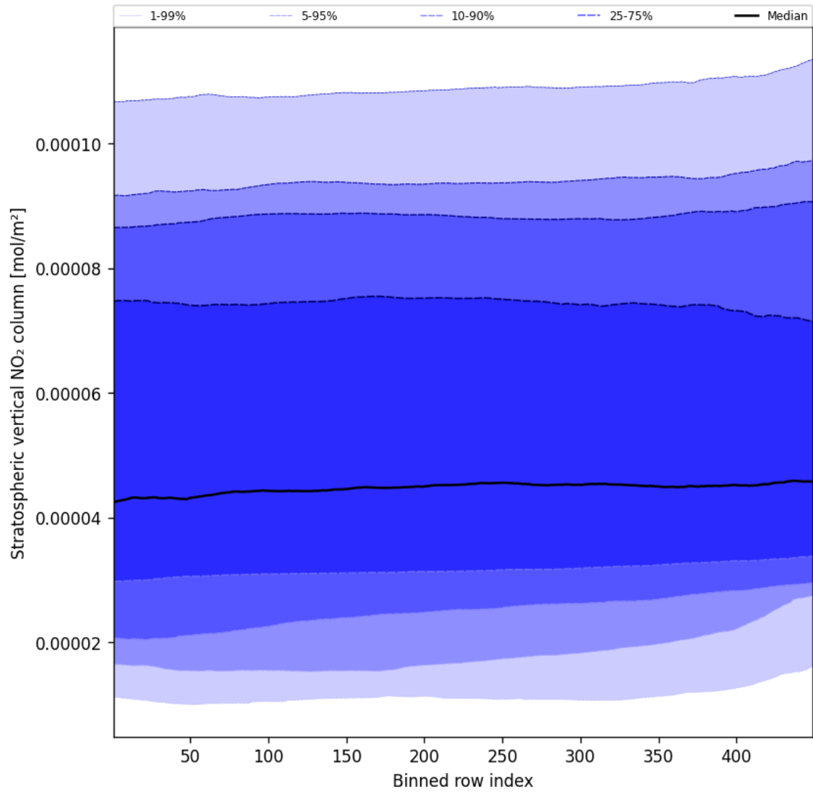
Figure 51: Along track statistics of “Stratospheric vertical NO 2 column” for 2024-12-24 to 2024-12-25
