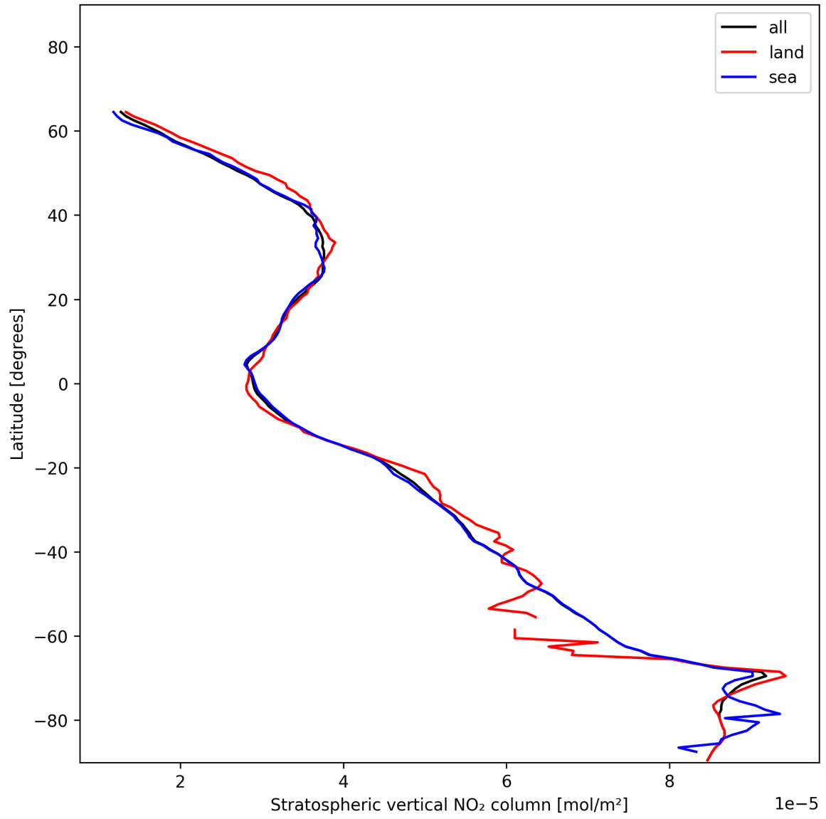
Figure 17: Zonal average of “Stratospheric vertical NO 2 column” for 2024-12-24 to 2024-12-25.
