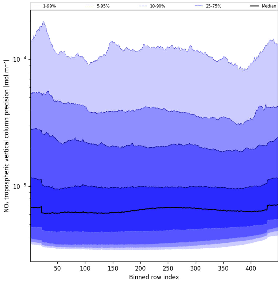
Figure 45: Along track statistics of “NO 2 tropospheric vertical column precision” for 2024-12-24 to 2024-12-25
