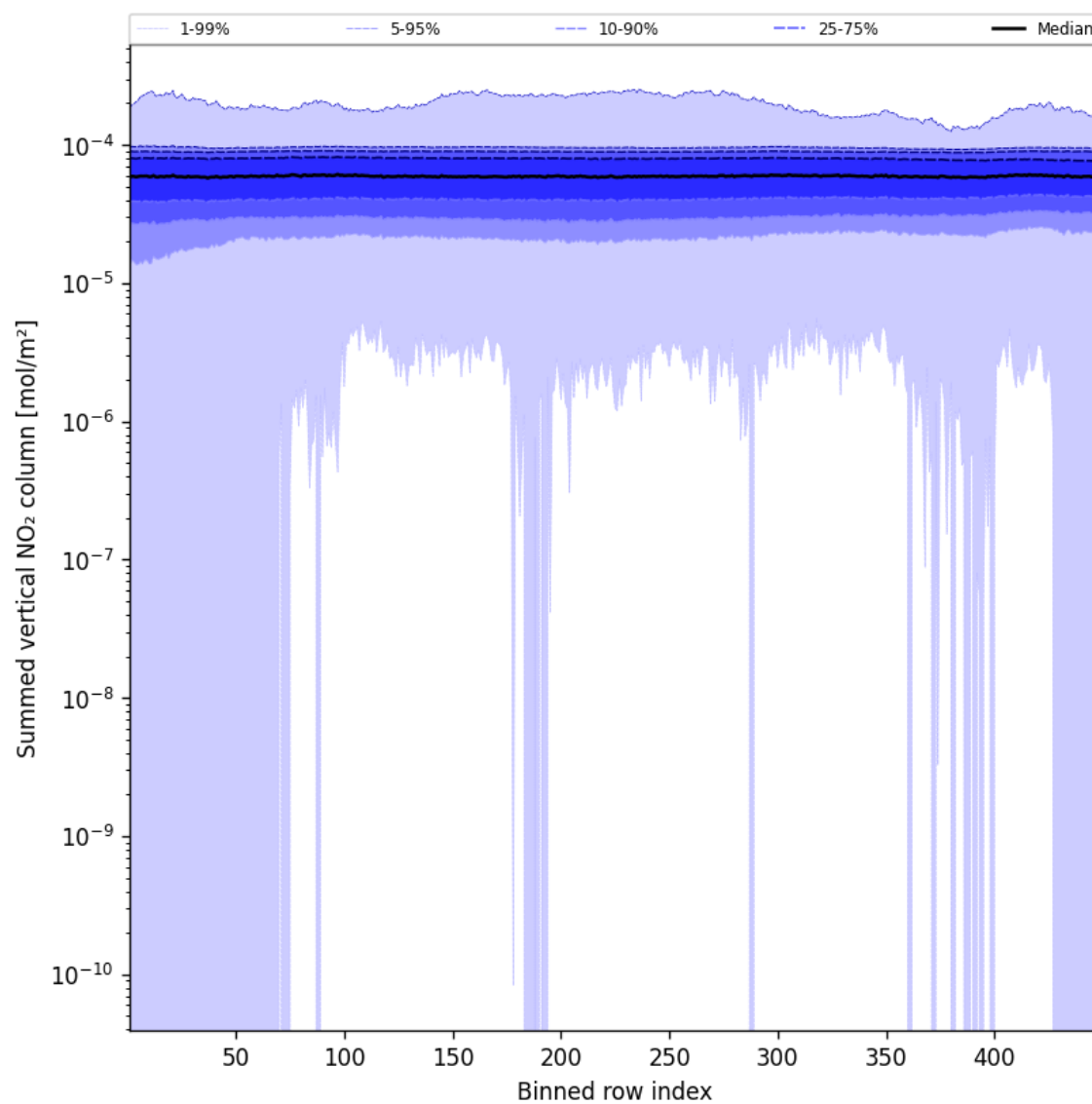
Figure 55: Along track statistics of “Summed vertical NO 2 column” for 2024-12-24 to 2024-12-25
