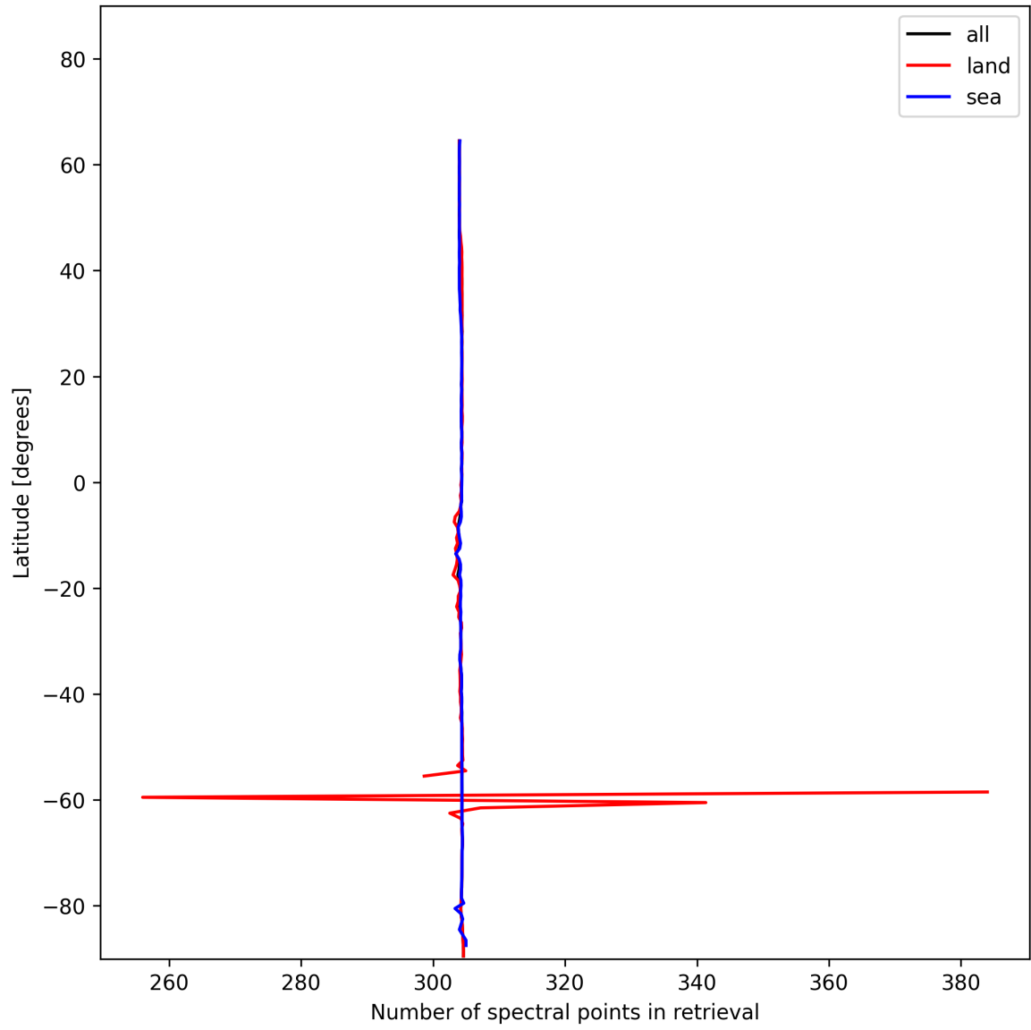
Figure 14: Zonal average of “Number of spectral points in retrieval” for 2024-12-24 to 2024-12-25.
