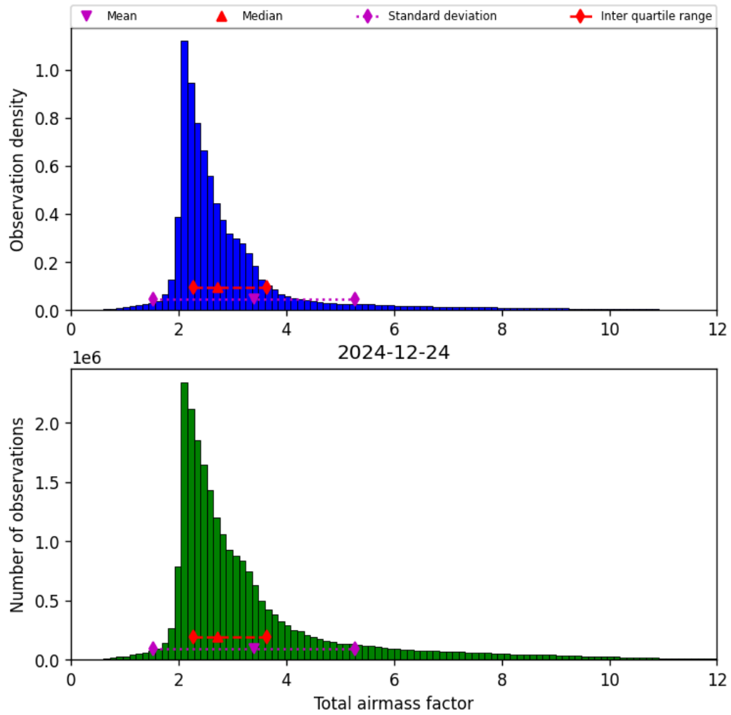
Figure 30: Histogram of “Total airmass factor” for 2024-12-24 to 2024-12-25
