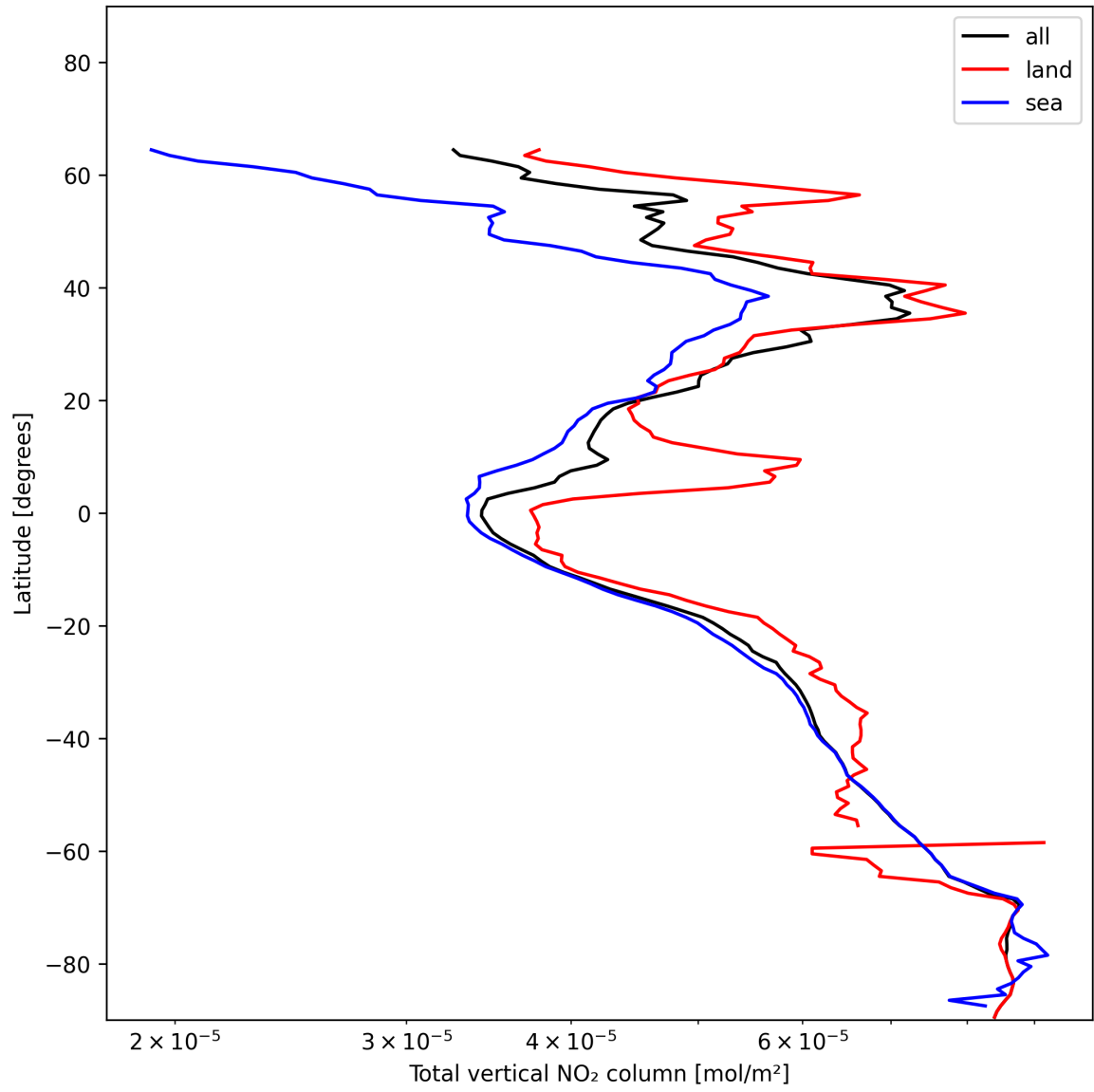
Figure 19: Zonal average of “Total vertical NO 2 column” for 2024-12-24 to 2024-12-25.
