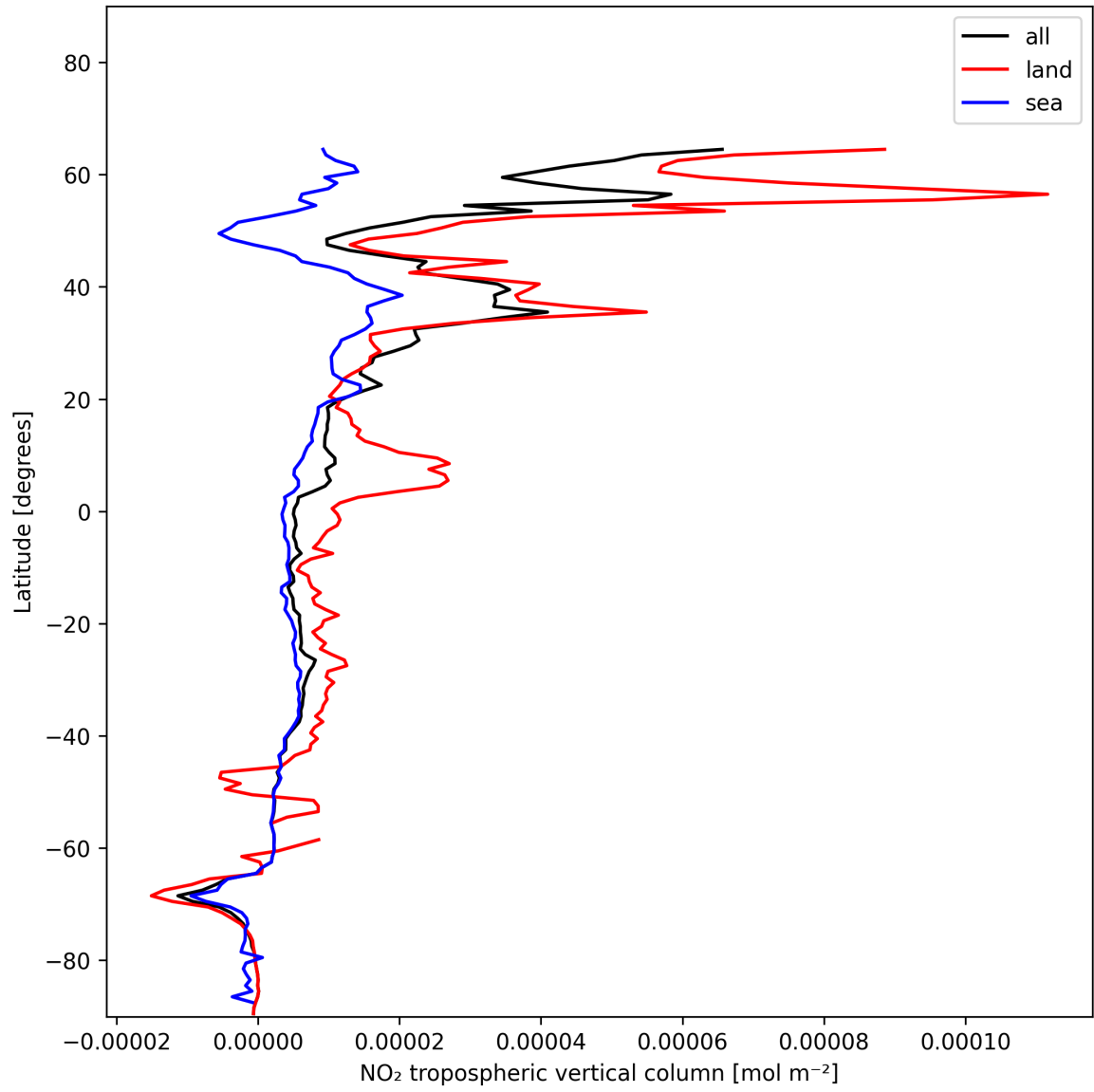
Figure 10: Zonal average of “NO 2 tropospheric vertical column” for 2024-12-24 to 2024-12-25.
