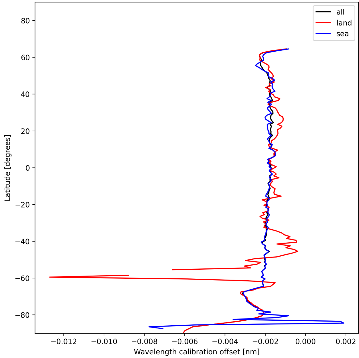
Figure 16: Zonal average of “Wavelength calibration offset” for 2024-12-24 to 2024-12-25.
