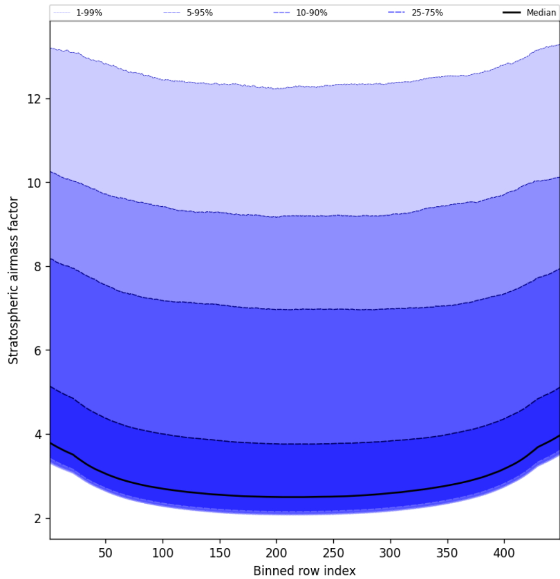
Figure 59: Along track statistics of “Stratospheric airmass factor” for 2024-12-24 to 2024-12-25
