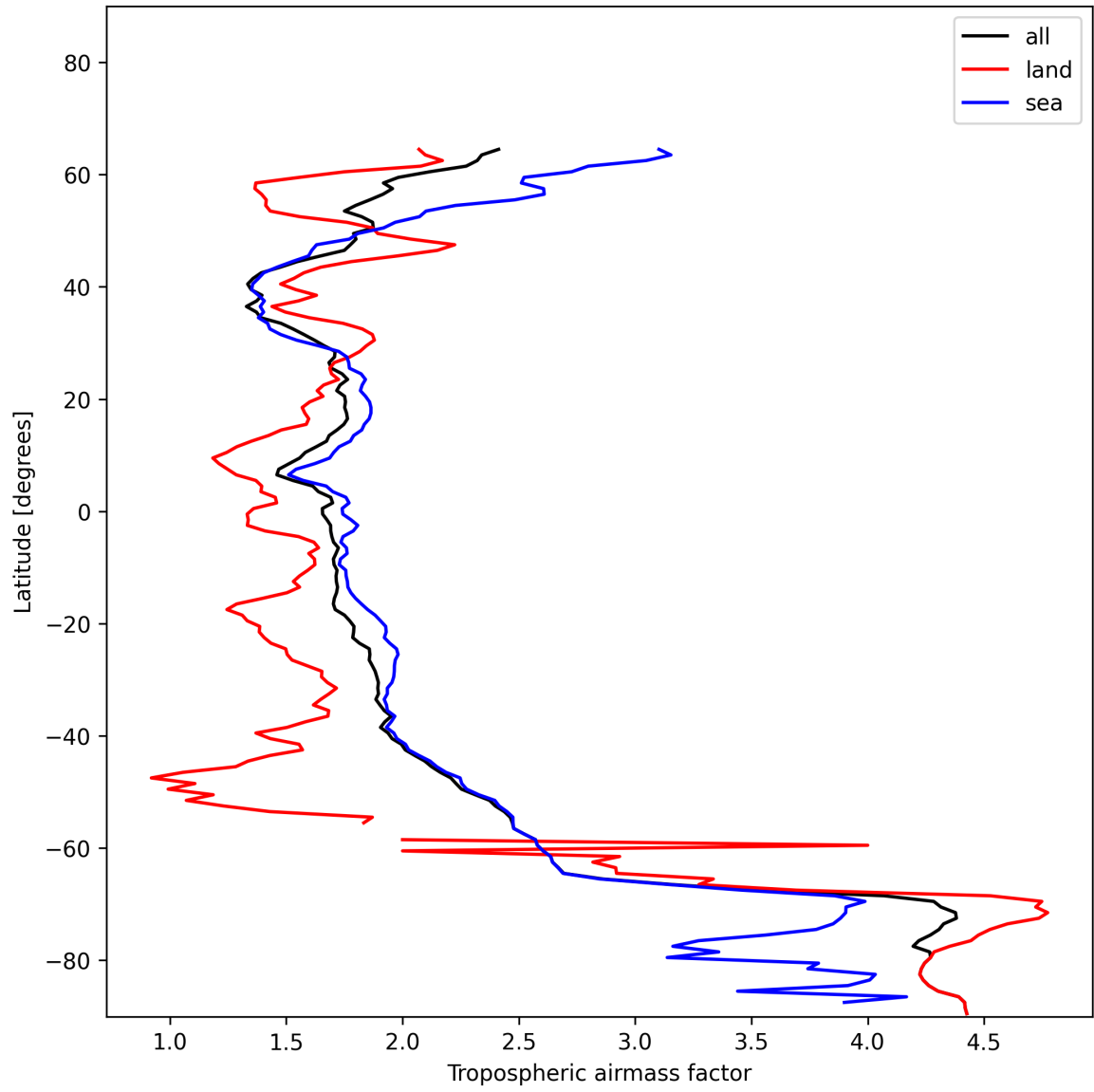
Figure 12: Zonal average of “Tropospheric airmass factor” for 2024-12-24 to 2024-12-25.
