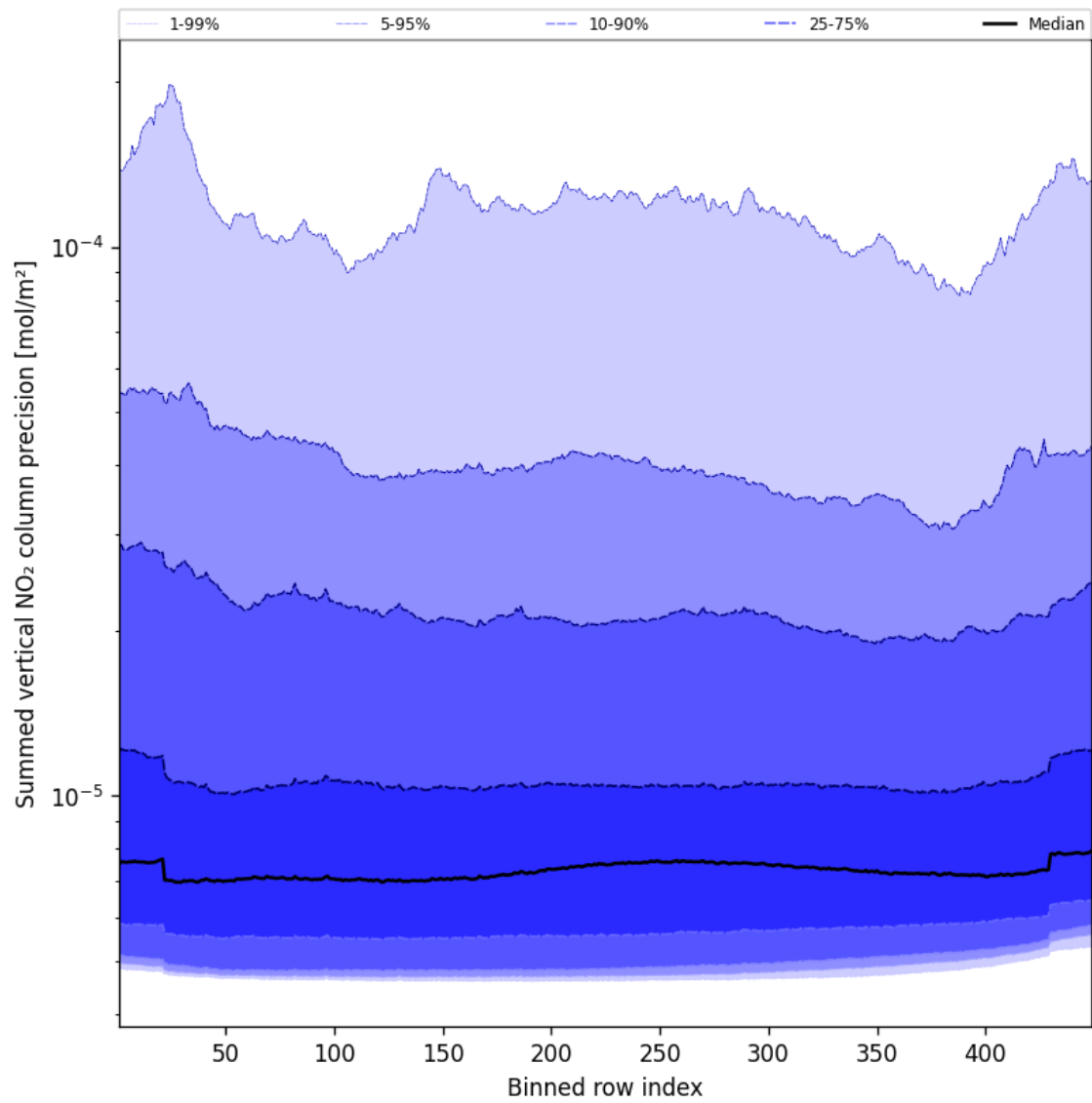
Figure 56: Along track statistics of “Summed vertical NO 2 column precision” for 2024-12-24 to 2024-12-25
