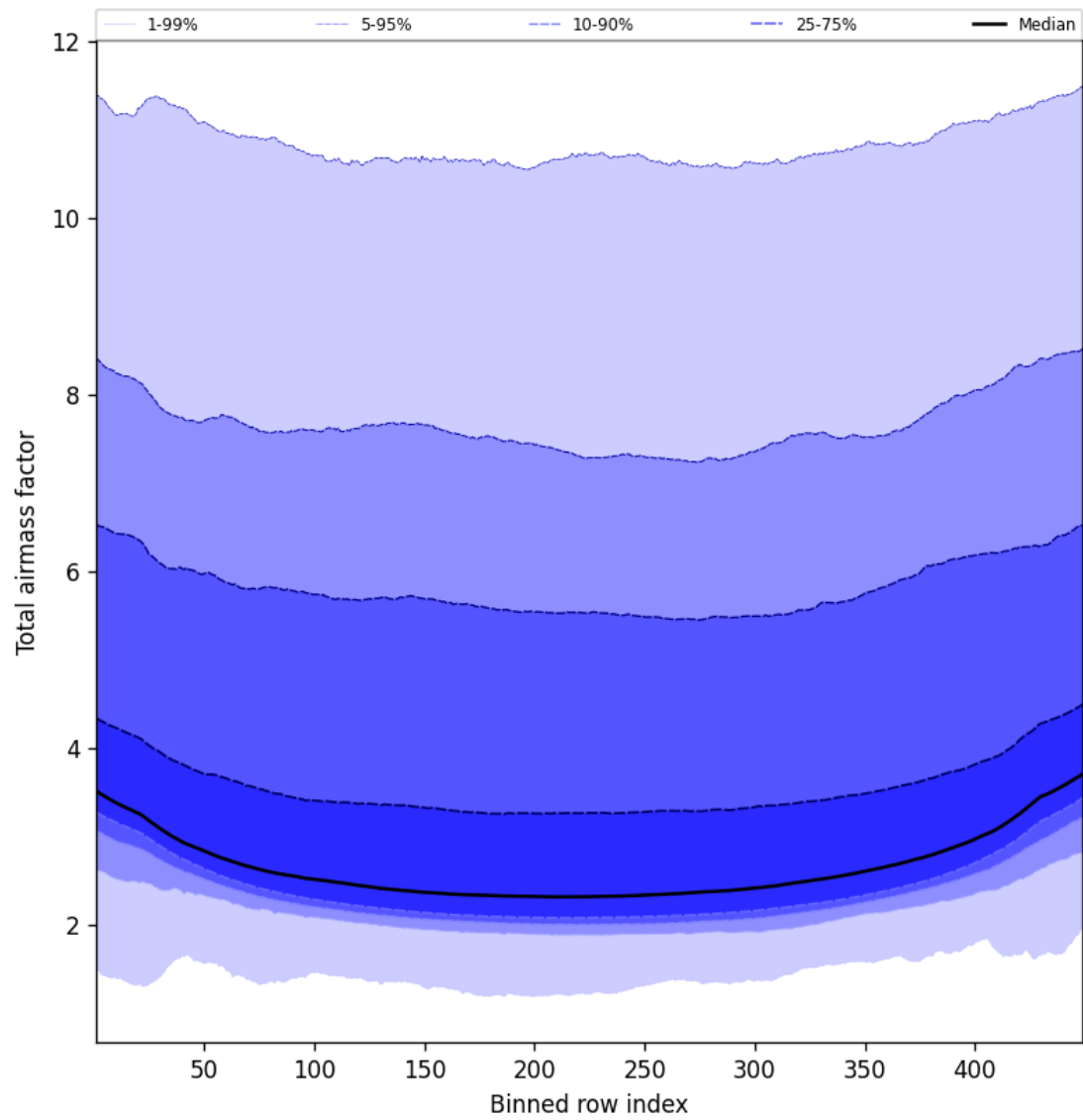
Figure 47: Along track statistics of “Total airmass factor” for 2024-12-24 to 2024-12-25
