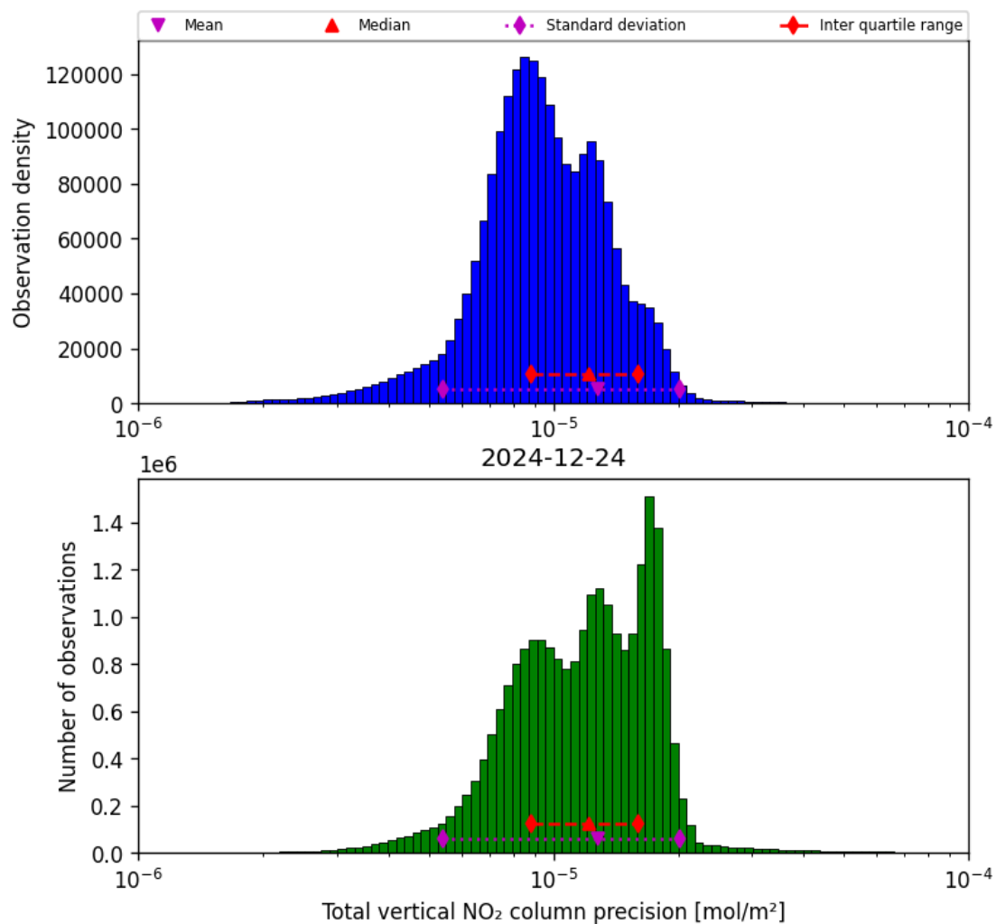
Figure 37: Histogram of “Total vertical NO 2 column precision” for 2024-12-24 to 2024-12-25
