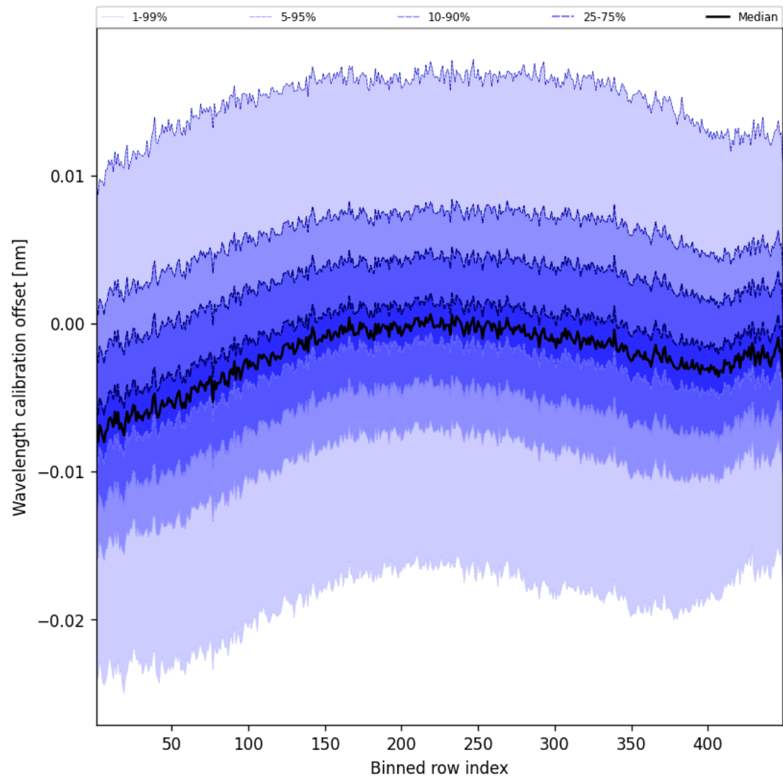
Figure 50: Along track statistics of “Wavelength calibration offset” for 2024-12-24 to 2024-12-25
