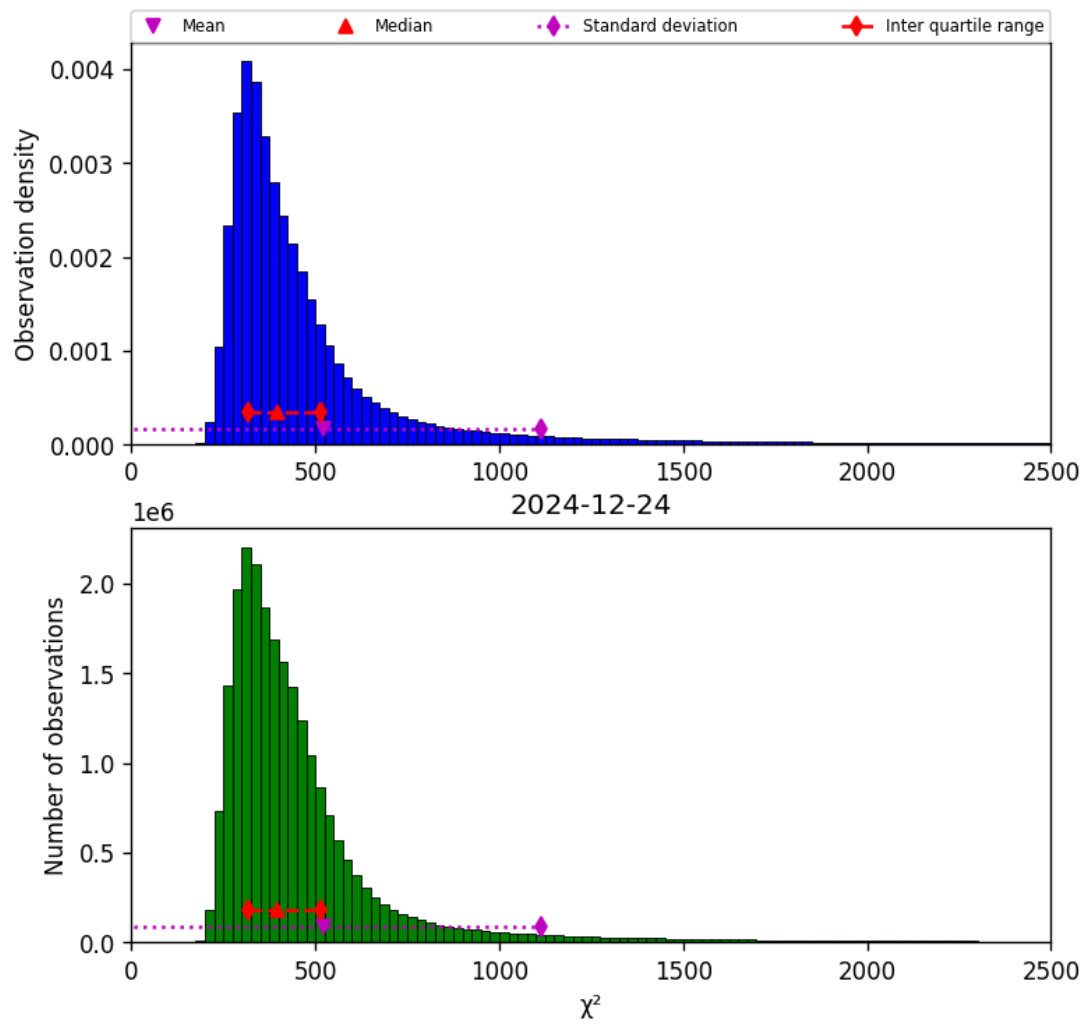
Figure 40: Histogram of " \chi^2 " for 2024-12-24 to 2024-12-25
