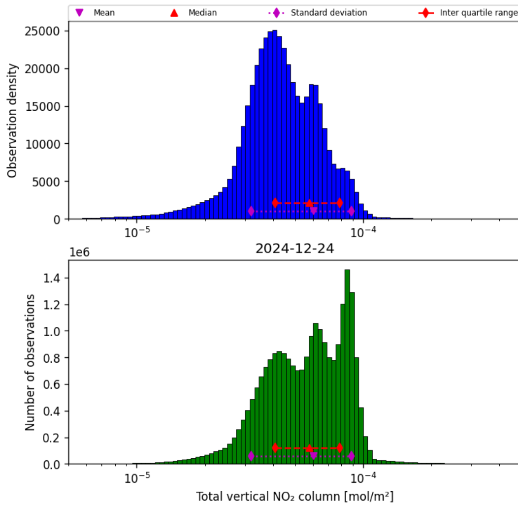
Figure 36: Histogram of “Total vertical NO 2 column” for 2024-12-24 to 2024-12-25
