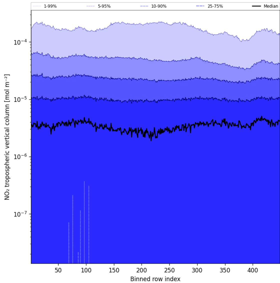
Figure 44: Along track statistics of “NO 2 tropospheric vertical column” for 2024-12-24 to 2024-12-25
