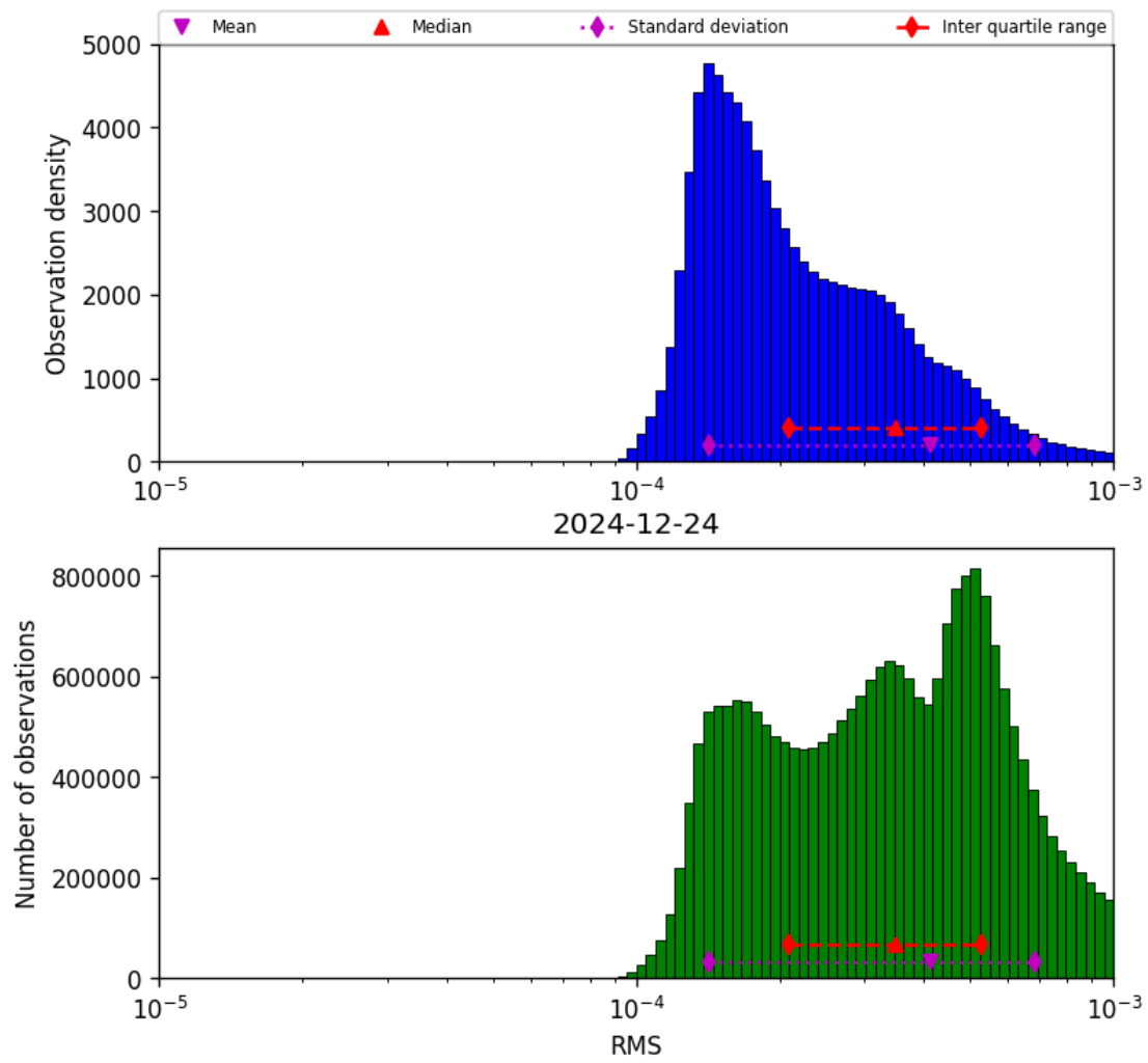
Figure 41: Histogram of “RMS” for 2024-12-24 to 2024-12-25
