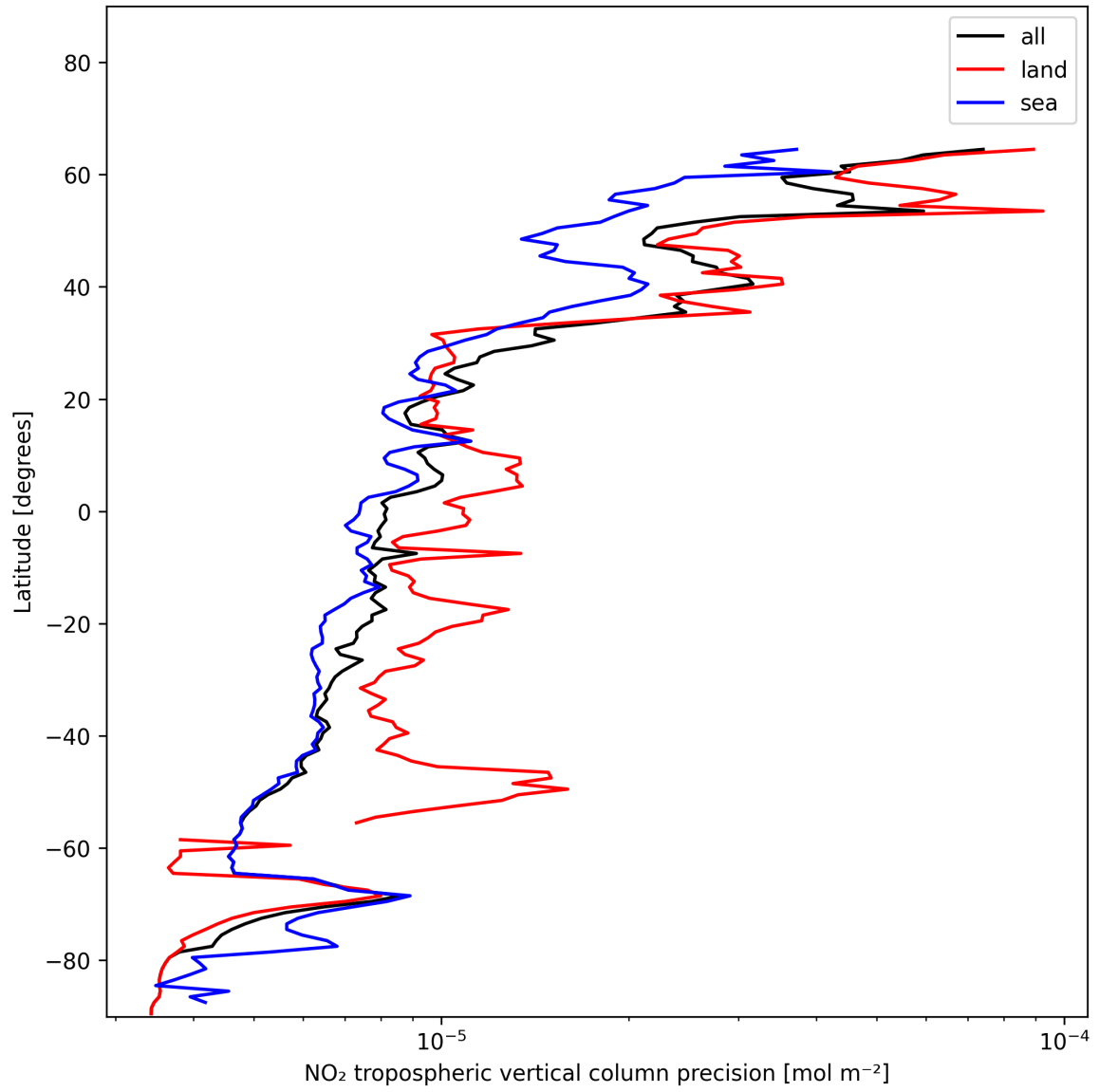
Figure 11: Zonal average of “NO 2 tropospheric vertical column precision” for 2024-12-24 to 2024-12-25.
