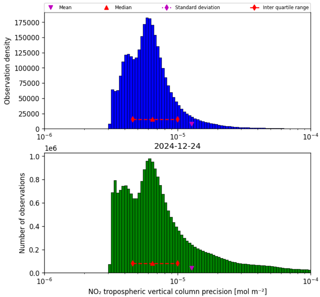
Figure 28: Histogram of “NO 2 tropospheric vertical column precision” for 2024-12-24 to 2024-12-25
