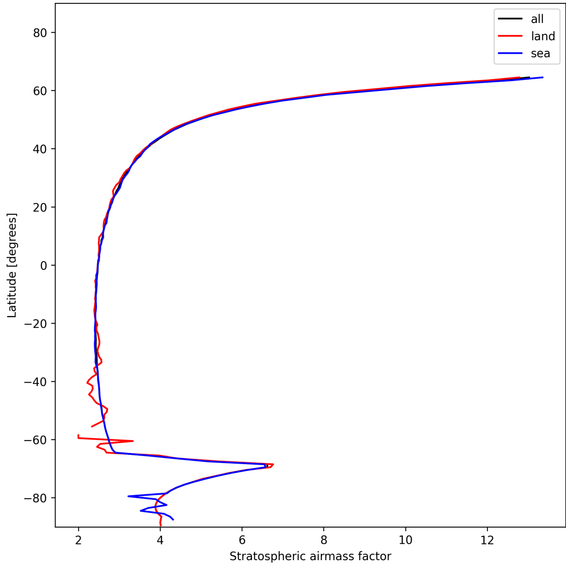
Figure 25: Zonal average of “Stratospheric airmass factor” for 2024-12-24 to 2024-12-25.
