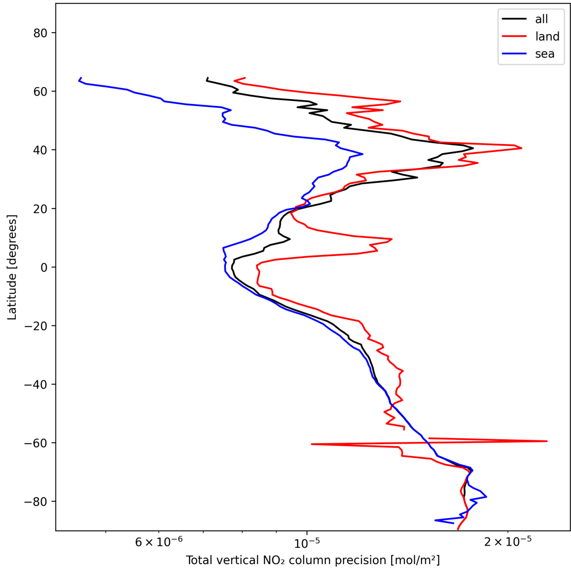
Figure 20: Zonal average of “Total vertical NO 2 column precision” for 2024-12-24 to 2024-12-25.
