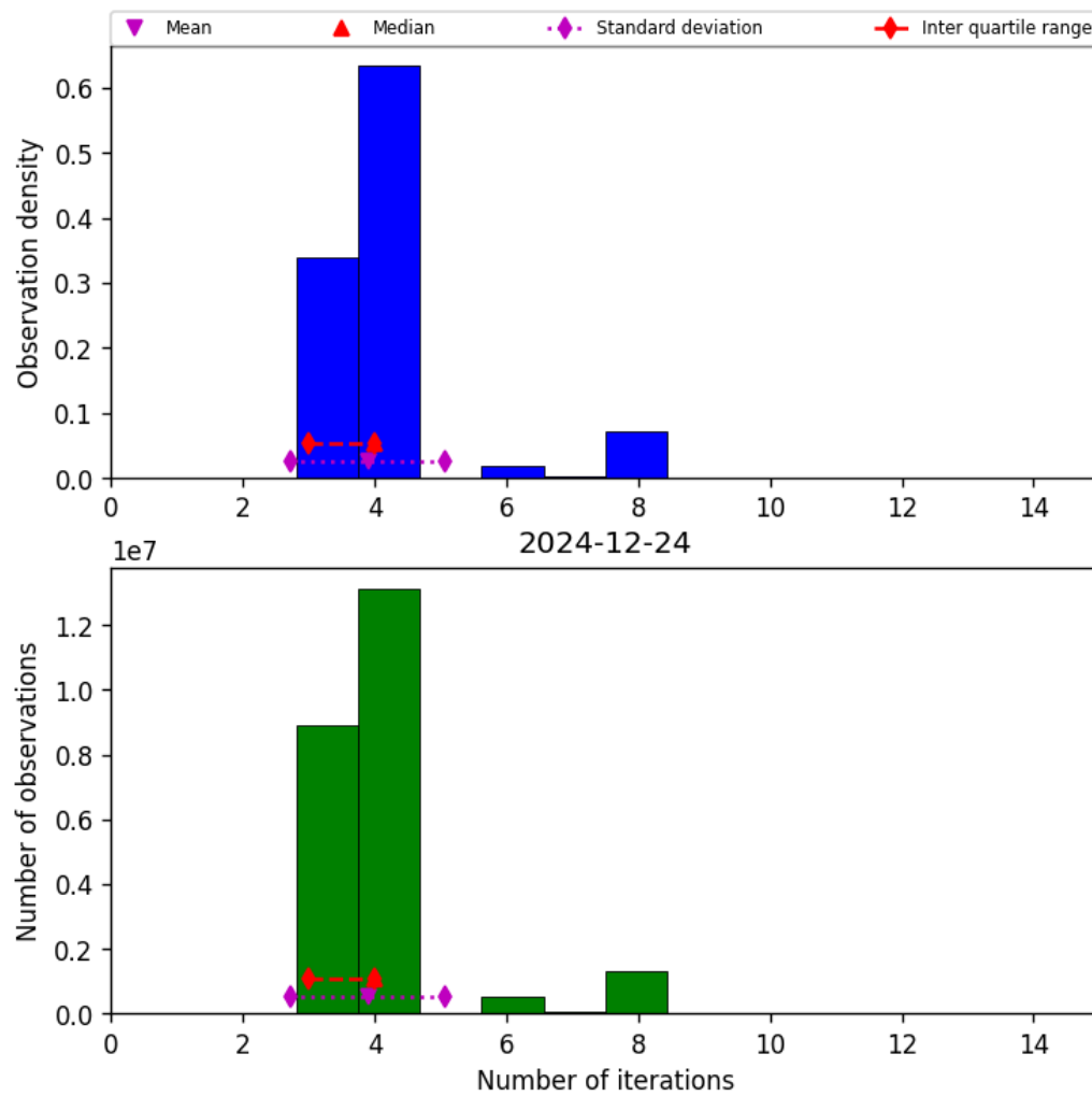
Figure 32: Histogram of “Number of iterations” for 2024-12-24 to 2024-12-25
