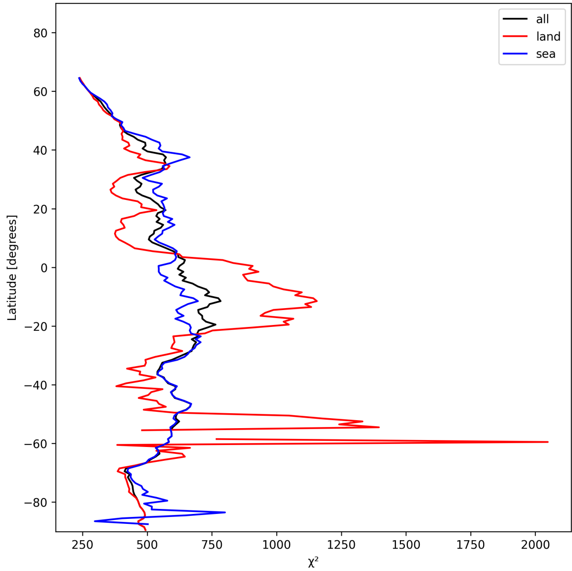
Figure 23: Zonal average of “ \chi^2 ” for 2024-12-24 to 2024-12-25.
