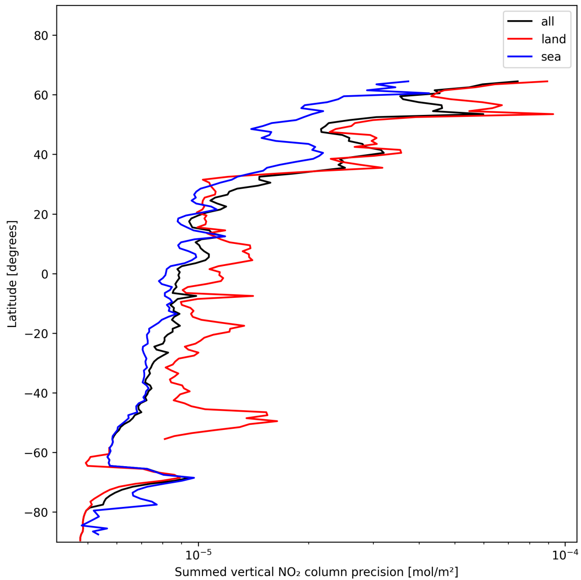
Figure 22: Zonal average of “Summed vertical NO 2 column precision” for 2024-12-24 to 2024-12-25.
