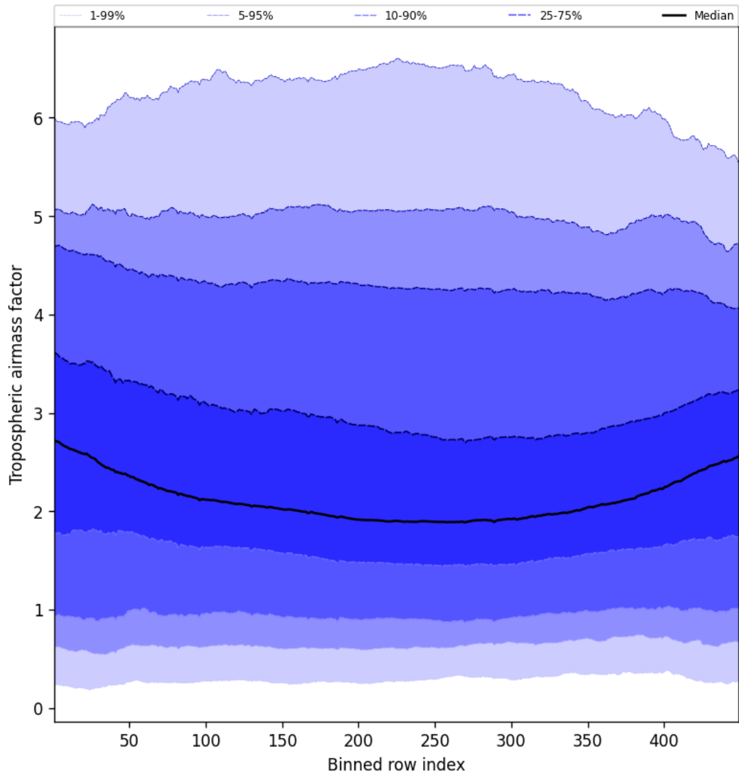
Figure 46: Along track statistics of “Tropospheric airmass factor” for 2024-12-24 to 2024-12-25
