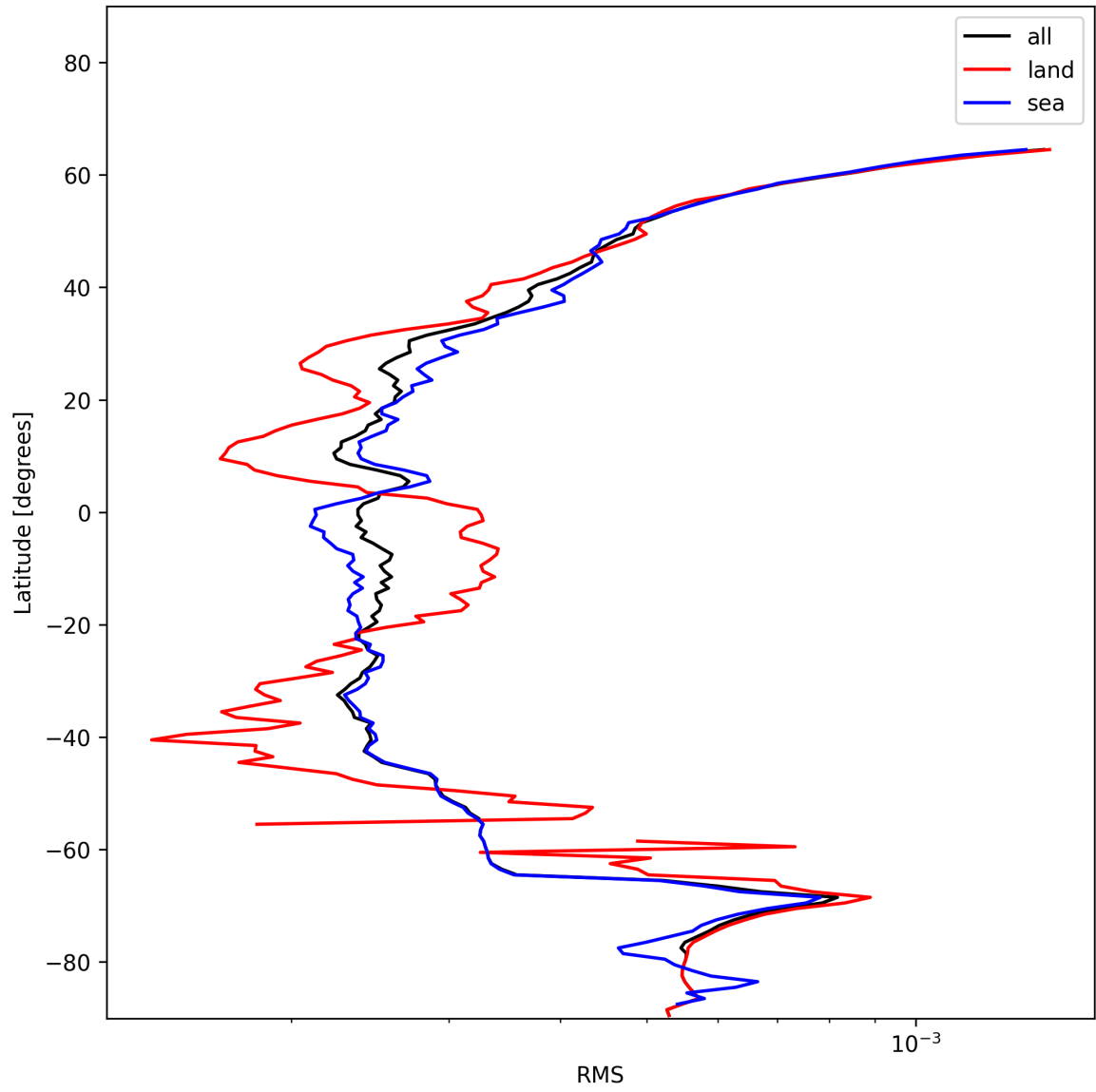
Figure 24: Zonal average of “RMS” for 2024-12-24 to 2024-12-25.
