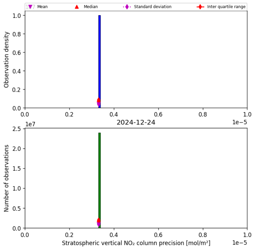
Figure 35: Histogram of “Stratospheric vertical NO 2 column precision” for 2024-12-24 to 2024-12-25
