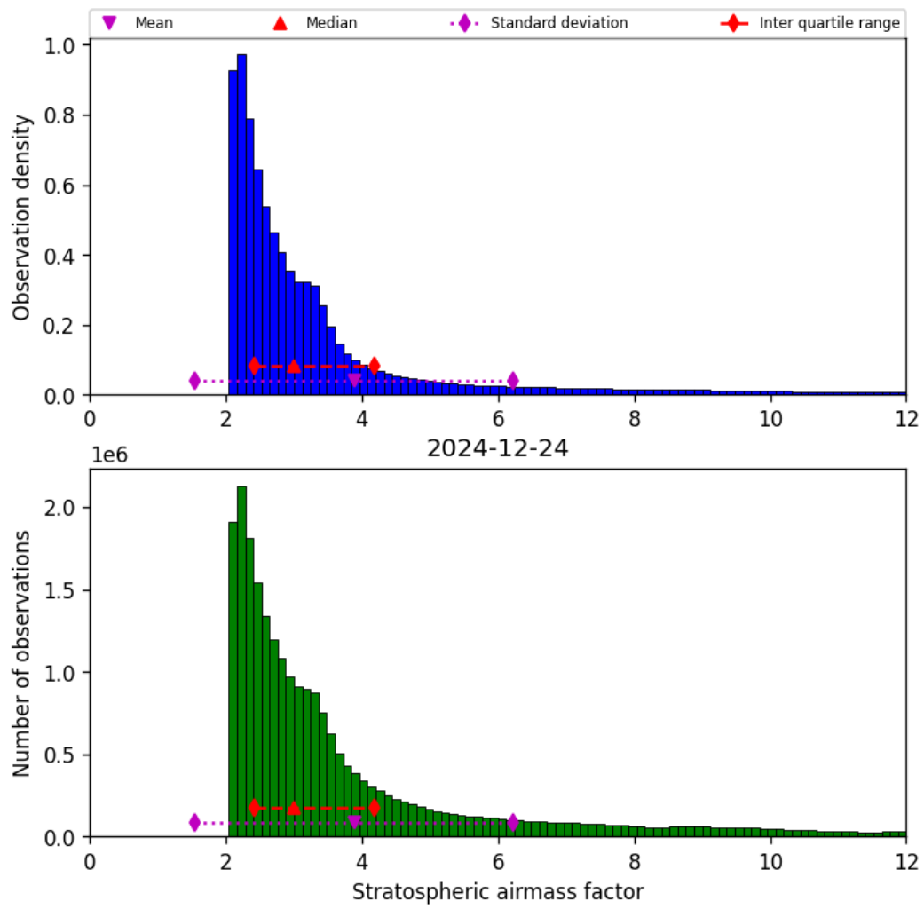
Figure 42: Histogram of “Stratospheric airmass factor” for 2024-12-24 to 2024-12-25
