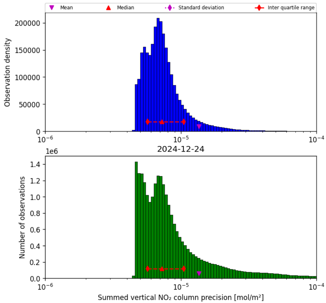
Figure 39: Histogram of "Summed vertical NO 2 column precision" for 2024-12-24 to 2024-12-25
