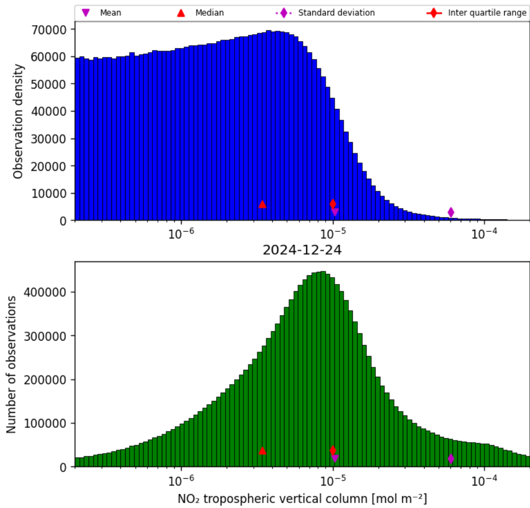
Figure 27: Histogram of “NO 2 tropospheric vertical column” for 2024-12-24 to 2024-12-25
