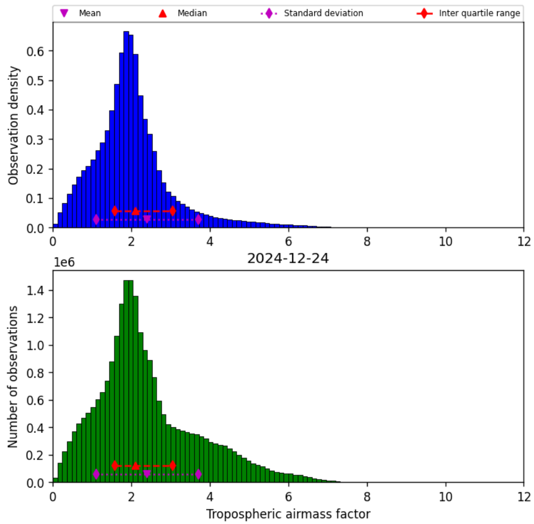
Figure 29: Histogram of “Tropospheric airmass factor” for 2024-12-24 to 2024-12-25
