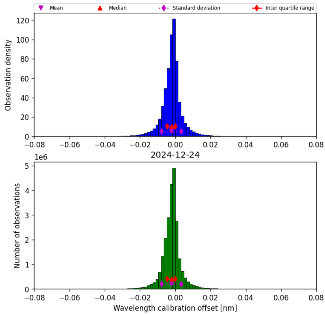
Figure 33: Histogram of “Wavelength calibration offset” for 2024-12-24 to 2024-12-25
