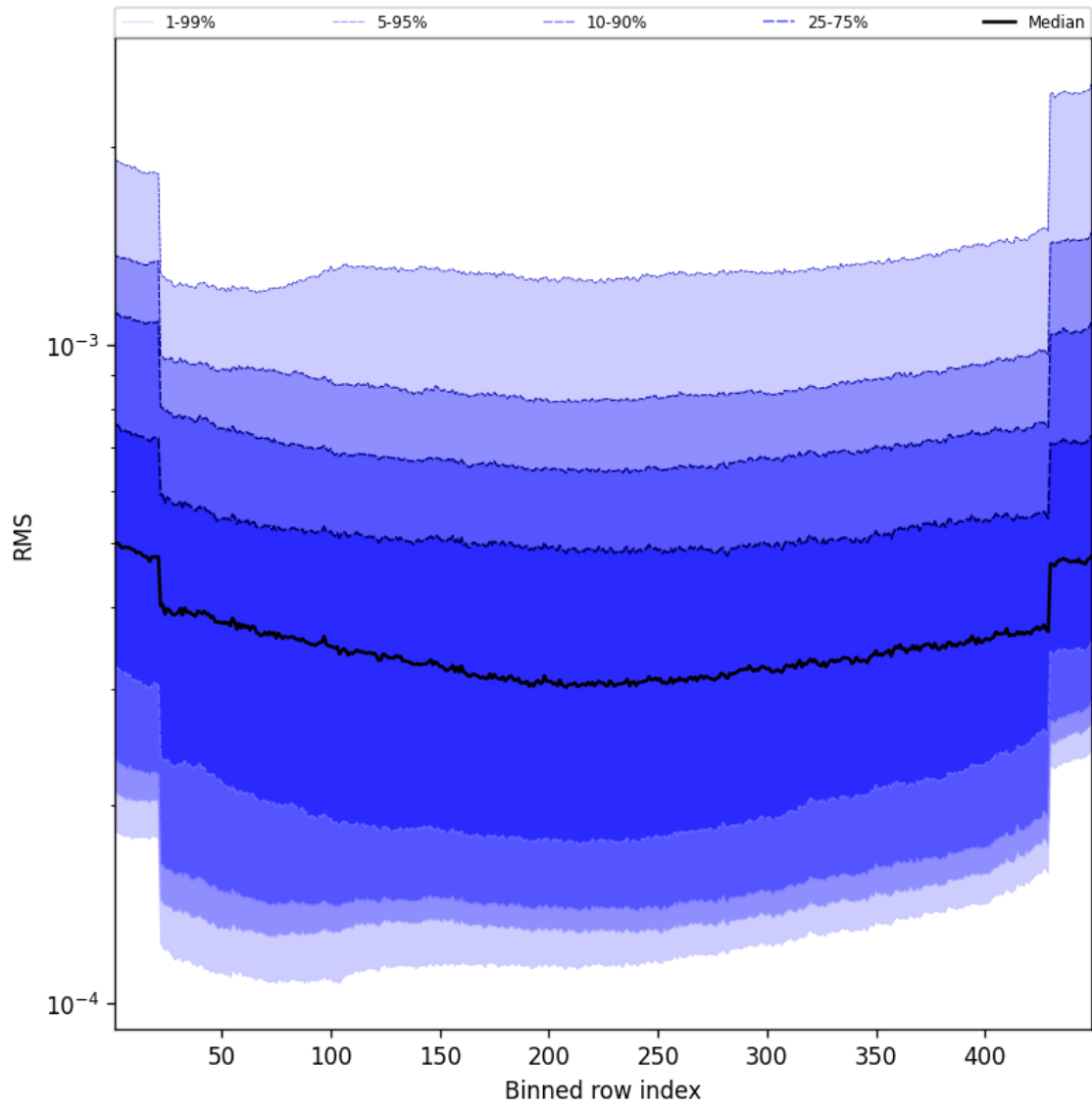
Figure 58: Along track statistics of “RMS” for 2024-12-24 to 2024-12-25
