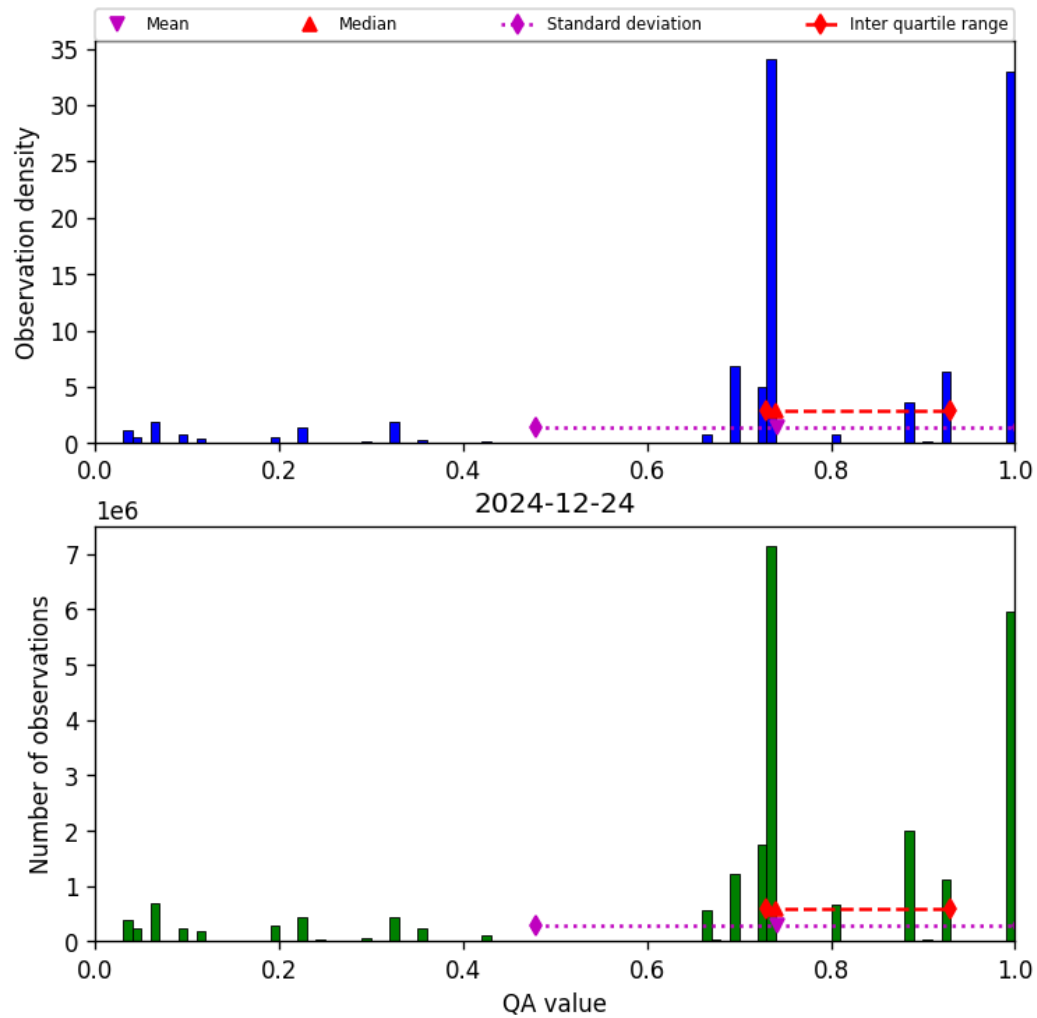
Figure 26: Histogram of “QA value” for 2024-12-24 to 2024-12-25
