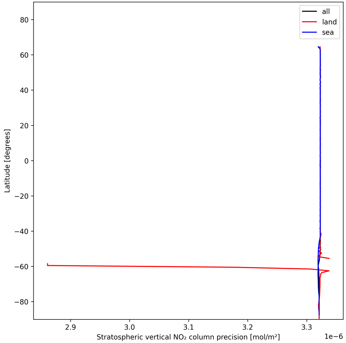
Figure 18: Zonal average of “Stratospheric vertical NO 2 column precision” for 2024-12-24 to 2024-12-25.
