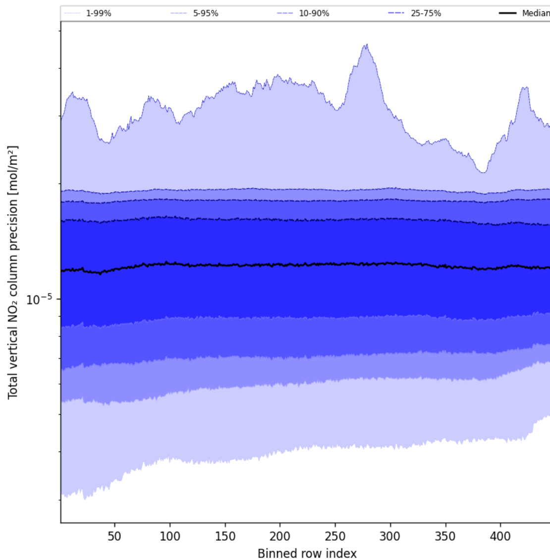
Figure 54: Along track statistics of “Total vertical NO 2 column precision” for 2024-12-24 to 2024-12-25
