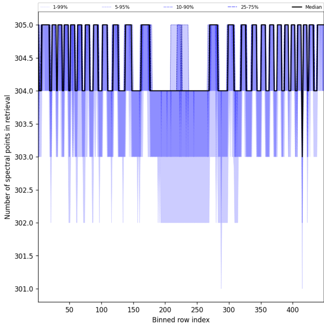
Figure 48: Along track statistics of “Number of spectral points in retrieval” for 2024-12-24 to 2024-12-25
