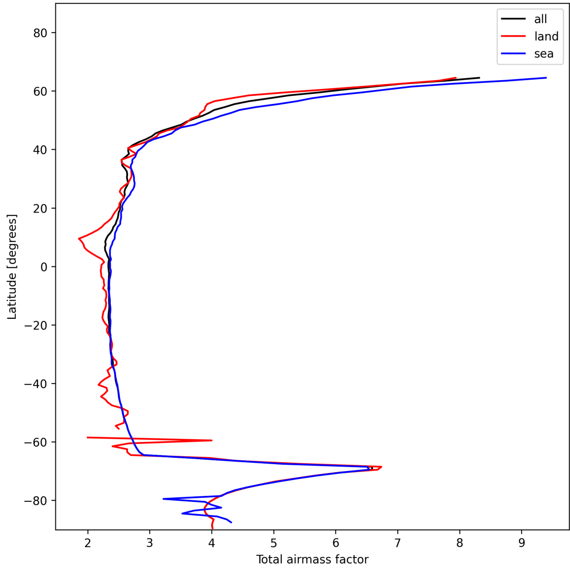
Figure 13: Zonal average of “Total airmass factor” for 2024-12-24 to 2024-12-25.
