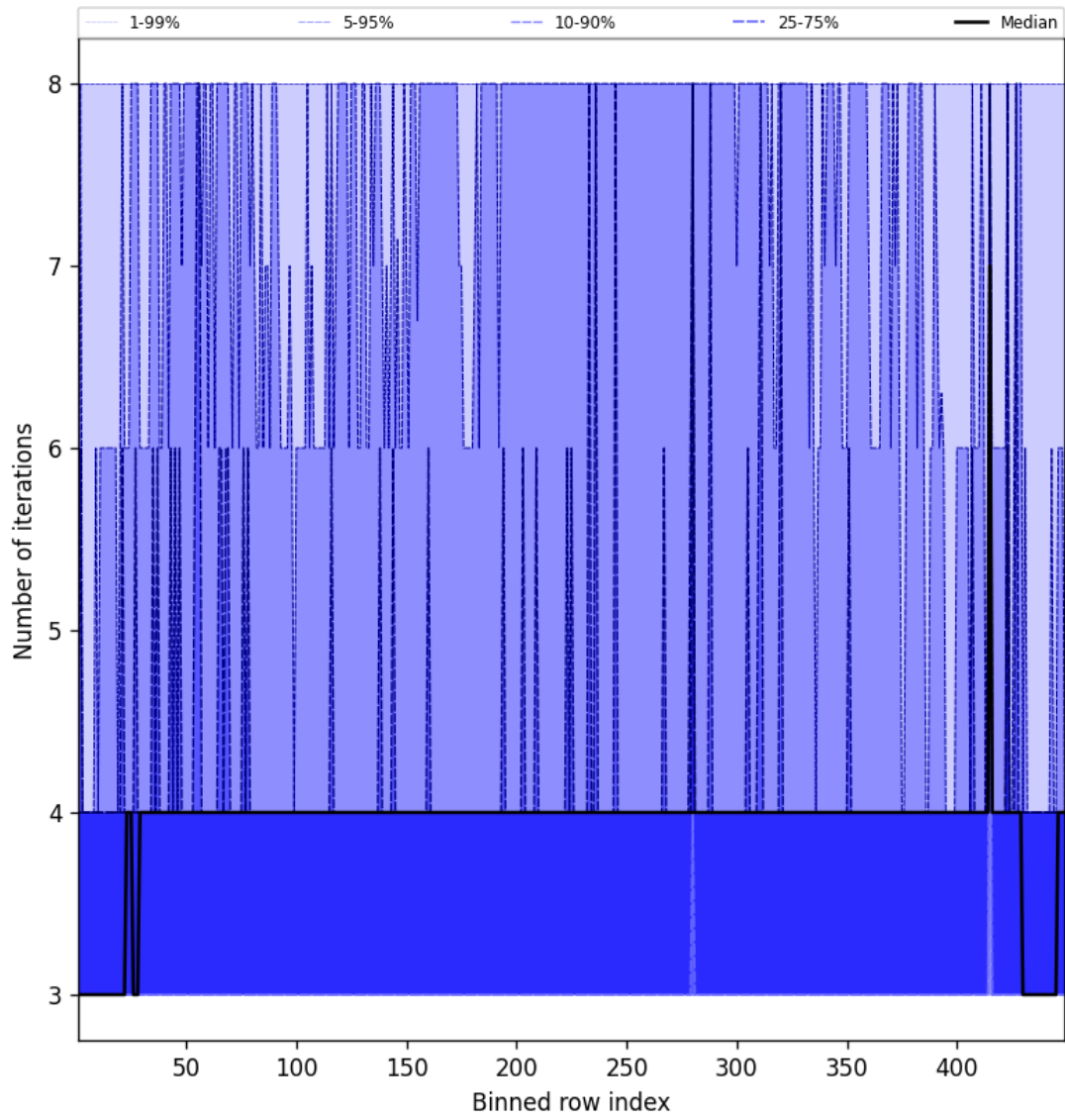
Figure 49: Along track statistics of “Number of iterations” for 2024-12-24 to 2024-12-25
