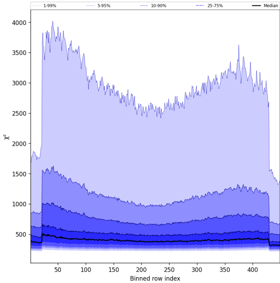
Figure 57: Along track statistics of “ \chi^2 ” for 2024-12-24 to 2024-12-25
