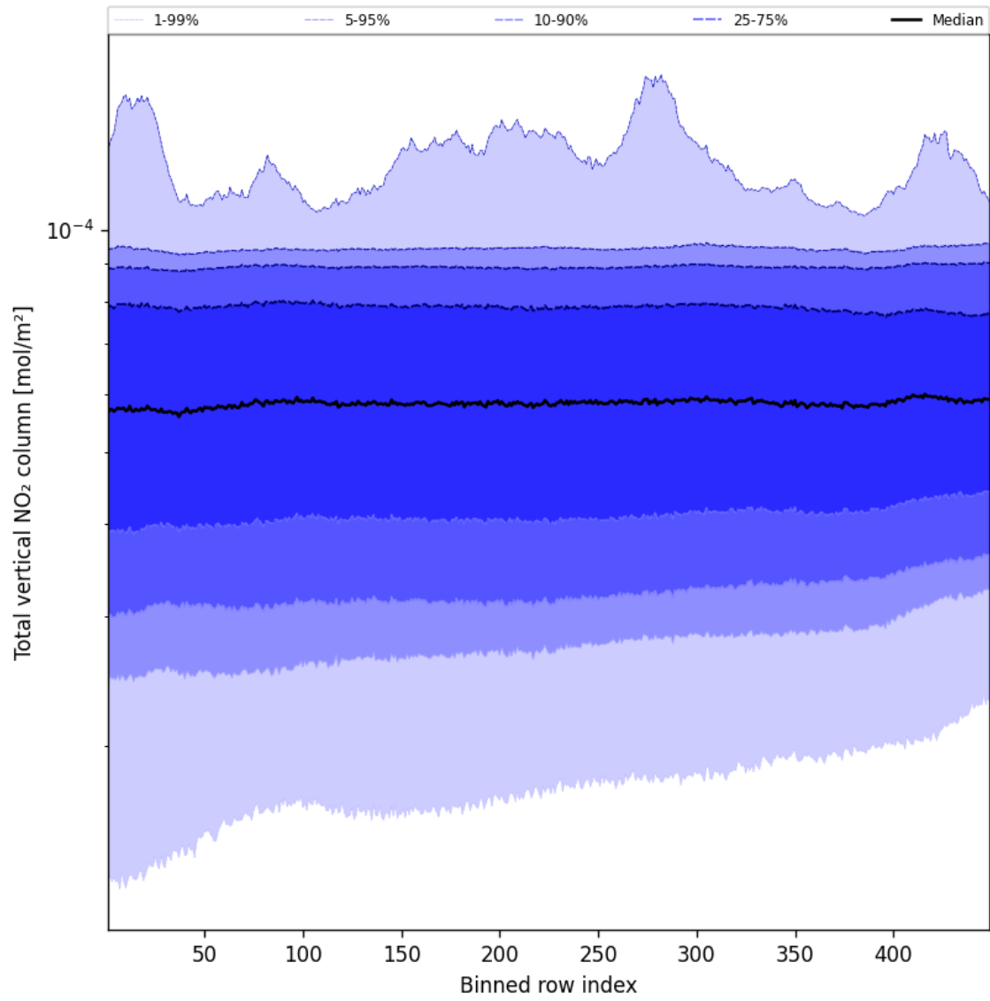
Figure 53: Along track statistics of “Total vertical NO 2 column” for 2024-12-24 to 2024-12-25
