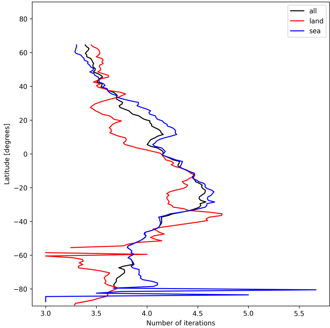
Figure 15: Zonal average of “Number of iterations” for 2024-12-24 to 2024-12-25.
