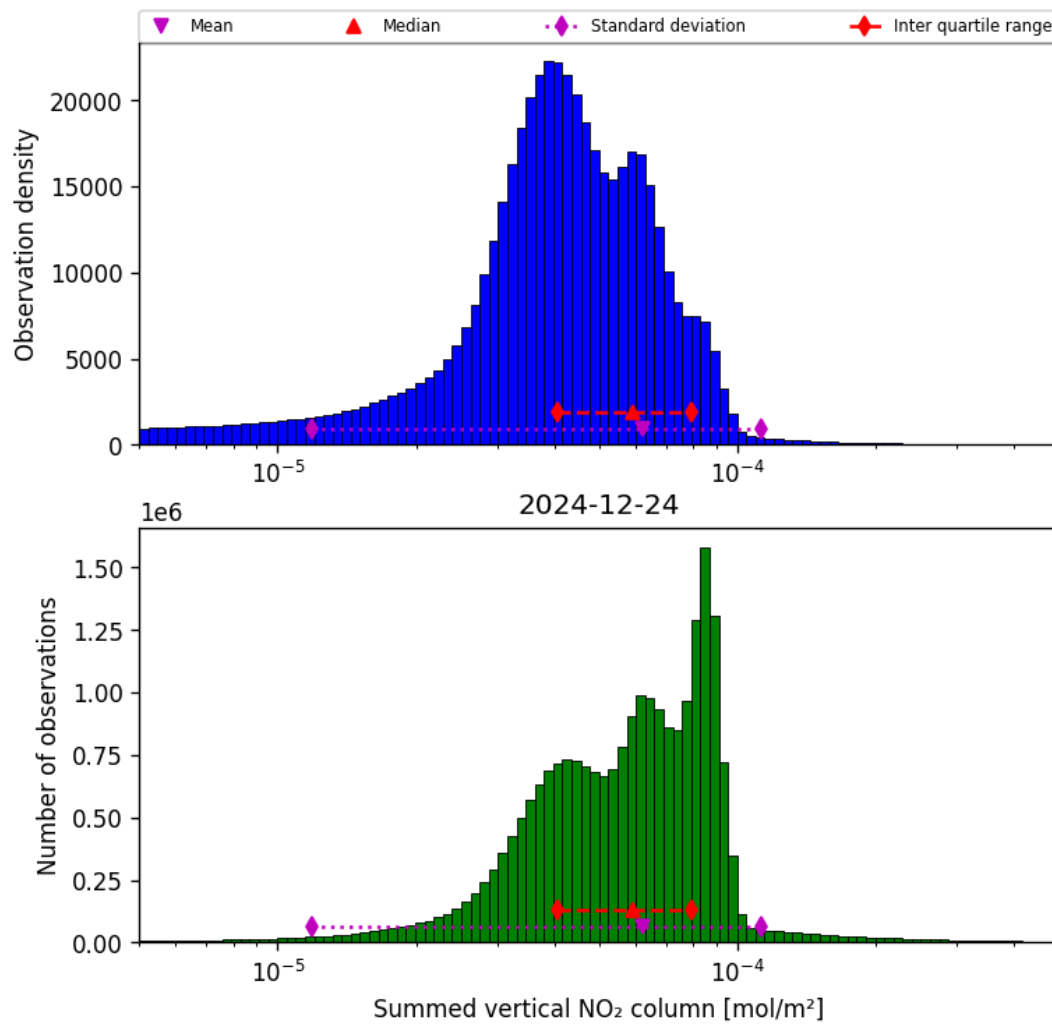
Figure 38: Histogram of “Summed vertical NO 2 column” for 2024-12-24 to 2024-12-25
