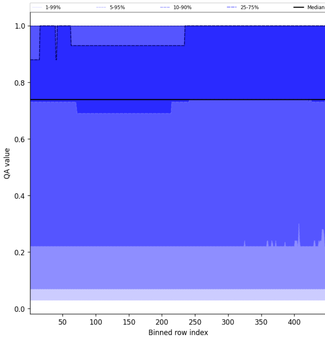
Figure 43: Along track statistics of “QA value” for 2024-12-24 to 2024-12-25
