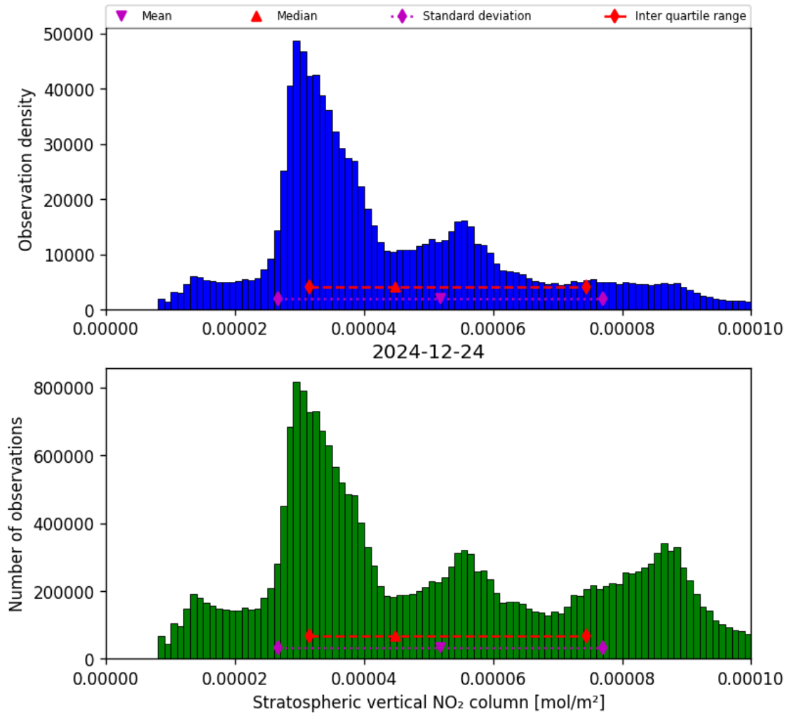
Figure 34: Histogram of “Stratospheric vertical NO 2 column” for 2024-12-24 to 2024-12-25
