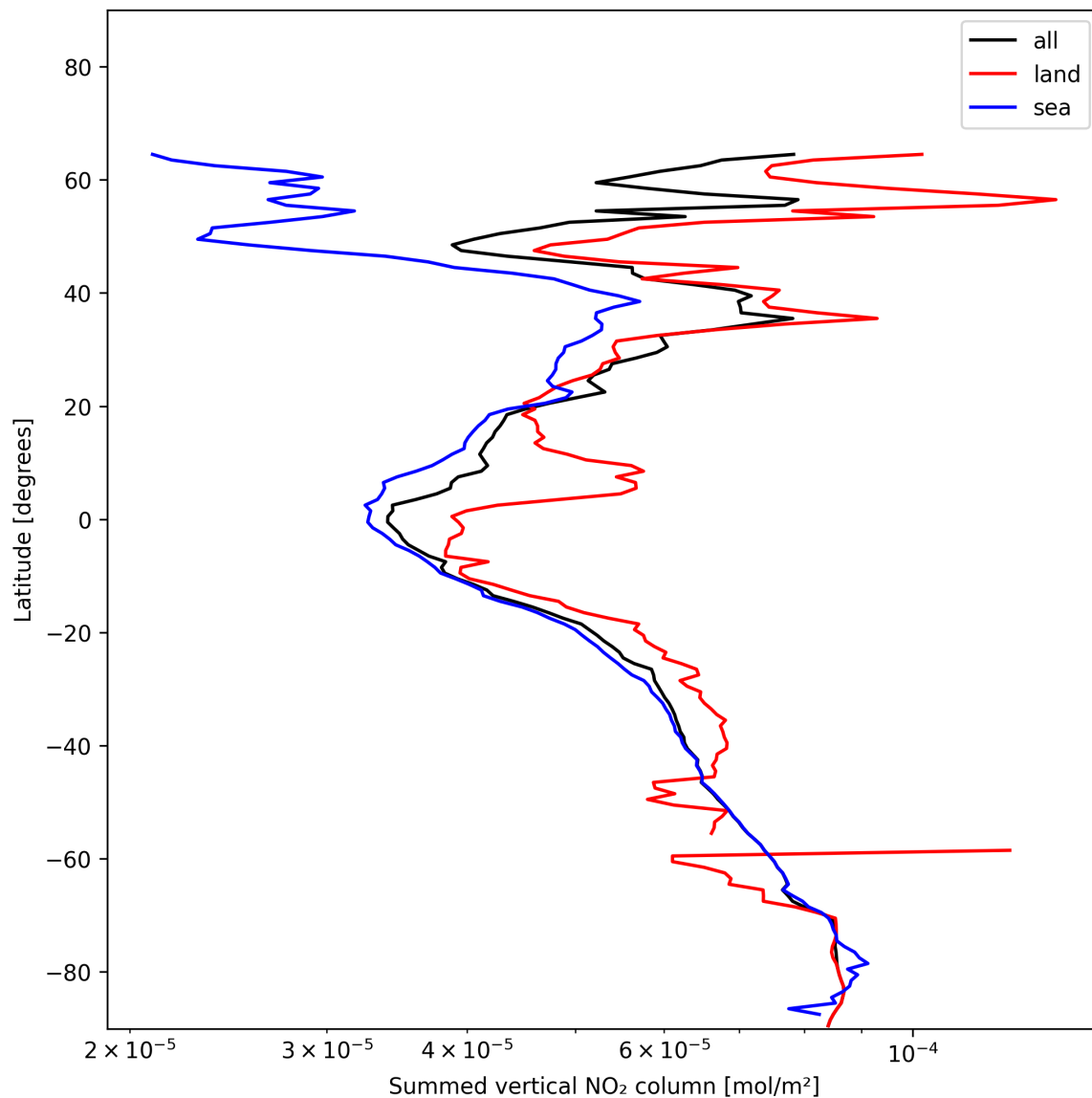
Figure 21: Zonal average of “Summed vertical NO 2 column” for 2024-12-24 to 2024-12-25.
