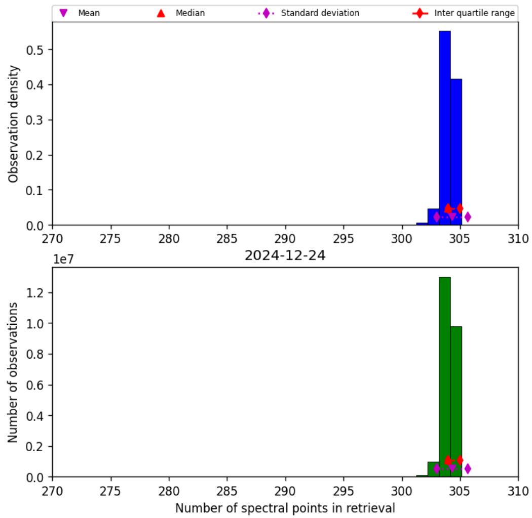
Figure 31: Histogram of “Number of spectral points in retrieval” for 2024-12-24 to 2024-12-25
