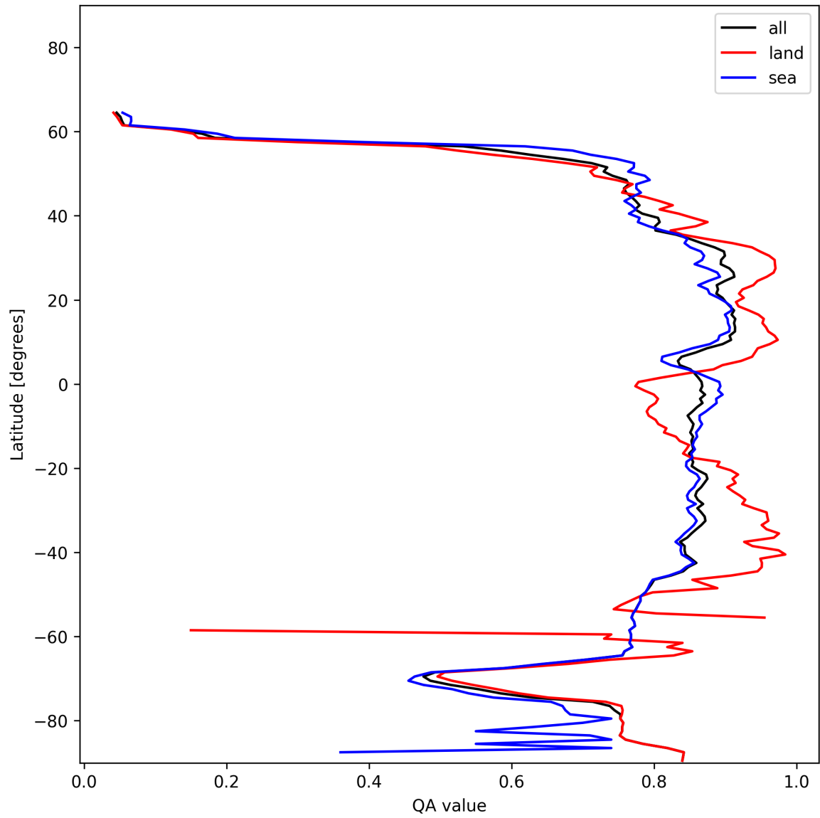
Figure 9: Zonal average of “QA value” for 2024-12-24 to 2024-12-25.
