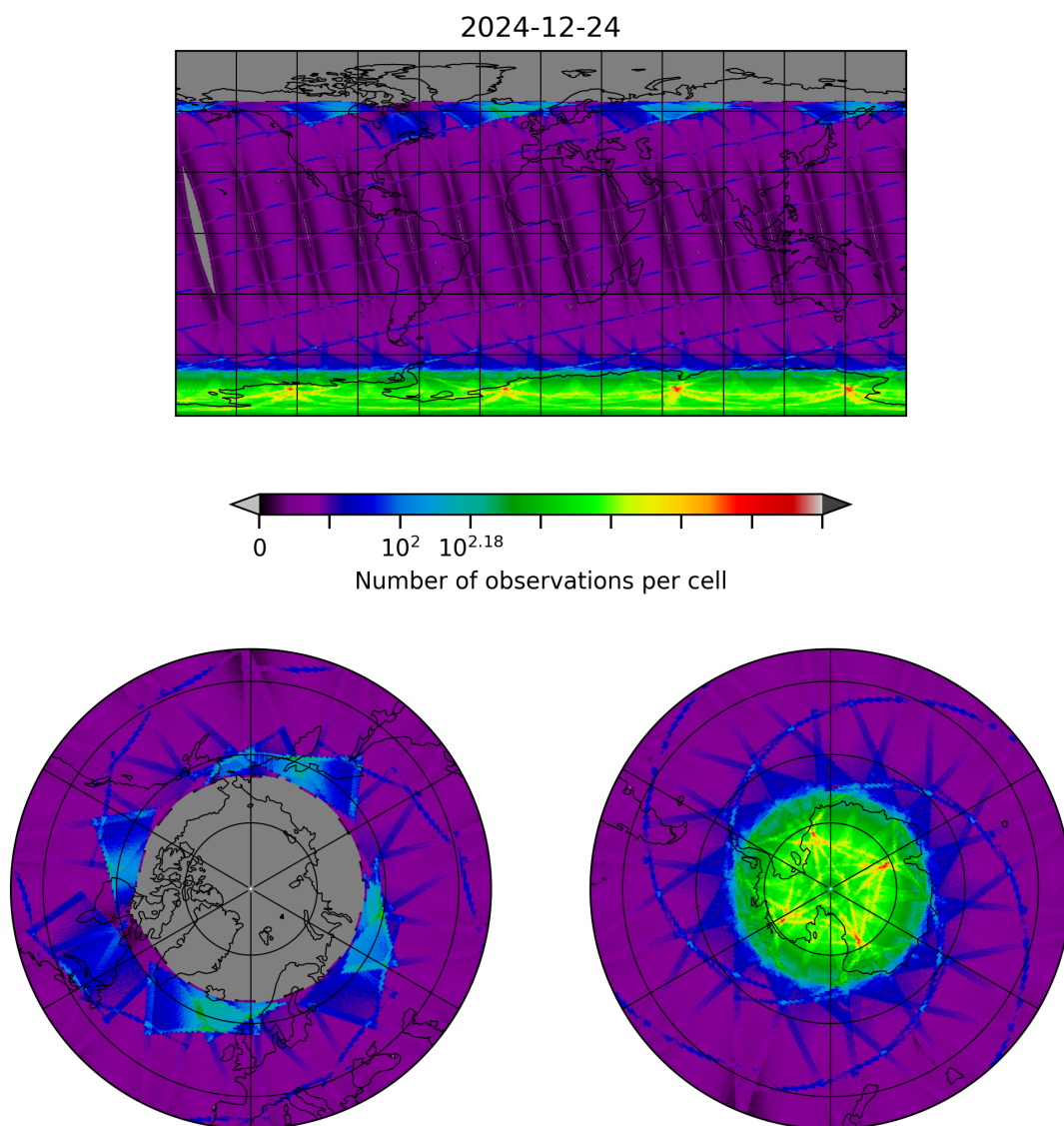
Figure 8: Map of the number of observations for 2024-12-24 to 2024-12-25
