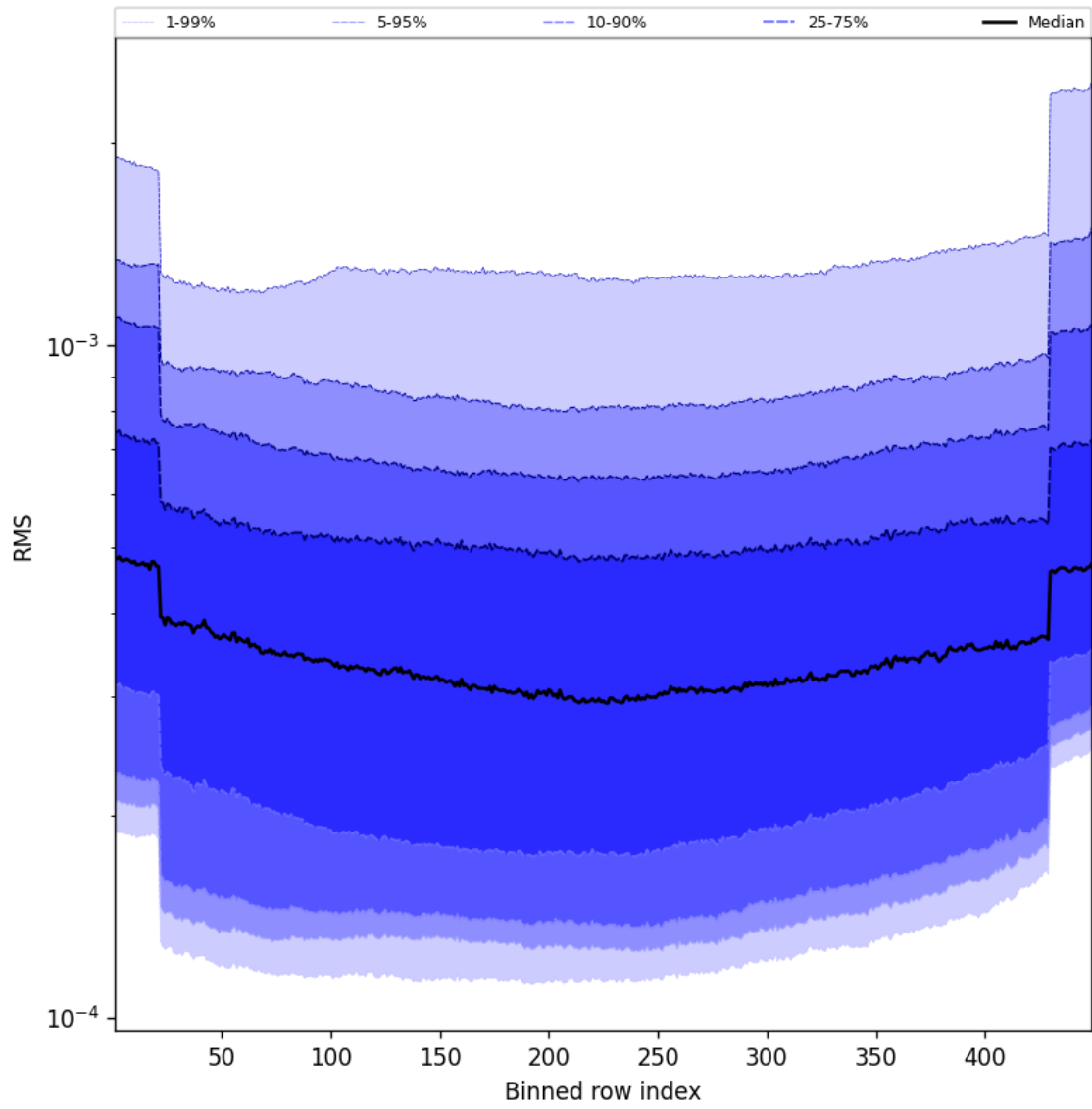
Figure 58: Along track statistics of “RMS” for 2024-12-26 to 2024-12-27
