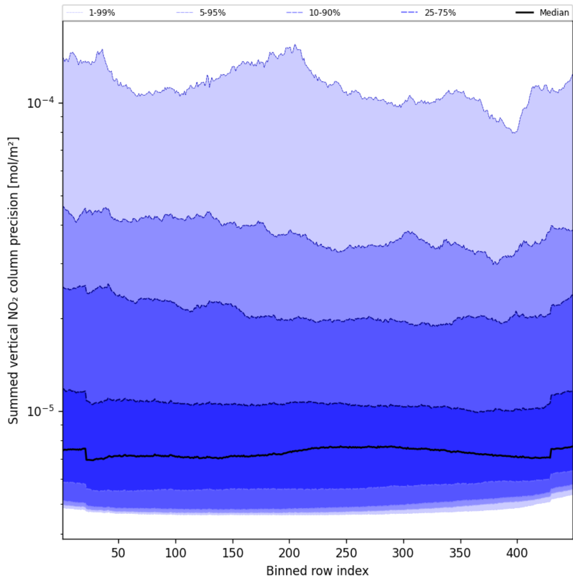
Figure 56: Along track statistics of “Summed vertical NO 2 column precision” for 2024-12-26 to 2024-12-27
