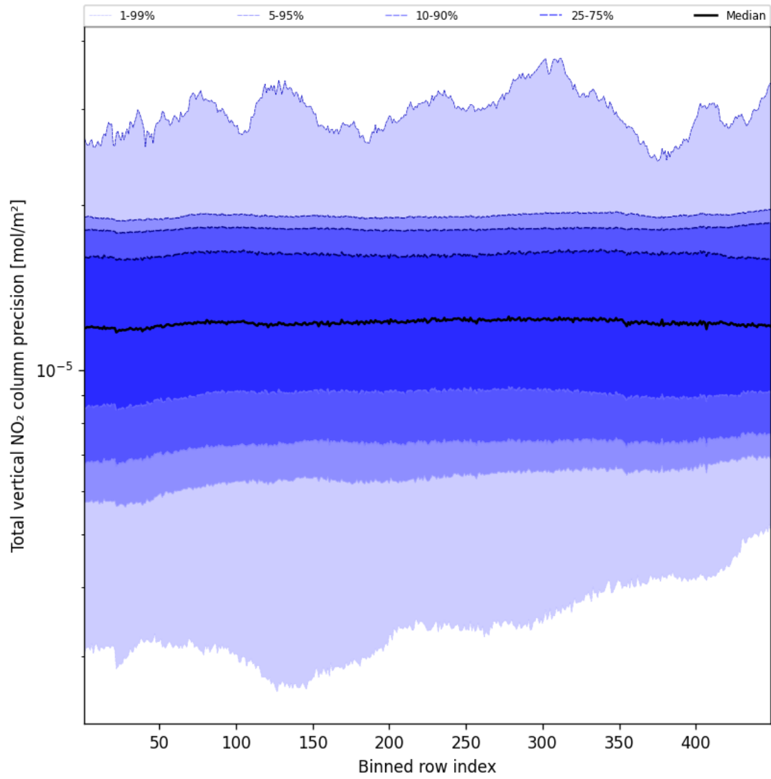
Figure 54: Along track statistics of “Total vertical NO 2 column precision” for 2024-12-26 to 2024-12-27
