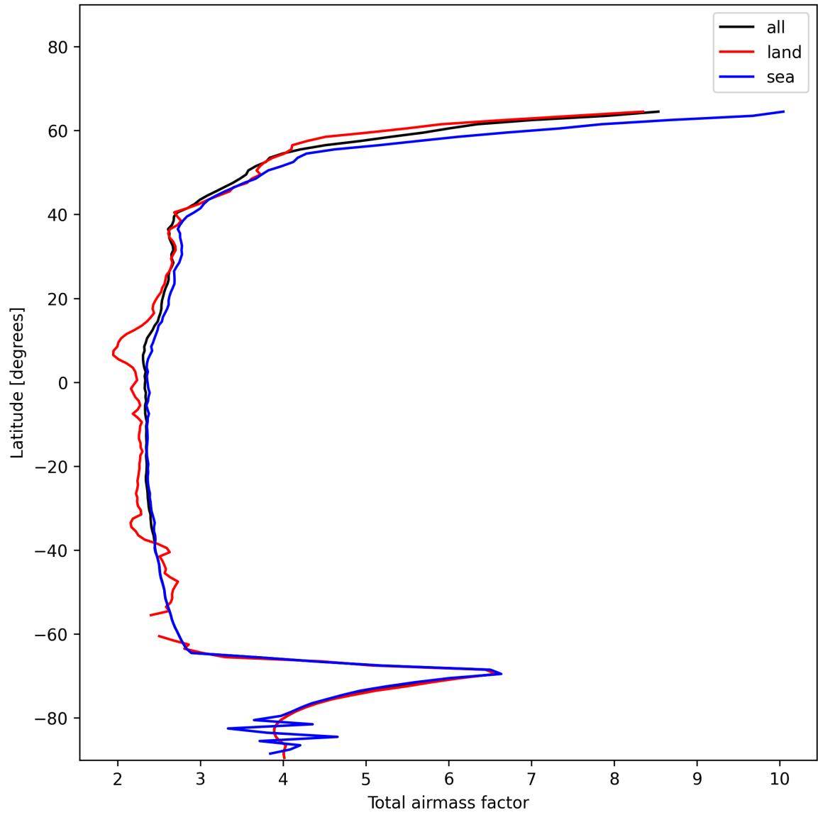
Figure 13: Zonal average of “Total airmass factor” for 2024-12-26 to 2024-12-27.
