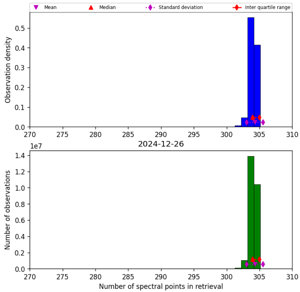
Figure 31: Histogram of “Number of spectral points in retrieval” for 2024-12-26 to 2024-12-27
