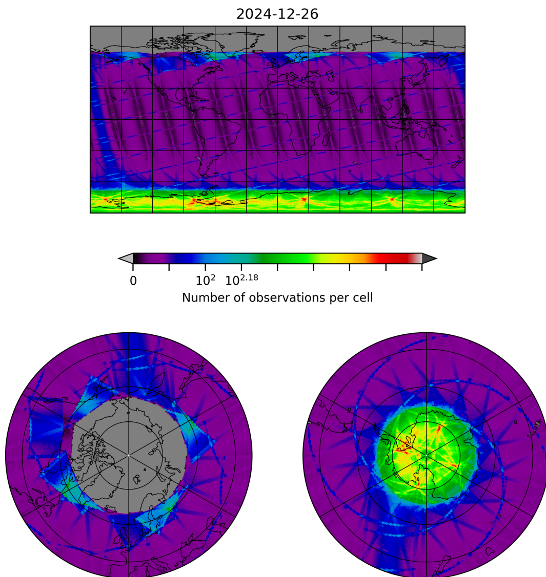
Figure 8: Map of the number of observations for 2024-12-26 to 2024-12-27
