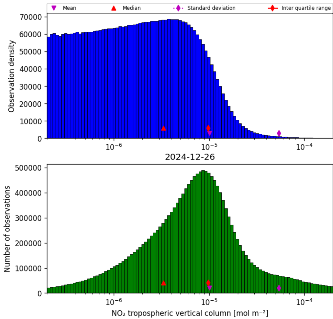
Figure 27: Histogram of “NO 2 tropospheric vertical column” for 2024-12-26 to 2024-12-27
