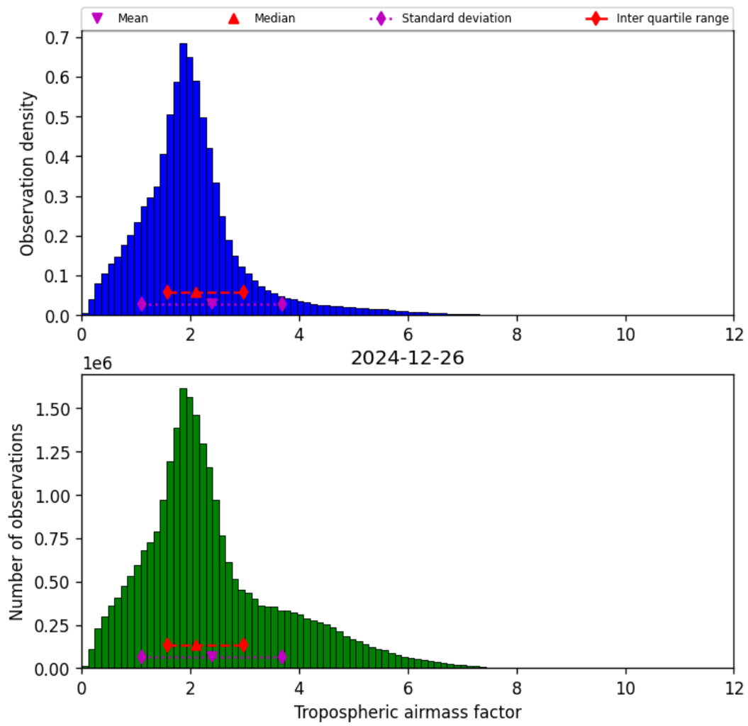
Figure 29: Histogram of “Tropospheric airmass factor” for 2024-12-26 to 2024-12-27
