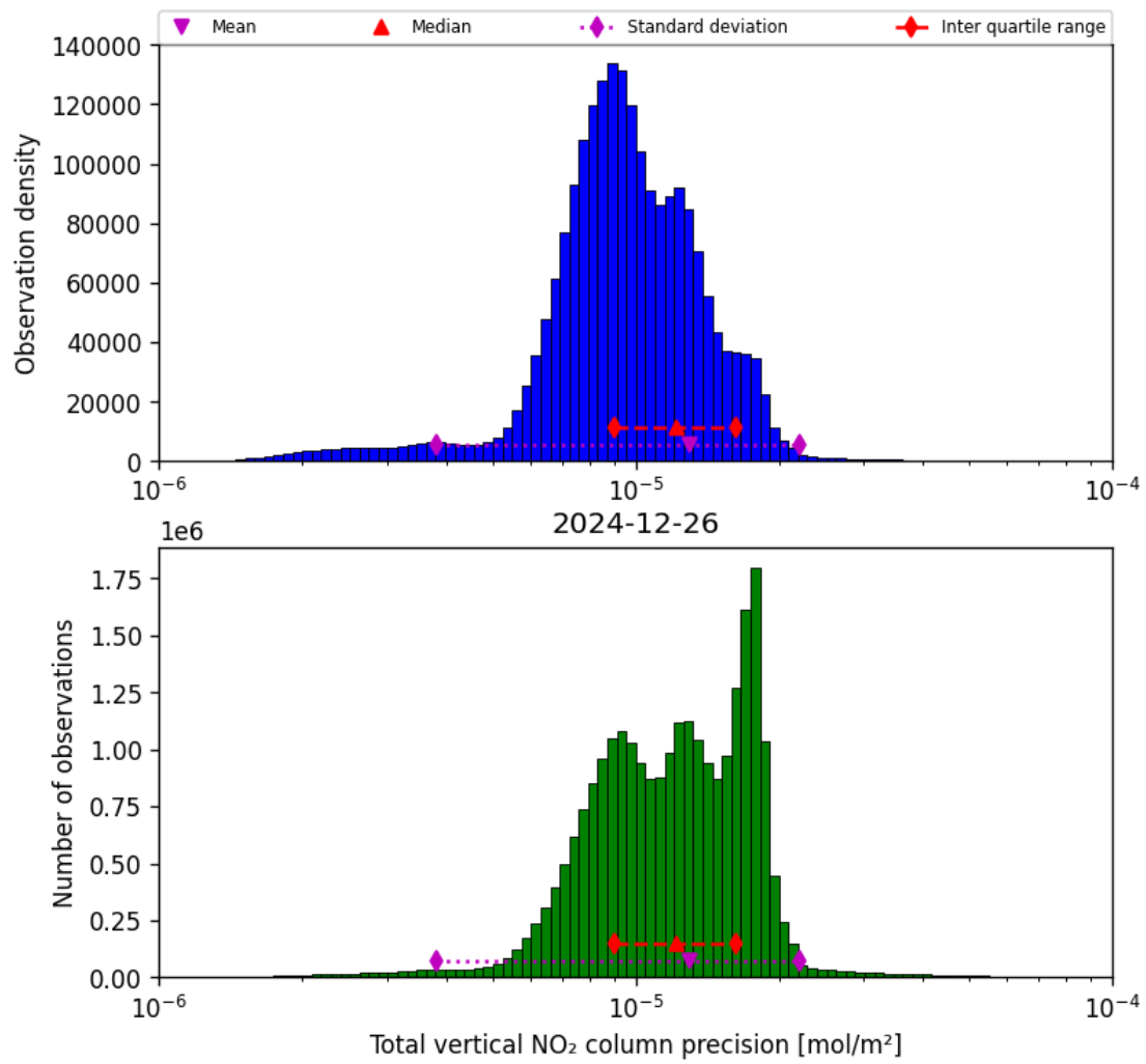
Figure 37: Histogram of “Total vertical NO 2 column precision” for 2024-12-26 to 2024-12-27
