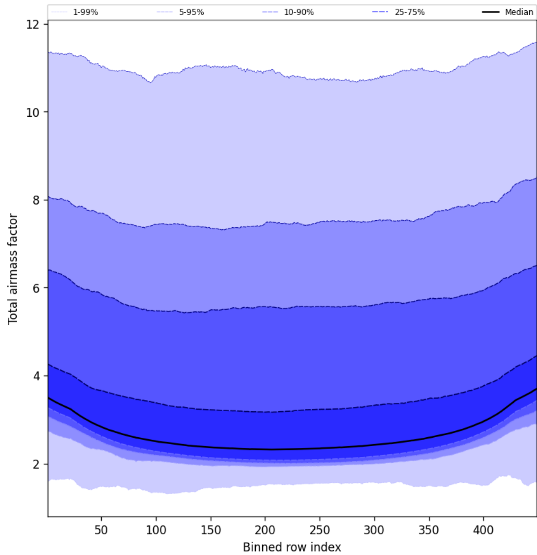
Figure 47: Along track statistics of “Total airmass factor” for 2024-12-26 to 2024-12-27
