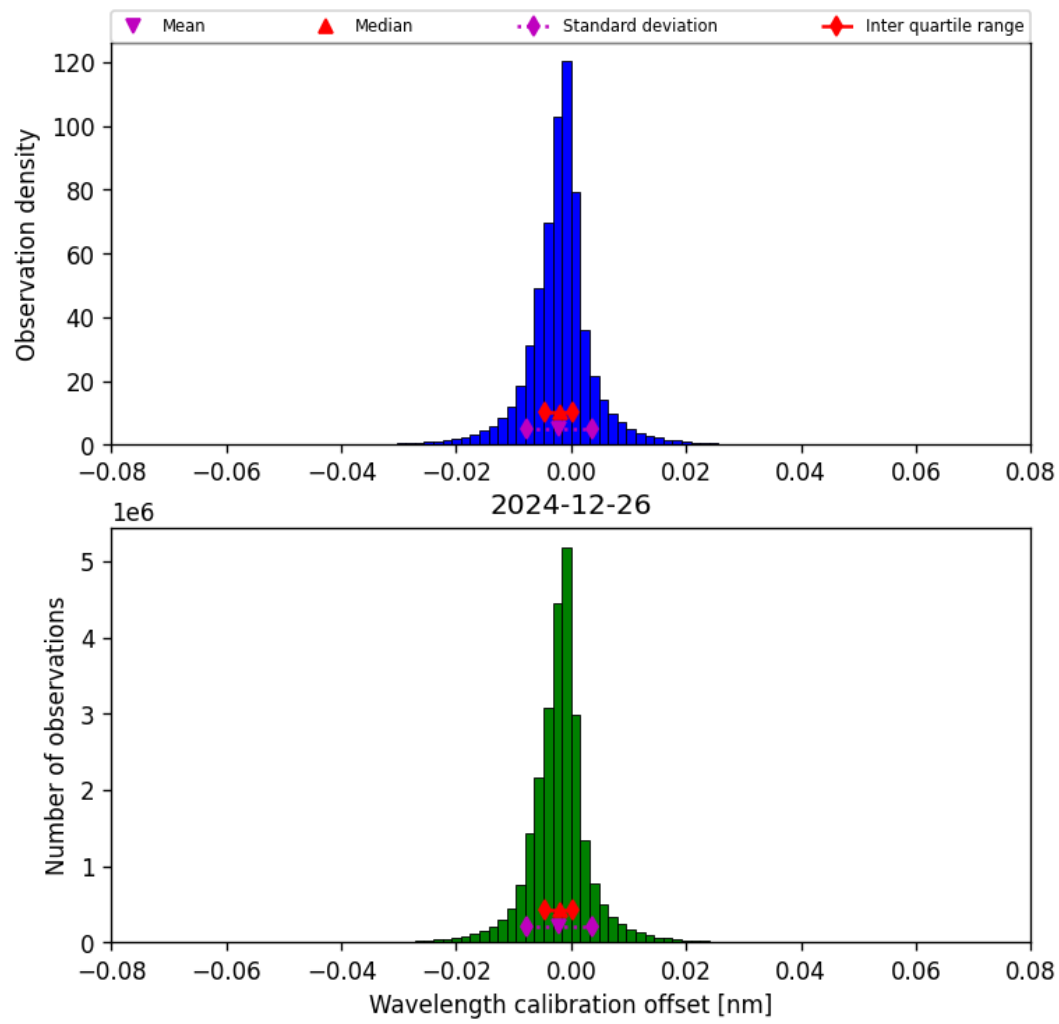
Figure 33: Histogram of “Wavelength calibration offset” for 2024-12-26 to 2024-12-27
