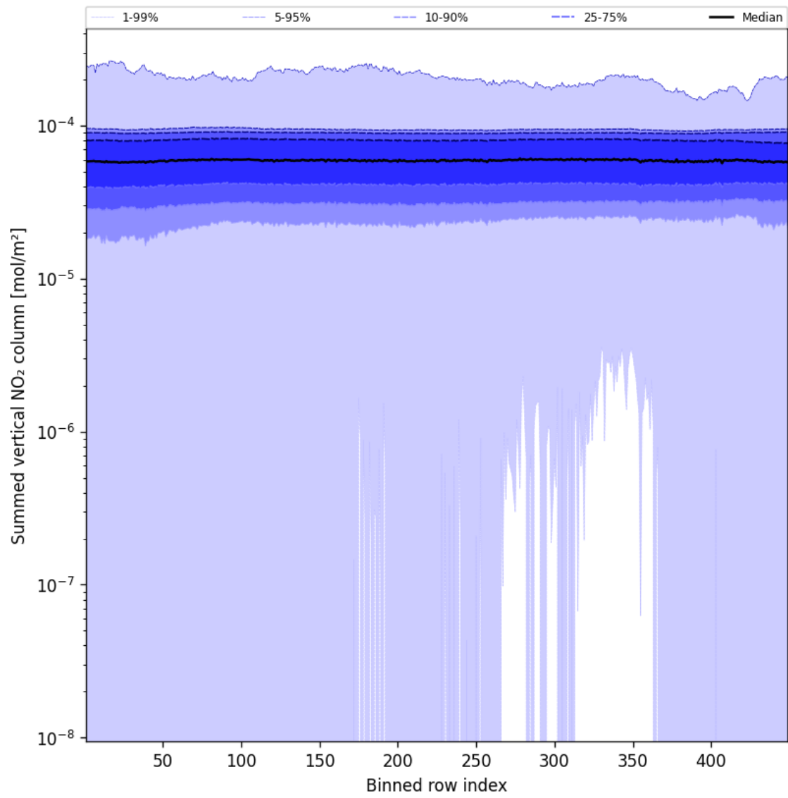
Figure 55: Along track statistics of “Summed vertical NO 2 column” for 2024-12-26 to 2024-12-27
