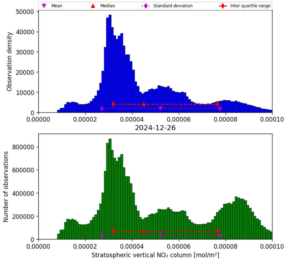
Figure 34: Histogram of “Stratospheric vertical NO 2 column” for 2024-12-26 to 2024-12-27
