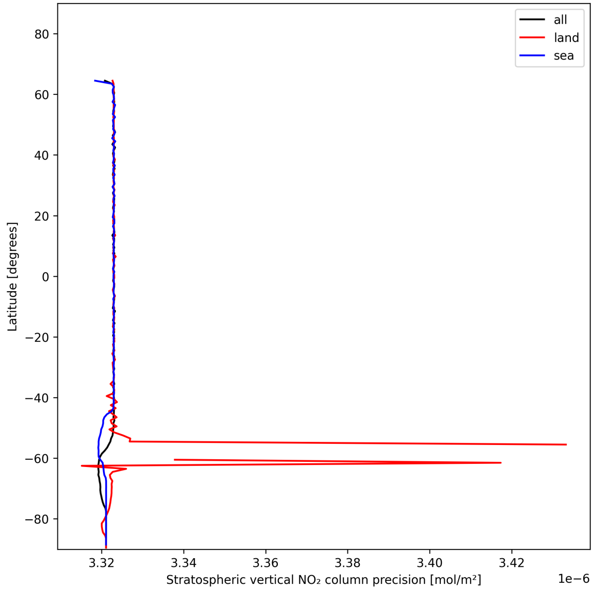
Figure 18: Zonal average of "Stratospheric vertical NO 2 column precision" for 2024-12-26 to 2024-12-27.
