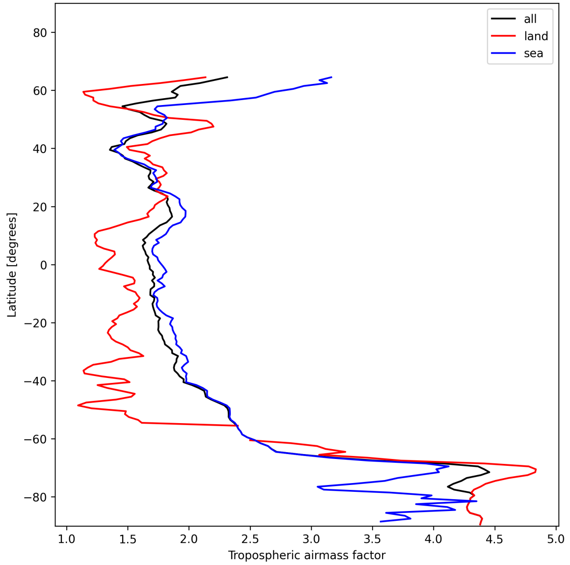
Figure 12: Zonal average of “Tropospheric airmass factor” for 2024-12-26 to 2024-12-27.
