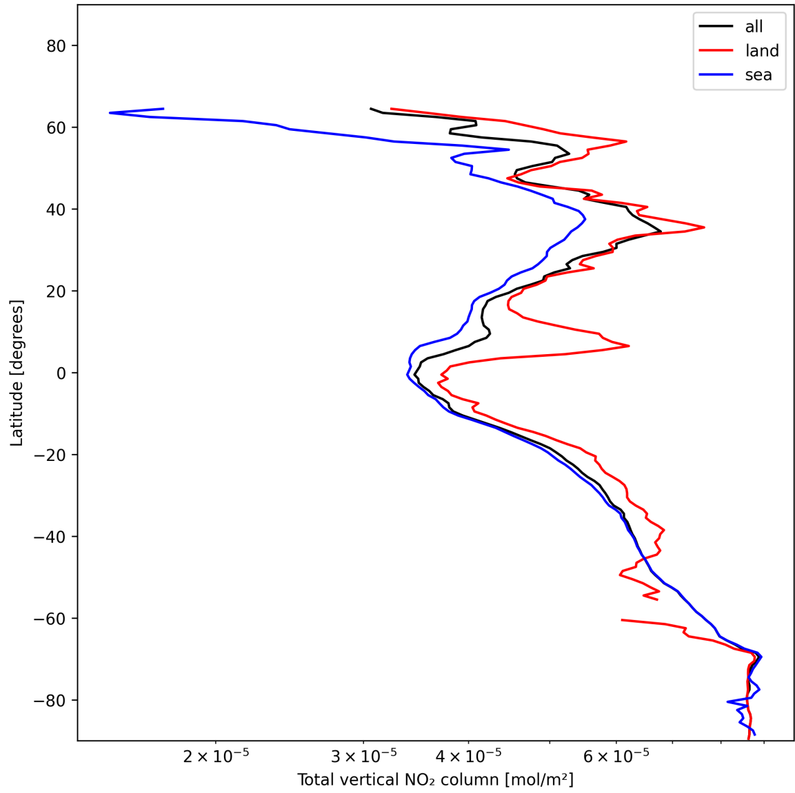
Figure 19: Zonal average of “Total vertical NO 2 column” for 2024-12-26 to 2024-12-27.
