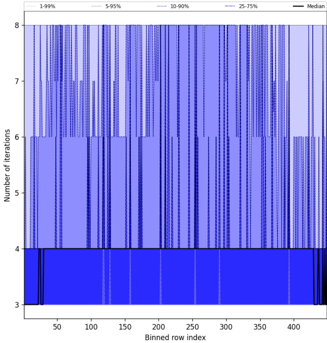
Figure 49: Along track statistics of “Number of iterations” for 2024-12-26 to 2024-12-27
