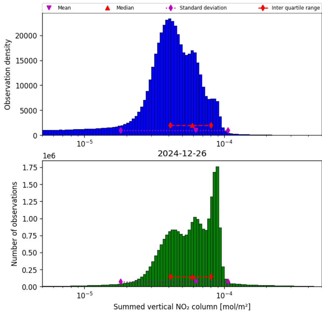
Figure 38: Histogram of “Summed vertical NO 2 column” for 2024-12-26 to 2024-12-27
