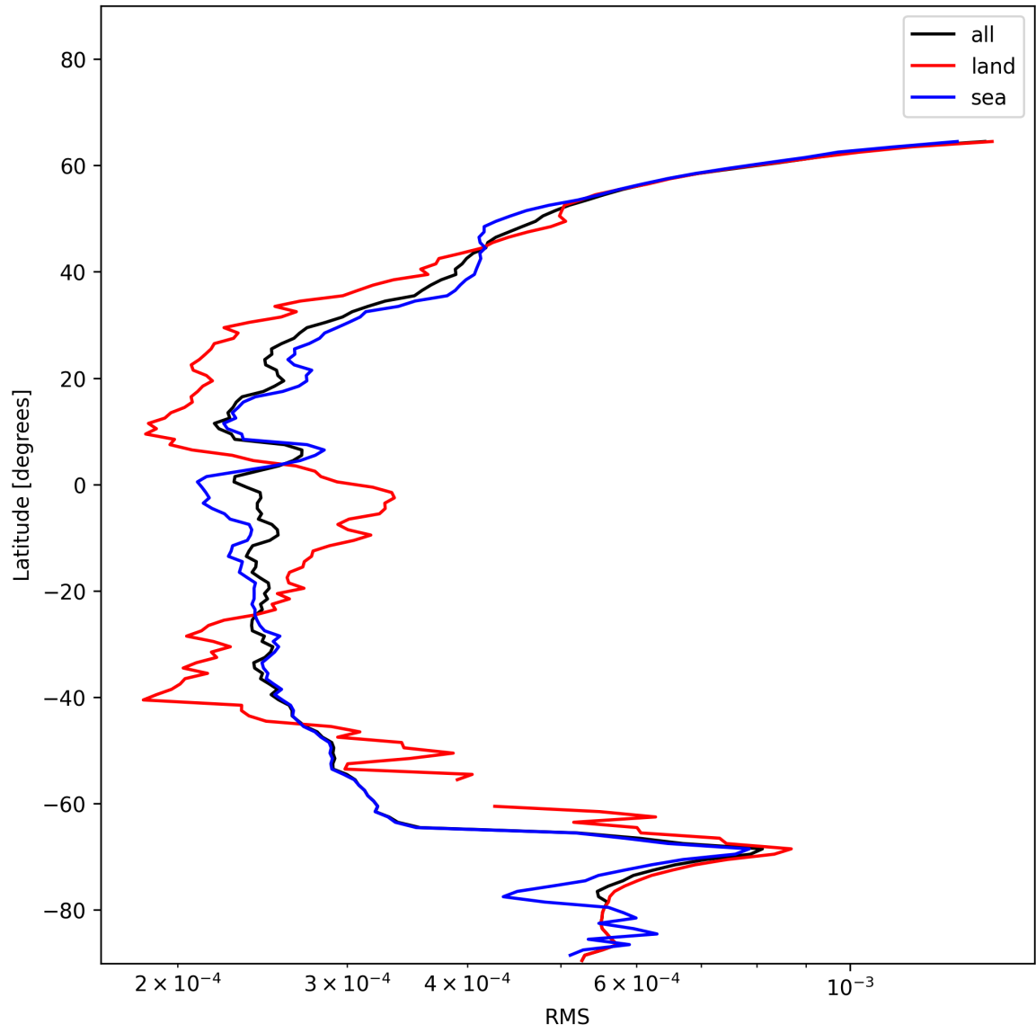
Figure 24: Zonal average of “RMS” for 2024-12-26 to 2024-12-27.
