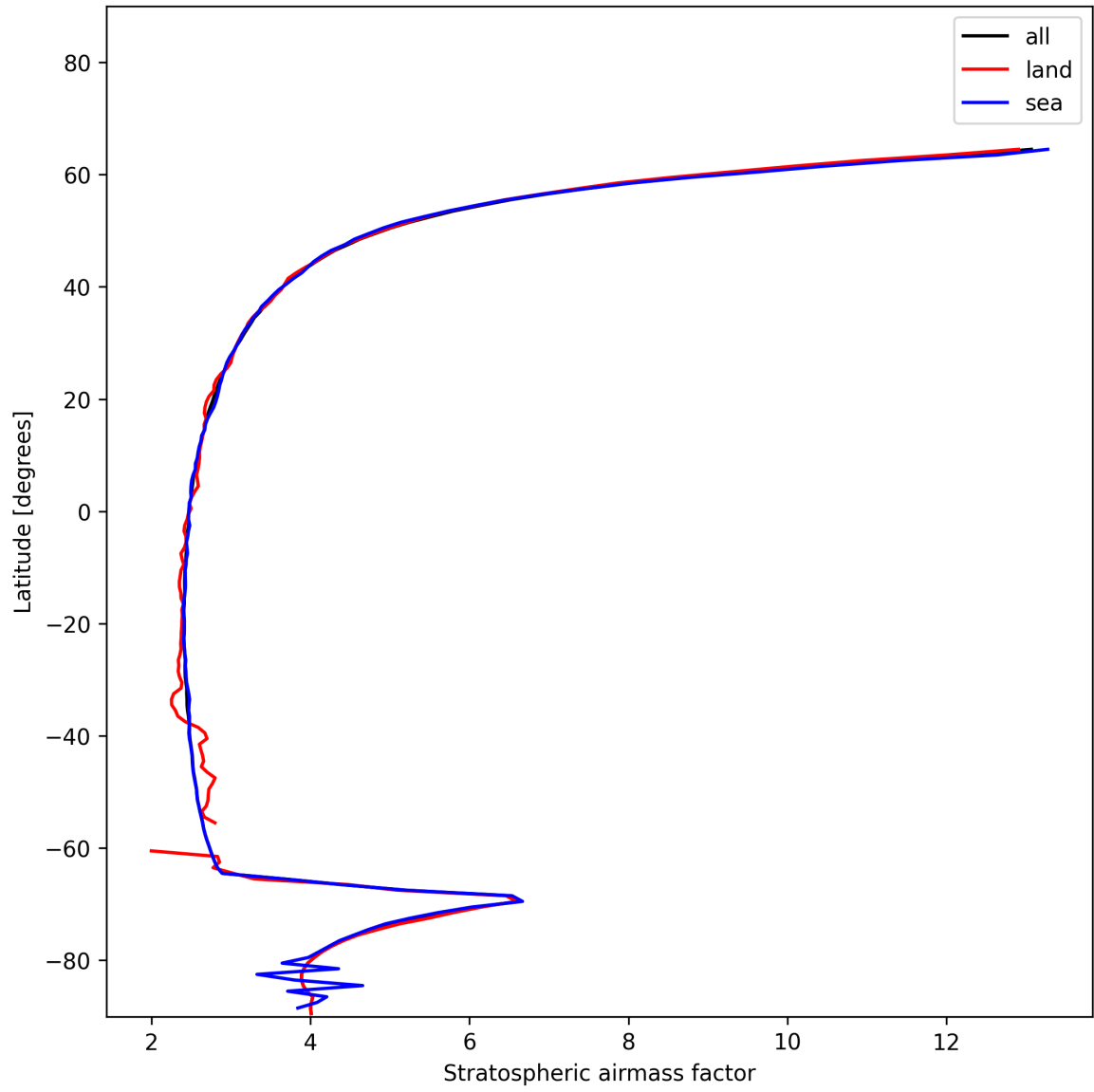
Figure 25: Zonal average of “Stratospheric airmass factor” for 2024-12-26 to 2024-12-27.
