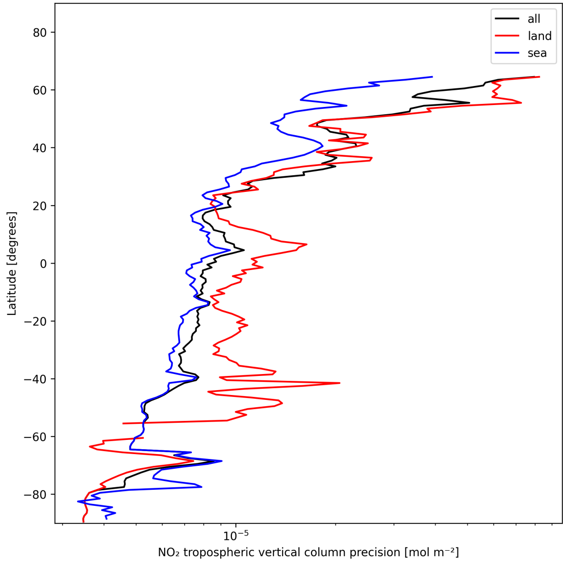
Figure 11: Zonal average of “NO 2 tropospheric vertical column precision” for 2024-12-26 to 2024-12-27.
