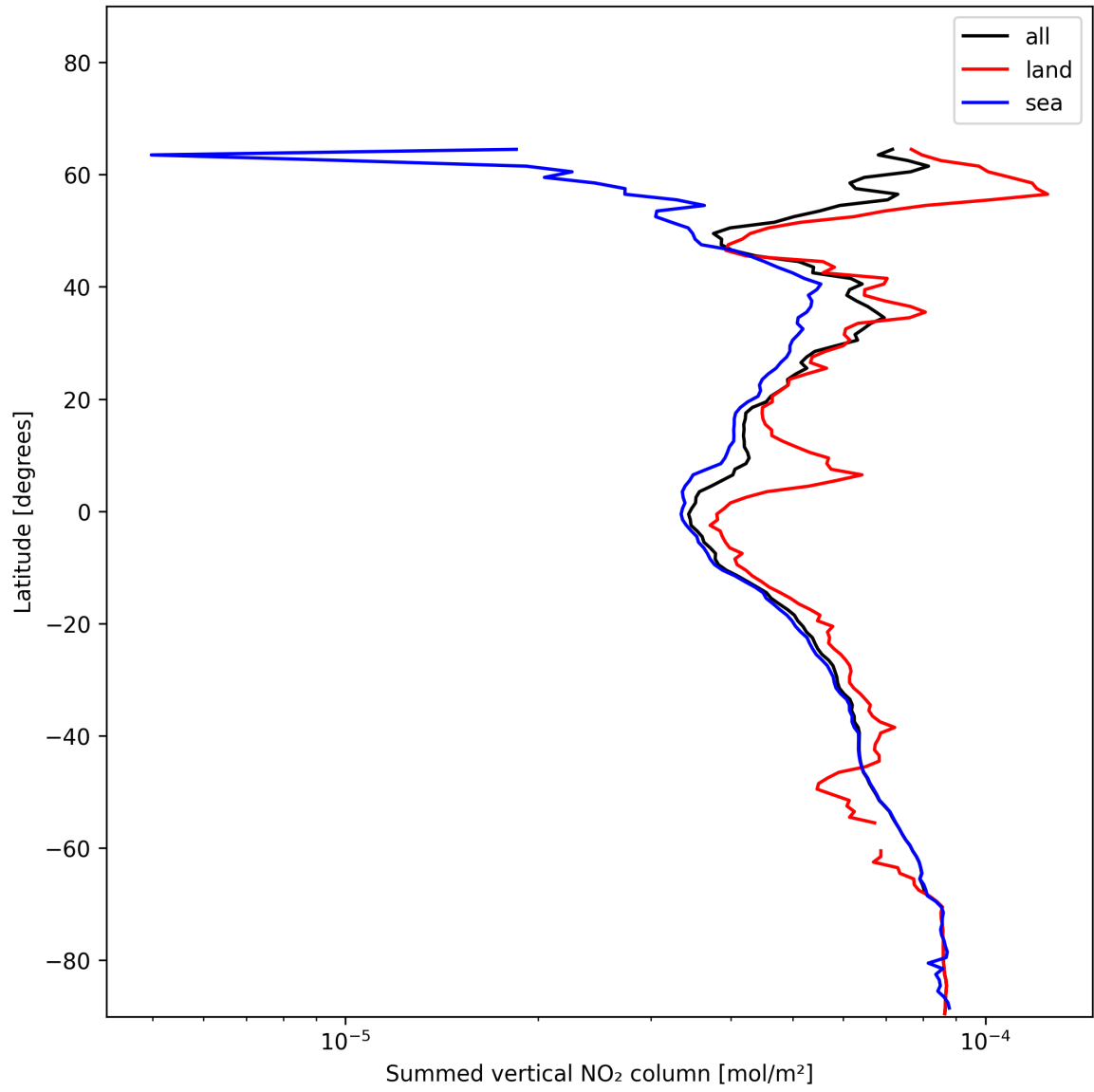
Figure 21: Zonal average of “Summed vertical NO 2 column” for 2024-12-26 to 2024-12-27.
