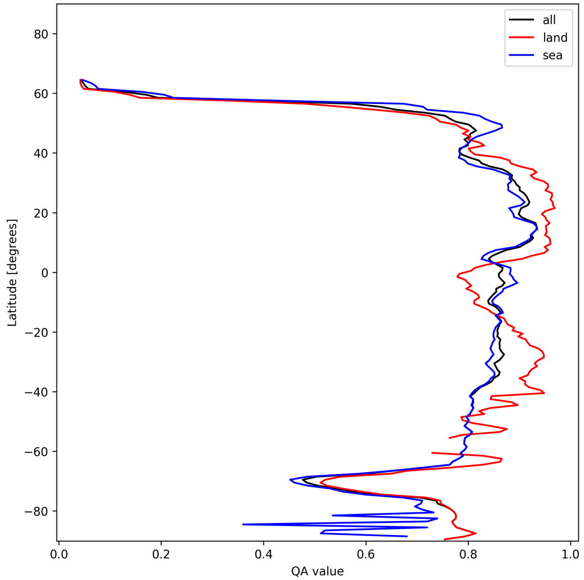
Figure 9: Zonal average of “QA value” for 2024-12-26 to 2024-12-27.
