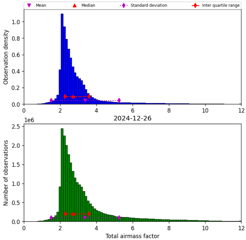
Figure 30: Histogram of “Total airmass factor” for 2024-12-26 to 2024-12-27
