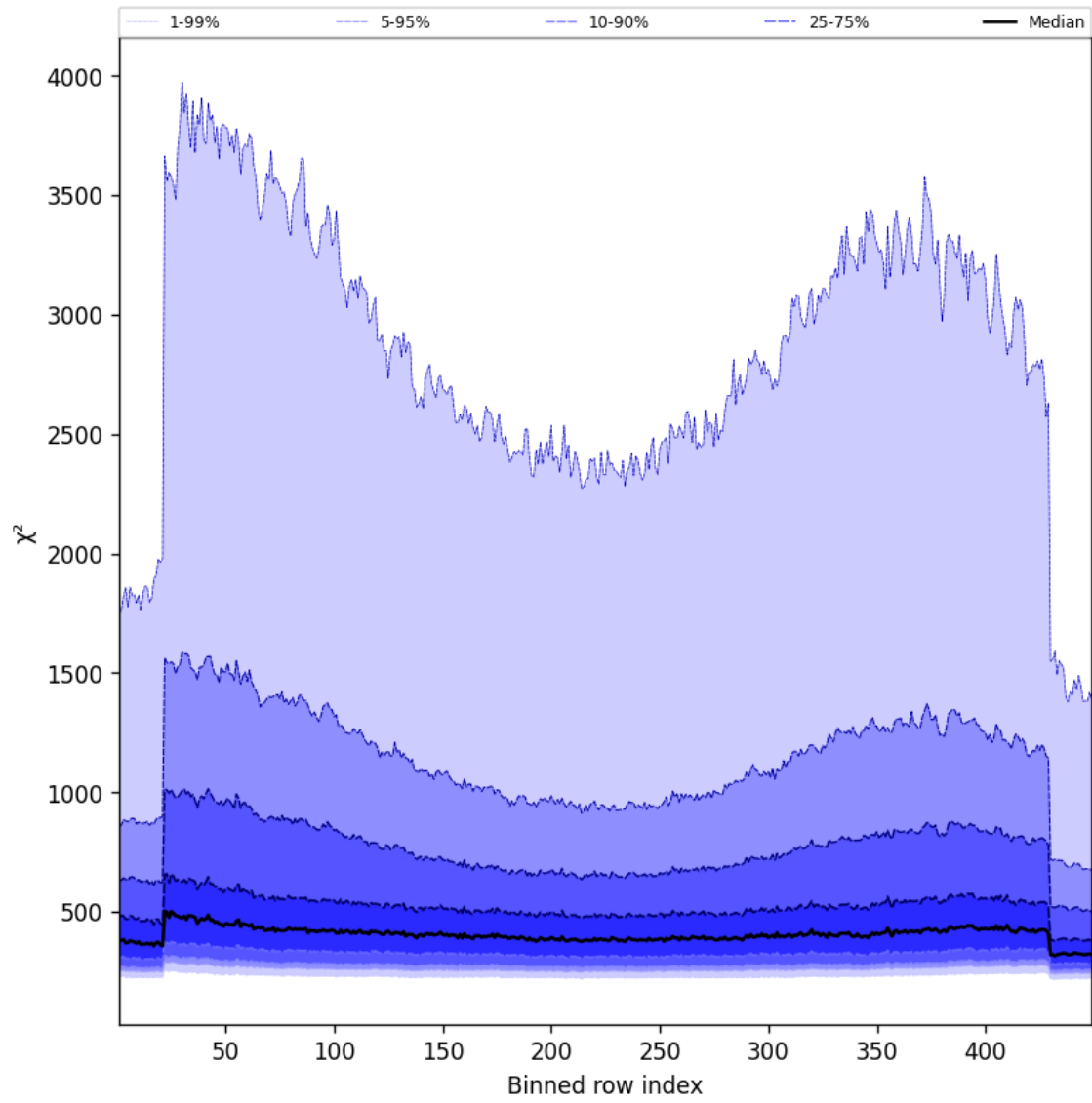
Figure 57: Along track statistics of “ \chi^2 ” for 2024-12-26 to 2024-12-27
