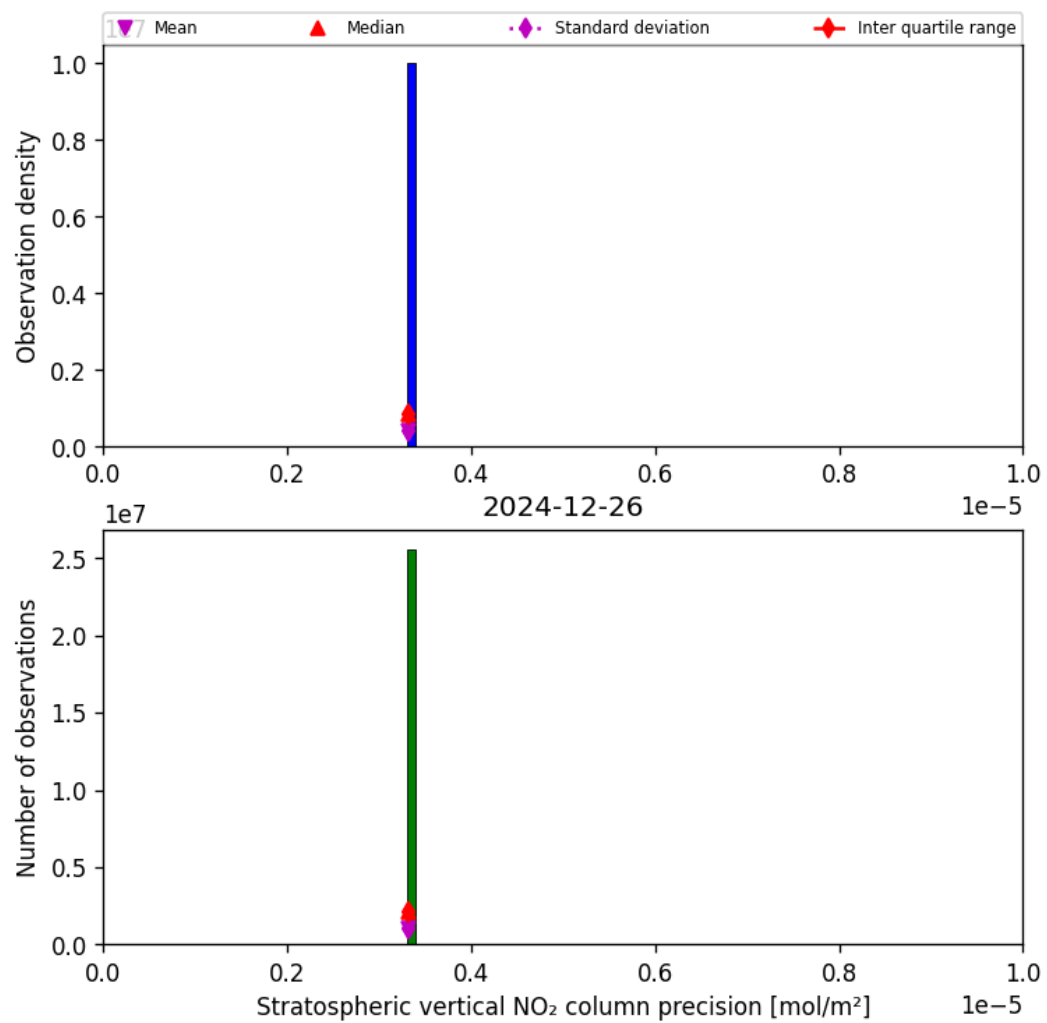
Figure 35: Histogram of “Stratospheric vertical NO 2 column precision” for 2024-12-26 to 2024-12-27
