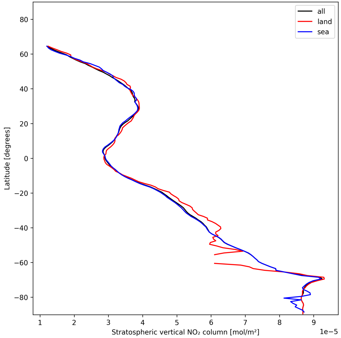
Figure 17: Zonal average of “Stratospheric vertical NO 2 column” for 2024-12-26 to 2024-12-27.
