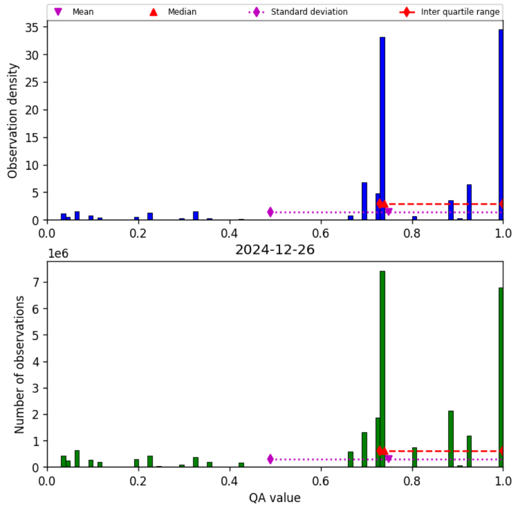
Figure 26: Histogram of “QA value” for 2024-12-26 to 2024-12-27
