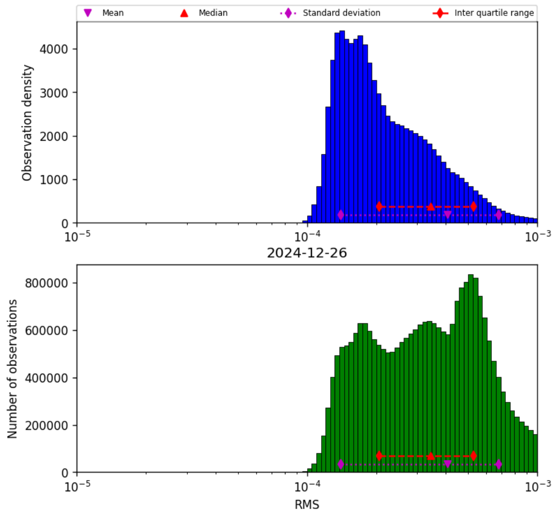
Figure 41: Histogram of “RMS” for 2024-12-26 to 2024-12-27
