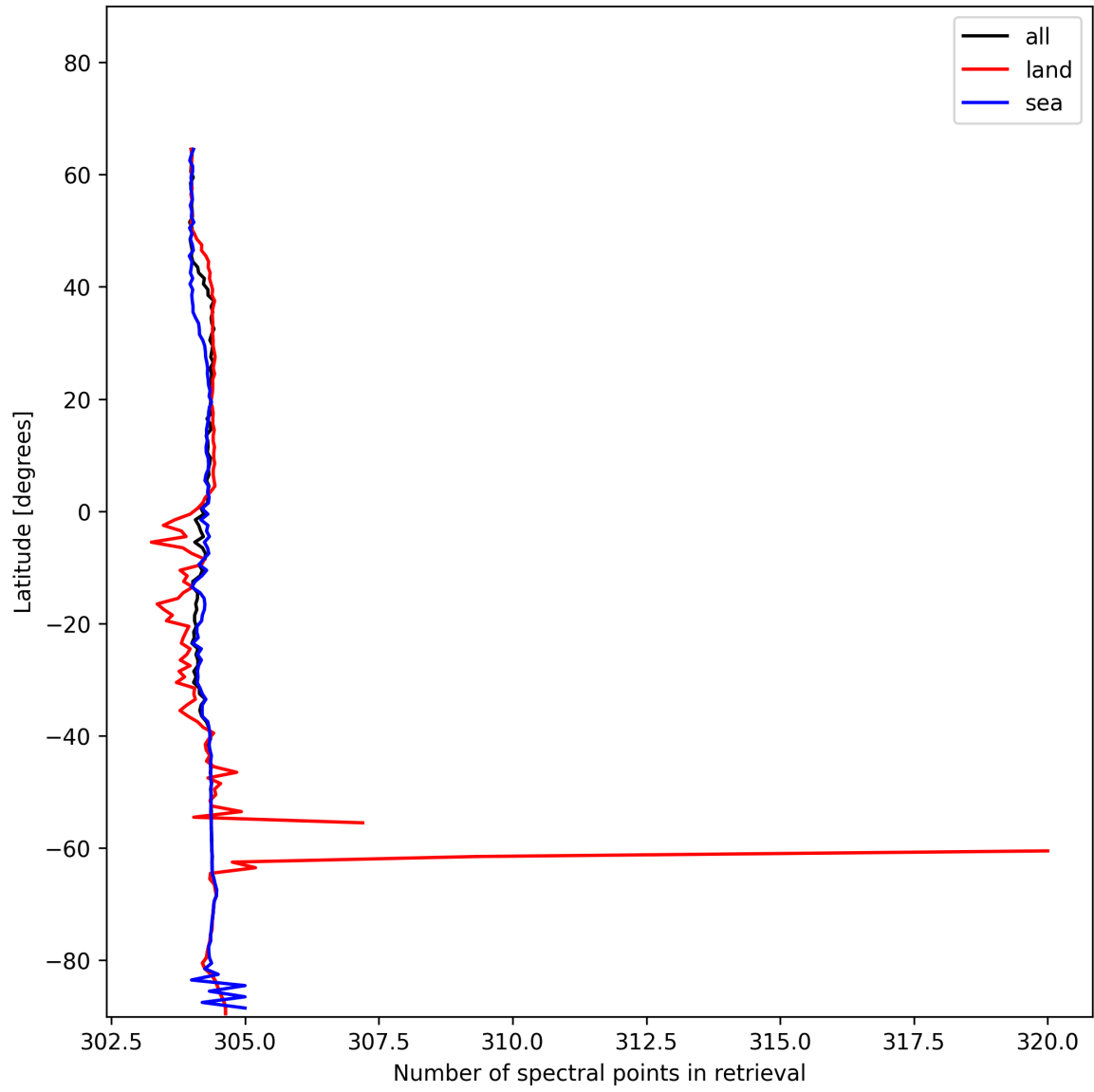
Figure 14: Zonal average of “Number of spectral points in retrieval” for 2024-12-26 to 2024-12-27.
