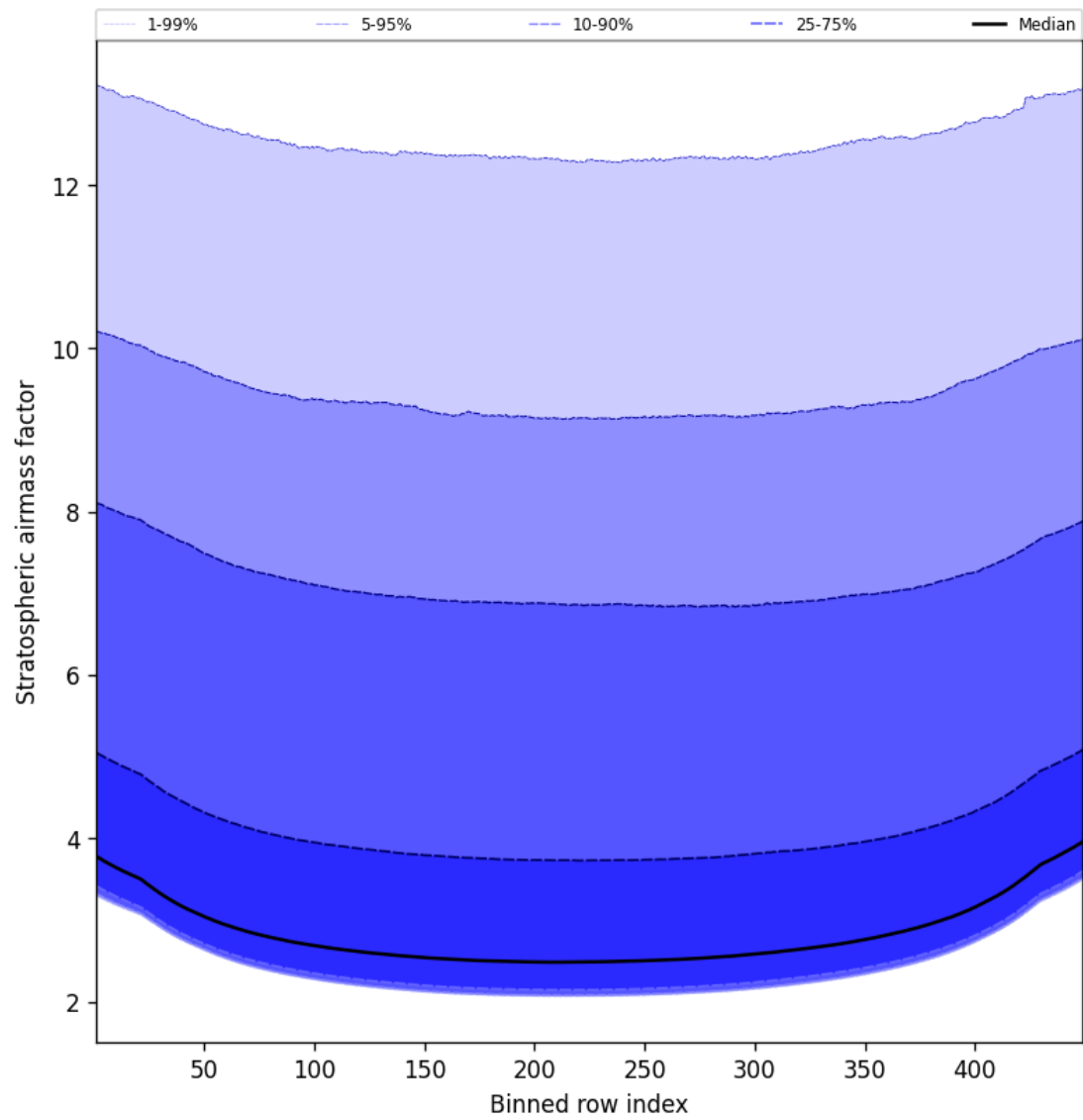
Figure 59: Along track statistics of “Stratospheric airmass factor” for 2024-12-26 to 2024-12-27
