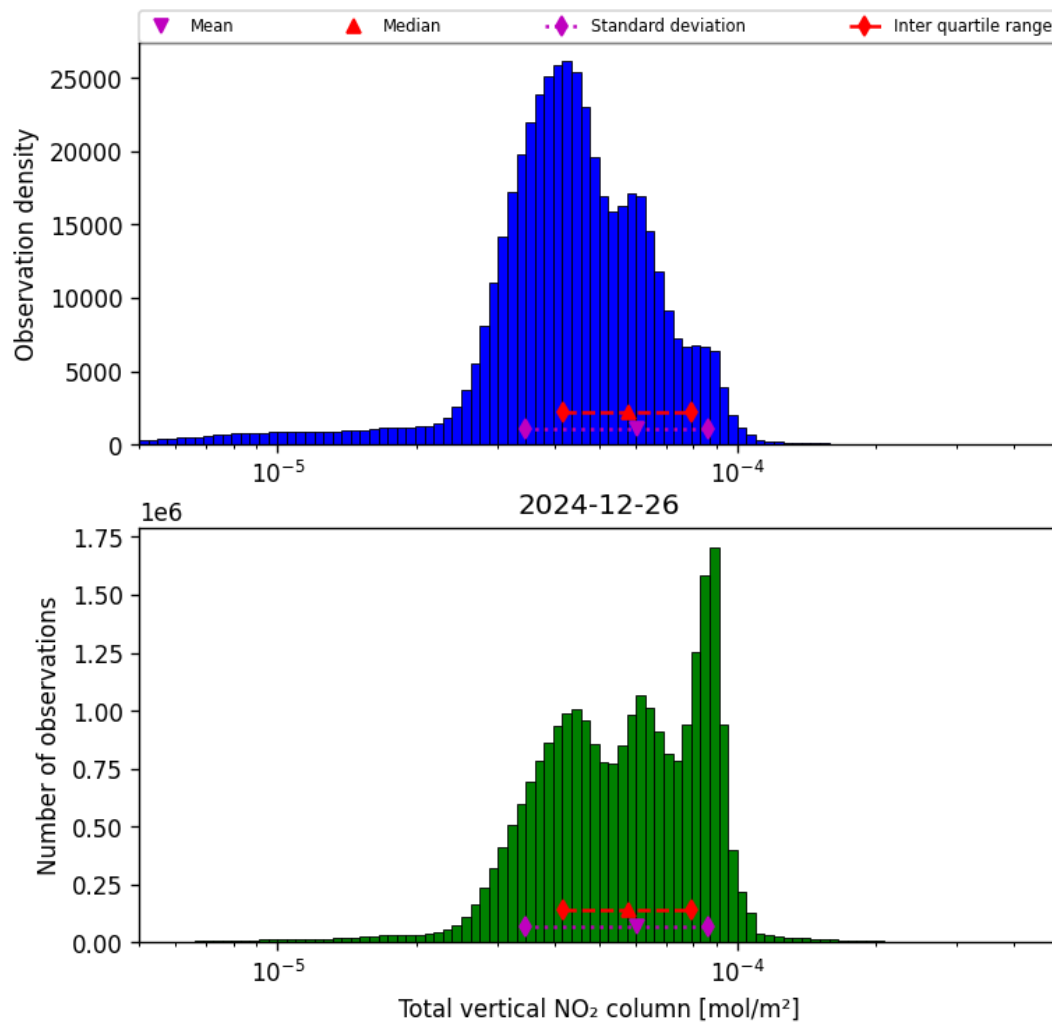
Figure 36: Histogram of “Total vertical NO 2 column” for 2024-12-26 to 2024-12-27
