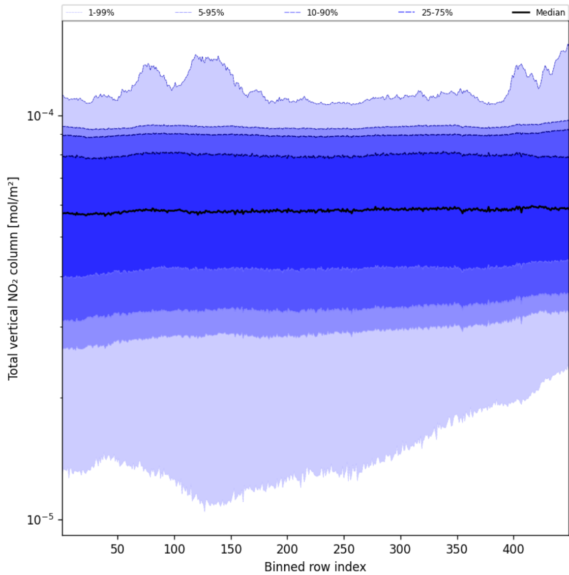
Figure 53: Along track statistics of “Total vertical NO 2 column” for 2024-12-26 to 2024-12-27
