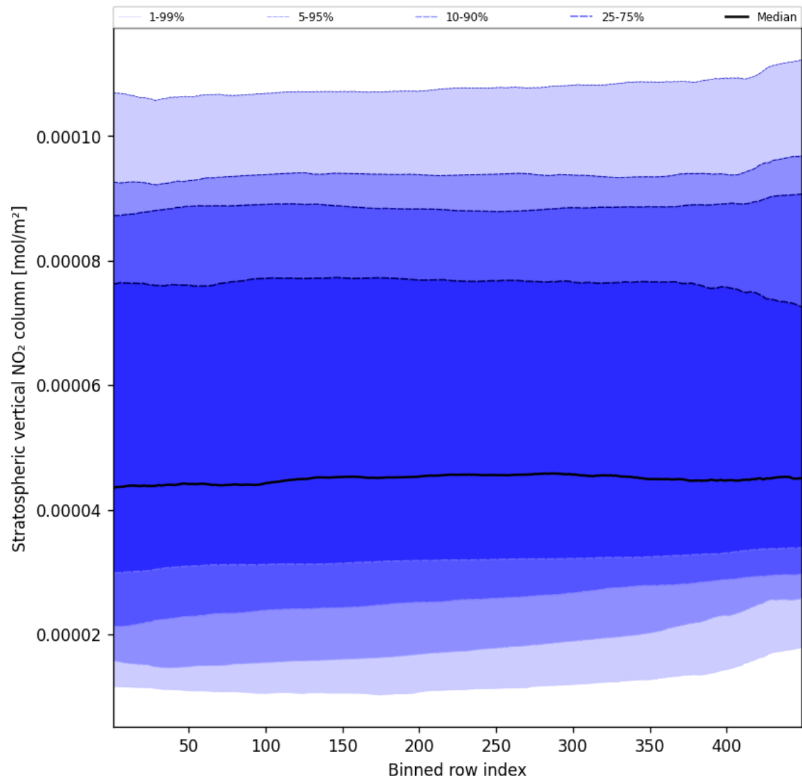
Figure 51: Along track statistics of “Stratospheric vertical NO 2 column” for 2024-12-26 to 2024-12-27
