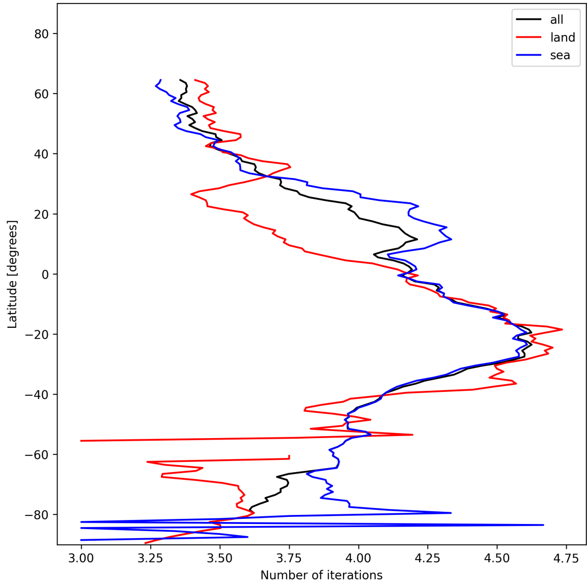
Figure 15: Zonal average of “Number of iterations” for 2024-12-26 to 2024-12-27.
