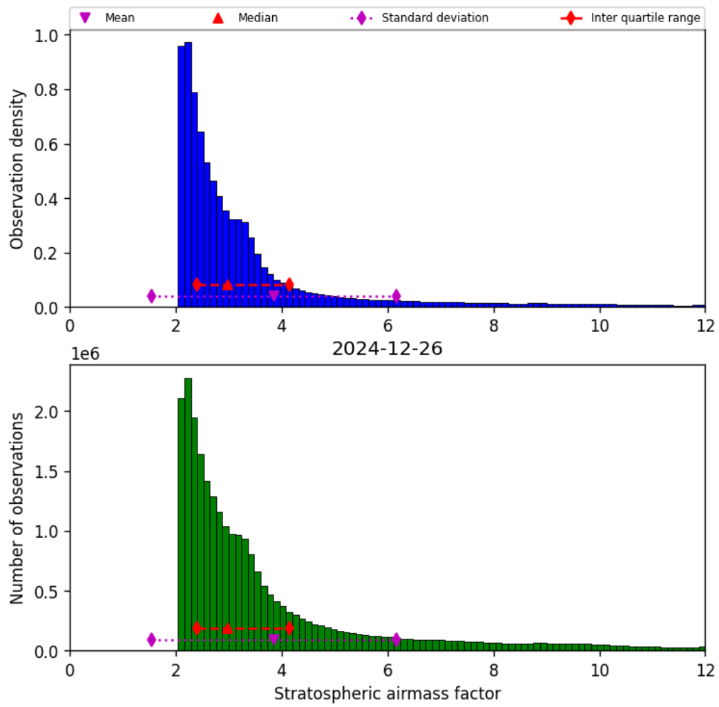
Figure 42: Histogram of “Stratospheric airmass factor” for 2024-12-26 to 2024-12-27
