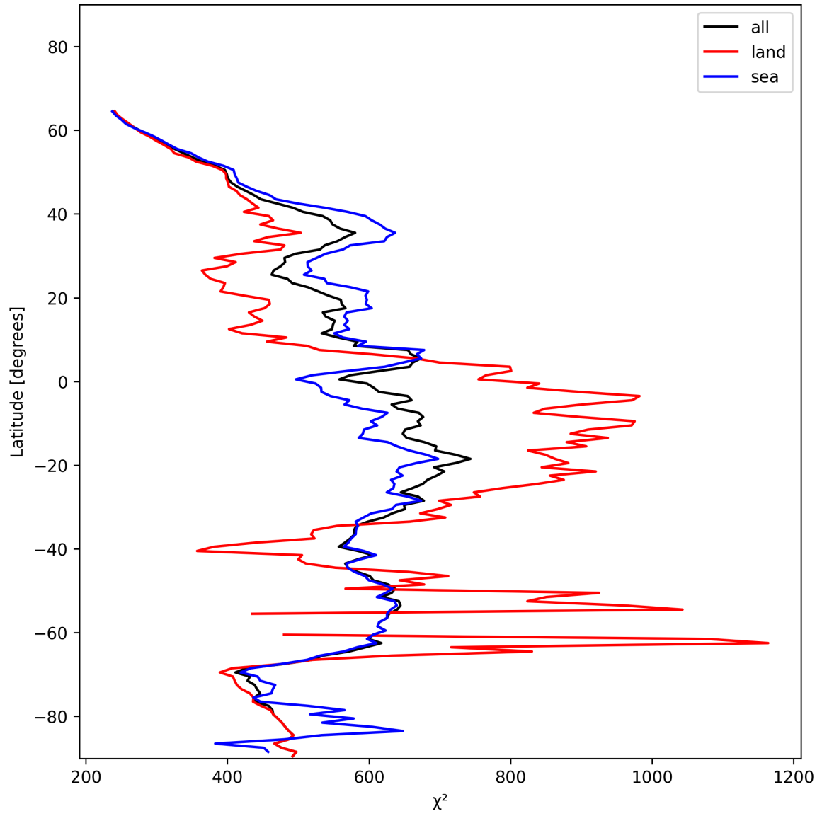
Figure 23: Zonal average of “ \chi^2 ” for 2024-12-26 to 2024-12-27.
