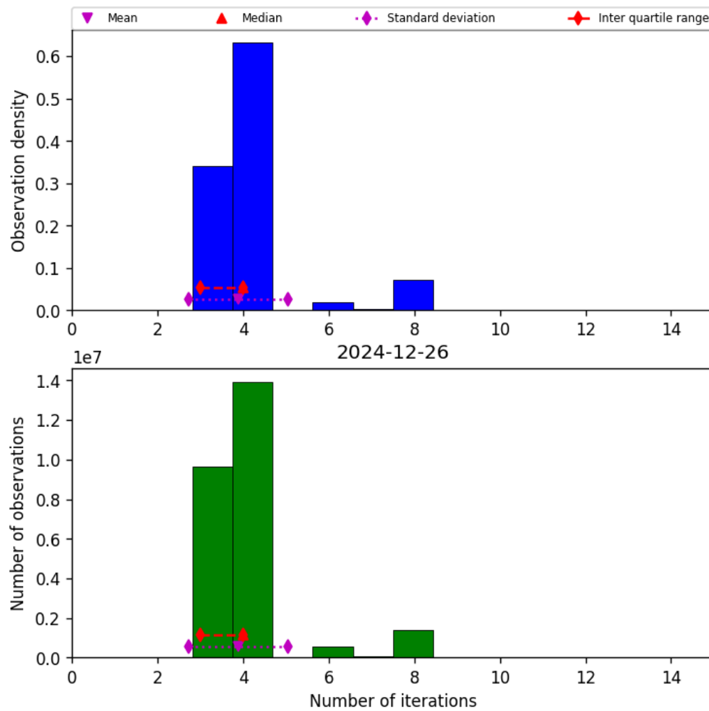
Figure 32: Histogram of “Number of iterations” for 2024-12-26 to 2024-12-27
