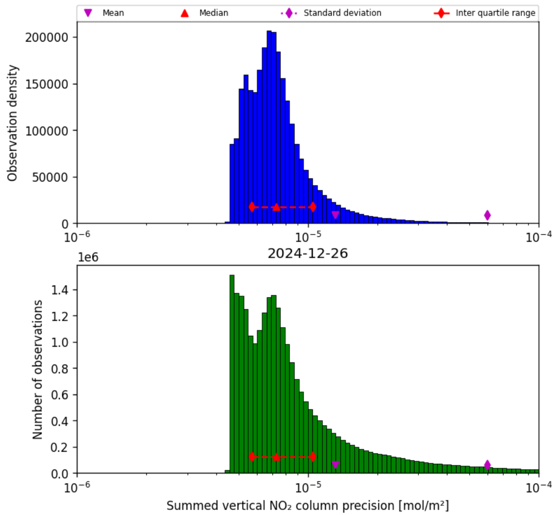
Figure 39: Histogram of "Summed vertical NO 2 column precision" for 2024-12-26 to 2024-12-27
