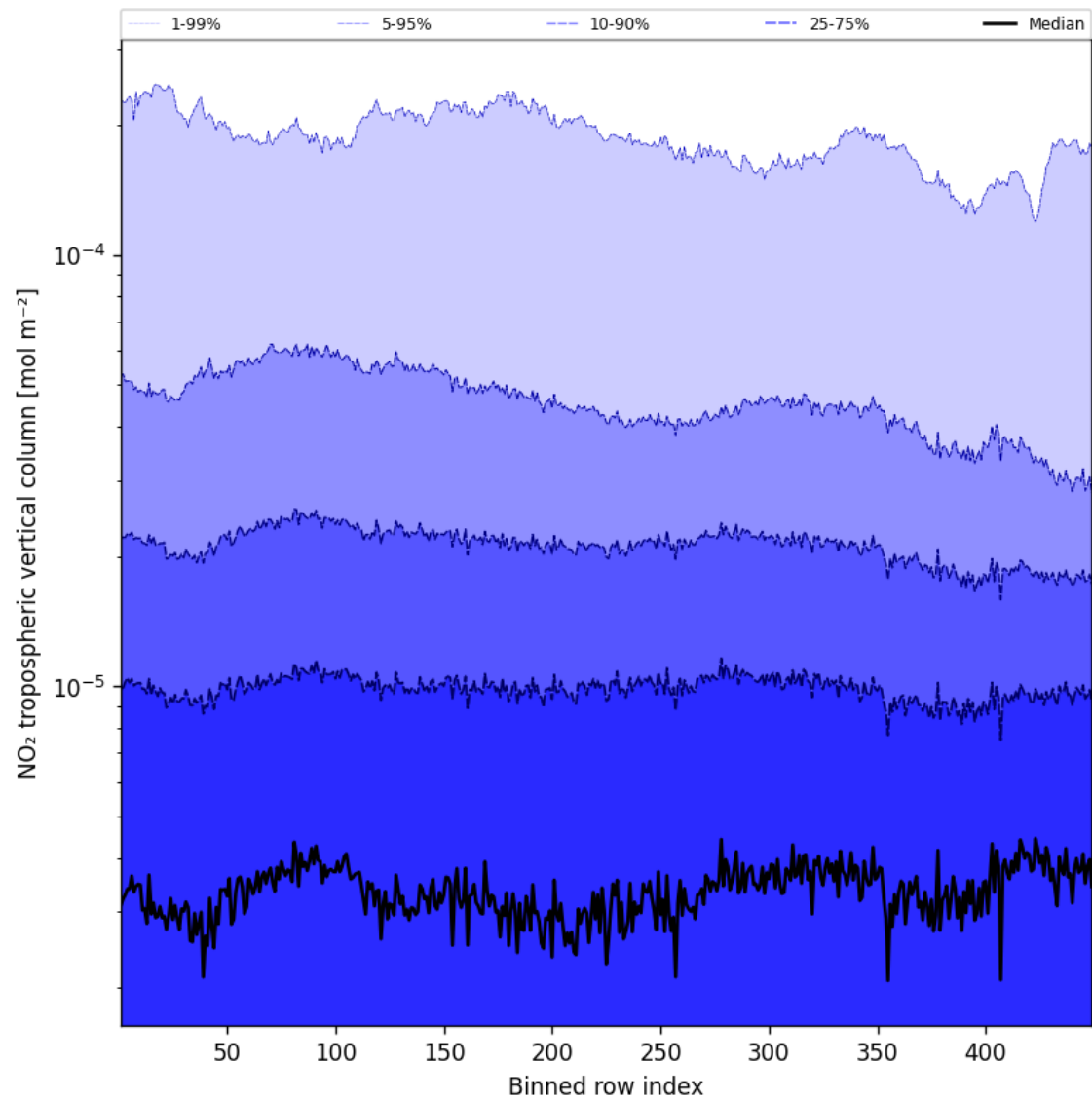
Figure 44: Along track statistics of “NO 2 tropospheric vertical column” for 2024-12-26 to 2024-12-27
