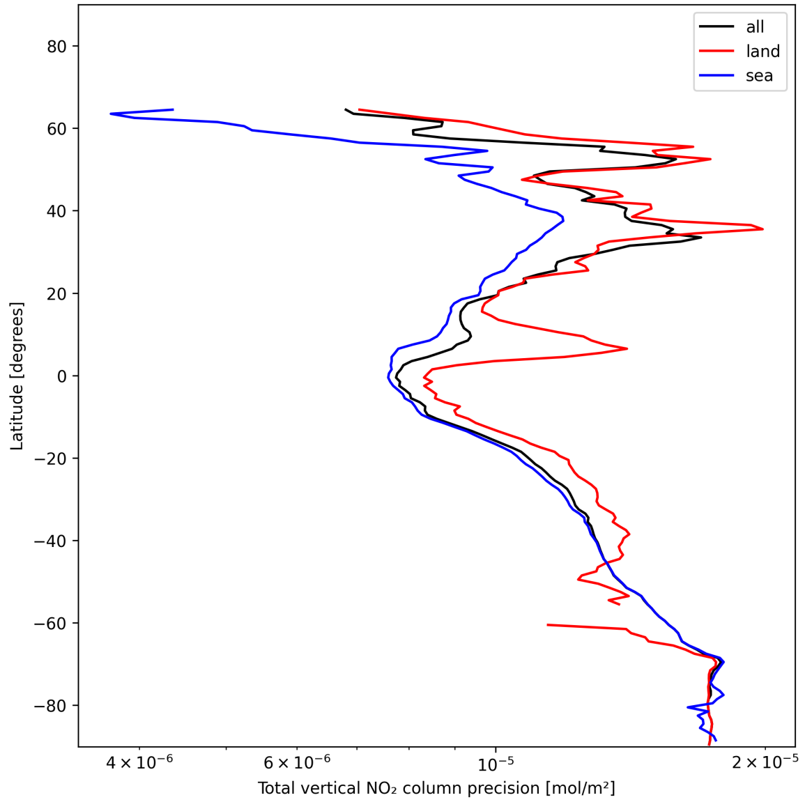
Figure 20: Zonal average of “Total vertical NO 2 column precision” for 2024-12-26 to 2024-12-27.
