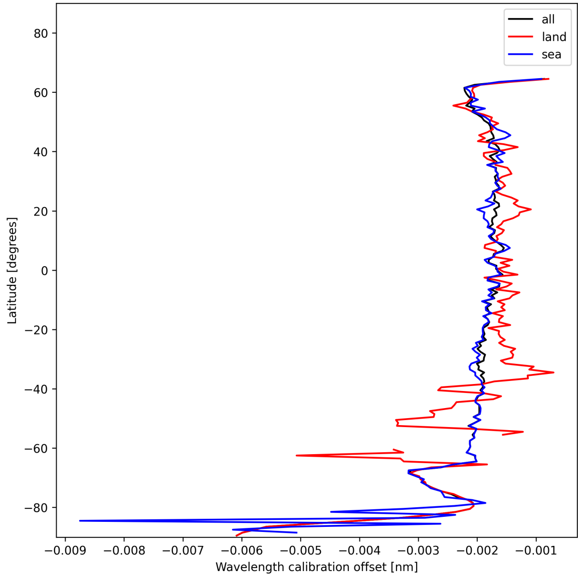
Figure 16: Zonal average of “Wavelength calibration offset” for 2024-12-26 to 2024-12-27.
