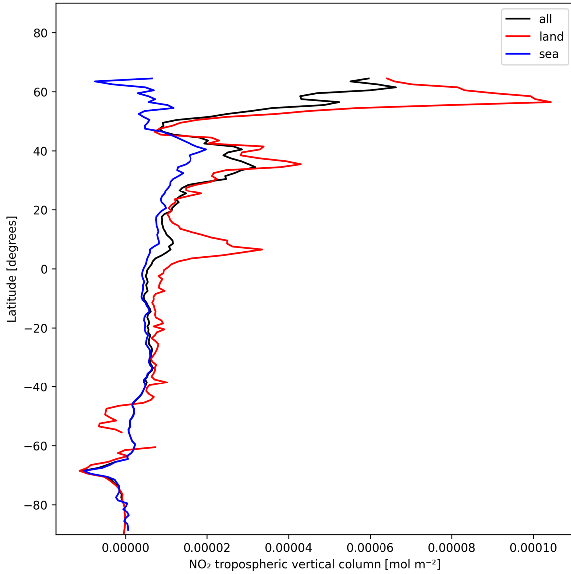
Figure 10: Zonal average of “NO 2 tropospheric vertical column” for 2024-12-26 to 2024-12-27.
