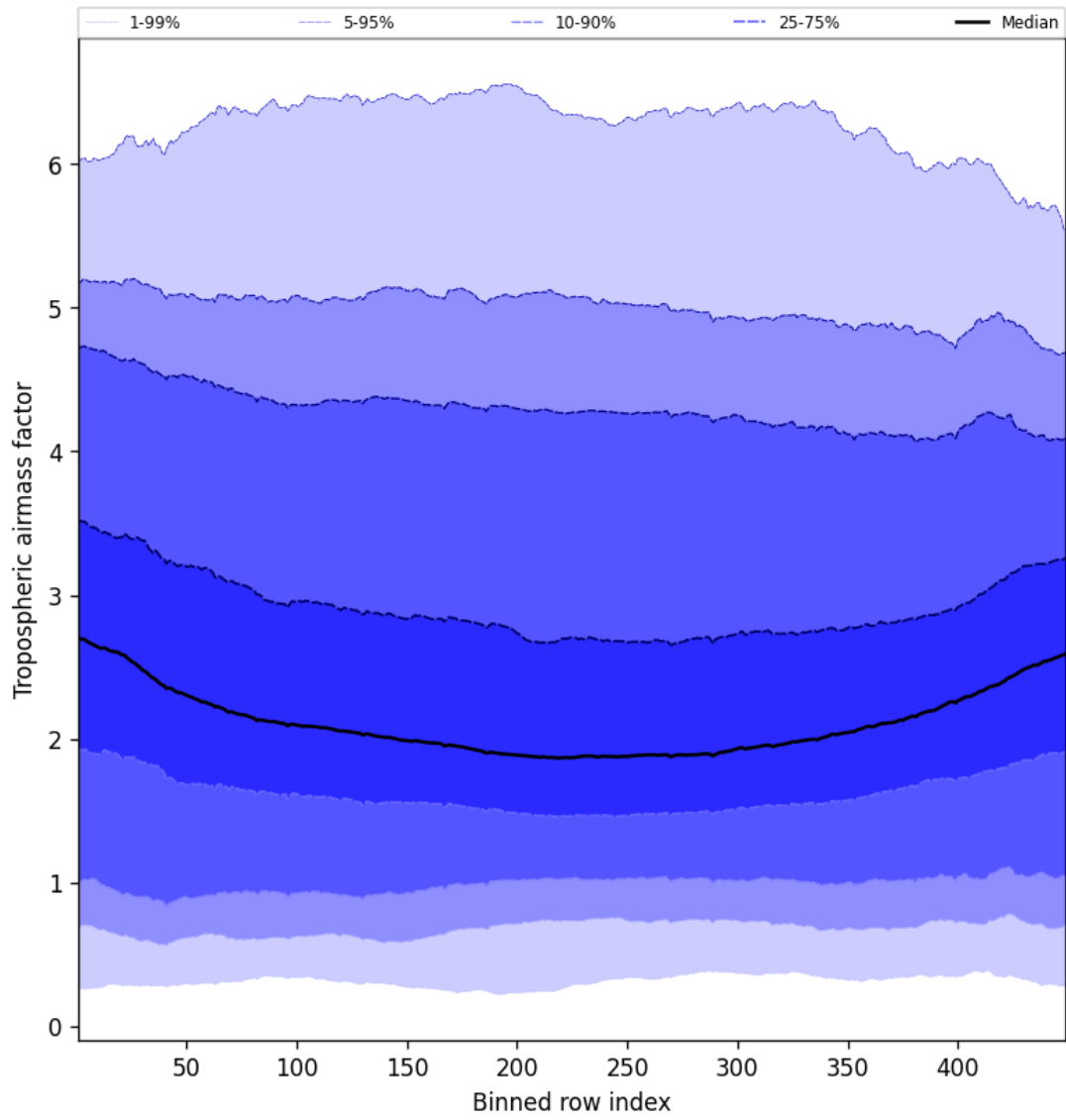
Figure 46: Along track statistics of “Tropospheric airmass factor” for 2024-12-26 to 2024-12-27
