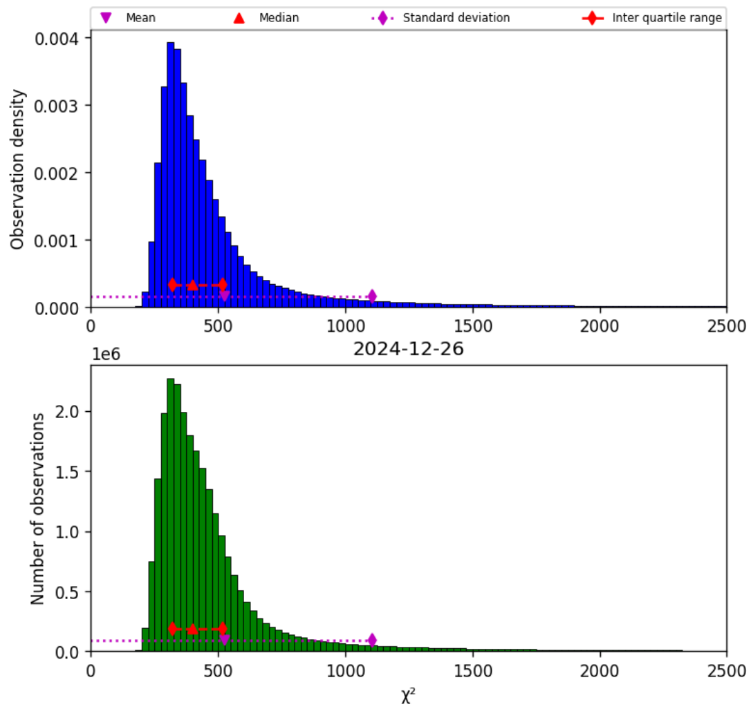
Figure 40: Histogram of “ \chi^2 ” for 2024-12-26 to 2024-12-27
