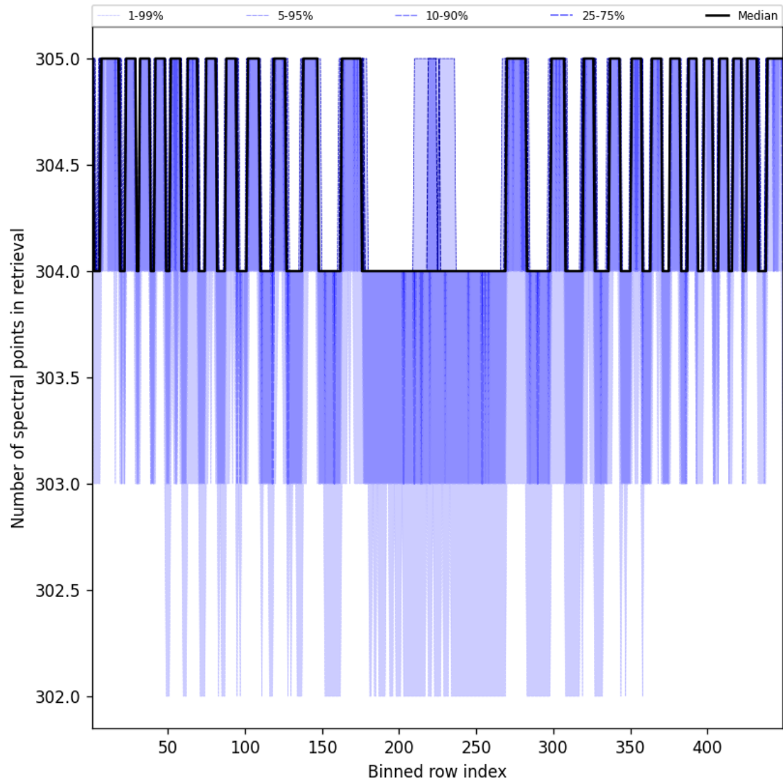
Figure 48: Along track statistics of “Number of spectral points in retrieval” for 2024-12-26 to 2024-12-27
