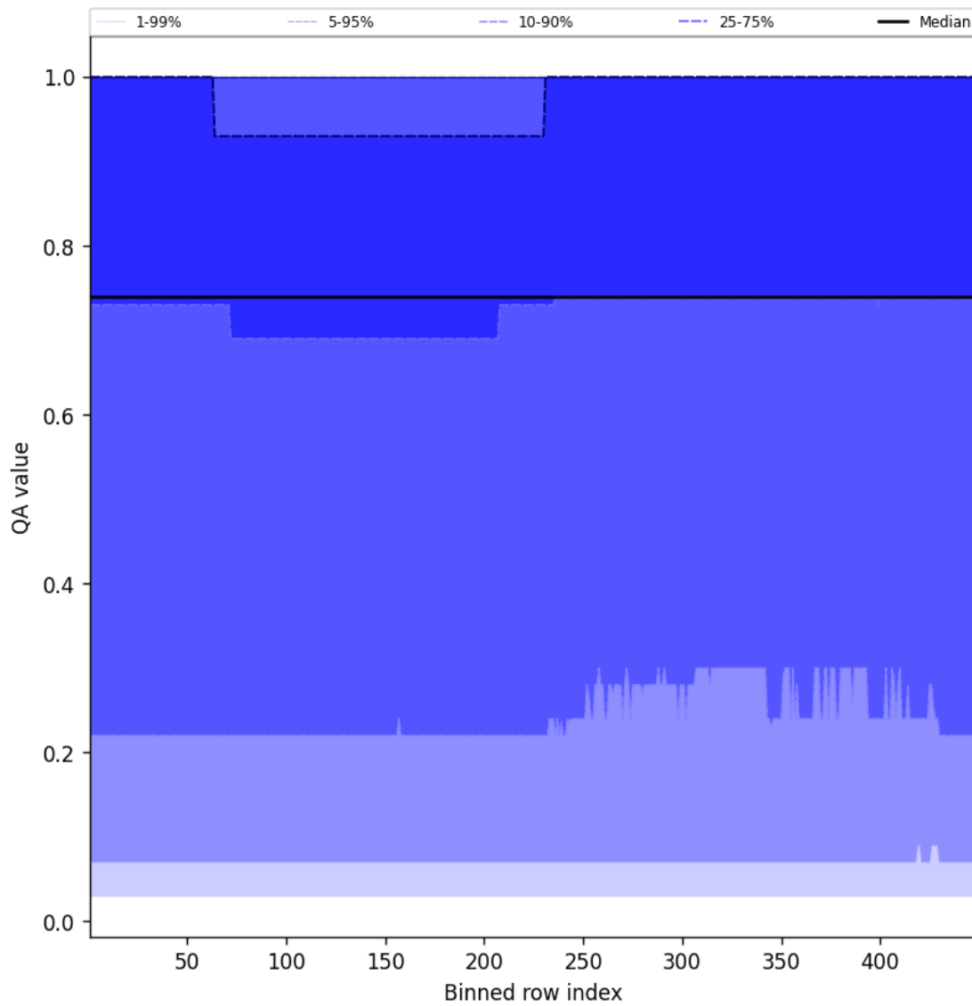
Figure 43: Along track statistics of “QA value” for 2024-12-26 to 2024-12-27
