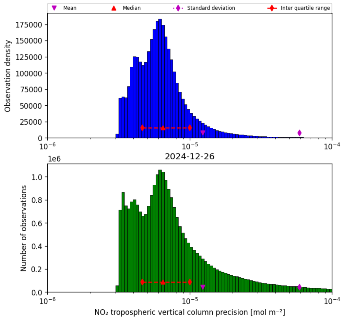
Figure 28: Histogram of “NO 2 tropospheric vertical column precision” for 2024-12-26 to 2024-12-27
