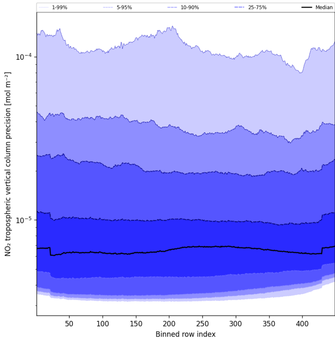
Figure 45: Along track statistics of “NO 2 tropospheric vertical column precision” for 2024-12-26 to 2024-12-27
