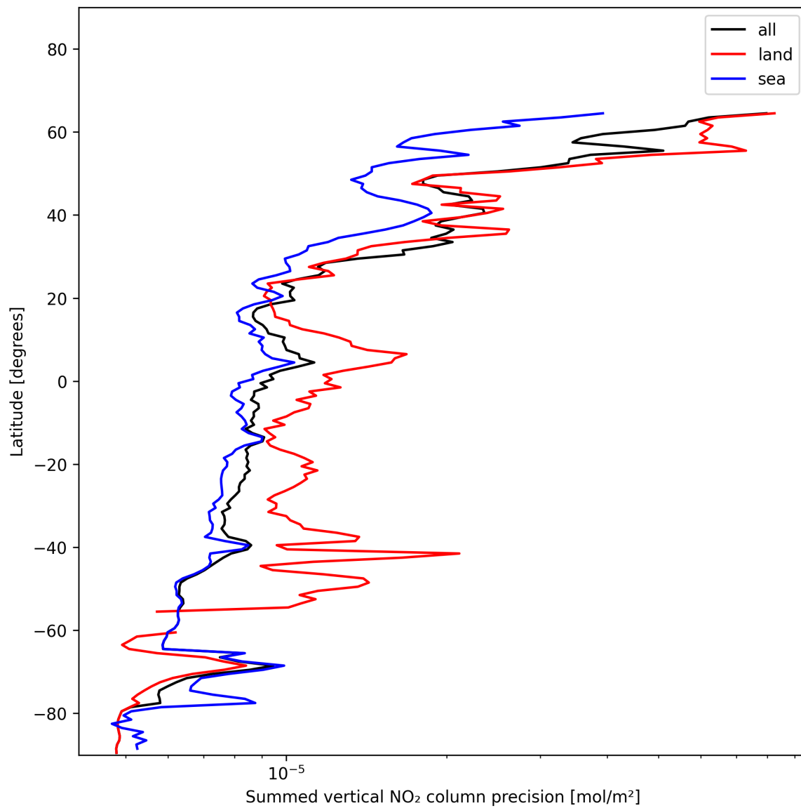
Figure 22: Zonal average of “Summed vertical NO 2 column precision” for 2024-12-26 to 2024-12-27.
