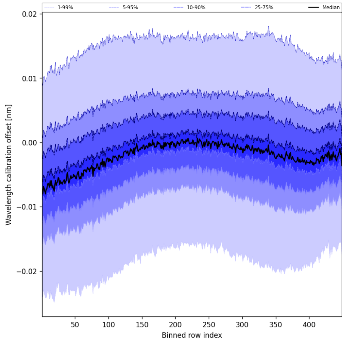
Figure 50: Along track statistics of “Wavelength calibration offset” for 2024-12-26 to 2024-12-27
