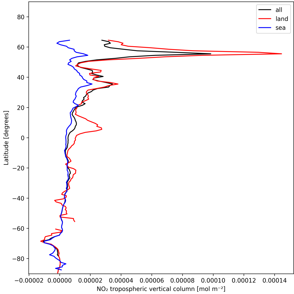
Figure 10: Zonal average of “NO 2 tropospheric vertical column” for 2024-12-27 to 2024-12-28.
