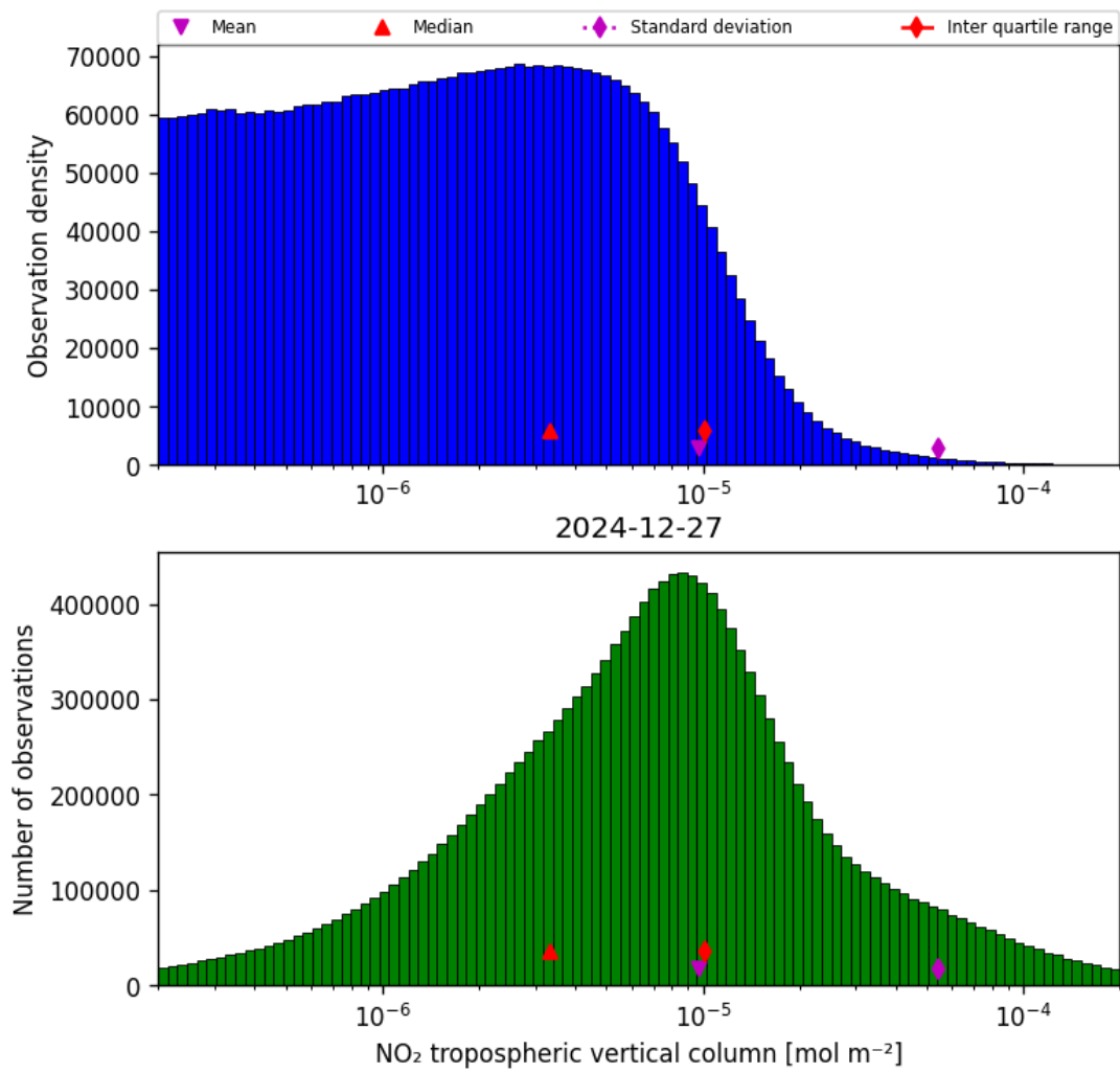
Figure 27: Histogram of “NO 2 tropospheric vertical column” for 2024-12-27 to 2024-12-28
