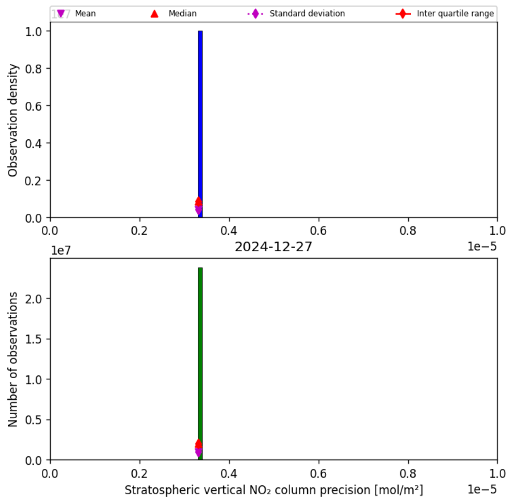
Figure 35: Histogram of “Stratospheric vertical NO 2 column precision” for 2024-12-27 to 2024-12-28
