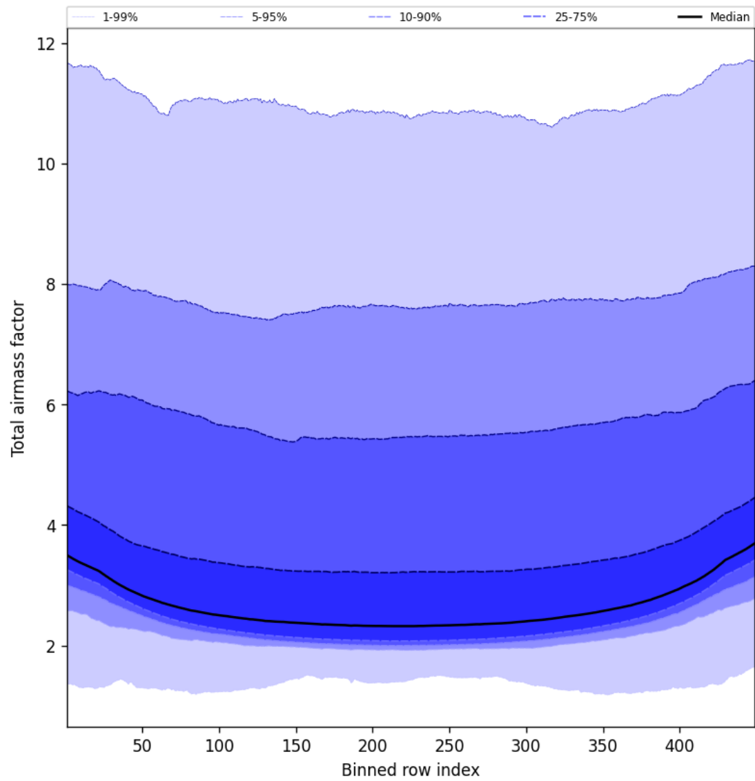
Figure 47: Along track statistics of “Total airmass factor” for 2024-12-27 to 2024-12-28
