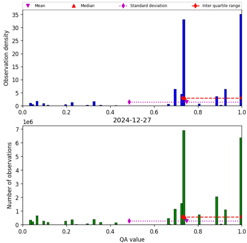
Figure 26: Histogram of “QA value” for 2024-12-27 to 2024-12-28
