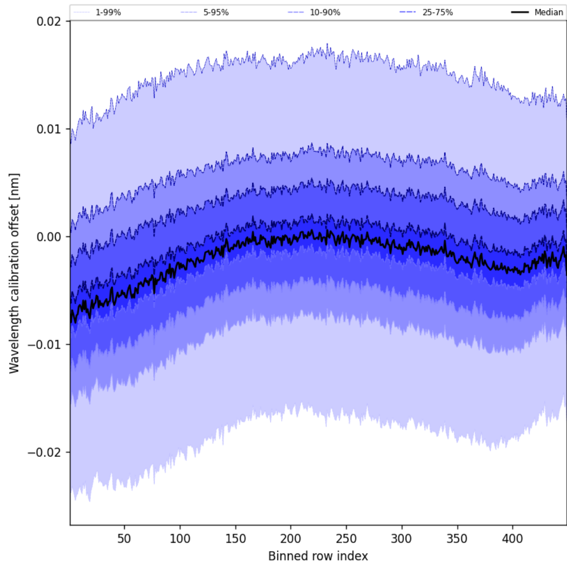
Figure 50: Along track statistics of “Wavelength calibration offset” for 2024-12-27 to 2024-12-28
