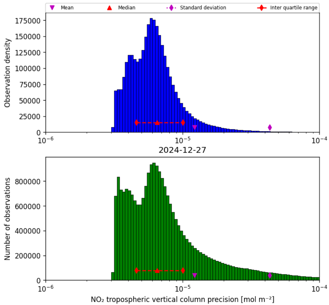
Figure 28: Histogram of “NO 2 tropospheric vertical column precision” for 2024-12-27 to 2024-12-28
