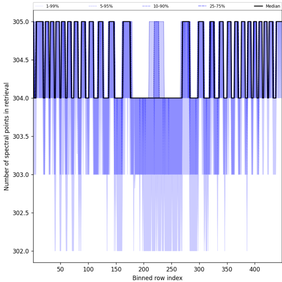
Figure 48: Along track statistics of “Number of spectral points in retrieval” for 2024-12-27 to 2024-12-28
