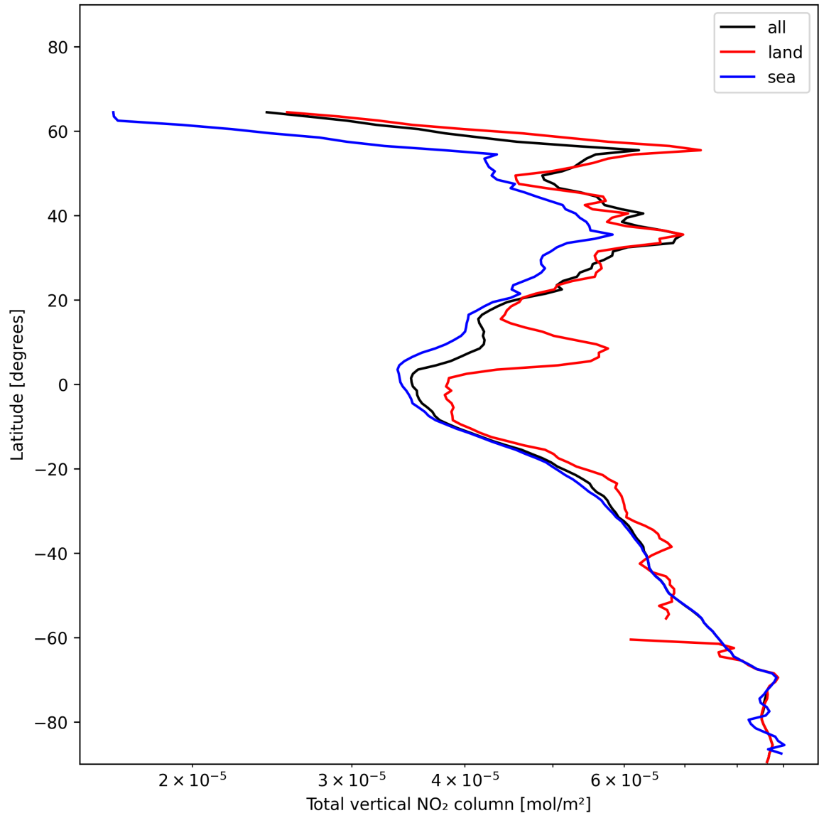
Figure 19: Zonal average of “Total vertical NO 2 column” for 2024-12-27 to 2024-12-28.
