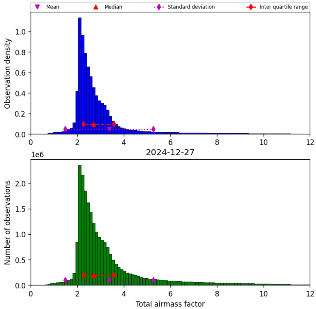
Figure 30: Histogram of “Total airmass factor” for 2024-12-27 to 2024-12-28
