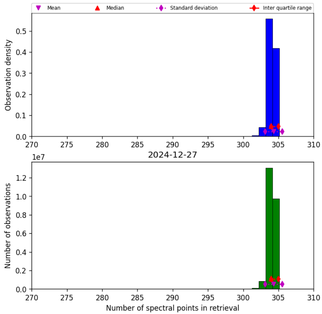
Figure 31: Histogram of “Number of spectral points in retrieval” for 2024-12-27 to 2024-12-28
