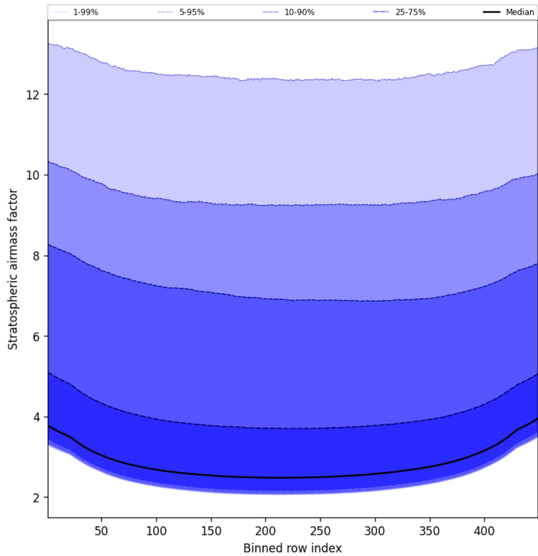
Figure 59: Along track statistics of “Stratospheric airmass factor” for 2024-12-27 to 2024-12-28
