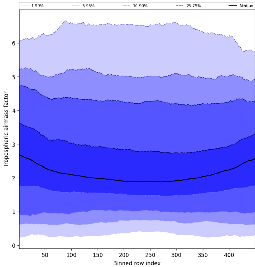
Figure 46: Along track statistics of “Tropospheric air mass factor” for 2024-12-27 to 2024-12-28
