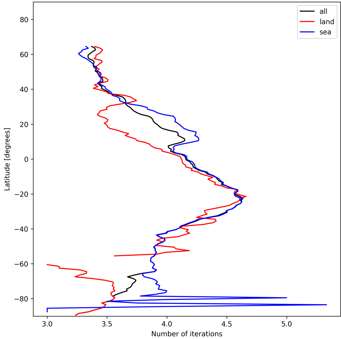
Figure 15: Zonal average of “Number of iterations” for 2024-12-27 to 2024-12-28.
