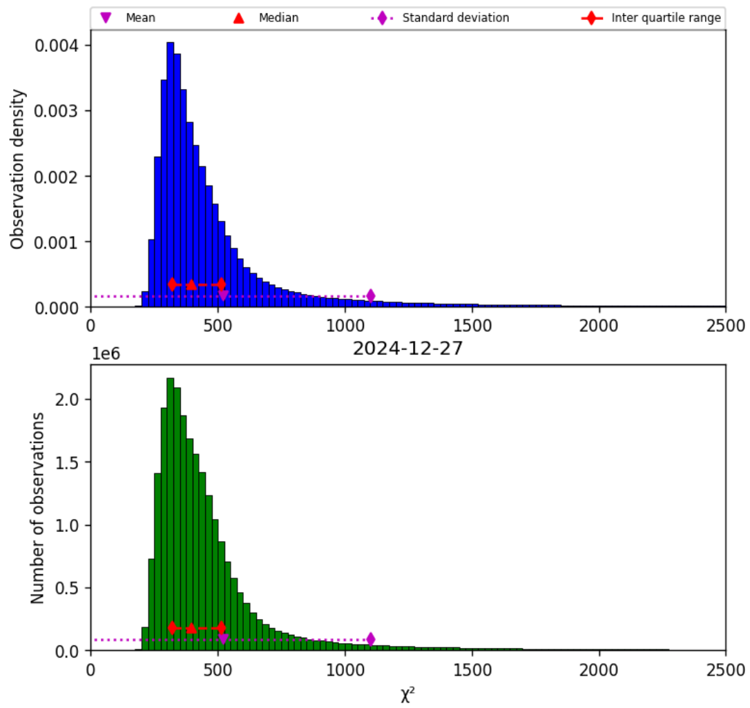
Figure 40: Histogram of “ \chi^2 ” for 2024-12-27 to 2024-12-28
