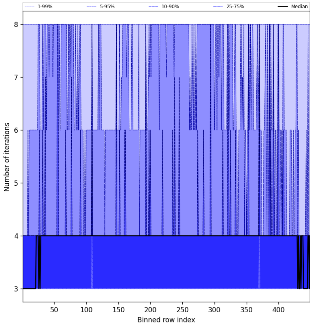
Figure 49: Along track statistics of “Number of iterations” for 2024-12-27 to 2024-12-28
