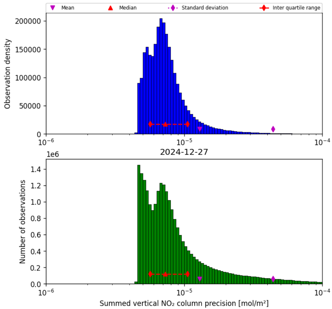
Figure 39: Histogram of “Summed vertical NO 2 column precision” for 2024-12-27 to 2024-12-28
