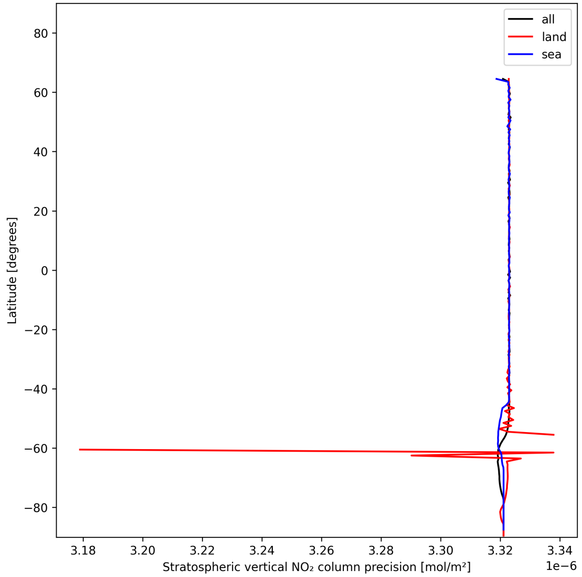
Figure 18: Zonal average of “Stratospheric vertical NO 2 column precision” for 2024-12-27 to 2024-12-28.
