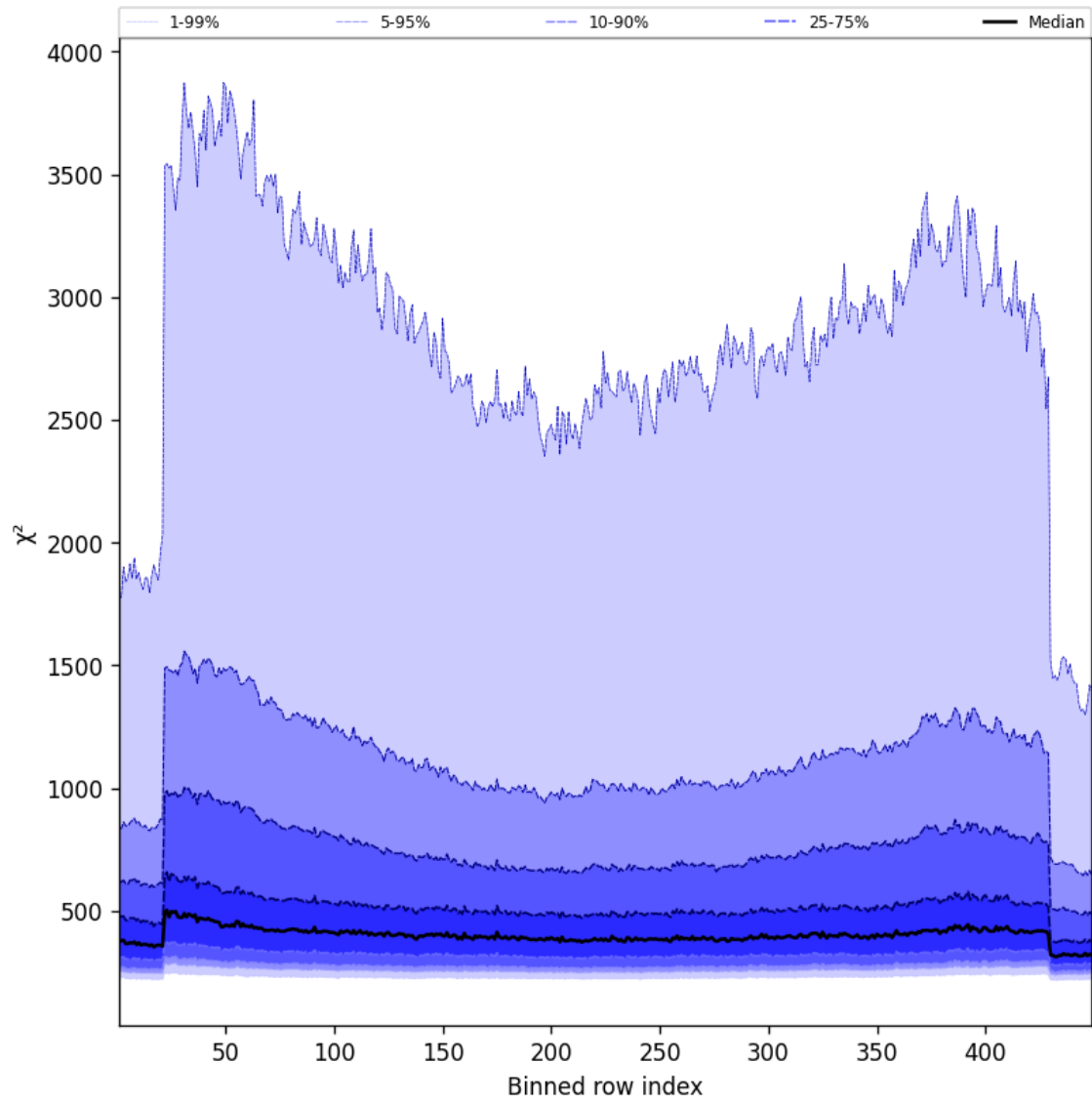
Figure 57: Along track statistics of “ \chi^2 ” for 2024-12-27 to 2024-12-28
