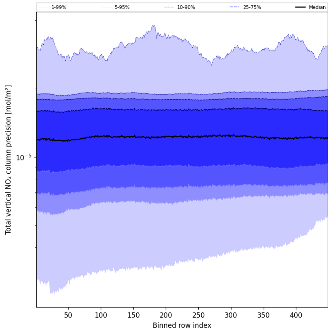
Figure 54: Along track statistics of “Total vertical NO 2 column precision” for 2024-12-27 to 2024-12-28
