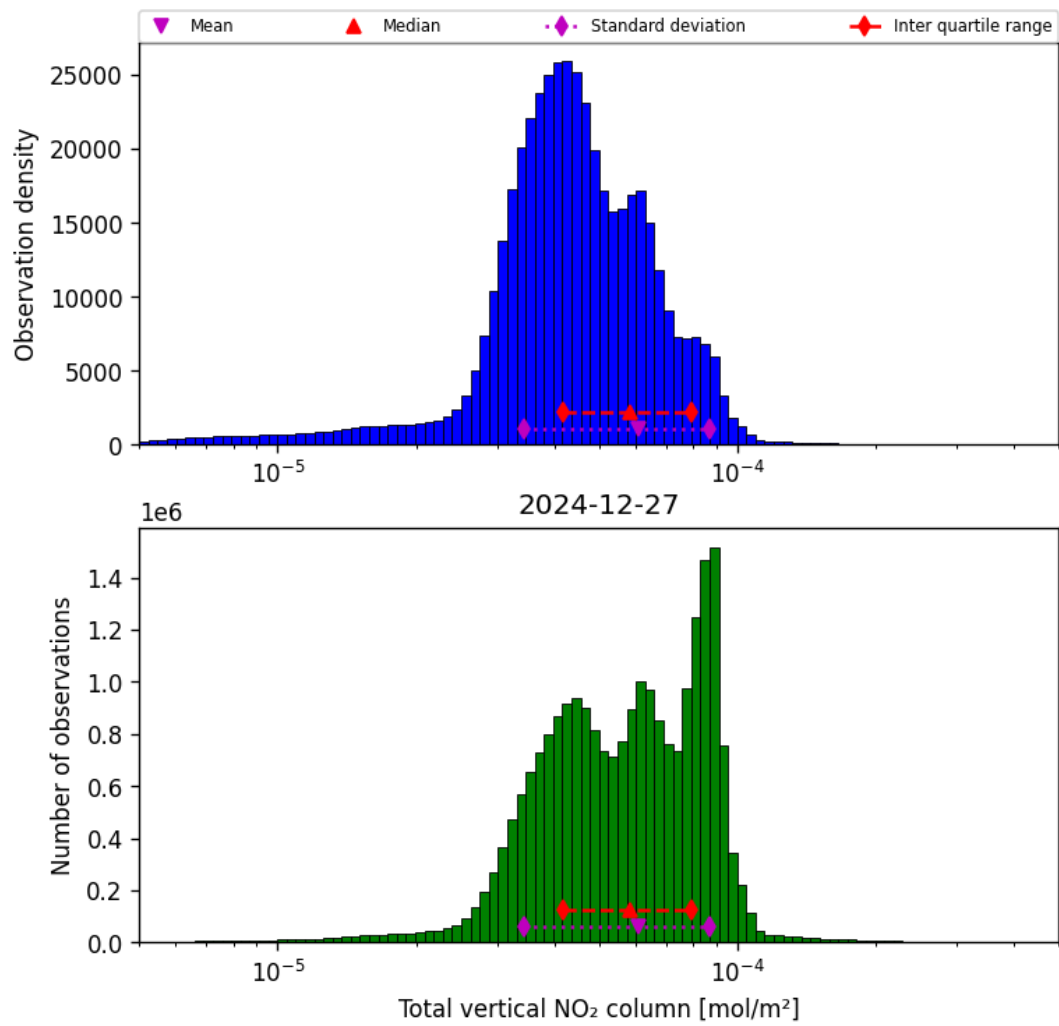
Figure 36: Histogram of “Total vertical NO 2 column” for 2024-12-27 to 2024-12-28
