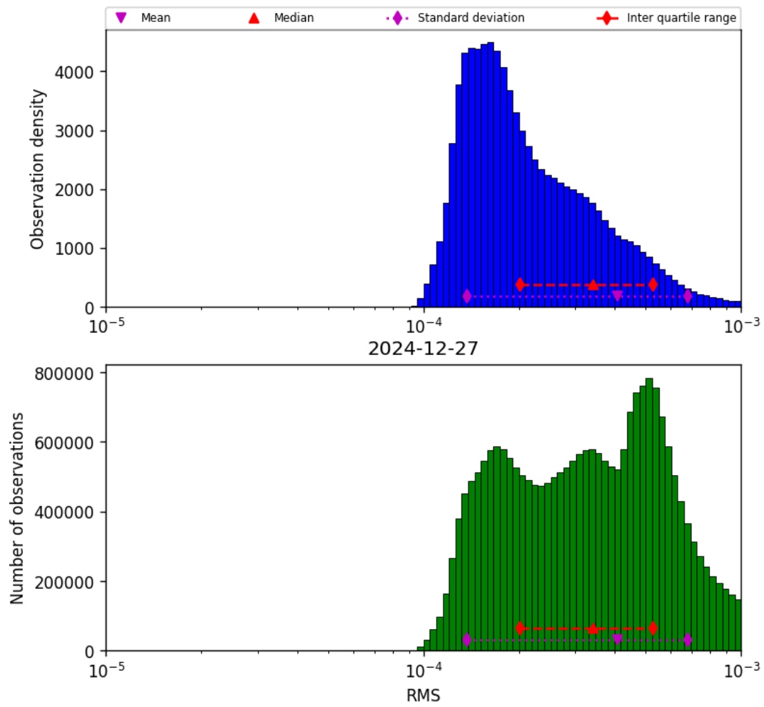
Figure 41: Histogram of “RMS” for 2024-12-27 to 2024-12-28
