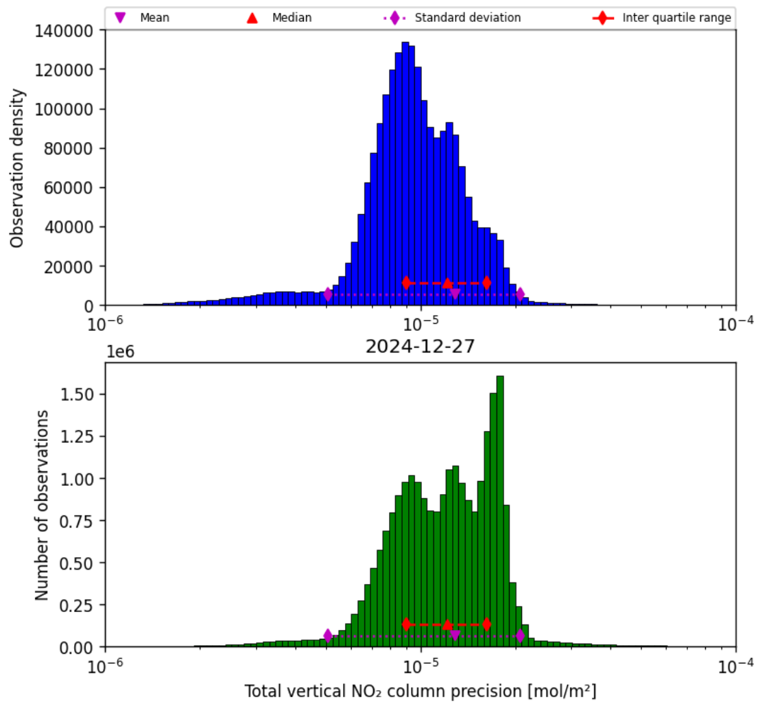
Figure 37: Histogram of “Total vertical NO 2 column precision” for 2024-12-27 to 2024-12-28
