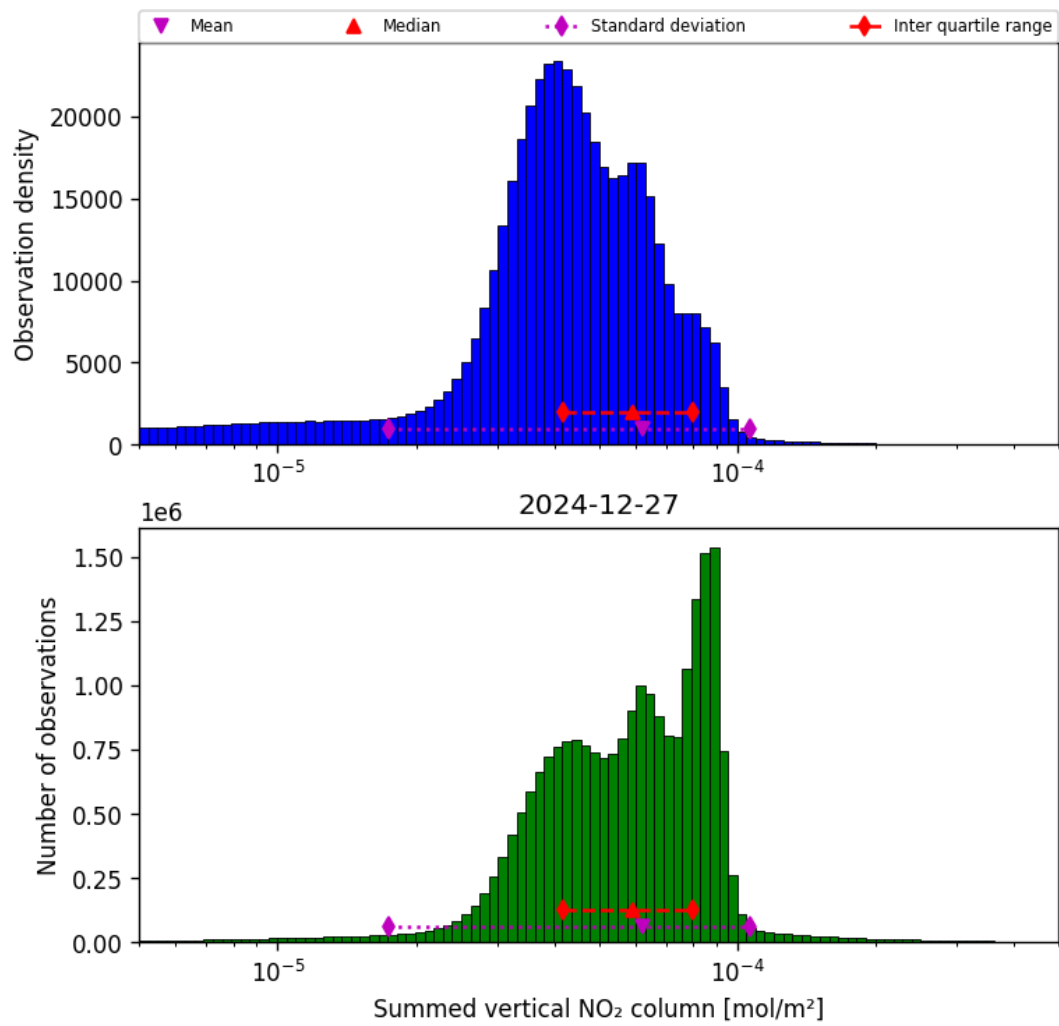
Figure 38: Histogram of “Summed vertical NO 2 column” for 2024-12-27 to 2024-12-28
