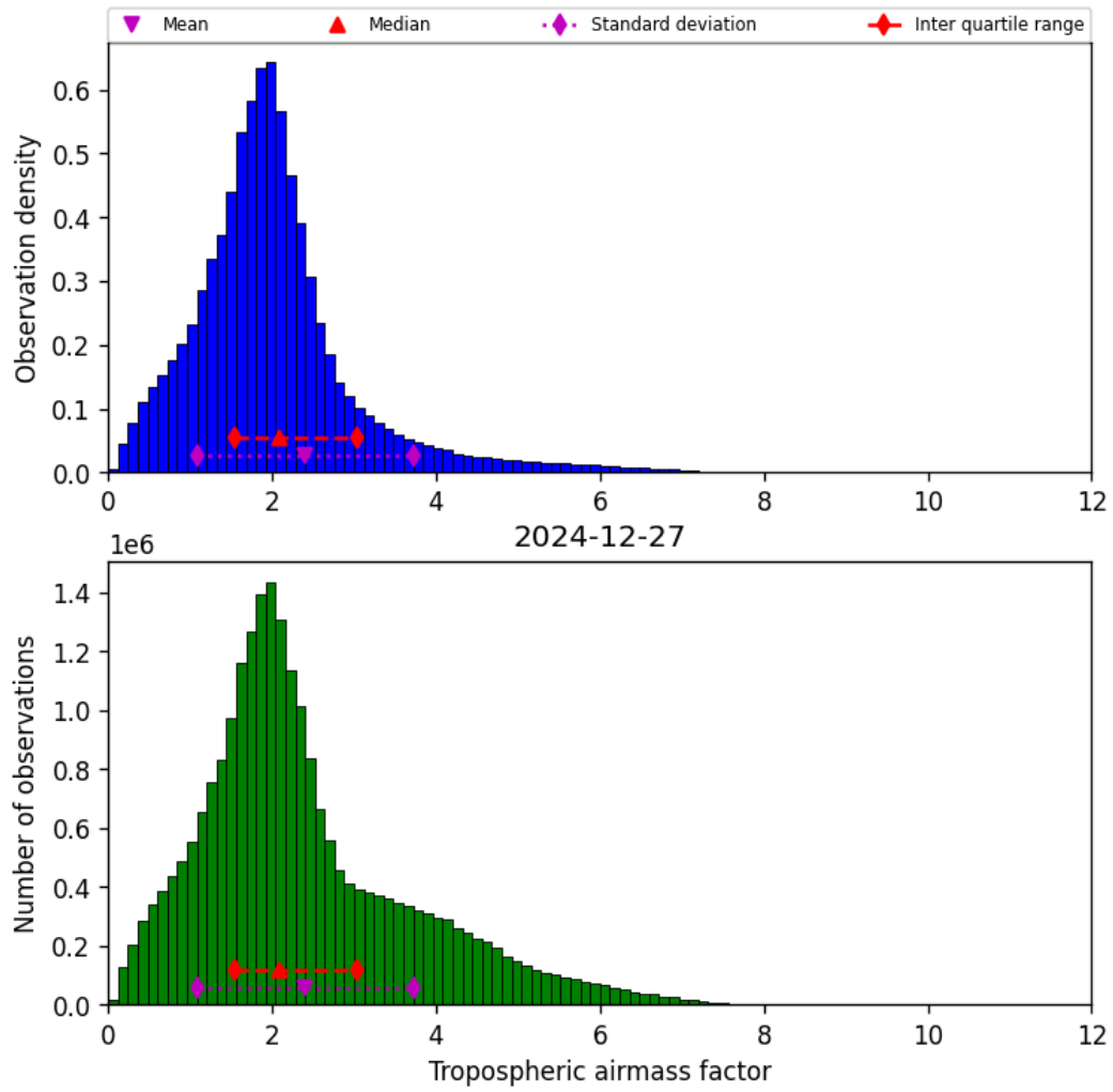
Figure 29: Histogram of “Tropospheric airmass factor” for 2024-12-27 to 2024-12-28
