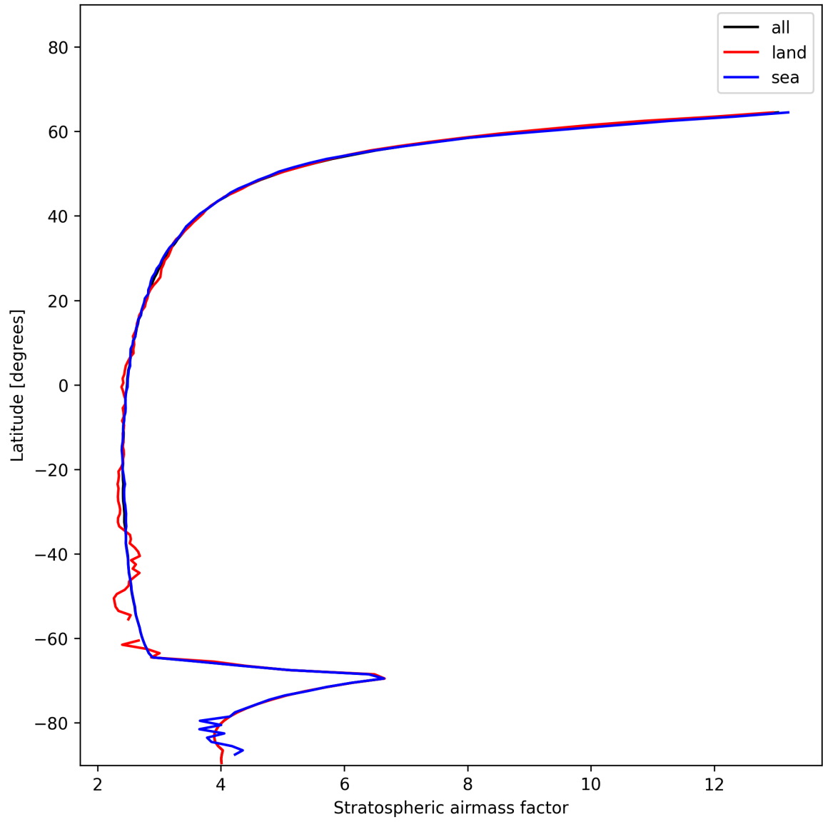
Figure 25: Zonal average of “Stratospheric air mass factor” for 2024-12-27 to 2024-12-28.
