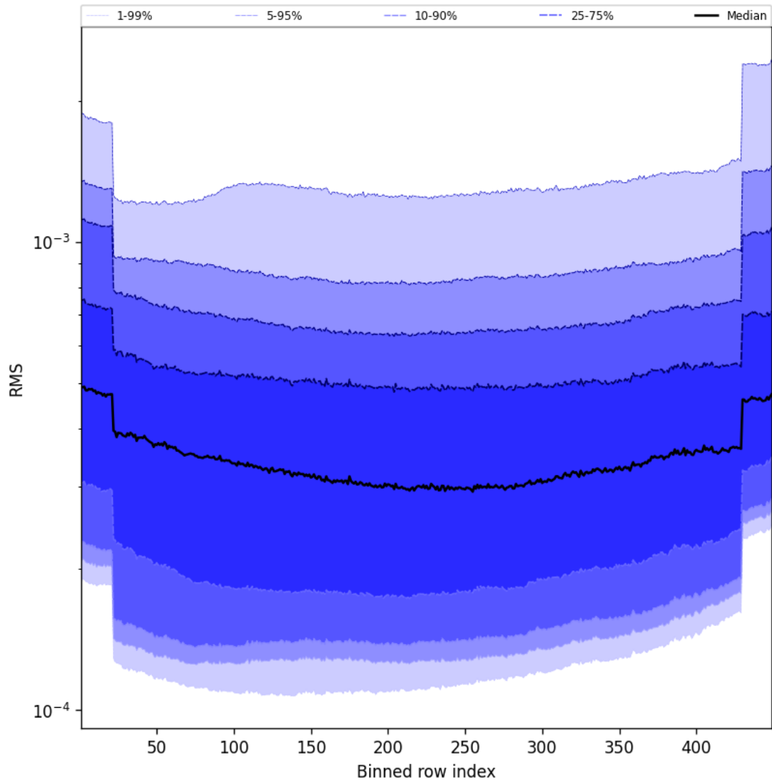
Figure 58: Along track statistics of “RMS” for 2024-12-27 to 2024-12-28
