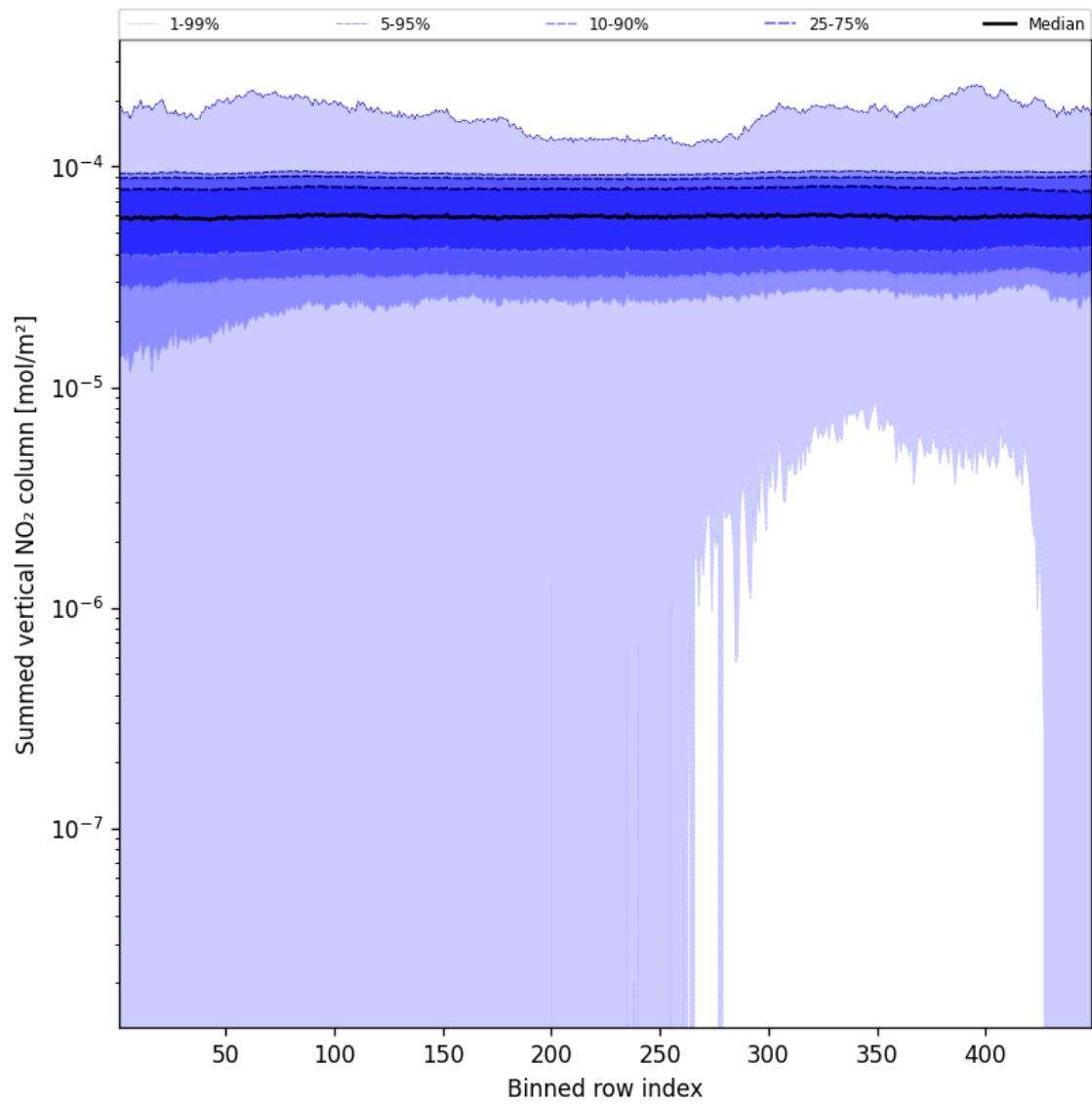
Figure 55: Along track statistics of “Summed vertical NO 2 column” for 2024-12-27 to 2024-12-28
