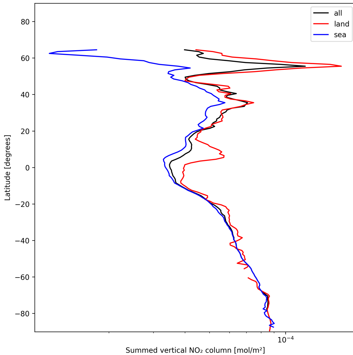
Figure 21: Zonal average of “Summed vertical NO 2 column” for 2024-12-27 to 2024-12-28.
