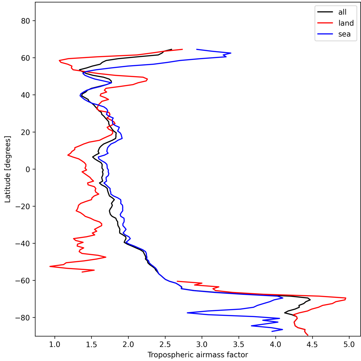
Figure 12: Zonal average of “Tropospheric airmass factor” for 2024-12-27 to 2024-12-28.
