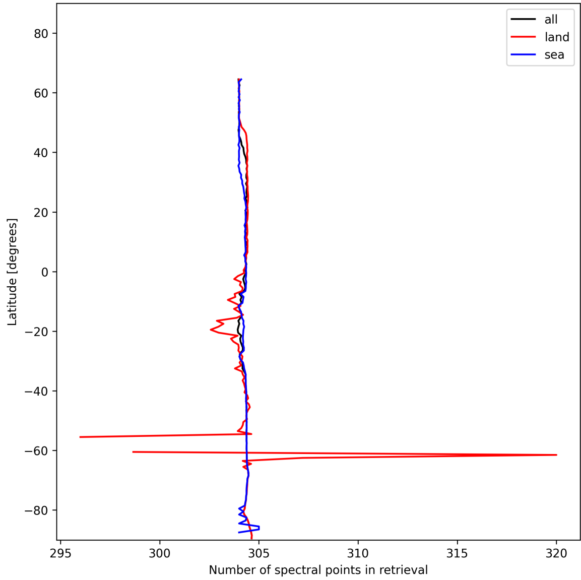
Figure 14: Zonal average of “Number of spectral points in retrieval” for 2024-12-27 to 2024-12-28.
