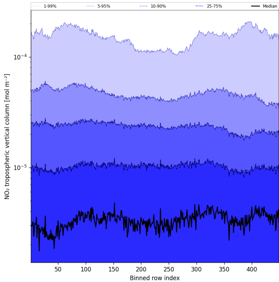
Figure 44: Along track statistics of “NO 2 tropospheric vertical column” for 2024-12-27 to 2024-12-28
