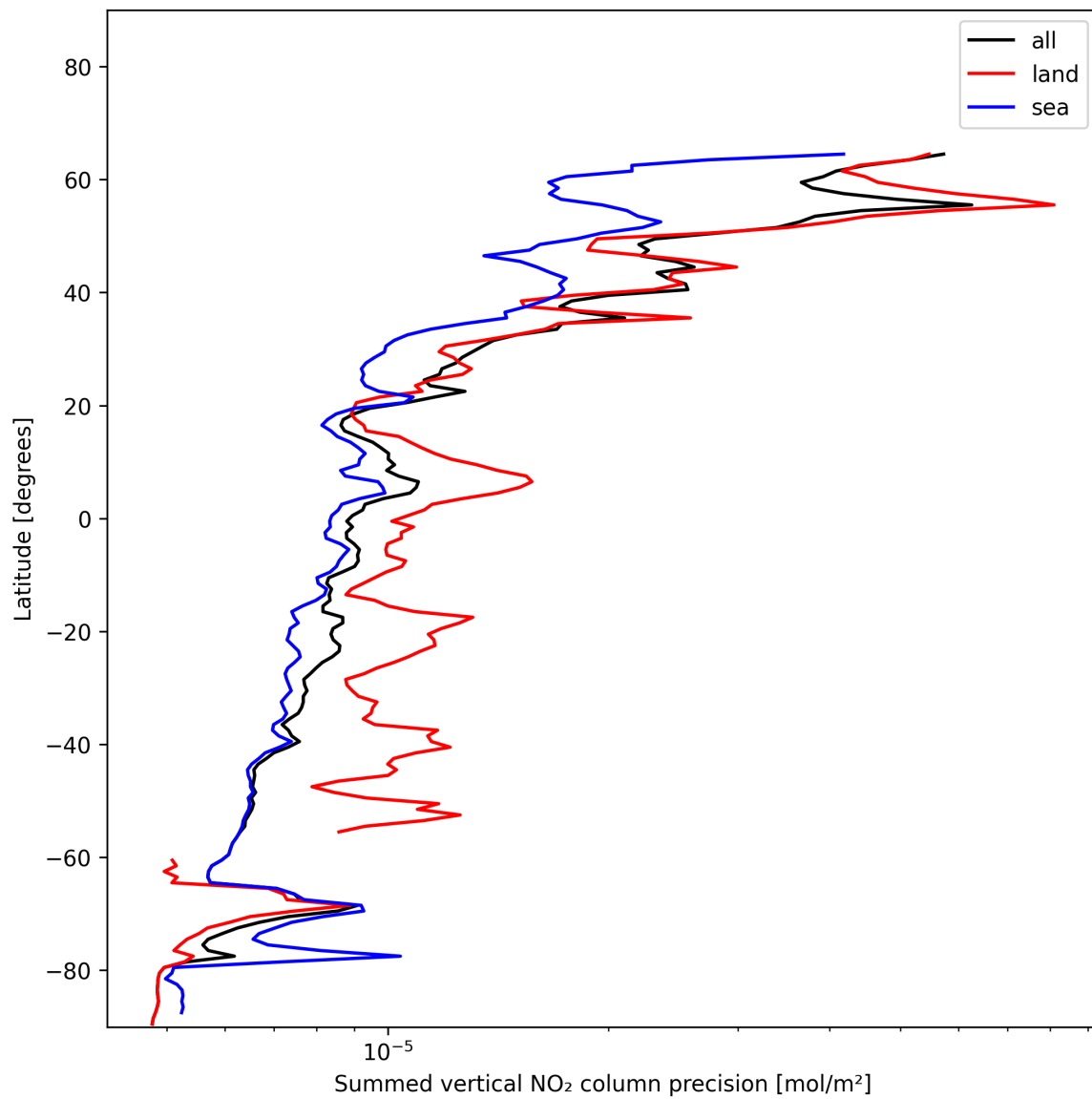
Figure 22: Zonal average of “Summed vertical NO 2 column precision” for 2024-12-27 to 2024-12-28.
