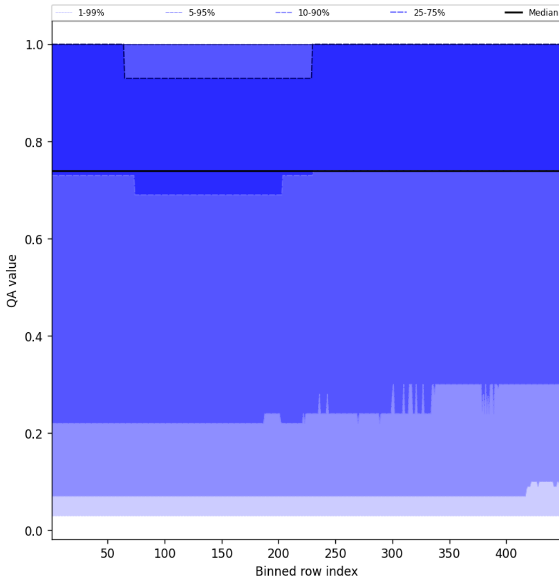
Figure 43: Along track statistics of “QA value” for 2024-12-27 to 2024-12-28
