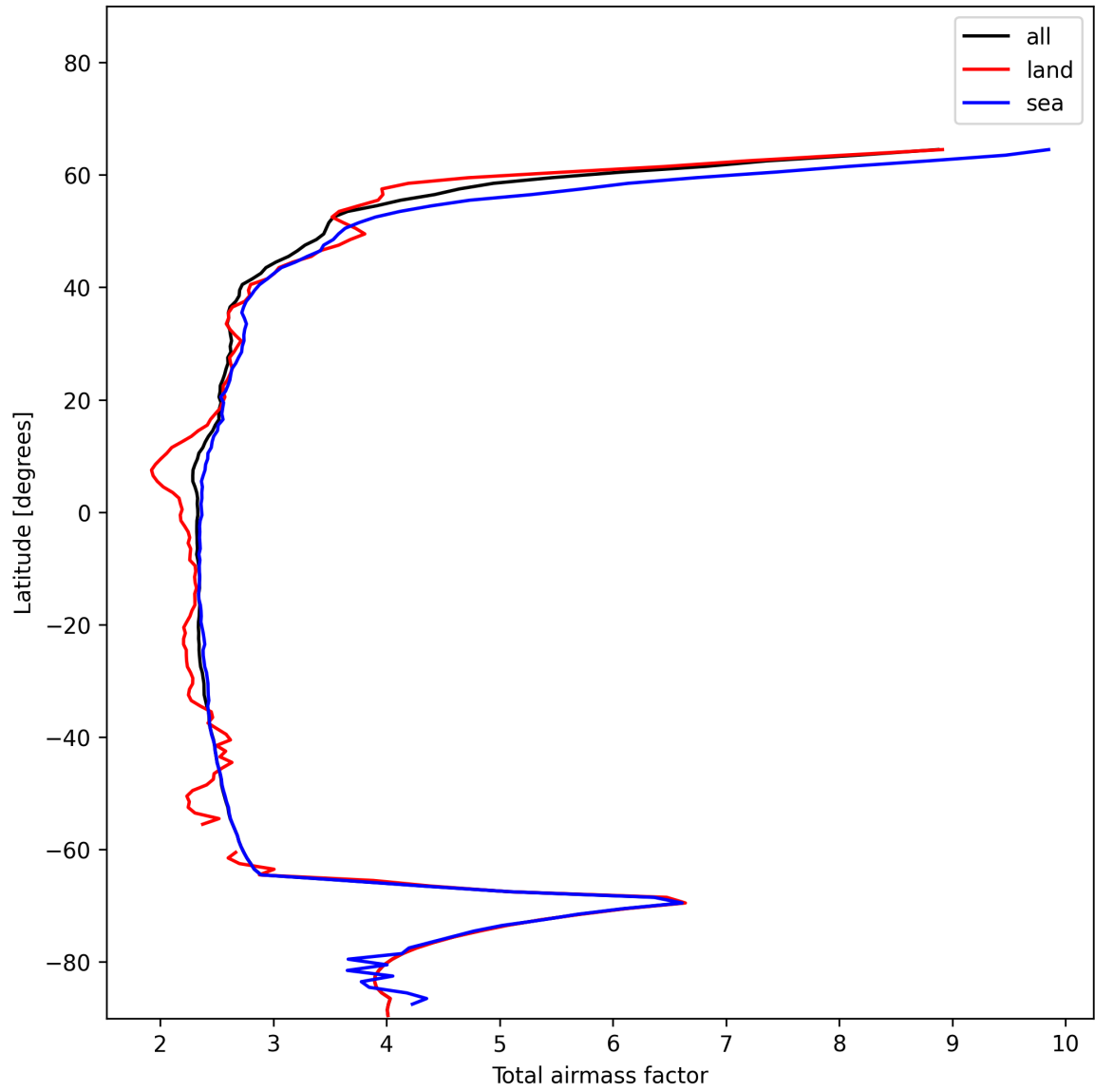
Figure 13: Zonal average of “Total airmass factor” for 2024-12-27 to 2024-12-28.
