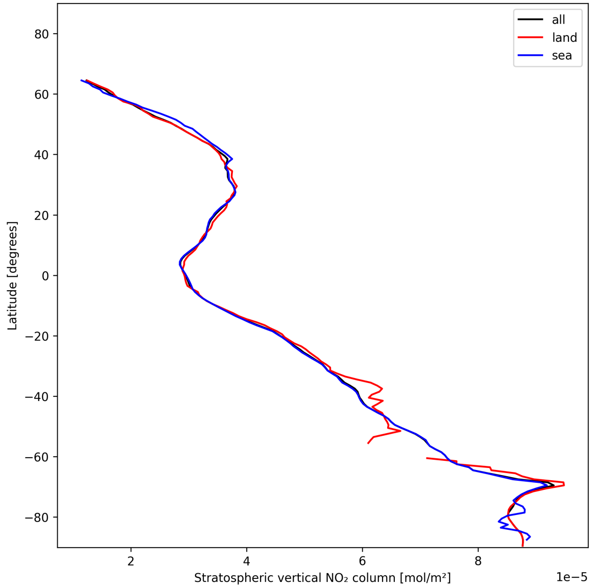
Figure 17: Zonal average of “Stratospheric vertical NO 2 column” for 2024-12-27 to 2024-12-28.
