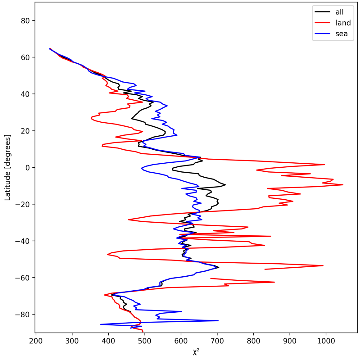
Figure 23: Zonal average of “ \chi^2 ” for 2024-12-27 to 2024-12-28.
