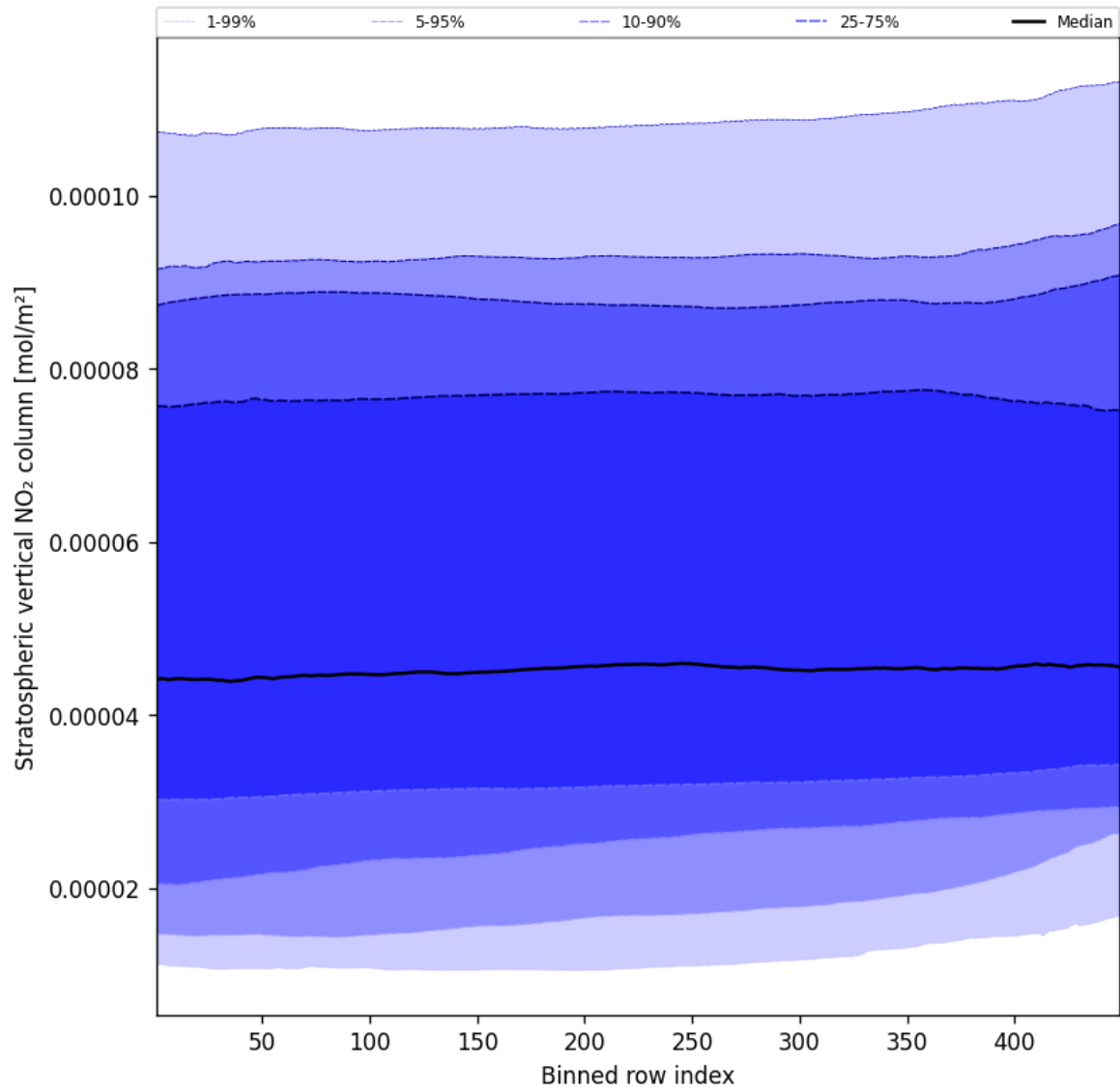
Figure 51: Along track statistics of “Stratospheric vertical NO 2 column” for 2024-12-27 to 2024-12-28
