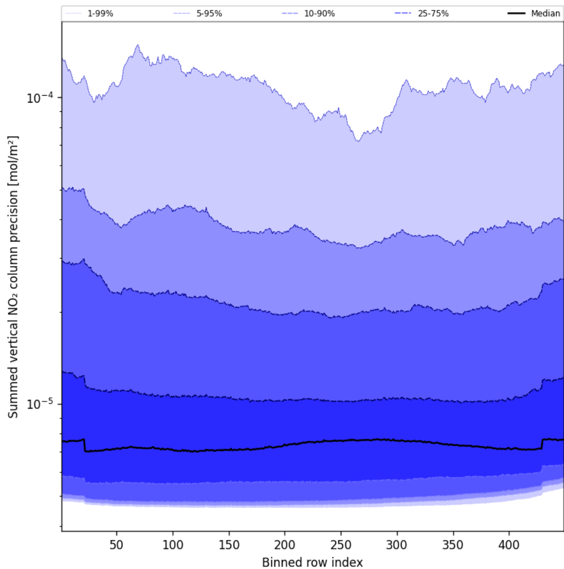
Figure 56: Along track statistics of “Summed vertical NO 2 column precision” for 2024-12-27 to 2024-12-28
