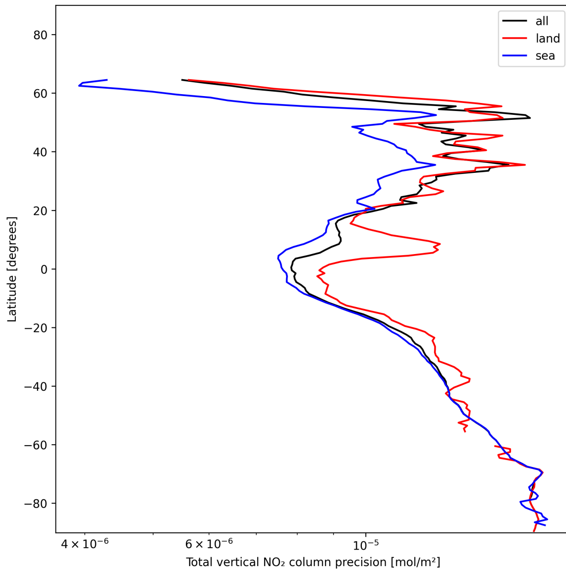
Figure 20: Zonal average of “Total vertical NO 2 column precision” for 2024-12-27 to 2024-12-28.
