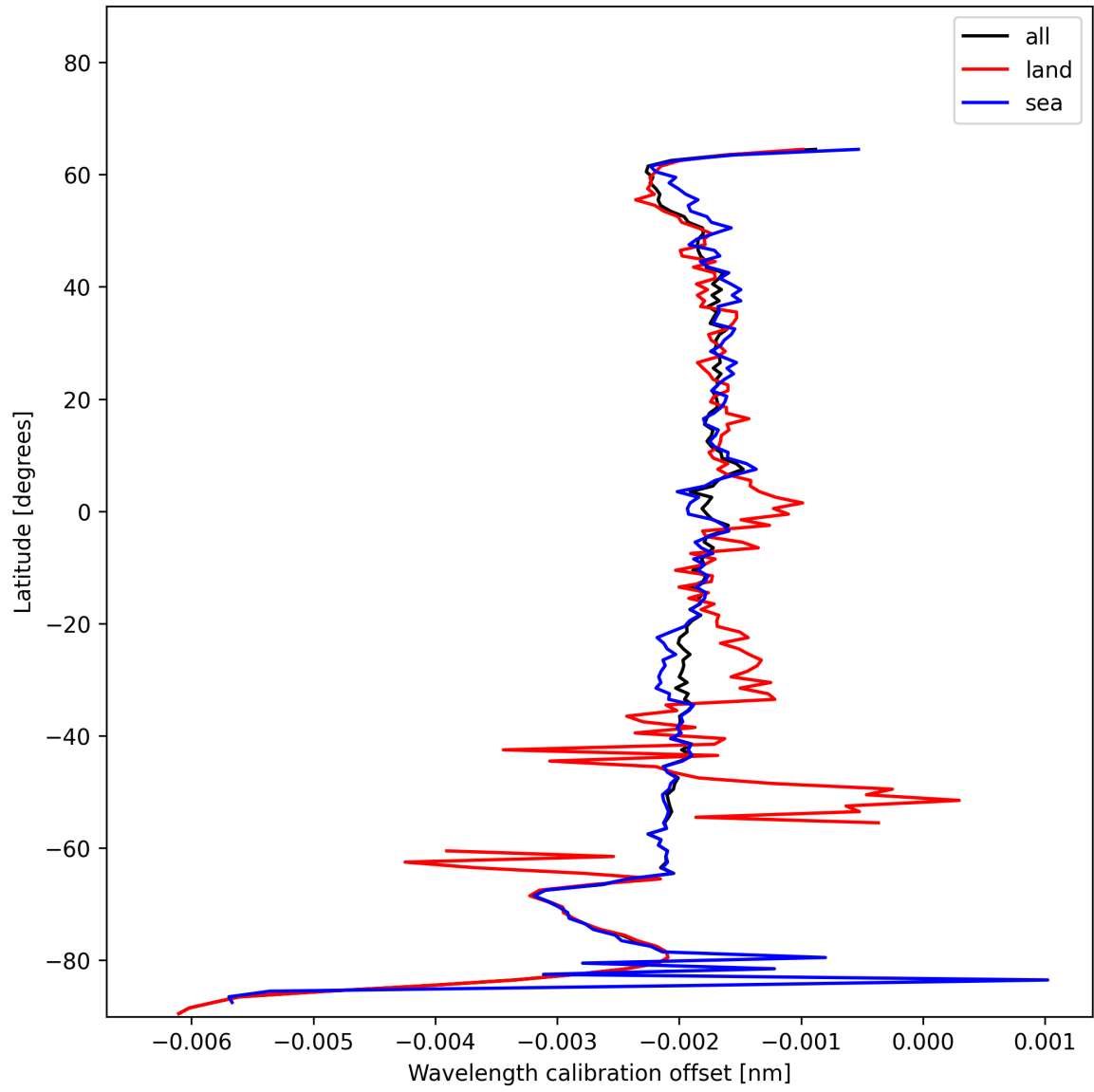
Figure 16: Zonal average of “Wavelength calibration offset” for 2024-12-27 to 2024-12-28.
