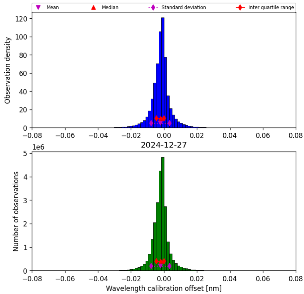
Figure 33: Histogram of “Wavelength calibration offset” for 2024-12-27 to 2024-12-28
