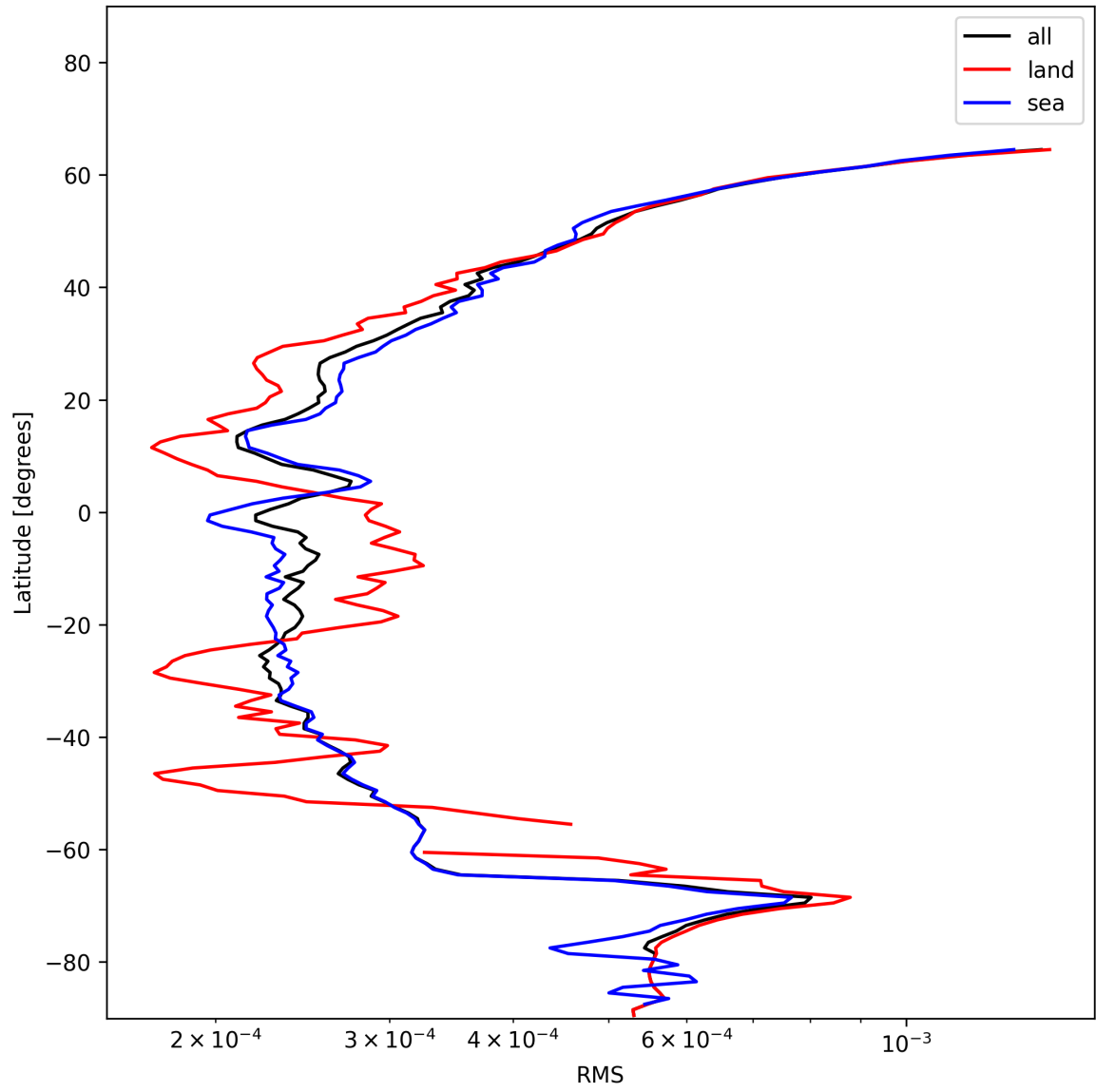
Figure 24: Zonal average of “RMS” for 2024-12-27 to 2024-12-28.
