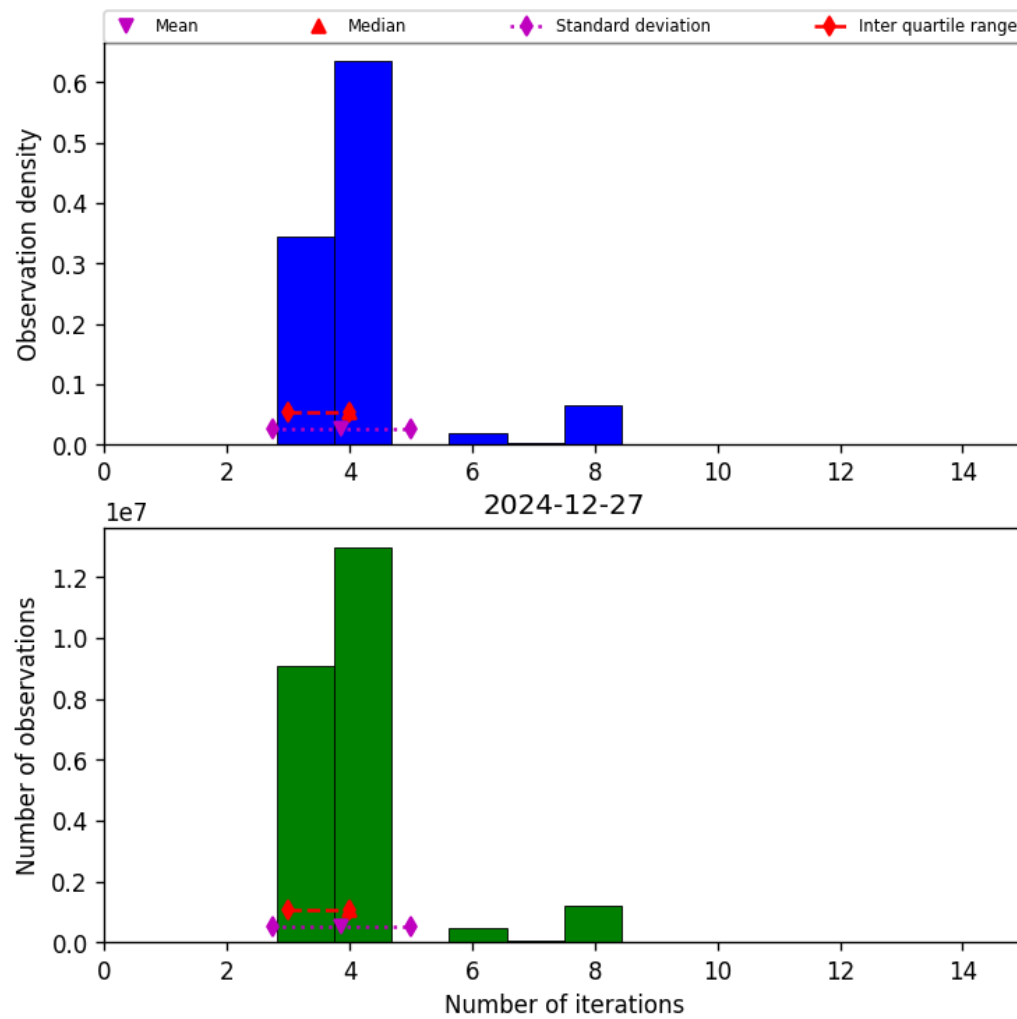
Figure 32: Histogram of “Number of iterations” for 2024-12-27 to 2024-12-28
