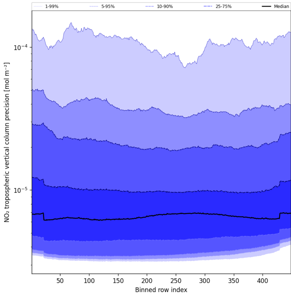
Figure 45: Along track statistics of “NO 2 tropospheric vertical column precision” for 2024-12-27 to 2024-12-28
