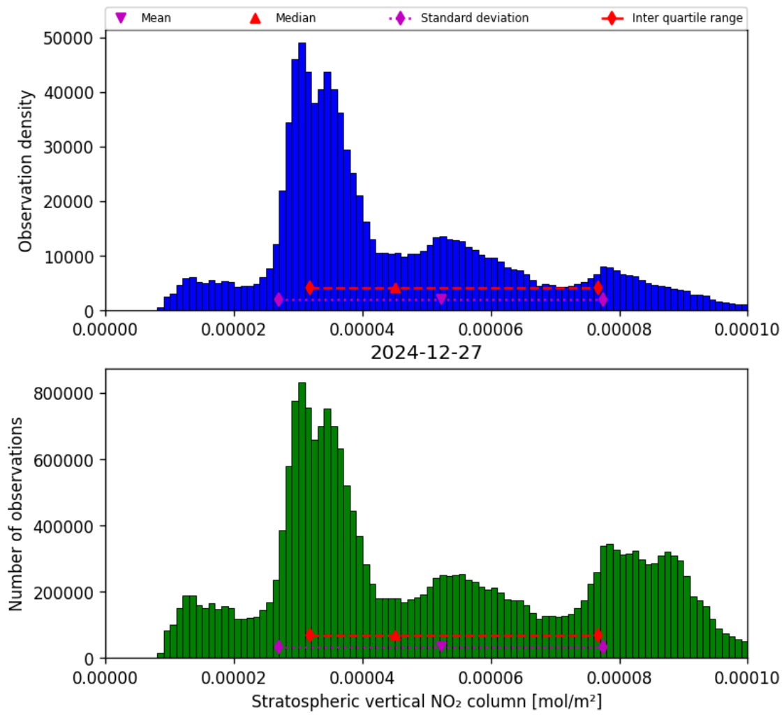
Figure 34: Histogram of “Stratospheric vertical NO 2 column” for 2024-12-27 to 2024-12-28
