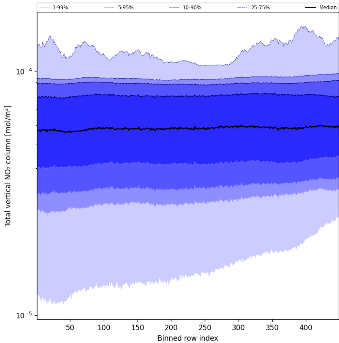
Figure 53: Along track statistics of “Total vertical NO 2 column” for 2024-12-27 to 2024-12-28
