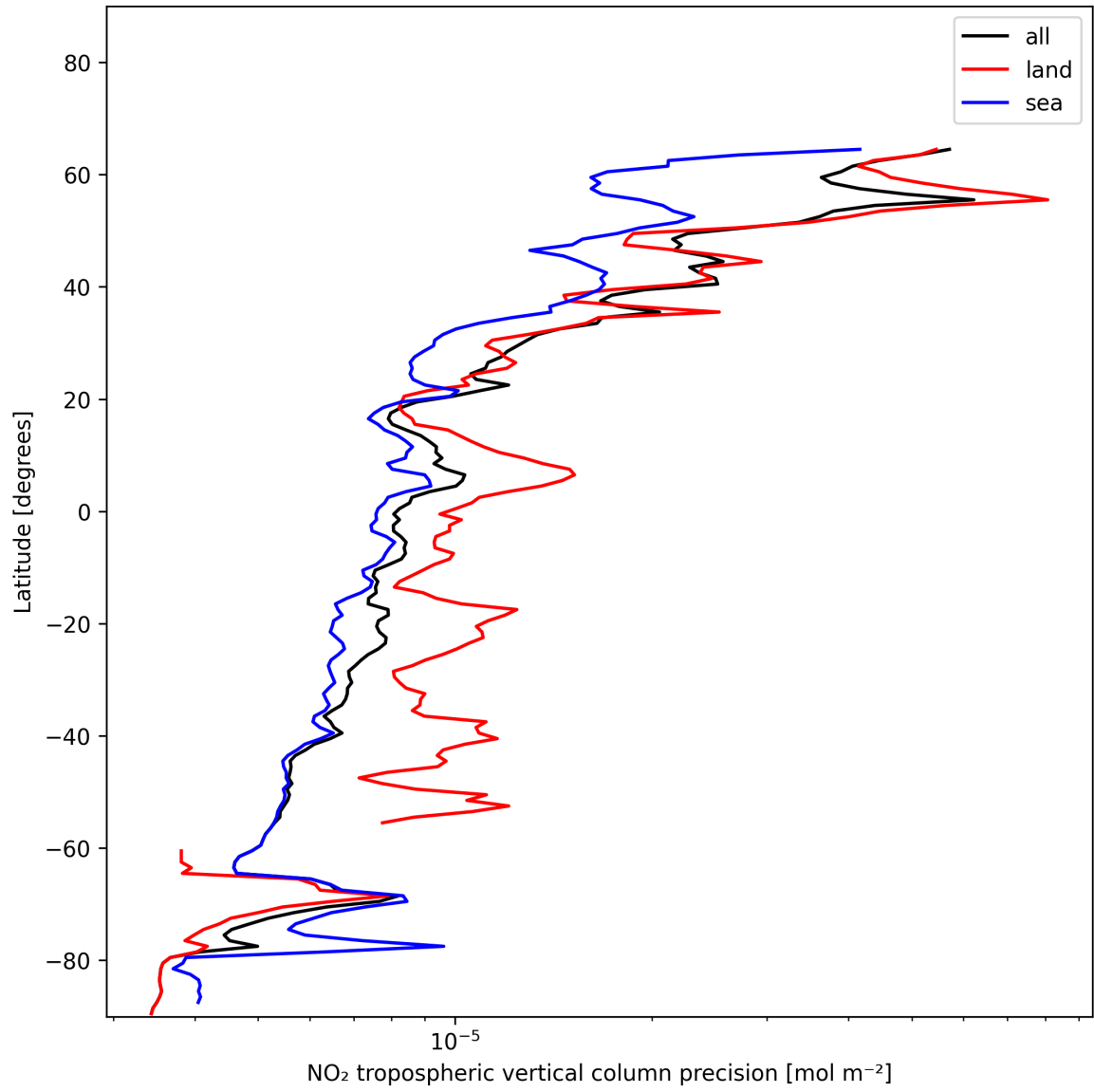
Figure 11: Zonal average of “NO 2 tropospheric vertical column precision” for 2024-12-27 to 2024-12-28.
