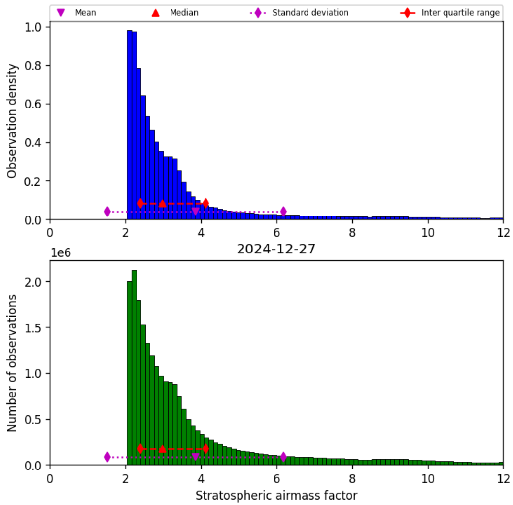
Figure 42: Histogram of “Stratospheric airmass factor” for 2024-12-27 to 2024-12-28
