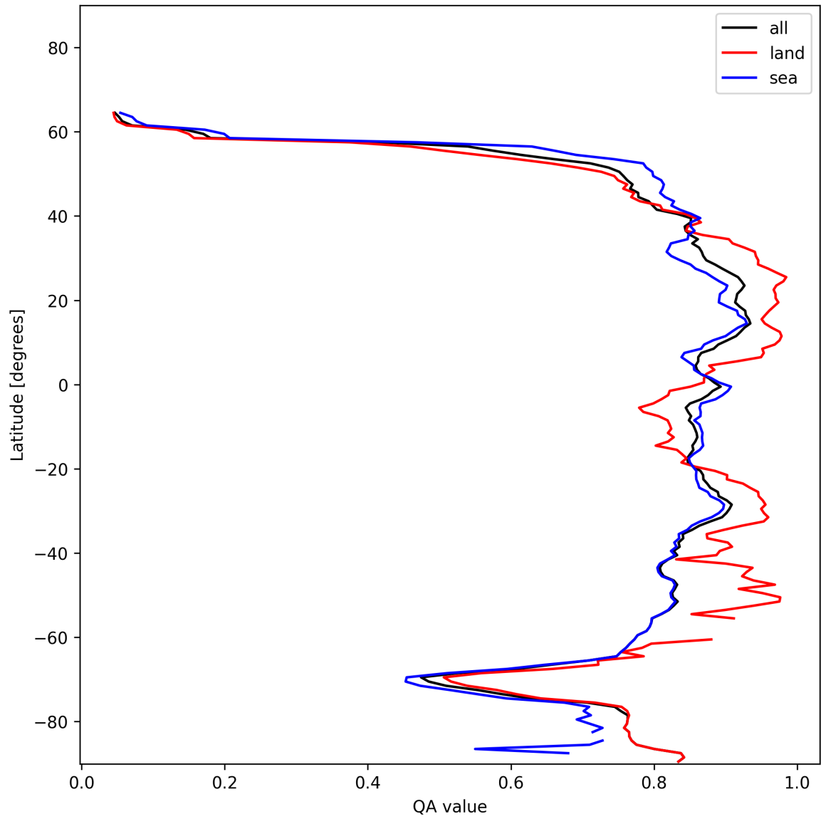
Figure 9: Zonal average of “QA value” for 2024-12-29 to 2024-12-30.
