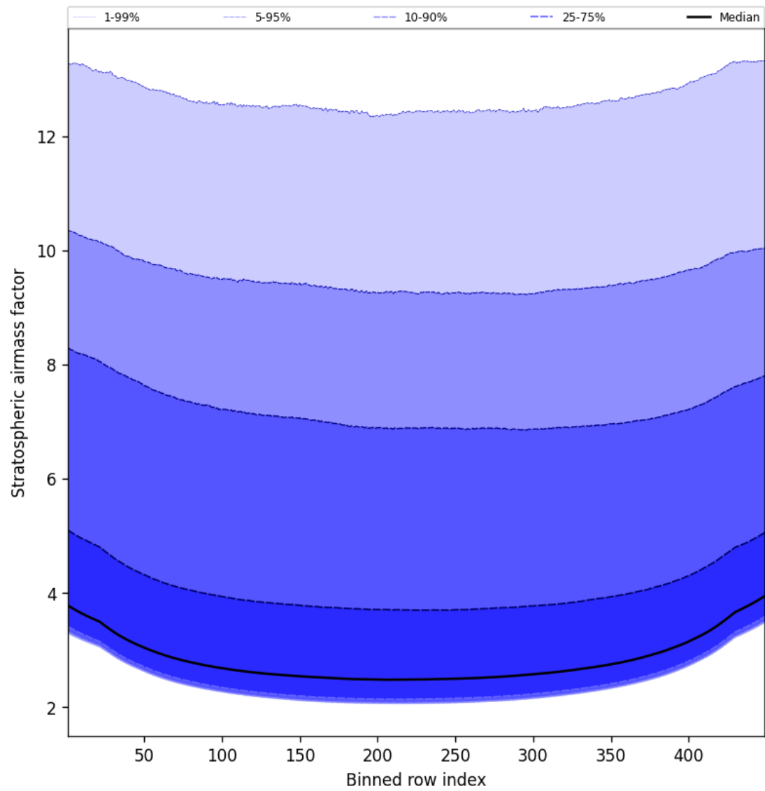
Figure 59: Along track statistics of “Stratospheric airmass factor” for 2024-12-29 to 2024-12-30
