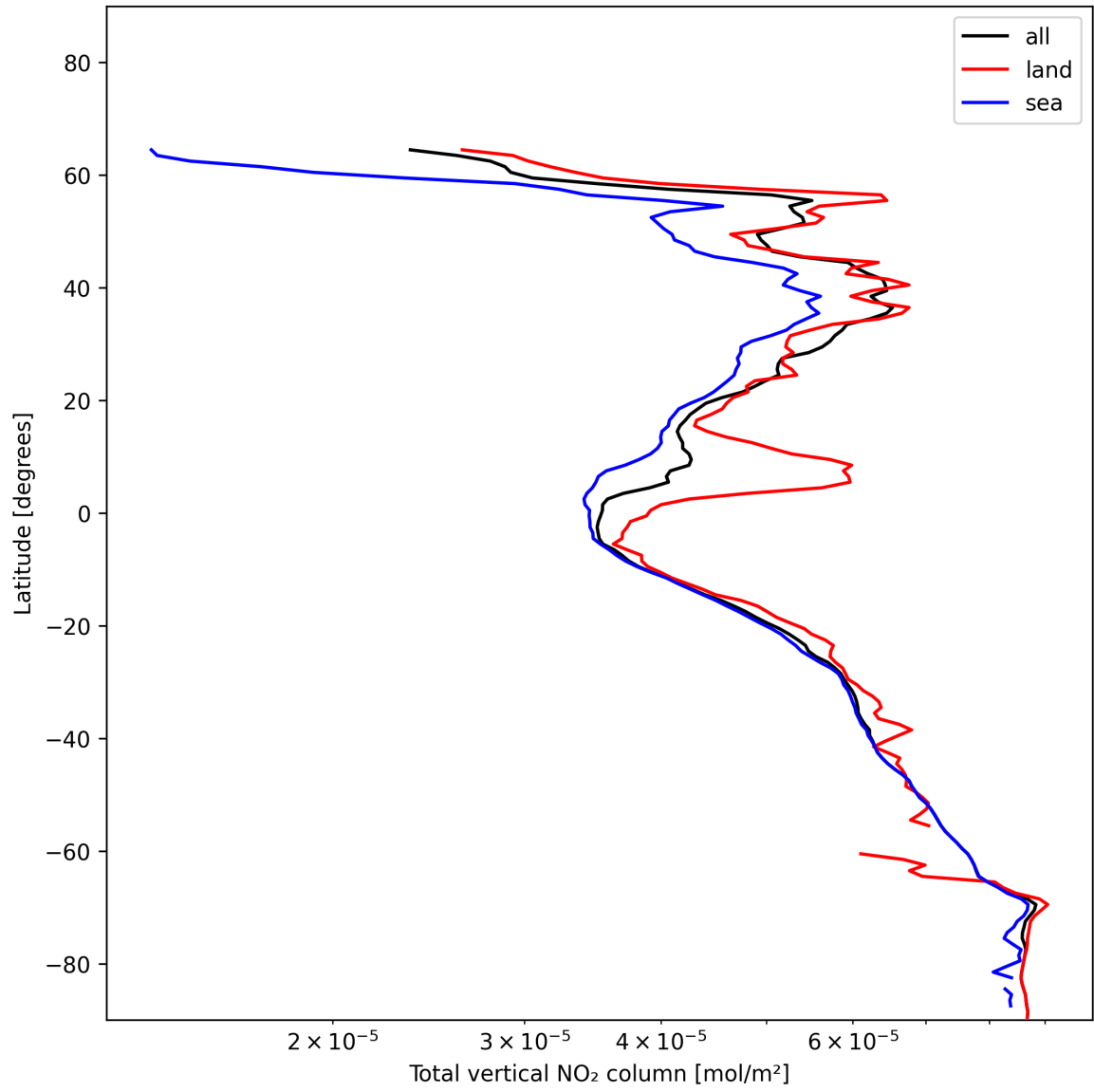
Figure 19: Zonal average of “Total vertical NO 2 column” for 2024-12-29 to 2024-12-30.
