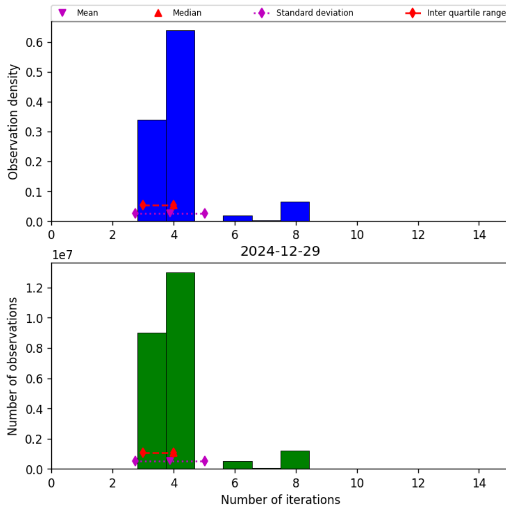
Figure 32: Histogram of “Number of iterations” for 2024-12-29 to 2024-12-30
