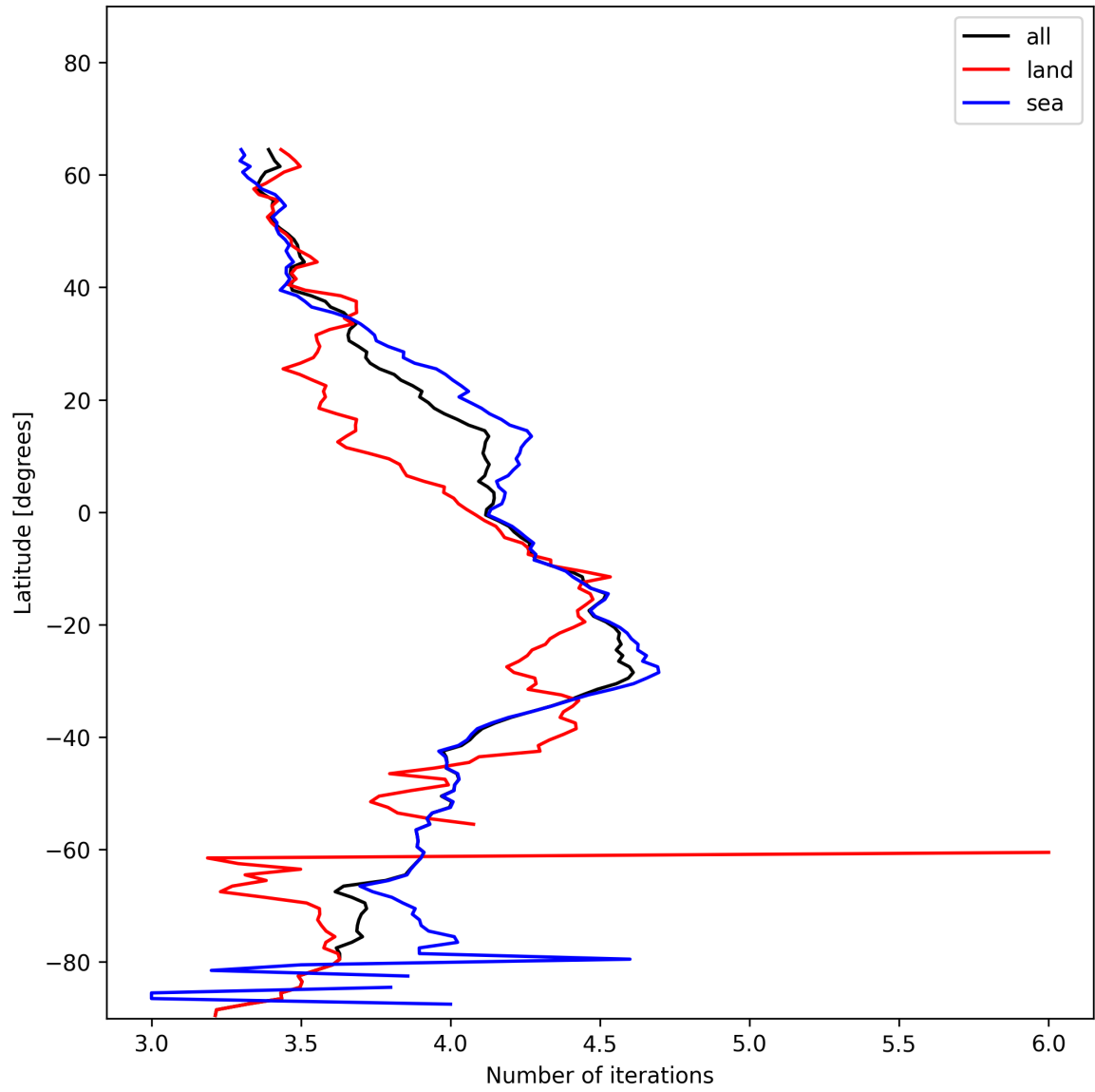
Figure 15: Zonal average of “Number of iterations” for 2024-12-29 to 2024-12-30.
