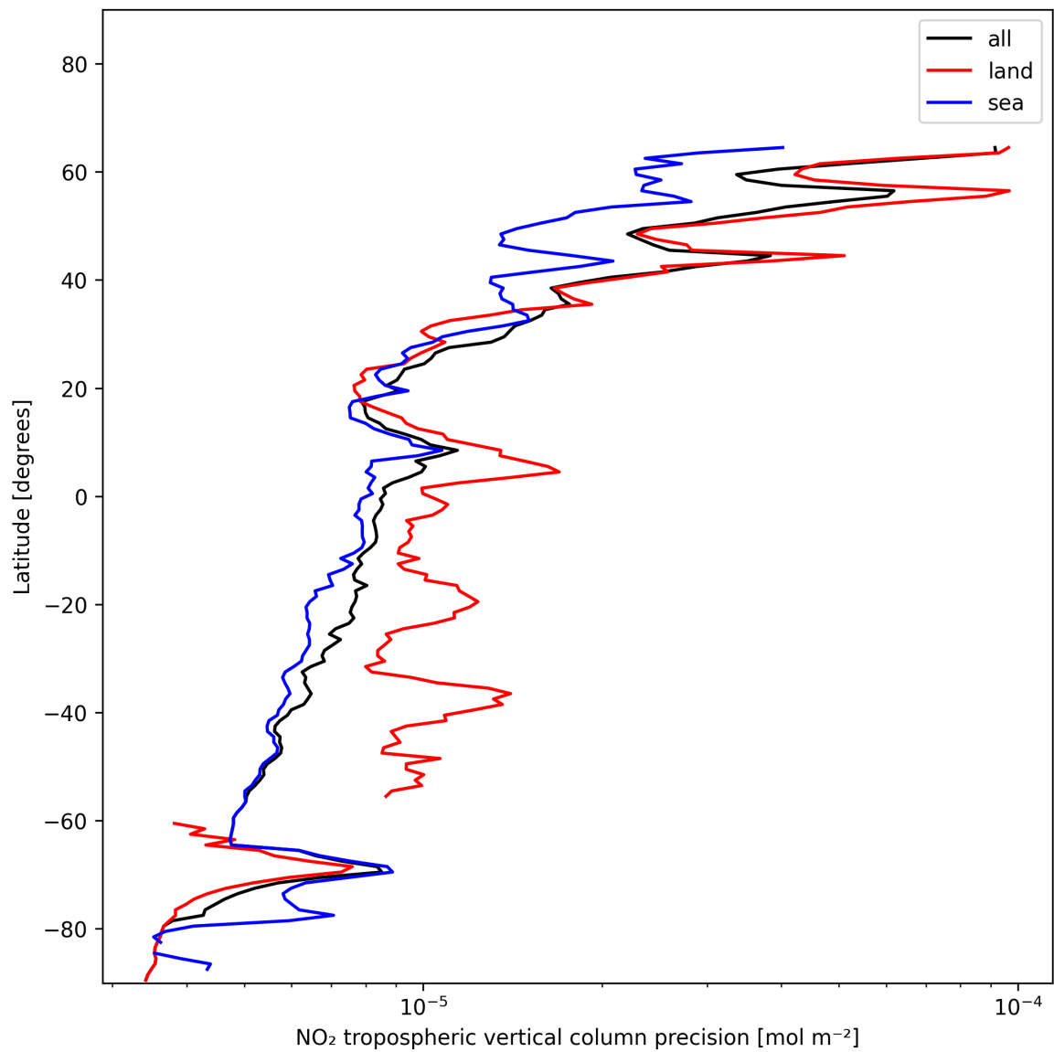
Figure 11: Zonal average of “NO 2 tropospheric vertical column precision” for 2024-12-29 to 2024-12-30.
