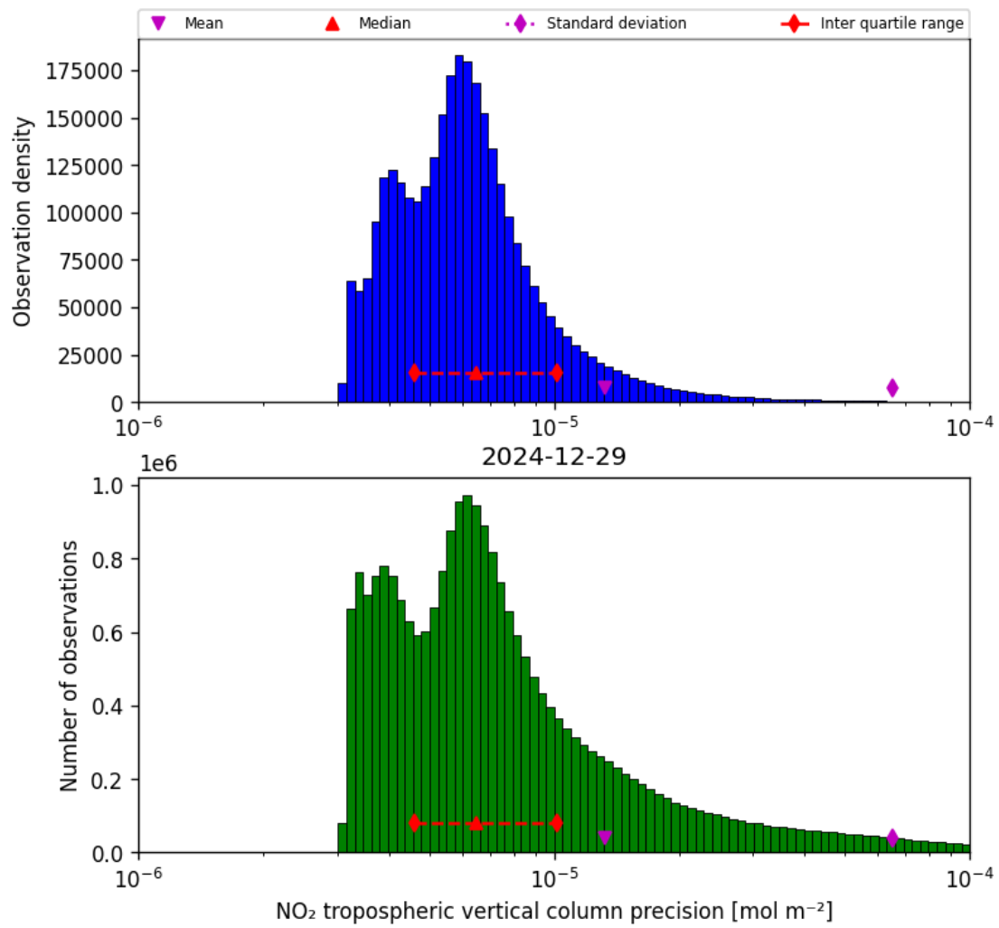
Figure 28: Histogram of “NO 2 tropospheric vertical column precision” for 2024-12-29 to 2024-12-30
