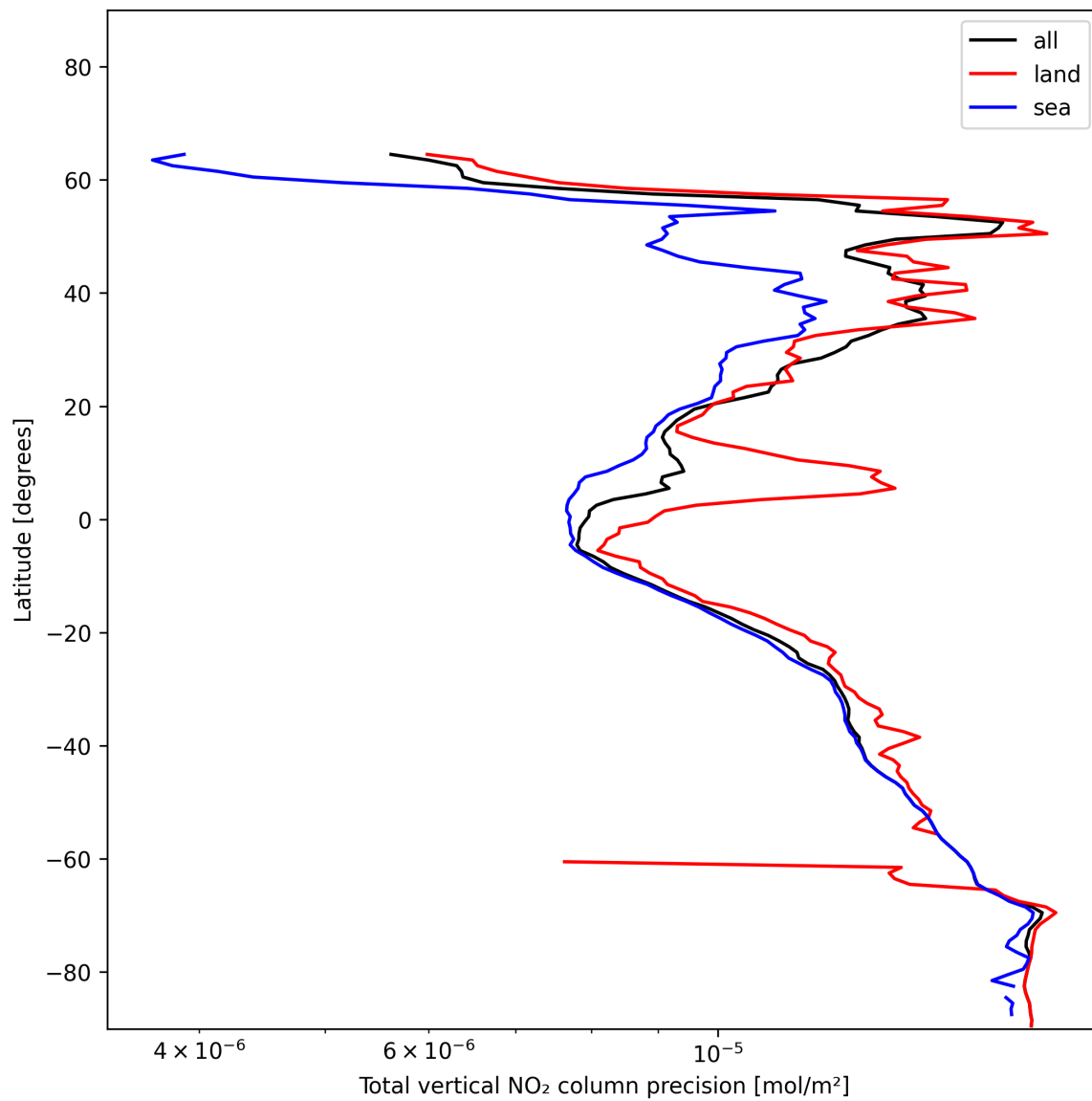
Figure 20: Zonal average of “Total vertical NO 2 column precision” for 2024-12-29 to 2024-12-30.
