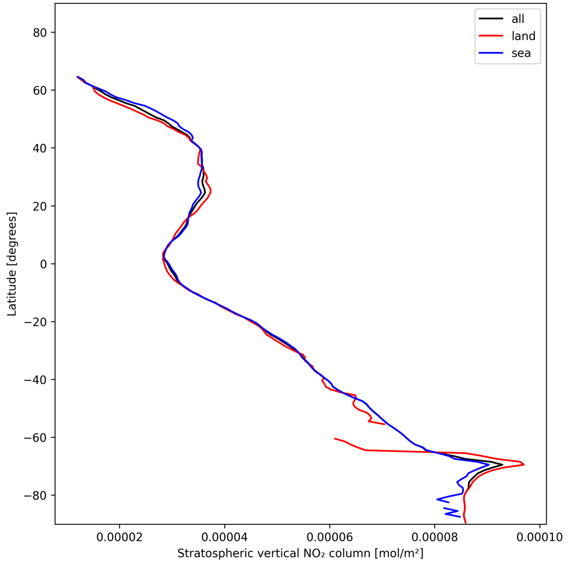
Figure 17: Zonal average of “Stratospheric vertical NO 2 column” for 2024-12-29 to 2024-12-30.
