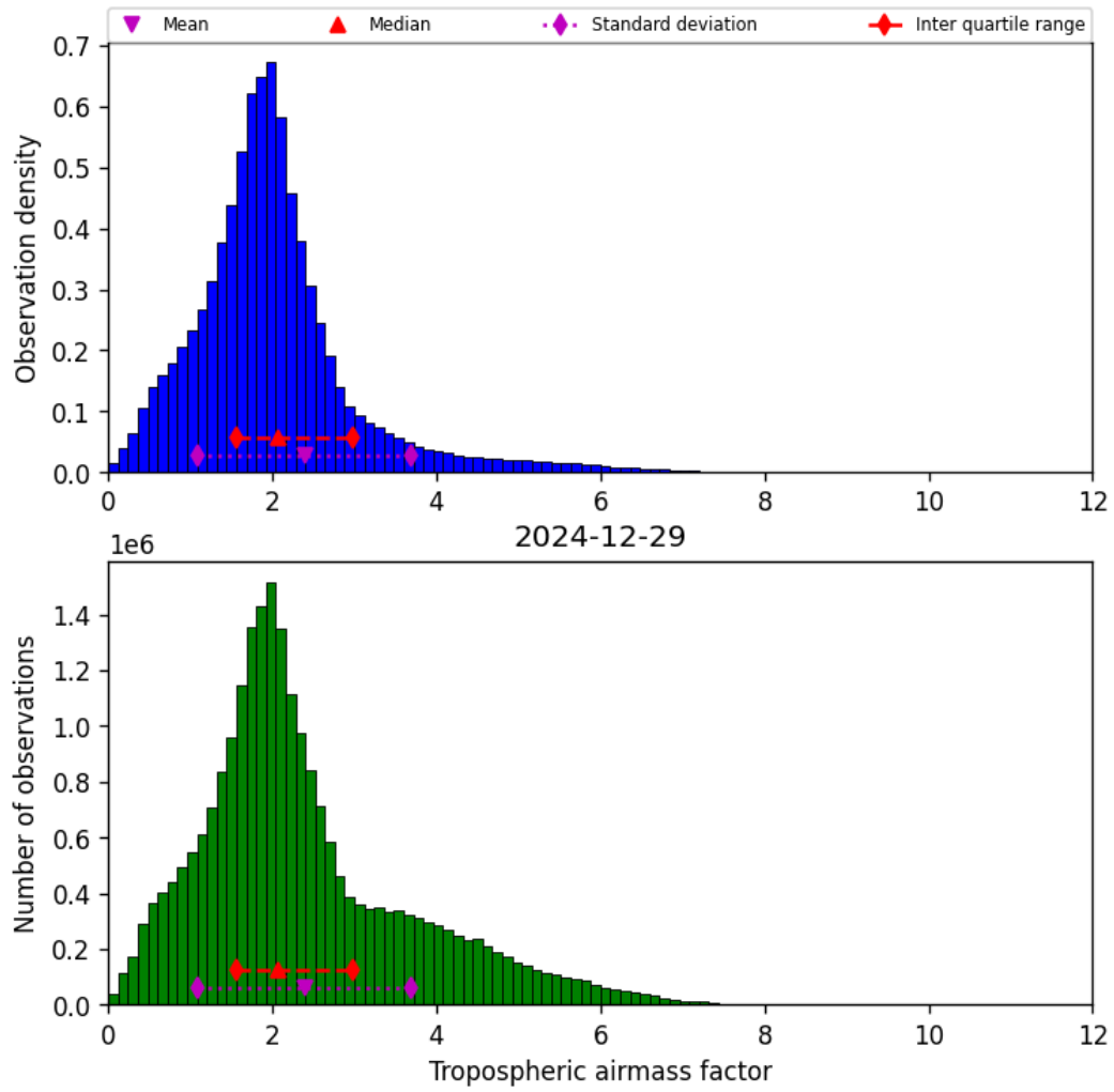
Figure 29: Histogram of “Tropospheric airmass factor” for 2024-12-29 to 2024-12-30
