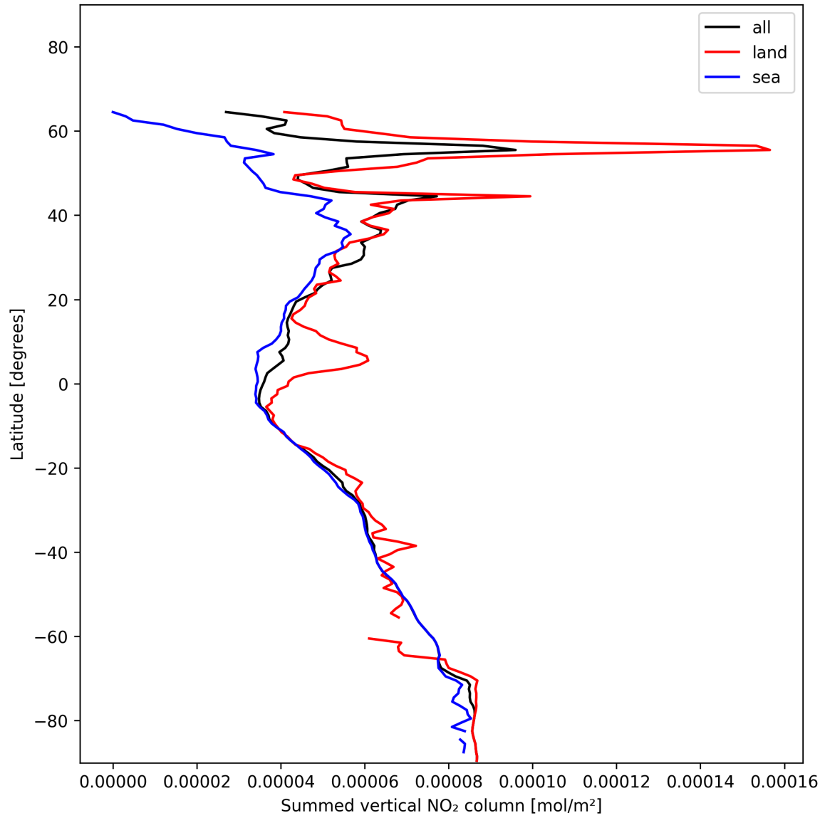
Figure 21: Zonal average of “Summed vertical NO 2 column” for 2024-12-29 to 2024-12-30.
