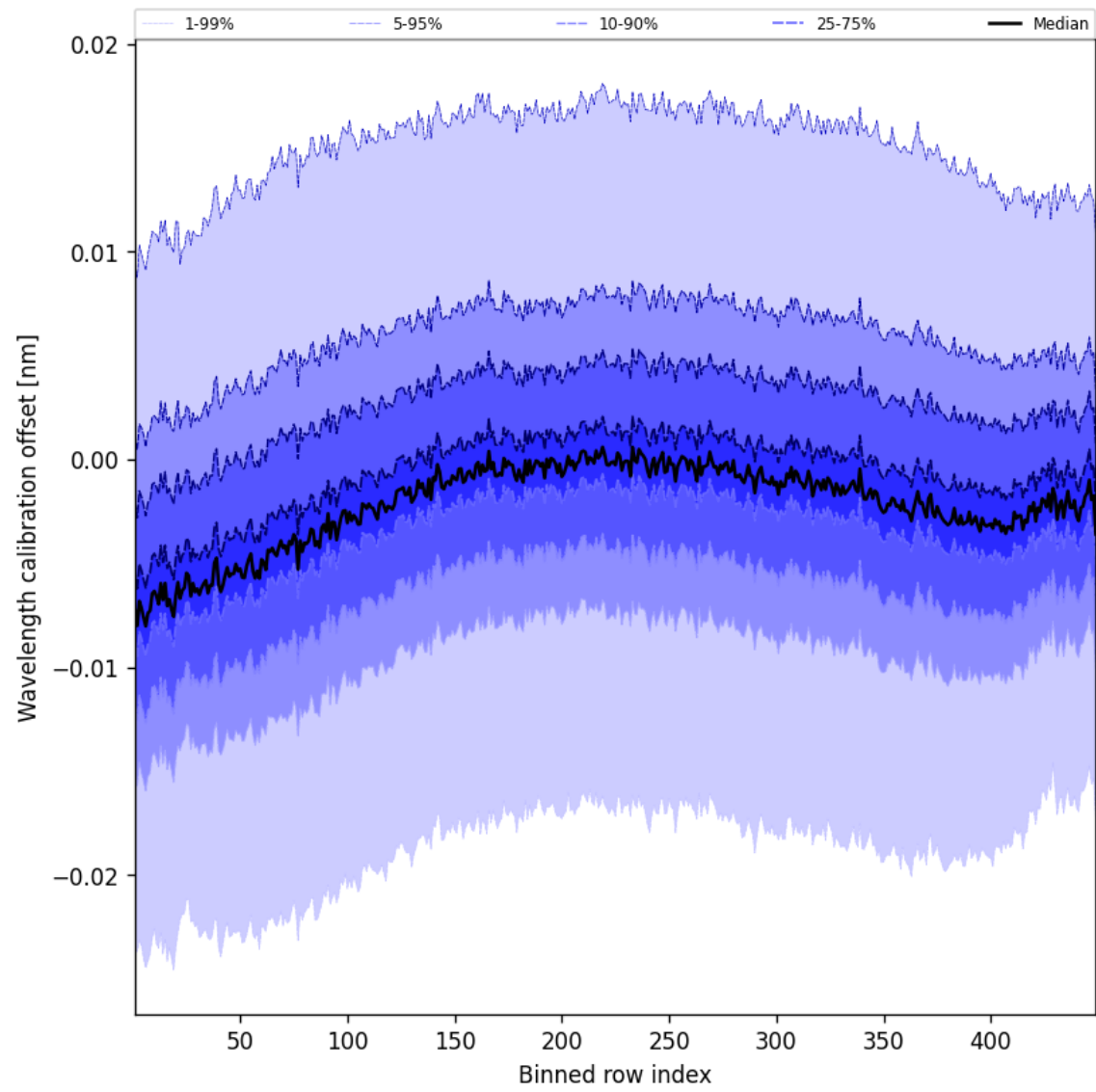
Figure 50: Along track statistics of “Wavelength calibration offset” for 2024-12-29 to 2024-12-30
