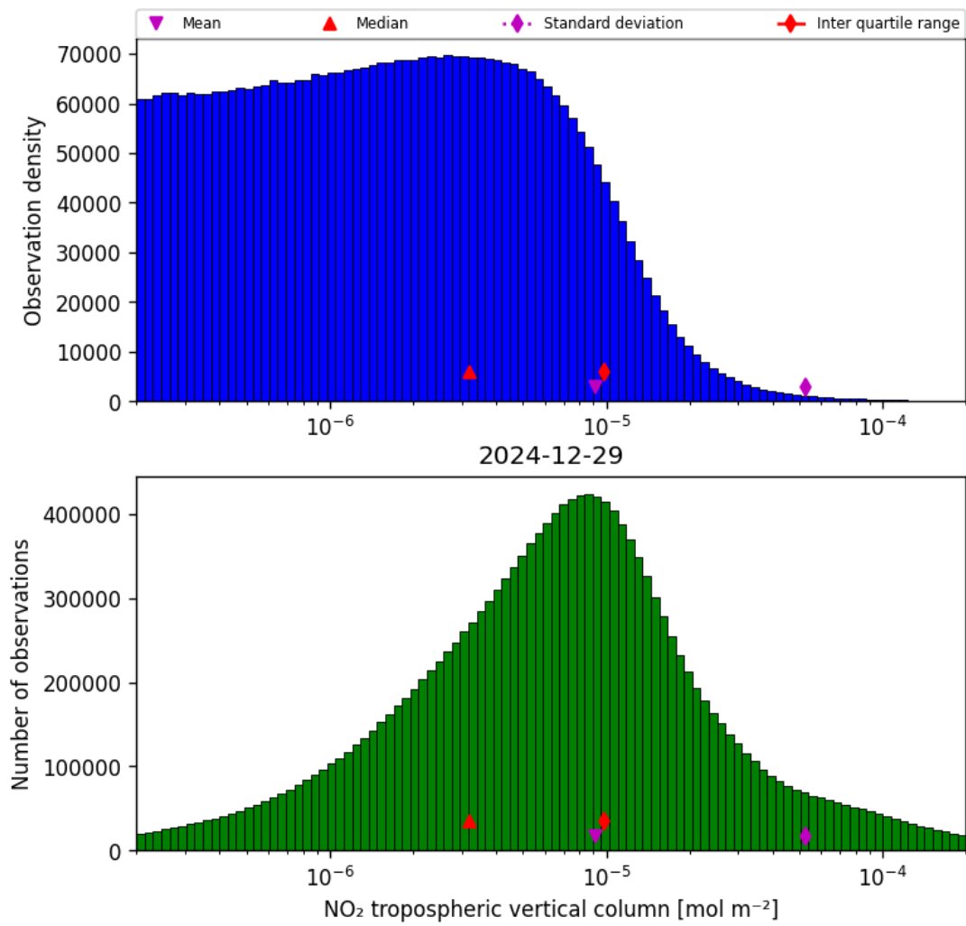
Figure 27: Histogram of “NO 2 tropospheric vertical column” for 2024-12-29 to 2024-12-30
