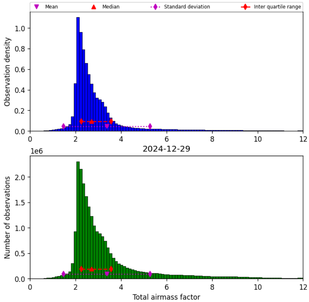
Figure 30: Histogram of “Total airmass factor” for 2024-12-29 to 2024-12-30
