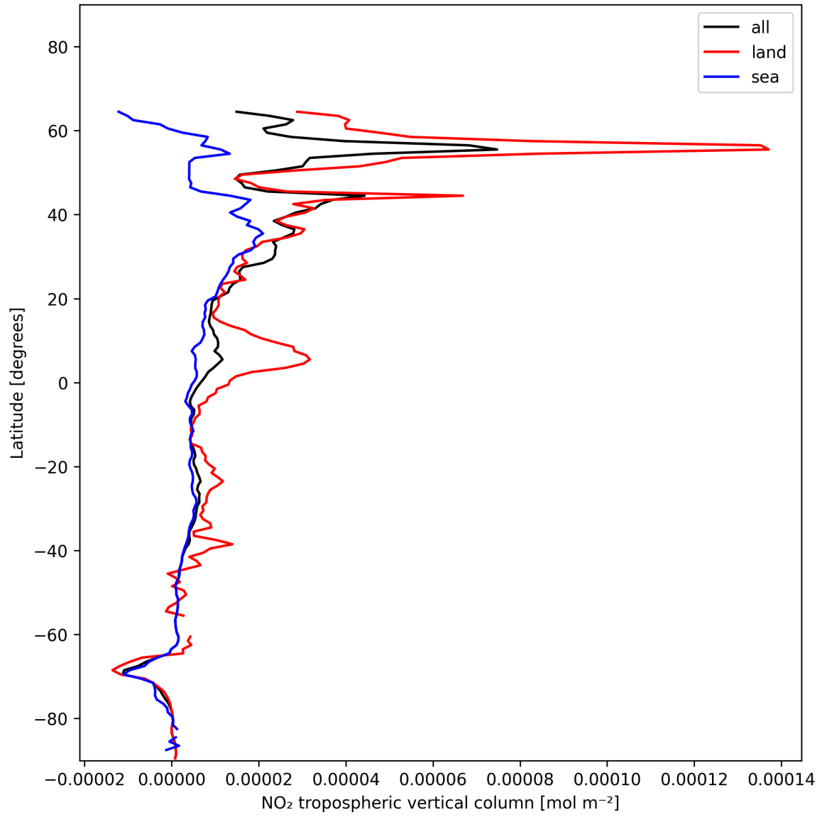
Figure 10: Zonal average of “NO 2 tropospheric vertical column” for 2024-12-29 to 2024-12-30.
