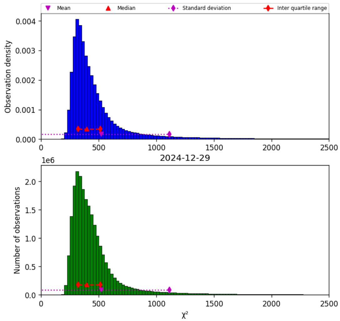
Figure 40: Histogram of “ \chi^2 ” for 2024-12-29 to 2024-12-30
