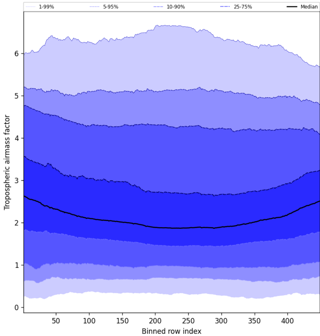
Figure 46: Along track statistics of “Tropospheric airmass factor” for 2024-12-29 to 2024-12-30
