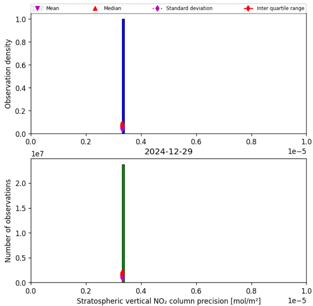
Figure 35: Histogram of “Stratospheric vertical NO 2 column precision” for 2024-12-29 to 2024-12-30
