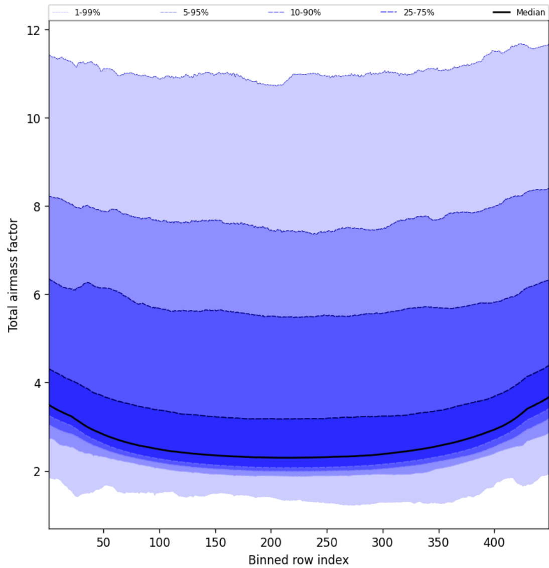
Figure 47: Along track statistics of “Total airmass factor” for 2024-12-29 to 2024-12-30
