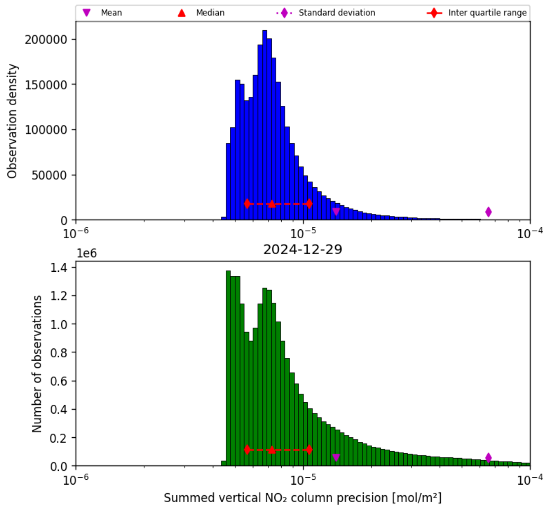
Figure 39: Histogram of "Summed vertical NO 2 column precision" for 2024-12-29 to 2024-12-30
