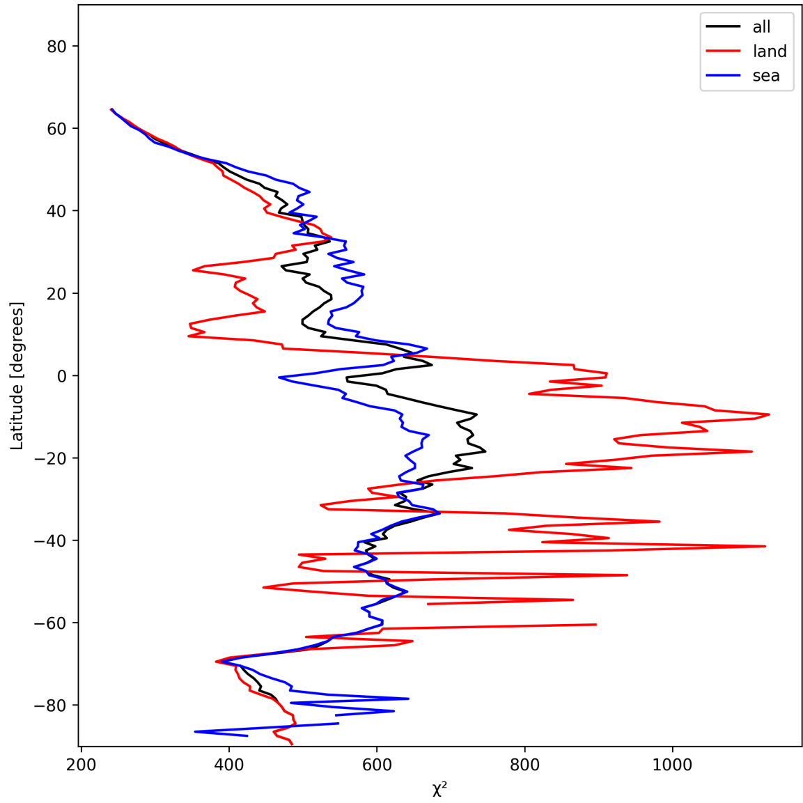
Figure 23: Zonal average of “ \chi^2 ” for 2024-12-29 to 2024-12-30.
