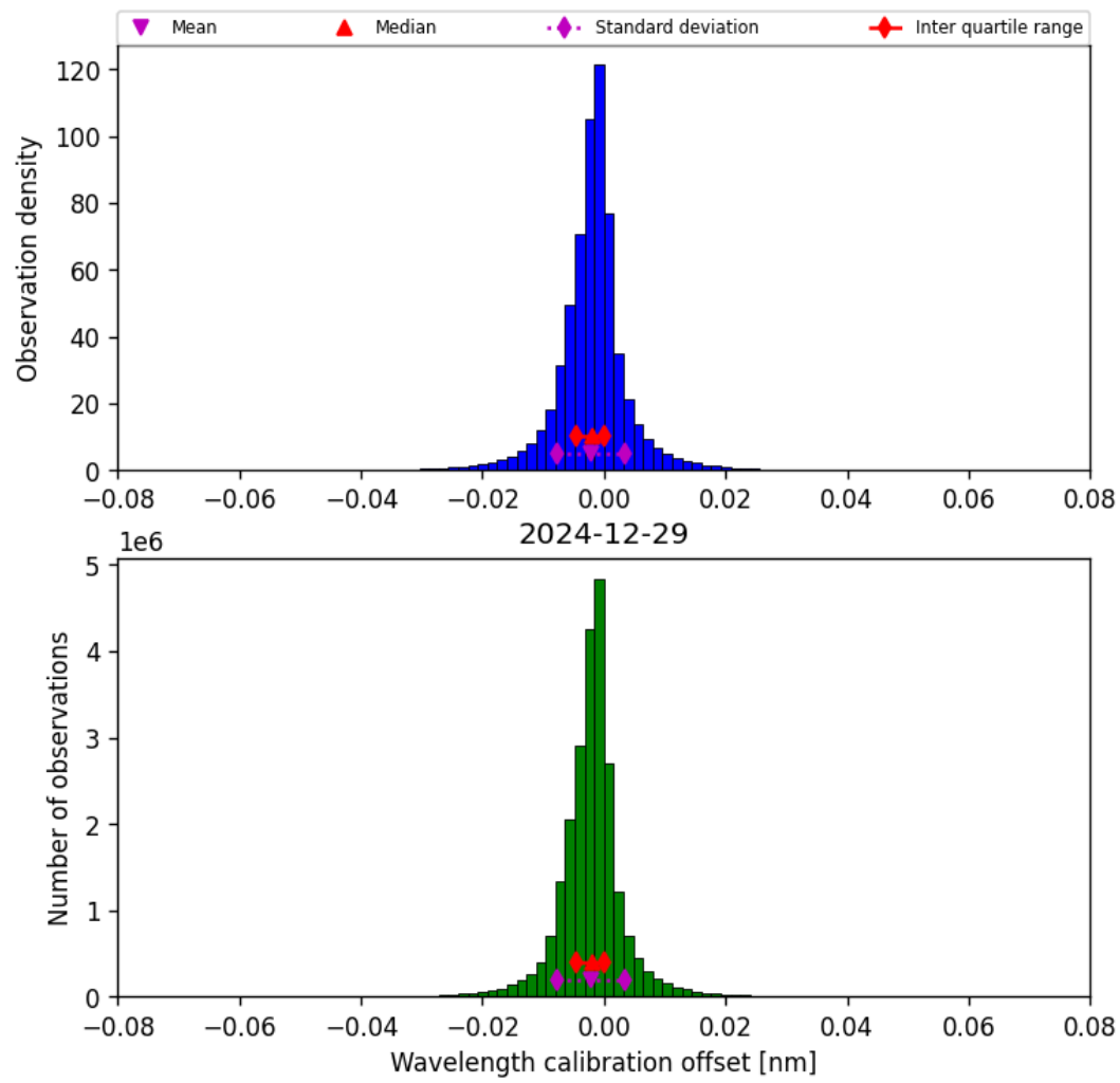
Figure 33: Histogram of “Wavelength calibration offset” for 2024-12-29 to 2024-12-30
