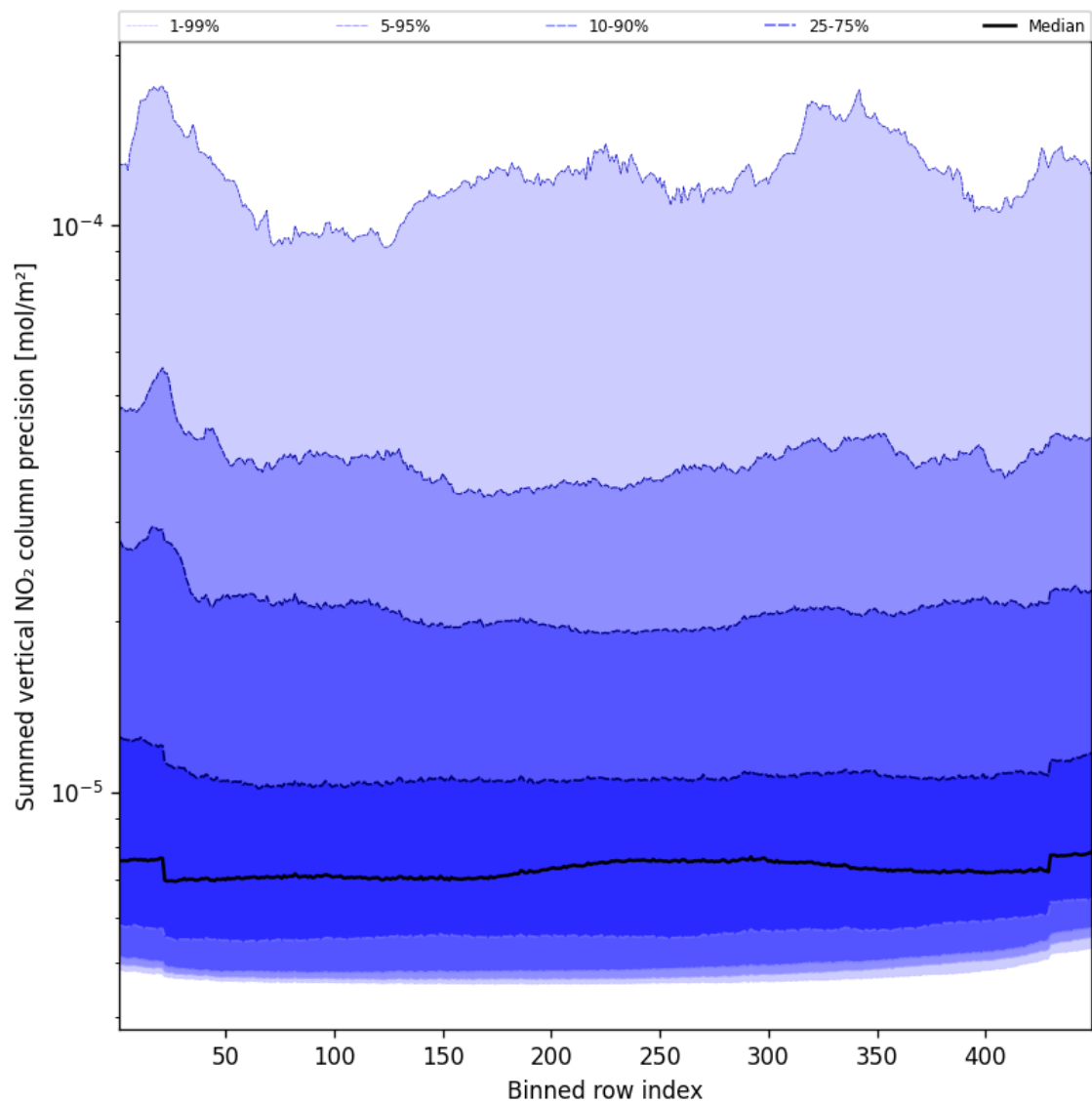
Figure 56: Along track statistics of “Summed vertical NO 2 column precision” for 2024-12-29 to 2024-12-30
