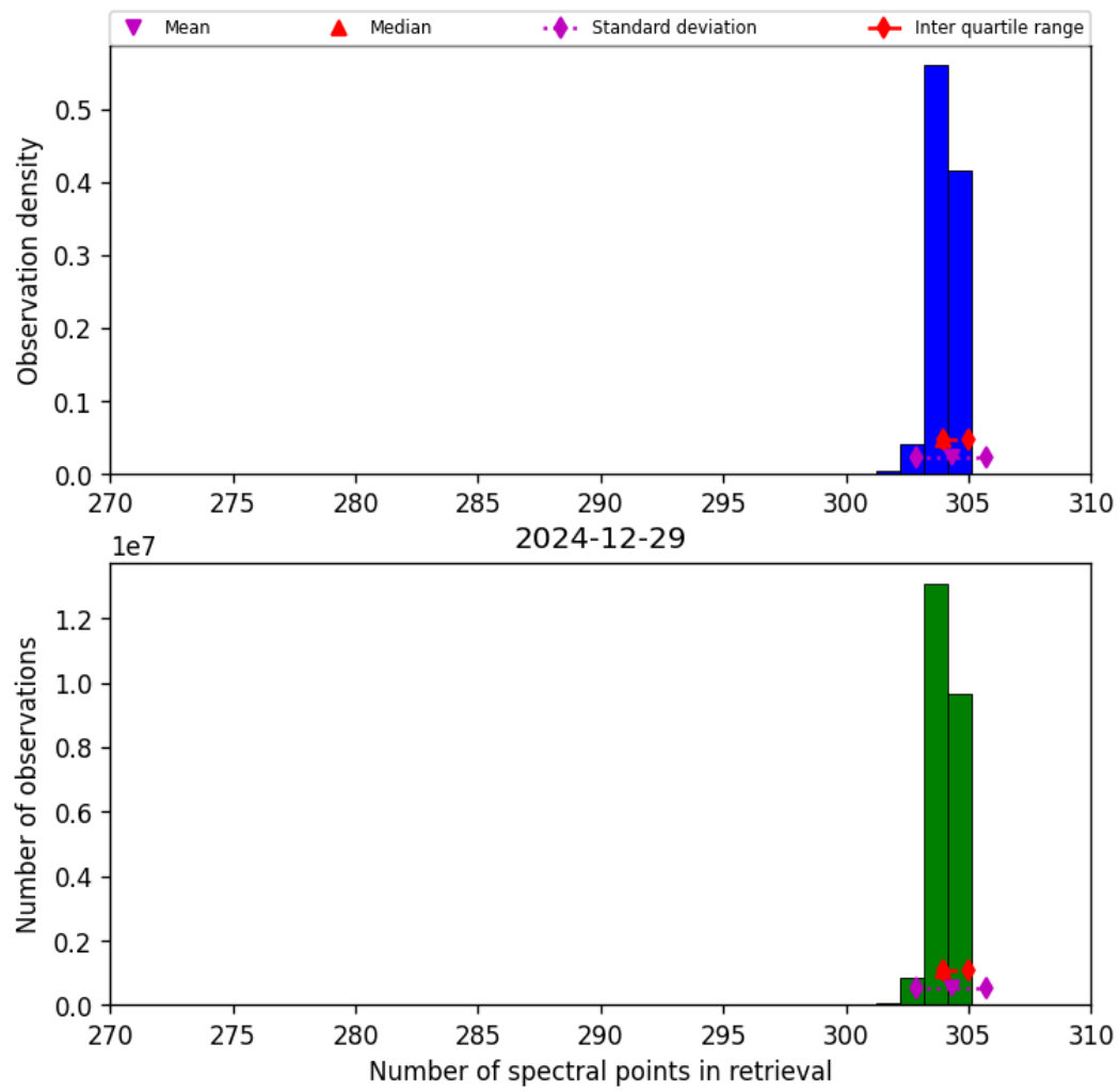
Figure 31: Histogram of “Number of spectral points in retrieval” for 2024-12-29 to 2024-12-30
