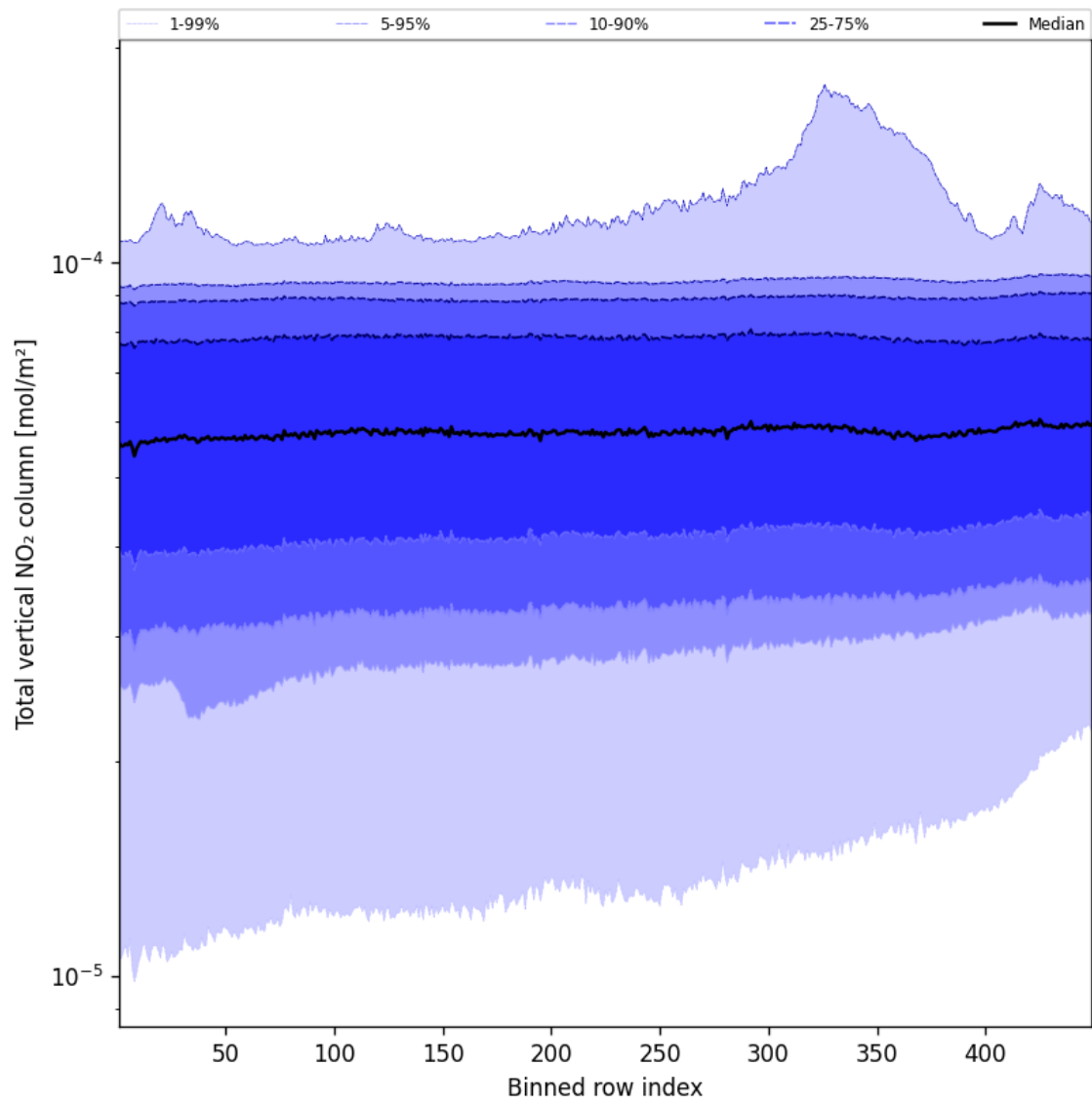
Figure 53: Along track statistics of “Total vertical NO 2 column” for 2024-12-29 to 2024-12-30
