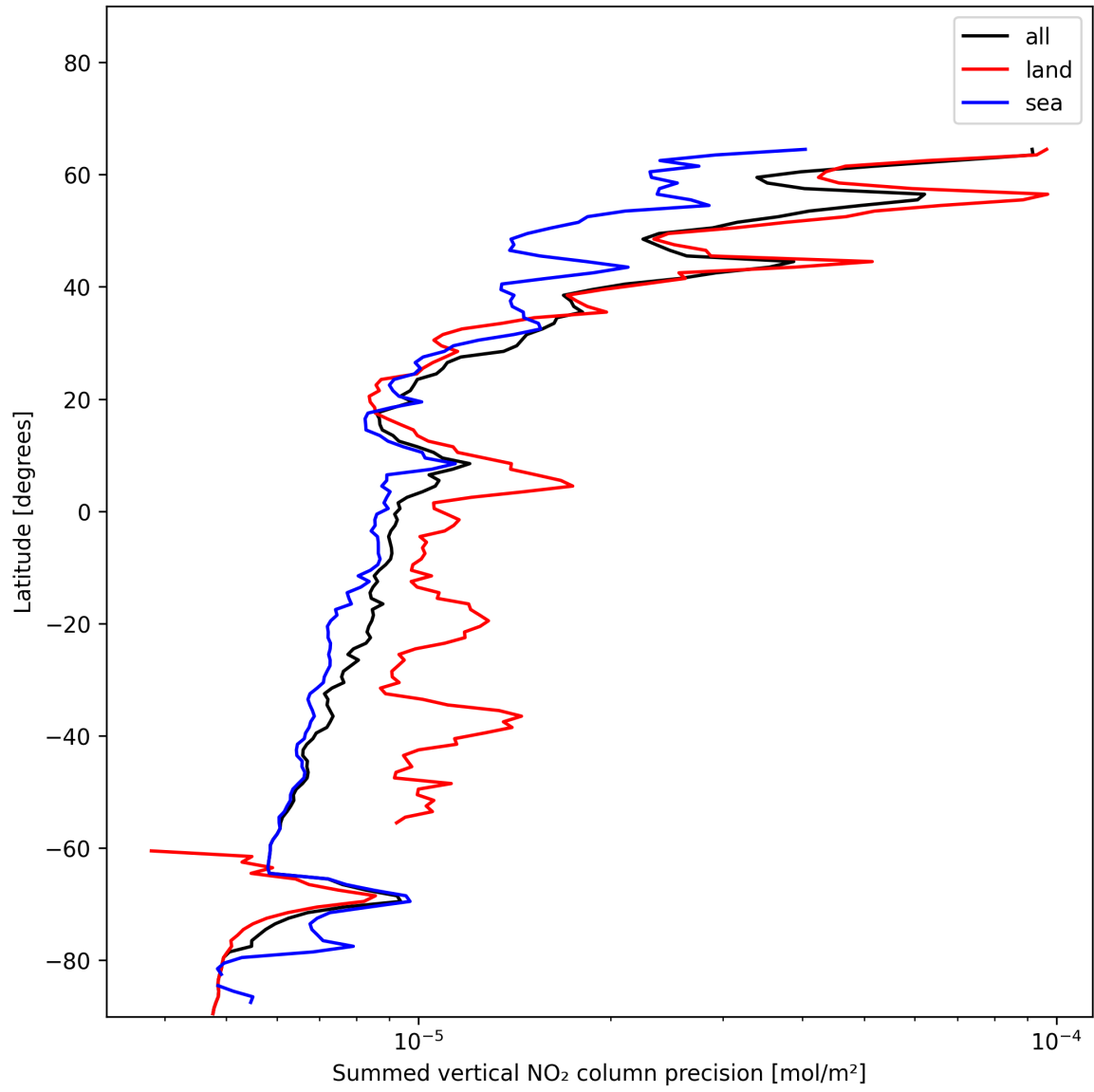
Figure 22: Zonal average of “Summed vertical NO 2 column precision” for 2024-12-29 to 2024-12-30.
