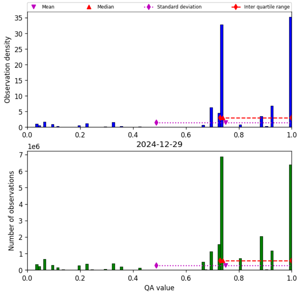
Figure 26: Histogram of “QA value” for 2024-12-29 to 2024-12-30
