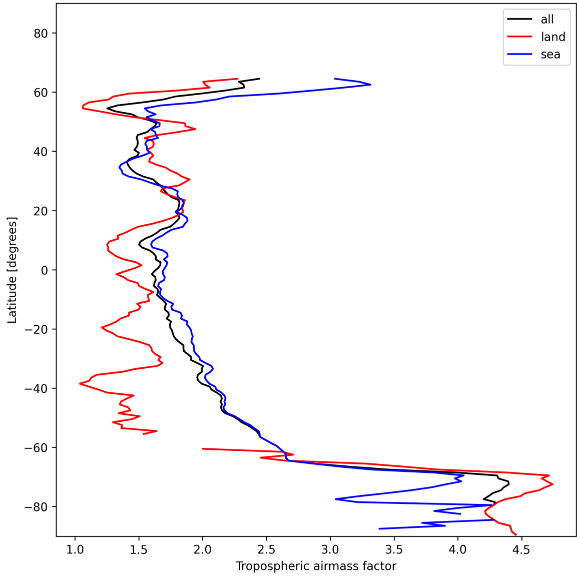
Figure 12: Zonal average of “Tropospheric airmass factor” for 2024-12-29 to 2024-12-30.
