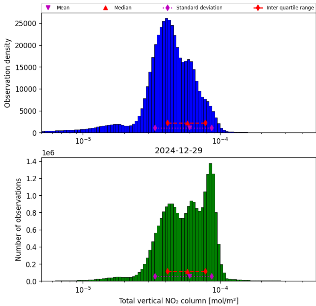
Figure 36: Histogram of “Total vertical NO 2 column” for 2024-12-29 to 2024-12-30
