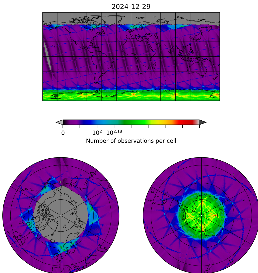
Figure 8: Map of the number of observations for 2024-12-29 to 2024-12-30
