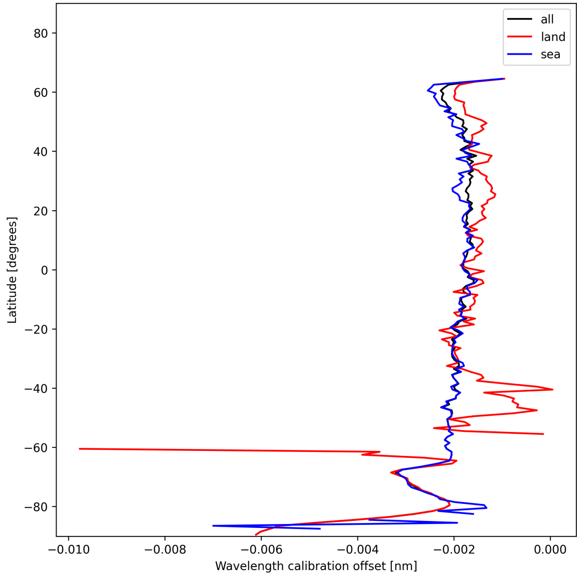
Figure 16: Zonal average of “Wavelength calibration offset” for 2024-12-29 to 2024-12-30.
