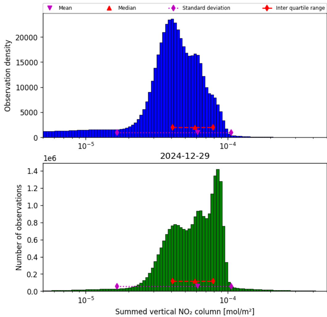
Figure 38: Histogram of “Summed vertical NO 2 column” for 2024-12-29 to 2024-12-30
