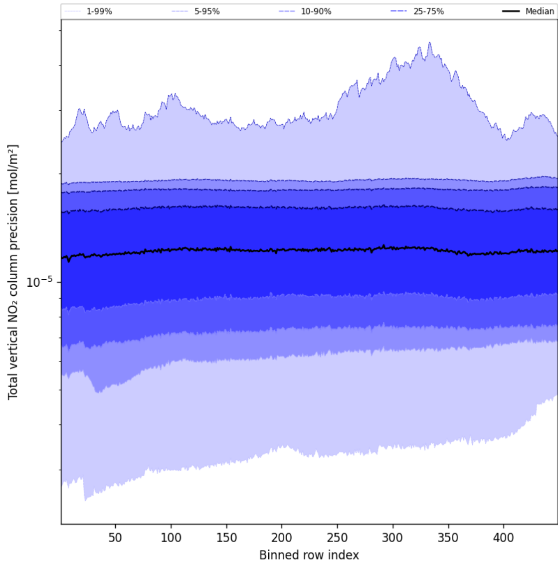
Figure 54: Along track statistics of “Total vertical NO 2 column precision” for 2024-12-29 to 2024-12-30
