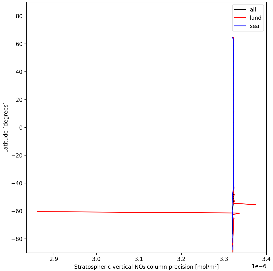
Figure 18: Zonal average of “Stratospheric vertical NO 2 column precision” for 2024-12-29 to 2024-12-30.
