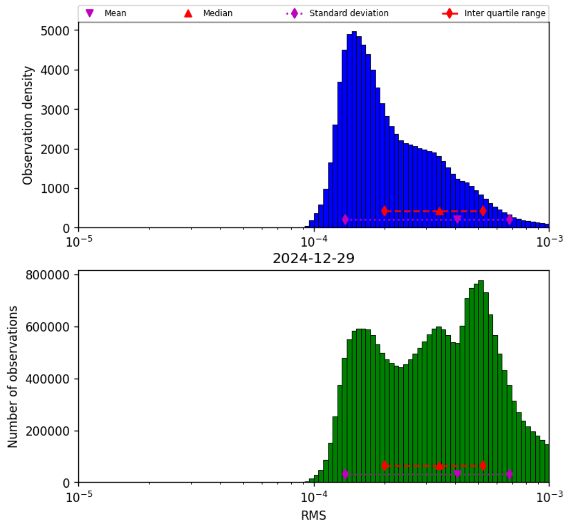
Figure 41: Histogram of “RMS” for 2024-12-29 to 2024-12-30
