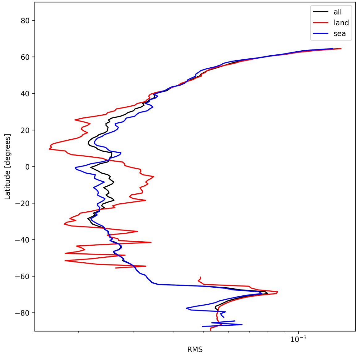
Figure 24: Zonal average of “RMS” for 2024-12-29 to 2024-12-30.
