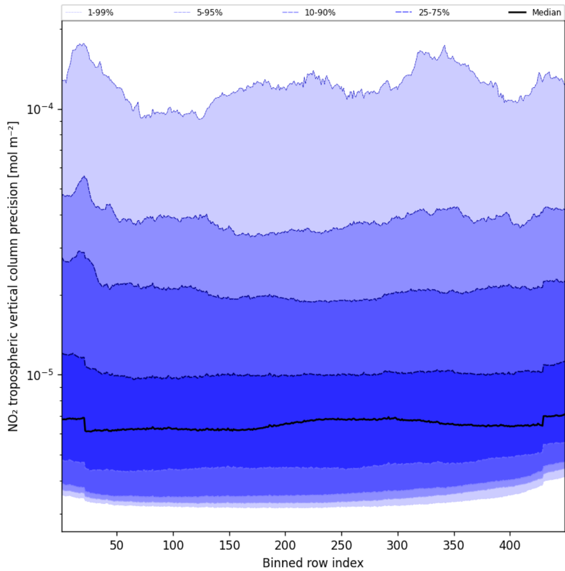
Figure 45: Along track statistics of “NO 2 tropospheric vertical column precision” for 2024-12-29 to 2024-12-30
