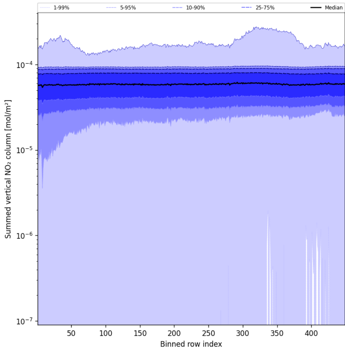
Figure 55: Along track statistics of “Summed vertical NO 2 column” for 2024-12-29 to 2024-12-30
