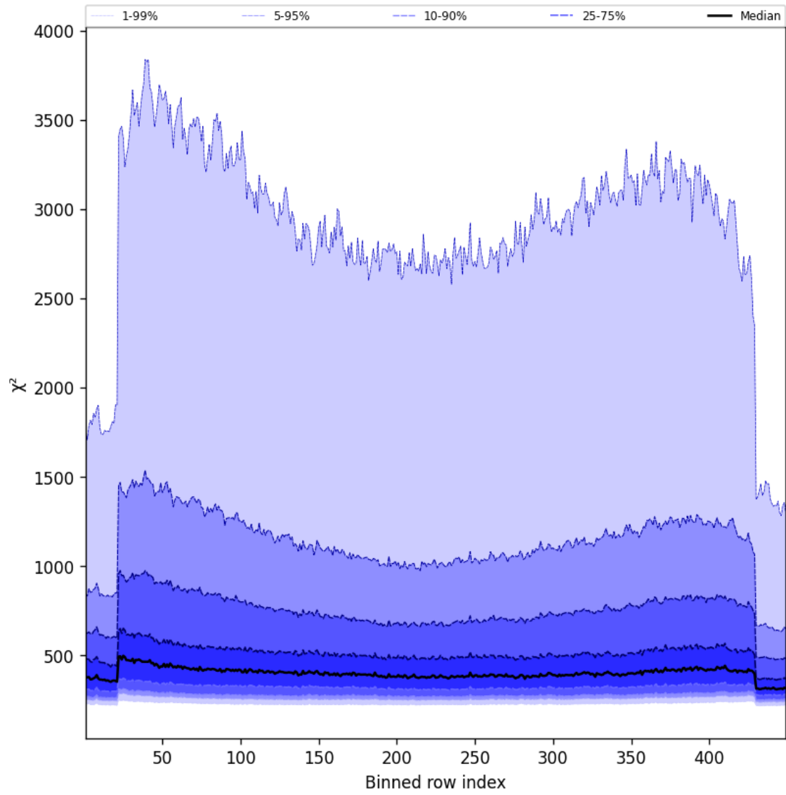
Figure 57: Along track statistics of “ \chi^2 ” for 2024-12-29 to 2024-12-30
