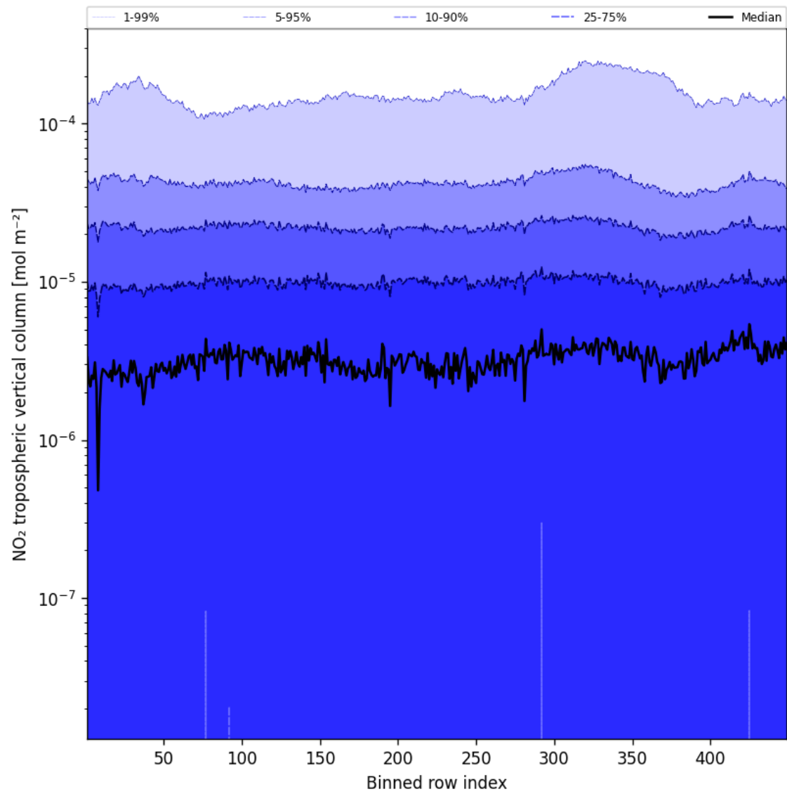
Figure 44: Along track statistics of “NO 2 tropospheric vertical column” for 2024-12-29 to 2024-12-30
