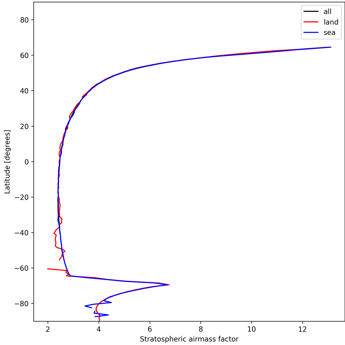
Figure 25: Zonal average of “Stratospheric airmass factor” for 2024-12-29 to 2024-12-30.
