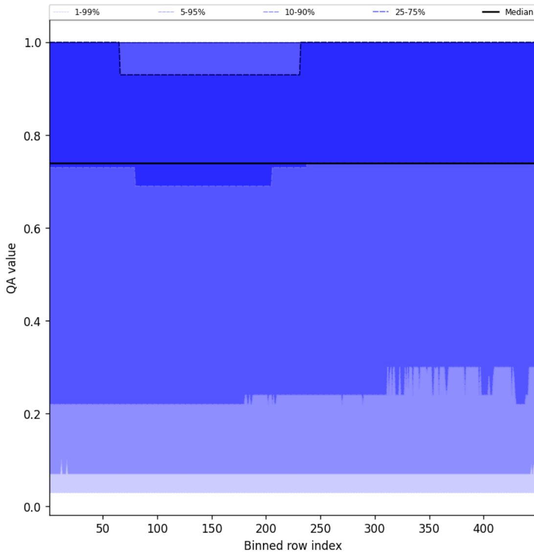
Figure 43: Along track statistics of “QA value” for 2024-12-29 to 2024-12-30
