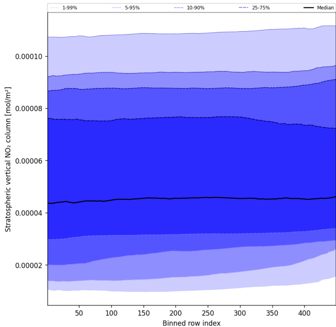
Figure 51: Along track statistics of “Stratospheric vertical NO 2 column” for 2024-12-29 to 2024-12-30
