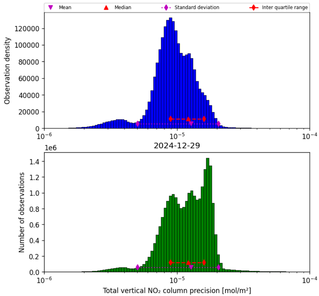
Figure 37: Histogram of “Total vertical NO 2 column precision” for 2024-12-29 to 2024-12-30
