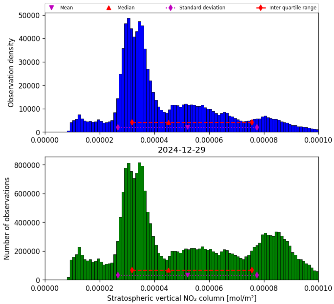
Figure 34: Histogram of “Stratospheric vertical NO 2 column” for 2024-12-29 to 2024-12-30
