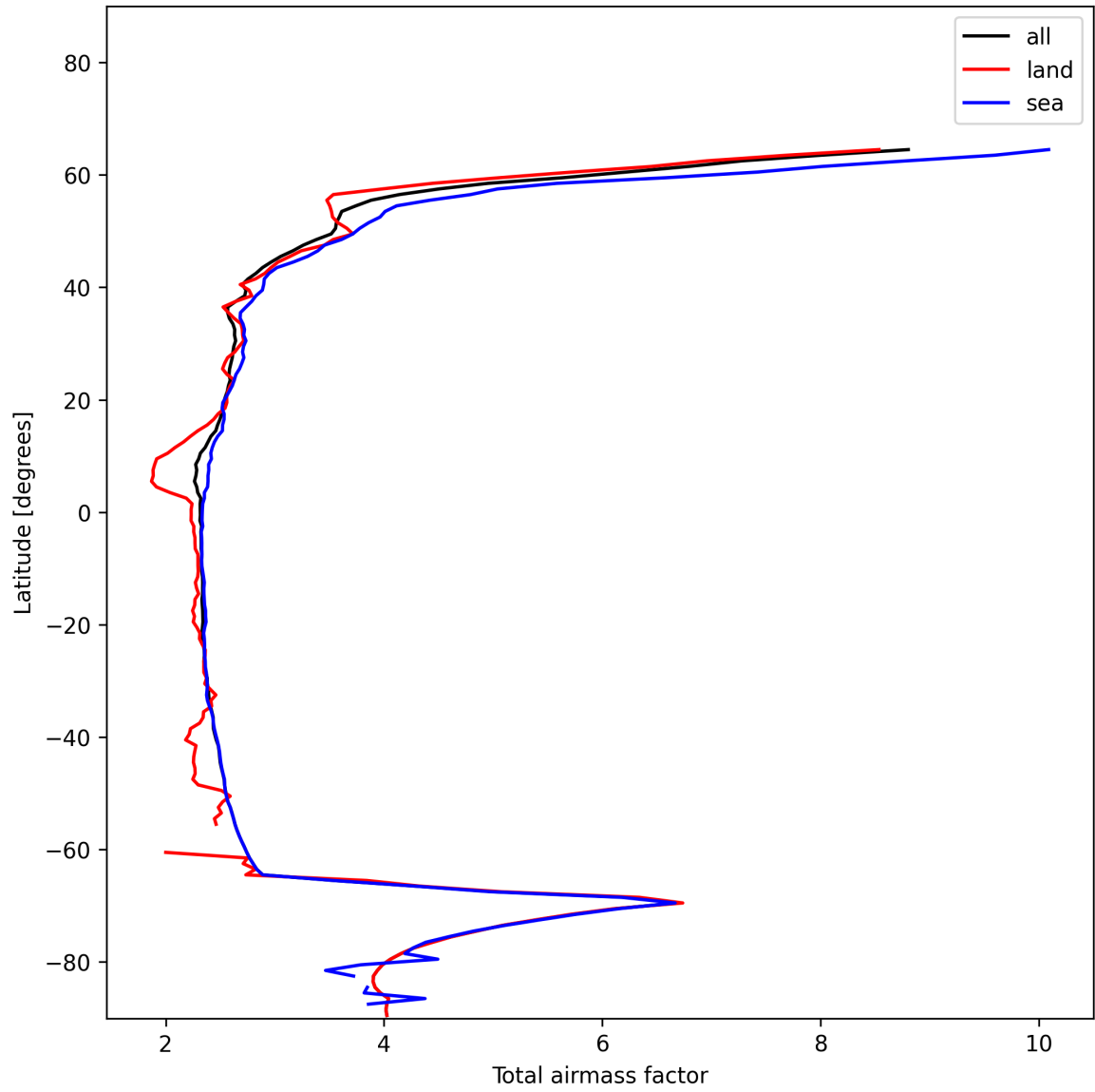
Figure 13: Zonal average of “Total airmass factor” for 2024-12-29 to 2024-12-30.
