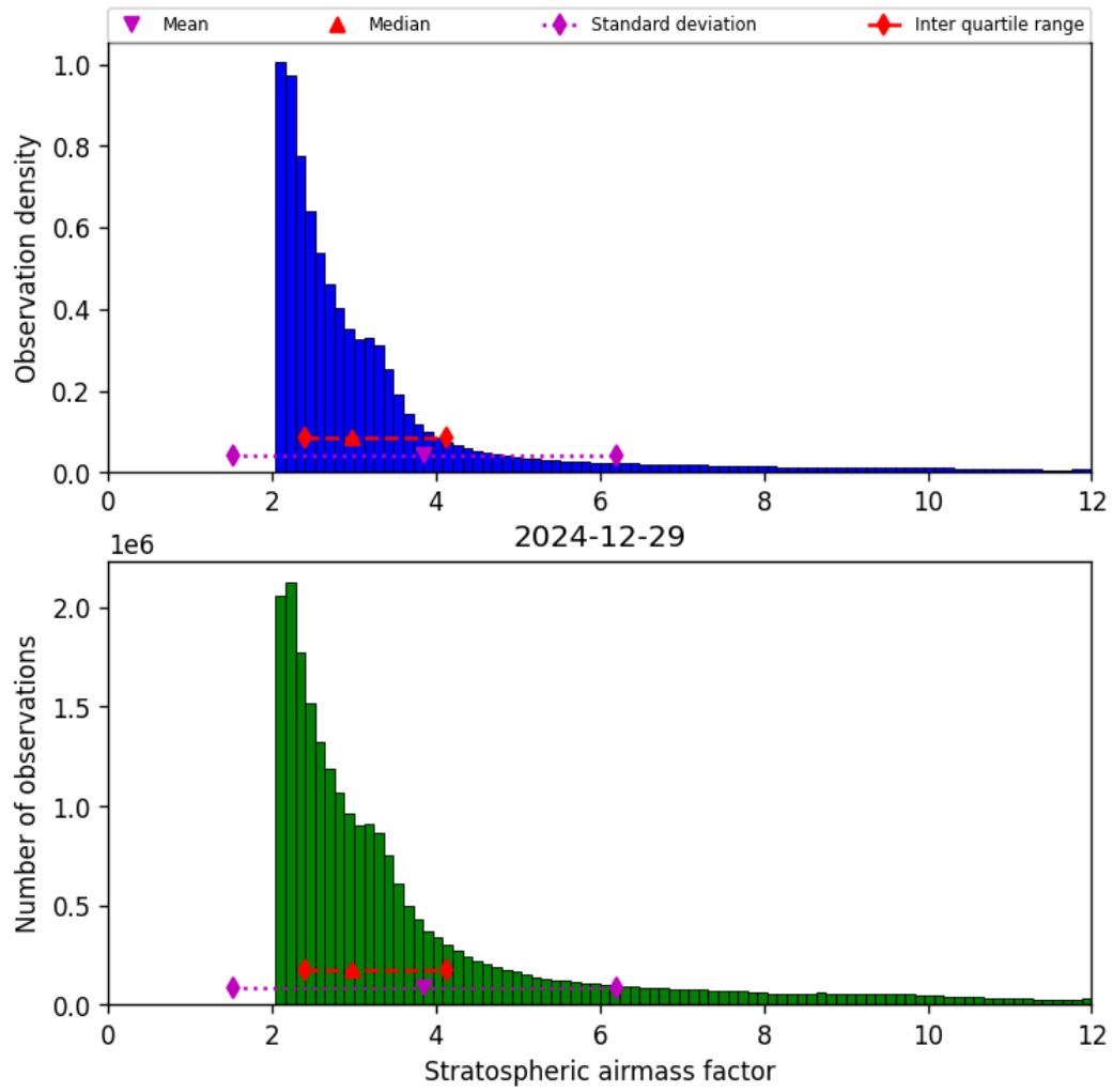
Figure 42: Histogram of “Stratospheric airmass factor” for 2024-12-29 to 2024-12-30
