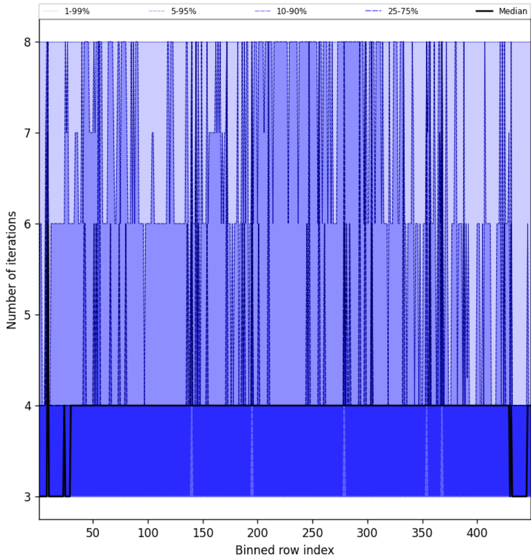
Figure 49: Along track statistics of “Number of iterations” for 2024-12-29 to 2024-12-30
