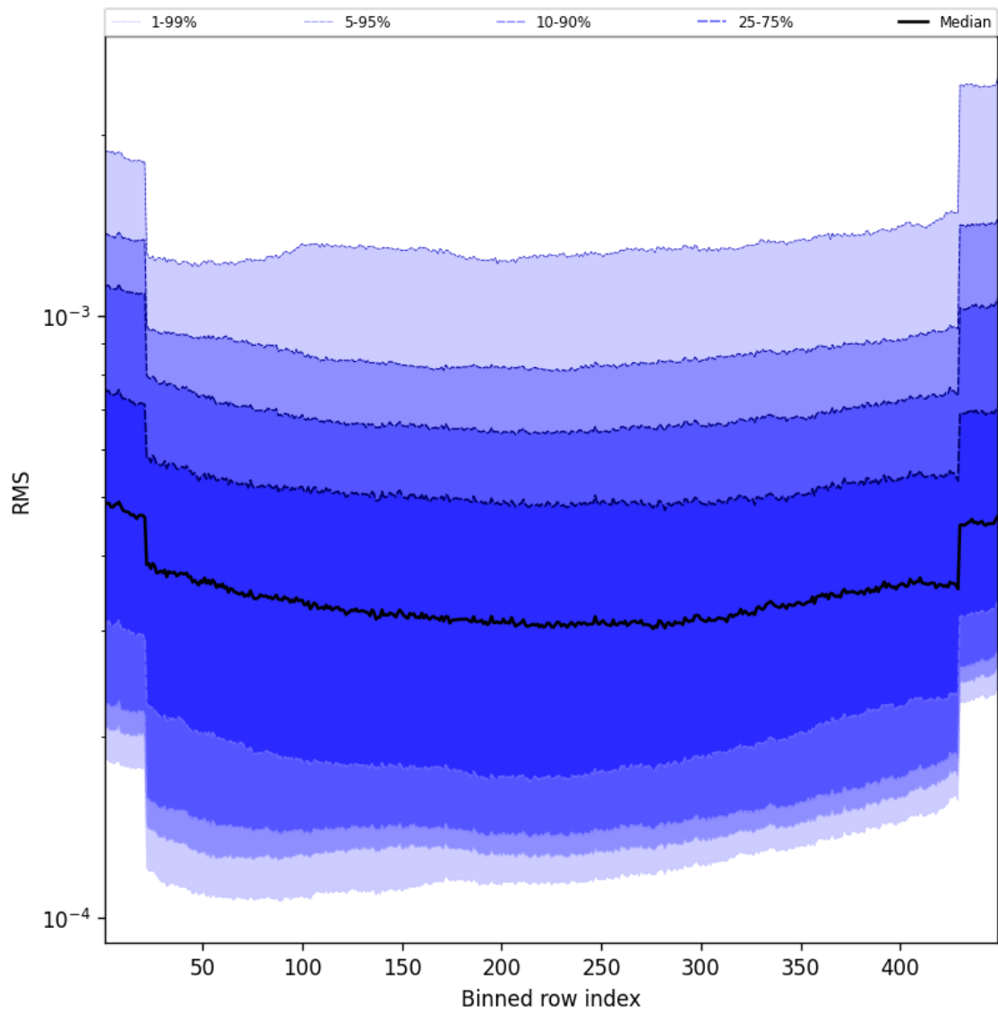
Figure 58: Along track statistics of “RMS” for 2024-12-29 to 2024-12-30
