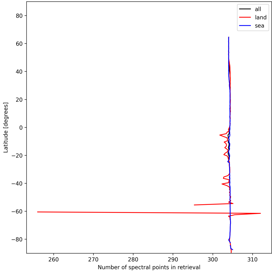
Figure 14: Zonal average of “Number of spectral points in retrieval” for 2024-12-29 to 2024-12-30.
