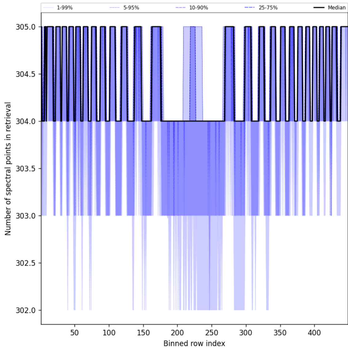
Figure 48: Along track statistics of “Number of spectral points in retrieval” for 2024-12-29 to 2024-12-30
