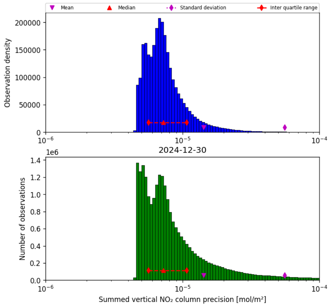
Figure 39: Histogram of "Summed vertical NO 2 column precision" for 2024-12-30 to 2024-12-30
