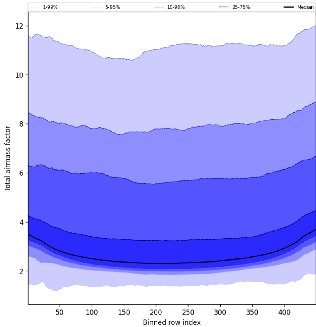
Figure 47: Along track statistics of “Total airmass factor” for 2024-12-30 to 2024-12-30
