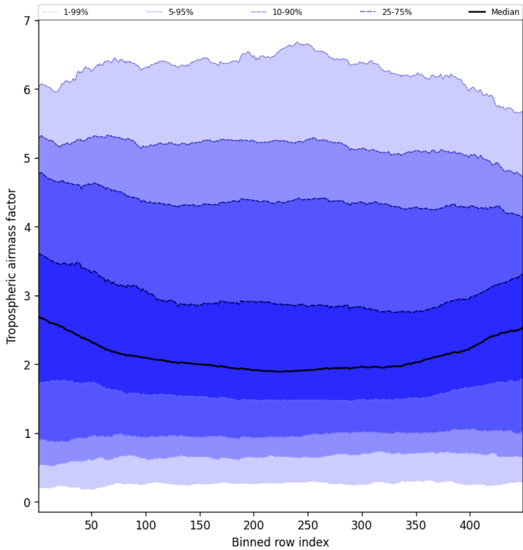
Figure 46: Along track statistics of “Tropospheric air mass factor” for 2024-12-30 to 2024-12-30
