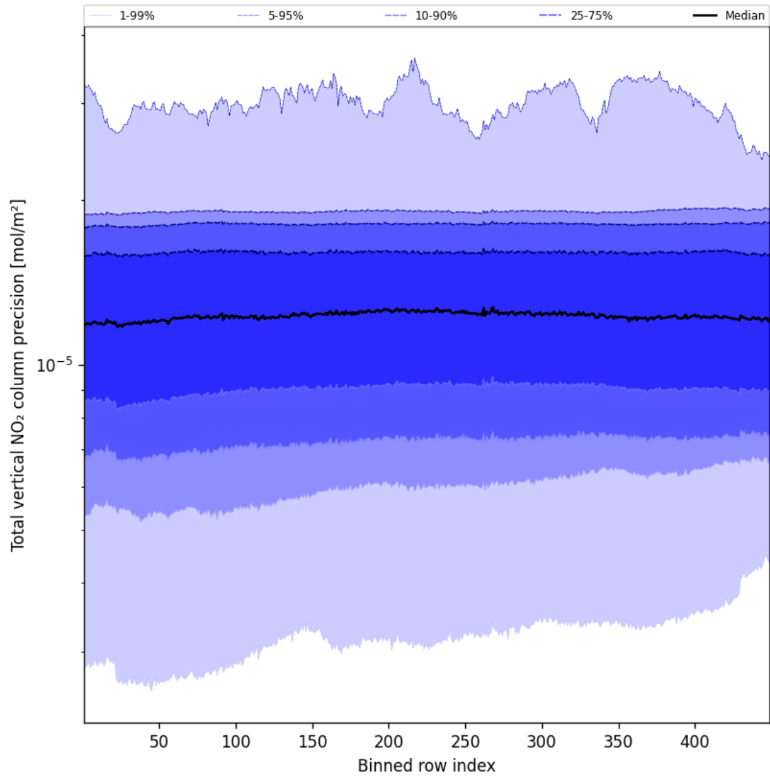
Figure 54: Along track statistics of “Total vertical NO 2 column precision” for 2024-12-30 to 2024-12-30
