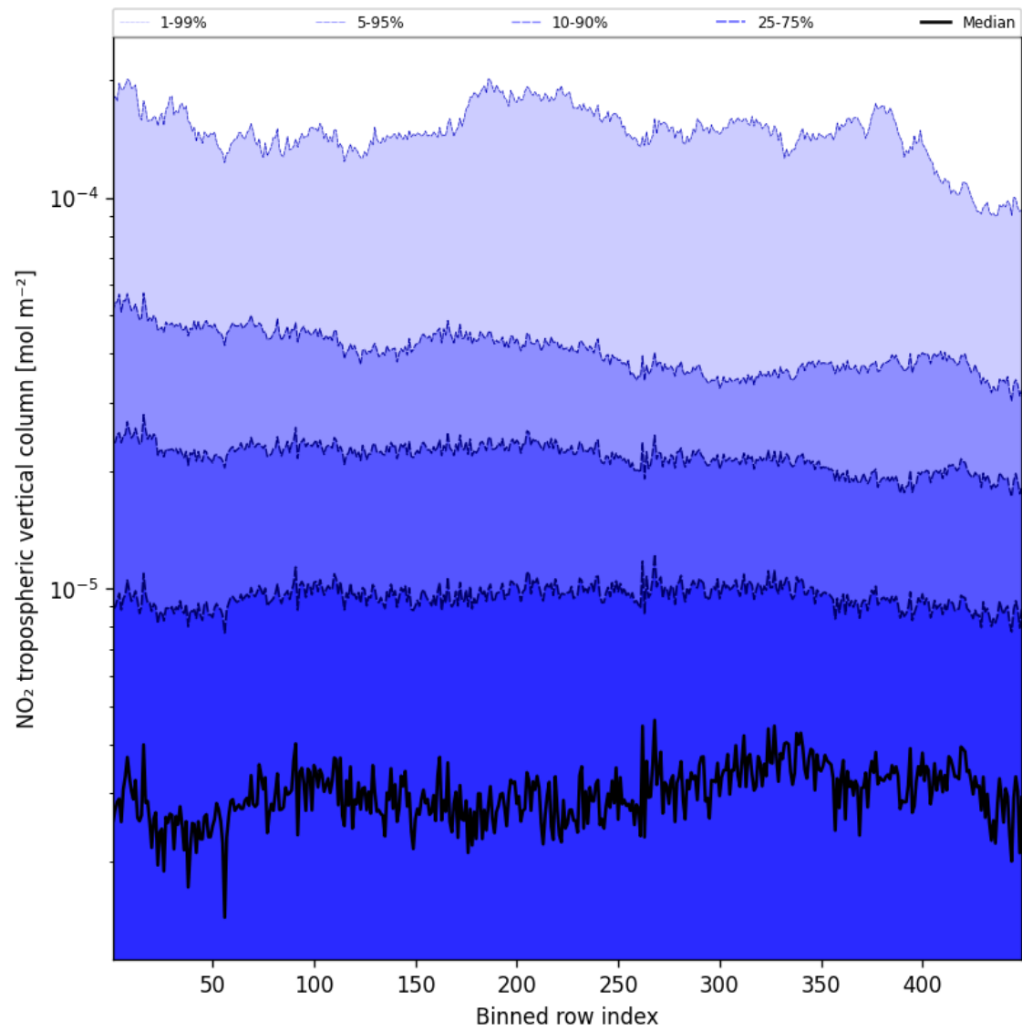
Figure 44: Along track statistics of “NO 2 tropospheric vertical column” for 2024-12-30 to 2024-12-30
