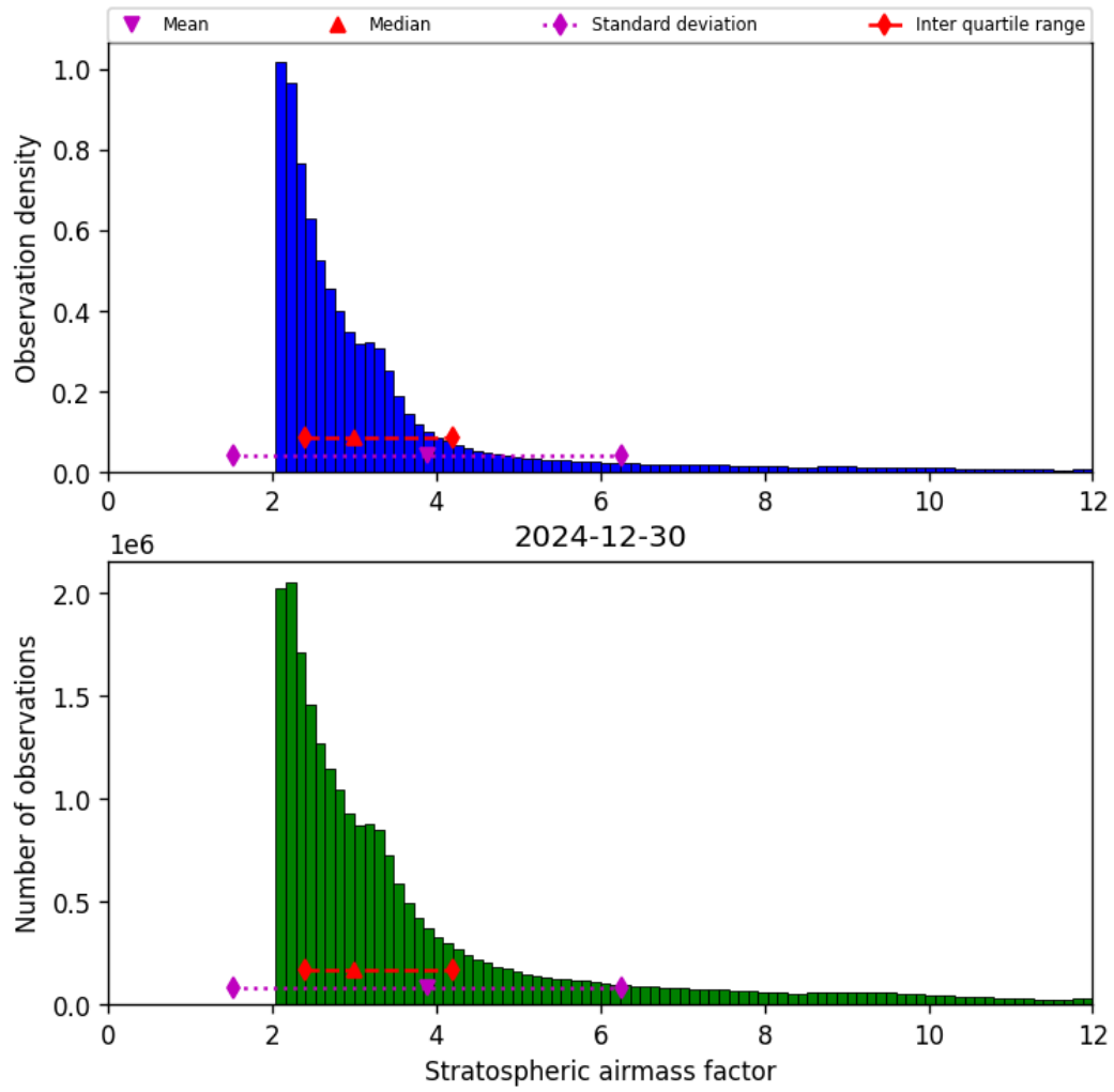
Figure 42: Histogram of “Stratospheric airmass factor” for 2024-12-30 to 2024-12-30
