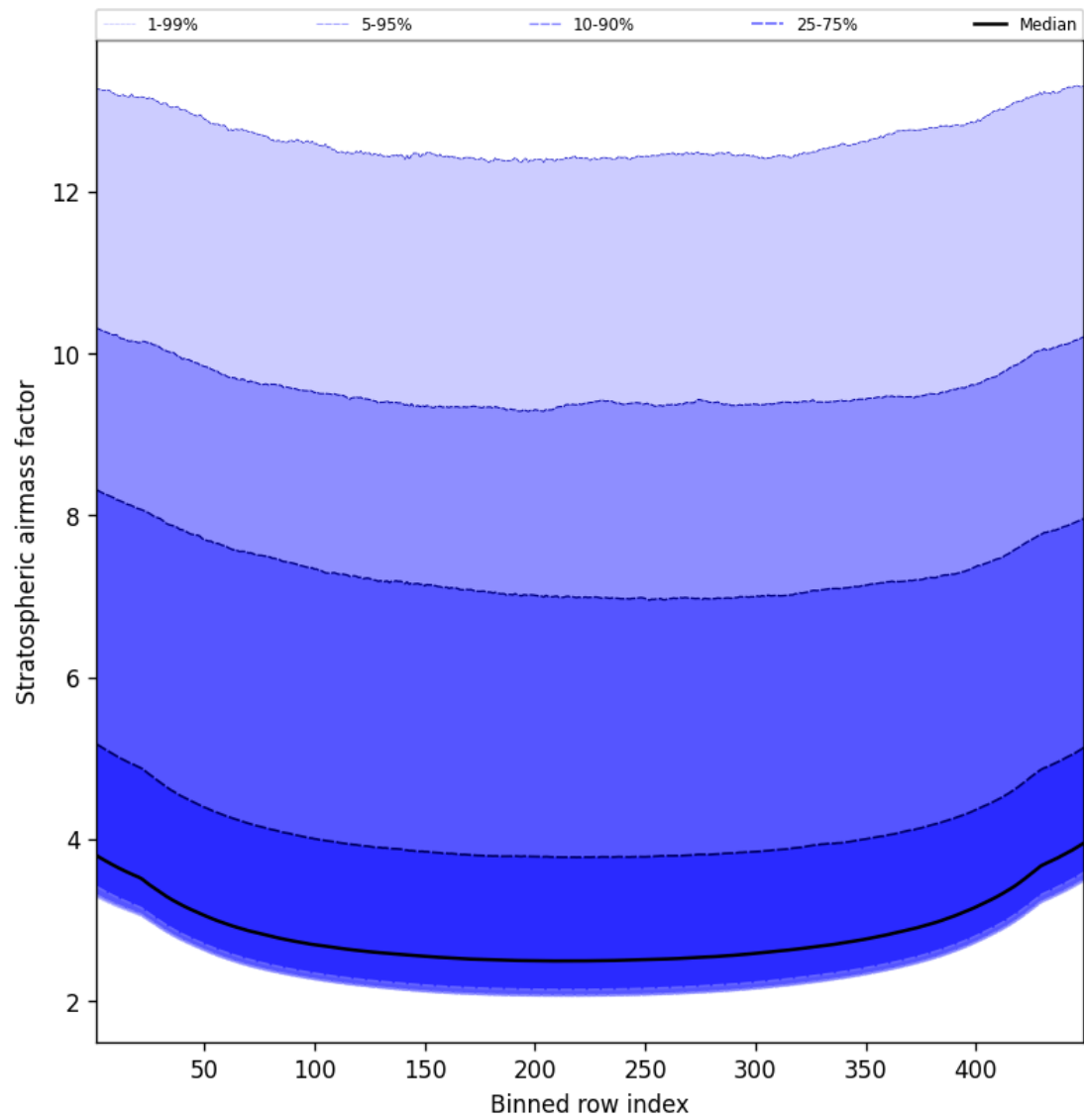
Figure 59: Along track statistics of “Stratospheric airmass factor” for 2024-12-30 to 2024-12-30
