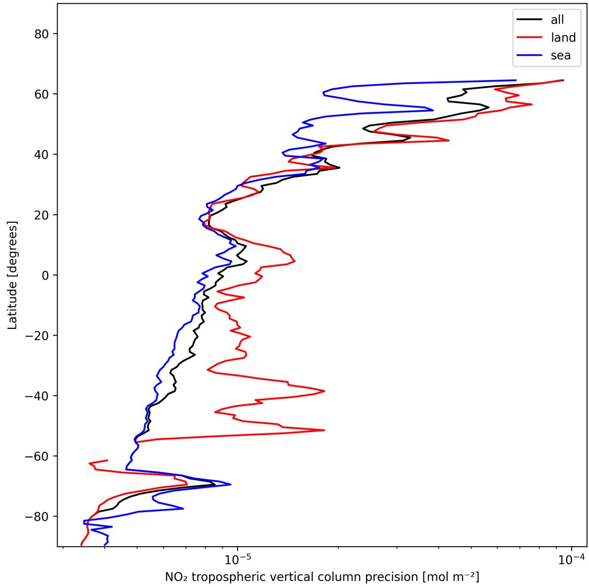
Figure 11: Zonal average of “NO 2 tropospheric vertical column precision” for 2024-12-30 to 2024-12-30.
