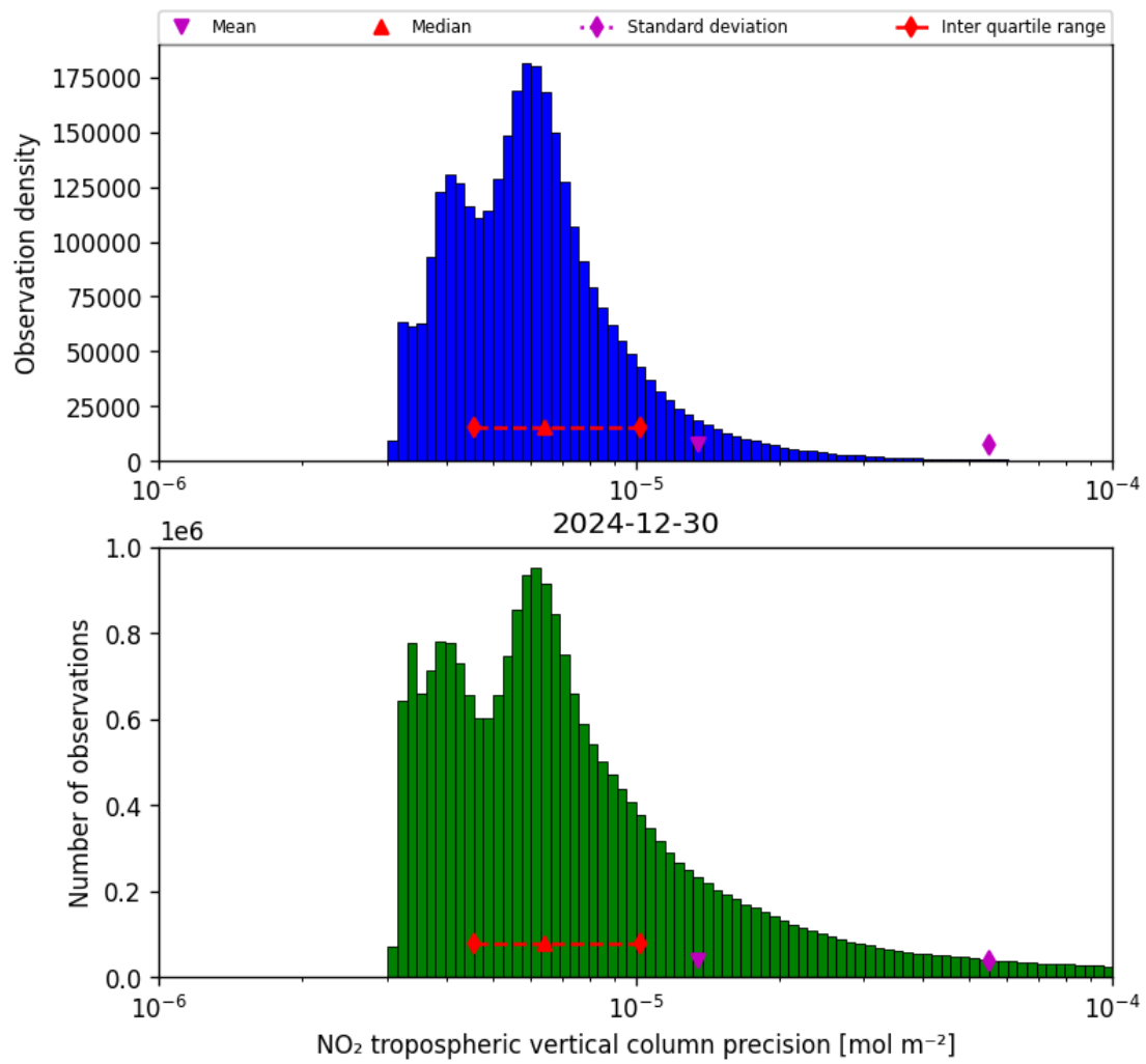
Figure 28: Histogram of “NO 2 tropospheric vertical column precision” for 2024-12-30 to 2024-12-30
