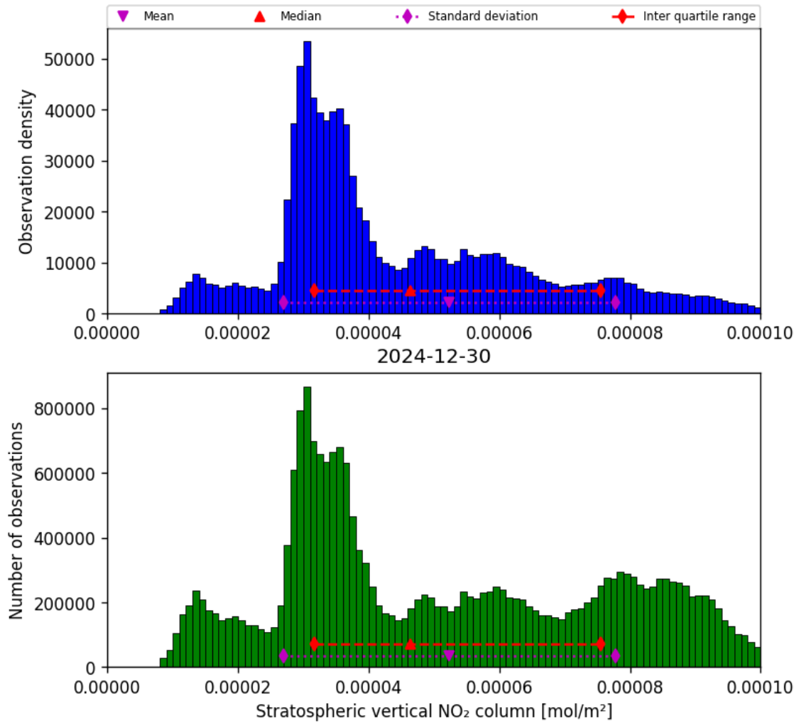
Figure 34: Histogram of “Stratospheric vertical NO 2 column” for 2024-12-30 to 2024-12-30
