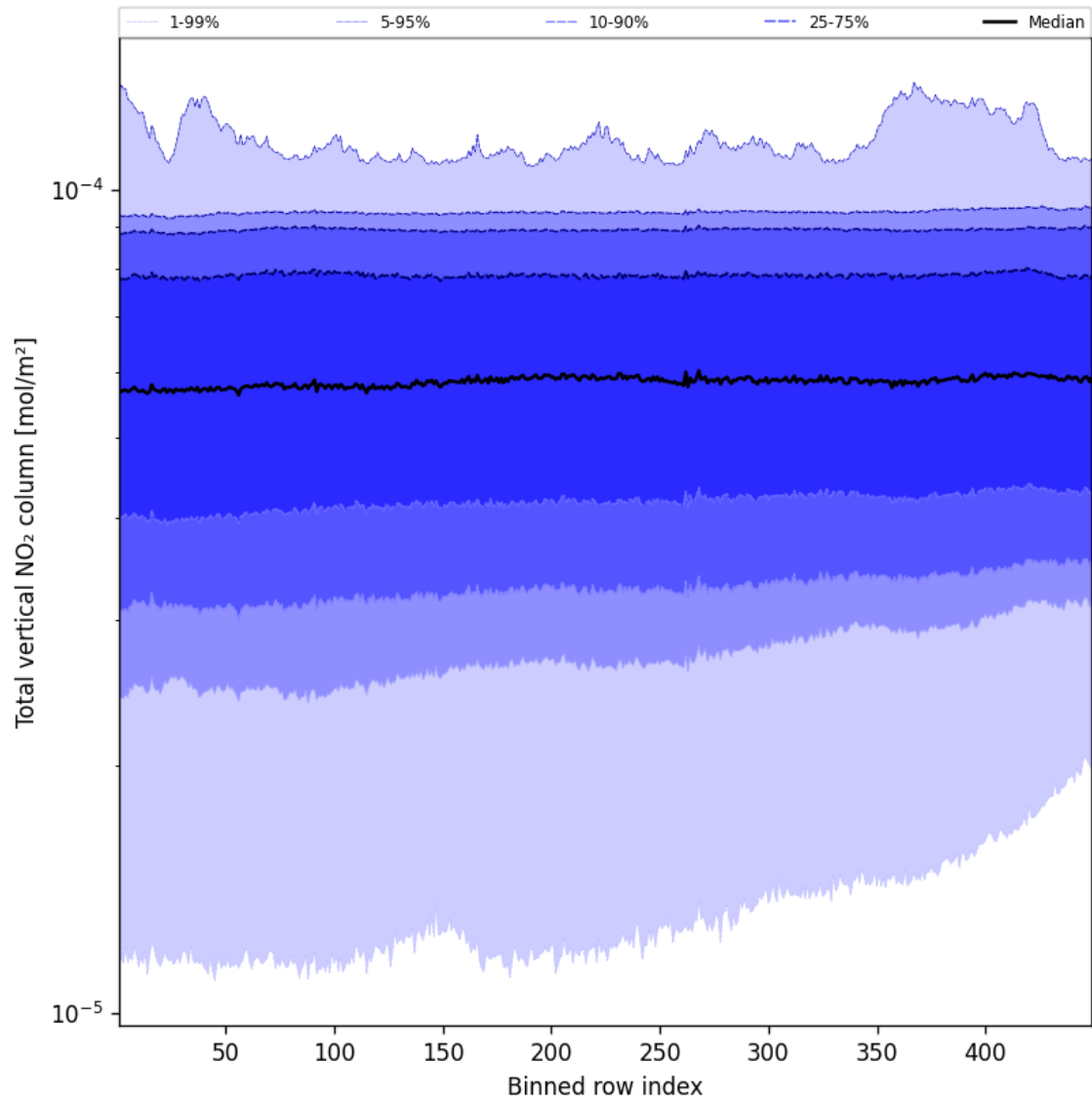
Figure 53: Along track statistics of “Total vertical NO 2 column” for 2024-12-30 to 2024-12-30
