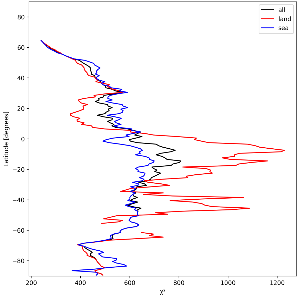
Figure 23: Zonal average of “ \chi^2 ” for 2024-12-30 to 2024-12-30.
