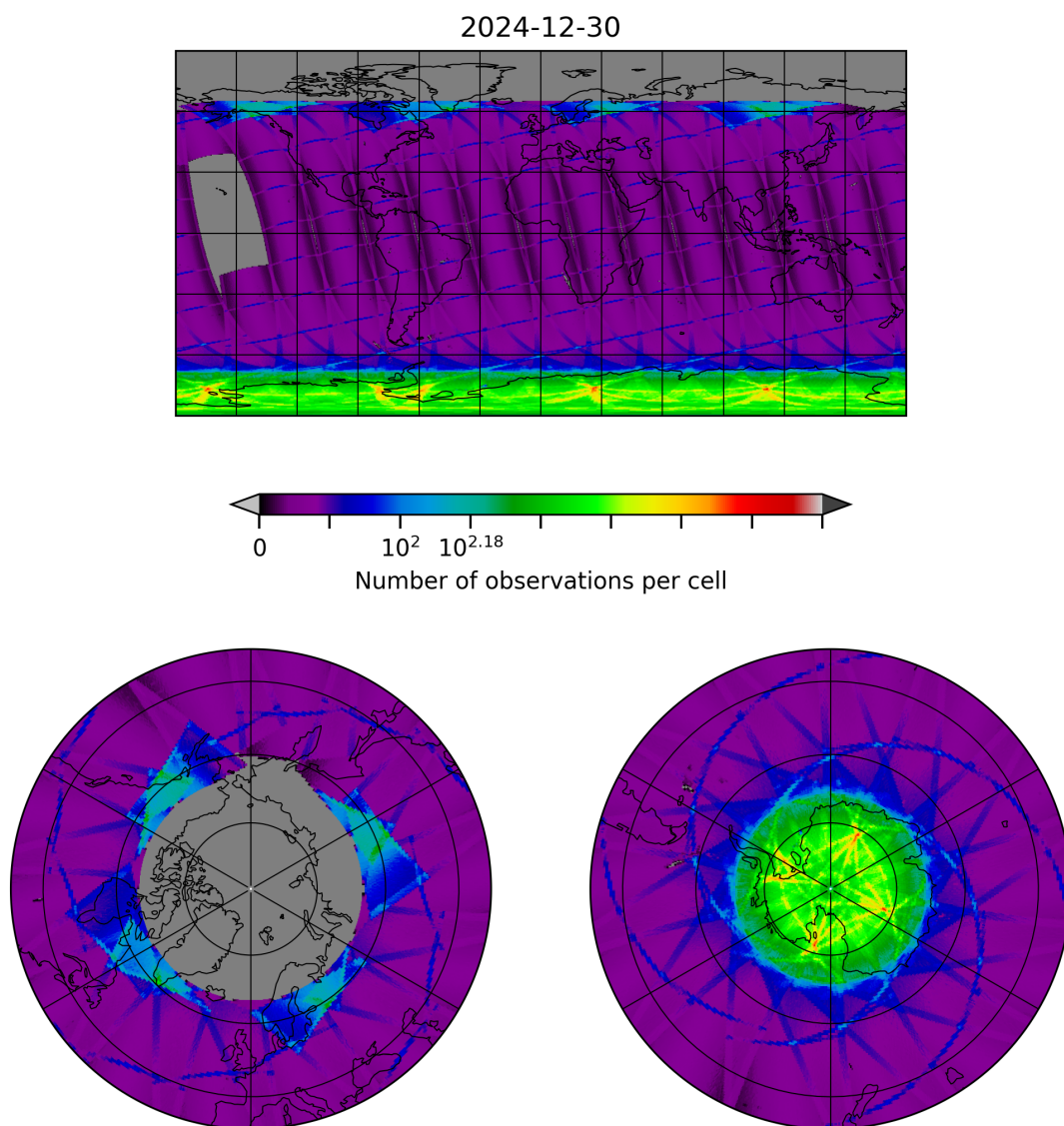
Figure 8: Map of the number of observations for 2024-12-30 to 2024-12-30
