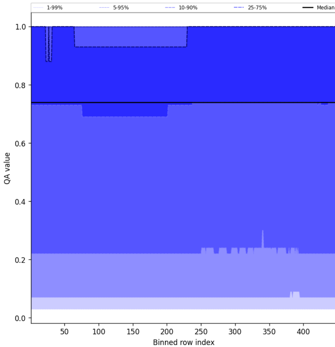
Figure 43: Along track statistics of “QA value” for 2024-12-30 to 2024-12-30
