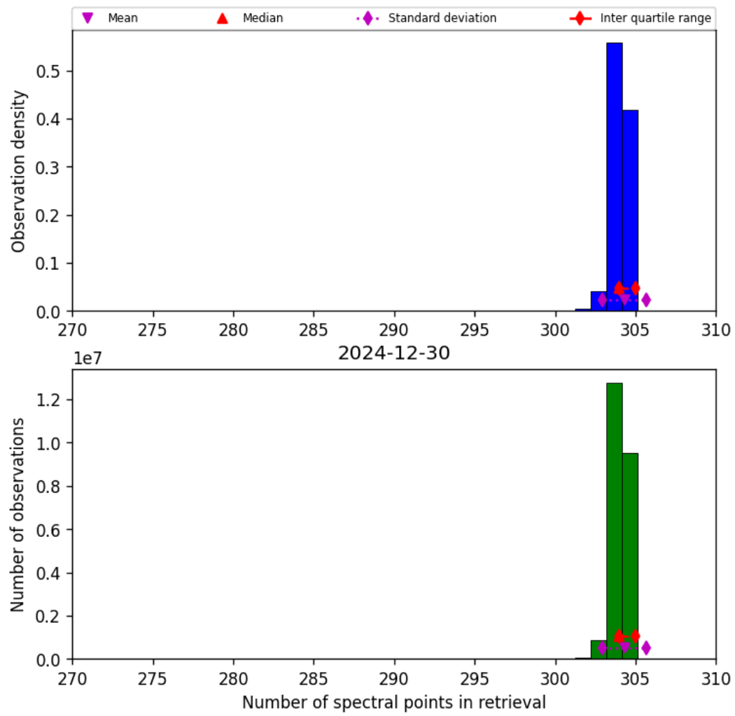
Figure 31: Histogram of “Number of spectral points in retrieval” for 2024-12-30 to 2024-12-30
