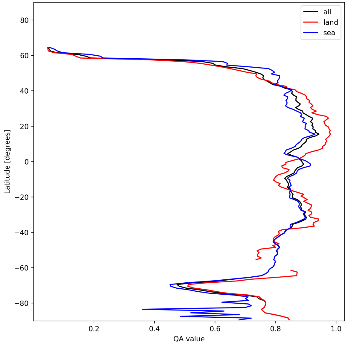
Figure 9: Zonal average of “QA value” for 2024-12-30 to 2024-12-30.
