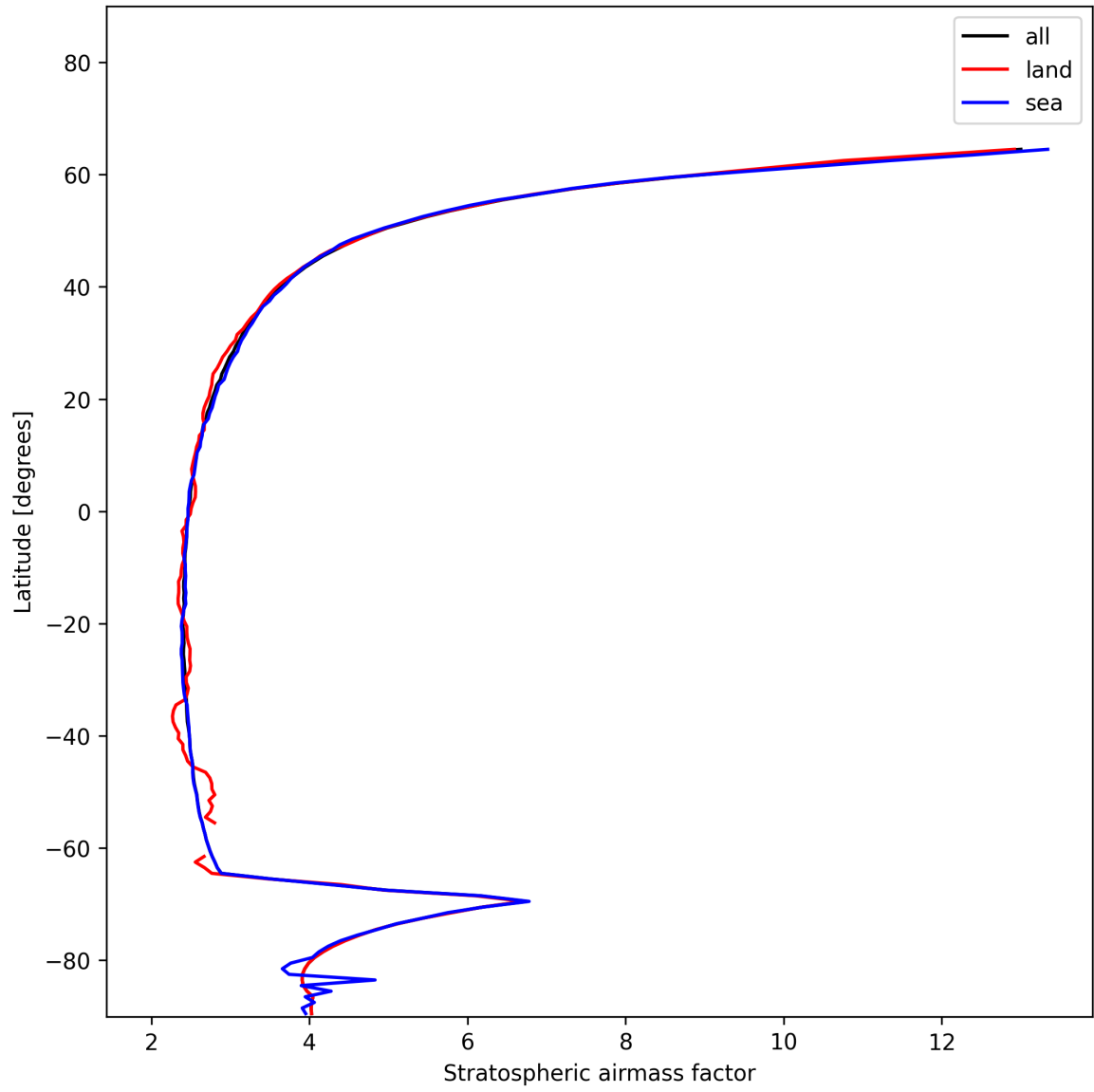
Figure 25: Zonal average of “Stratospheric airmass factor” for 2024-12-30 to 2024-12-30.
