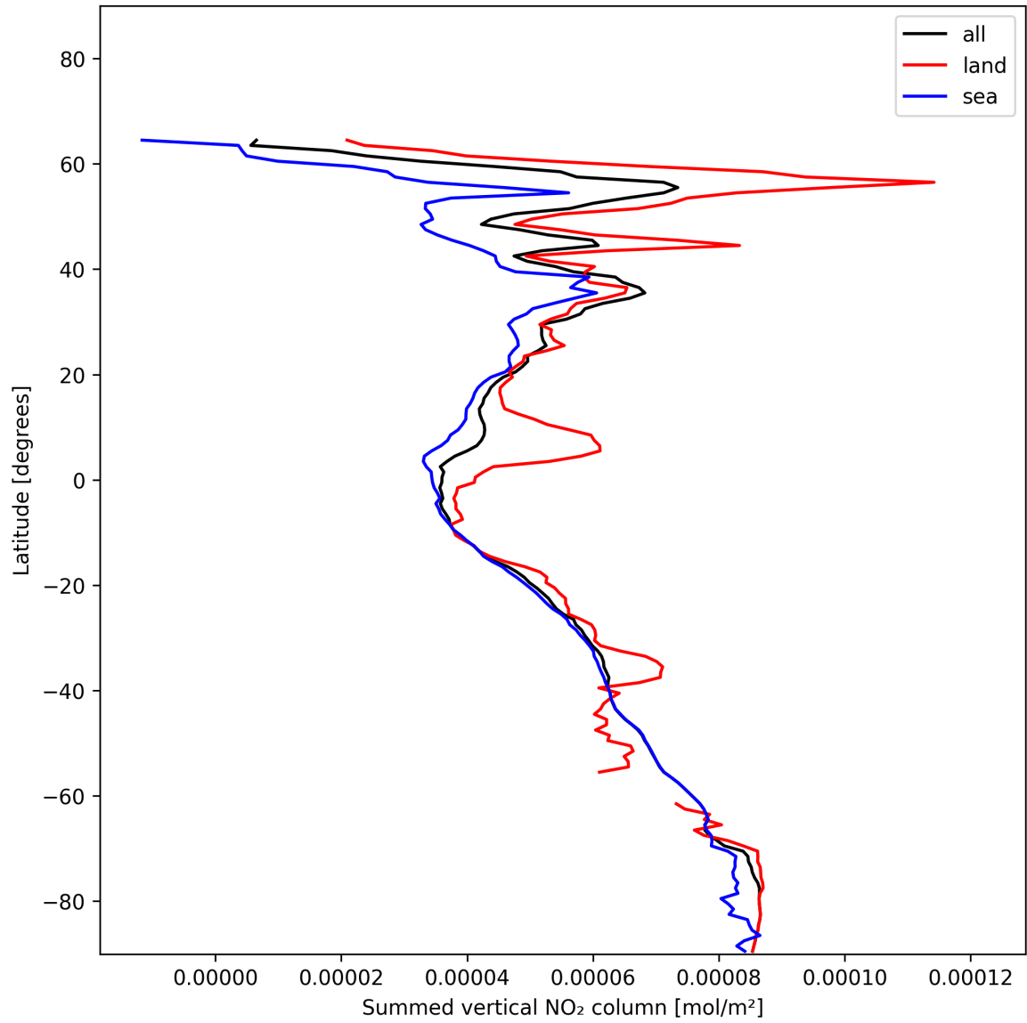
Figure 21: Zonal average of “Summed vertical NO 2 column” for 2024-12-30 to 2024-12-30.
