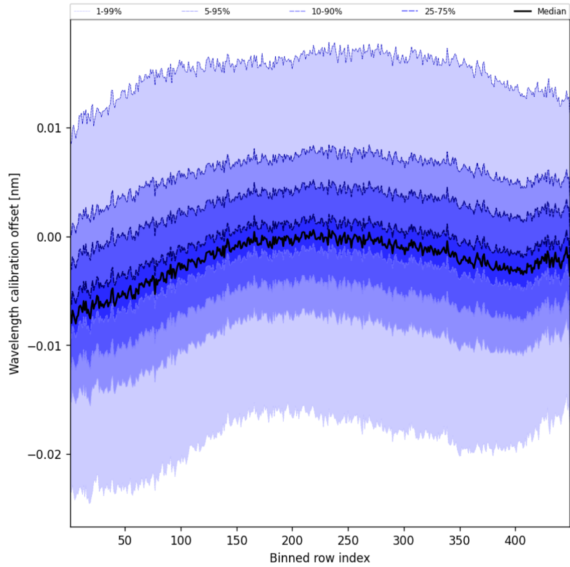
Figure 50: Along track statistics of “Wavelength calibration offset” for 2024-12-30 to 2024-12-30
