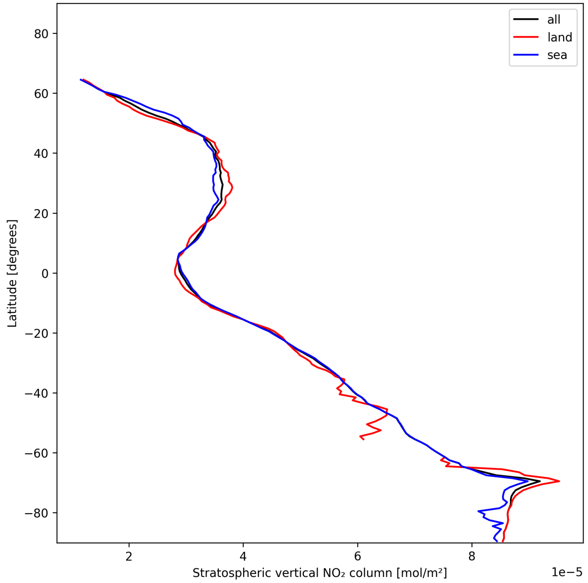
Figure 17: Zonal average of “Stratospheric vertical NO 2 column” for 2024-12-30 to 2024-12-30.
