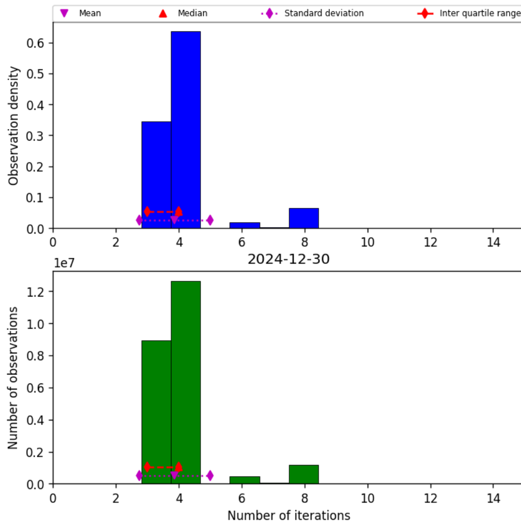
Figure 32: Histogram of “Number of iterations” for 2024-12-30 to 2024-12-30
