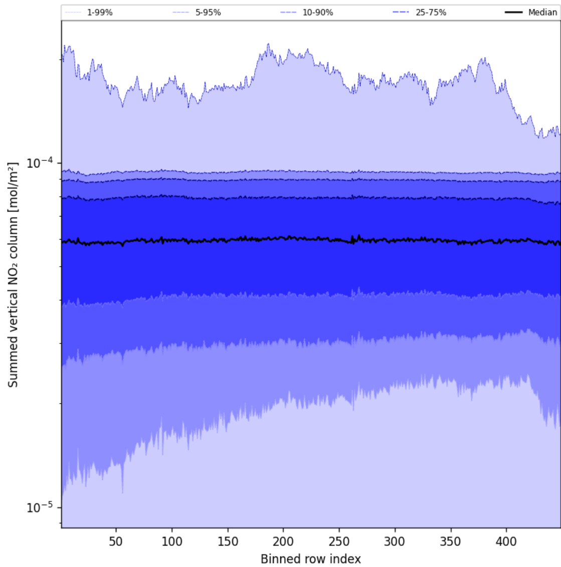
Figure 55: Along track statistics of “Summed vertical NO 2 column” for 2024-12-30 to 2024-12-30
