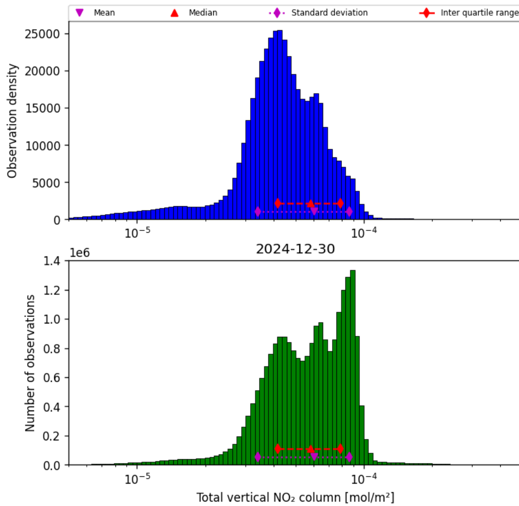
Figure 36: Histogram of “Total vertical NO 2 column” for 2024-12-30 to 2024-12-30
