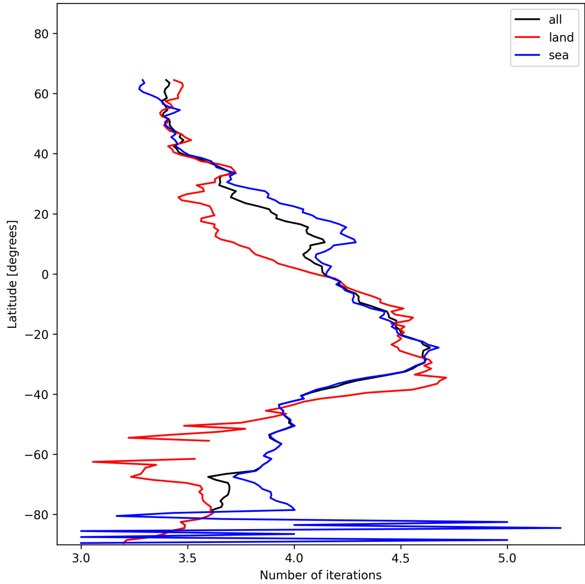
Figure 15: Zonal average of “Number of iterations” for 2024-12-30 to 2024-12-30.
