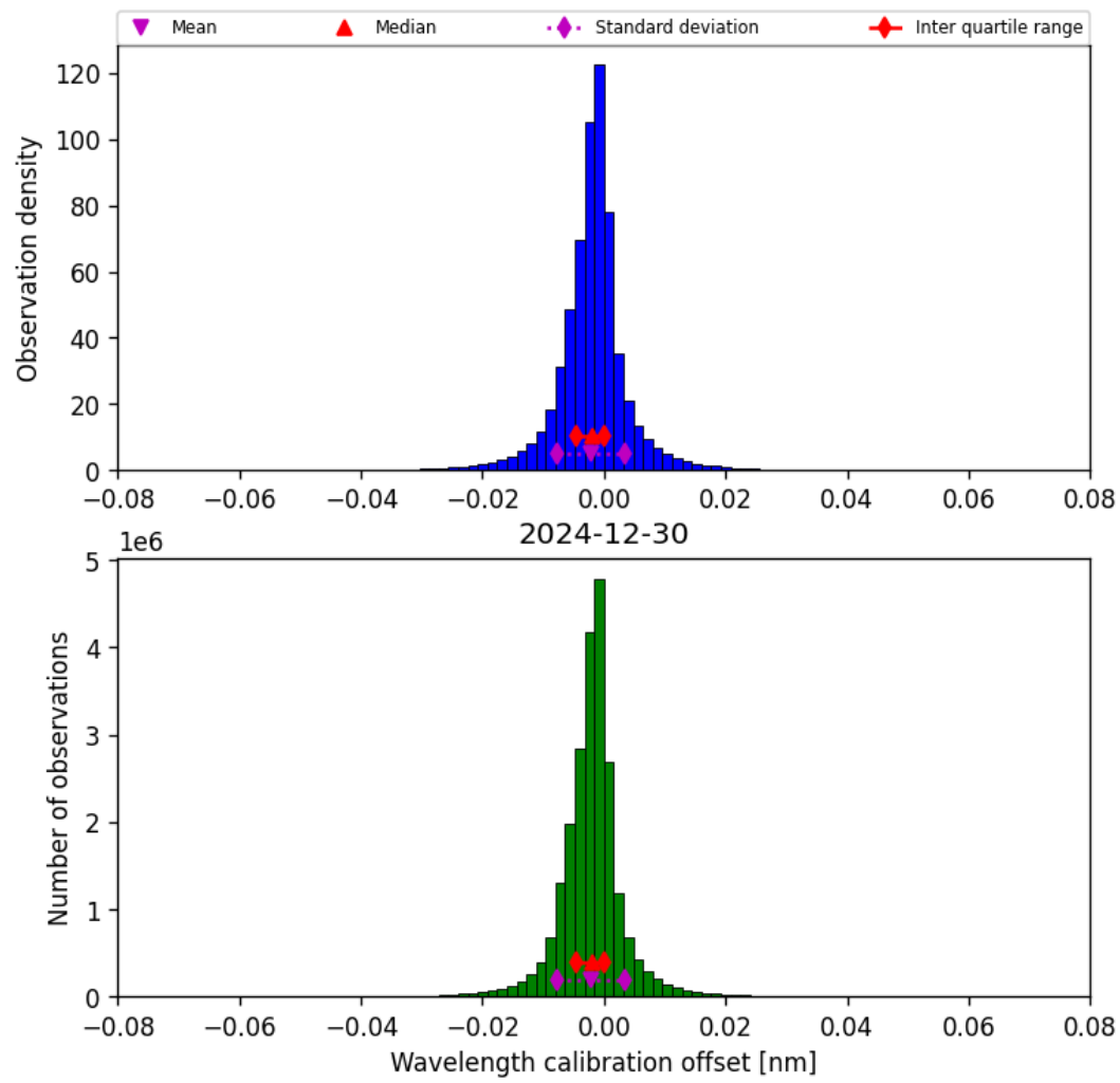
Figure 33: Histogram of “Wavelength calibration offset” for 2024-12-30 to 2024-12-30
