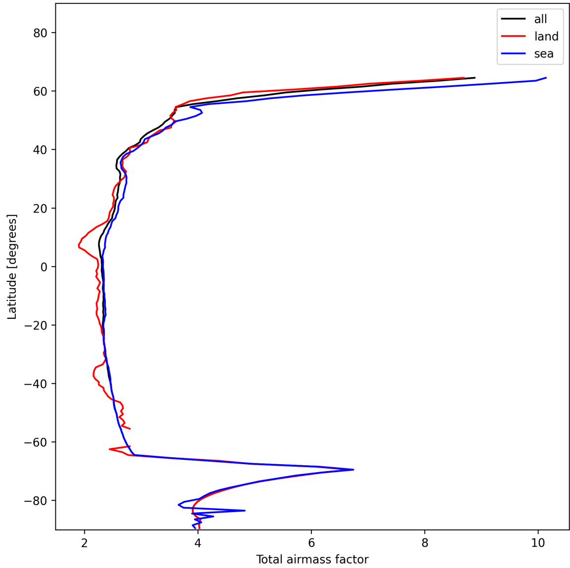
Figure 13: Zonal average of “Total airmass factor” for 2024-12-30 to 2024-12-30.
