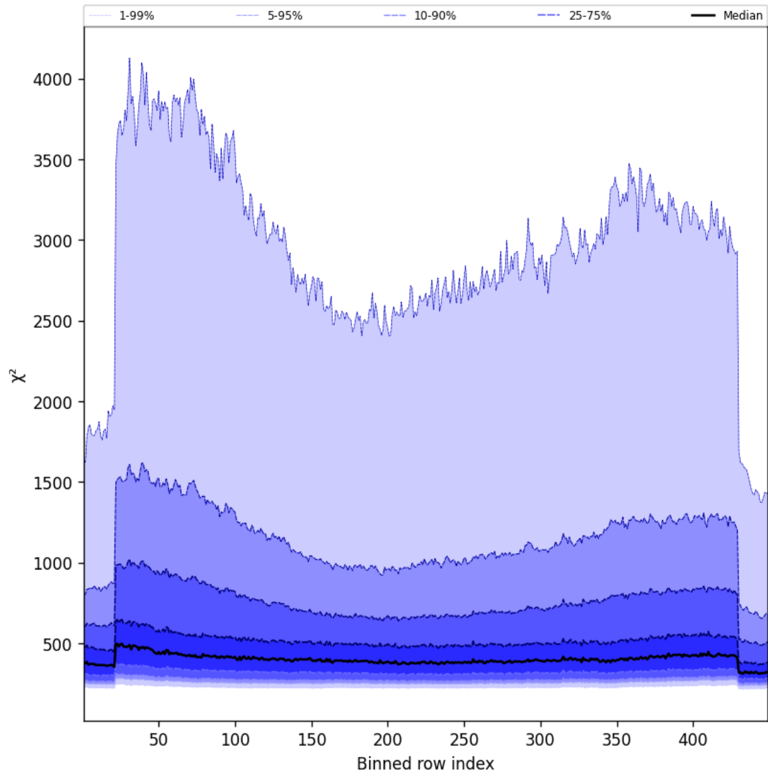
Figure 57: Along track statistics of “ \chi^2 ” for 2024-12-30 to 2024-12-30
