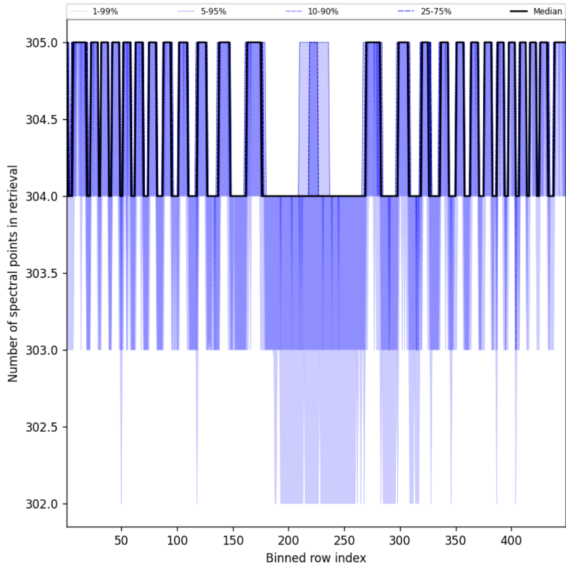
Figure 48: Along track statistics of “Number of spectral points in retrieval” for 2024-12-30 to 2024-12-30
