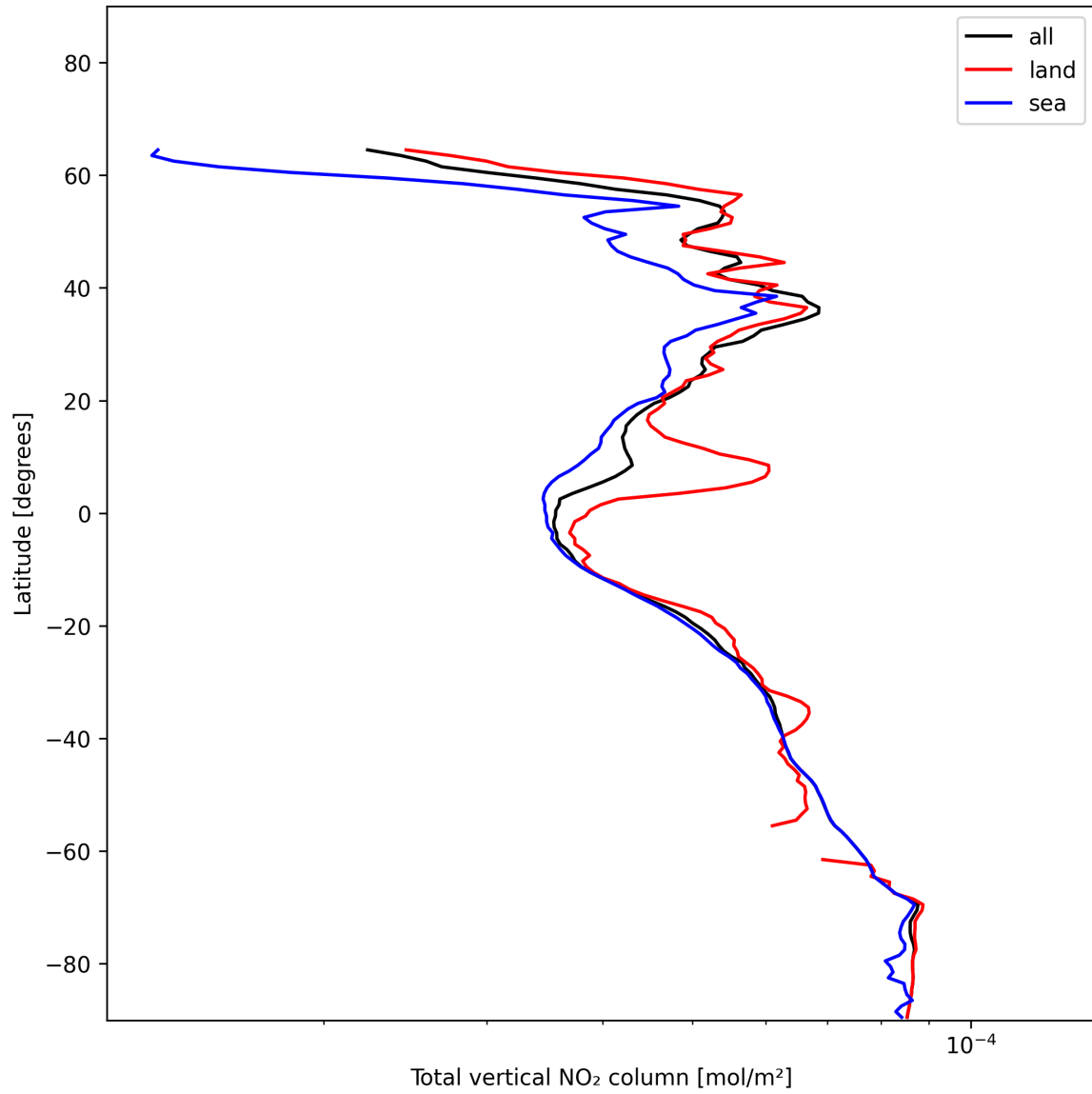
Figure 19: Zonal average of “Total vertical NO 2 column” for 2024-12-30 to 2024-12-30.
