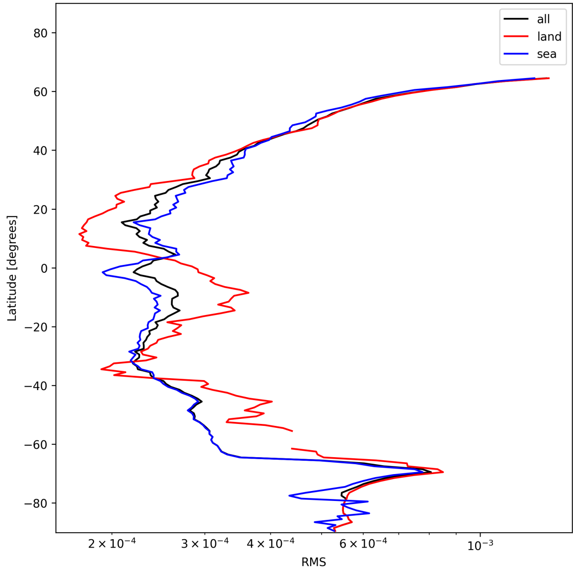
Figure 24: Zonal average of “RMS” for 2024-12-30 to 2024-12-30.
