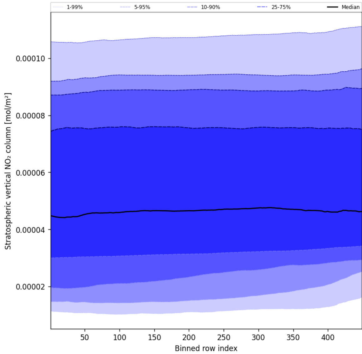
Figure 51: Along track statistics of “Stratospheric vertical NO 2 column” for 2024-12-30 to 2024-12-30
