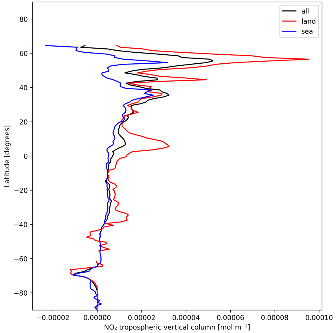
Figure 10: Zonal average of “NO 2 tropospheric vertical column” for 2024-12-30 to 2024-12-30.
