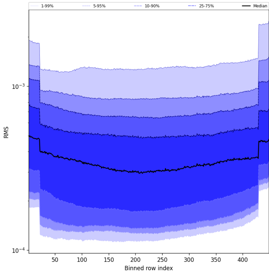
Figure 58: Along track statistics of “RMS” for 2024-12-30 to 2024-12-30
