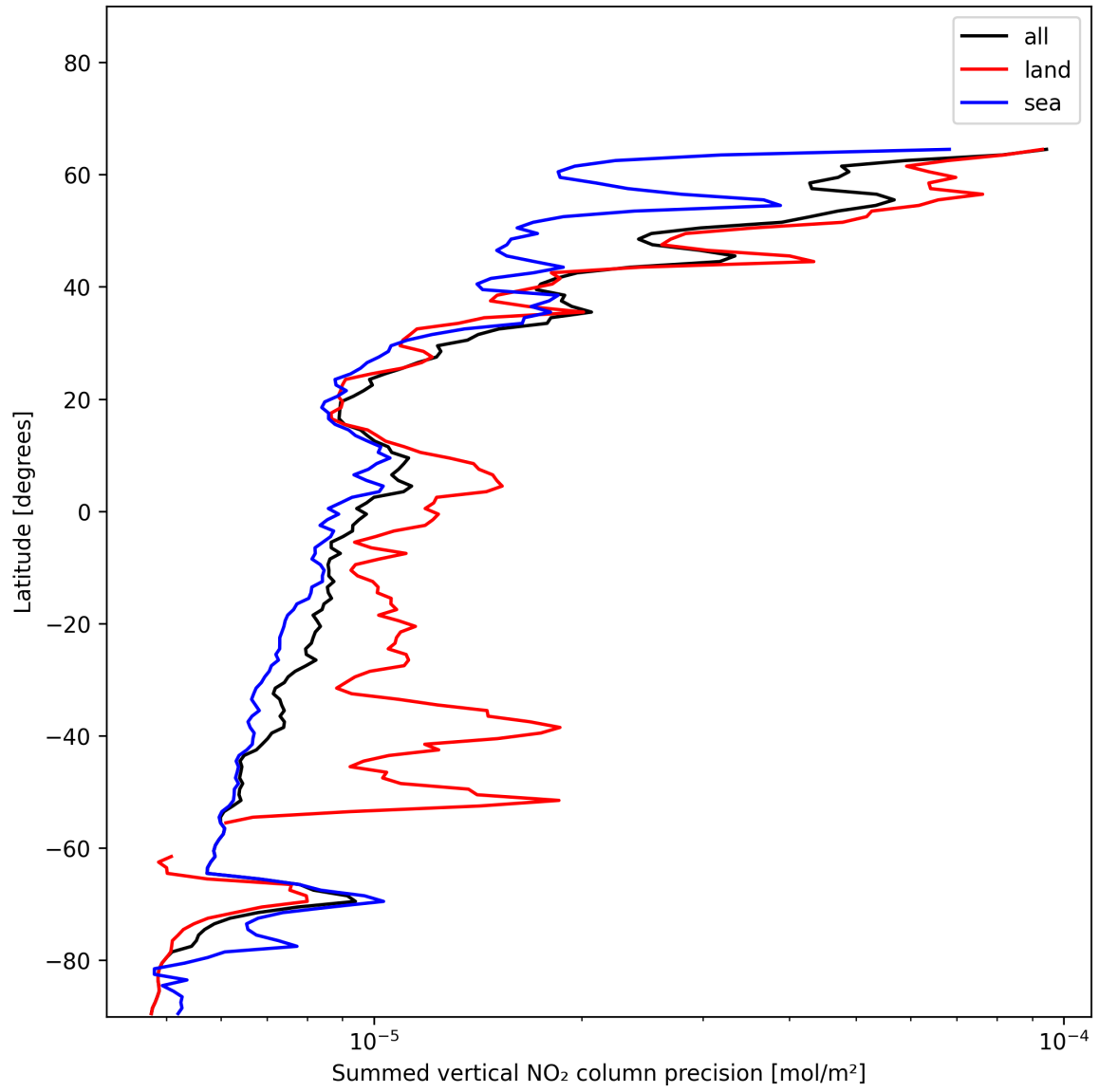
Figure 22: Zonal average of “Summed vertical NO 2 column precision” for 2024-12-30 to 2024-12-30.
