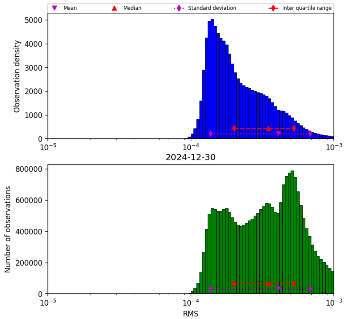
Figure 41: Histogram of “RMS” for 2024-12-30 to 2024-12-30
