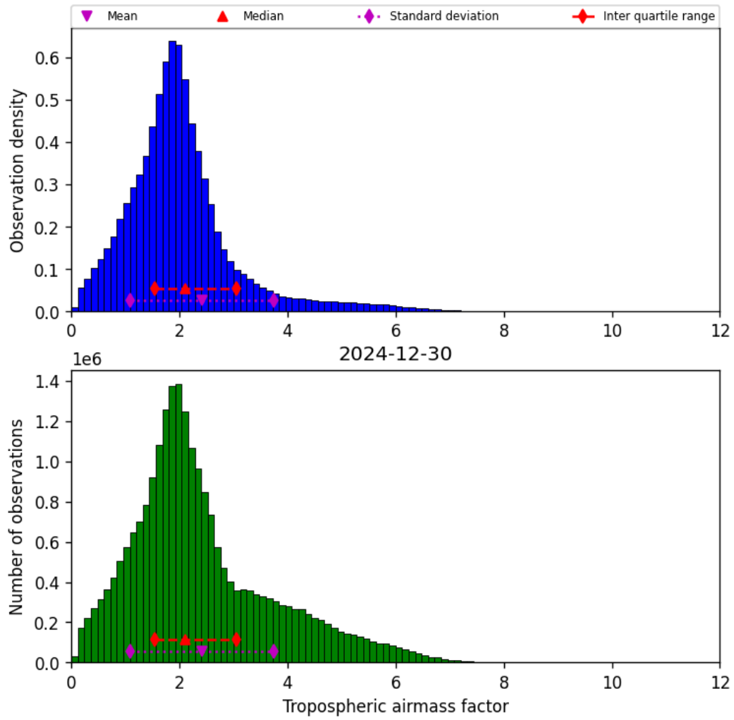
Figure 29: Histogram of “Tropospheric airmass factor” for 2024-12-30 to 2024-12-30
