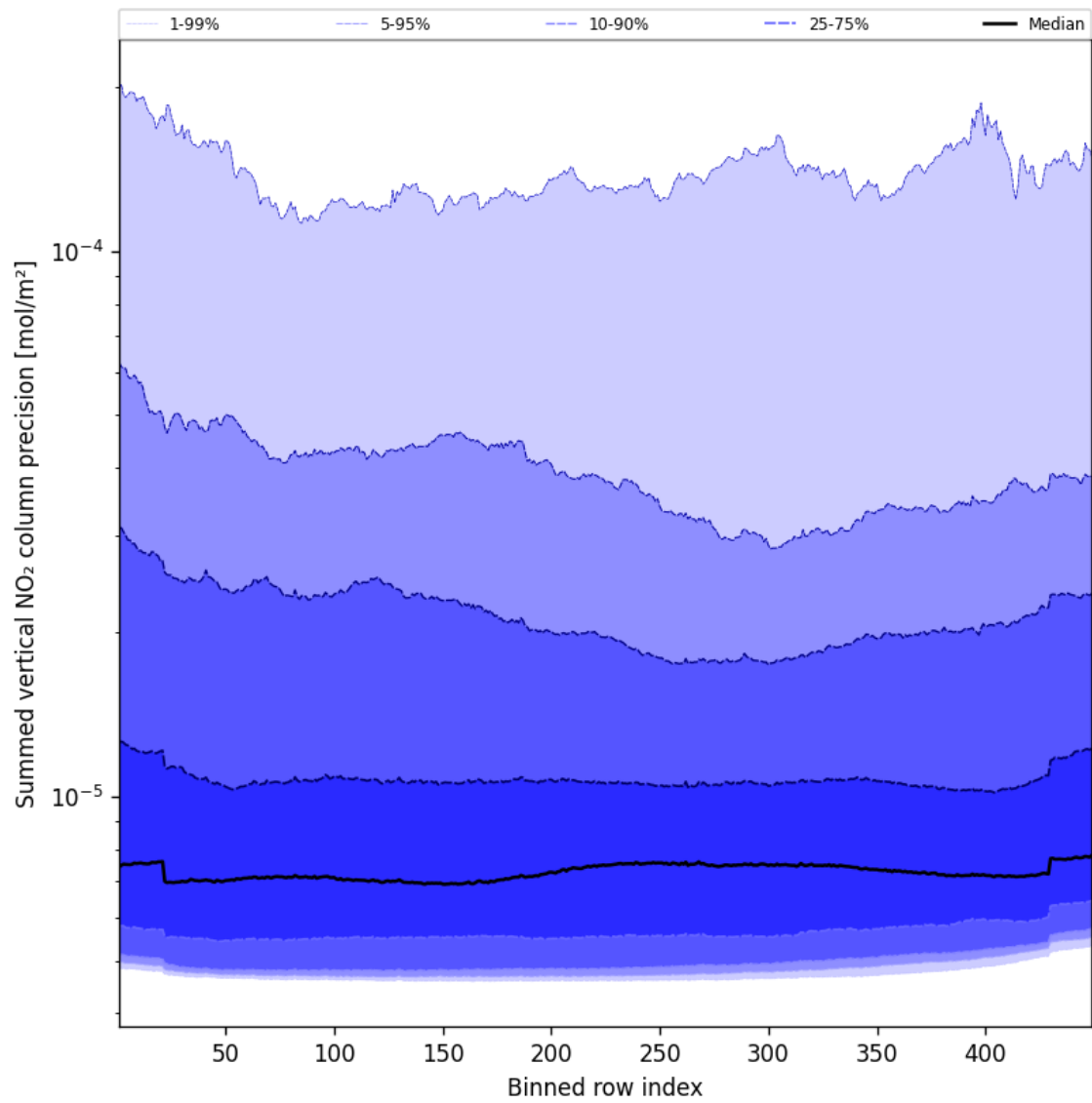
Figure 56: Along track statistics of “Summed vertical NO 2 column precision” for 2024-12-30 to 2024-12-30
