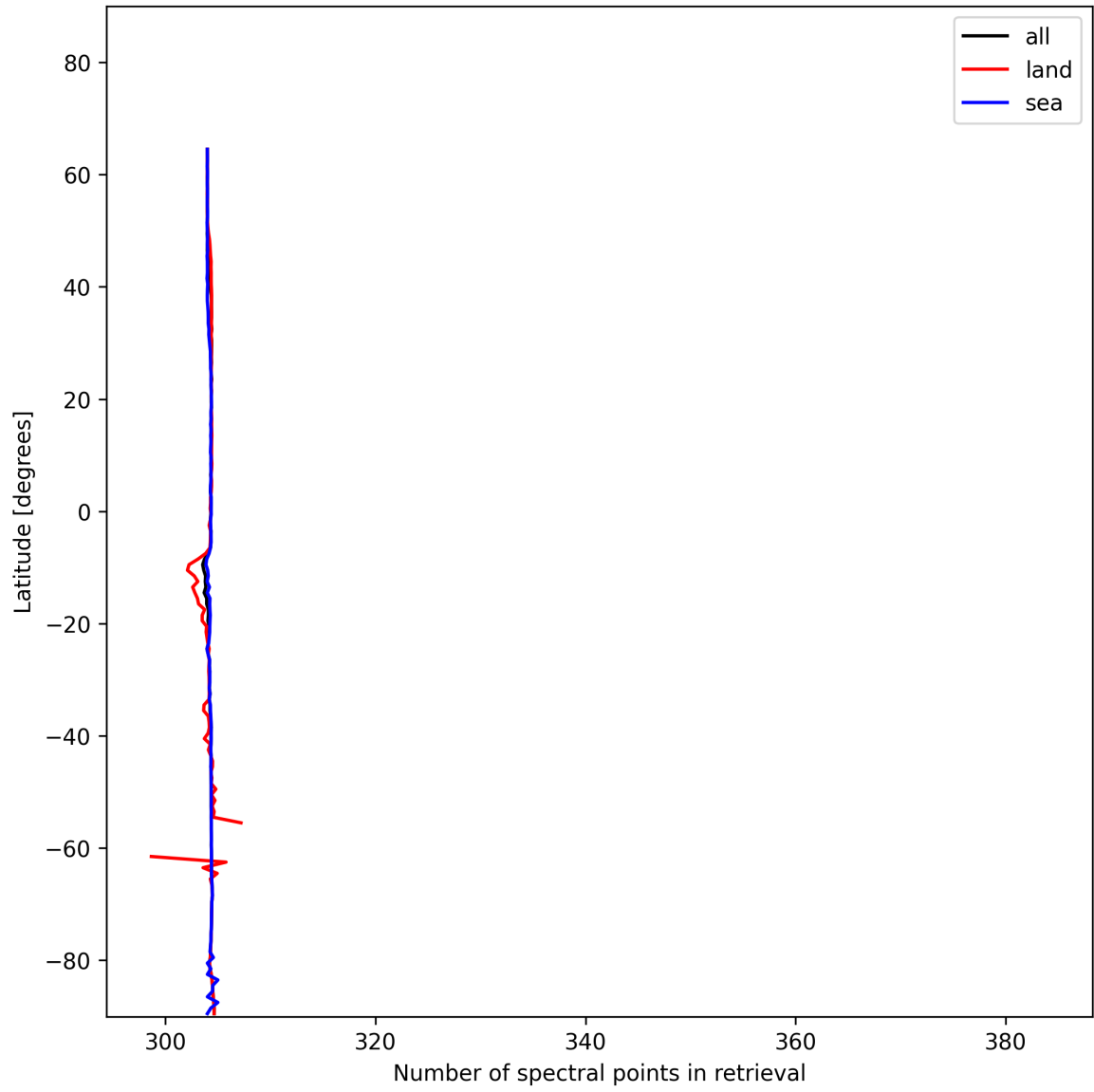
Figure 14: Zonal average of “Number of spectral points in retrieval” for 2024-12-30 to 2024-12-30.
