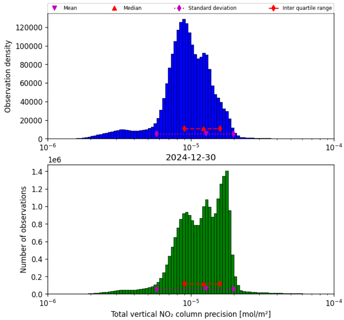
Figure 37: Histogram of “Total vertical NO 2 column precision” for 2024-12-30 to 2024-12-30
