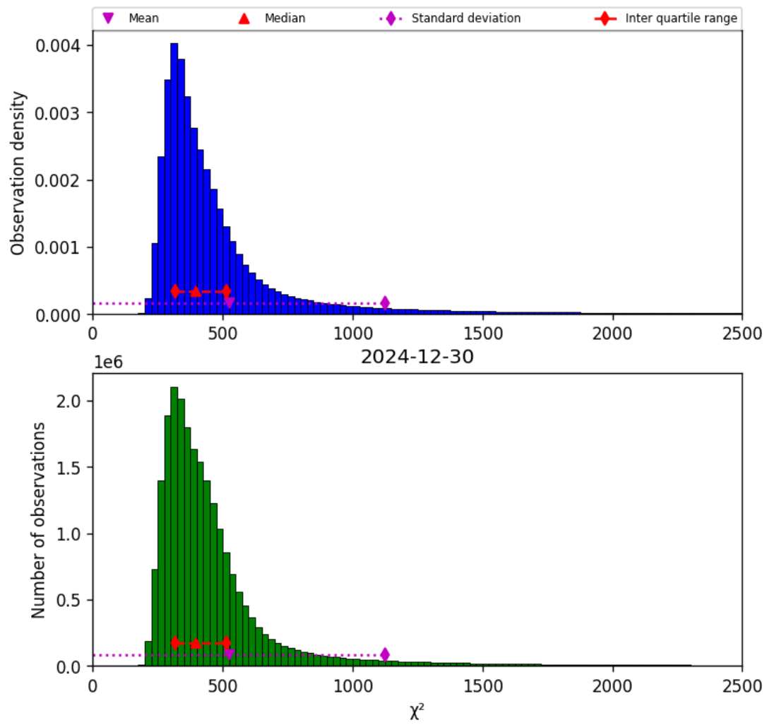
Figure 40: Histogram of " \chi^2 " for 2024-12-30 to 2024-12-30
