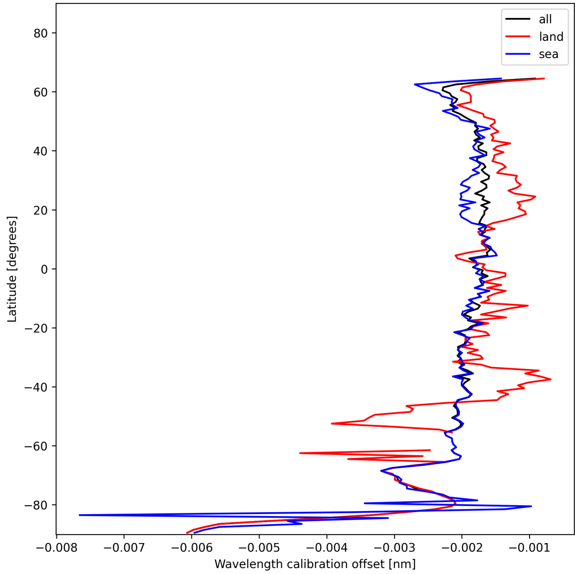
Figure 16: Zonal average of “Wavelength calibration offset” for 2024-12-30 to 2024-12-30.
