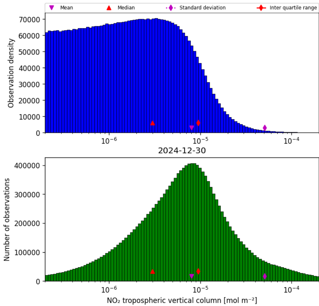
Figure 27: Histogram of “NO 2 tropospheric vertical column” for 2024-12-30 to 2024-12-30
