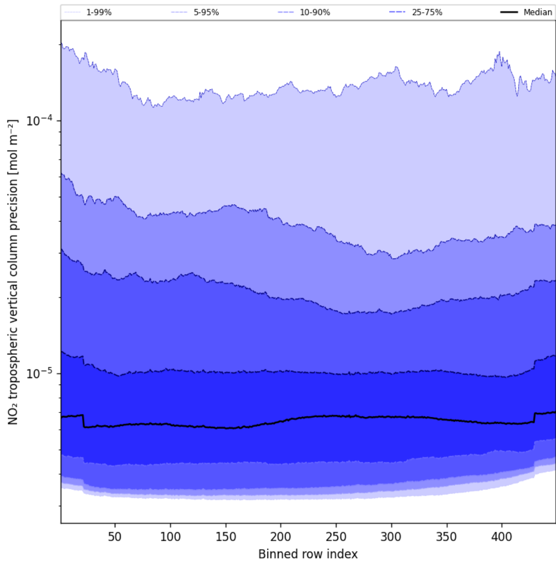
Figure 45: Along track statistics of “NO 2 tropospheric vertical column precision” for 2024-12-30 to 2024-12-30
