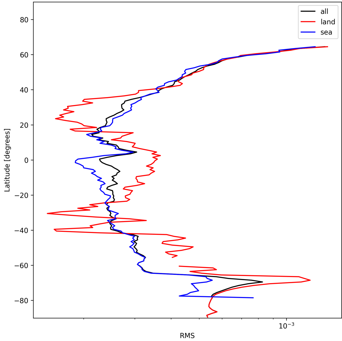
Figure 24: Zonal average of “RMS” for 2024-12-31 to 2024-12-31.
