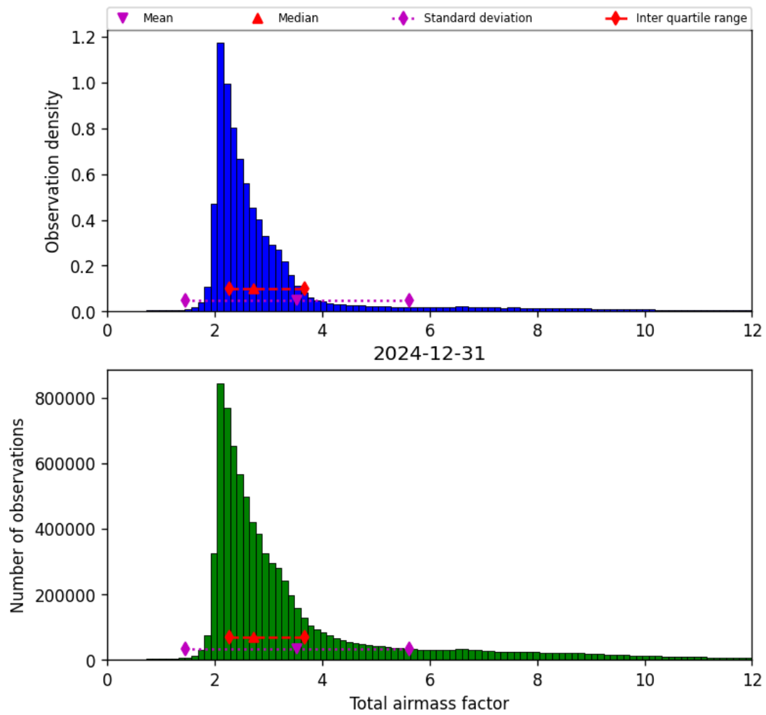
Figure 30: Histogram of “Total airmass factor” for 2024-12-31 to 2024-12-31
