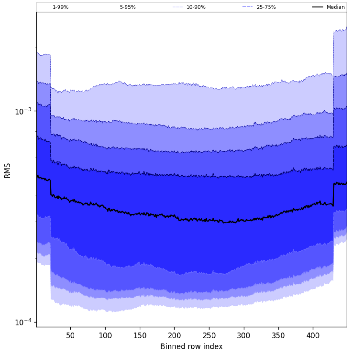
Figure 58: Along track statistics of “RMS” for 2024-12-31 to 2024-12-31
