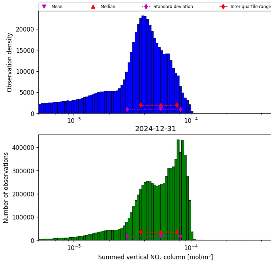
Figure 38: Histogram of “Summed vertical NO 2 column” for 2024-12-31 to 2024-12-31
