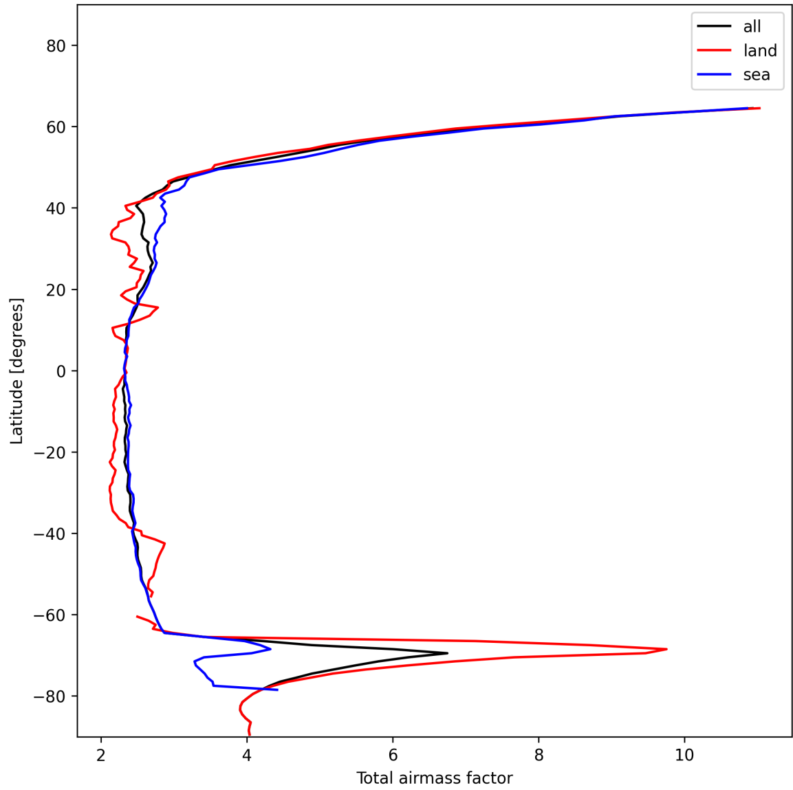
Figure 13: Zonal average of “Total airmass factor” for 2024-12-31 to 2024-12-31.
