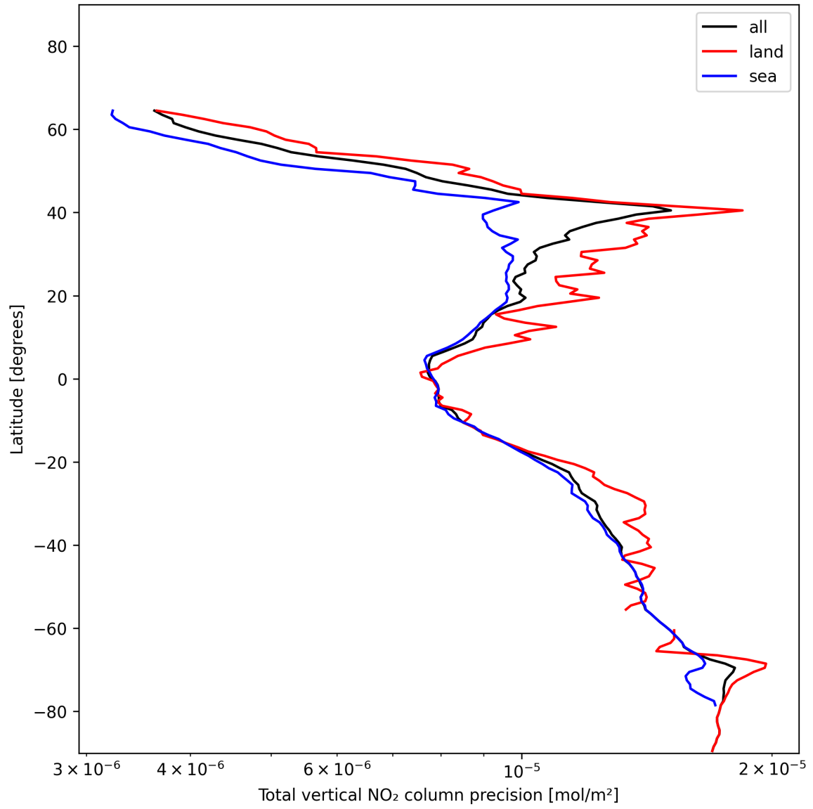
Figure 20: Zonal average of “Total vertical NO 2 column precision” for 2024-12-31 to 2024-12-31.
