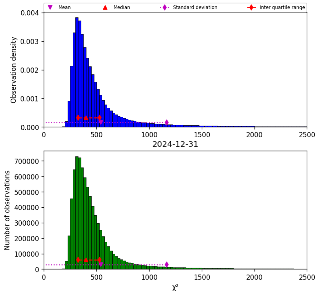
Figure 40: Histogram of " \chi^2 " for 2024-12-31 to 2024-12-31
