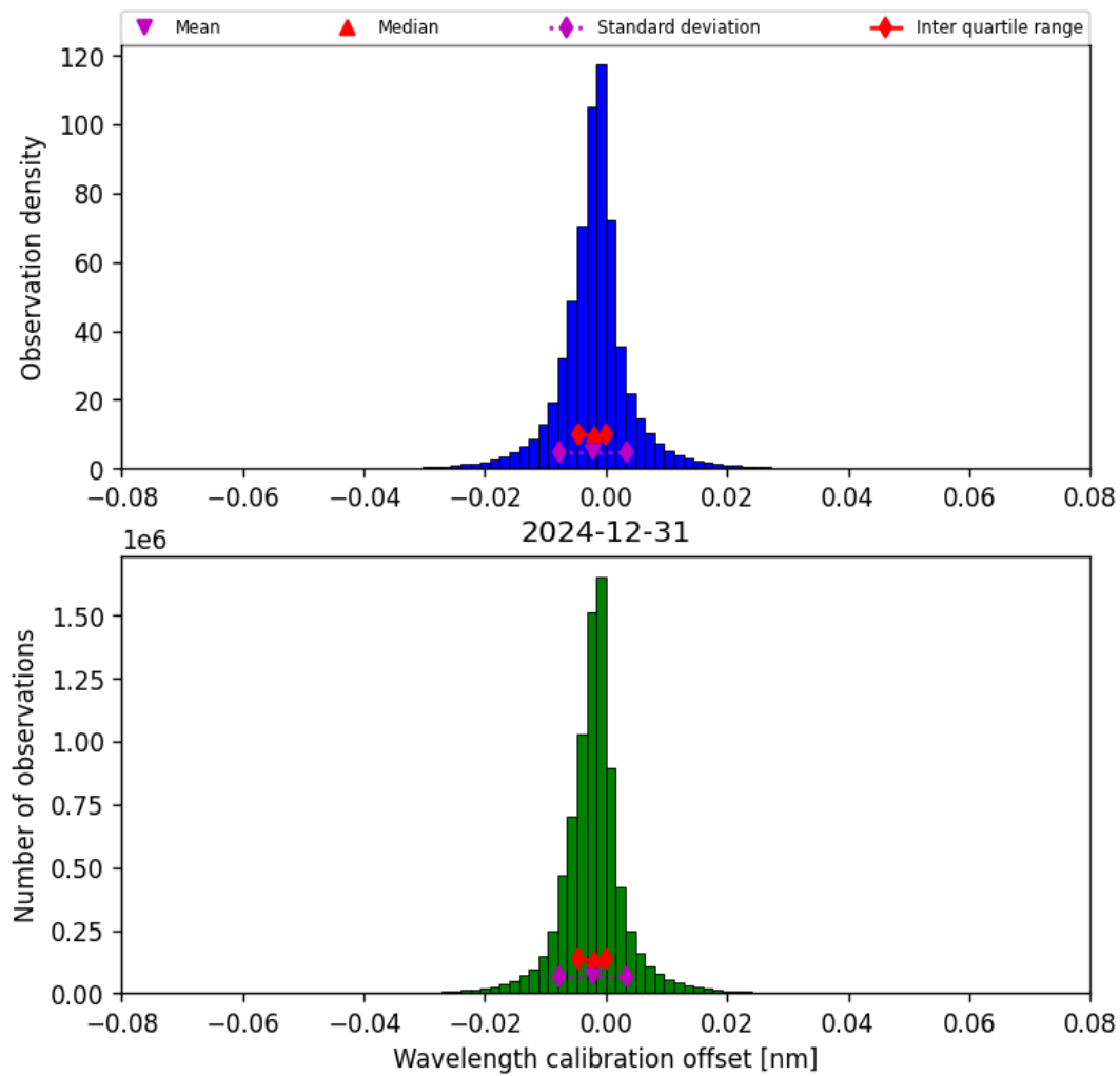
Figure 33: Histogram of “Wavelength calibration offset” for 2024-12-31 to 2024-12-31
