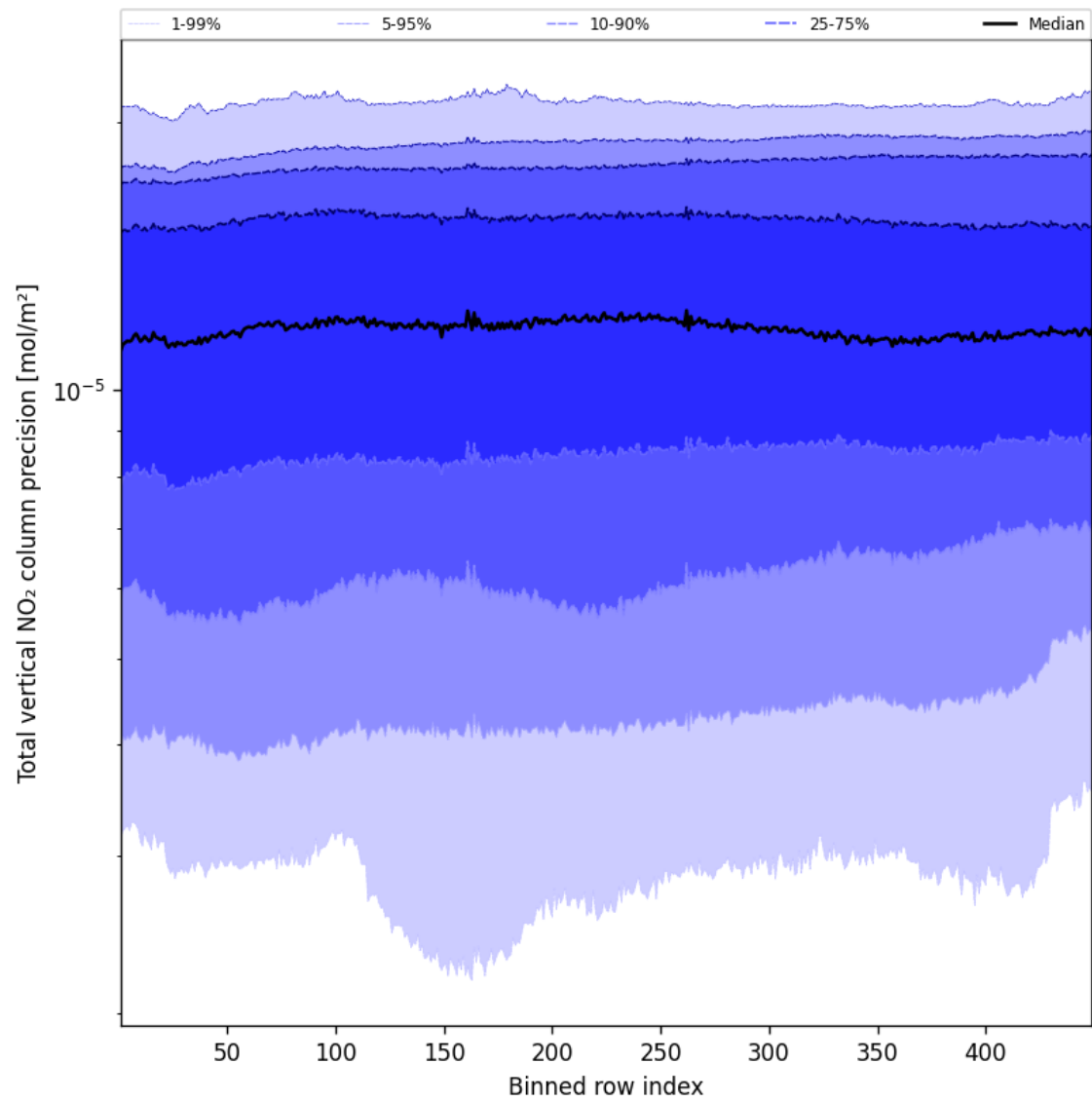
Figure 54: Along track statistics of “Total vertical NO 2 column precision” for 2024-12-31 to 2024-12-31
