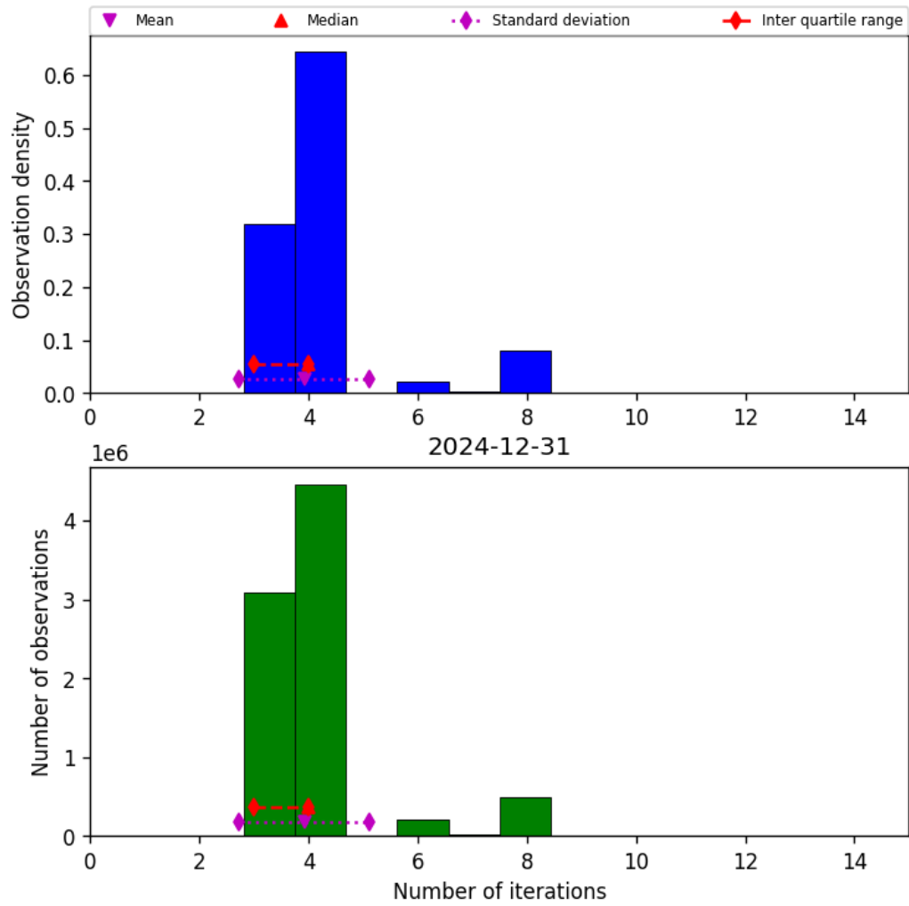
Figure 32: Histogram of “Number of iterations” for 2024-12-31 to 2024-12-31
