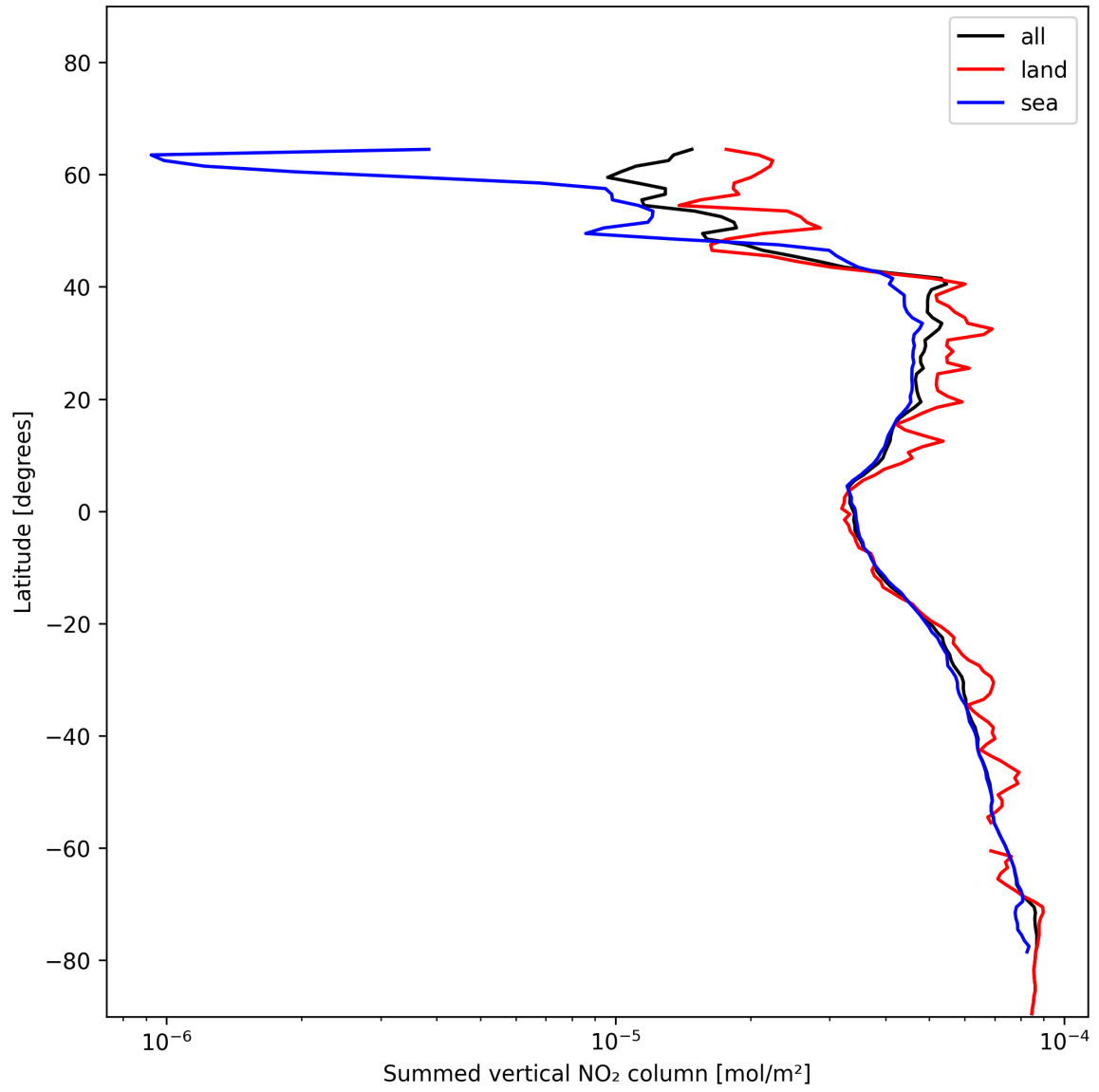
Figure 21: Zonal average of “Summed vertical NO 2 column” for 2024-12-31 to 2024-12-31.
