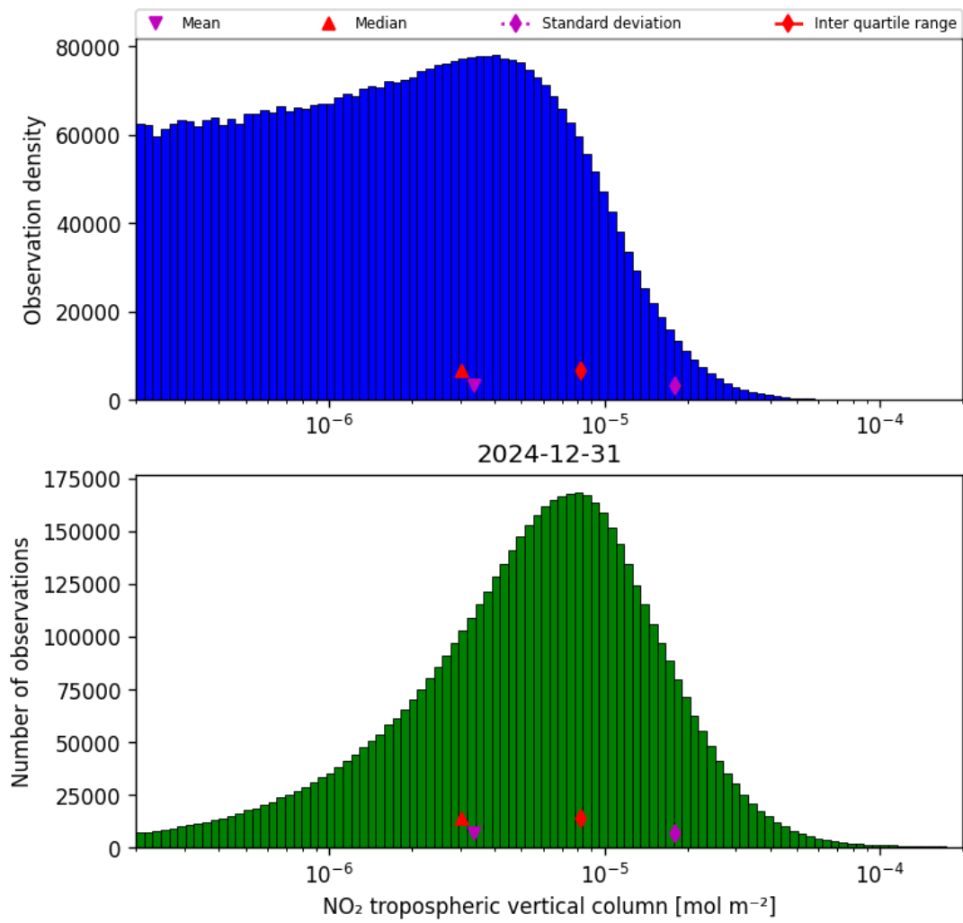
Figure 27: Histogram of “NO 2 tropospheric vertical column” for 2024-12-31 to 2024-12-31
