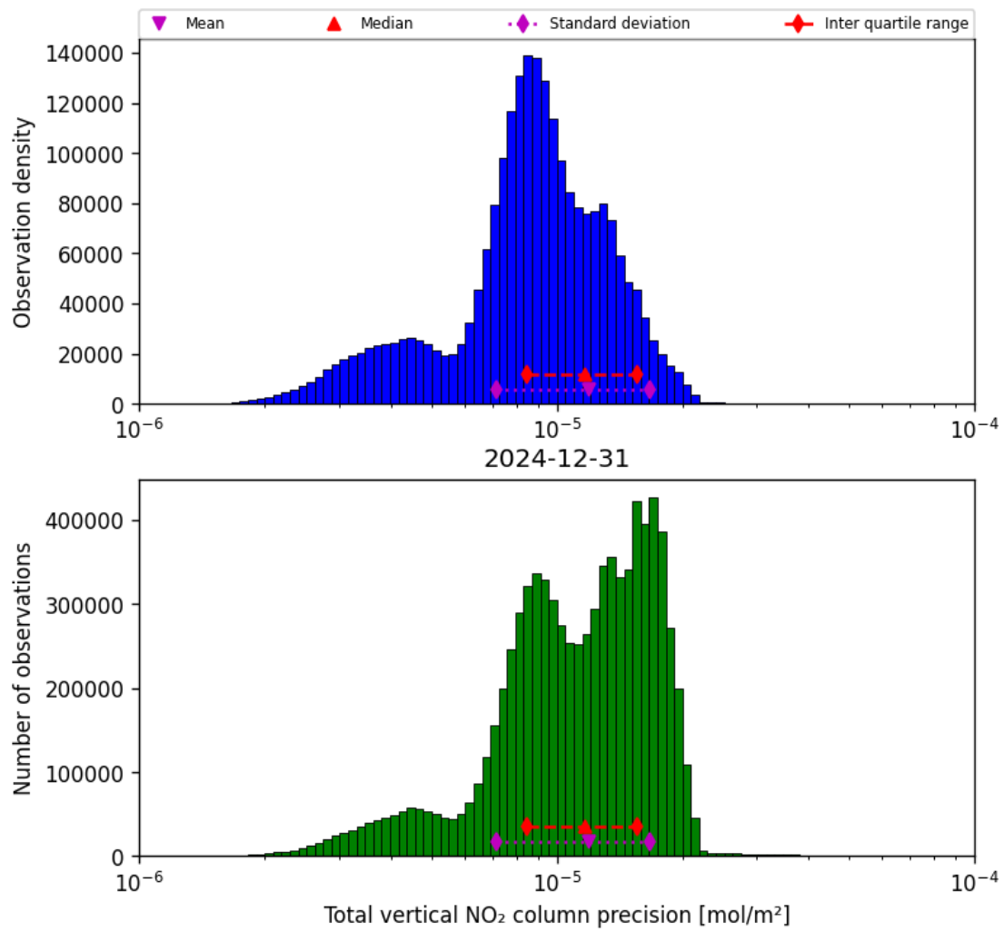
Figure 37: Histogram of “Total vertical NO 2 column precision” for 2024-12-31 to 2024-12-31
