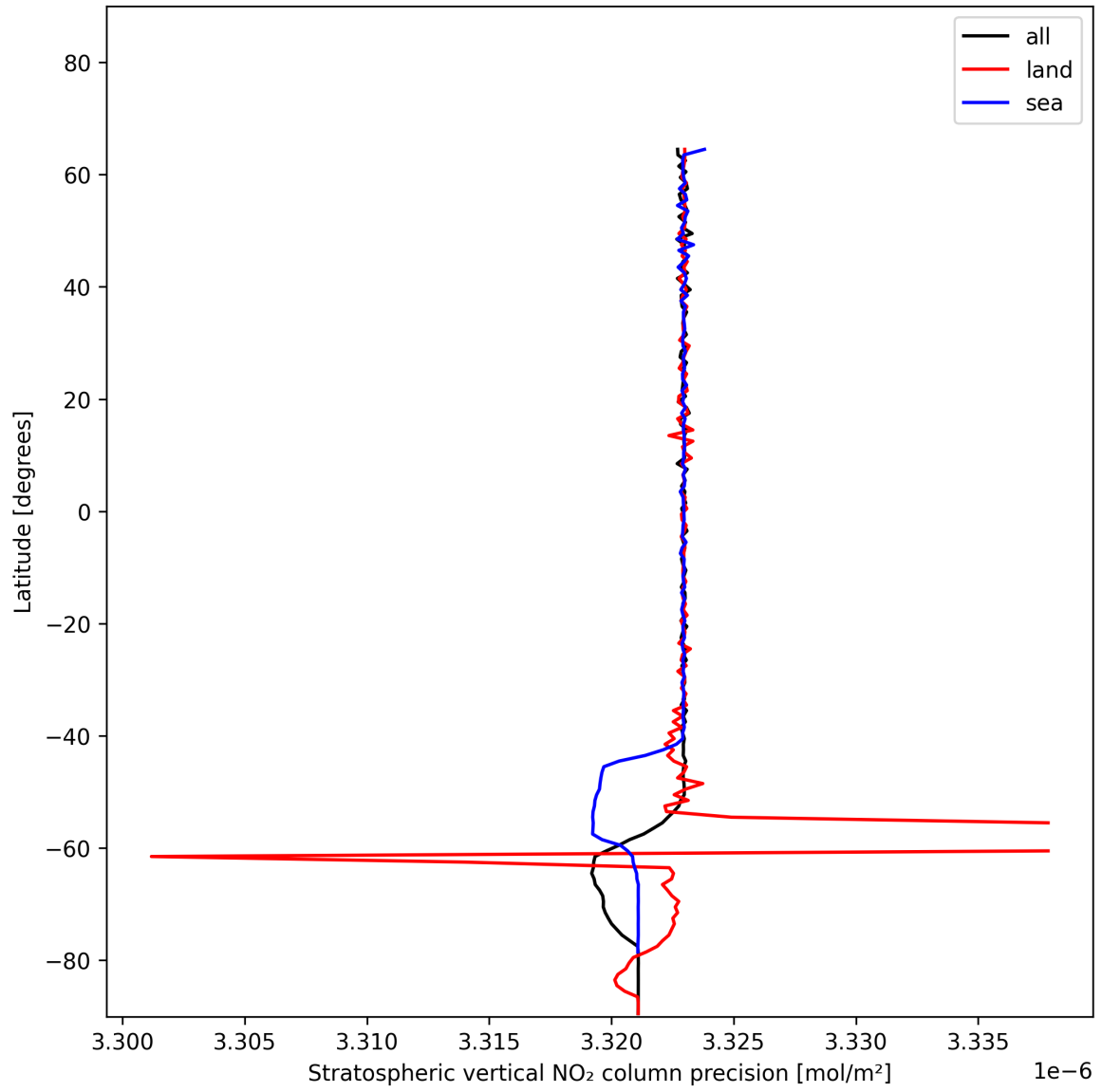
Figure 18: Zonal average of “Stratospheric vertical NO 2 column precision” for 2024-12-31 to 2024-12-31.
