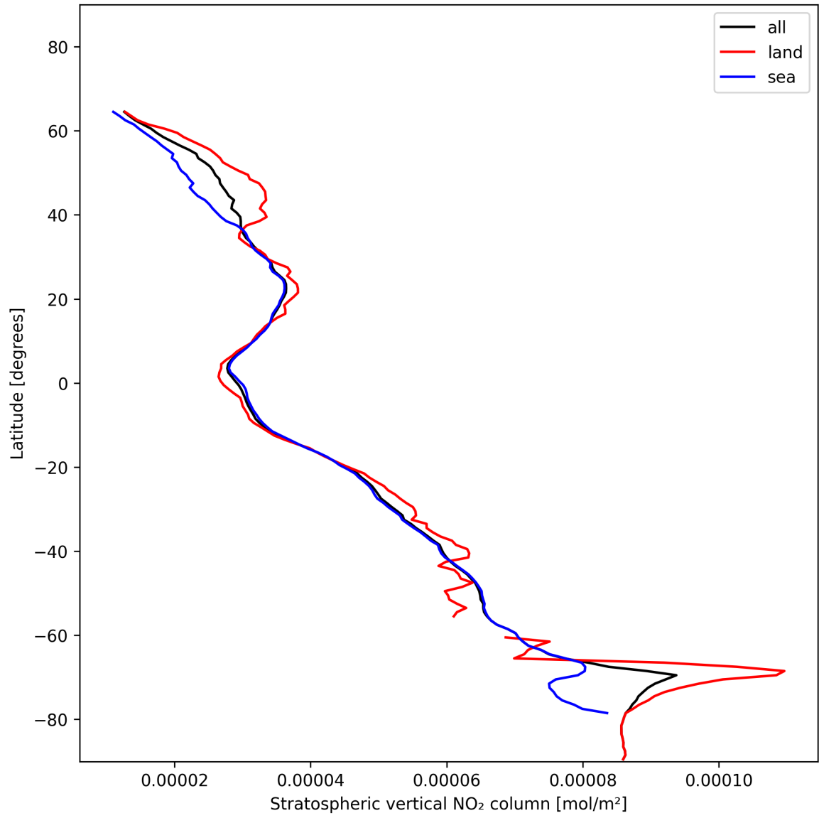
Figure 17: Zonal average of “Stratospheric vertical NO 2 column” for 2024-12-31 to 2024-12-31.
