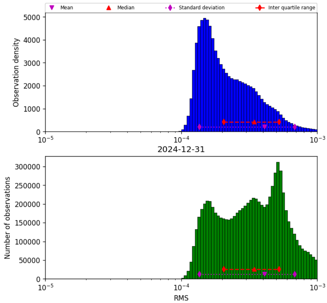
Figure 41: Histogram of “RMS” for 2024-12-31 to 2024-12-31
