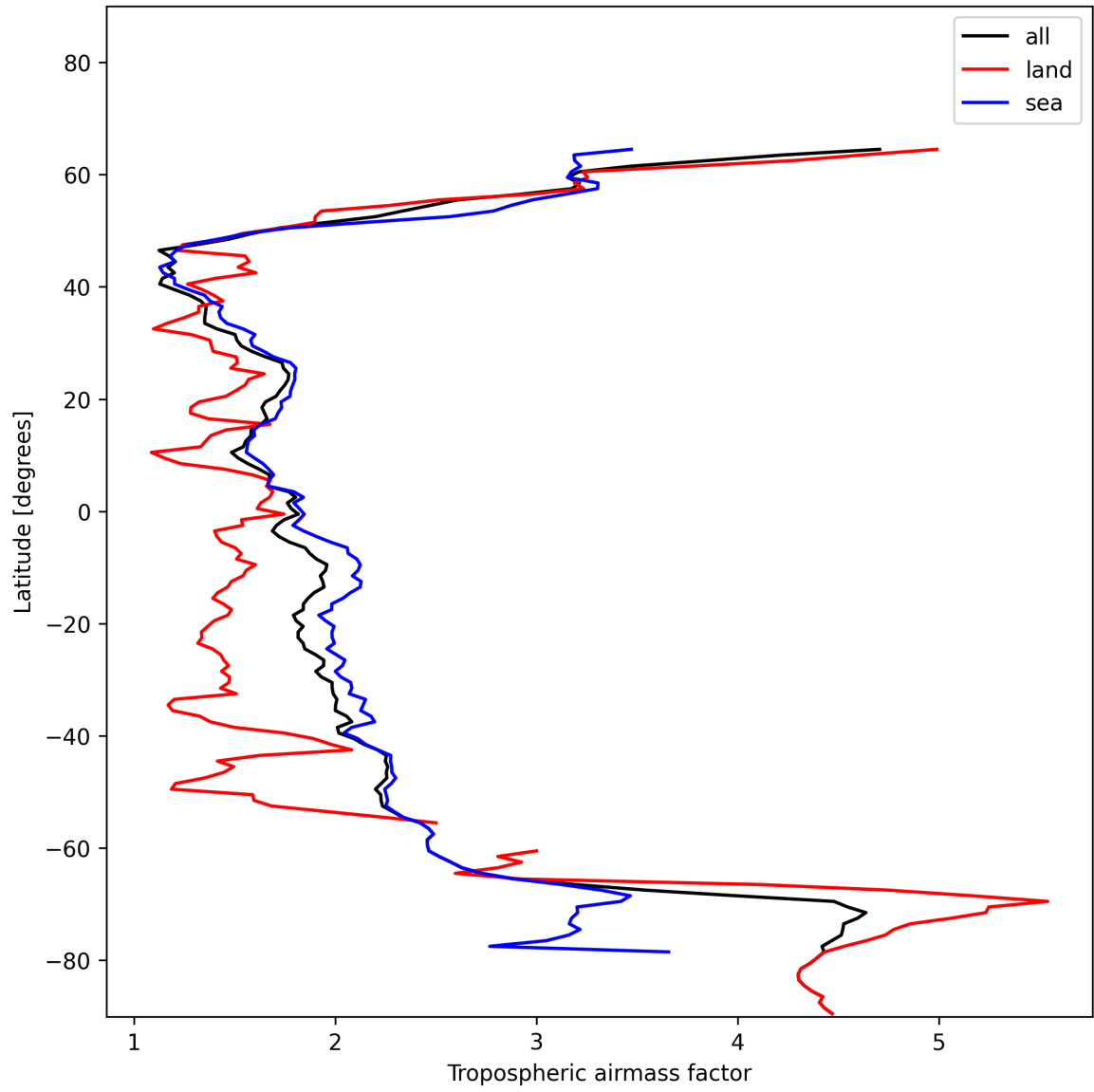
Figure 12: Zonal average of “Tropospheric airmass factor” for 2024-12-31 to 2024-12-31.
