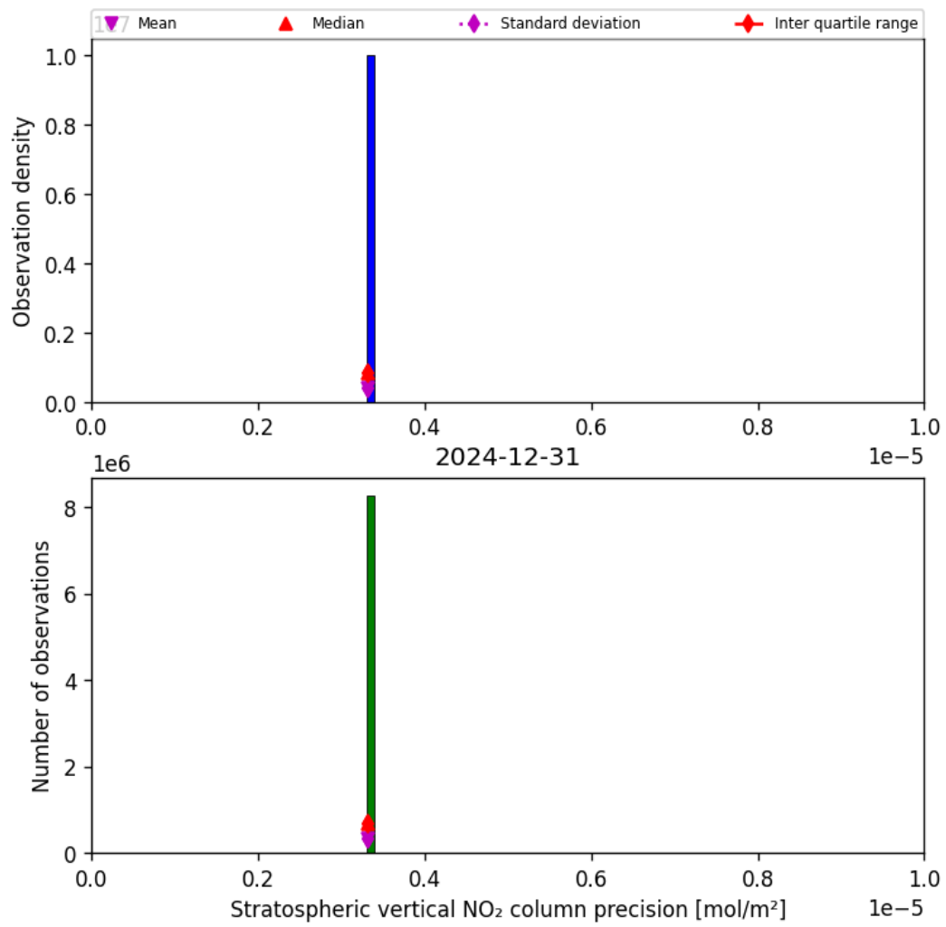
Figure 35: Histogram of “Stratospheric vertical NO 2 column precision” for 2024-12-31 to 2024-12-31
