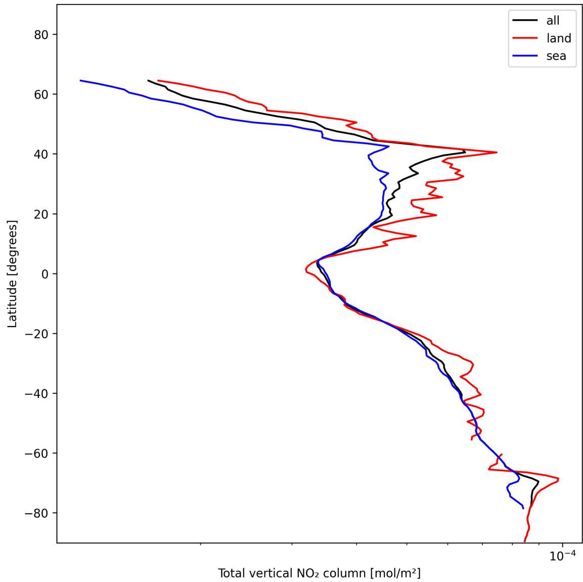
Figure 19: Zonal average of “Total vertical NO 2 column” for 2024-12-31 to 2024-12-31.
