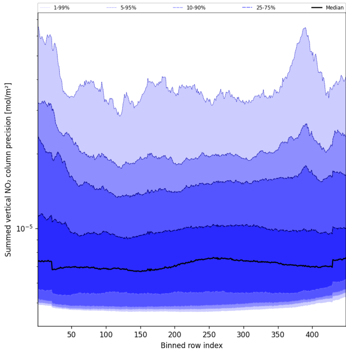
Figure 56: Along track statistics of “Summed vertical NO 2 column precision” for 2024-12-31 to 2024-12-31
