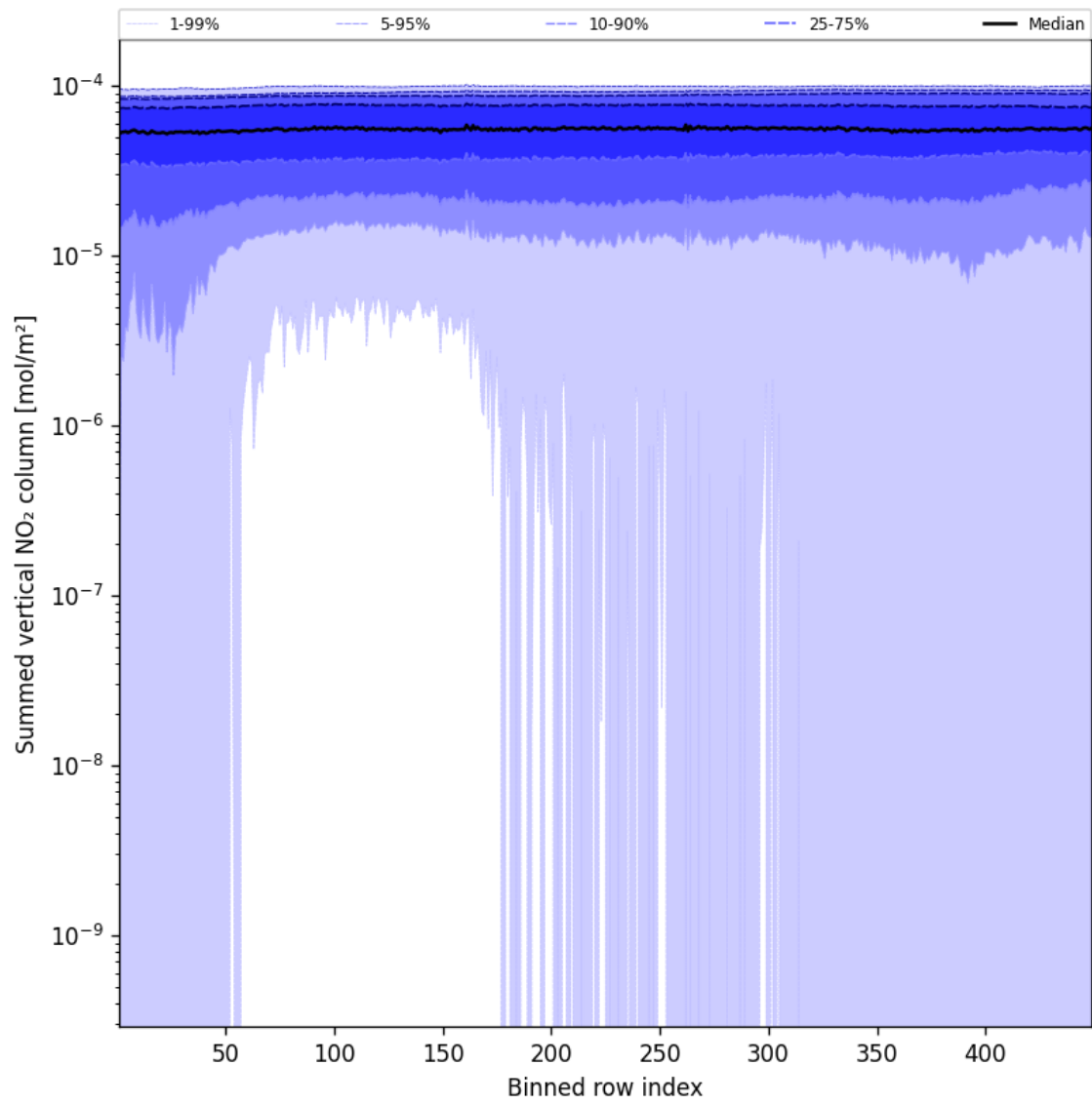
Figure 55: Along track statistics of “Summed vertical NO 2 column” for 2024-12-31 to 2024-12-31
