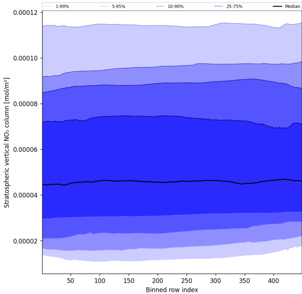
Figure 51: Along track statistics of “Stratospheric vertical NO 2 column” for 2024-12-31 to 2024-12-31
