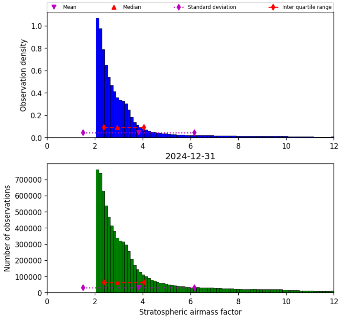
Figure 42: Histogram of “Stratospheric airmass factor” for 2024-12-31 to 2024-12-31
