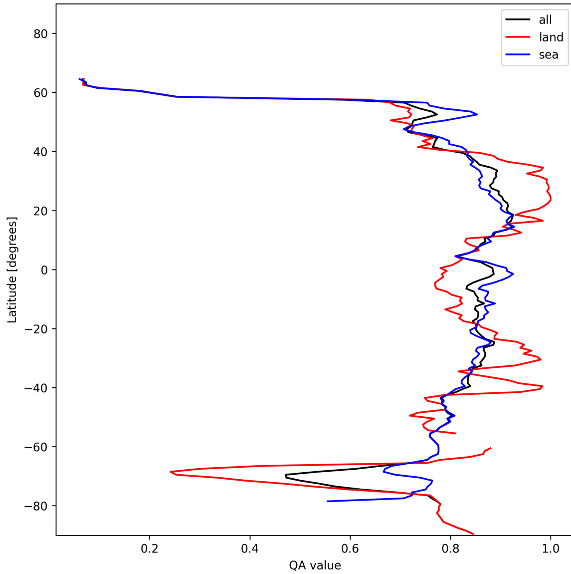
Figure 9: Zonal average of “QA value” for 2024-12-31 to 2024-12-31.
