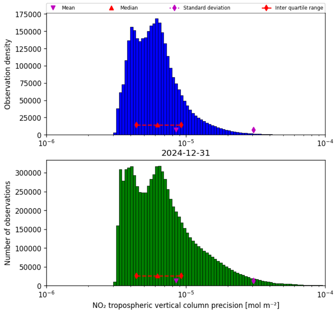
Figure 28: Histogram of “NO 2 tropospheric vertical column precision” for 2024-12-31 to 2024-12-31
