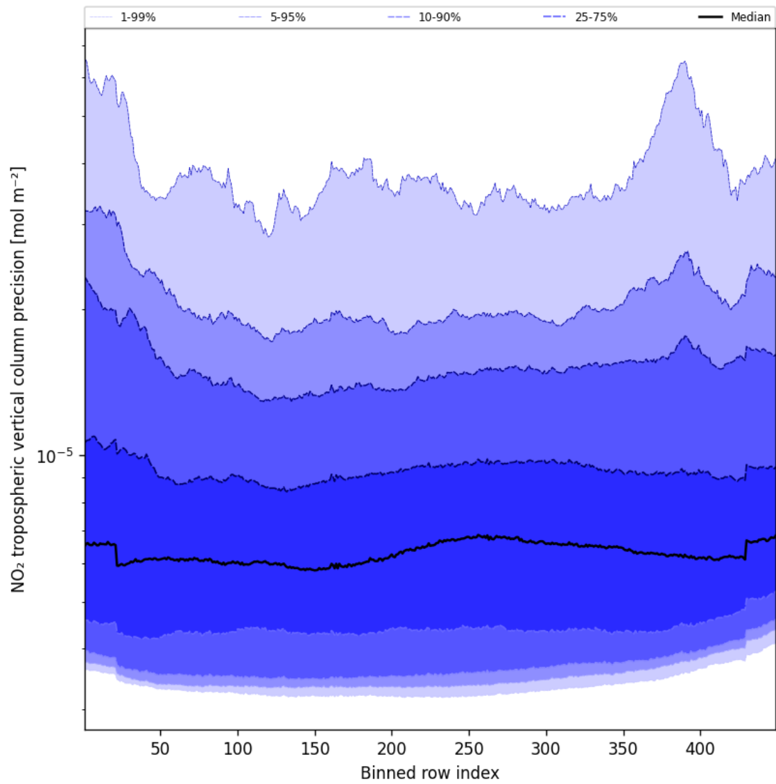
Figure 45: Along track statistics of “NO 2 tropospheric vertical column precision” for 2024-12-31 to 2024-12-31
