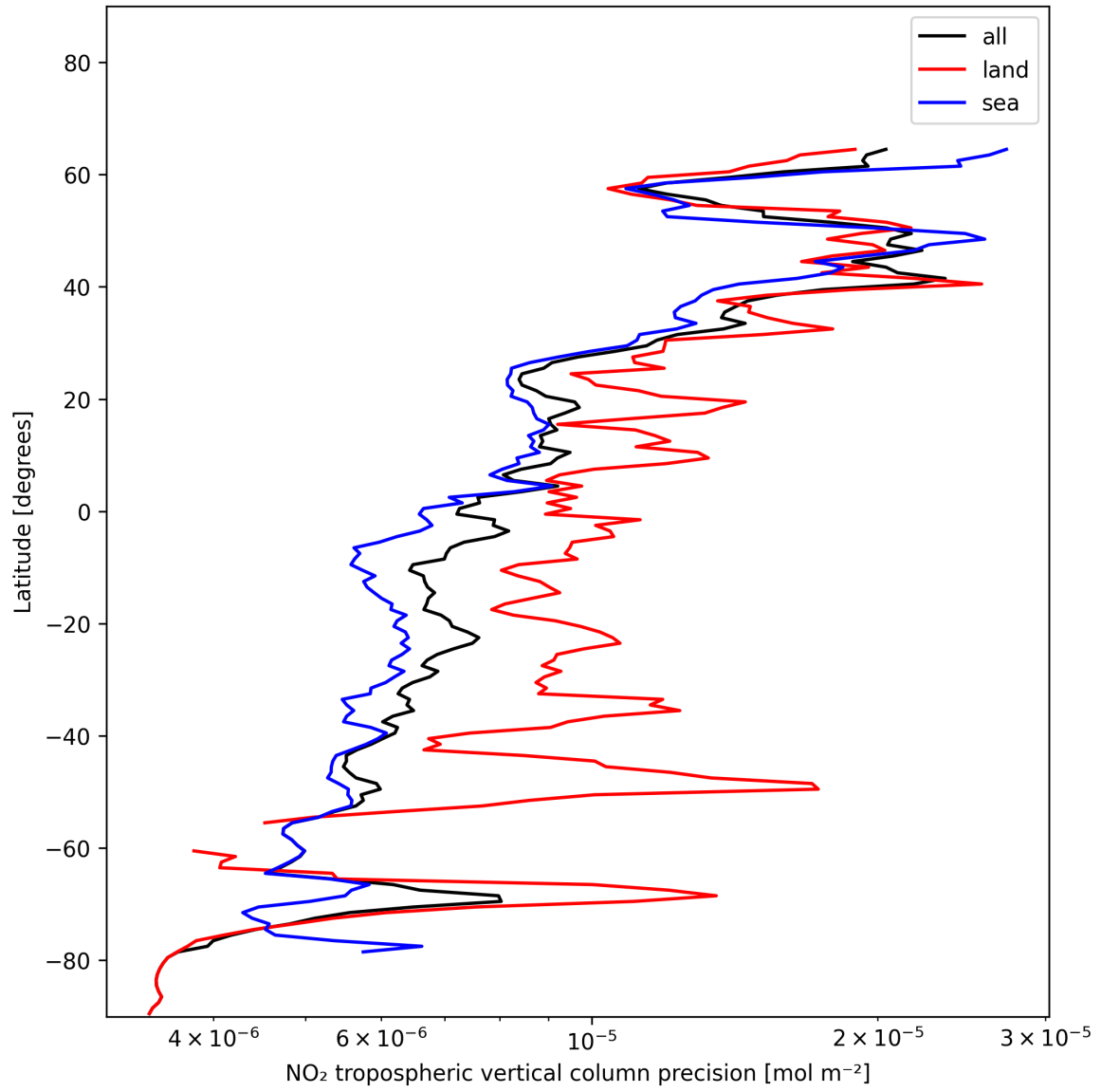
Figure 11: Zonal average of “NO 2 tropospheric vertical column precision” for 2024-12-31 to 2024-12-31.
