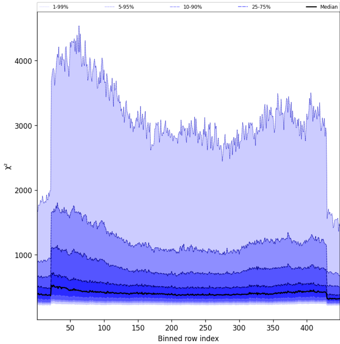
Figure 57: Along track statistics of “ \chi^2 ” for 2024-12-31 to 2024-12-31
