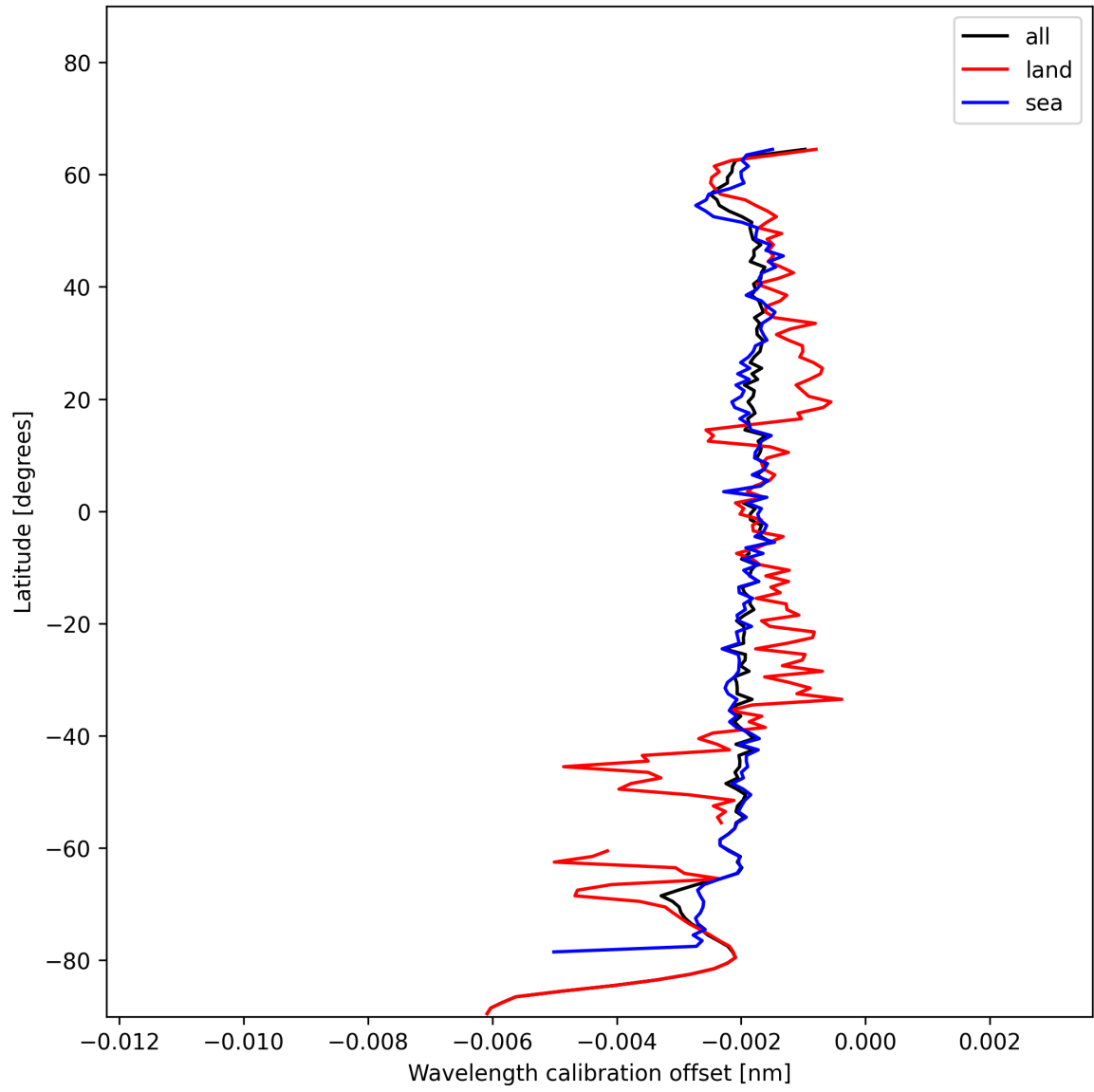
Figure 16: Zonal average of “Wavelength calibration offset” for 2024-12-31 to 2024-12-31.
