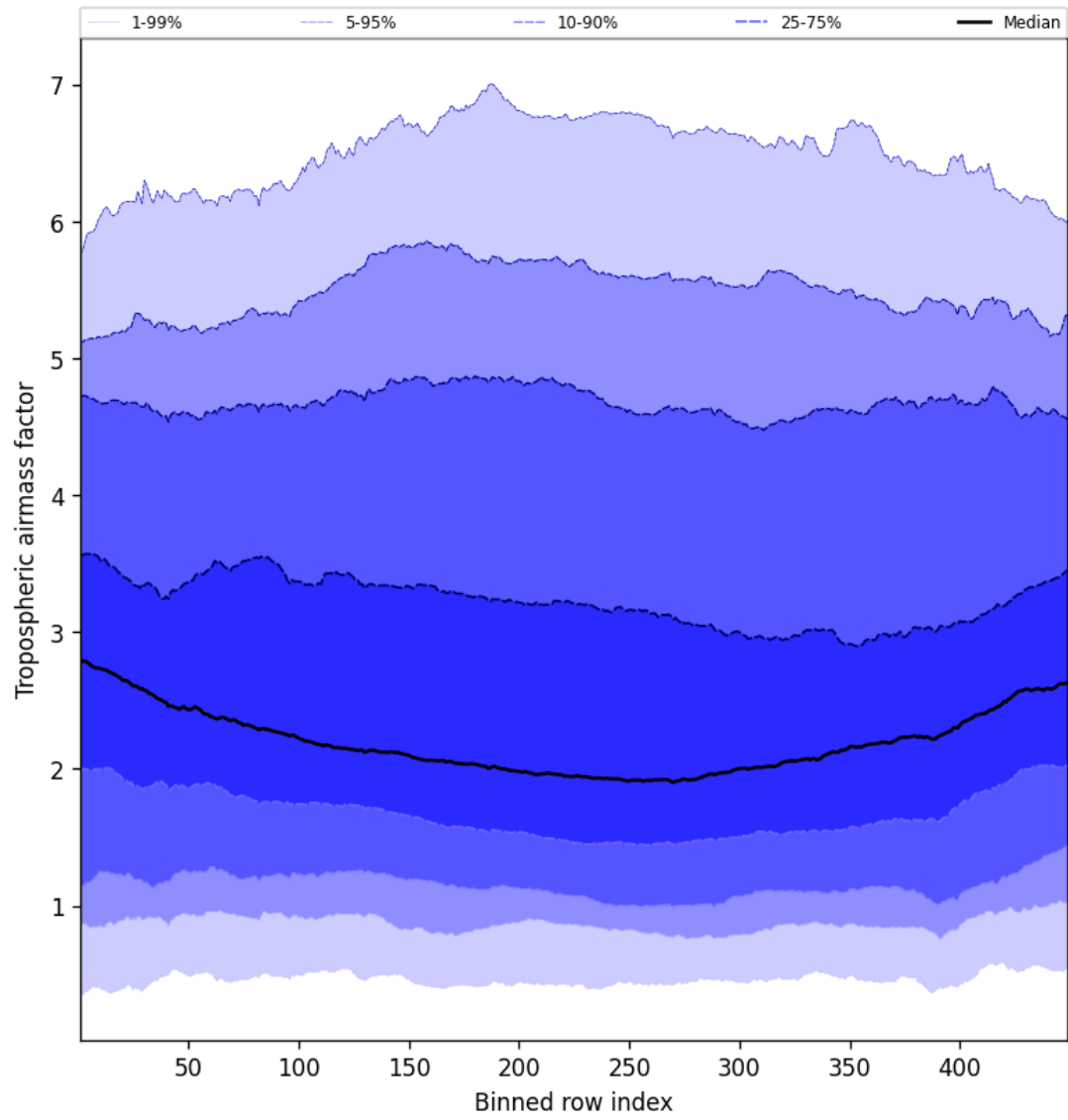
Figure 46: Along track statistics of “Tropospheric airmass factor” for 2024-12-31 to 2024-12-31
