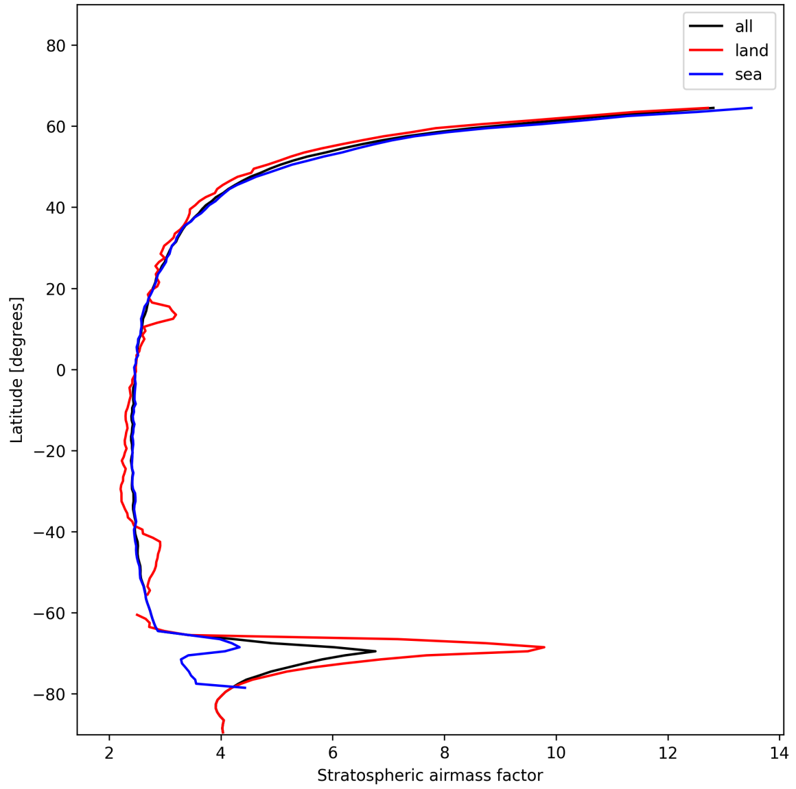
Figure 25: Zonal average of “Stratospheric airmass factor” for 2024-12-31 to 2024-12-31.
