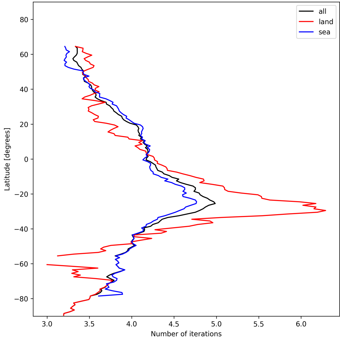
Figure 15: Zonal average of “Number of iterations” for 2024-12-31 to 2024-12-31.
