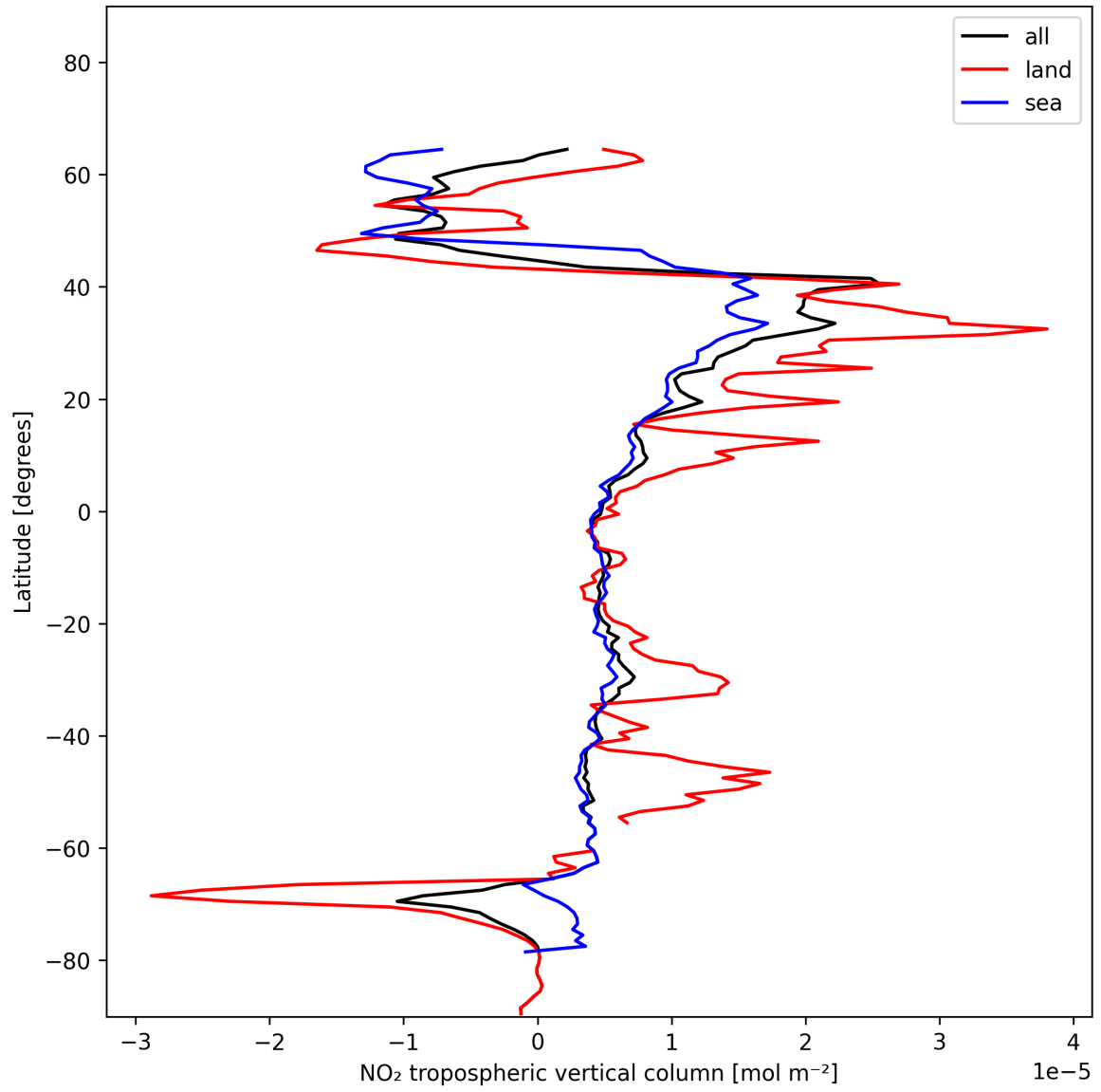
Figure 10: Zonal average of “NO 2 tropospheric vertical column” for 2024-12-31 to 2024-12-31.
