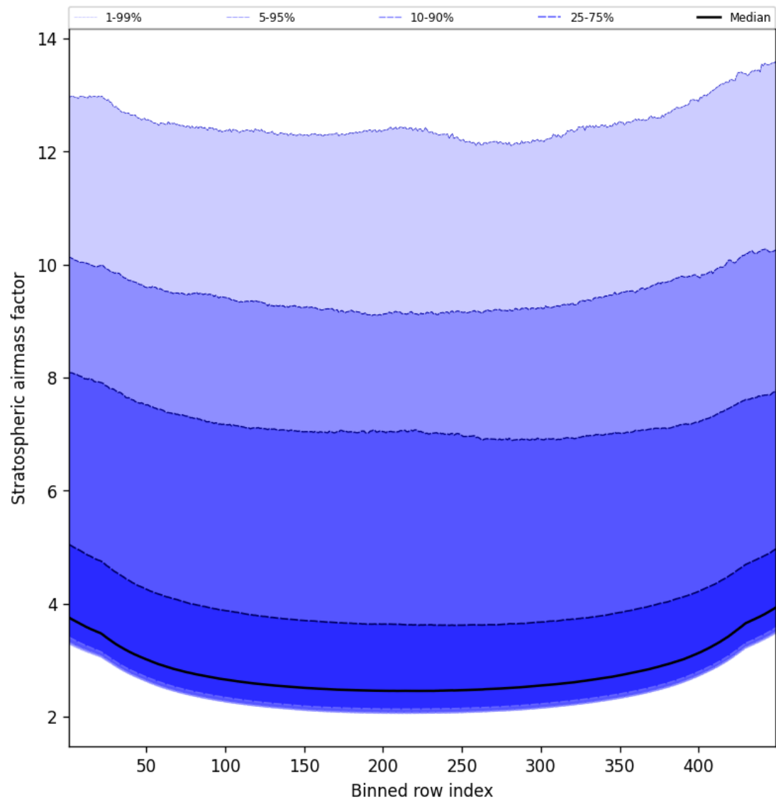
Figure 59: Along track statistics of “Stratospheric air mass factor” for 2024-12-31 to 2024-12-31
