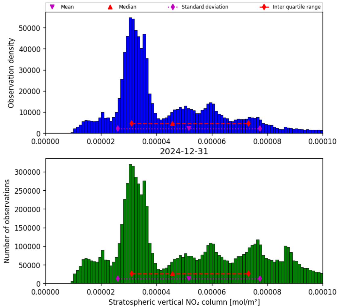
Figure 34: Histogram of “Stratospheric vertical NO 2 column” for 2024-12-31 to 2024-12-31
