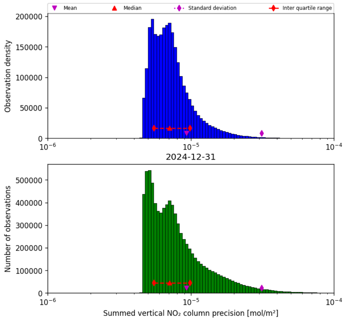
Figure 39: Histogram of “Summed vertical NO 2 column precision” for 2024-12-31 to 2024-12-31
