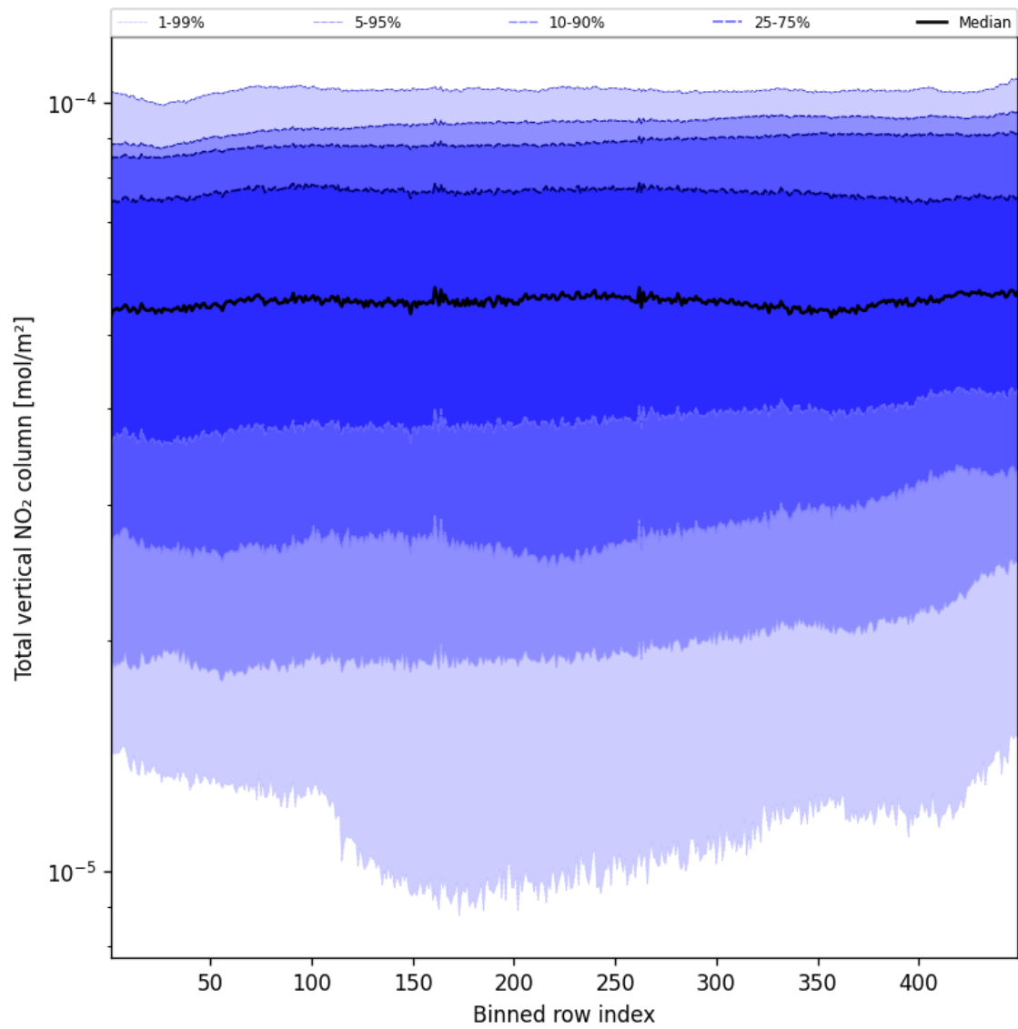
Figure 53: Along track statistics of “Total vertical NO 2 column” for 2024-12-31 to 2024-12-31
