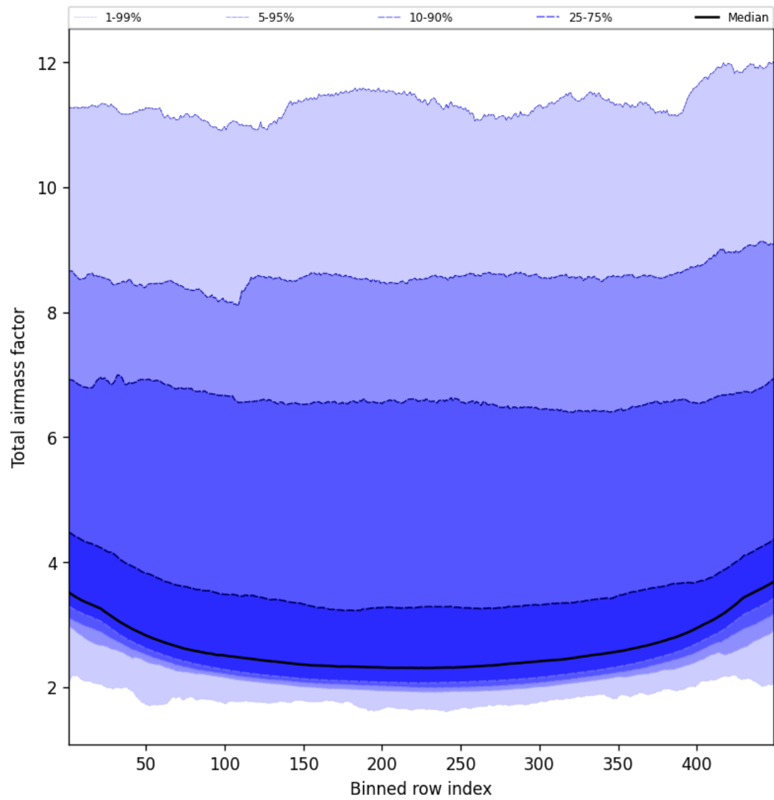
Figure 47: Along track statistics of “Total airmass factor” for 2024-12-31 to 2024-12-31
