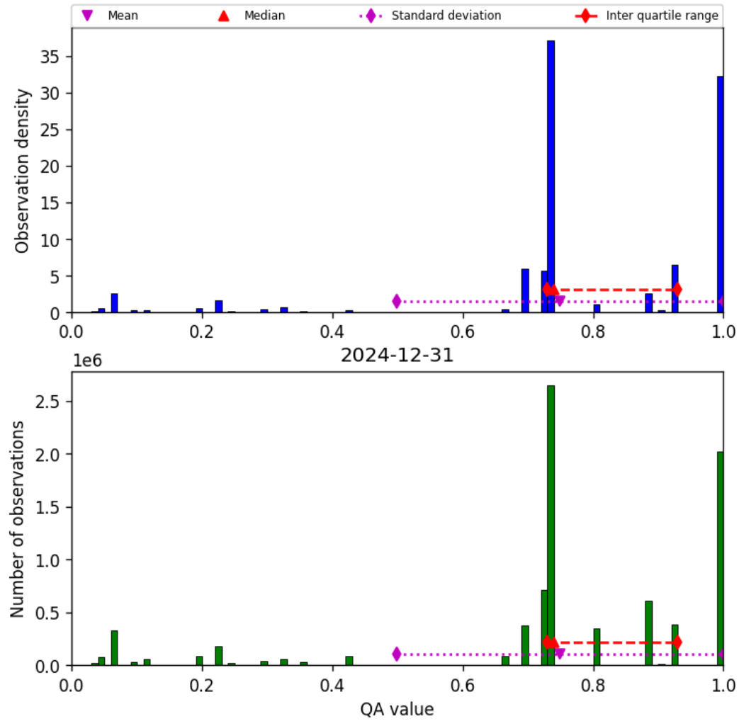
Figure 26: Histogram of “QA value” for 2024-12-31 to 2024-12-31
