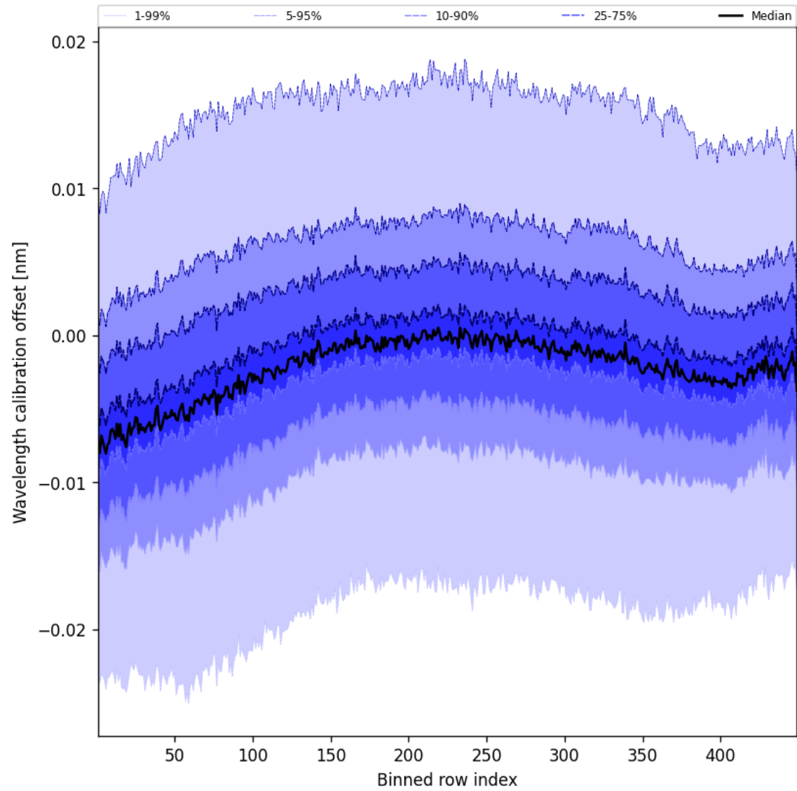
Figure 50: Along track statistics of “Wavelength calibration offset” for 2024-12-31 to 2024-12-31
