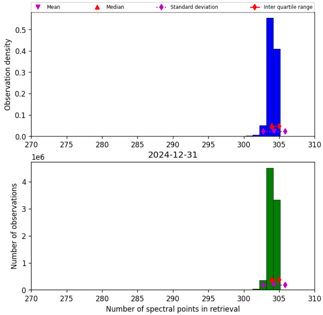
Figure 31: Histogram of “Number of spectral points in retrieval” for 2024-12-31 to 2024-12-31
