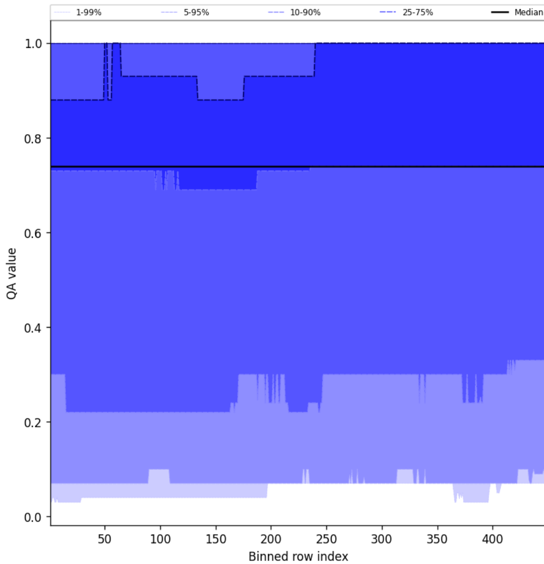
Figure 43: Along track statistics of "QA value" for 2024-12-31 to 2024-12-31
