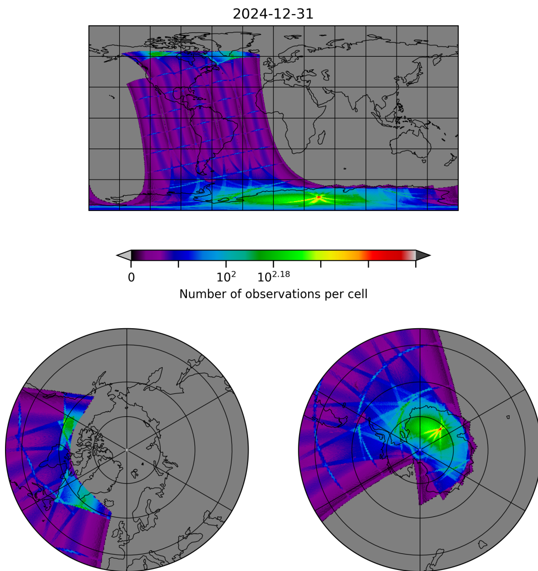
Figure 8: Map of the number of observations for 2024-12-31 to 2024-12-31
