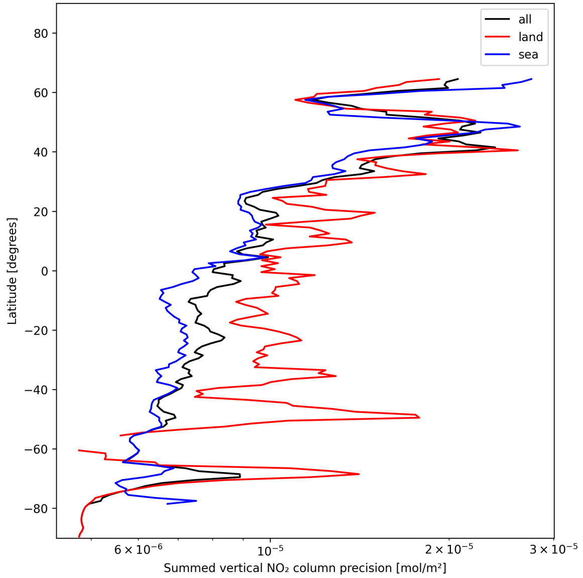
Figure 22: Zonal average of “Summed vertical NO 2 column precision” for 2024-12-31 to 2024-12-31.
