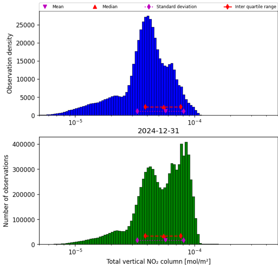
Figure 36: Histogram of “Total vertical NO 2 column” for 2024-12-31 to 2024-12-31
