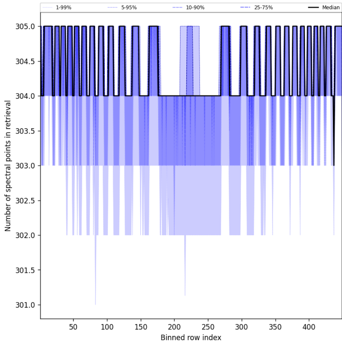
Figure 48: Along track statistics of “Number of spectral points in retrieval” for 2024-12-31 to 2024-12-31
