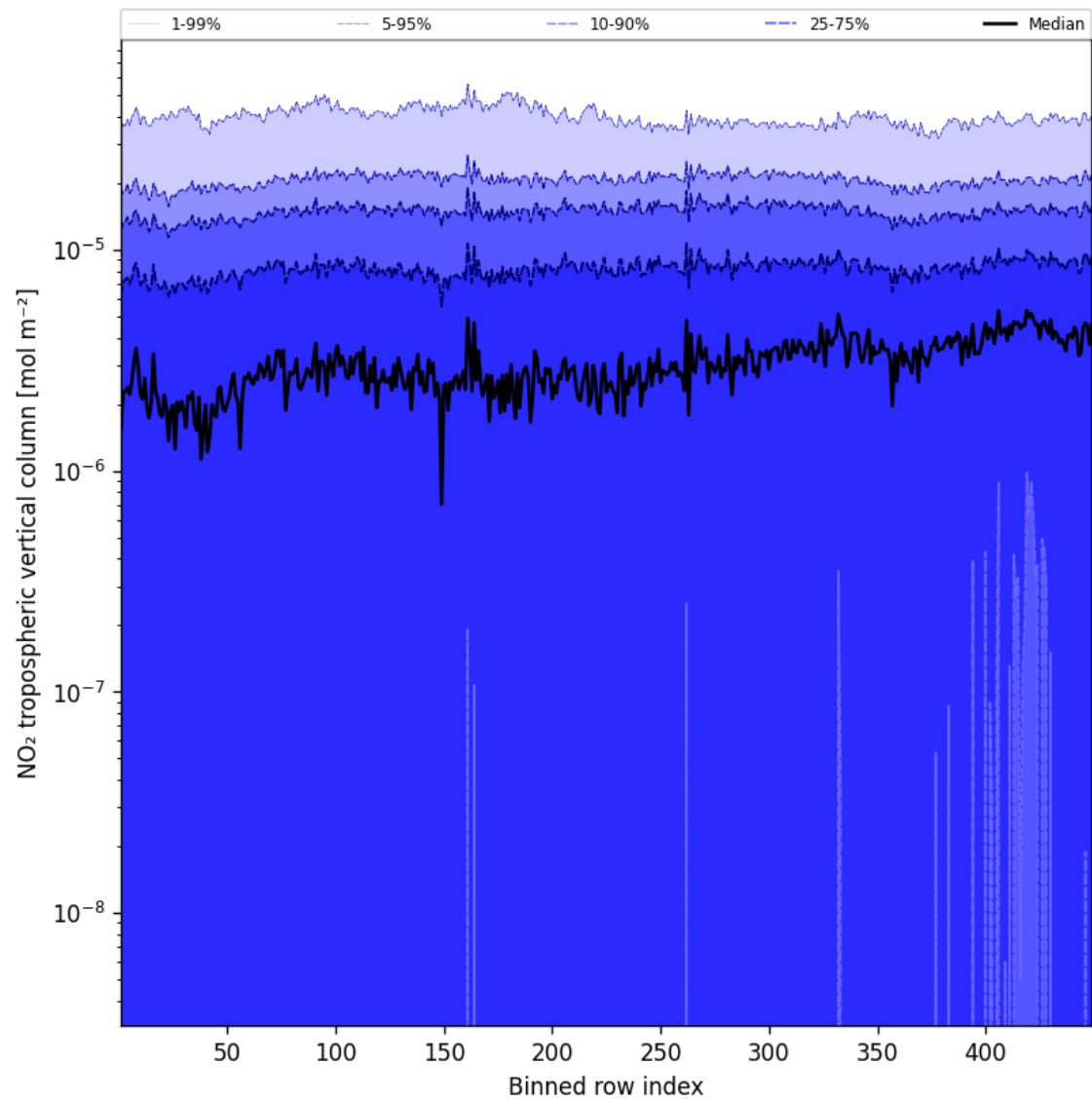
Figure 44: Along track statistics of “NO 2 tropospheric vertical column” for 2024-12-31 to 2024-12-31
