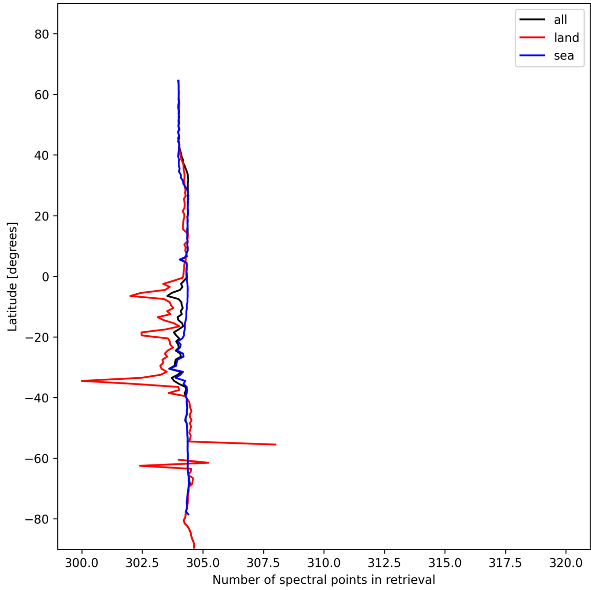
Figure 14: Zonal average of “Number of spectral points in retrieval” for 2024-12-31 to 2024-12-31.
