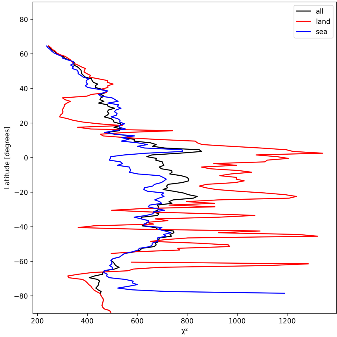
Figure 23: Zonal average of “ \chi^2 ” for 2024-12-31 to 2024-12-31.
