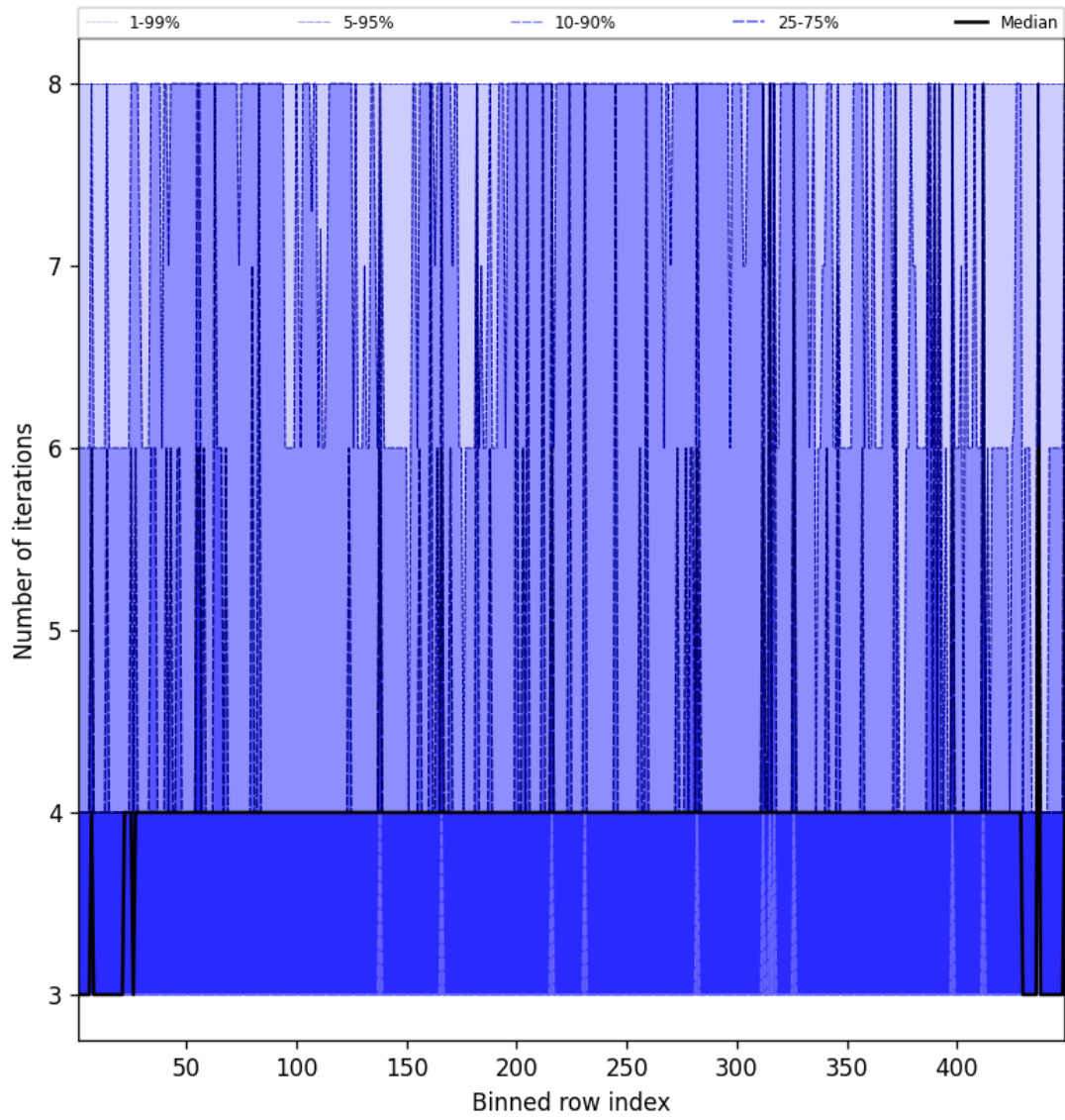
Figure 49: Along track statistics of “Number of iterations” for 2024-12-31 to 2024-12-31
