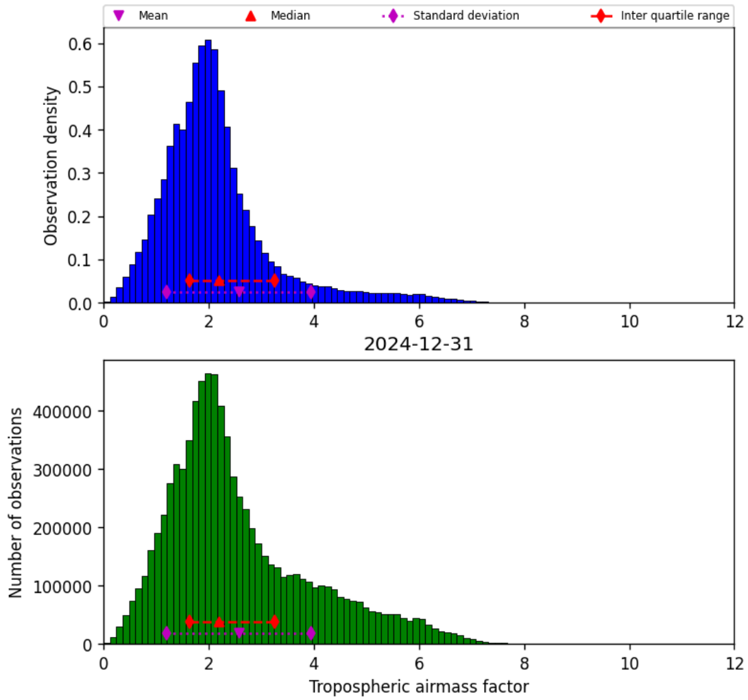
Figure 29: Histogram of “Tropospheric airmass factor” for 2024-12-31 to 2024-12-31
