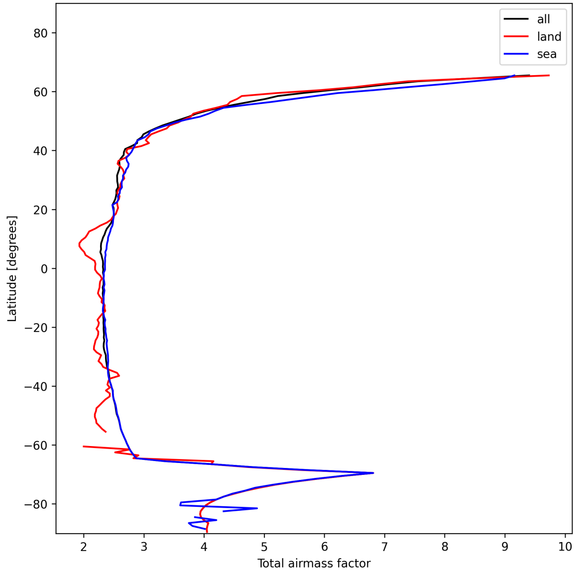
Figure 13: Zonal average of “Total airmass factor” for 2025-01-02 to 2025-01-03.
