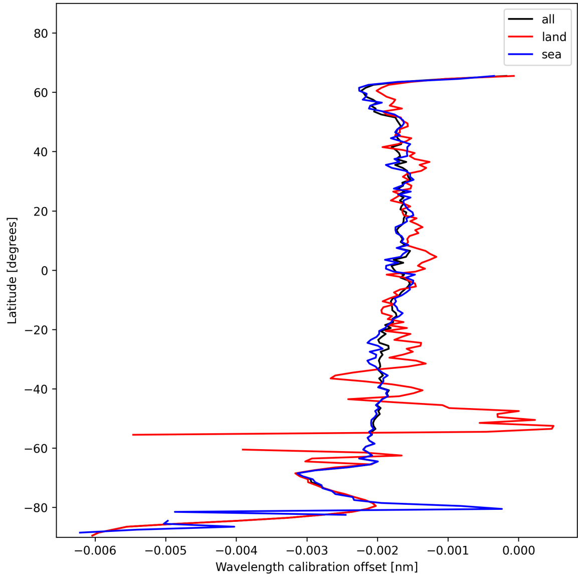
Figure 16: Zonal average of “Wavelength calibration offset” for 2025-01-02 to 2025-01-03.
