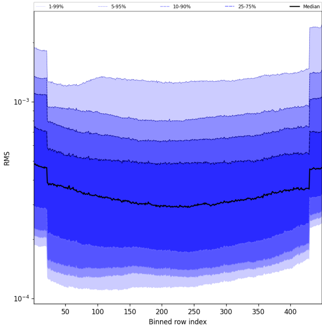
Figure 58: Along track statistics of “RMS” for 2025-01-02 to 2025-01-03
