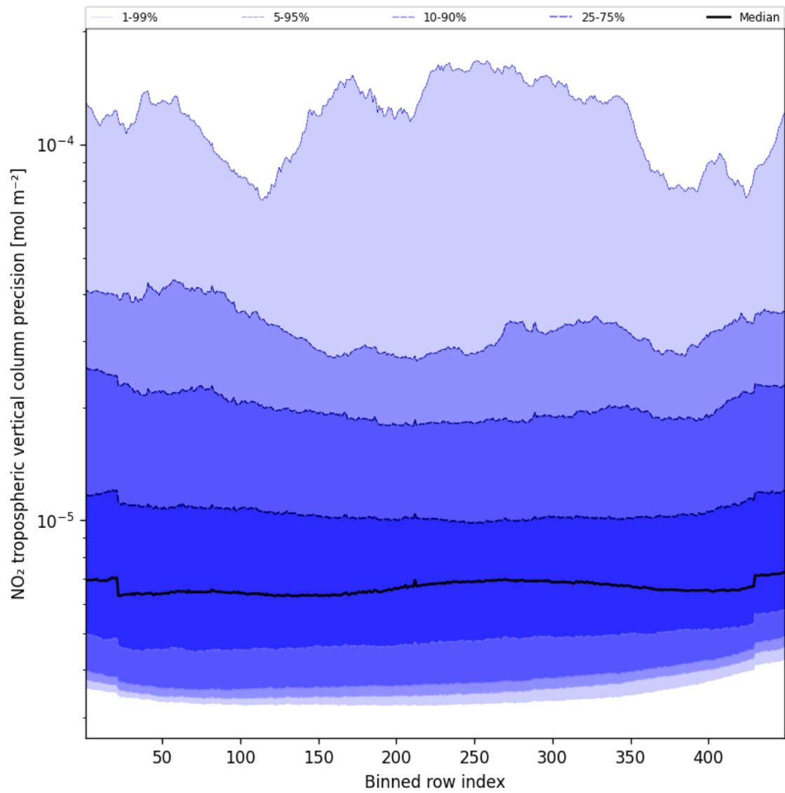
Figure 45: Along track statistics of “NO 2 tropospheric vertical column precision” for 2025-01-02 to 2025-01-03
