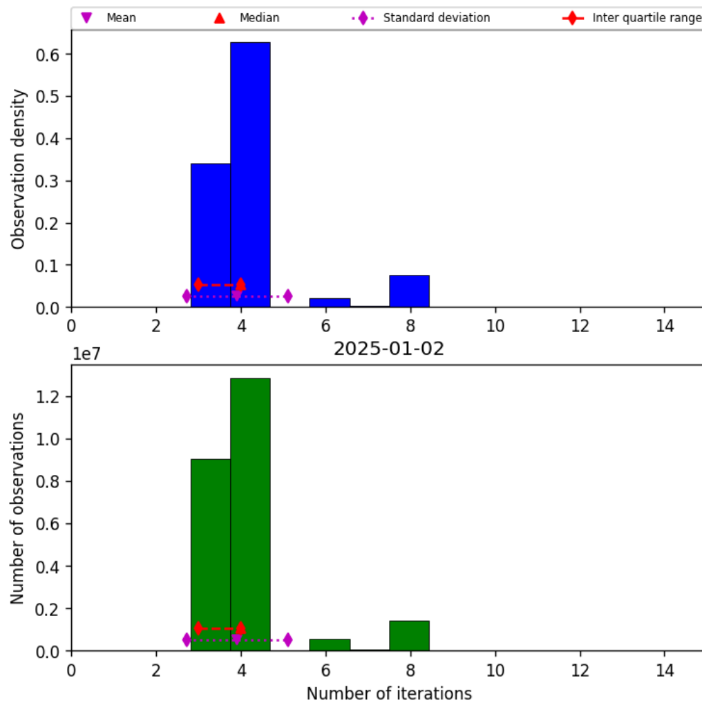
Figure 32: Histogram of “Number of iterations” for 2025-01-02 to 2025-01-03
