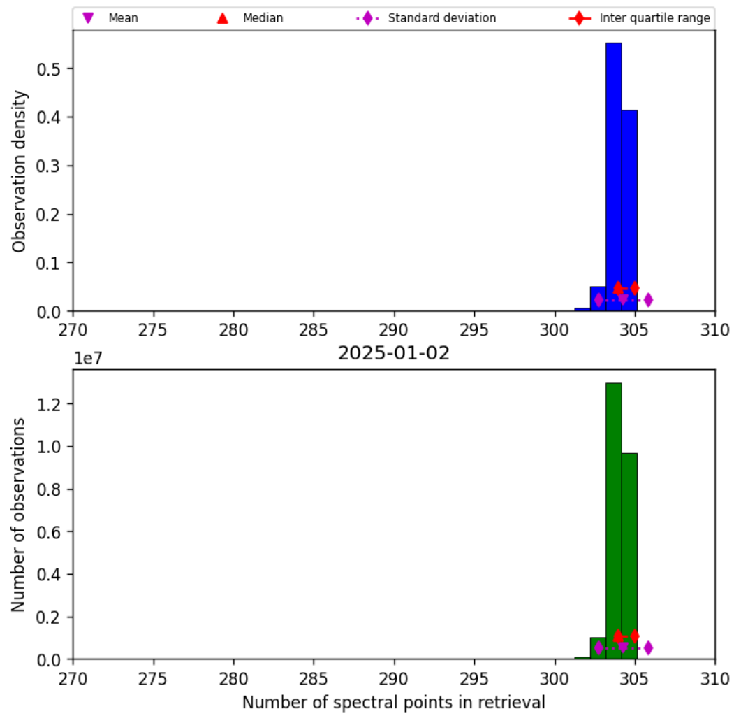
Figure 31: Histogram of “Number of spectral points in retrieval” for 2025-01-02 to 2025-01-03
