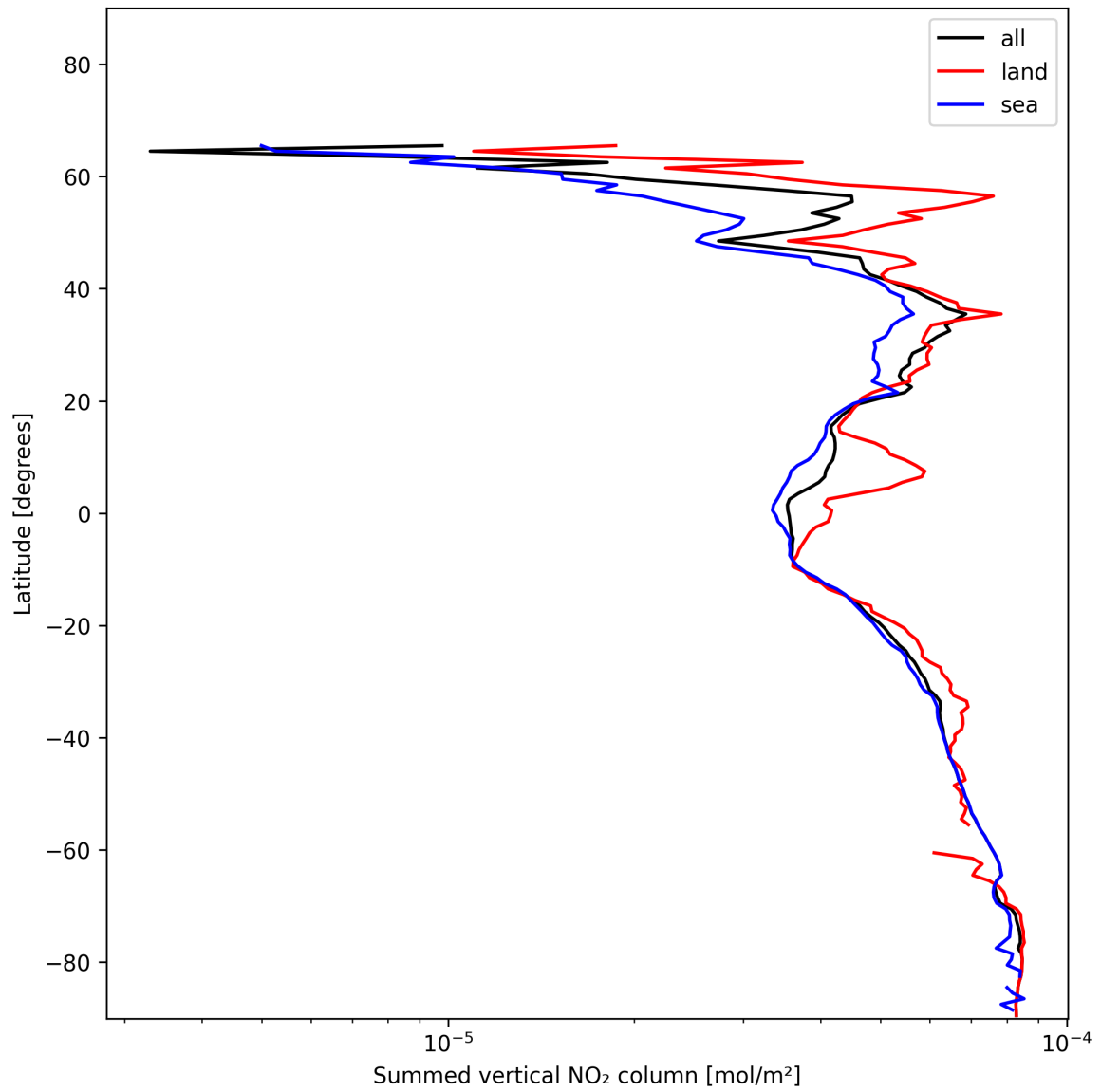
Figure 21: Zonal average of “Summed vertical NO 2 column” for 2025-01-02 to 2025-01-03.
