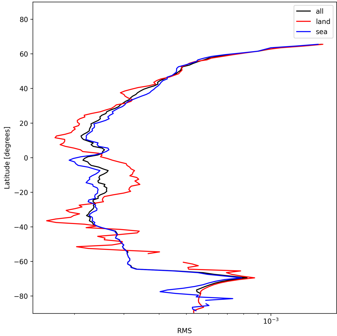
Figure 24: Zonal average of “RMS” for 2025-01-02 to 2025-01-03.
