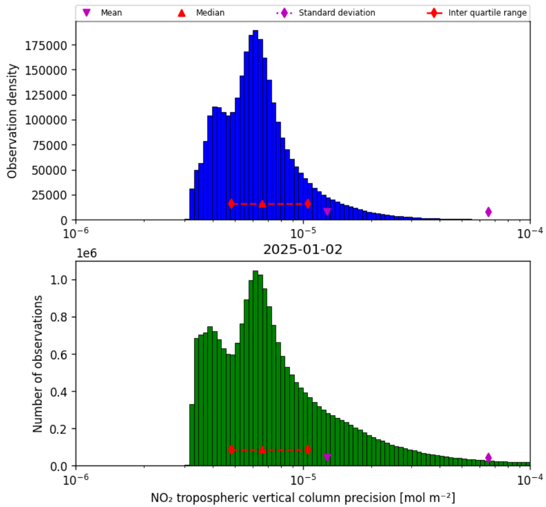
Figure 28: Histogram of “NO 2 tropospheric vertical column precision” for 2025-01-02 to 2025-01-03
