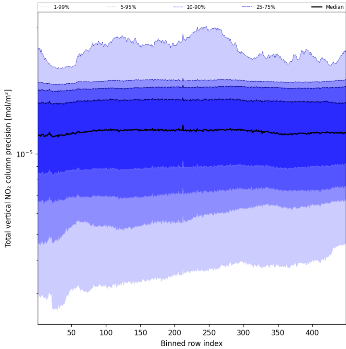
Figure 54: Along track statistics of “Total vertical NO 2 column precision” for 2025-01-02 to 2025-01-03
