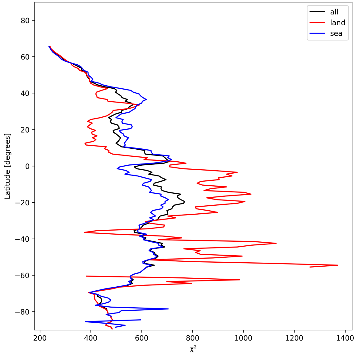
Figure 23: Zonal average of “ \chi^2 ” for 2025-01-02 to 2025-01-03.
