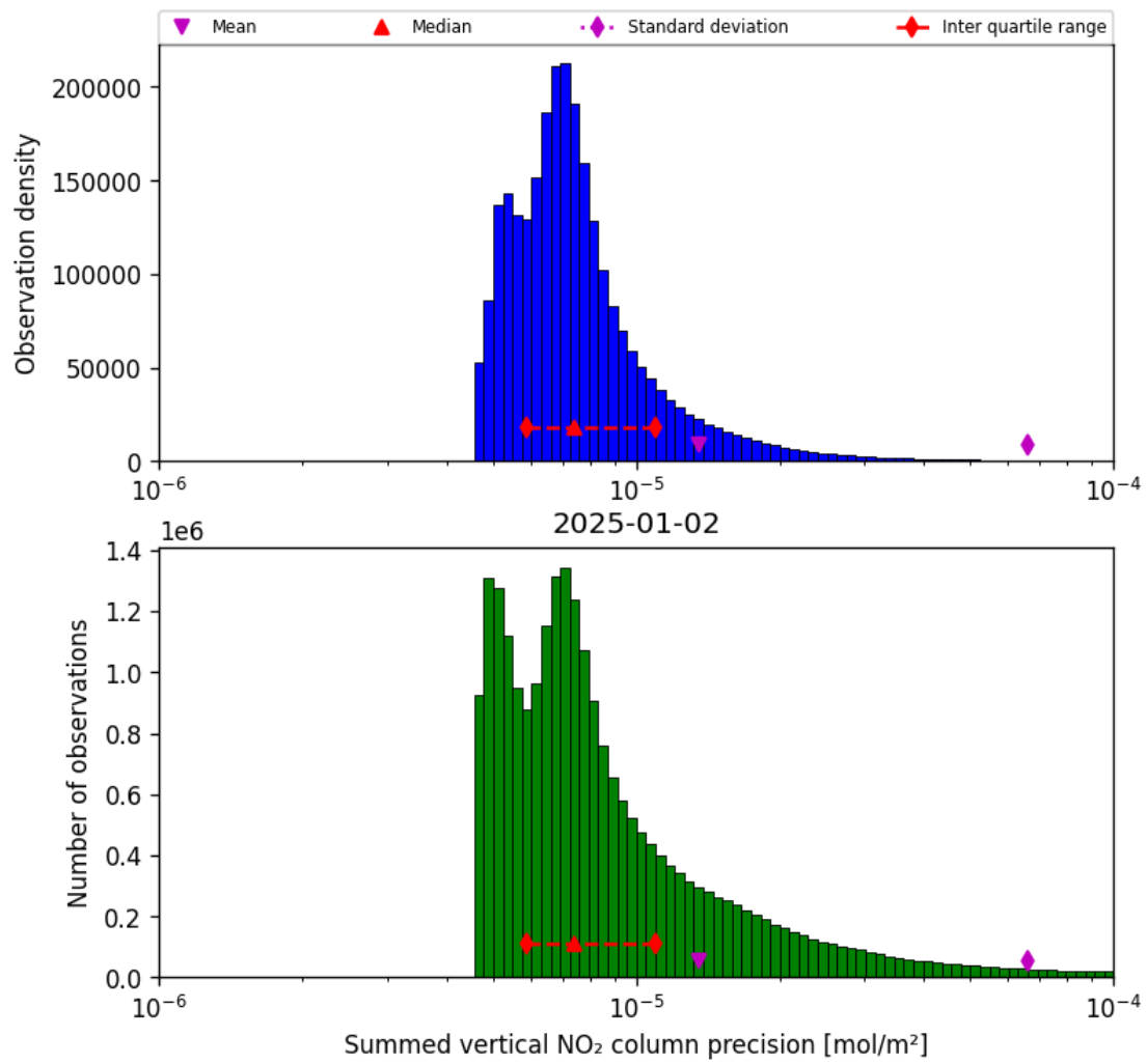
Figure 39: Histogram of "Summed vertical NO 2 column precision" for 2025-01-02 to 2025-01-03
