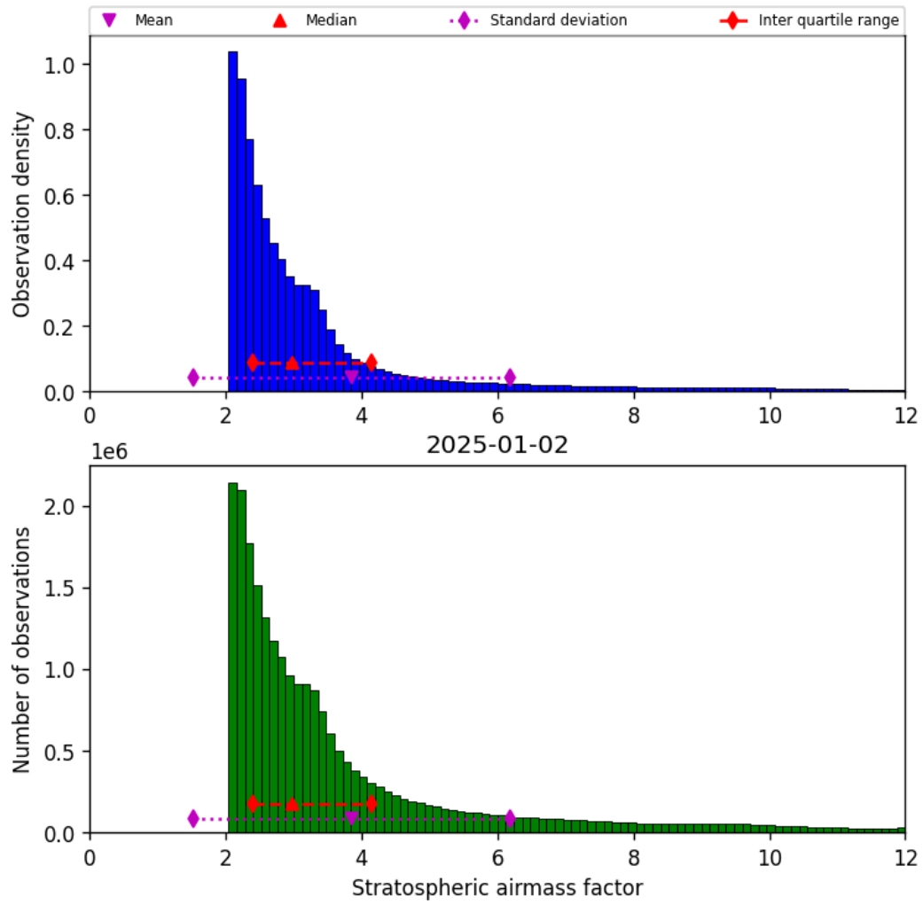
Figure 42: Histogram of “Stratospheric airmass factor” for 2025-01-02 to 2025-01-03
