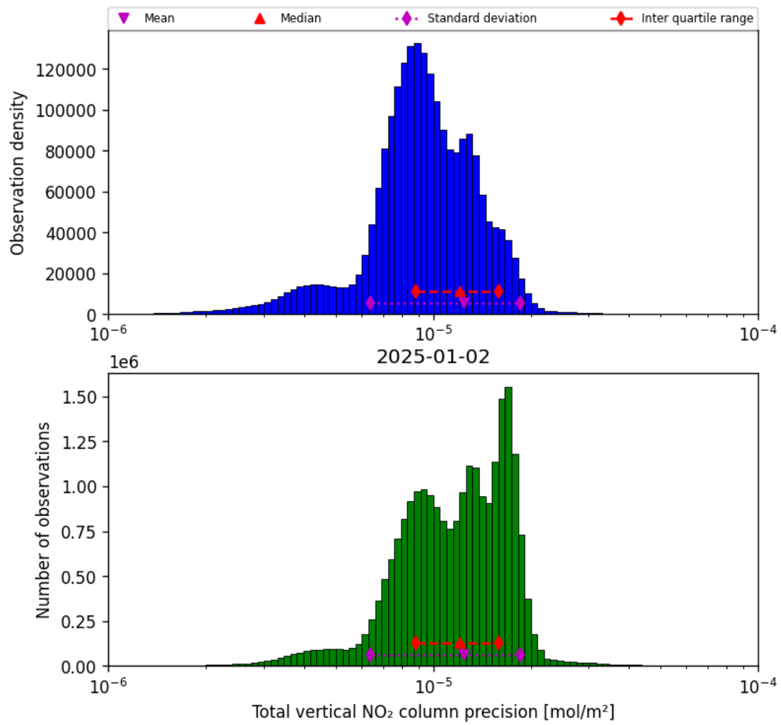
Figure 37: Histogram of “Total vertical NO 2 column precision” for 2025-01-02 to 2025-01-03
