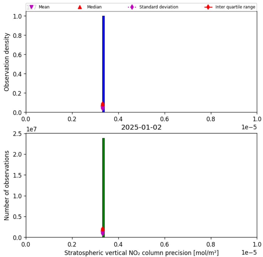
Figure 35: Histogram of “Stratospheric vertical NO 2 column precision” for 2025-01-02 to 2025-01-03
