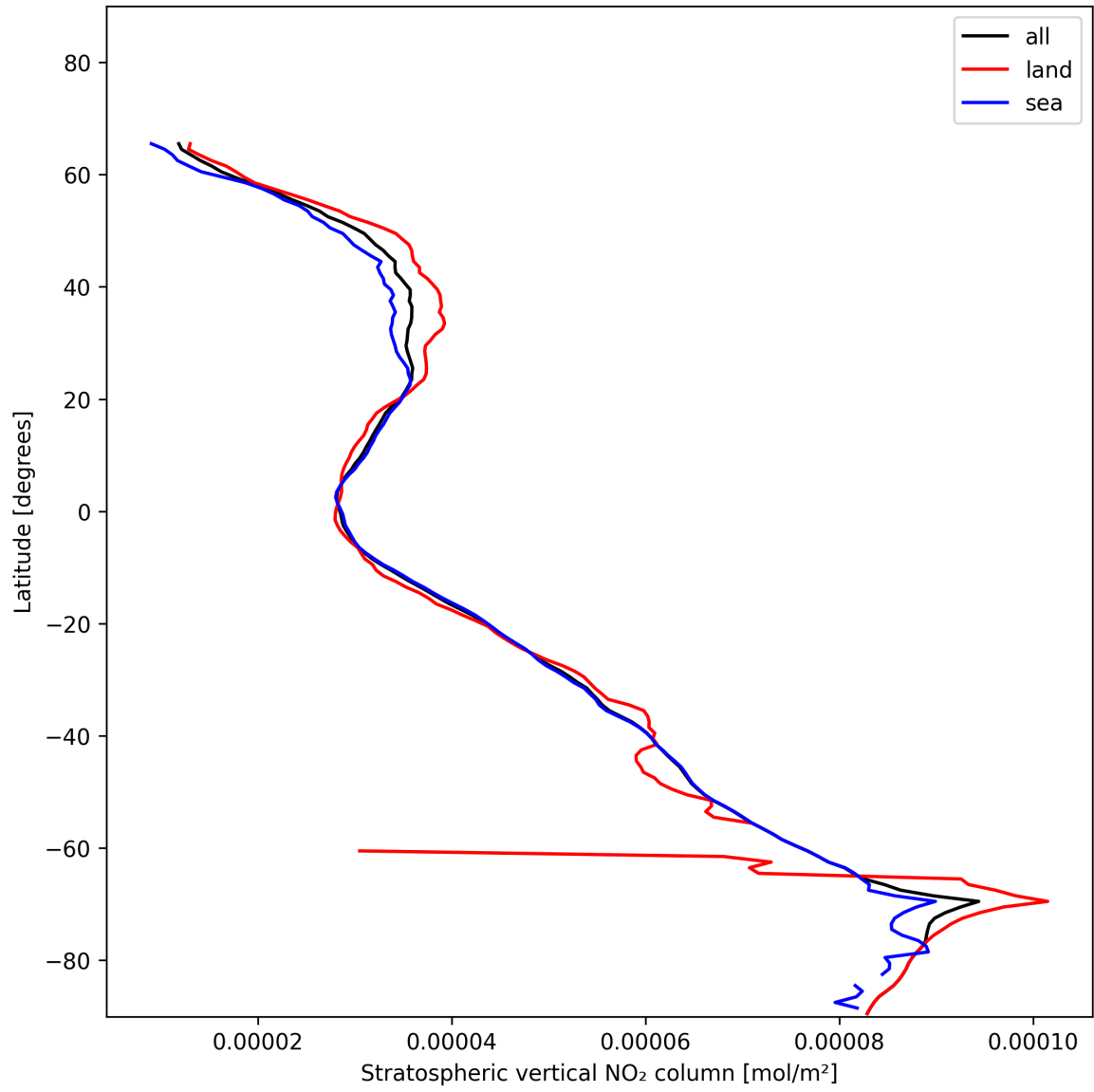
Figure 17: Zonal average of “Stratospheric vertical NO 2 column” for 2025-01-02 to 2025-01-03.
