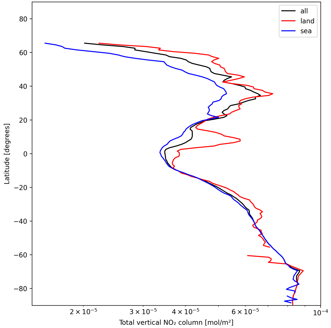
Figure 19: Zonal average of “Total vertical NO 2 column” for 2025-01-02 to 2025-01-03.
