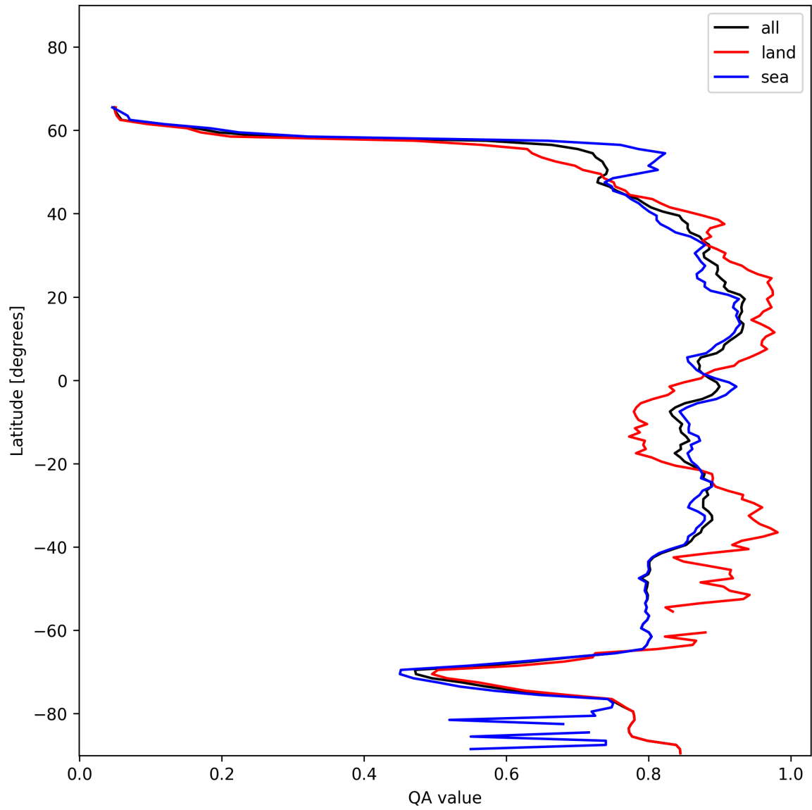
Figure 9: Zonal average of “QA value” for 2025-01-02 to 2025-01-03.
