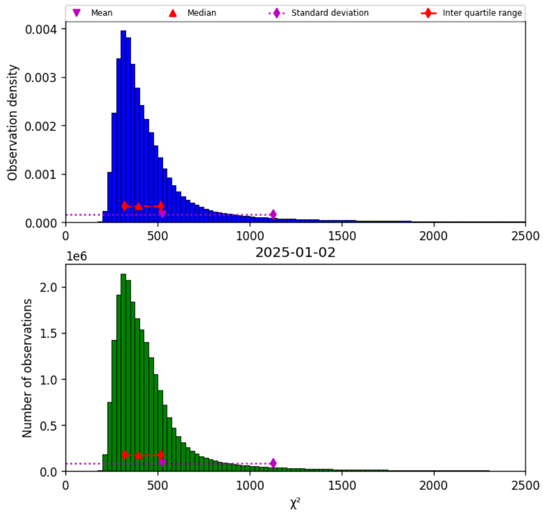
Figure 40: Histogram of “ \chi^2 ” for 2025-01-02 to 2025-01-03
