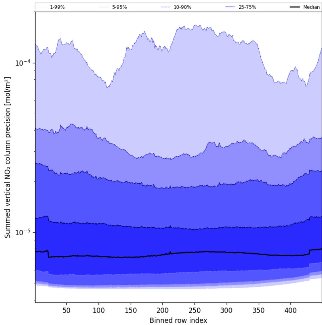
Figure 56: Along track statistics of “Summed vertical NO 2 column precision” for 2025-01-02 to 2025-01-03
