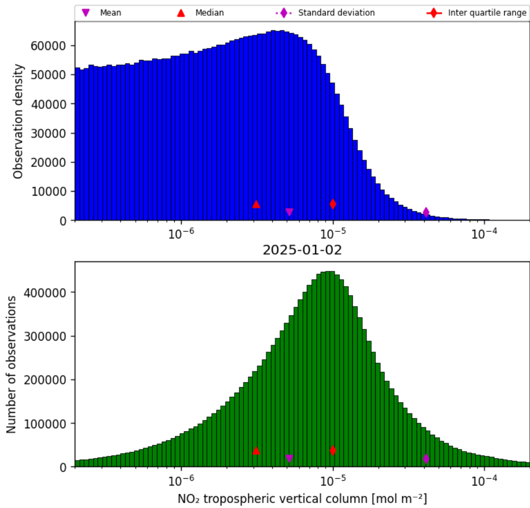
Figure 27: Histogram of “NO 2 tropospheric vertical column” for 2025-01-02 to 2025-01-03
