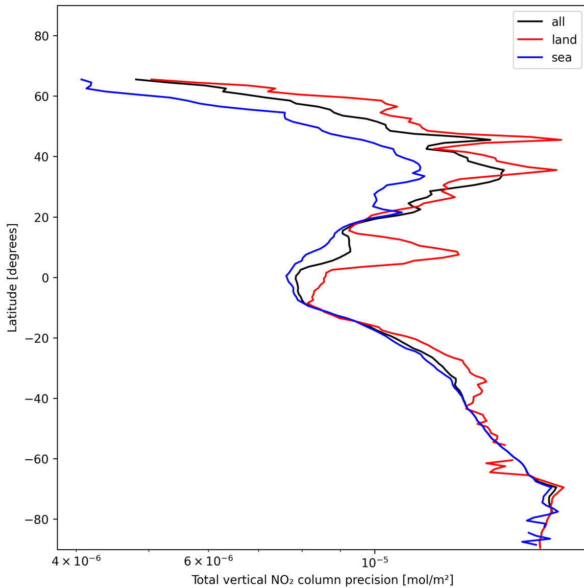
Figure 20: Zonal average of “Total vertical NO 2 column precision” for 2025-01-02 to 2025-01-03.
