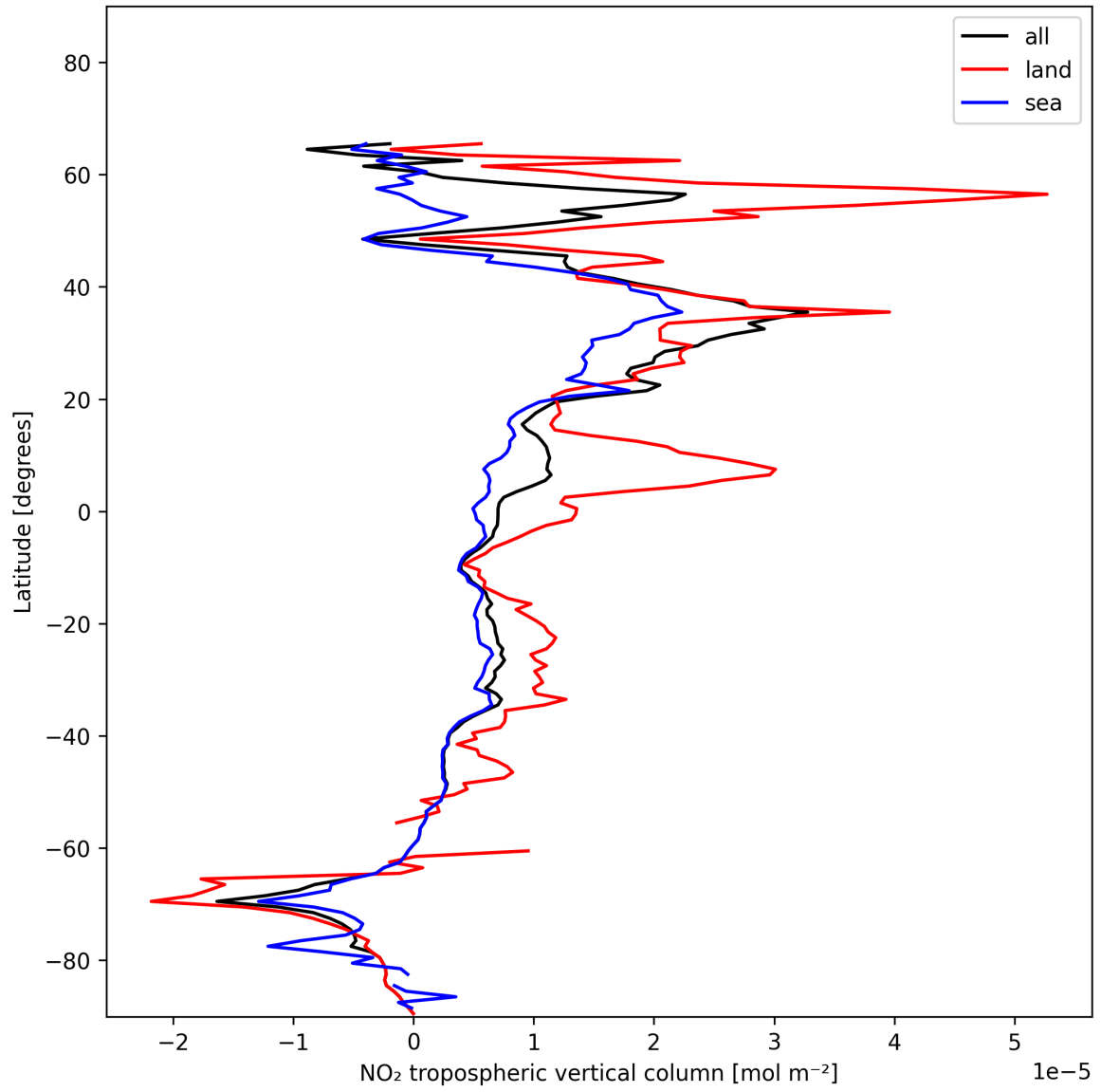
Figure 10: Zonal average of “NO 2 tropospheric vertical column” for 2025-01-02 to 2025-01-03.
