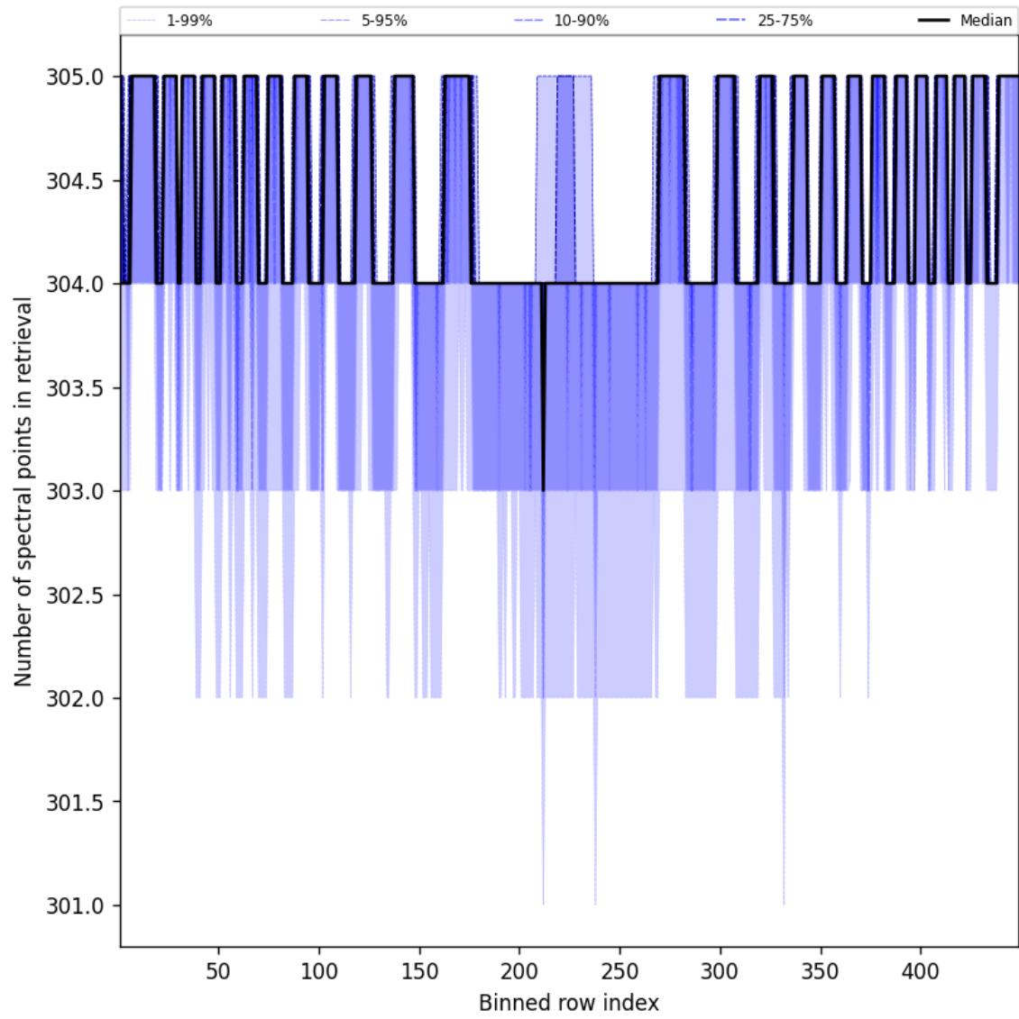
Figure 48: Along track statistics of “Number of spectral points in retrieval” for 2025-01-02 to 2025-01-03
