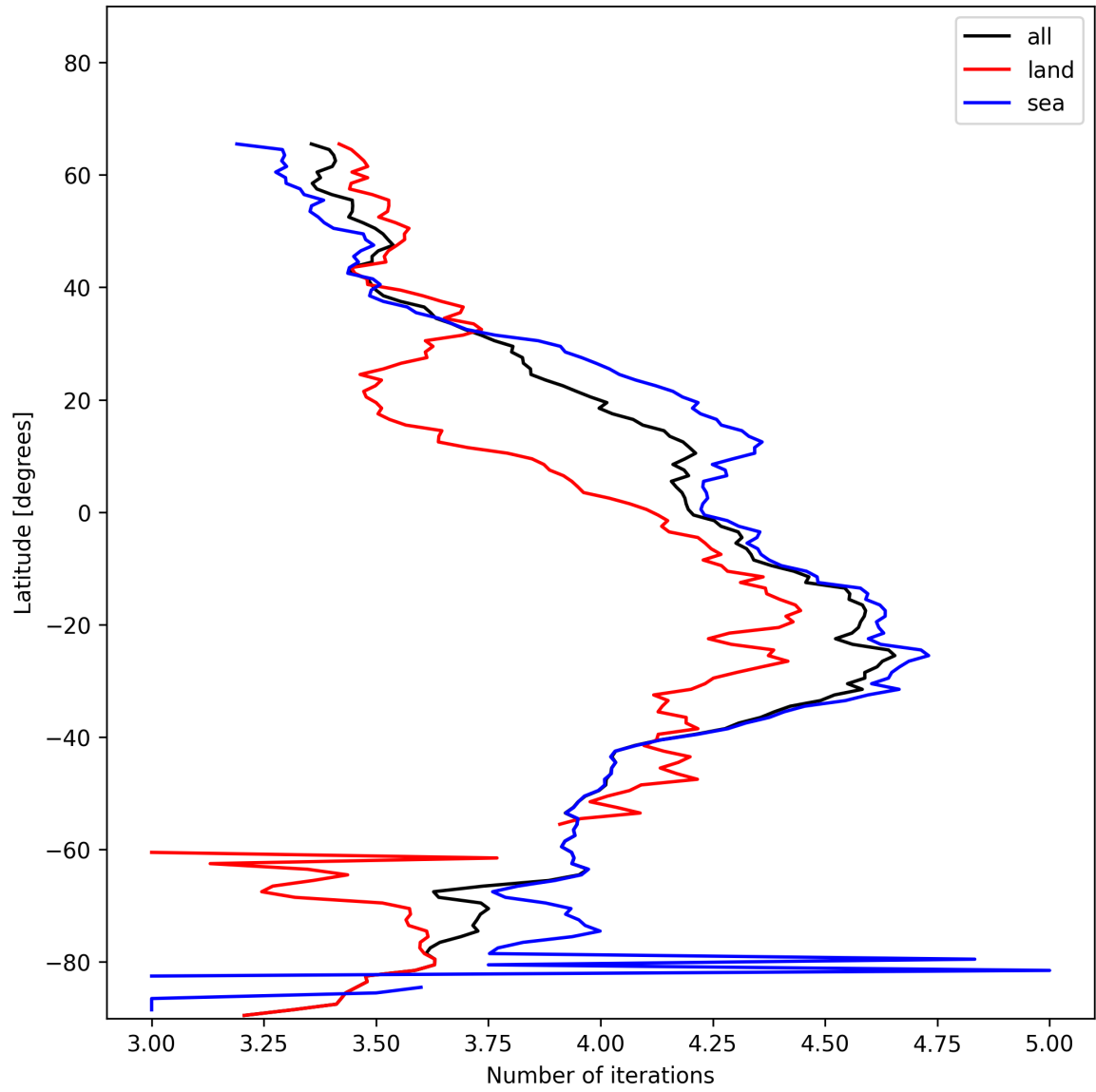
Figure 15: Zonal average of “Number of iterations” for 2025-01-02 to 2025-01-03.
