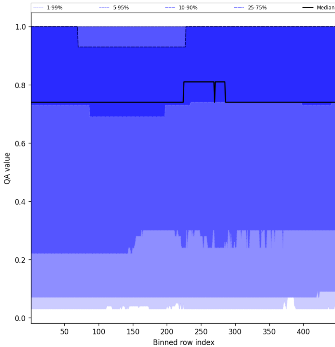
Figure 43: Along track statistics of “QA value” for 2025-01-02 to 2025-01-03
