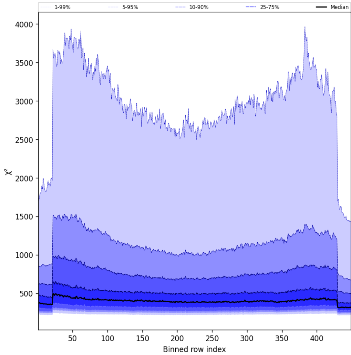
Figure 57: Along track statistics of “ \chi^2 ” for 2025-01-02 to 2025-01-03
