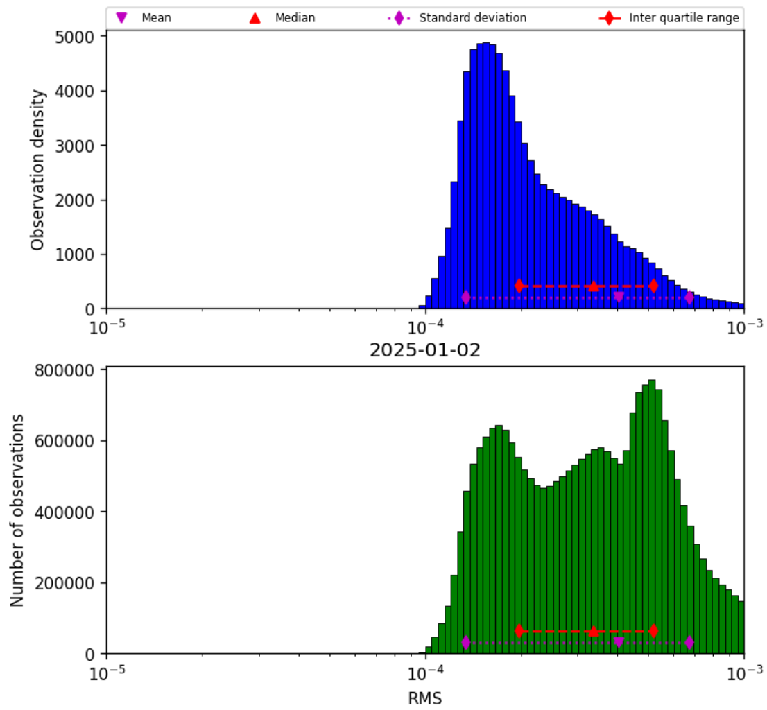
Figure 41: Histogram of “RMS” for 2025-01-02 to 2025-01-03
