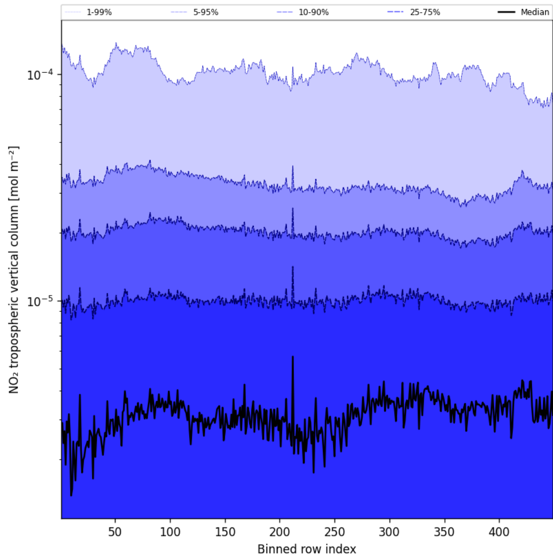
Figure 44: Along track statistics of “NO 2 tropospheric vertical column” for 2025-01-02 to 2025-01-03
