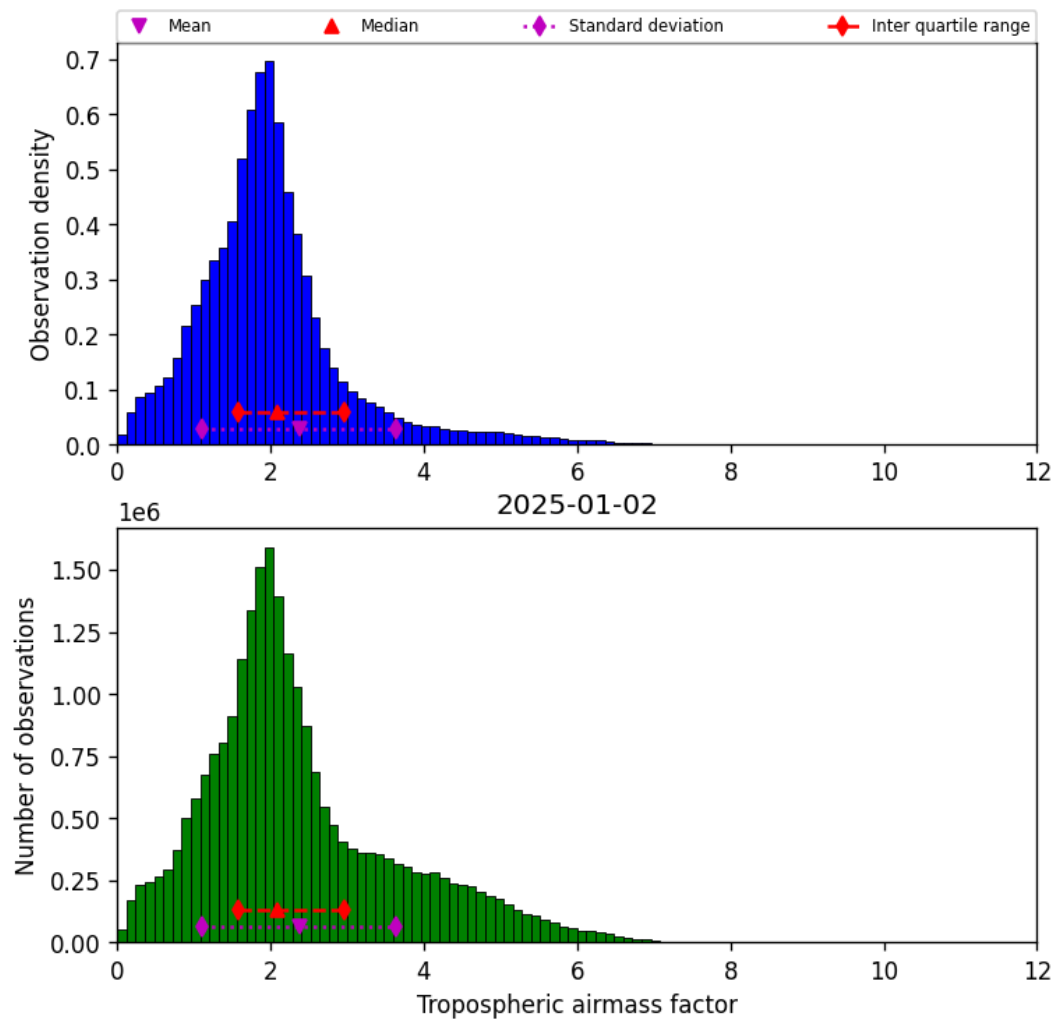
Figure 29: Histogram of “Tropospheric airmass factor” for 2025-01-02 to 2025-01-03
