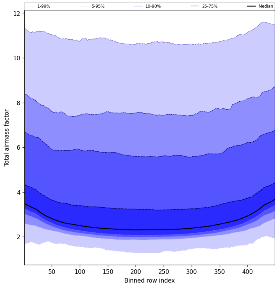
Figure 47: Along track statistics of “Total airmass factor” for 2025-01-02 to 2025-01-03
