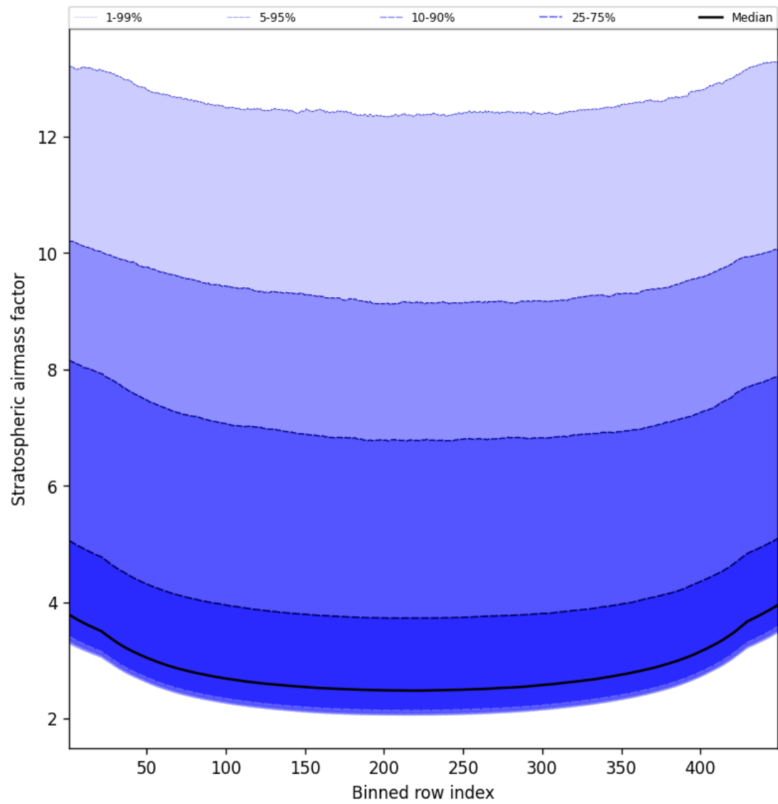
Figure 59: Along track statistics of “Stratospheric airmass factor” for 2025-01-02 to 2025-01-03
