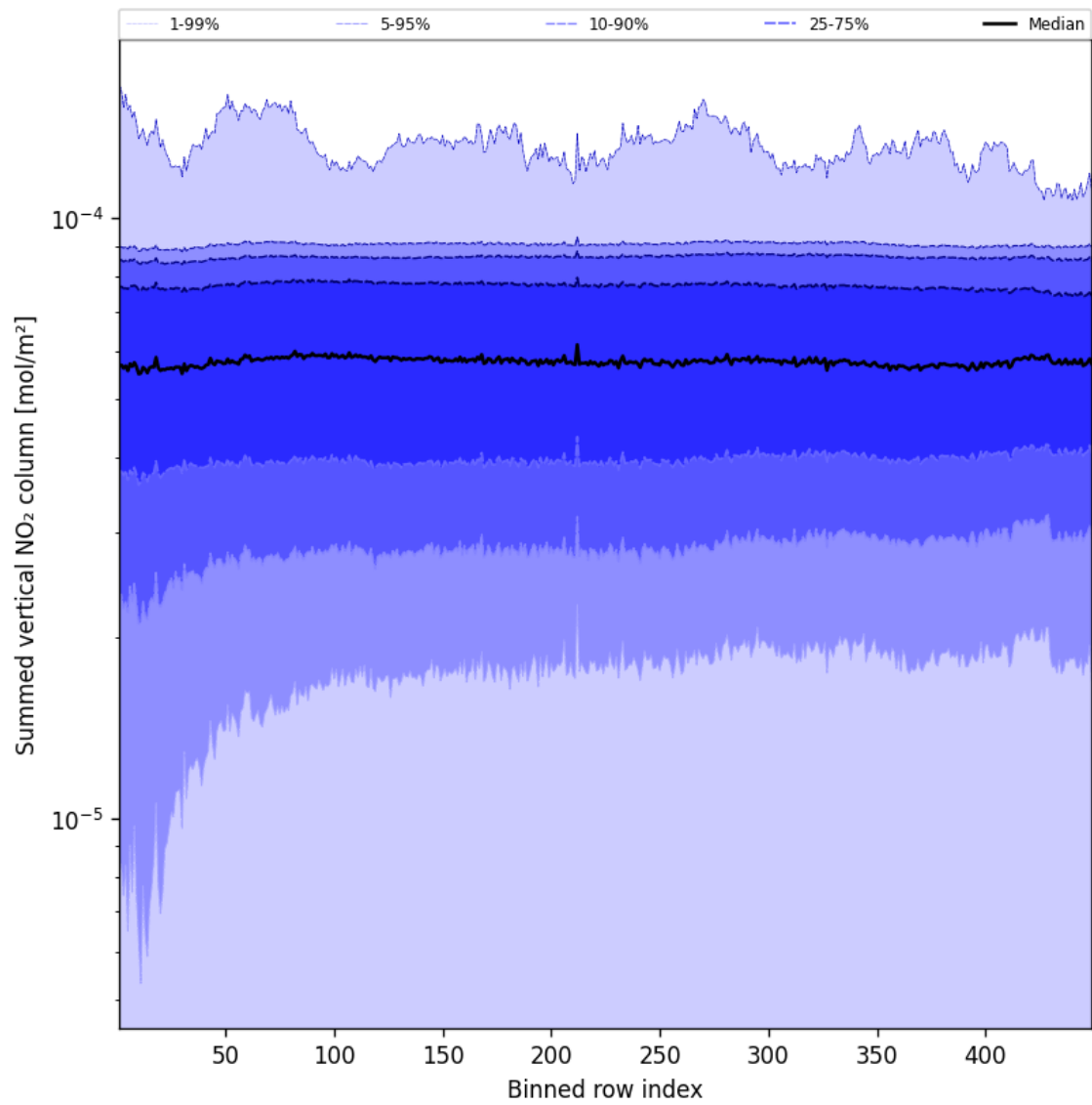
Figure 55: Along track statistics of “Summed vertical NO 2 column” for 2025-01-02 to 2025-01-03
