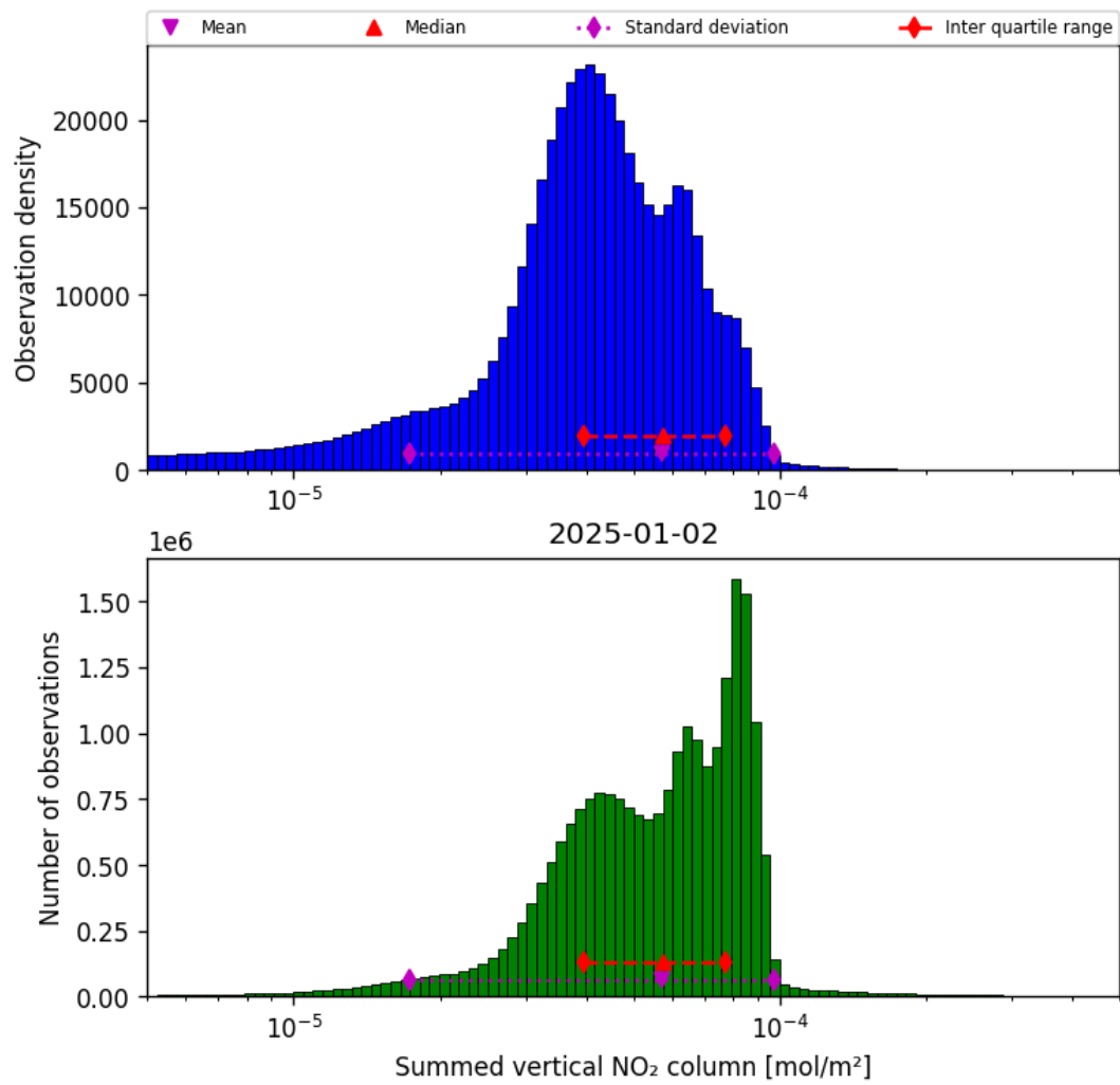
Figure 38: Histogram of “Summed vertical NO 2 column” for 2025-01-02 to 2025-01-03
