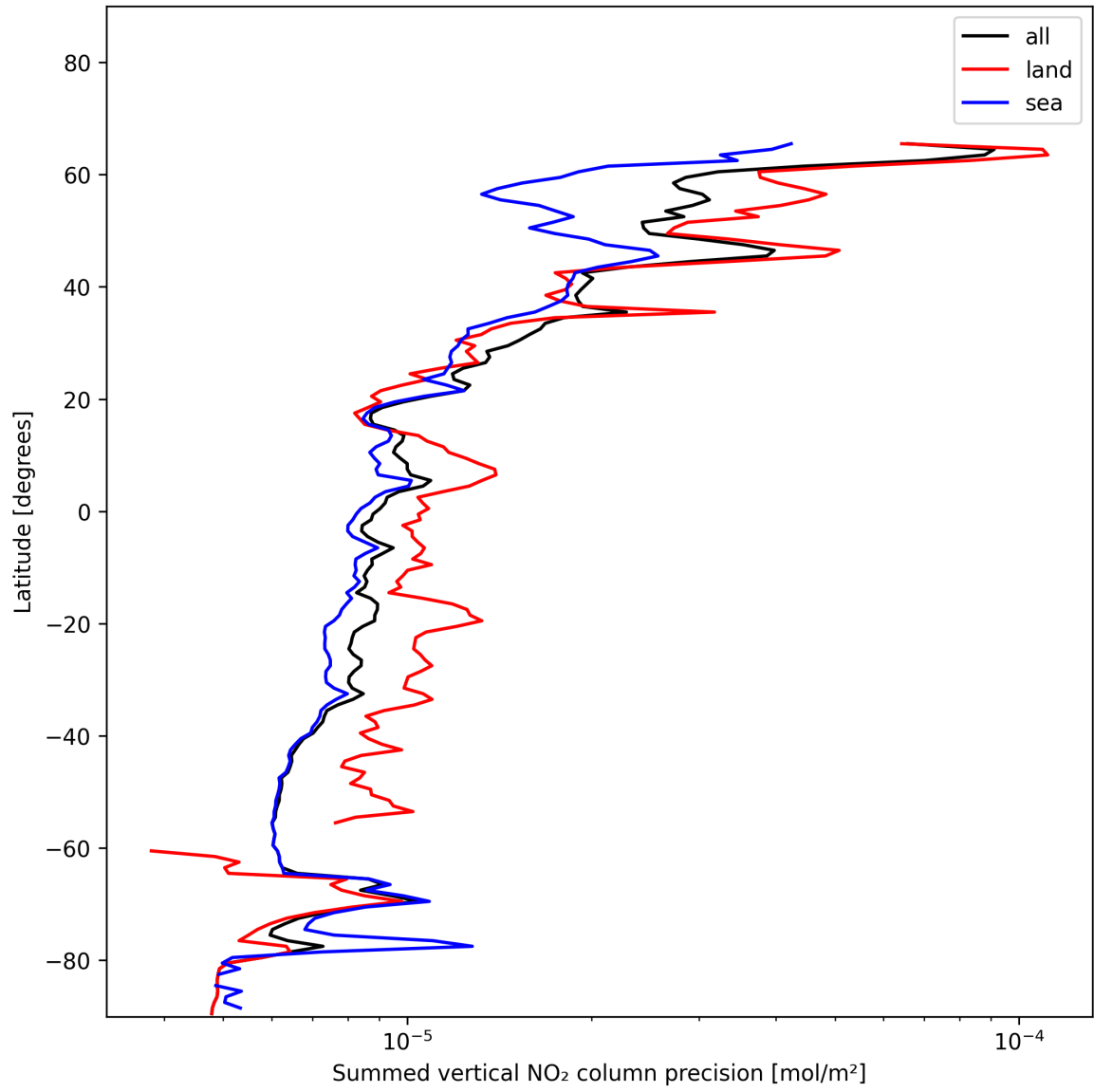
Figure 22: Zonal average of “Summed vertical NO 2 column precision” for 2025-01-02 to 2025-01-03.
