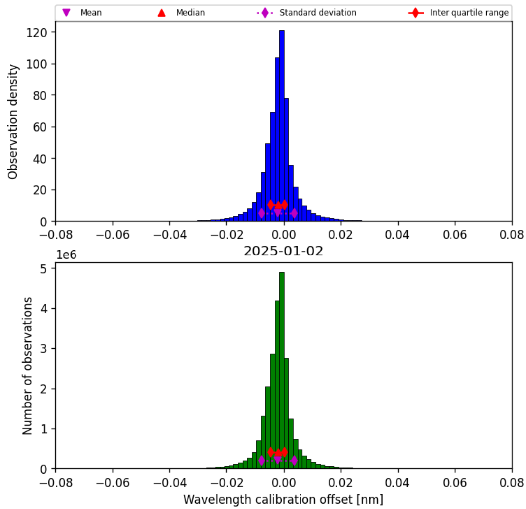
Figure 33: Histogram of “Wavelength calibration offset” for 2025-01-02 to 2025-01-03
