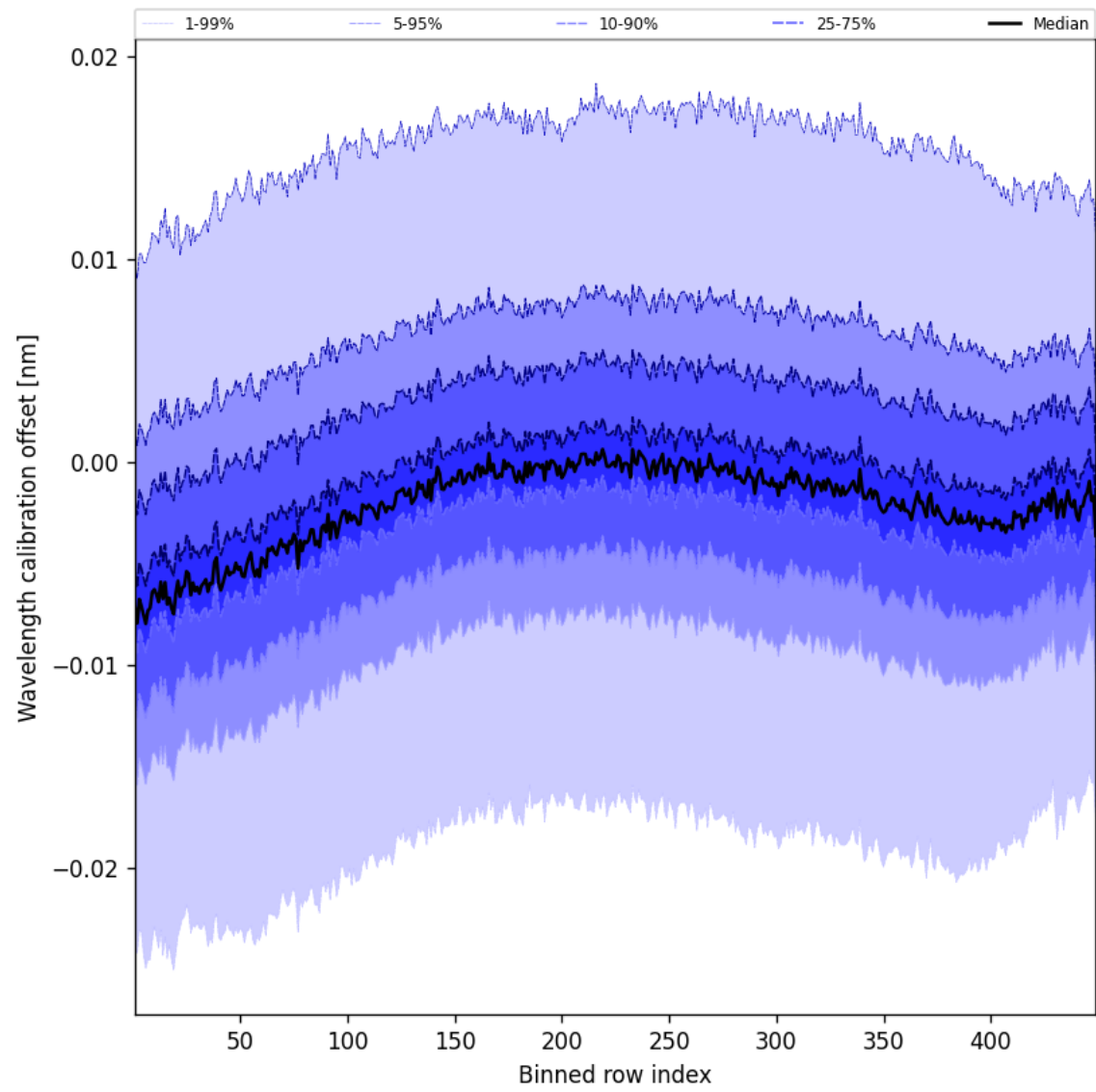
Figure 50: Along track statistics of “Wavelength calibration offset” for 2025-01-02 to 2025-01-03
