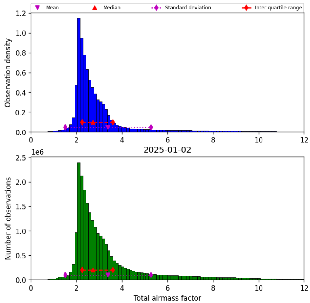
Figure 30: Histogram of “Total airmass factor” for 2025-01-02 to 2025-01-03
