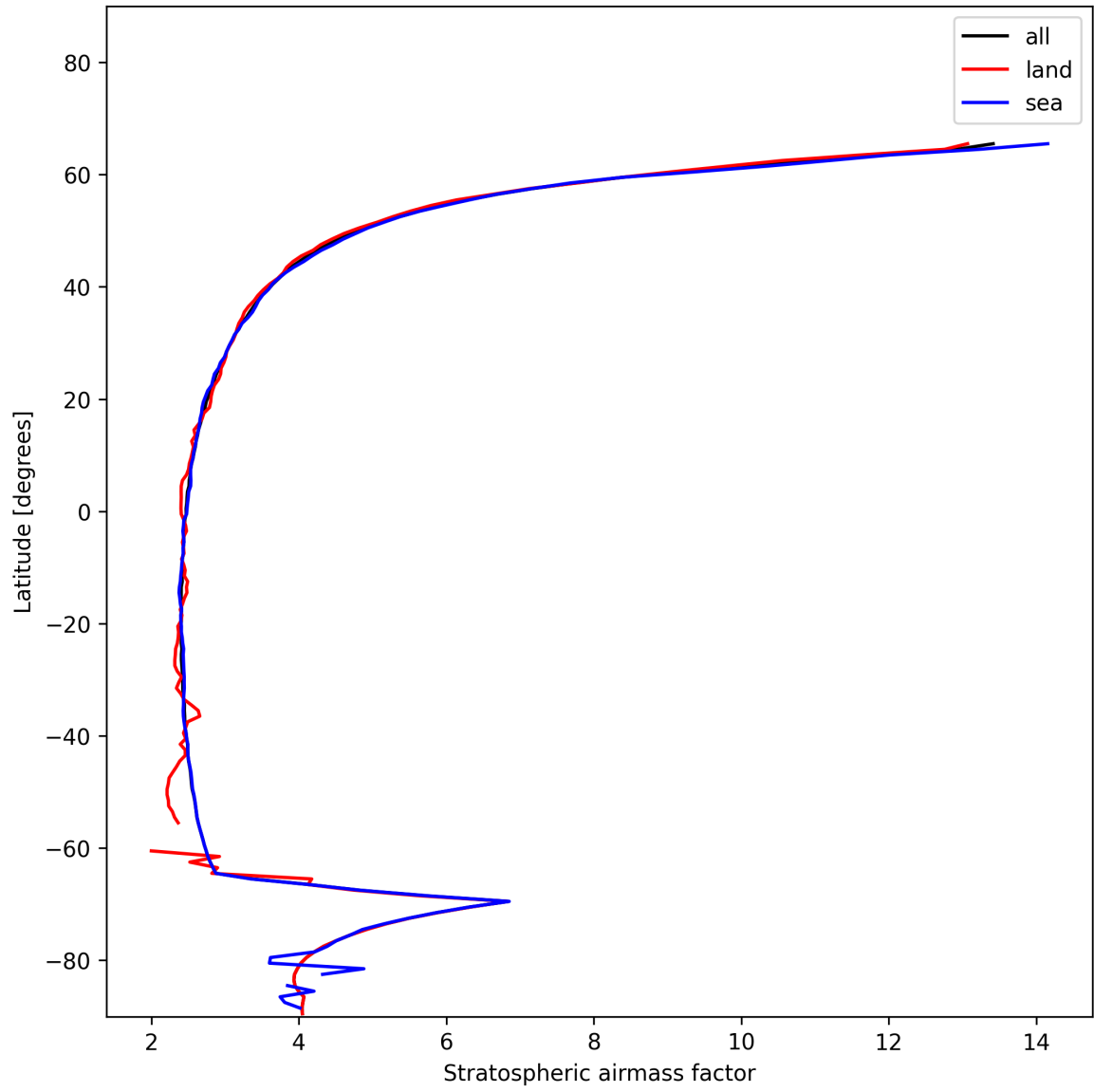
Figure 25: Zonal average of “Stratospheric air mass factor” for 2025-01-02 to 2025-01-03.
