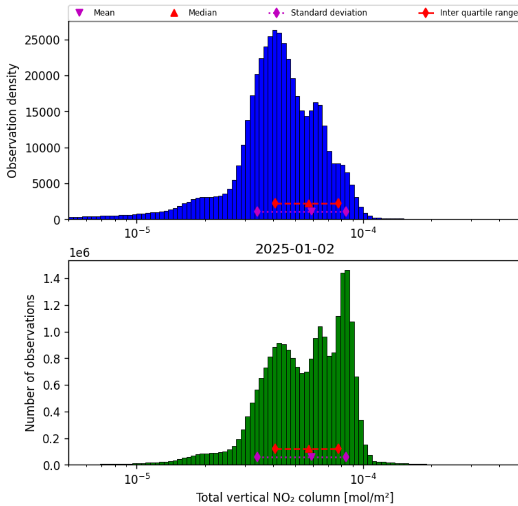
Figure 36: Histogram of “Total vertical NO 2 column” for 2025-01-02 to 2025-01-03
