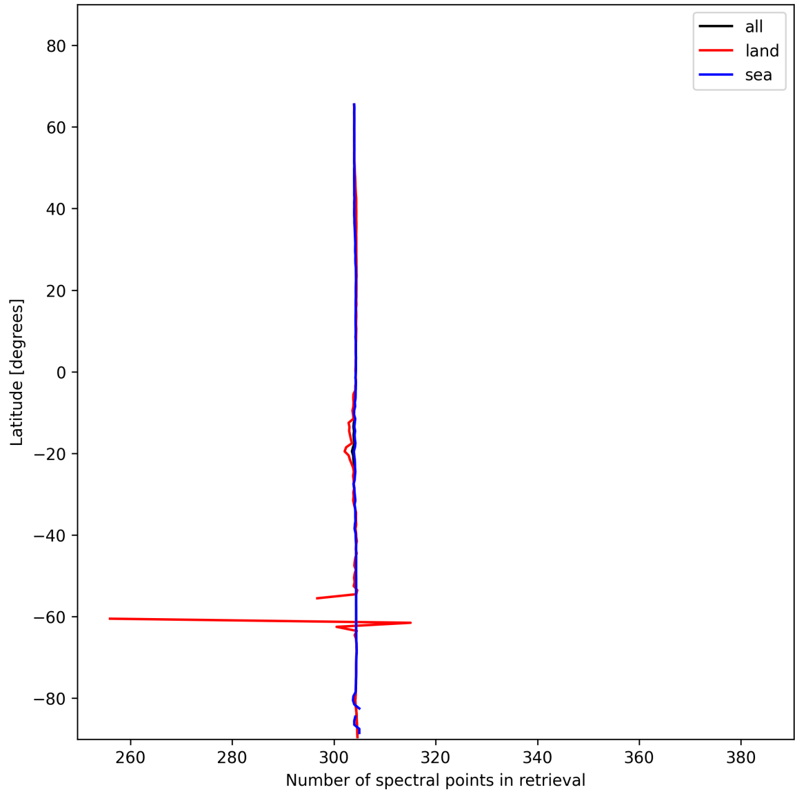
Figure 14: Zonal average of “Number of spectral points in retrieval” for 2025-01-02 to 2025-01-03.
