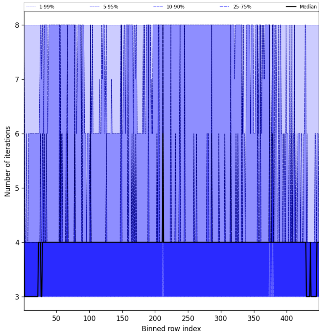
Figure 49: Along track statistics of “Number of iterations” for 2025-01-02 to 2025-01-03
