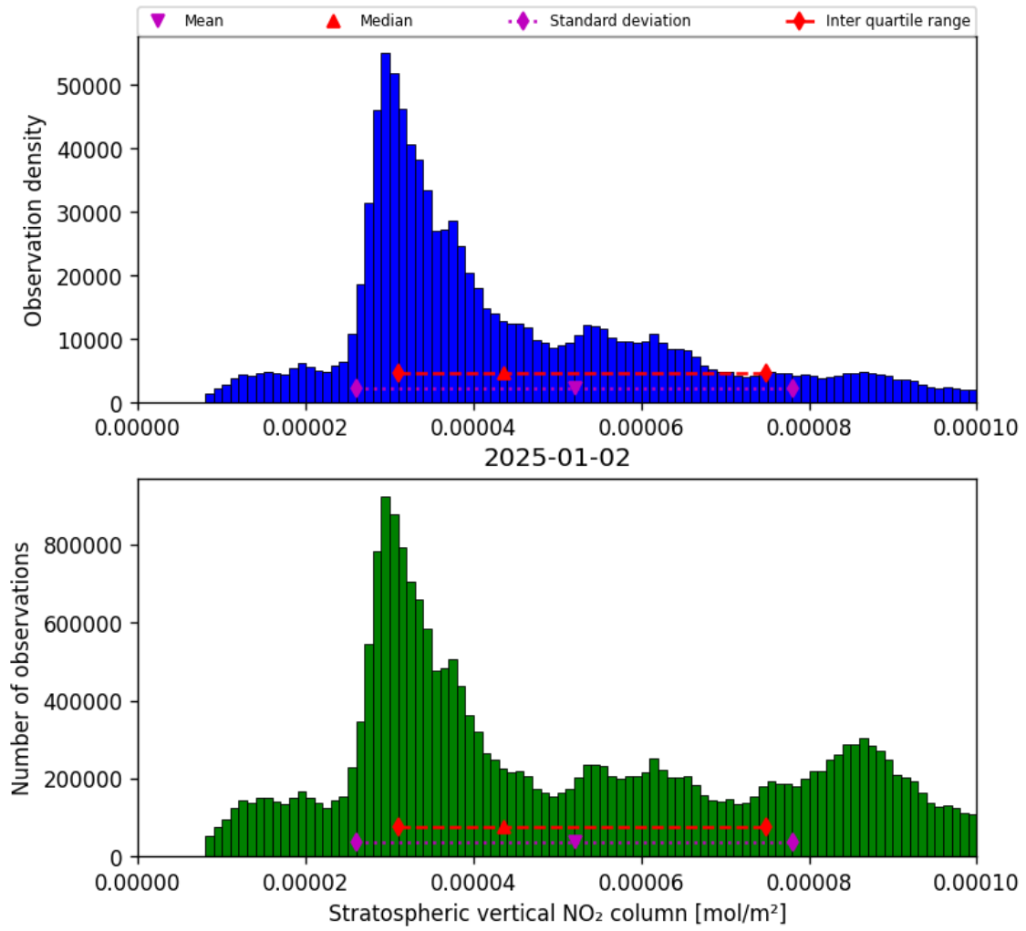
Figure 34: Histogram of “Stratospheric vertical NO 2 column” for 2025-01-02 to 2025-01-03
