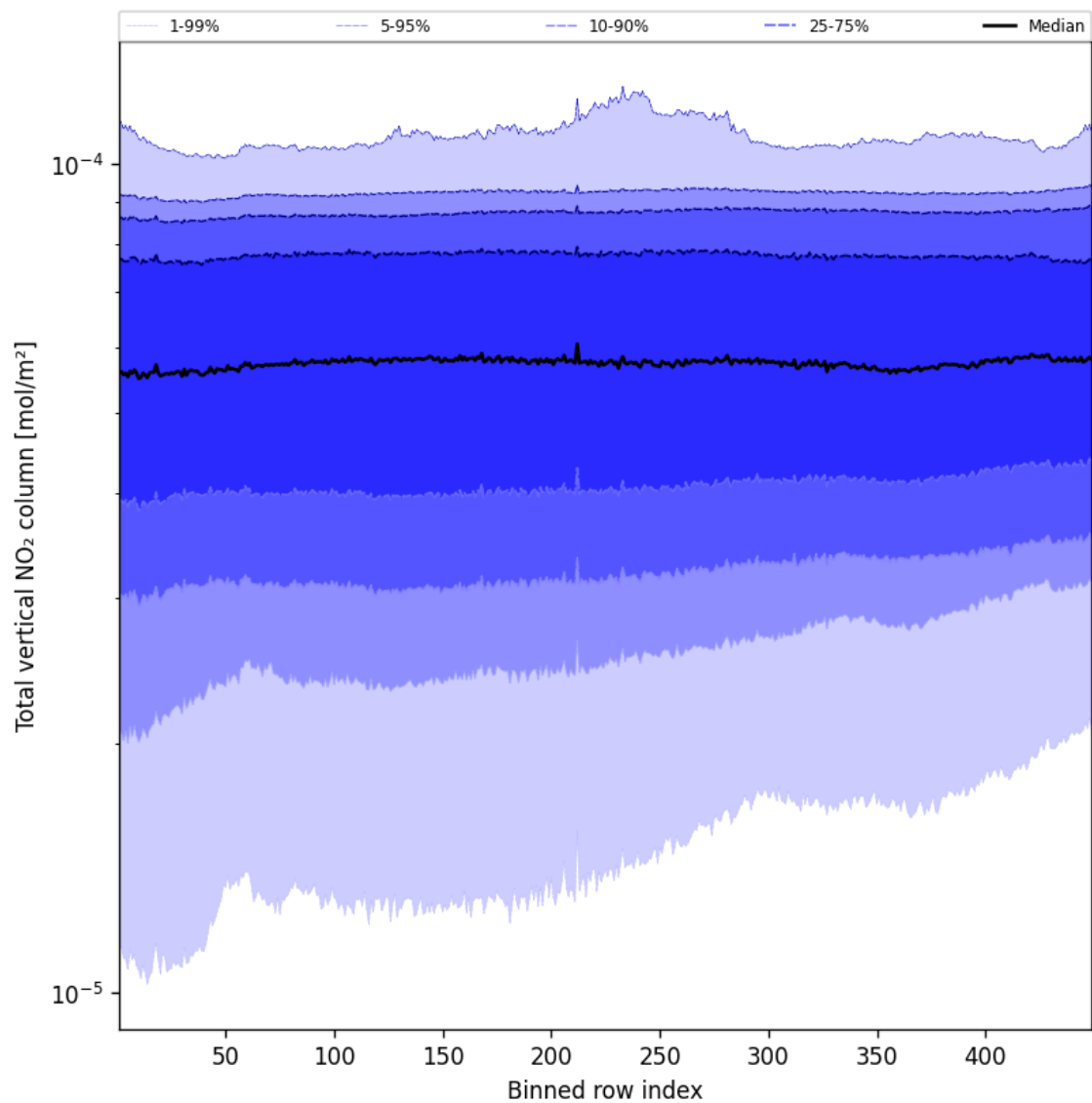
Figure 53: Along track statistics of “Total vertical NO 2 column” for 2025-01-02 to 2025-01-03
