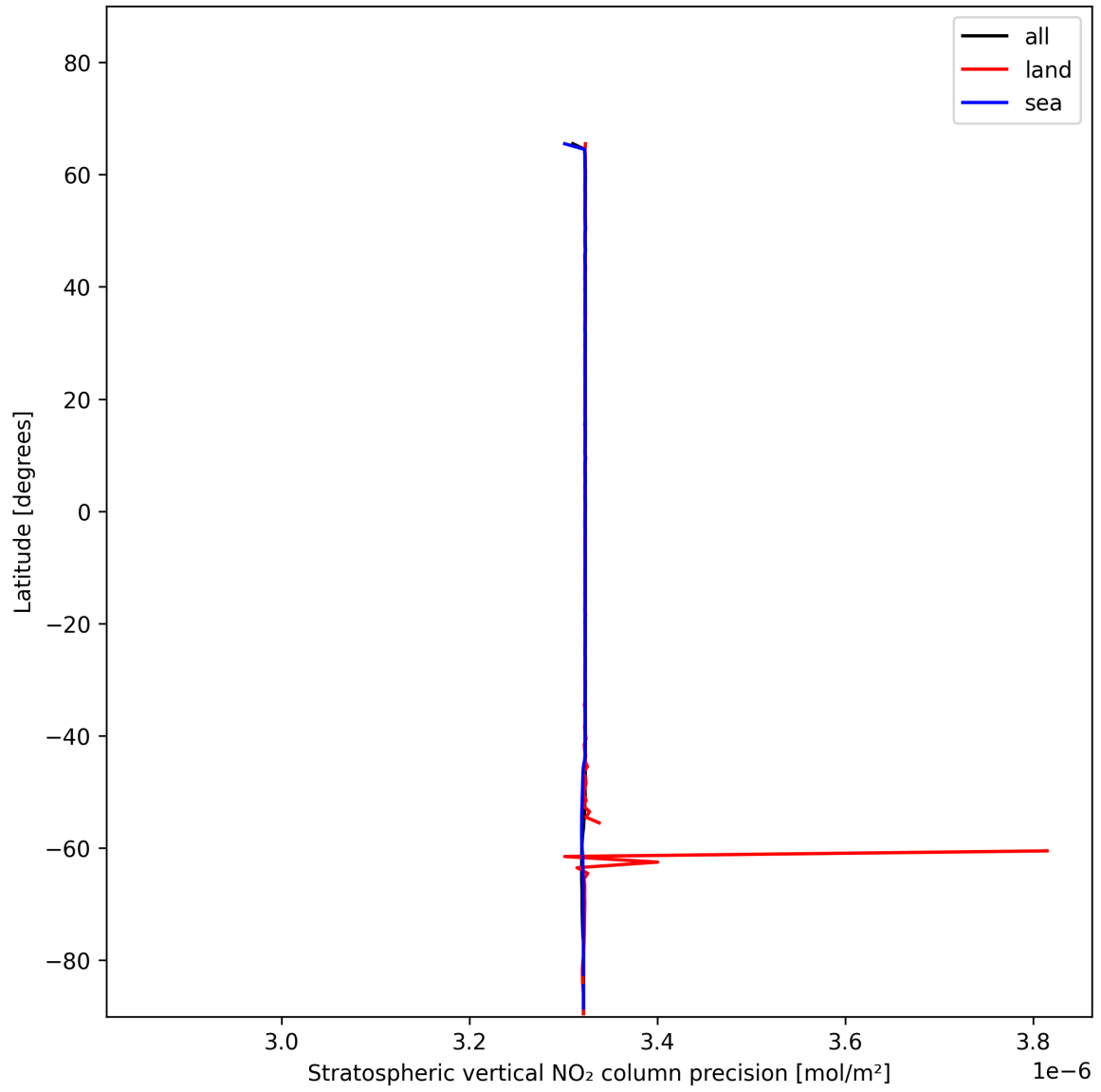
Figure 18: Zonal average of “Stratospheric vertical NO 2 column precision” for 2025-01-02 to 2025-01-03.
