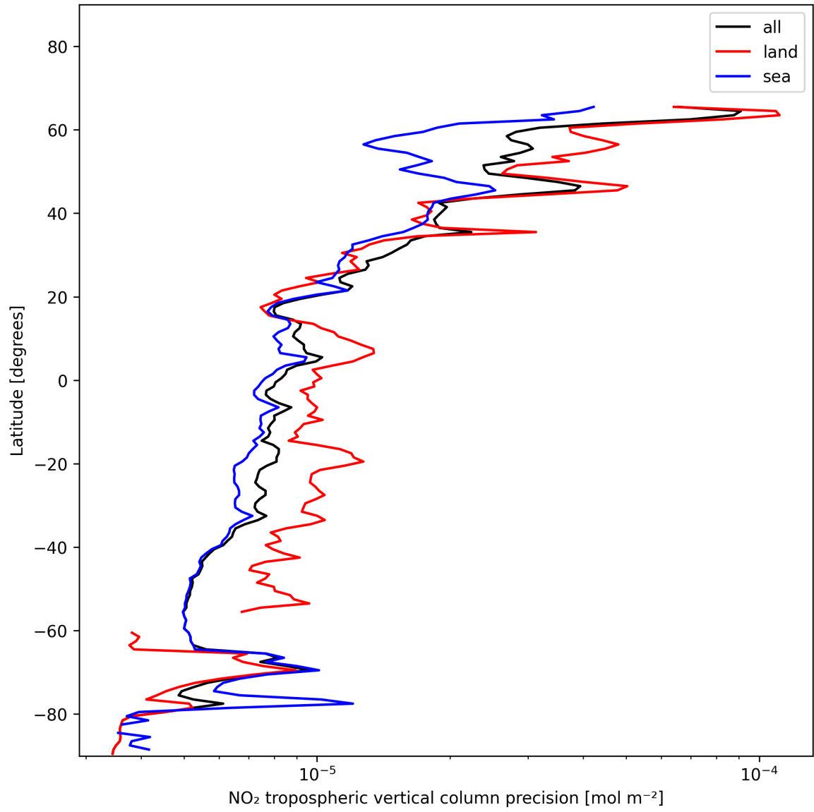
Figure 11: Zonal average of “NO 2 tropospheric vertical column precision” for 2025-01-02 to 2025-01-03.
