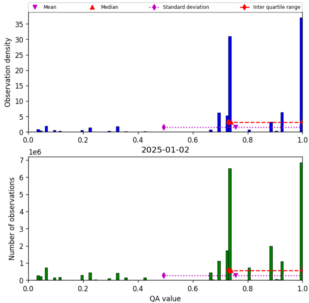
Figure 26: Histogram of “QA value” for 2025-01-02 to 2025-01-03
