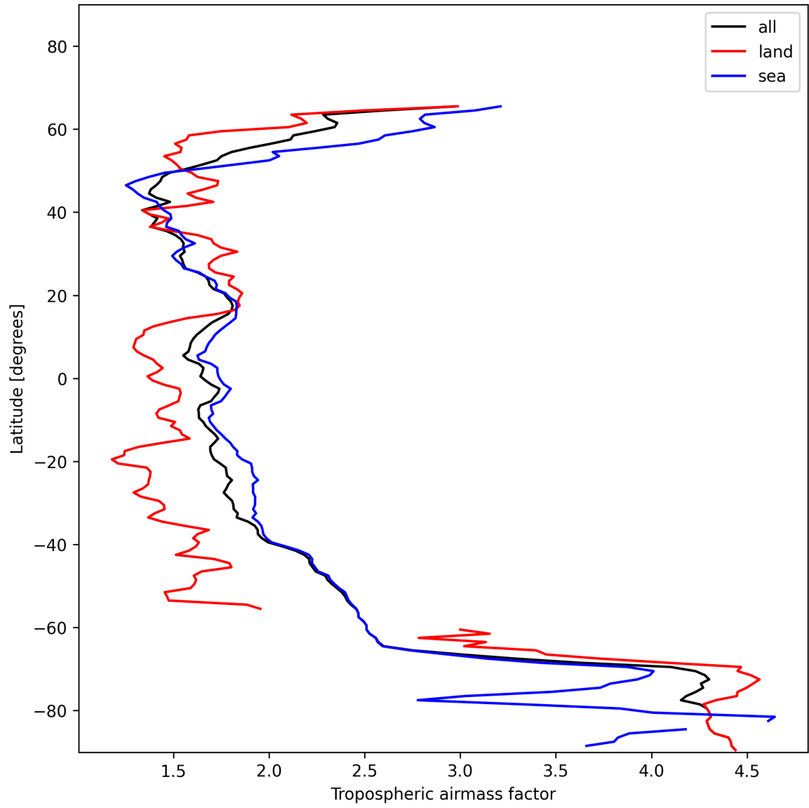
Figure 12: Zonal average of “Tropospheric airmass factor” for 2025-01-02 to 2025-01-03.
