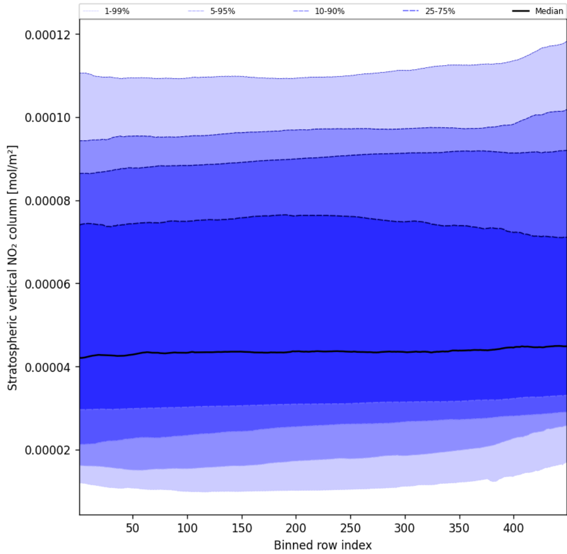
Figure 51: Along track statistics of “Stratospheric vertical NO 2 column” for 2025-01-02 to 2025-01-03
