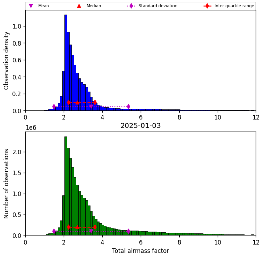
Figure 30: Histogram of “Total airmass factor” for 2025-01-03 to 2025-01-04
