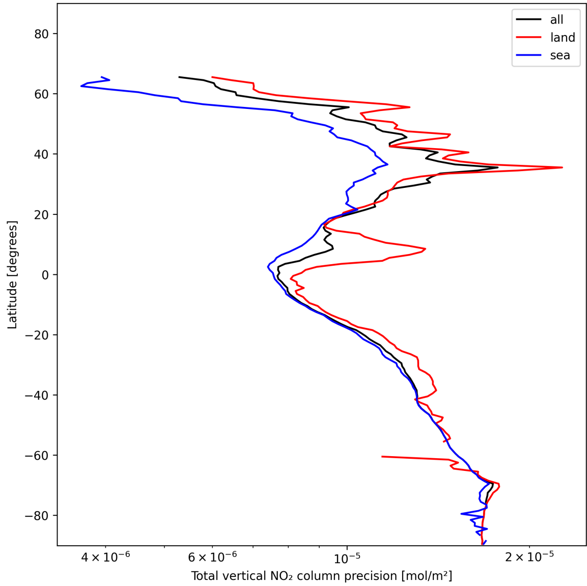
Figure 20: Zonal average of “Total vertical NO 2 column precision” for 2025-01-03 to 2025-01-04.
