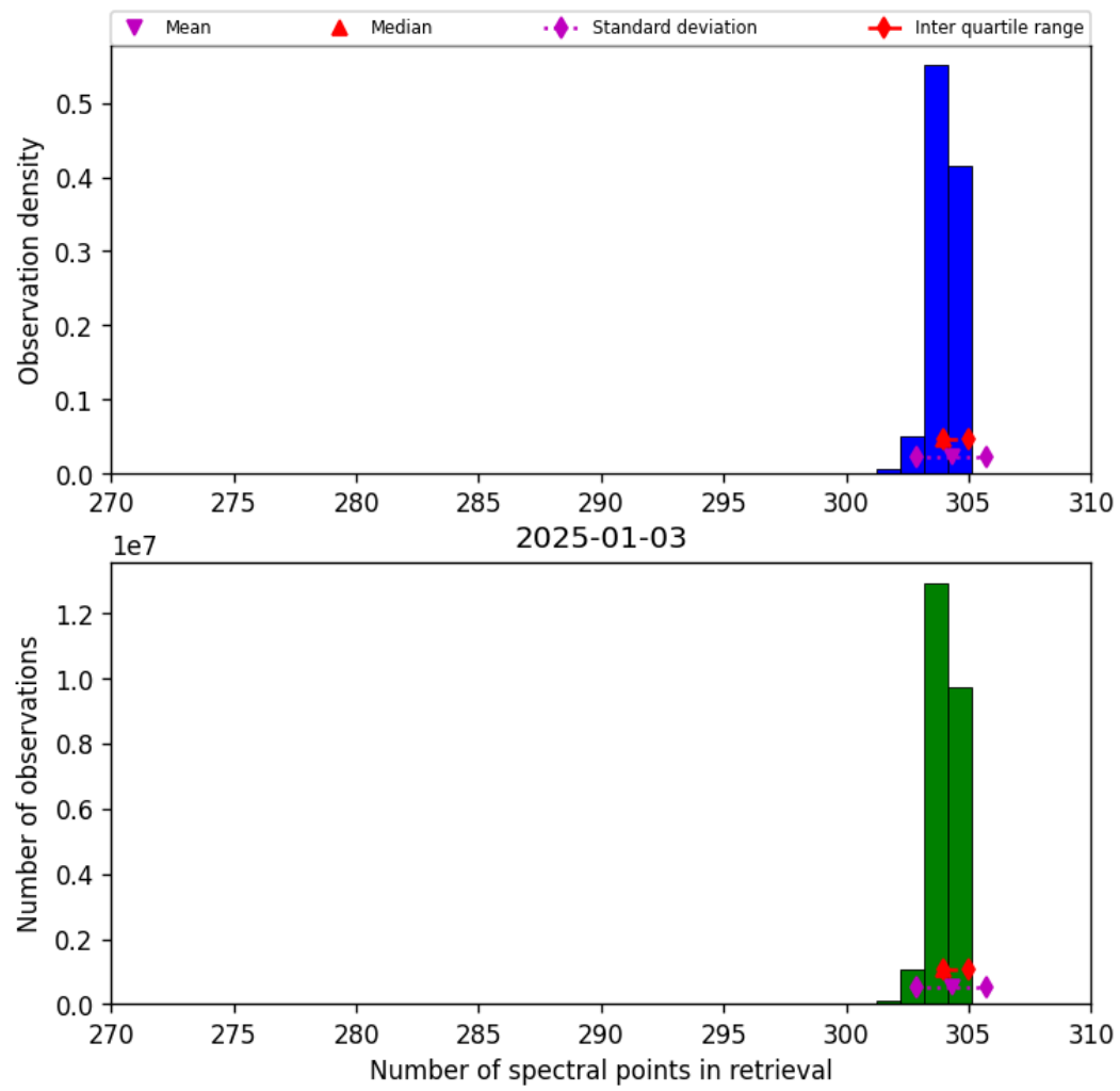
Figure 31: Histogram of “Number of spectral points in retrieval” for 2025-01-03 to 2025-01-04
