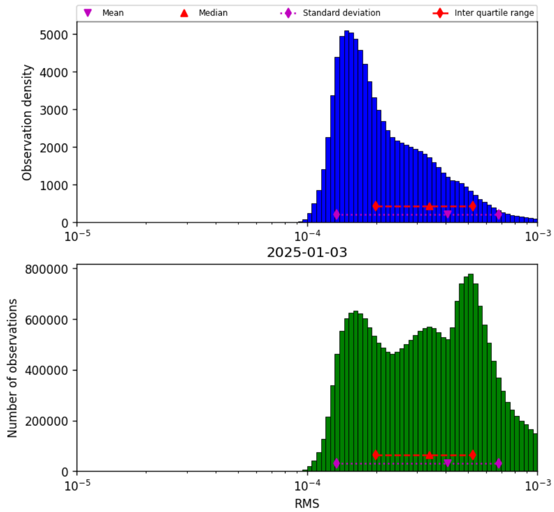
Figure 41: Histogram of “RMS” for 2025-01-03 to 2025-01-04
