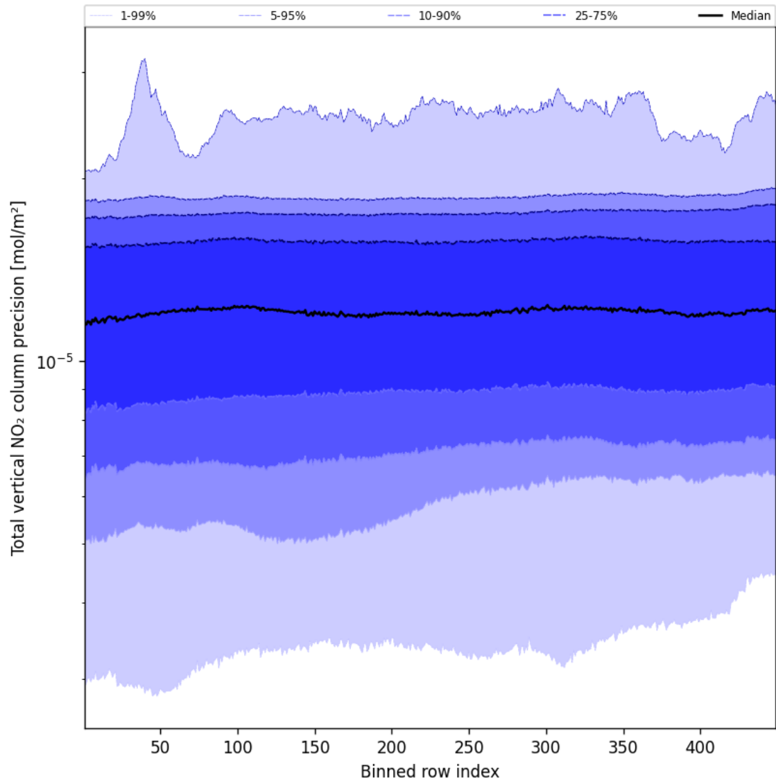
Figure 54: Along track statistics of “Total vertical NO 2 column precision” for 2025-01-03 to 2025-01-04
