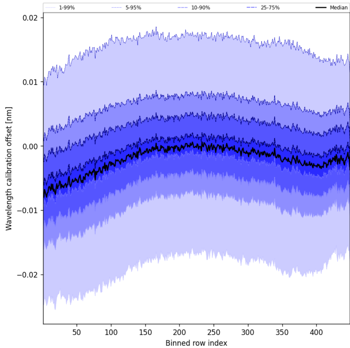
Figure 50: Along track statistics of “Wavelength calibration offset” for 2025-01-03 to 2025-01-04
