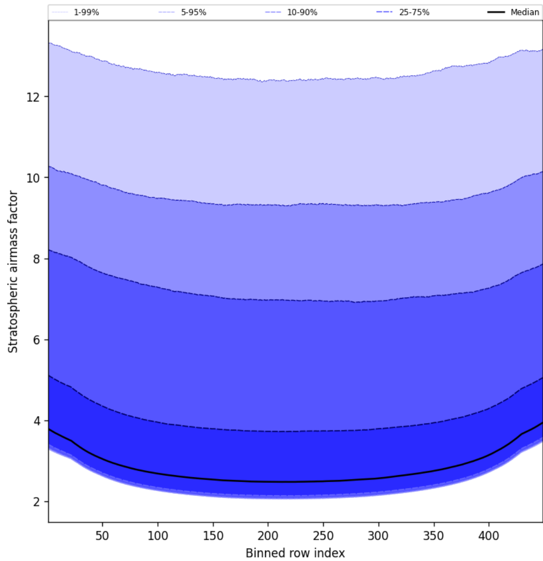
Figure 59: Along track statistics of “Stratospheric airmass factor” for 2025-01-03 to 2025-01-04
