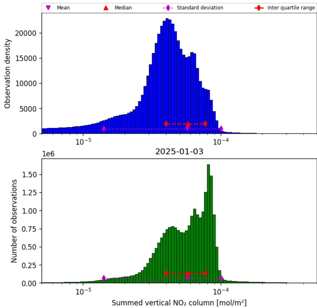
Figure 38: Histogram of “Summed vertical NO 2 column” for 2025-01-03 to 2025-01-04
