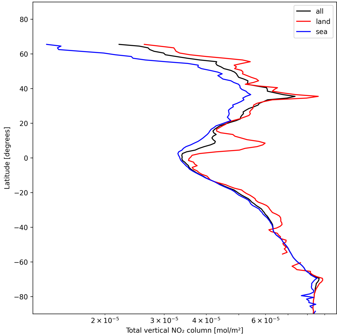
Figure 19: Zonal average of “Total vertical NO 2 column” for 2025-01-03 to 2025-01-04.
