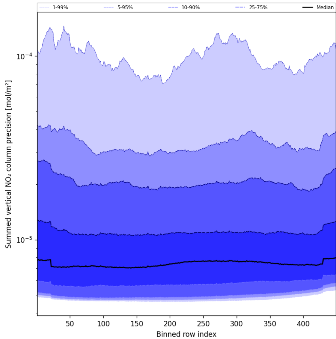
Figure 56: Along track statistics of “Summed vertical NO 2 column precision” for 2025-01-03 to 2025-01-04
