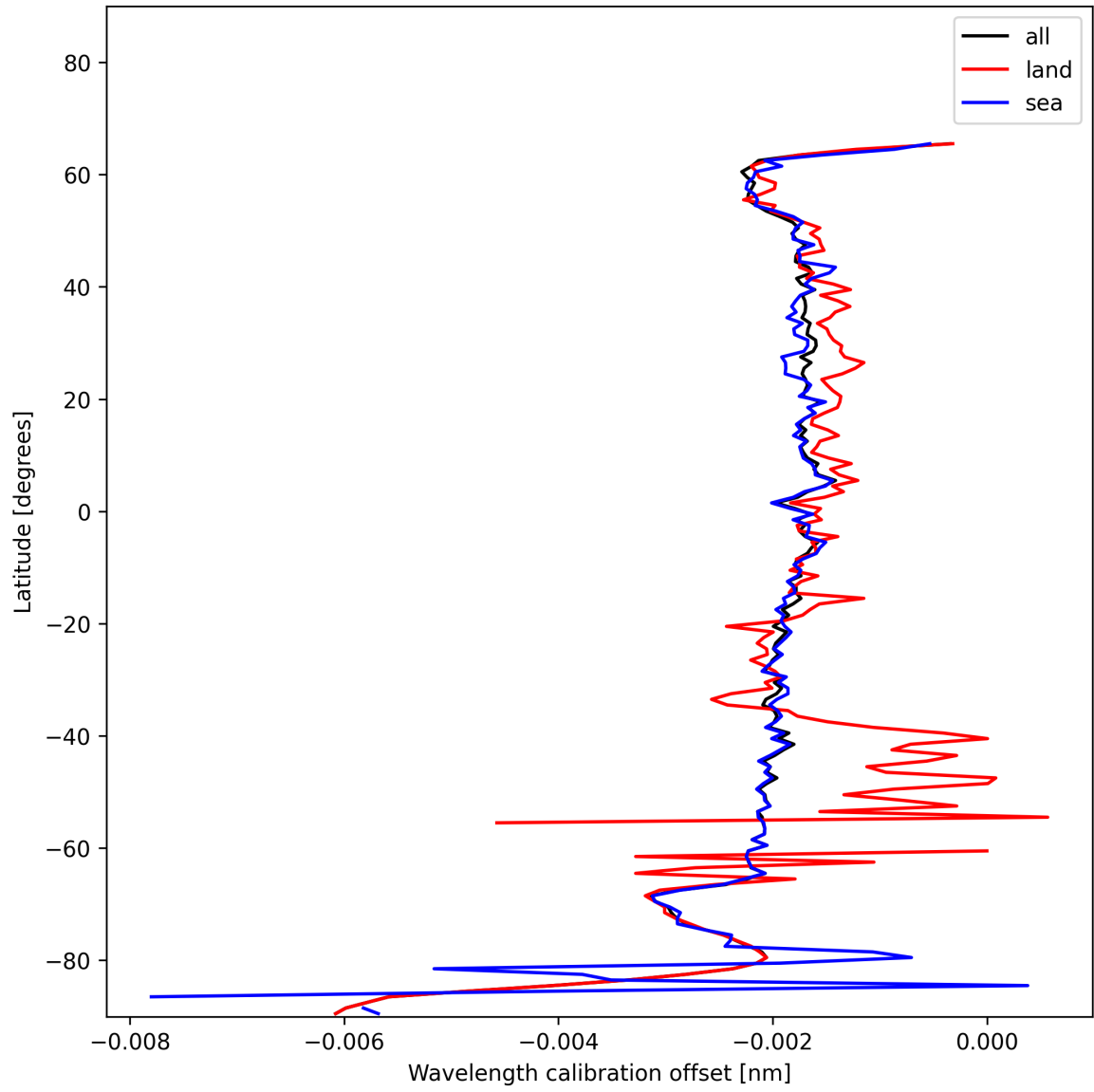
Figure 16: Zonal average of “Wavelength calibration offset” for 2025-01-03 to 2025-01-04.
