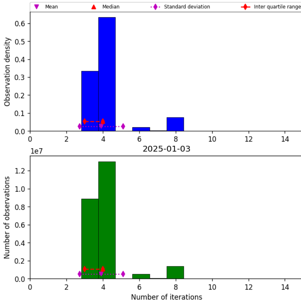
Figure 32: Histogram of “Number of iterations” for 2025-01-03 to 2025-01-04
