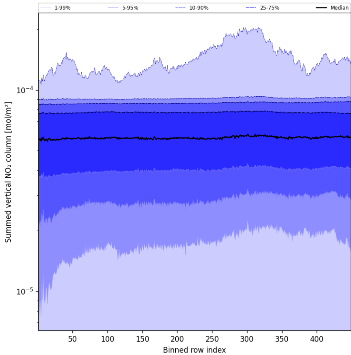
Figure 55: Along track statistics of “Summed vertical NO 2 column” for 2025-01-03 to 2025-01-04
