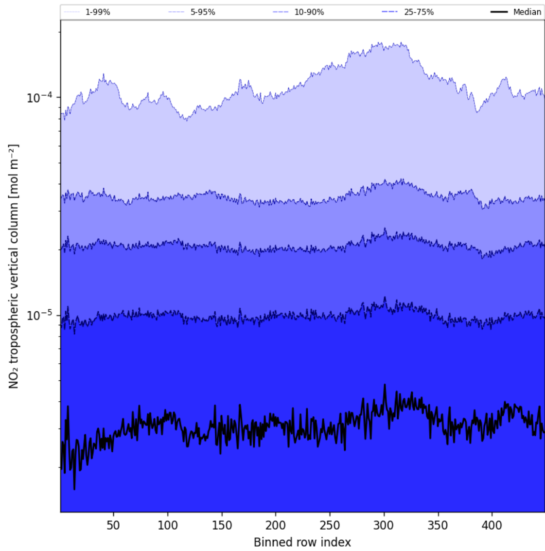
Figure 44: Along track statistics of “NO 2 tropospheric vertical column” for 2025-01-03 to 2025-01-04
