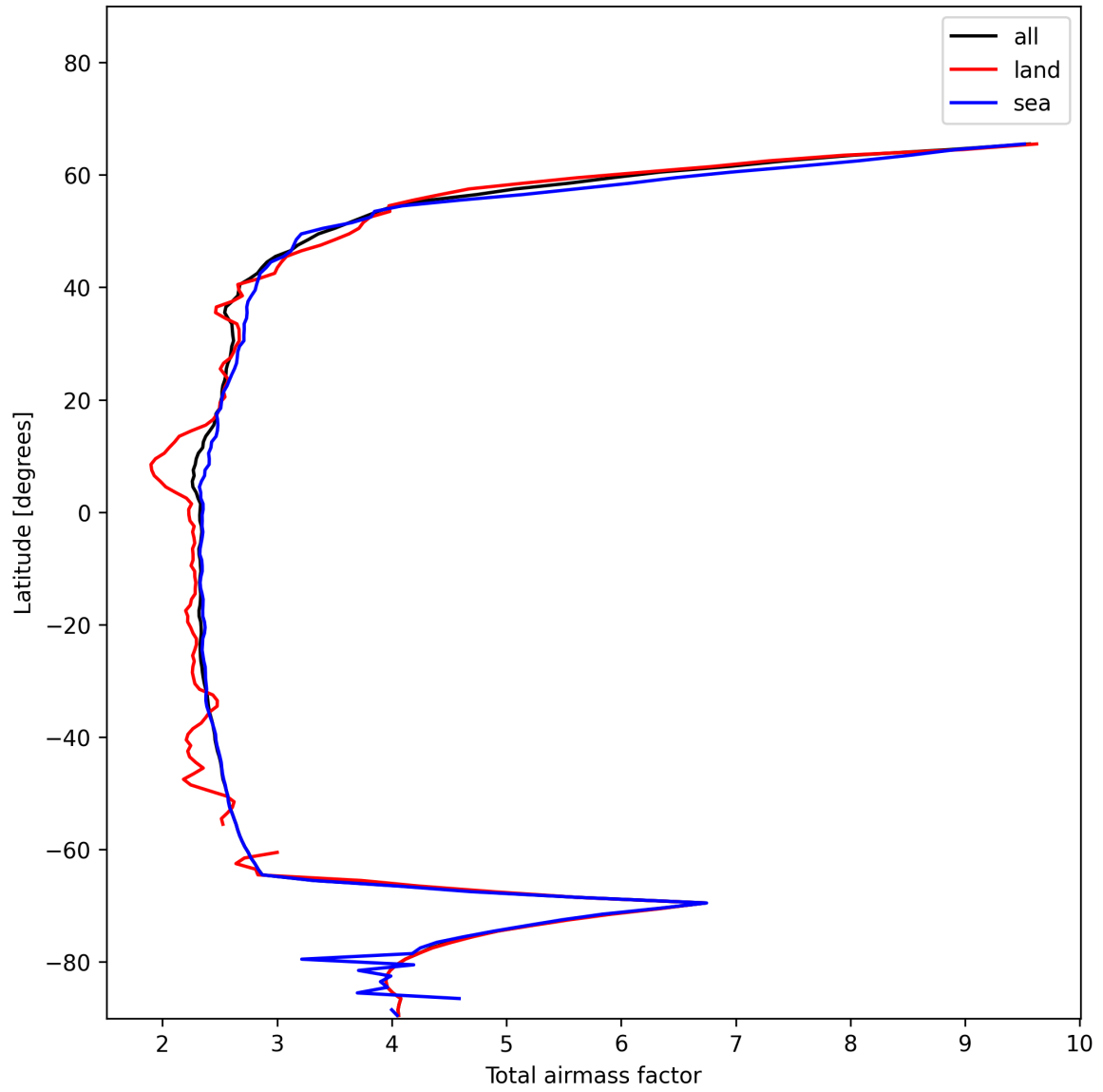
Figure 13: Zonal average of “Total airmass factor” for 2025-01-03 to 2025-01-04.
