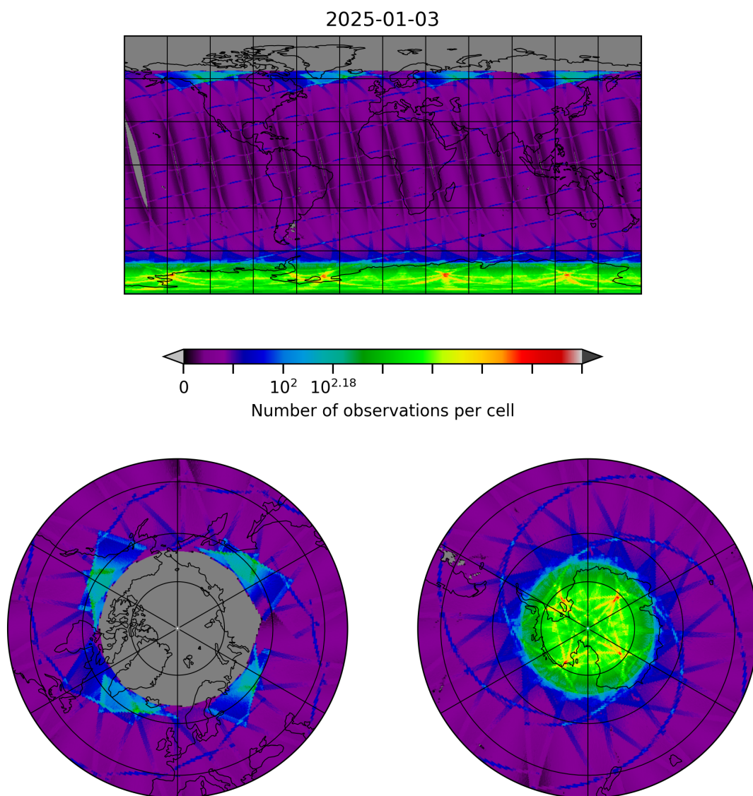
Figure 8: Map of the number of observations for 2025-01-03 to 2025-01-04
