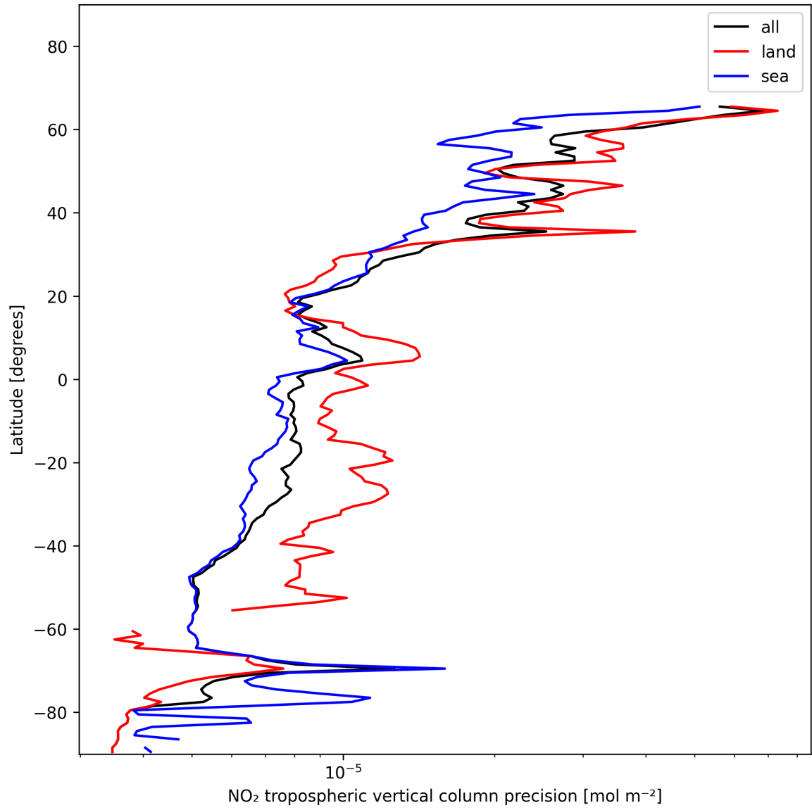
Figure 11: Zonal average of “NO 2 tropospheric vertical column precision” for 2025-01-03 to 2025-01-04.
