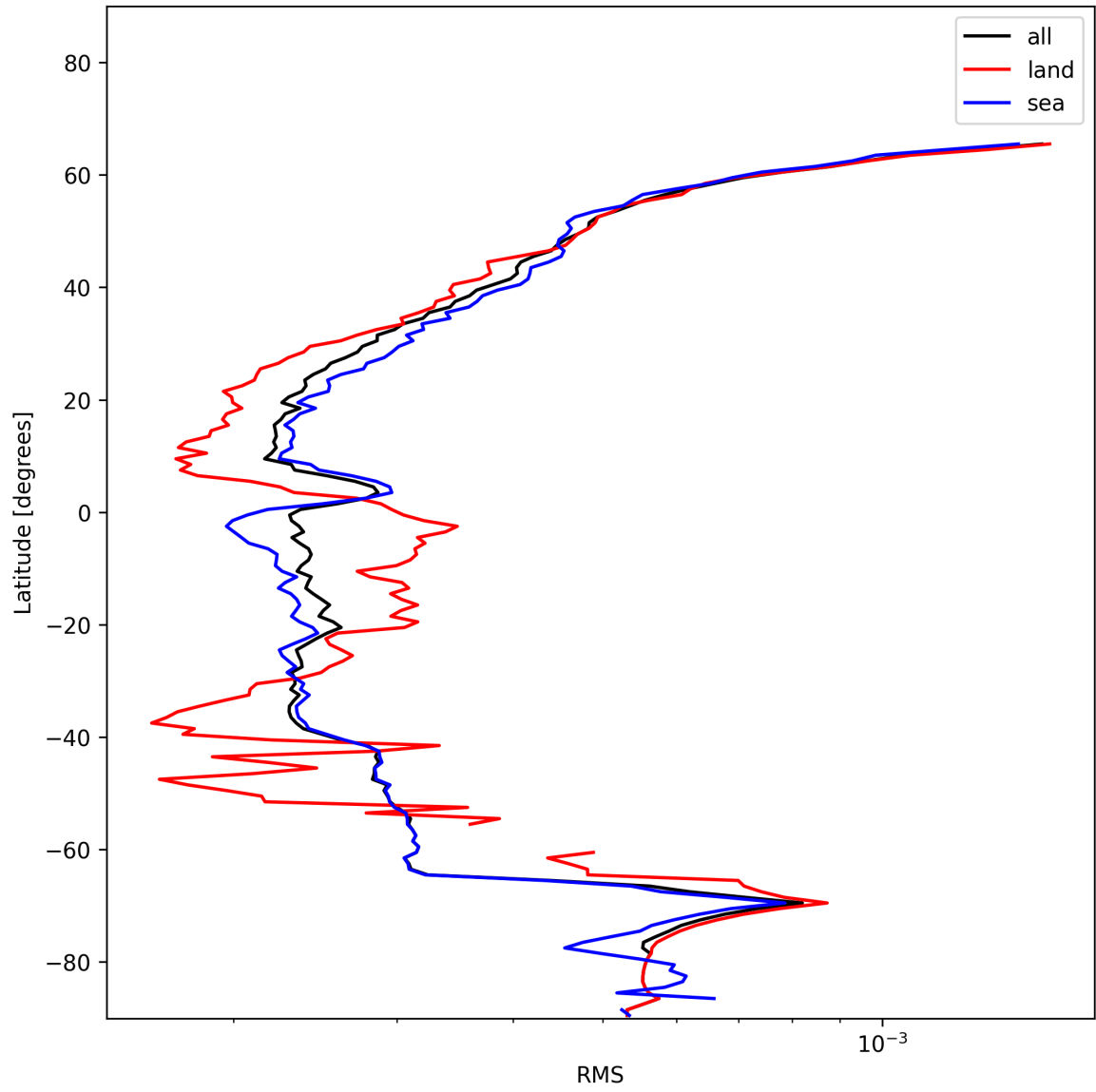
Figure 24: Zonal average of “RMS” for 2025-01-03 to 2025-01-04.
