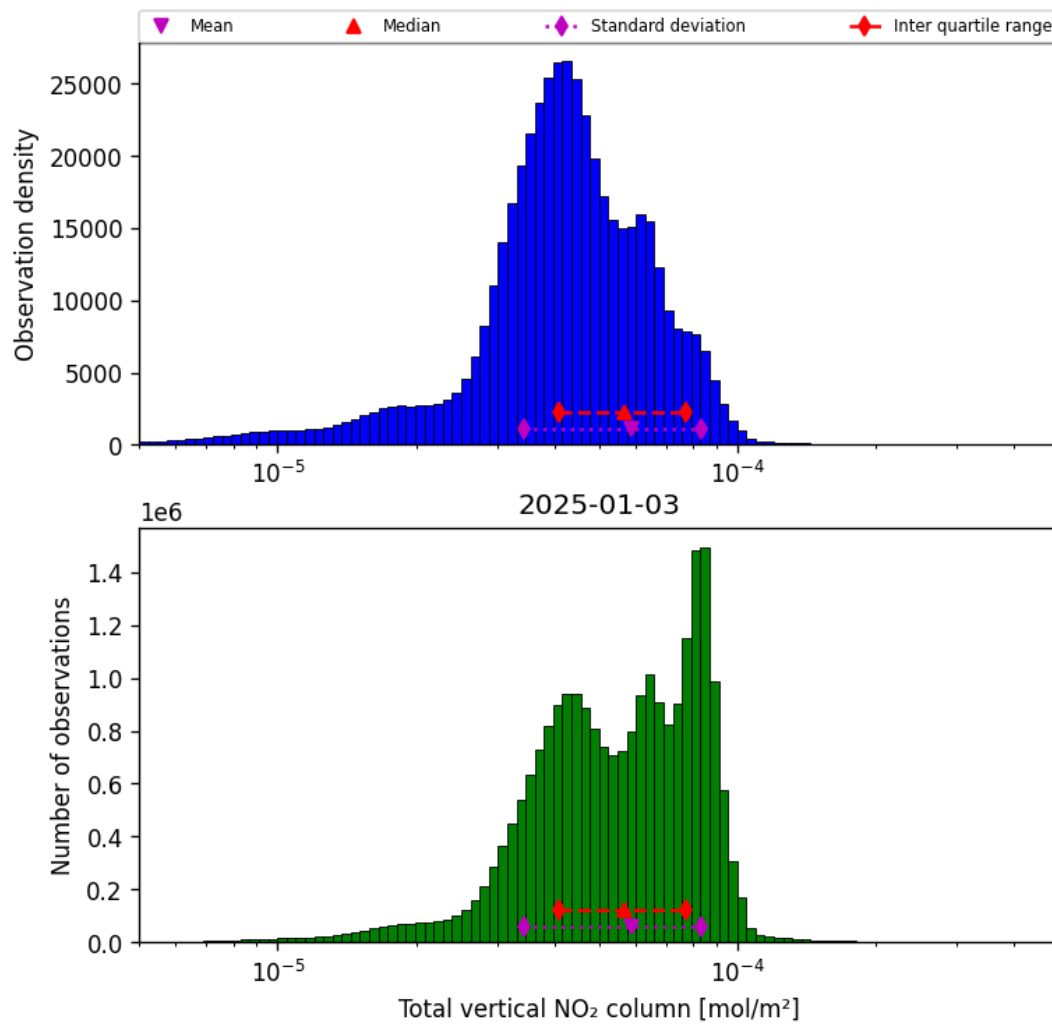
Figure 36: Histogram of “Total vertical NO 2 column” for 2025-01-03 to 2025-01-04
