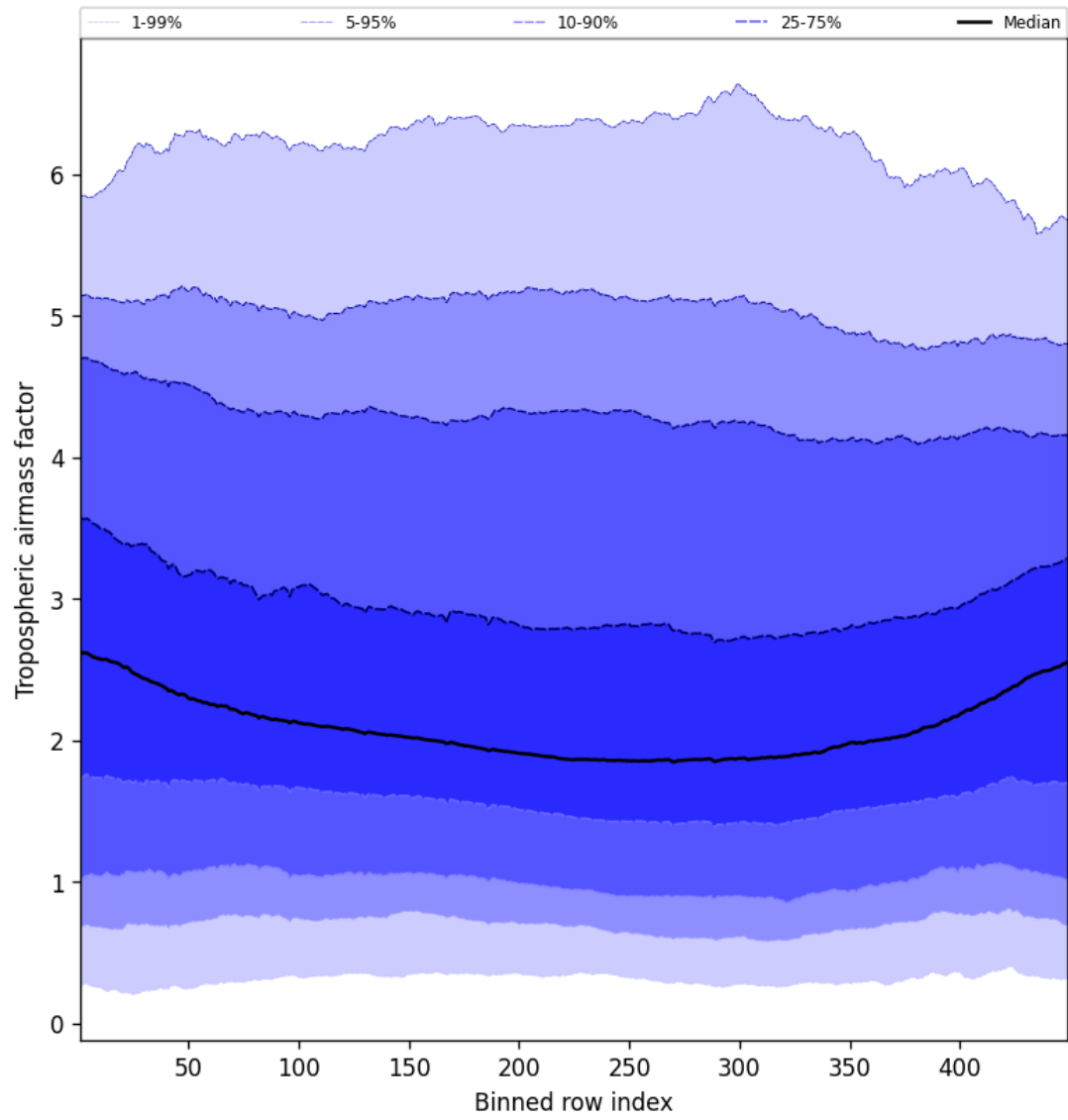
Figure 46: Along track statistics of “Tropospheric airmass factor” for 2025-01-03 to 2025-01-04
