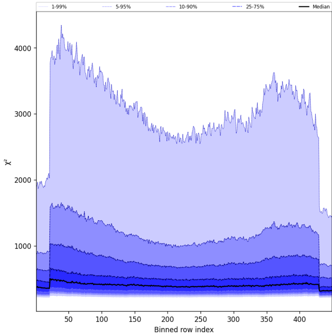
Figure 57: Along track statistics of “ \chi^2 ” for 2025-01-03 to 2025-01-04
