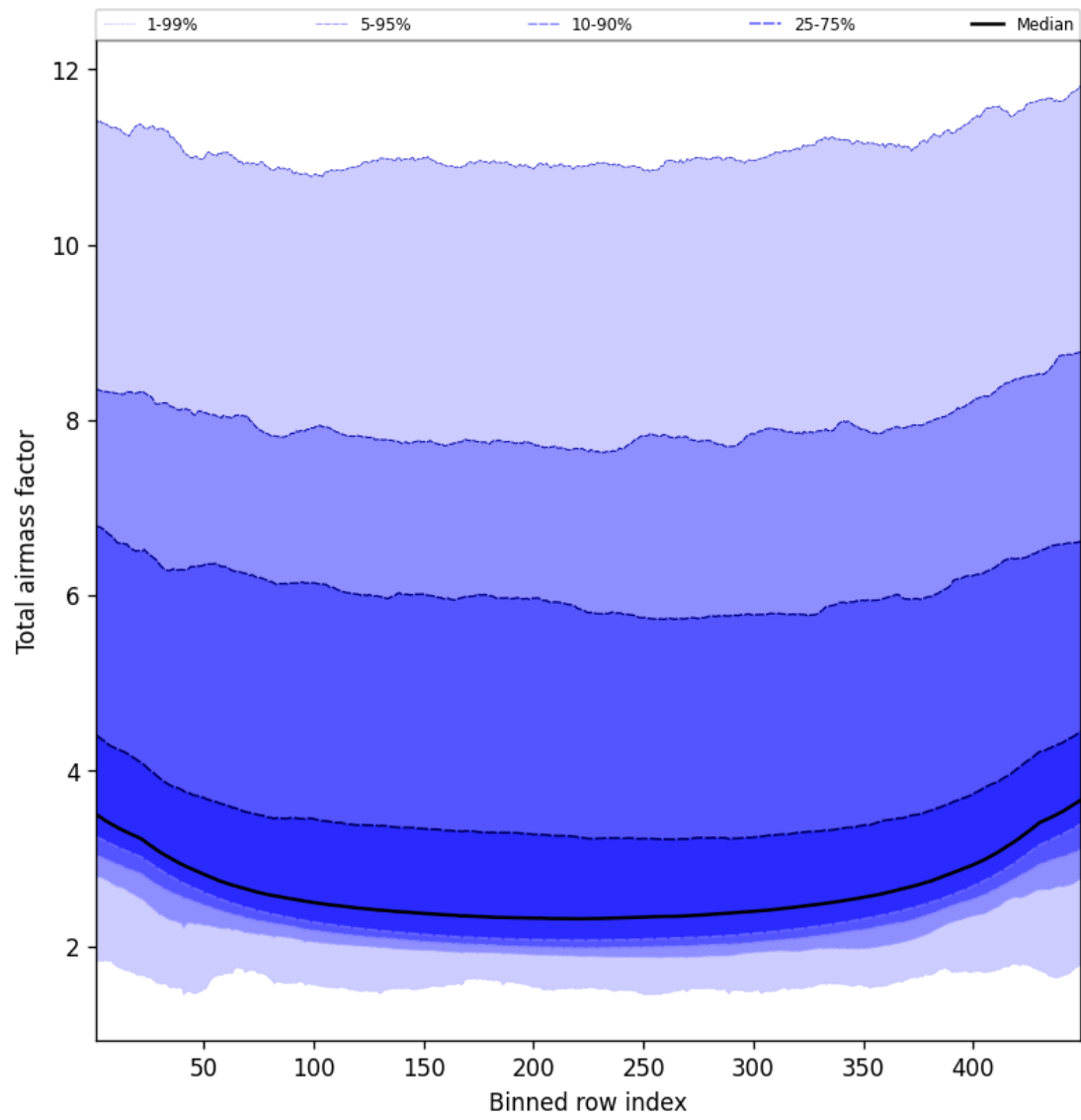
Figure 47: Along track statistics of “Total airmass factor” for 2025-01-03 to 2025-01-04
