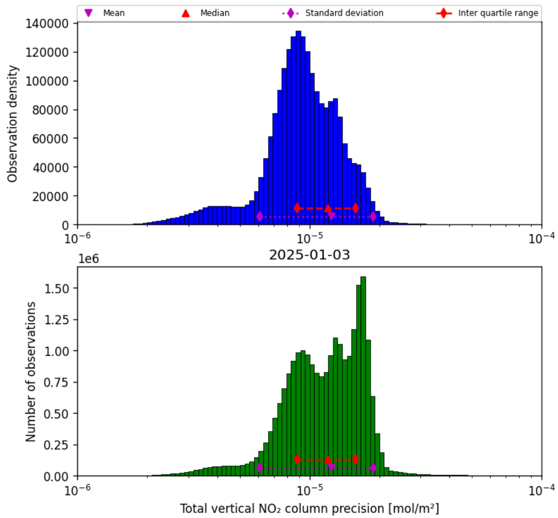
Figure 37: Histogram of “Total vertical NO 2 column precision” for 2025-01-03 to 2025-01-04
