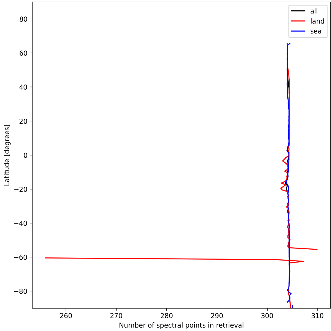
Figure 14: Zonal average of “Number of spectral points in retrieval” for 2025-01-03 to 2025-01-04.
