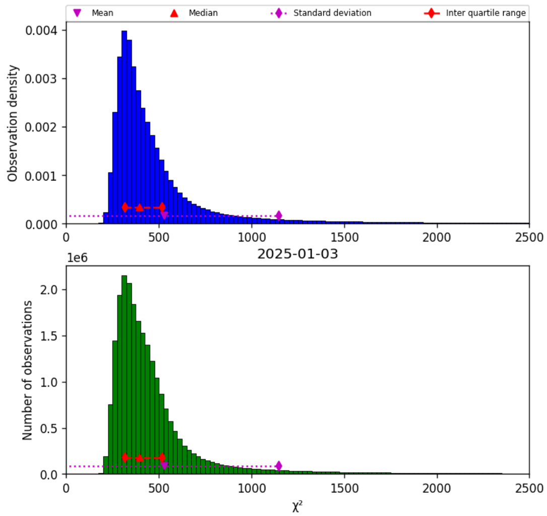
Figure 40: Histogram of “ \chi^2 ” for 2025-01-03 to 2025-01-04
