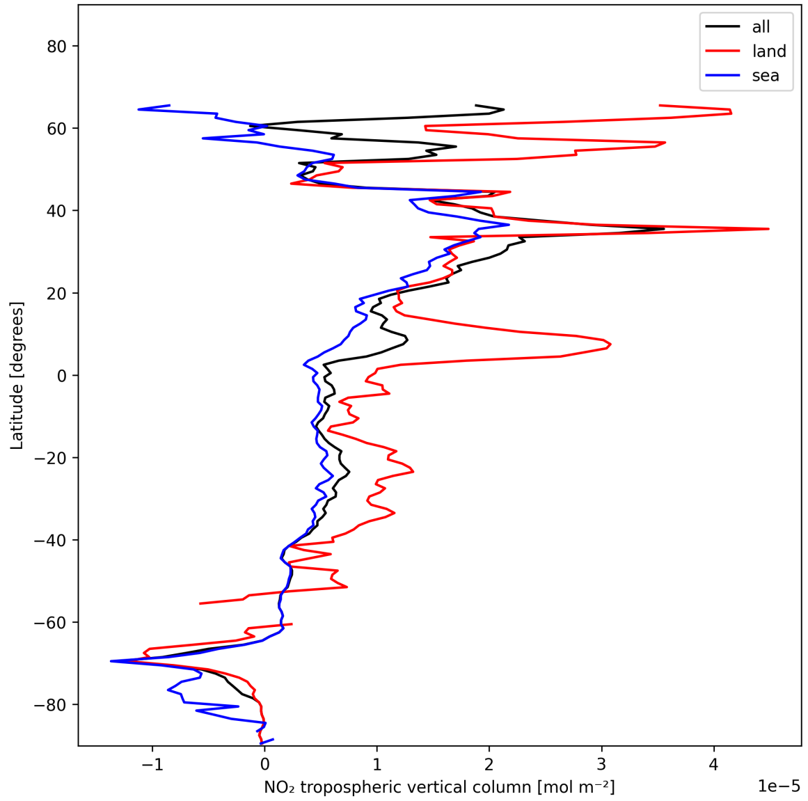
Figure 10: Zonal average of “NO 2 tropospheric vertical column” for 2025-01-03 to 2025-01-04.
