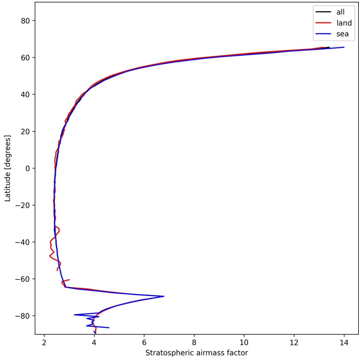
Figure 25: Zonal average of “Stratospheric airmass factor” for 2025-01-03 to 2025-01-04.
