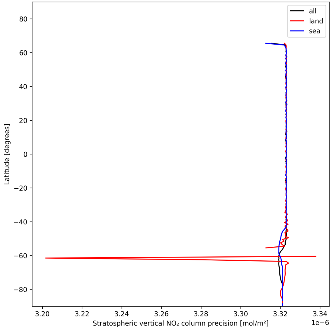
Figure 18: Zonal average of “Stratospheric vertical NO 2 column precision” for 2025-01-03 to 2025-01-04.
