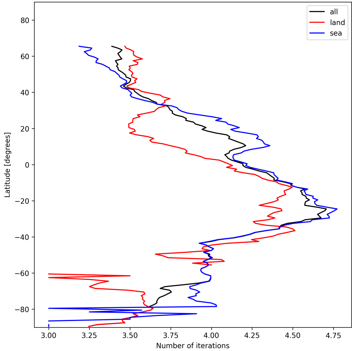
Figure 15: Zonal average of “Number of iterations” for 2025-01-03 to 2025-01-04.
