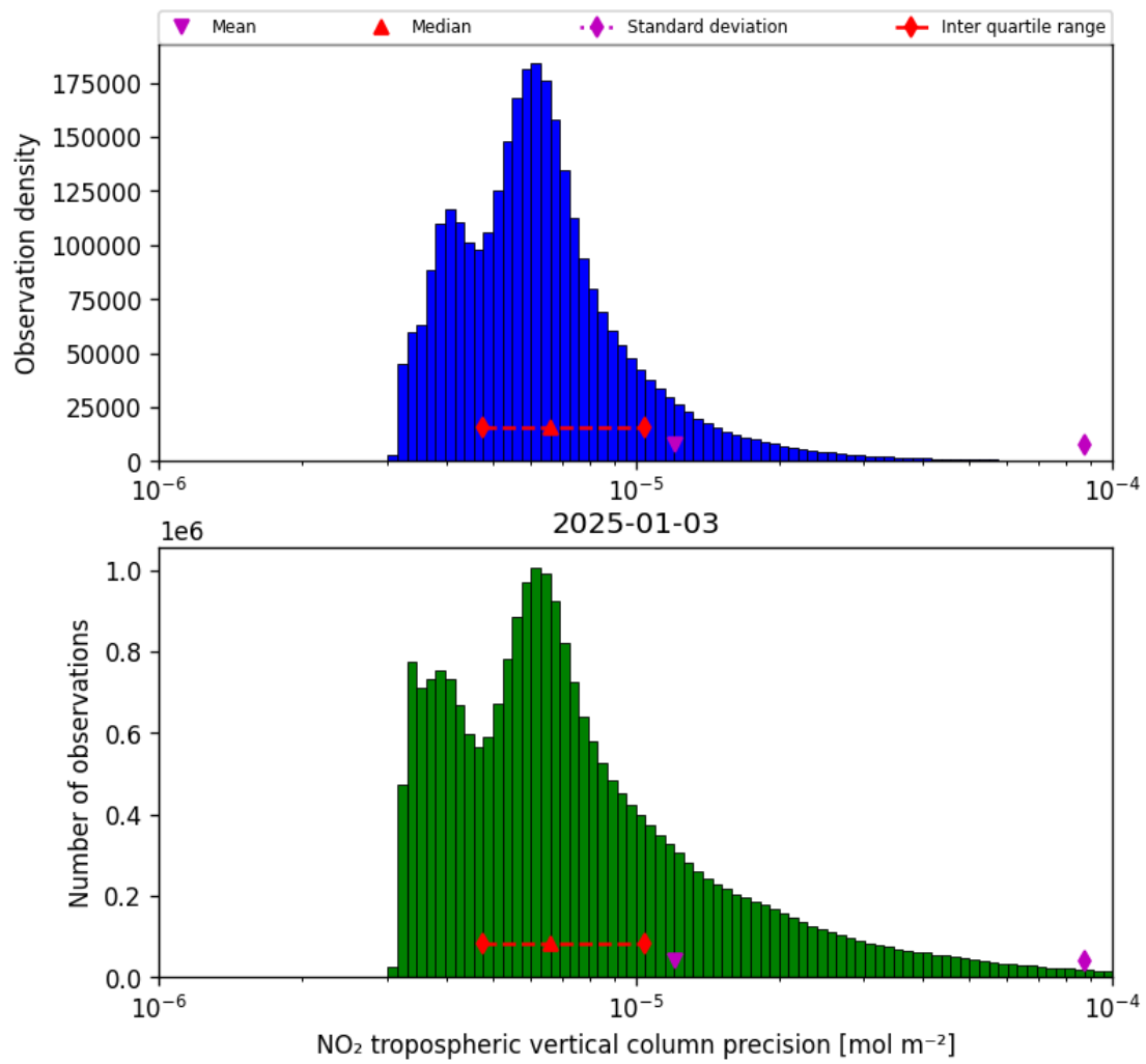
Figure 28: Histogram of “NO 2 tropospheric vertical column precision” for 2025-01-03 to 2025-01-04
