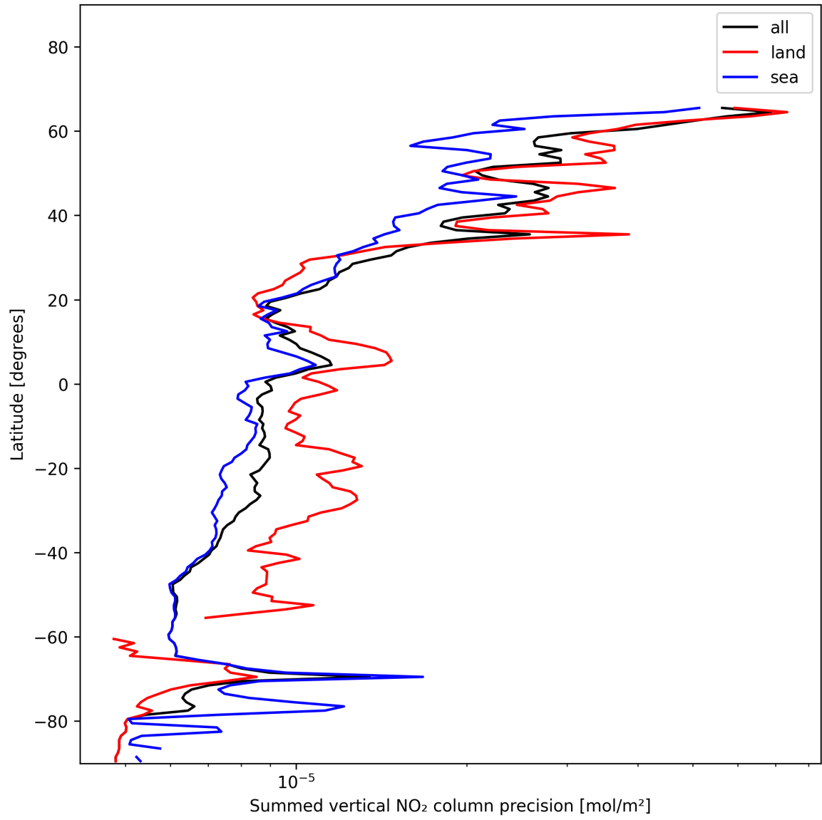
Figure 22: Zonal average of “Summed vertical NO 2 column precision” for 2025-01-03 to 2025-01-04.
