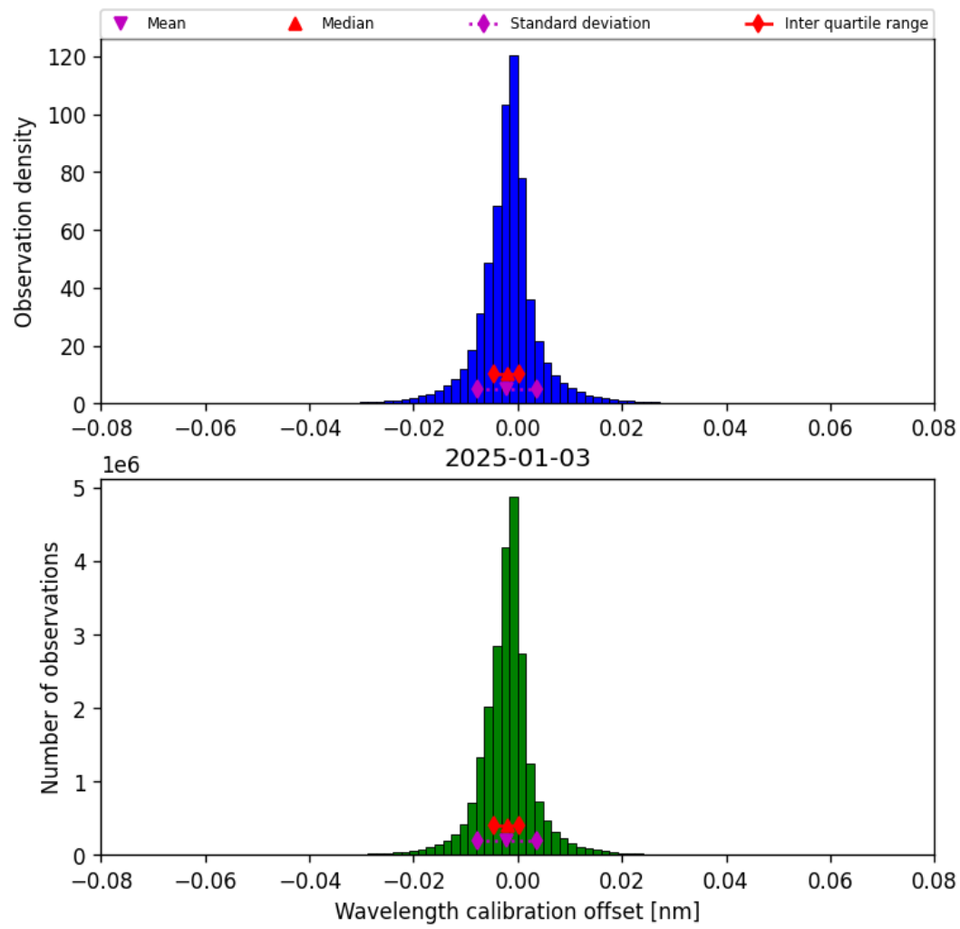
Figure 33: Histogram of “Wavelength calibration offset” for 2025-01-03 to 2025-01-04
