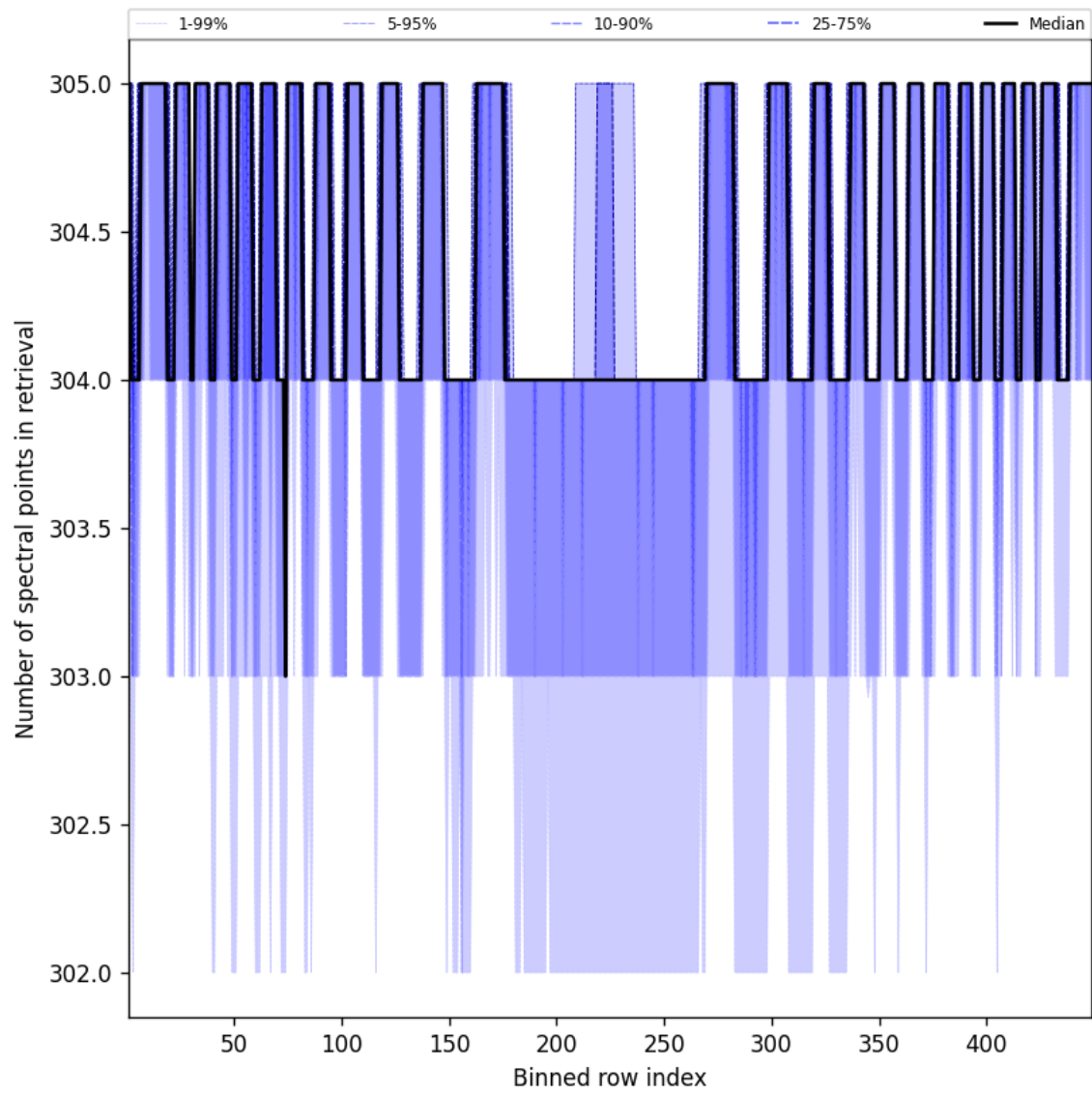
Figure 48: Along track statistics of “Number of spectral points in retrieval” for 2025-01-03 to 2025-01-04
