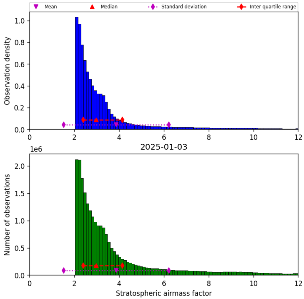
Figure 42: Histogram of “Stratospheric airmass factor” for 2025-01-03 to 2025-01-04
