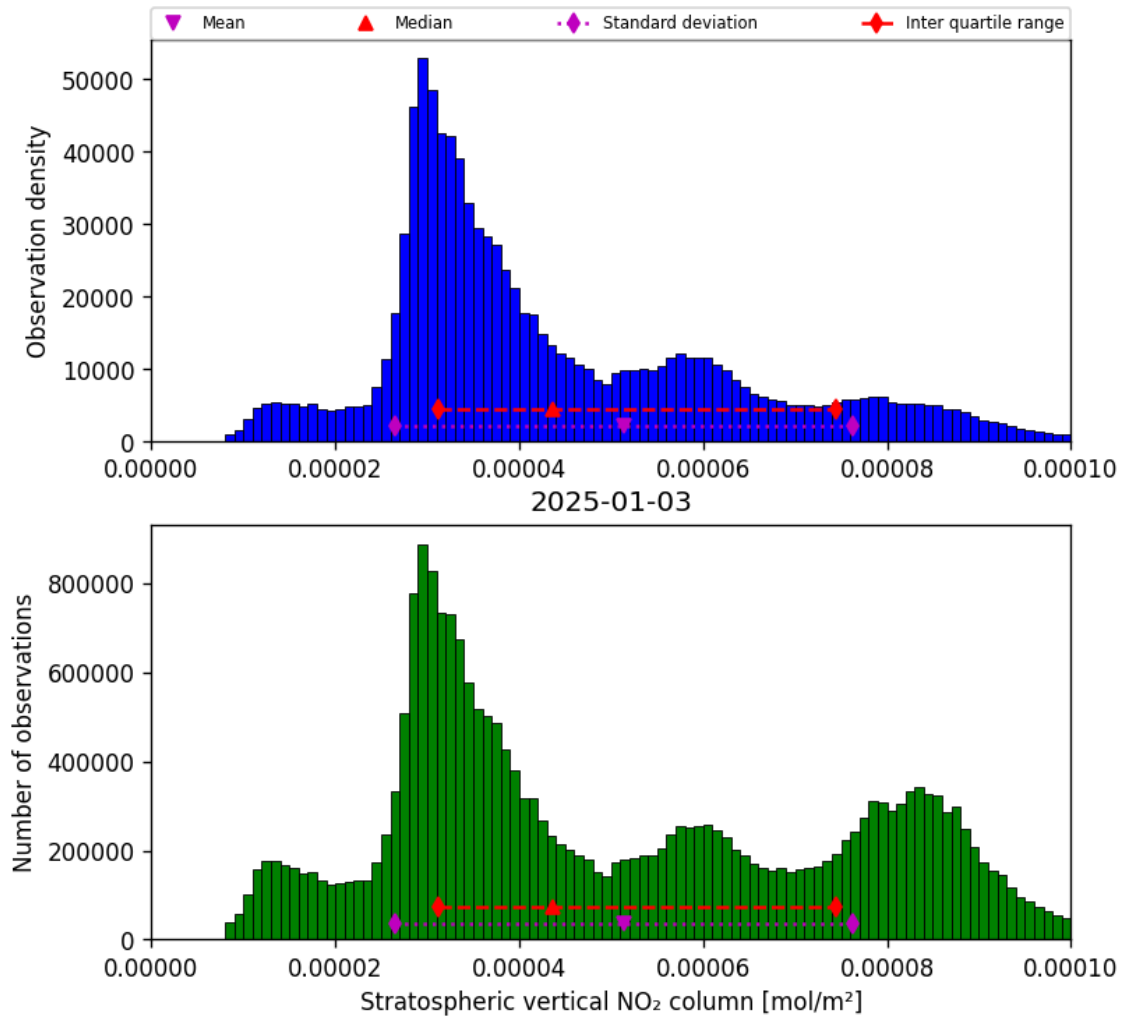
Figure 34: Histogram of “Stratospheric vertical NO 2 column” for 2025-01-03 to 2025-01-04
