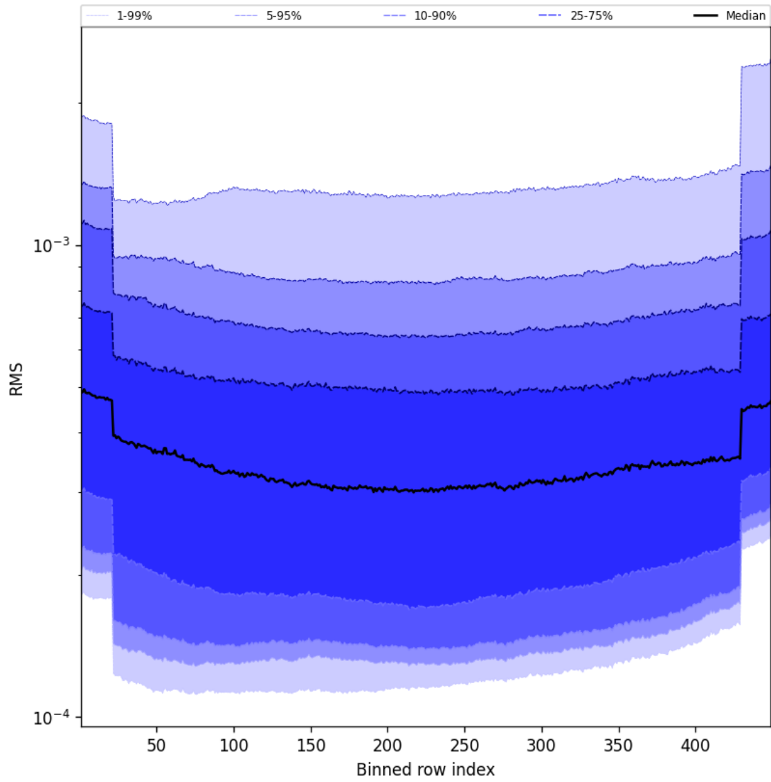
Figure 58: Along track statistics of “RMS” for 2025-01-03 to 2025-01-04
