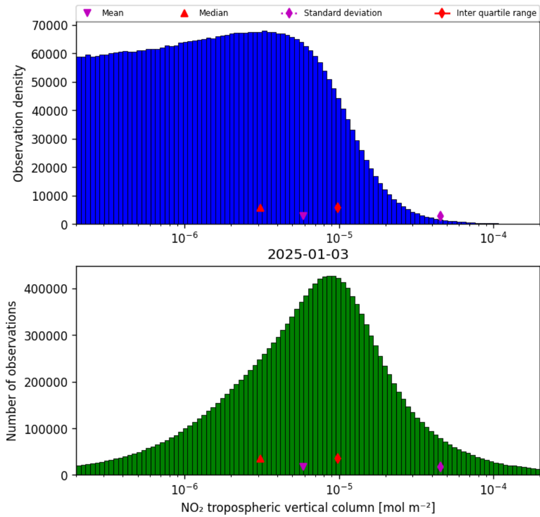
Figure 27: Histogram of “NO 2 tropospheric vertical column” for 2025-01-03 to 2025-01-04
