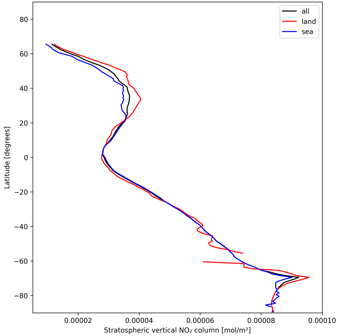
Figure 17: Zonal average of “Stratospheric vertical NO 2 column” for 2025-01-03 to 2025-01-04.
