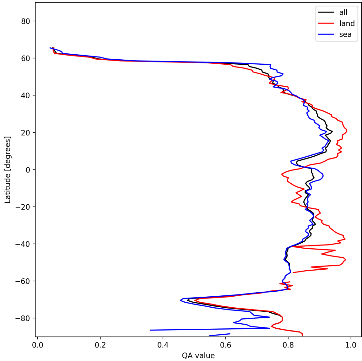
Figure 9: Zonal average of “QA value” for 2025-01-03 to 2025-01-04.
