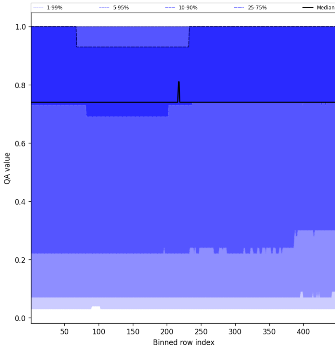
Figure 43: Along track statistics of “QA value” for 2025-01-03 to 2025-01-04
