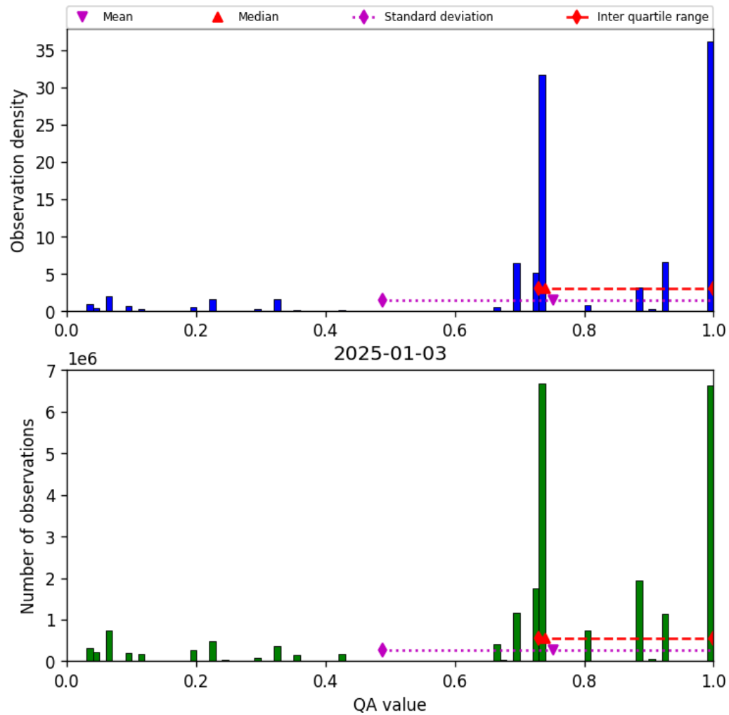
Figure 26: Histogram of “QA value” for 2025-01-03 to 2025-01-04
