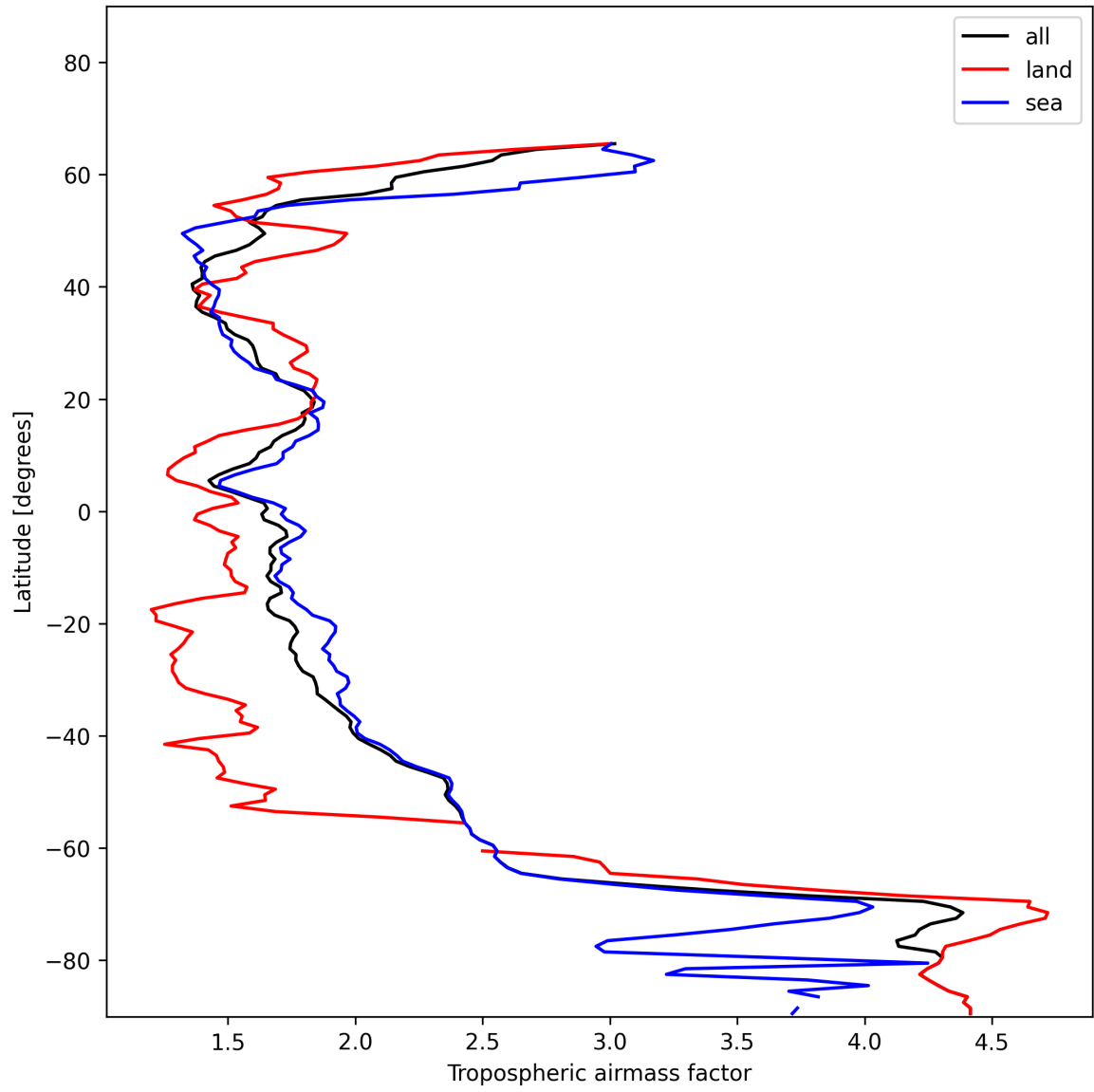
Figure 12: Zonal average of “Tropospheric airmass factor” for 2025-01-03 to 2025-01-04.
