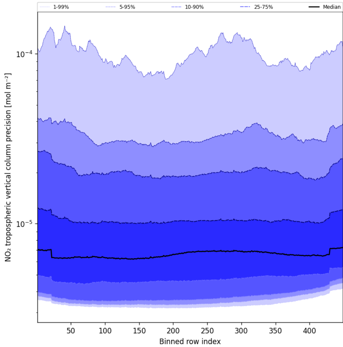
Figure 45: Along track statistics of “NO 2 tropospheric vertical column precision” for 2025-01-03 to 2025-01-04
