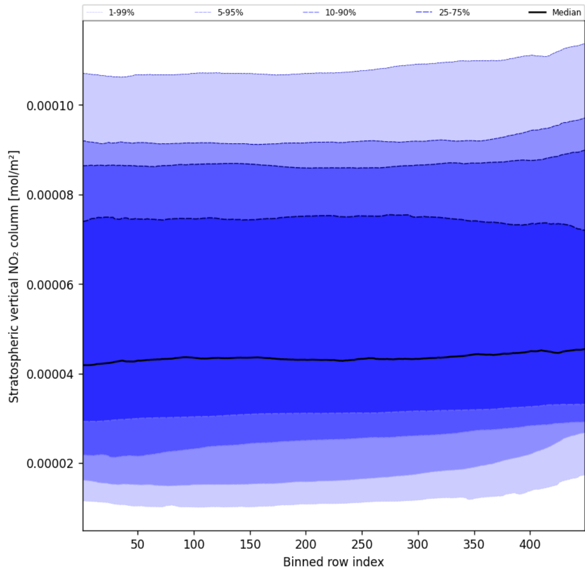
Figure 51: Along track statistics of “Stratospheric vertical NO 2 column” for 2025-01-03 to 2025-01-04
