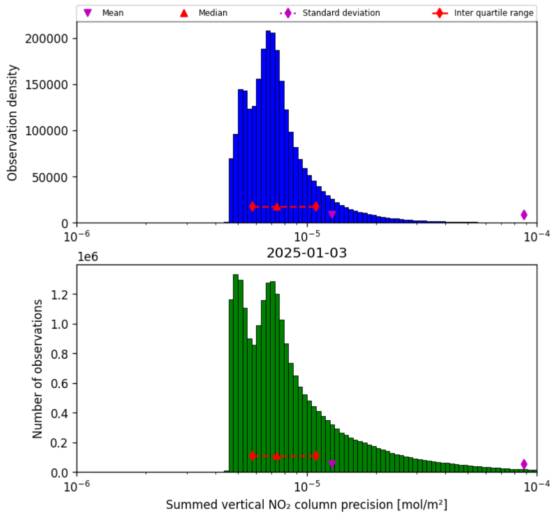
Figure 39: Histogram of "Summed vertical NO 2 column precision" for 2025-01-03 to 2025-01-04
