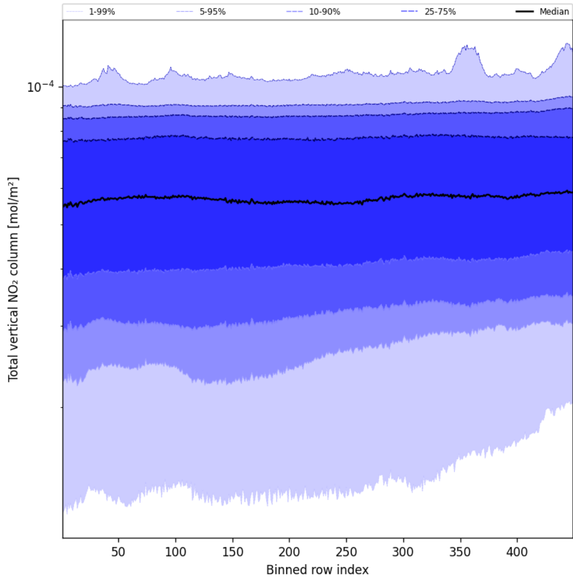
Figure 53: Along track statistics of “Total vertical NO 2 column” for 2025-01-03 to 2025-01-04
