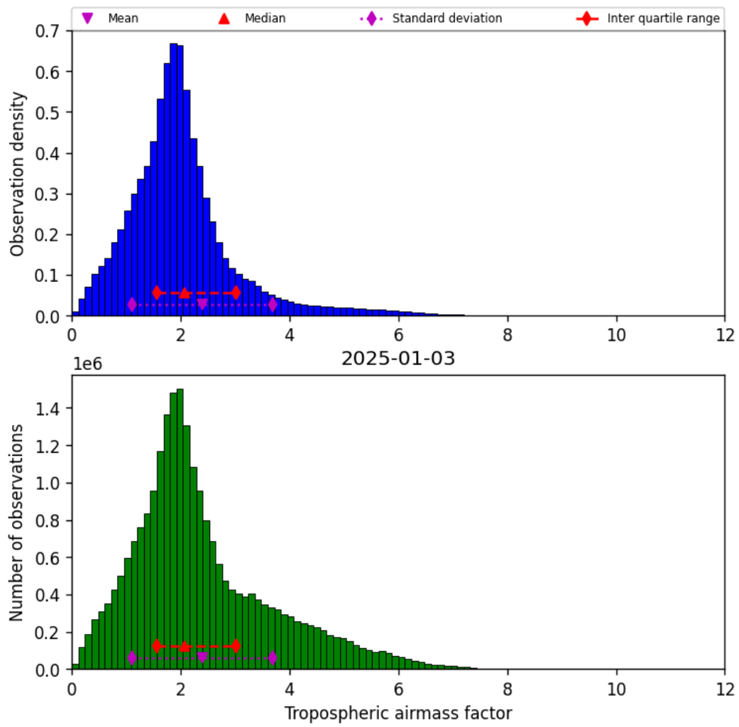
Figure 29: Histogram of “Tropospheric airmass factor” for 2025-01-03 to 2025-01-04
