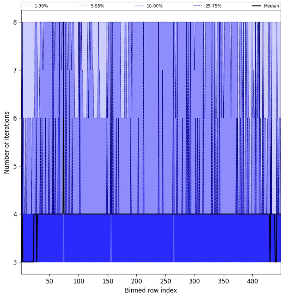
Figure 49: Along track statistics of “Number of iterations” for 2025-01-03 to 2025-01-04
