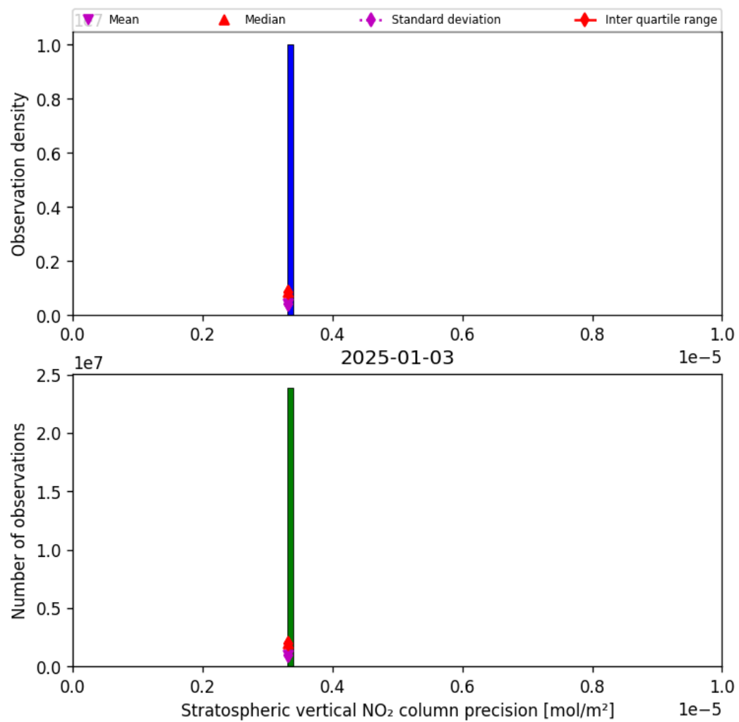
Figure 35: Histogram of “Stratospheric vertical NO 2 column precision” for 2025-01-03 to 2025-01-04
