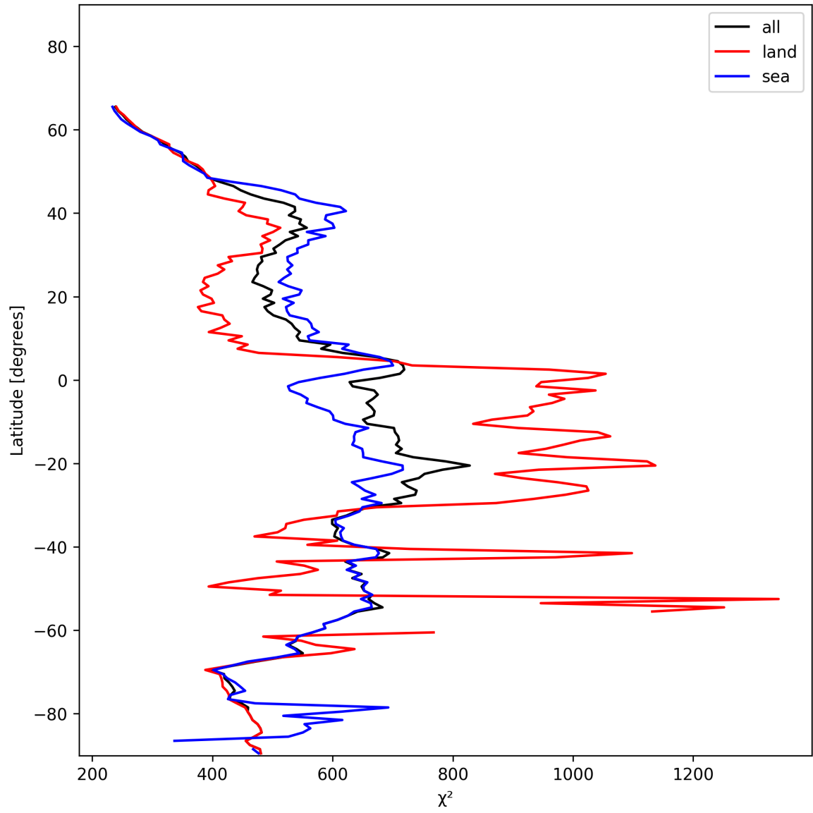
Figure 23: Zonal average of “ \chi^2 ” for 2025-01-03 to 2025-01-04.
