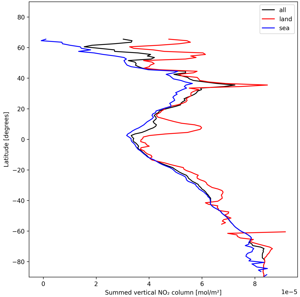
Figure 21: Zonal average of “Summed vertical NO 2 column” for 2025-01-03 to 2025-01-04.
