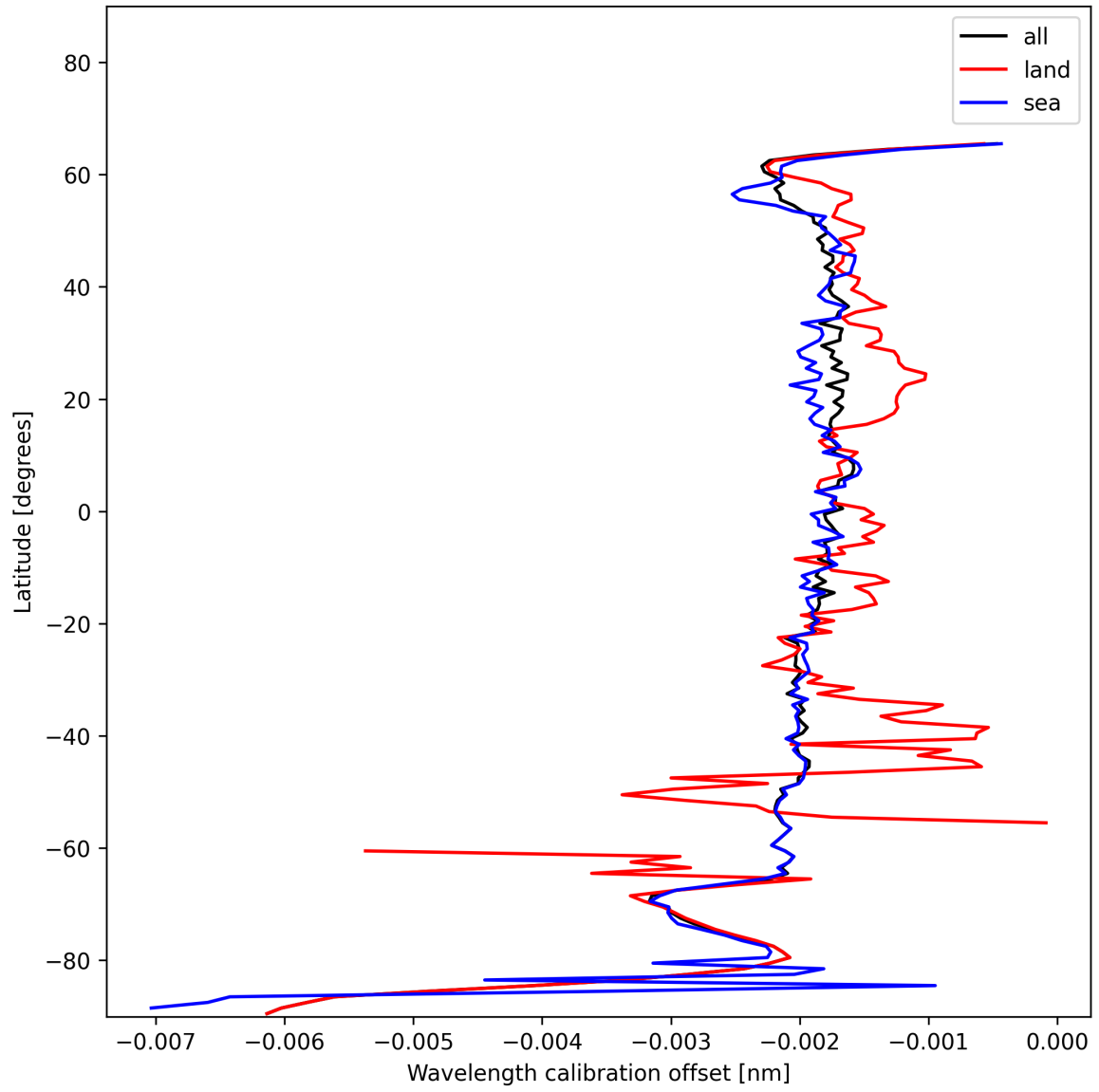
Figure 16: Zonal average of “Wavelength calibration offset” for 2025-01-04 to 2025-01-04.
