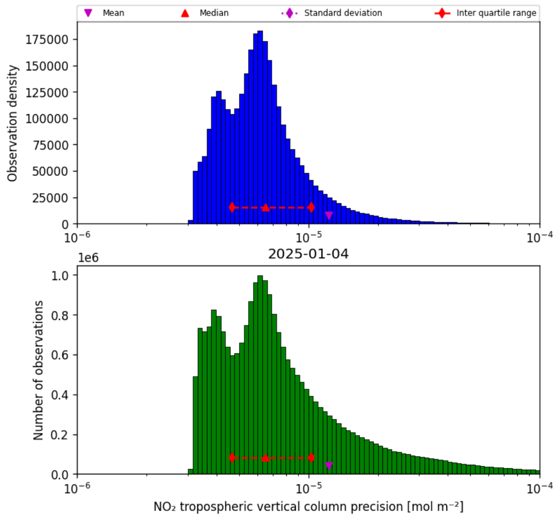
Figure 28: Histogram of "NO 2 tropospheric vertical column precision" for 2025-01-04 to 2025-01-04
