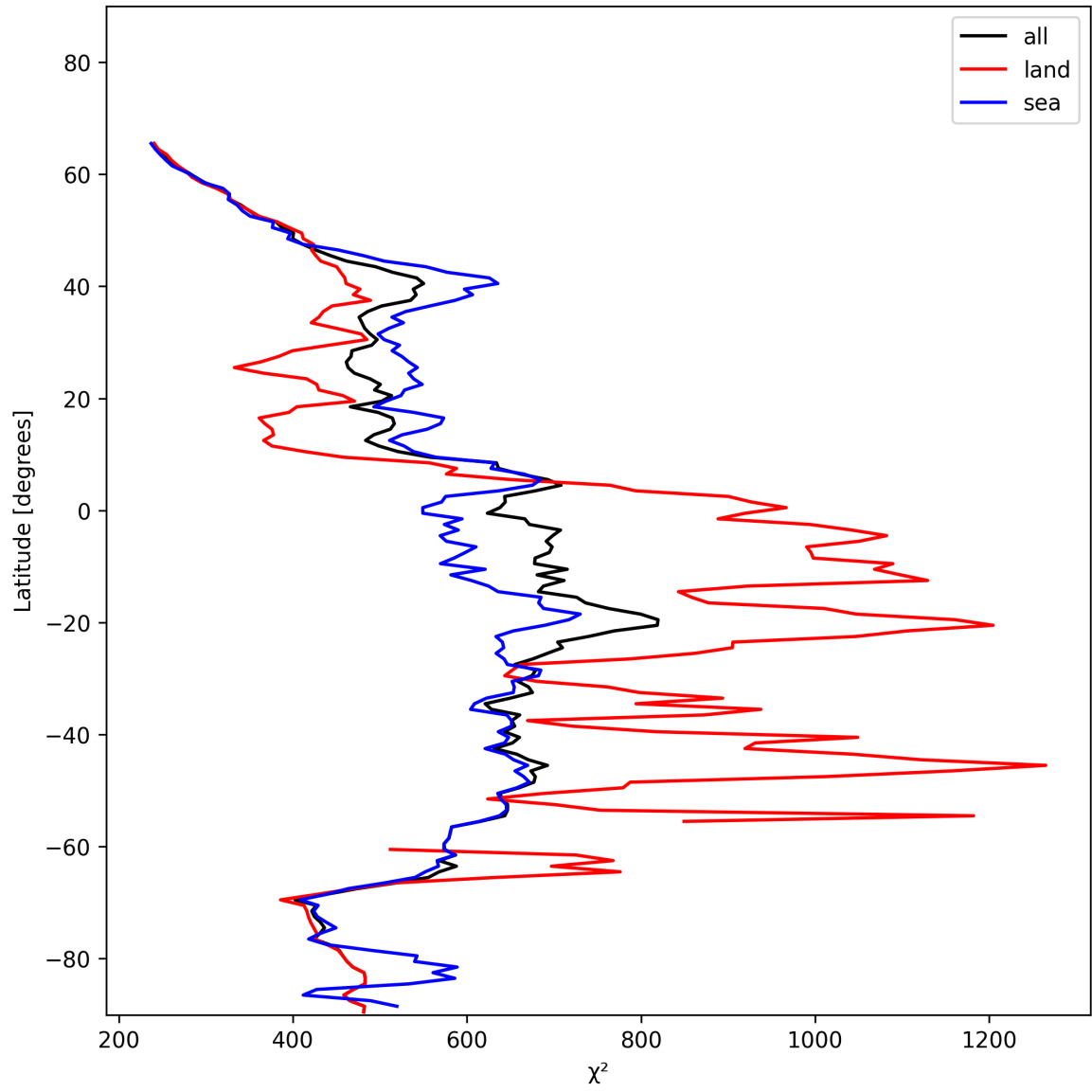
Figure 23: Zonal average of “ \chi^2 ” for 2025-01-04 to 2025-01-04.
