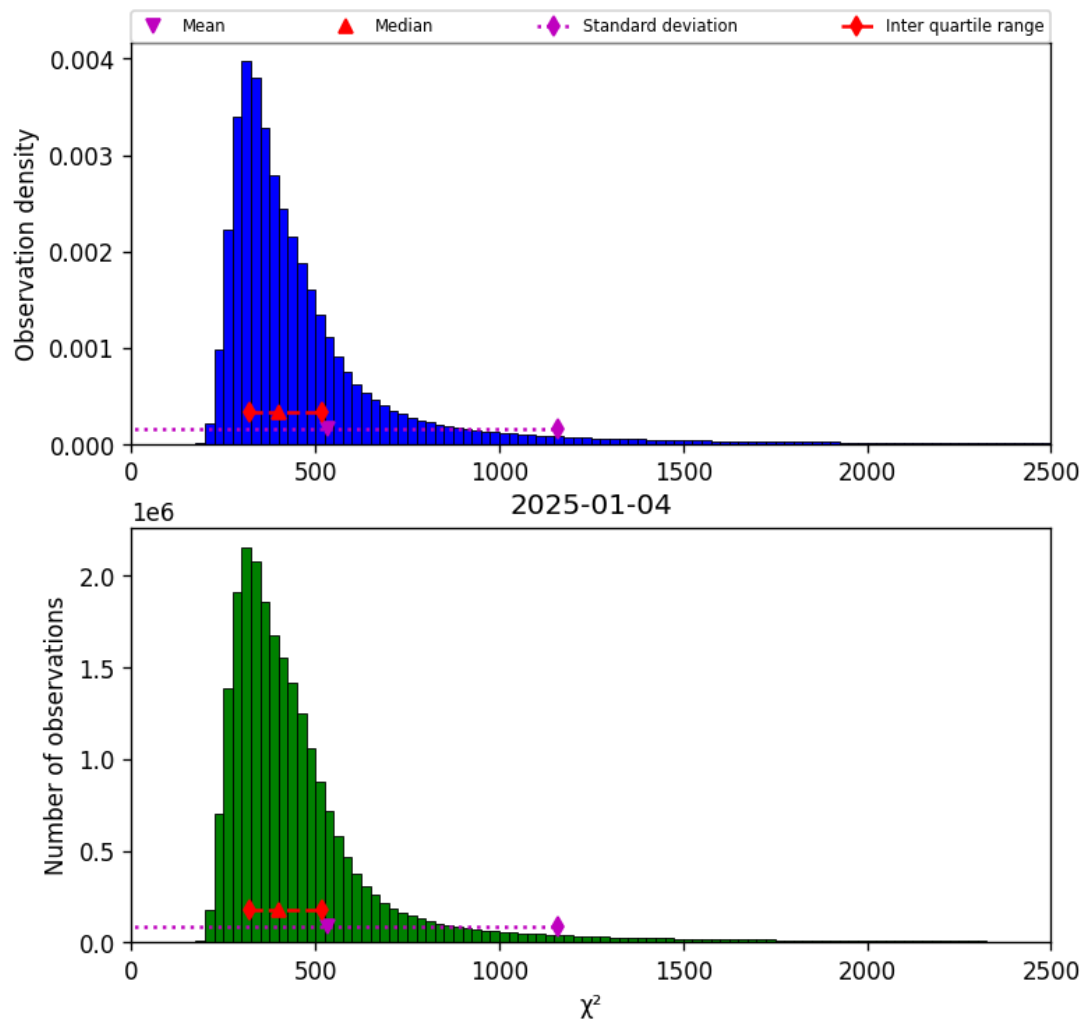
Figure 40: Histogram of " \chi^2 " for 2025-01-04 to 2025-01-04
