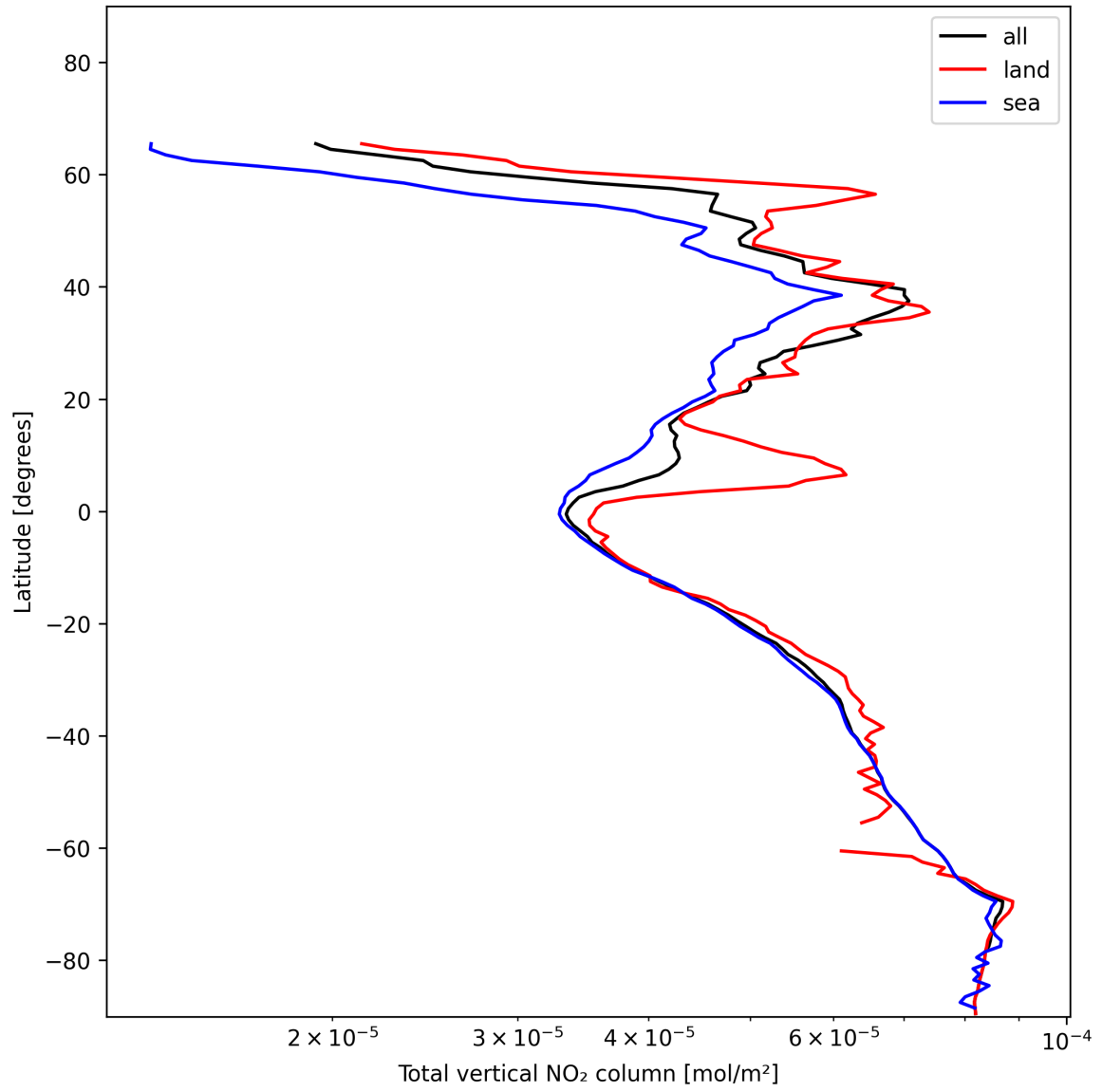
Figure 19: Zonal average of “Total vertical NO 2 column” for 2025-01-04 to 2025-01-04.
