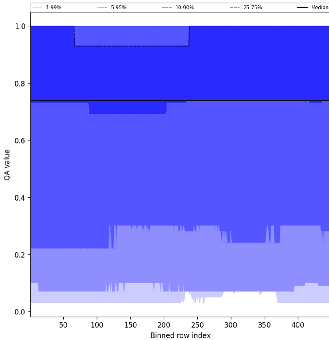
Figure 43: Along track statistics of “QA value” for 2025-01-04 to 2025-01-04
