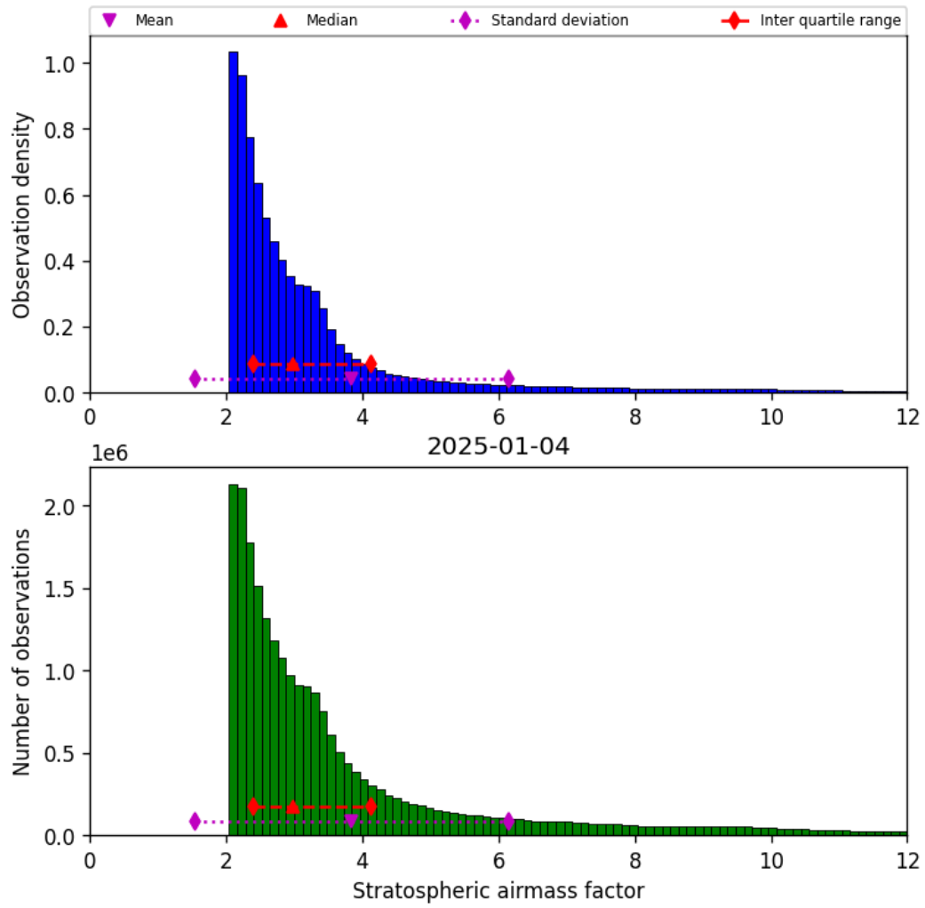
Figure 42: Histogram of “Stratospheric airmass factor” for 2025-01-04 to 2025-01-04
