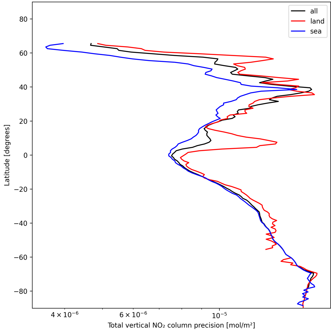
Figure 20: Zonal average of “Total vertical NO 2 column precision” for 2025-01-04 to 2025-01-04.
