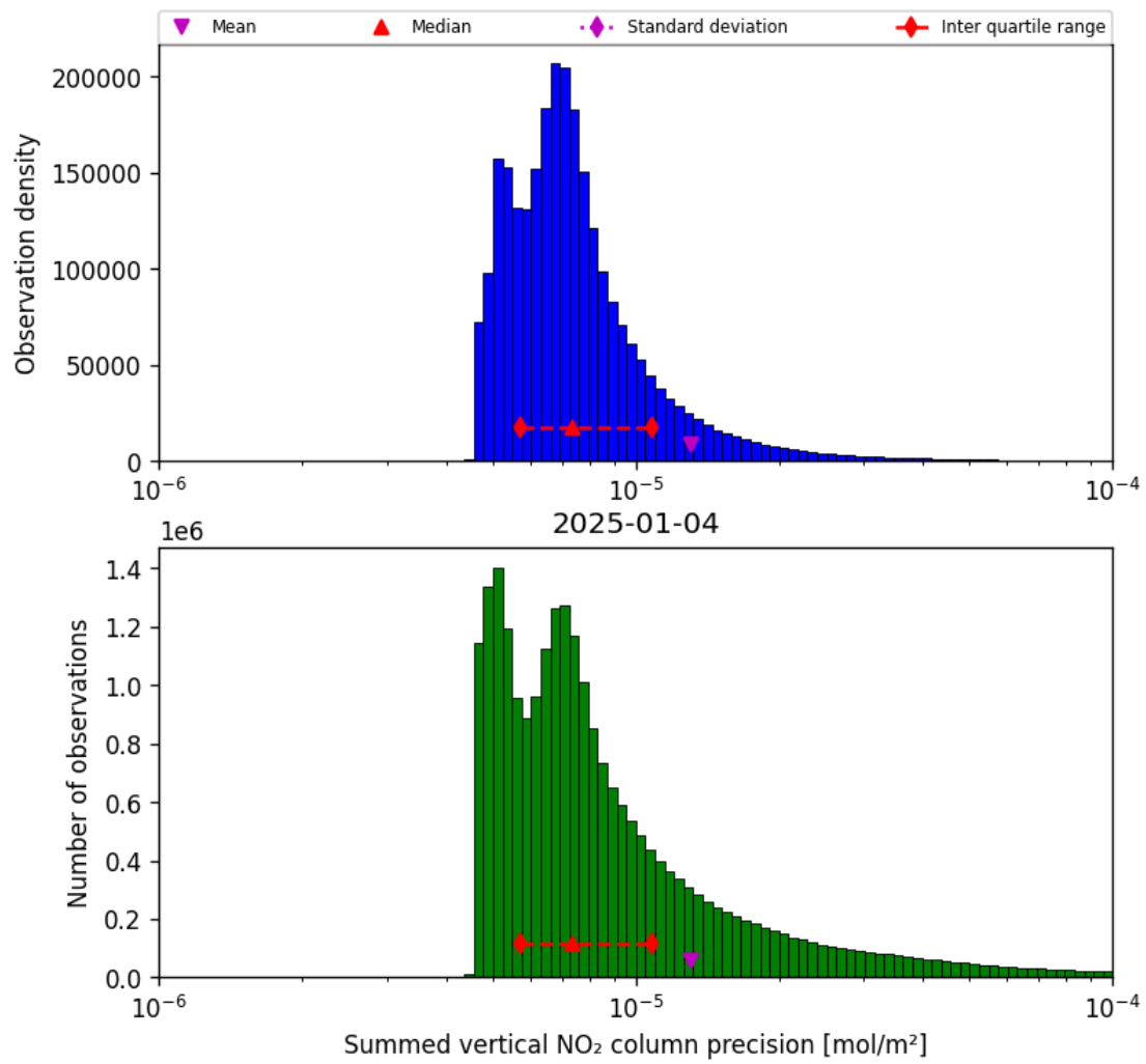
Figure 39: Histogram of "Summed vertical NO 2 column precision" for 2025-01-04 to 2025-01-04
