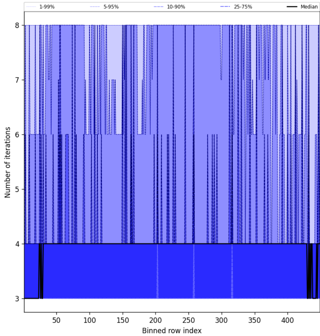
Figure 49: Along track statistics of “Number of iterations” for 2025-01-04 to 2025-01-04
