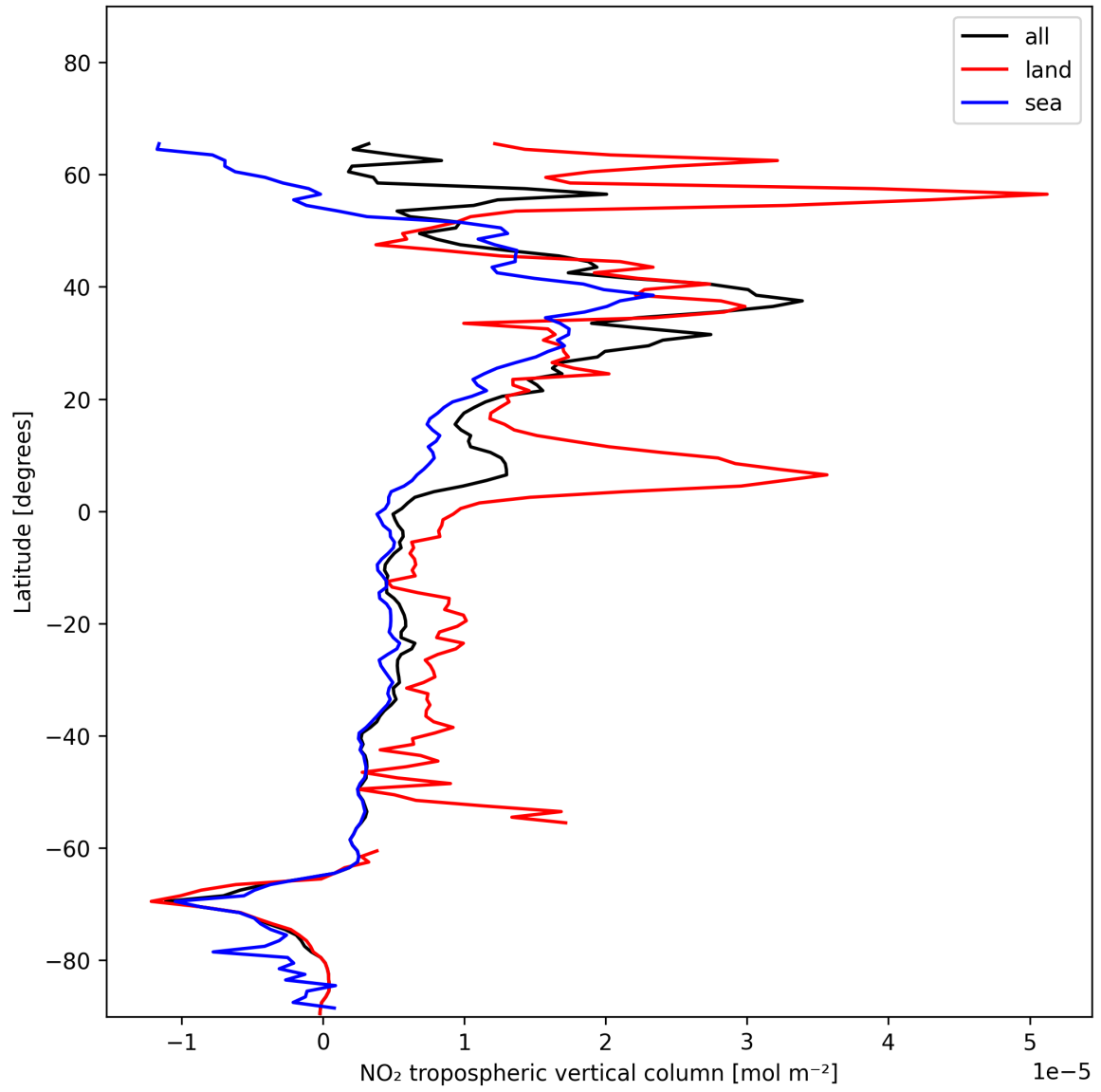
Figure 10: Zonal average of “NO 2 tropospheric vertical column” for 2025-01-04 to 2025-01-04.
