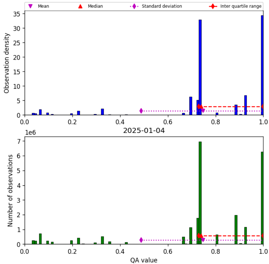
Figure 26: Histogram of “QA value” for 2025-01-04 to 2025-01-04
