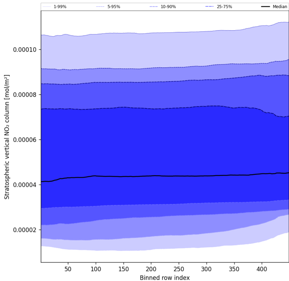
Figure 51: Along track statistics of “Stratospheric vertical NO 2 column” for 2025-01-04 to 2025-01-04
