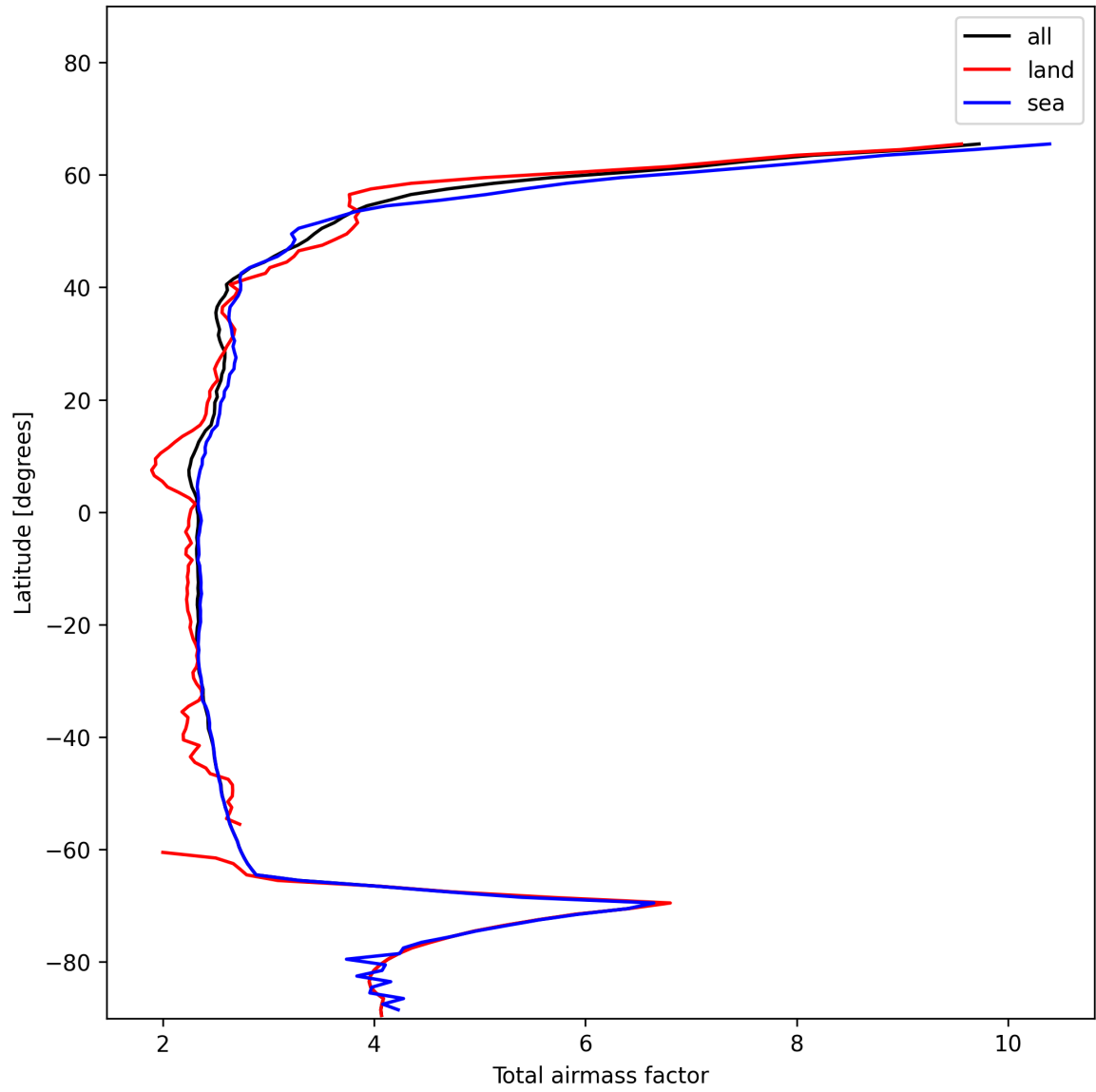
Figure 13: Zonal average of “Total airmass factor” for 2025-01-04 to 2025-01-04.
