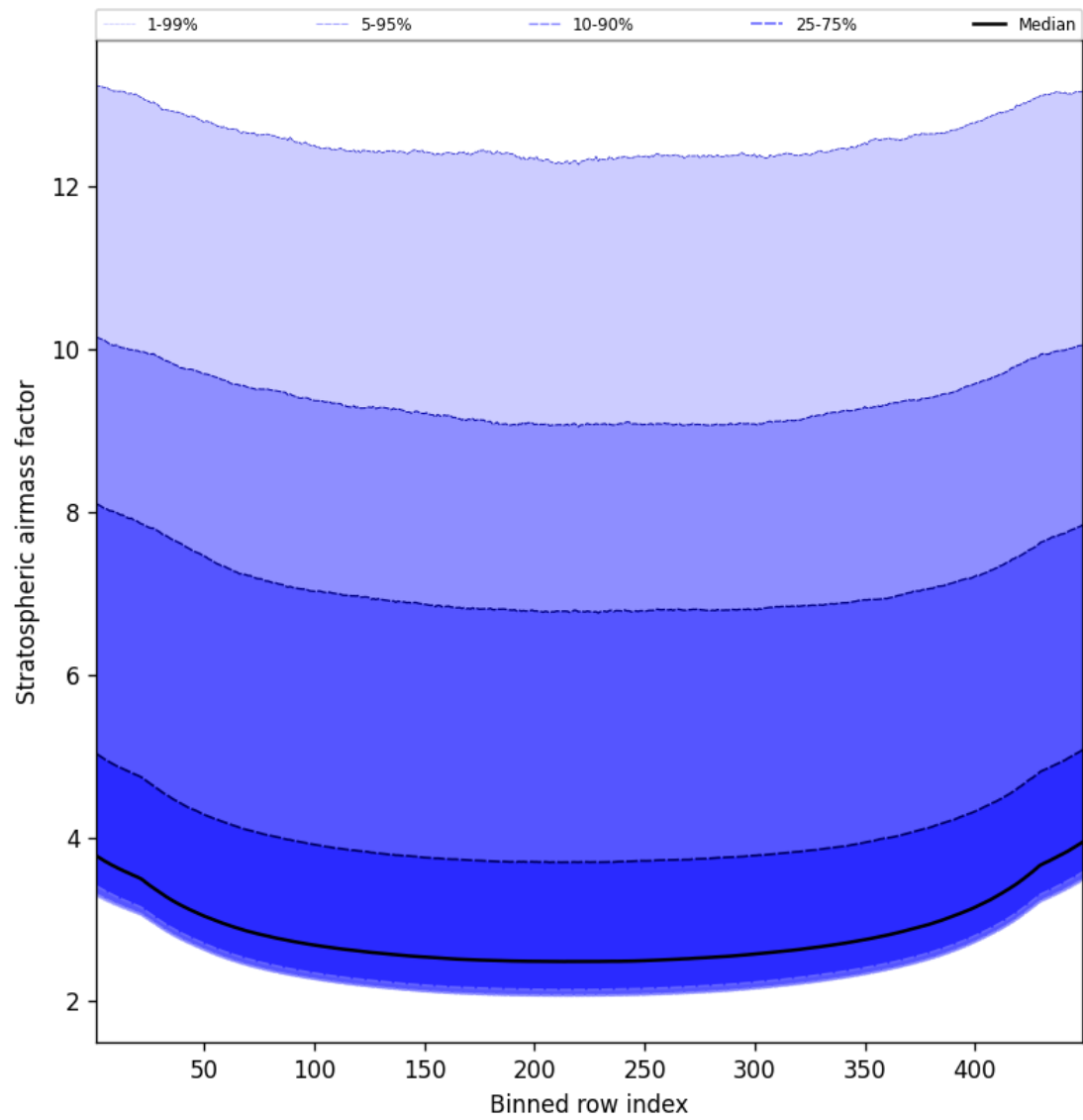
Figure 59: Along track statistics of “Stratospheric airmass factor” for 2025-01-04 to 2025-01-04
