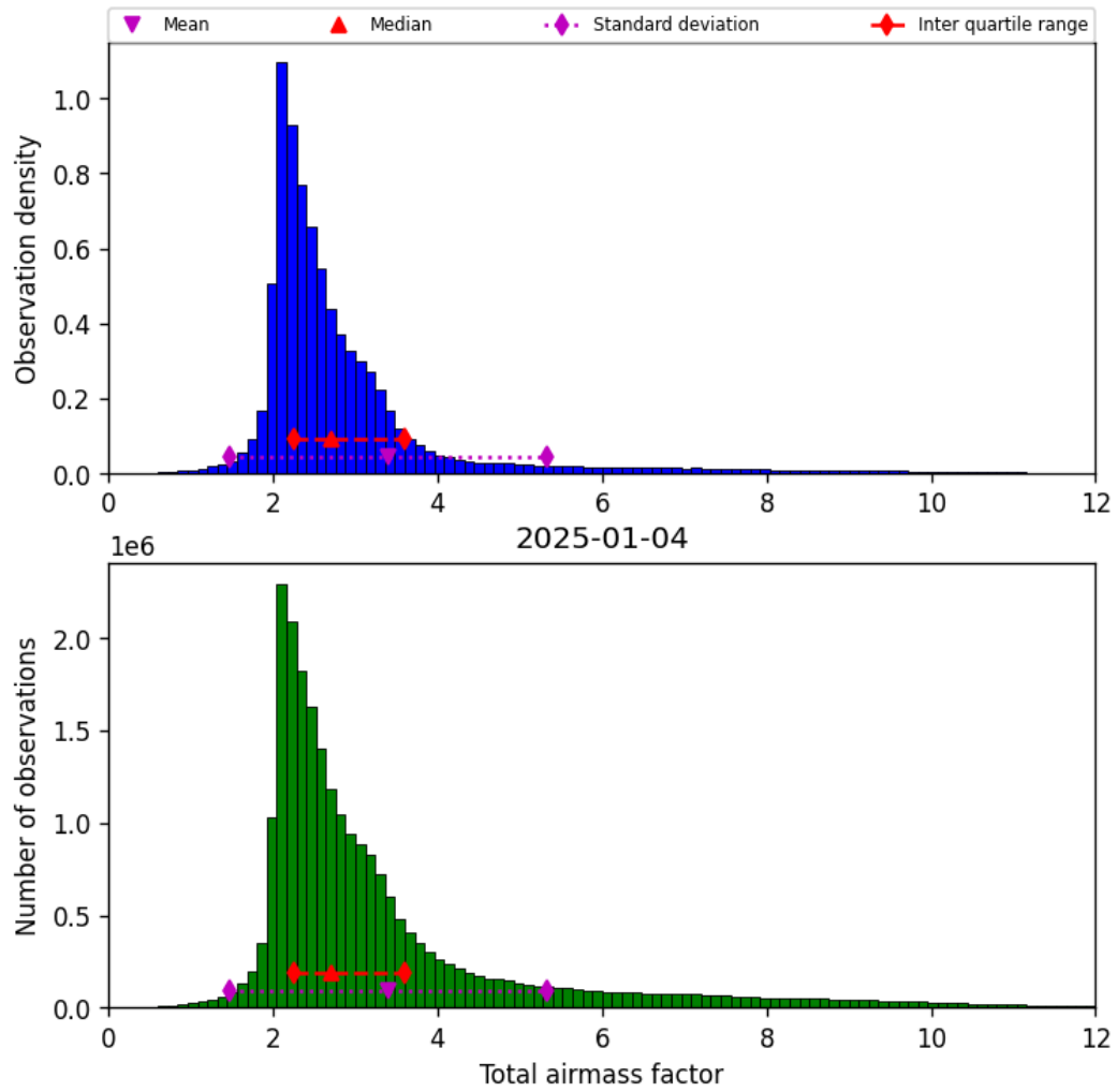
Figure 30: Histogram of “Total airmass factor” for 2025-01-04 to 2025-01-04
