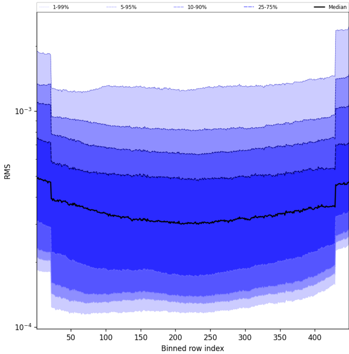
Figure 58: Along track statistics of “RMS” for 2025-01-04 to 2025-01-04
