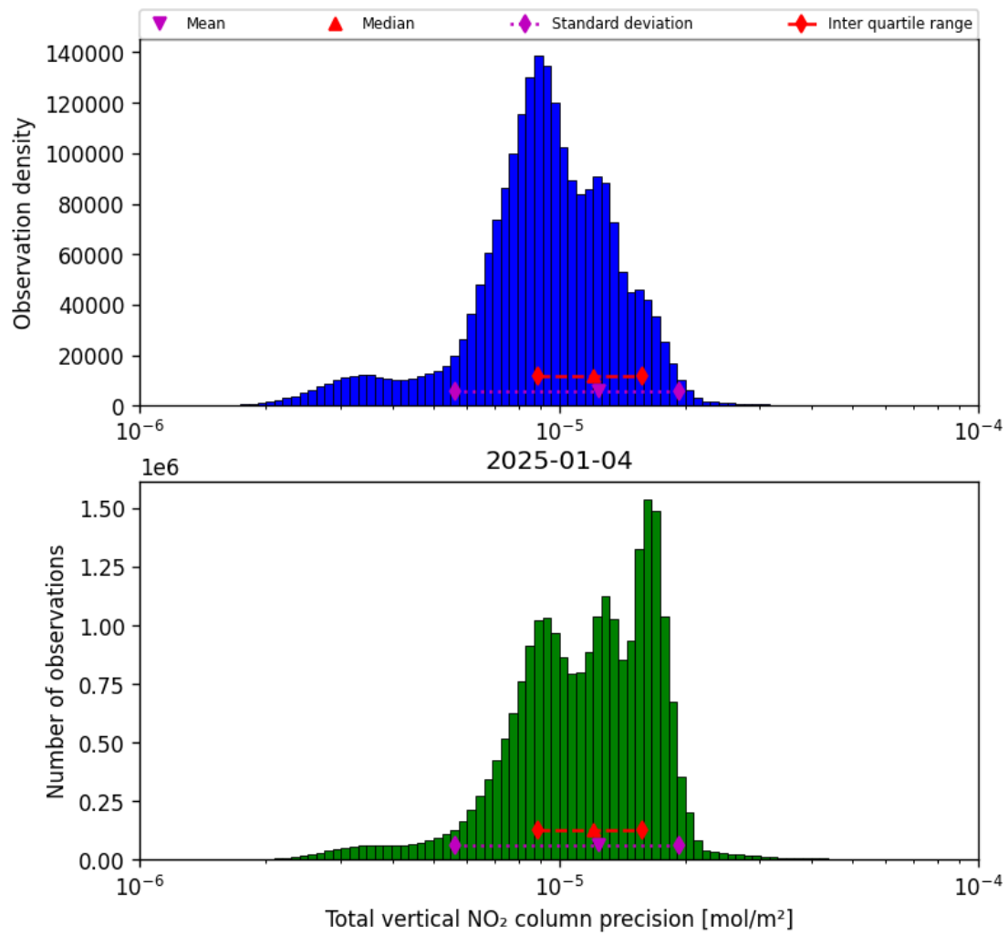
Figure 37: Histogram of “Total vertical NO 2 column precision” for 2025-01-04 to 2025-01-04
