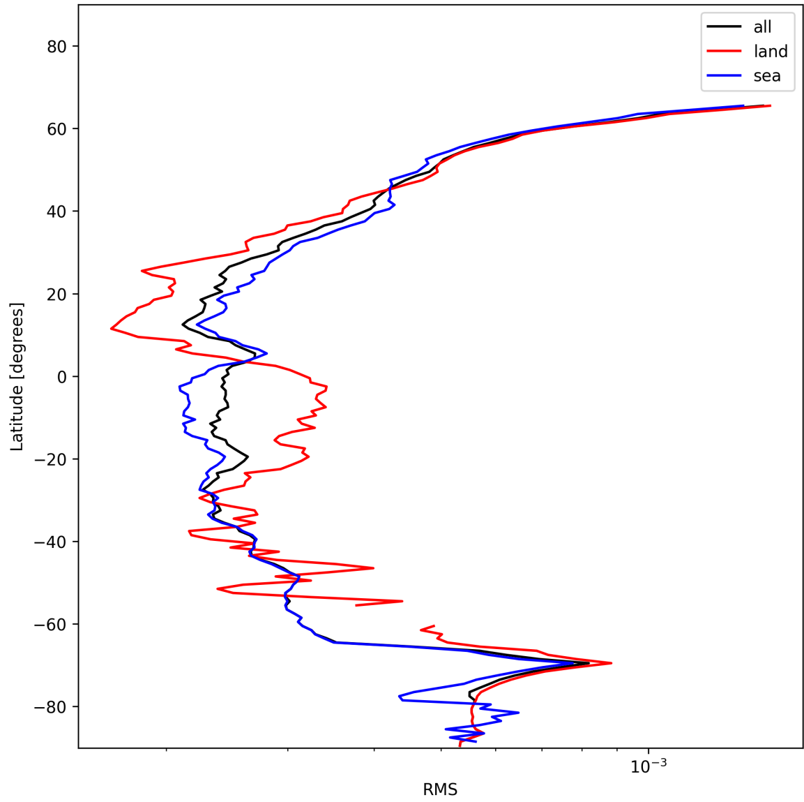
Figure 24: Zonal average of “RMS” for 2025-01-04 to 2025-01-04.
