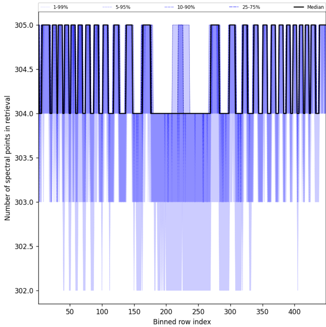
Figure 48: Along track statistics of “Number of spectral points in retrieval” for 2025-01-04 to 2025-01-04
