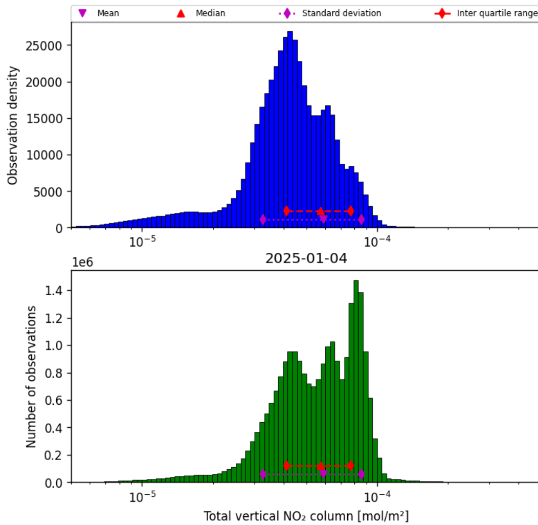
Figure 36: Histogram of “Total vertical NO 2 column” for 2025-01-04 to 2025-01-04
