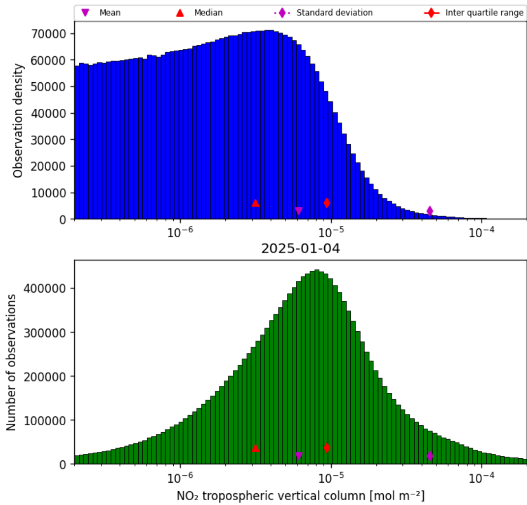
Figure 27: Histogram of “NO 2 tropospheric vertical column” for 2025-01-04 to 2025-01-04
