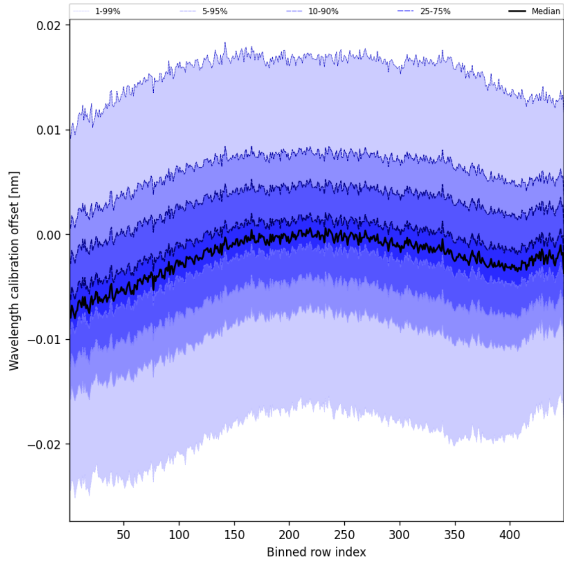
Figure 50: Along track statistics of “Wavelength calibration offset” for 2025-01-04 to 2025-01-04
