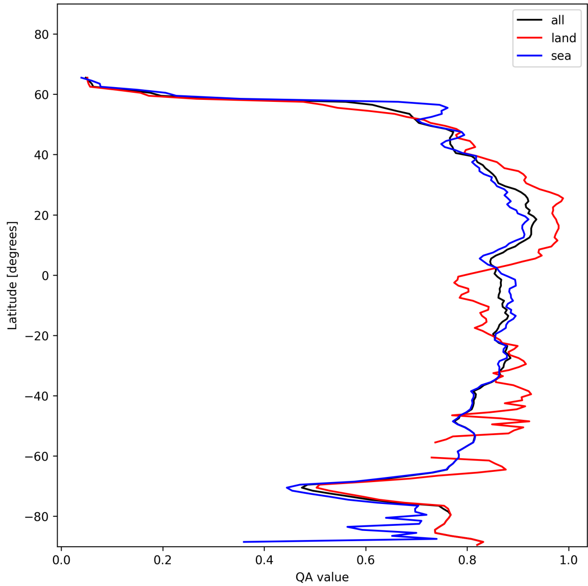
Figure 9: Zonal average of “QA value” for 2025-01-04 to 2025-01-04.
