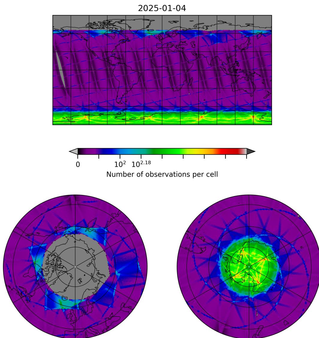
Figure 8: Map of the number of observations for 2025-01-04 to 2025-01-04
