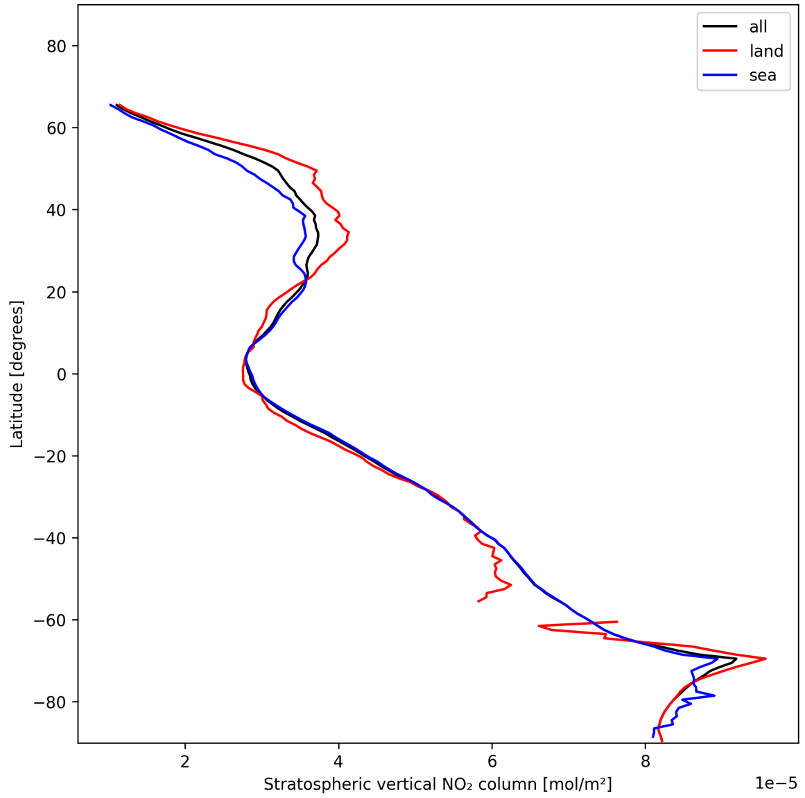
Figure 17: Zonal average of “Stratospheric vertical NO 2 column” for 2025-01-04 to 2025-01-04.
