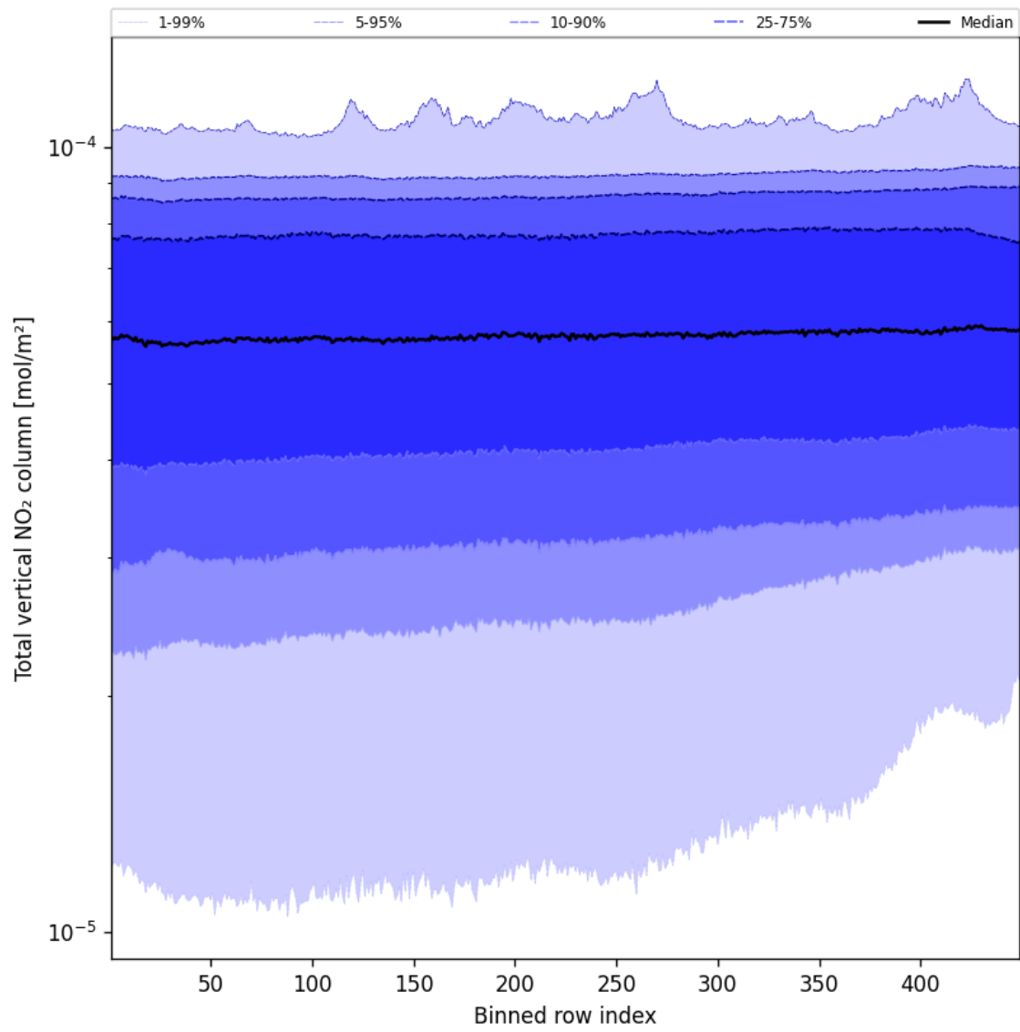
Figure 53: Along track statistics of “Total vertical NO 2 column” for 2025-01-04 to 2025-01-04
