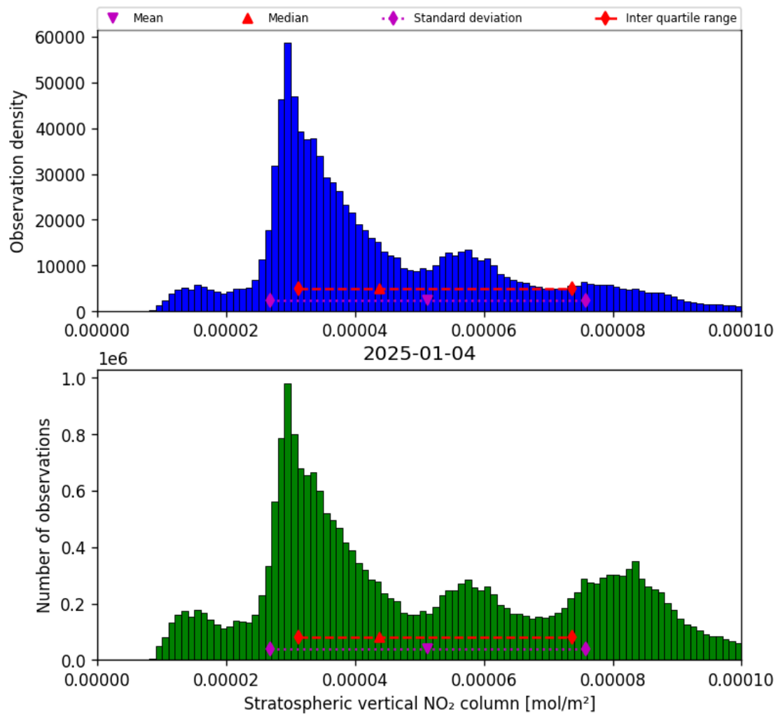
Figure 34: Histogram of “Stratospheric vertical NO 2 column” for 2025-01-04 to 2025-01-04
