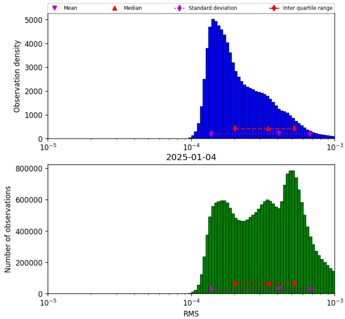
Figure 41: Histogram of “RMS” for 2025-01-04 to 2025-01-04
