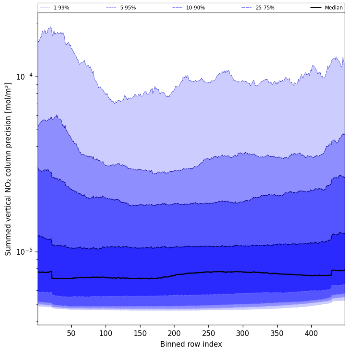
Figure 56: Along track statistics of “Summed vertical NO 2 column precision” for 2025-01-04 to 2025-01-04
