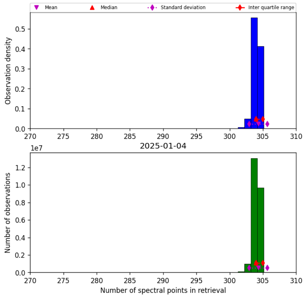
Figure 31: Histogram of “Number of spectral points in retrieval” for 2025-01-04 to 2025-01-04
