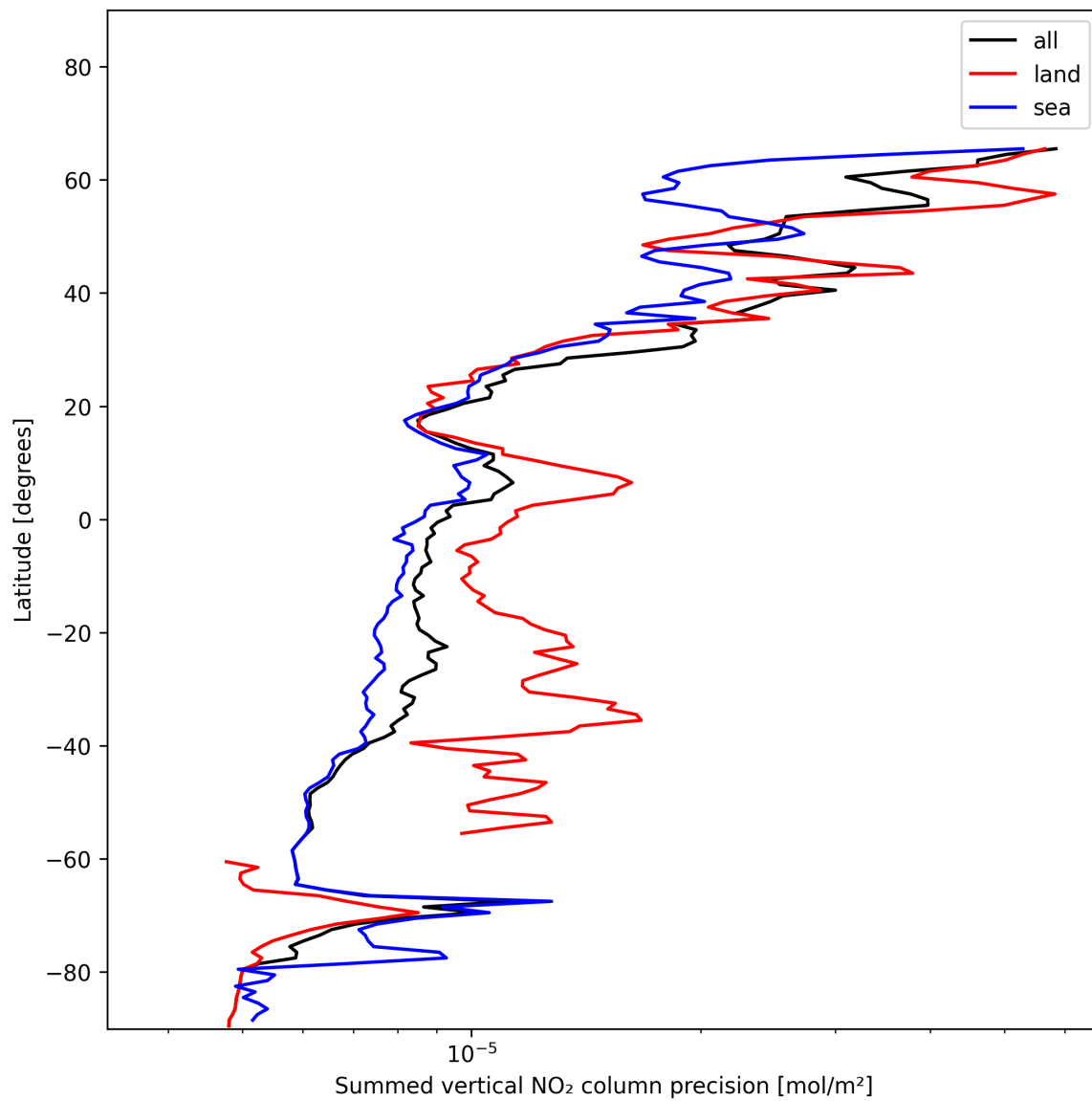
Figure 22: Zonal average of “Summed vertical NO 2 column precision” for 2025-01-04 to 2025-01-04.
