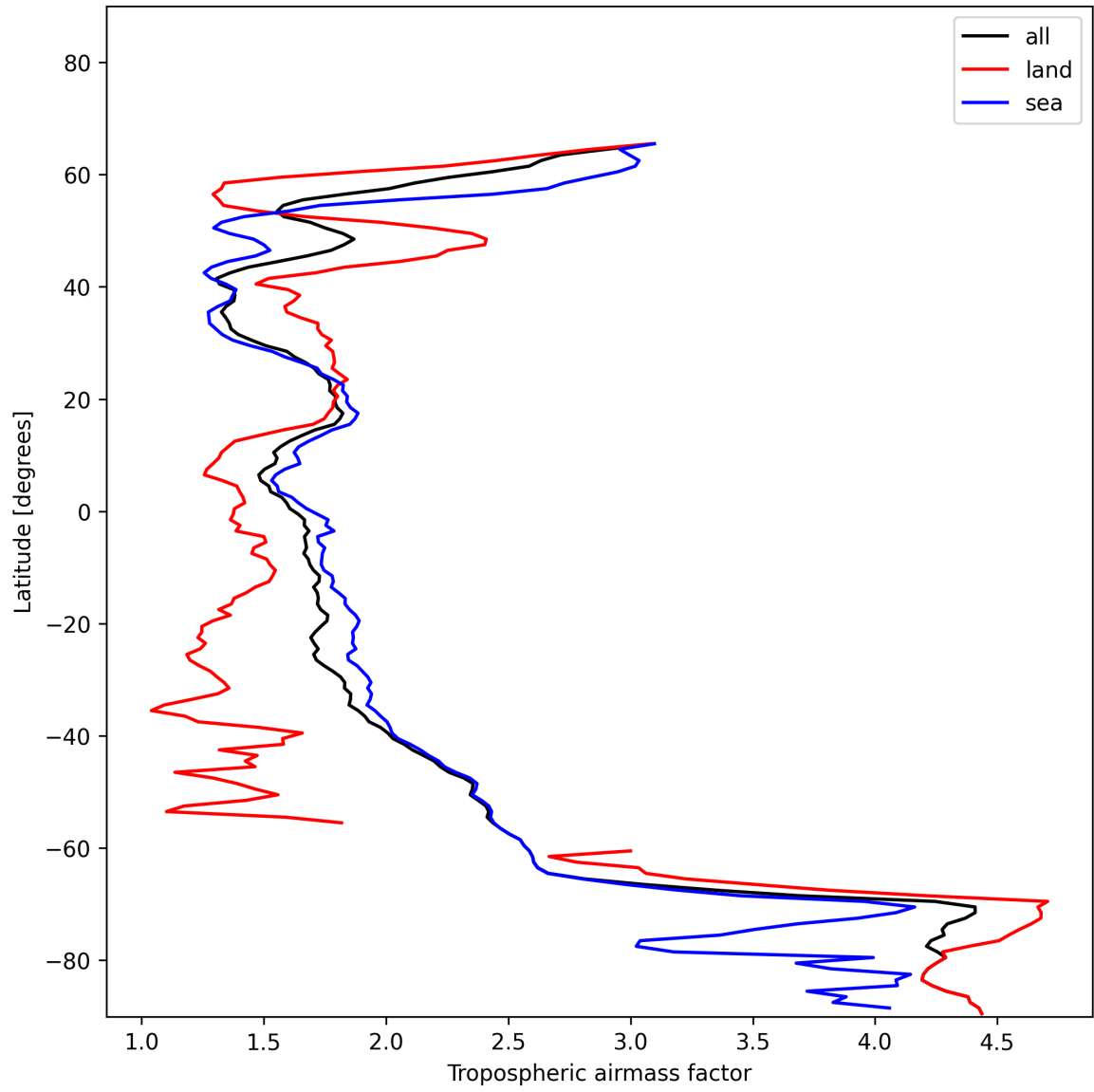
Figure 12: Zonal average of “Tropospheric airmass factor” for 2025-01-04 to 2025-01-04.
