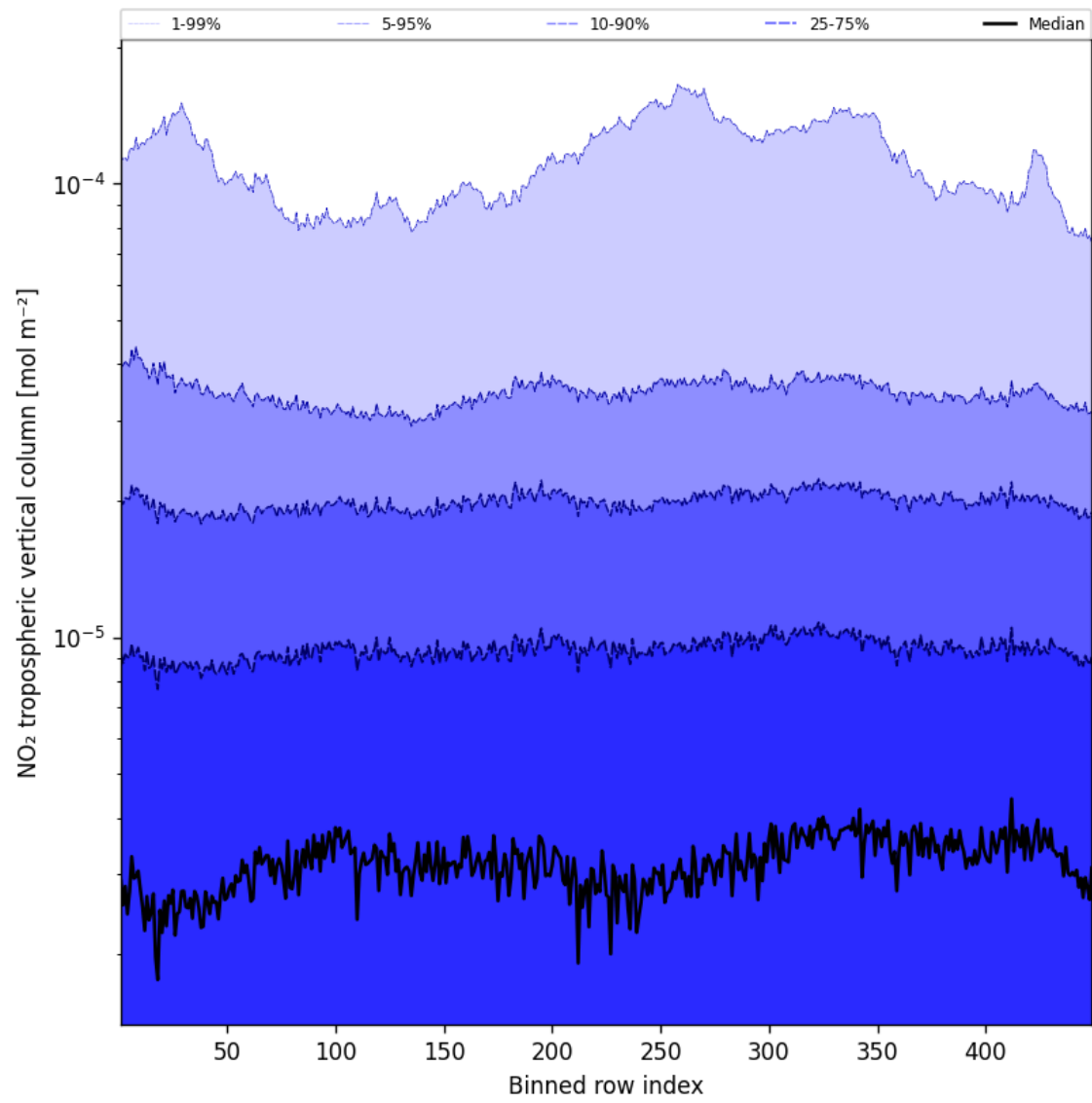
Figure 44: Along track statistics of “NO 2 tropospheric vertical column” for 2025-01-04 to 2025-01-04
