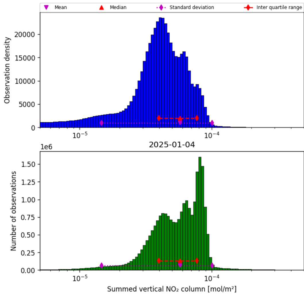
Figure 38: Histogram of “Summed vertical NO 2 column” for 2025-01-04 to 2025-01-04
