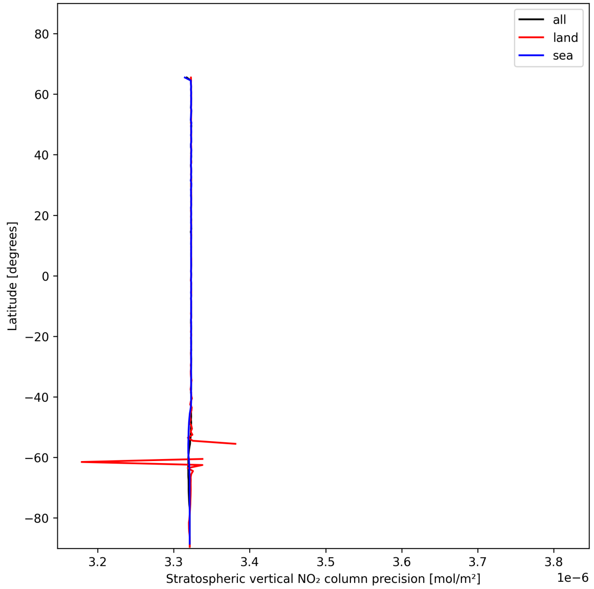
Figure 18: Zonal average of “Stratospheric vertical NO 2 column precision” for 2025-01-04 to 2025-01-04.
