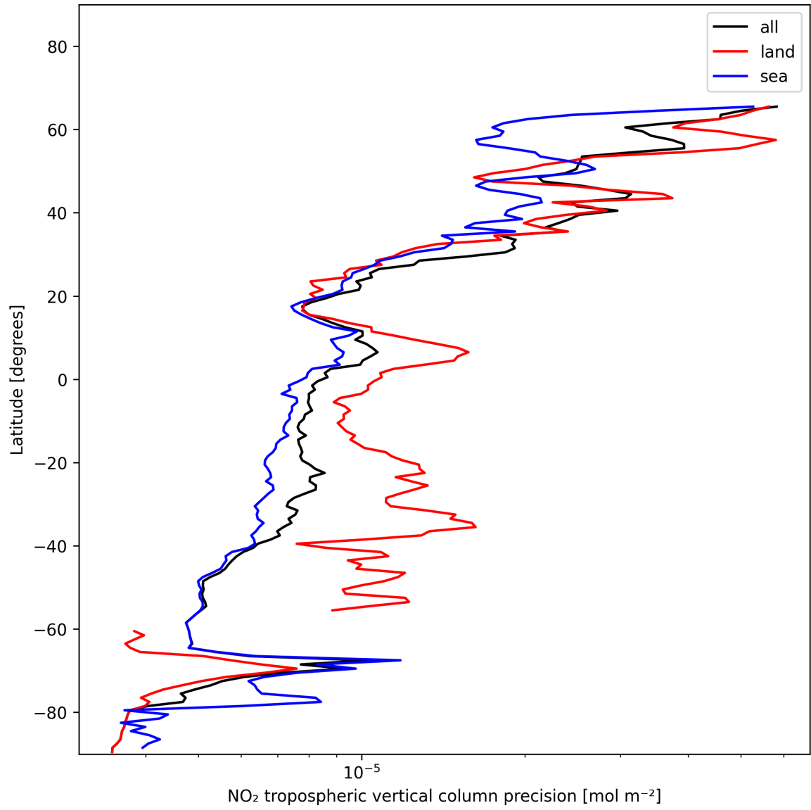
Figure 11: Zonal average of “NO 2 tropospheric vertical column precision” for 2025-01-04 to 2025-01-04.
