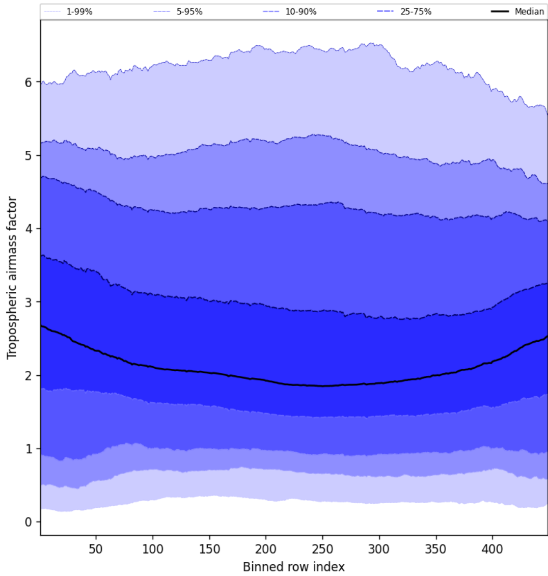
Figure 46: Along track statistics of “Tropospheric airmass factor” for 2025-01-04 to 2025-01-04
