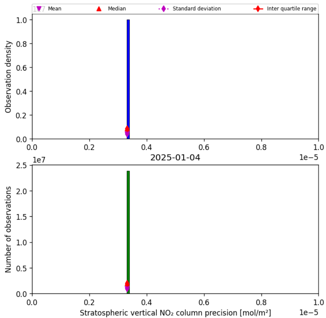
Figure 35: Histogram of “Stratospheric vertical NO 2 column precision” for 2025-01-04 to 2025-01-04
