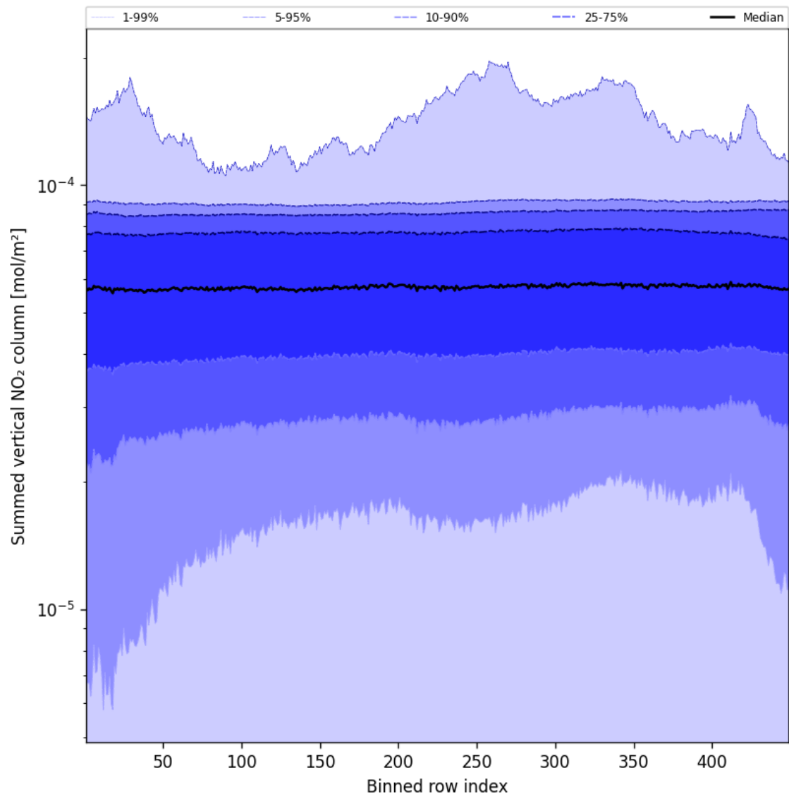
Figure 55: Along track statistics of “Summed vertical NO 2 column” for 2025-01-04 to 2025-01-04
