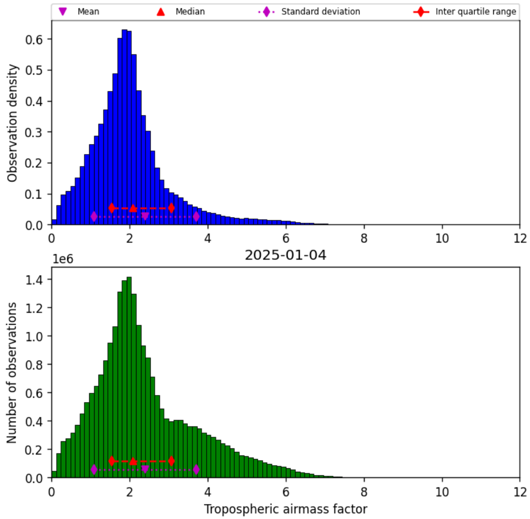
Figure 29: Histogram of “Tropospheric airmass factor” for 2025-01-04 to 2025-01-04
