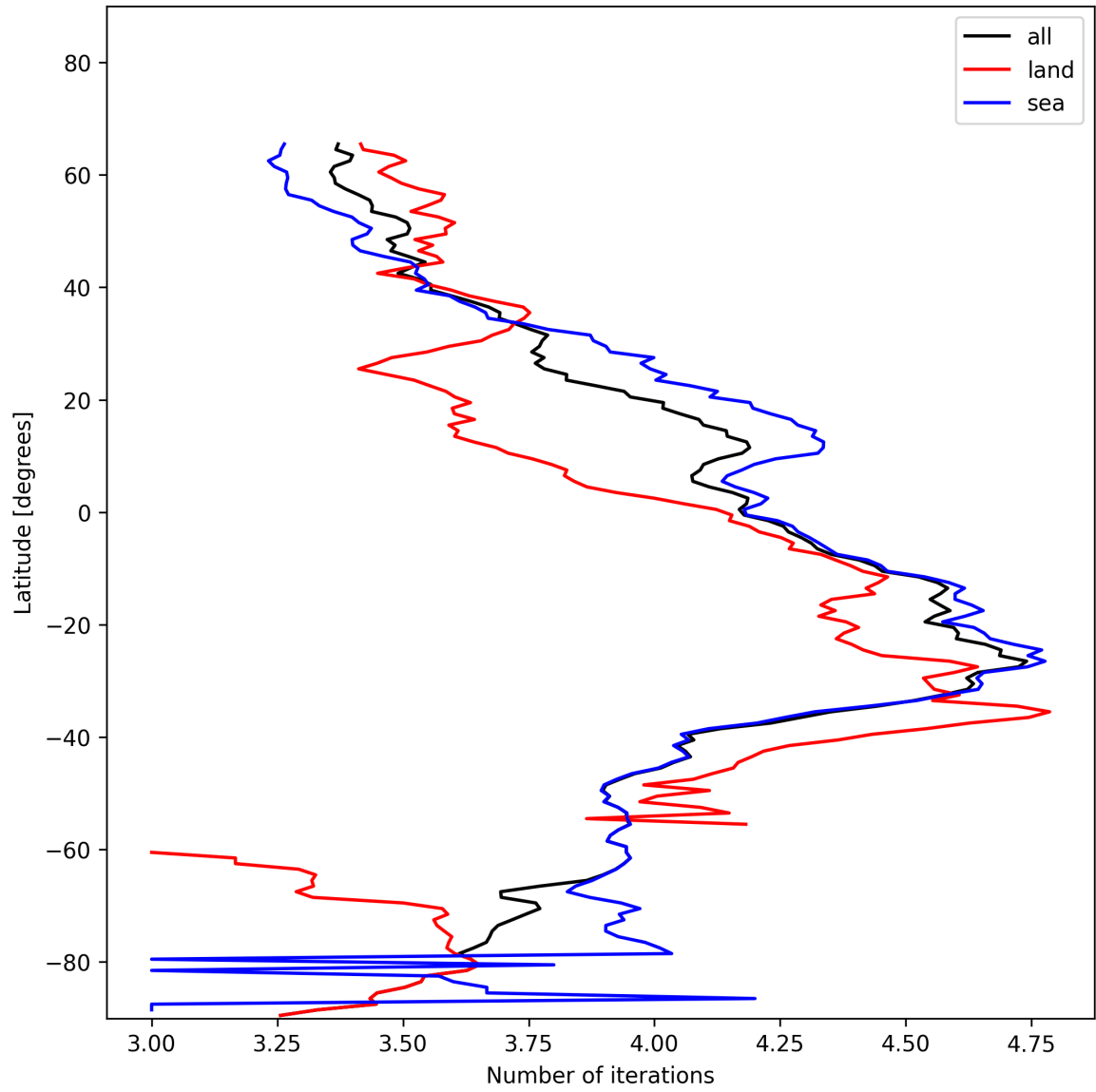
Figure 15: Zonal average of “Number of iterations” for 2025-01-04 to 2025-01-04.
