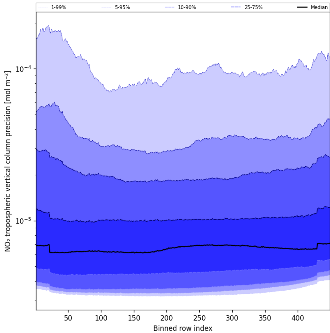
Figure 45: Along track statistics of “NO 2 tropospheric vertical column precision” for 2025-01-04 to 2025-01-04
