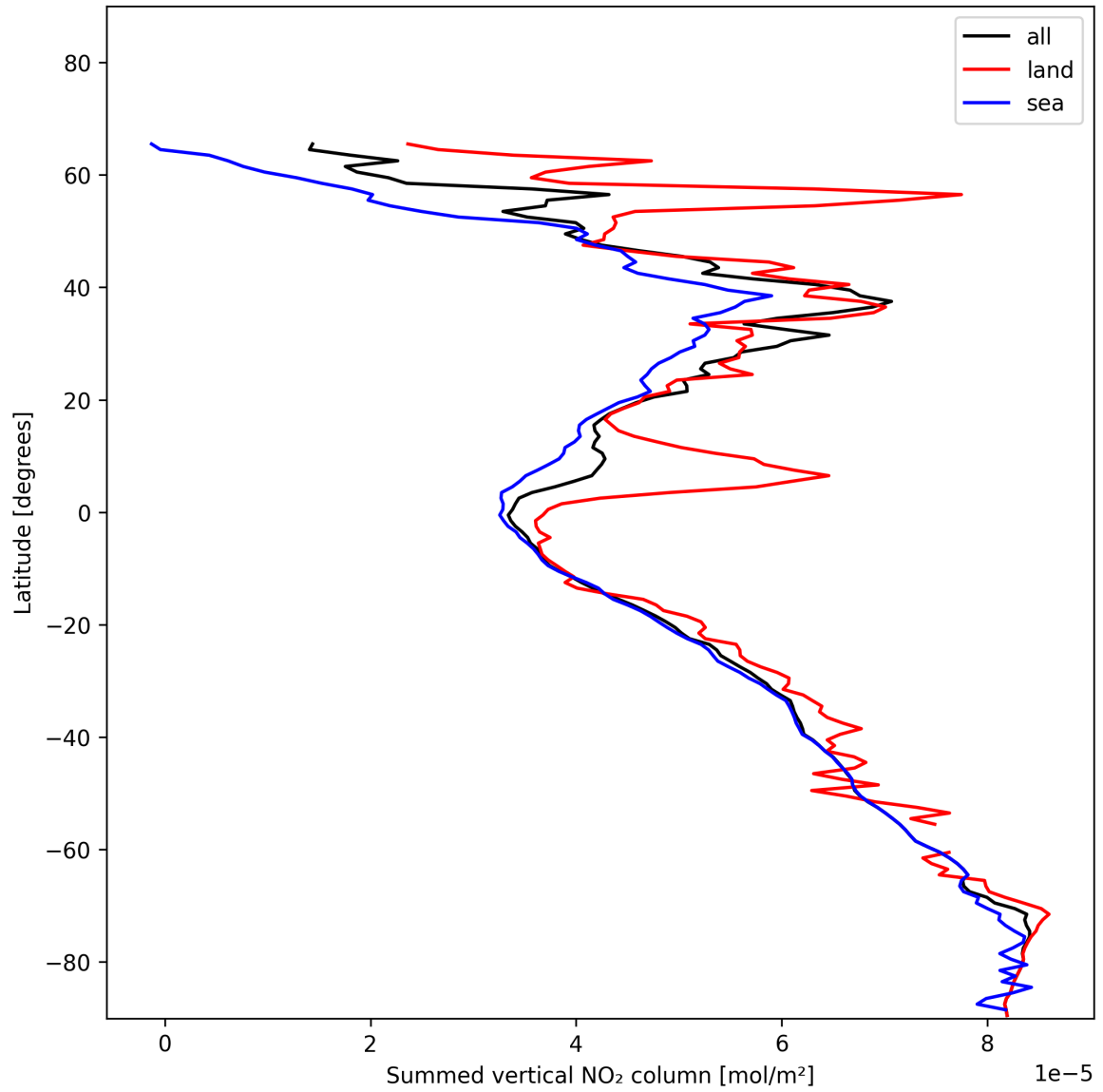
Figure 21: Zonal average of “Summed vertical NO 2 column” for 2025-01-04 to 2025-01-04.
