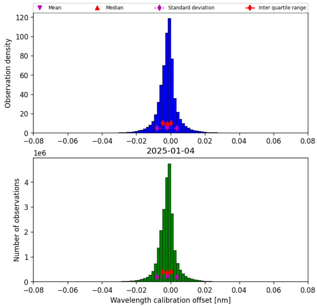
Figure 33: Histogram of “Wavelength calibration offset” for 2025-01-04 to 2025-01-04
