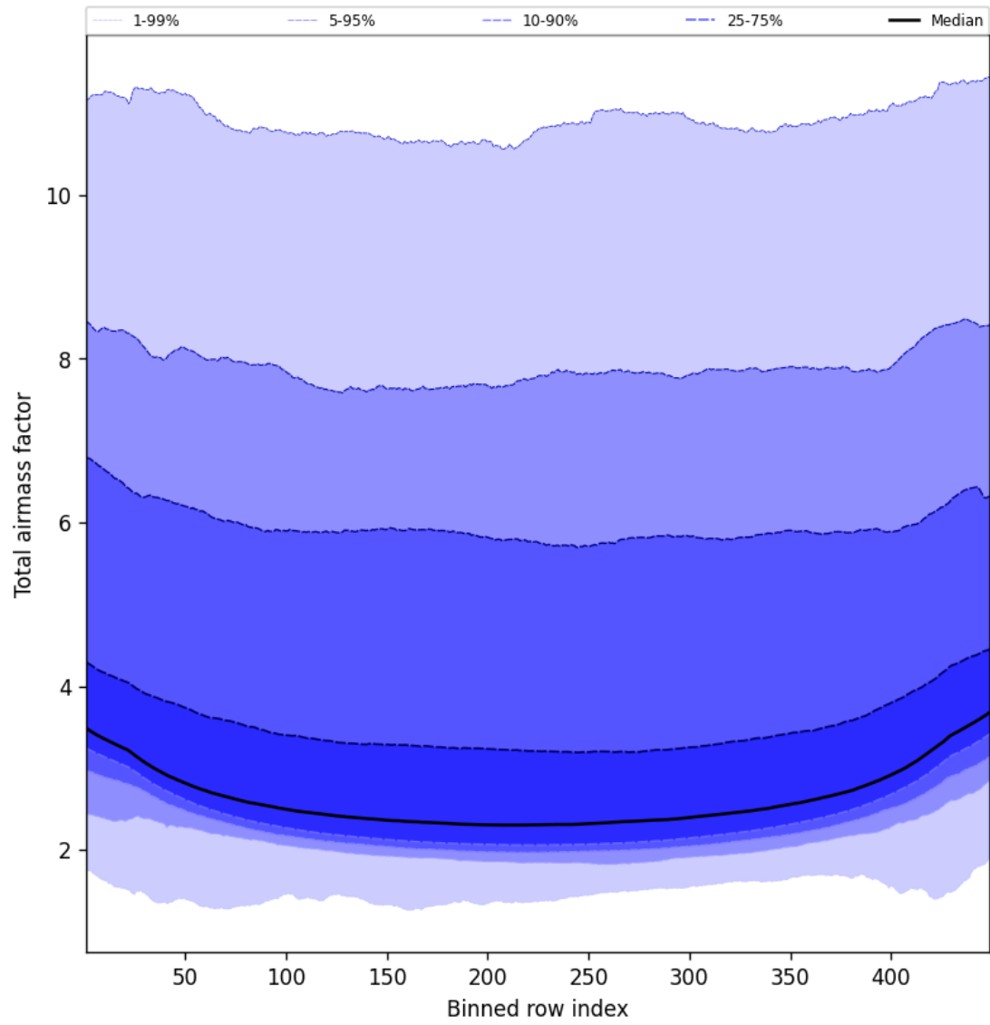
Figure 47: Along track statistics of “Total airmass factor” for 2025-01-04 to 2025-01-04
