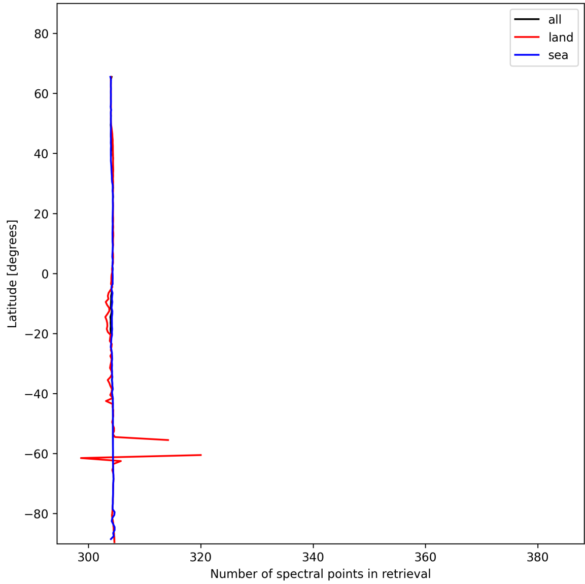
Figure 14: Zonal average of “Number of spectral points in retrieval” for 2025-01-04 to 2025-01-04.
