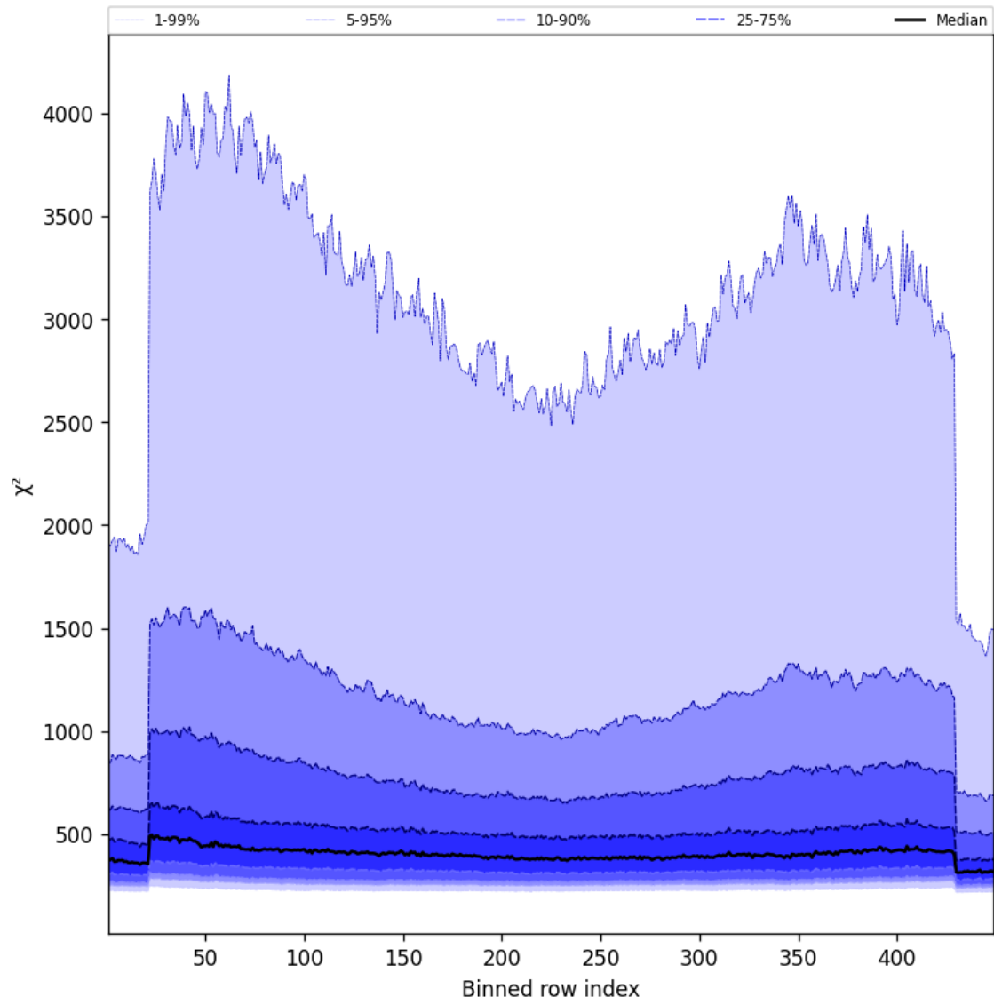
Figure 57: Along track statistics of “ \chi^2 ” for 2025-01-04 to 2025-01-04
