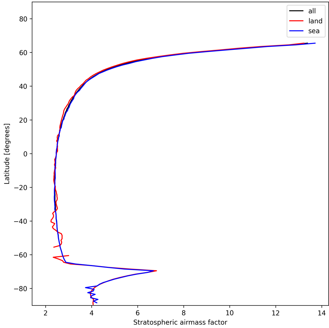
Figure 25: Zonal average of “Stratospheric air mass factor” for 2025-01-04 to 2025-01-04.
