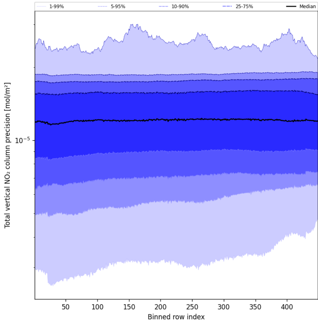
Figure 54: Along track statistics of “Total vertical NO 2 column precision” for 2025-01-04 to 2025-01-04
