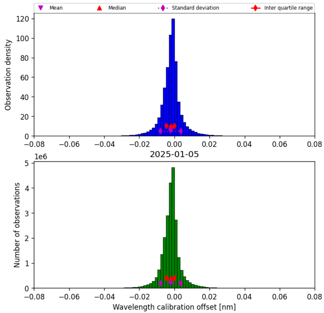
Figure 33: Histogram of “Wavelength calibration offset” for 2025-01-05 to 2025-01-05
