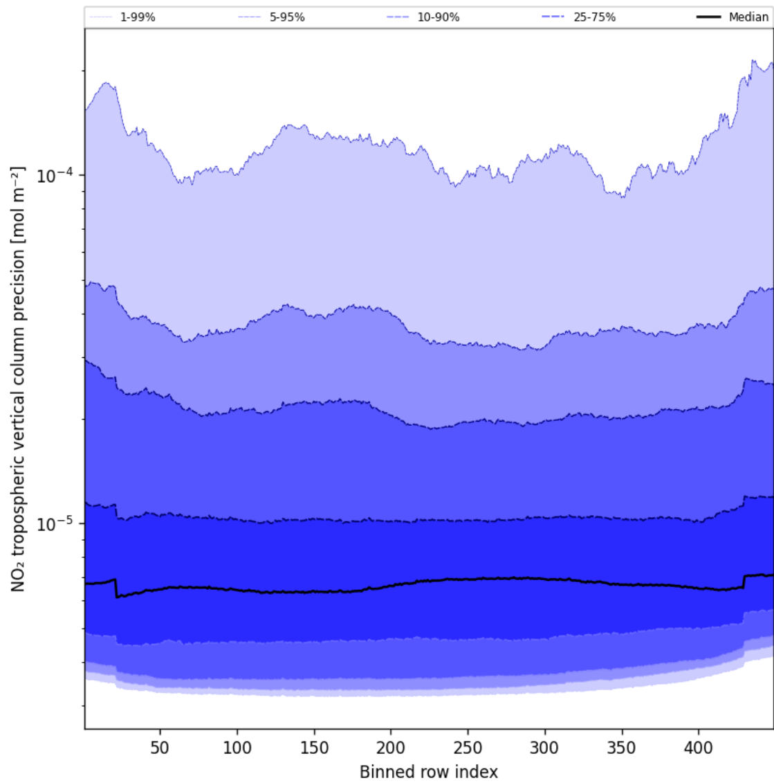
Figure 45: Along track statistics of “NO 2 tropospheric vertical column precision” for 2025-01-05 to 2025-01-05
