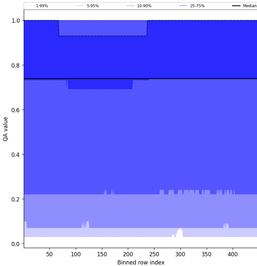
Figure 43: Along track statistics of “QA value” for 2025-01-05 to 2025-01-05
