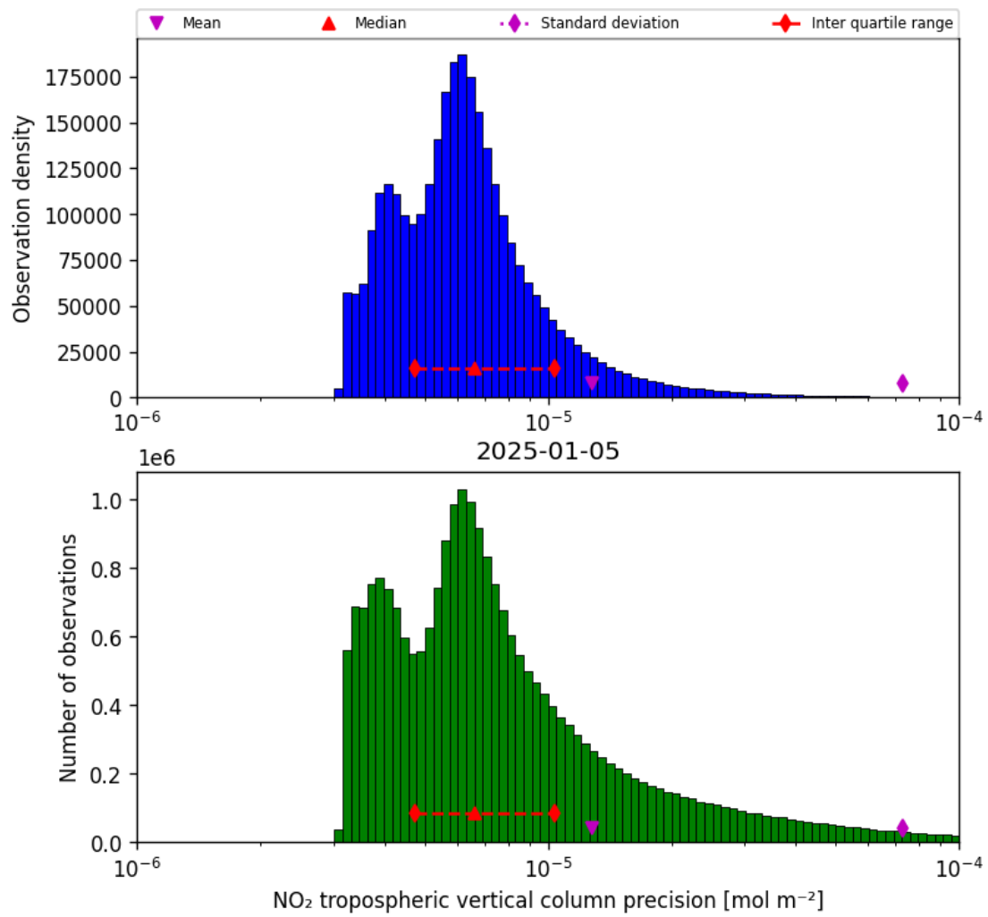
Figure 28: Histogram of "NO 2 tropospheric vertical column precision" for 2025-01-05 to 2025-01-05
