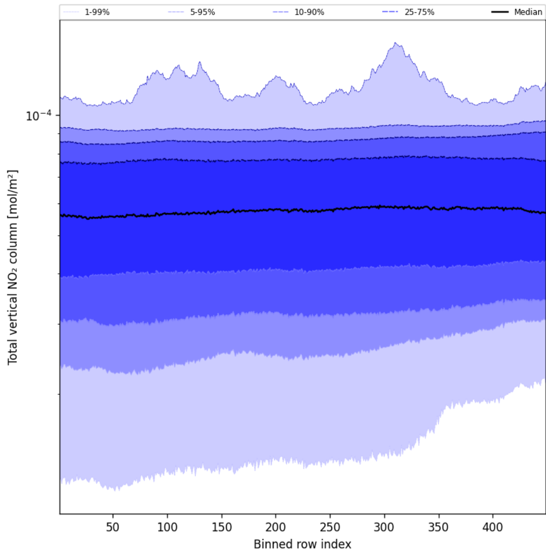
Figure 53: Along track statistics of “Total vertical NO 2 column” for 2025-01-05 to 2025-01-05
