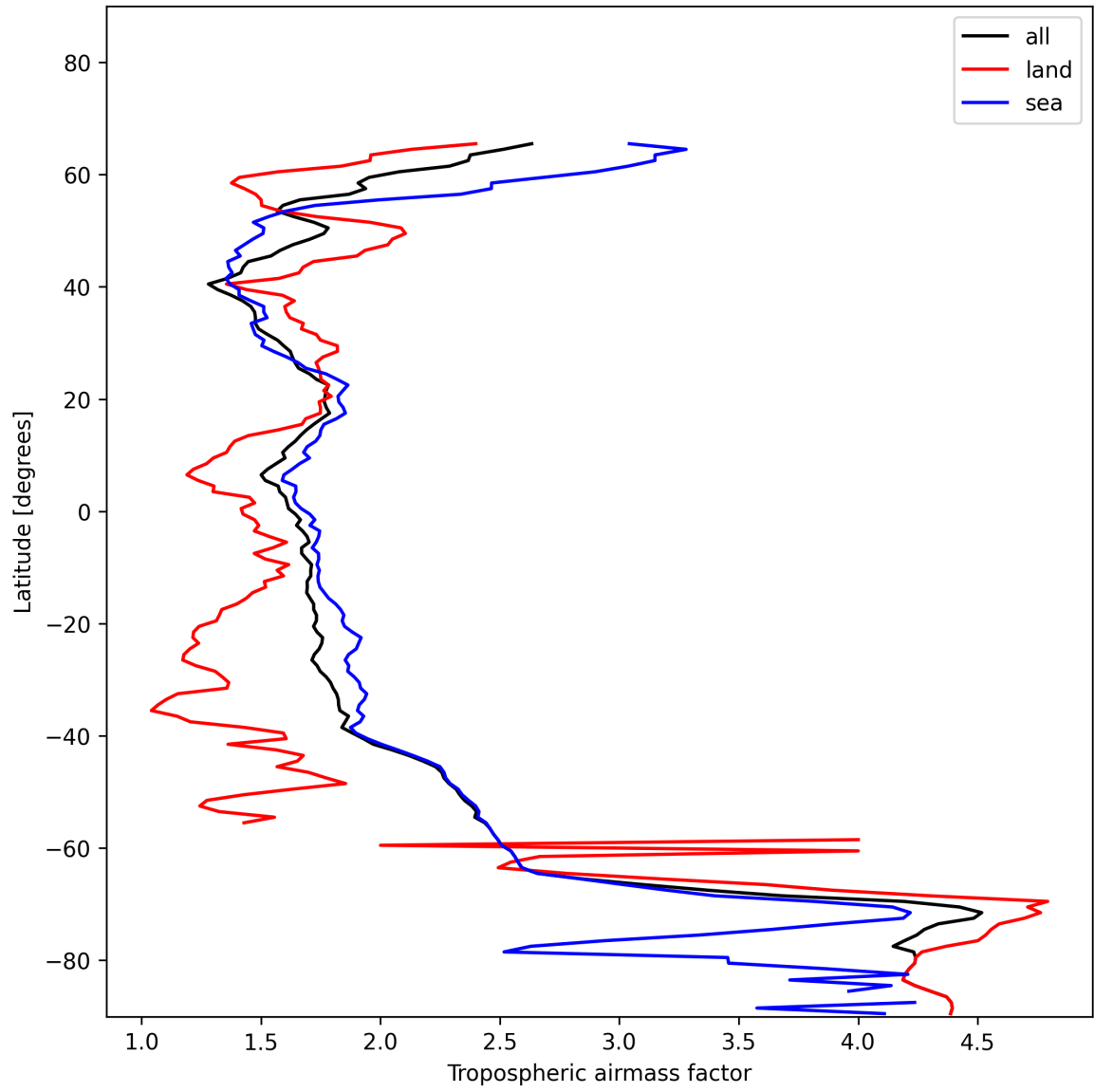
Figure 12: Zonal average of “Tropospheric airmass factor” for 2025-01-05 to 2025-01-05.
