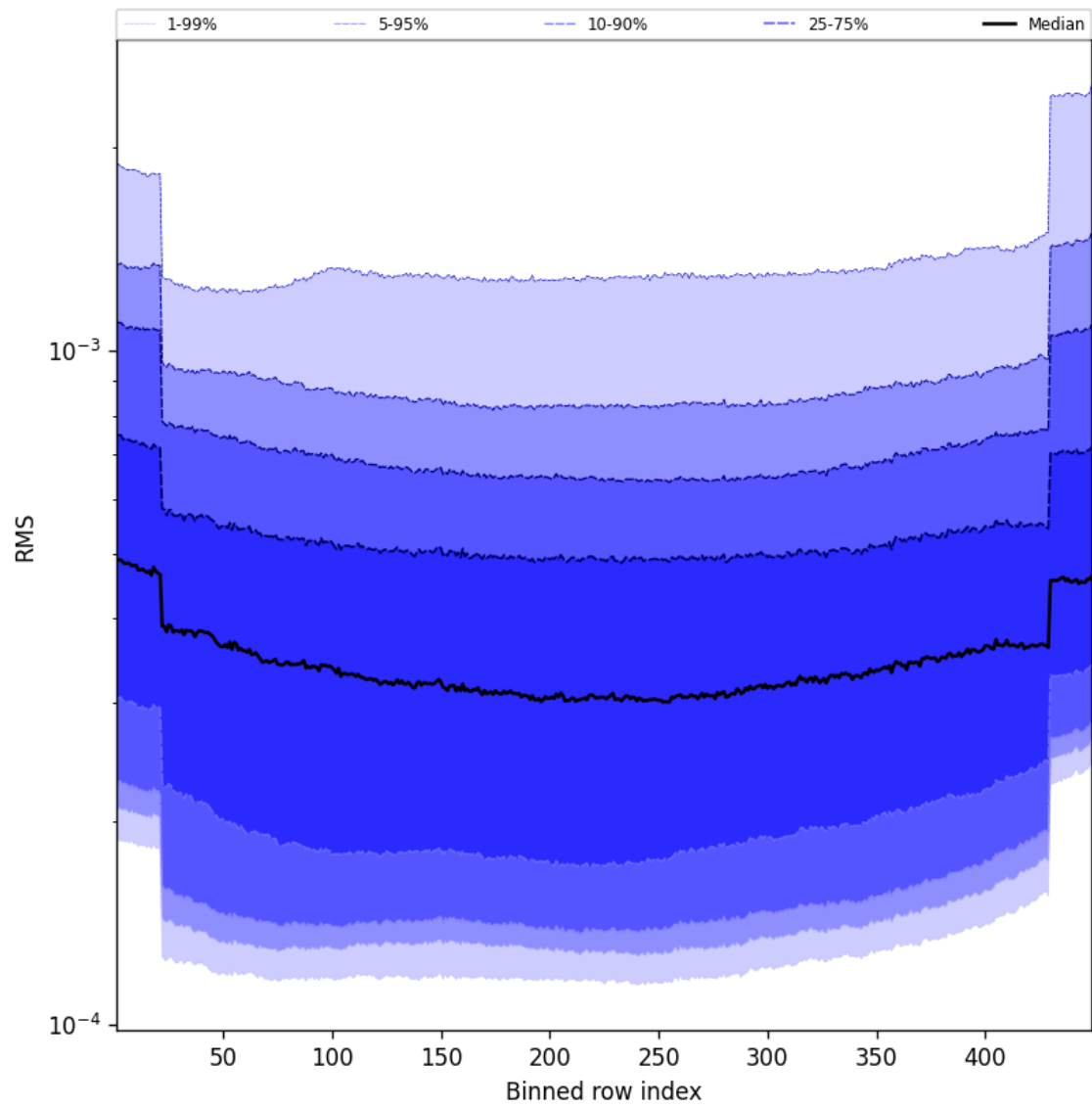
Figure 58: Along track statistics of “RMS” for 2025-01-05 to 2025-01-05
