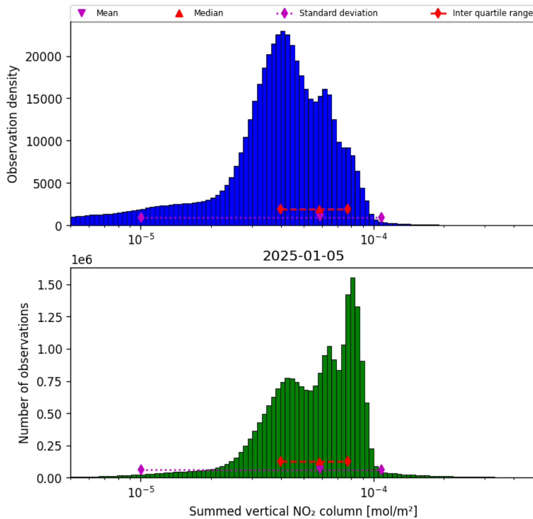
Figure 38: Histogram of “Summed vertical NO 2 column” for 2025-01-05 to 2025-01-05
