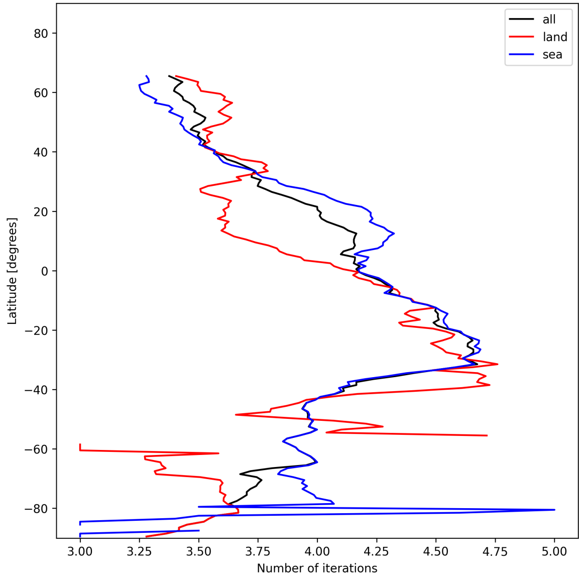
Figure 15: Zonal average of “Number of iterations” for 2025-01-05 to 2025-01-05.
