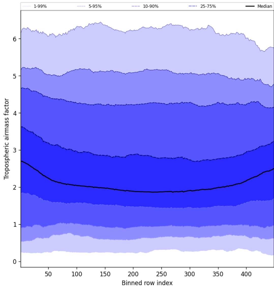
Figure 46: Along track statistics of “Tropospheric air mass factor” for 2025-01-05 to 2025-01-05
