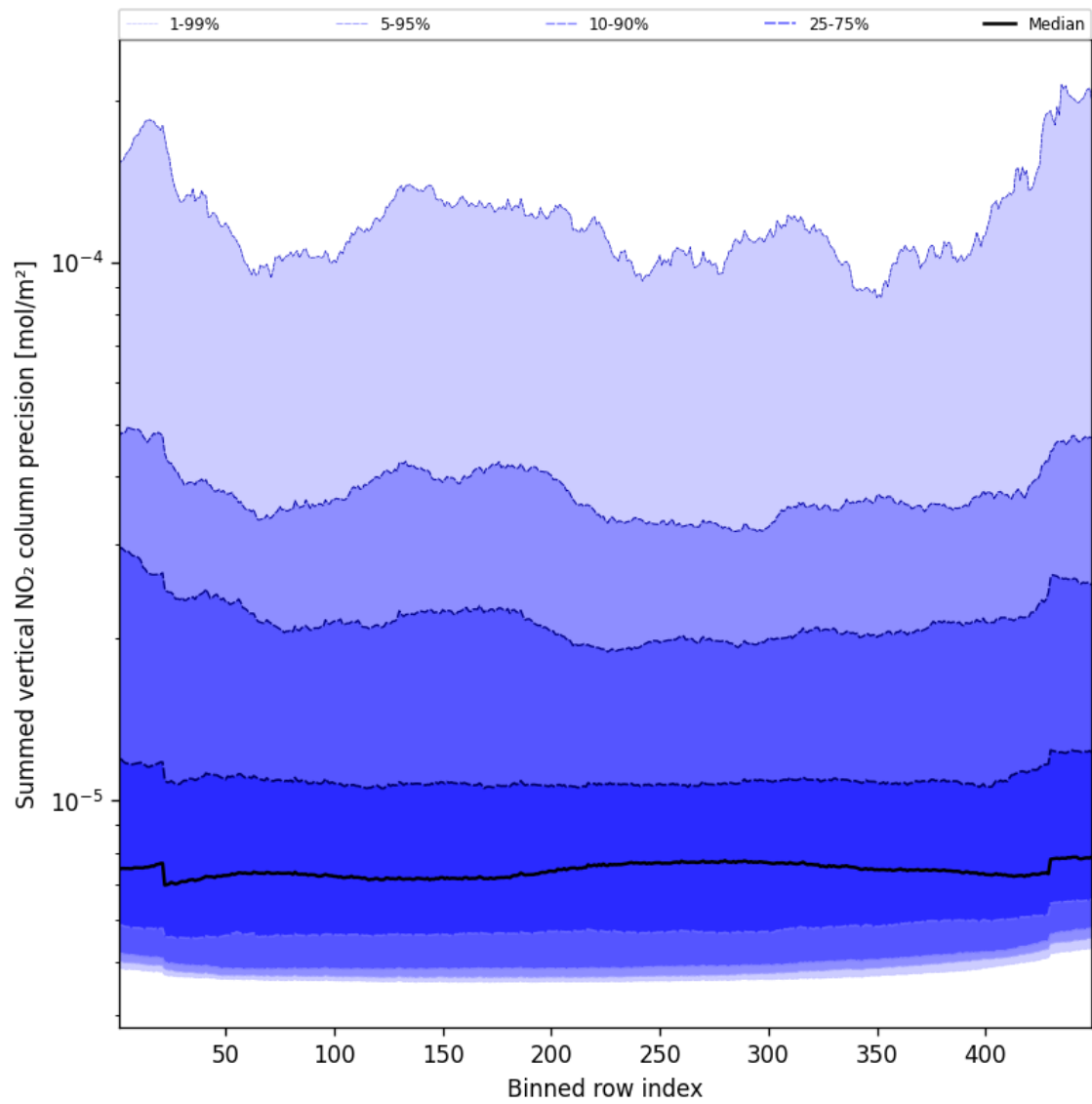
Figure 56: Along track statistics of “Summed vertical NO 2 column precision” for 2025-01-05 to 2025-01-05
