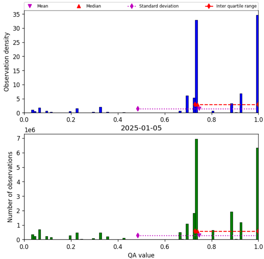
Figure 26: Histogram of “QA value” for 2025-01-05 to 2025-01-05
