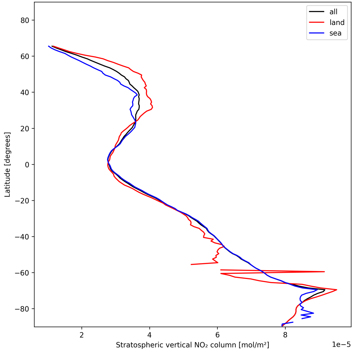
Figure 17: Zonal average of “Stratospheric vertical NO 2 column” for 2025-01-05 to 2025-01-05.
