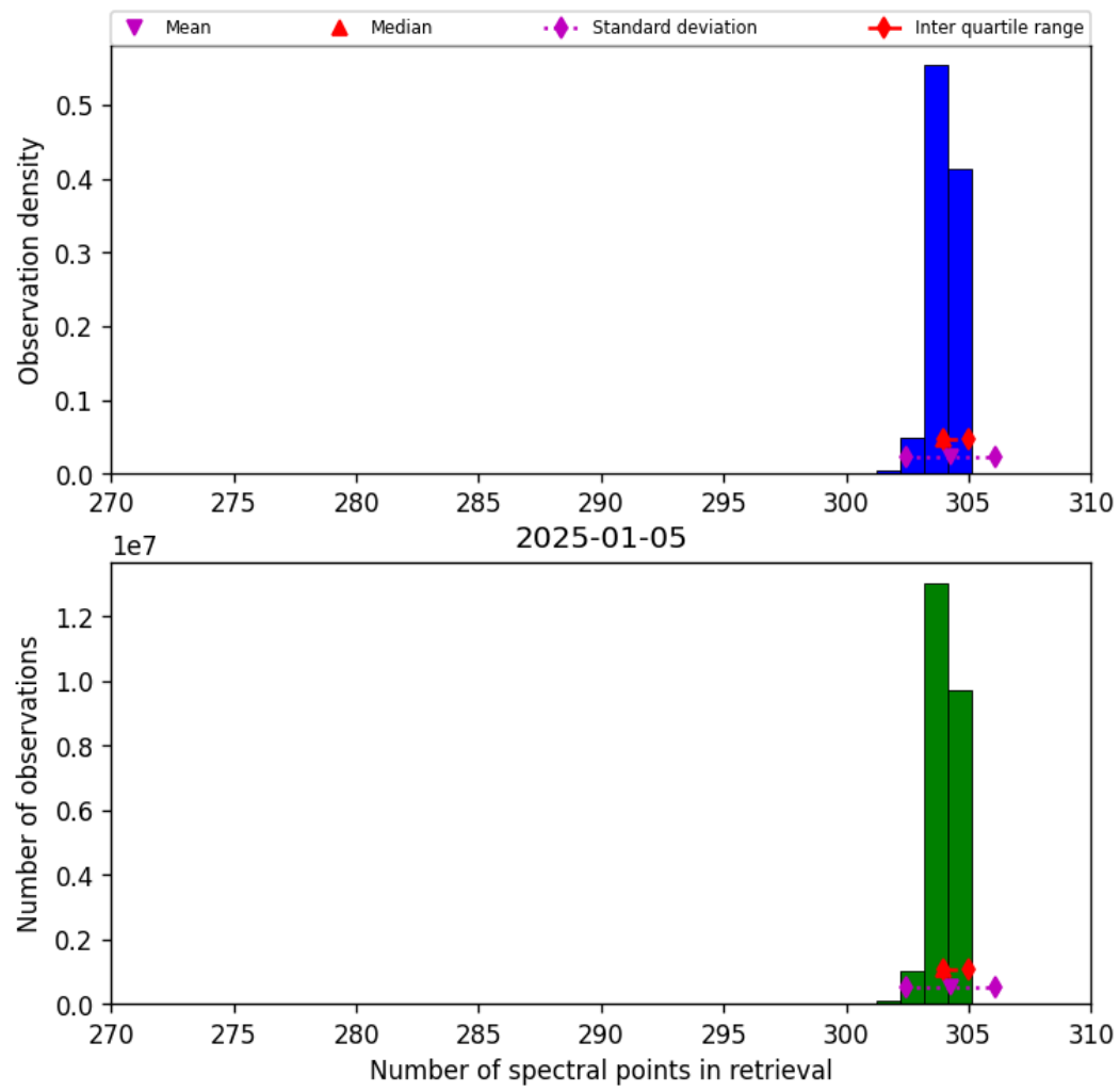
Figure 31: Histogram of “Number of spectral points in retrieval” for 2025-01-05 to 2025-01-05
