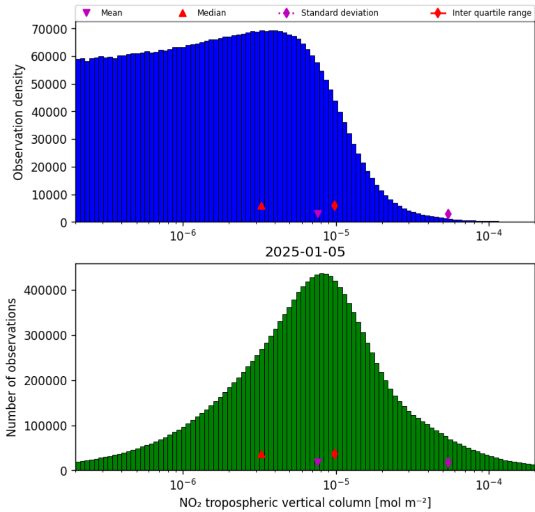
Figure 27: Histogram of “NO 2 tropospheric vertical column” for 2025-01-05 to 2025-01-05
