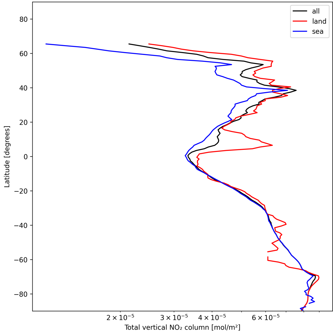
Figure 19: Zonal average of “Total vertical NO 2 column” for 2025-01-05 to 2025-01-05.
