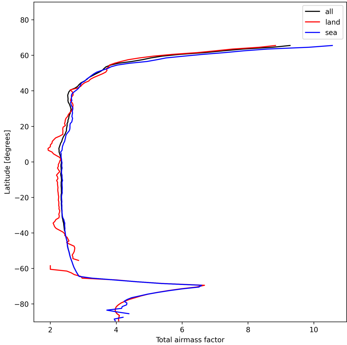
Figure 13: Zonal average of “Total airmass factor” for 2025-01-05 to 2025-01-05.
