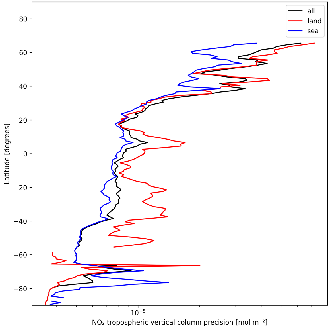
Figure 11: Zonal average of “NO 2 tropospheric vertical column precision” for 2025-01-05 to 2025-01-05.
