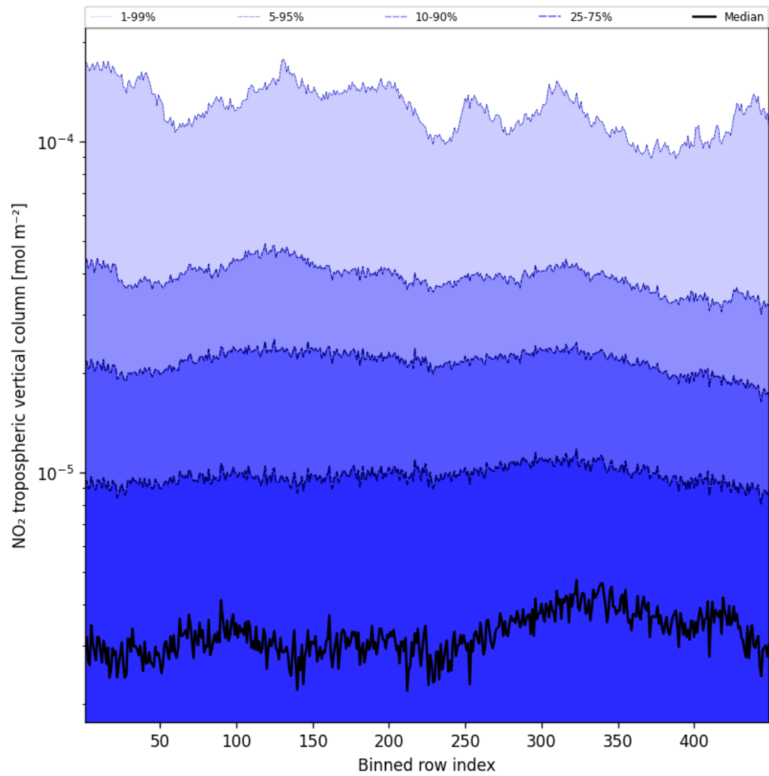
Figure 44: Along track statistics of “NO 2 tropospheric vertical column” for 2025-01-05 to 2025-01-05
