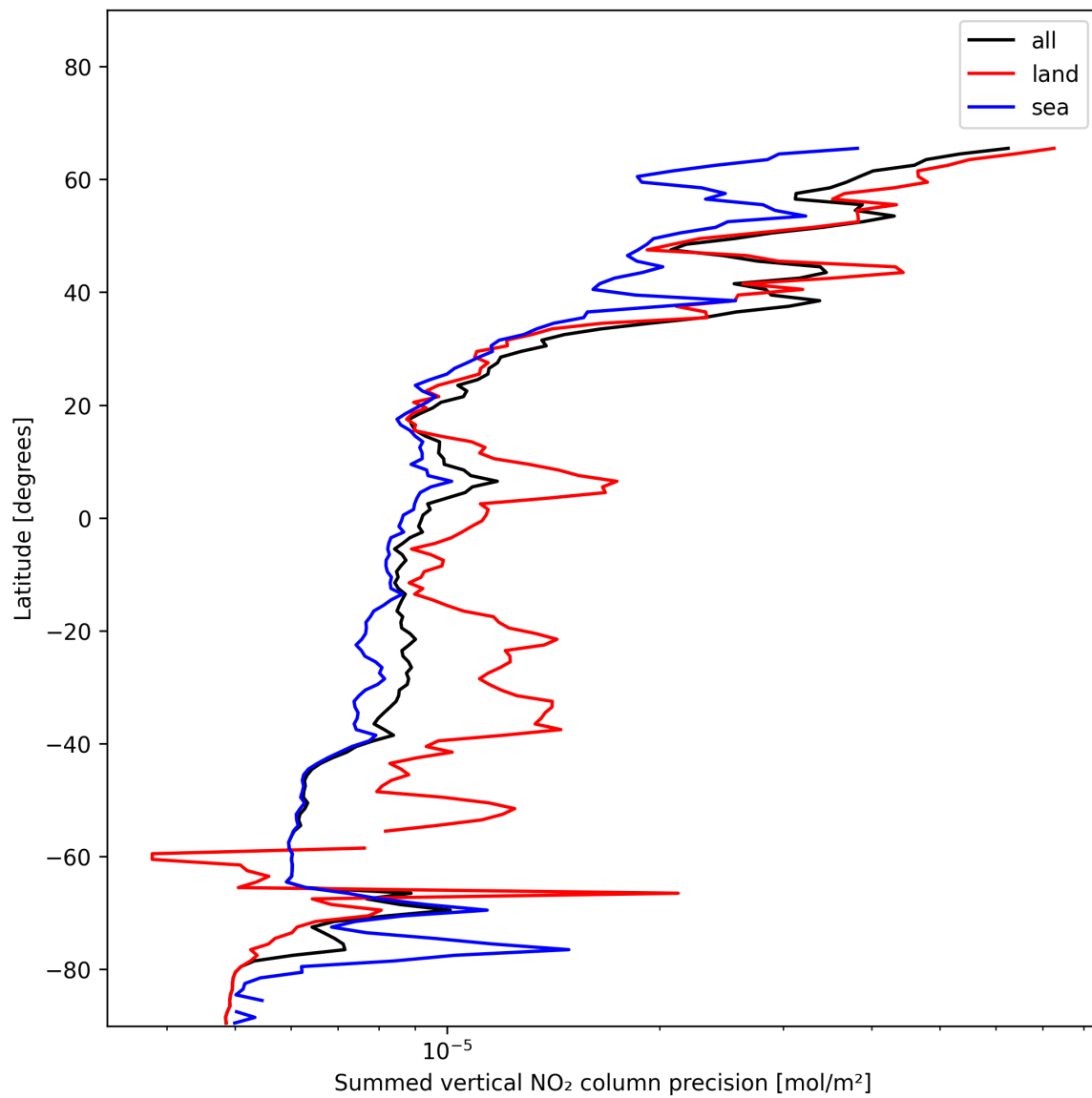
Figure 22: Zonal average of “Summed vertical NO 2 column precision” for 2025-01-05 to 2025-01-05.
