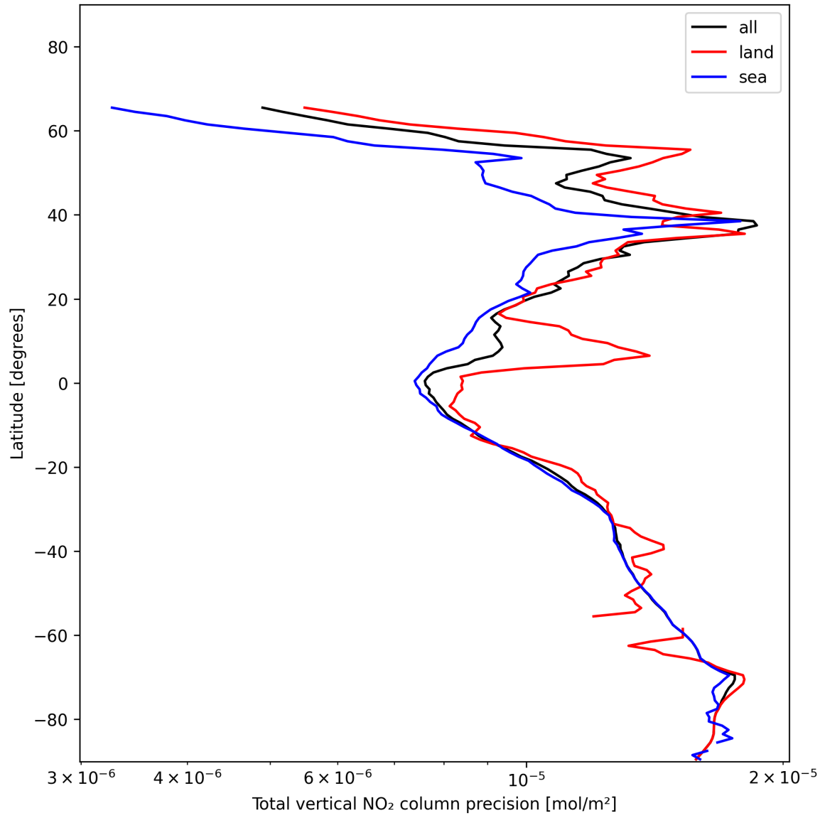
Figure 20: Zonal average of “Total vertical NO 2 column precision” for 2025-01-05 to 2025-01-05.
