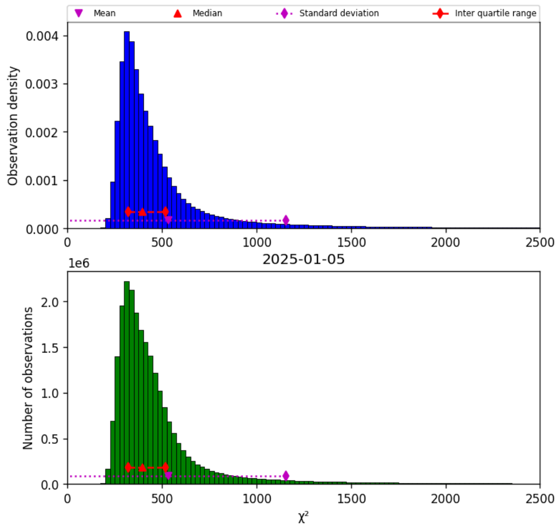
Figure 40: Histogram of " \chi^2 " for 2025-01-05 to 2025-01-05
