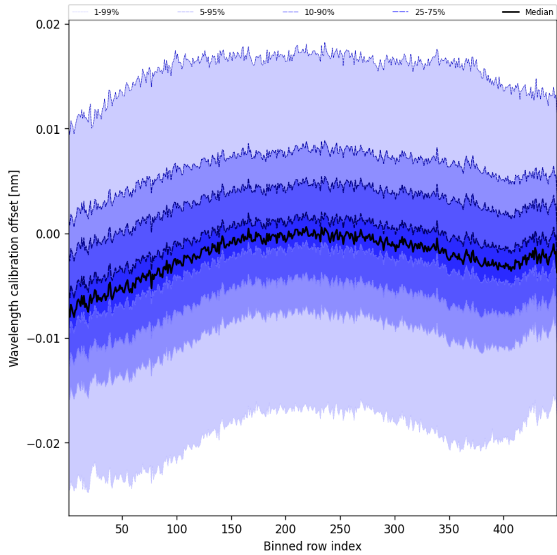
Figure 50: Along track statistics of “Wavelength calibration offset” for 2025-01-05 to 2025-01-05
