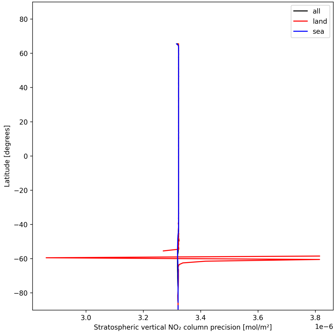
Figure 18: Zonal average of “Stratospheric vertical NO 2 column precision” for 2025-01-05 to 2025-01-05.
