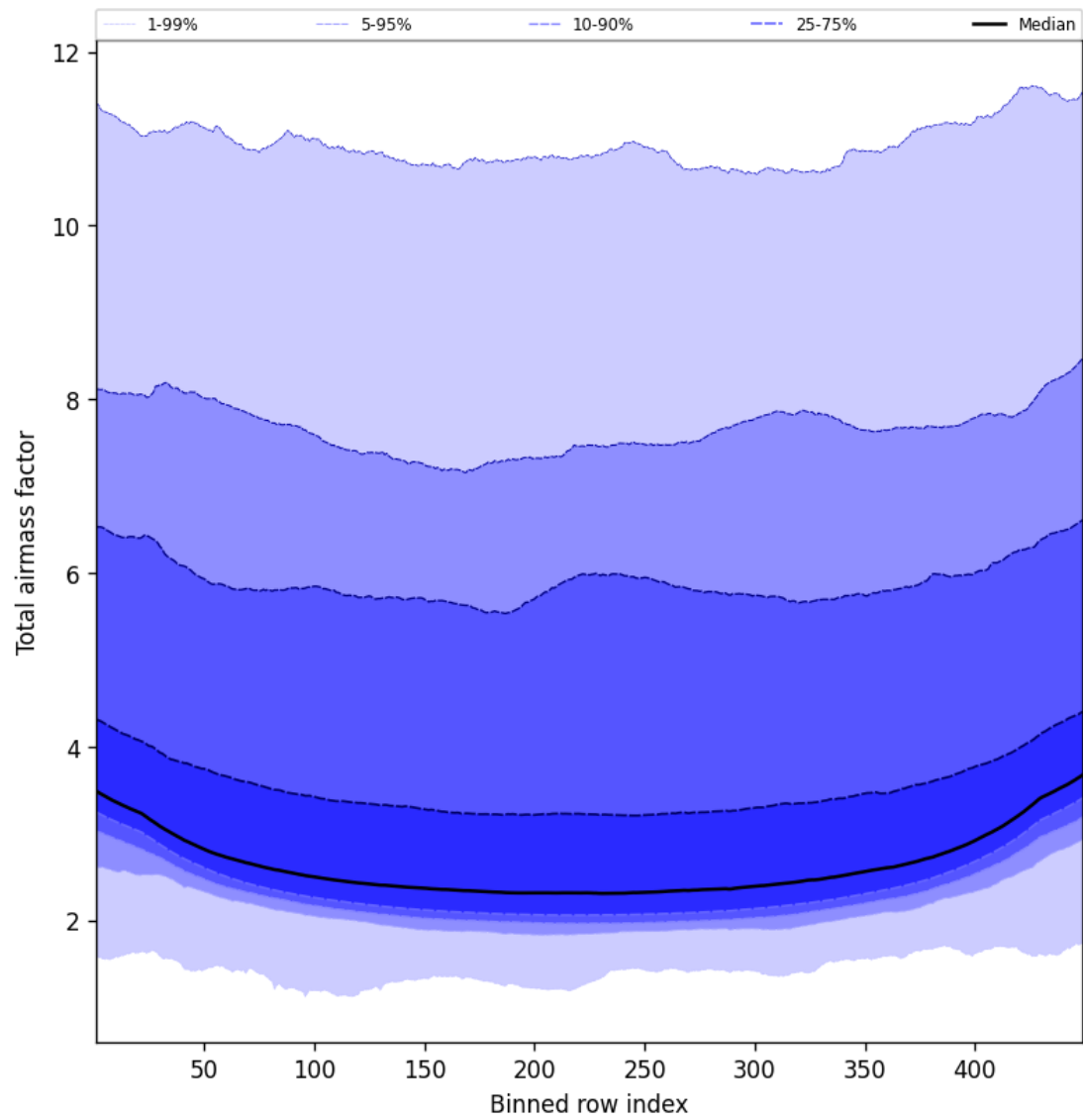
Figure 47: Along track statistics of “Total airmass factor” for 2025-01-05 to 2025-01-05
