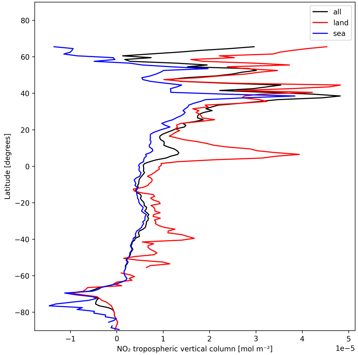
Figure 10: Zonal average of “NO 2 tropospheric vertical column” for 2025-01-05 to 2025-01-05.
