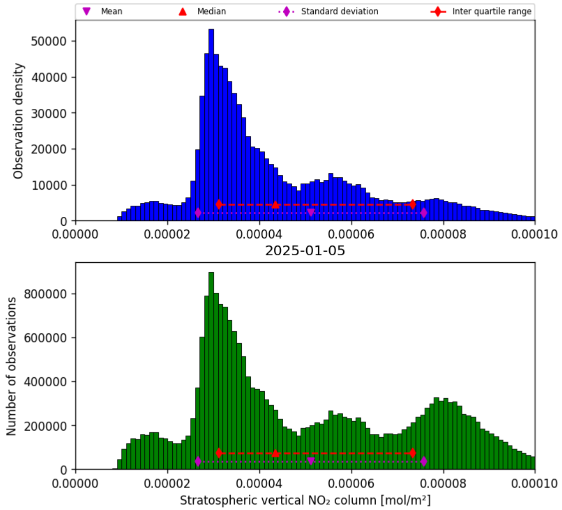
Figure 34: Histogram of “Stratospheric vertical NO 2 column” for 2025-01-05 to 2025-01-05
