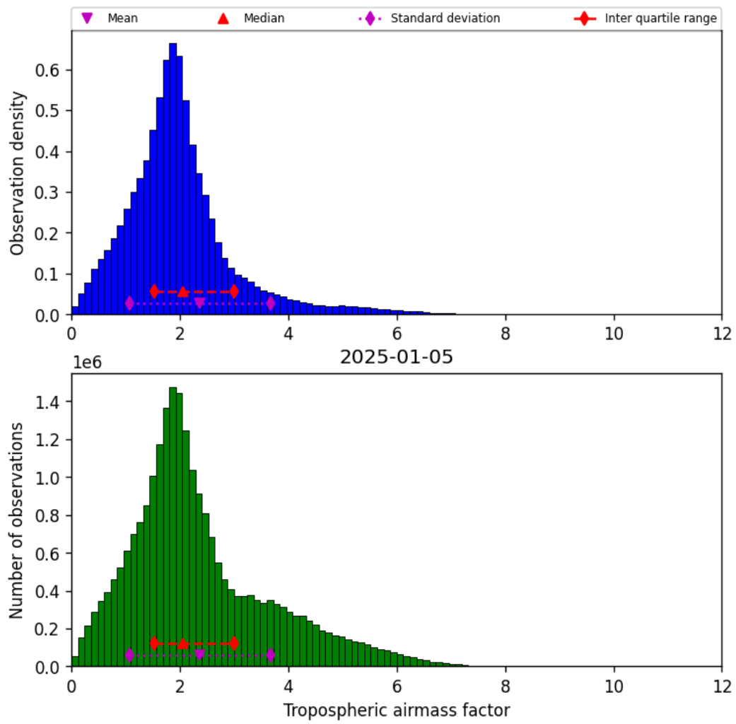
Figure 29: Histogram of “Tropospheric airmass factor” for 2025-01-05 to 2025-01-05
