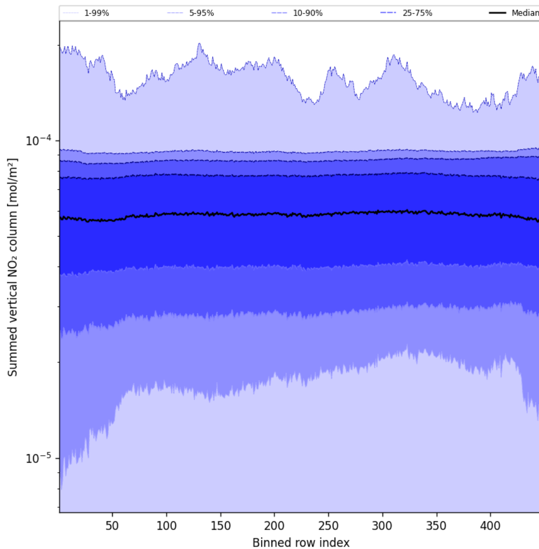
Figure 55: Along track statistics of “Summed vertical NO 2 column” for 2025-01-05 to 2025-01-05
