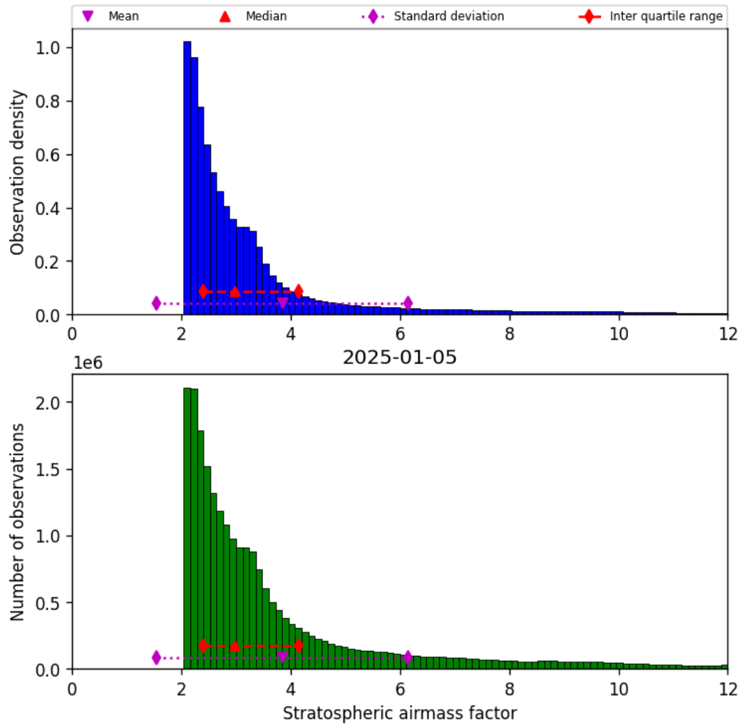
Figure 42: Histogram of “Stratospheric airmass factor” for 2025-01-05 to 2025-01-05
