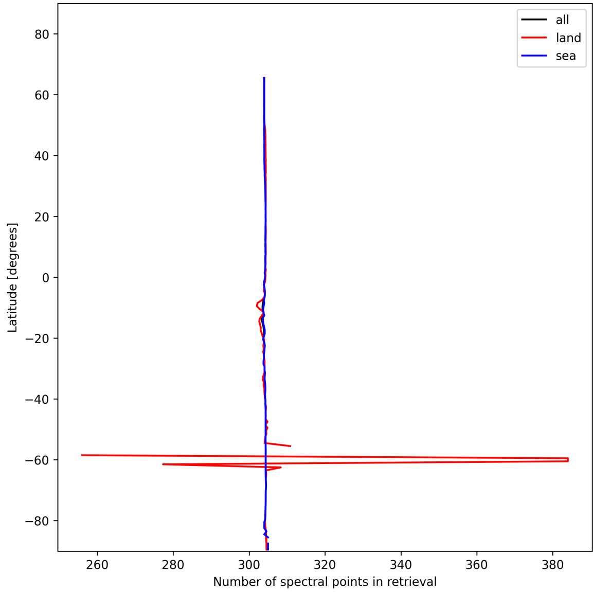
Figure 14: Zonal average of “Number of spectral points in retrieval” for 2025-01-05 to 2025-01-05.
