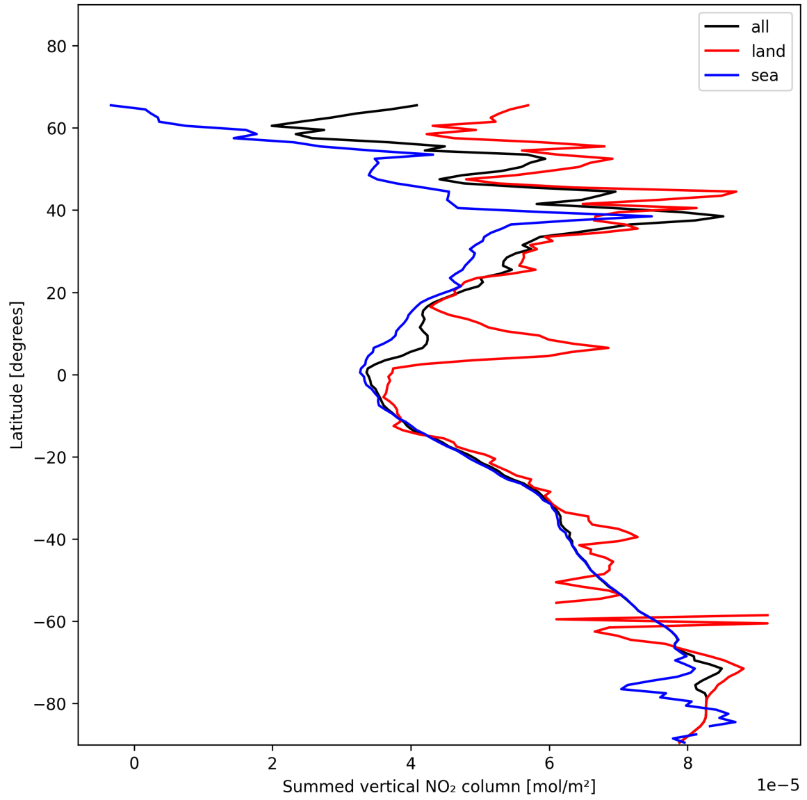
Figure 21: Zonal average of “Summed vertical NO 2 column” for 2025-01-05 to 2025-01-05.
