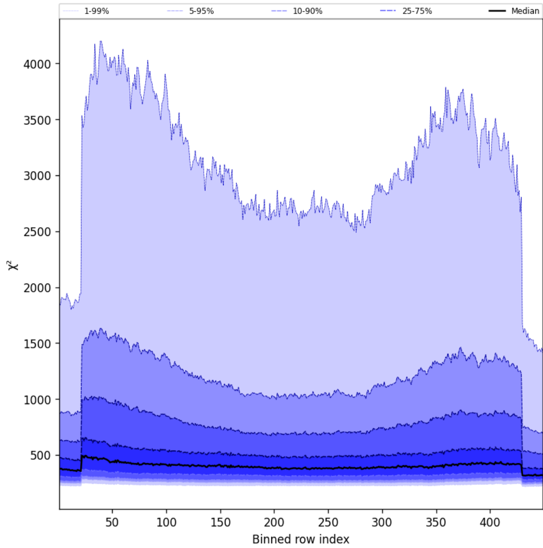
Figure 57: Along track statistics of “ \chi^2 ” for 2025-01-05 to 2025-01-05
