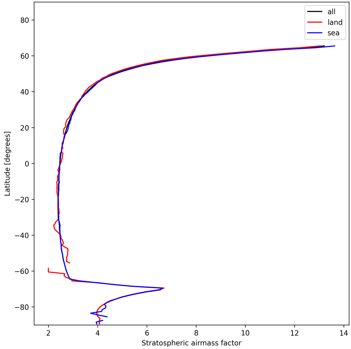
Figure 25: Zonal average of “Stratospheric air mass factor” for 2025-01-05 to 2025-01-05.
