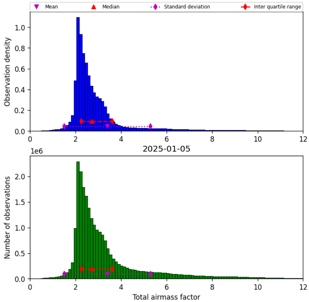
Figure 30: Histogram of “Total airmass factor” for 2025-01-05 to 2025-01-05
