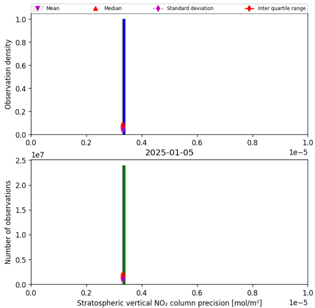
Figure 35: Histogram of “Stratospheric vertical NO 2 column precision” for 2025-01-05 to 2025-01-05
