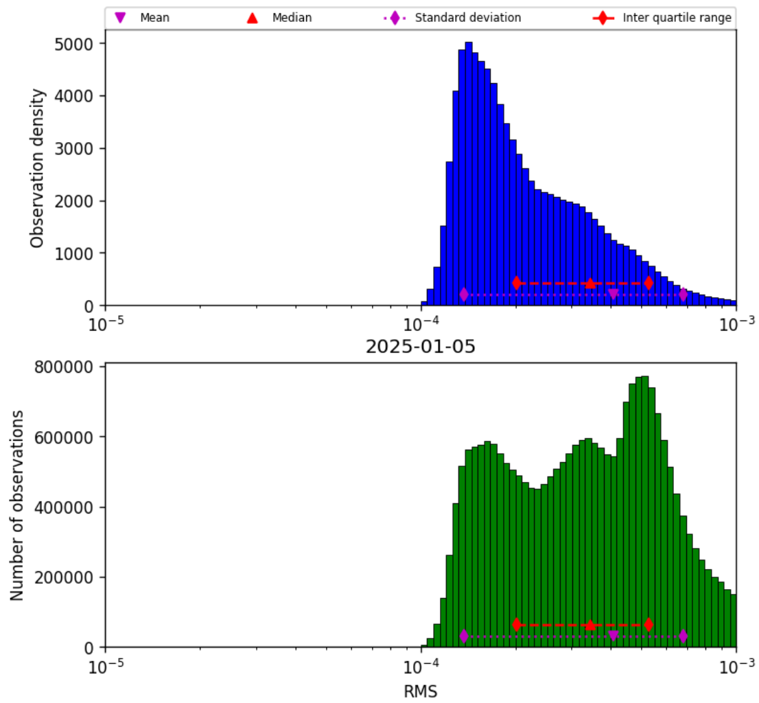
Figure 41: Histogram of “RMS” for 2025-01-05 to 2025-01-05
