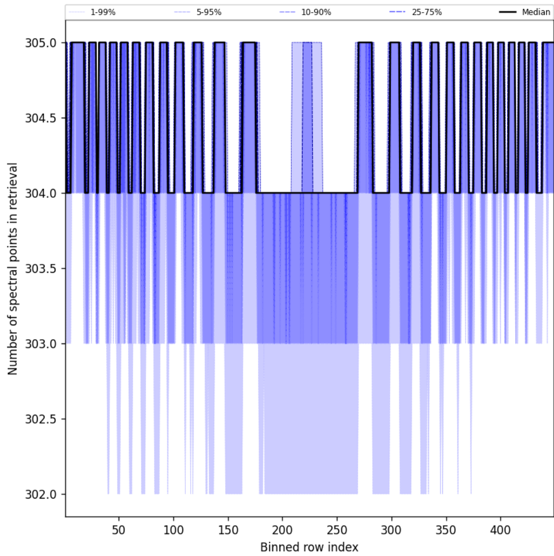
Figure 48: Along track statistics of “Number of spectral points in retrieval” for 2025-01-05 to 2025-01-05
