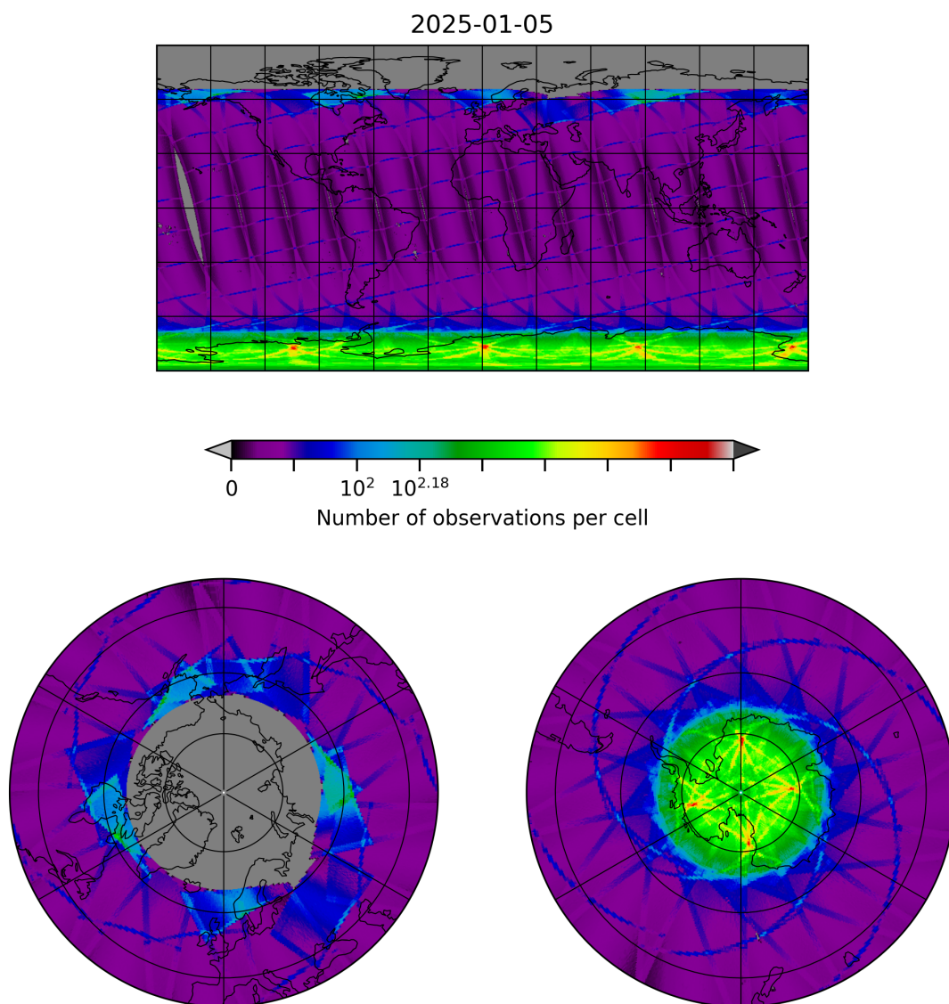
Figure 8: Map of the number of observations for 2025-01-05 to 2025-01-05
