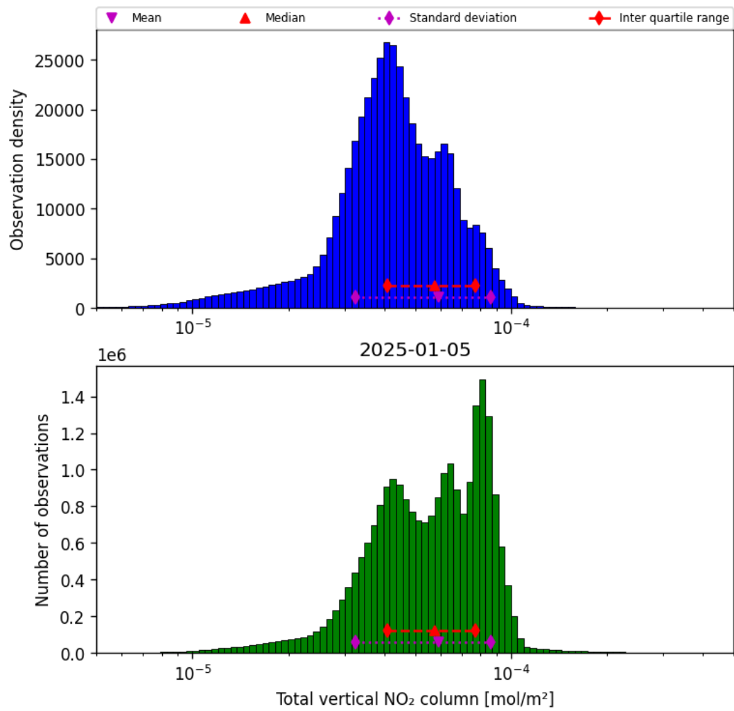
Figure 36: Histogram of “Total vertical NO 2 column” for 2025-01-05 to 2025-01-05
