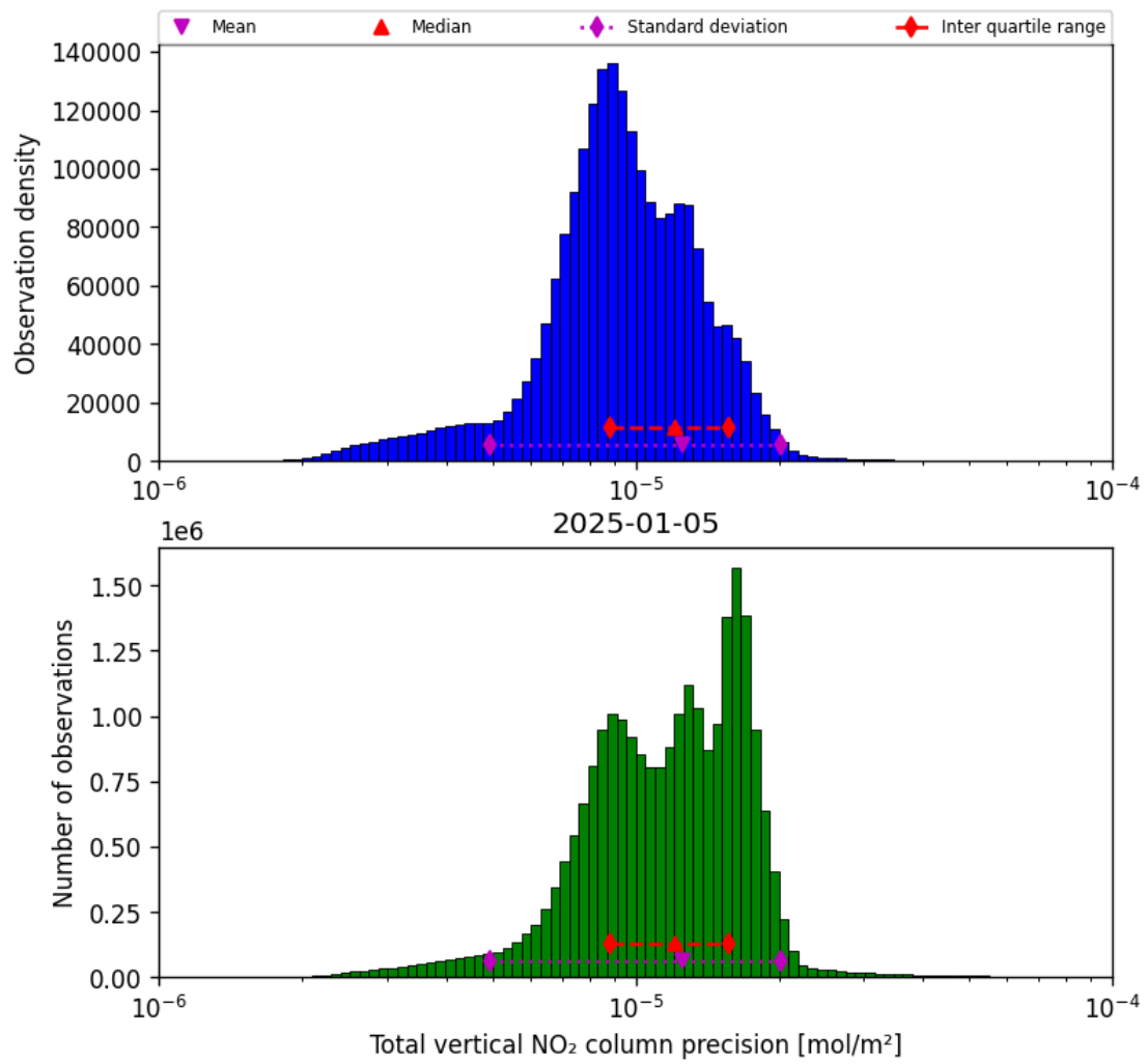
Figure 37: Histogram of “Total vertical NO 2 column precision” for 2025-01-05 to 2025-01-05
