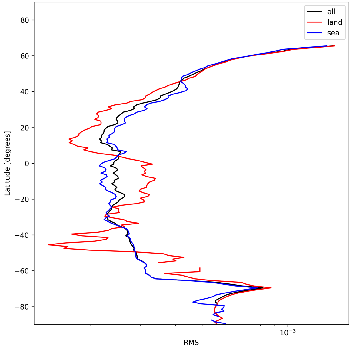
Figure 24: Zonal average of “RMS” for 2025-01-05 to 2025-01-05.
