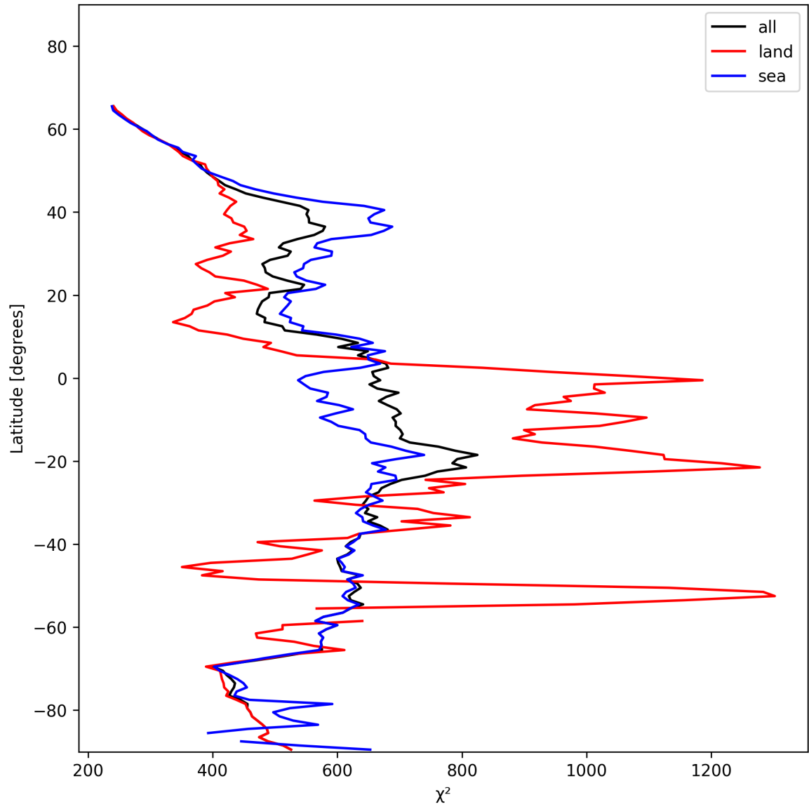
Figure 23: Zonal average of “ \chi^2 ” for 2025-01-05 to 2025-01-05.
