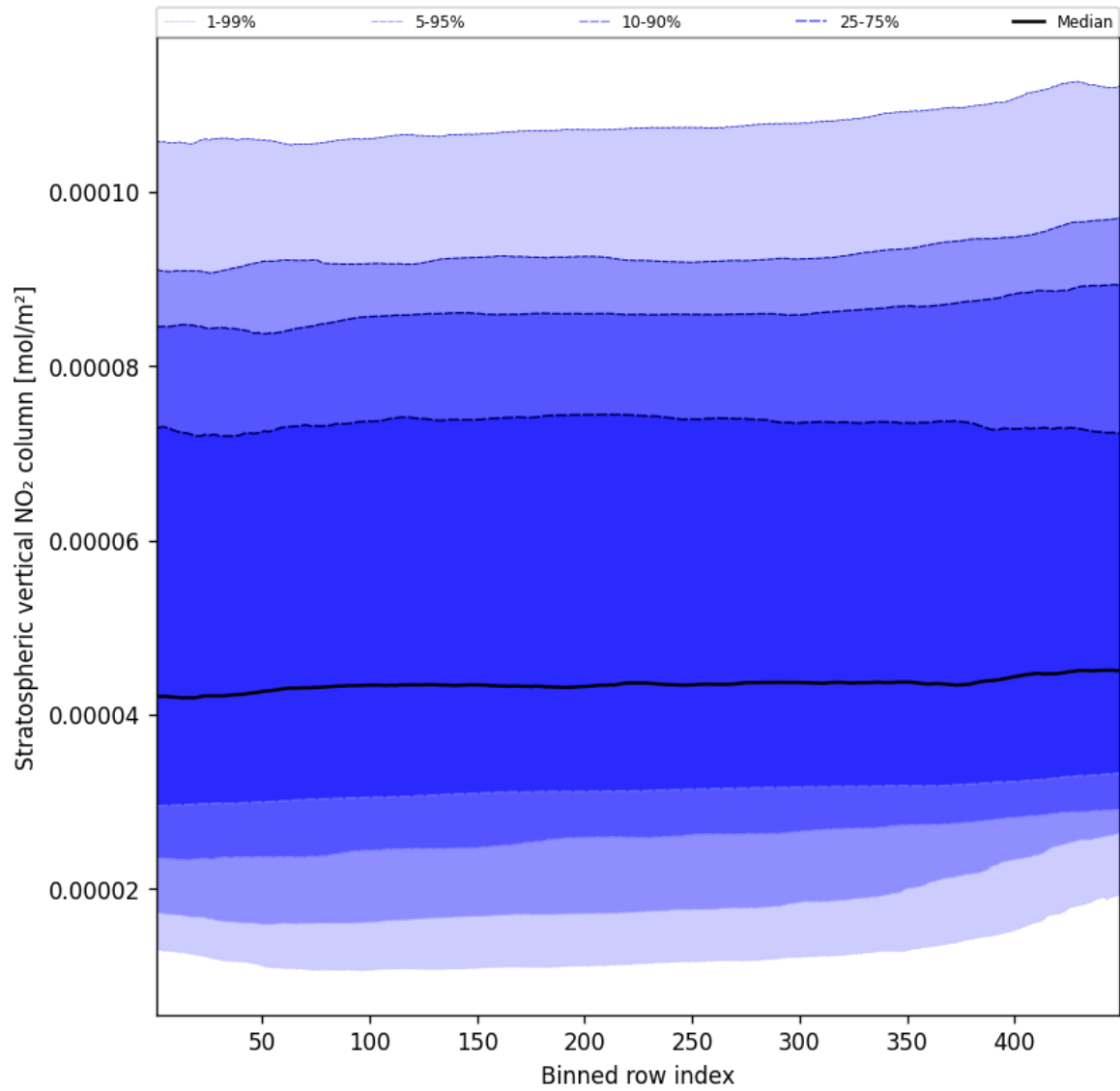
Figure 51: Along track statistics of “Stratospheric vertical NO 2 column” for 2025-01-05 to 2025-01-05
