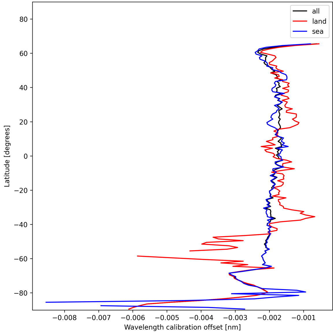
Figure 16: Zonal average of “Wavelength calibration offset” for 2025-01-05 to 2025-01-05.
