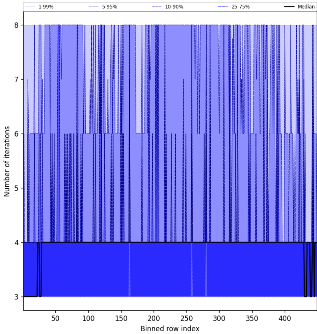
Figure 49: Along track statistics of “Number of iterations” for 2025-01-05 to 2025-01-05
