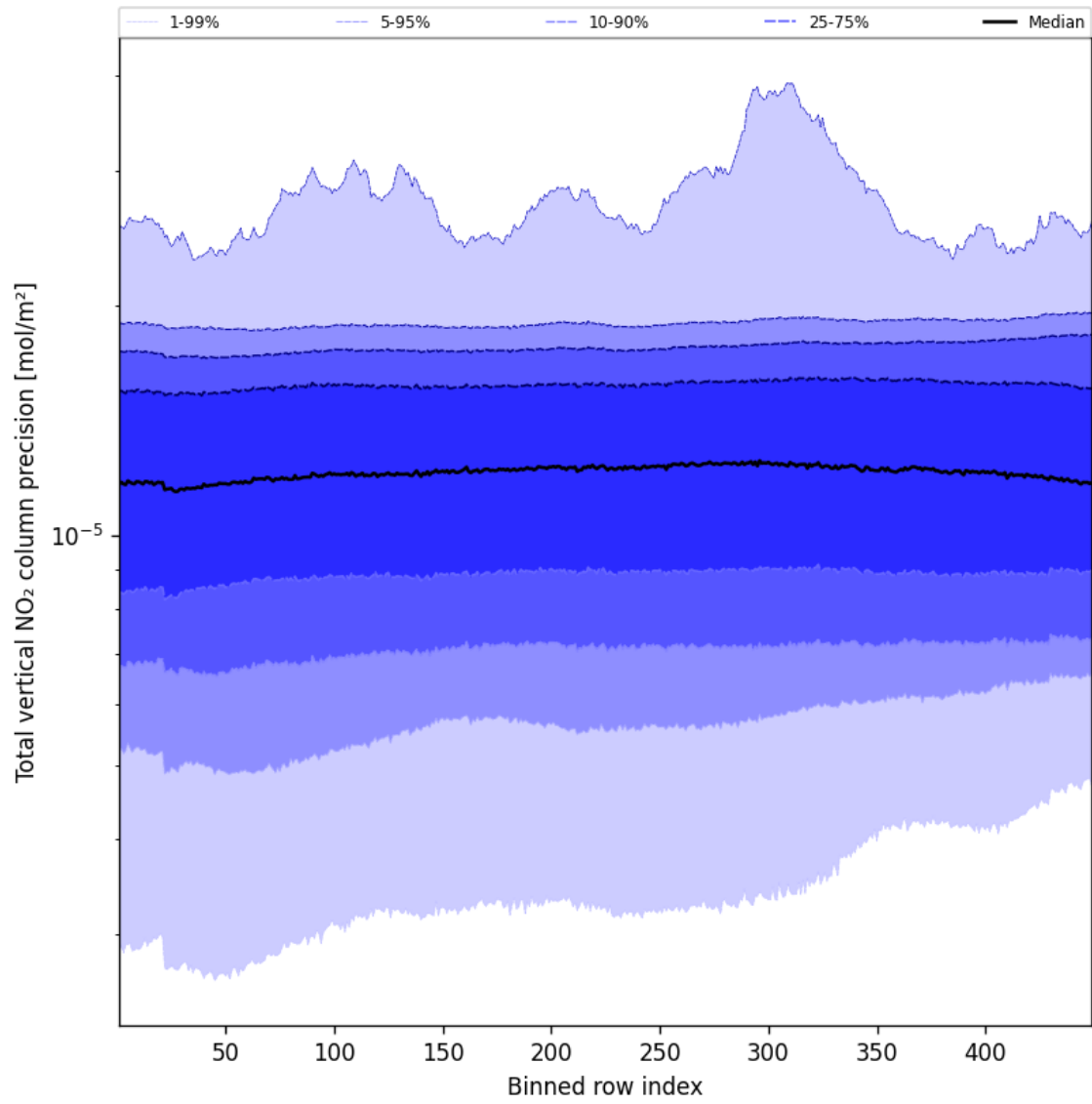
Figure 54: Along track statistics of “Total vertical NO 2 column precision” for 2025-01-05 to 2025-01-05
