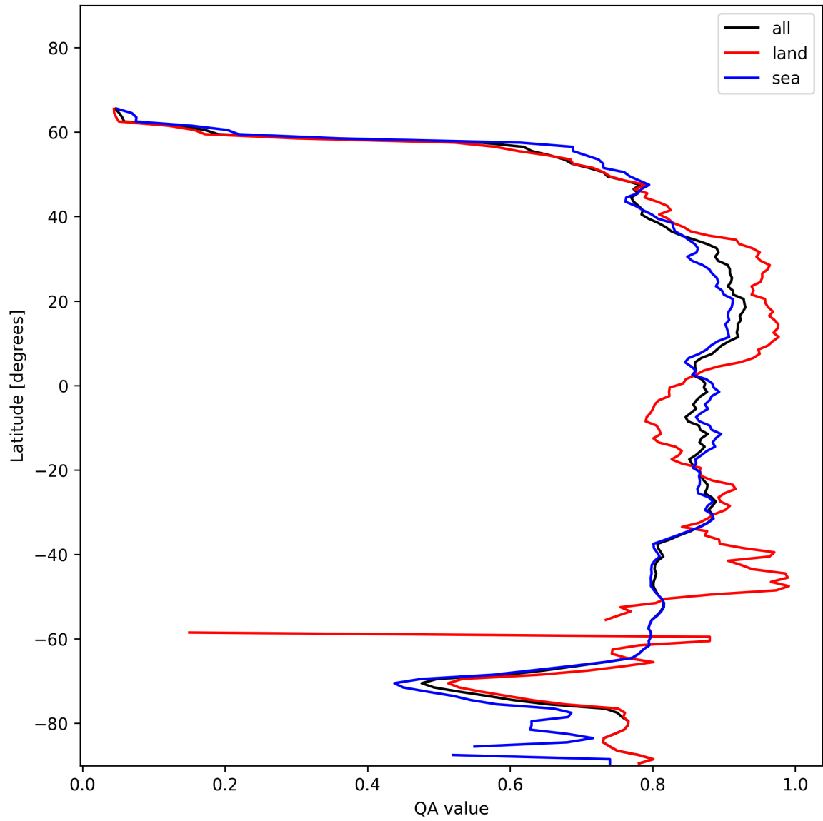
Figure 9: Zonal average of “QA value” for 2025-01-05 to 2025-01-05.
