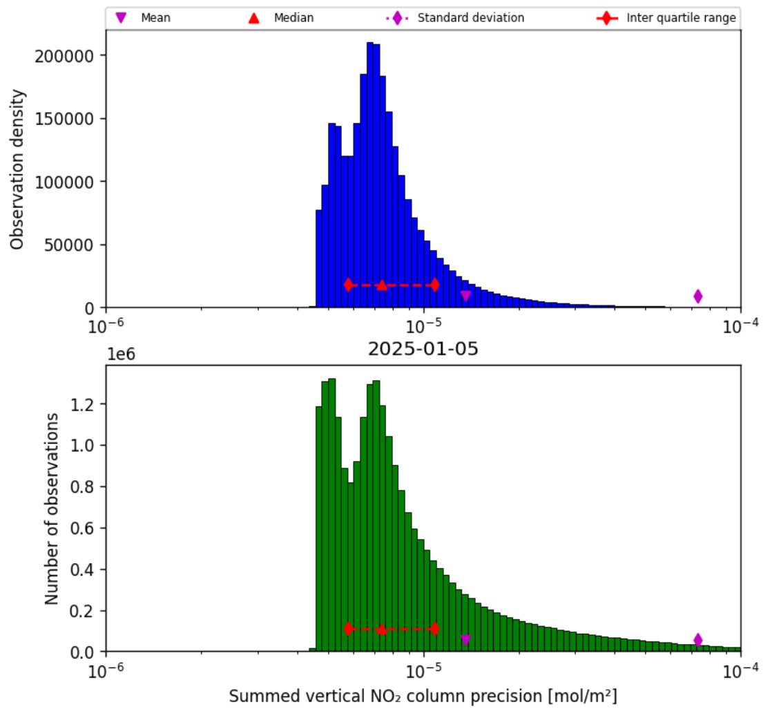
Figure 39: Histogram of "Summed vertical NO 2 column precision" for 2025-01-05 to 2025-01-05
