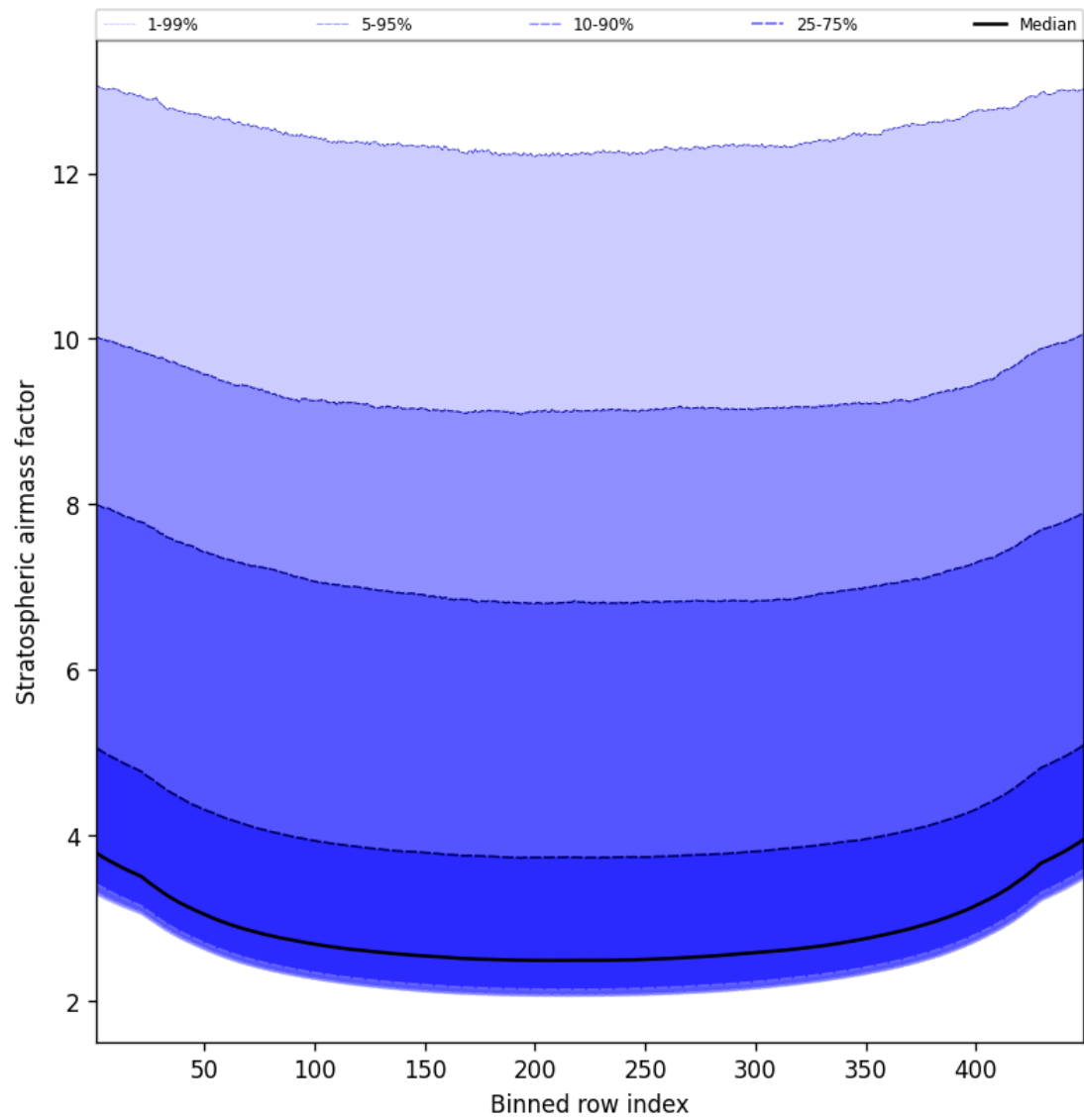
Figure 59: Along track statistics of “Stratospheric airmass factor” for 2025-01-05 to 2025-01-05
