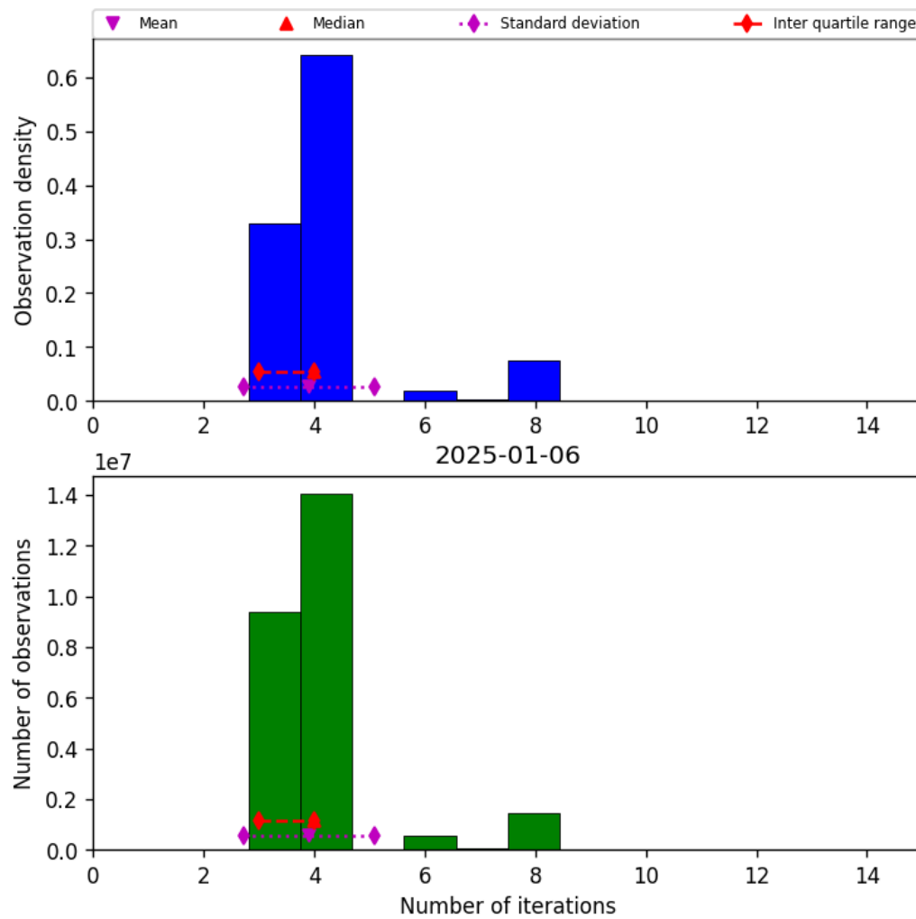
Figure 32: Histogram of “Number of iterations” for 2025-01-06 to 2025-01-07
