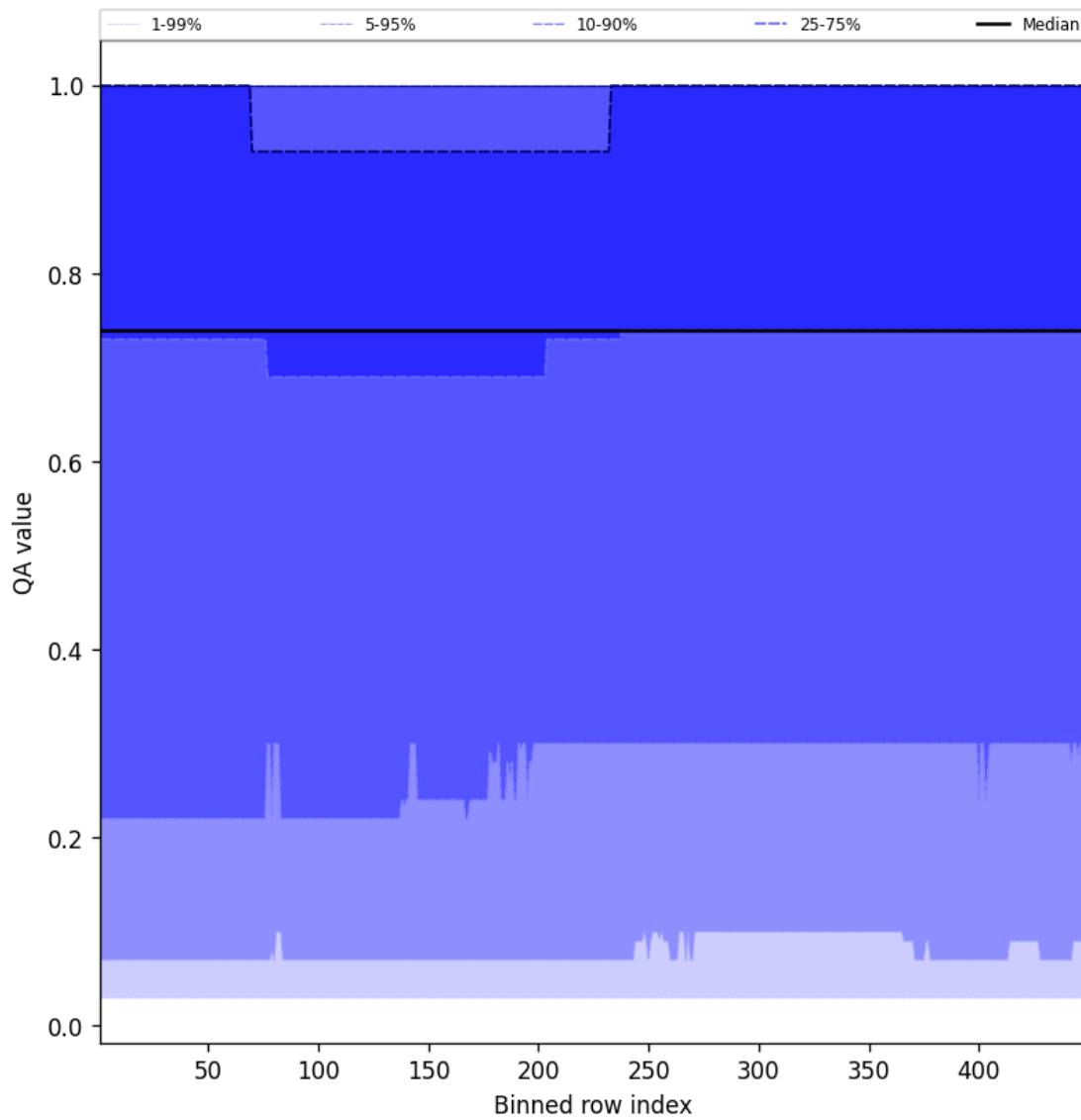
Figure 43: Along track statistics of “QA value” for 2025-01-06 to 2025-01-07
