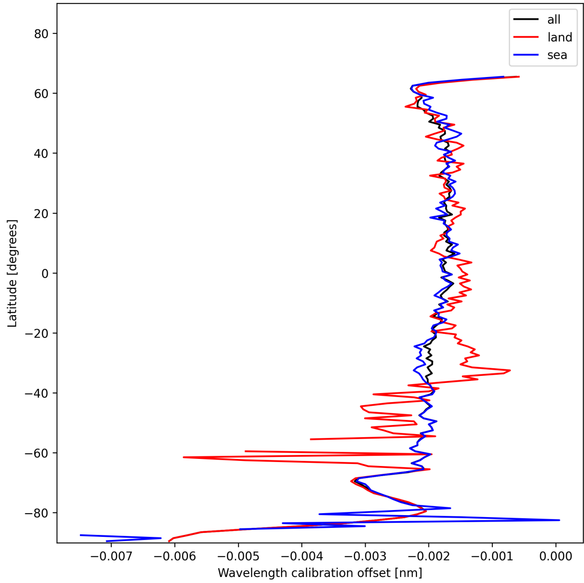
Figure 16: Zonal average of “Wavelength calibration offset” for 2025-01-06 to 2025-01-07.
