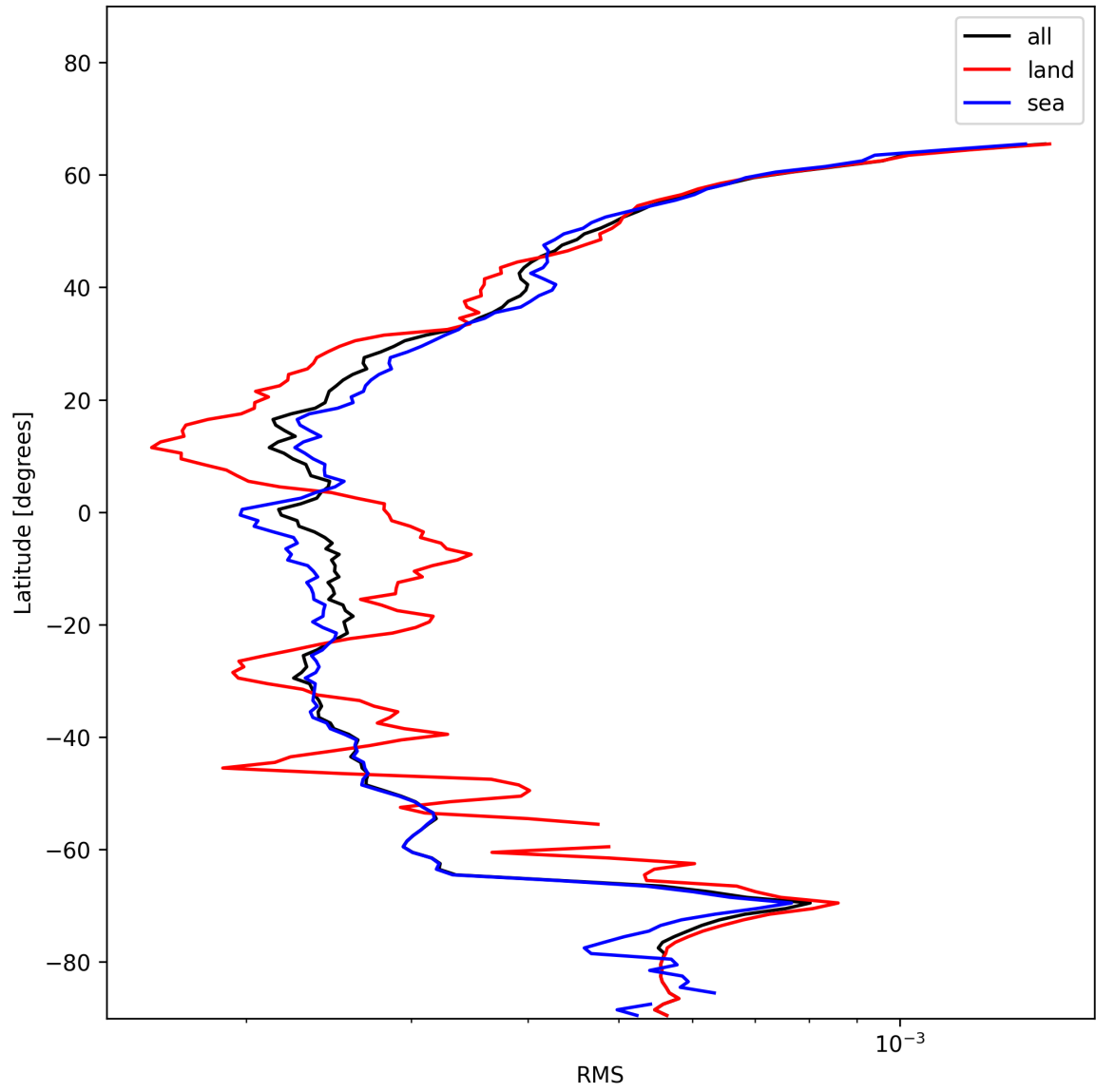
Figure 24: Zonal average of “RMS” for 2025-01-06 to 2025-01-07.
