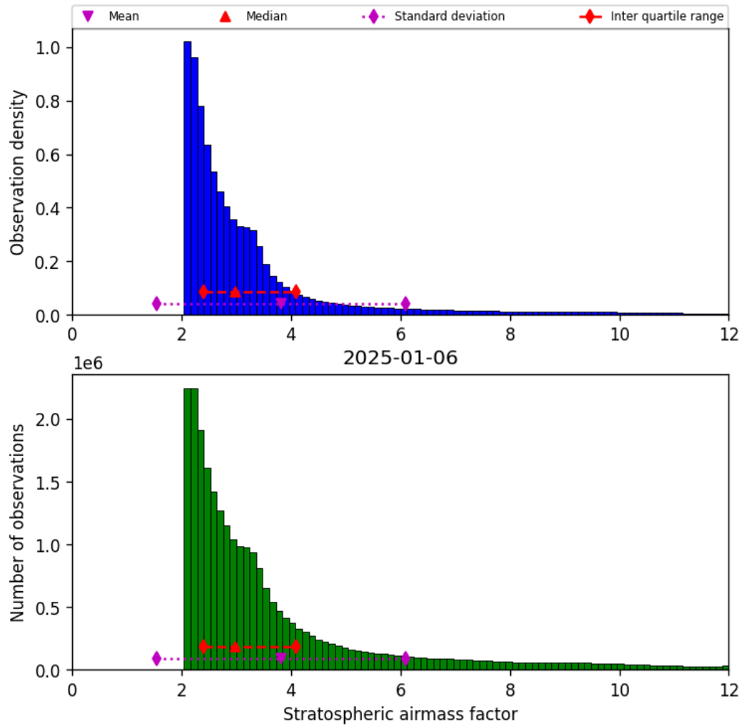
Figure 42: Histogram of “Stratospheric airmass factor” for 2025-01-06 to 2025-01-07
