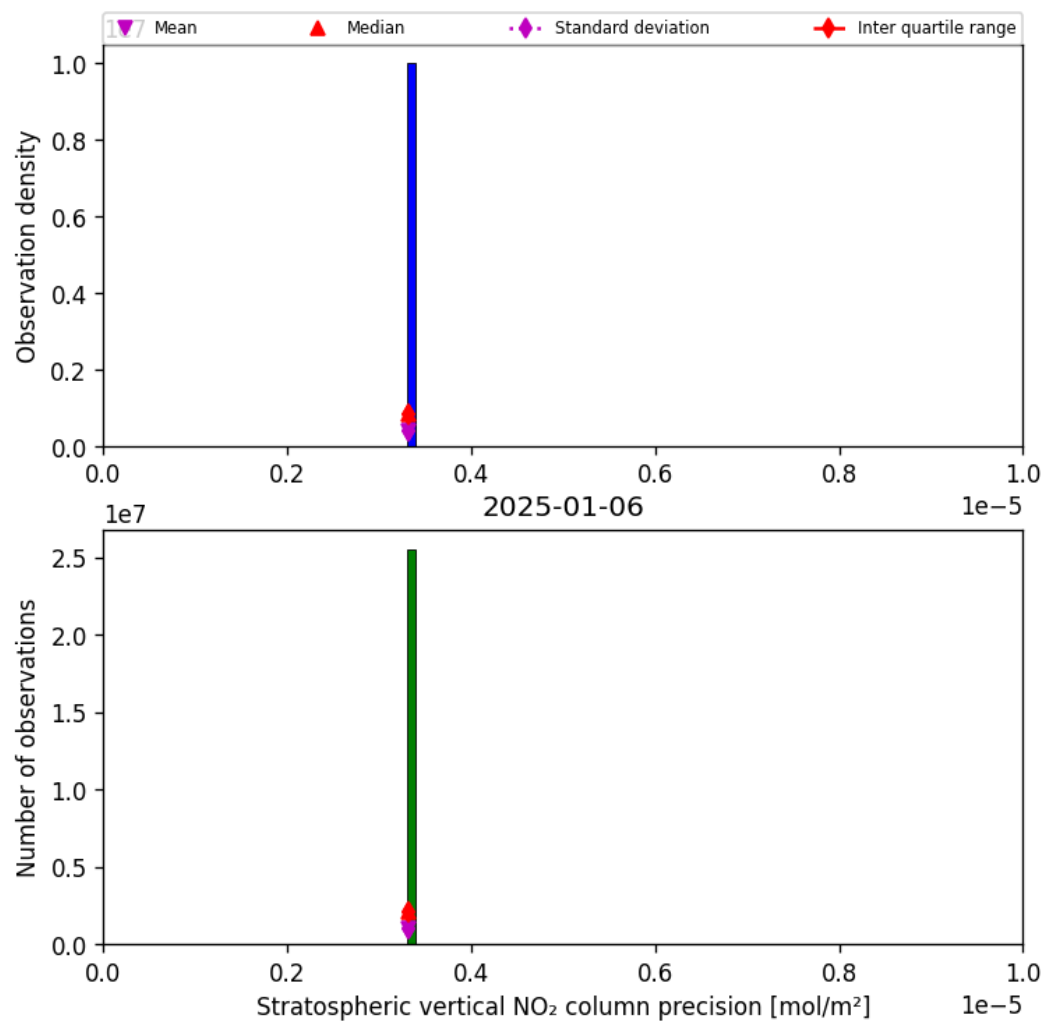
Figure 35: Histogram of “Stratospheric vertical NO 2 column precision” for 2025-01-06 to 2025-01-07
