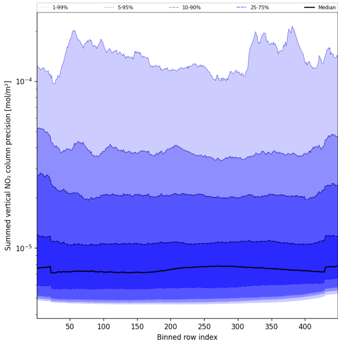
Figure 56: Along track statistics of “Summed vertical NO 2 column precision” for 2025-01-06 to 2025-01-07
