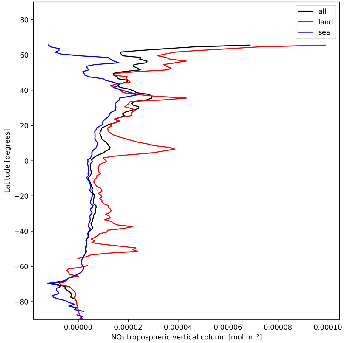
Figure 10: Zonal average of “NO 2 tropospheric vertical column” for 2025-01-06 to 2025-01-07.
