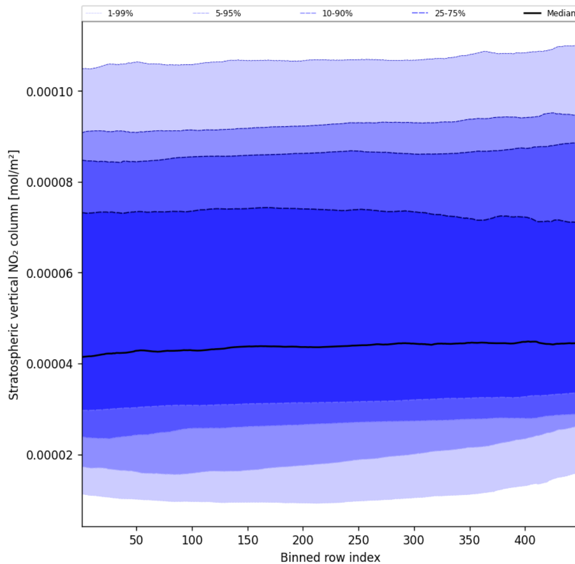
Figure 51: Along track statistics of “Stratospheric vertical NO 2 column” for 2025-01-06 to 2025-01-07
