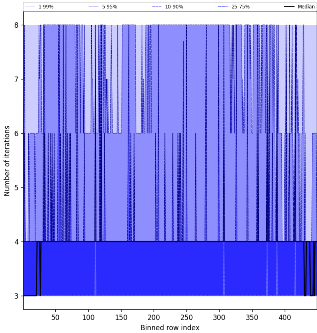
Figure 49: Along track statistics of “Number of iterations” for 2025-01-06 to 2025-01-07
