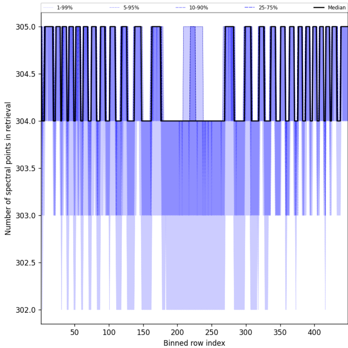
Figure 48: Along track statistics of “Number of spectral points in retrieval” for 2025-01-06 to 2025-01-07
