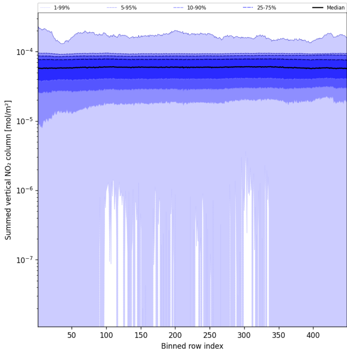
Figure 55: Along track statistics of “Summed vertical NO 2 column” for 2025-01-06 to 2025-01-07
