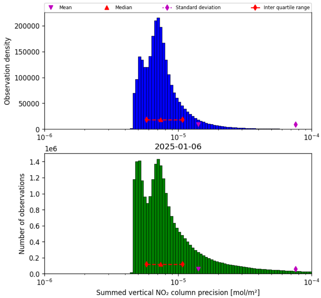
Figure 39: Histogram of "Summed vertical NO 2 column precision" for 2025-01-06 to 2025-01-07
