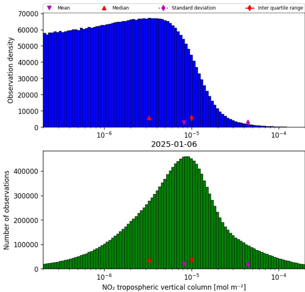
Figure 27: Histogram of “NO 2 tropospheric vertical column” for 2025-01-06 to 2025-01-07
