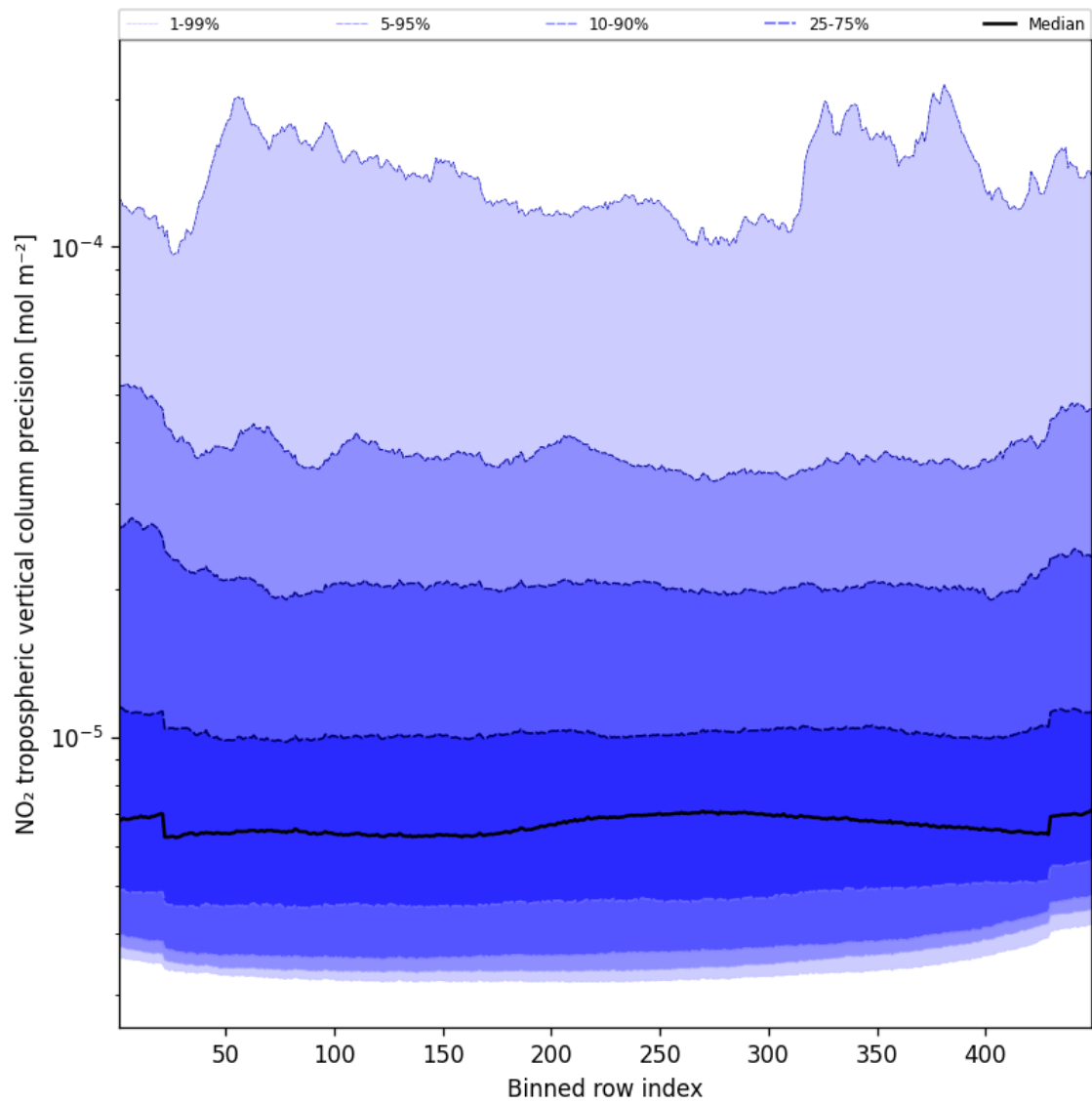
Figure 45: Along track statistics of “NO 2 tropospheric vertical column precision” for 2025-01-06 to 2025-01-07
