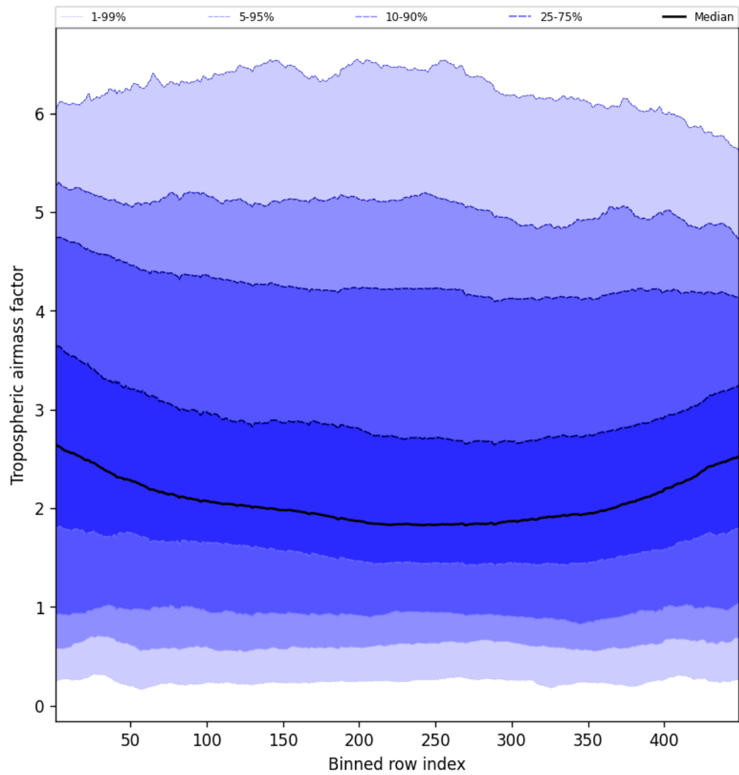
Figure 46: Along track statistics of “Tropospheric air mass factor” for 2025-01-06 to 2025-01-07
