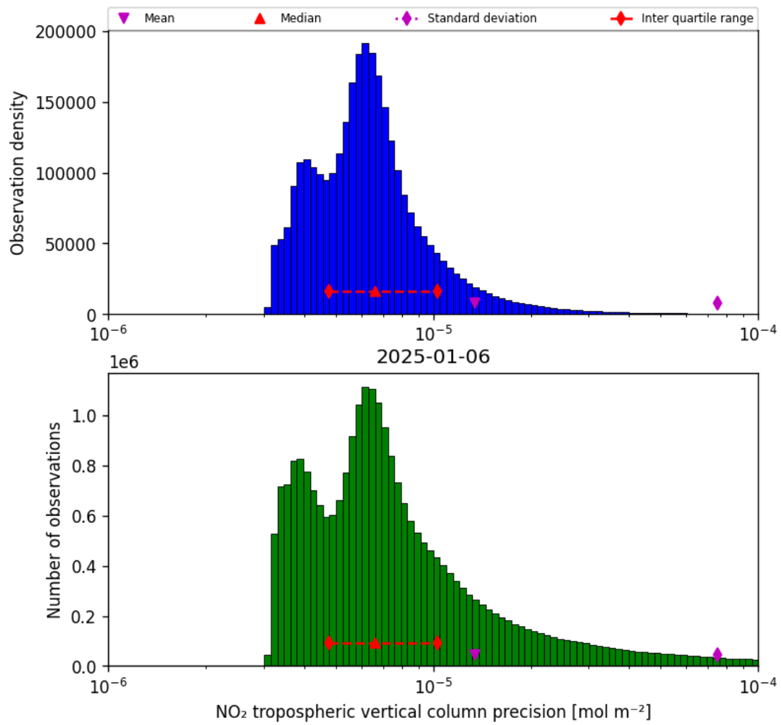
Figure 28: Histogram of “NO 2 tropospheric vertical column precision” for 2025-01-06 to 2025-01-07
