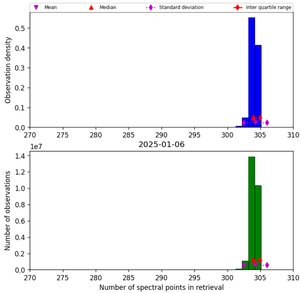
Figure 31: Histogram of “Number of spectral points in retrieval” for 2025-01-06 to 2025-01-07
