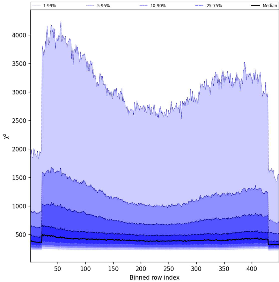
Figure 57: Along track statistics of “ \chi^2 ” for 2025-01-06 to 2025-01-07
