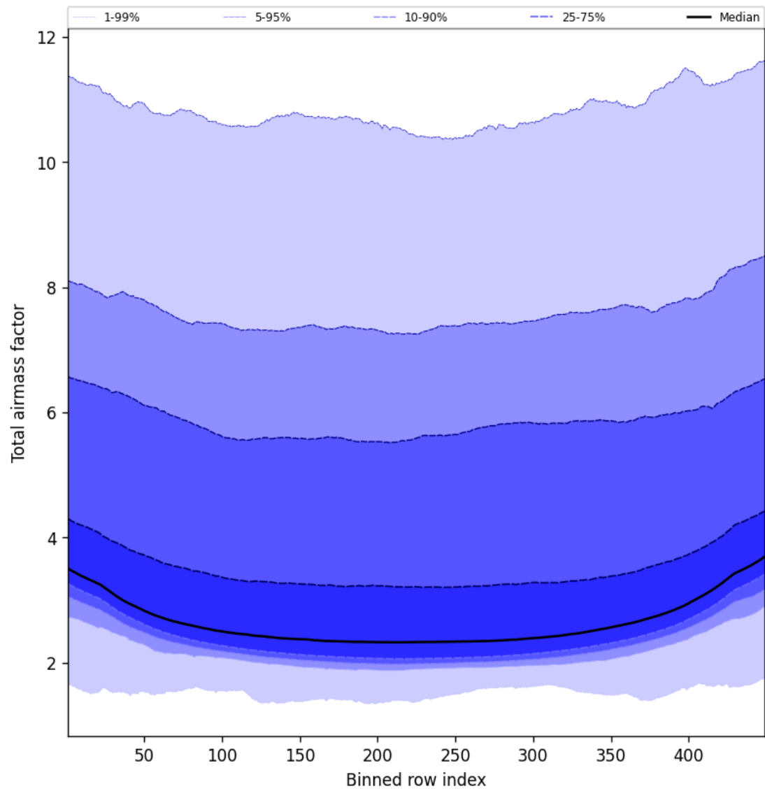
Figure 47: Along track statistics of “Total airmass factor” for 2025-01-06 to 2025-01-07
