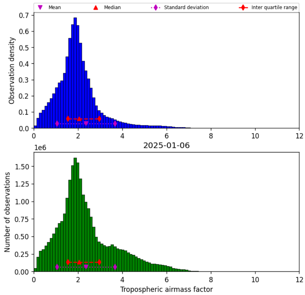
Figure 29: Histogram of “Tropospheric airmass factor” for 2025-01-06 to 2025-01-07
