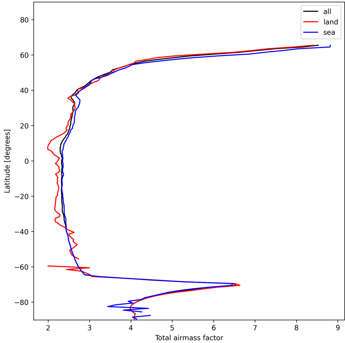
Figure 13: Zonal average of “Total airmass factor” for 2025-01-06 to 2025-01-07.
