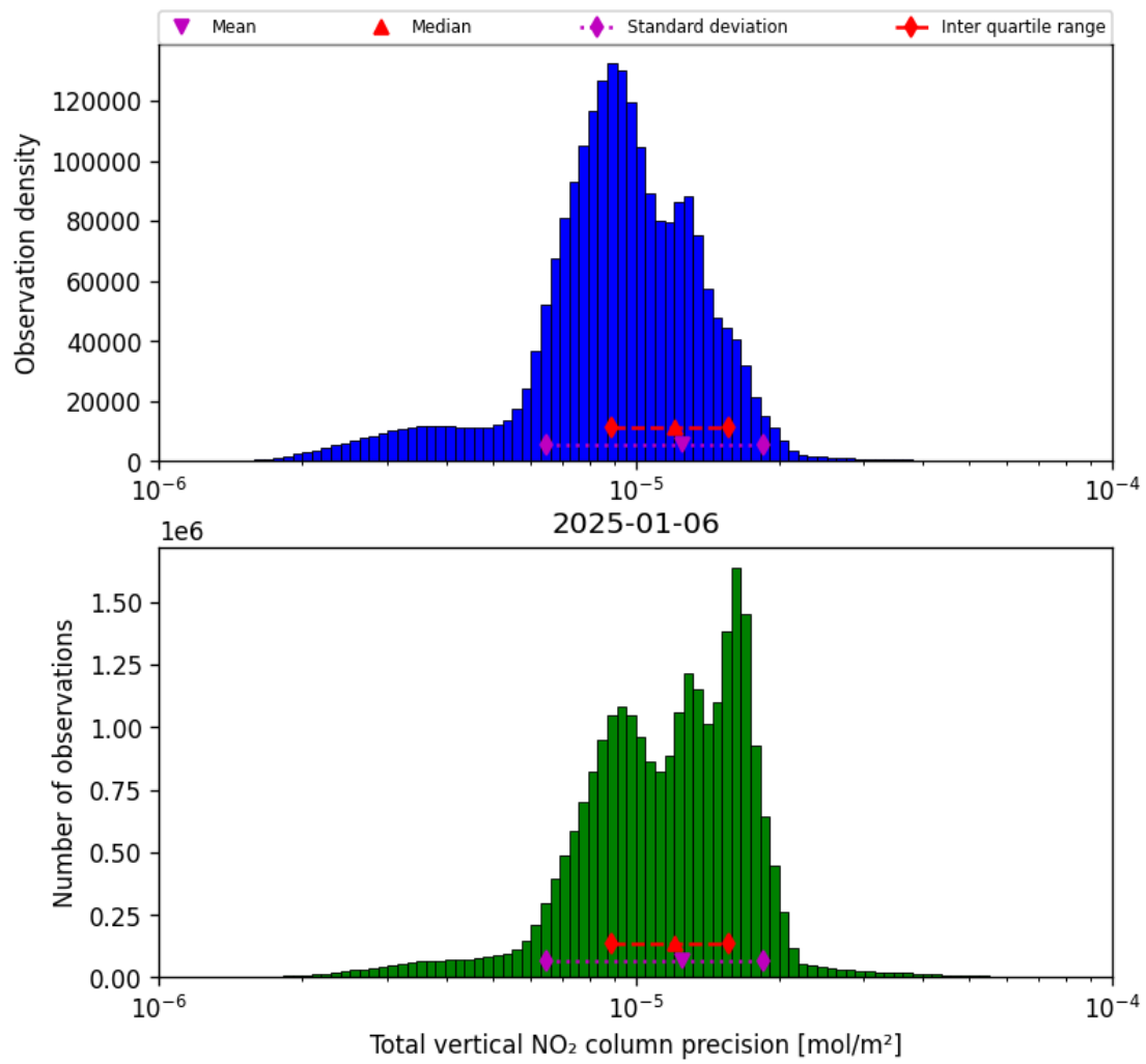
Figure 37: Histogram of “Total vertical NO 2 column precision” for 2025-01-06 to 2025-01-07
