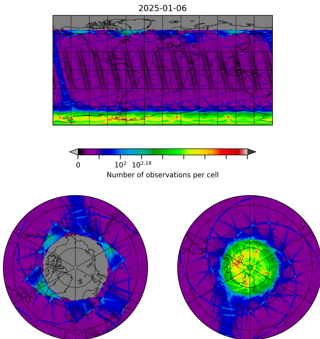
Figure 8: Map of the number of observations for 2025-01-06 to 2025-01-07
