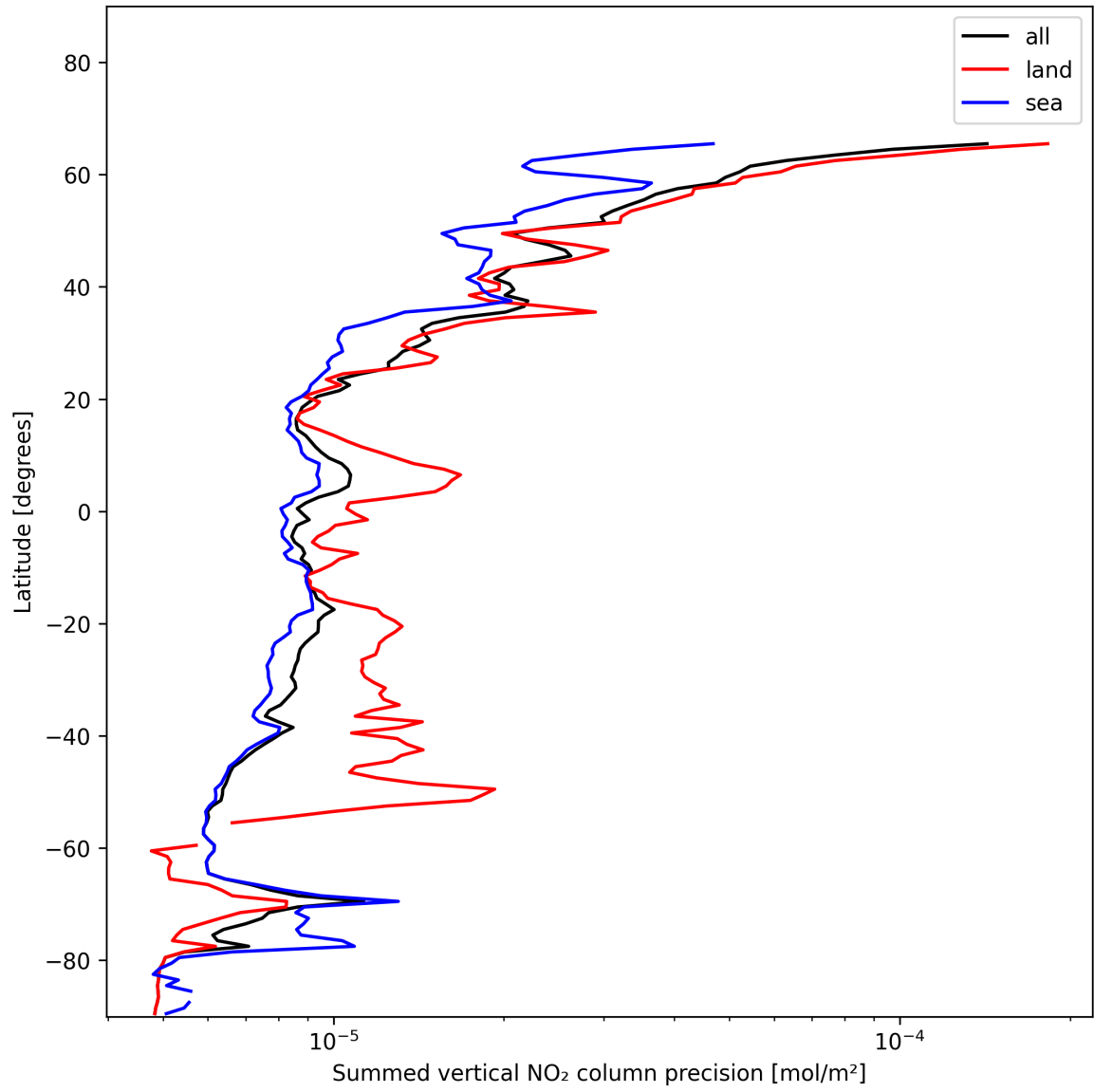
Figure 22: Zonal average of “Summed vertical NO 2 column precision” for 2025-01-06 to 2025-01-07.
