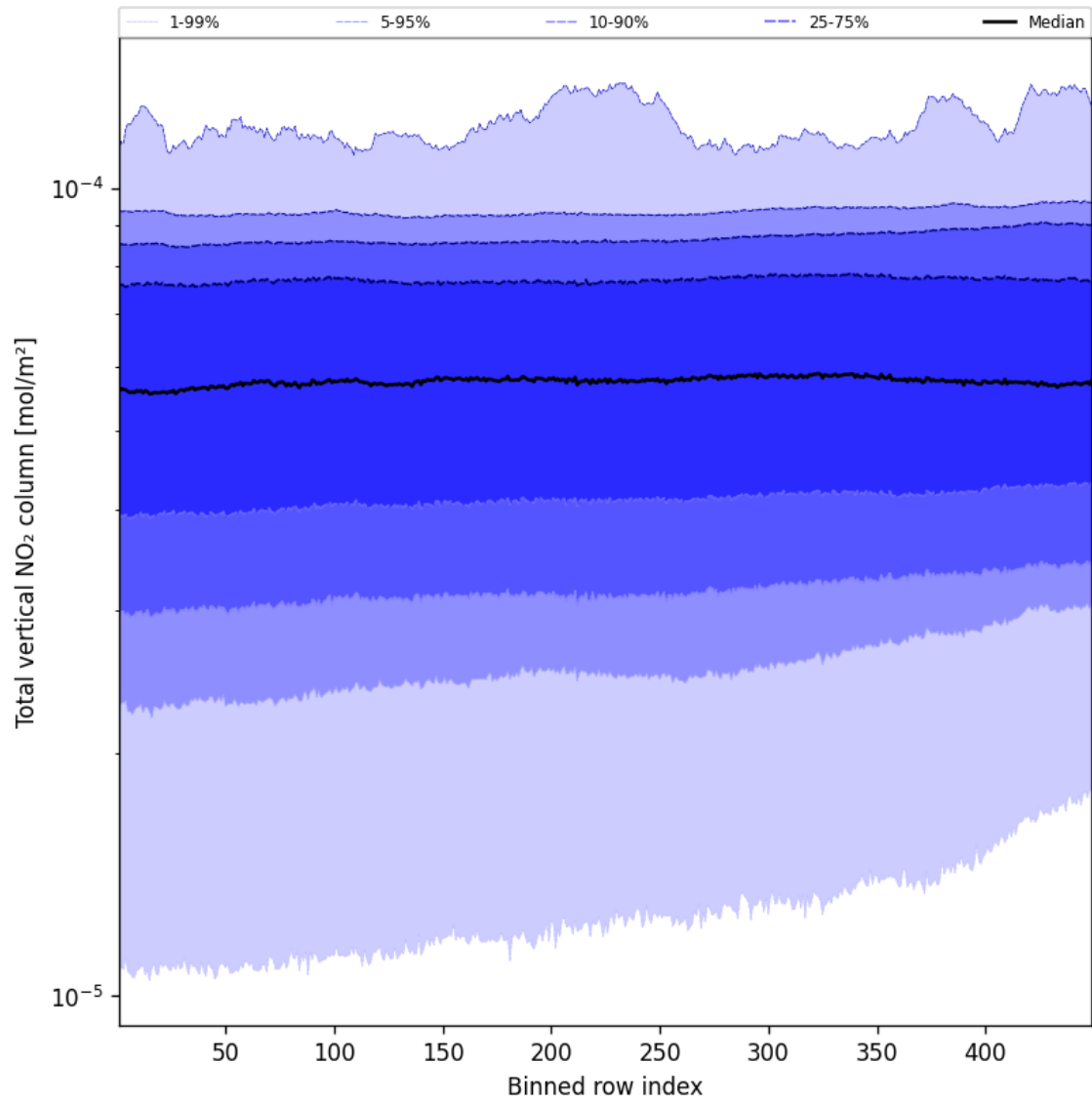
Figure 53: Along track statistics of “Total vertical NO 2 column” for 2025-01-06 to 2025-01-07
