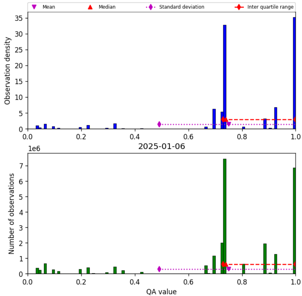
Figure 26: Histogram of “QA value” for 2025-01-06 to 2025-01-07
