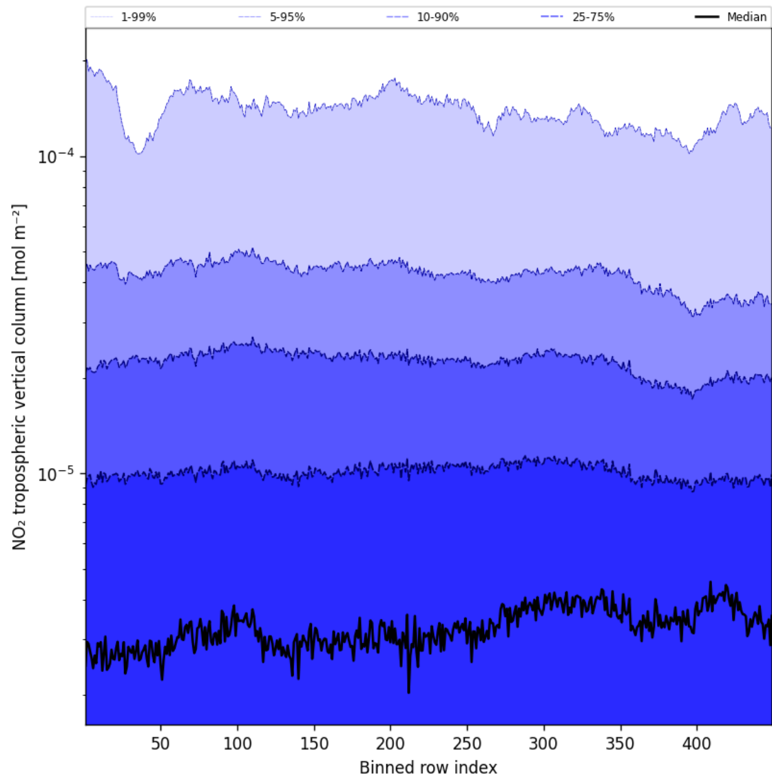
Figure 44: Along track statistics of “NO 2 tropospheric vertical column” for 2025-01-06 to 2025-01-07
