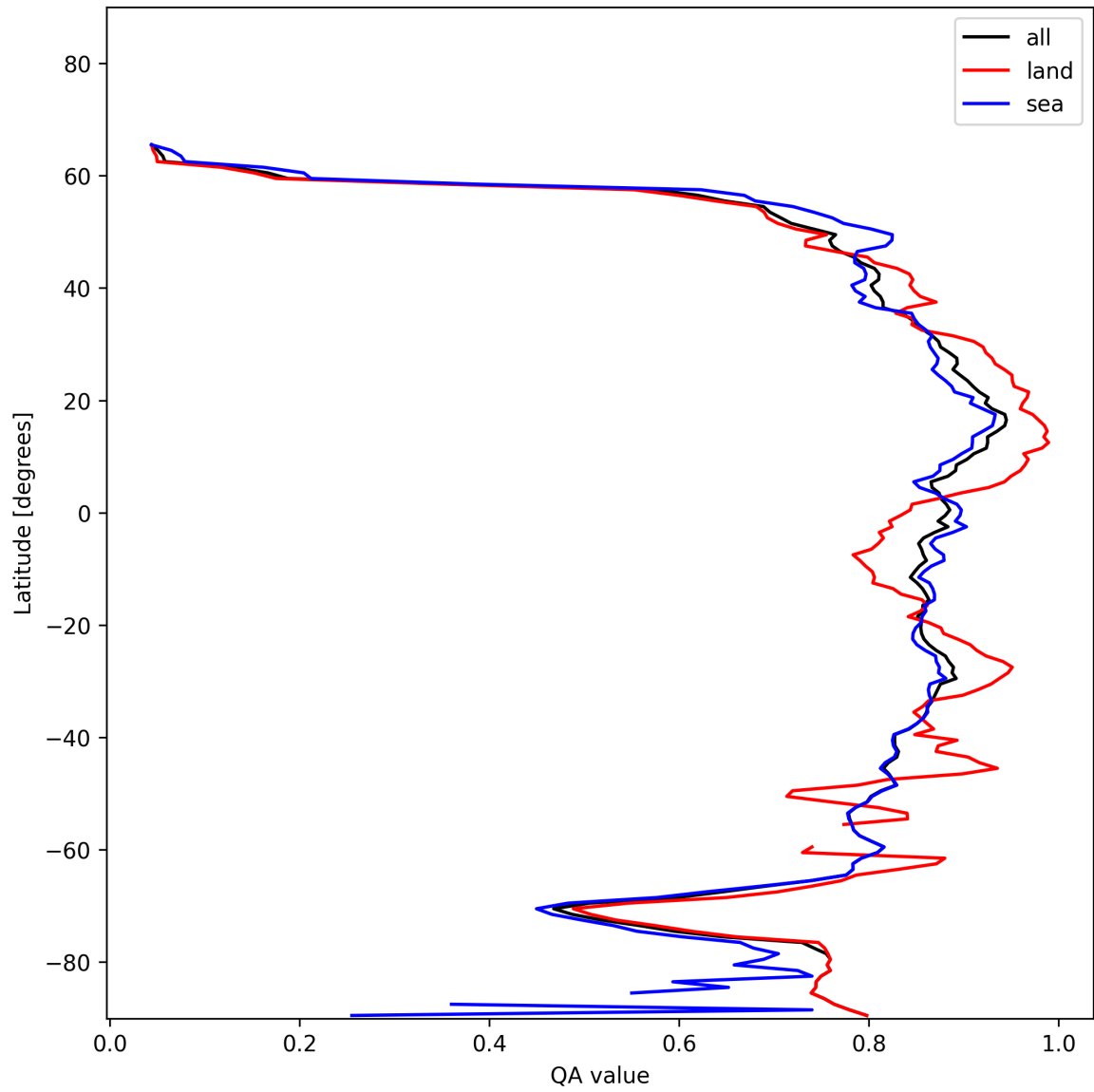
Figure 9: Zonal average of “QA value” for 2025-01-06 to 2025-01-07.
