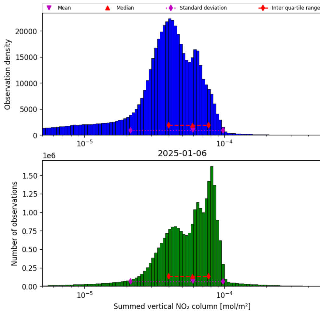
Figure 38: Histogram of “Summed vertical NO 2 column” for 2025-01-06 to 2025-01-07
