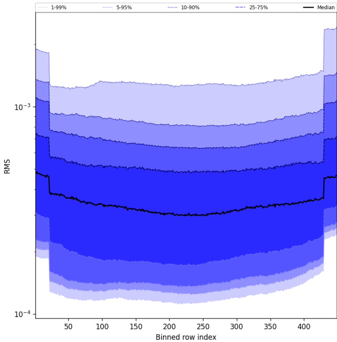
Figure 58: Along track statistics of “RMS” for 2025-01-06 to 2025-01-07
