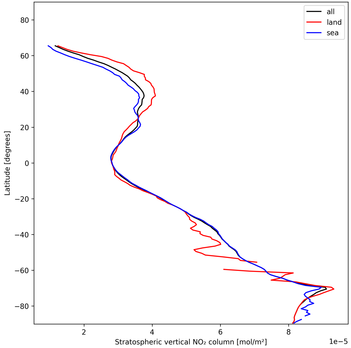
Figure 17: Zonal average of “Stratospheric vertical NO 2 column” for 2025-01-06 to 2025-01-07.
