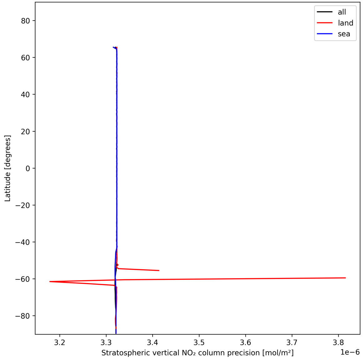
Figure 18: Zonal average of “Stratospheric vertical NO 2 column precision” for 2025-01-06 to 2025-01-07.
