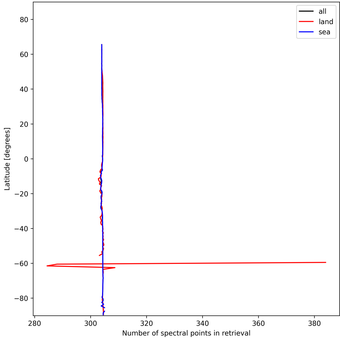
Figure 14: Zonal average of “Number of spectral points in retrieval” for 2025-01-06 to 2025-01-07.
