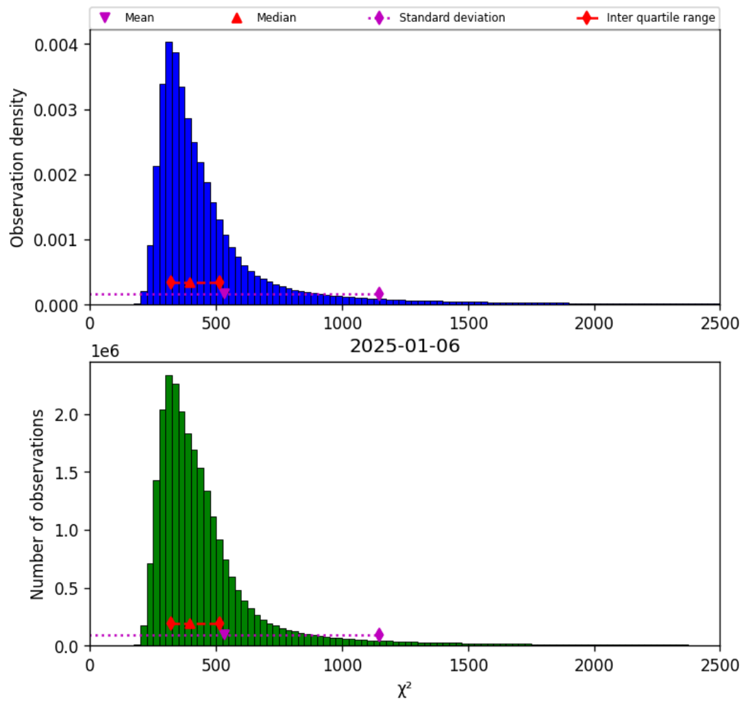
Figure 40: Histogram of “ \chi^2 ” for 2025-01-06 to 2025-01-07
