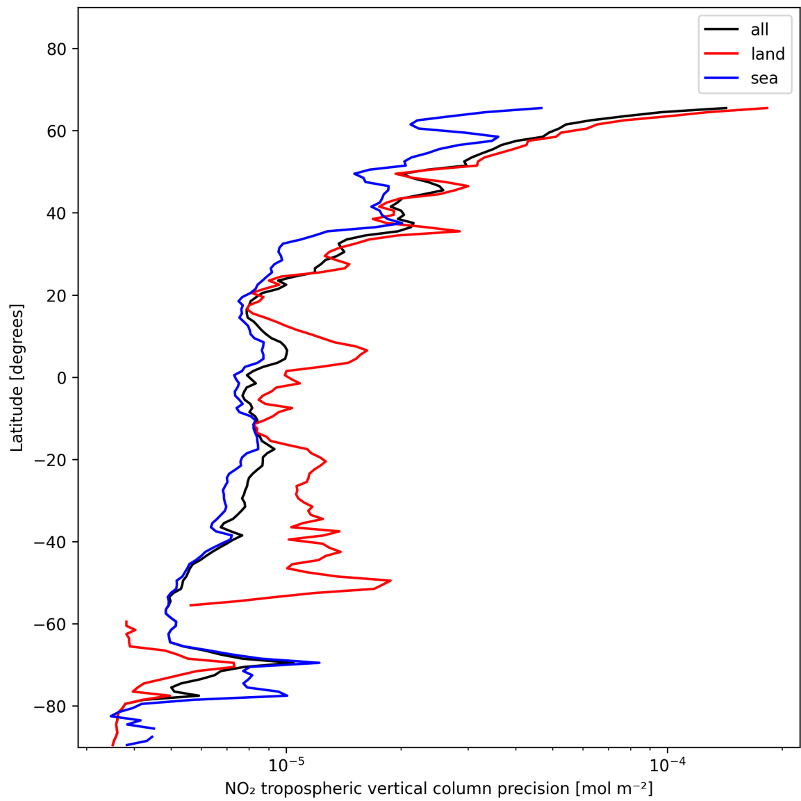
Figure 11: Zonal average of “NO 2 tropospheric vertical column precision” for 2025-01-06 to 2025-01-07.
