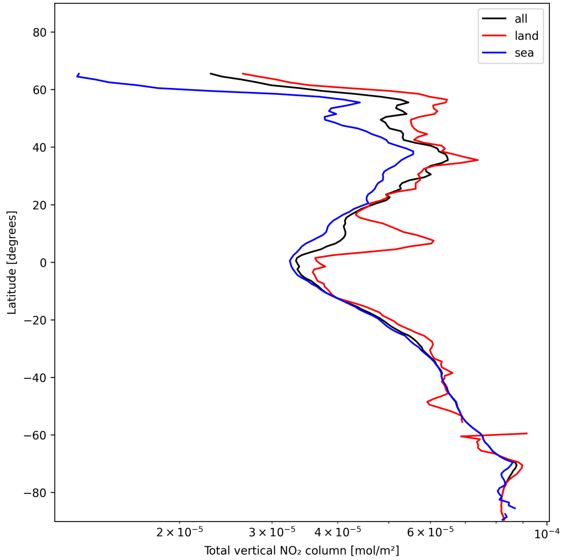
Figure 19: Zonal average of “Total vertical NO 2 column” for 2025-01-06 to 2025-01-07.
