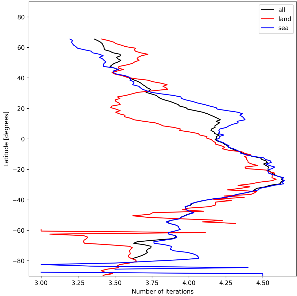
Figure 15: Zonal average of “Number of iterations” for 2025-01-06 to 2025-01-07.
