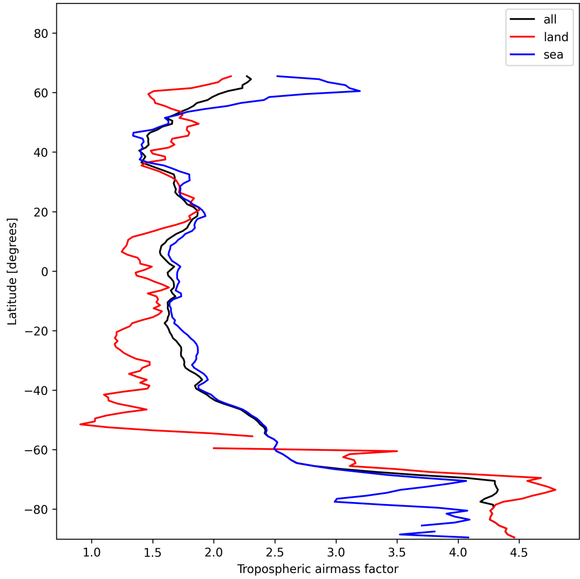
Figure 12: Zonal average of “Tropospheric airmass factor” for 2025-01-06 to 2025-01-07.
