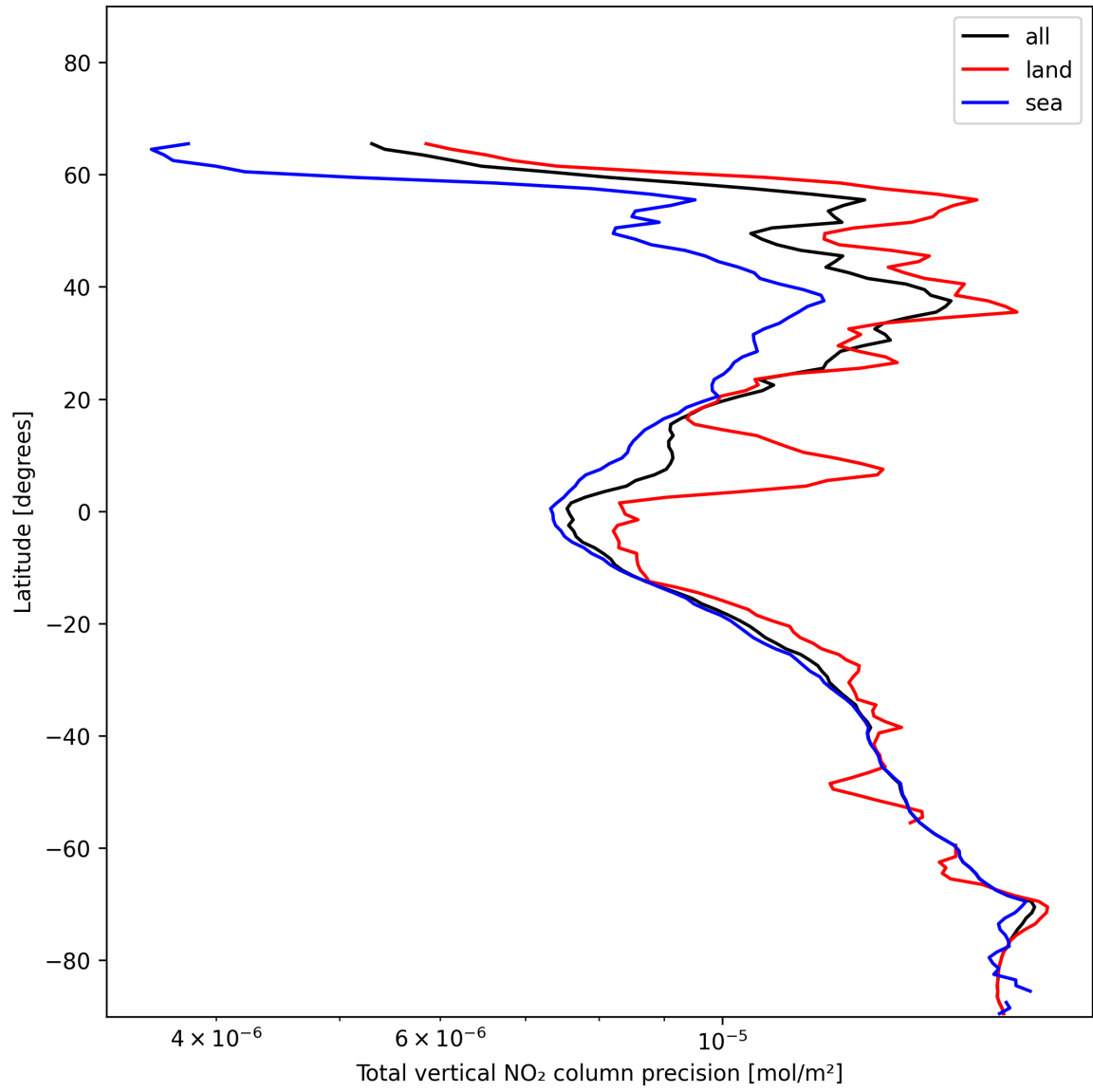
Figure 20: Zonal average of “Total vertical NO 2 column precision” for 2025-01-06 to 2025-01-07.
