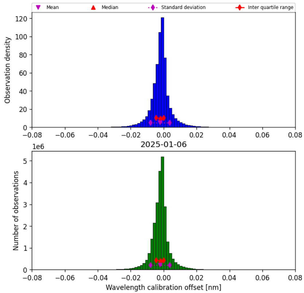
Figure 33: Histogram of “Wavelength calibration offset” for 2025-01-06 to 2025-01-07
