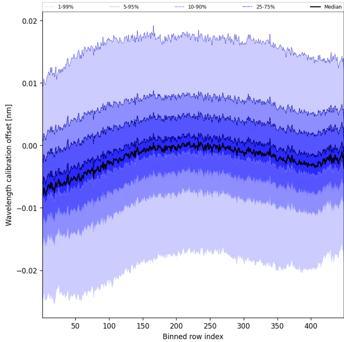
Figure 50: Along track statistics of “Wavelength calibration offset” for 2025-01-06 to 2025-01-07
