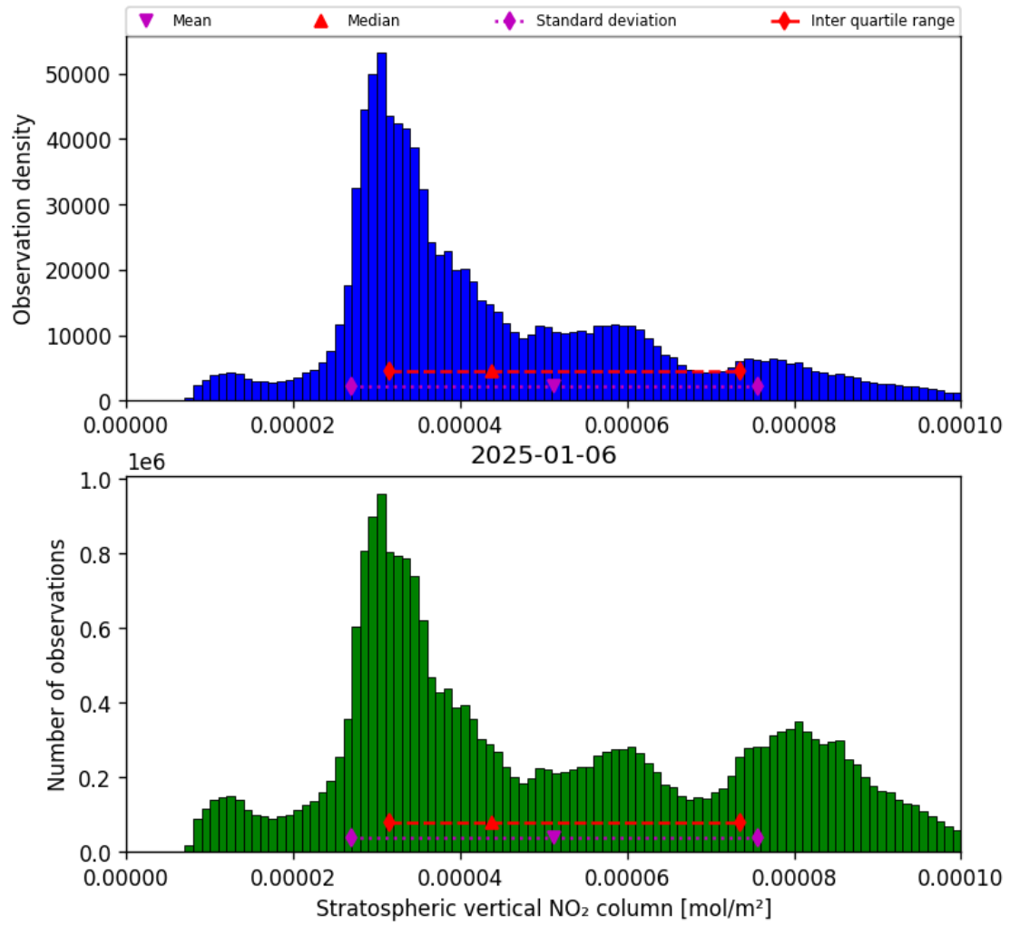
Figure 34: Histogram of “Stratospheric vertical NO 2 column” for 2025-01-06 to 2025-01-07
