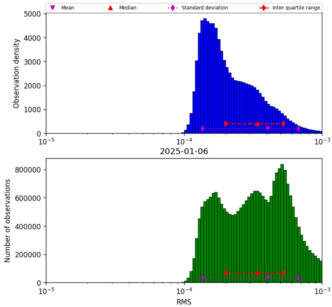
Figure 41: Histogram of “RMS” for 2025-01-06 to 2025-01-07
