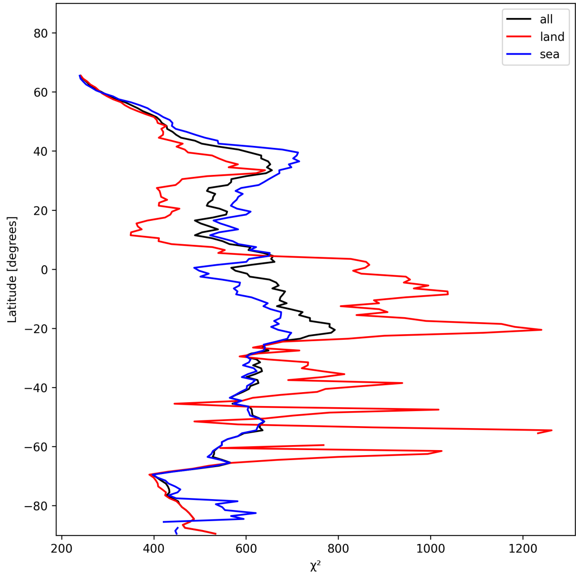
Figure 23: Zonal average of “ \chi^2 ” for 2025-01-06 to 2025-01-07.
