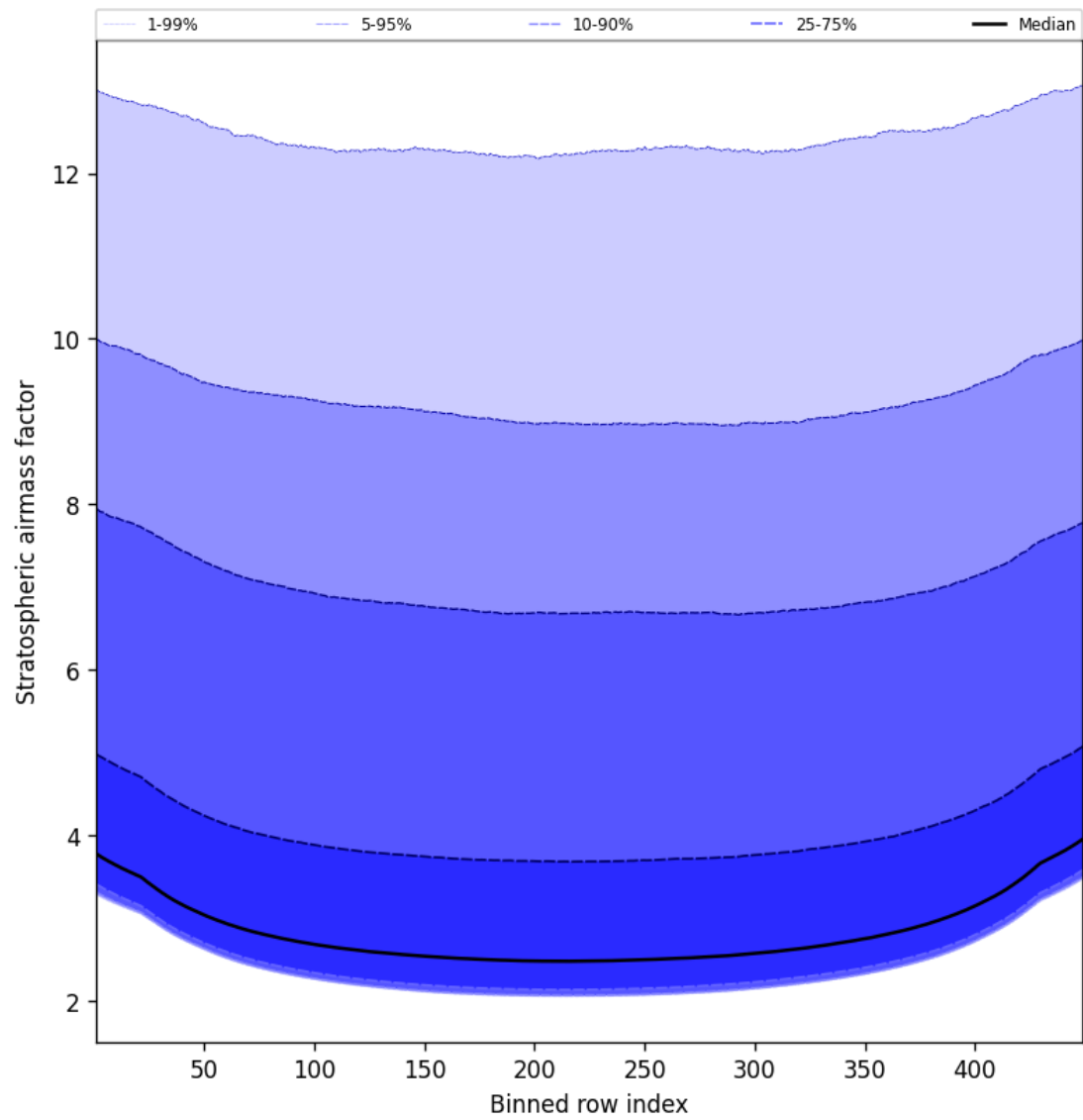
Figure 59: Along track statistics of “Stratospheric airmass factor” for 2025-01-06 to 2025-01-07
