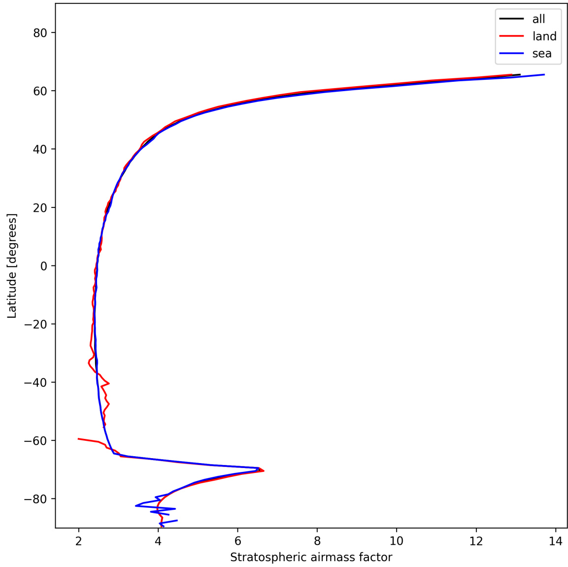
Figure 25: Zonal average of “Stratospheric air mass factor” for 2025-01-06 to 2025-01-07.
