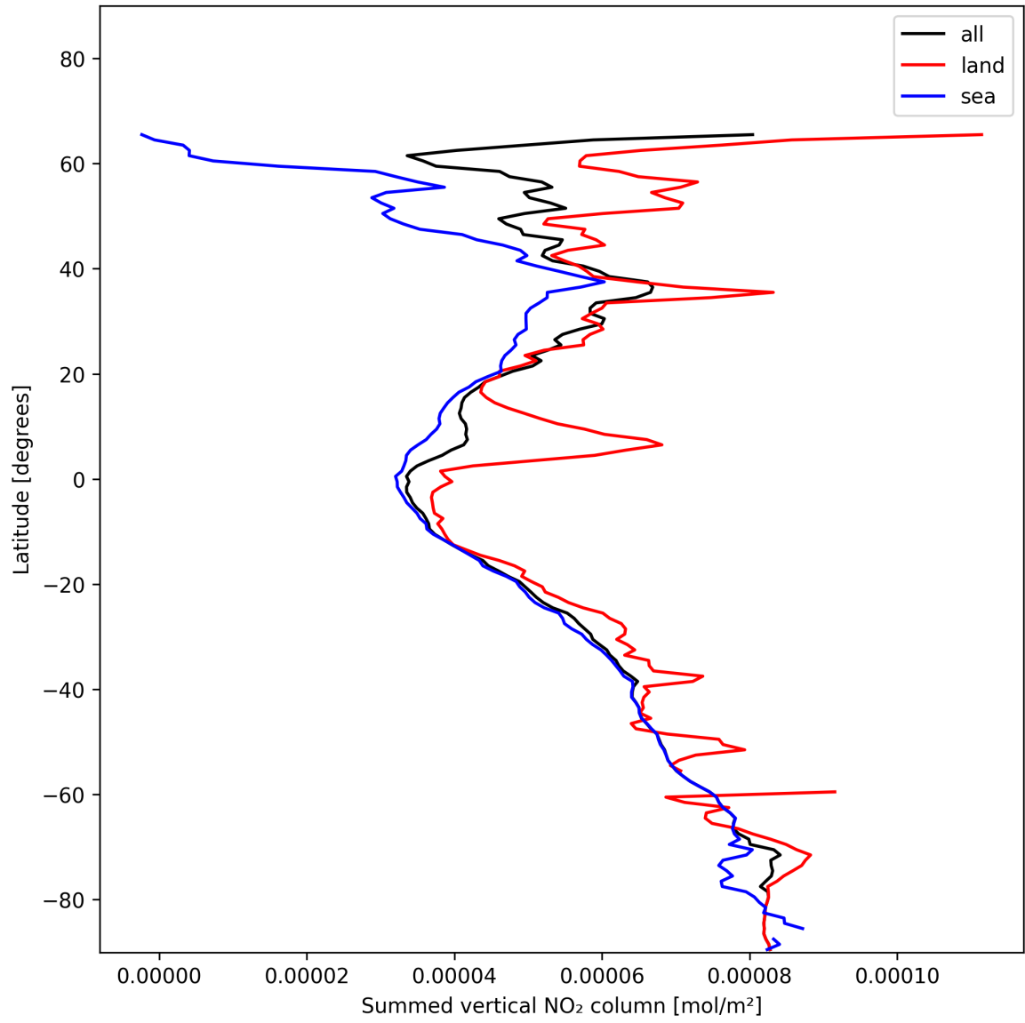
Figure 21: Zonal average of “Summed vertical NO 2 column” for 2025-01-06 to 2025-01-07.
