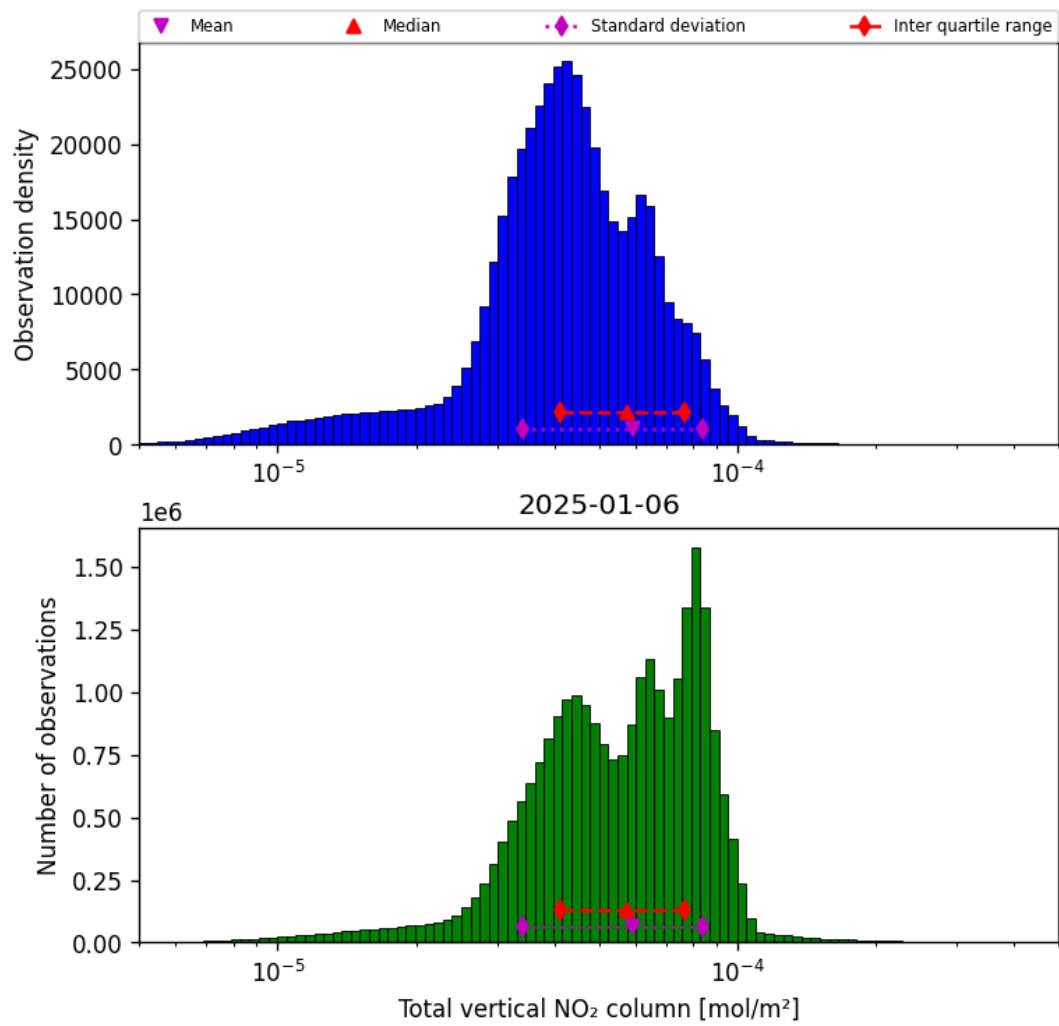
Figure 36: Histogram of “Total vertical NO 2 column” for 2025-01-06 to 2025-01-07
