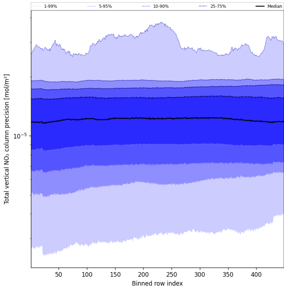
Figure 54: Along track statistics of “Total vertical NO 2 column precision” for 2025-01-06 to 2025-01-07
