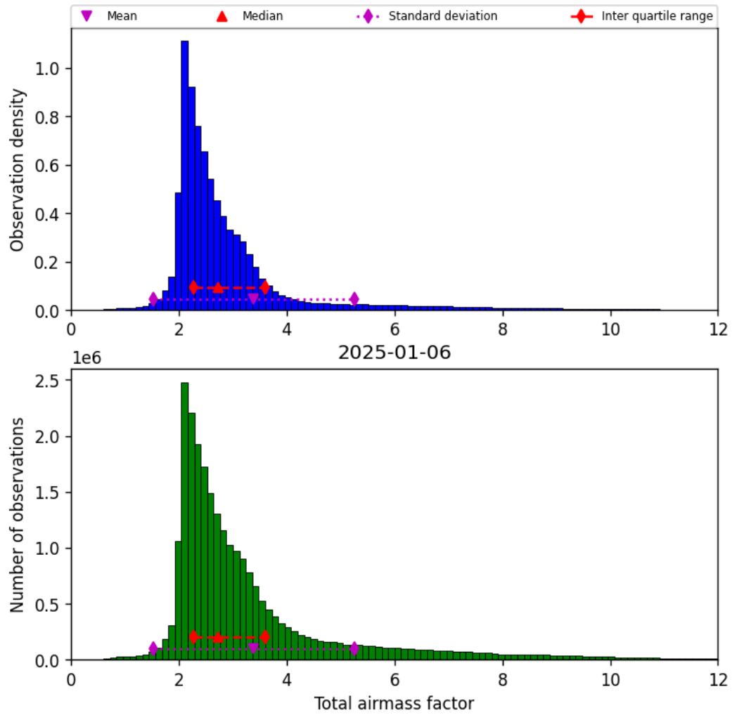
Figure 30: Histogram of “Total airmass factor” for 2025-01-06 to 2025-01-07
