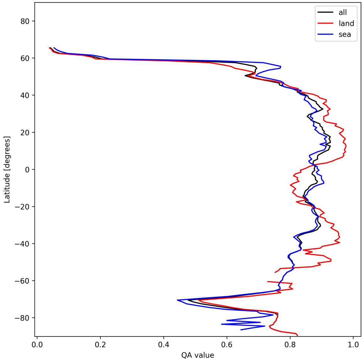
Figure 9: Zonal average of “QA value” for 2025-01-08 to 2025-01-09.
