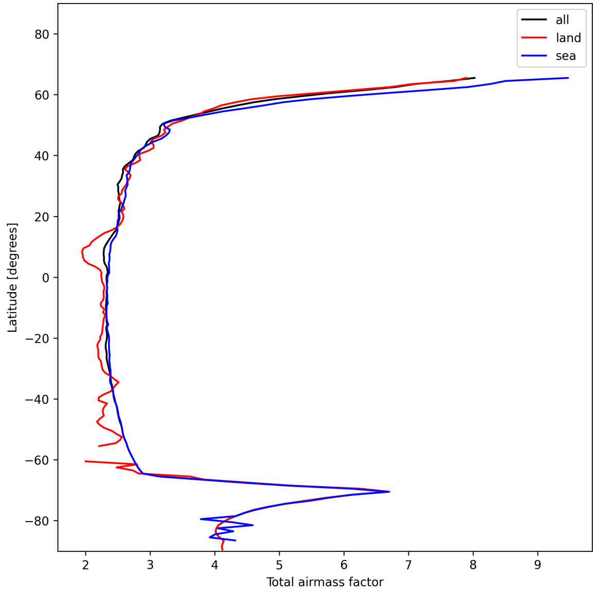
Figure 13: Zonal average of “Total airmass factor” for 2025-01-08 to 2025-01-09.
