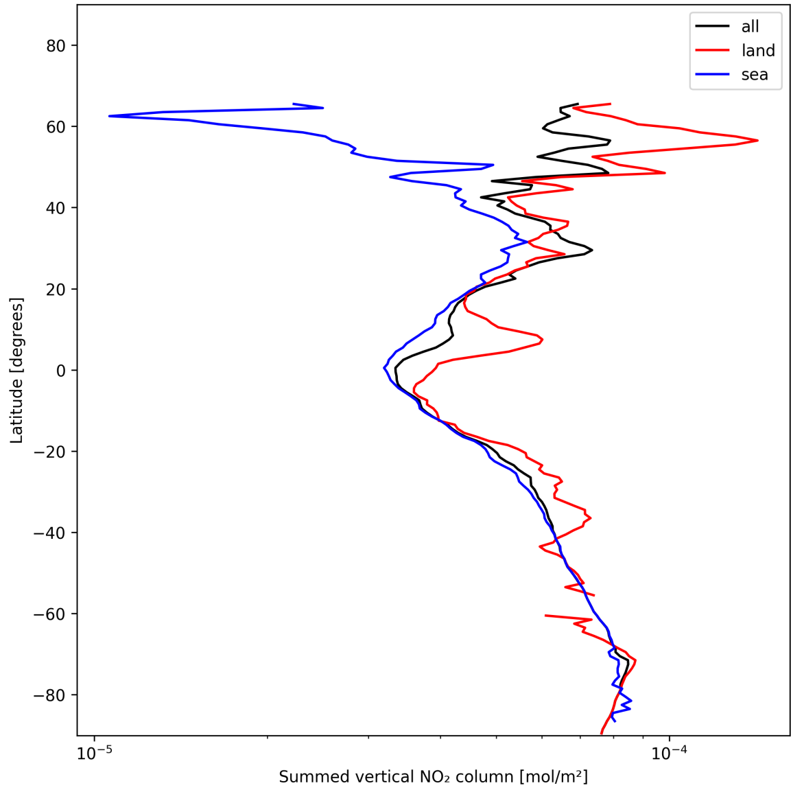
Figure 21: Zonal average of “Summed vertical NO 2 column” for 2025-01-08 to 2025-01-09.
