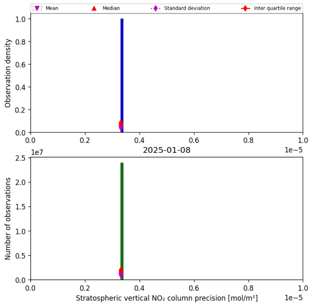
Figure 35: Histogram of “Stratospheric vertical NO 2 column precision” for 2025-01-08 to 2025-01-09
