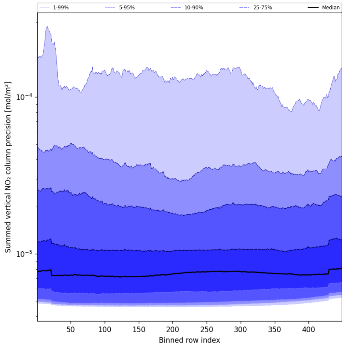
Figure 56: Along track statistics of “Summed vertical NO 2 column precision” for 2025-01-08 to 2025-01-09
