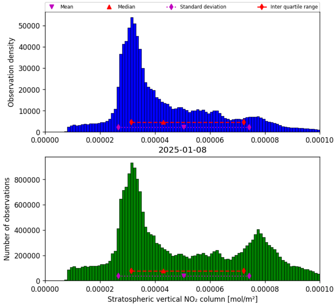
Figure 34: Histogram of “Stratospheric vertical NO 2 column” for 2025-01-08 to 2025-01-09
