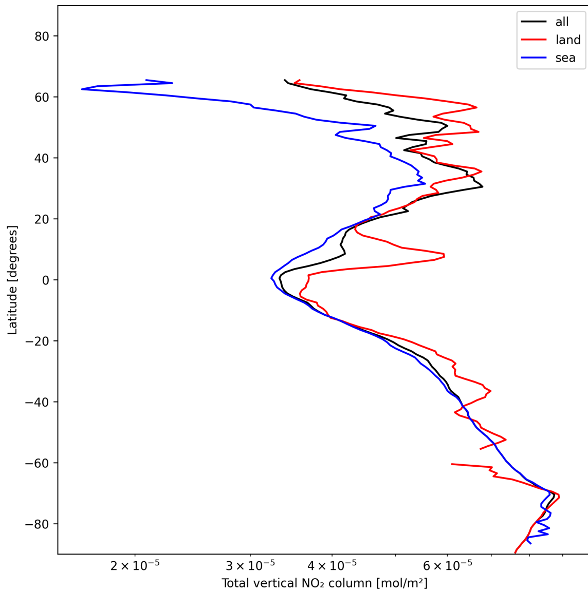
Figure 19: Zonal average of “Total vertical NO 2 column” for 2025-01-08 to 2025-01-09.
