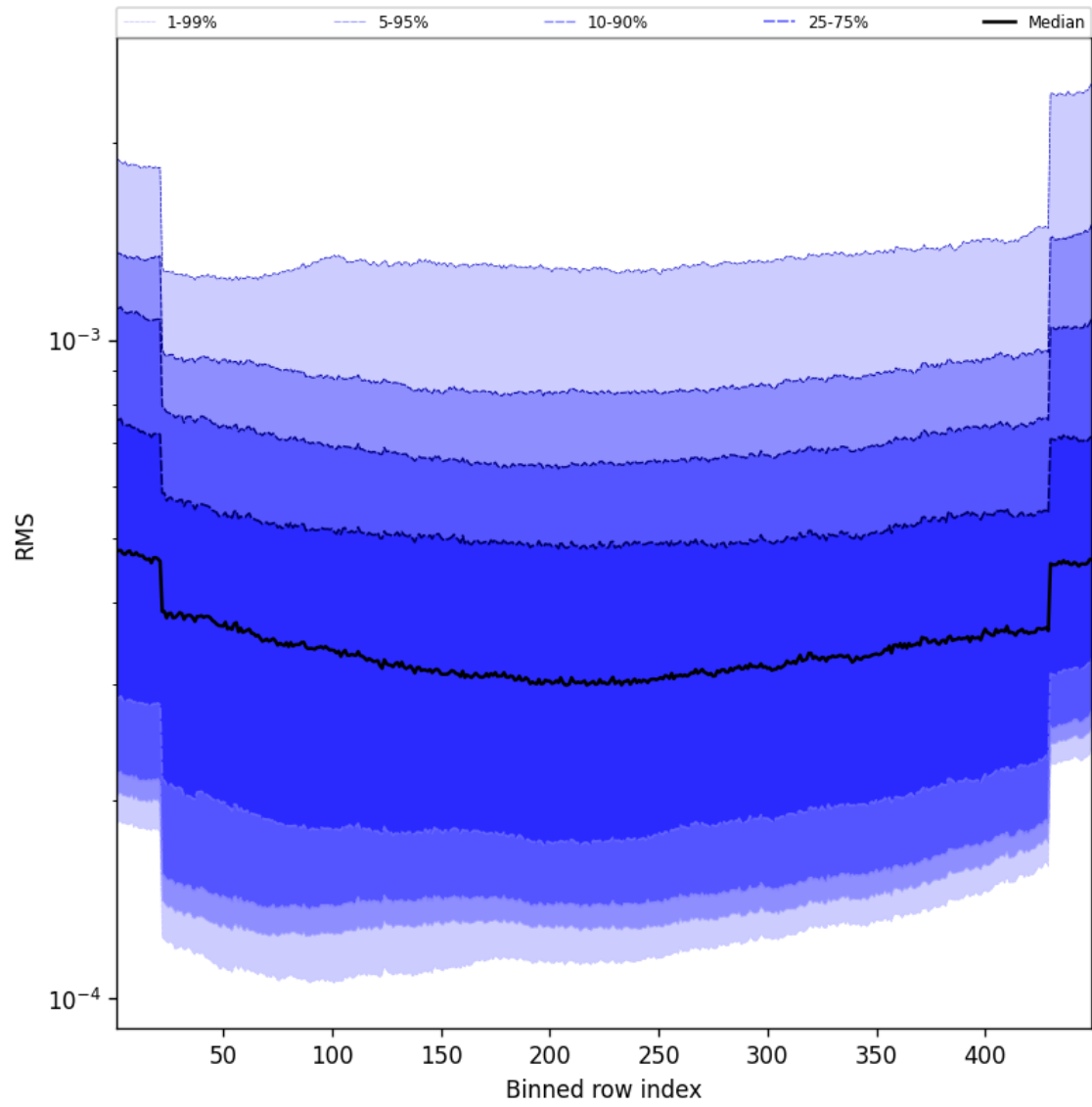
Figure 58: Along track statistics of “RMS” for 2025-01-08 to 2025-01-09
