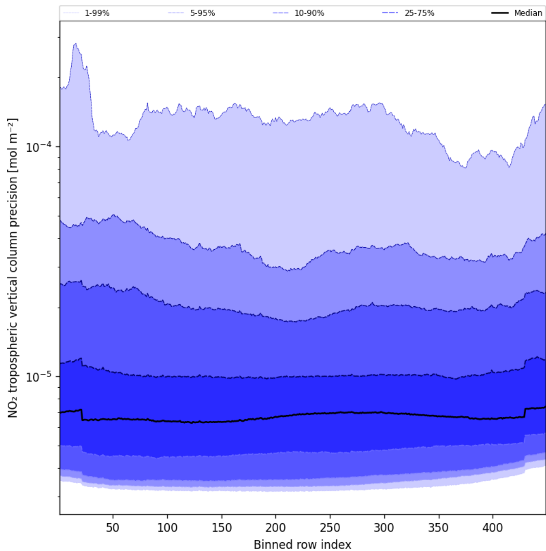
Figure 45: Along track statistics of “NO 2 tropospheric vertical column precision” for 2025-01-08 to 2025-01-09
