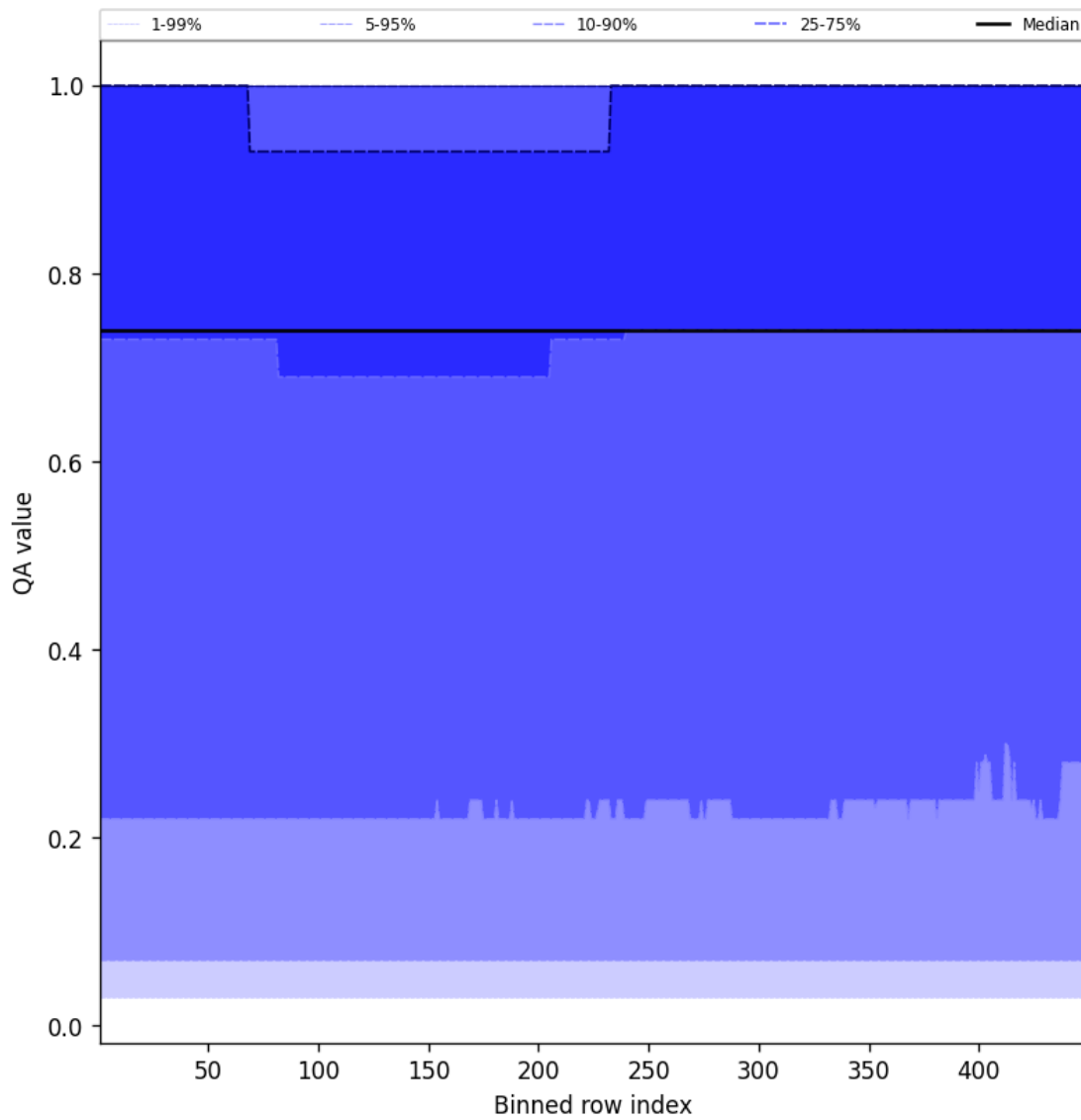
Figure 43: Along track statistics of “QA value” for 2025-01-08 to 2025-01-09
