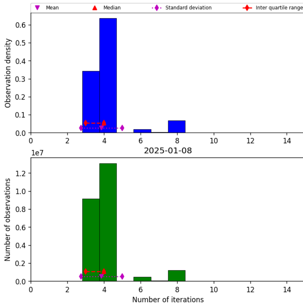
Figure 32: Histogram of “Number of iterations” for 2025-01-08 to 2025-01-09
