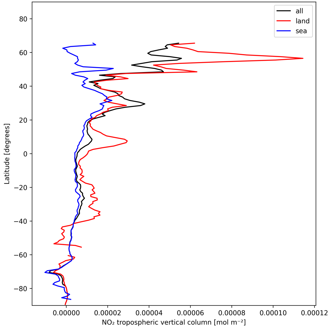
Figure 10: Zonal average of “NO 2 tropospheric vertical column” for 2025-01-08 to 2025-01-09.
