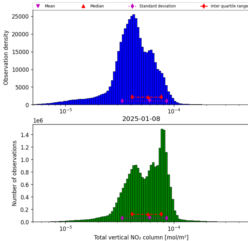
Figure 36: Histogram of “Total vertical NO 2 column” for 2025-01-08 to 2025-01-09
