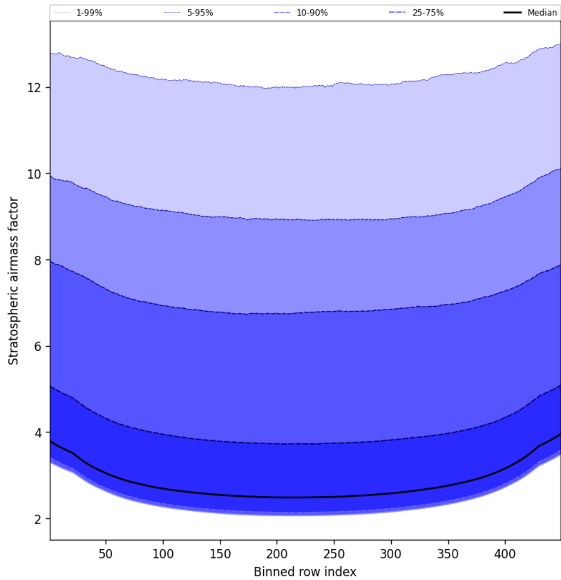
Figure 59: Along track statistics of “Stratospheric airmass factor” for 2025-01-08 to 2025-01-09
