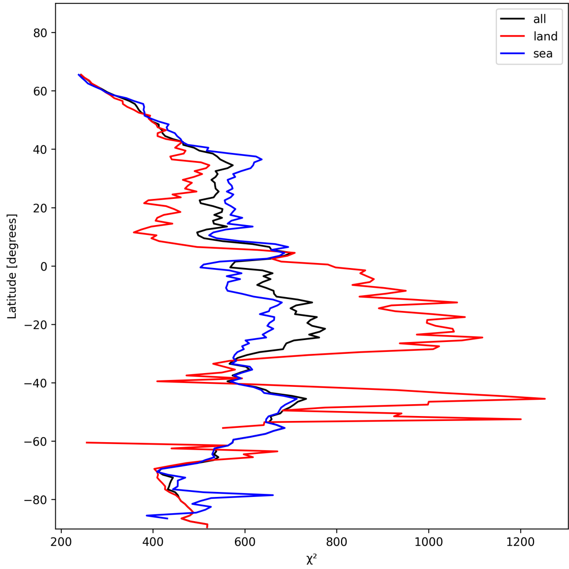
Figure 23: Zonal average of “ \chi^2 ” for 2025-01-08 to 2025-01-09.
