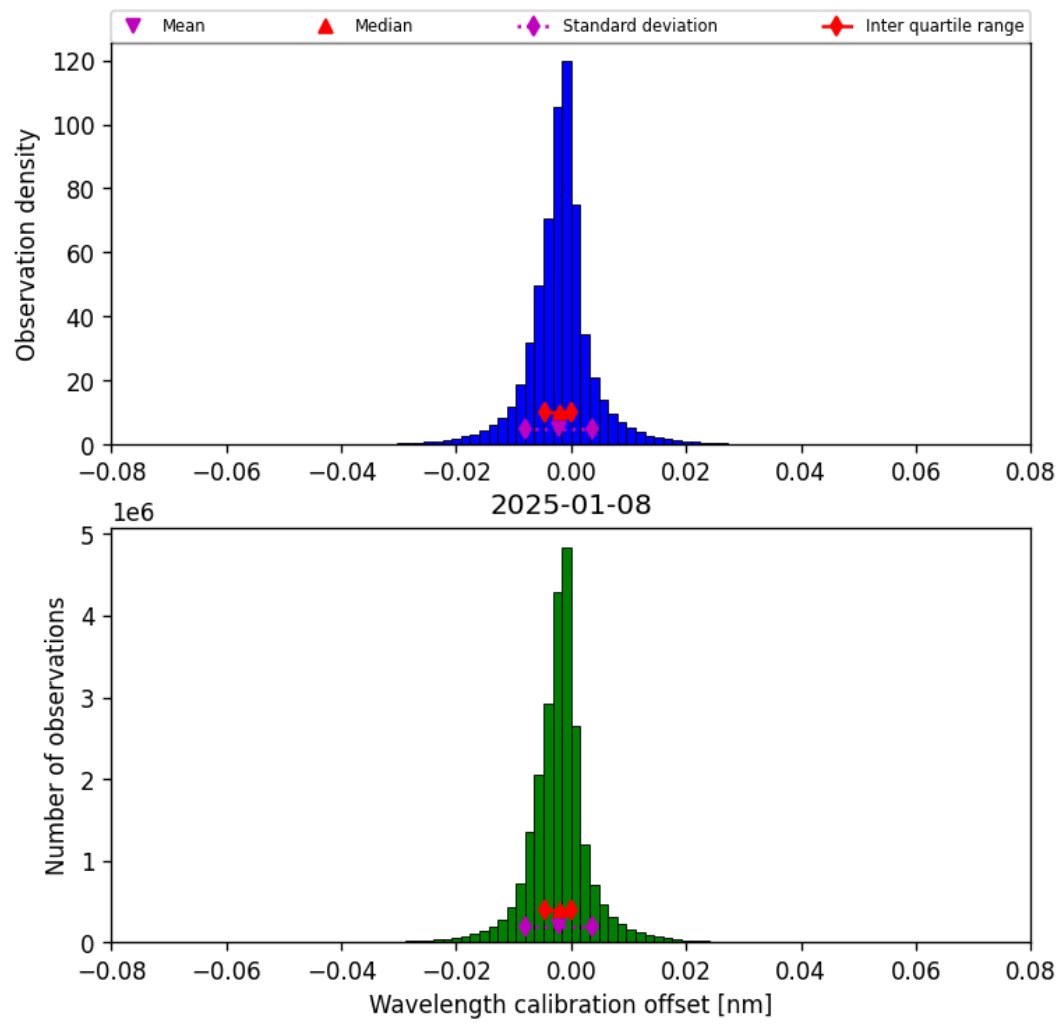
Figure 33: Histogram of “Wavelength calibration offset” for 2025-01-08 to 2025-01-09
