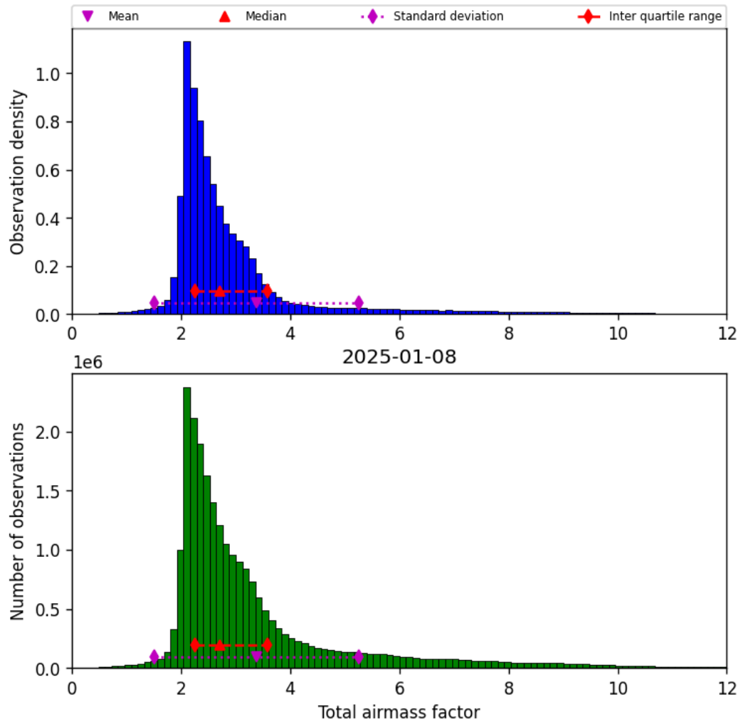
Figure 30: Histogram of “Total airmass factor” for 2025-01-08 to 2025-01-09
