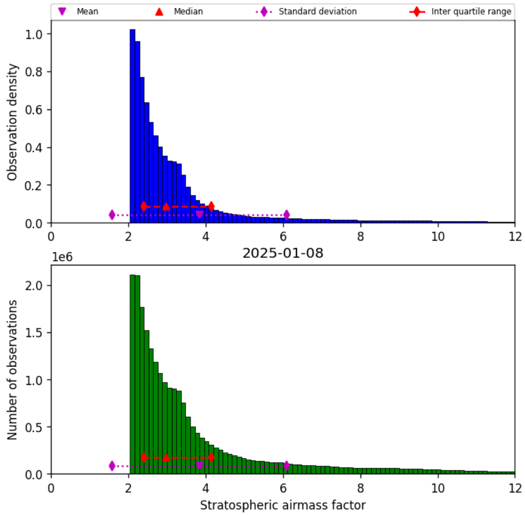
Figure 42: Histogram of “Stratospheric airmass factor” for 2025-01-08 to 2025-01-09
