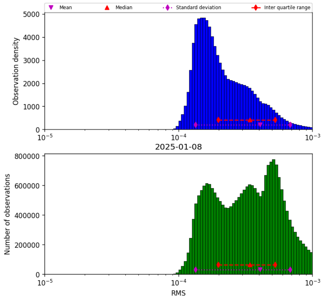
Figure 41: Histogram of “RMS” for 2025-01-08 to 2025-01-09
