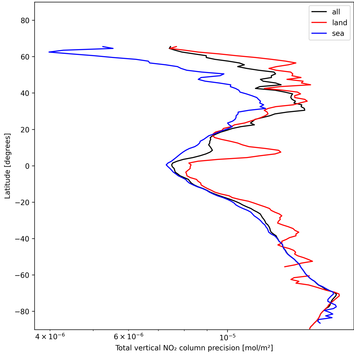
Figure 20: Zonal average of “Total vertical NO 2 column precision” for 2025-01-08 to 2025-01-09.
