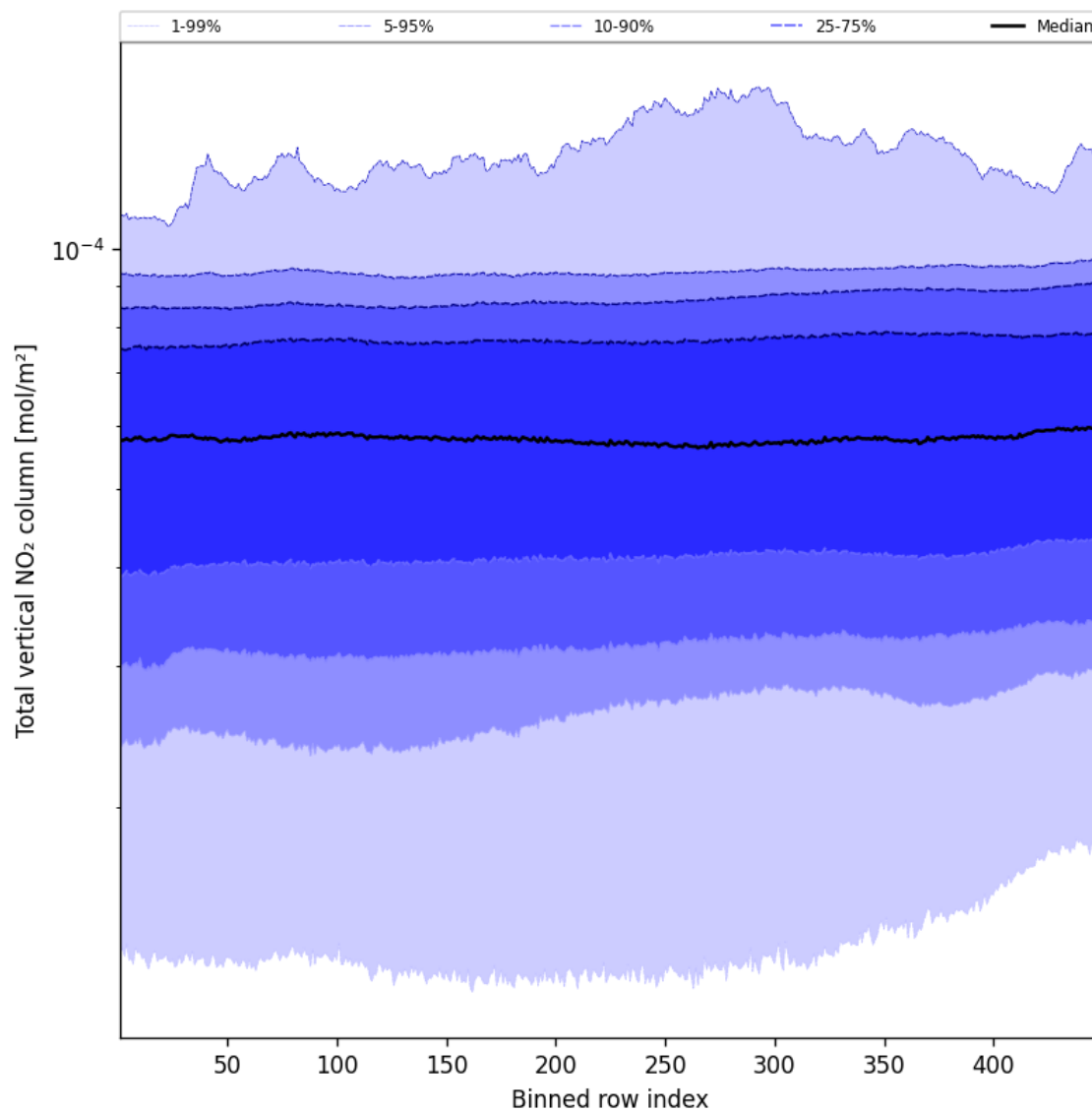
Figure 53: Along track statistics of “Total vertical NO 2 column” for 2025-01-08 to 2025-01-09
