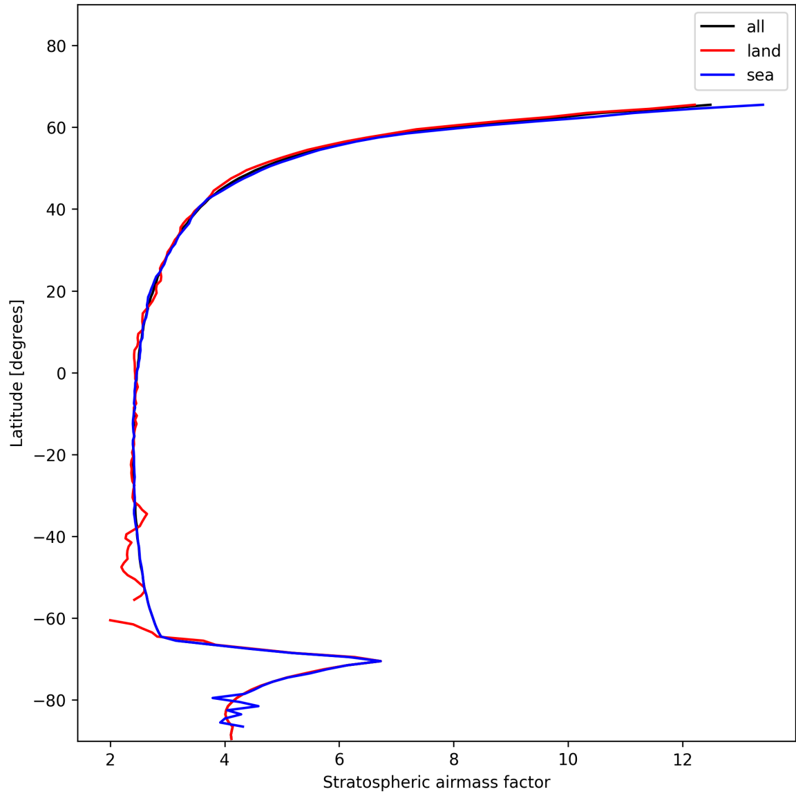
Figure 25: Zonal average of “Stratospheric air mass factor” for 2025-01-08 to 2025-01-09.
