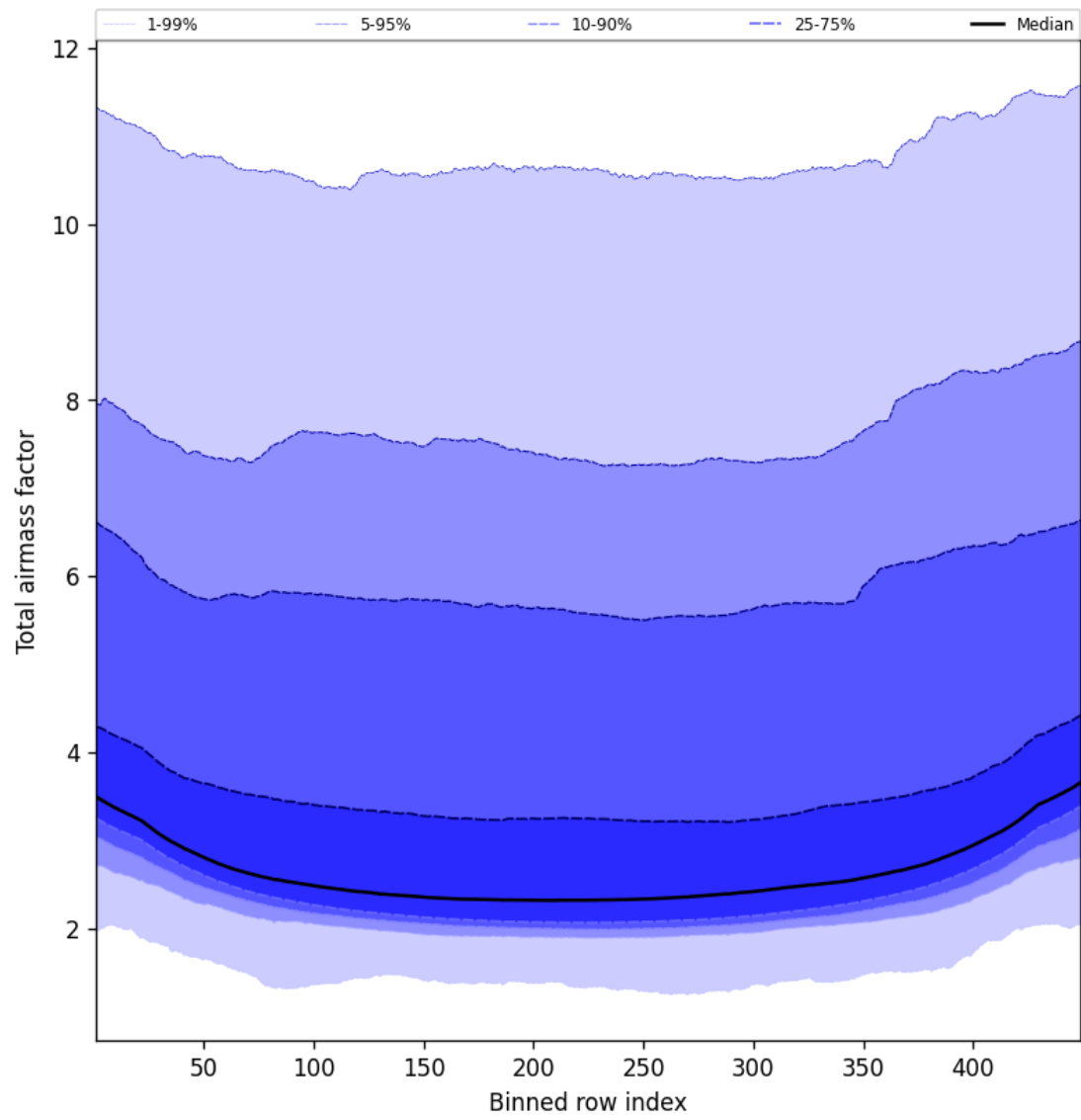
Figure 47: Along track statistics of “Total airmass factor” for 2025-01-08 to 2025-01-09
