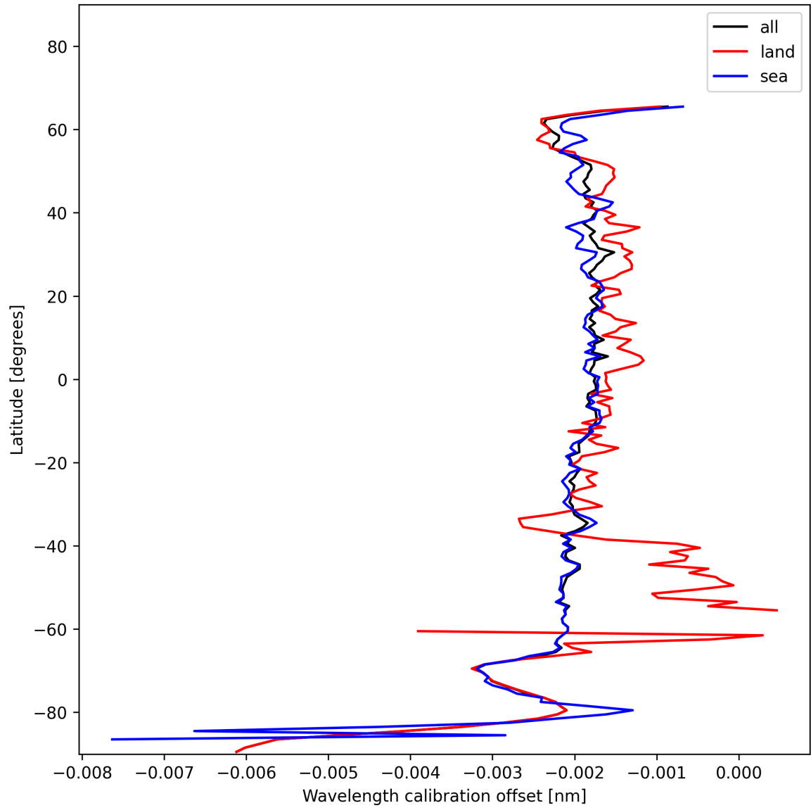
Figure 16: Zonal average of “Wavelength calibration offset” for 2025-01-08 to 2025-01-09.
