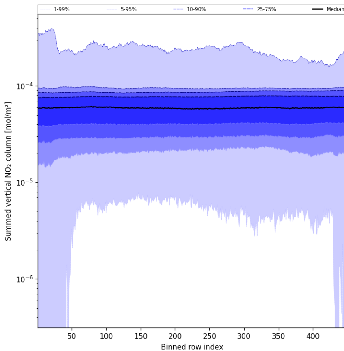
Figure 55: Along track statistics of “Summed vertical NO 2 column” for 2025-01-08 to 2025-01-09
