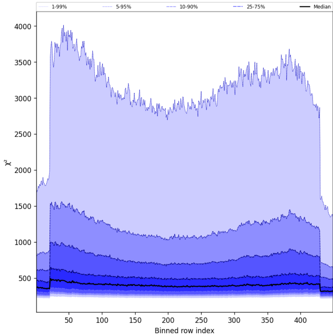
Figure 57: Along track statistics of “ \chi^2 ” for 2025-01-08 to 2025-01-09
