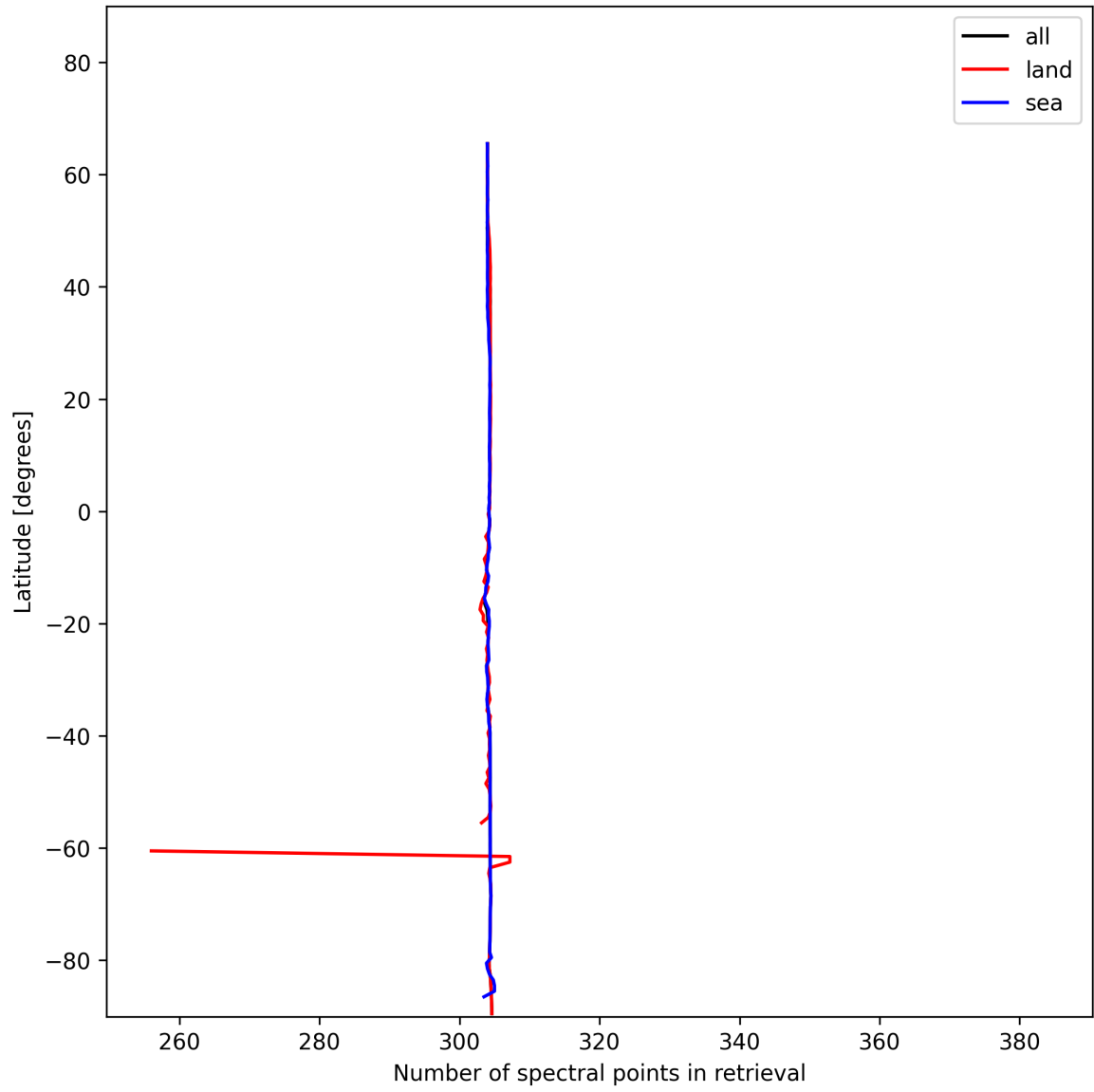
Figure 14: Zonal average of “Number of spectral points in retrieval” for 2025-01-08 to 2025-01-09.
