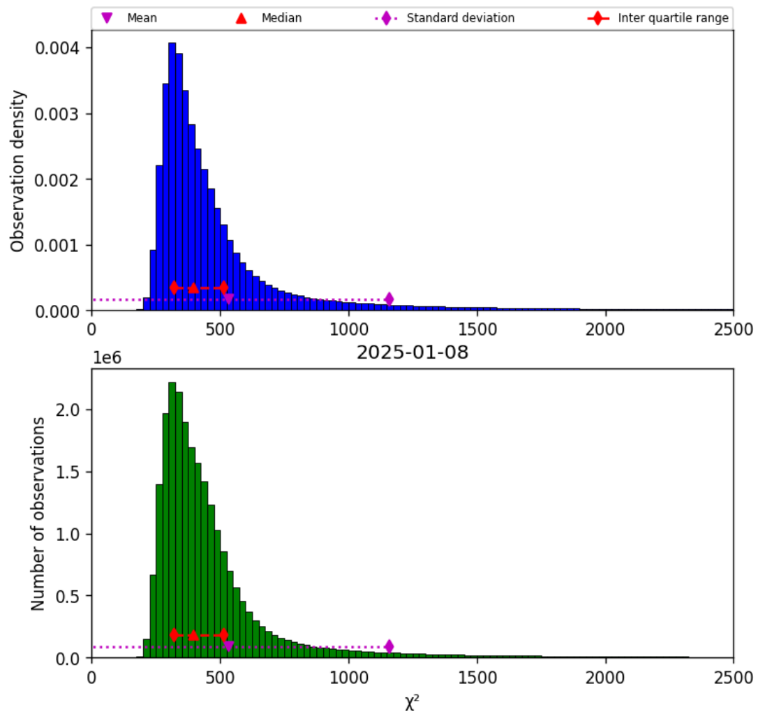
Figure 40: Histogram of “ \chi^2 ” for 2025-01-08 to 2025-01-09
