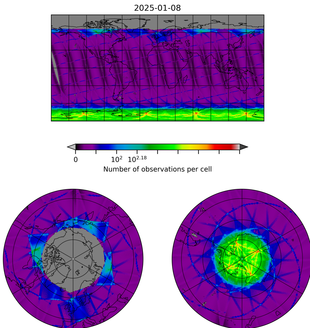
Figure 8: Map of the number of observations for 2025-01-08 to 2025-01-09
