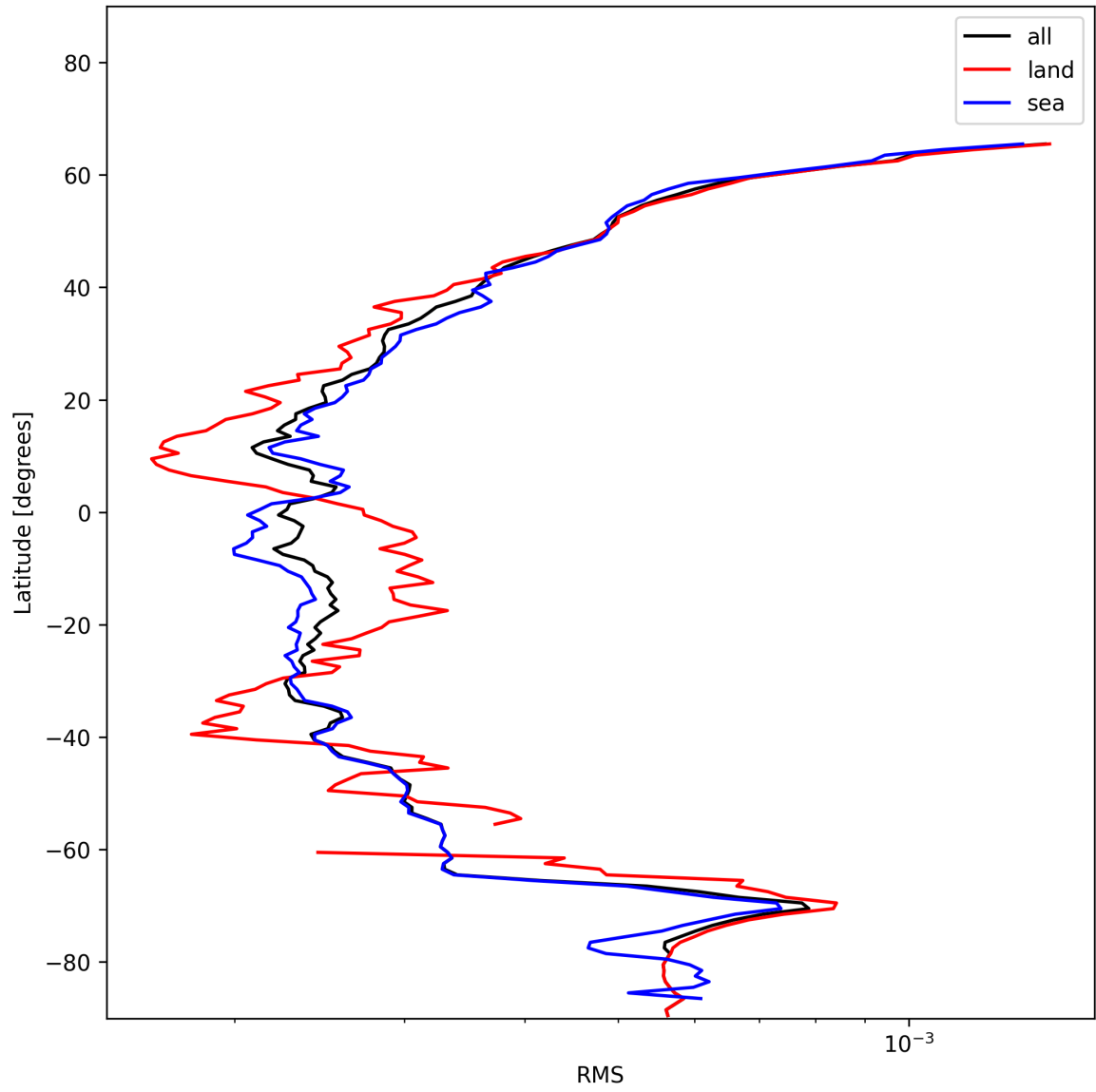
Figure 24: Zonal average of “RMS” for 2025-01-08 to 2025-01-09.
