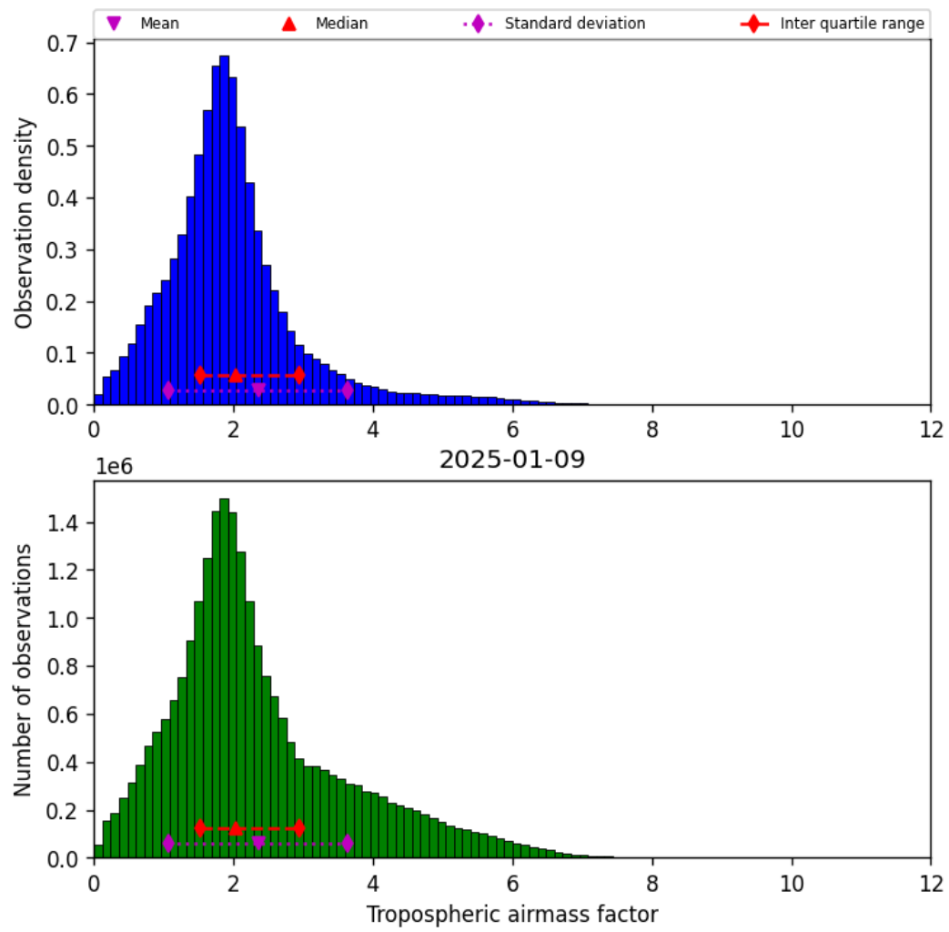
Figure 29: Histogram of “Tropospheric airmass factor” for 2025-01-09 to 2025-01-10
