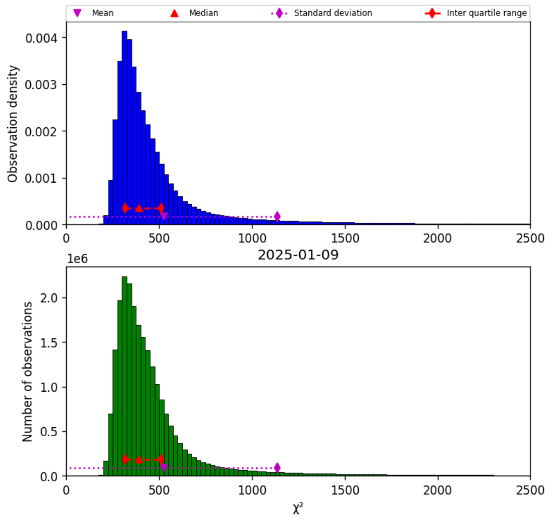
Figure 40: Histogram of “ \chi^2 ” for 2025-01-09 to 2025-01-10
