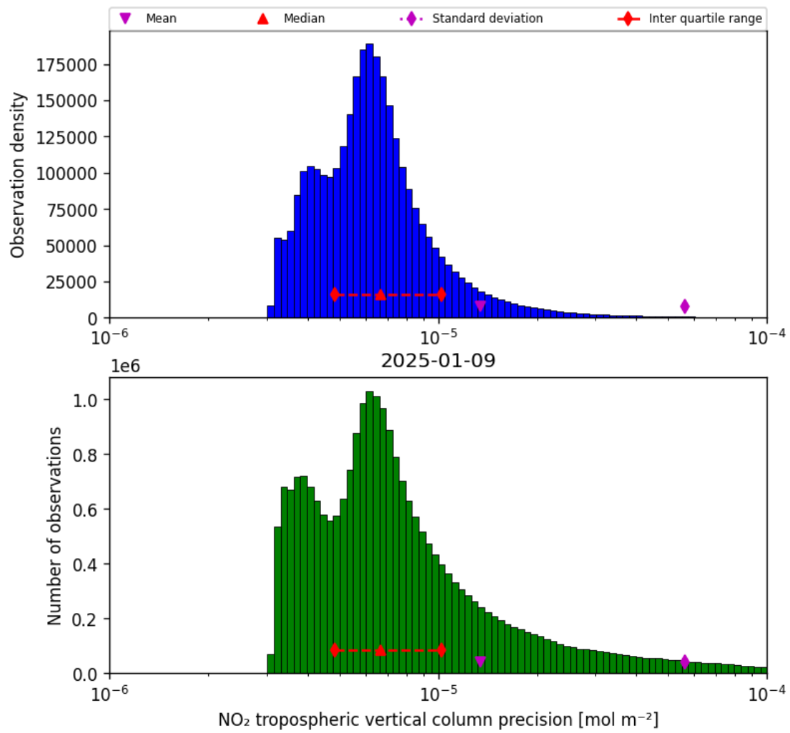
Figure 28: Histogram of “NO 2 tropospheric vertical column precision” for 2025-01-09 to 2025-01-10
