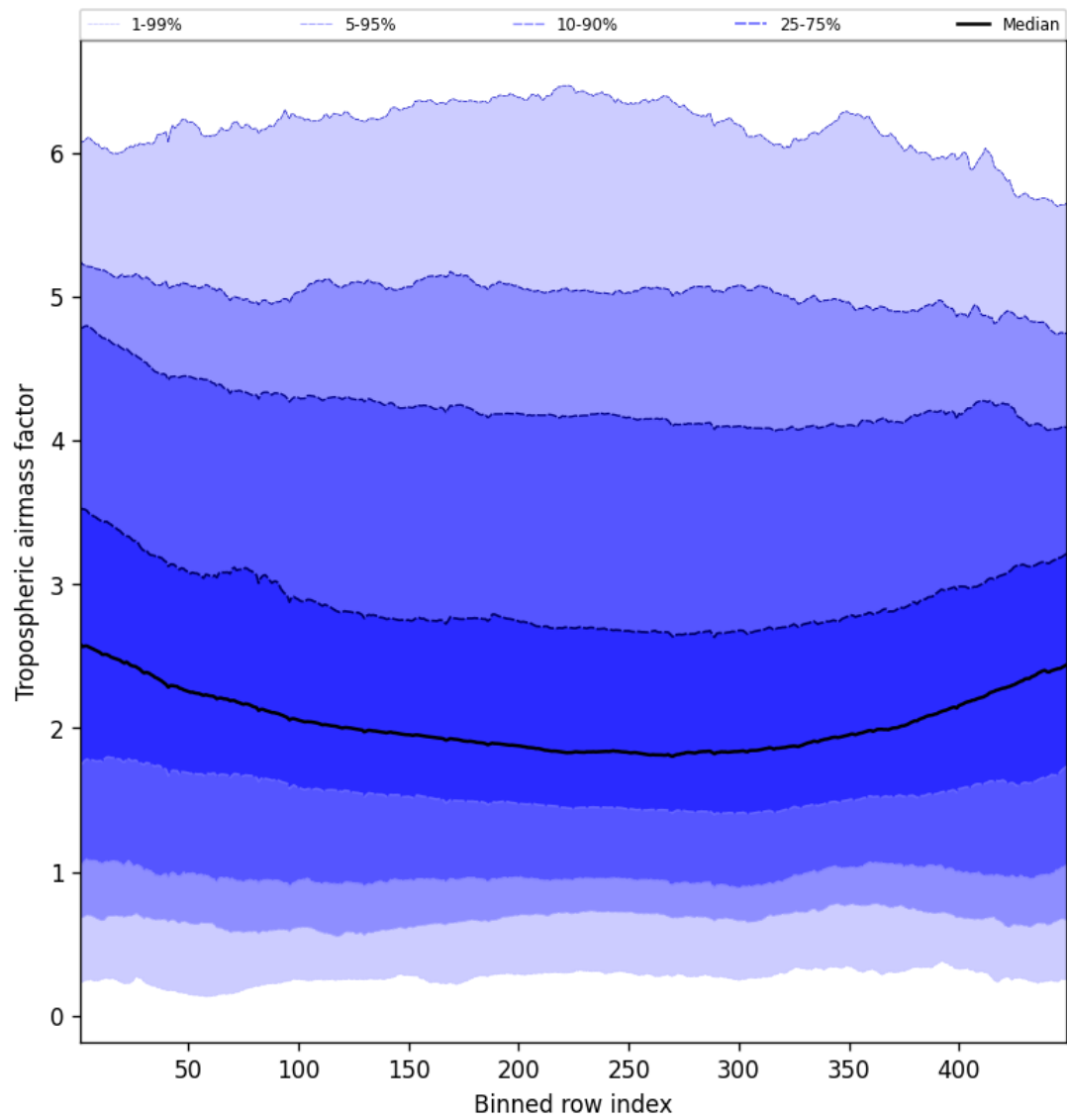
Figure 46: Along track statistics of “Tropospheric airmass factor” for 2025-01-09 to 2025-01-10
