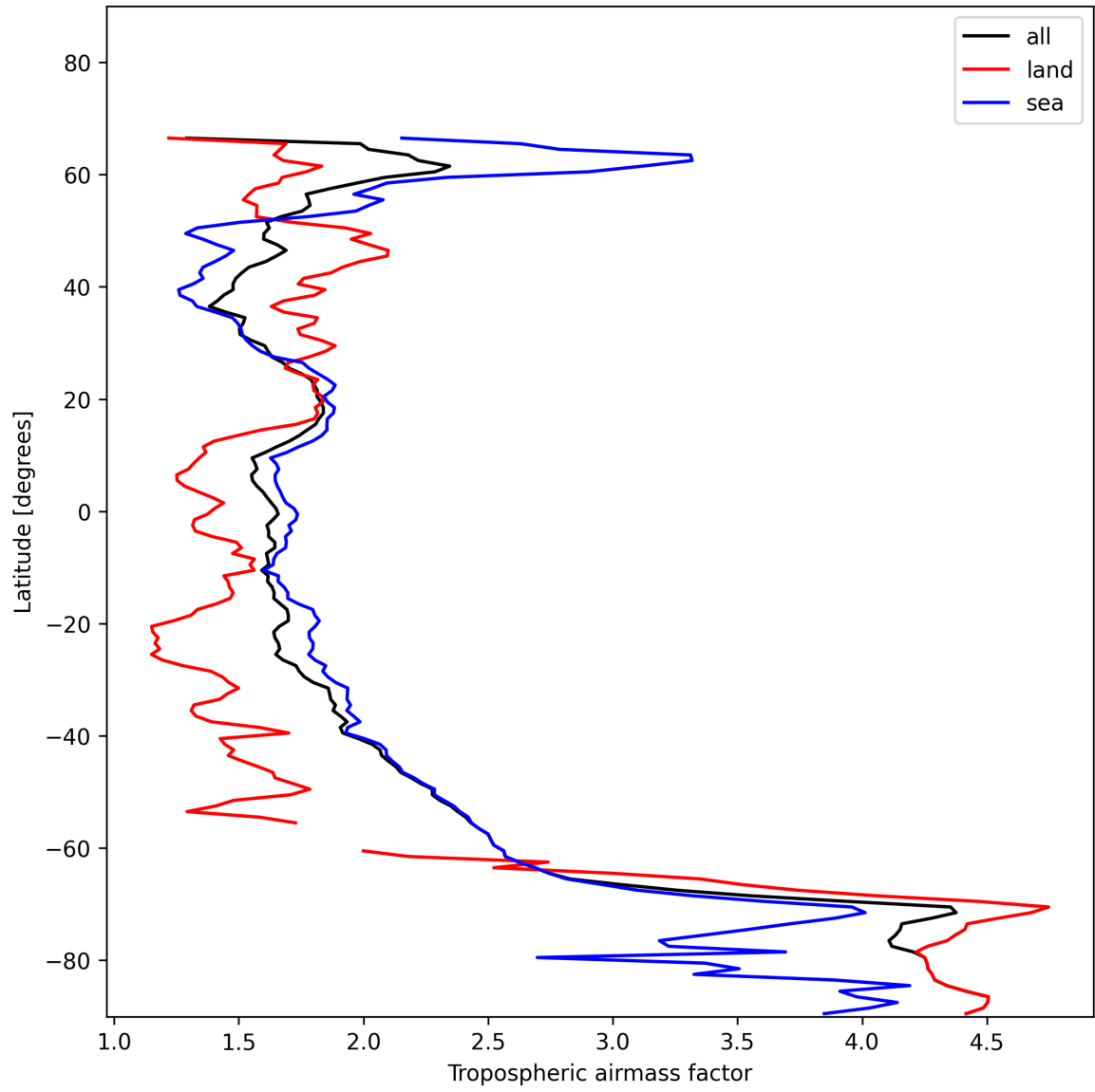
Figure 12: Zonal average of “Tropospheric airmass factor” for 2025-01-09 to 2025-01-10.
