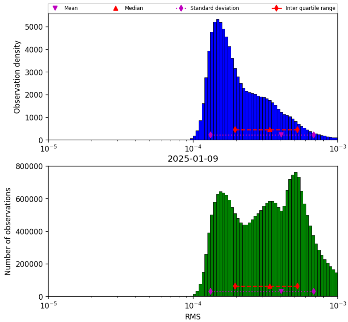
Figure 41: Histogram of “RMS” for 2025-01-09 to 2025-01-10
