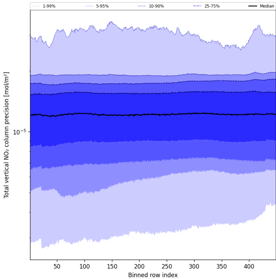
Figure 54: Along track statistics of “Total vertical NO 2 column precision” for 2025-01-09 to 2025-01-10
