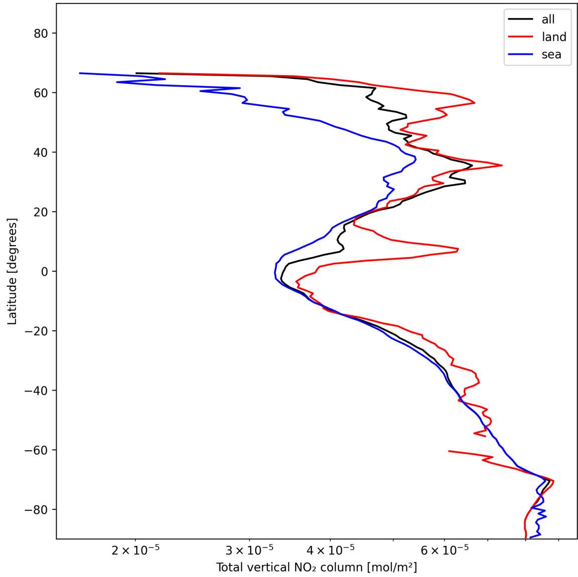
Figure 19: Zonal average of “Total vertical NO 2 column” for 2025-01-09 to 2025-01-10.
