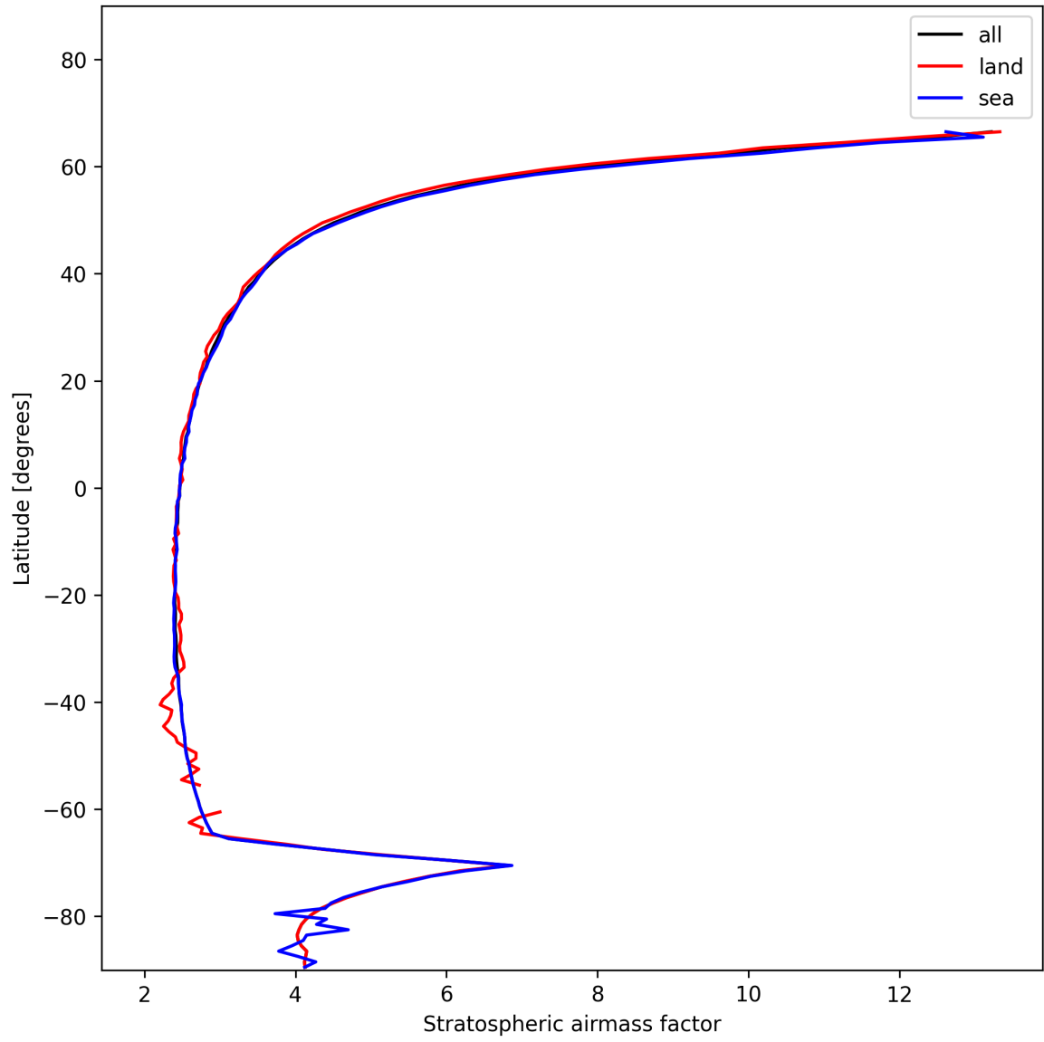
Figure 25: Zonal average of “Stratospheric airmass factor” for 2025-01-09 to 2025-01-10.
