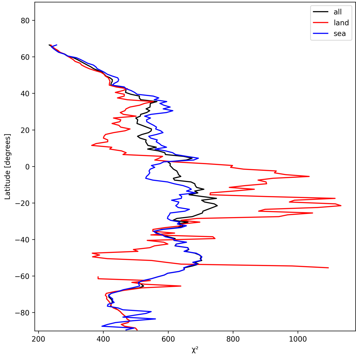
Figure 23: Zonal average of “ \chi^2 ” for 2025-01-09 to 2025-01-10.
