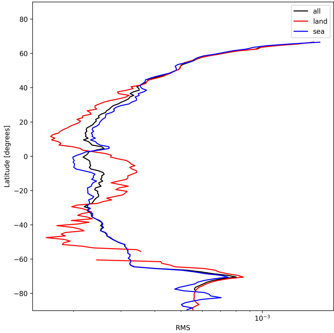
Figure 24: Zonal average of “RMS” for 2025-01-09 to 2025-01-10.
