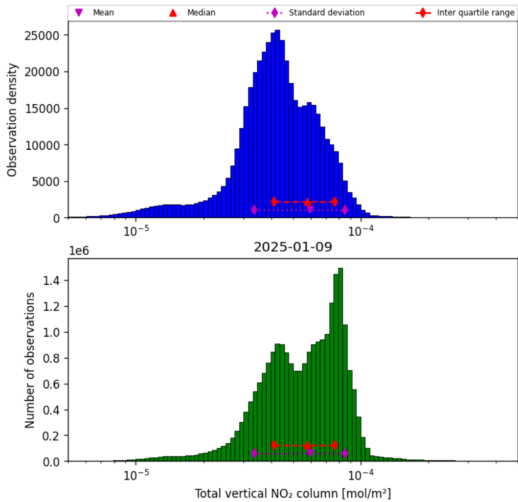
Figure 36: Histogram of “Total vertical NO 2 column” for 2025-01-09 to 2025-01-10
