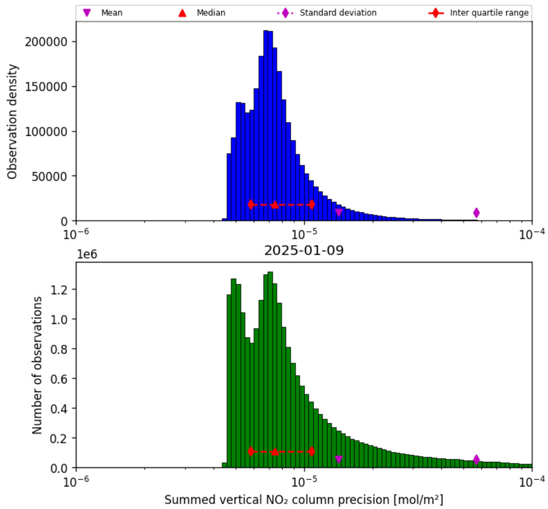
Figure 39: Histogram of "Summed vertical NO 2 column precision" for 2025-01-09 to 2025-01-10
