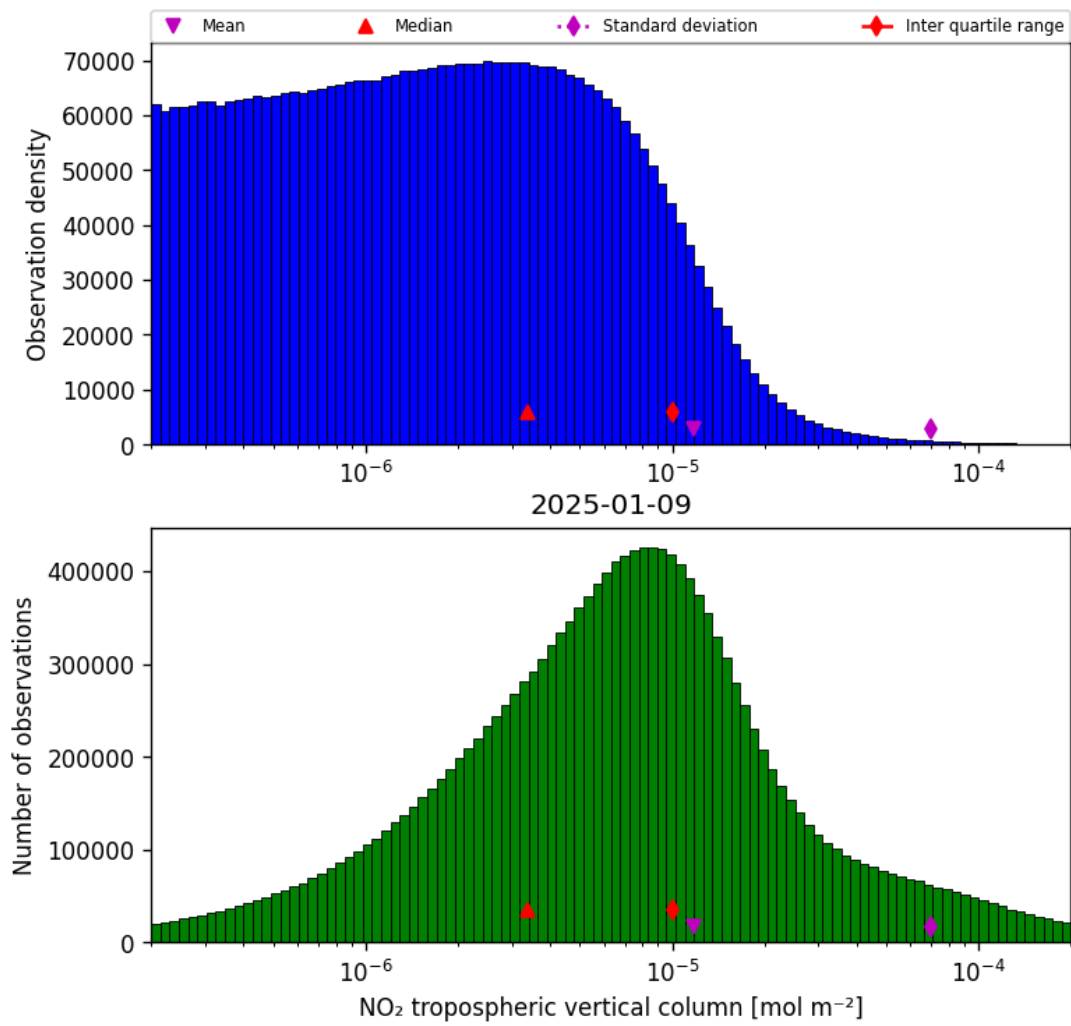
Figure 27: Histogram of “NO 2 tropospheric vertical column” for 2025-01-09 to 2025-01-10
