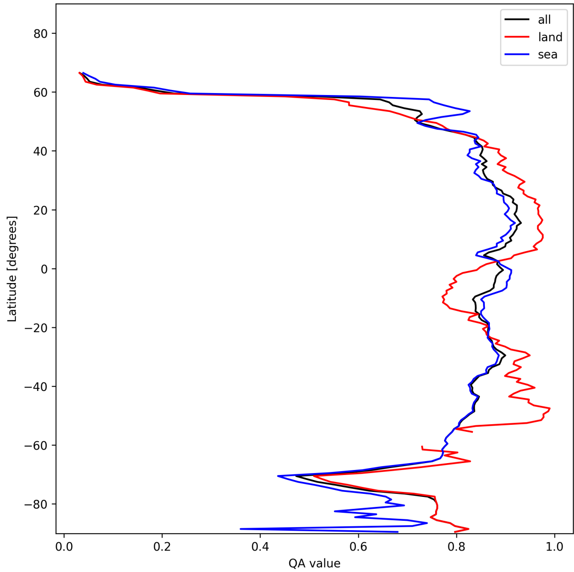
Figure 9: Zonal average of “QA value” for 2025-01-09 to 2025-01-10.
