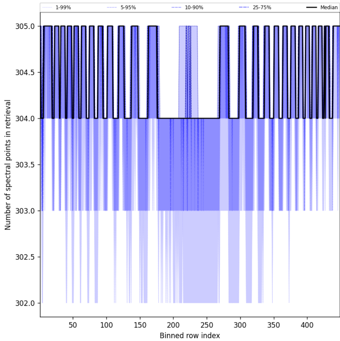
Figure 48: Along track statistics of “Number of spectral points in retrieval” for 2025-01-09 to 2025-01-10
