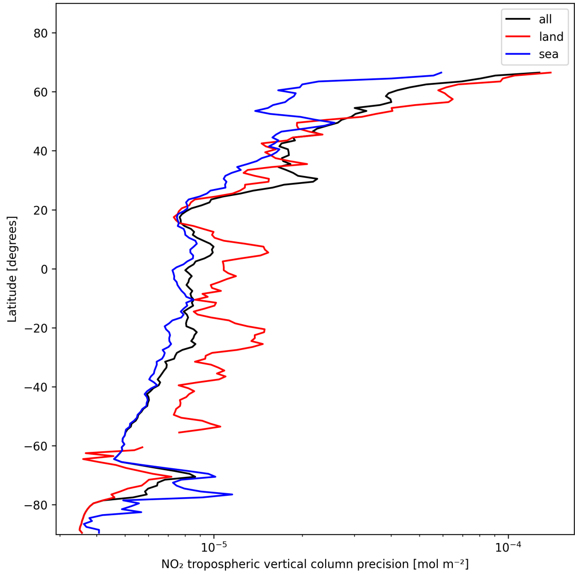
Figure 11: Zonal average of “NO 2 tropospheric vertical column precision” for 2025-01-09 to 2025-01-10.
