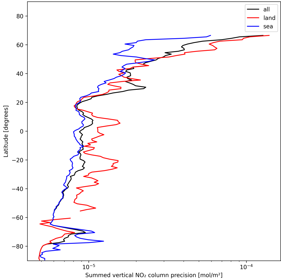
Figure 22: Zonal average of “Summed vertical NO 2 column precision” for 2025-01-09 to 2025-01-10.
