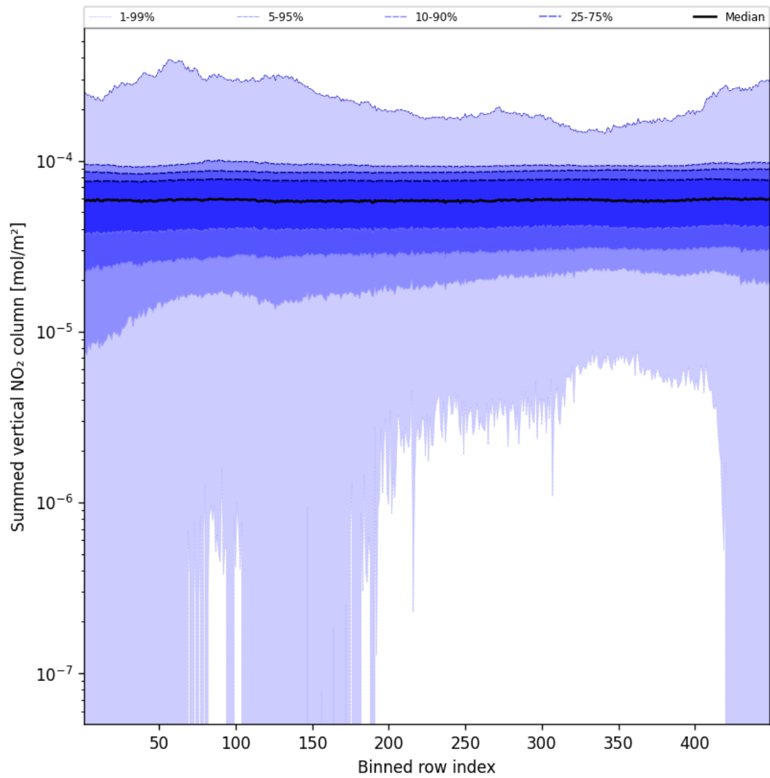
Figure 55: Along track statistics of “Summed vertical NO 2 column” for 2025-01-09 to 2025-01-10
