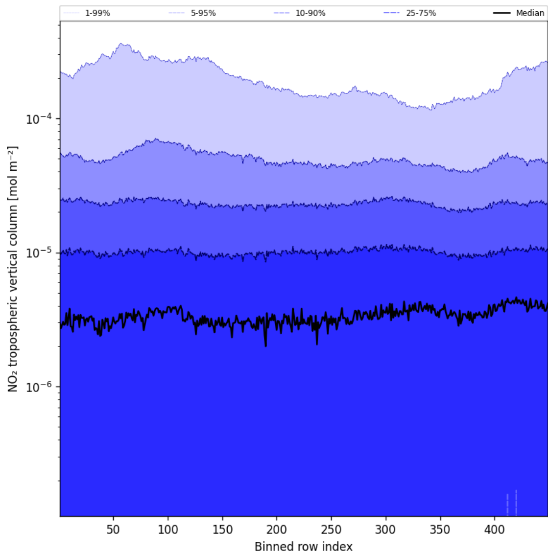
Figure 44: Along track statistics of “NO 2 tropospheric vertical column” for 2025-01-09 to 2025-01-10
