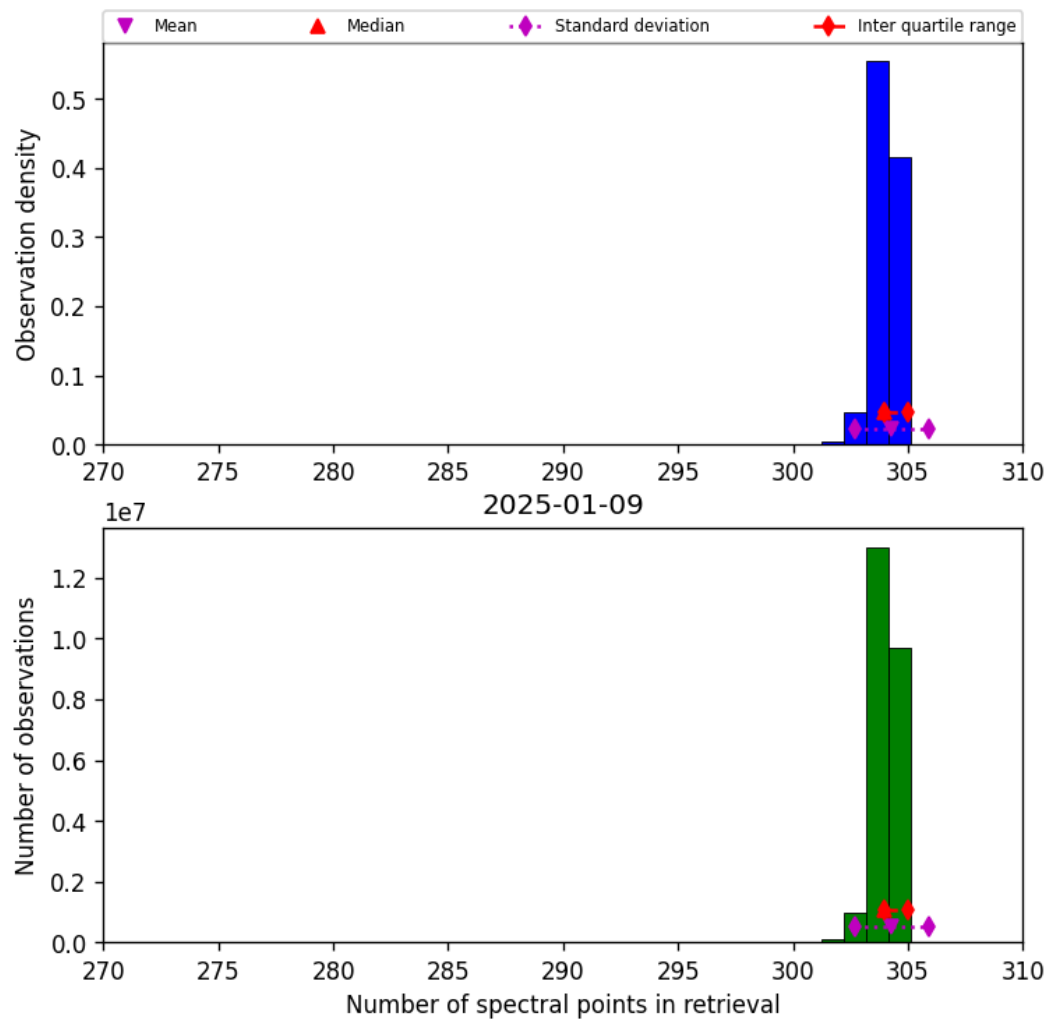
Figure 31: Histogram of “Number of spectral points in retrieval” for 2025-01-09 to 2025-01-10
