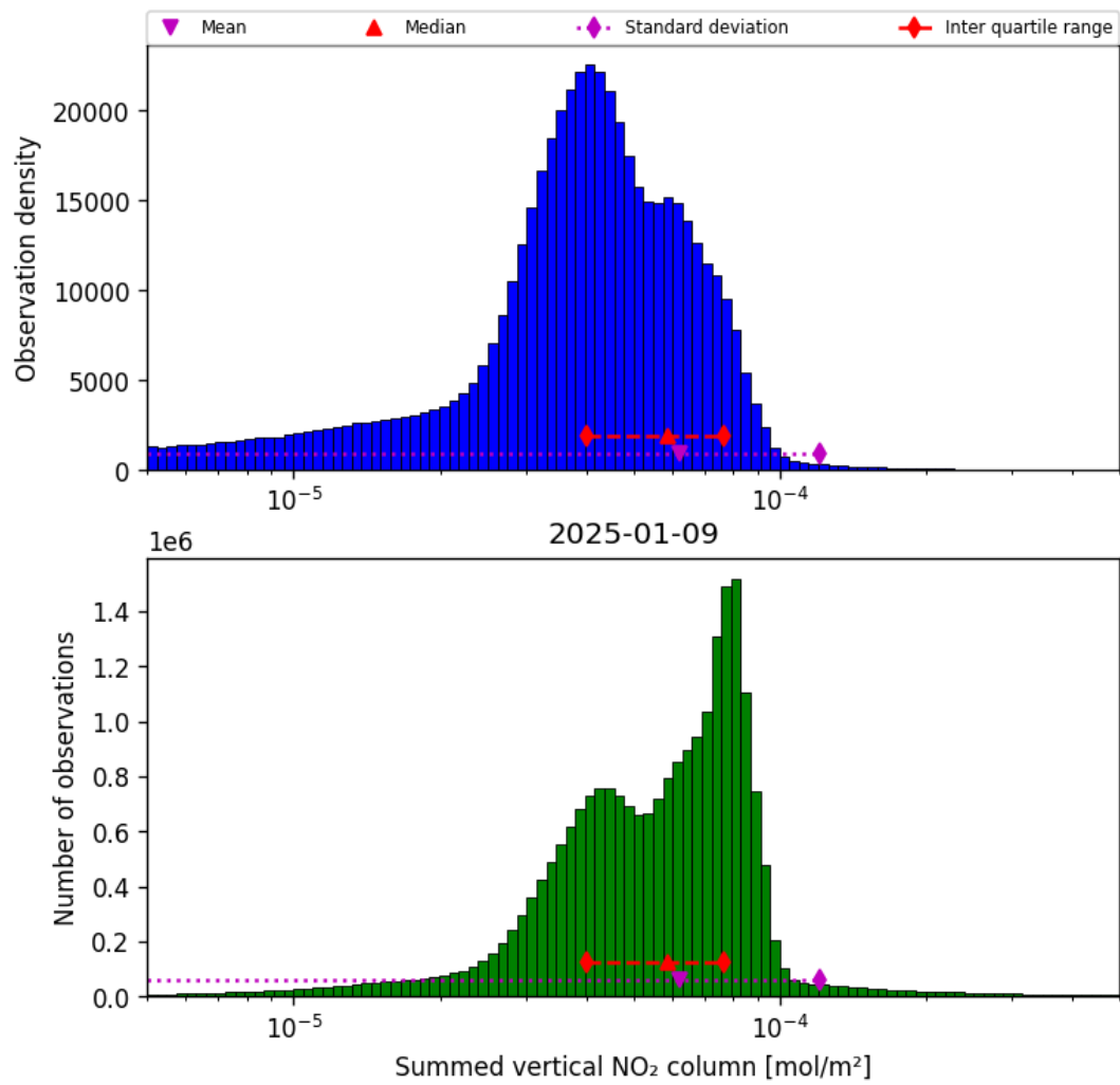
Figure 38: Histogram of “Summed vertical NO 2 column” for 2025-01-09 to 2025-01-10
