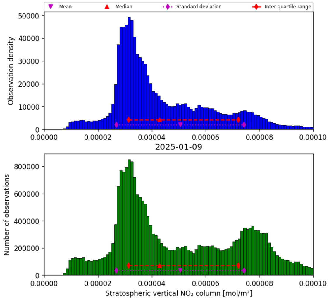
Figure 34: Histogram of “Stratospheric vertical NO 2 column” for 2025-01-09 to 2025-01-10
