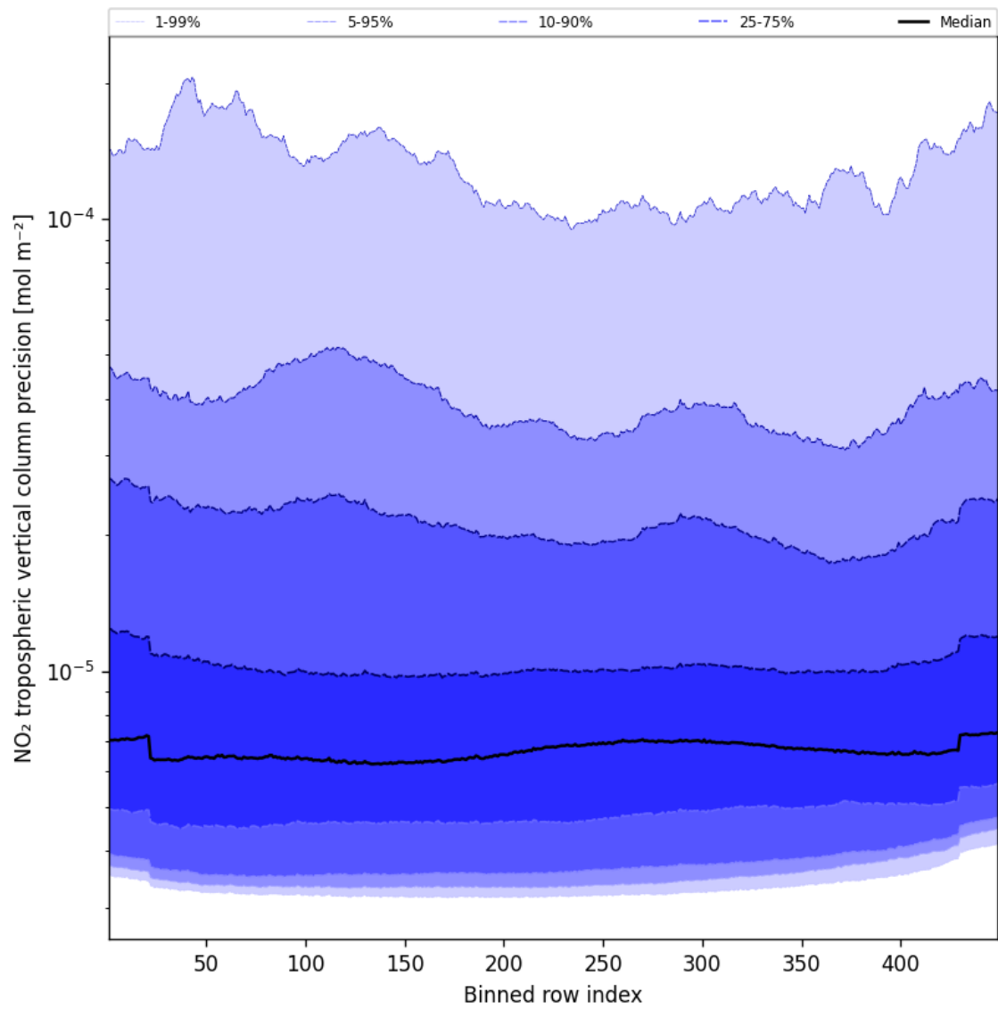
Figure 45: Along track statistics of “NO 2 tropospheric vertical column precision” for 2025-01-09 to 2025-01-10
