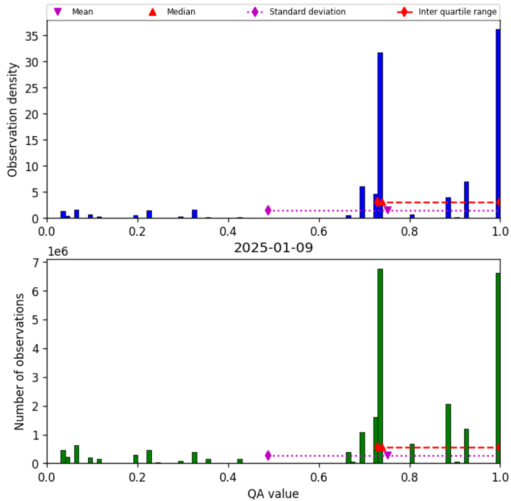
Figure 26: Histogram of “QA value” for 2025-01-09 to 2025-01-10
