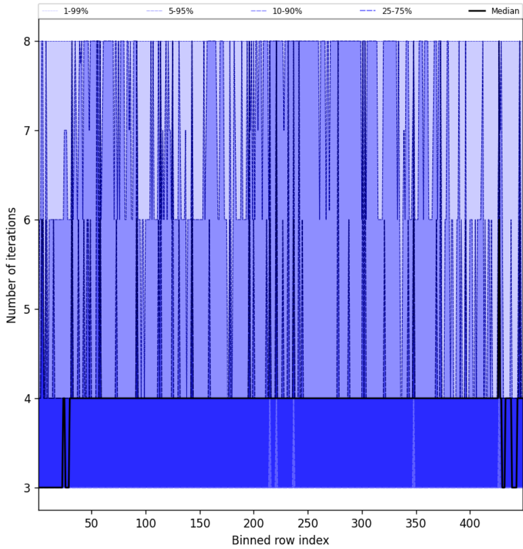
Figure 49: Along track statistics of “Number of iterations” for 2025-01-09 to 2025-01-10
