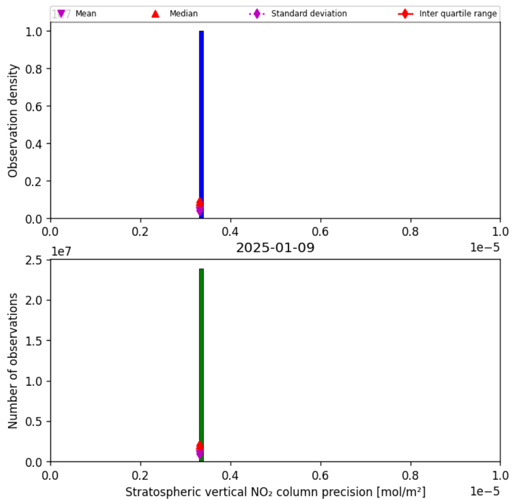
Figure 35: Histogram of “Stratospheric vertical NO 2 column precision” for 2025-01-09 to 2025-01-10
