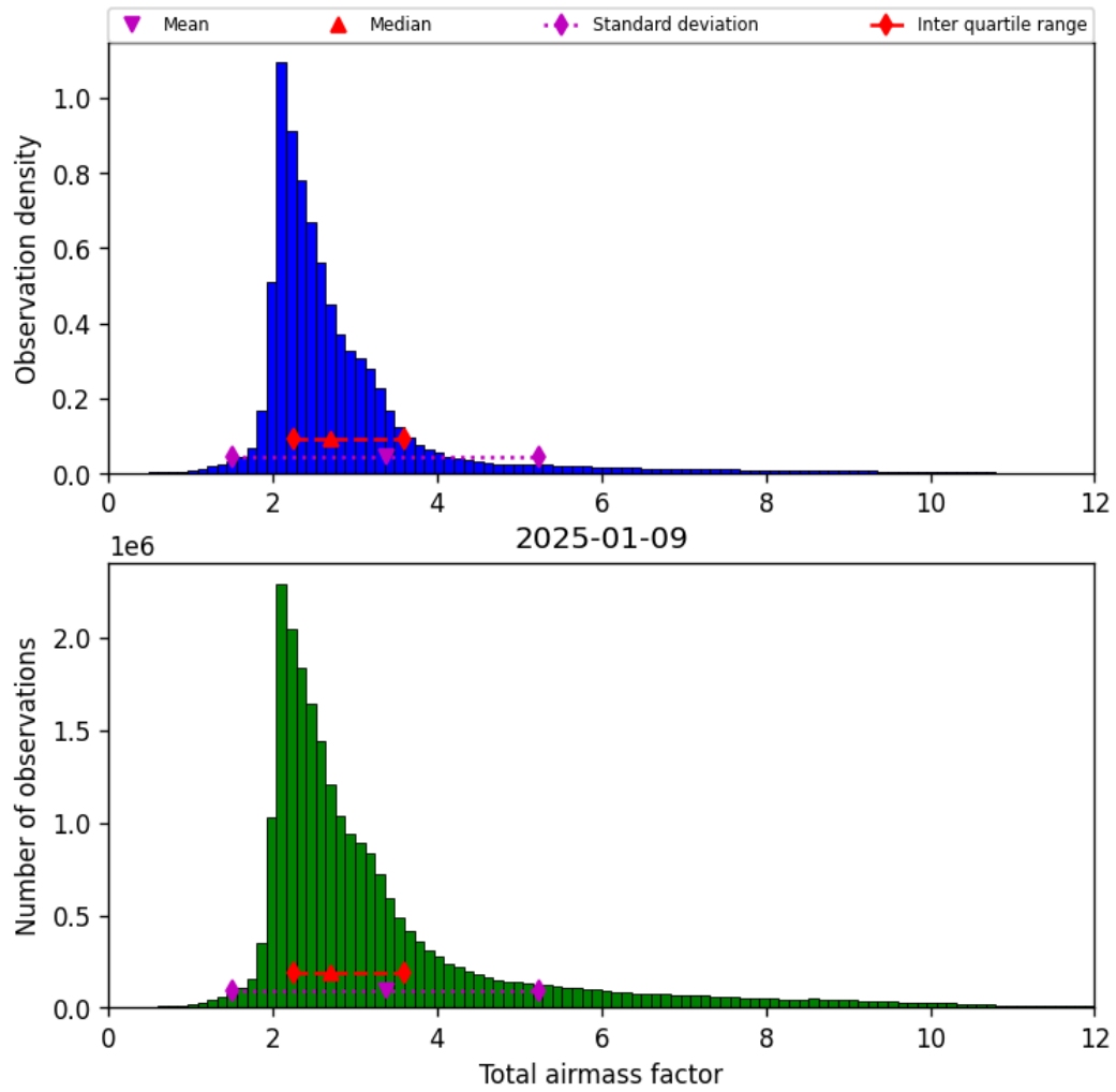
Figure 30: Histogram of “Total airmass factor” for 2025-01-09 to 2025-01-10
