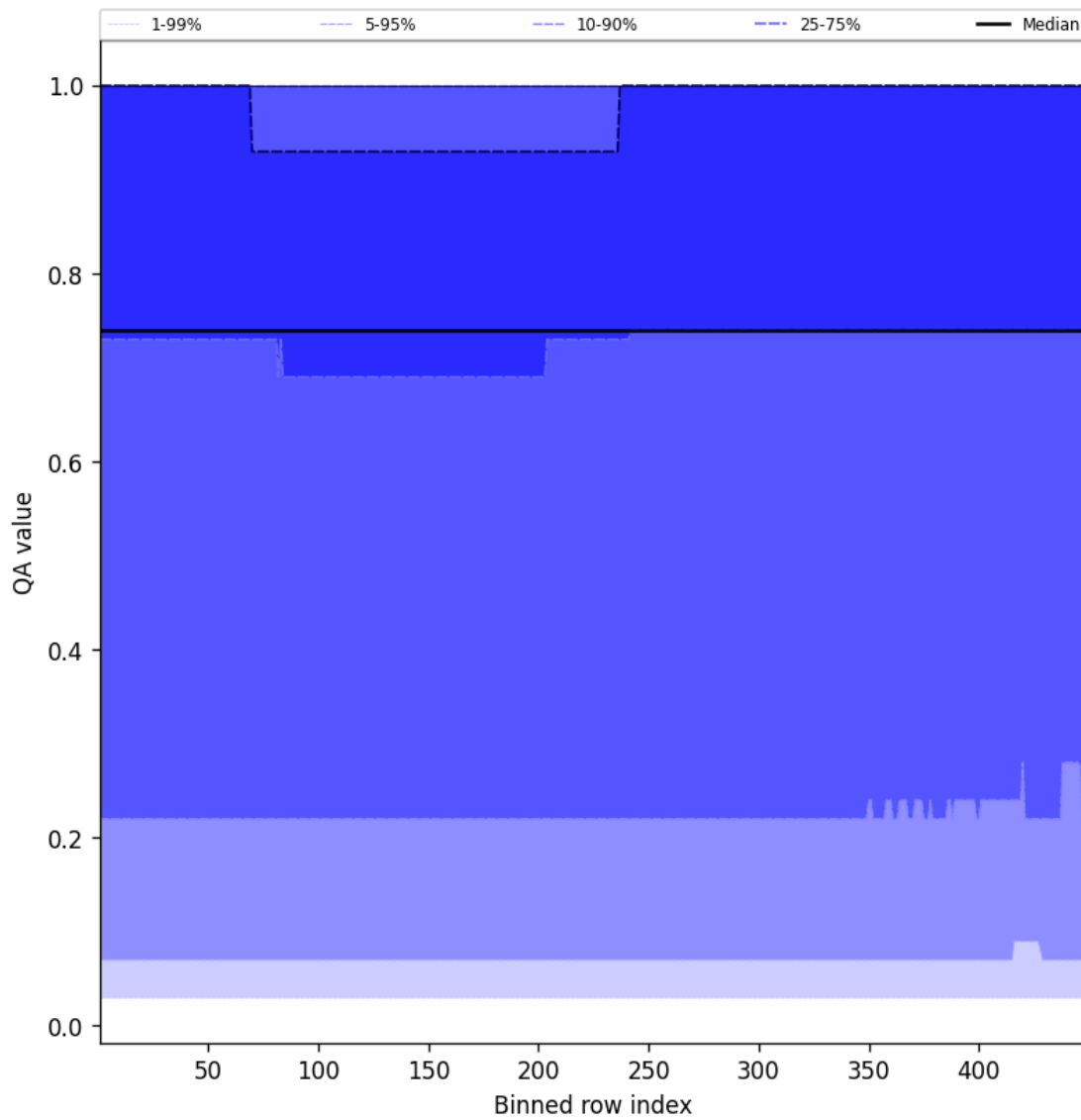
Figure 43: Along track statistics of “QA value” for 2025-01-09 to 2025-01-10
