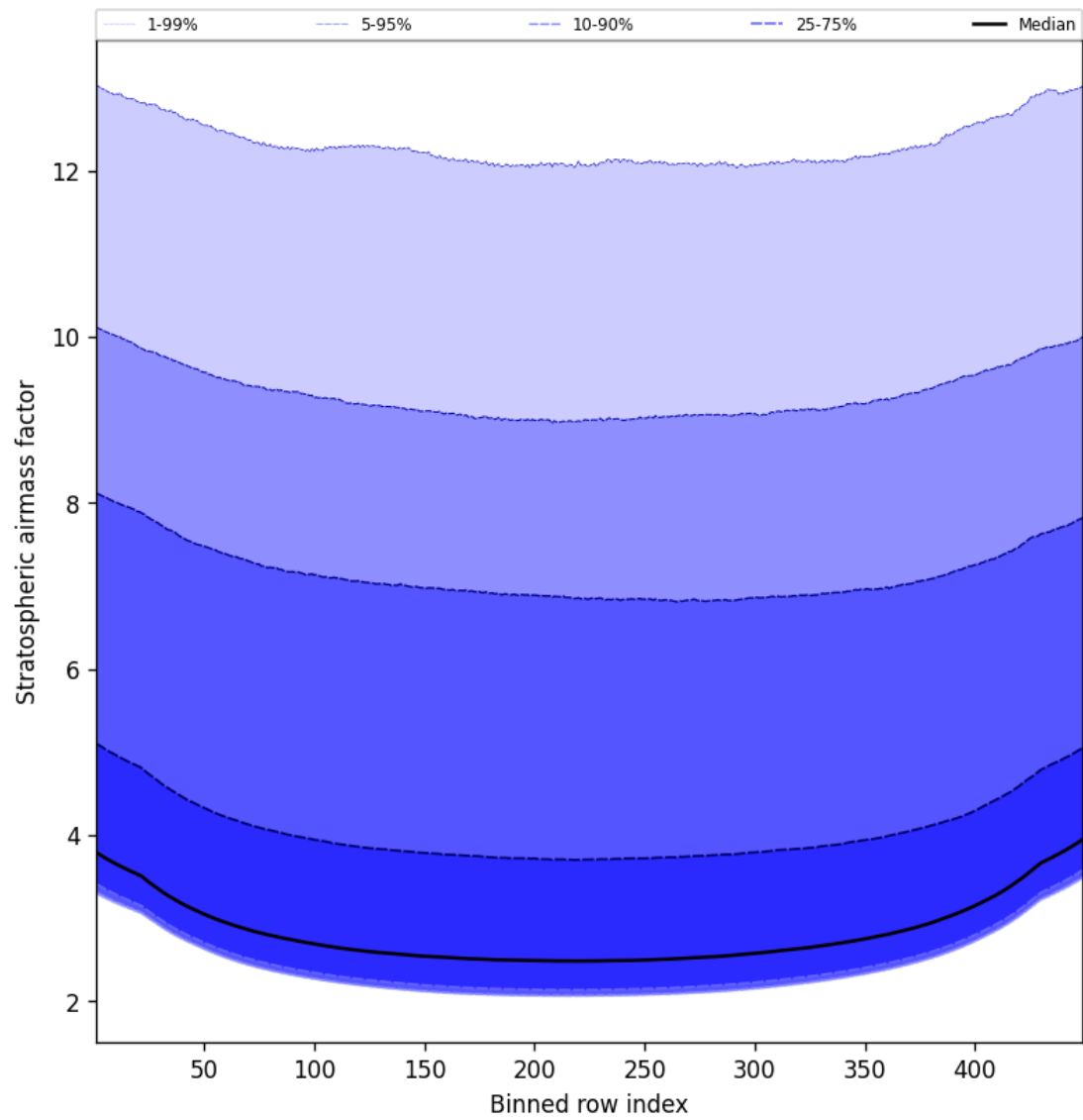
Figure 59: Along track statistics of “Stratospheric airmass factor” for 2025-01-09 to 2025-01-10
