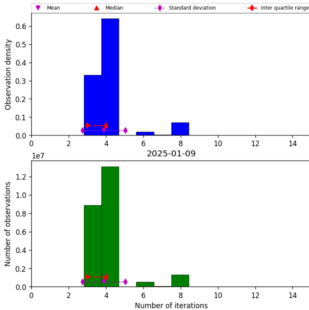
Figure 32: Histogram of “Number of iterations” for 2025-01-09 to 2025-01-10
