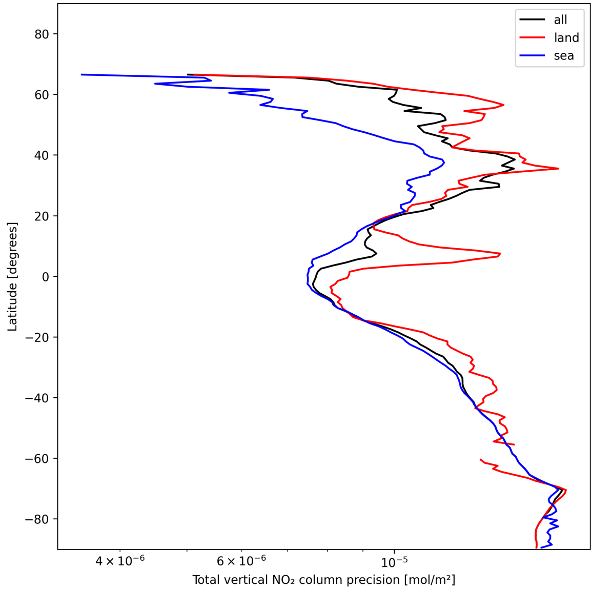
Figure 20: Zonal average of “Total vertical NO 2 column precision” for 2025-01-09 to 2025-01-10.
