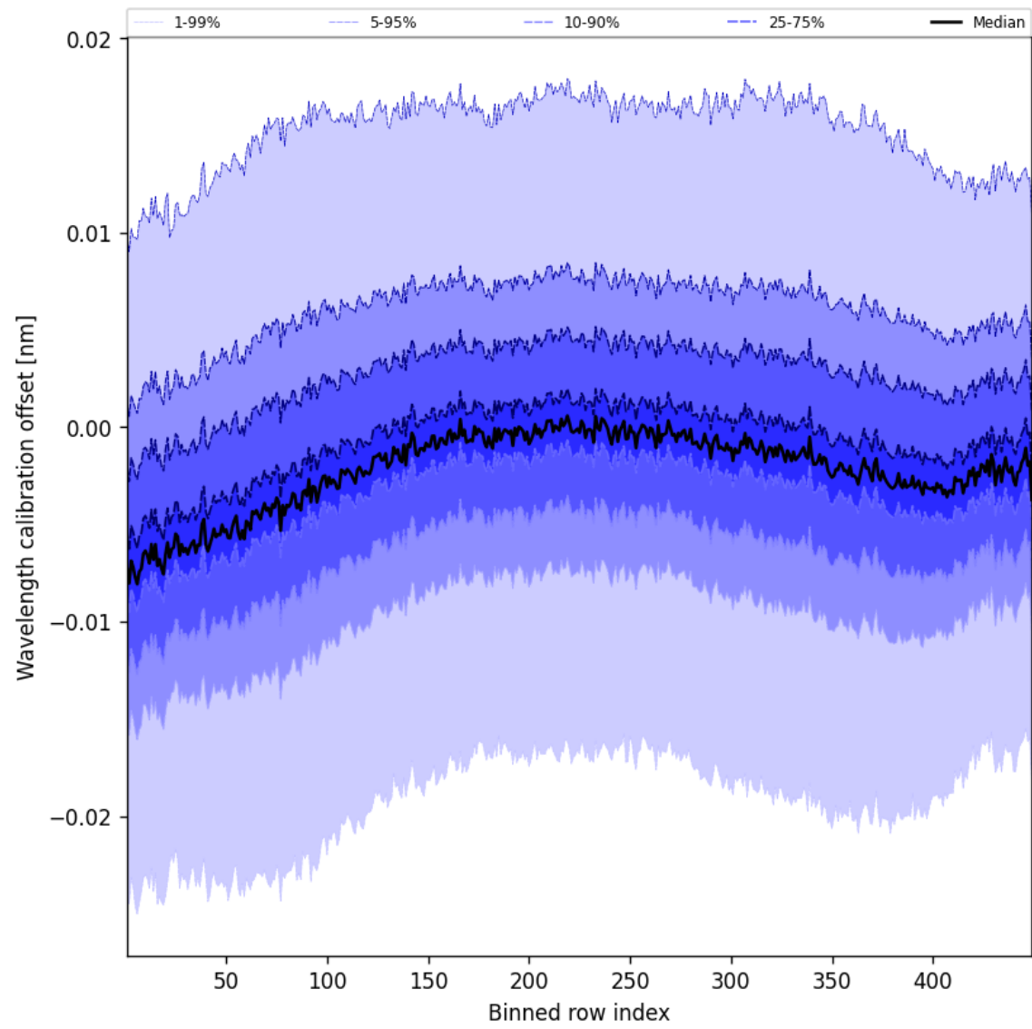
Figure 50: Along track statistics of “Wavelength calibration offset” for 2025-01-09 to 2025-01-10
