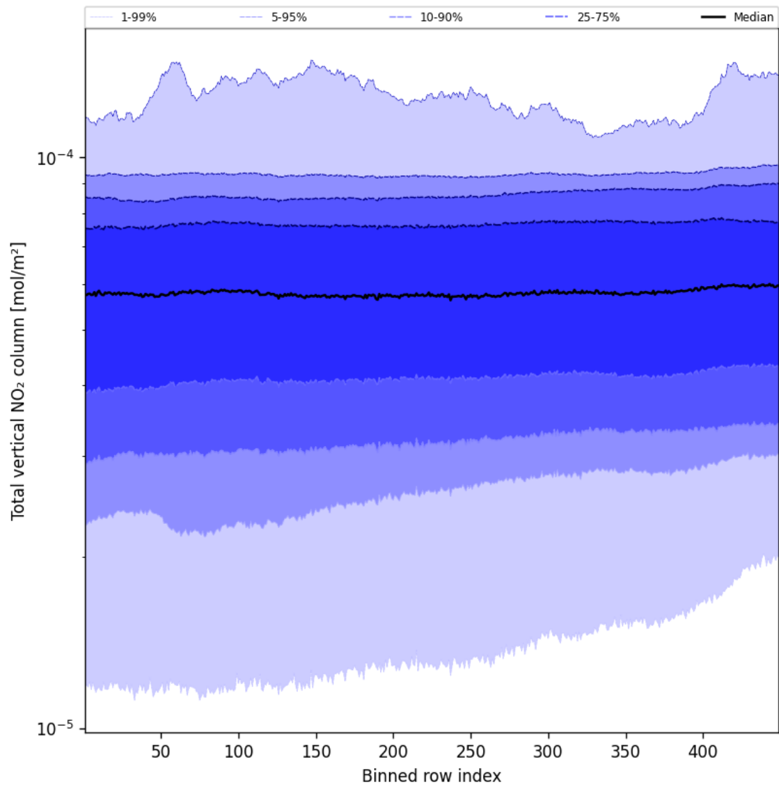
Figure 53: Along track statistics of “Total vertical NO 2 column” for 2025-01-09 to 2025-01-10
