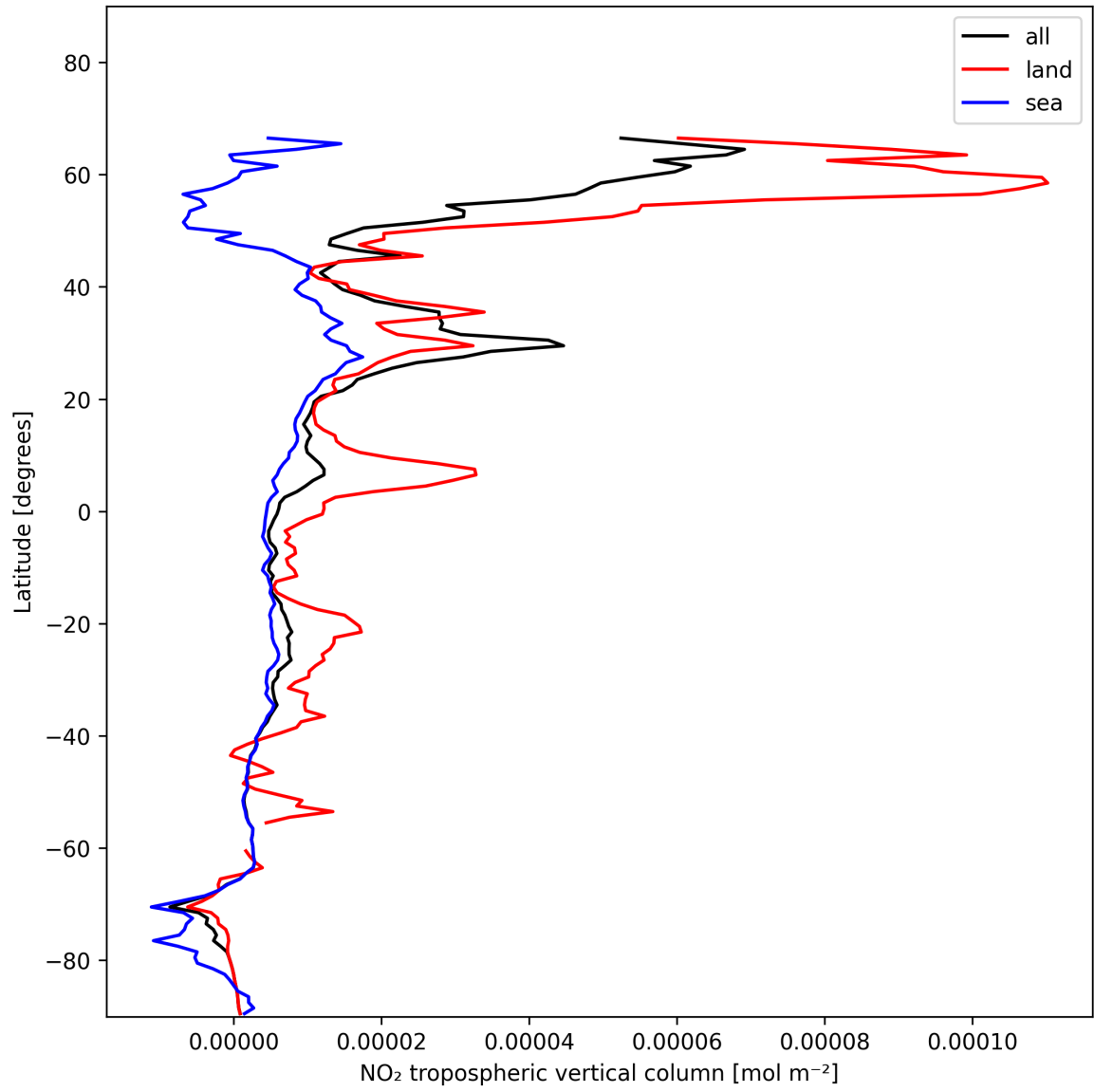
Figure 10: Zonal average of “NO 2 tropospheric vertical column” for 2025-01-09 to 2025-01-10.
