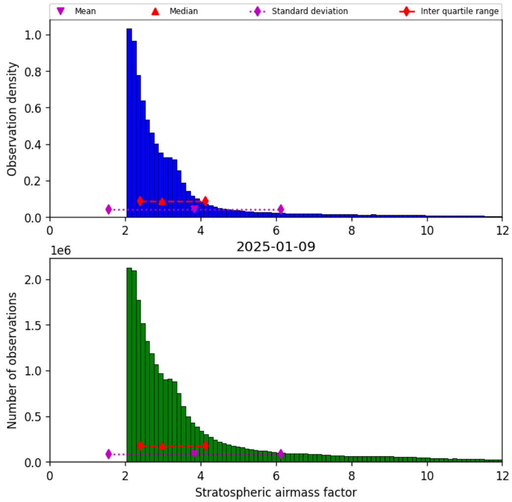
Figure 42: Histogram of “Stratospheric airmass factor” for 2025-01-09 to 2025-01-10
