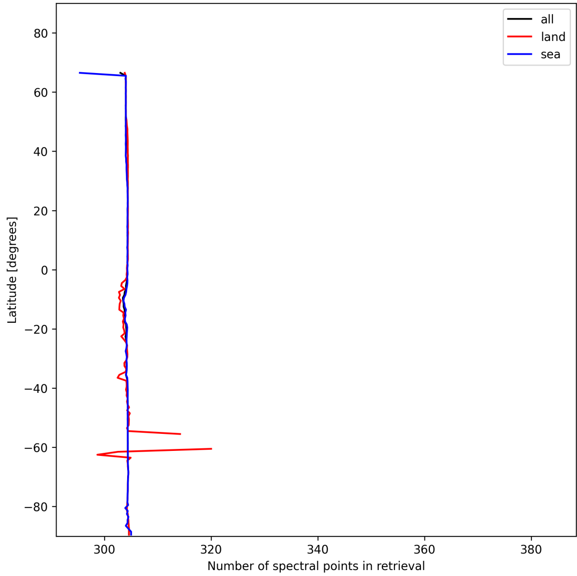
Figure 14: Zonal average of “Number of spectral points in retrieval” for 2025-01-09 to 2025-01-10.
