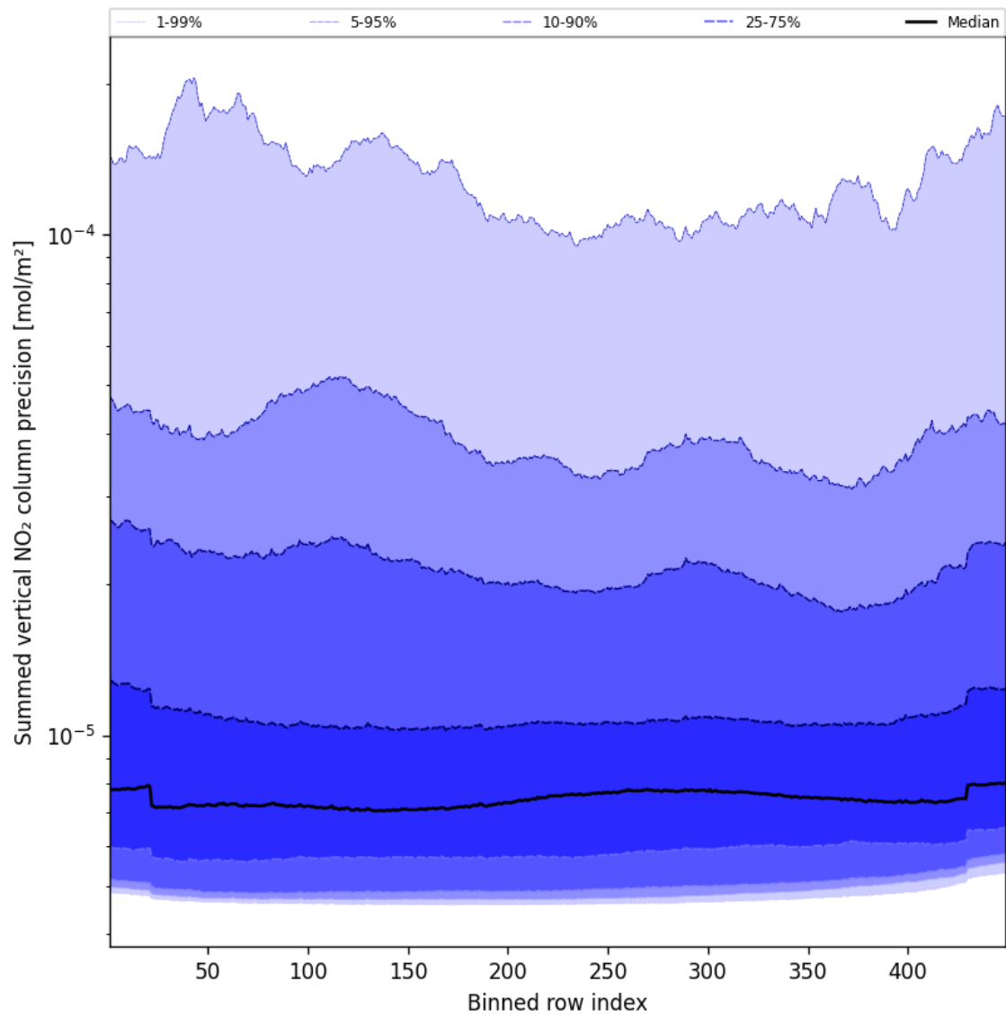
Figure 56: Along track statistics of “Summed vertical NO 2 column precision” for 2025-01-09 to 2025-01-10
