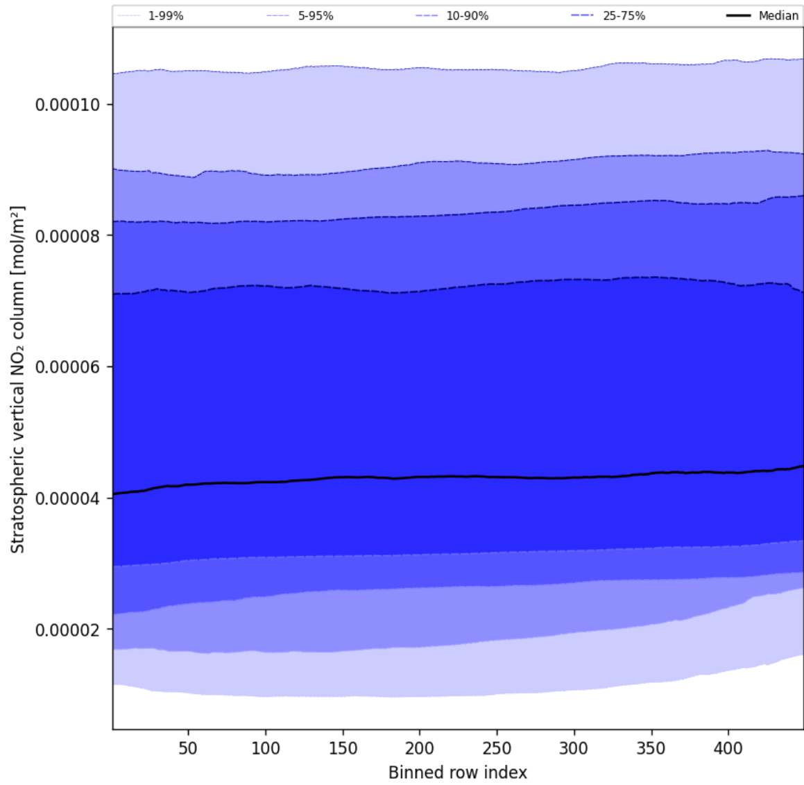
Figure 51: Along track statistics of “Stratospheric vertical NO 2 column” for 2025-01-09 to 2025-01-10
