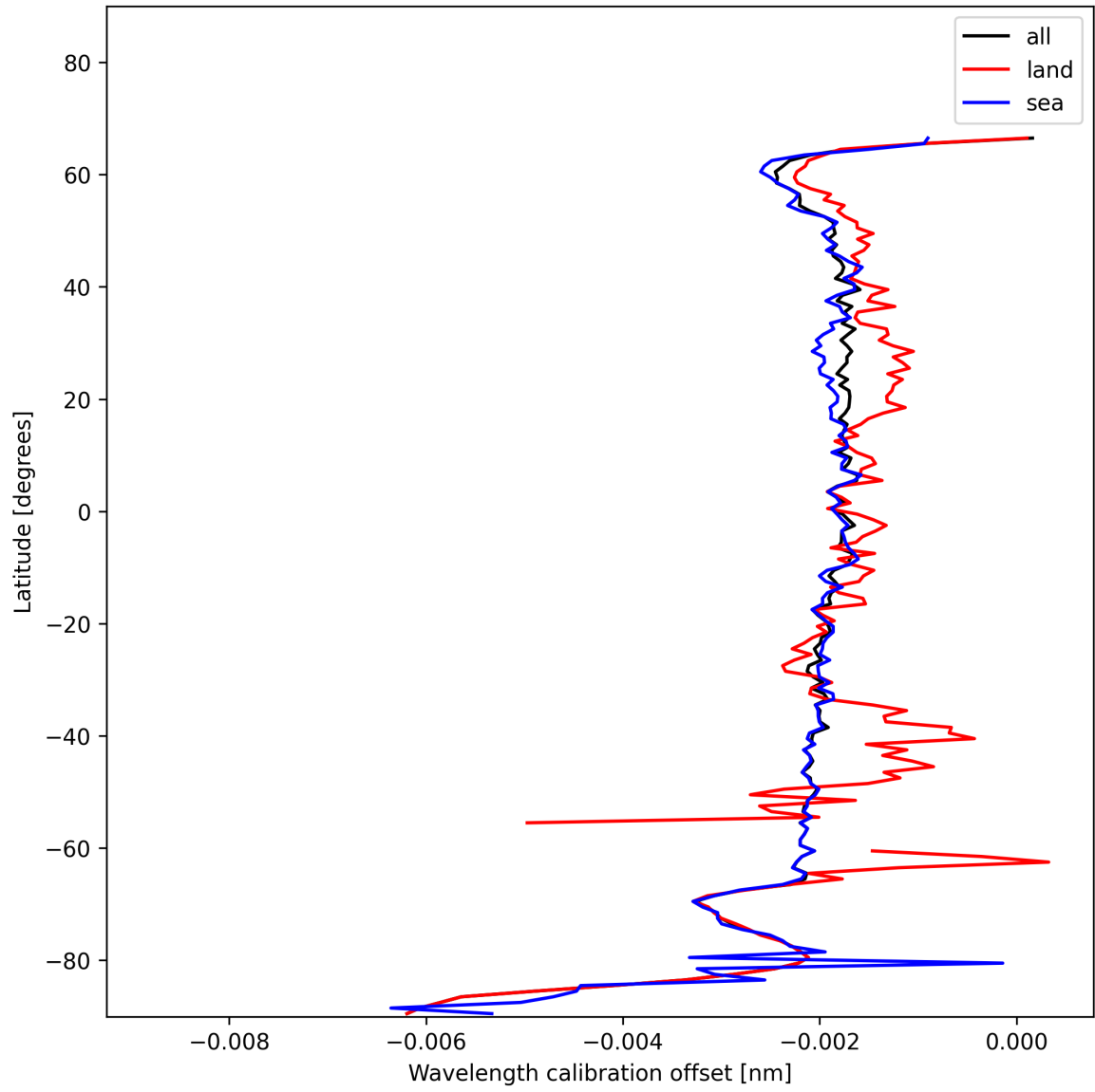
Figure 16: Zonal average of “Wavelength calibration offset” for 2025-01-09 to 2025-01-10.
