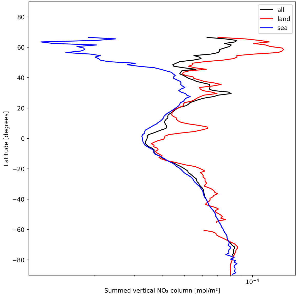
Figure 21: Zonal average of “Summed vertical NO 2 column” for 2025-01-09 to 2025-01-10.
