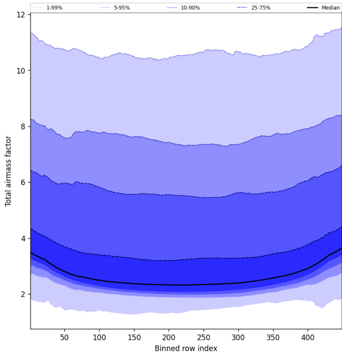
Figure 47: Along track statistics of “Total airmass factor” for 2025-01-09 to 2025-01-10
