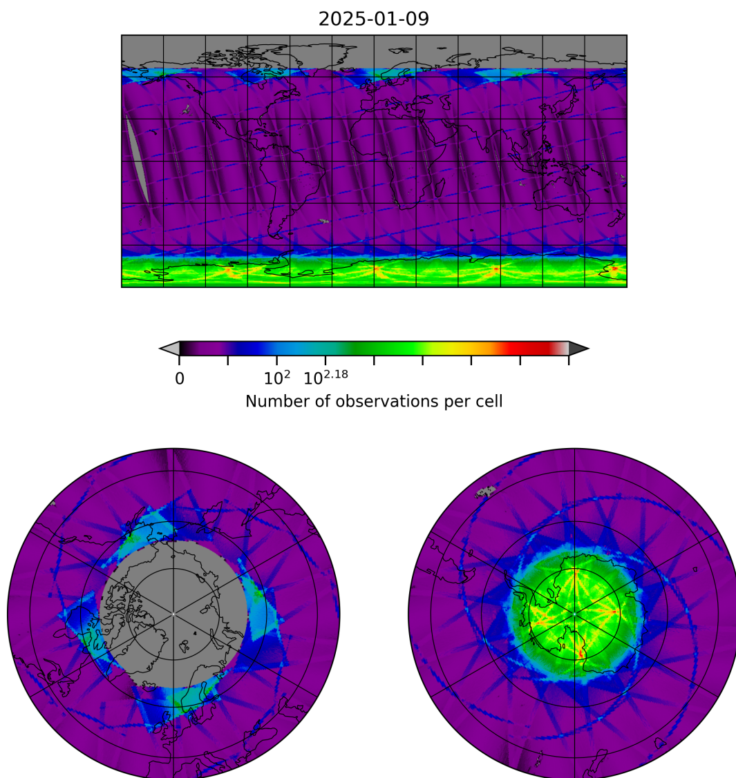
Figure 8: Map of the number of observations for 2025-01-09 to 2025-01-10
