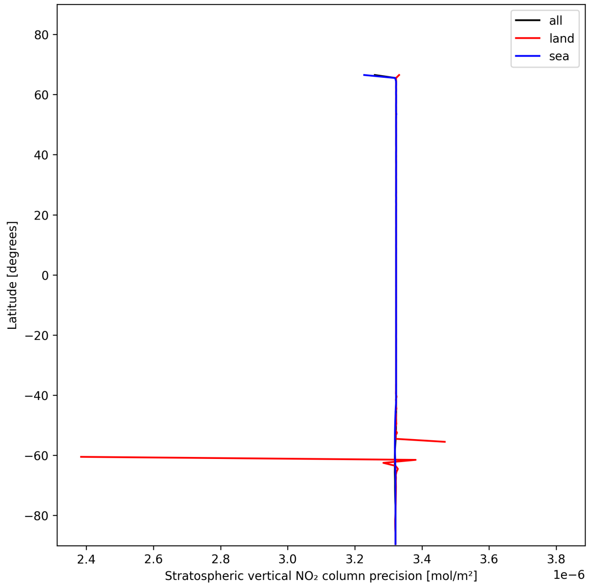
Figure 18: Zonal average of “Stratospheric vertical NO 2 column precision” for 2025-01-09 to 2025-01-10.
