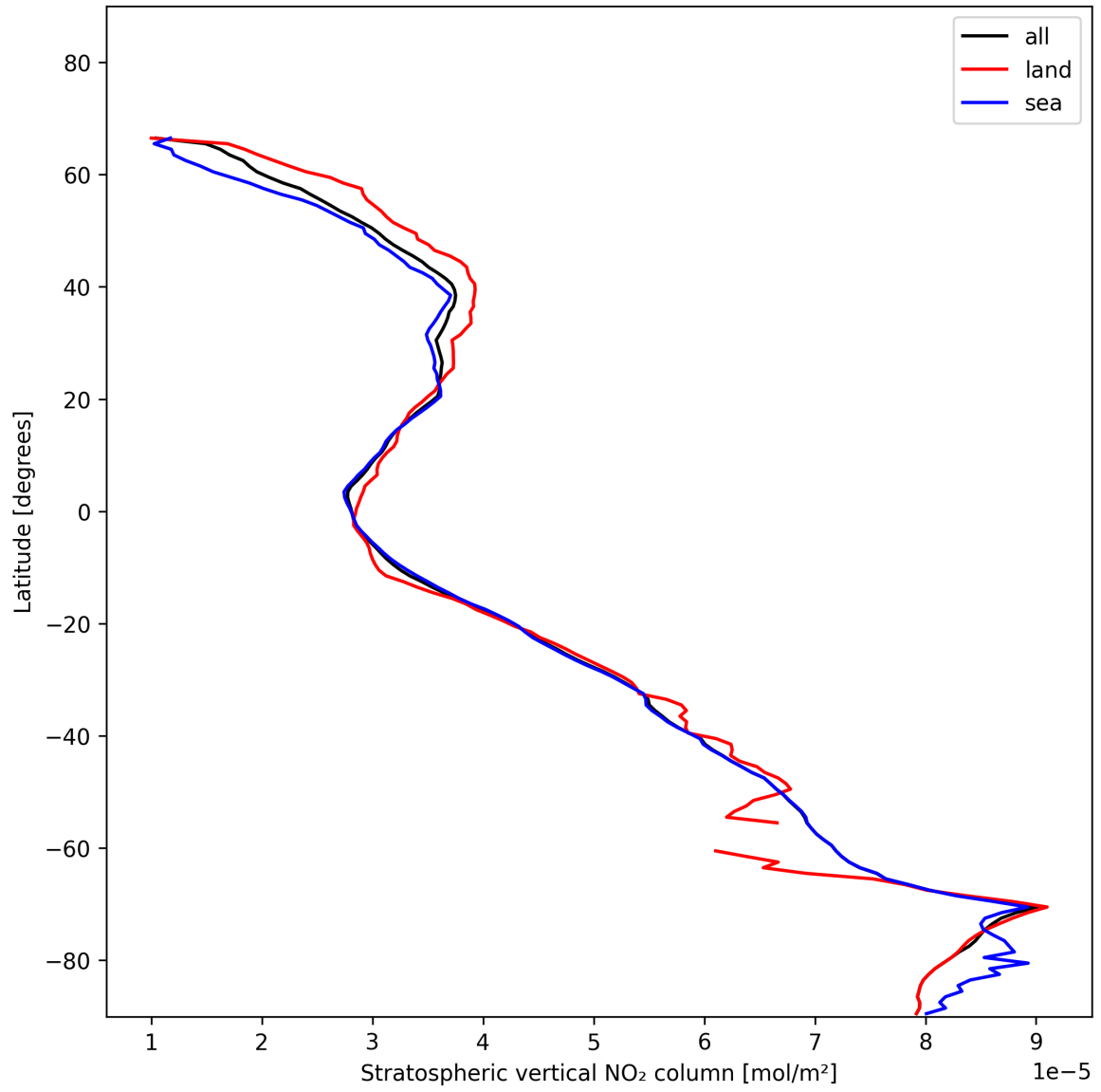
Figure 17: Zonal average of “Stratospheric vertical NO 2 column” for 2025-01-09 to 2025-01-10.
