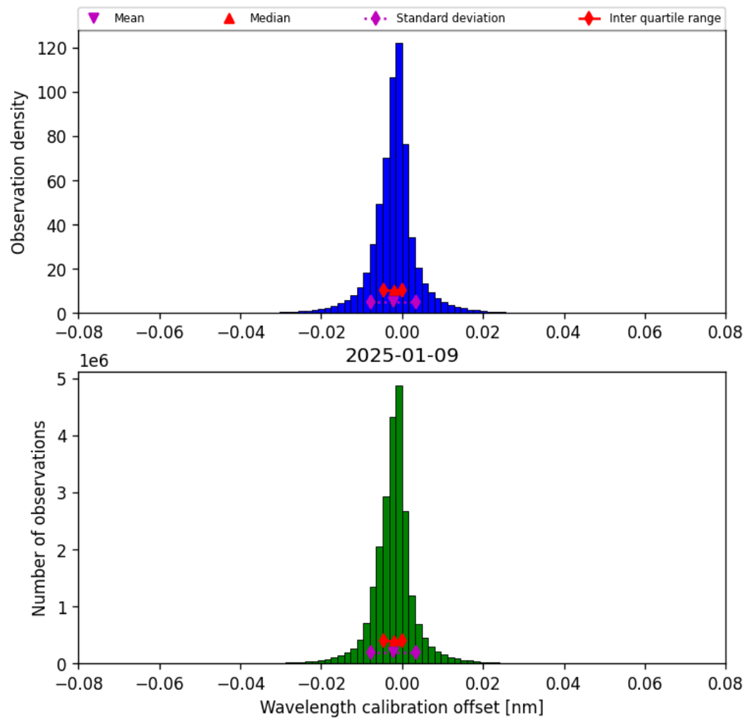
Figure 33: Histogram of “Wavelength calibration offset” for 2025-01-09 to 2025-01-10
