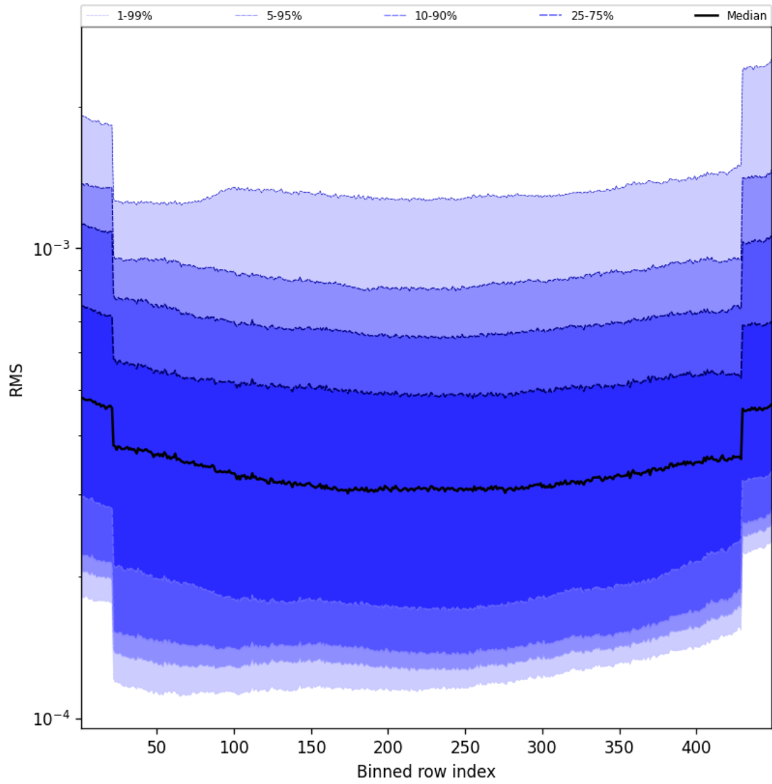
Figure 58: Along track statistics of “RMS” for 2025-01-09 to 2025-01-10
