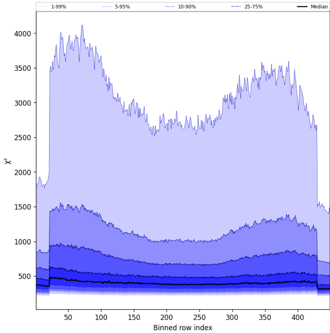
Figure 57: Along track statistics of “ \chi^2 ” for 2025-01-09 to 2025-01-10
