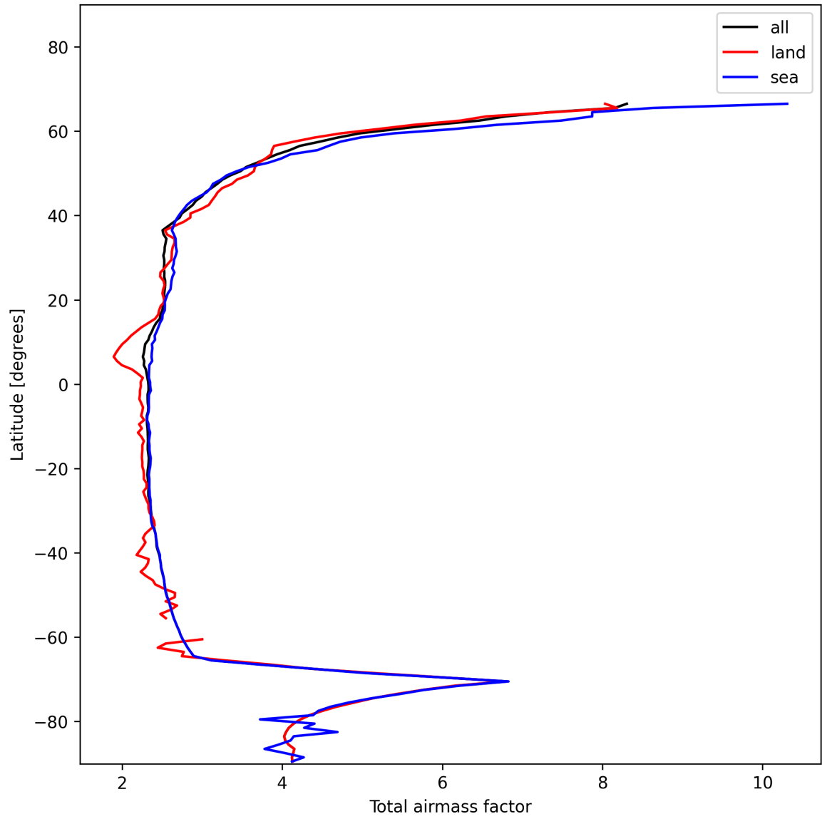
Figure 13: Zonal average of “Total airmass factor” for 2025-01-09 to 2025-01-10.
