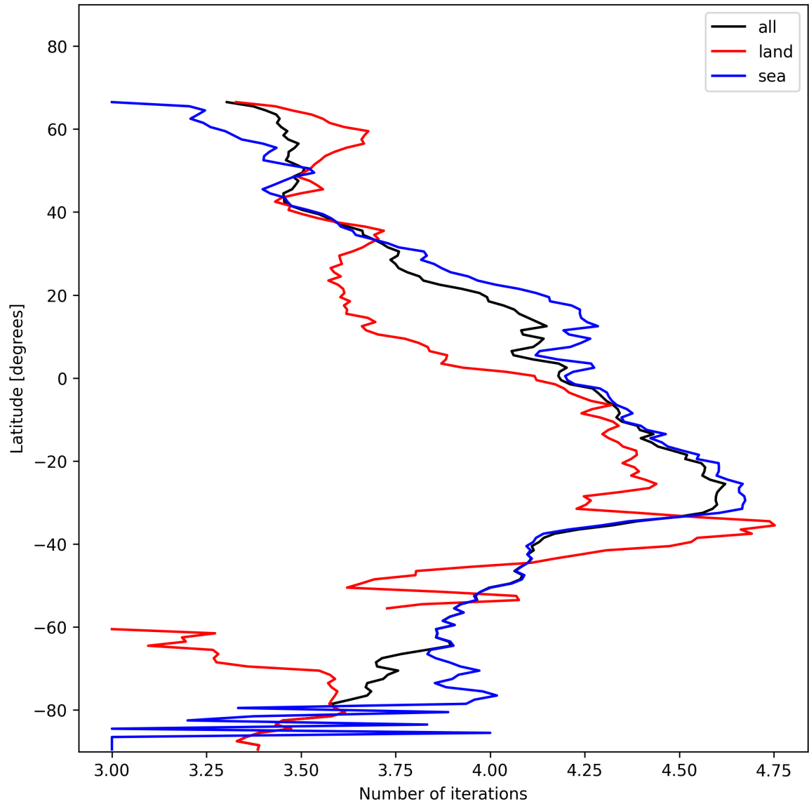
Figure 15: Zonal average of “Number of iterations” for 2025-01-09 to 2025-01-10.
