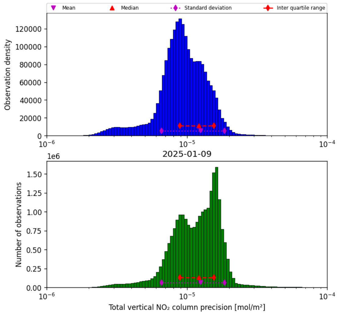
Figure 37: Histogram of “Total vertical NO 2 column precision” for 2025-01-09 to 2025-01-10
