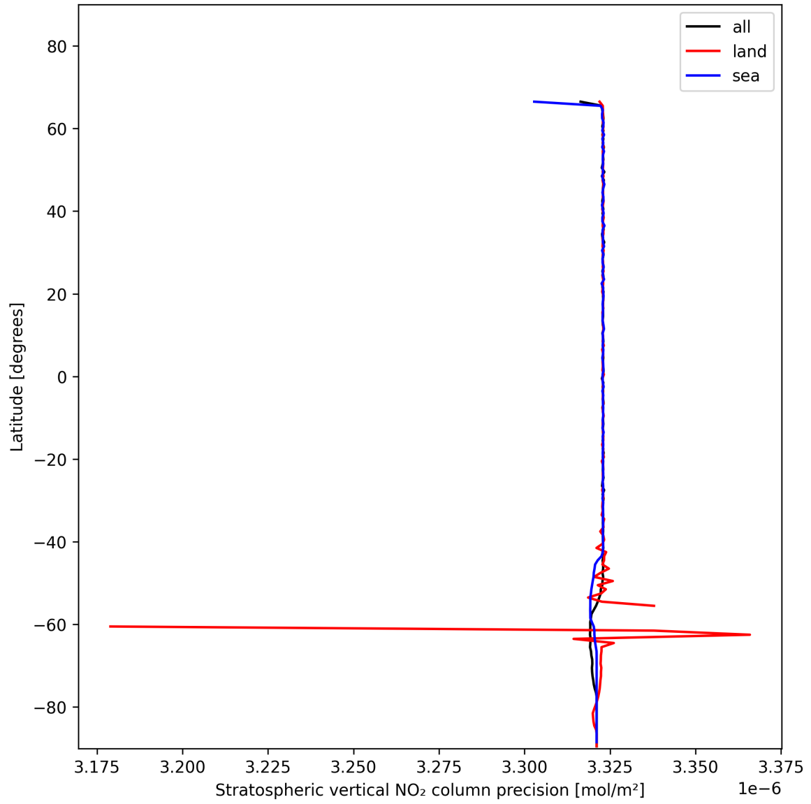
Figure 18: Zonal average of "Stratospheric vertical NO 2 column precision" for 2025-01-11 to 2025-01-12.
