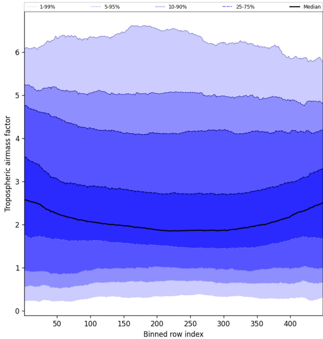
Figure 46: Along track statistics of “Tropospheric airmass factor” for 2025-01-11 to 2025-01-12
