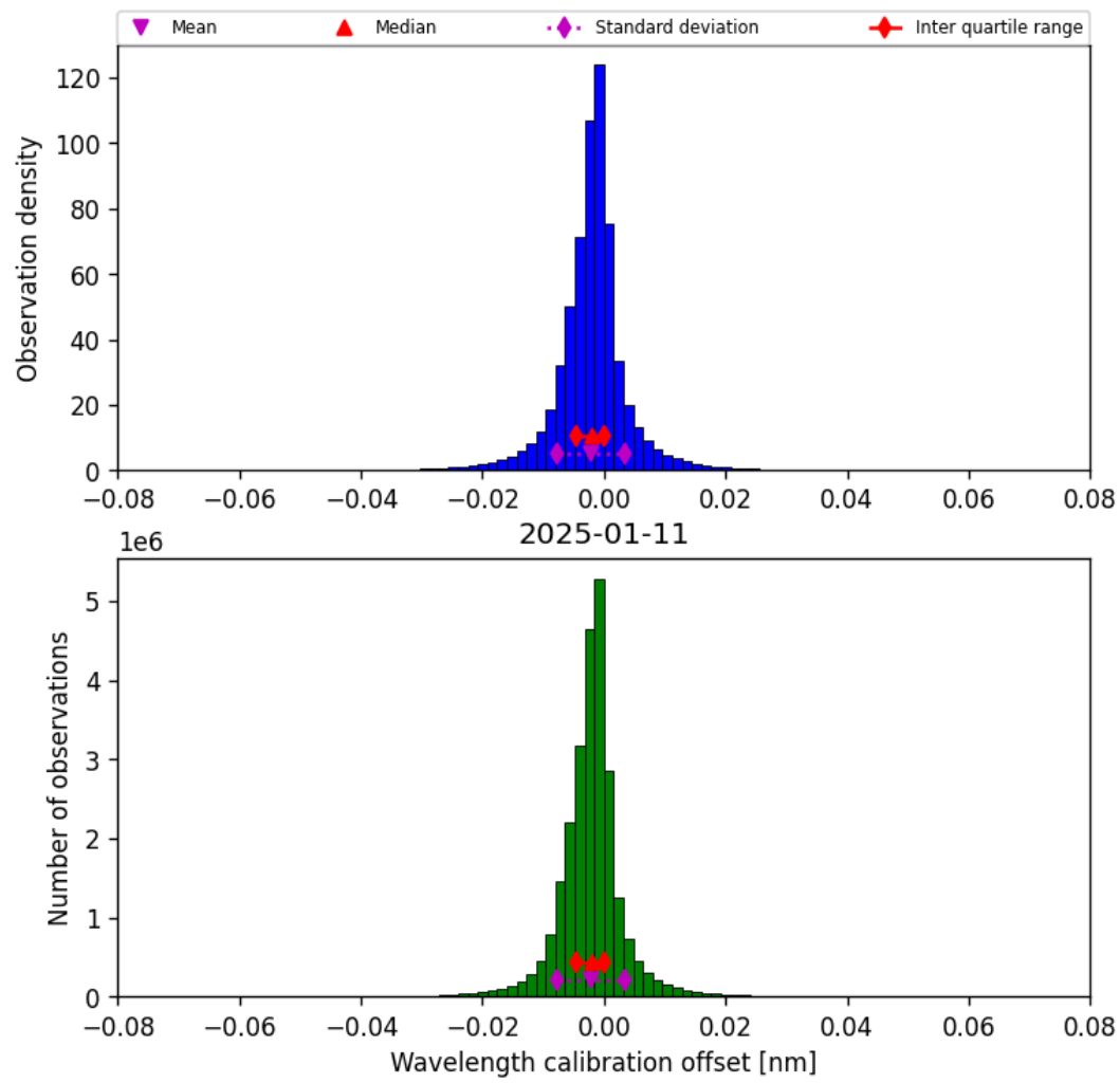
Figure 33: Histogram of “Wavelength calibration offset” for 2025-01-11 to 2025-01-12
