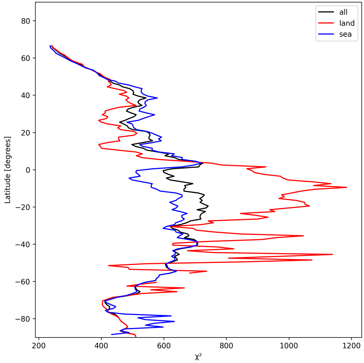
Figure 23: Zonal average of “ \chi^2 ” for 2025-01-11 to 2025-01-12.
