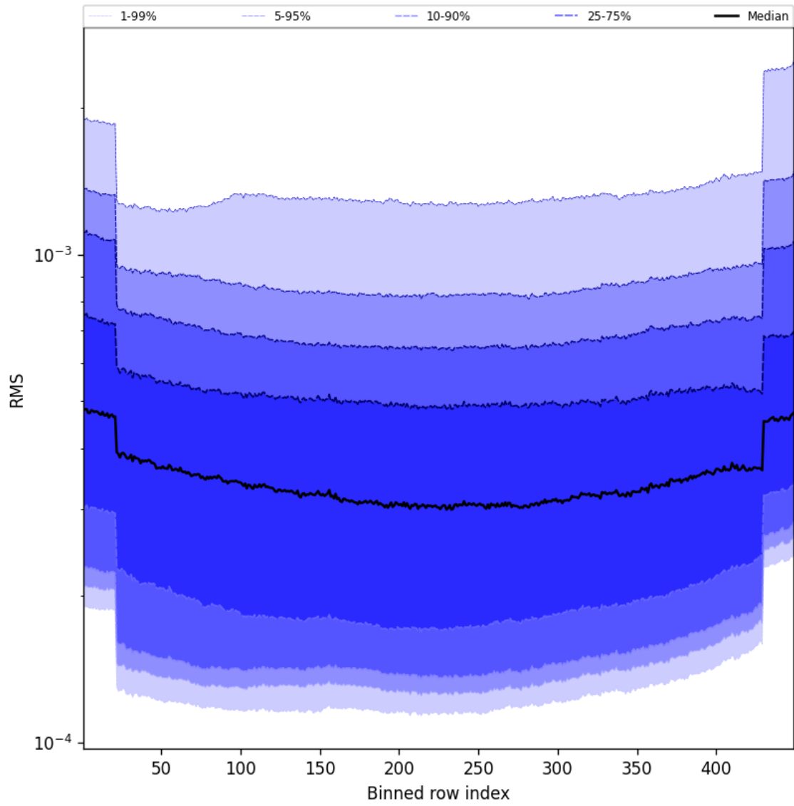
Figure 58: Along track statistics of “RMS” for 2025-01-11 to 2025-01-12
