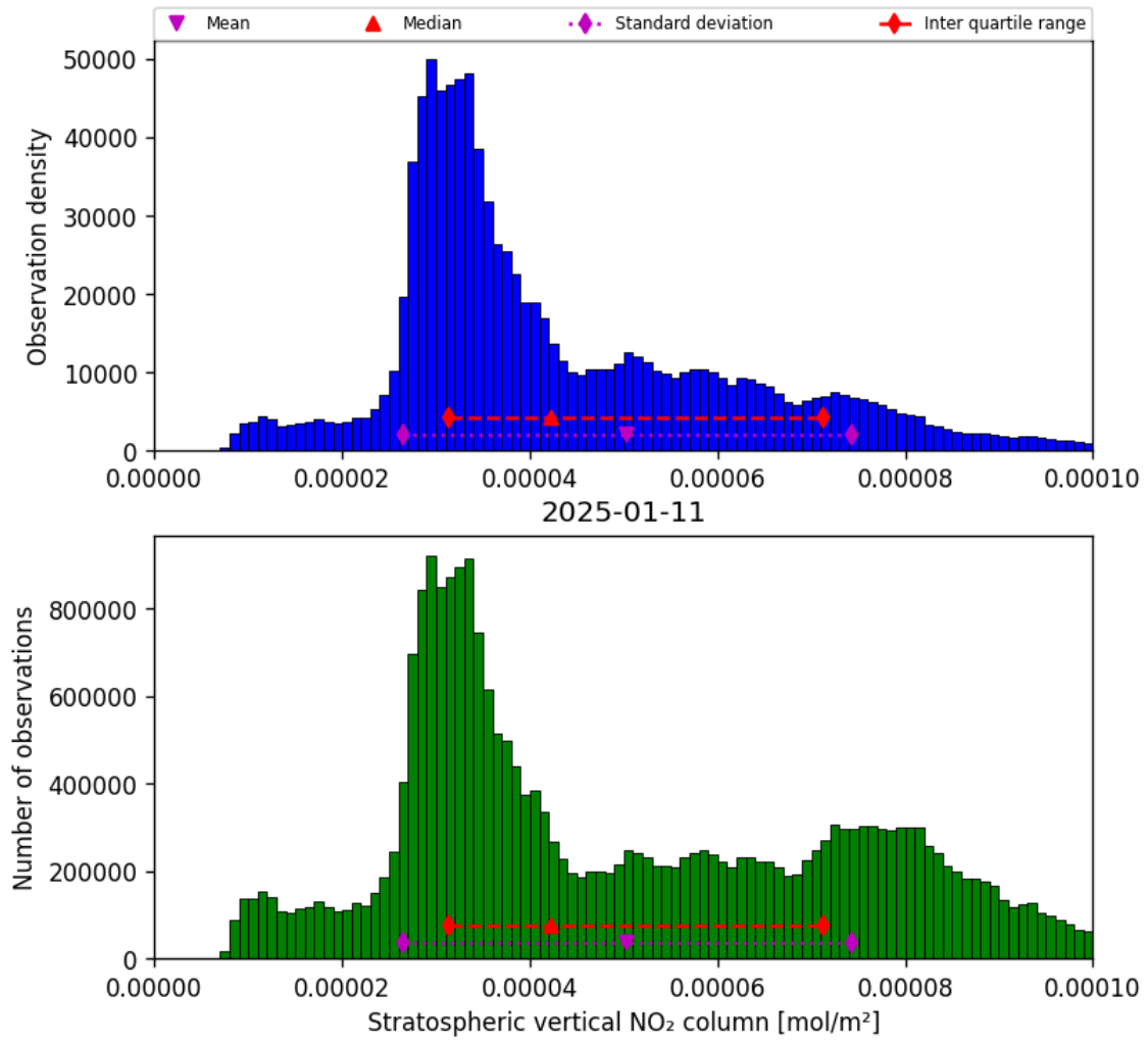
Figure 34: Histogram of “Stratospheric vertical NO 2 column” for 2025-01-11 to 2025-01-12
