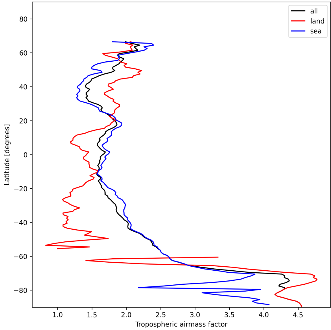
Figure 12: Zonal average of “Tropospheric airmass factor” for 2025-01-11 to 2025-01-12.
