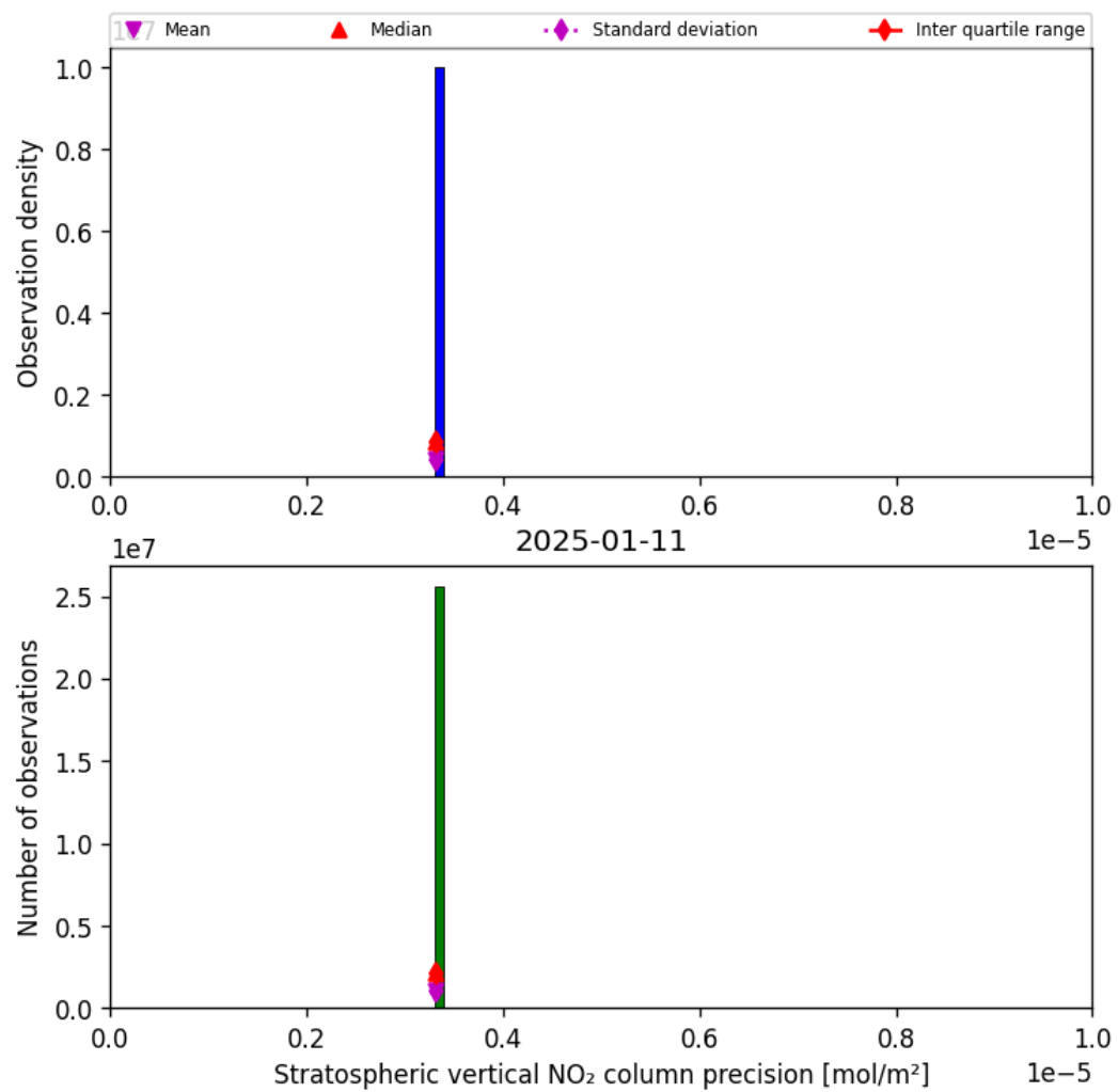
Figure 35: Histogram of “Stratospheric vertical NO 2 column precision” for 2025-01-11 to 2025-01-12
