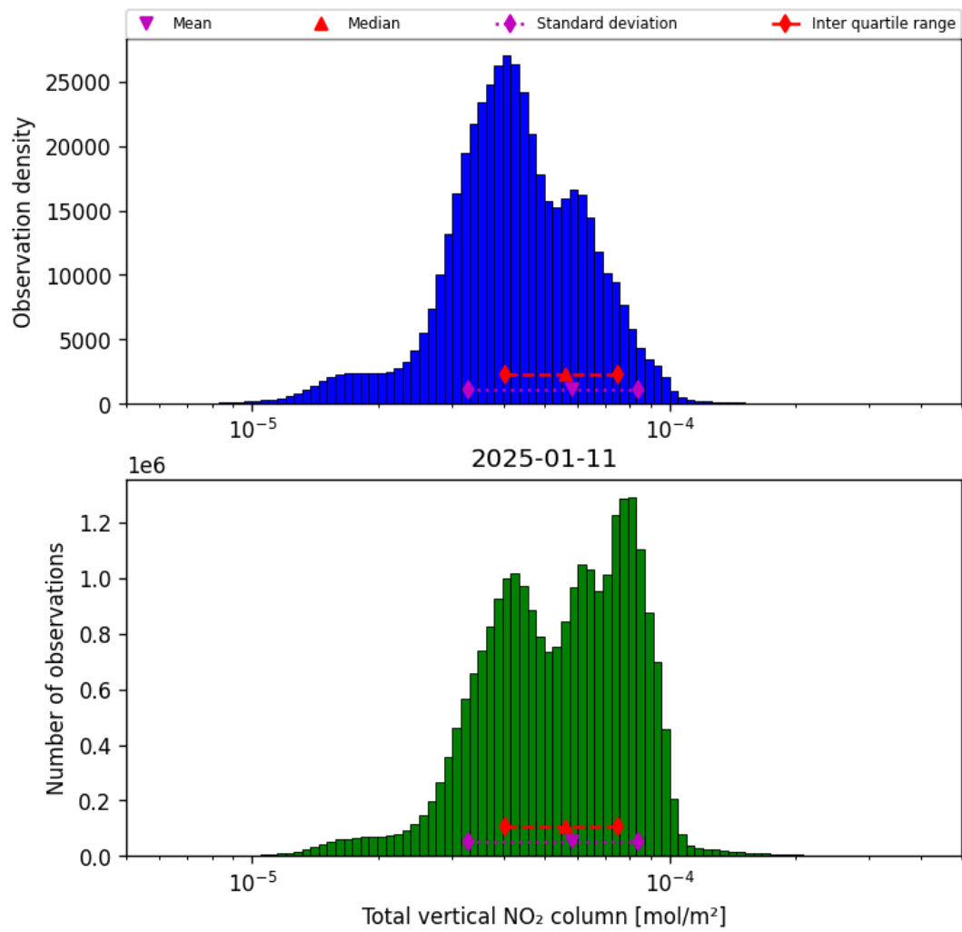
Figure 36: Histogram of “Total vertical NO 2 column” for 2025-01-11 to 2025-01-12
