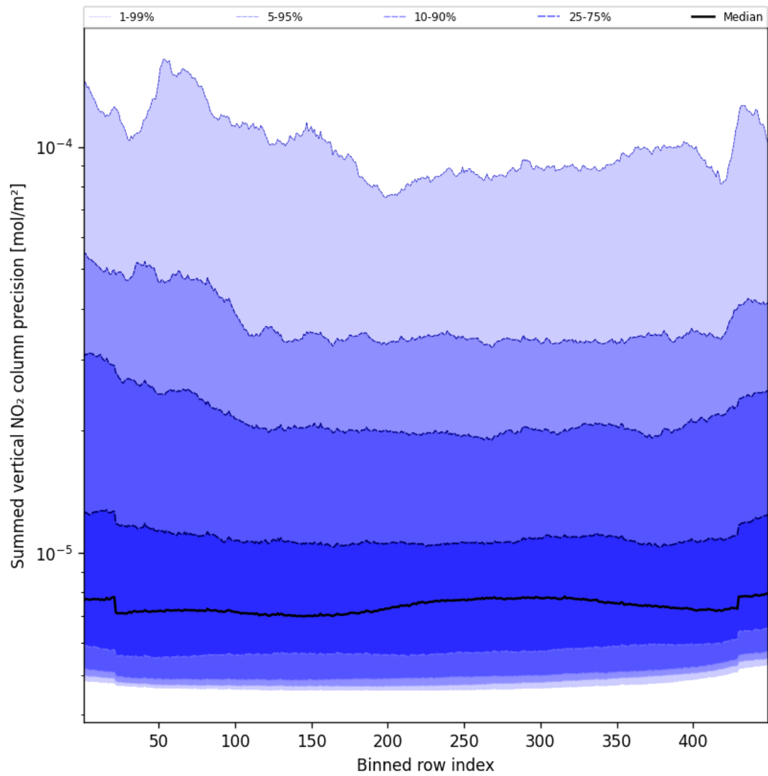
Figure 56: Along track statistics of “Summed vertical NO 2 column precision” for 2025-01-11 to 2025-01-12
