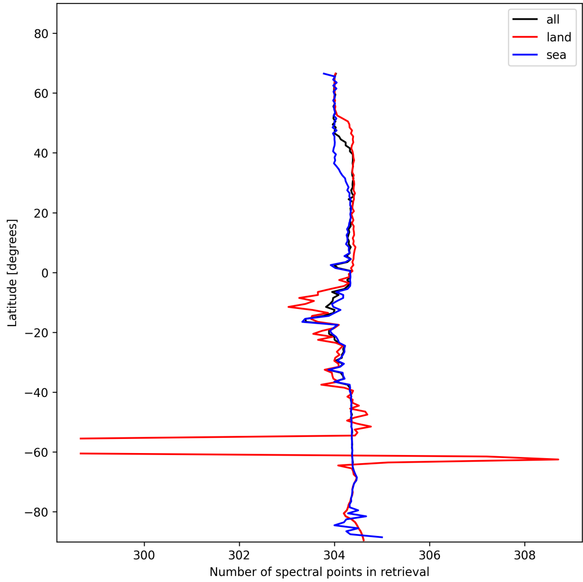
Figure 14: Zonal average of “Number of spectral points in retrieval” for 2025-01-11 to 2025-01-12.
