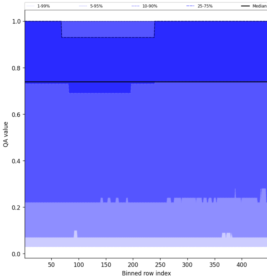
Figure 43: Along track statistics of “QA value” for 2025-01-11 to 2025-01-12
