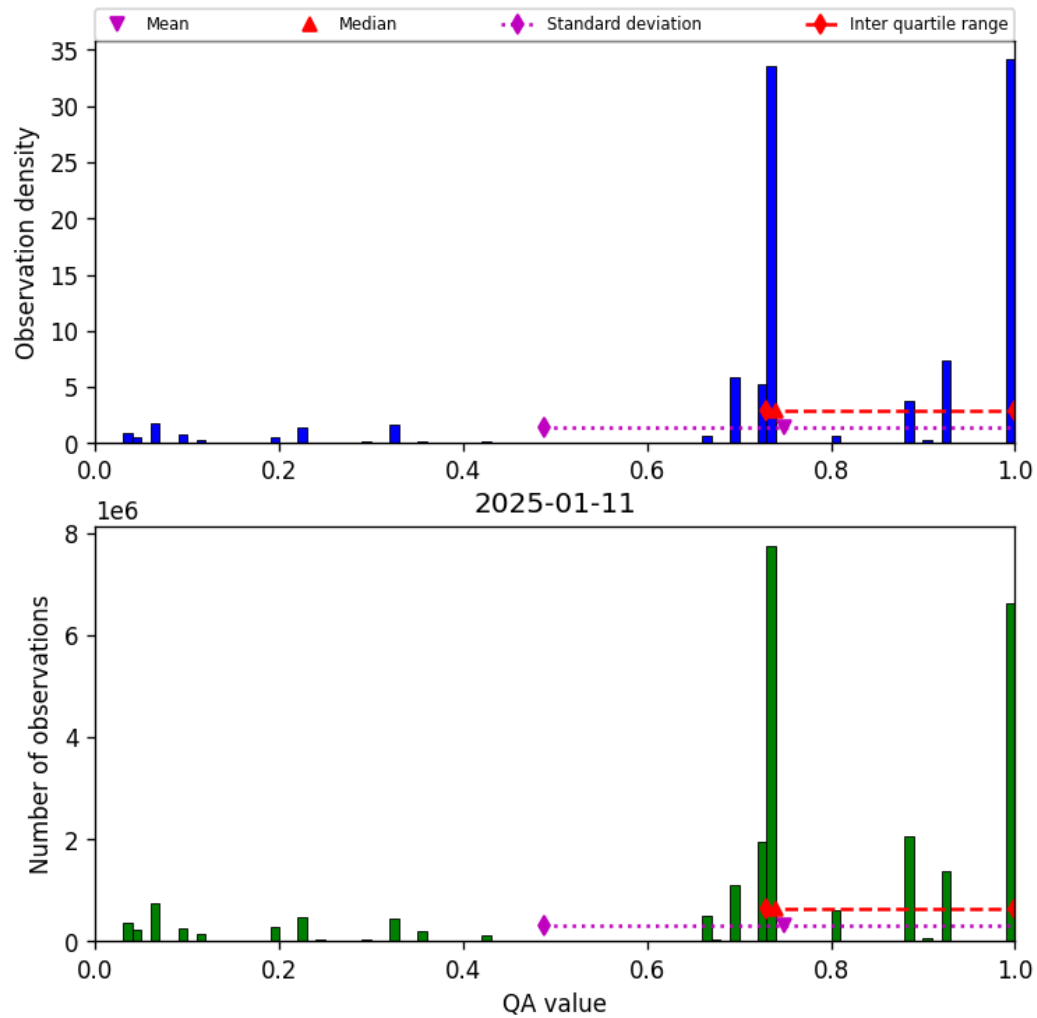
Figure 26: Histogram of “QA value” for 2025-01-11 to 2025-01-12
