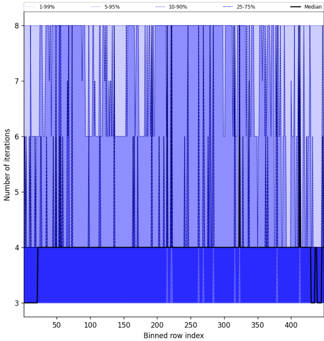
Figure 49: Along track statistics of “Number of iterations” for 2025-01-11 to 2025-01-12
