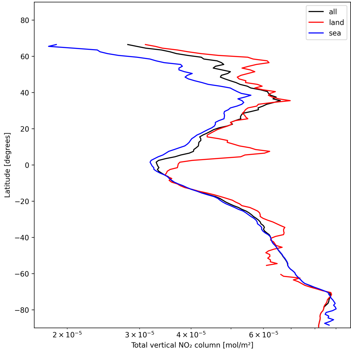
Figure 19: Zonal average of “Total vertical NO 2 column” for 2025-01-11 to 2025-01-12.
