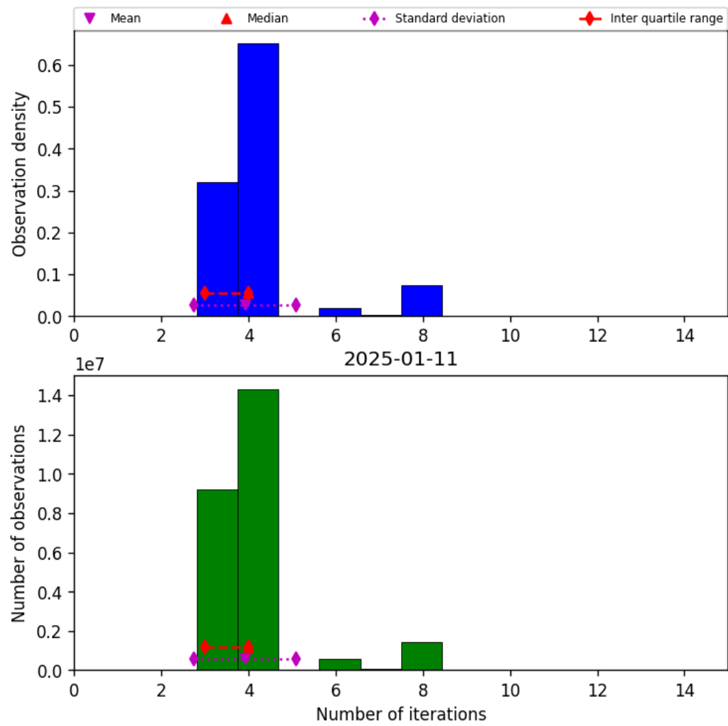
Figure 32: Histogram of “Number of iterations” for 2025-01-11 to 2025-01-12
