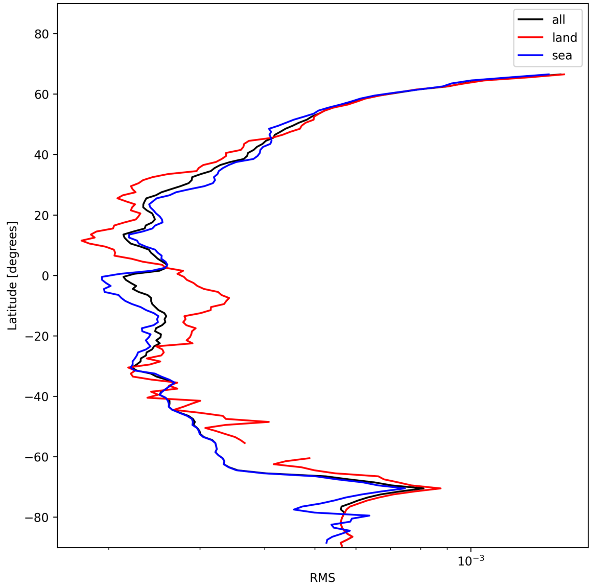
Figure 24: Zonal average of “RMS” for 2025-01-11 to 2025-01-12.
