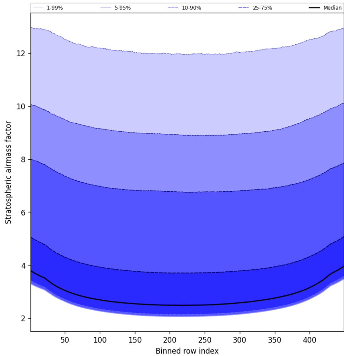
Figure 59: Along track statistics of “Stratospheric airmass factor” for 2025-01-11 to 2025-01-12
