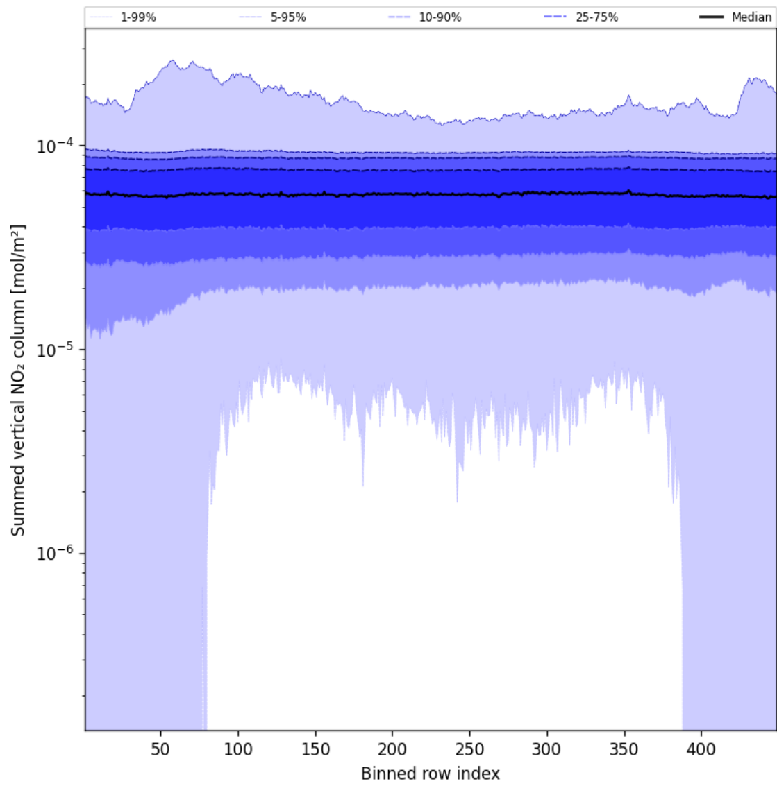
Figure 55: Along track statistics of “Summed vertical NO 2 column” for 2025-01-11 to 2025-01-12
