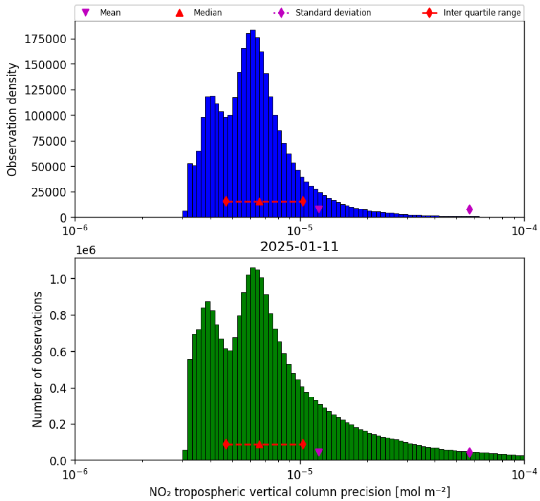
Figure 28: Histogram of “NO 2 tropospheric vertical column precision” for 2025-01-11 to 2025-01-12
