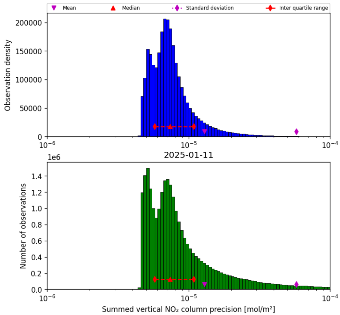
Figure 39: Histogram of “Summed vertical NO 2 column precision” for 2025-01-11 to 2025-01-12
