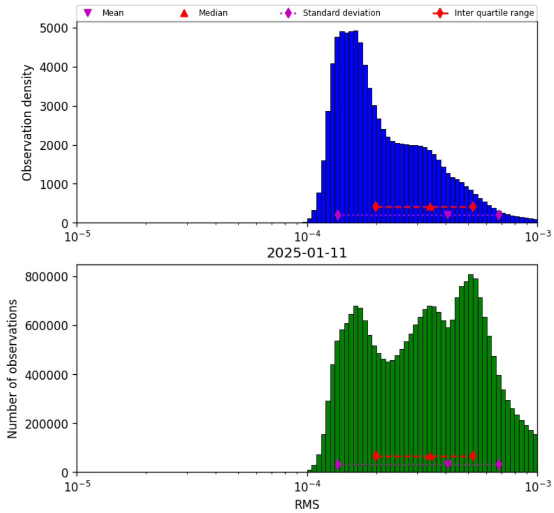
Figure 41: Histogram of “RMS” for 2025-01-11 to 2025-01-12
