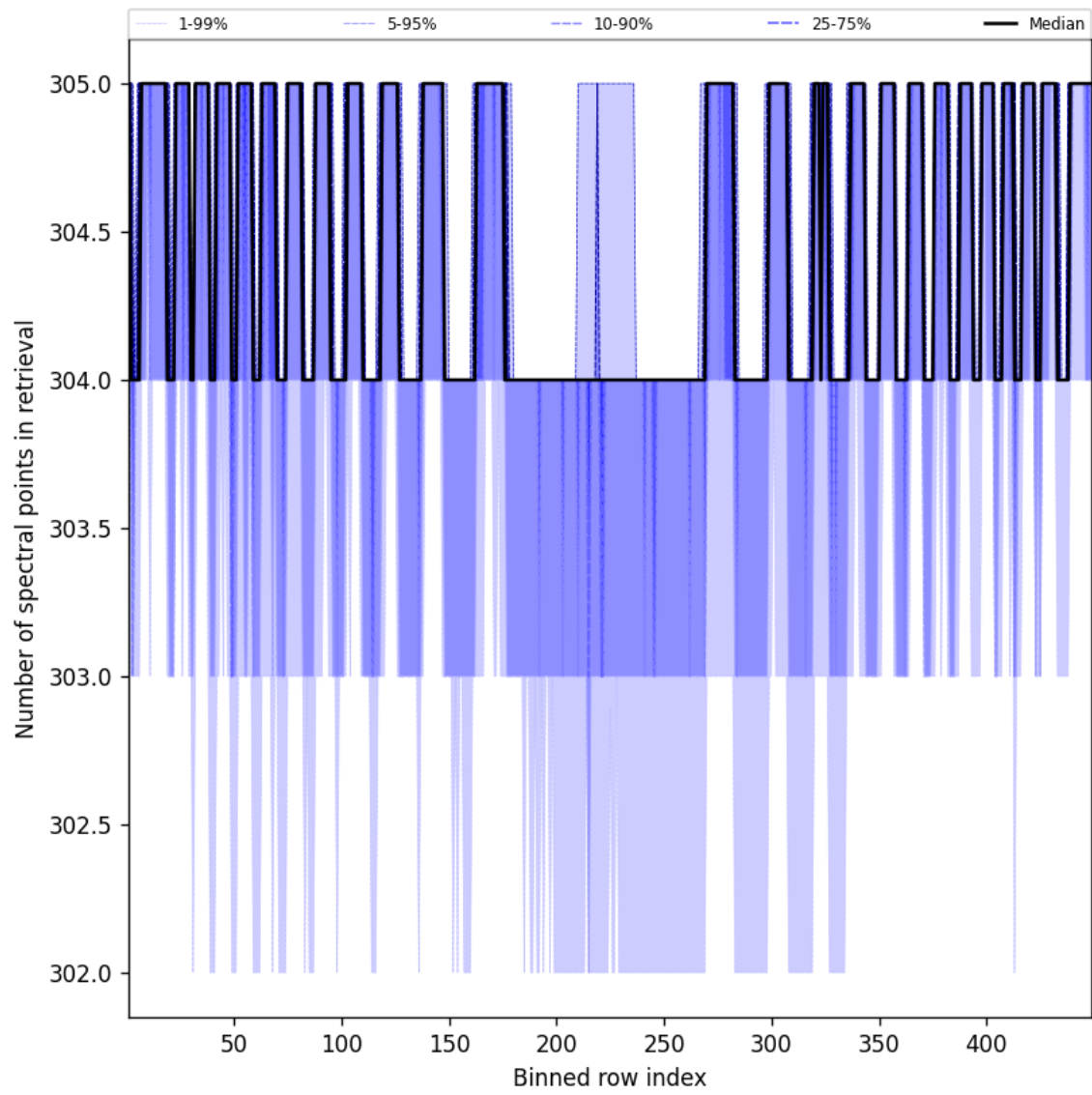
Figure 48: Along track statistics of “Number of spectral points in retrieval” for 2025-01-11 to 2025-01-12
