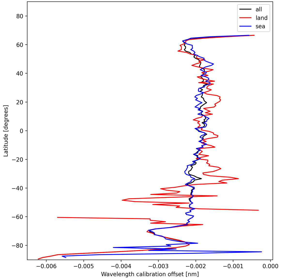
Figure 16: Zonal average of “Wavelength calibration offset” for 2025-01-11 to 2025-01-12.
