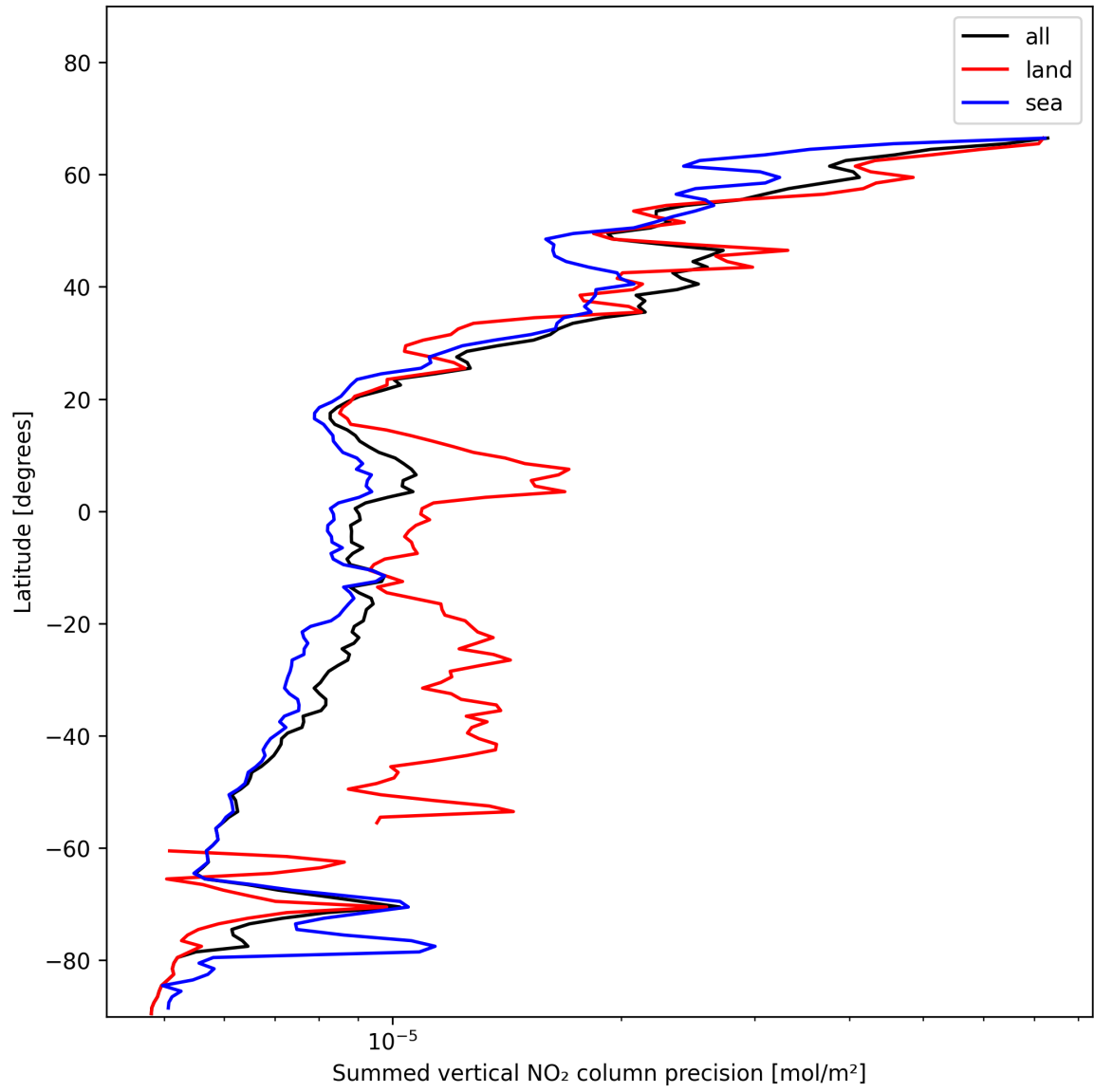
Figure 22: Zonal average of “Summed vertical NO 2 column precision” for 2025-01-11 to 2025-01-12.
