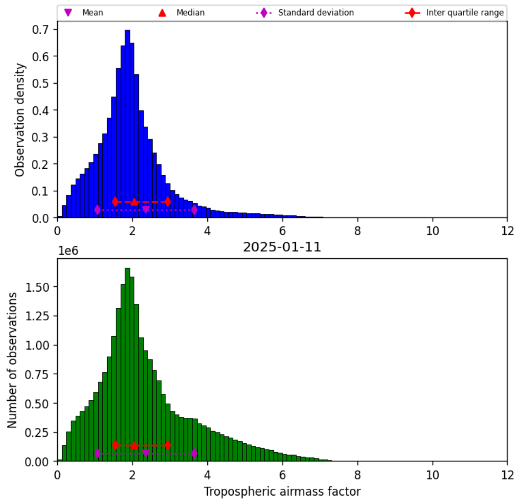
Figure 29: Histogram of “Tropospheric airmass factor” for 2025-01-11 to 2025-01-12
