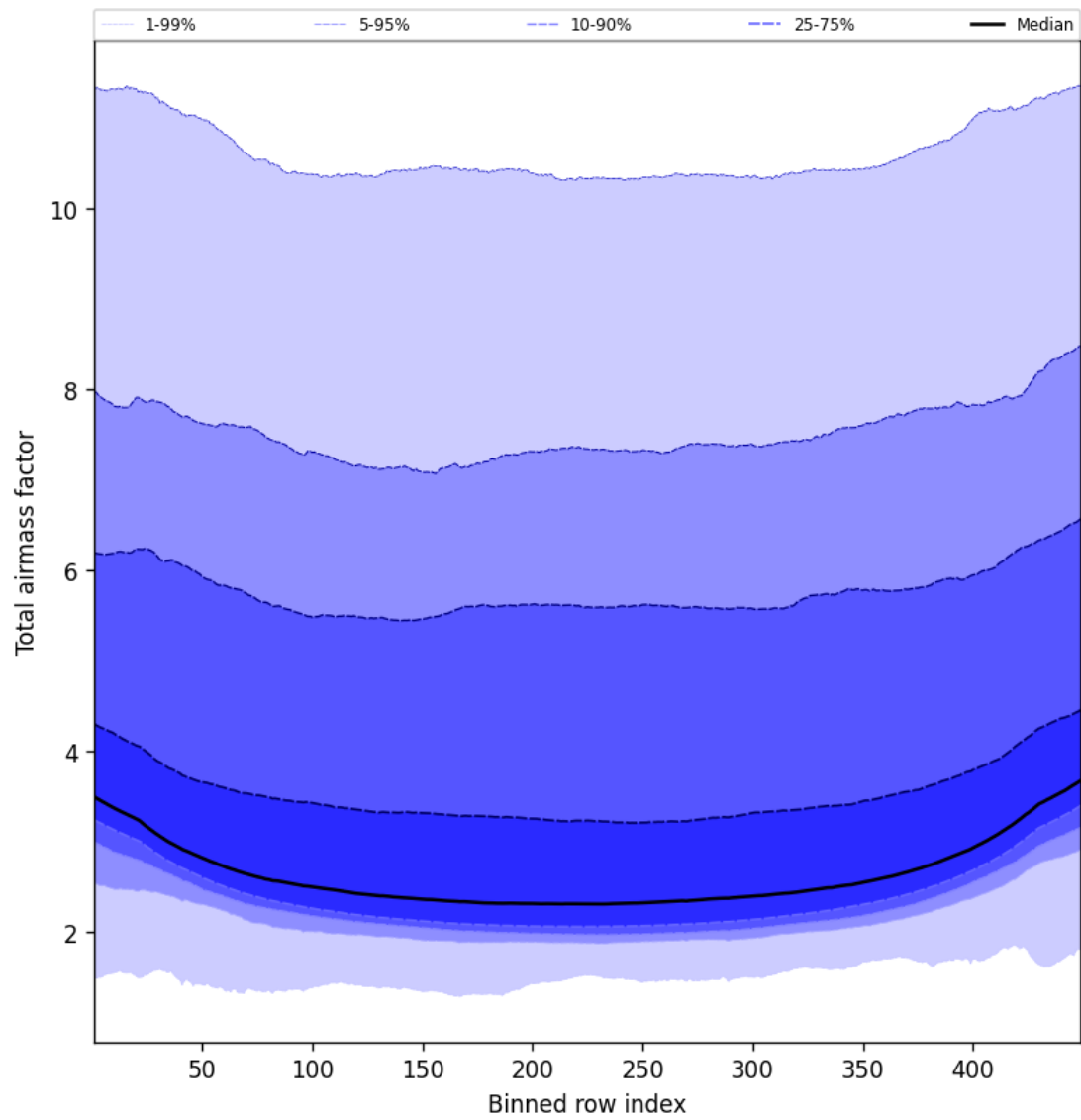
Figure 47: Along track statistics of “Total airmass factor” for 2025-01-11 to 2025-01-12
