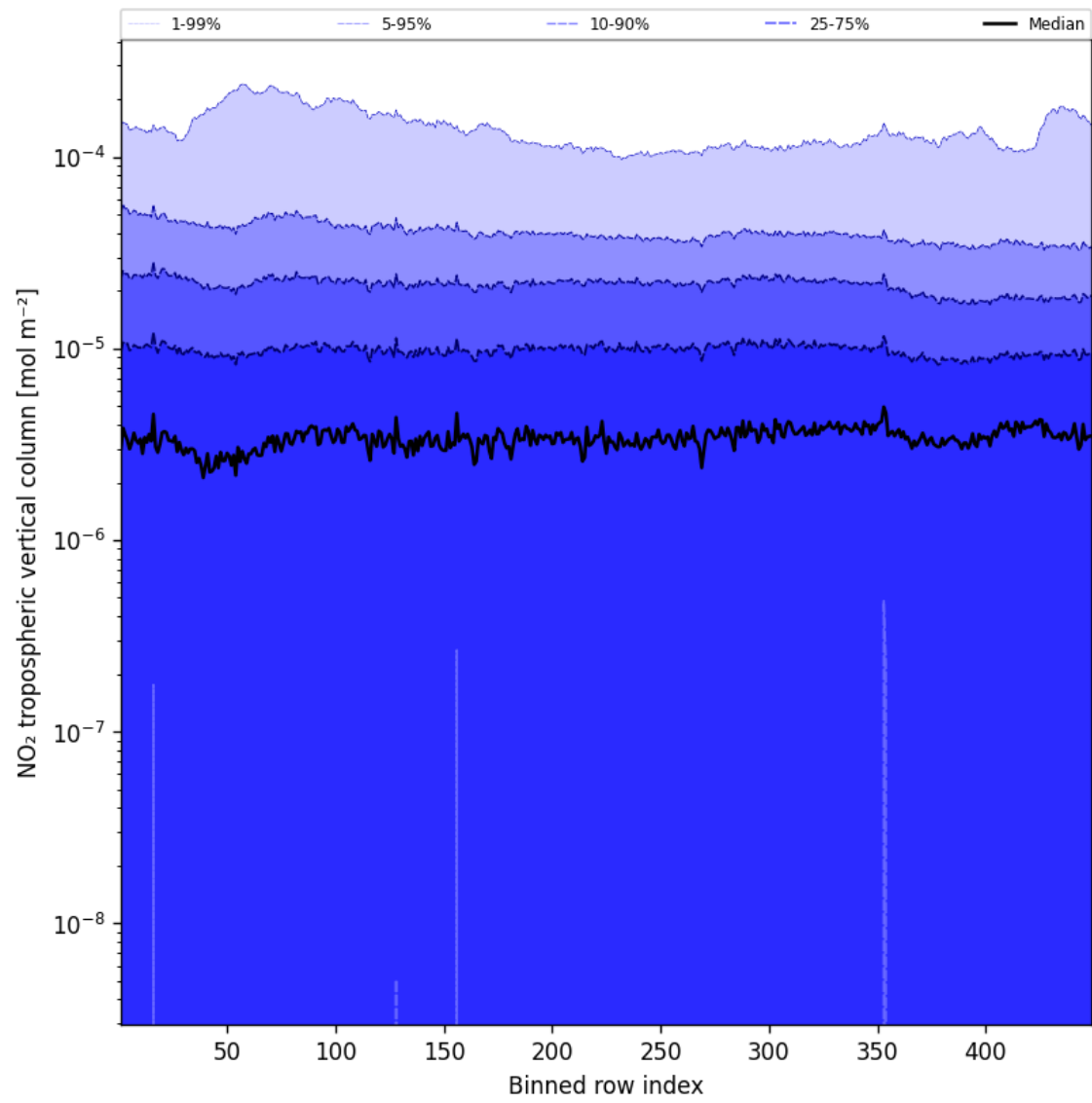
Figure 44: Along track statistics of “NO 2 tropospheric vertical column” for 2025-01-11 to 2025-01-12
