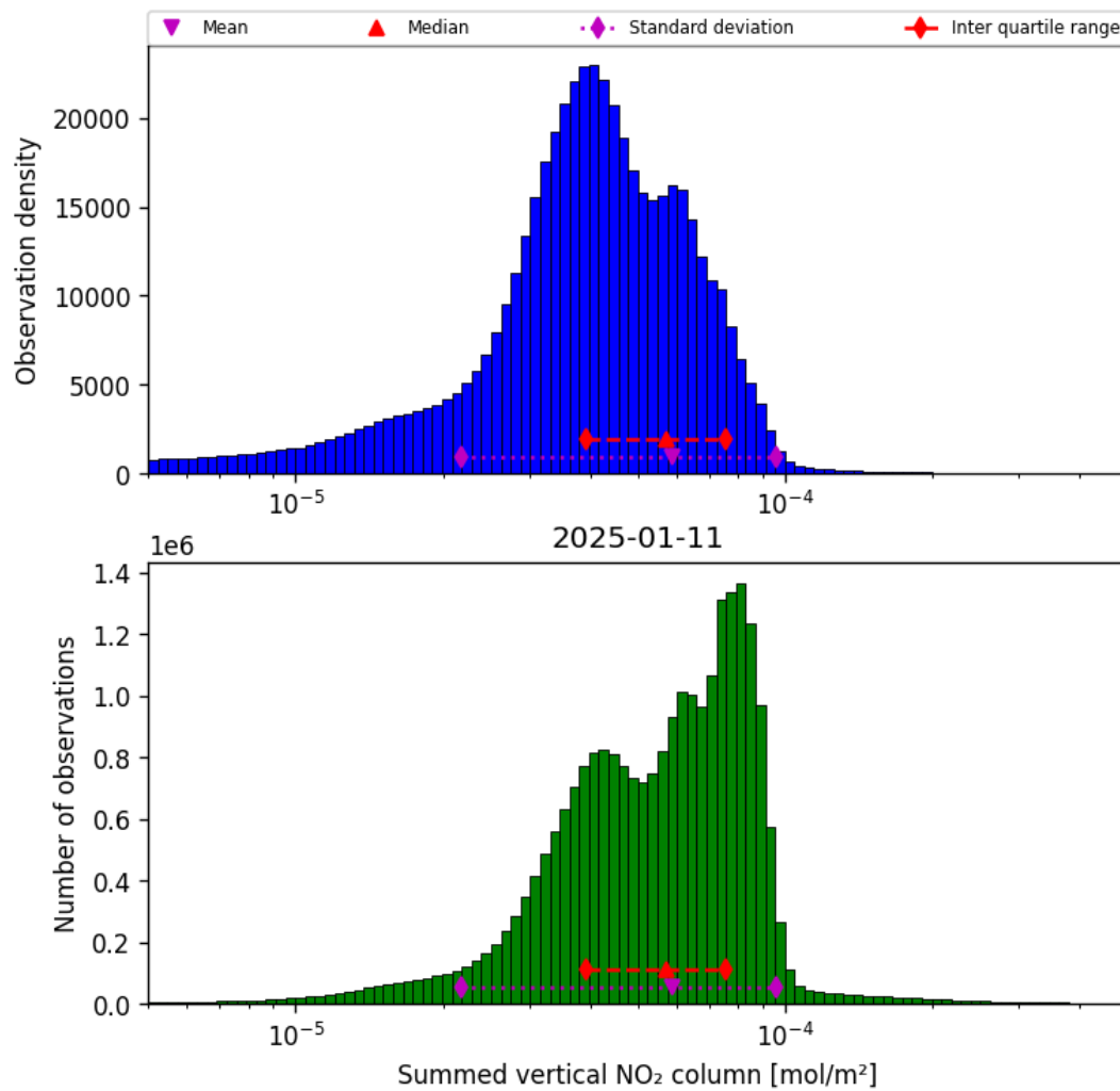
Figure 38: Histogram of “Summed vertical NO 2 column” for 2025-01-11 to 2025-01-12
