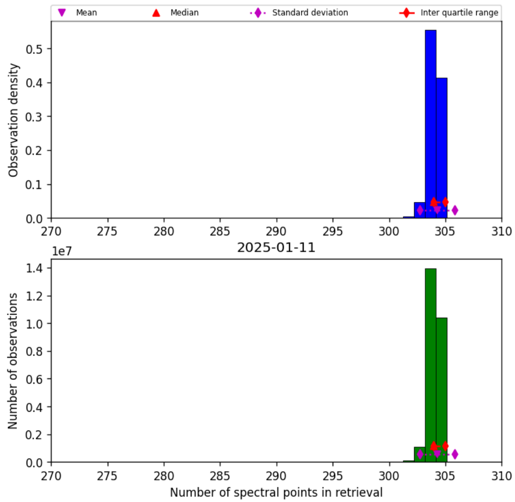
Figure 31: Histogram of “Number of spectral points in retrieval” for 2025-01-11 to 2025-01-12
