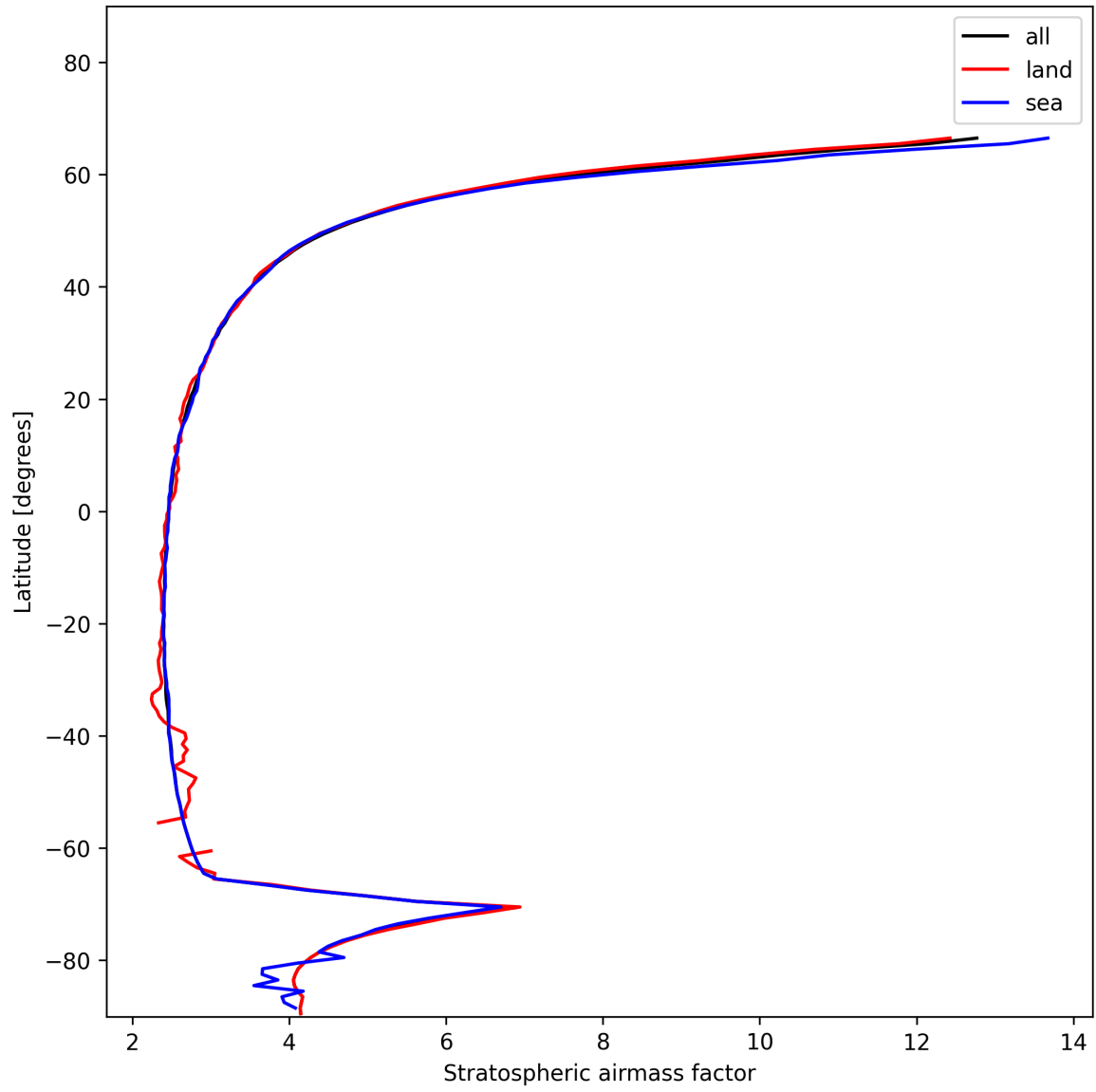
Figure 25: Zonal average of “Stratospheric airmass factor” for 2025-01-11 to 2025-01-12.
