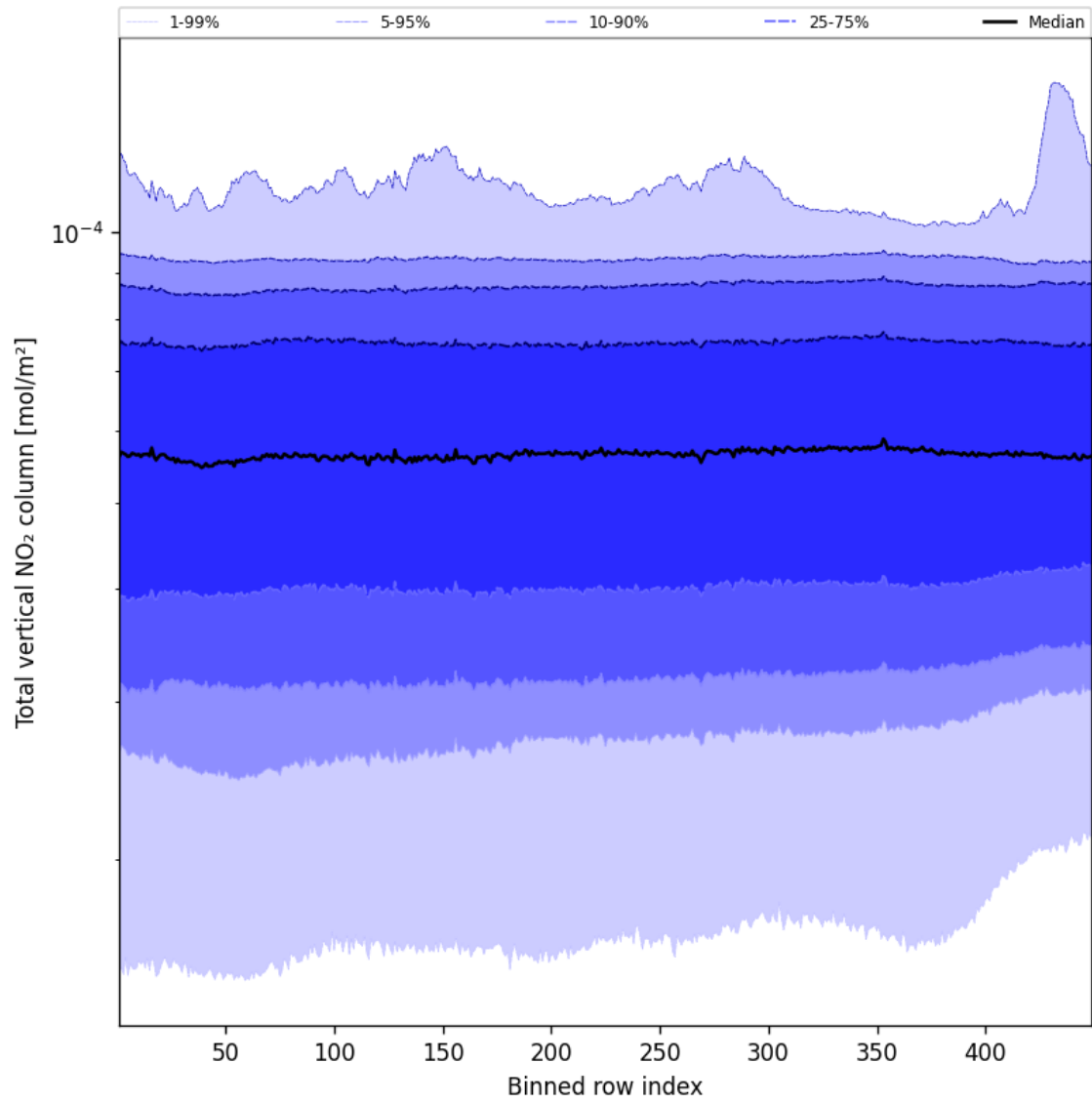
Figure 53: Along track statistics of “Total vertical NO 2 column” for 2025-01-11 to 2025-01-12
