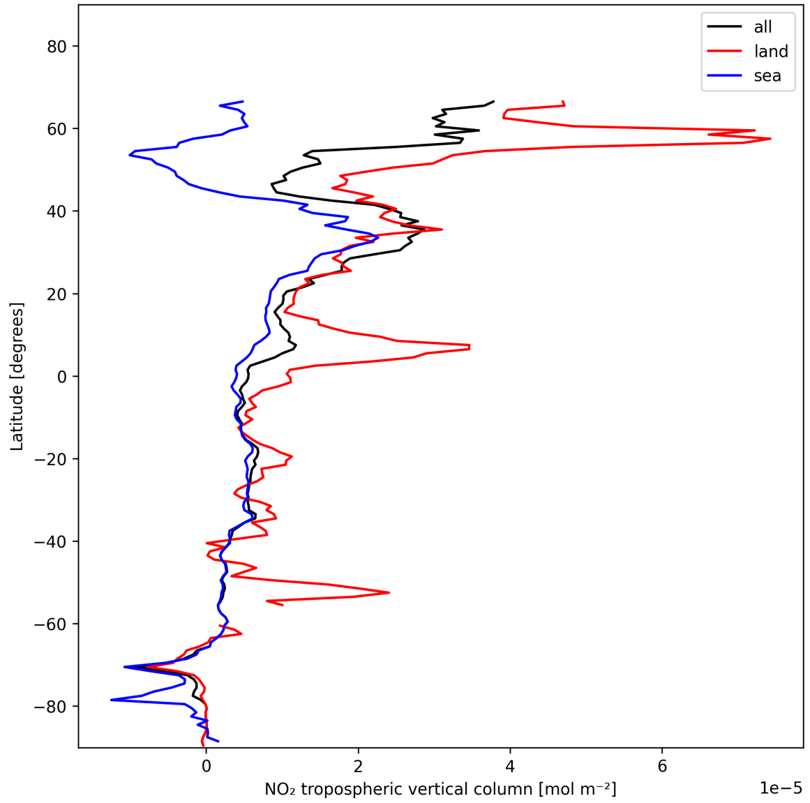
Figure 10: Zonal average of “NO 2 tropospheric vertical column” for 2025-01-11 to 2025-01-12.
