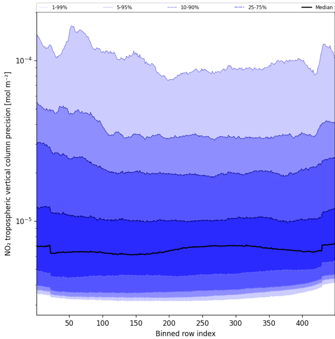
Figure 45: Along track statistics of “NO 2 tropospheric vertical column precision” for 2025-01-11 to 2025-01-12
