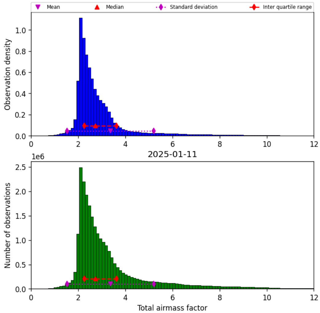
Figure 30: Histogram of “Total airmass factor” for 2025-01-11 to 2025-01-12
