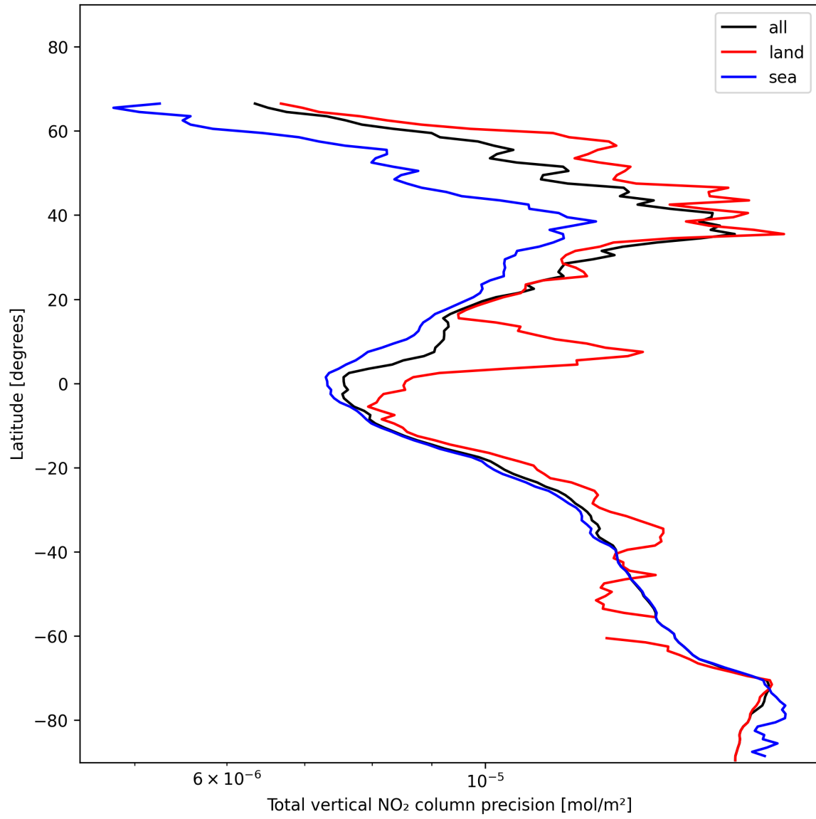
Figure 20: Zonal average of “Total vertical NO 2 column precision” for 2025-01-11 to 2025-01-12.
