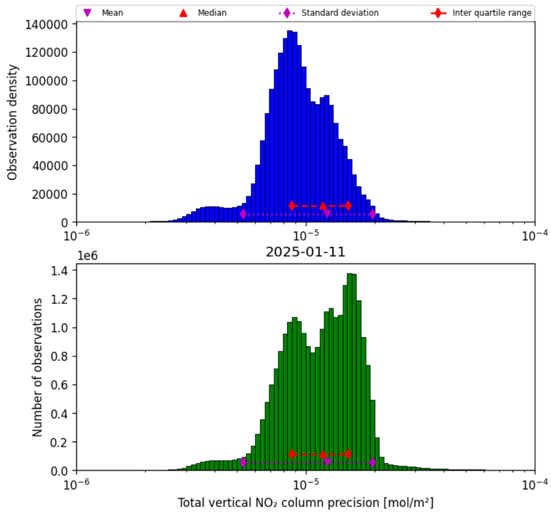
Figure 37: Histogram of “Total vertical NO 2 column precision” for 2025-01-11 to 2025-01-12
