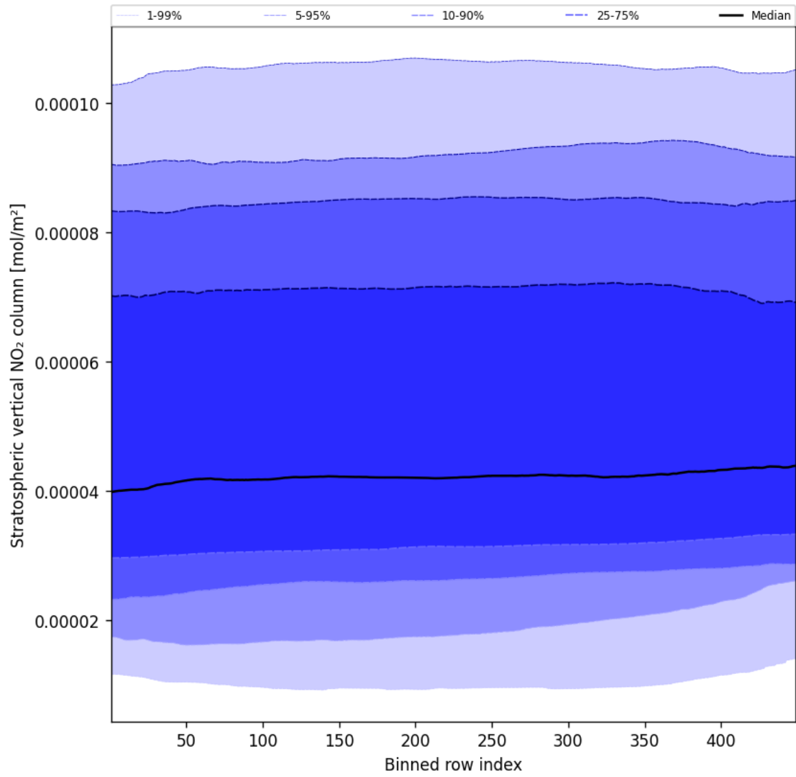
Figure 51: Along track statistics of “Stratospheric vertical NO 2 column” for 2025-01-11 to 2025-01-12
