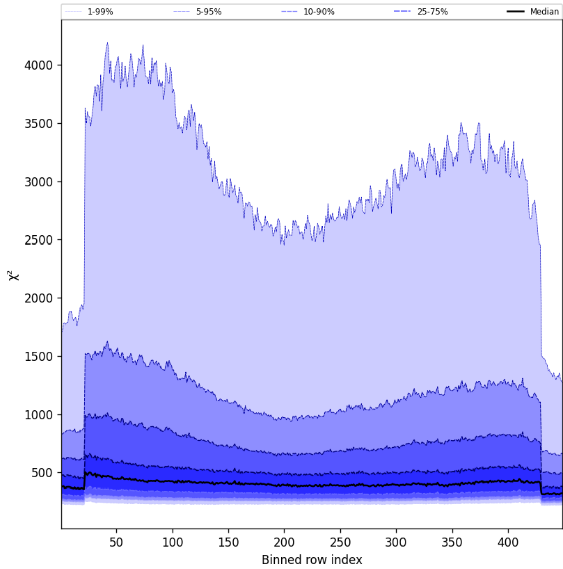
Figure 57: Along track statistics of “ \chi^2 ” for 2025-01-11 to 2025-01-12
