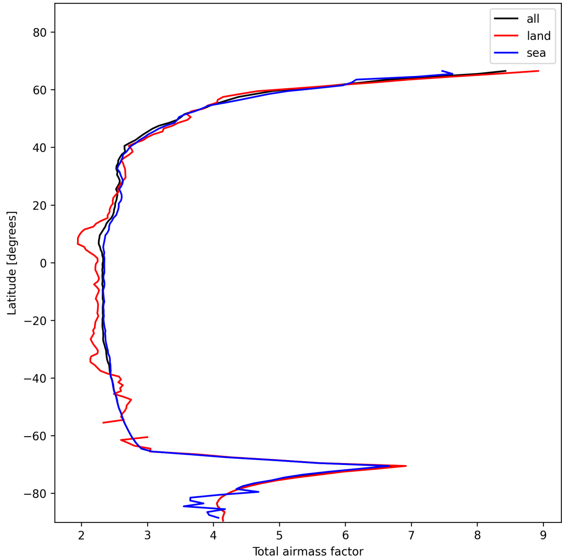
Figure 13: Zonal average of “Total airmass factor” for 2025-01-11 to 2025-01-12.
