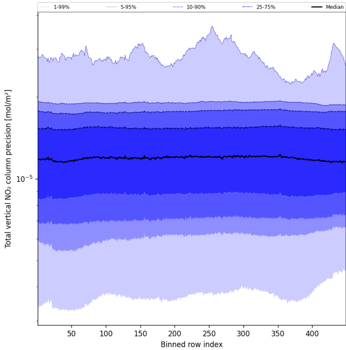
Figure 54: Along track statistics of “Total vertical NO 2 column precision” for 2025-01-11 to 2025-01-12
