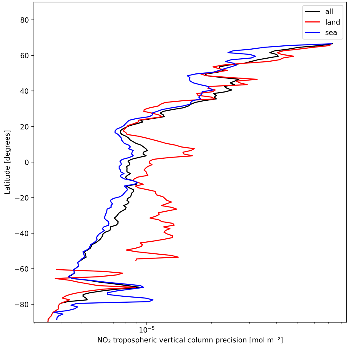
Figure 11: Zonal average of “NO 2 tropospheric vertical column precision” for 2025-01-11 to 2025-01-12.
