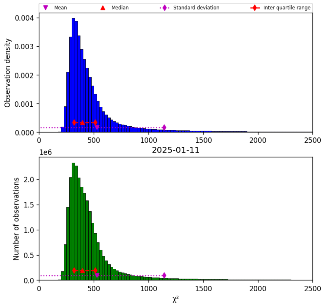
Figure 40: Histogram of “ \chi^2 ” for 2025-01-11 to 2025-01-12
