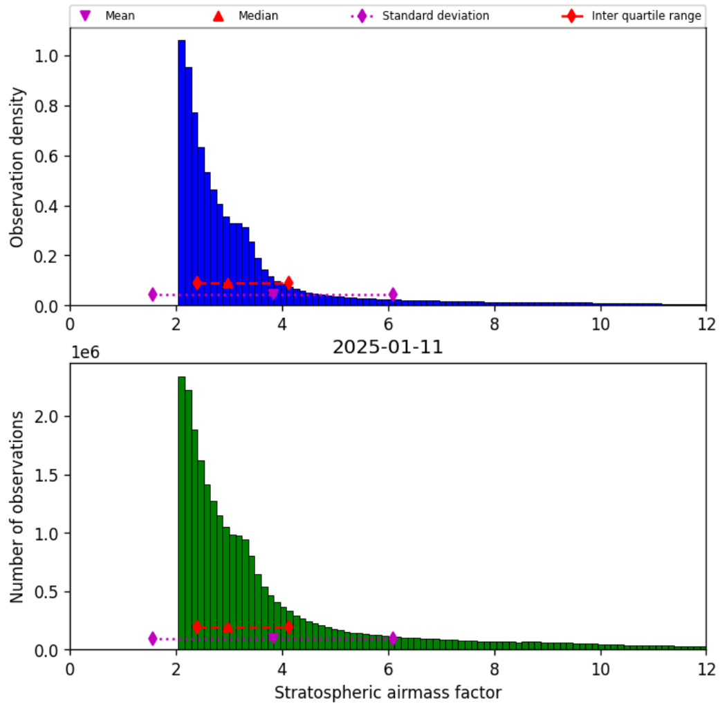
Figure 42: Histogram of “Stratospheric airmass factor” for 2025-01-11 to 2025-01-12
