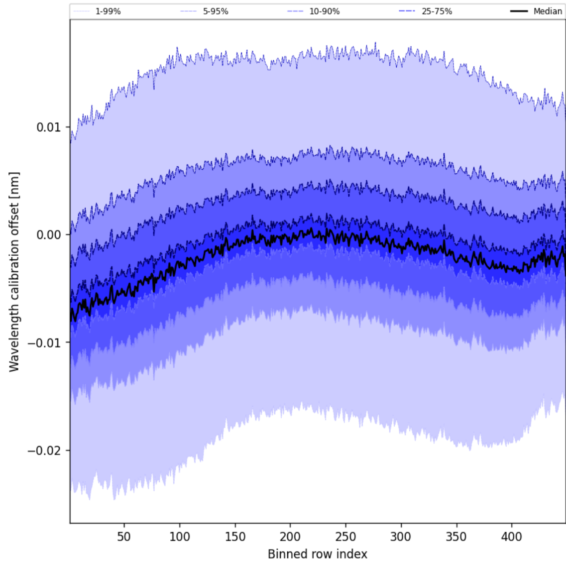
Figure 50: Along track statistics of “Wavelength calibration offset” for 2025-01-11 to 2025-01-12
