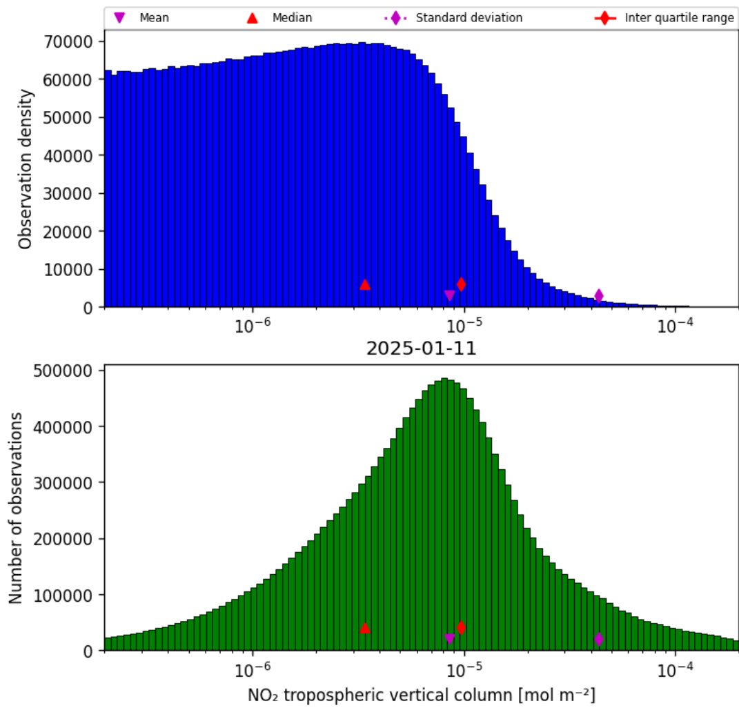
Figure 27: Histogram of “NO 2 tropospheric vertical column” for 2025-01-11 to 2025-01-12
