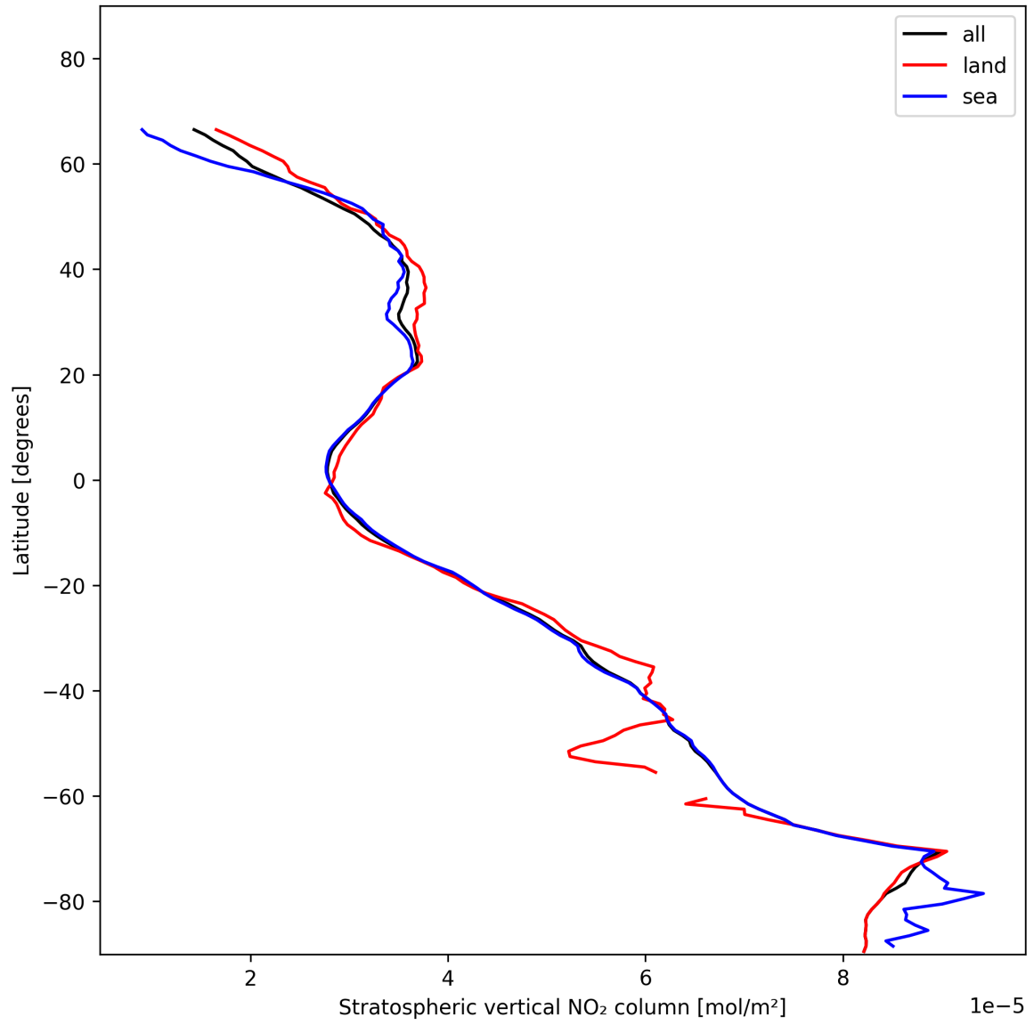
Figure 17: Zonal average of “Stratospheric vertical NO 2 column” for 2025-01-11 to 2025-01-12.
