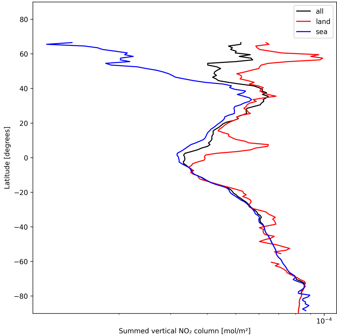
Figure 21: Zonal average of “Summed vertical NO 2 column” for 2025-01-11 to 2025-01-12.
