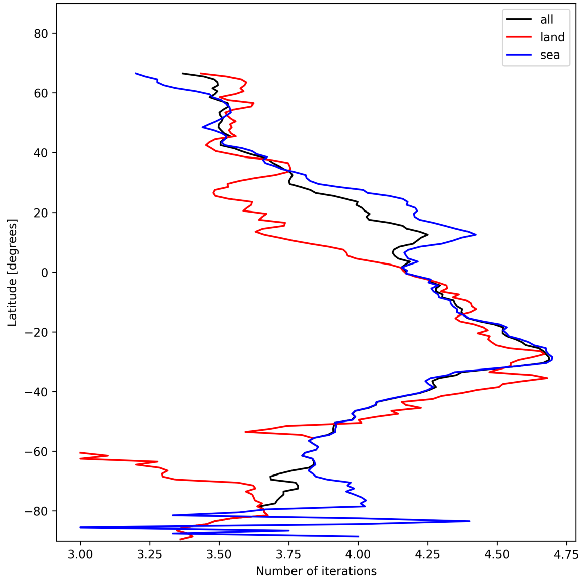
Figure 15: Zonal average of “Number of iterations” for 2025-01-11 to 2025-01-12.
