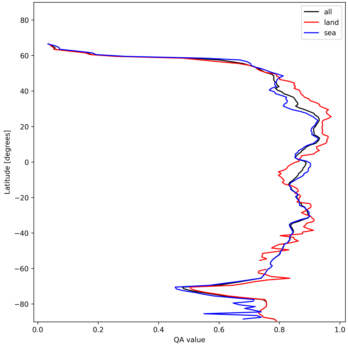
Figure 9: Zonal average of “QA value” for 2025-01-11 to 2025-01-12.
