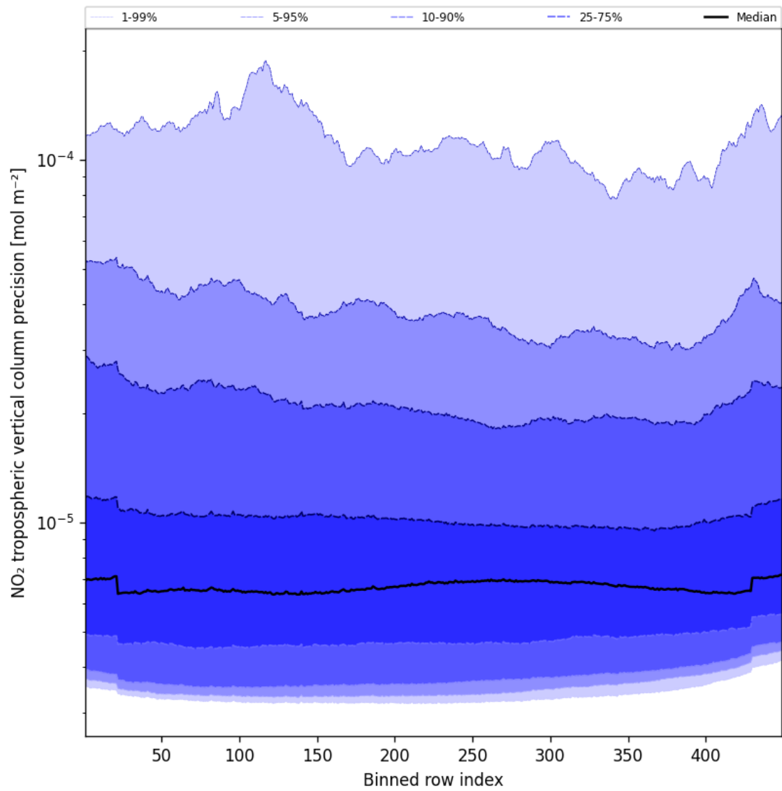
Figure 45: Along track statistics of “NO 2 tropospheric vertical column precision” for 2025-01-12 to 2025-01-13
