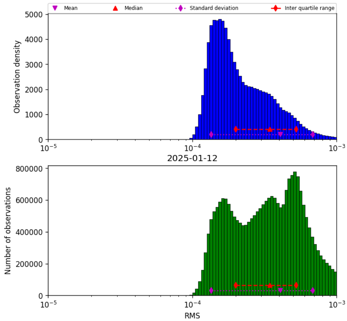
Figure 41: Histogram of “RMS” for 2025-01-12 to 2025-01-13
