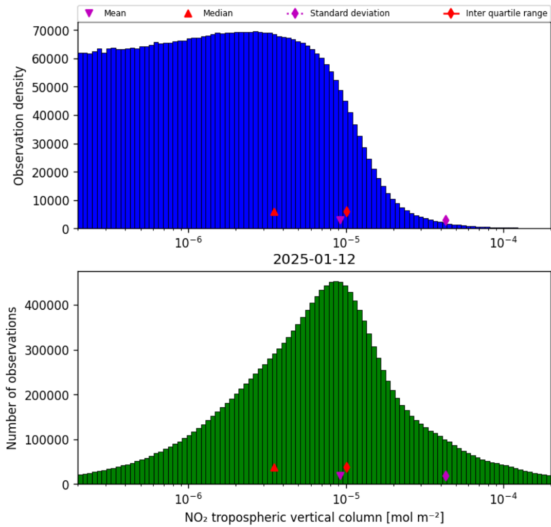
Figure 27: Histogram of “NO 2 tropospheric vertical column” for 2025-01-12 to 2025-01-13
