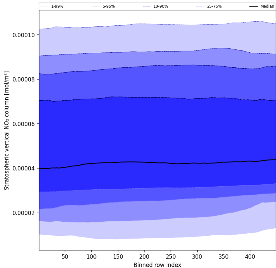
Figure 51: Along track statistics of “Stratospheric vertical NO 2 column” for 2025-01-12 to 2025-01-13
