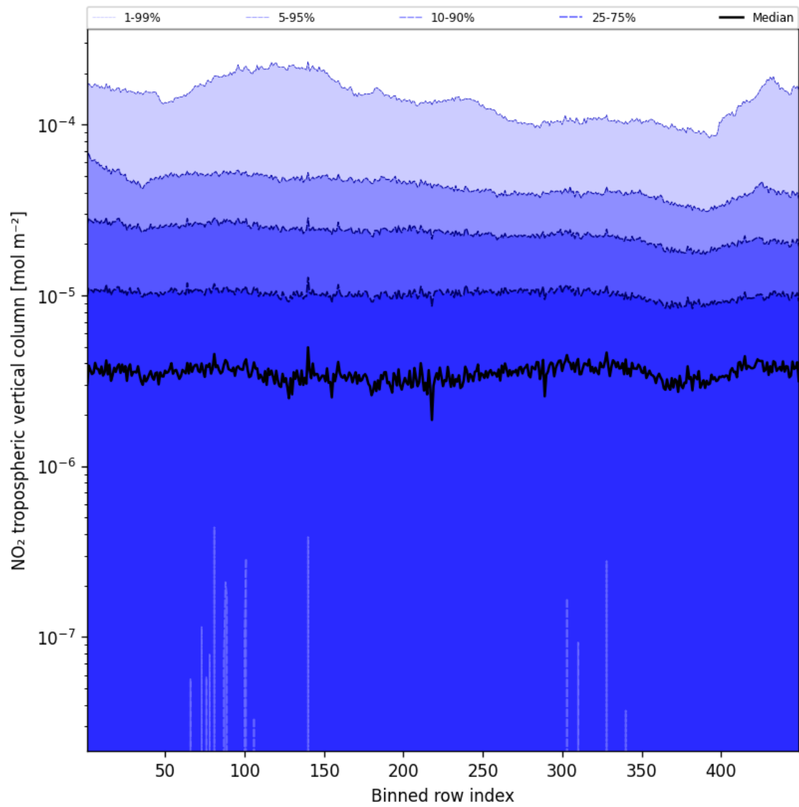
Figure 44: Along track statistics of “NO 2 tropospheric vertical column” for 2025-01-12 to 2025-01-13
