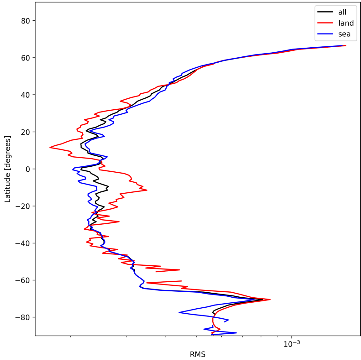
Figure 24: Zonal average of “RMS” for 2025-01-12 to 2025-01-13.
