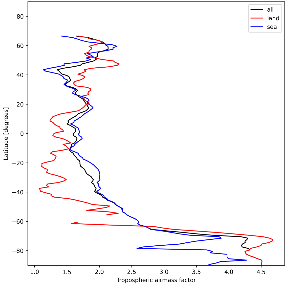
Figure 12: Zonal average of “Tropospheric airmass factor” for 2025-01-12 to 2025-01-13.
