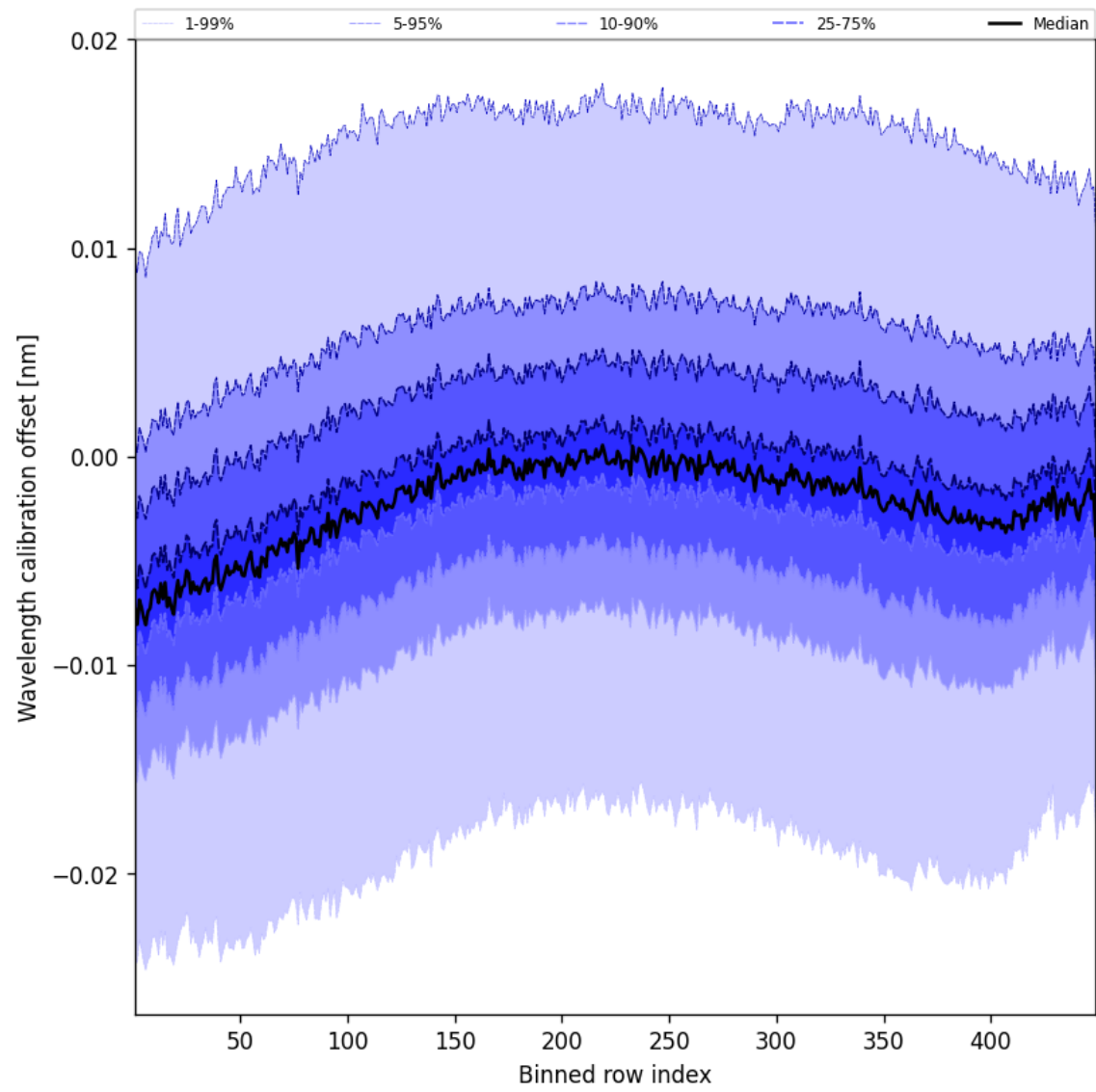
Figure 50: Along track statistics of “Wavelength calibration offset” for 2025-01-12 to 2025-01-13
