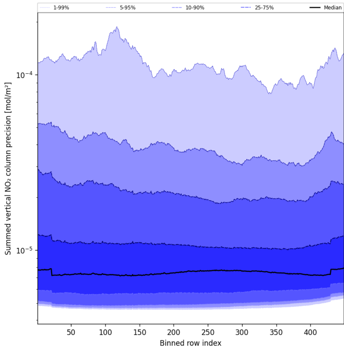
Figure 56: Along track statistics of “Summed vertical NO 2 column precision” for 2025-01-12 to 2025-01-13
