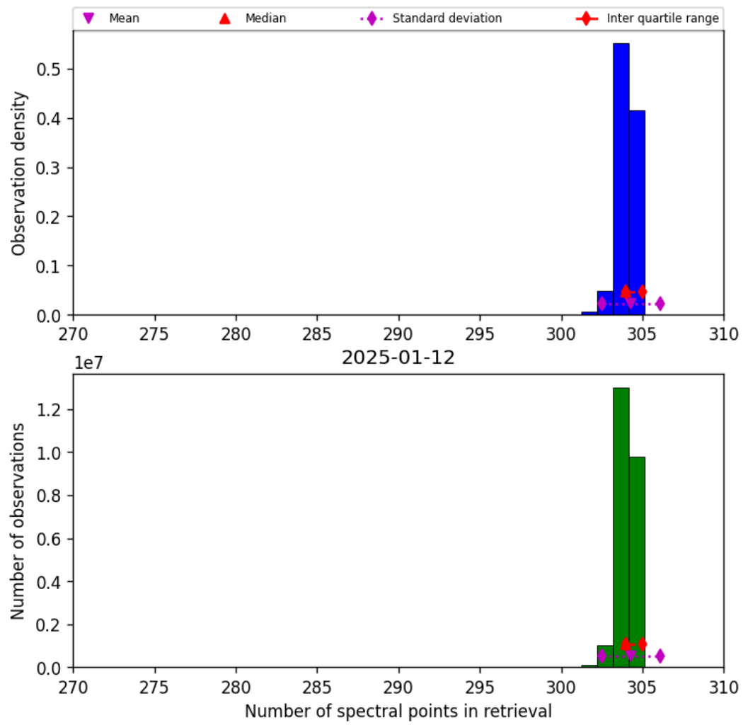
Figure 31: Histogram of “Number of spectral points in retrieval” for 2025-01-12 to 2025-01-13
