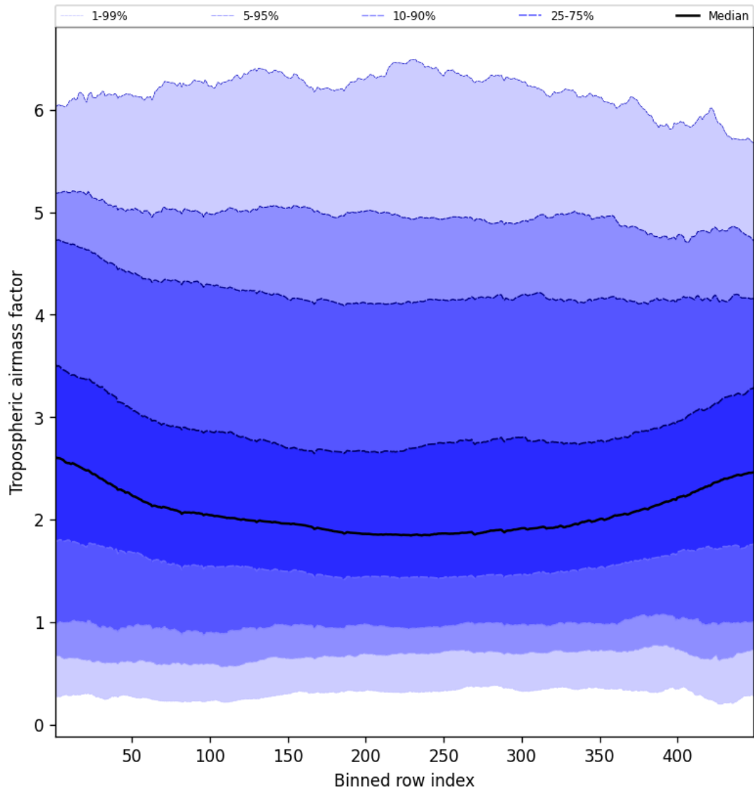
Figure 46: Along track statistics of “Tropospheric airmass factor” for 2025-01-12 to 2025-01-13
