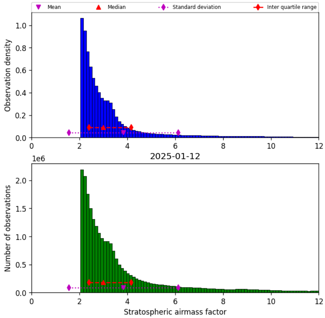
Figure 42: Histogram of “Stratospheric airmass factor” for 2025-01-12 to 2025-01-13
