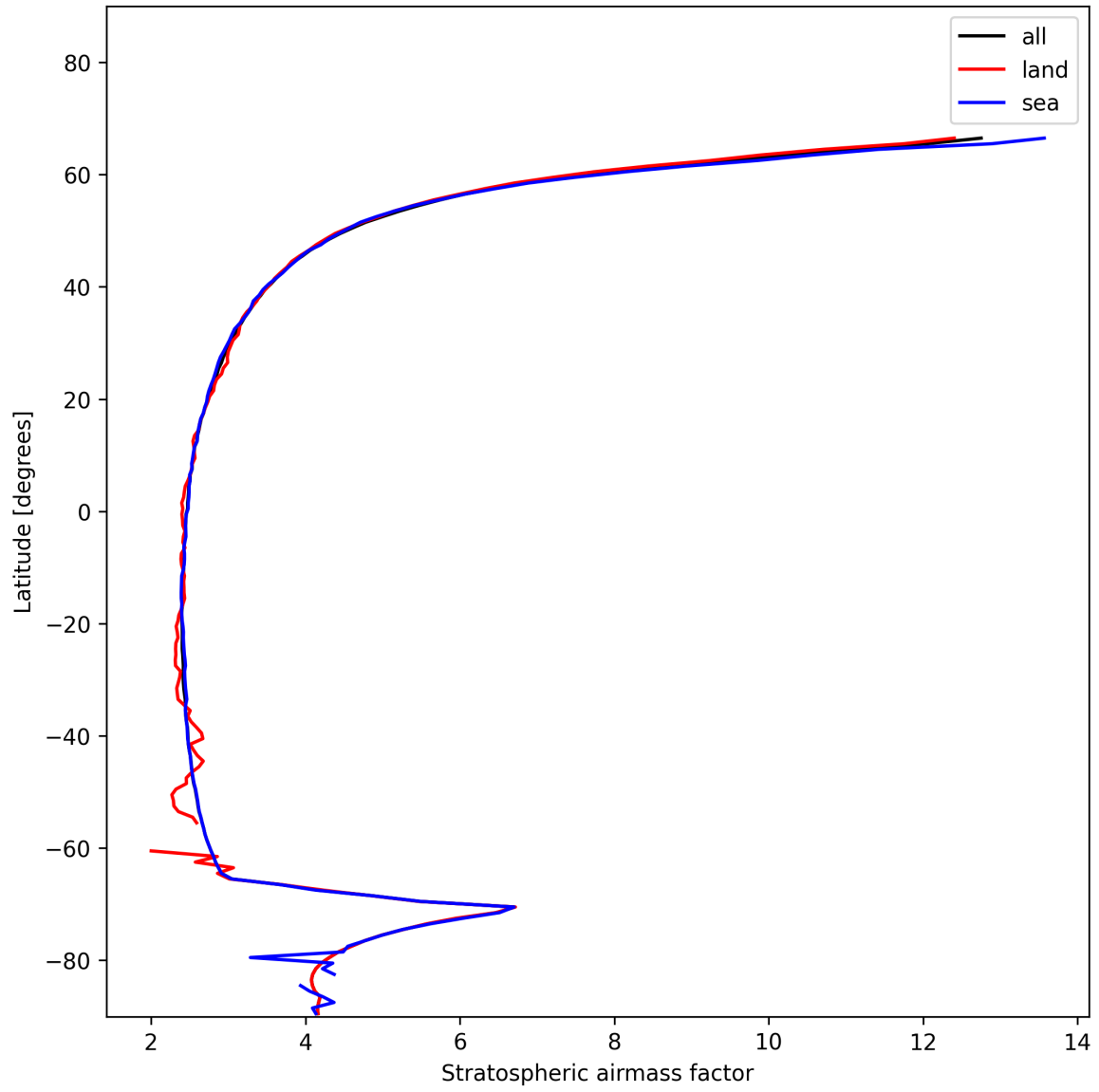
Figure 25: Zonal average of “Stratospheric airmass factor” for 2025-01-12 to 2025-01-13.
