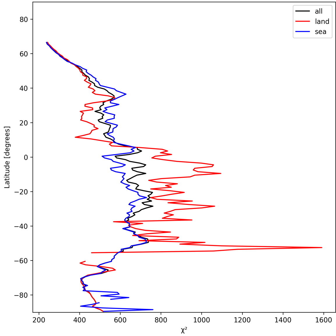
Figure 23: Zonal average of “ \chi^2 ” for 2025-01-12 to 2025-01-13.
