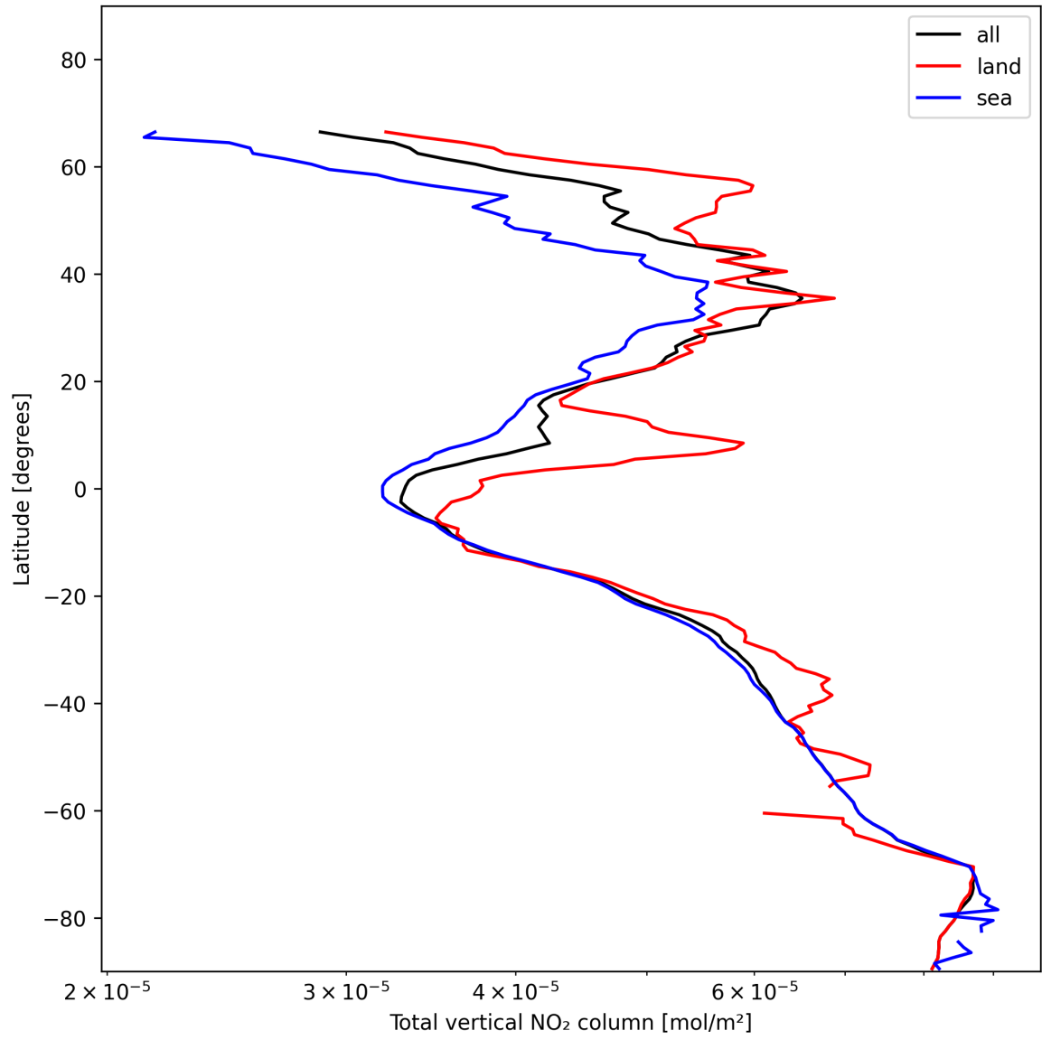
Figure 19: Zonal average of “Total vertical NO 2 column” for 2025-01-12 to 2025-01-13.
