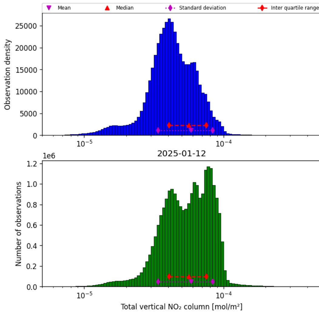
Figure 36: Histogram of “Total vertical NO 2 column” for 2025-01-12 to 2025-01-13
