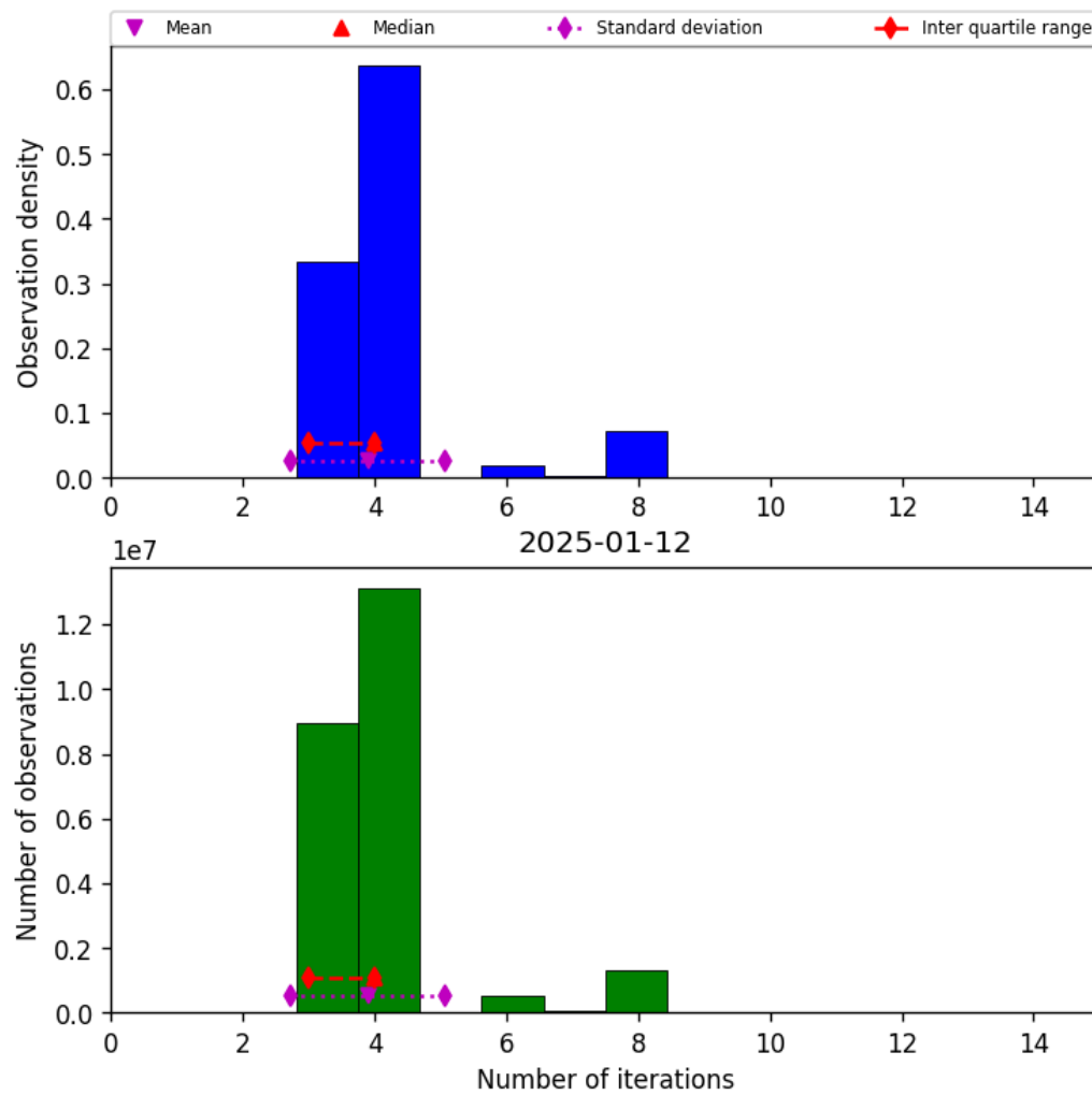
Figure 32: Histogram of “Number of iterations” for 2025-01-12 to 2025-01-13
