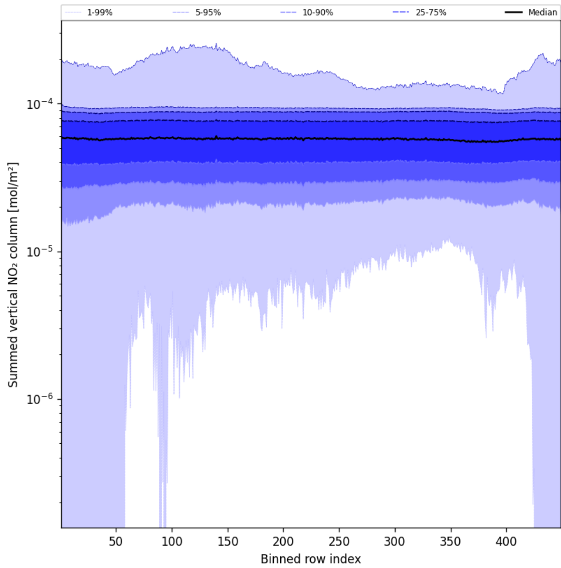
Figure 55: Along track statistics of “Summed vertical NO 2 column” for 2025-01-12 to 2025-01-13
