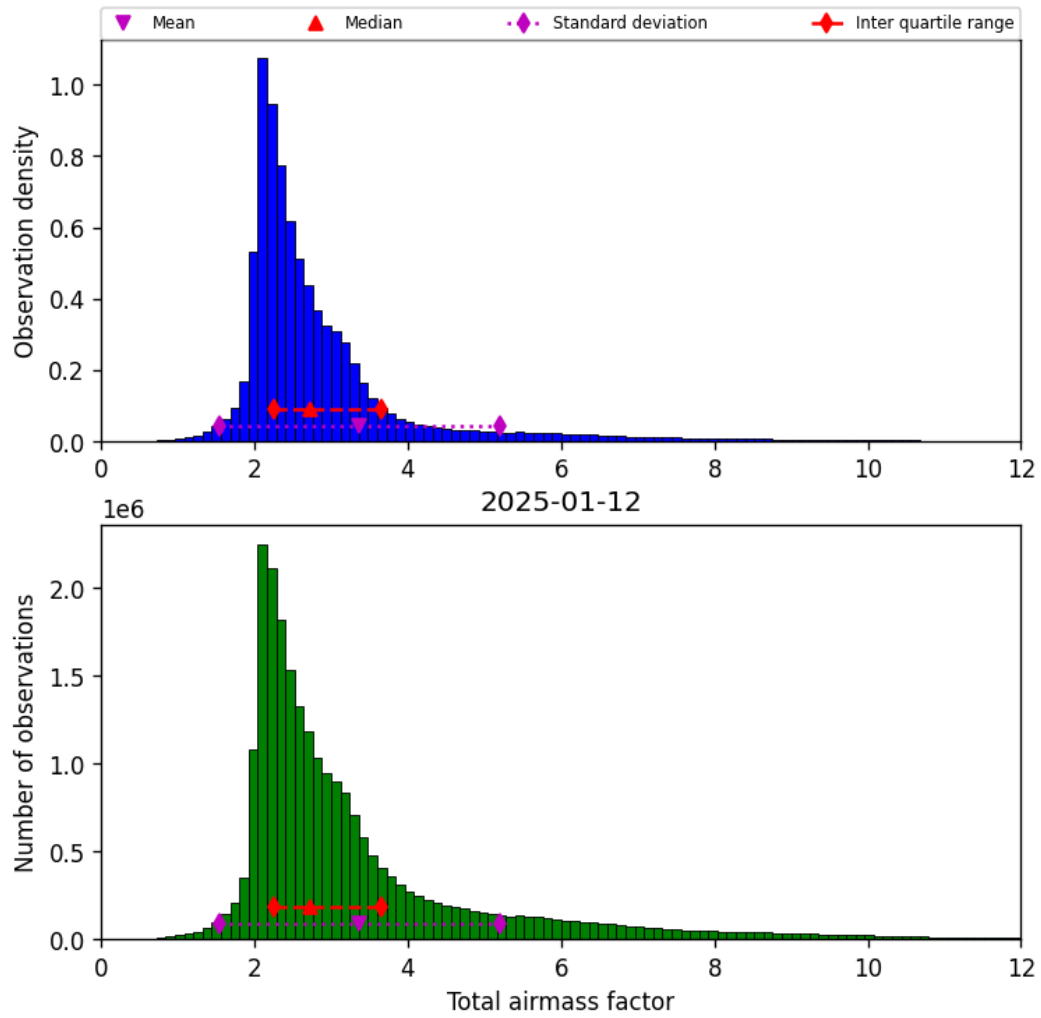
Figure 30: Histogram of “Total airmass factor” for 2025-01-12 to 2025-01-13
