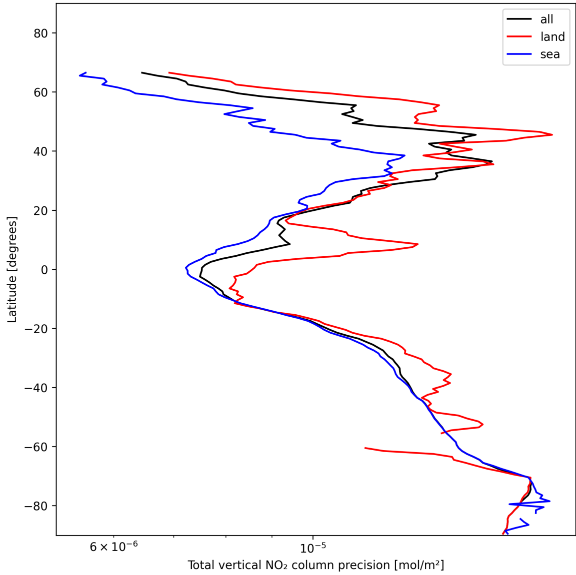
Figure 20: Zonal average of “Total vertical NO 2 column precision” for 2025-01-12 to 2025-01-13.
