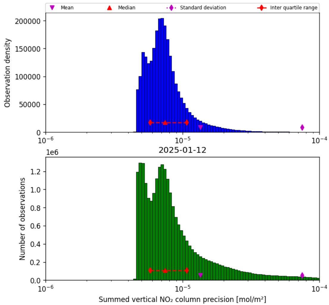
Figure 39: Histogram of "Summed vertical NO 2 column precision" for 2025-01-12 to 2025-01-13
