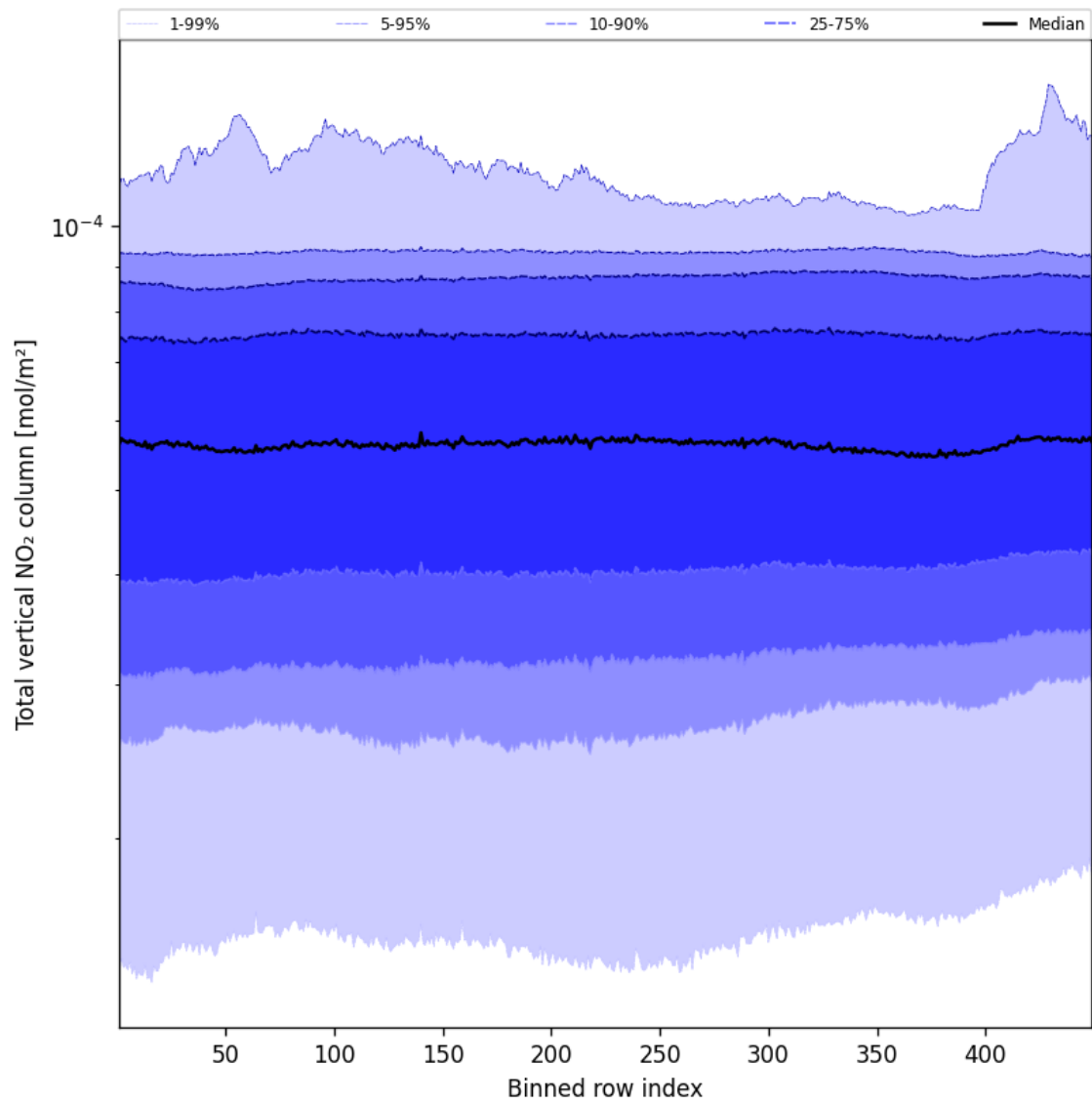
Figure 53: Along track statistics of “Total vertical NO 2 column” for 2025-01-12 to 2025-01-13
