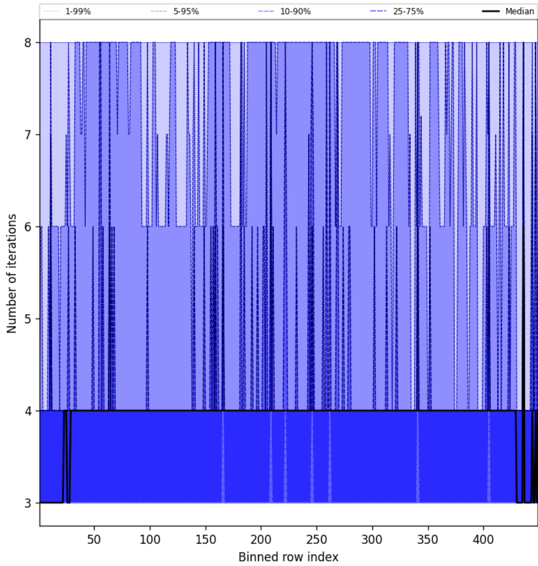
Figure 49: Along track statistics of “Number of iterations” for 2025-01-12 to 2025-01-13
