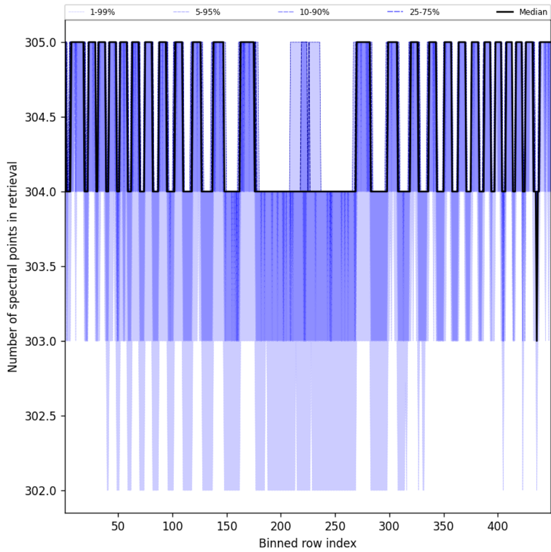
Figure 48: Along track statistics of “Number of spectral points in retrieval” for 2025-01-12 to 2025-01-13
