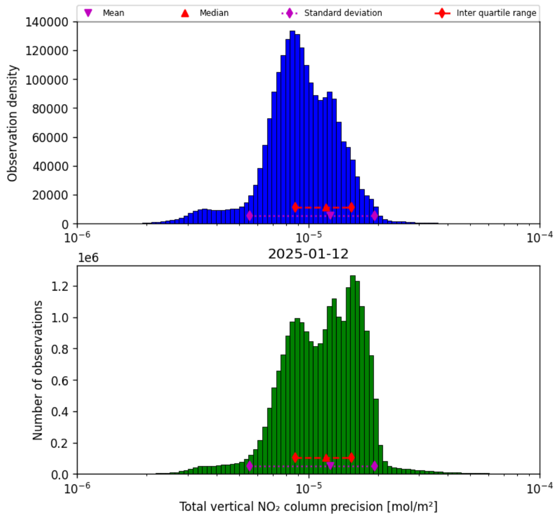
Figure 37: Histogram of “Total vertical NO 2 column precision” for 2025-01-12 to 2025-01-13
