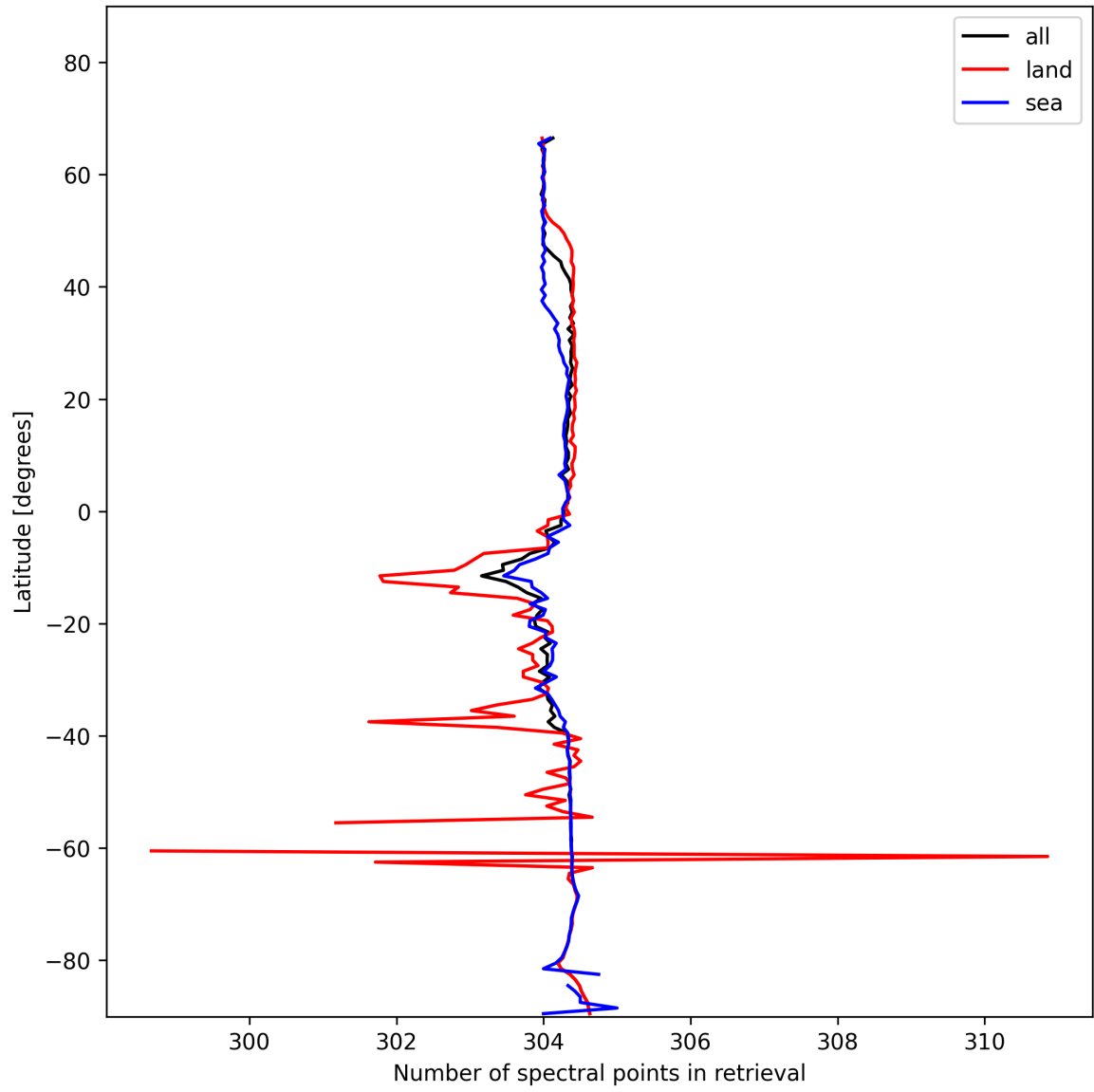
Figure 14: Zonal average of “Number of spectral points in retrieval” for 2025-01-12 to 2025-01-13.
