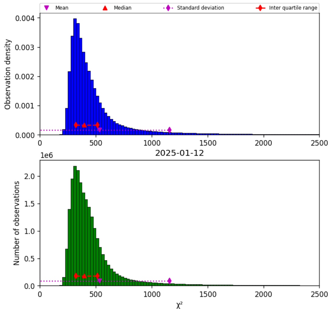
Figure 40: Histogram of “ \chi^2 ” for 2025-01-12 to 2025-01-13
