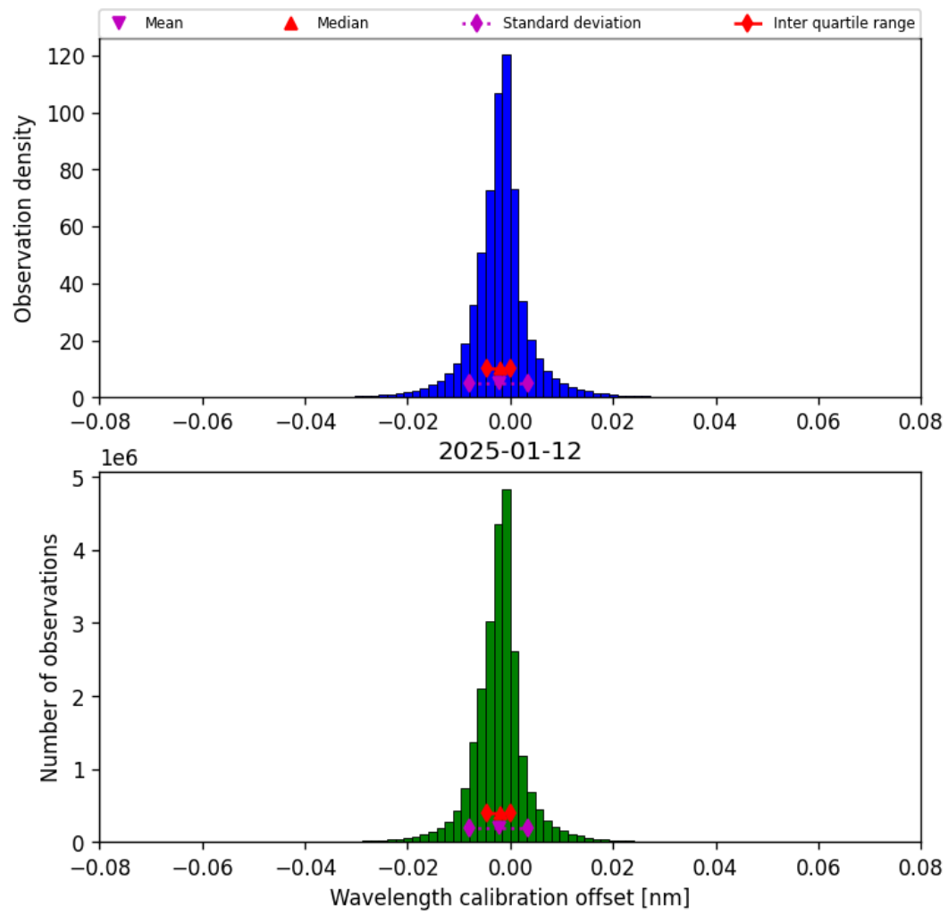
Figure 33: Histogram of “Wavelength calibration offset” for 2025-01-12 to 2025-01-13
