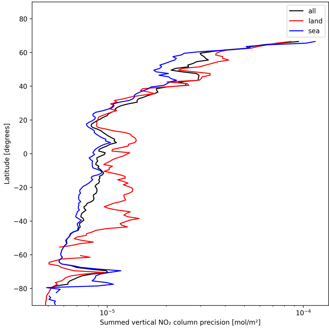
Figure 22: Zonal average of “Summed vertical NO 2 column precision” for 2025-01-12 to 2025-01-13.
