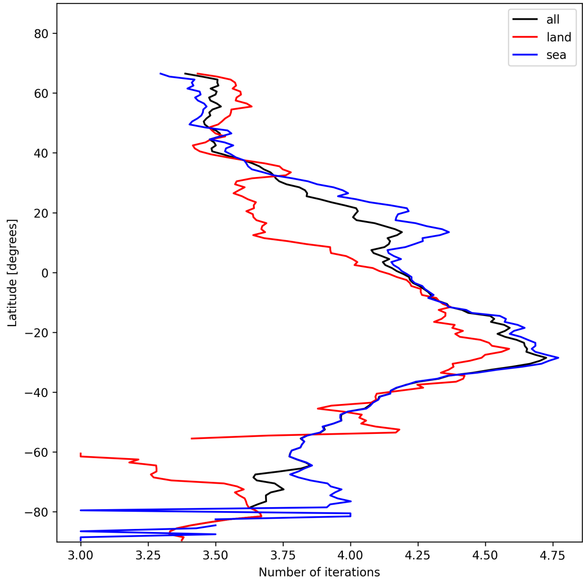
Figure 15: Zonal average of “Number of iterations” for 2025-01-12 to 2025-01-13.
