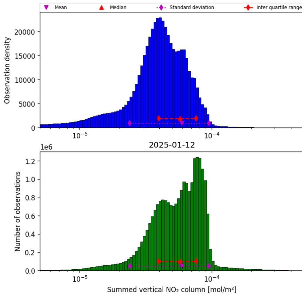
Figure 38: Histogram of “Summed vertical NO 2 column” for 2025-01-12 to 2025-01-13
