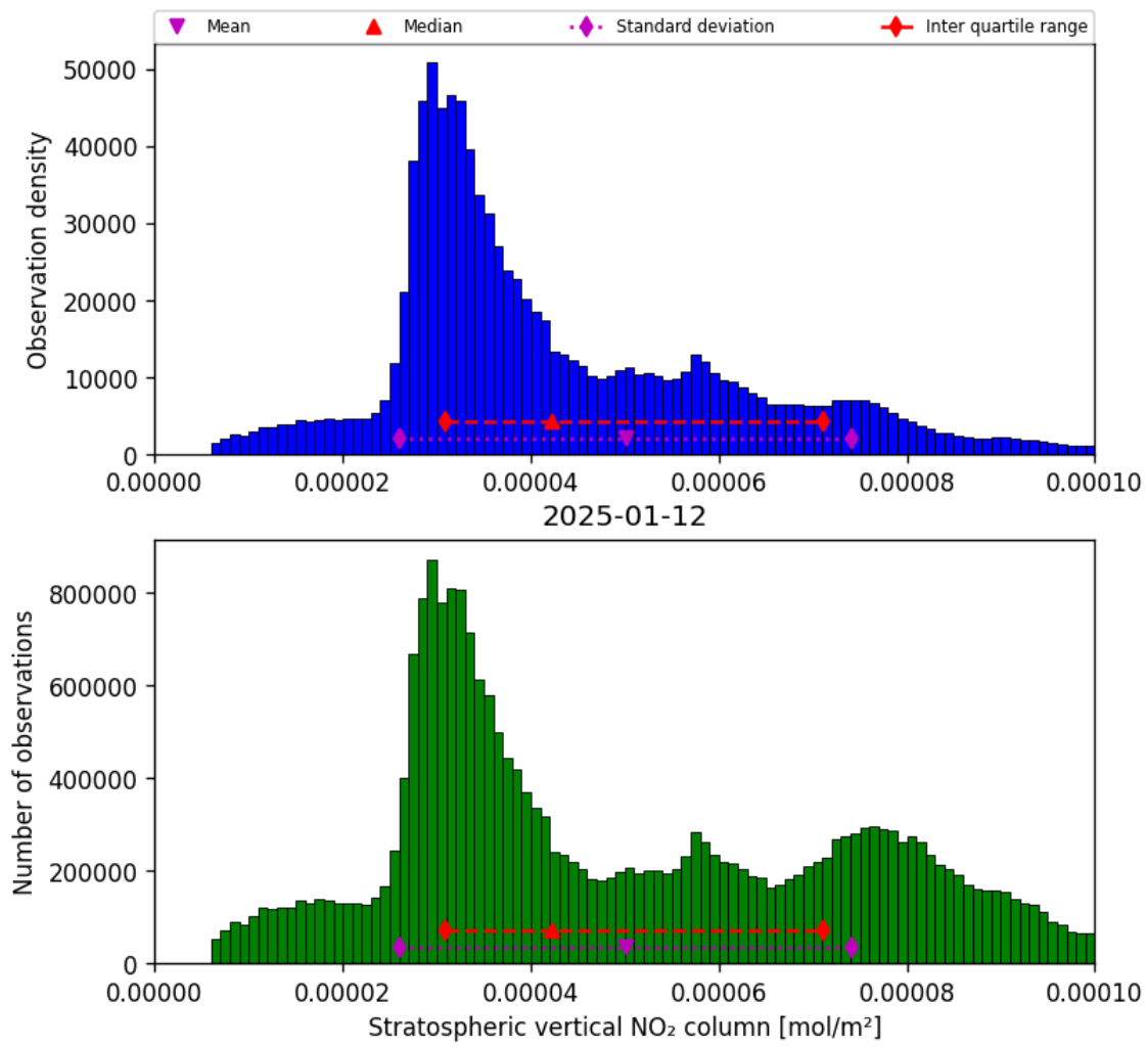
Figure 34: Histogram of “Stratospheric vertical NO 2 column” for 2025-01-12 to 2025-01-13
