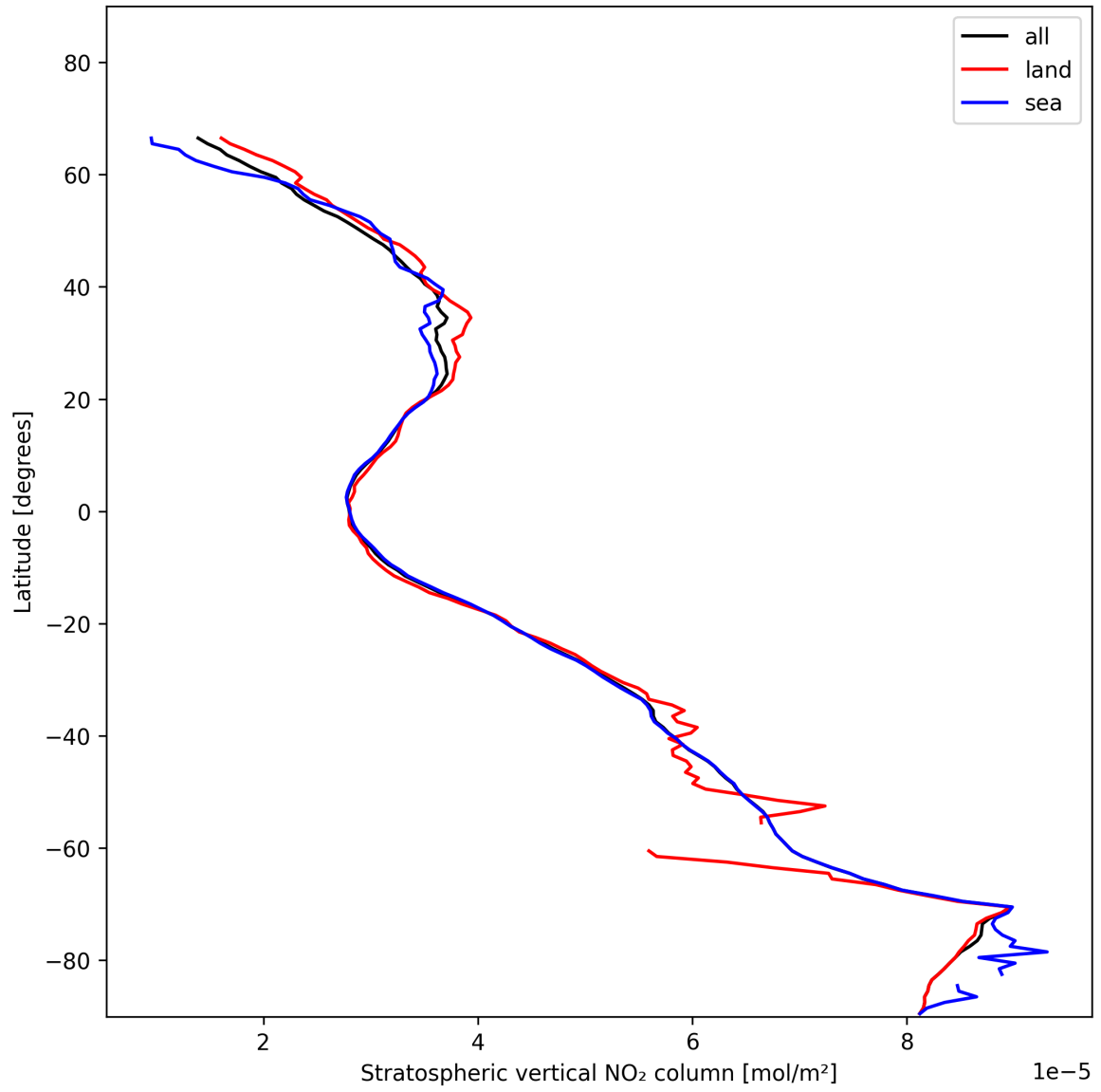
Figure 17: Zonal average of “Stratospheric vertical NO 2 column” for 2025-01-12 to 2025-01-13.
