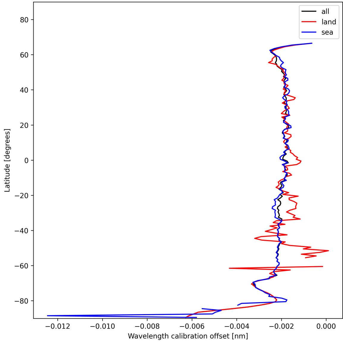
Figure 16: Zonal average of “Wavelength calibration offset” for 2025-01-12 to 2025-01-13.
