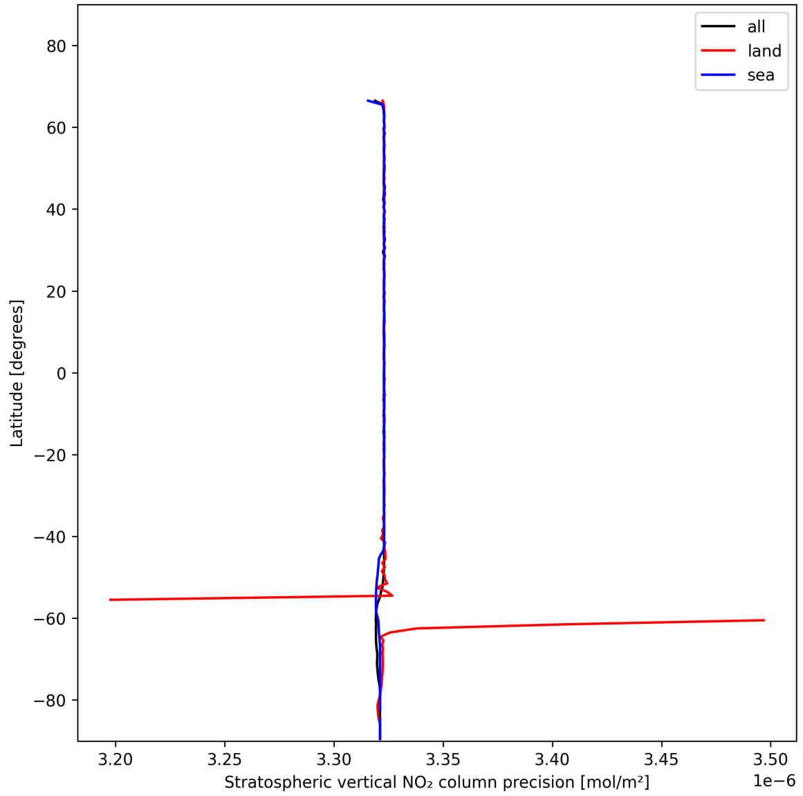
Figure 18: Zonal average of “Stratospheric vertical NO 2 column precision” for 2025-01-12 to 2025-01-13.
