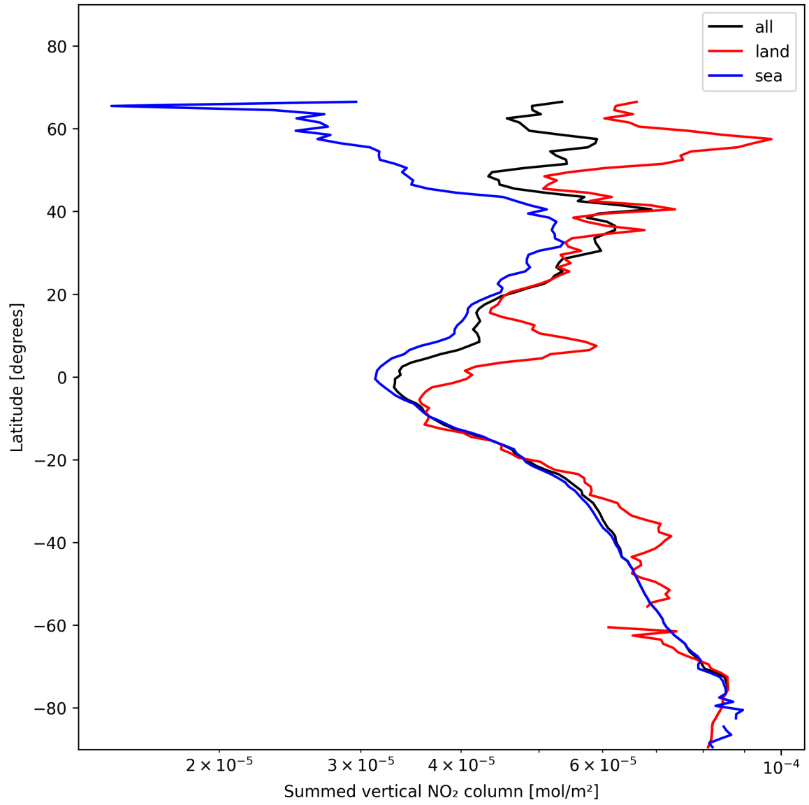
Figure 21: Zonal average of “Summed vertical NO 2 column” for 2025-01-12 to 2025-01-13.
