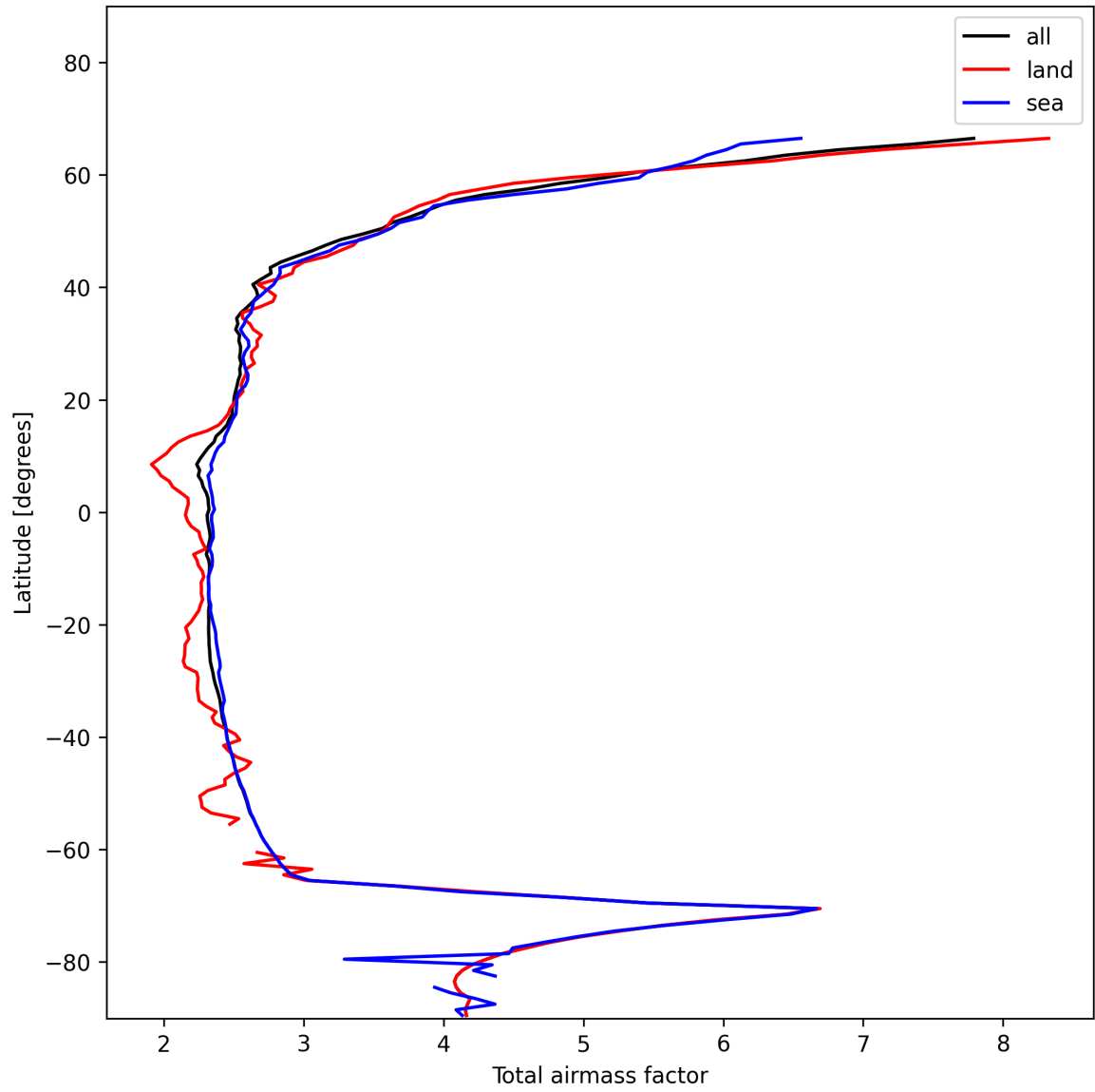
Figure 13: Zonal average of “Total airmass factor” for 2025-01-12 to 2025-01-13.
