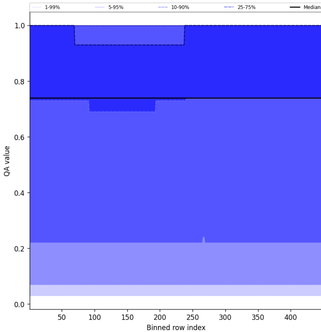
Figure 43: Along track statistics of “QA value” for 2025-01-12 to 2025-01-13
