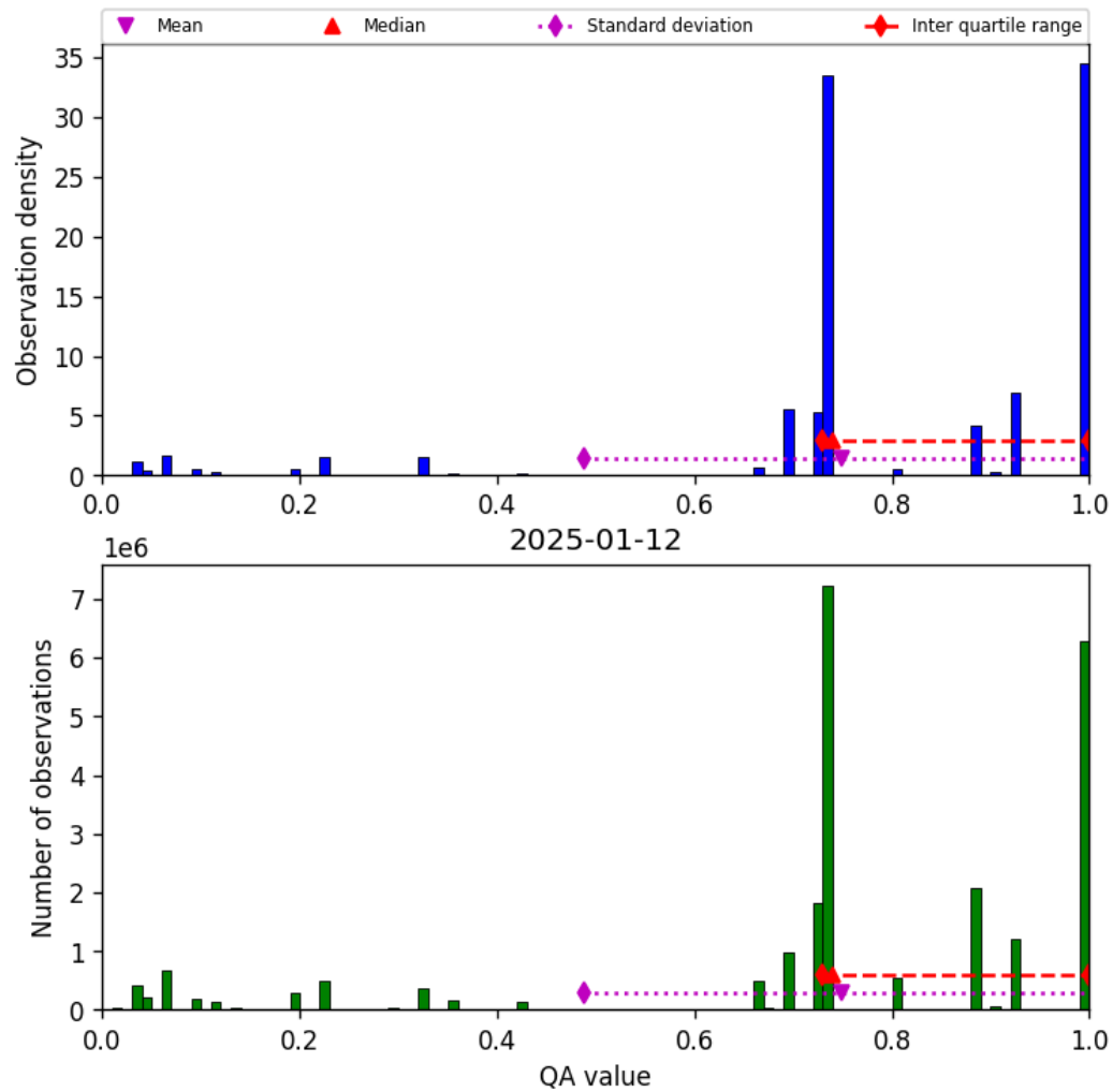
Figure 26: Histogram of “QA value” for 2025-01-12 to 2025-01-13
