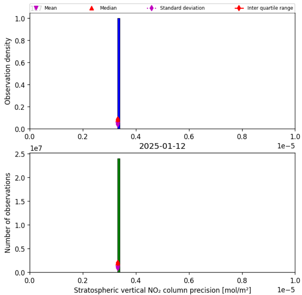
Figure 35: Histogram of “Stratospheric vertical NO 2 column precision” for 2025-01-12 to 2025-01-13
