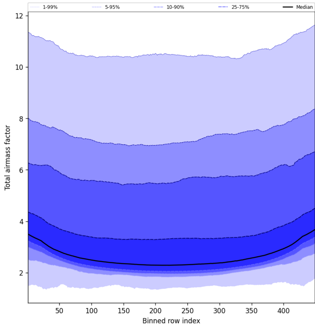
Figure 47: Along track statistics of “Total airmass factor” for 2025-01-12 to 2025-01-13
