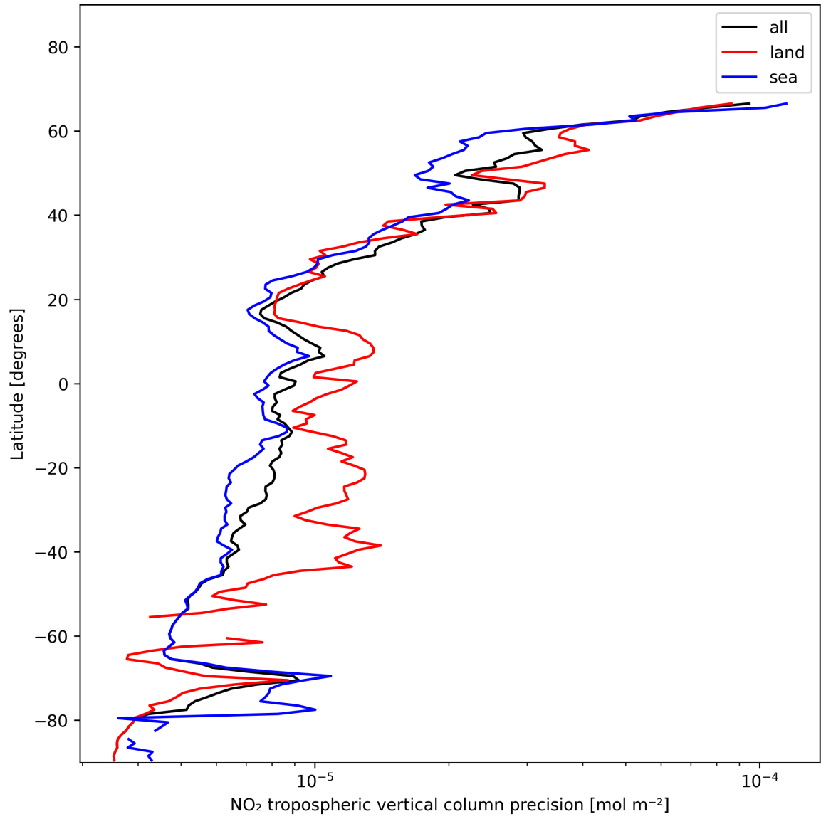
Figure 11: Zonal average of “NO 2 tropospheric vertical column precision” for 2025-01-12 to 2025-01-13.
