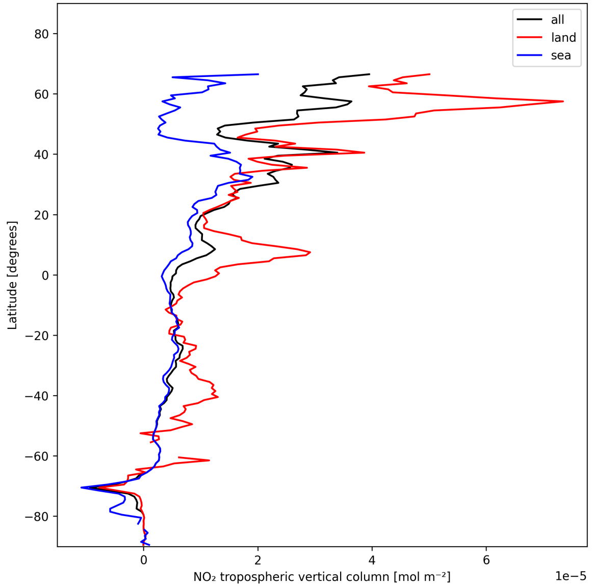
Figure 10: Zonal average of “NO 2 tropospheric vertical column” for 2025-01-12 to 2025-01-13.
