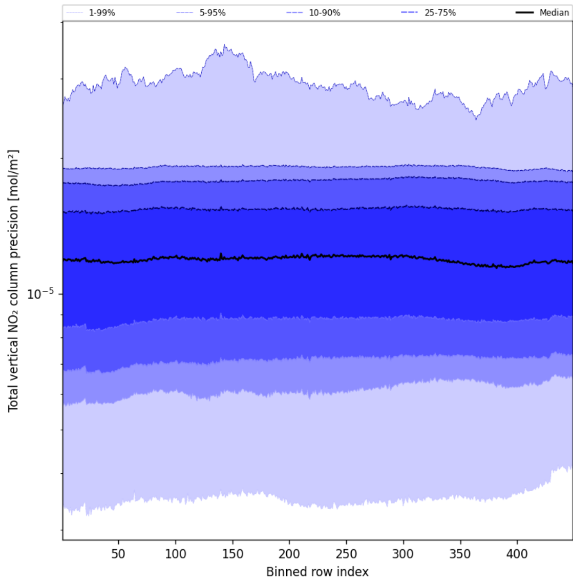
Figure 54: Along track statistics of “Total vertical NO 2 column precision” for 2025-01-12 to 2025-01-13
