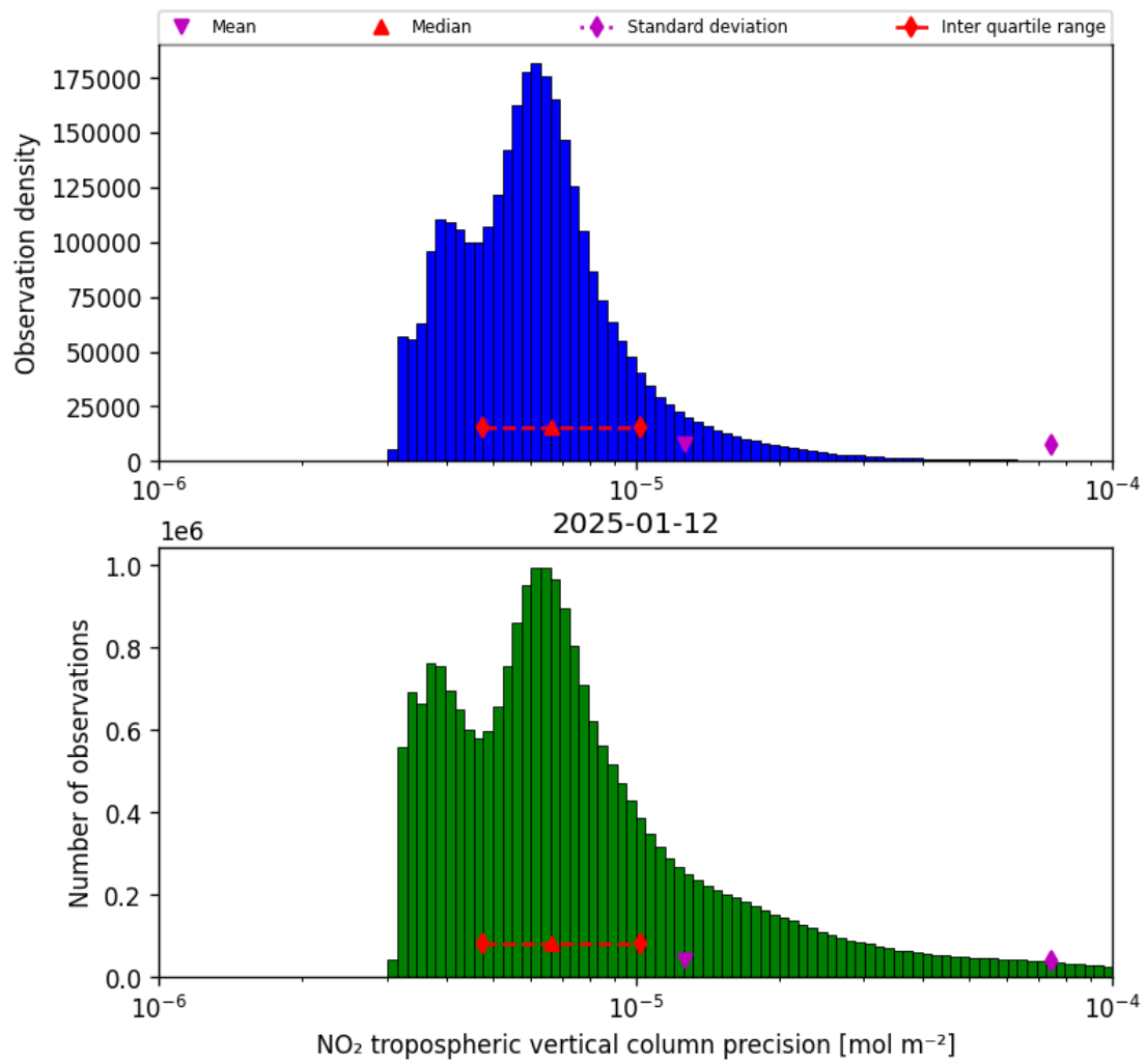
Figure 28: Histogram of “NO 2 tropospheric vertical column precision” for 2025-01-12 to 2025-01-13
