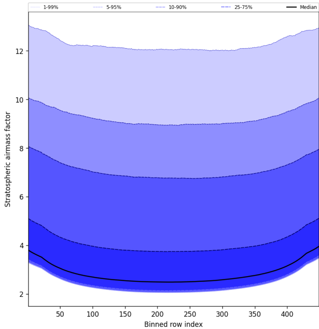
Figure 59: Along track statistics of “Stratospheric airmass factor” for 2025-01-12 to 2025-01-13
