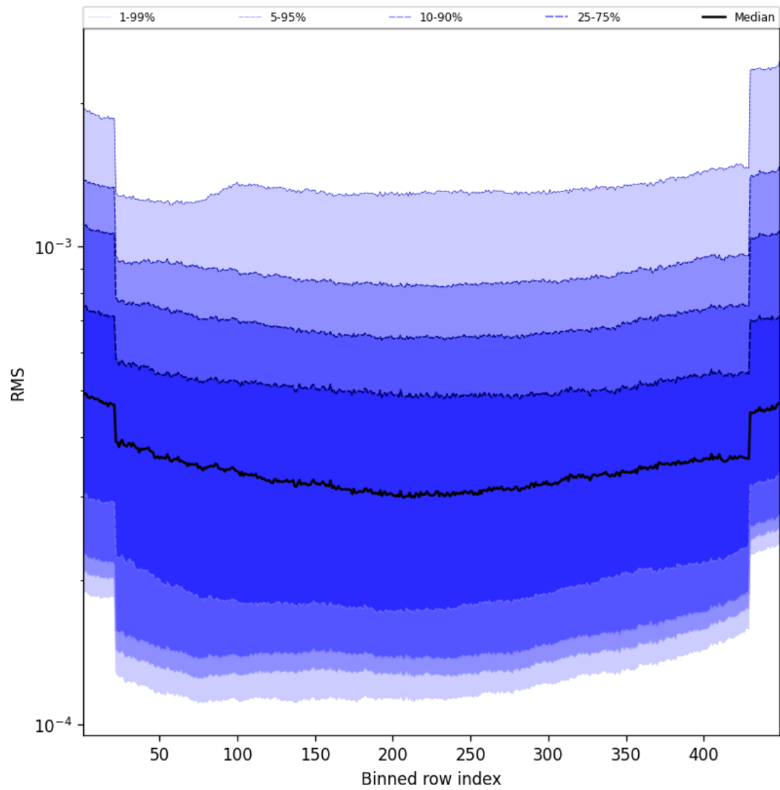
Figure 58: Along track statistics of “RMS” for 2025-01-12 to 2025-01-13
