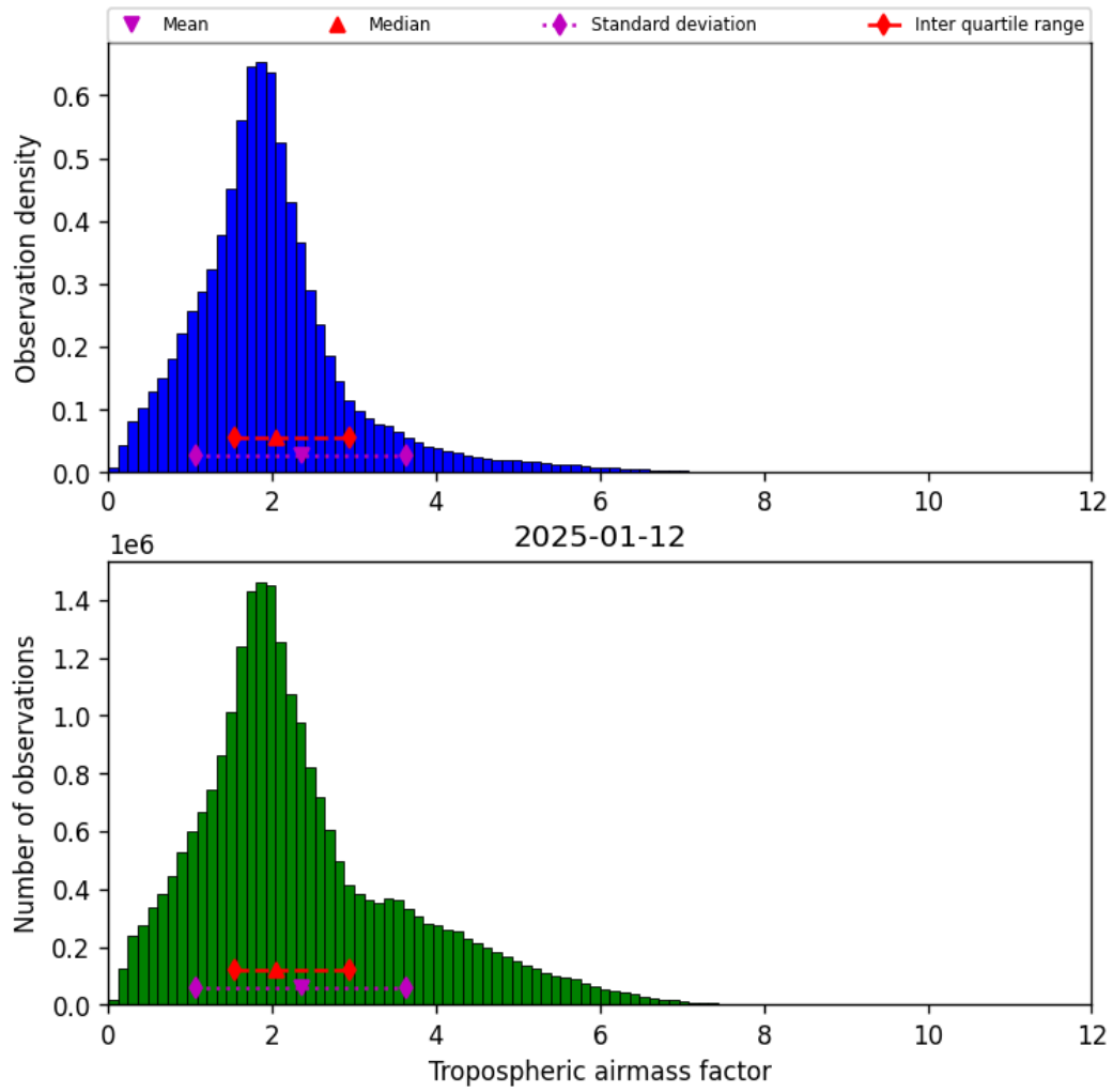
Figure 29: Histogram of “Tropospheric airmass factor” for 2025-01-12 to 2025-01-13
