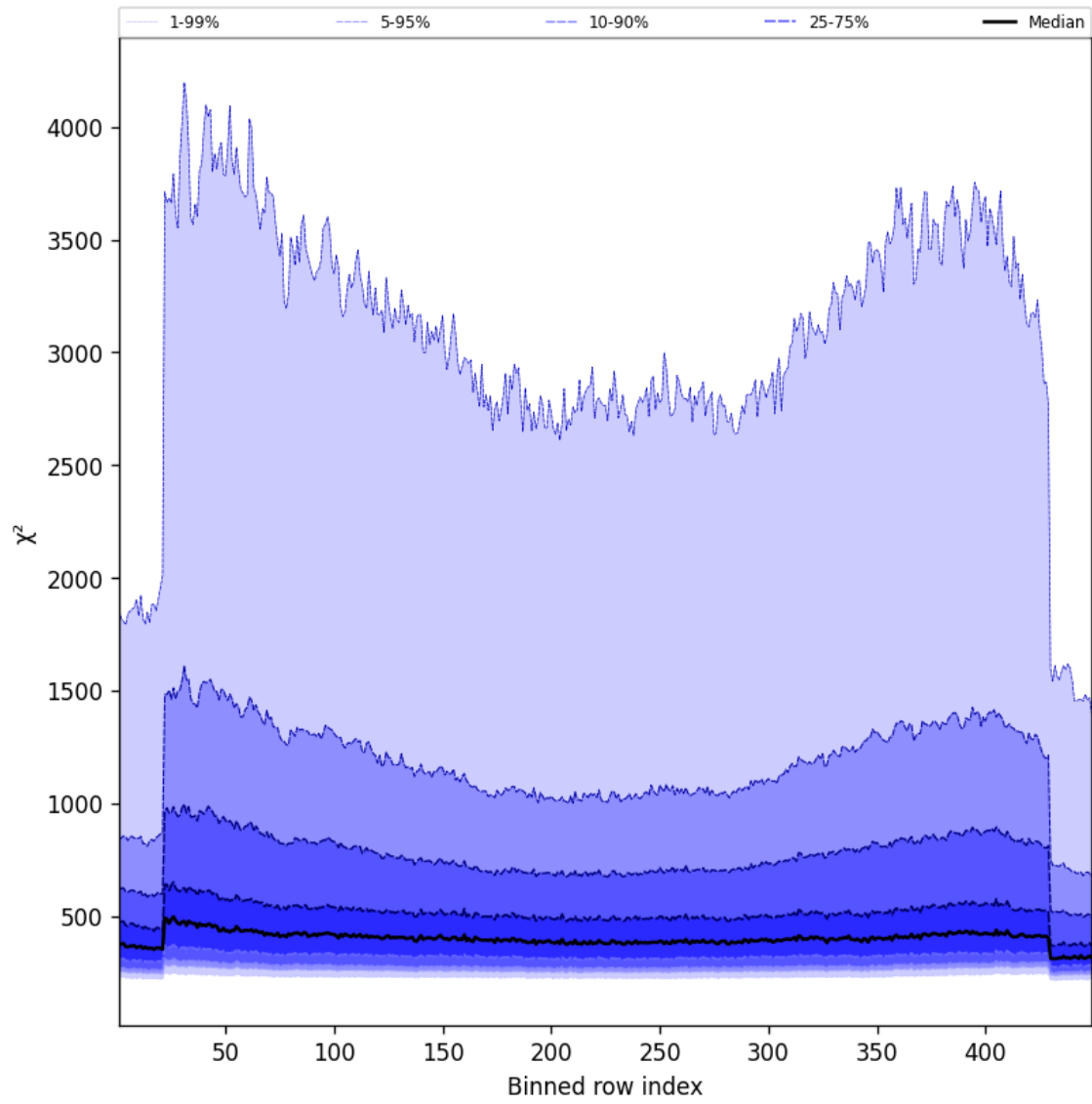
Figure 57: Along track statistics of “ \chi^2 ” for 2025-01-12 to 2025-01-13
