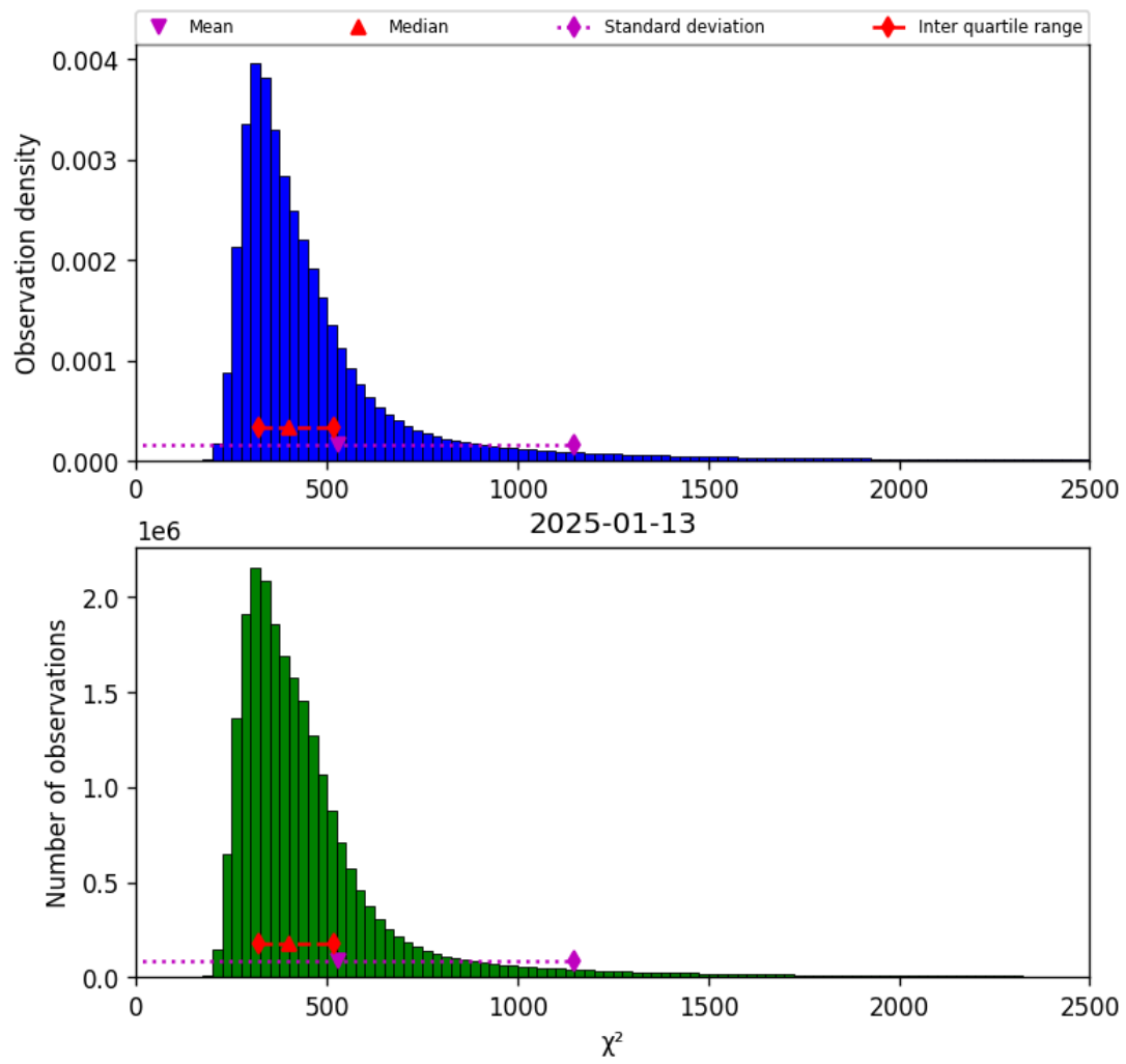
Figure 40: Histogram of “ \chi^2 ” for 2025-01-13 to 2025-01-14
