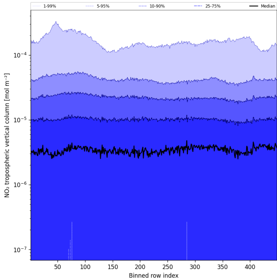
Figure 44: Along track statistics of “NO 2 tropospheric vertical column” for 2025-01-13 to 2025-01-14
