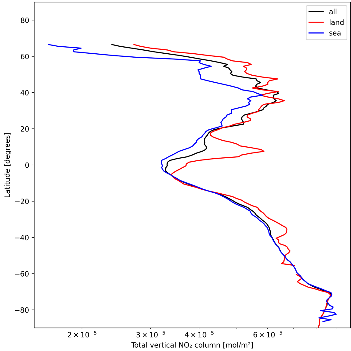
Figure 19: Zonal average of “Total vertical NO 2 column” for 2025-01-13 to 2025-01-14.
