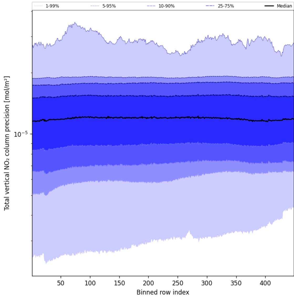
Figure 54: Along track statistics of “Total vertical NO 2 column precision” for 2025-01-13 to 2025-01-14
