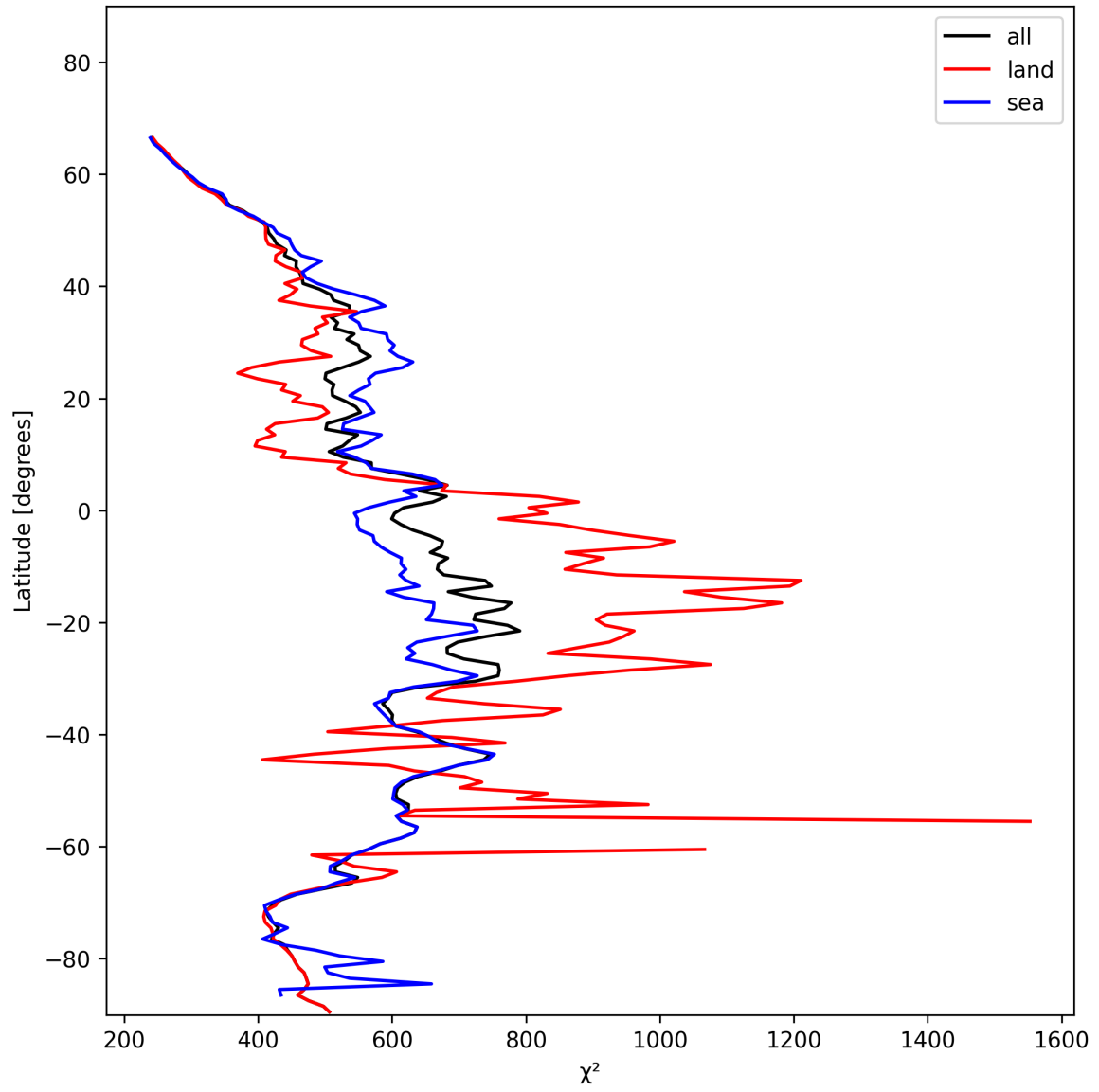
Figure 23: Zonal average of “ \chi^2 ” for 2025-01-13 to 2025-01-14.
