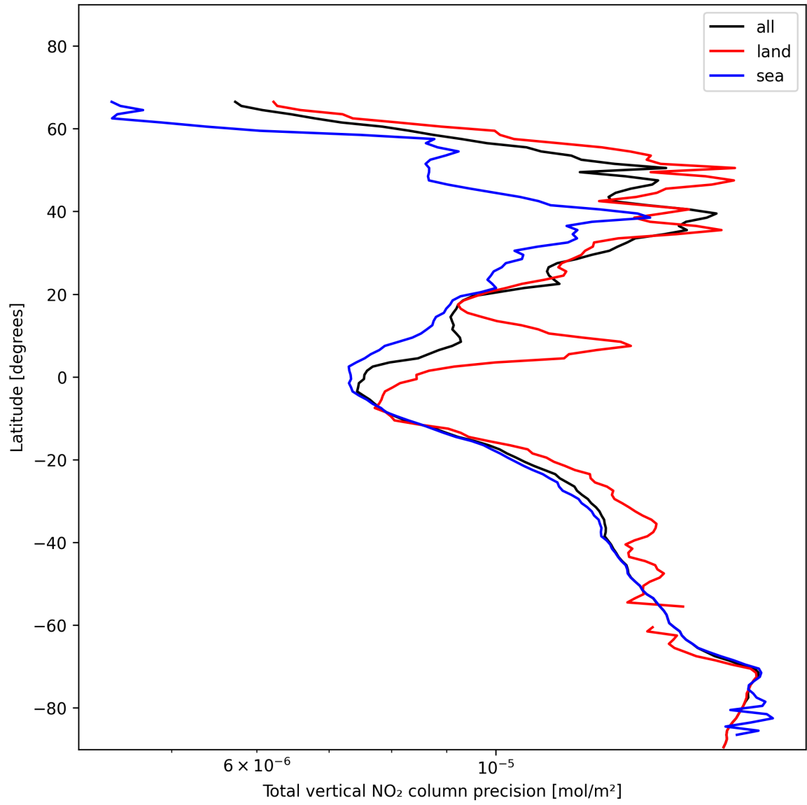
Figure 20: Zonal average of “Total vertical NO 2 column precision” for 2025-01-13 to 2025-01-14.
