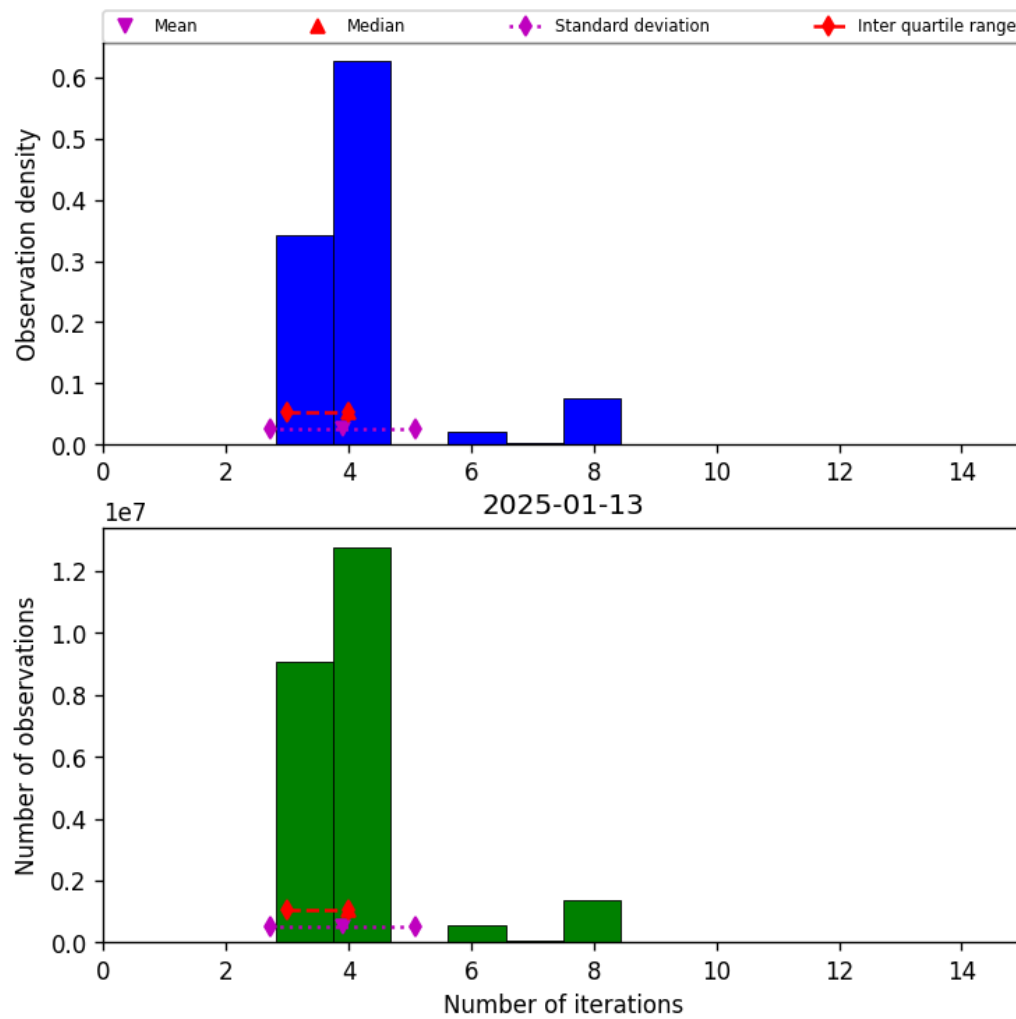
Figure 32: Histogram of “Number of iterations” for 2025-01-13 to 2025-01-14
