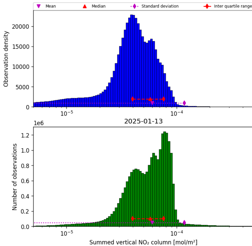
Figure 38: Histogram of “Summed vertical NO 2 column” for 2025-01-13 to 2025-01-14
