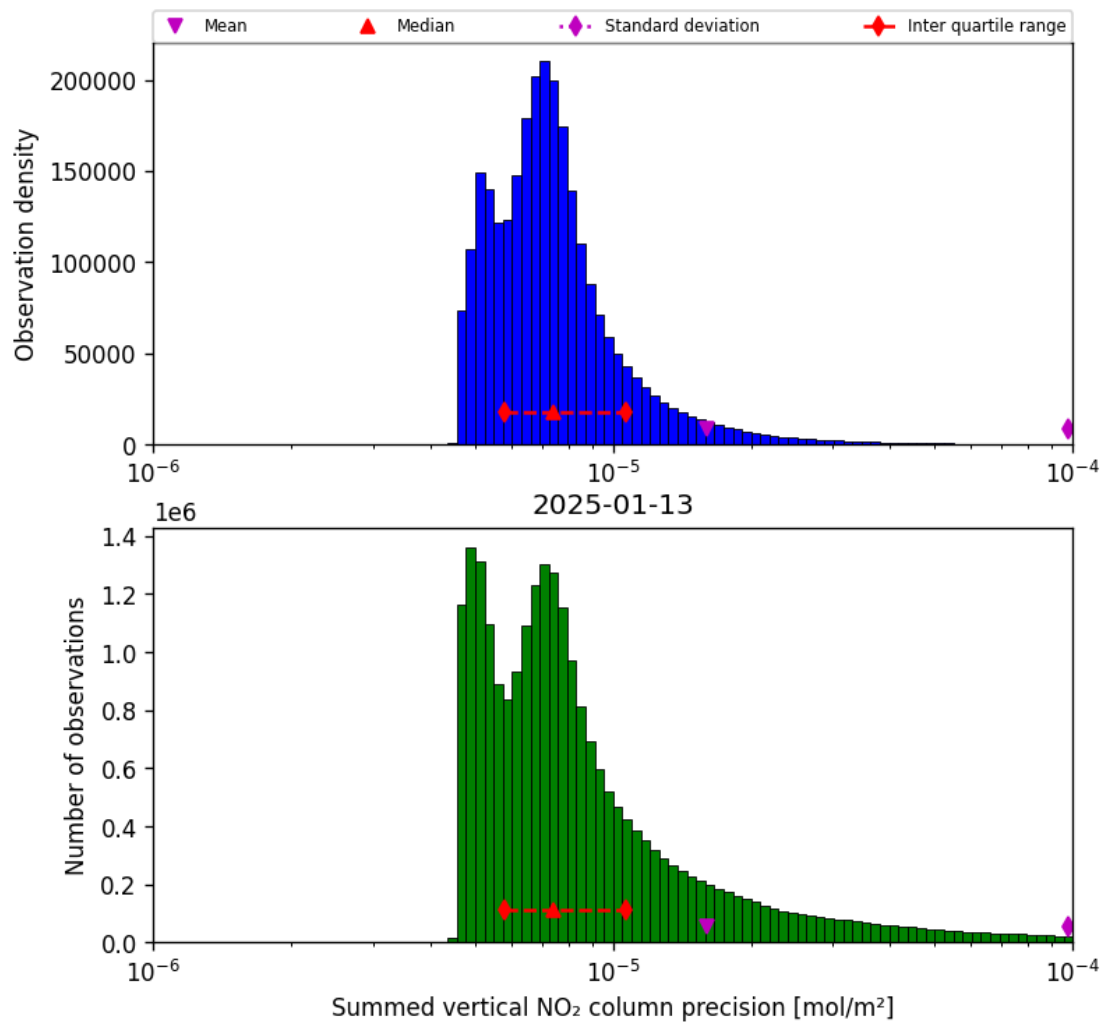
Figure 39: Histogram of "Summed vertical NO 2 column precision" for 2025-01-13 to 2025-01-14
