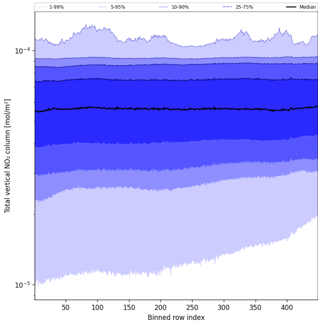
Figure 53: Along track statistics of “Total vertical NO 2 column” for 2025-01-13 to 2025-01-14
