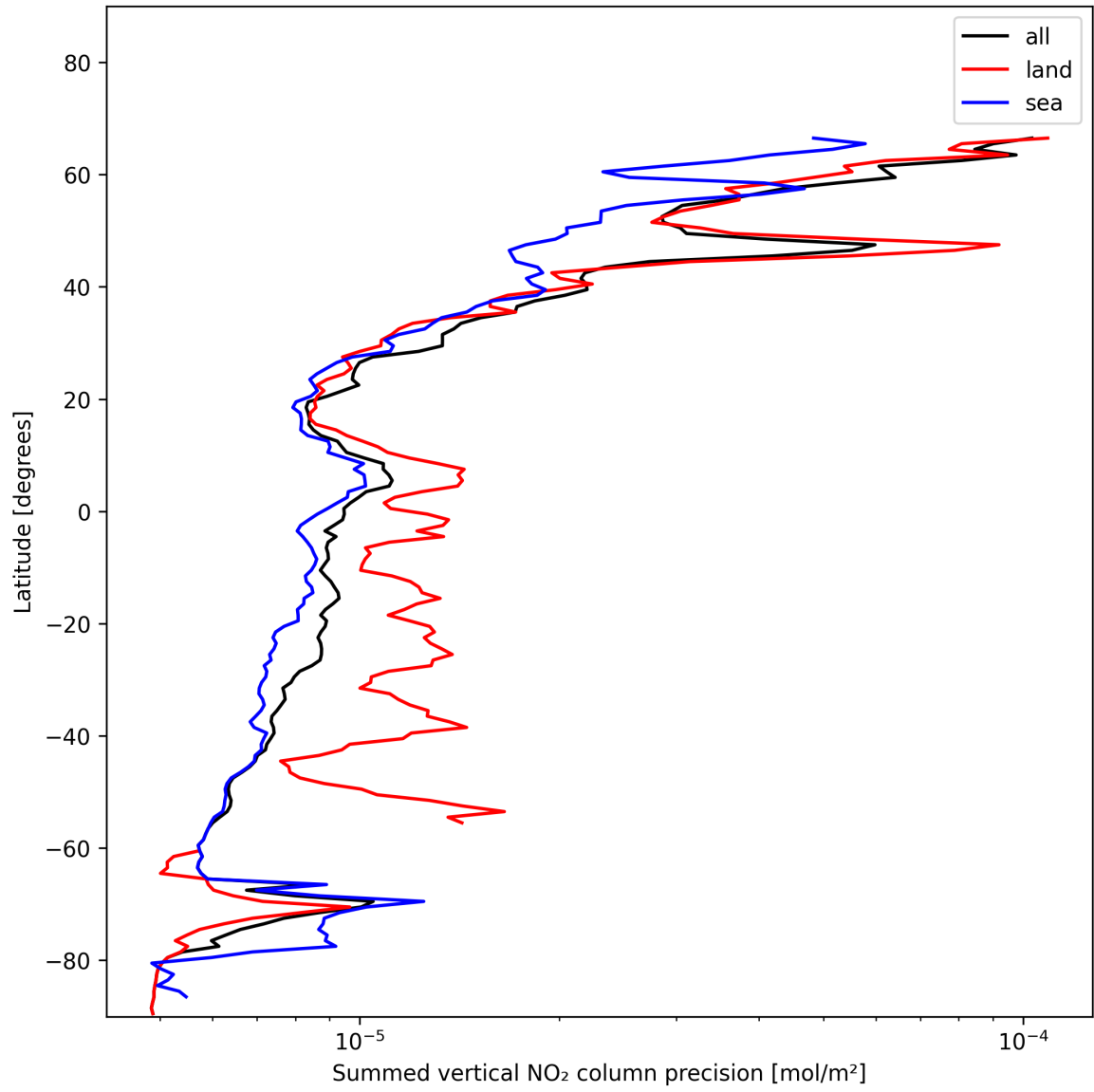
Figure 22: Zonal average of “Summed vertical NO 2 column precision” for 2025-01-13 to 2025-01-14.
