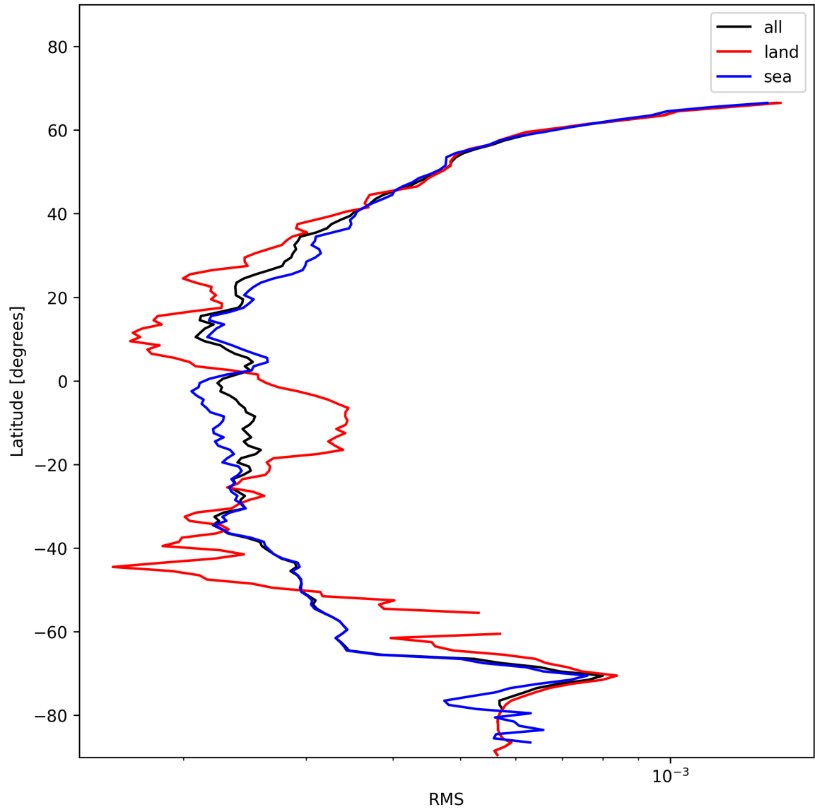
Figure 24: Zonal average of “RMS” for 2025-01-13 to 2025-01-14.
