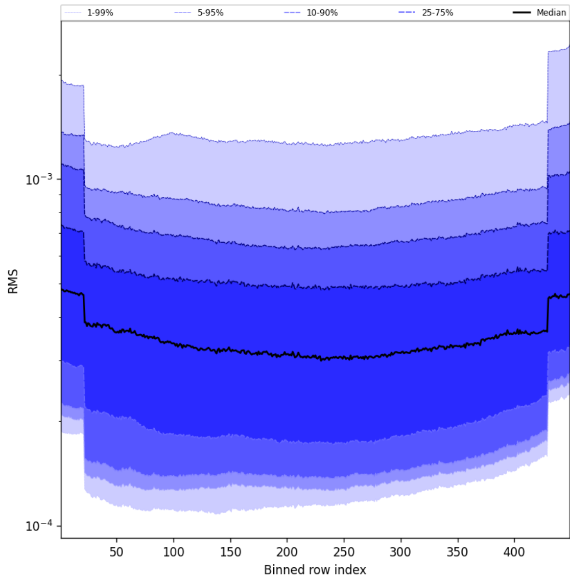
Figure 58: Along track statistics of “RMS” for 2025-01-13 to 2025-01-14
