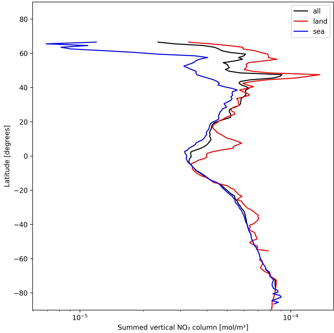
Figure 21: Zonal average of “Summed vertical NO 2 column” for 2025-01-13 to 2025-01-14.
