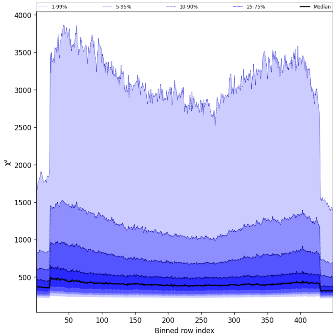
Figure 57: Along track statistics of “ \chi^2 ” for 2025-01-13 to 2025-01-14
