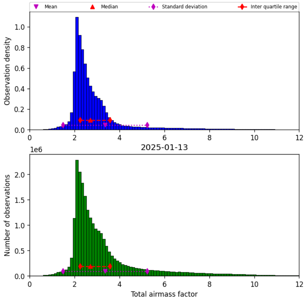
Figure 30: Histogram of “Total airmass factor” for 2025-01-13 to 2025-01-14
