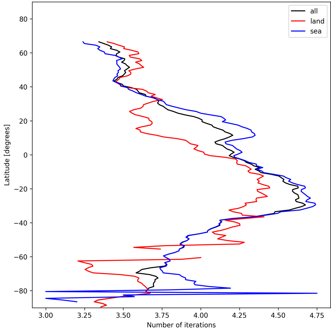
Figure 15: Zonal average of “Number of iterations” for 2025-01-13 to 2025-01-14.
