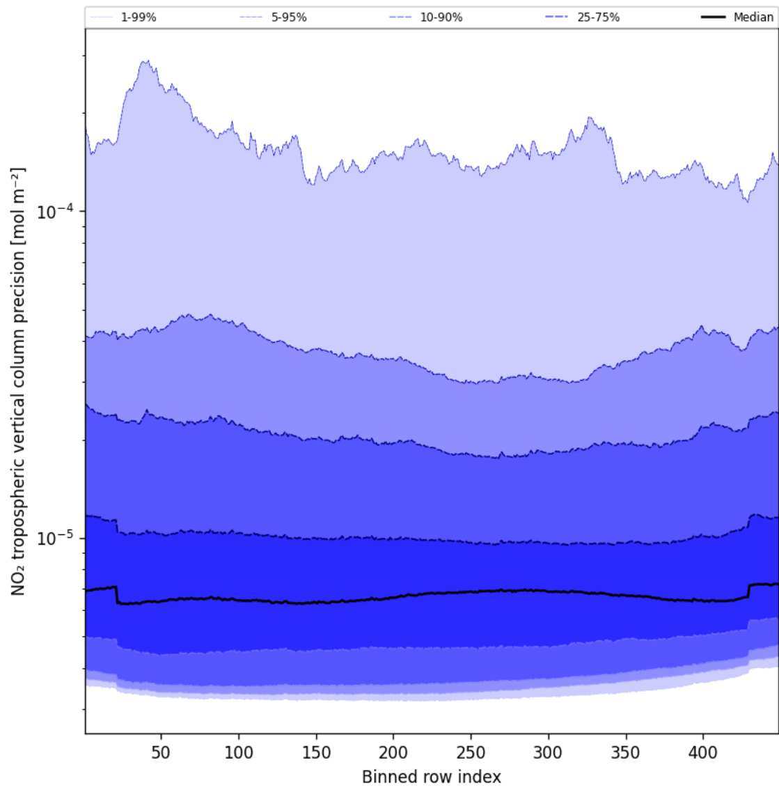
Figure 45: Along track statistics of “NO 2 tropospheric vertical column precision” for 2025-01-13 to 2025-01-14
