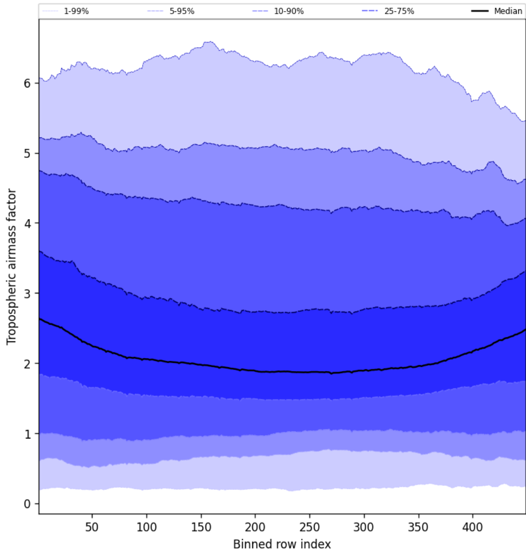
Figure 46: Along track statistics of “Tropospheric air mass factor” for 2025-01-13 to 2025-01-14
