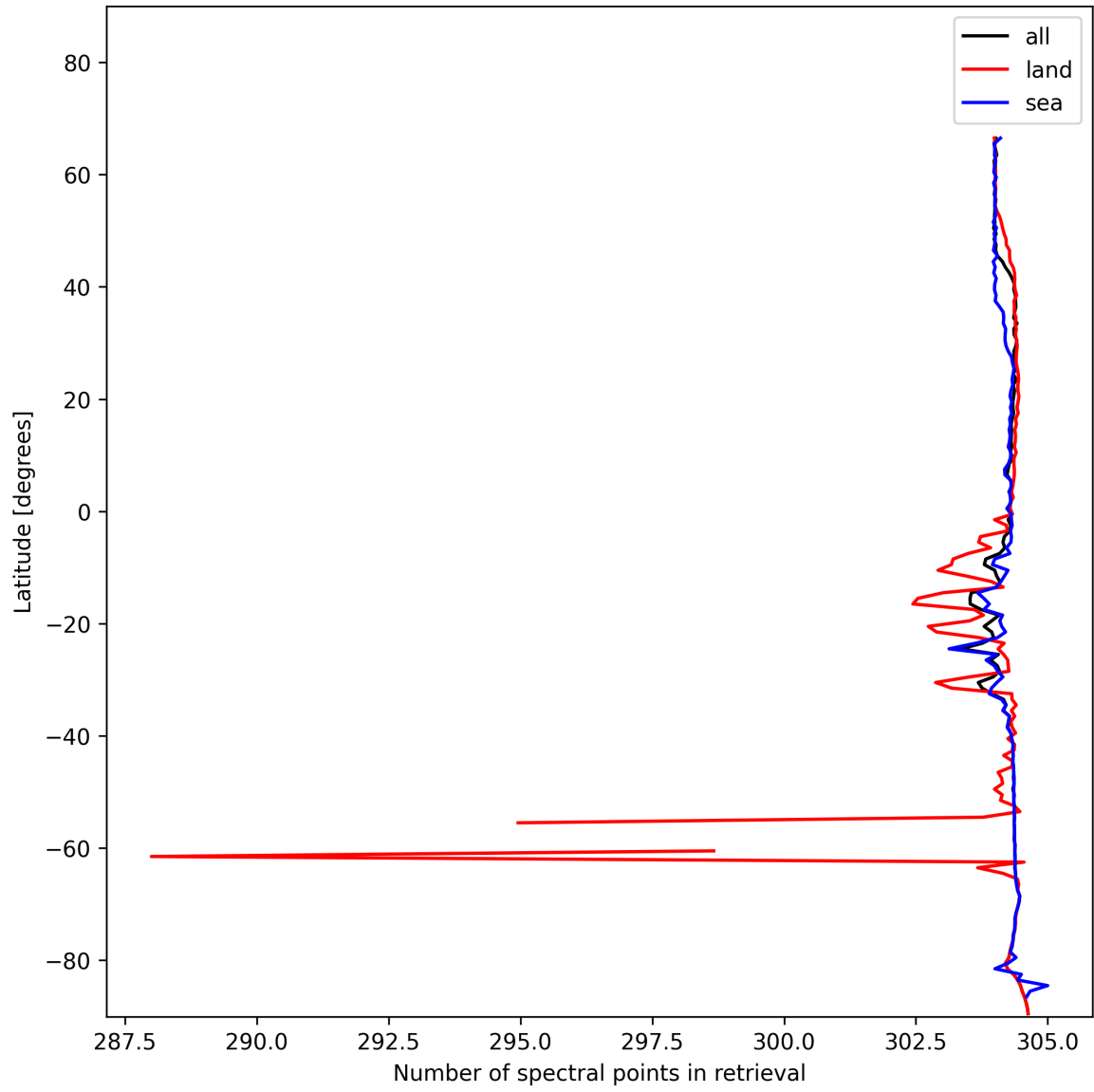
Figure 14: Zonal average of “Number of spectral points in retrieval” for 2025-01-13 to 2025-01-14.
