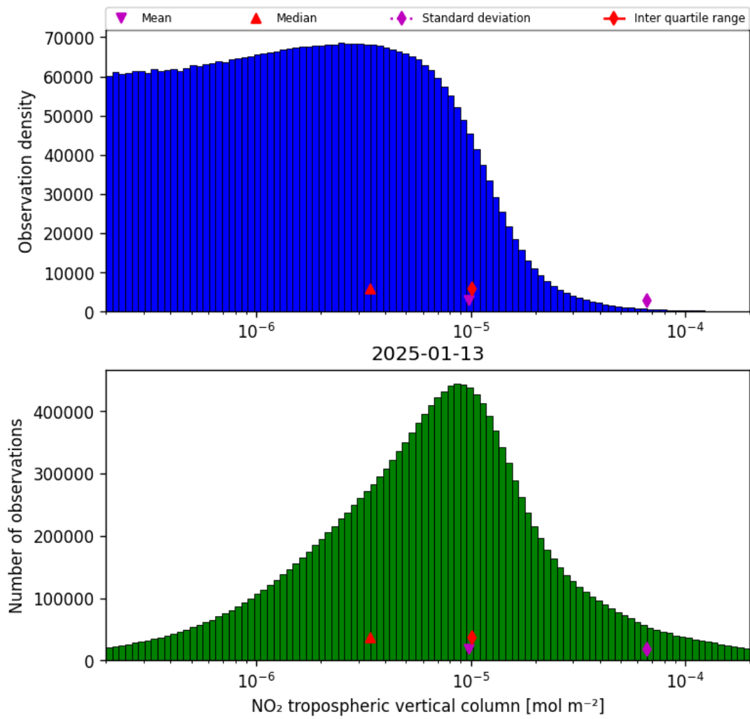
Figure 27: Histogram of “NO 2 tropospheric vertical column” for 2025-01-13 to 2025-01-14
