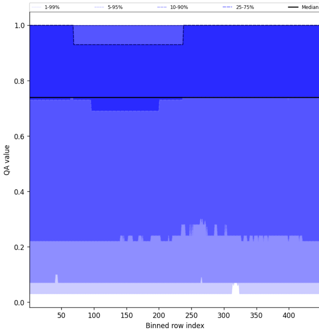
Figure 43: Along track statistics of “QA value” for 2025-01-13 to 2025-01-14
