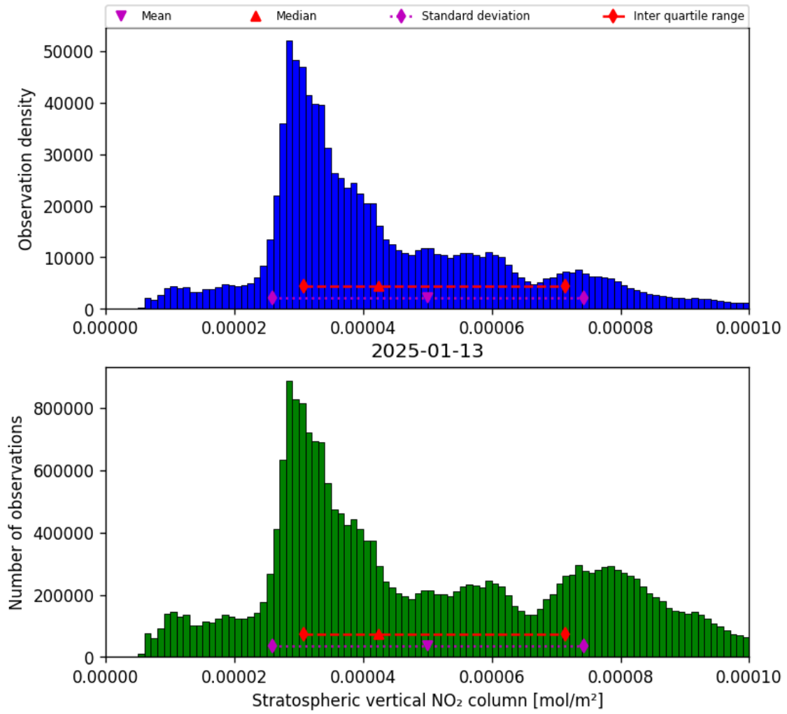
Figure 34: Histogram of “Stratospheric vertical NO 2 column” for 2025-01-13 to 2025-01-14
