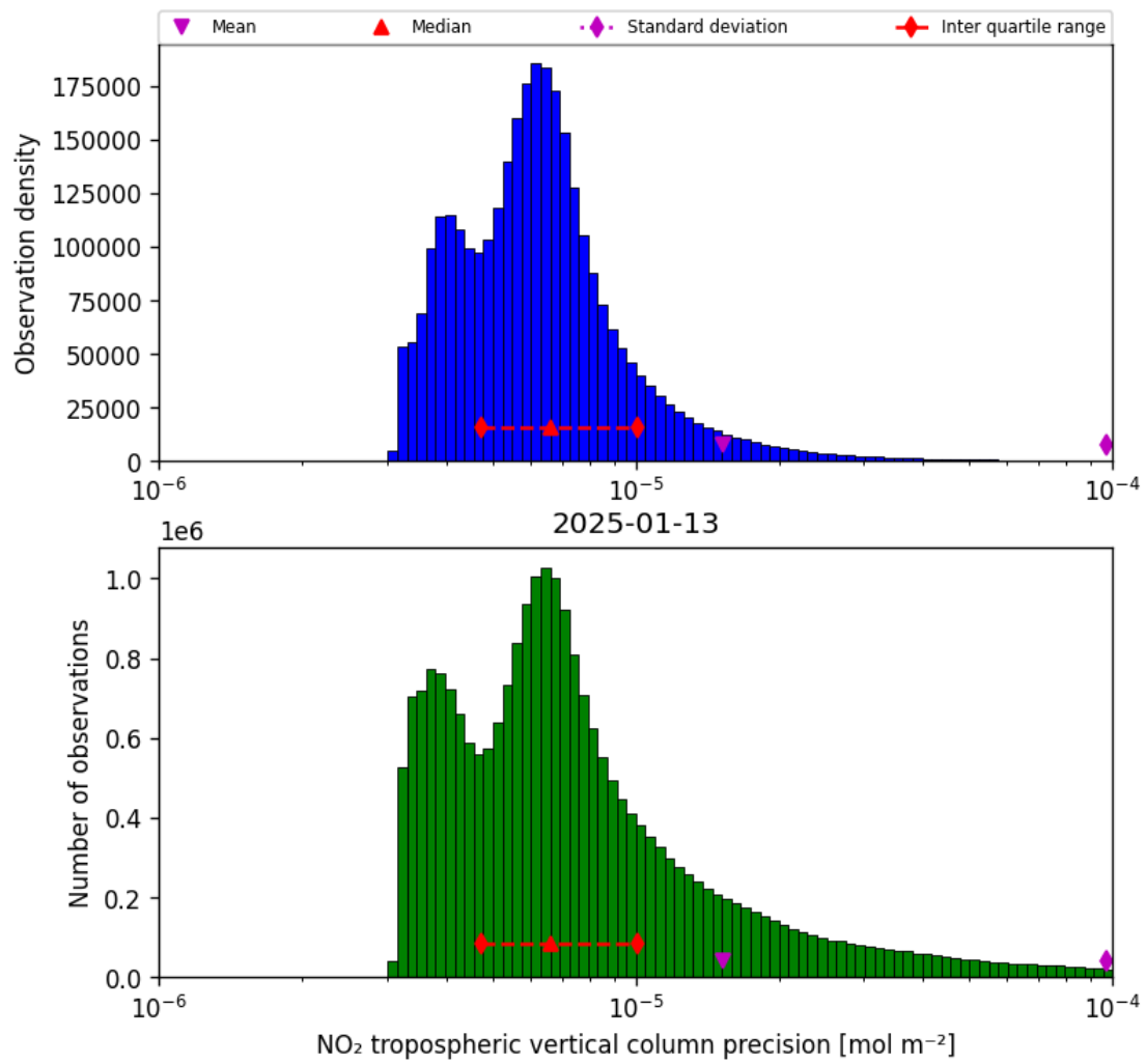
Figure 28: Histogram of “NO 2 tropospheric vertical column precision” for 2025-01-13 to 2025-01-14
