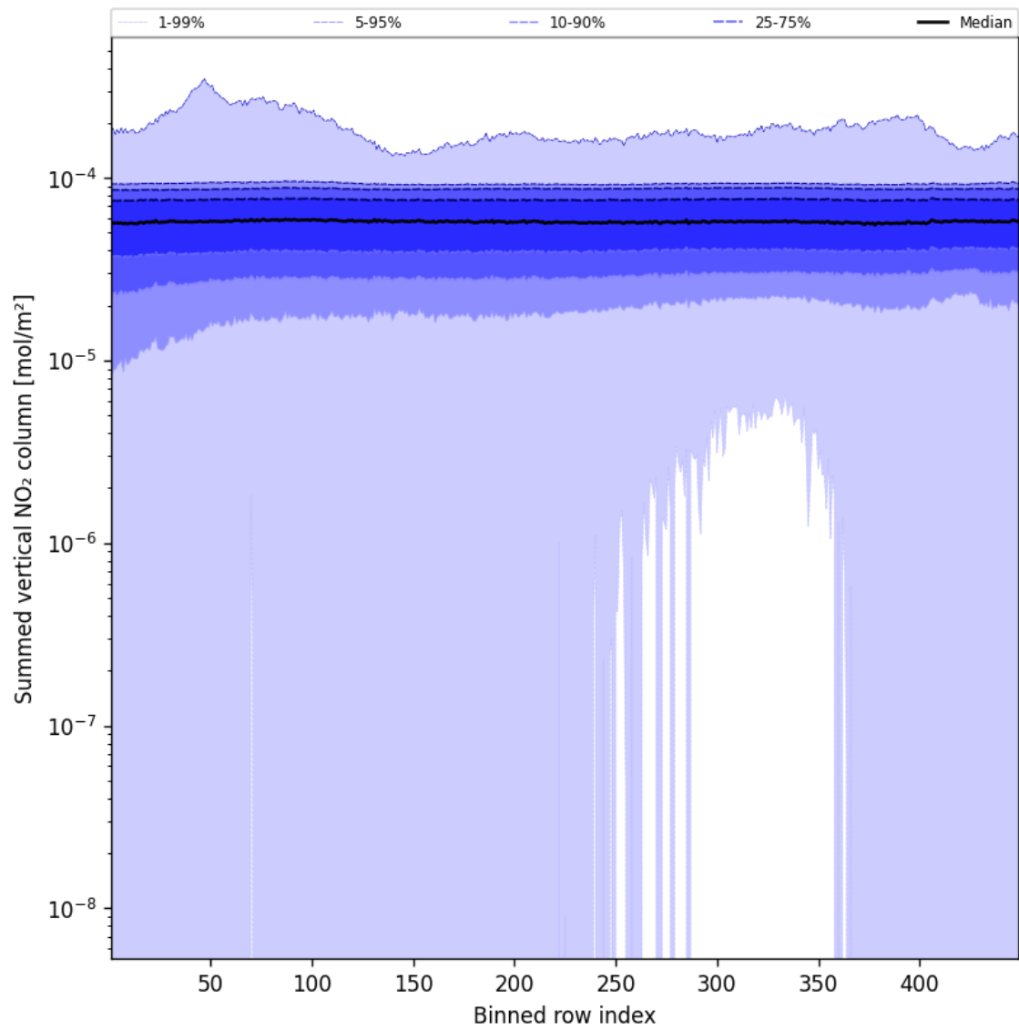
Figure 55: Along track statistics of “Summed vertical NO 2 column” for 2025-01-13 to 2025-01-14
