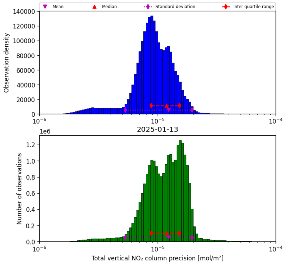
Figure 37: Histogram of “Total vertical NO 2 column precision” for 2025-01-13 to 2025-01-14
