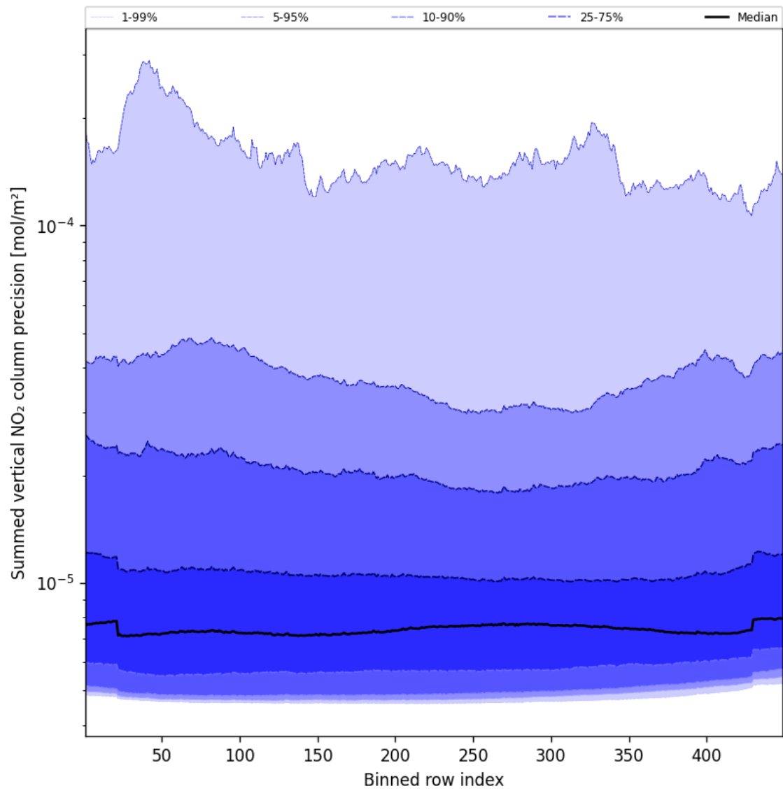
Figure 56: Along track statistics of “Summed vertical NO 2 column precision” for 2025-01-13 to 2025-01-14
