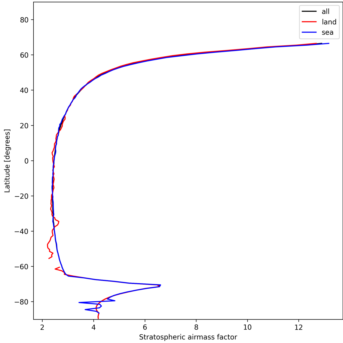
Figure 25: Zonal average of “Stratospheric airmass factor” for 2025-01-13 to 2025-01-14.
