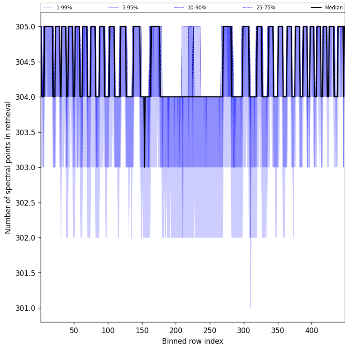
Figure 48: Along track statistics of “Number of spectral points in retrieval” for 2025-01-13 to 2025-01-14
