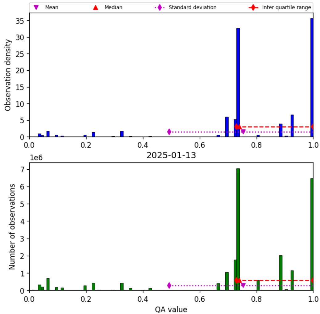
Figure 26: Histogram of “QA value” for 2025-01-13 to 2025-01-14
