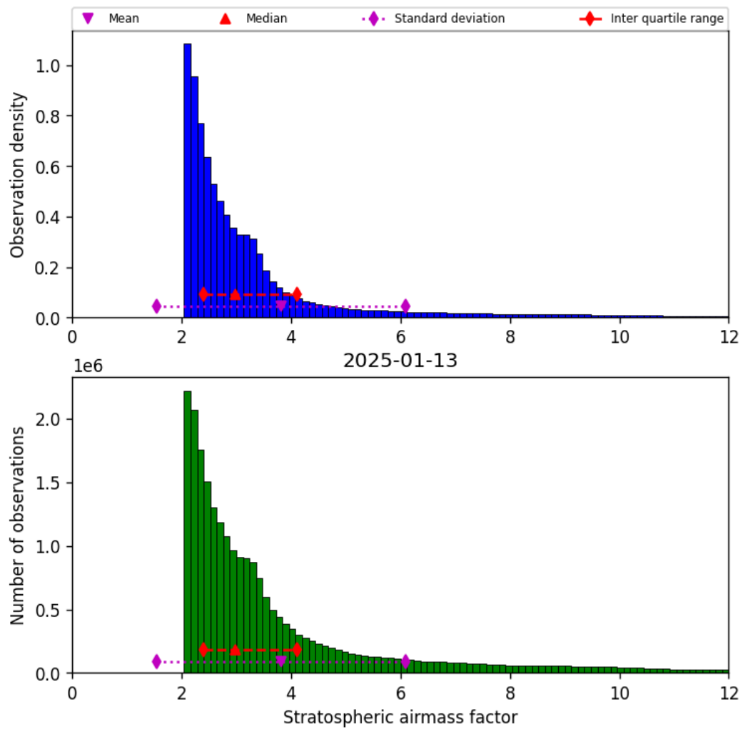
Figure 42: Histogram of “Stratospheric airmass factor” for 2025-01-13 to 2025-01-14
