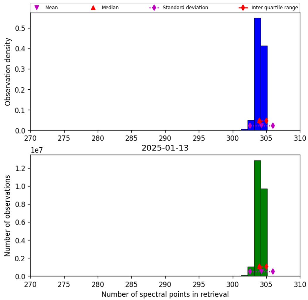
Figure 31: Histogram of “Number of spectral points in retrieval” for 2025-01-13 to 2025-01-14
