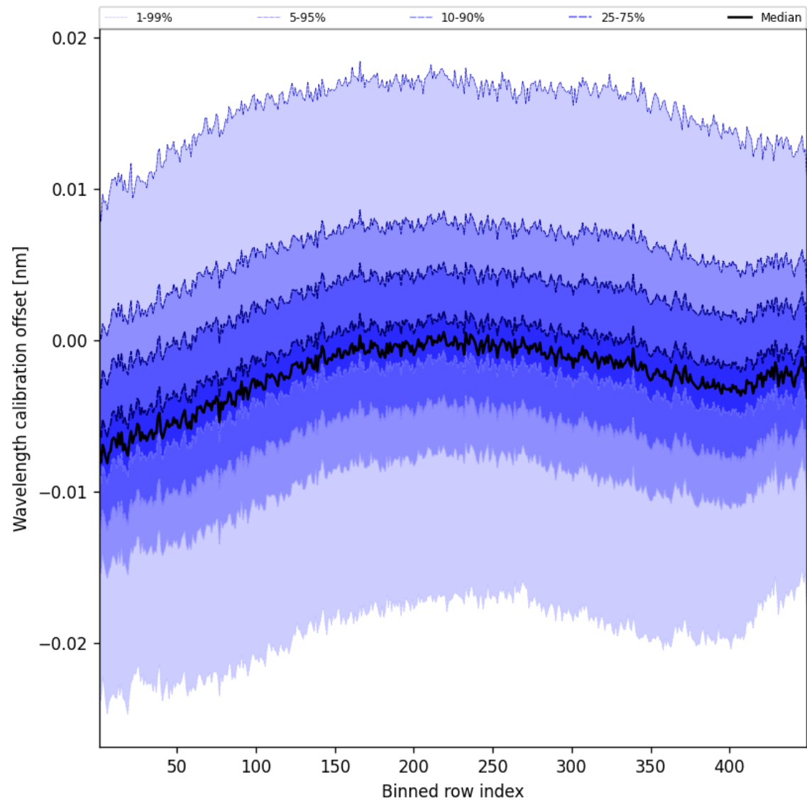
Figure 50: Along track statistics of “Wavelength calibration offset” for 2025-01-13 to 2025-01-14
