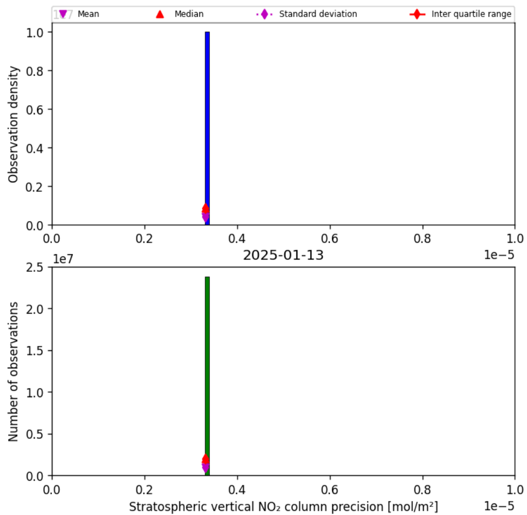
Figure 35: Histogram of “Stratospheric vertical NO 2 column precision” for 2025-01-13 to 2025-01-14
