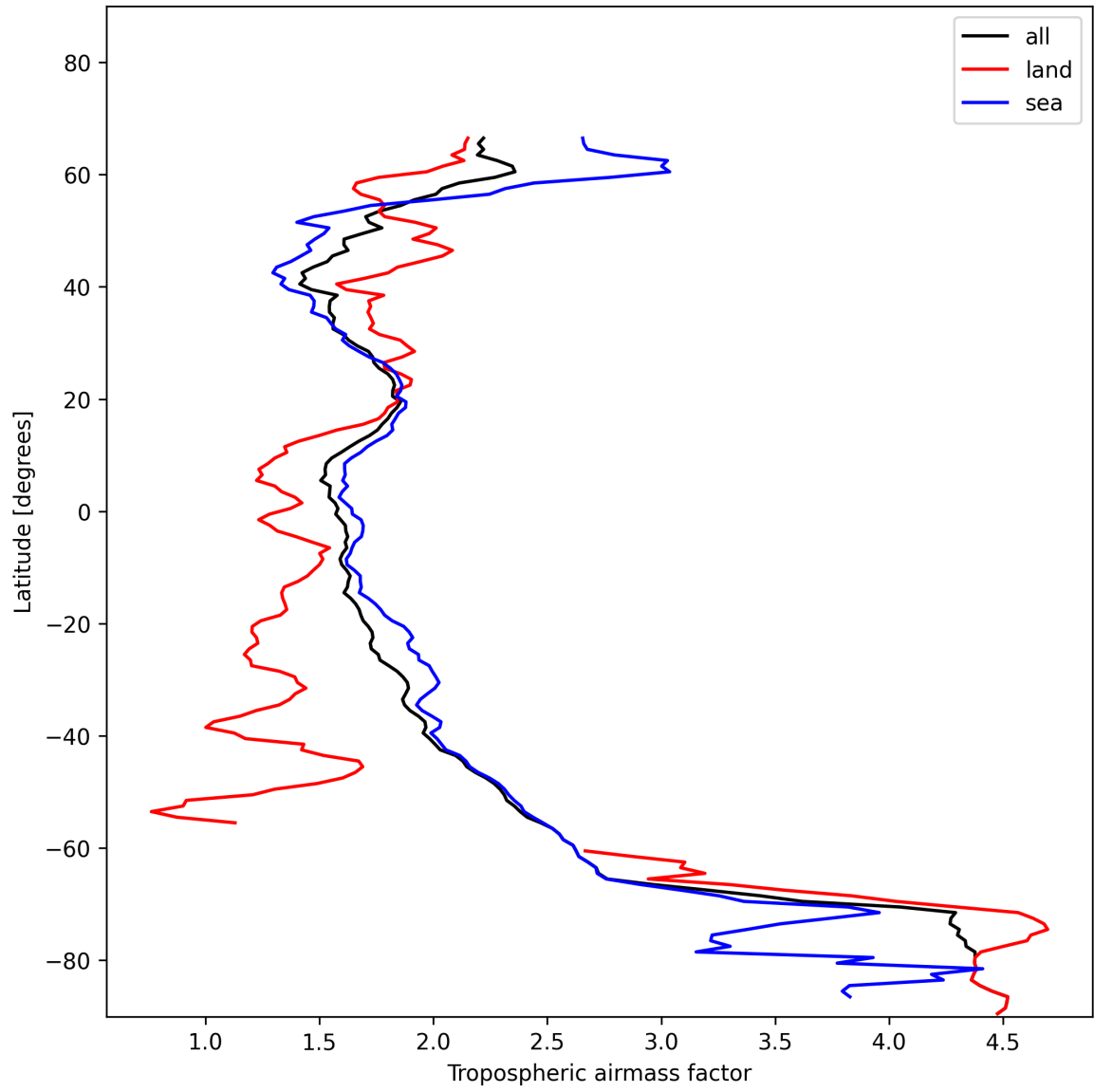
Figure 12: Zonal average of “Tropospheric airmass factor” for 2025-01-13 to 2025-01-14.
