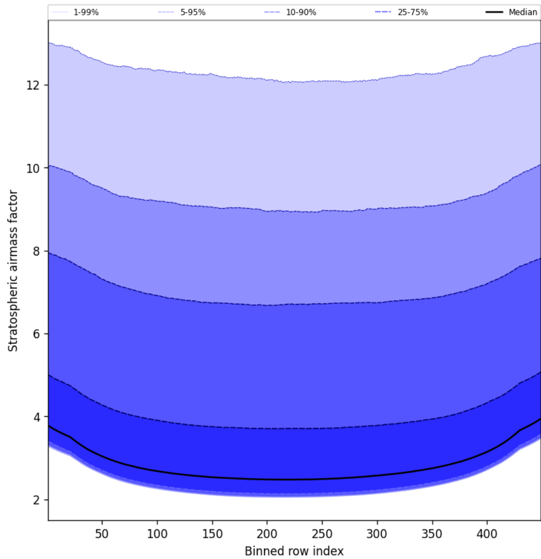
Figure 59: Along track statistics of “Stratospheric airmass factor” for 2025-01-13 to 2025-01-14
