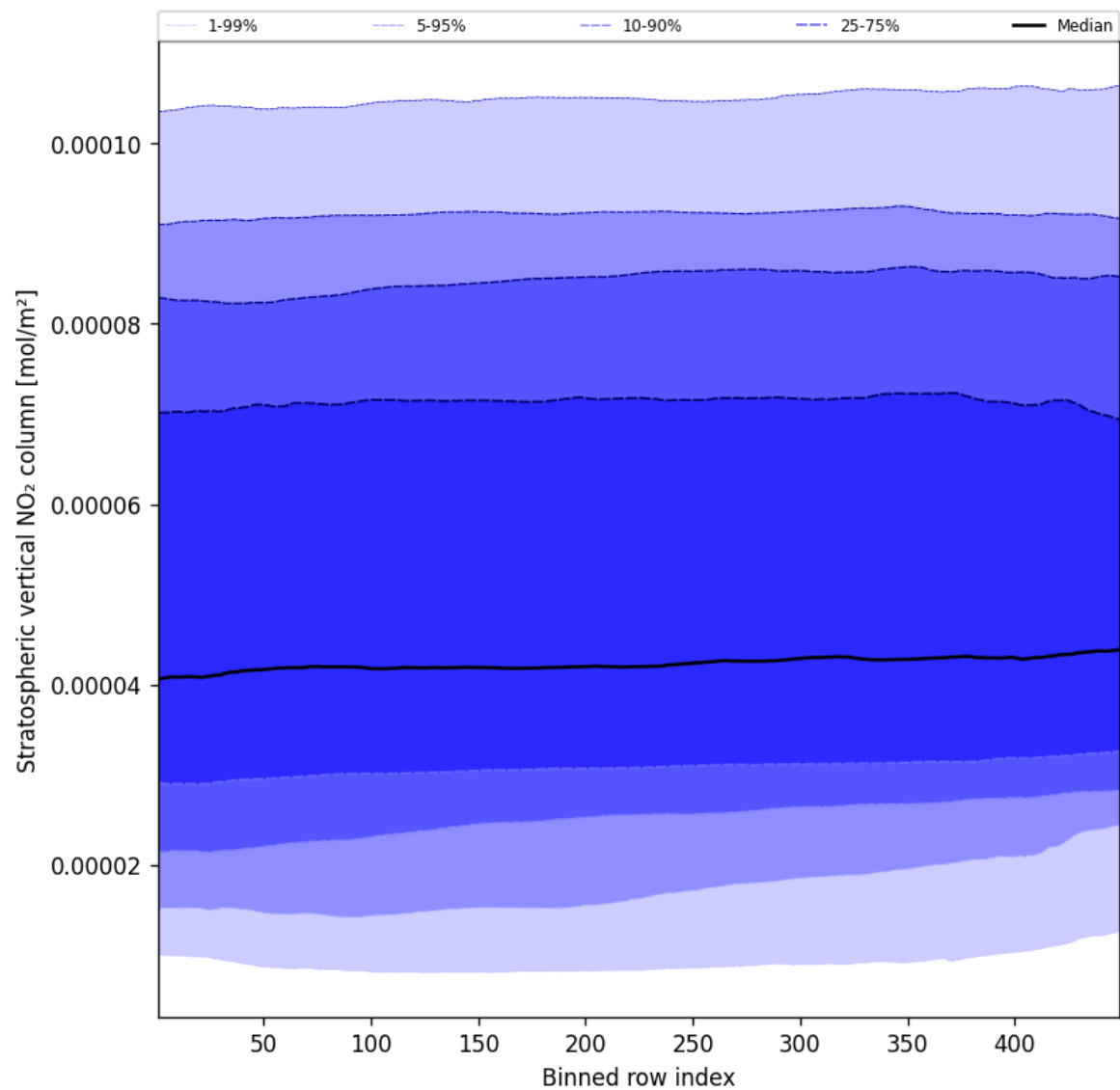
Figure 51: Along track statistics of “Stratospheric vertical NO 2 column” for 2025-01-13 to 2025-01-14
