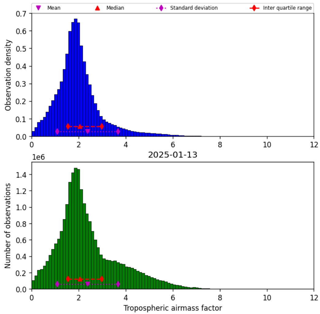
Figure 29: Histogram of “Tropospheric airmass factor” for 2025-01-13 to 2025-01-14
