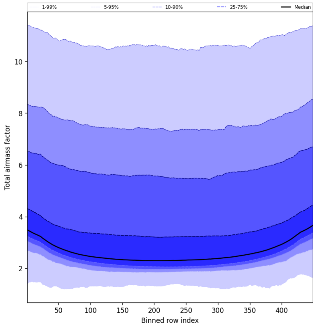
Figure 47: Along track statistics of “Total airmass factor” for 2025-01-13 to 2025-01-14
