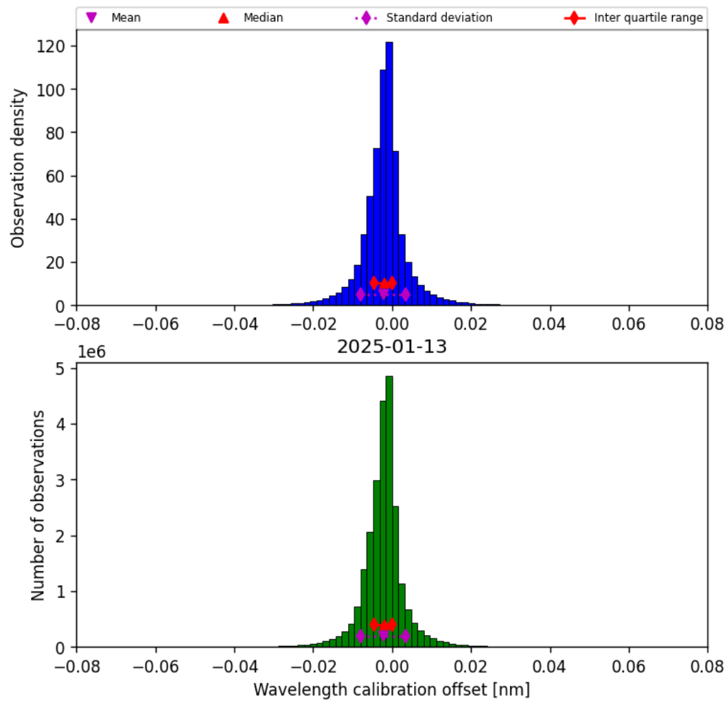
Figure 33: Histogram of “Wavelength calibration offset” for 2025-01-13 to 2025-01-14
