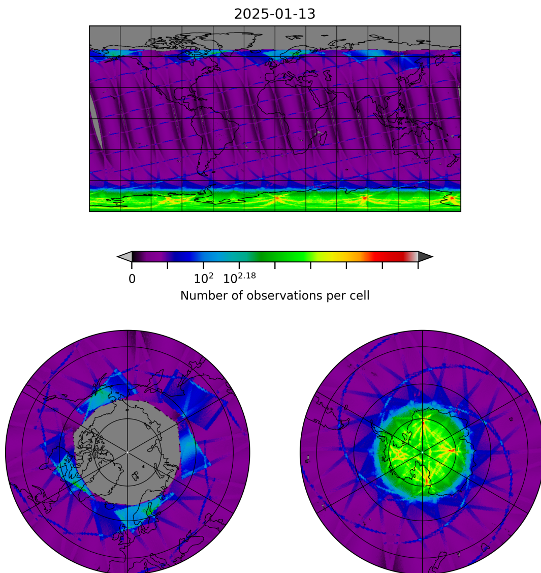
Figure 8: Map of the number of observations for 2025-01-13 to 2025-01-14
