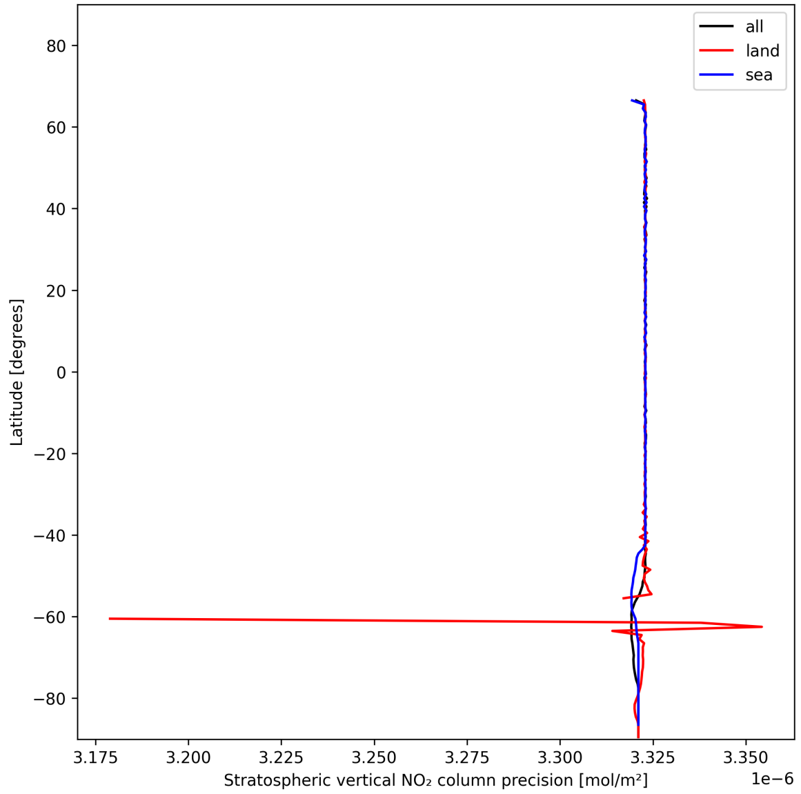
Figure 18: Zonal average of “Stratospheric vertical NO 2 column precision” for 2025-01-13 to 2025-01-14.
