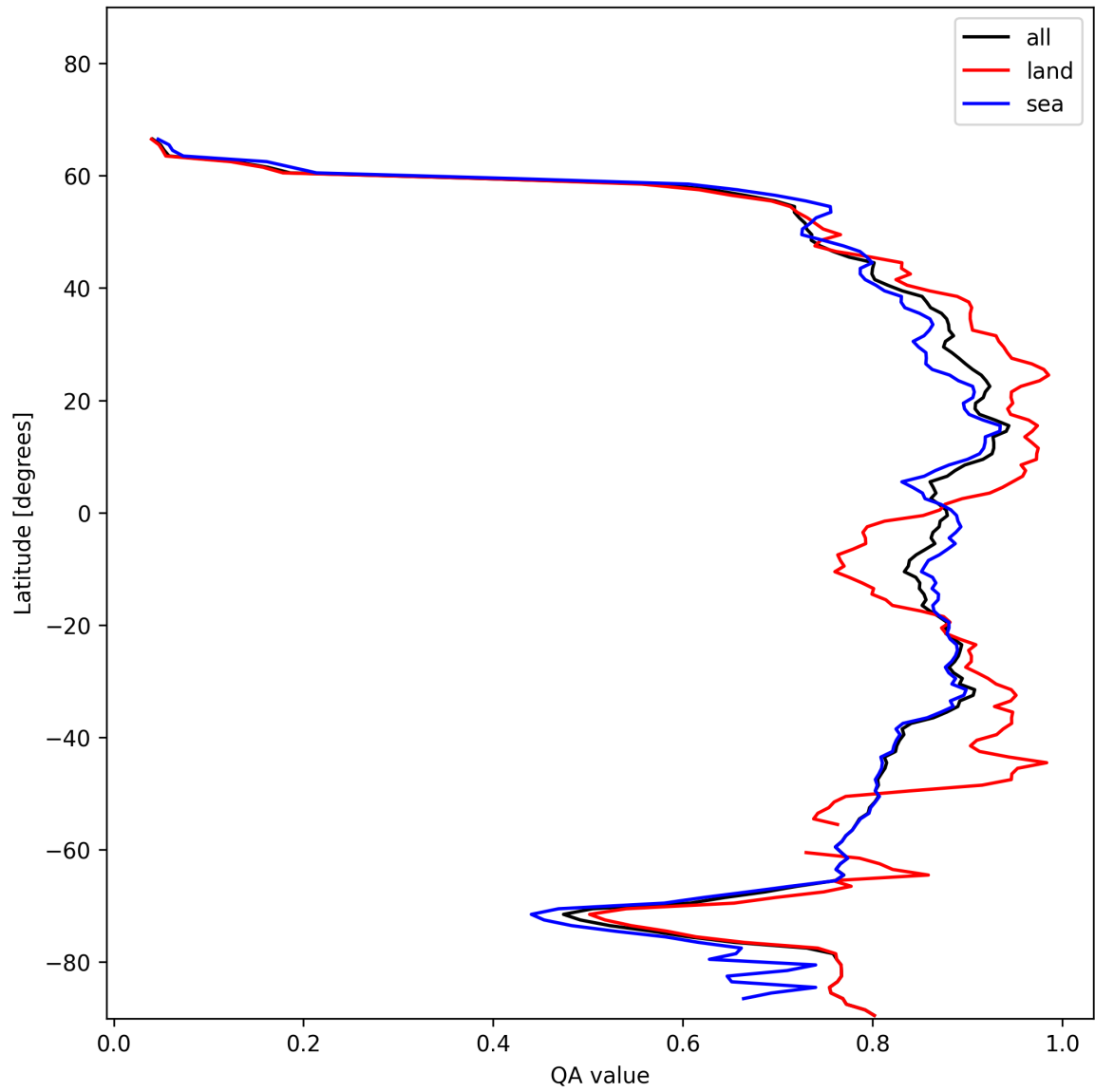
Figure 9: Zonal average of “QA value” for 2025-01-13 to 2025-01-14.
