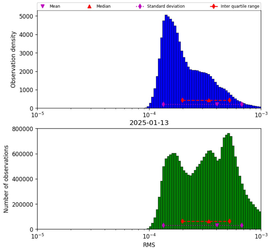
Figure 41: Histogram of “RMS” for 2025-01-13 to 2025-01-14
