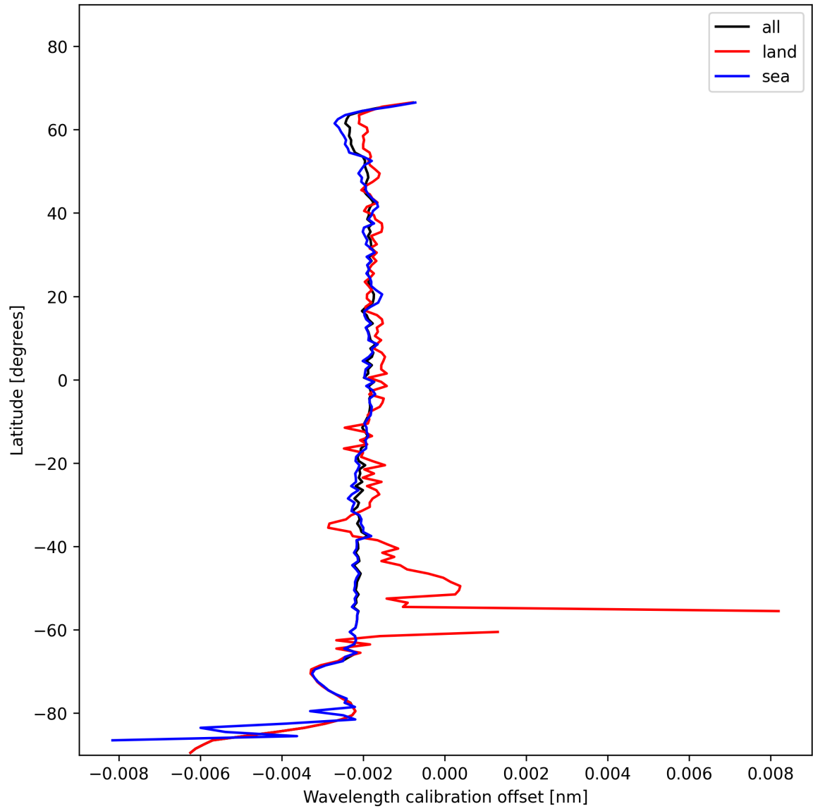
Figure 16: Zonal average of “Wavelength calibration offset” for 2025-01-13 to 2025-01-14.
