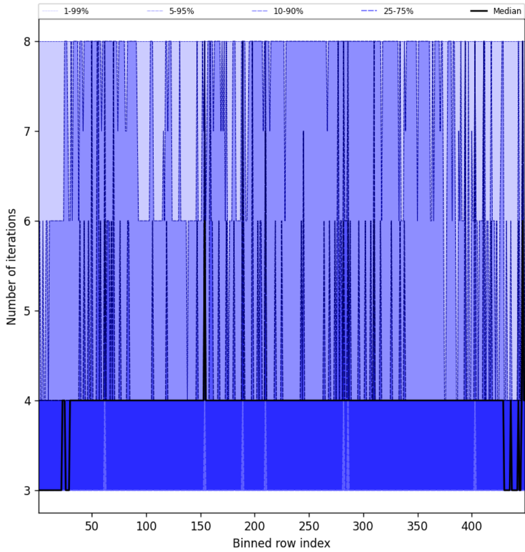
Figure 49: Along track statistics of “Number of iterations” for 2025-01-13 to 2025-01-14
