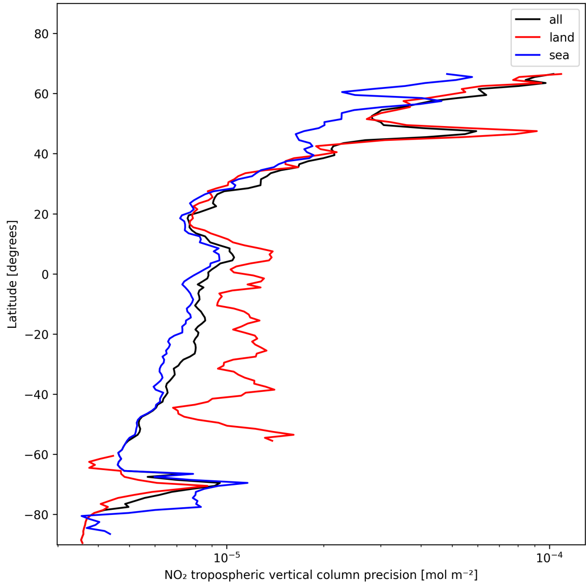
Figure 11: Zonal average of “NO 2 tropospheric vertical column precision” for 2025-01-13 to 2025-01-14.
