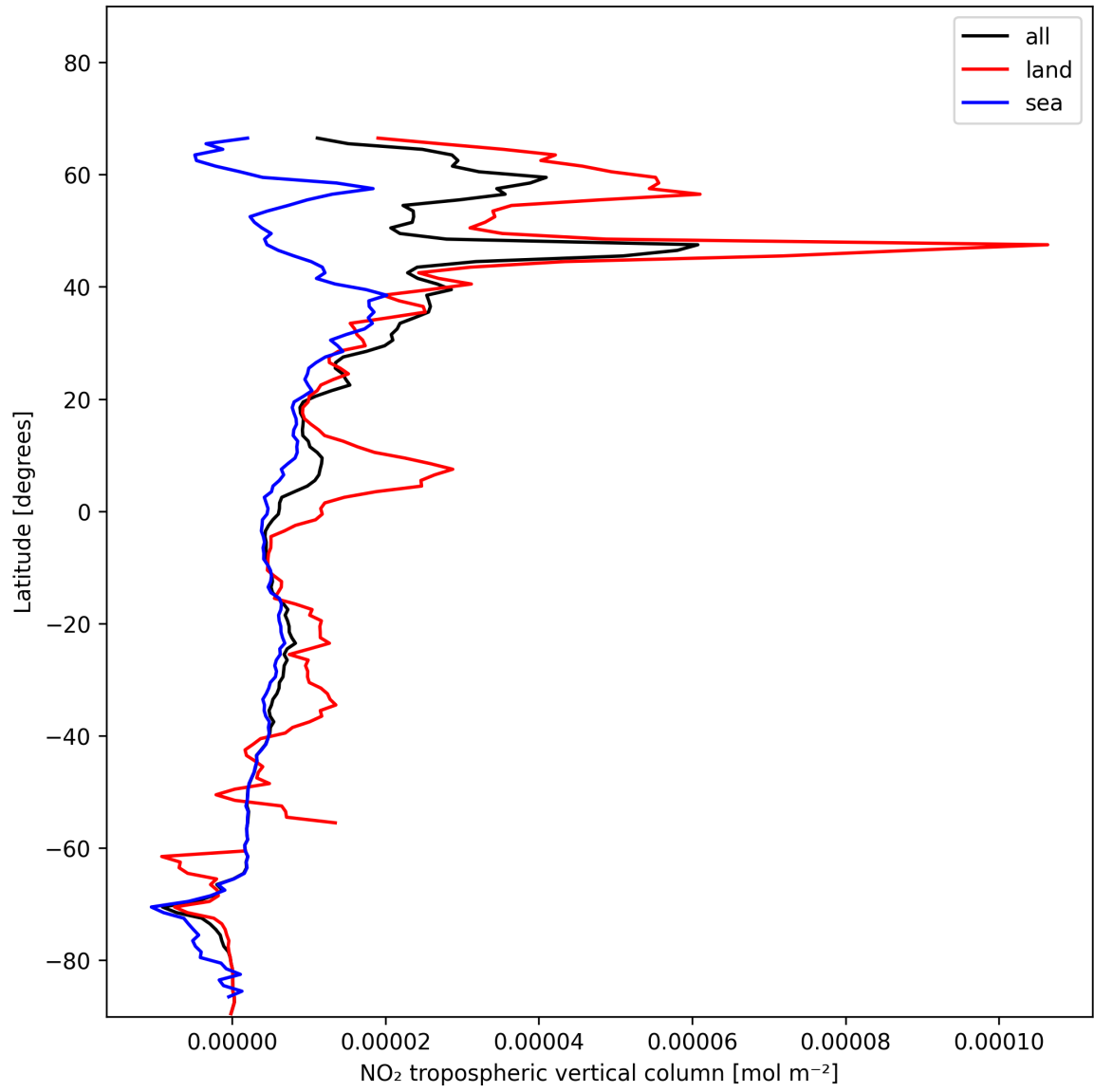
Figure 10: Zonal average of “NO 2 tropospheric vertical column” for 2025-01-13 to 2025-01-14.
