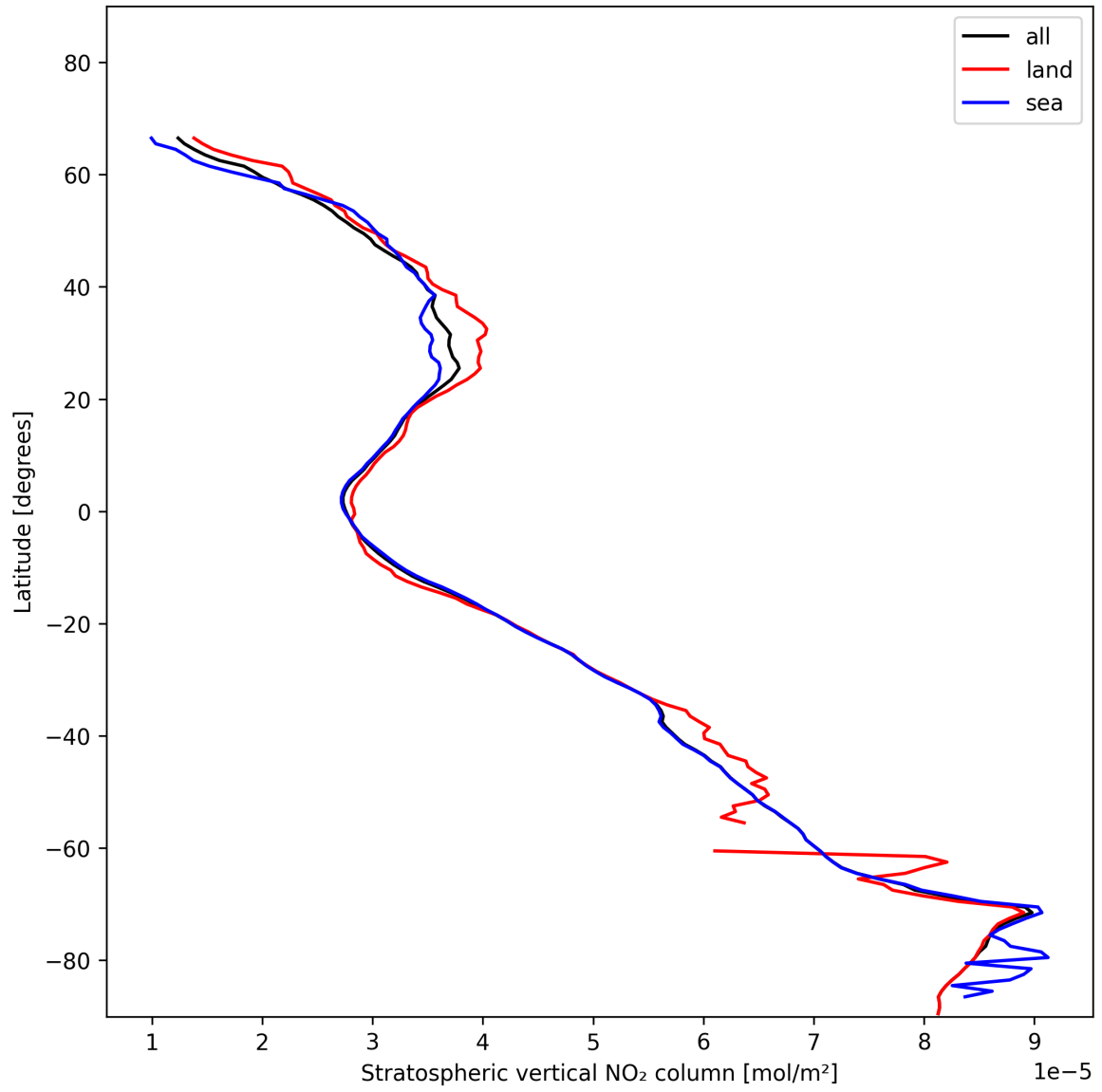
Figure 17: Zonal average of “Stratospheric vertical NO 2 column” for 2025-01-13 to 2025-01-14.
