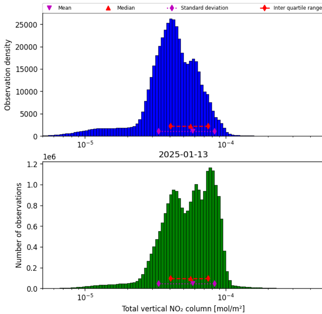
Figure 36: Histogram of “Total vertical NO 2 column” for 2025-01-13 to 2025-01-14
