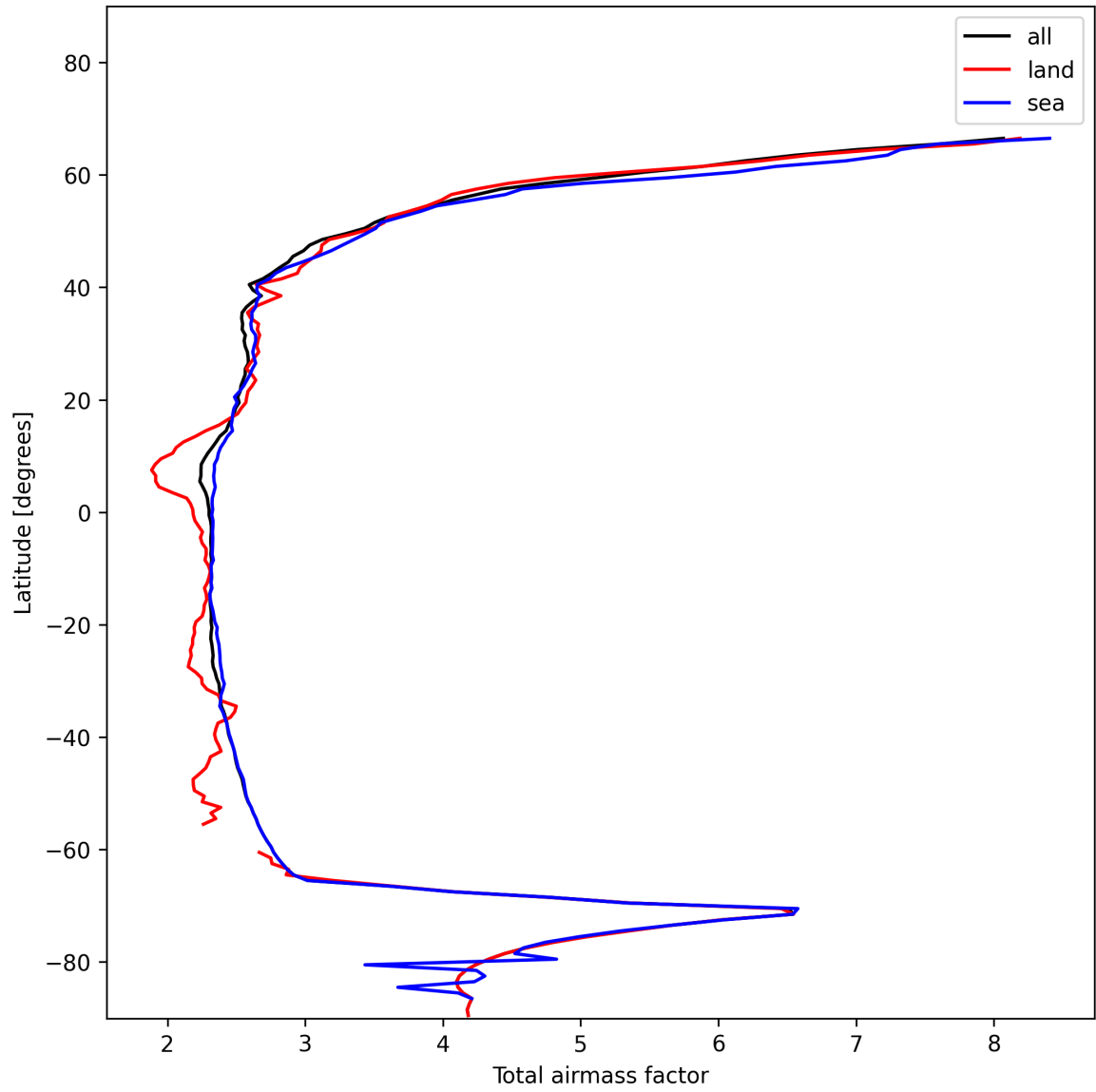
Figure 13: Zonal average of “Total airmass factor” for 2025-01-13 to 2025-01-14.
