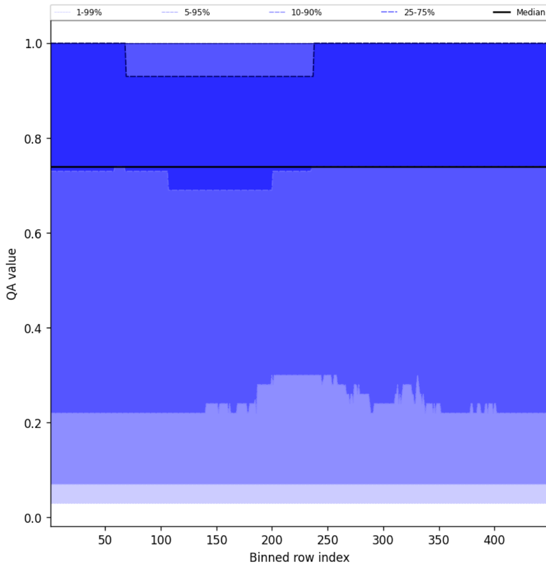
Figure 43: Along track statistics of “QA value” for 2025-01-14 to 2025-01-15
