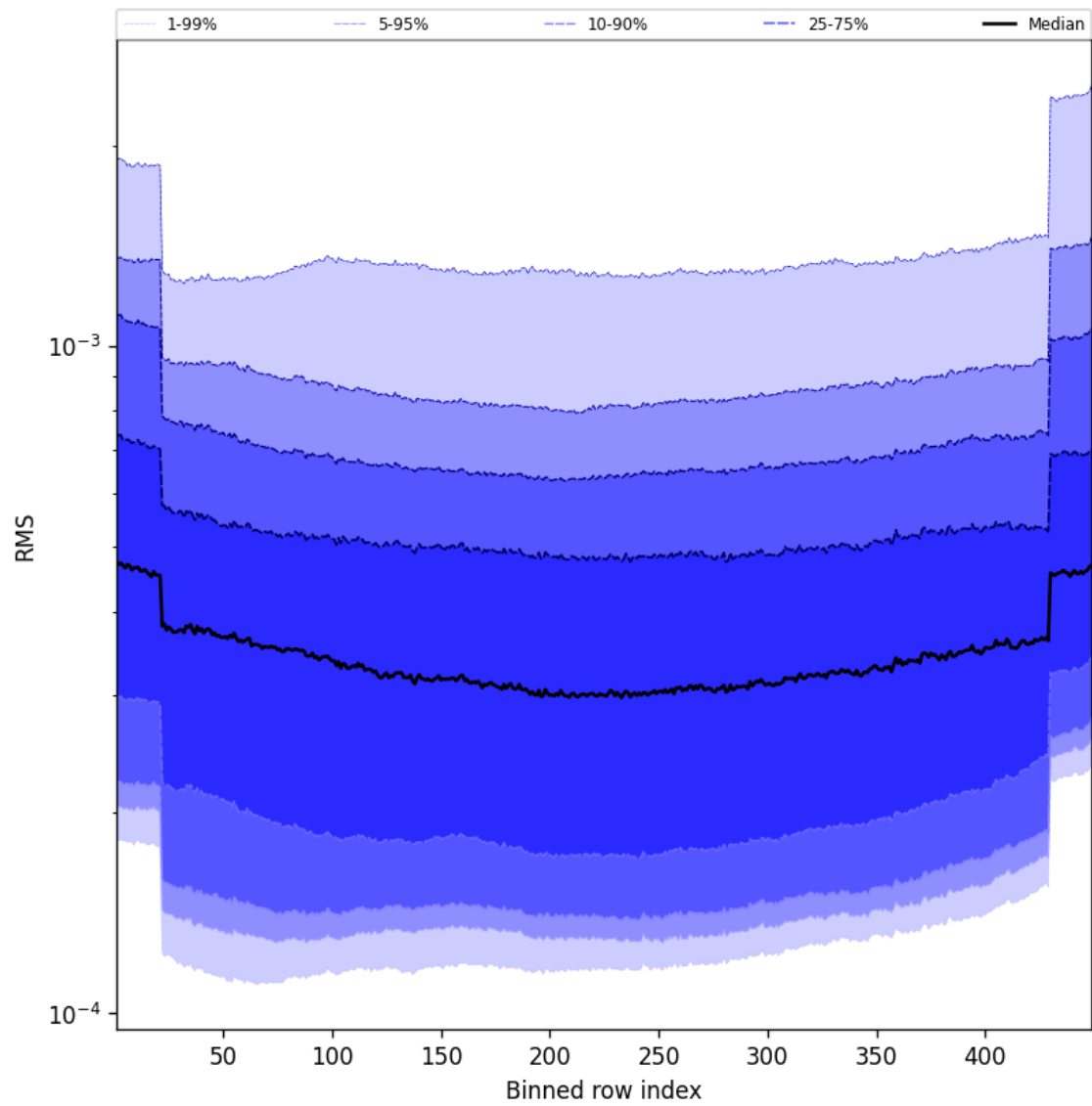
Figure 58: Along track statistics of “RMS” for 2025-01-14 to 2025-01-15
