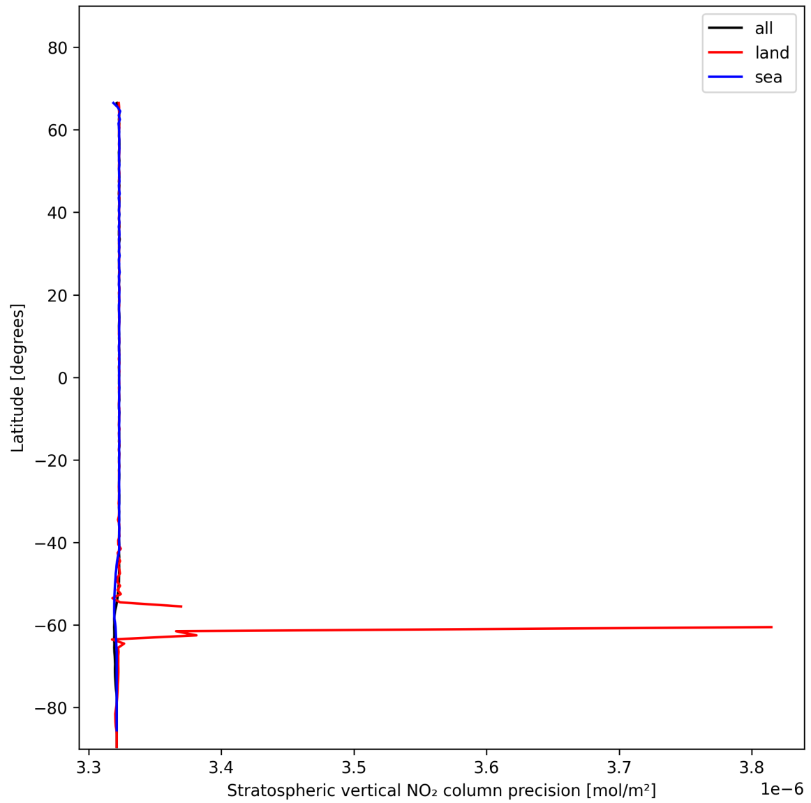
Figure 18: Zonal average of “Stratospheric vertical NO 2 column precision” for 2025-01-14 to 2025-01-15.
