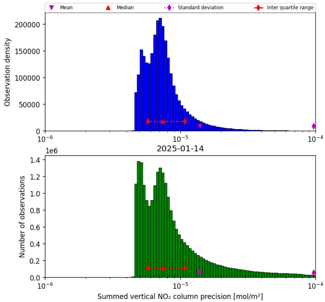
Figure 39: Histogram of “Summed vertical NO 2 column precision” for 2025-01-14 to 2025-01-15
