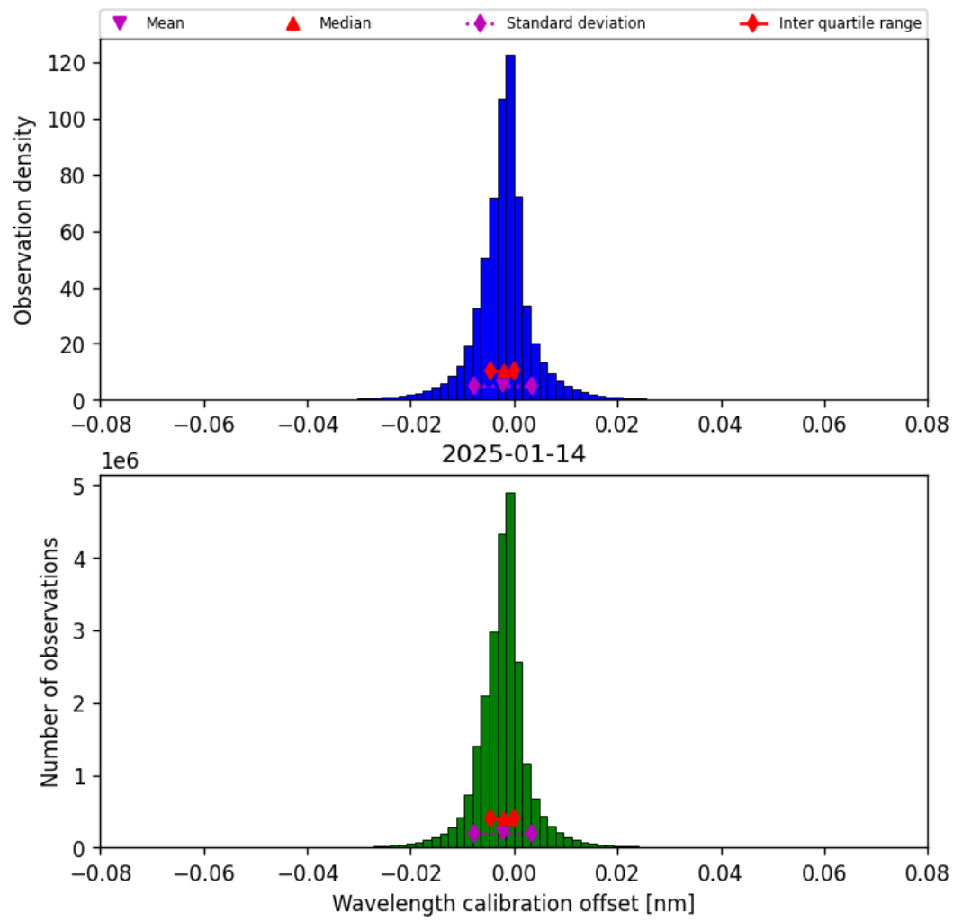
Figure 33: Histogram of “Wavelength calibration offset” for 2025-01-14 to 2025-01-15
