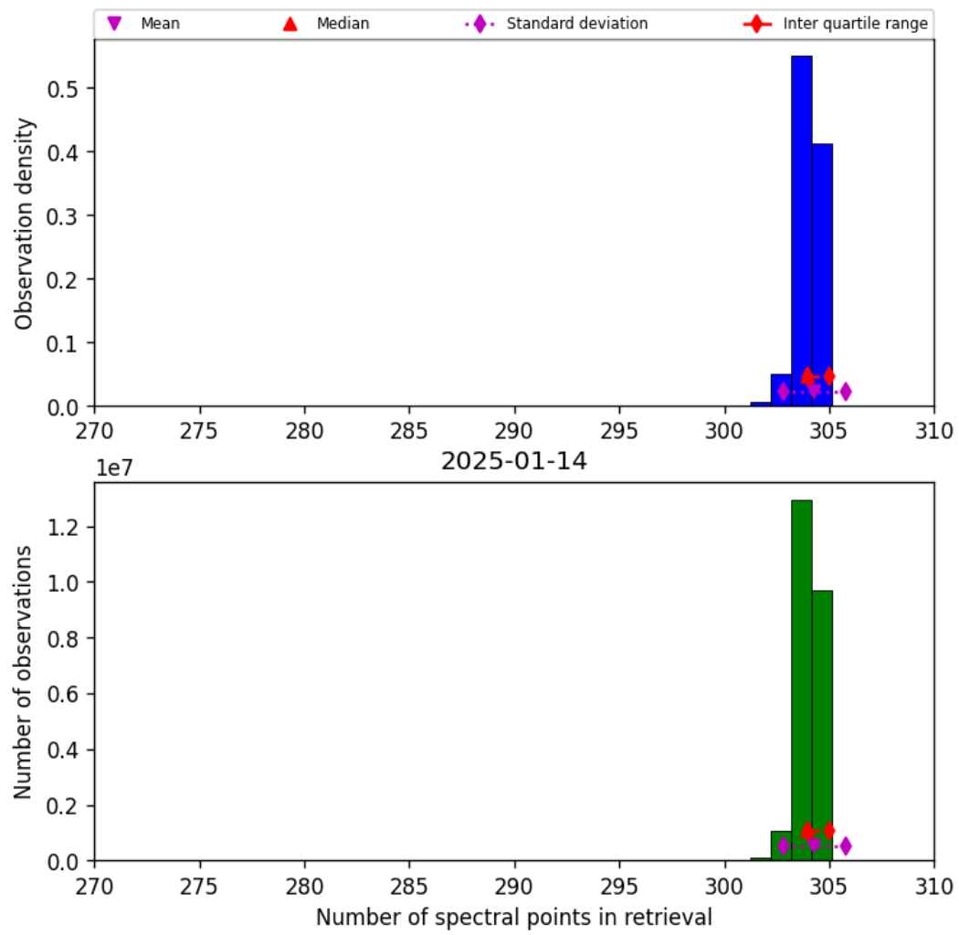
Figure 31: Histogram of “Number of spectral points in retrieval” for 2025-01-14 to 2025-01-15
