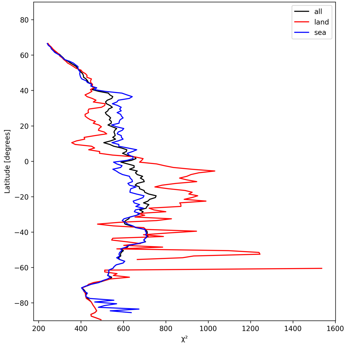
Figure 23: Zonal average of “ \chi^2 ” for 2025-01-14 to 2025-01-15.
