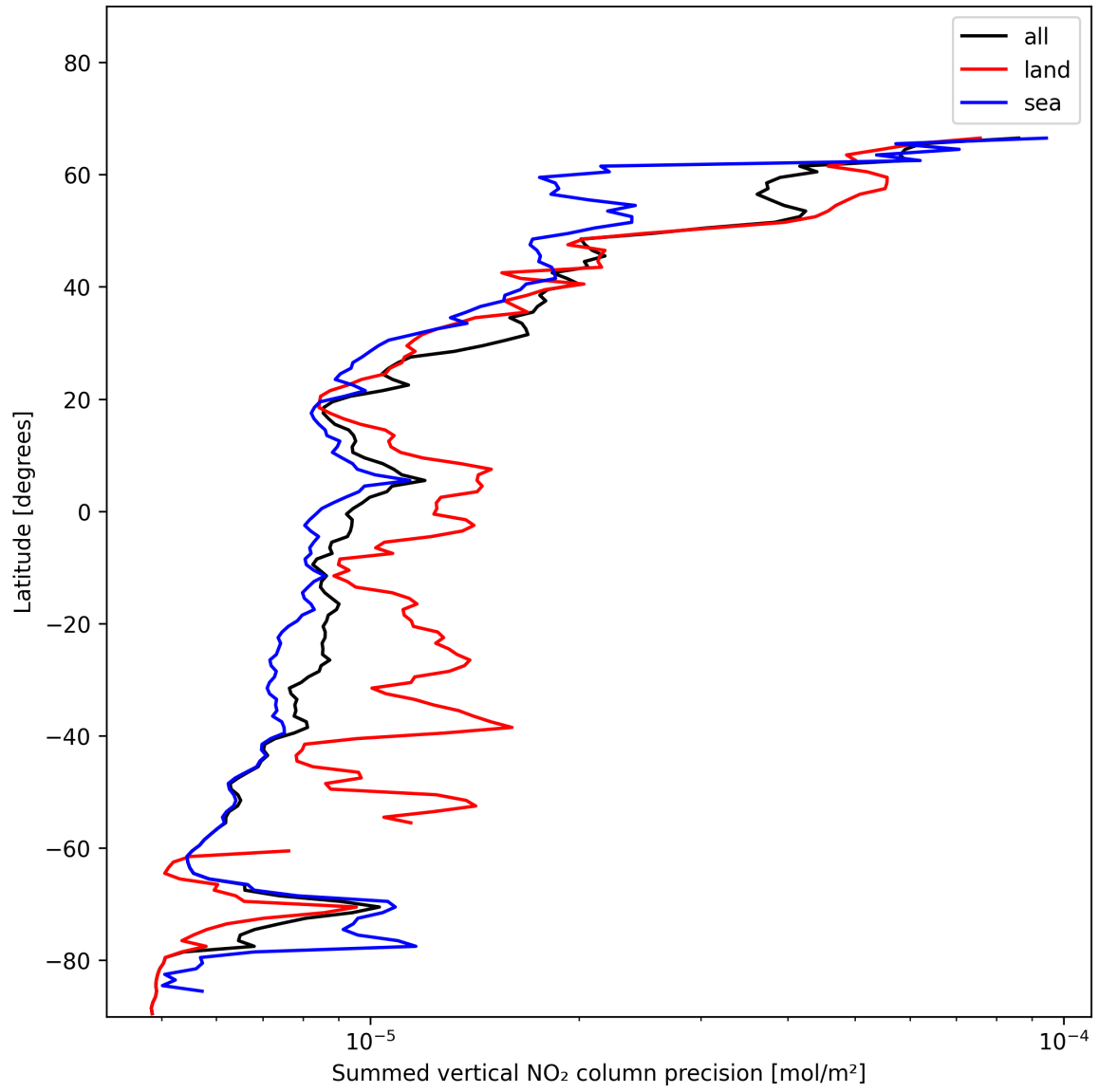
Figure 22: Zonal average of “Summed vertical NO 2 column precision” for 2025-01-14 to 2025-01-15.
