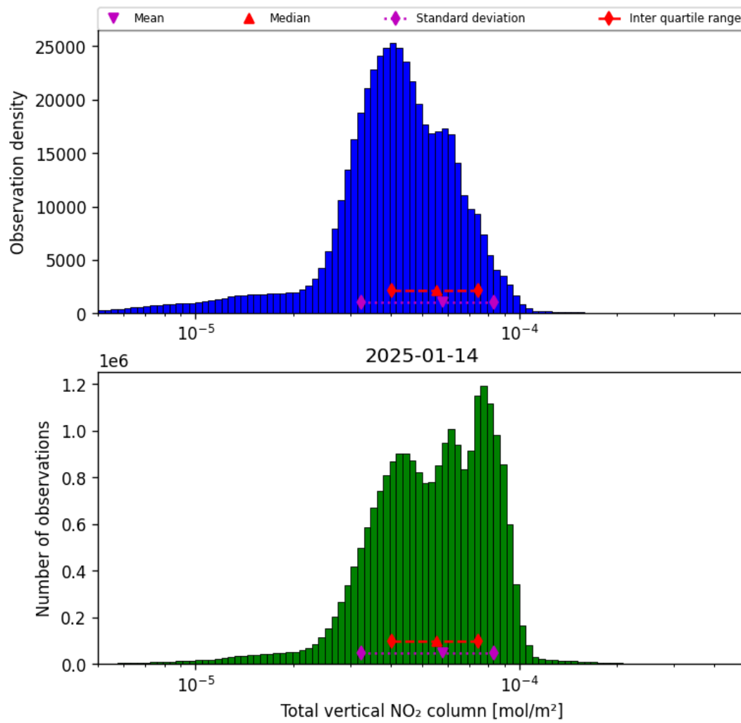
Figure 36: Histogram of “Total vertical NO 2 column” for 2025-01-14 to 2025-01-15
