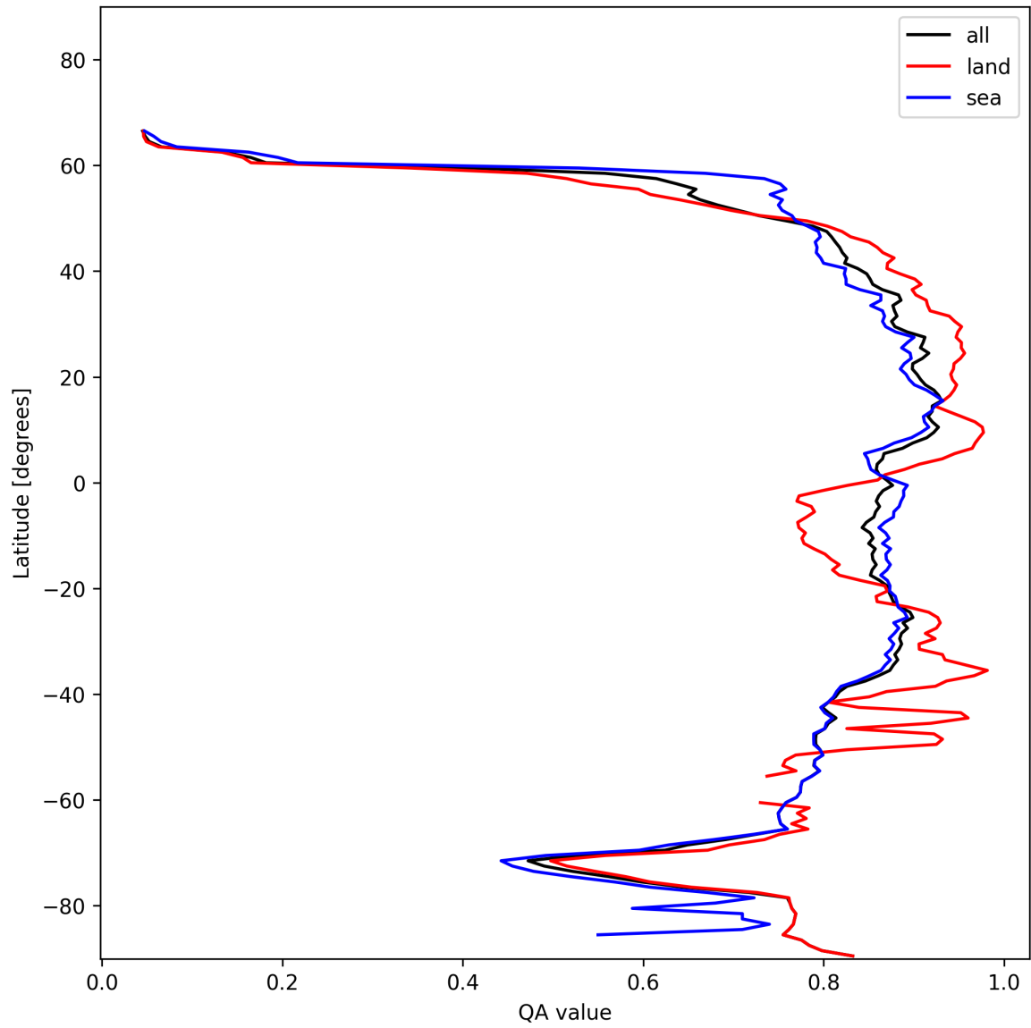
Figure 9: Zonal average of “QA value” for 2025-01-14 to 2025-01-15.
