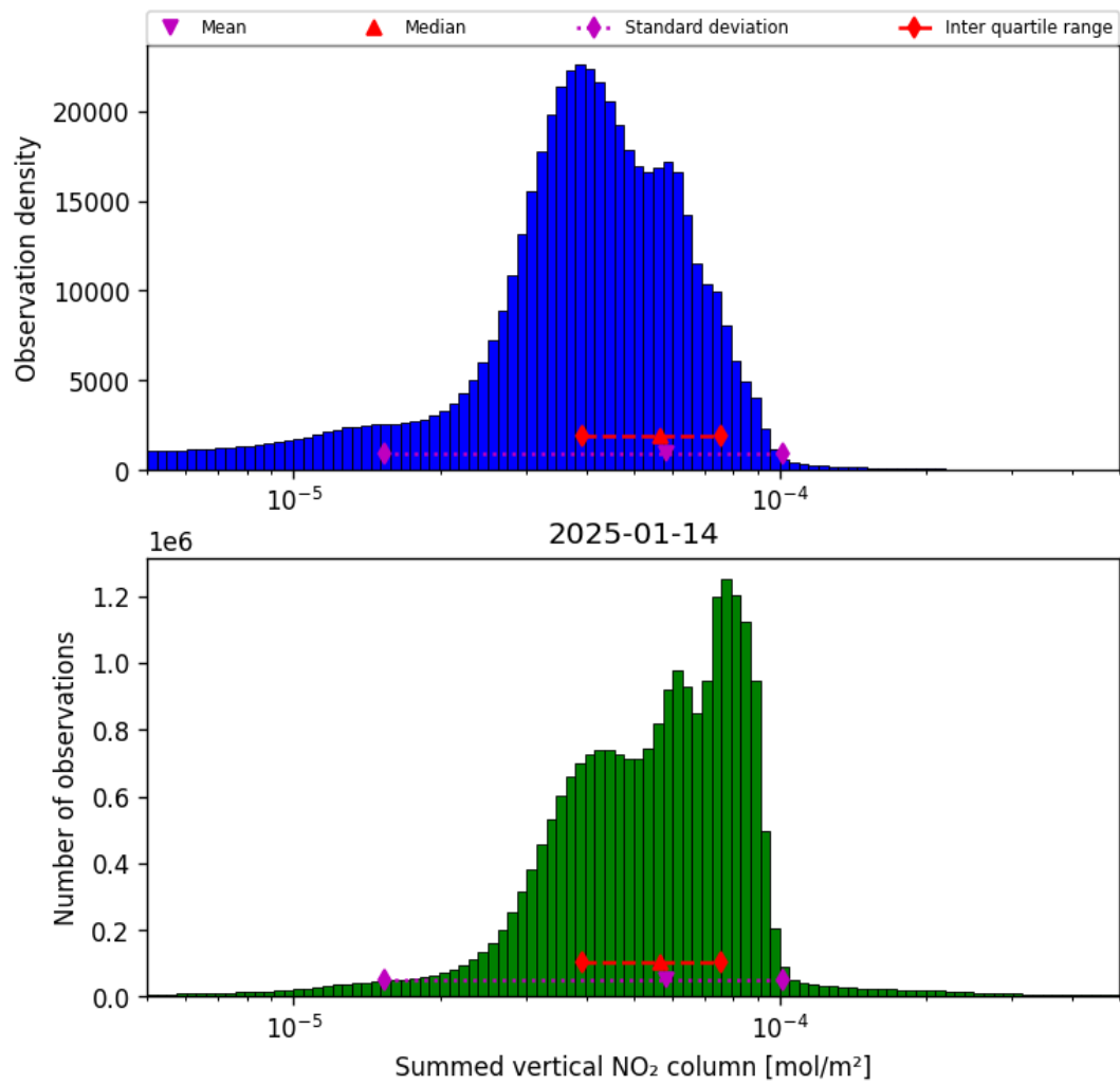
Figure 38: Histogram of “Summed vertical NO 2 column” for 2025-01-14 to 2025-01-15
