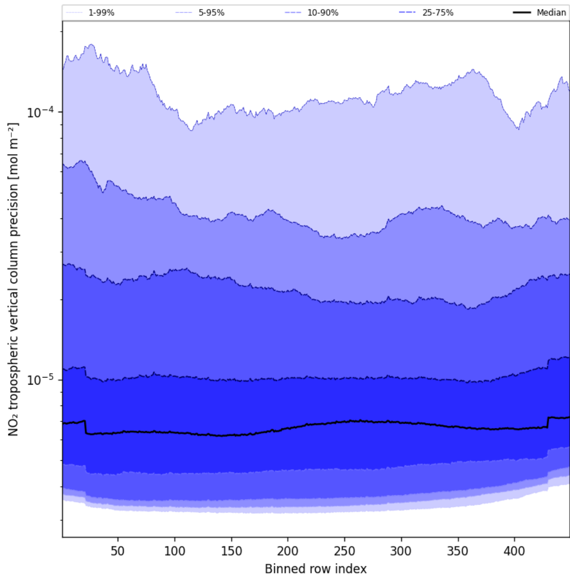
Figure 45: Along track statistics of “NO 2 tropospheric vertical column precision” for 2025-01-14 to 2025-01-15
