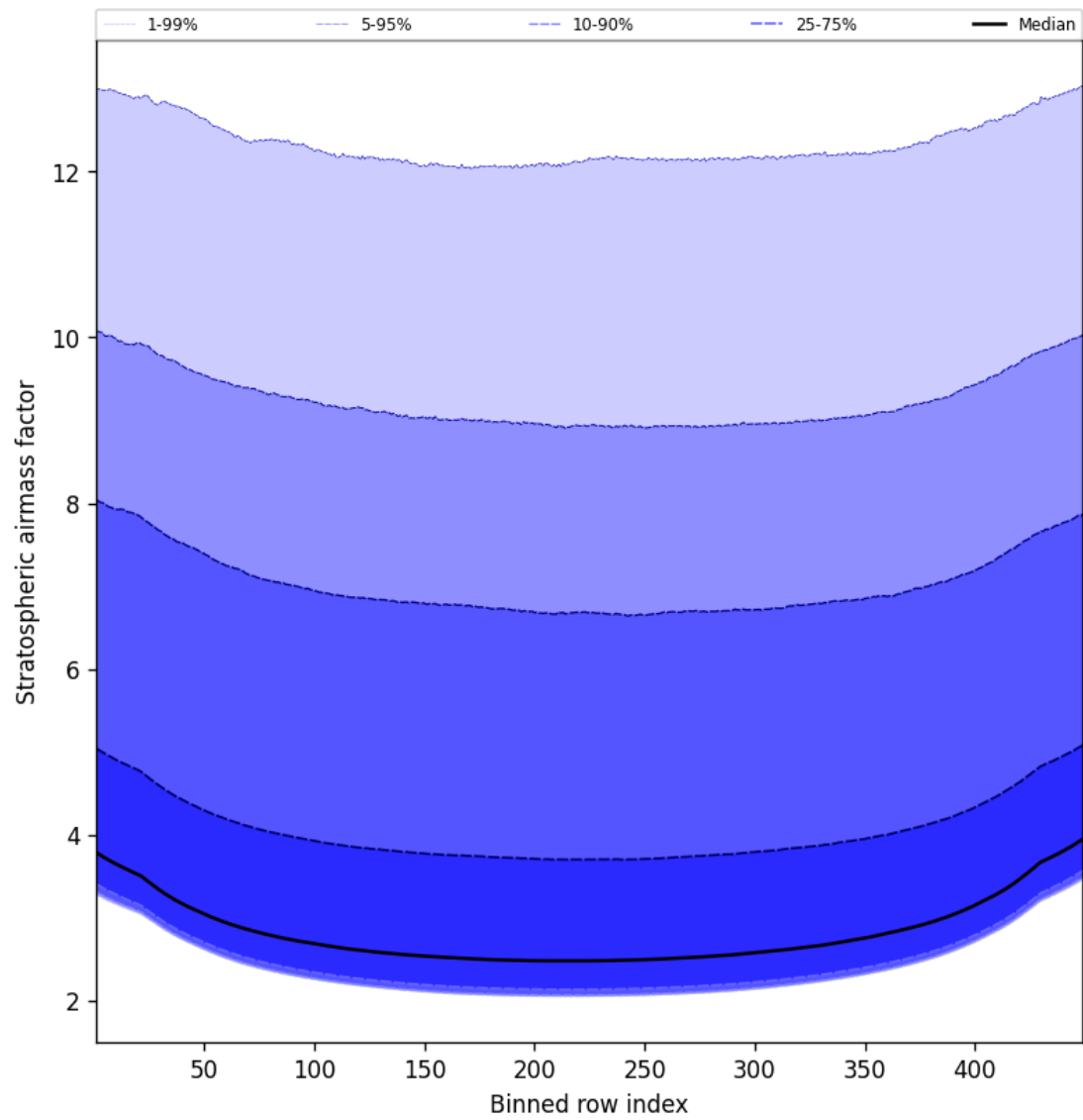
Figure 59: Along track statistics of “Stratospheric airmass factor” for 2025-01-14 to 2025-01-15
