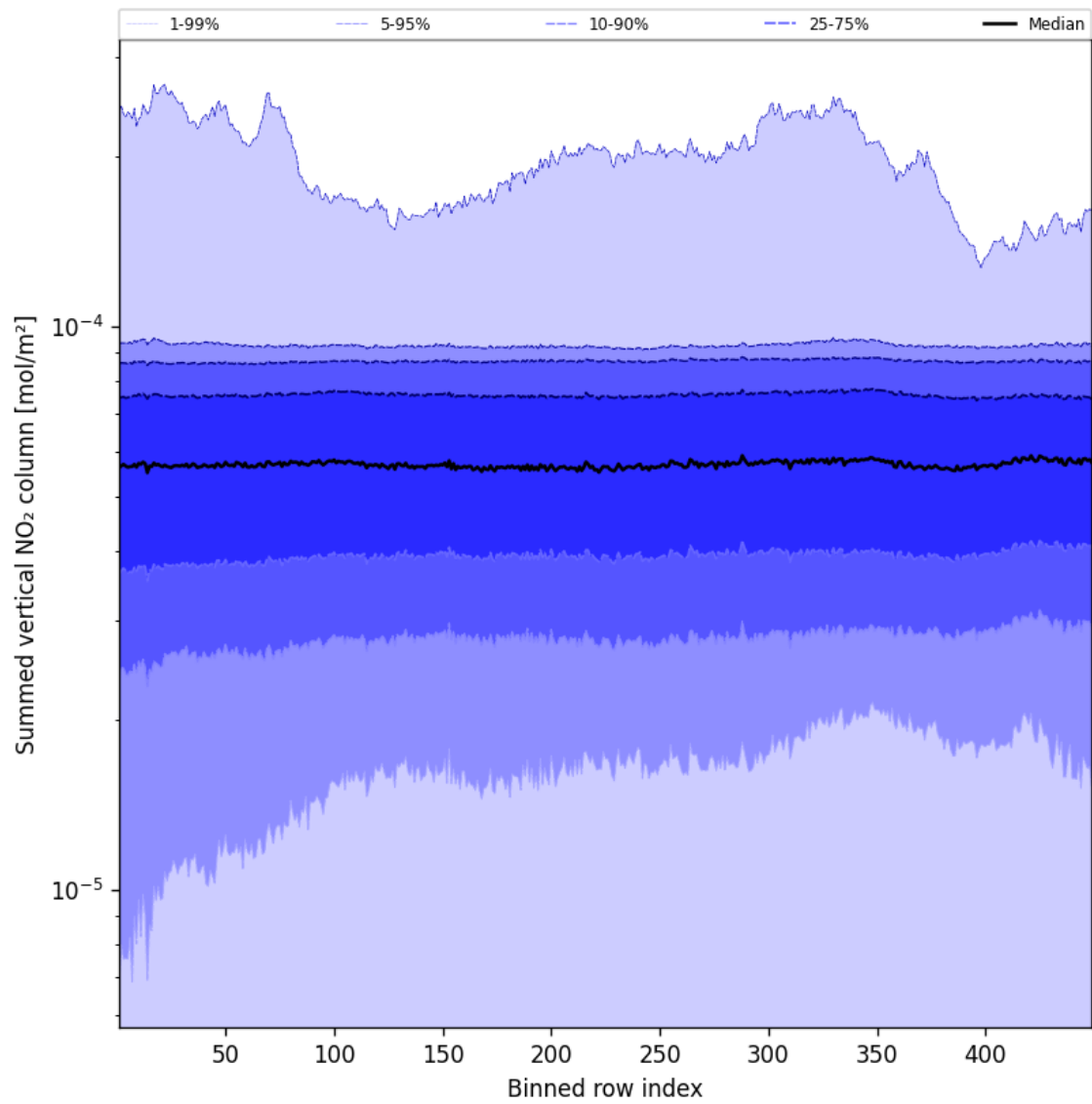
Figure 55: Along track statistics of “Summed vertical NO 2 column” for 2025-01-14 to 2025-01-15
