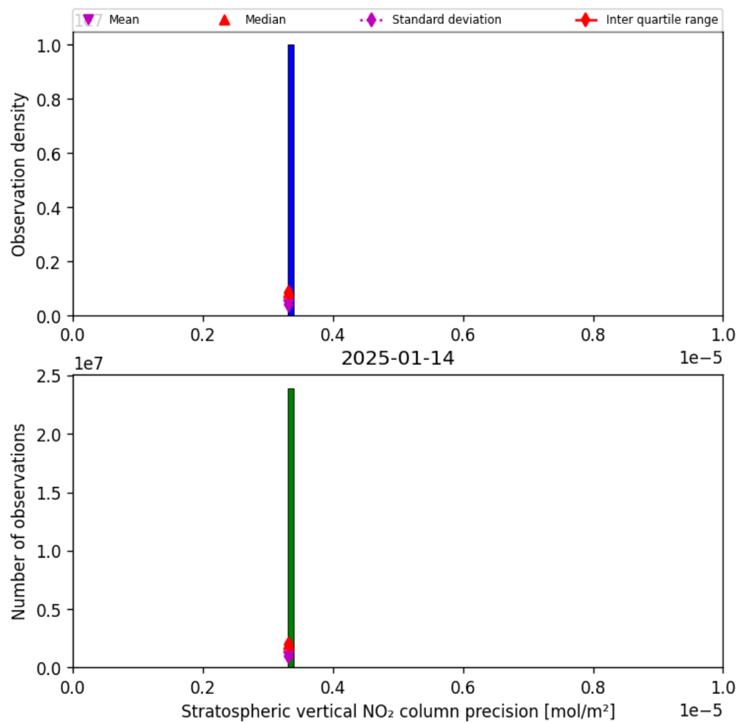
Figure 35: Histogram of “Stratospheric vertical NO 2 column precision” for 2025-01-14 to 2025-01-15
