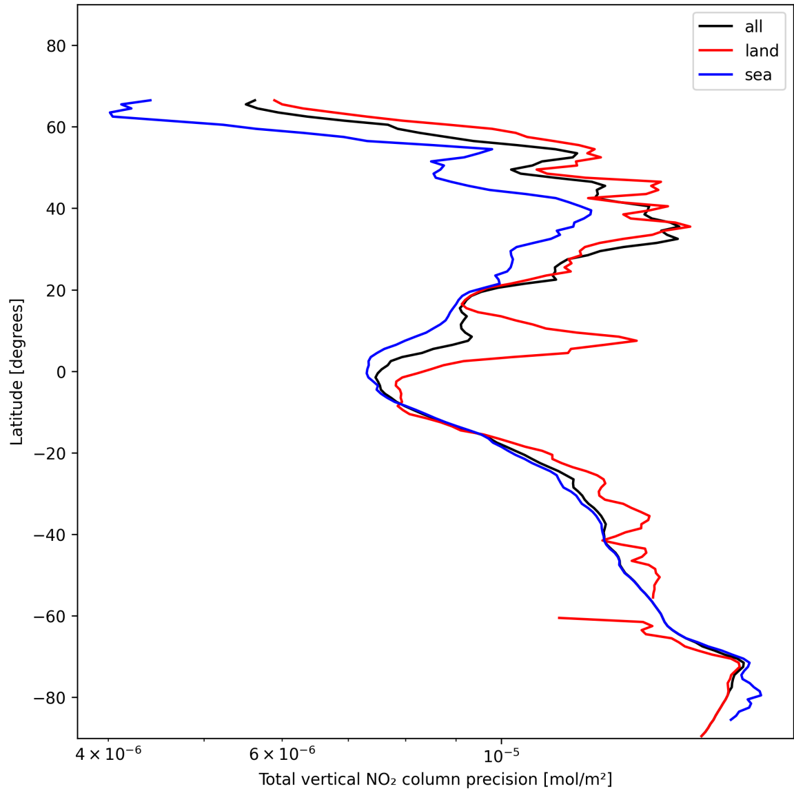
Figure 20: Zonal average of “Total vertical NO 2 column precision” for 2025-01-14 to 2025-01-15.
