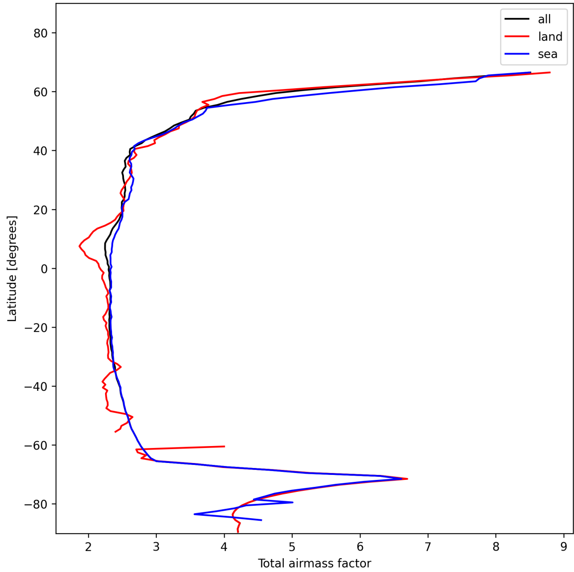
Figure 13: Zonal average of “Total airmass factor” for 2025-01-14 to 2025-01-15.
