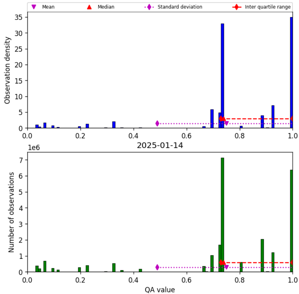
Figure 26: Histogram of “QA value” for 2025-01-14 to 2025-01-15
