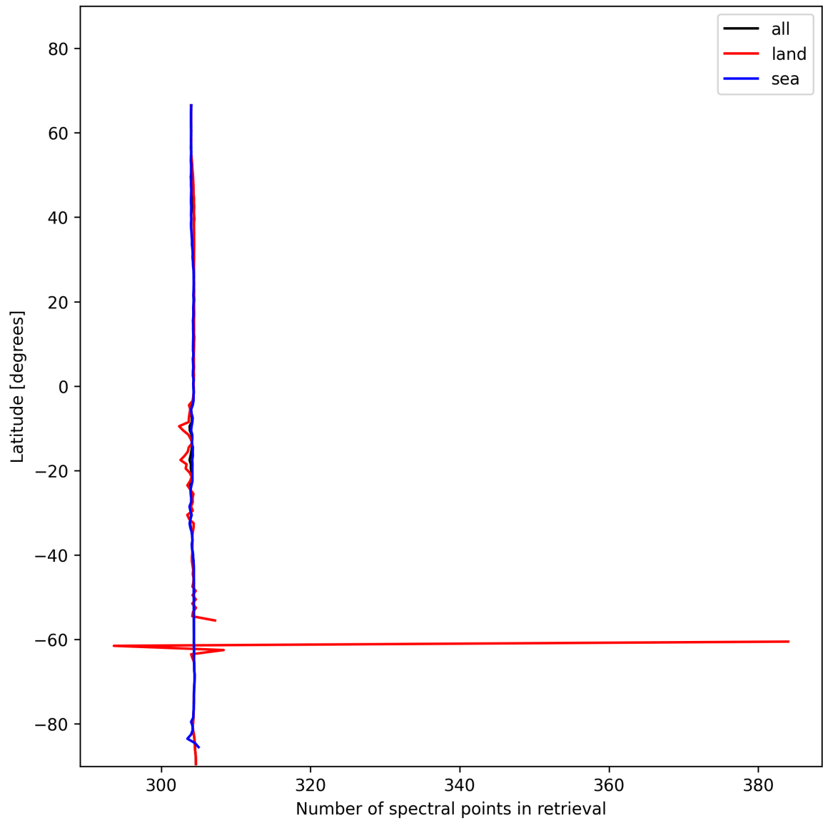
Figure 14: Zonal average of “Number of spectral points in retrieval” for 2025-01-14 to 2025-01-15.
