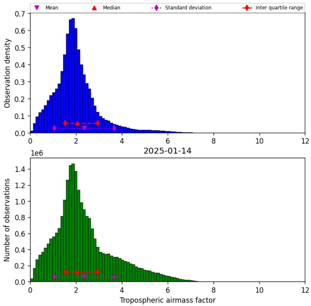
Figure 29: Histogram of “Tropospheric airmass factor” for 2025-01-14 to 2025-01-15
