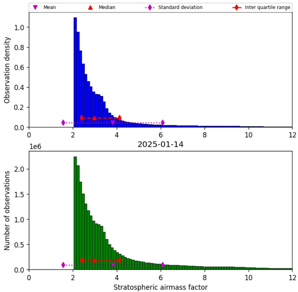
Figure 42: Histogram of “Stratospheric airmass factor” for 2025-01-14 to 2025-01-15
