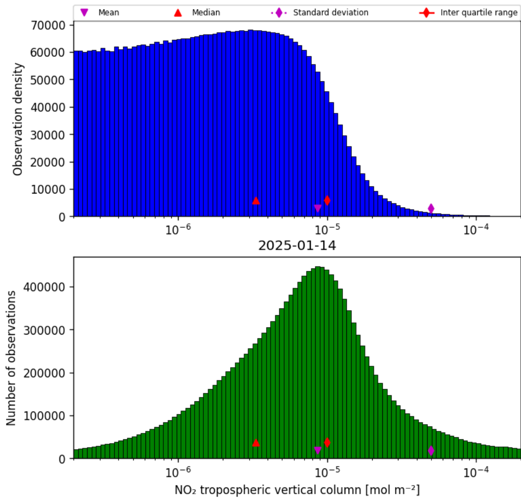
Figure 27: Histogram of “NO 2 tropospheric vertical column” for 2025-01-14 to 2025-01-15
