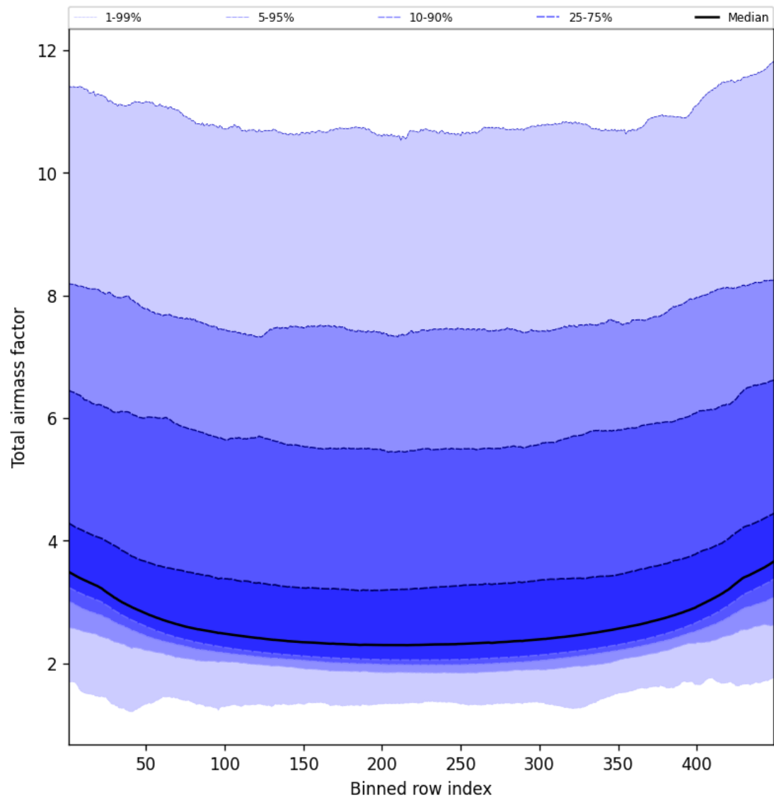
Figure 47: Along track statistics of “Total airmass factor” for 2025-01-14 to 2025-01-15
