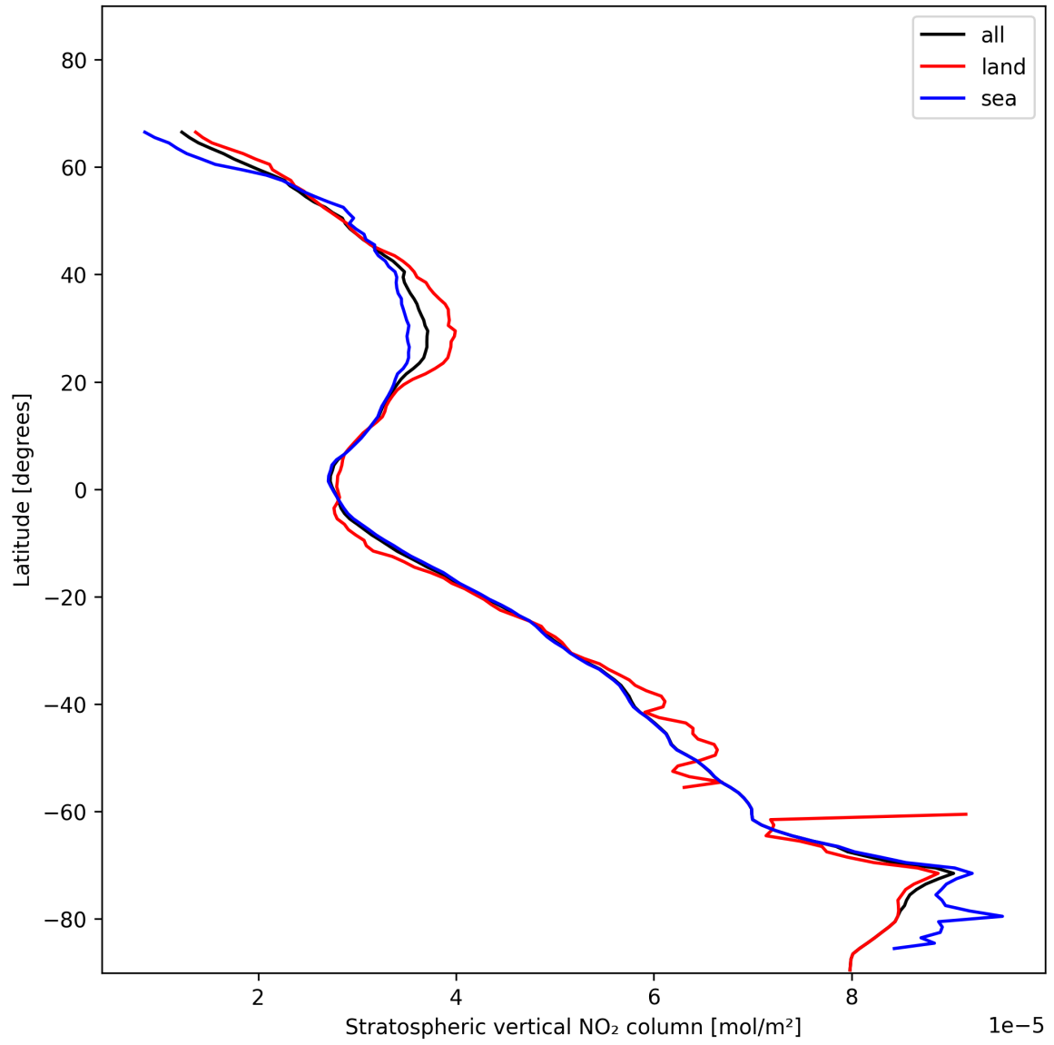
Figure 17: Zonal average of “Stratospheric vertical NO 2 column” for 2025-01-14 to 2025-01-15.
