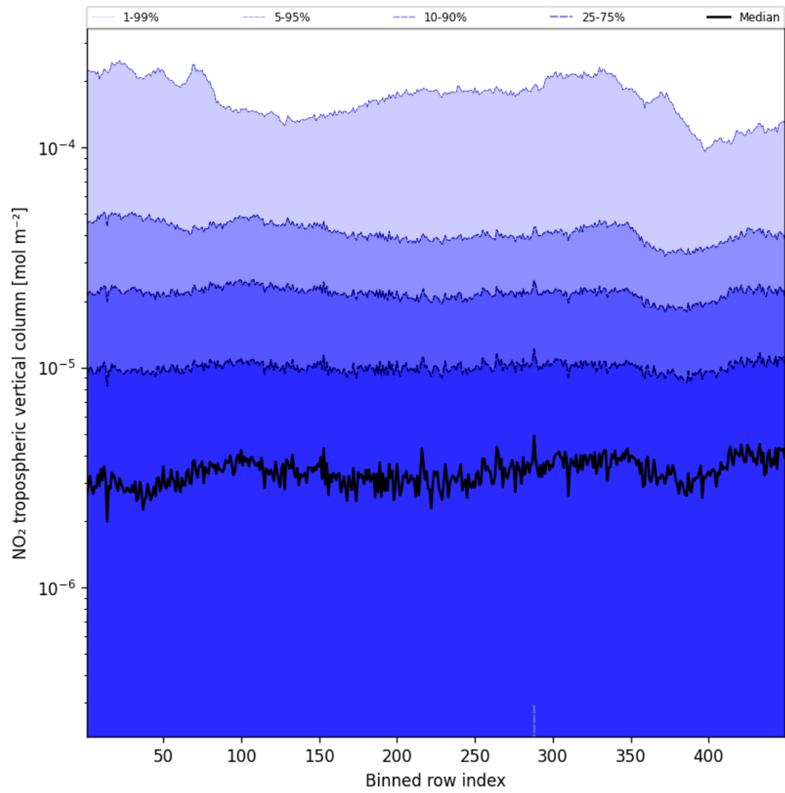
Figure 44: Along track statistics of “NO 2 tropospheric vertical column” for 2025-01-14 to 2025-01-15
