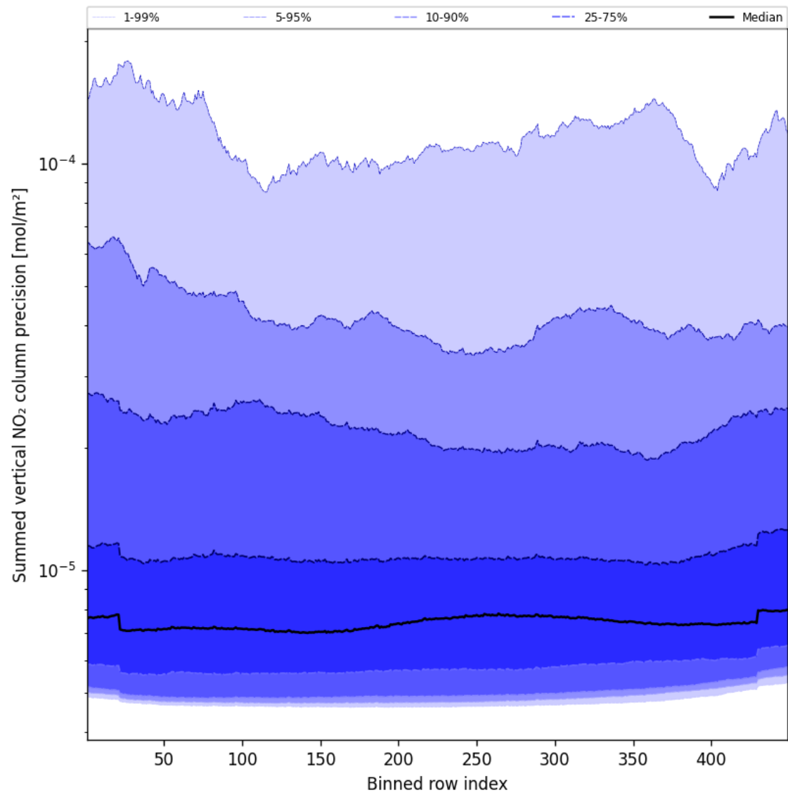
Figure 56: Along track statistics of “Summed vertical NO 2 column precision” for 2025-01-14 to 2025-01-15
