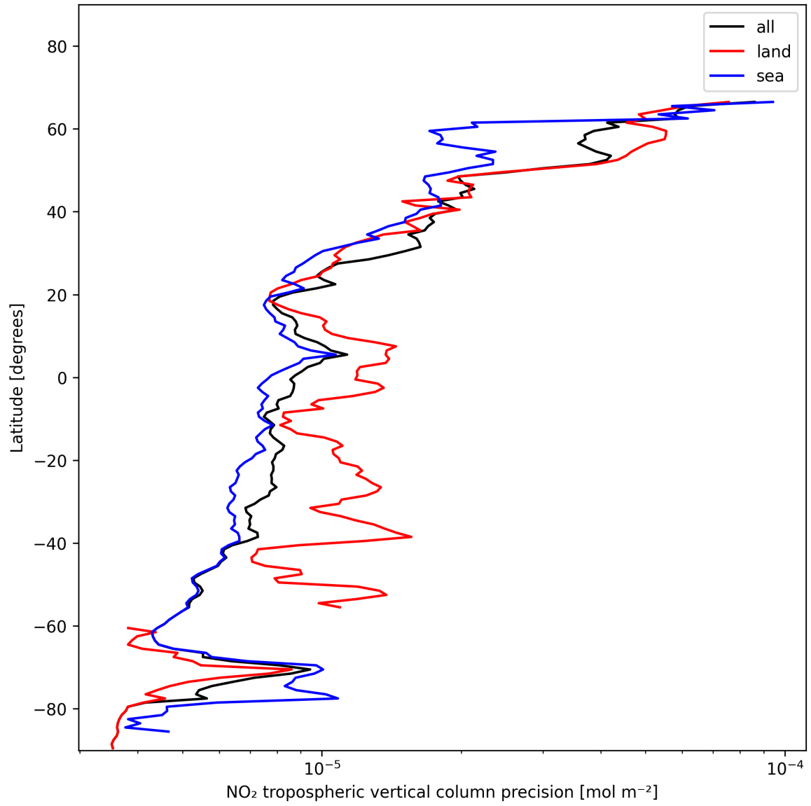
Figure 11: Zonal average of “NO 2 tropospheric vertical column precision” for 2025-01-14 to 2025-01-15.
