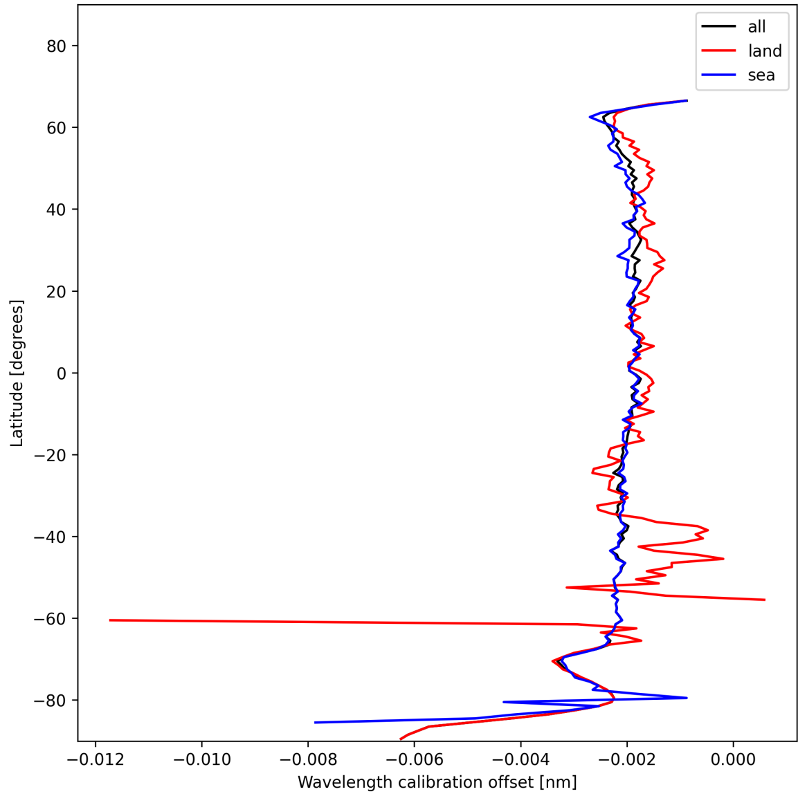
Figure 16: Zonal average of “Wavelength calibration offset” for 2025-01-14 to 2025-01-15.
