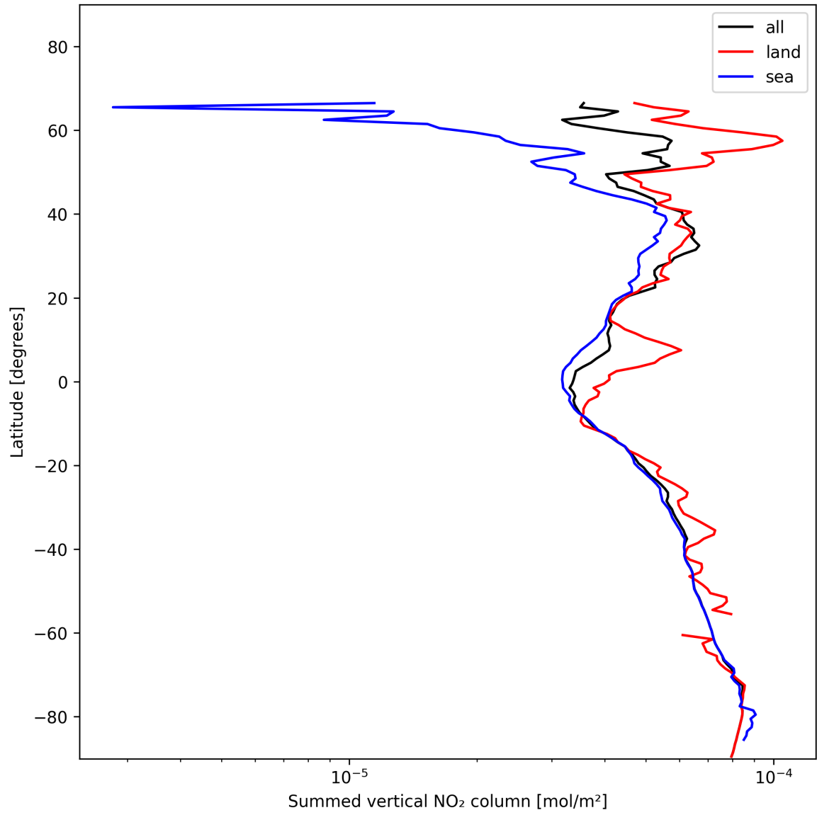
Figure 21: Zonal average of “Summed vertical NO 2 column” for 2025-01-14 to 2025-01-15.
