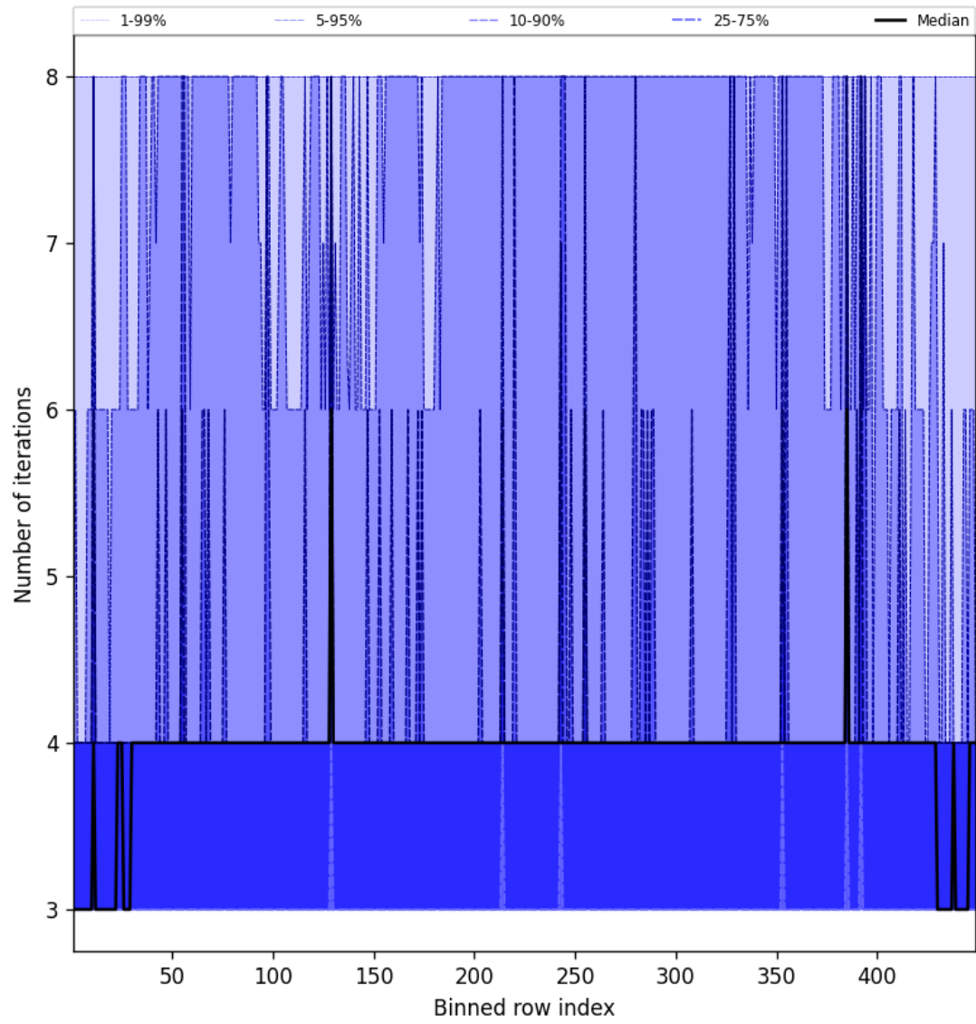
Figure 49: Along track statistics of “Number of iterations” for 2025-01-14 to 2025-01-15
