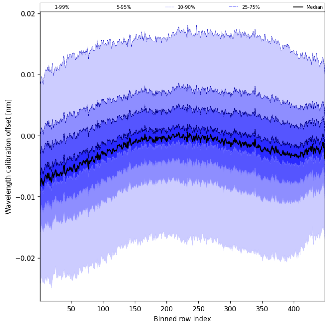
Figure 50: Along track statistics of “Wavelength calibration offset” for 2025-01-14 to 2025-01-15
