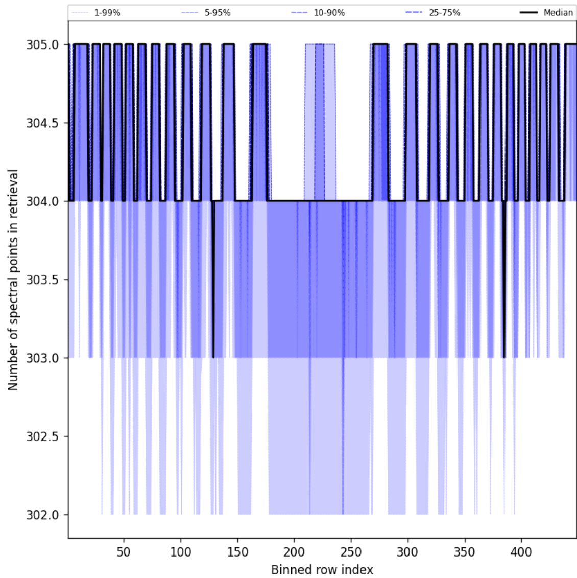
Figure 48: Along track statistics of “Number of spectral points in retrieval” for 2025-01-14 to 2025-01-15
