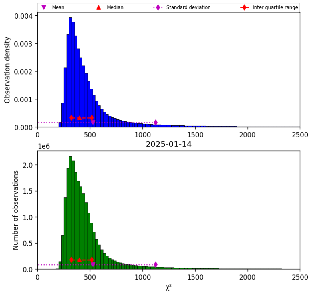
Figure 40: Histogram of “ \chi^2 ” for 2025-01-14 to 2025-01-15
