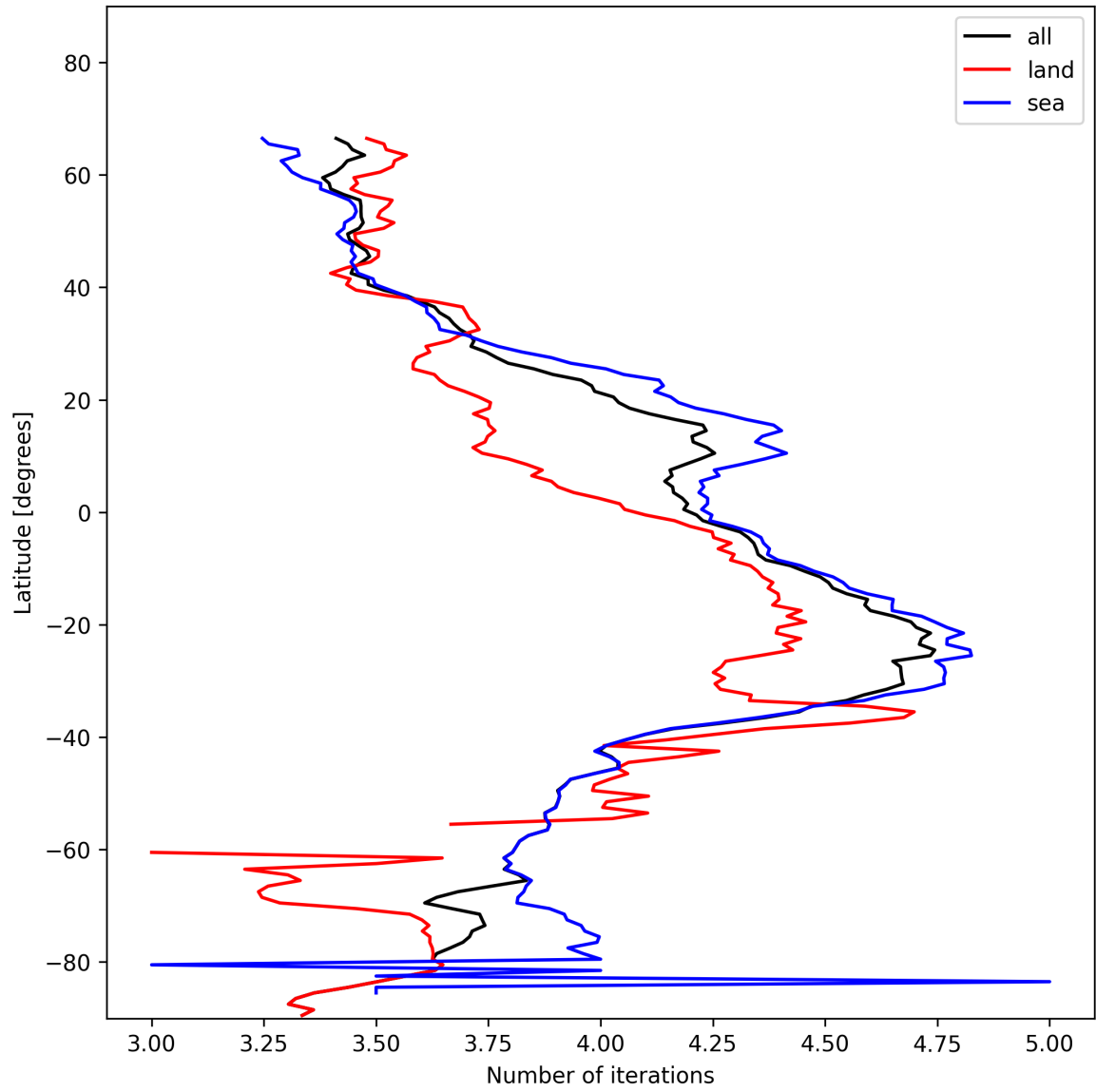
Figure 15: Zonal average of “Number of iterations” for 2025-01-14 to 2025-01-15.
