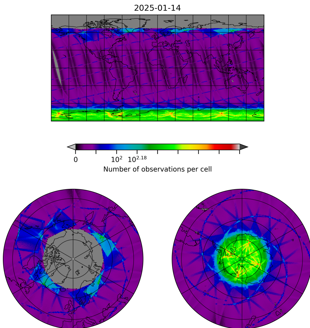
Figure 8: Map of the number of observations for 2025-01-14 to 2025-01-15
