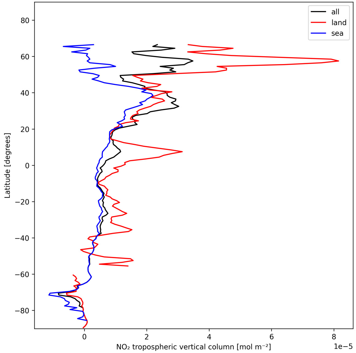
Figure 10: Zonal average of “NO 2 tropospheric vertical column” for 2025-01-14 to 2025-01-15.
