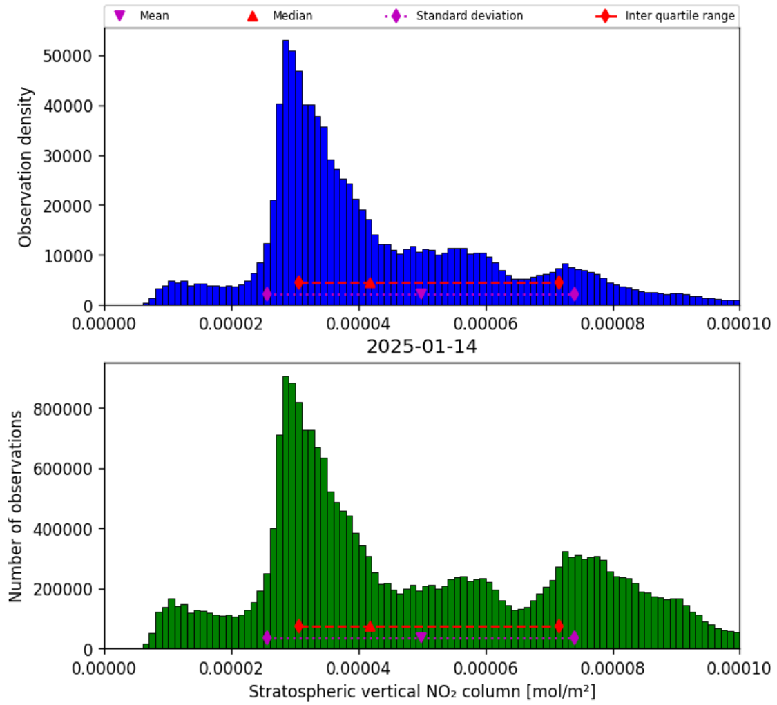
Figure 34: Histogram of “Stratospheric vertical NO 2 column” for 2025-01-14 to 2025-01-15
