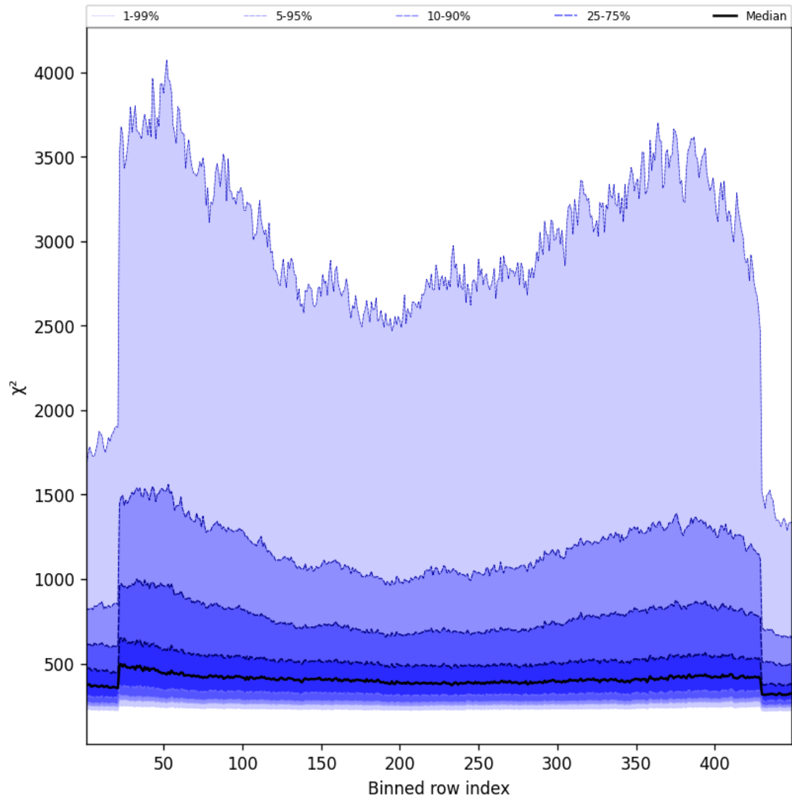
Figure 57: Along track statistics of “ \chi^2 ” for 2025-01-14 to 2025-01-15
