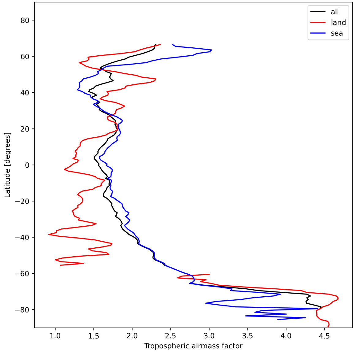
Figure 12: Zonal average of “Tropospheric airmass factor” for 2025-01-14 to 2025-01-15.
