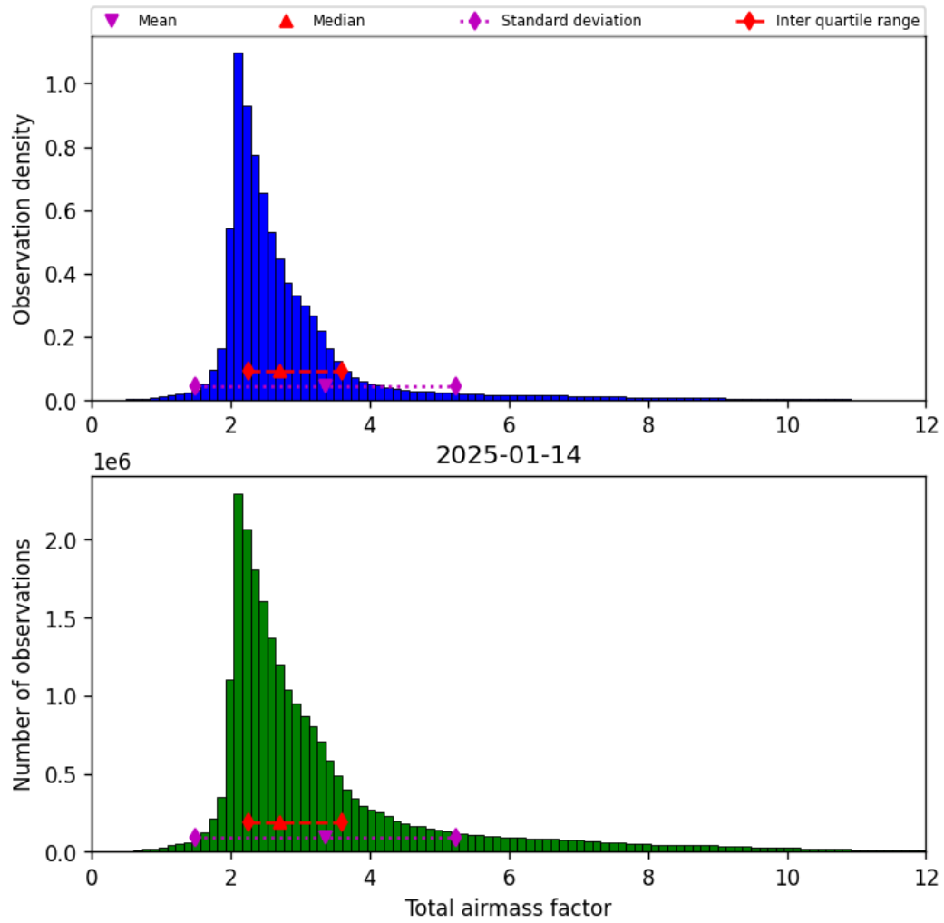
Figure 30: Histogram of “Total airmass factor” for 2025-01-14 to 2025-01-15
