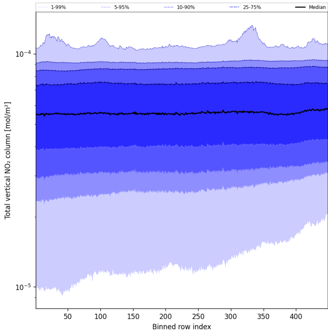
Figure 53: Along track statistics of “Total vertical NO 2 column” for 2025-01-14 to 2025-01-15
