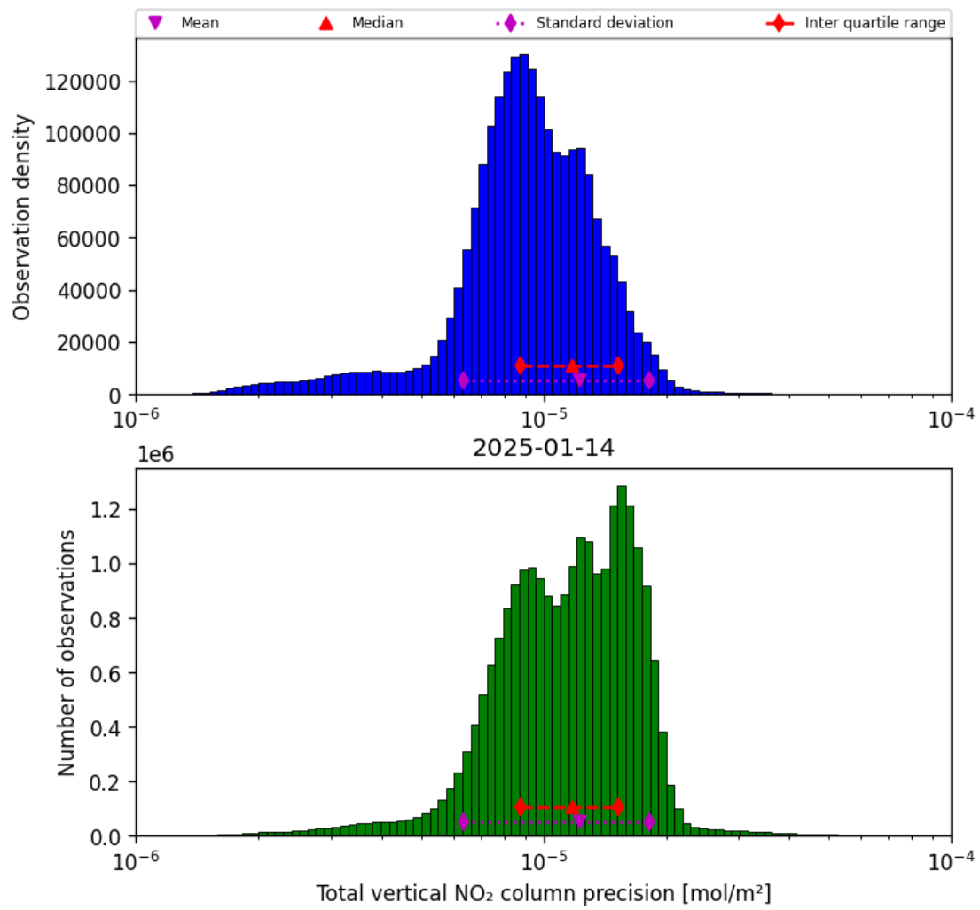
Figure 37: Histogram of “Total vertical NO 2 column precision” for 2025-01-14 to 2025-01-15
