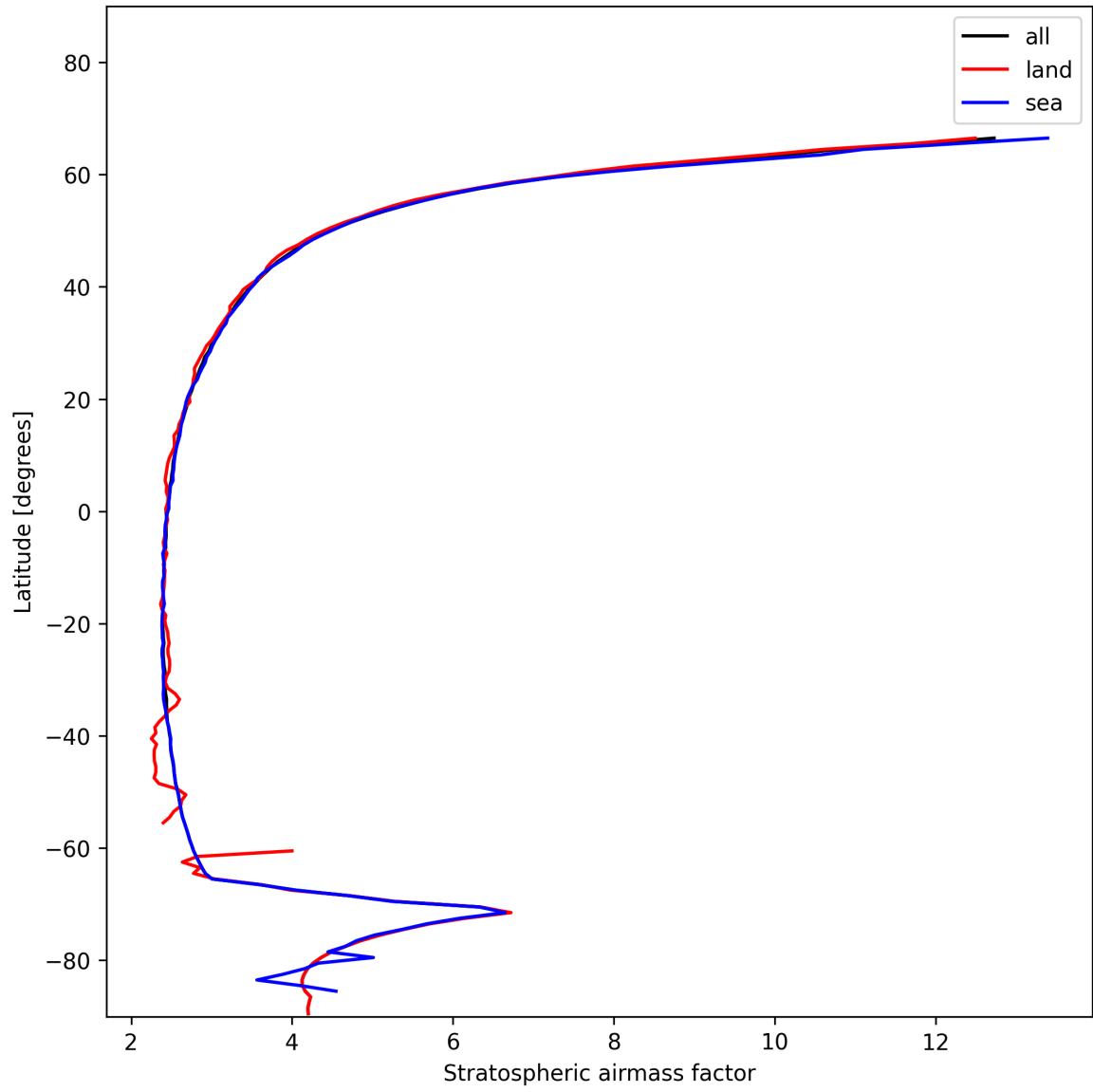
Figure 25: Zonal average of “Stratospheric air mass factor” for 2025-01-14 to 2025-01-15.
