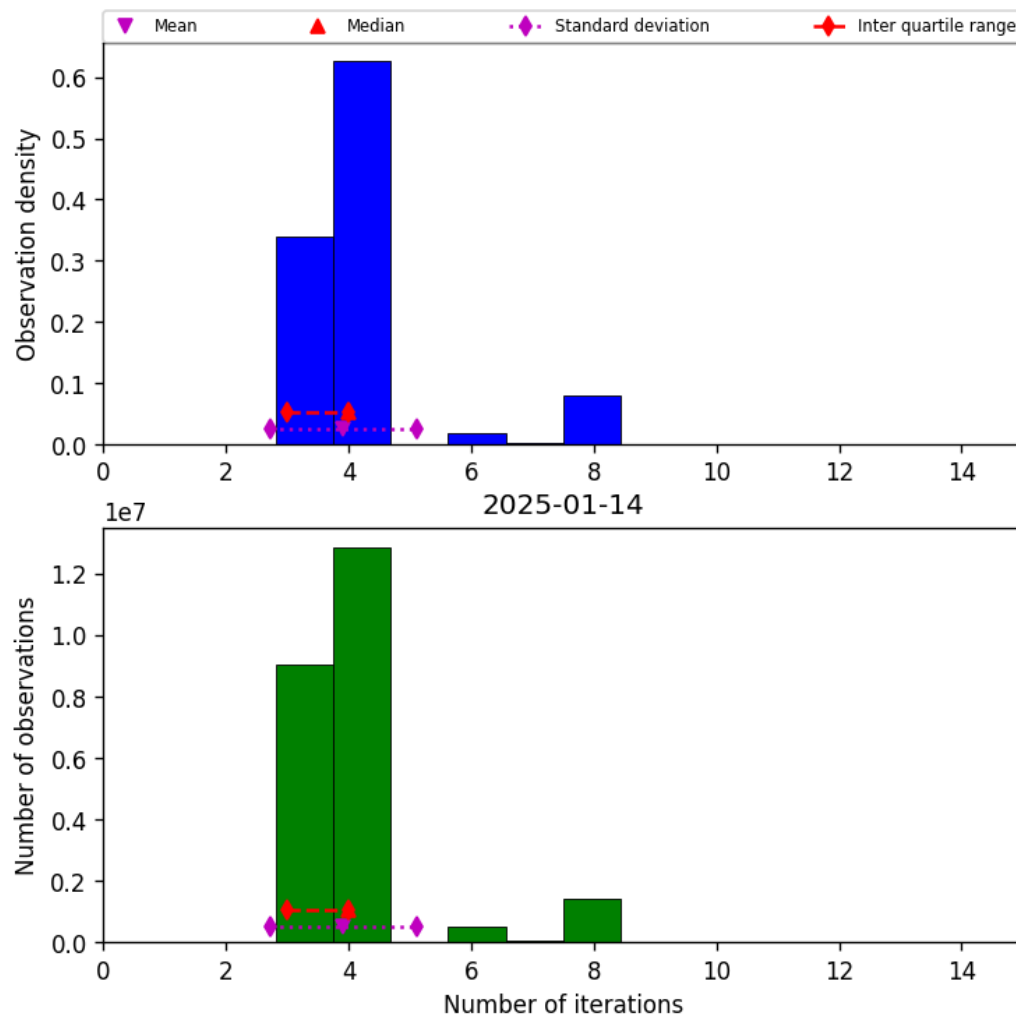
Figure 32: Histogram of “Number of iterations” for 2025-01-14 to 2025-01-15
