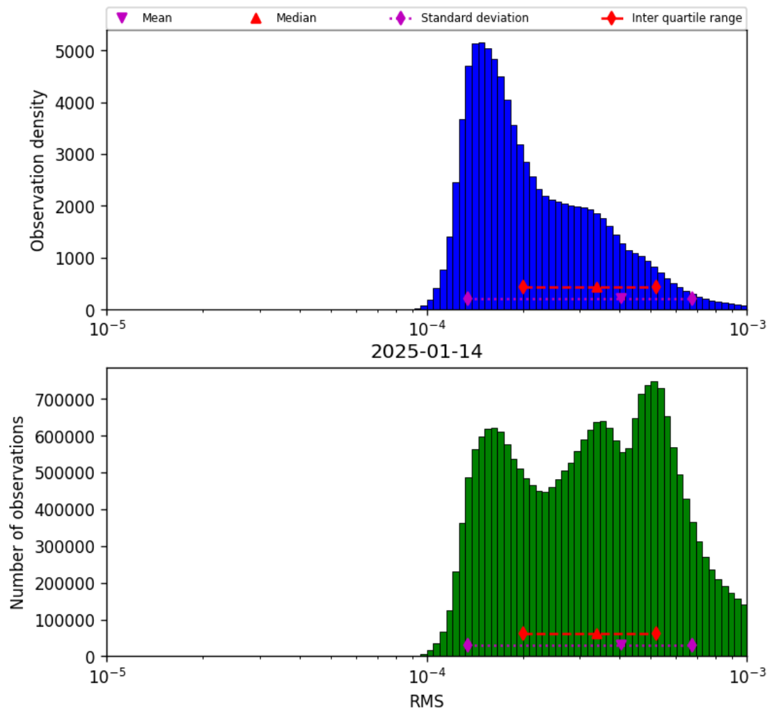
Figure 41: Histogram of “RMS” for 2025-01-14 to 2025-01-15
