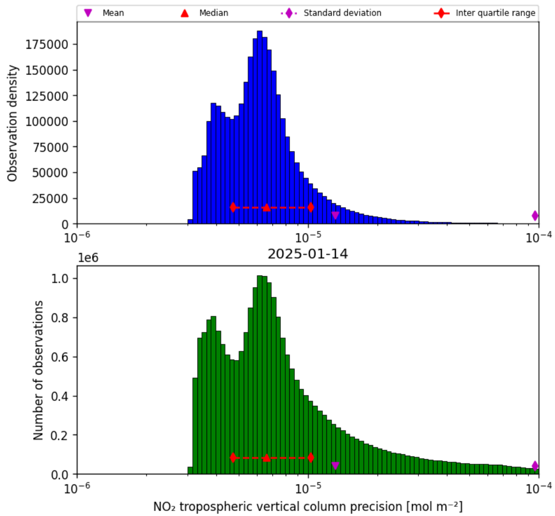
Figure 28: Histogram of “NO 2 tropospheric vertical column precision” for 2025-01-14 to 2025-01-15
