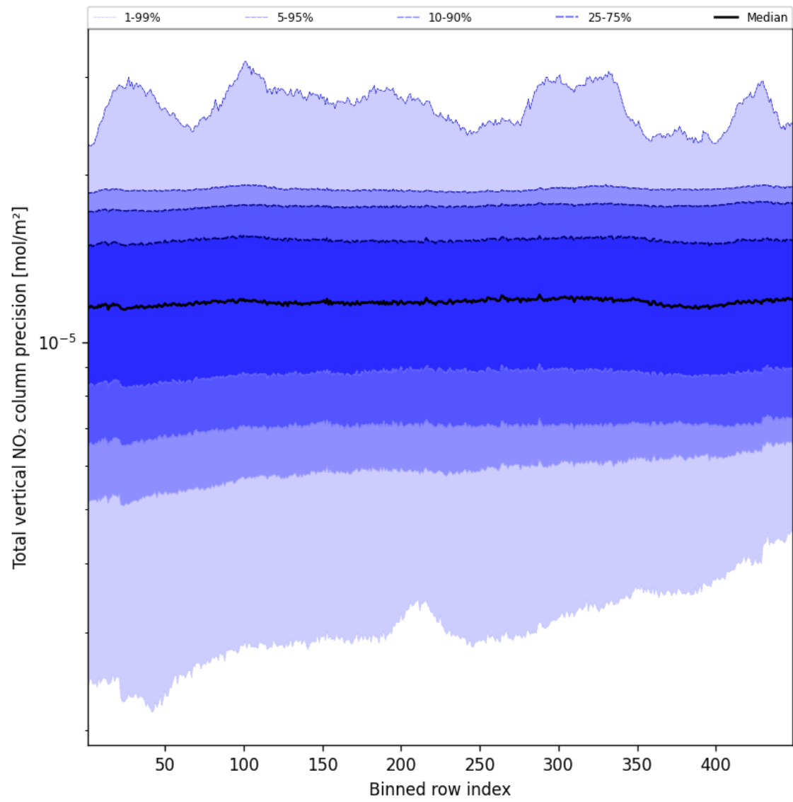
Figure 54: Along track statistics of “Total vertical NO 2 column precision” for 2025-01-14 to 2025-01-15
