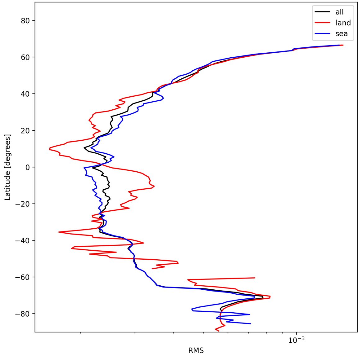
Figure 24: Zonal average of “RMS” for 2025-01-14 to 2025-01-15.
