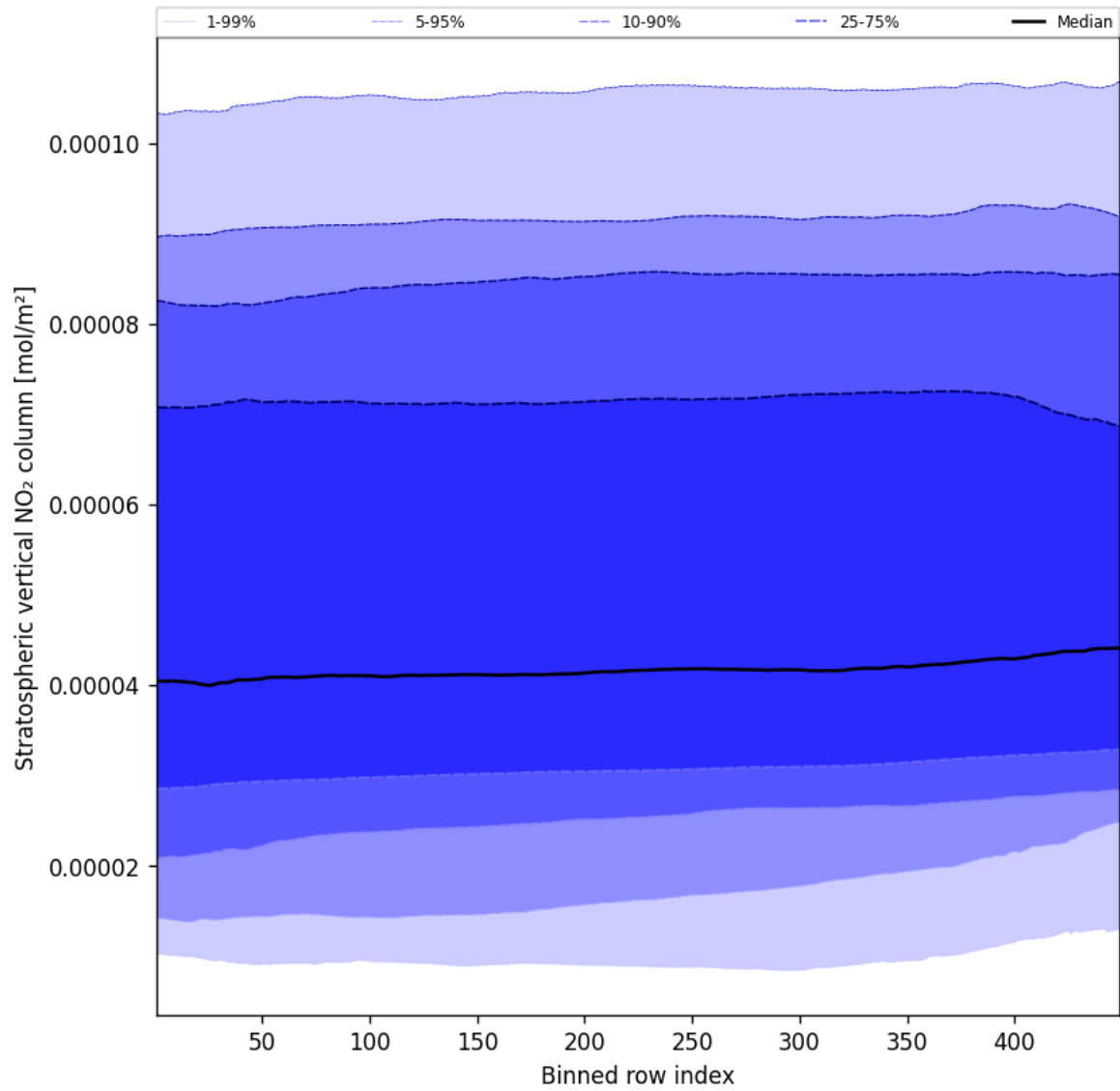
Figure 51: Along track statistics of “Stratospheric vertical NO 2 column” for 2025-01-14 to 2025-01-15
