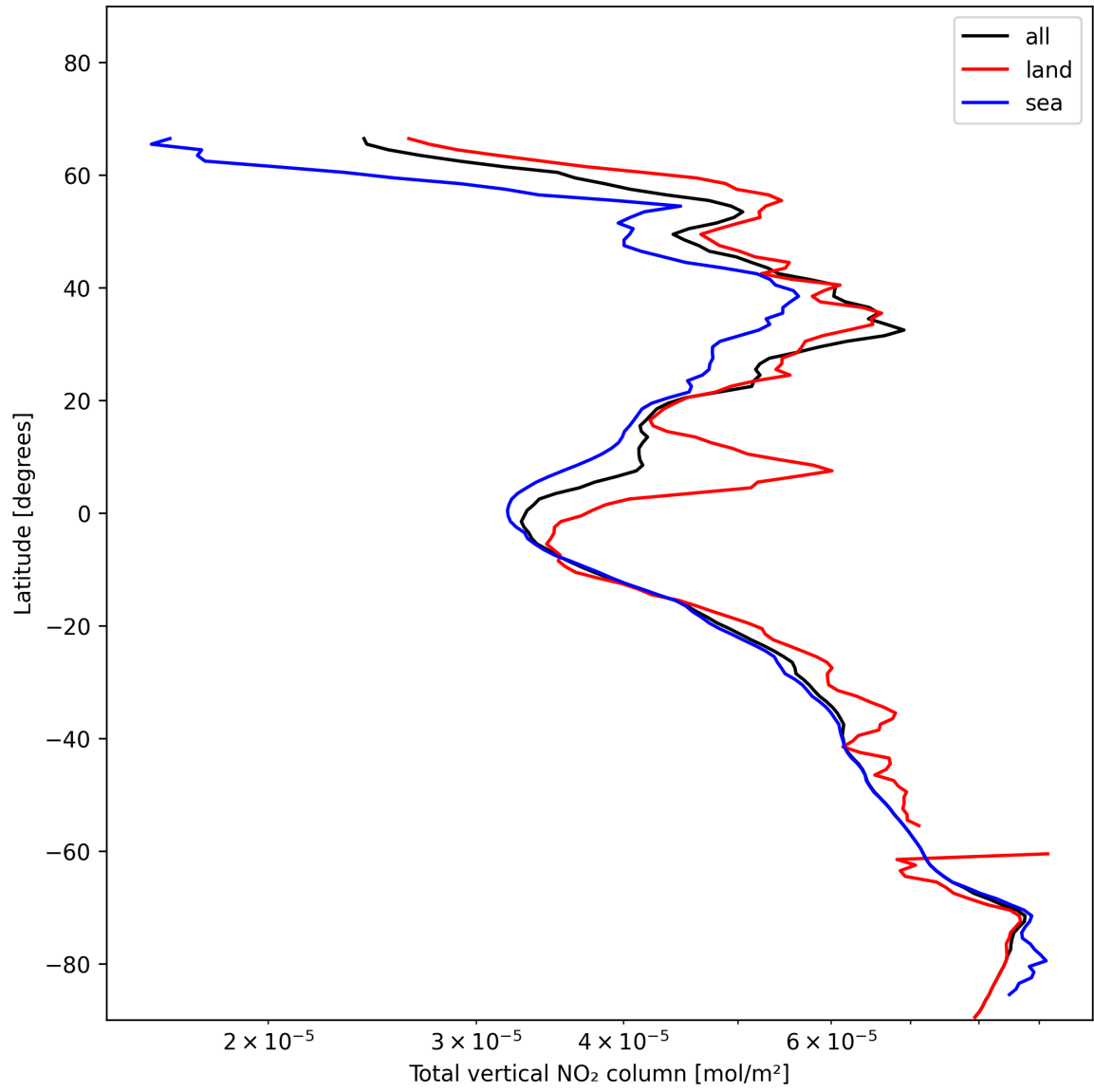
Figure 19: Zonal average of “Total vertical NO 2 column” for 2025-01-14 to 2025-01-15.
