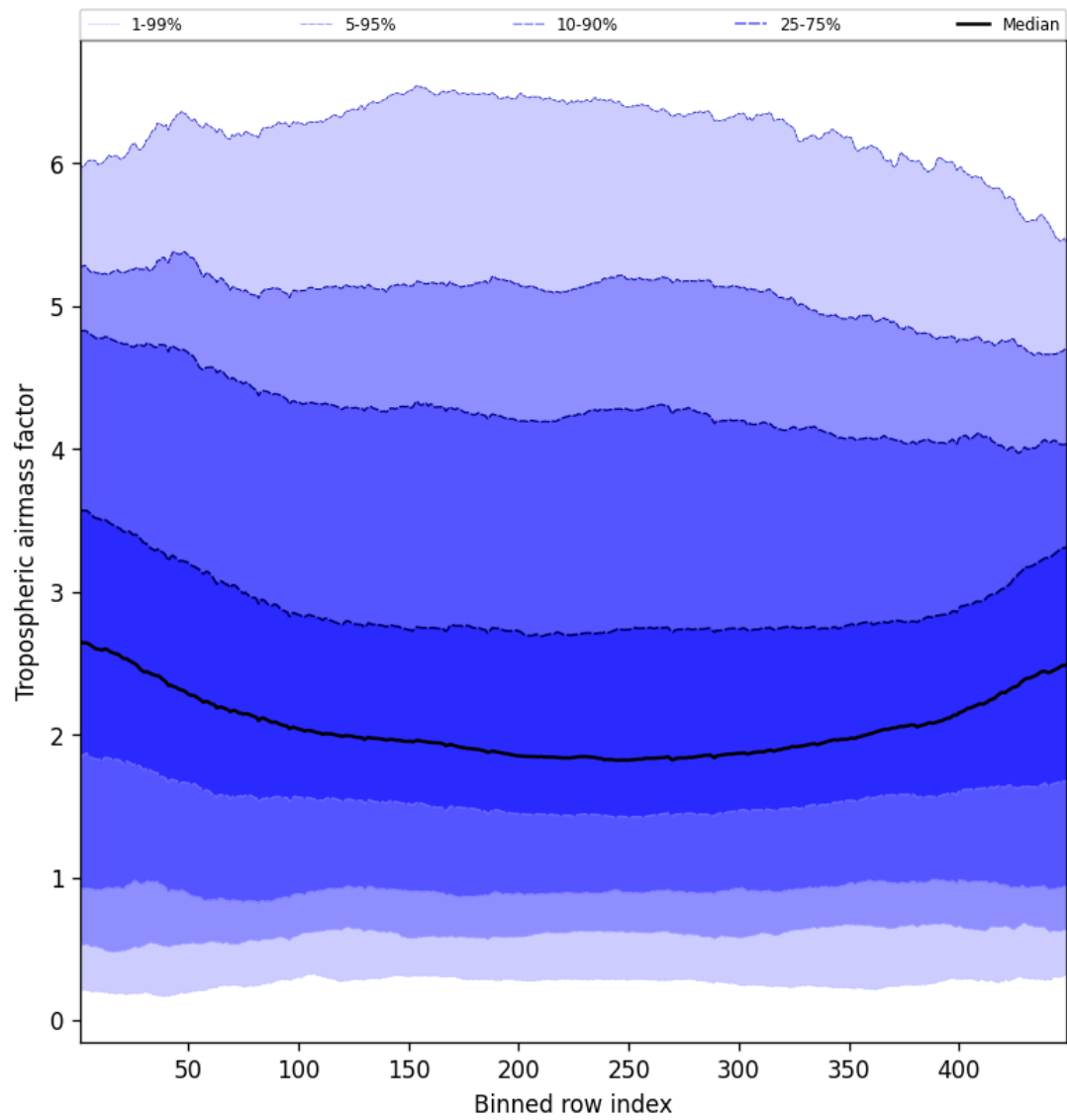
Figure 46: Along track statistics of “Tropospheric airmass factor” for 2025-01-14 to 2025-01-15
