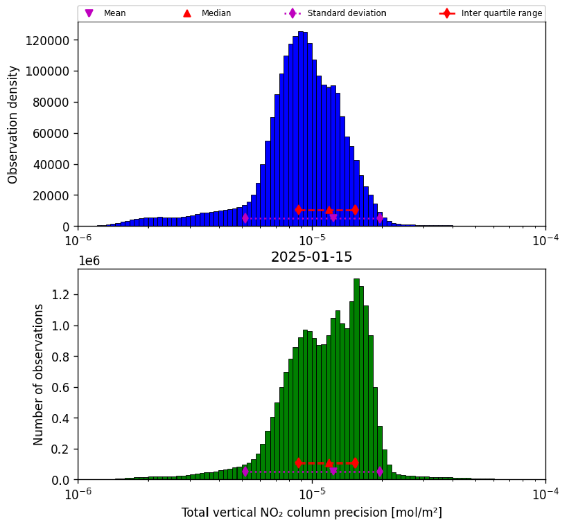
Figure 37: Histogram of “Total vertical NO 2 column precision” for 2025-01-15 to 2025-01-15
