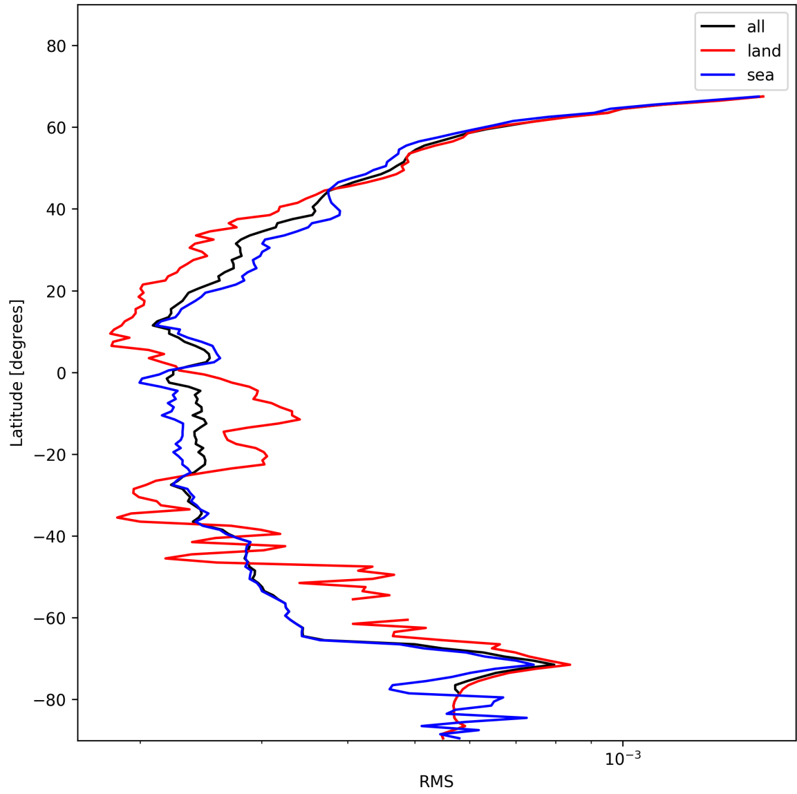
Figure 24: Zonal average of “RMS” for 2025-01-15 to 2025-01-15.
