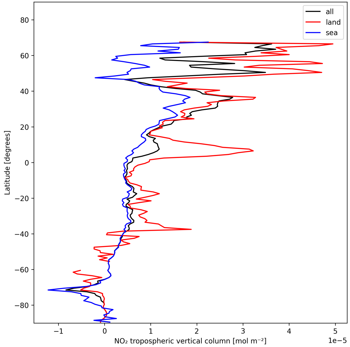
Figure 10: Zonal average of “NO 2 tropospheric vertical column” for 2025-01-15 to 2025-01-15.
