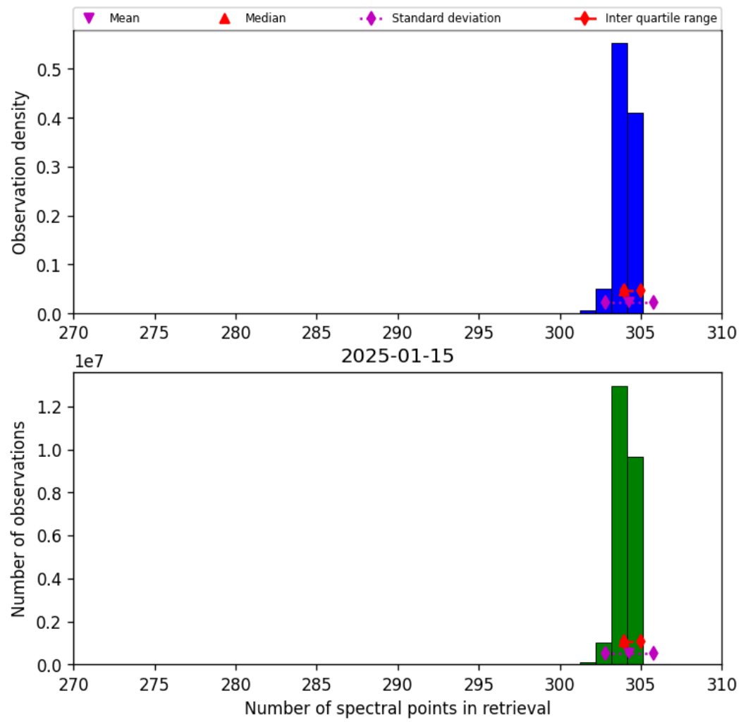
Figure 31: Histogram of “Number of spectral points in retrieval” for 2025-01-15 to 2025-01-15
