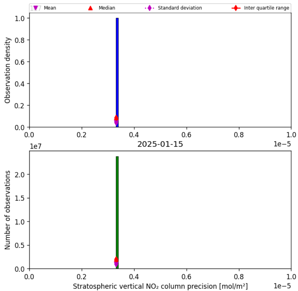
Figure 35: Histogram of “Stratospheric vertical NO 2 column precision” for 2025-01-15 to 2025-01-15
