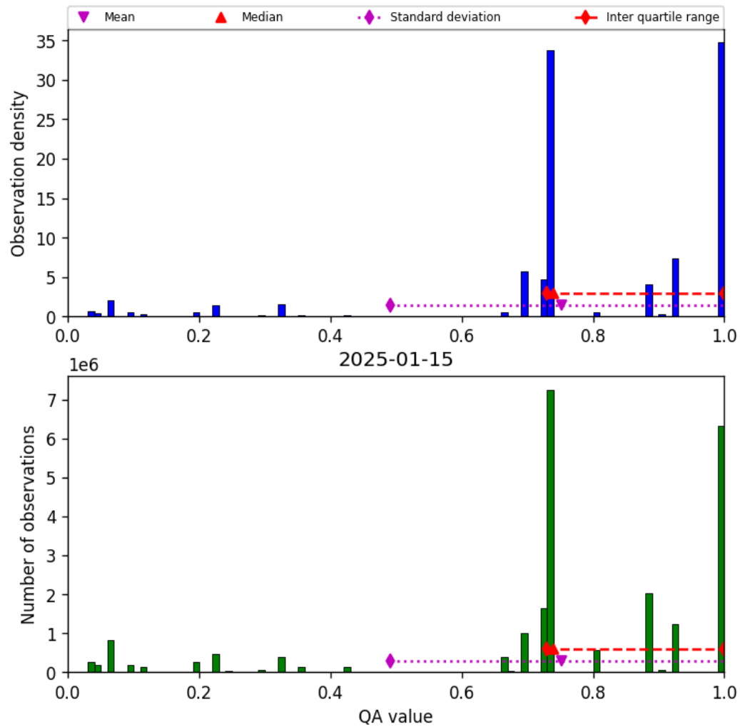
Figure 26: Histogram of “QA value” for 2025-01-15 to 2025-01-15
