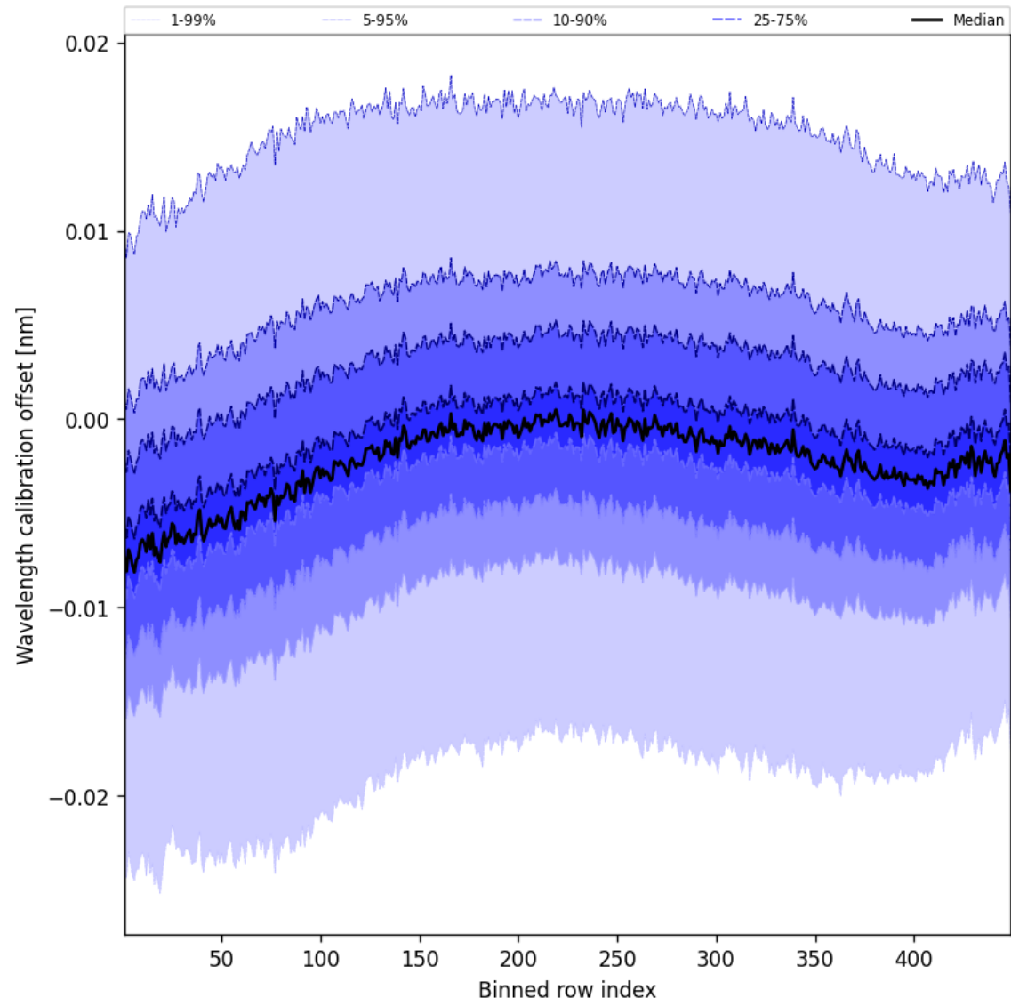
Figure 50: Along track statistics of “Wavelength calibration offset” for 2025-01-15 to 2025-01-15
