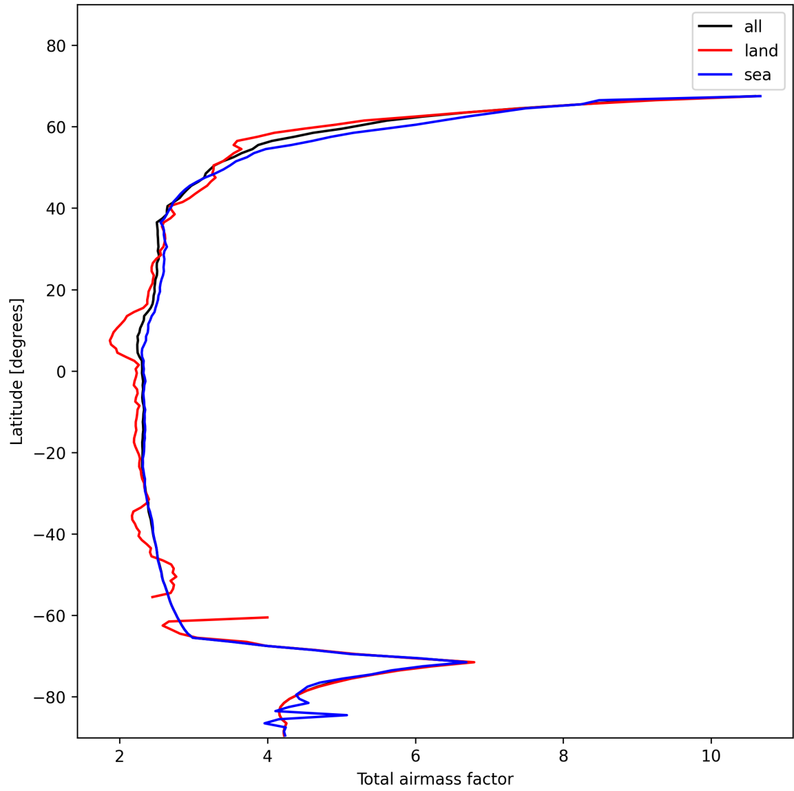
Figure 13: Zonal average of “Total airmass factor” for 2025-01-15 to 2025-01-15.
