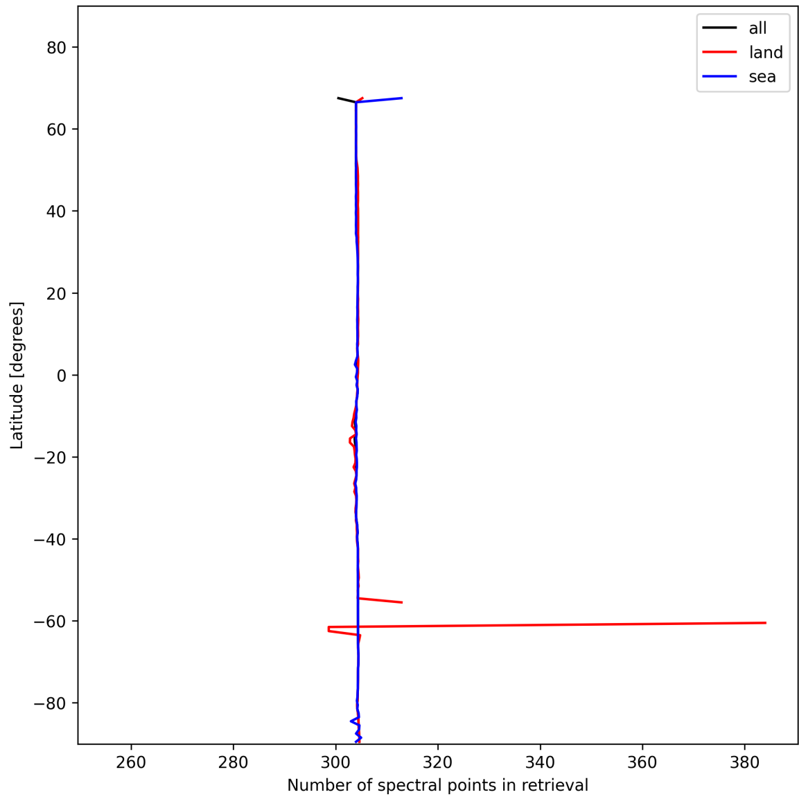
Figure 14: Zonal average of “Number of spectral points in retrieval” for 2025-01-15 to 2025-01-15.
