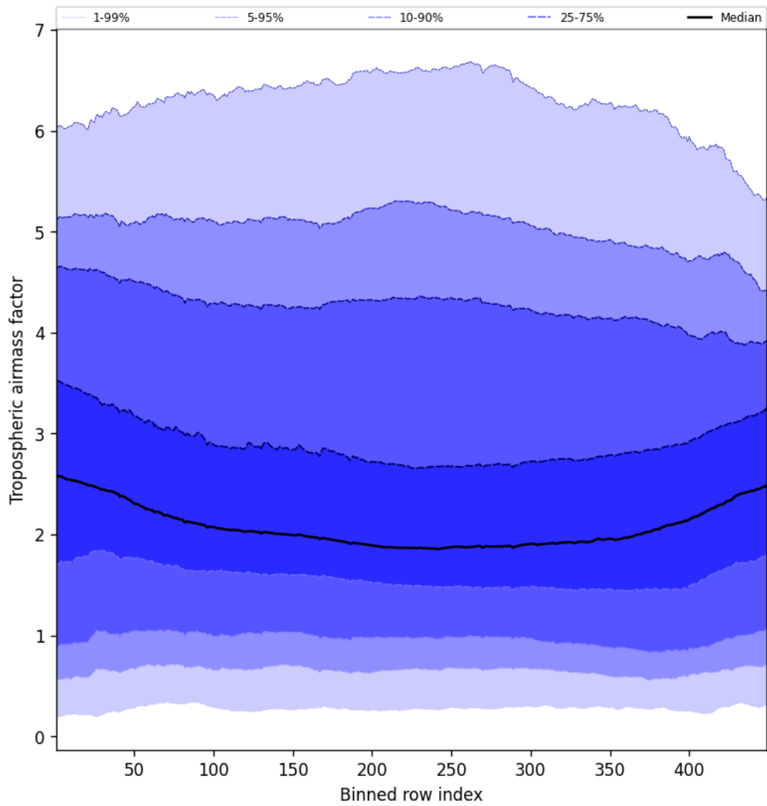
Figure 46: Along track statistics of “Tropospheric airmass factor” for 2025-01-15 to 2025-01-15
