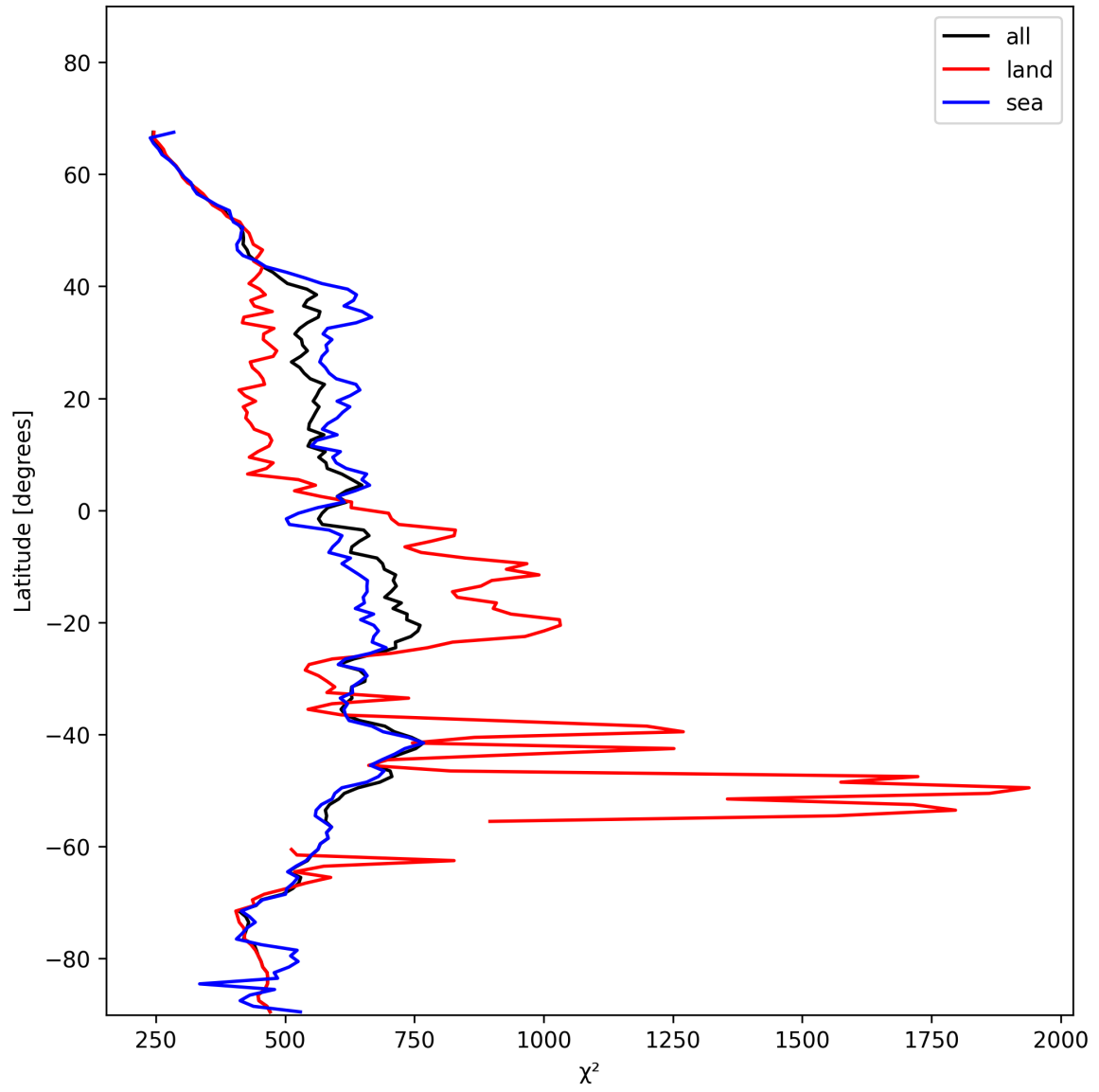
Figure 23: Zonal average of “ \chi^2 ” for 2025-01-15 to 2025-01-15.
