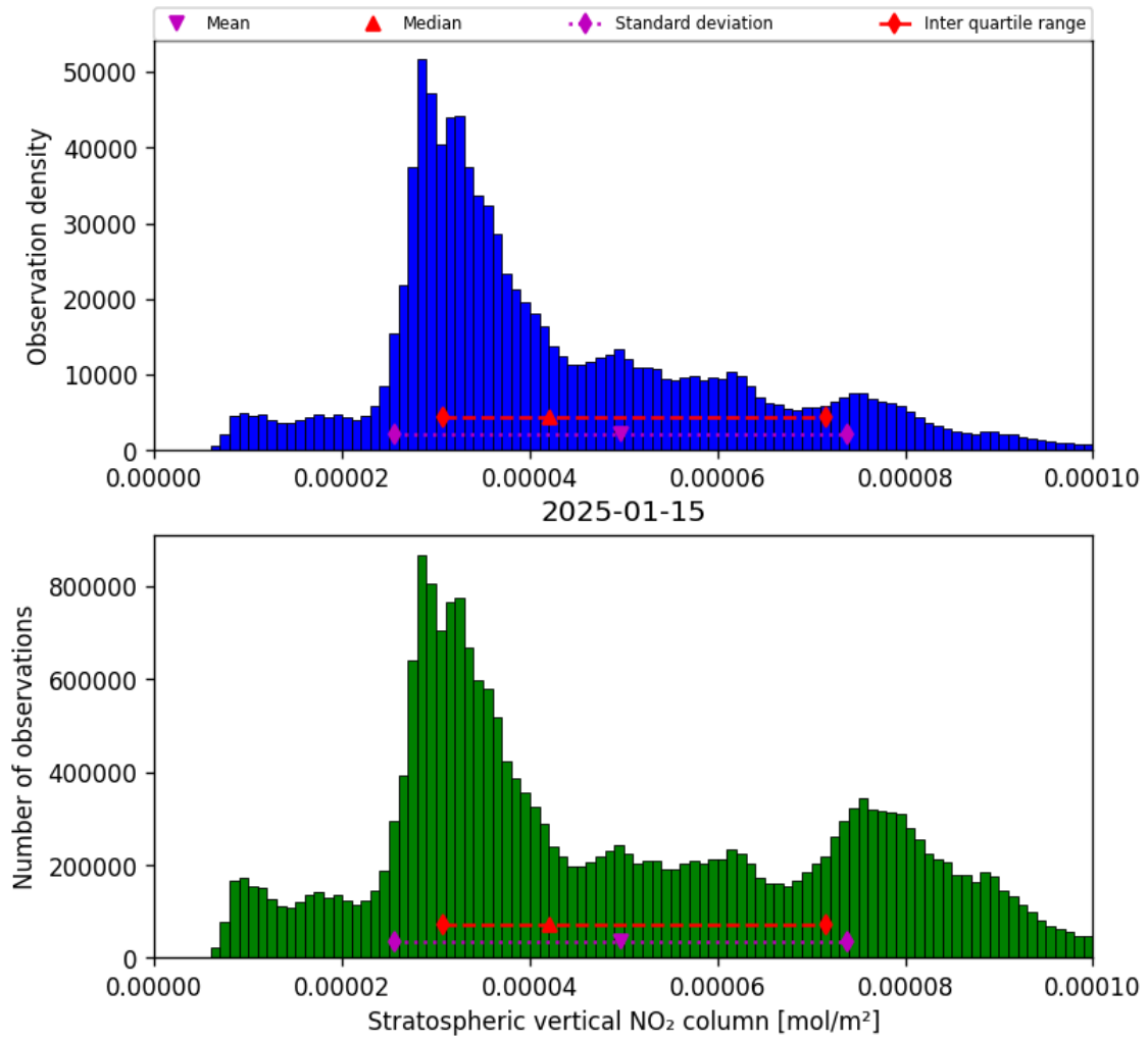
Figure 34: Histogram of “Stratospheric vertical NO 2 column” for 2025-01-15 to 2025-01-15
