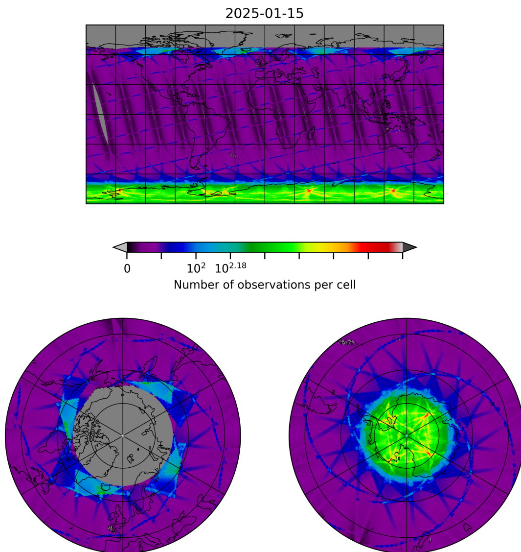
Figure 8: Map of the number of observations for 2025-01-15 to 2025-01-15
