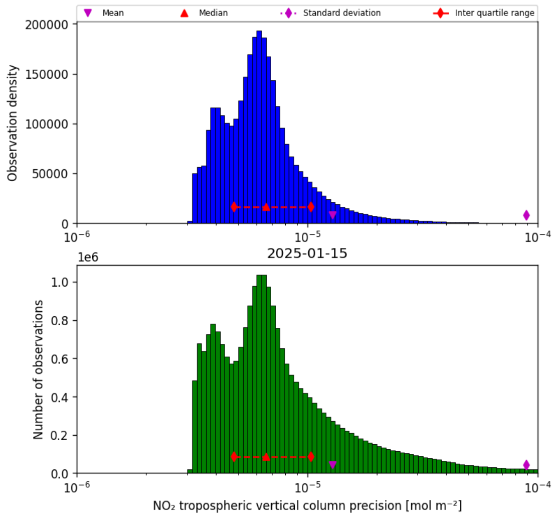
Figure 28: Histogram of "NO 2 tropospheric vertical column precision" for 2025-01-15 to 2025-01-15
