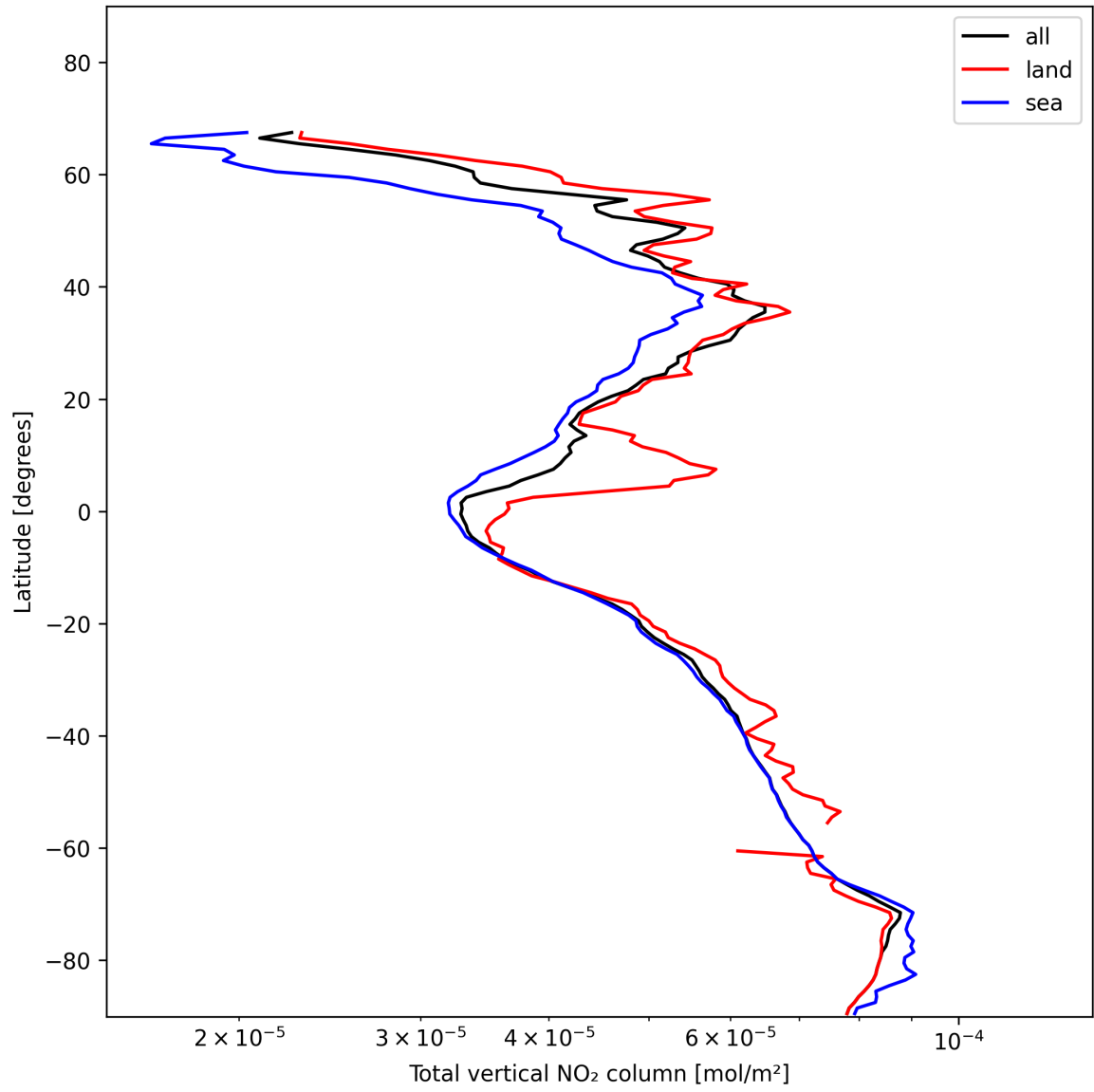
Figure 19: Zonal average of “Total vertical NO 2 column” for 2025-01-15 to 2025-01-15.
