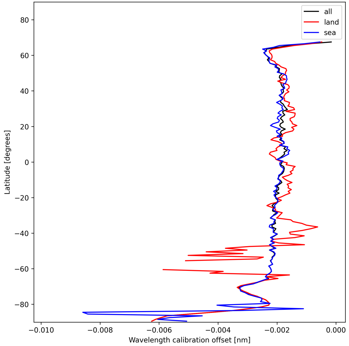
Figure 16: Zonal average of “Wavelength calibration offset” for 2025-01-15 to 2025-01-15.
