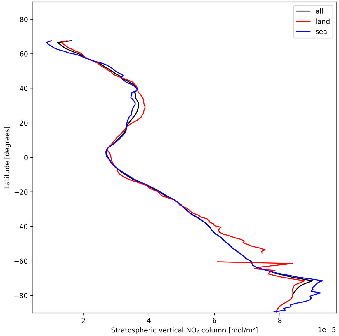
Figure 17: Zonal average of “Stratospheric vertical NO 2 column” for 2025-01-15 to 2025-01-15.
