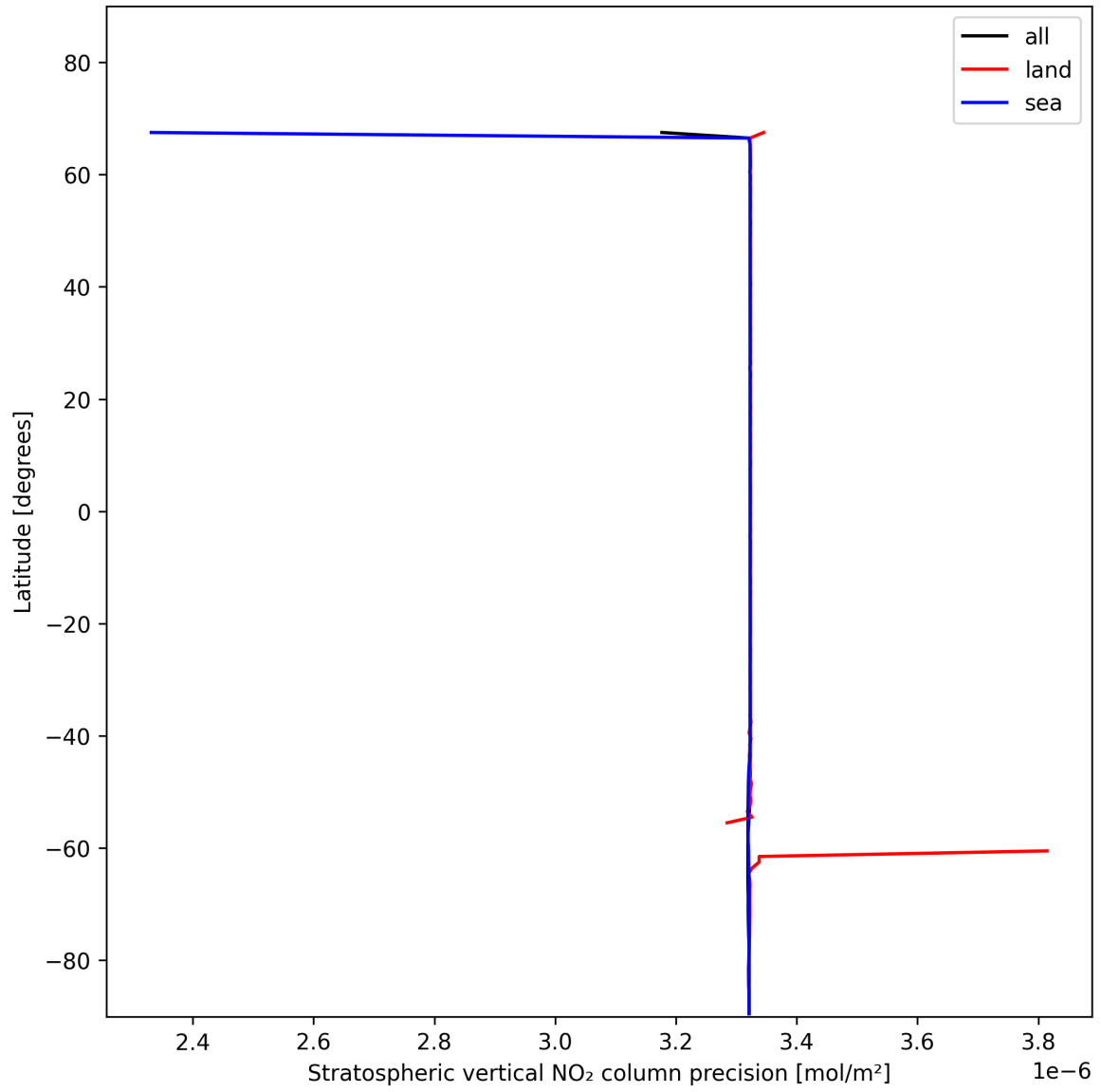
Figure 18: Zonal average of “Stratospheric vertical NO 2 column precision” for 2025-01-15 to 2025-01-15.
