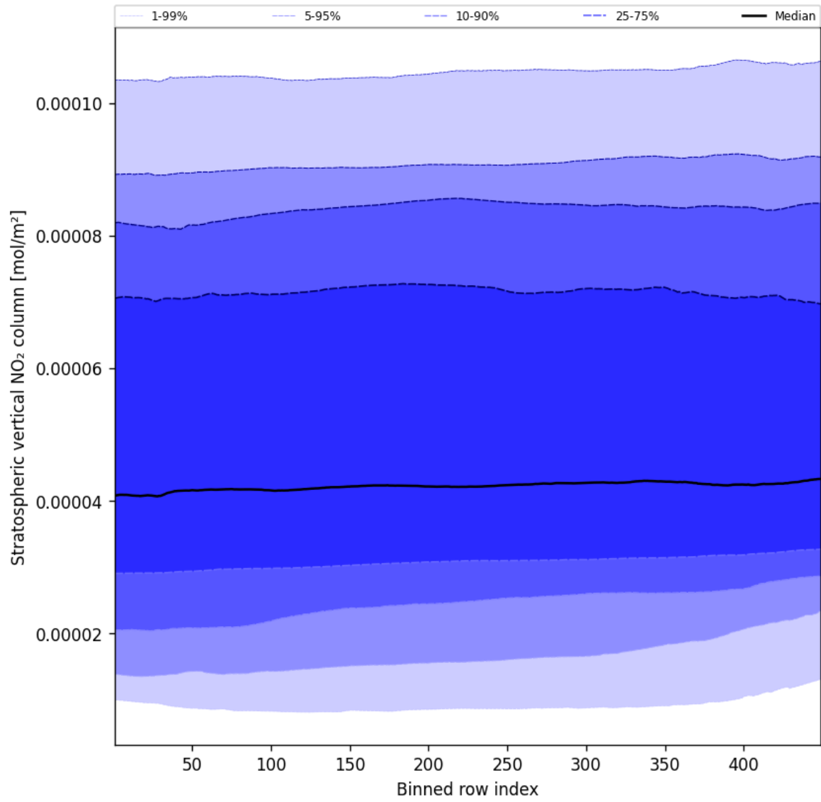
Figure 51: Along track statistics of “Stratospheric vertical NO 2 column” for 2025-01-15 to 2025-01-15
