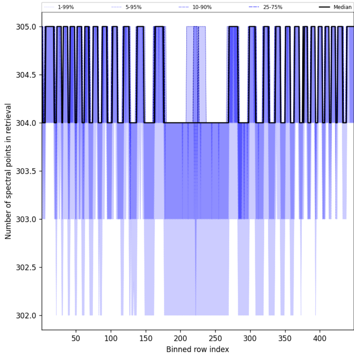
Figure 48: Along track statistics of “Number of spectral points in retrieval” for 2025-01-15 to 2025-01-15
