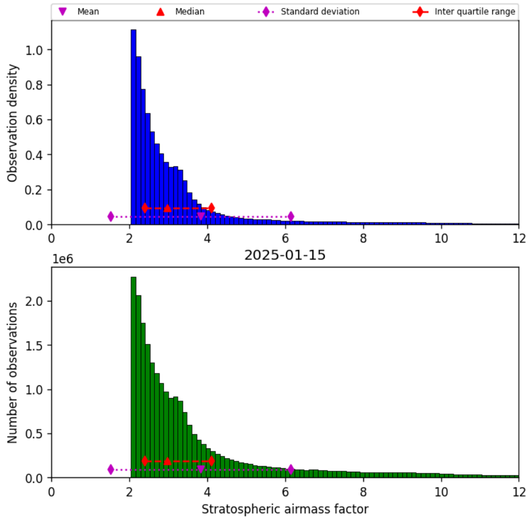
Figure 42: Histogram of “Stratospheric airmass factor” for 2025-01-15 to 2025-01-15
