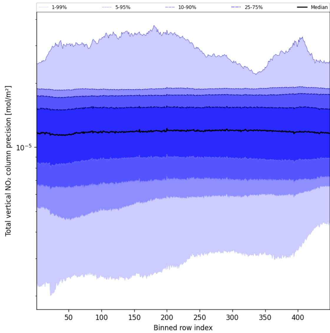
Figure 54: Along track statistics of “Total vertical NO 2 column precision” for 2025-01-15 to 2025-01-15
