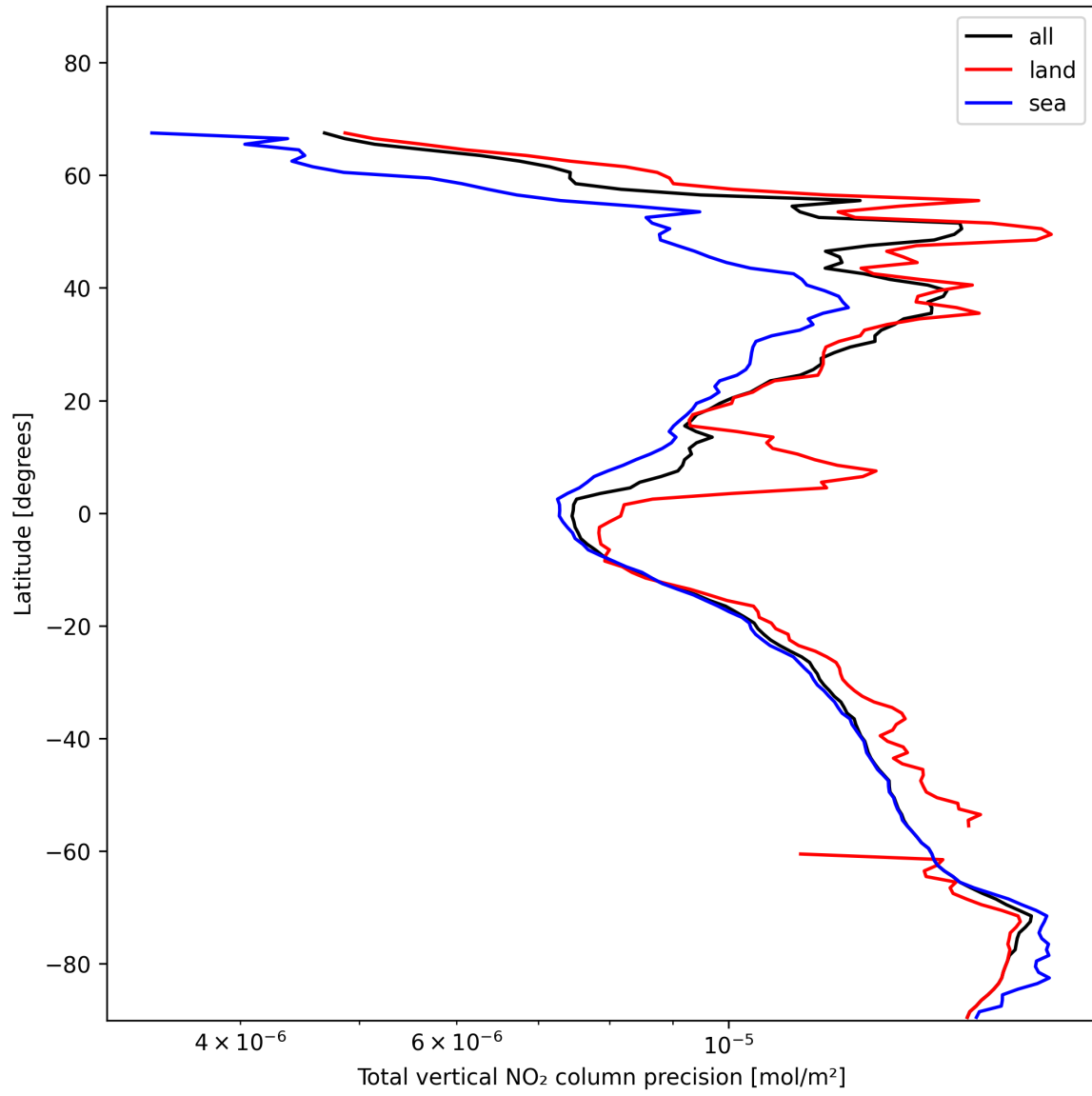
Figure 20: Zonal average of “Total vertical NO 2 column precision” for 2025-01-15 to 2025-01-15.
