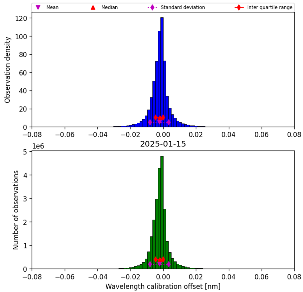
Figure 33: Histogram of “Wavelength calibration offset” for 2025-01-15 to 2025-01-15
