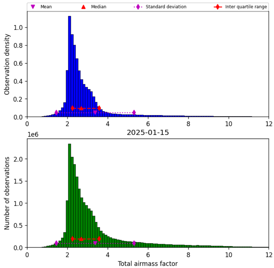
Figure 30: Histogram of “Total airmass factor” for 2025-01-15 to 2025-01-15
