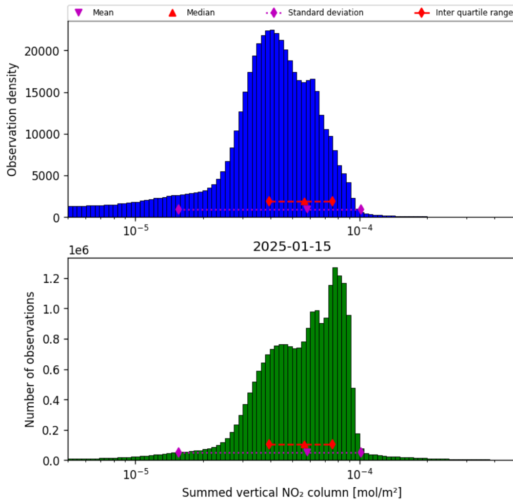
Figure 38: Histogram of “Summed vertical NO 2 column” for 2025-01-15 to 2025-01-15
