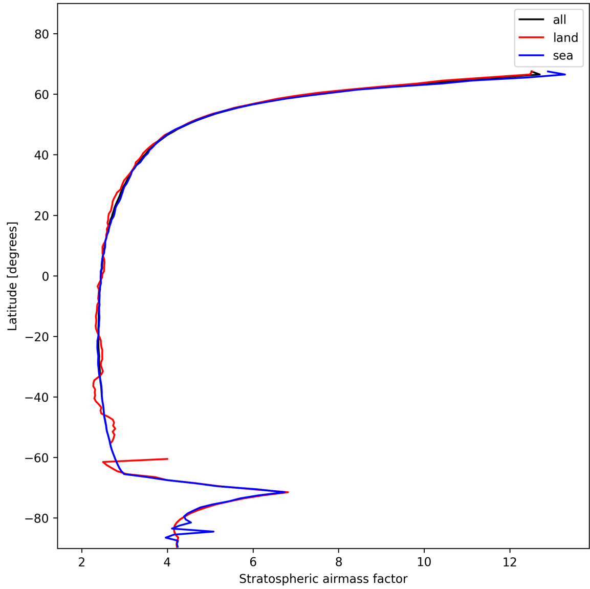
Figure 25: Zonal average of “Stratospheric airmass factor” for 2025-01-15 to 2025-01-15.
