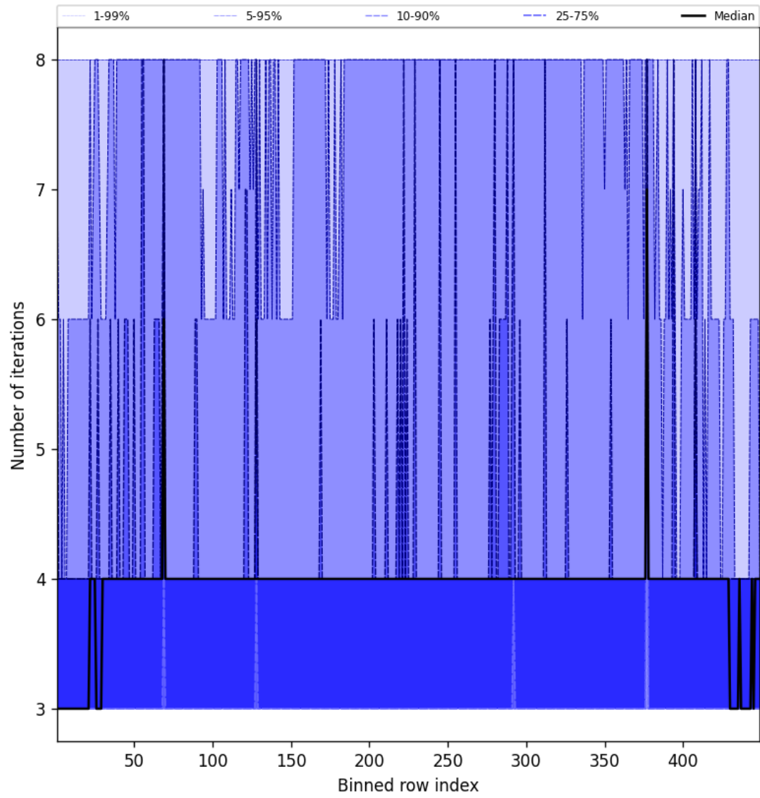
Figure 49: Along track statistics of “Number of iterations” for 2025-01-15 to 2025-01-15
