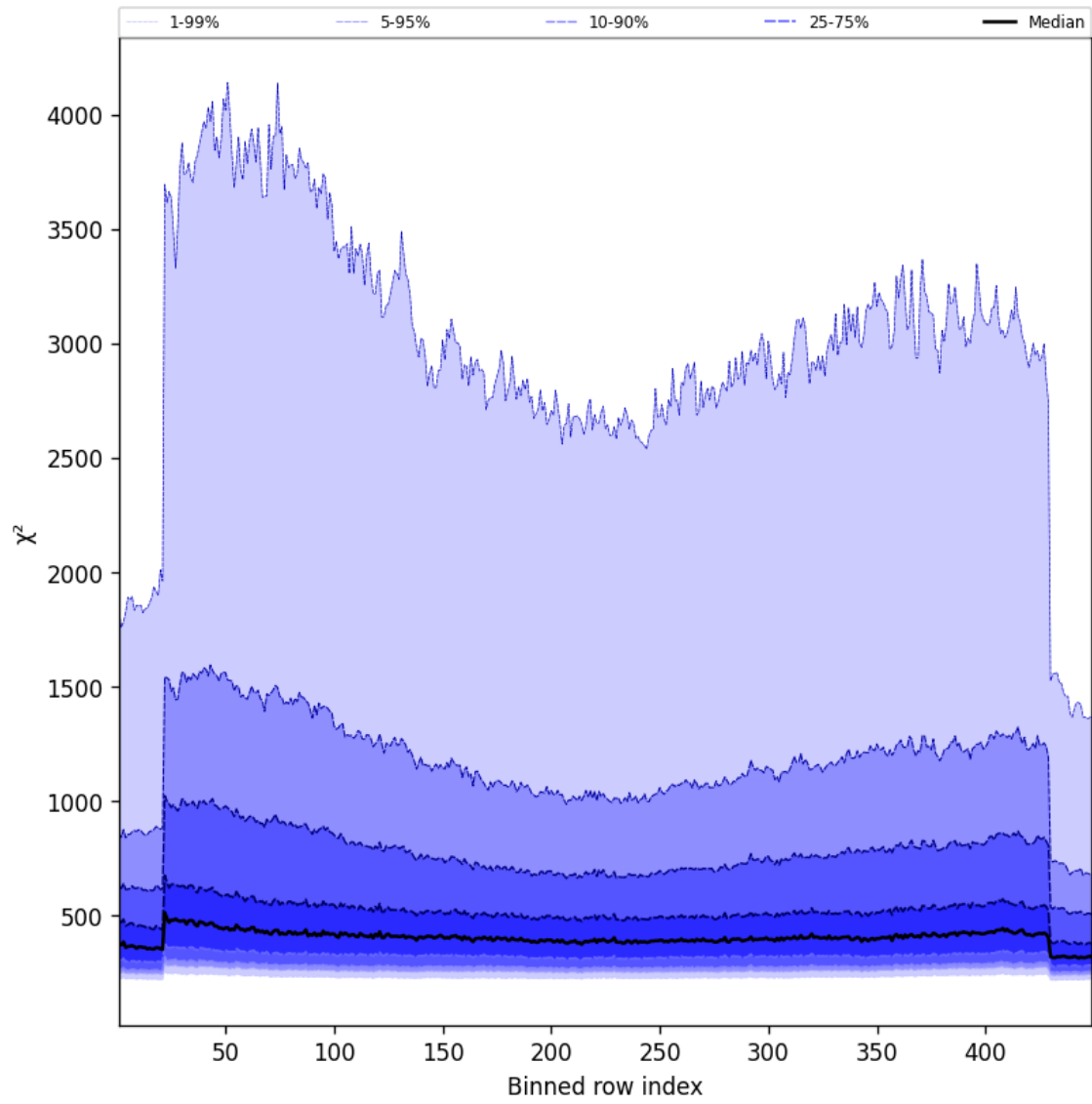
Figure 57: Along track statistics of “ \chi^2 ” for 2025-01-15 to 2025-01-15
