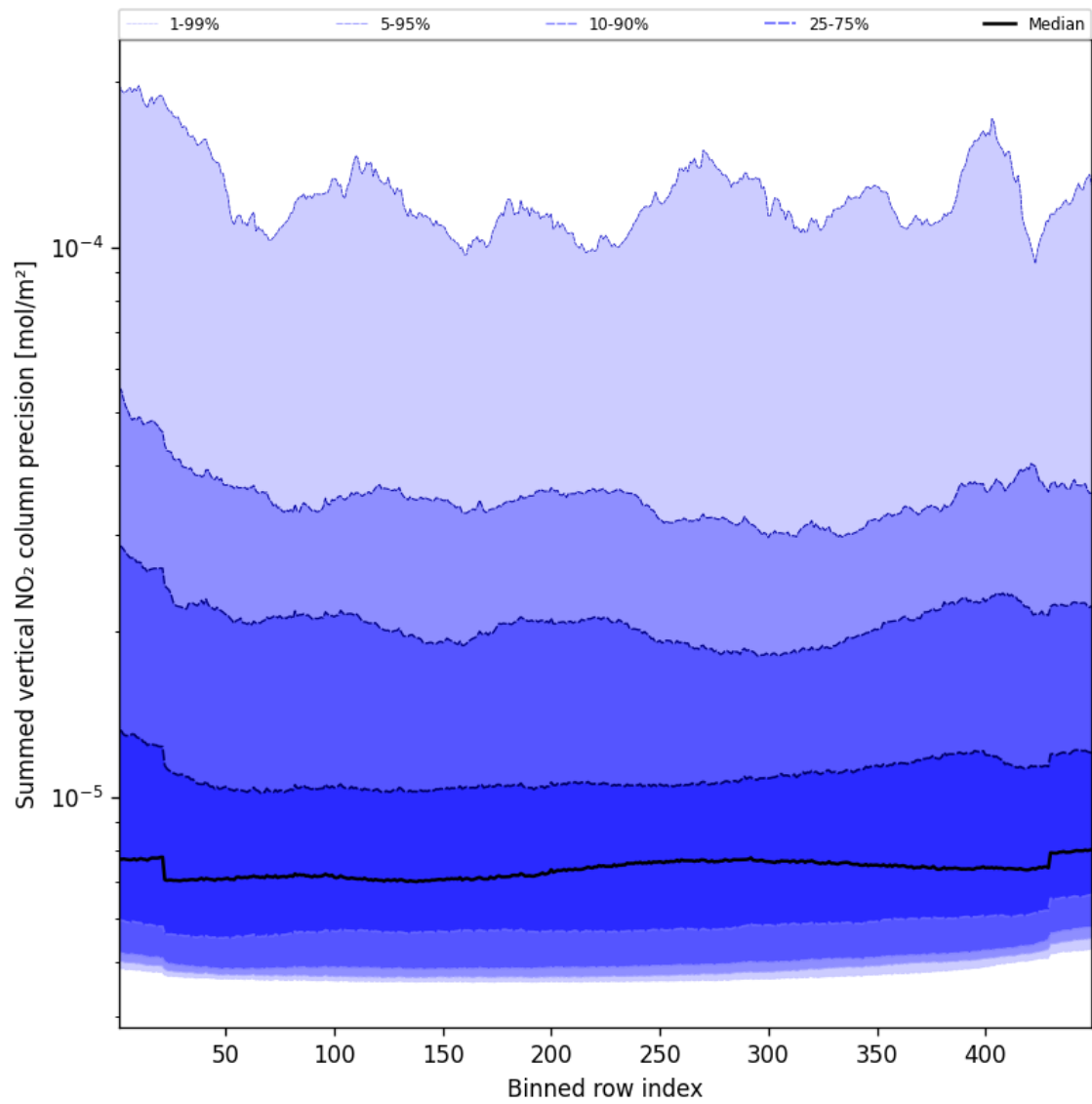
Figure 56: Along track statistics of “Summed vertical NO 2 column precision” for 2025-01-15 to 2025-01-15
