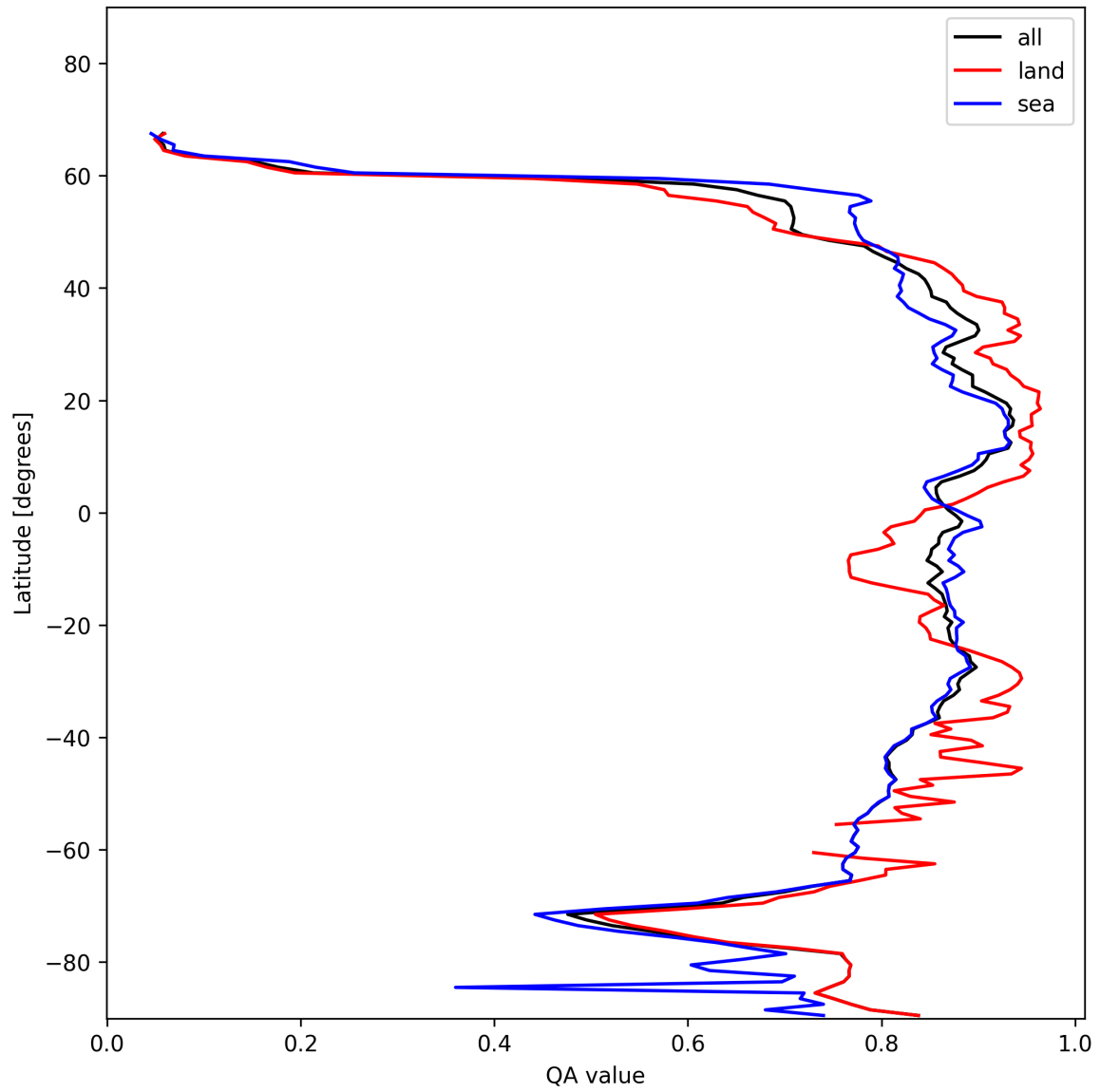
Figure 9: Zonal average of “QA value” for 2025-01-15 to 2025-01-15.
