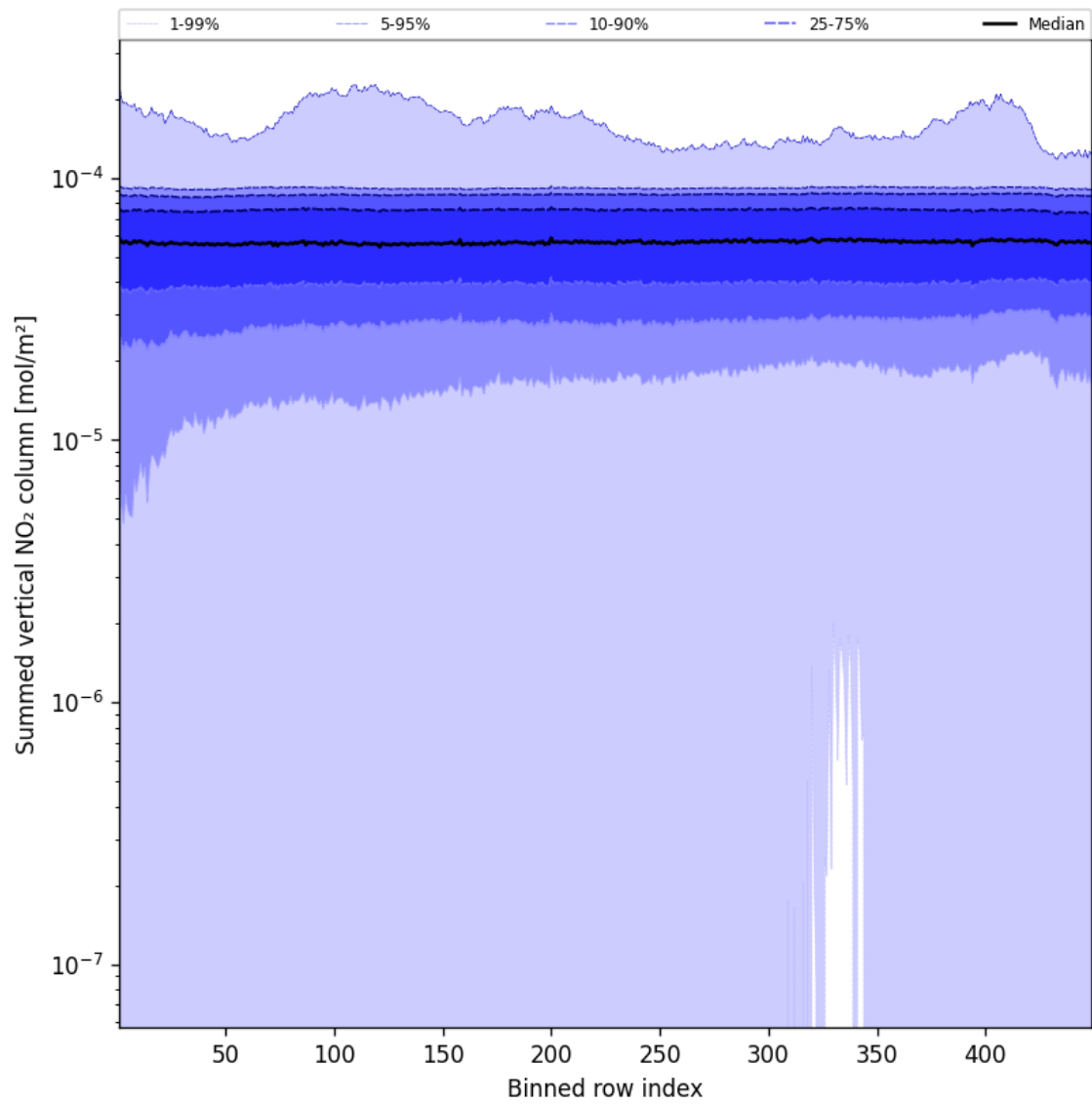
Figure 55: Along track statistics of “Summed vertical NO 2 column” for 2025-01-15 to 2025-01-15
