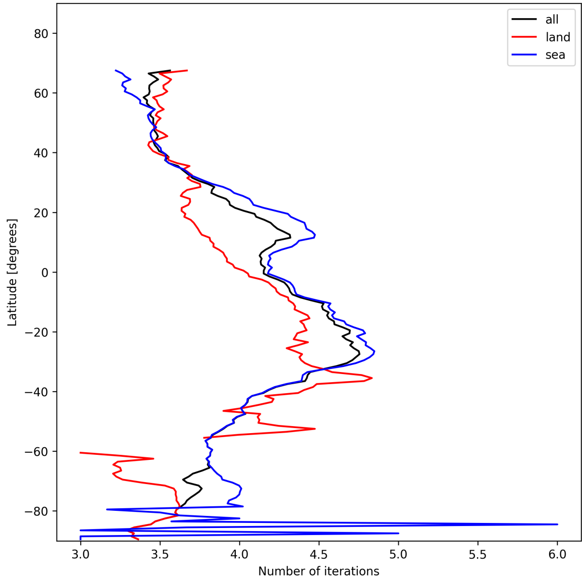
Figure 15: Zonal average of “Number of iterations” for 2025-01-15 to 2025-01-15.
