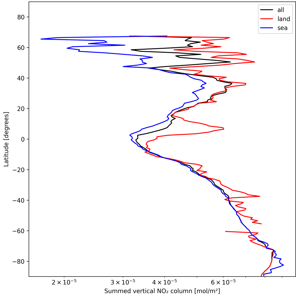
Figure 21: Zonal average of “Summed vertical NO 2 column” for 2025-01-15 to 2025-01-15.
