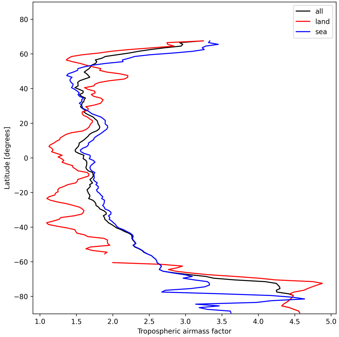
Figure 12: Zonal average of “Tropospheric airmass factor” for 2025-01-15 to 2025-01-15.
