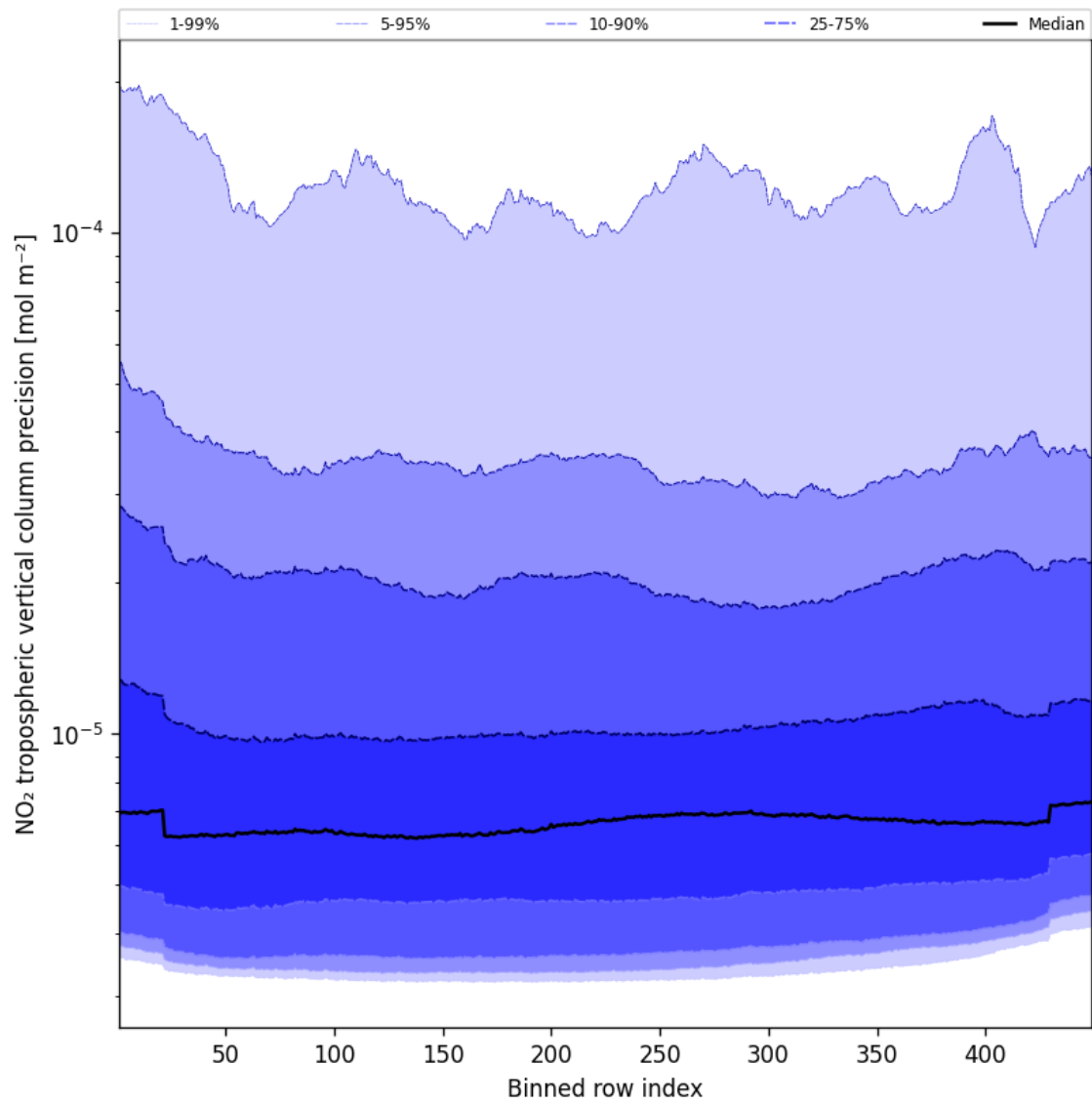
Figure 45: Along track statistics of “NO 2 tropospheric vertical column precision” for 2025-01-15 to 2025-01-15
