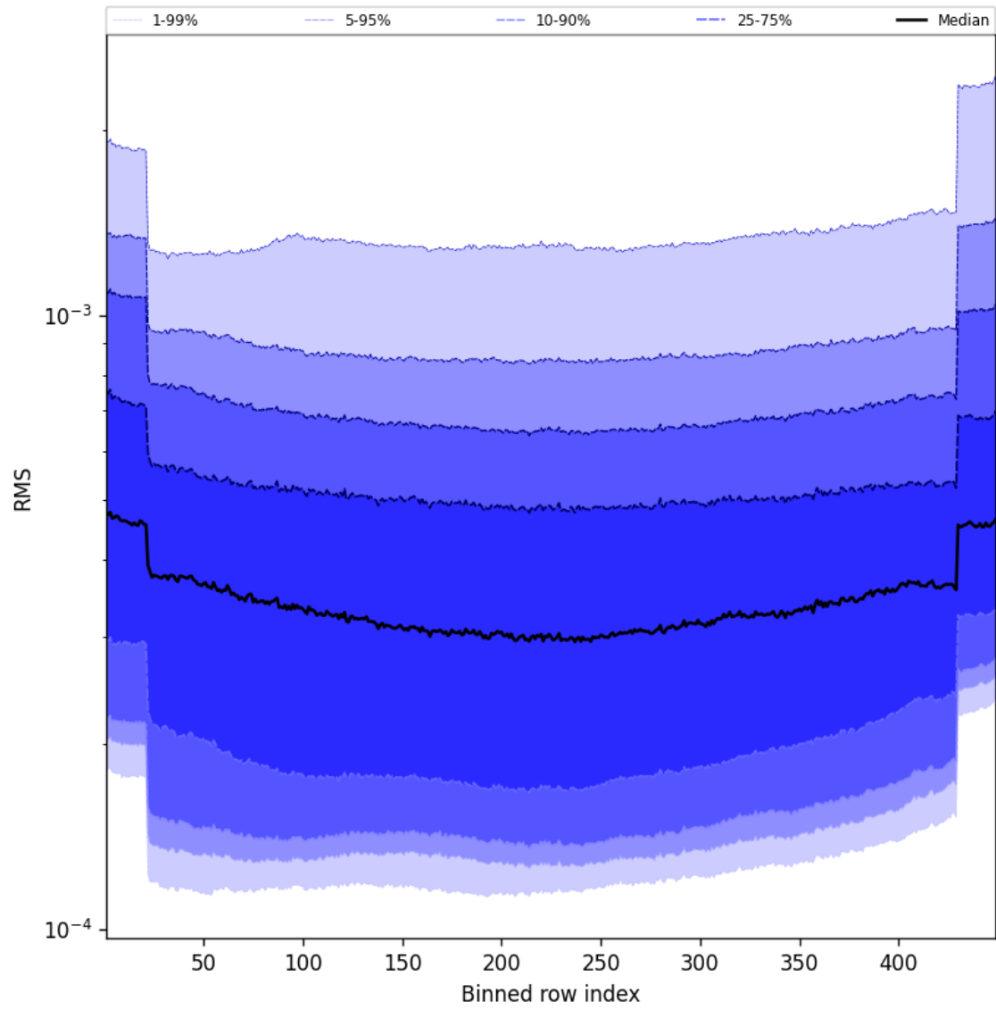
Figure 58: Along track statistics of “RMS” for 2025-01-15 to 2025-01-15
