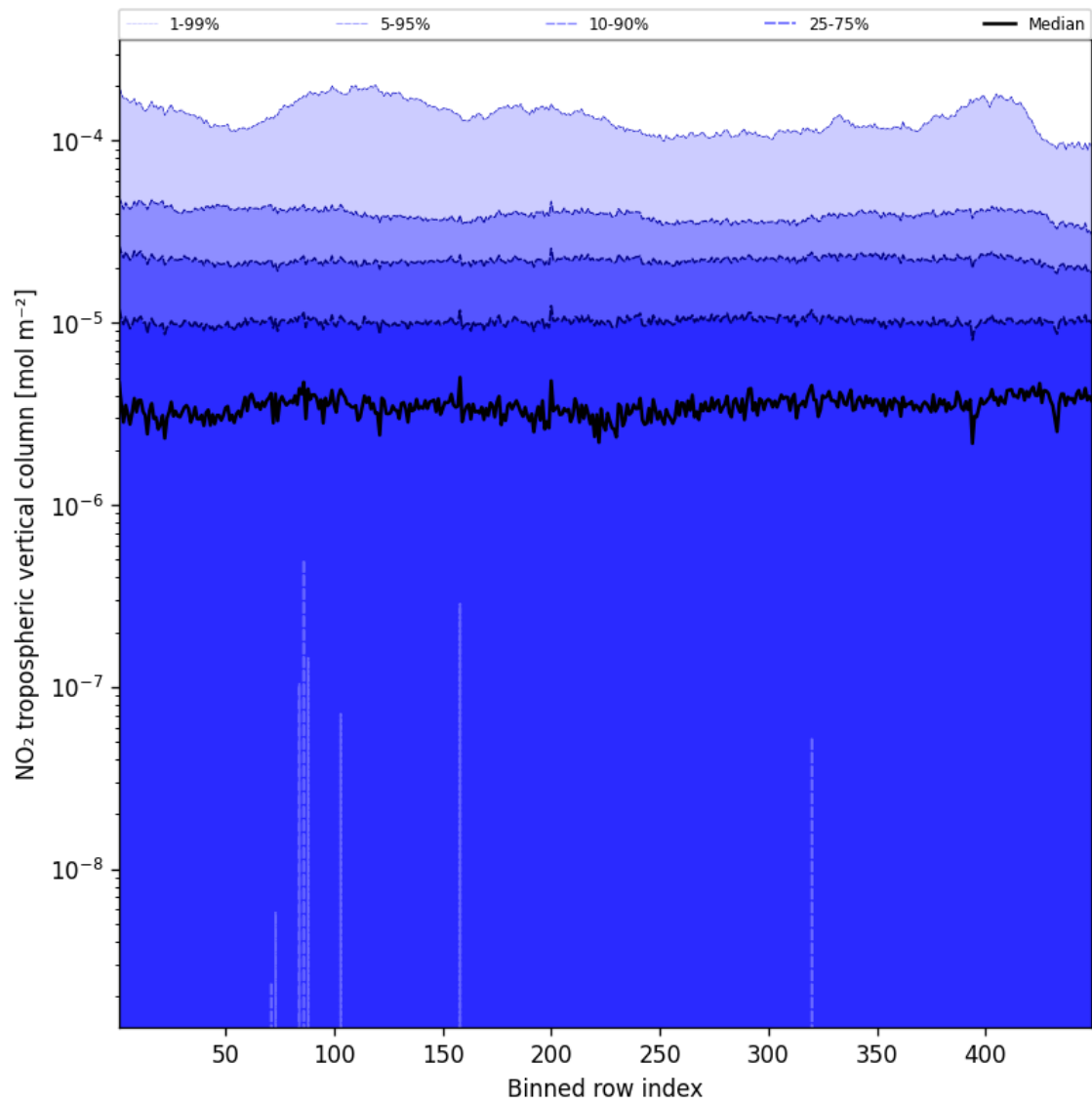
Figure 44: Along track statistics of “NO 2 tropospheric vertical column” for 2025-01-15 to 2025-01-15
