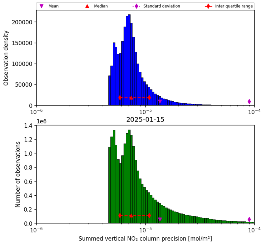
Figure 39: Histogram of "Summed vertical NO 2 column precision" for 2025-01-15 to 2025-01-15
