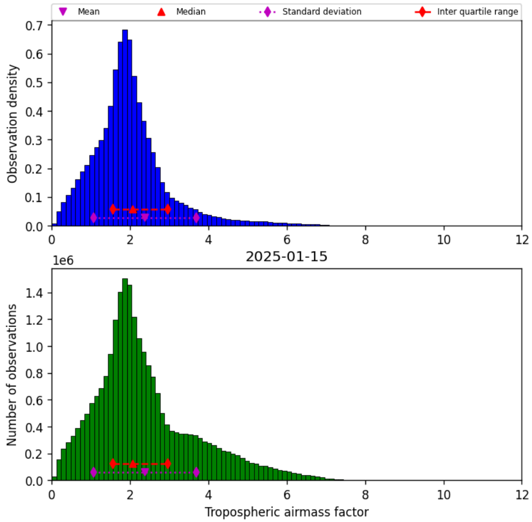
Figure 29: Histogram of “Tropospheric airmass factor” for 2025-01-15 to 2025-01-15
