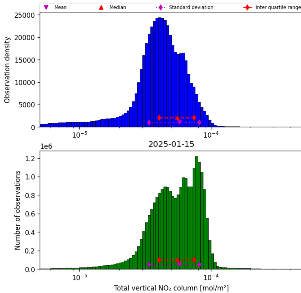
Figure 36: Histogram of “Total vertical NO 2 column” for 2025-01-15 to 2025-01-15
