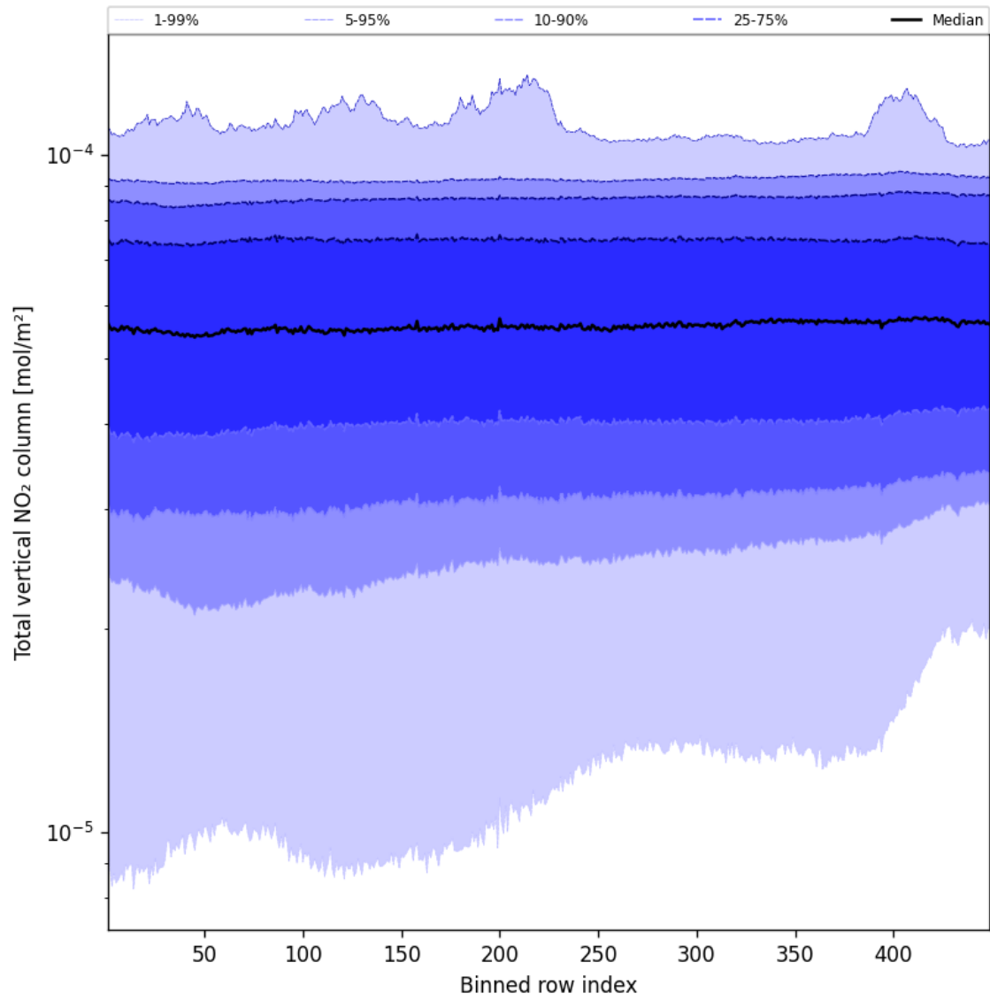
Figure 53: Along track statistics of “Total vertical NO 2 column” for 2025-01-15 to 2025-01-15
