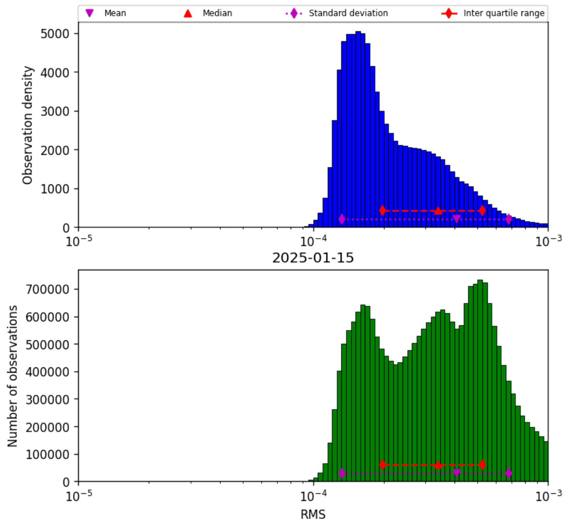
Figure 41: Histogram of “RMS” for 2025-01-15 to 2025-01-15
