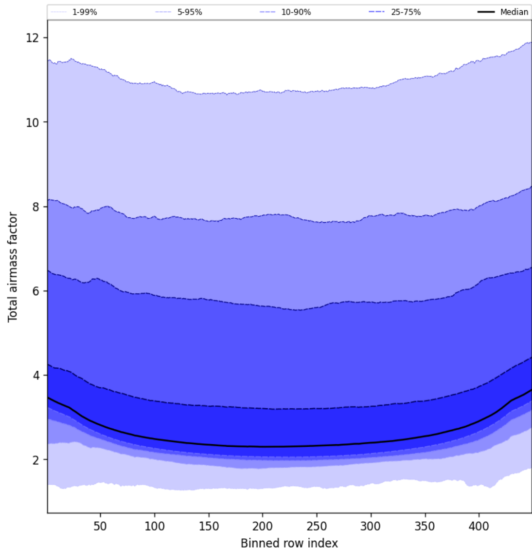
Figure 47: Along track statistics of “Total airmass factor” for 2025-01-15 to 2025-01-15
