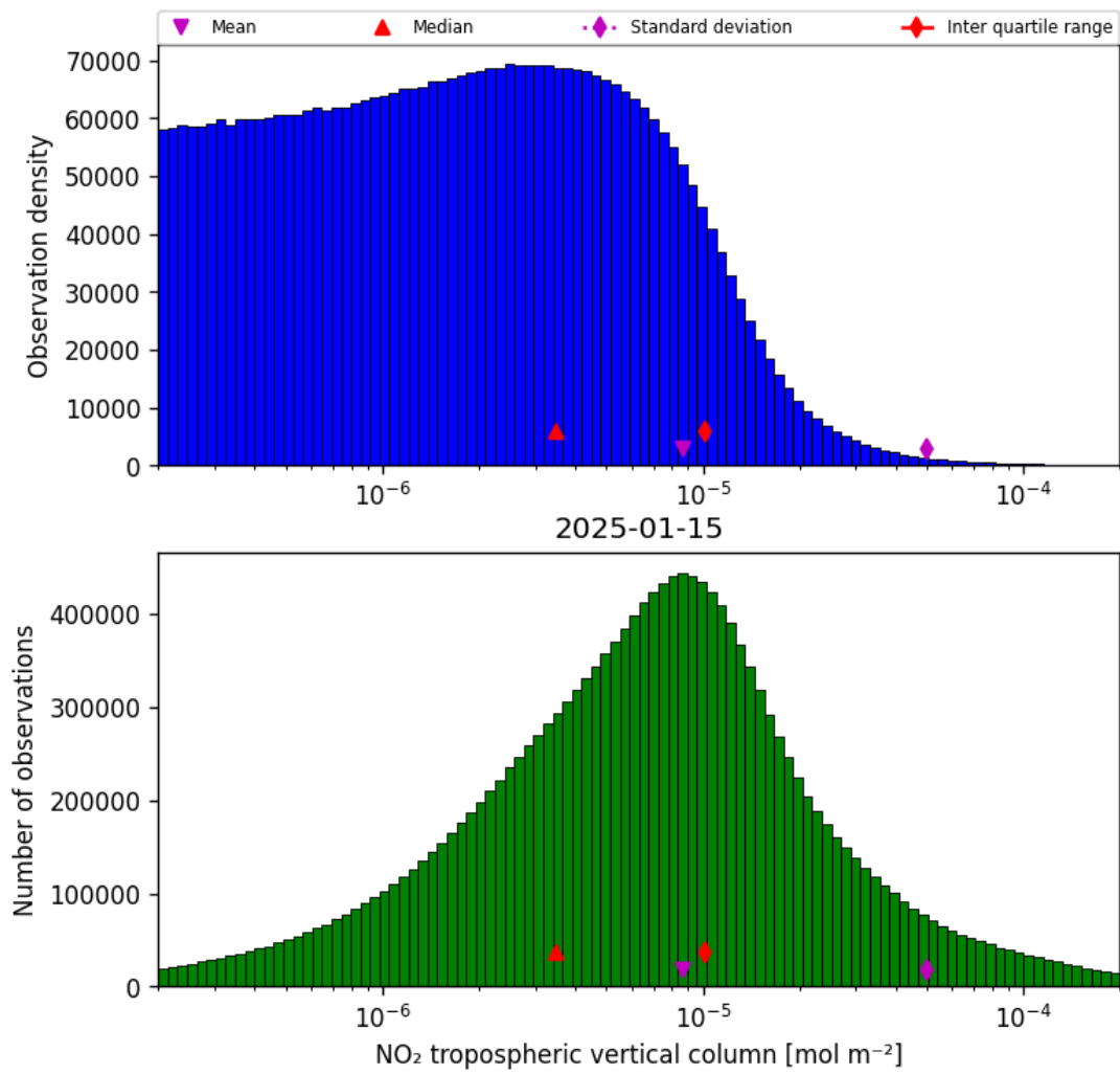
Figure 27: Histogram of “ \text{NO}_2 tropospheric vertical column” for 2025-01-15 to 2025-01-15
