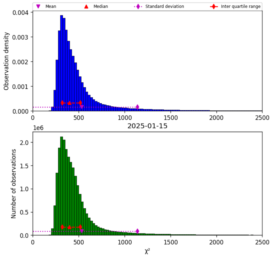
Figure 40: Histogram of “ \chi^2 ” for 2025-01-15 to 2025-01-15
