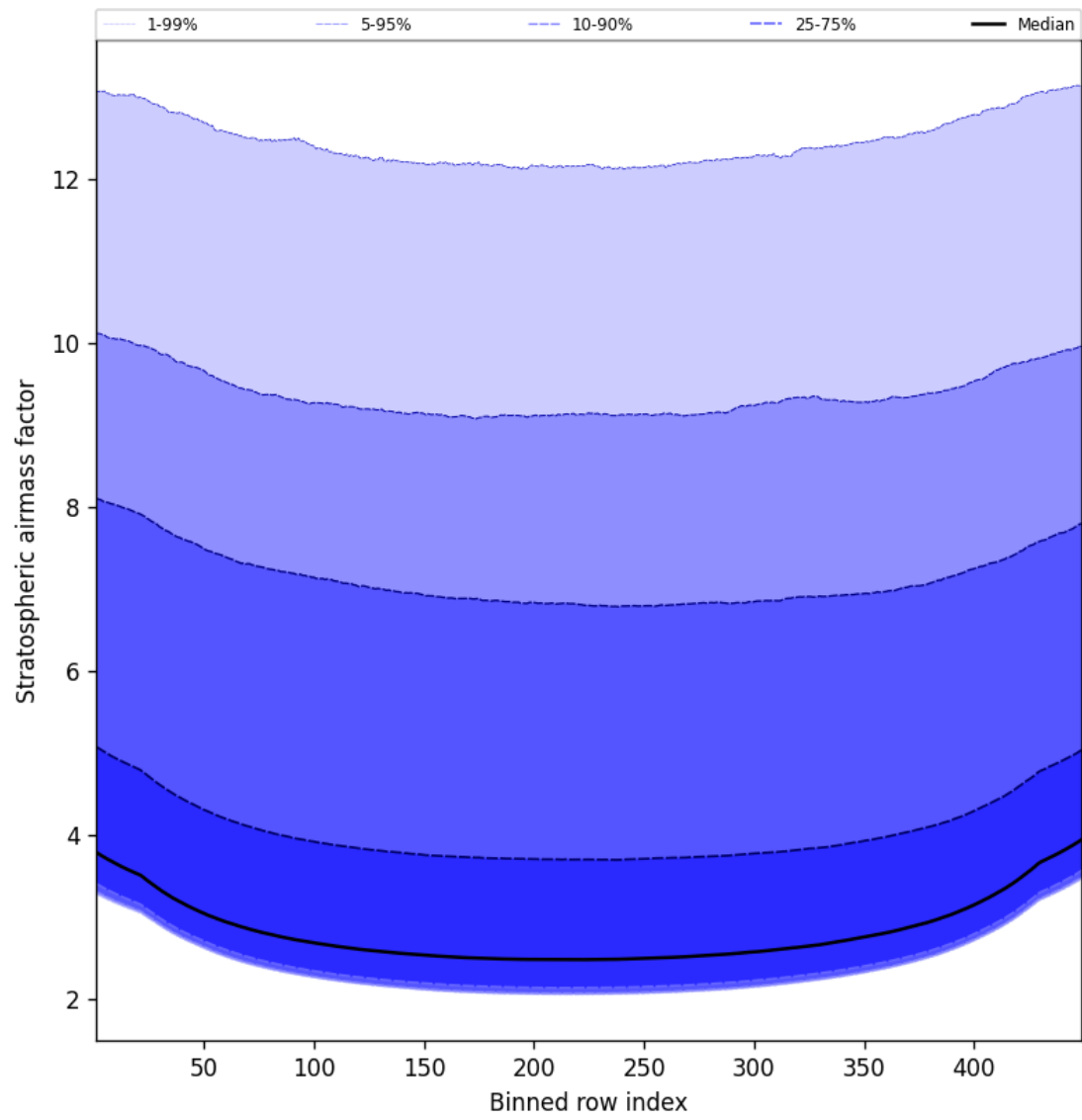
Figure 59: Along track statistics of “Stratospheric airmass factor” for 2025-01-15 to 2025-01-15
