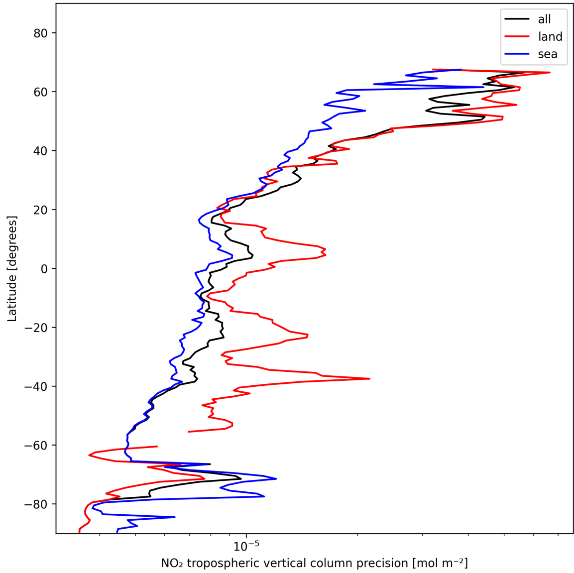
Figure 11: Zonal average of “NO 2 tropospheric vertical column precision” for 2025-01-15 to 2025-01-15.
