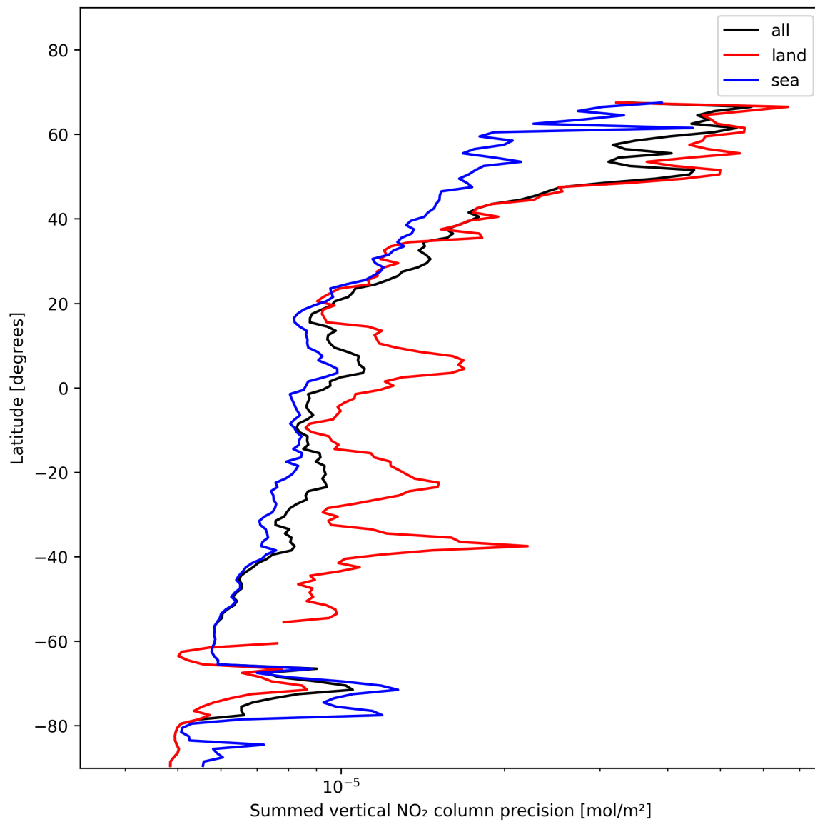
Figure 22: Zonal average of “Summed vertical NO 2 column precision” for 2025-01-15 to 2025-01-15.
