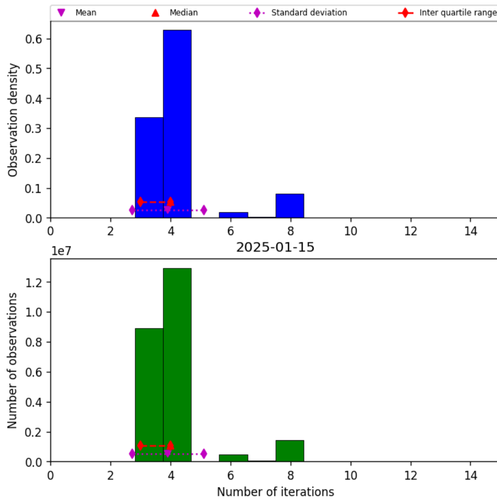
Figure 32: Histogram of “Number of iterations” for 2025-01-15 to 2025-01-15
