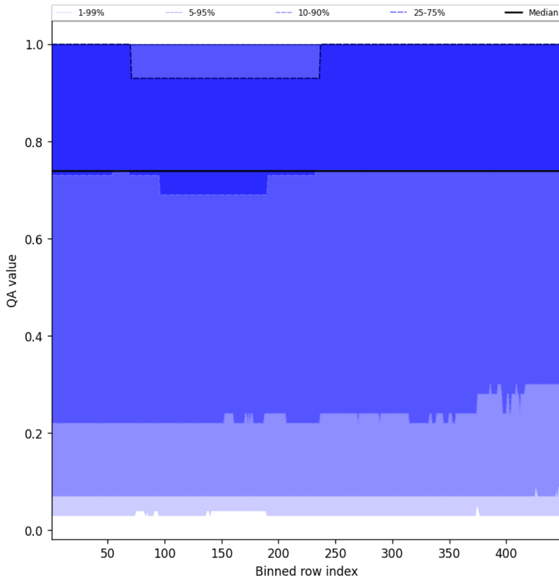
Figure 43: Along track statistics of “QA value” for 2025-01-15 to 2025-01-15
