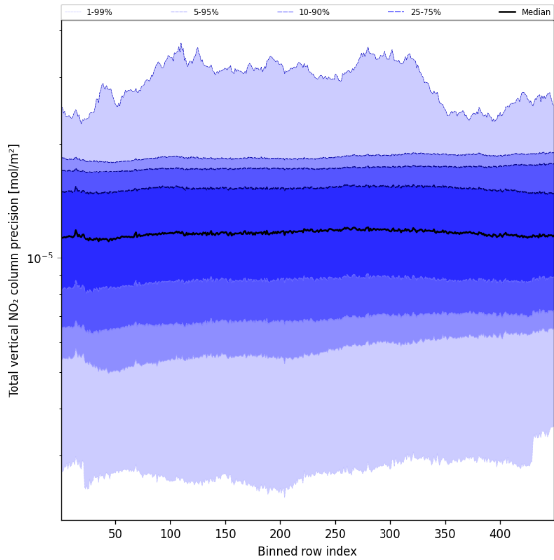
Figure 54: Along track statistics of “Total vertical NO 2 column precision” for 2025-01-16 to 2025-01-17
