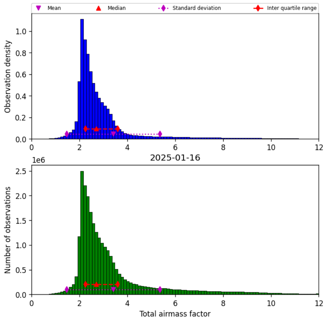
Figure 30: Histogram of “Total airmass factor” for 2025-01-16 to 2025-01-17
