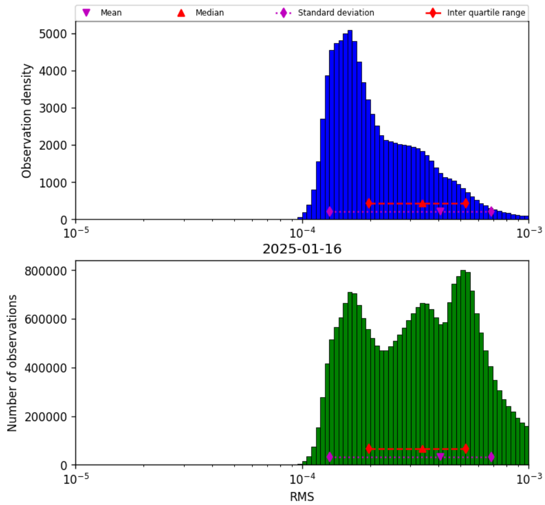
Figure 41: Histogram of “RMS” for 2025-01-16 to 2025-01-17
