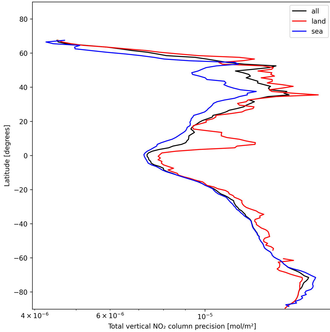
Figure 20: Zonal average of “Total vertical NO 2 column precision” for 2025-01-16 to 2025-01-17.
