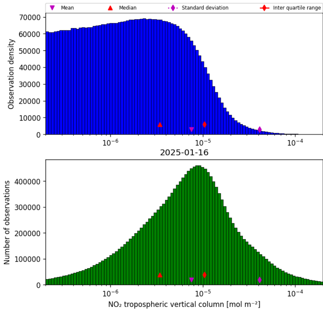
Figure 27: Histogram of “NO 2 tropospheric vertical column” for 2025-01-16 to 2025-01-17
