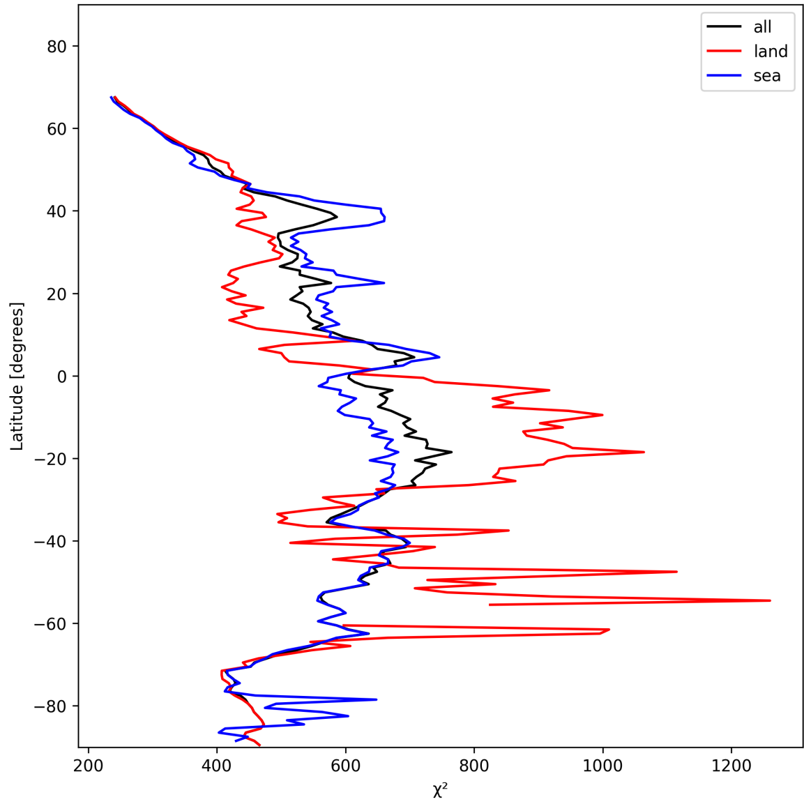
Figure 23: Zonal average of “ \chi^2 ” for 2025-01-16 to 2025-01-17.
