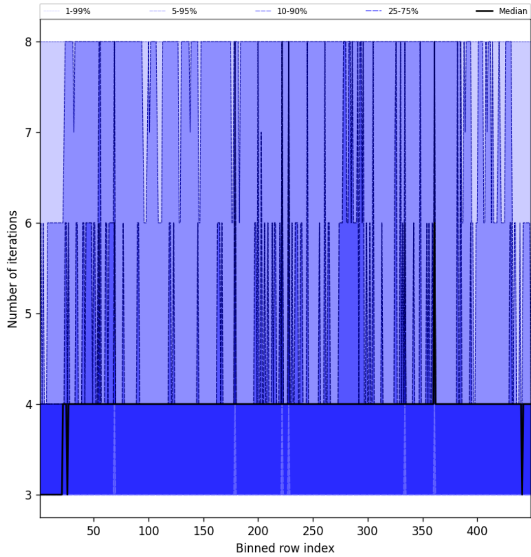
Figure 49: Along track statistics of “Number of iterations” for 2025-01-16 to 2025-01-17
