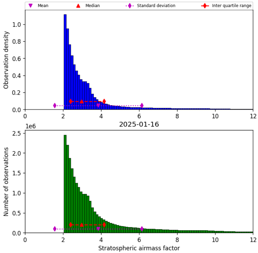
Figure 42: Histogram of “Stratospheric airmass factor” for 2025-01-16 to 2025-01-17
