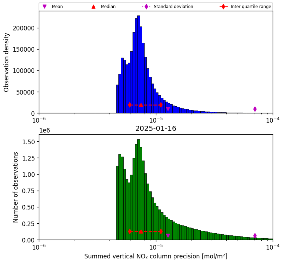
Figure 39: Histogram of “Summed vertical NO 2 column precision” for 2025-01-16 to 2025-01-17
