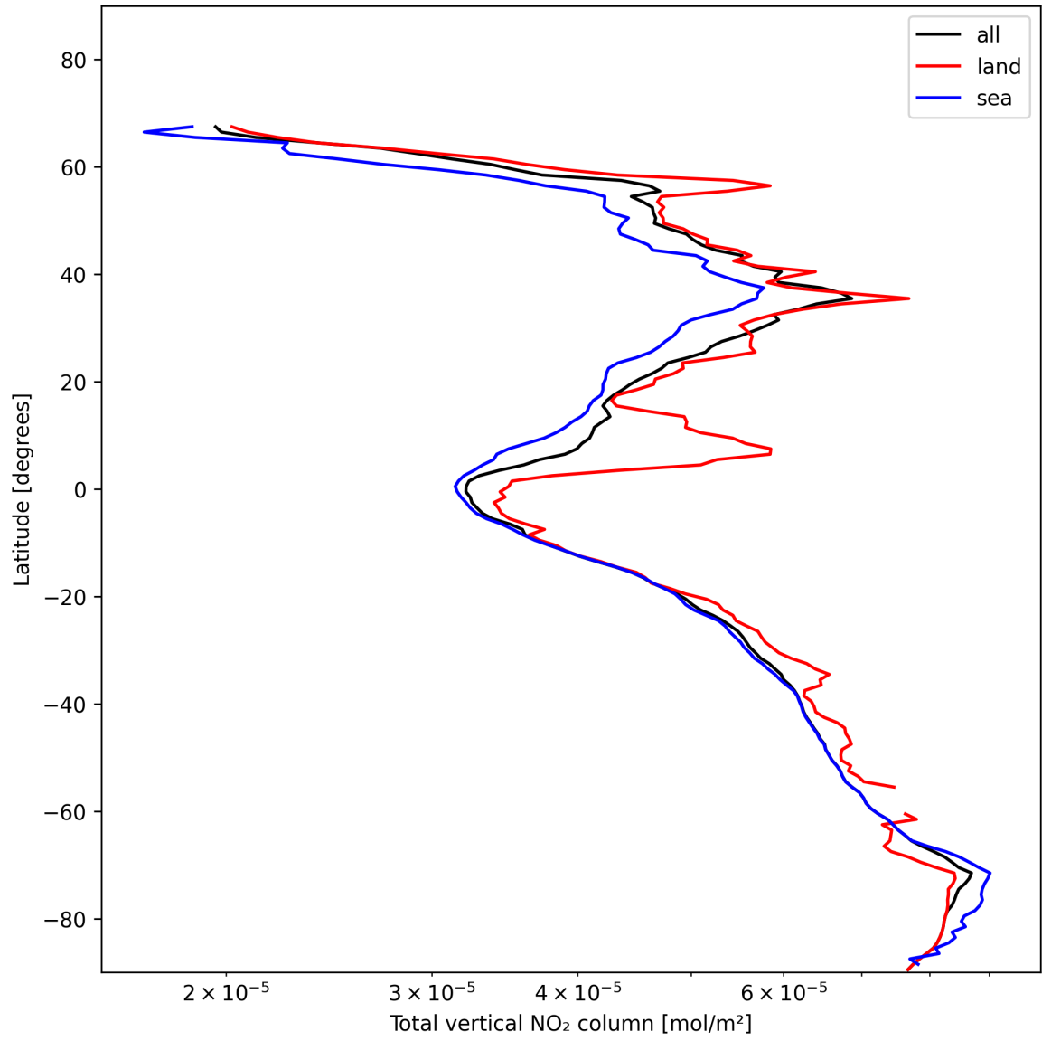
Figure 19: Zonal average of “Total vertical NO 2 column” for 2025-01-16 to 2025-01-17.
