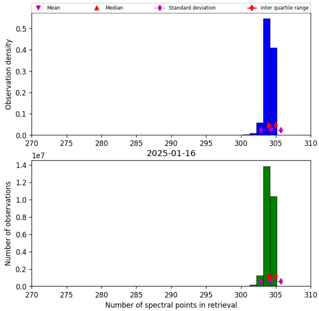
Figure 31: Histogram of “Number of spectral points in retrieval” for 2025-01-16 to 2025-01-17
