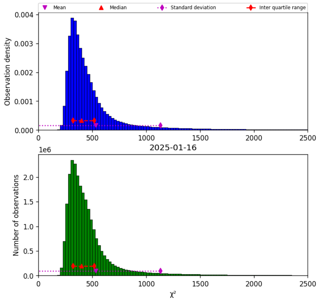
Figure 40: Histogram of “ \chi^2 ” for 2025-01-16 to 2025-01-17
