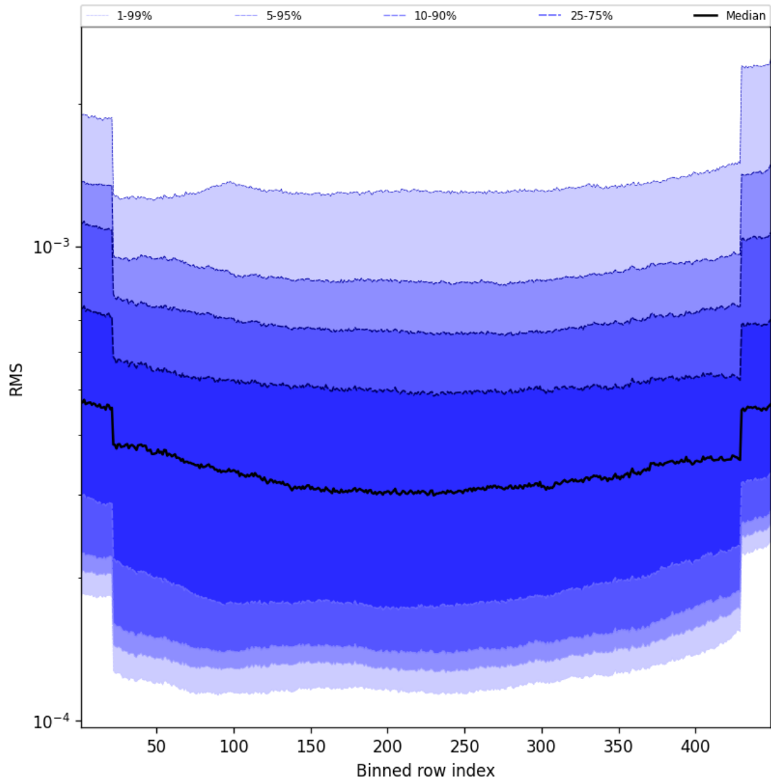
Figure 58: Along track statistics of “RMS” for 2025-01-16 to 2025-01-17
