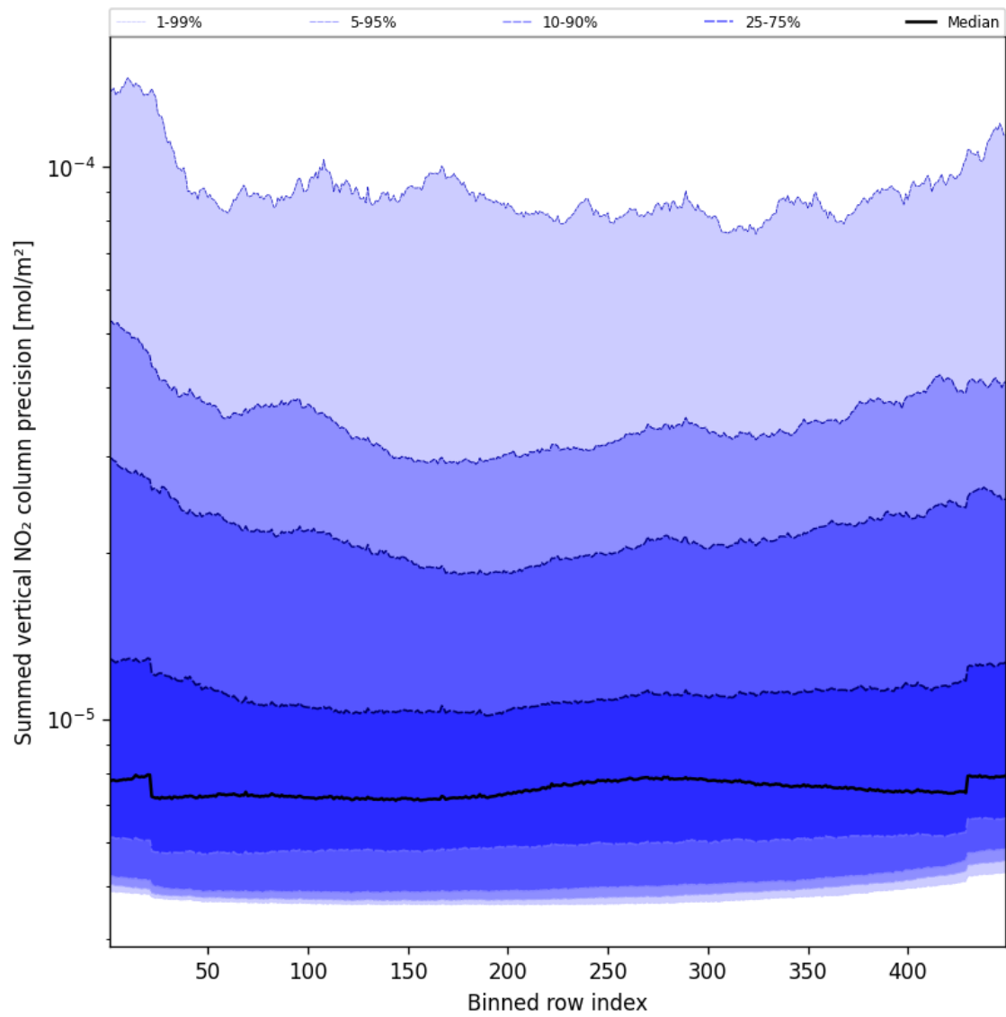
Figure 56: Along track statistics of “Summed vertical NO 2 column precision” for 2025-01-16 to 2025-01-17
