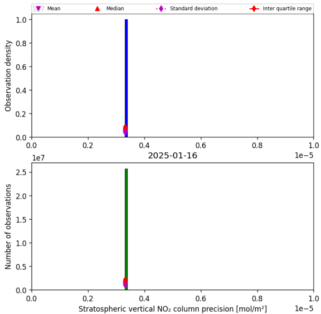
Figure 35: Histogram of “Stratospheric vertical NO 2 column precision” for 2025-01-16 to 2025-01-17
