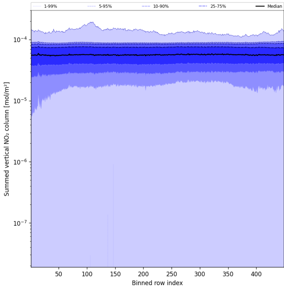
Figure 55: Along track statistics of “Summed vertical NO 2 column” for 2025-01-16 to 2025-01-17
