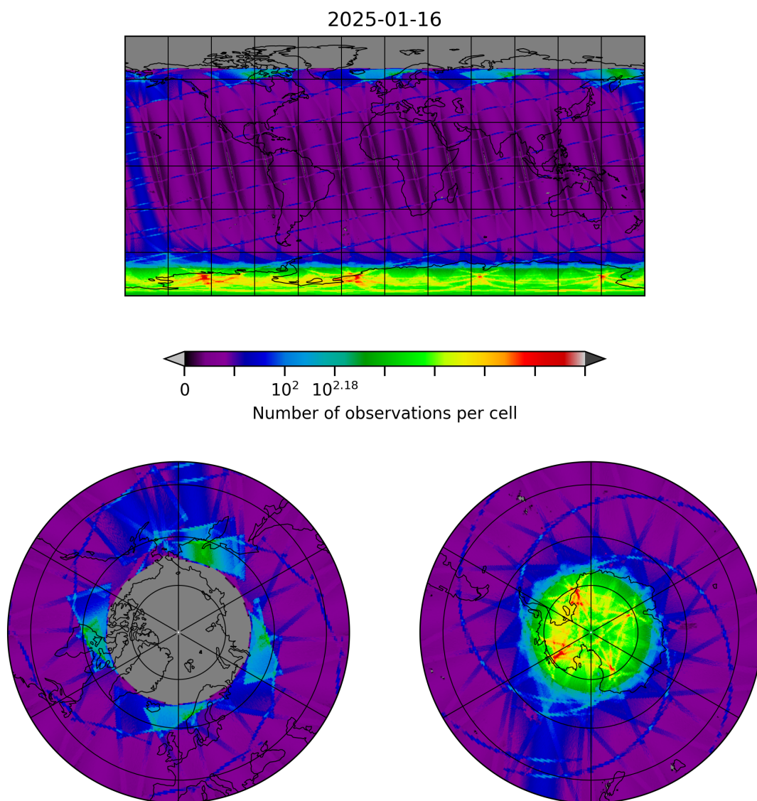
Figure 8: Map of the number of observations for 2025-01-16 to 2025-01-17
