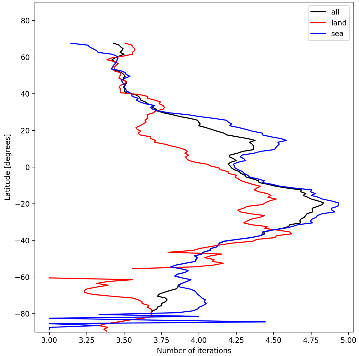
Figure 15: Zonal average of “Number of iterations” for 2025-01-16 to 2025-01-17.
