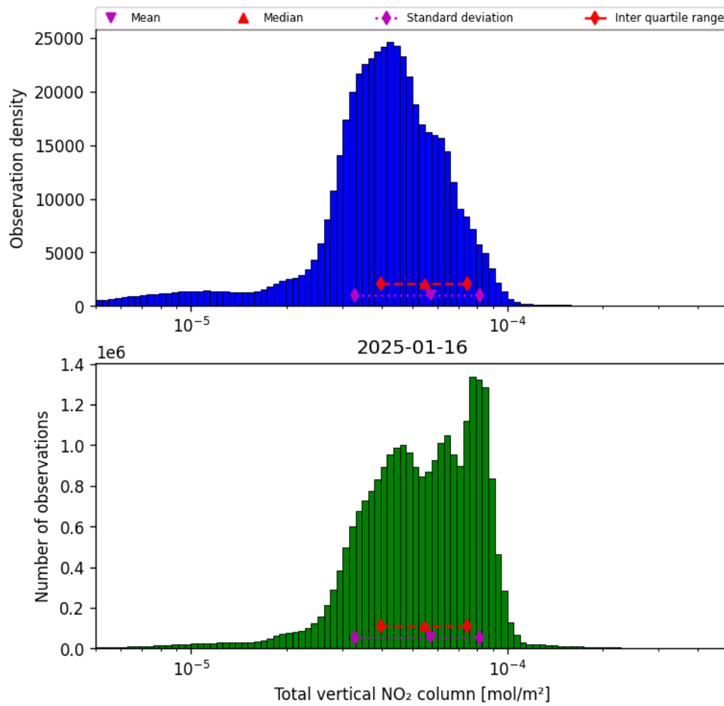
Figure 36: Histogram of “Total vertical NO 2 column” for 2025-01-16 to 2025-01-17
