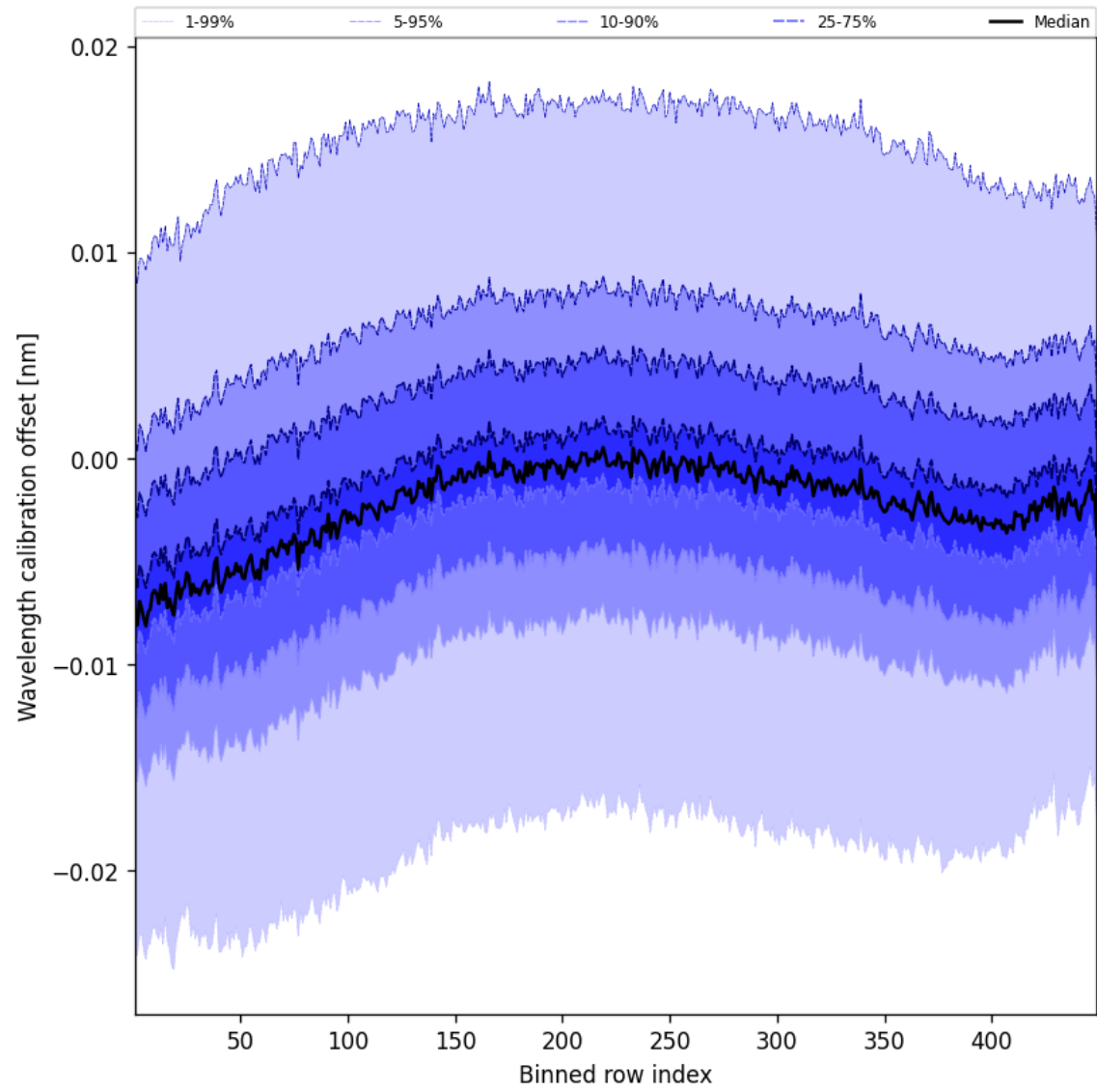
Figure 50: Along track statistics of “Wavelength calibration offset” for 2025-01-16 to 2025-01-17
