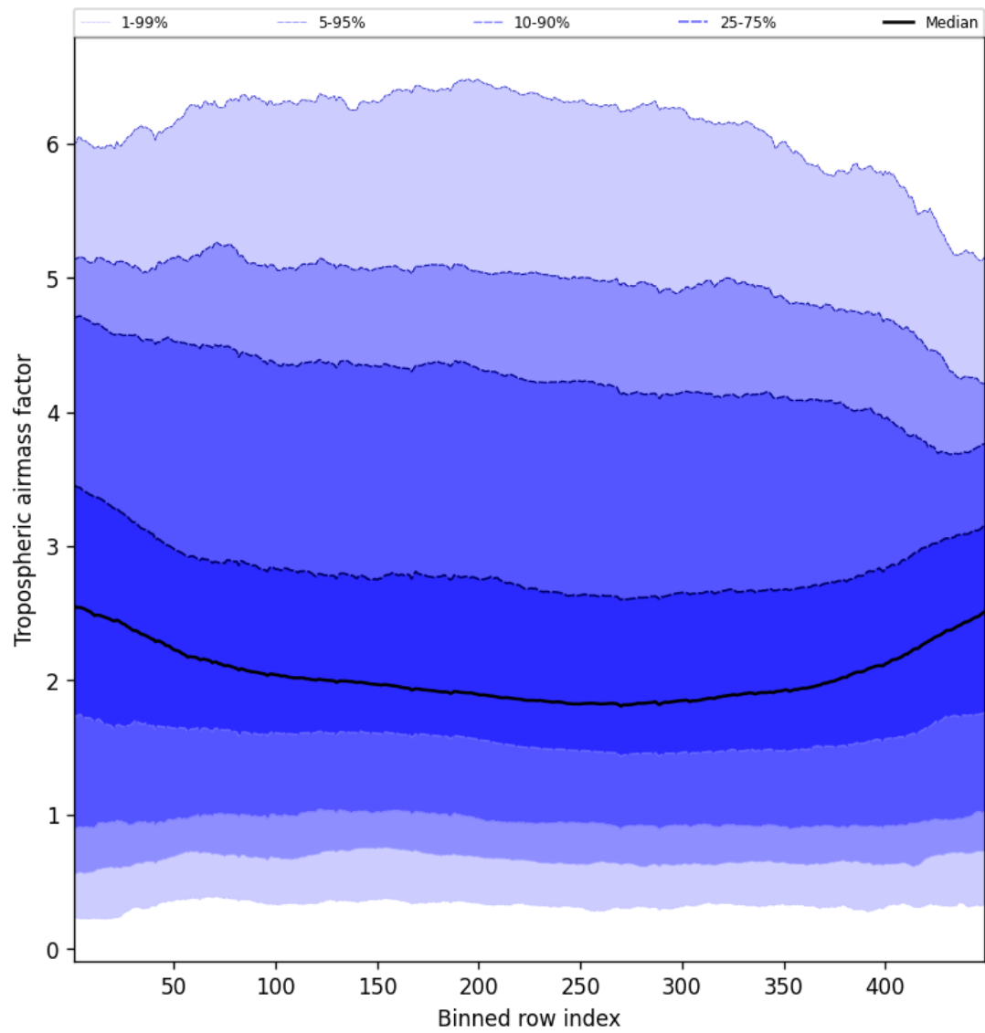
Figure 46: Along track statistics of “Tropospheric air mass factor” for 2025-01-16 to 2025-01-17
