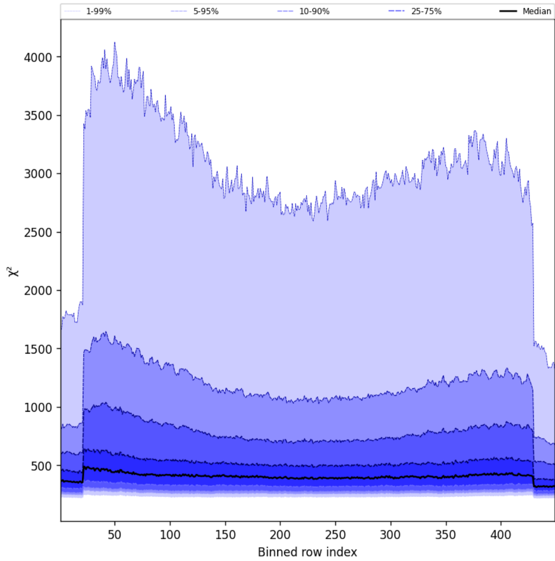
Figure 57: Along track statistics of “ \chi^2 ” for 2025-01-16 to 2025-01-17
