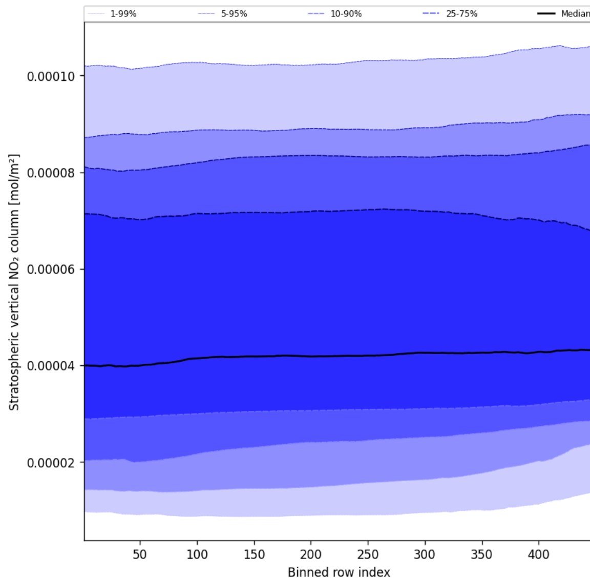
Figure 51: Along track statistics of “Stratospheric vertical NO 2 column” for 2025-01-16 to 2025-01-17
