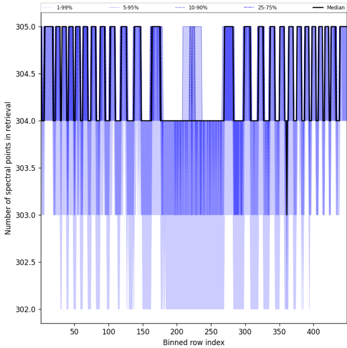
Figure 48: Along track statistics of “Number of spectral points in retrieval” for 2025-01-16 to 2025-01-17
