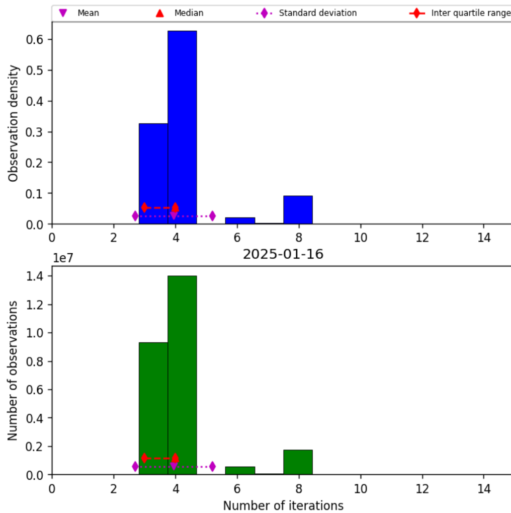
Figure 32: Histogram of “Number of iterations” for 2025-01-16 to 2025-01-17
