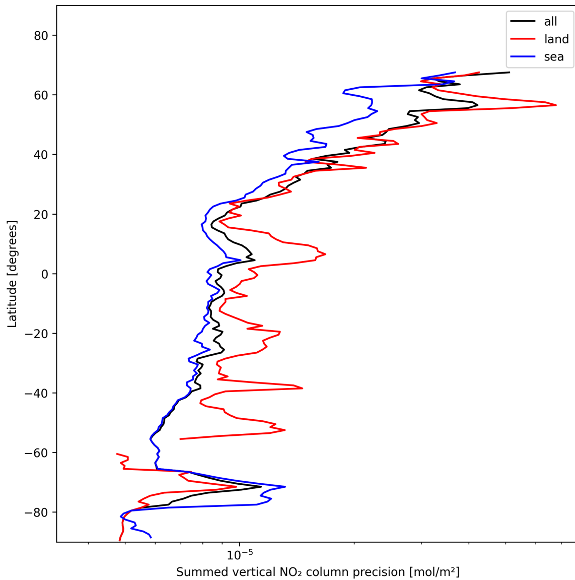
Figure 22: Zonal average of “Summed vertical NO 2 column precision” for 2025-01-16 to 2025-01-17.
