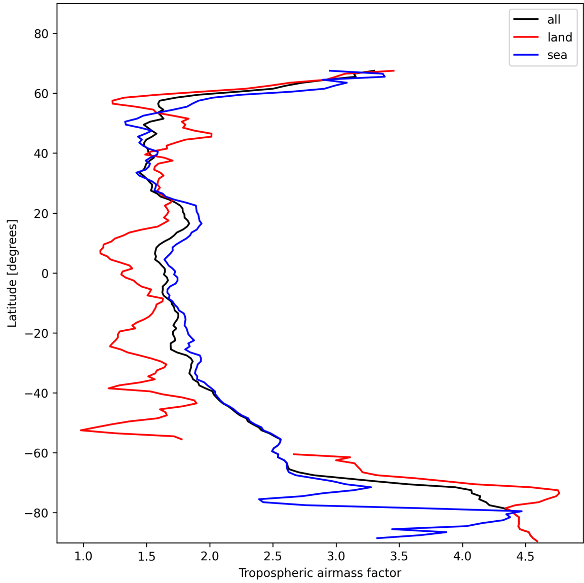
Figure 12: Zonal average of “Tropospheric airmass factor” for 2025-01-16 to 2025-01-17.
