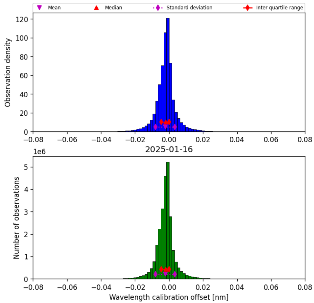
Figure 33: Histogram of “Wavelength calibration offset” for 2025-01-16 to 2025-01-17
