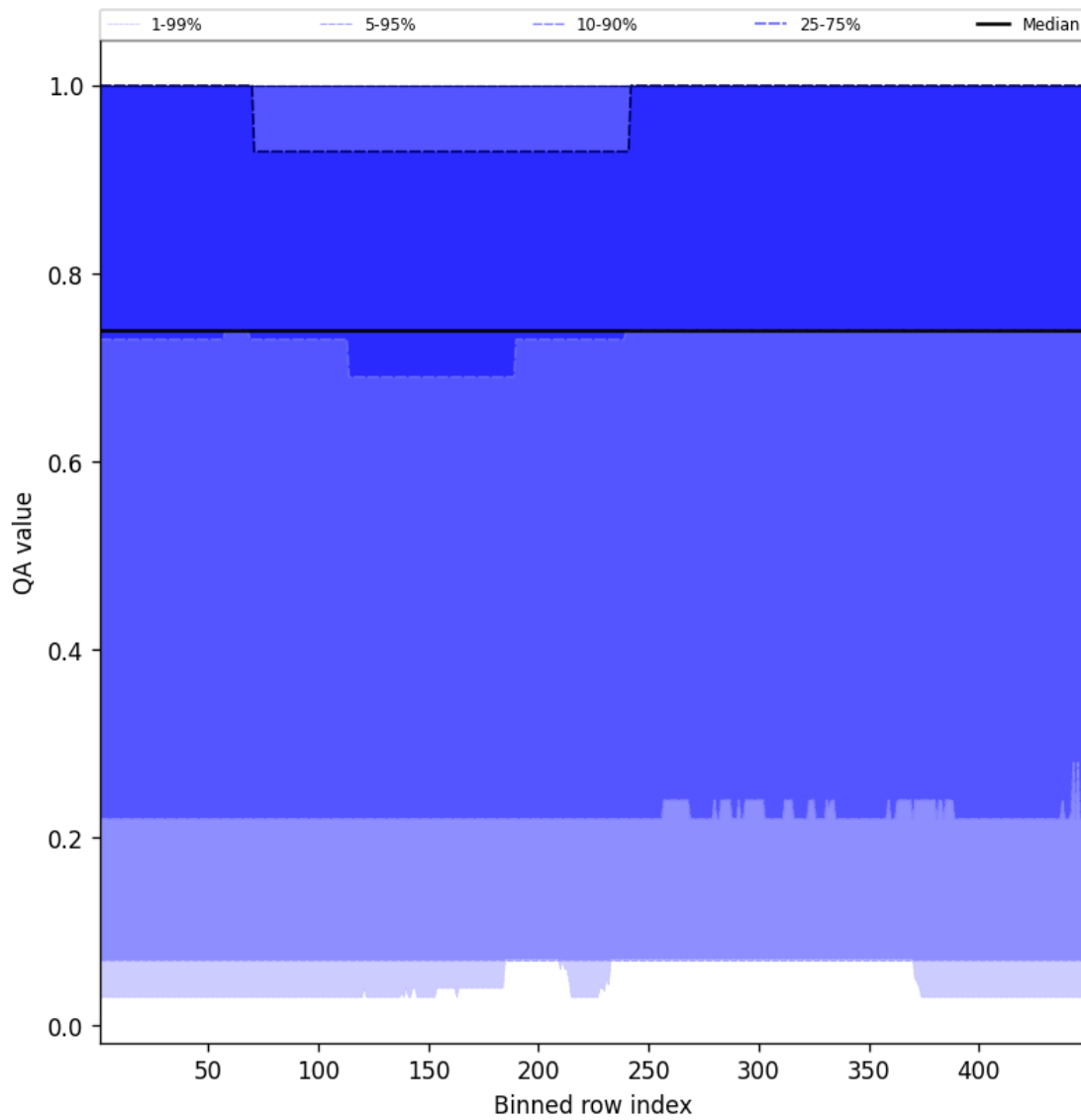
Figure 43: Along track statistics of “QA value” for 2025-01-16 to 2025-01-17
