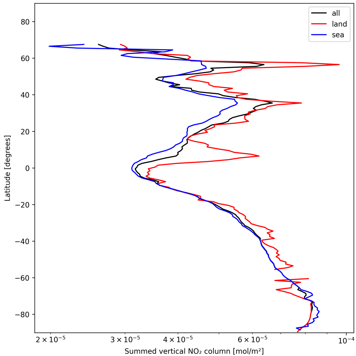
Figure 21: Zonal average of “Summed vertical NO 2 column” for 2025-01-16 to 2025-01-17.
