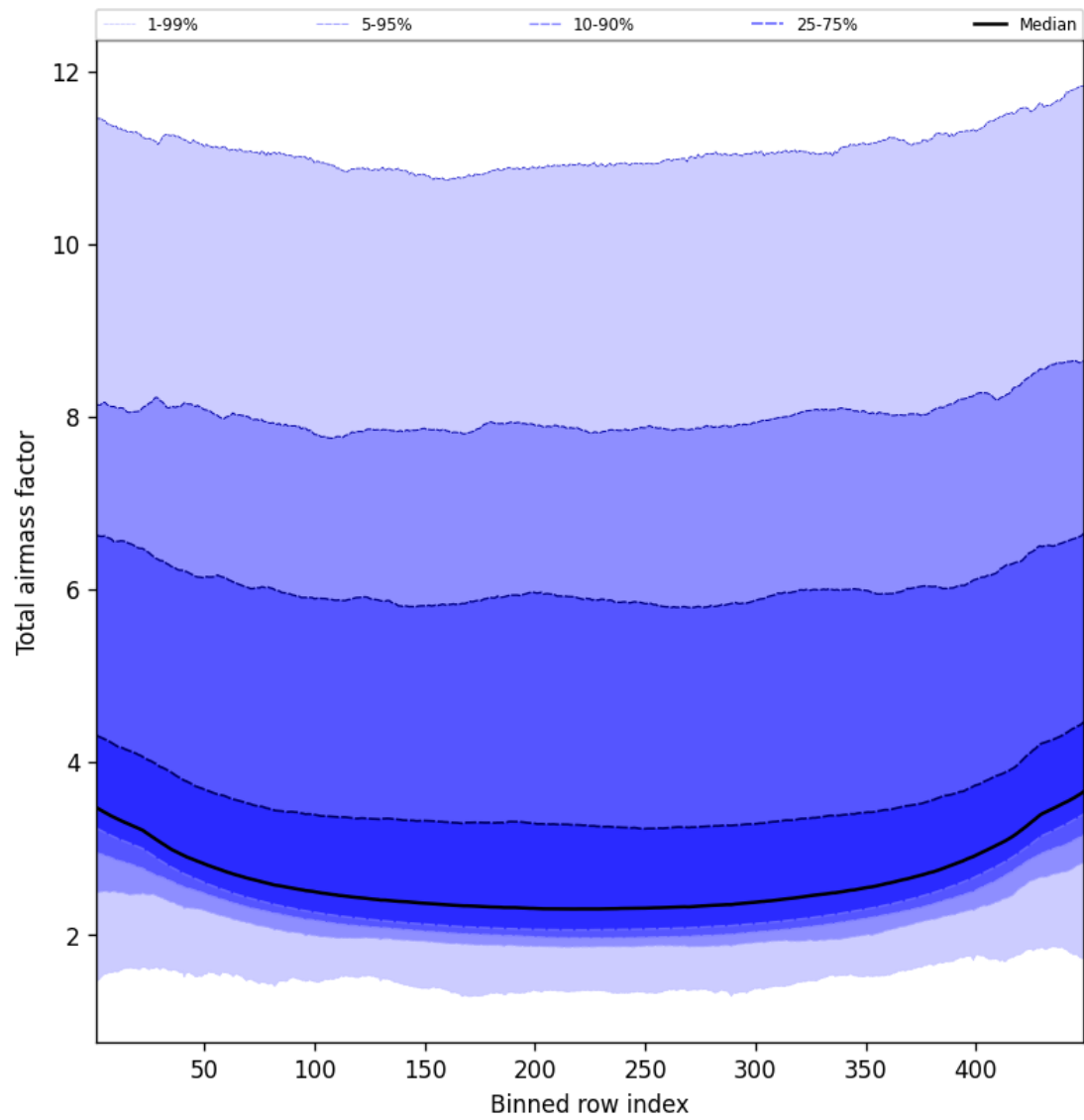
Figure 47: Along track statistics of “Total airmass factor” for 2025-01-16 to 2025-01-17
