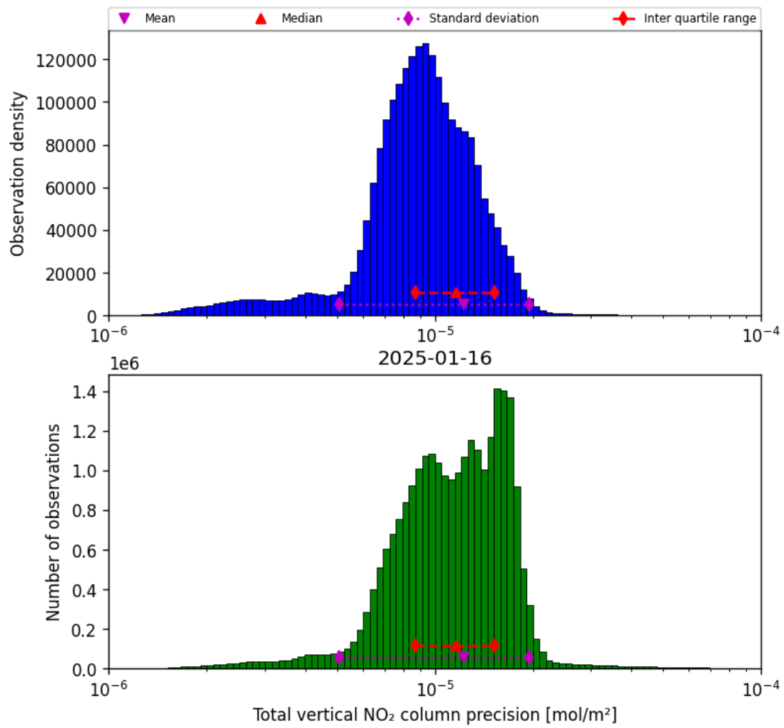
Figure 37: Histogram of “Total vertical NO 2 column precision” for 2025-01-16 to 2025-01-17
