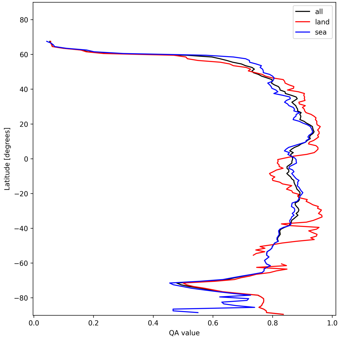
Figure 9: Zonal average of “QA value” for 2025-01-16 to 2025-01-17.
