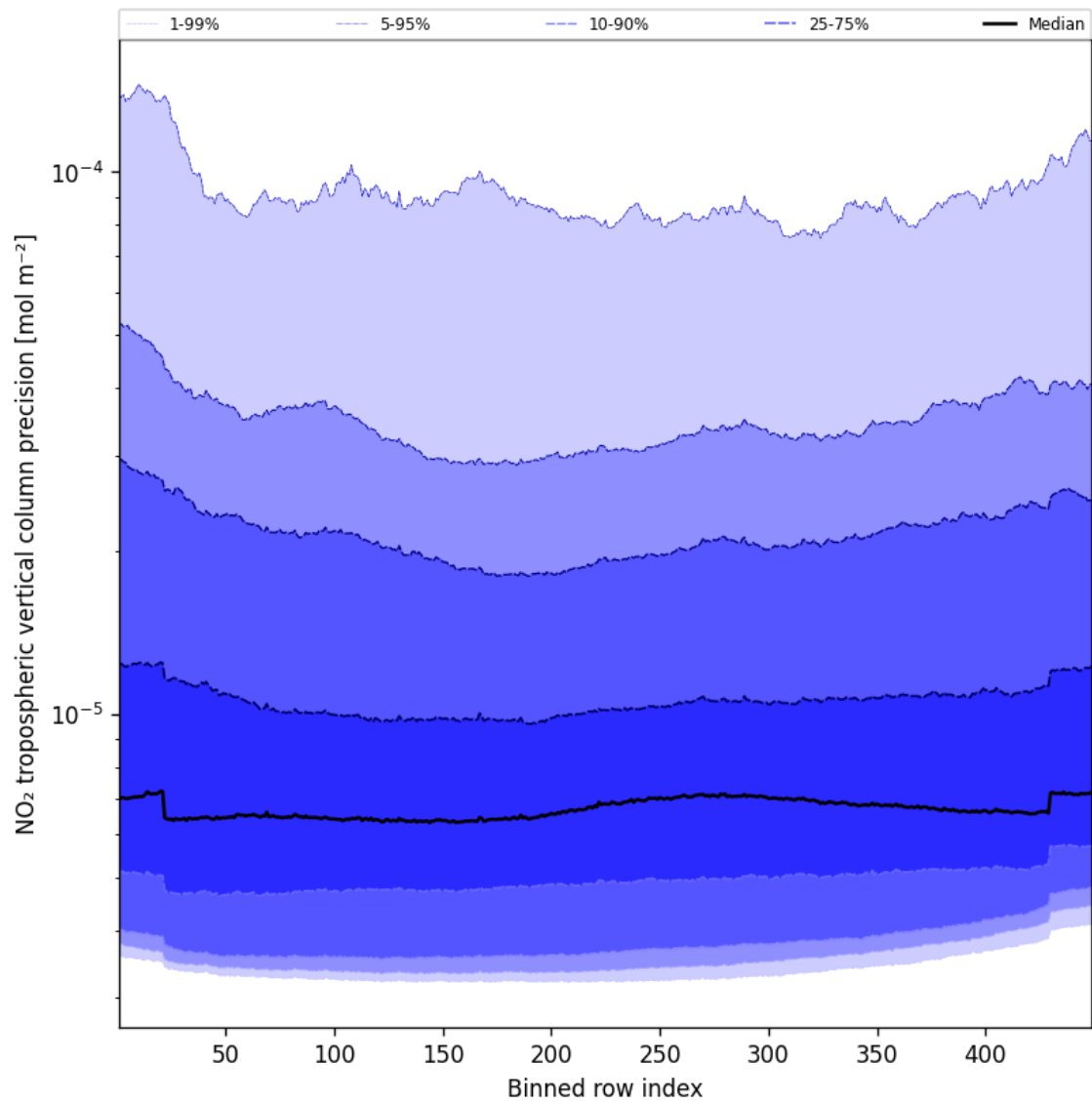
Figure 45: Along track statistics of “NO 2 tropospheric vertical column precision” for 2025-01-16 to 2025-01-17
