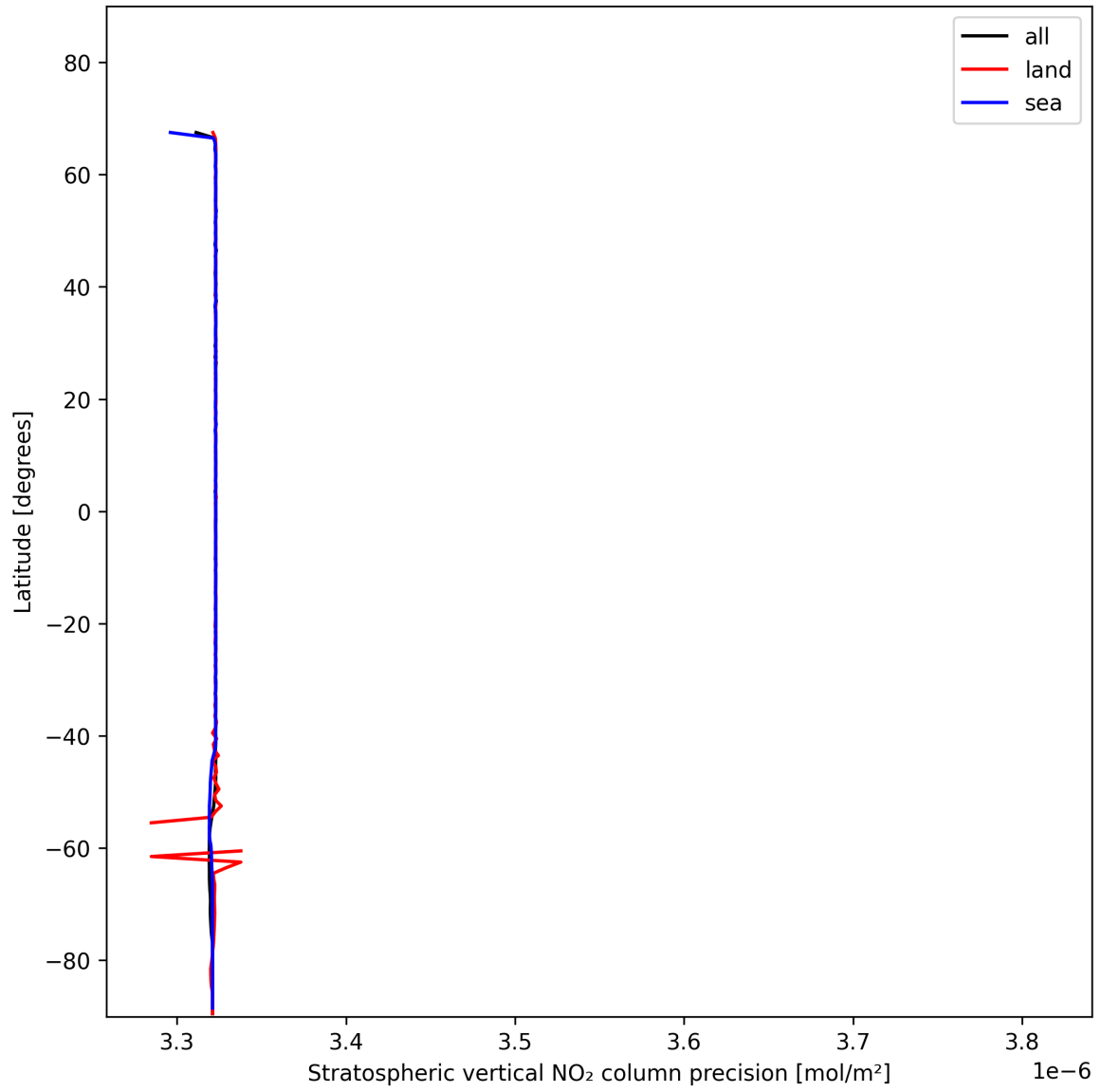
Figure 18: Zonal average of “Stratospheric vertical NO 2 column precision” for 2025-01-16 to 2025-01-17.
