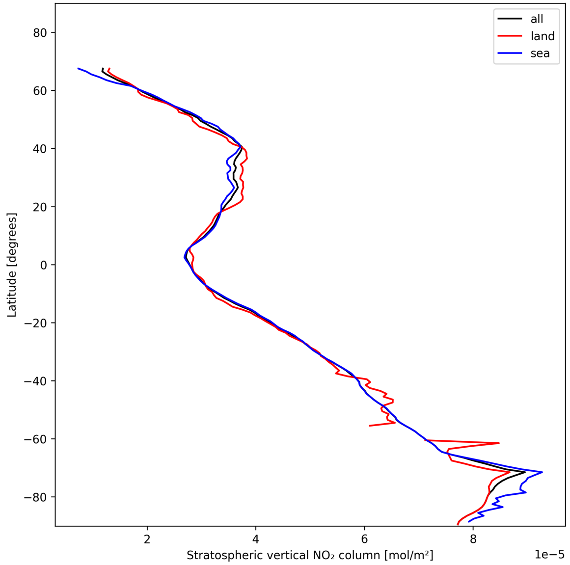
Figure 17: Zonal average of “Stratospheric vertical NO 2 column” for 2025-01-16 to 2025-01-17.
