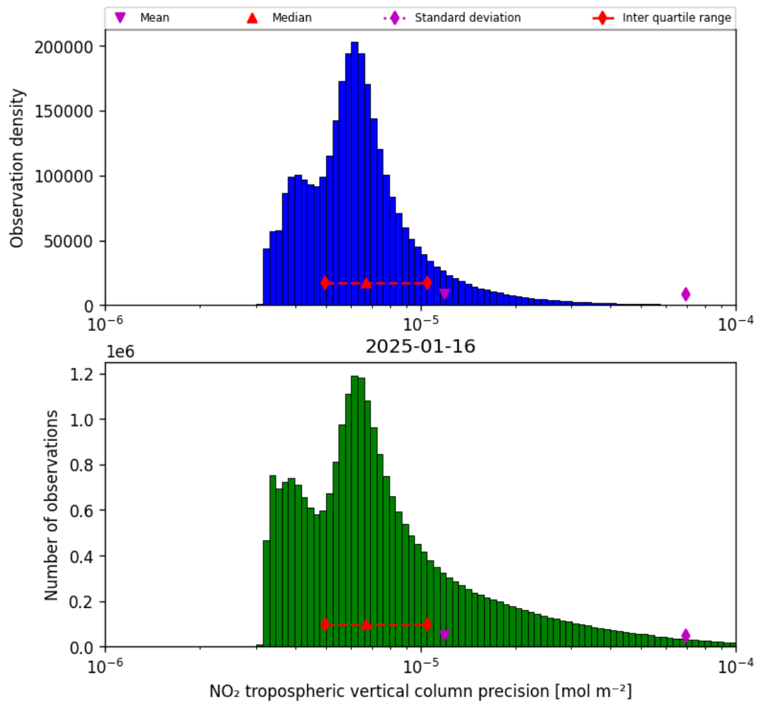
Figure 28: Histogram of “NO 2 tropospheric vertical column precision” for 2025-01-16 to 2025-01-17
