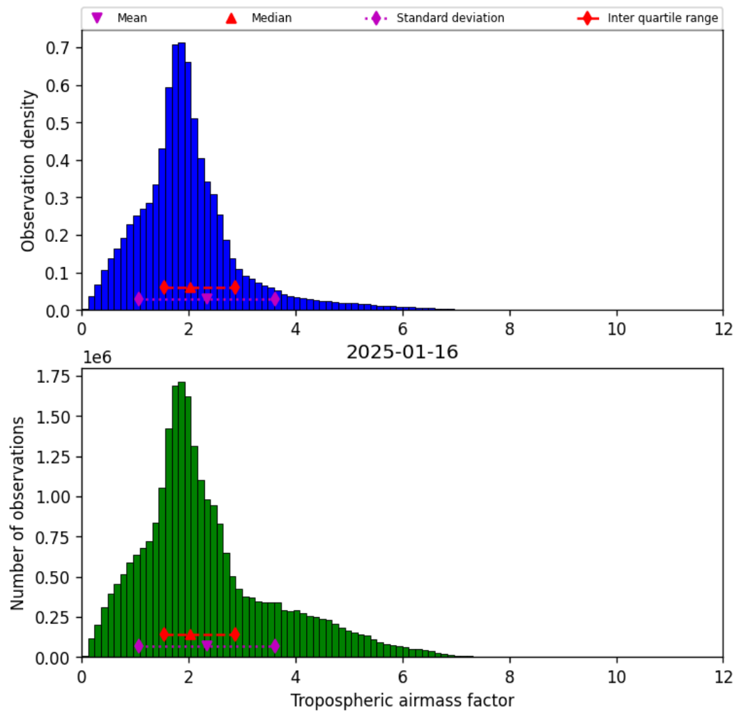
Figure 29: Histogram of “Tropospheric airmass factor” for 2025-01-16 to 2025-01-17
