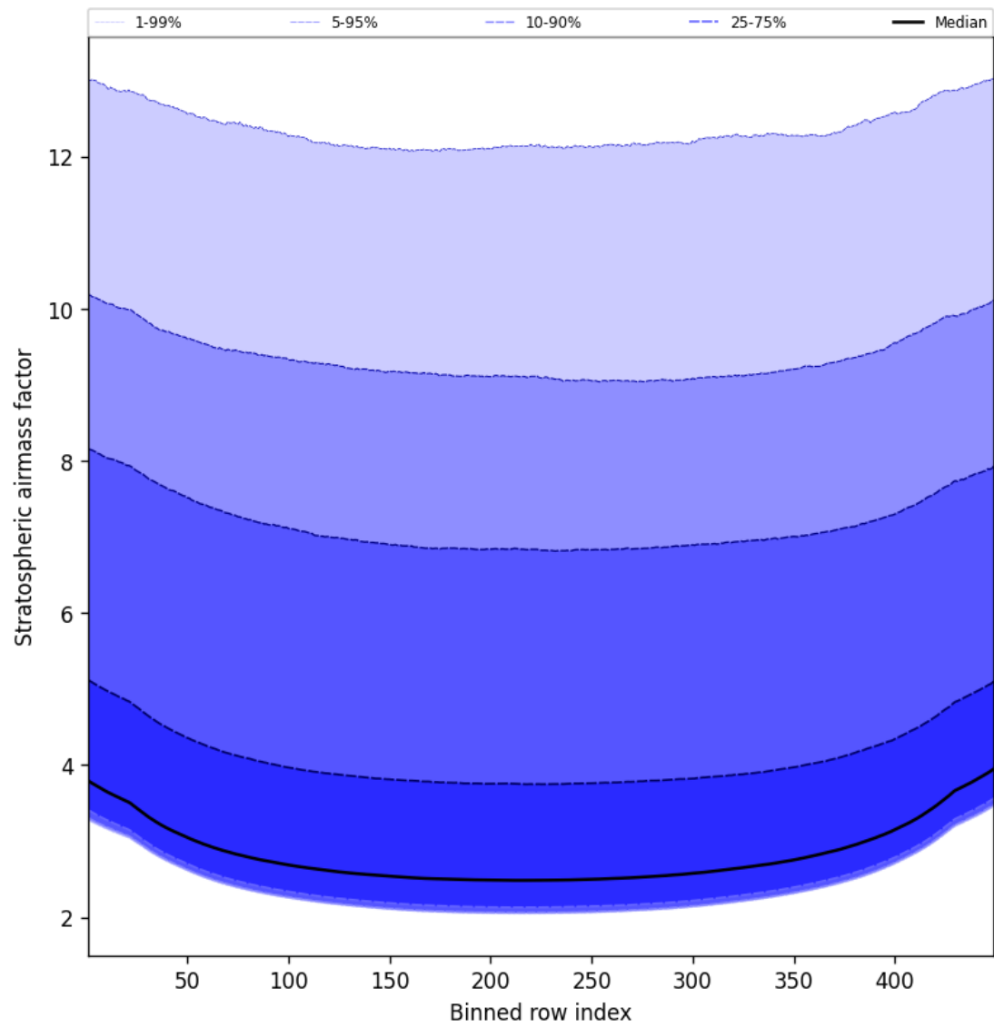
Figure 59: Along track statistics of “Stratospheric airmass factor” for 2025-01-16 to 2025-01-17
