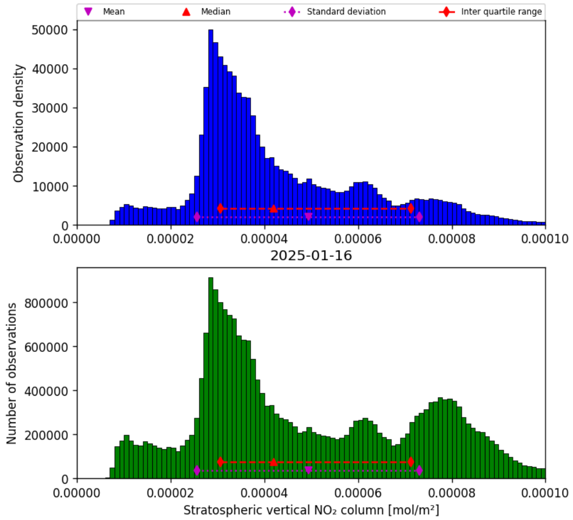
Figure 34: Histogram of “Stratospheric vertical NO 2 column” for 2025-01-16 to 2025-01-17
