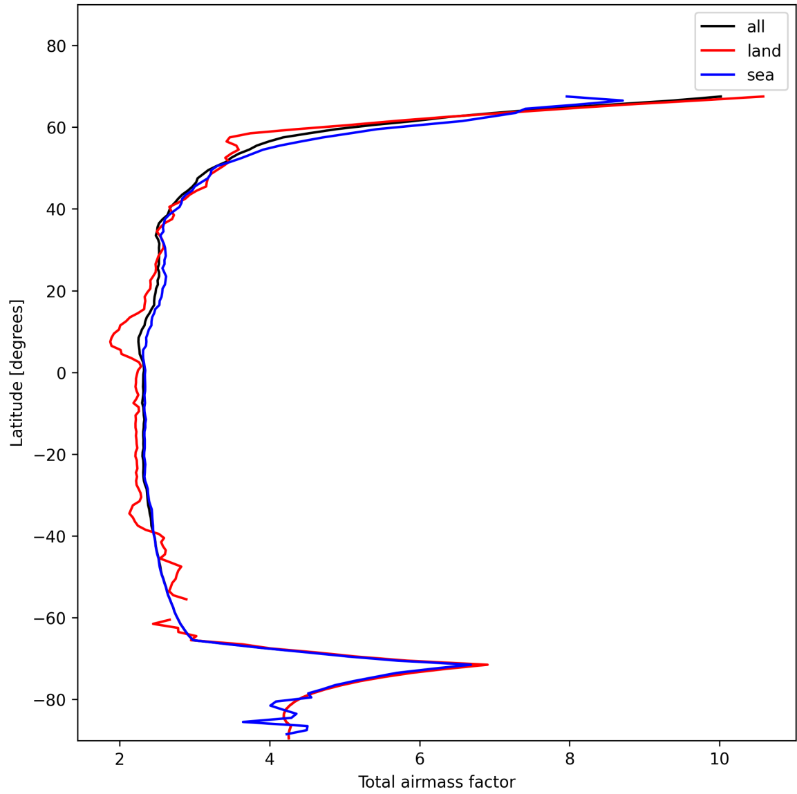
Figure 13: Zonal average of “Total airmass factor” for 2025-01-16 to 2025-01-17.
