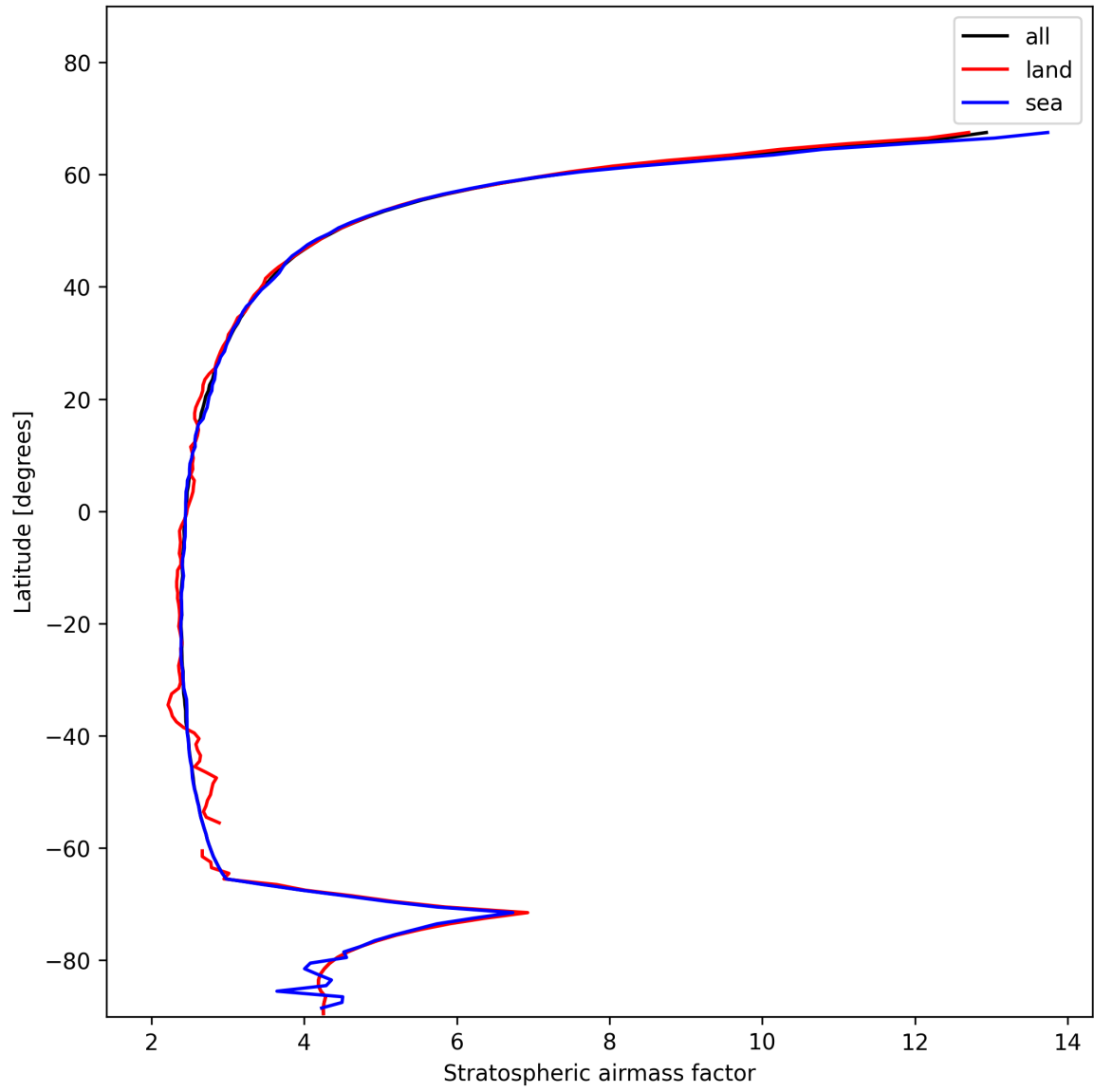
Figure 25: Zonal average of “Stratospheric air mass factor” for 2025-01-16 to 2025-01-17.
