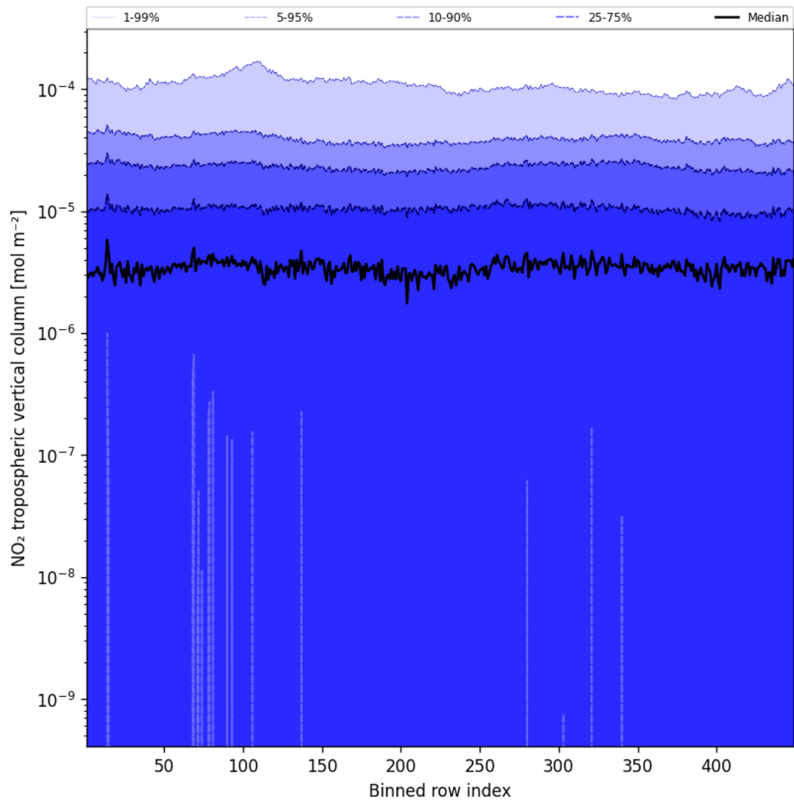
Figure 44: Along track statistics of “NO 2 tropospheric vertical column” for 2025-01-16 to 2025-01-17
