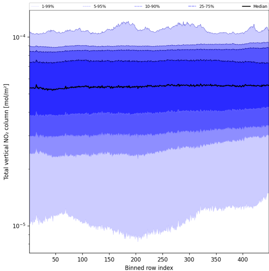
Figure 53: Along track statistics of “Total vertical NO 2 column” for 2025-01-16 to 2025-01-17
