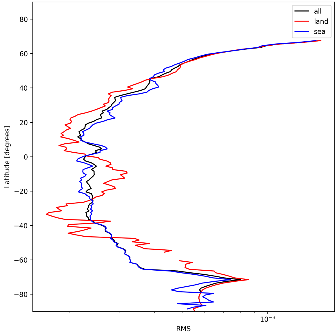
Figure 24: Zonal average of “RMS” for 2025-01-16 to 2025-01-17.
