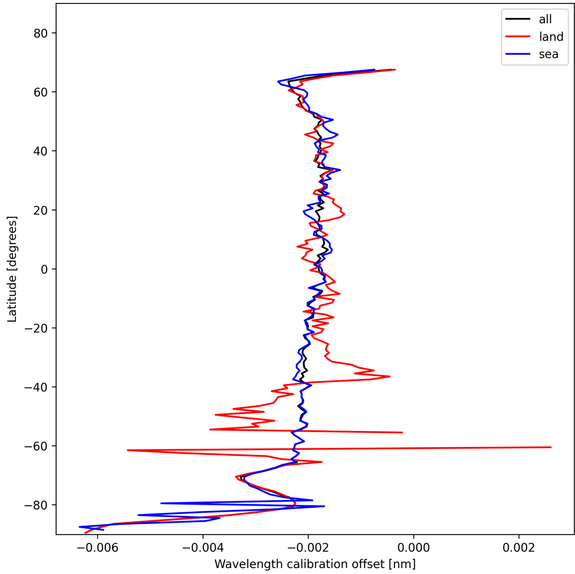
Figure 16: Zonal average of “Wavelength calibration offset” for 2025-01-16 to 2025-01-17.
