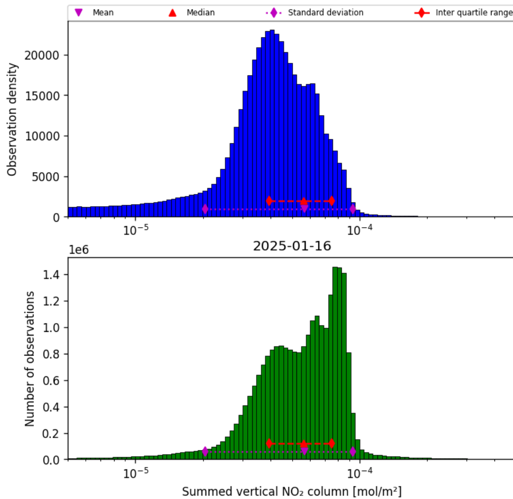
Figure 38: Histogram of “Summed vertical NO 2 column” for 2025-01-16 to 2025-01-17
