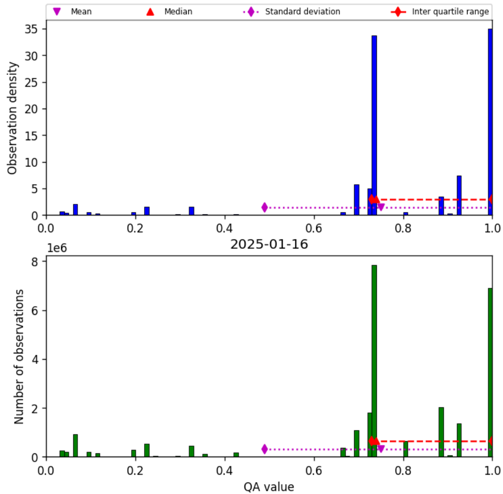
Figure 26: Histogram of “QA value” for 2025-01-16 to 2025-01-17
