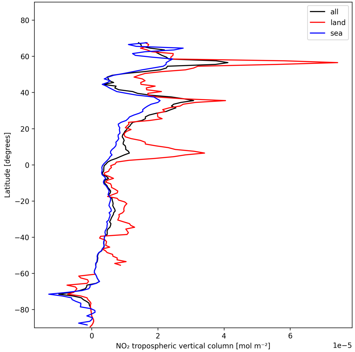
Figure 10: Zonal average of “NO 2 tropospheric vertical column” for 2025-01-16 to 2025-01-17.
