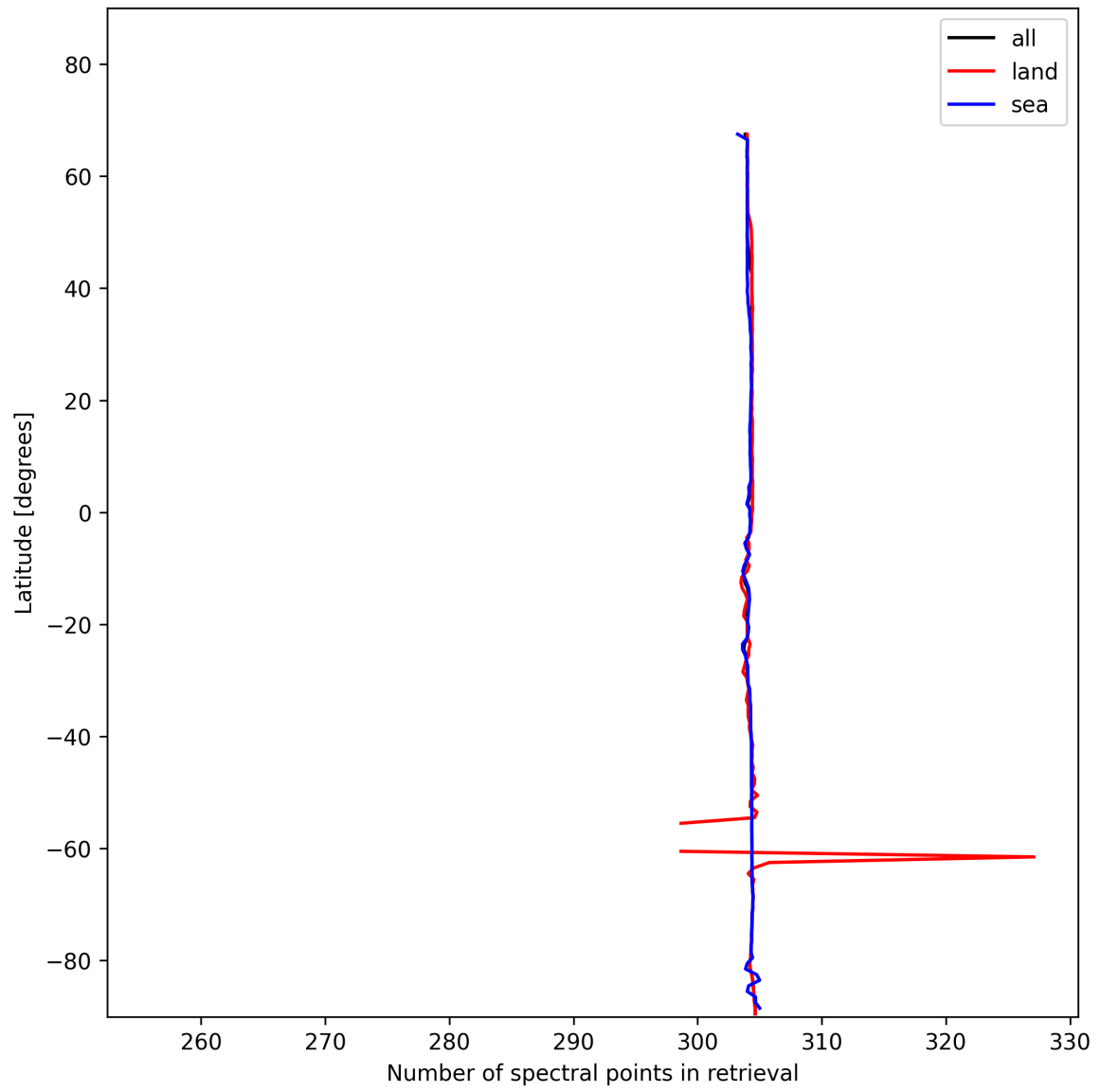
Figure 14: Zonal average of “Number of spectral points in retrieval” for 2025-01-16 to 2025-01-17.
