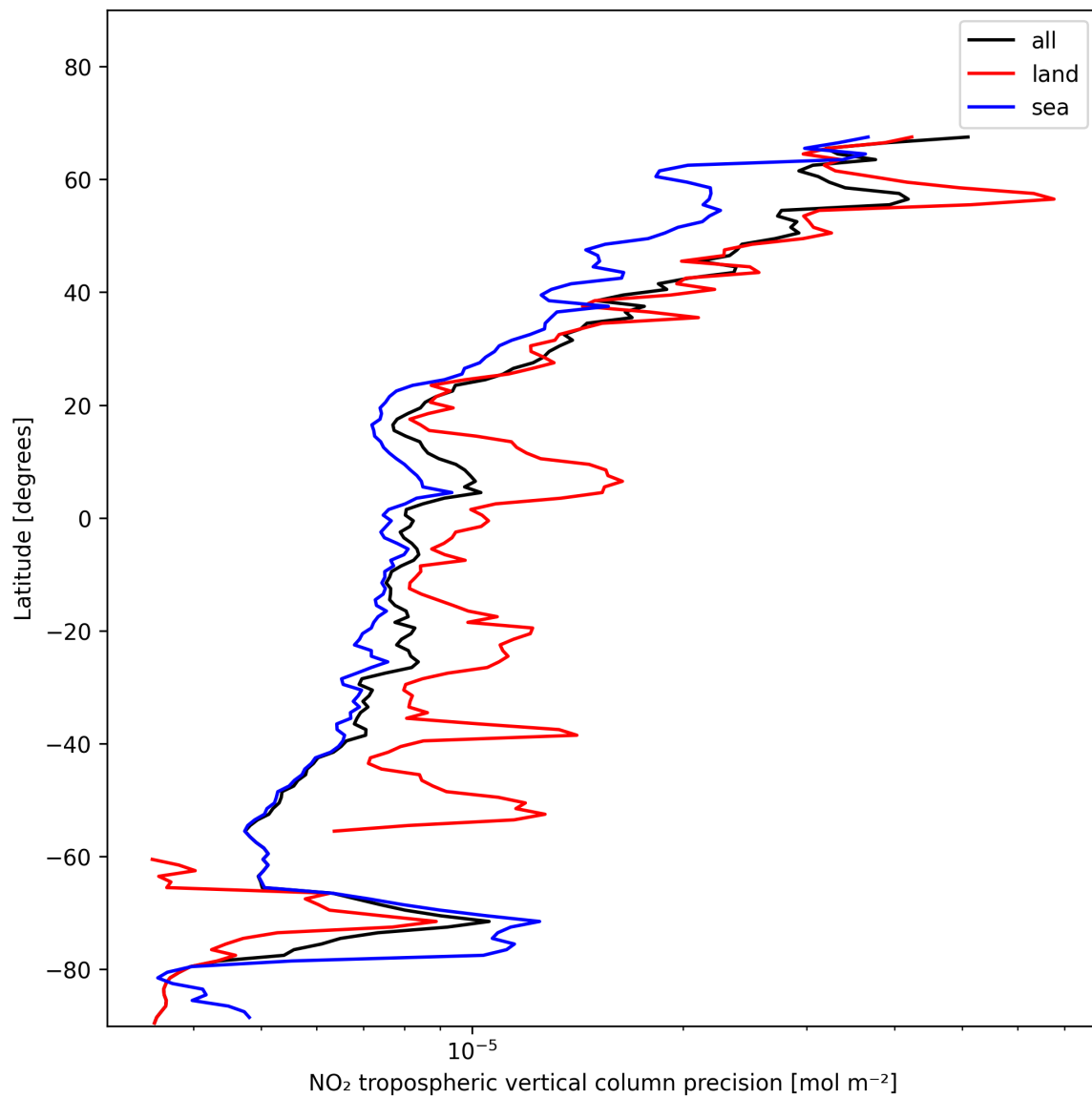
Figure 11: Zonal average of “NO 2 tropospheric vertical column precision” for 2025-01-16 to 2025-01-17.
