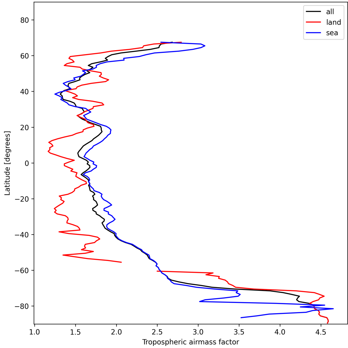
Figure 12: Zonal average of “Tropospheric airmass factor” for 2025-01-17 to 2025-01-18.
