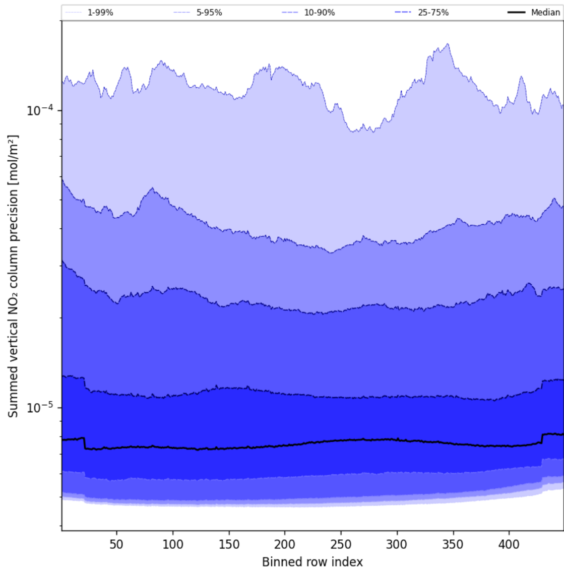
Figure 56: Along track statistics of “Summed vertical NO 2 column precision” for 2025-01-17 to 2025-01-18
