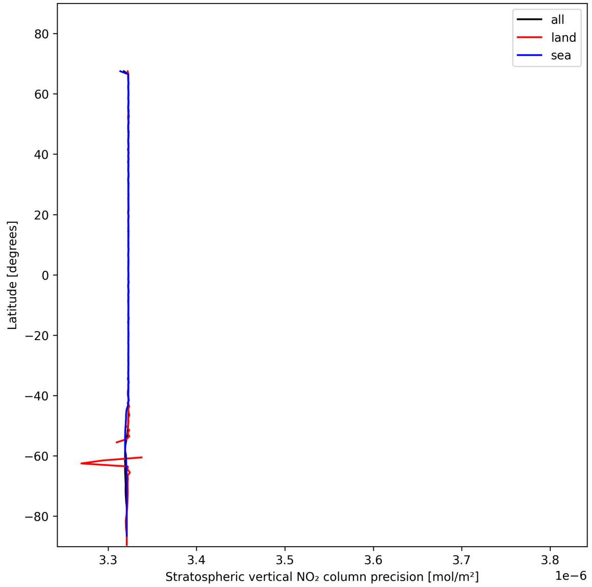
Figure 18: Zonal average of “Stratospheric vertical NO 2 column precision” for 2025-01-17 to 2025-01-18.
