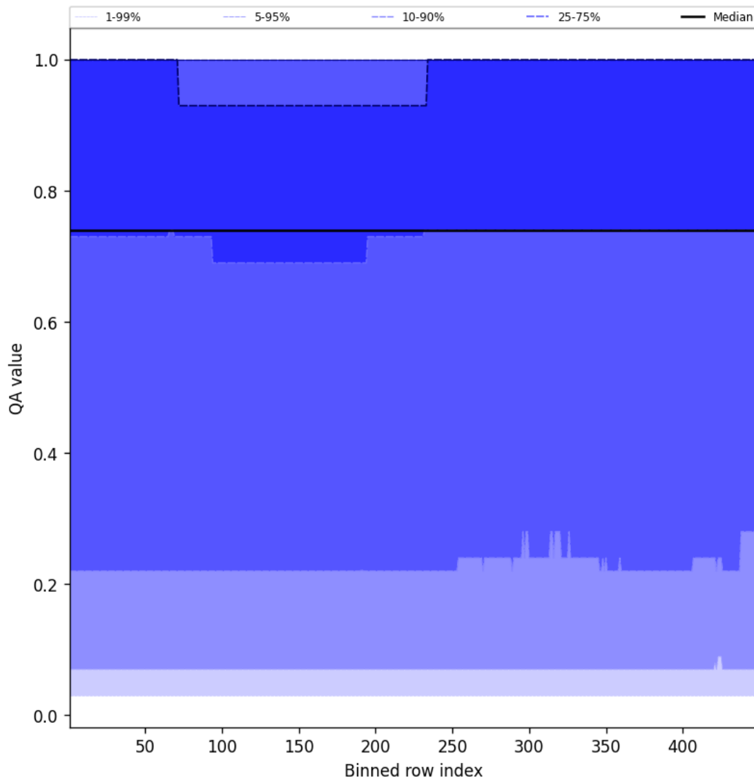
Figure 43: Along track statistics of “QA value” for 2025-01-17 to 2025-01-18
