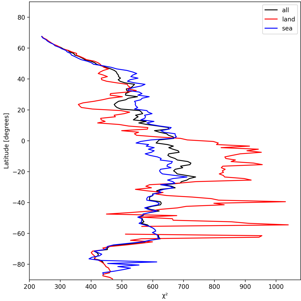
Figure 23: Zonal average of “ \chi^2 ” for 2025-01-17 to 2025-01-18.
