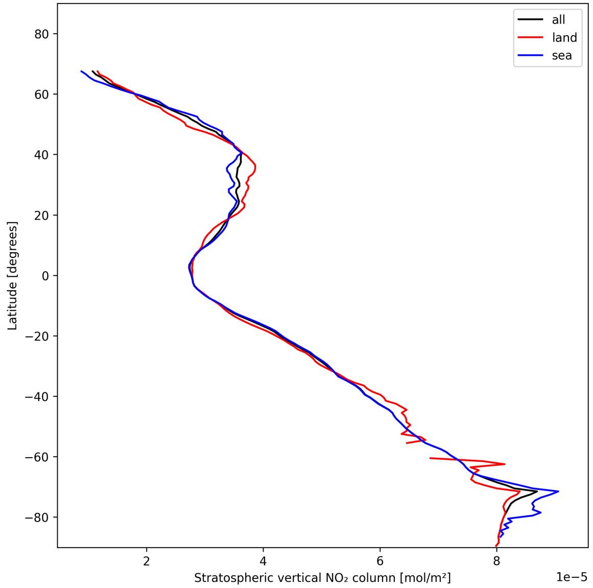
Figure 17: Zonal average of “Stratospheric vertical NO 2 column” for 2025-01-17 to 2025-01-18.
