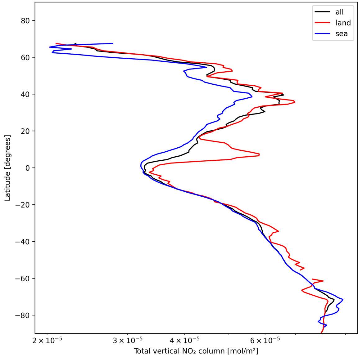
Figure 19: Zonal average of “Total vertical NO 2 column” for 2025-01-17 to 2025-01-18.
