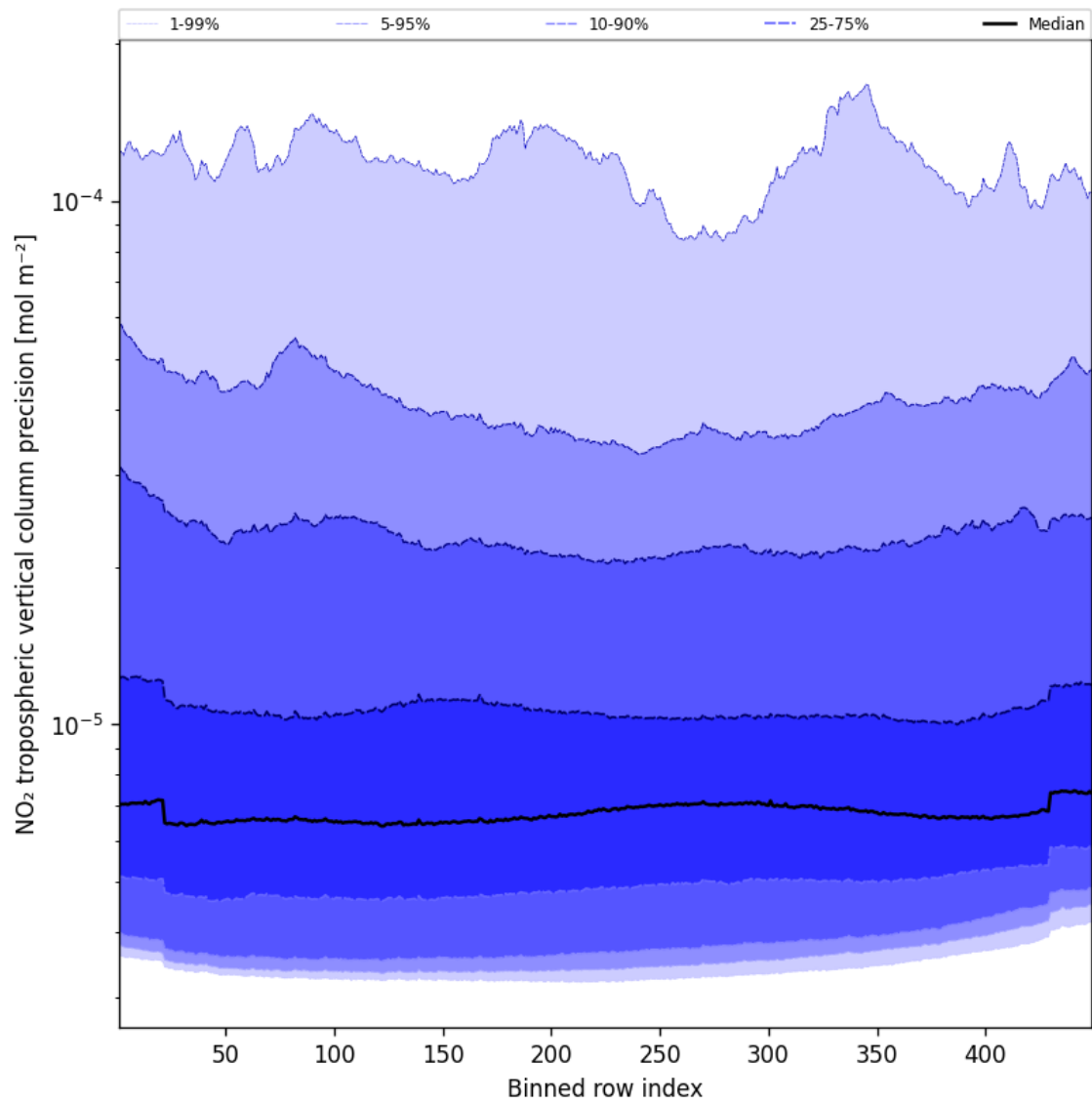
Figure 45: Along track statistics of “NO 2 tropospheric vertical column precision” for 2025-01-17 to 2025-01-18
