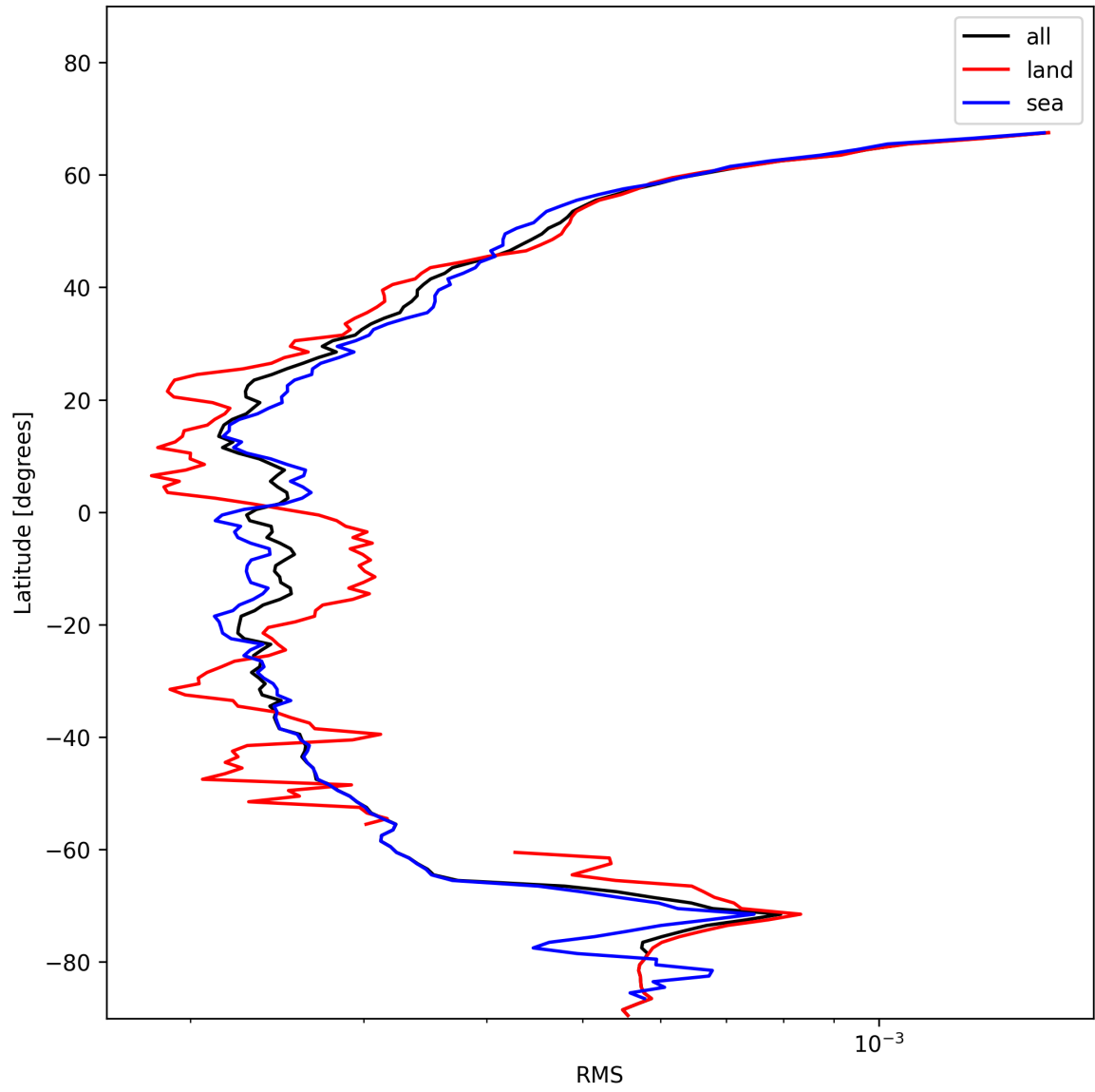
Figure 24: Zonal average of “RMS” for 2025-01-17 to 2025-01-18.
