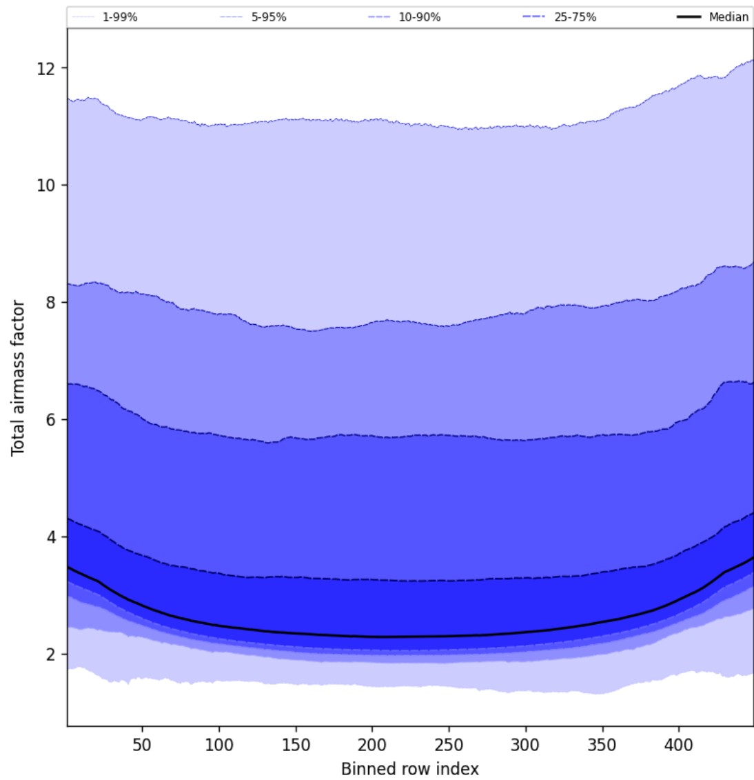
Figure 47: Along track statistics of “Total airmass factor” for 2025-01-17 to 2025-01-18
