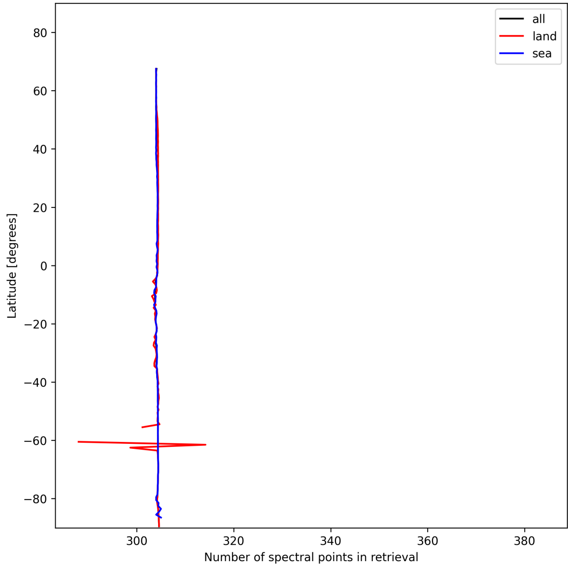
Figure 14: Zonal average of “Number of spectral points in retrieval” for 2025-01-17 to 2025-01-18.
