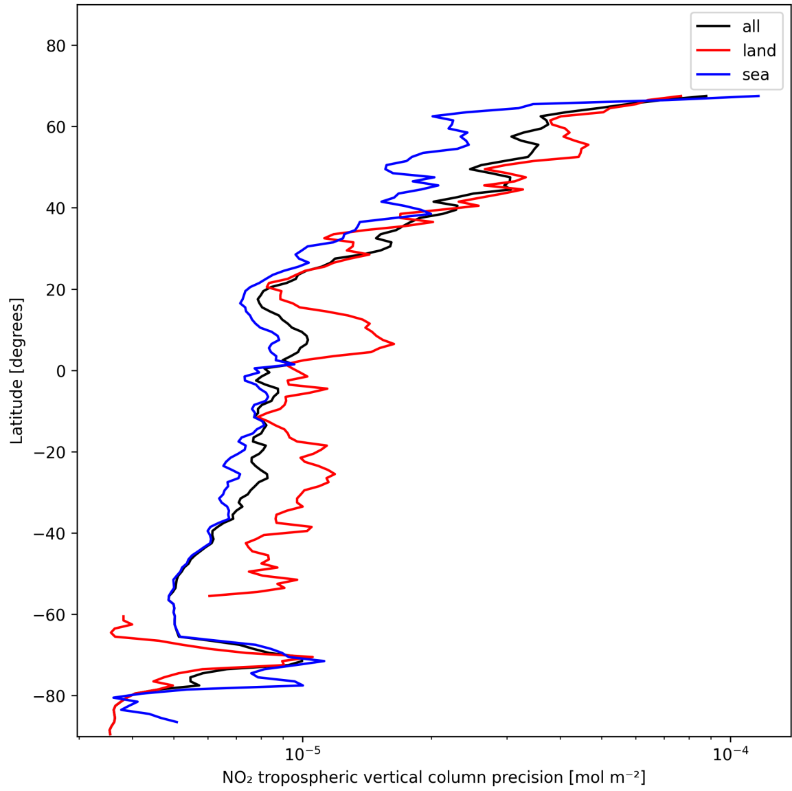
Figure 11: Zonal average of “NO 2 tropospheric vertical column precision” for 2025-01-17 to 2025-01-18.
