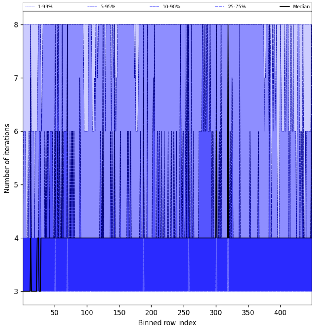
Figure 49: Along track statistics of “Number of iterations” for 2025-01-17 to 2025-01-18
