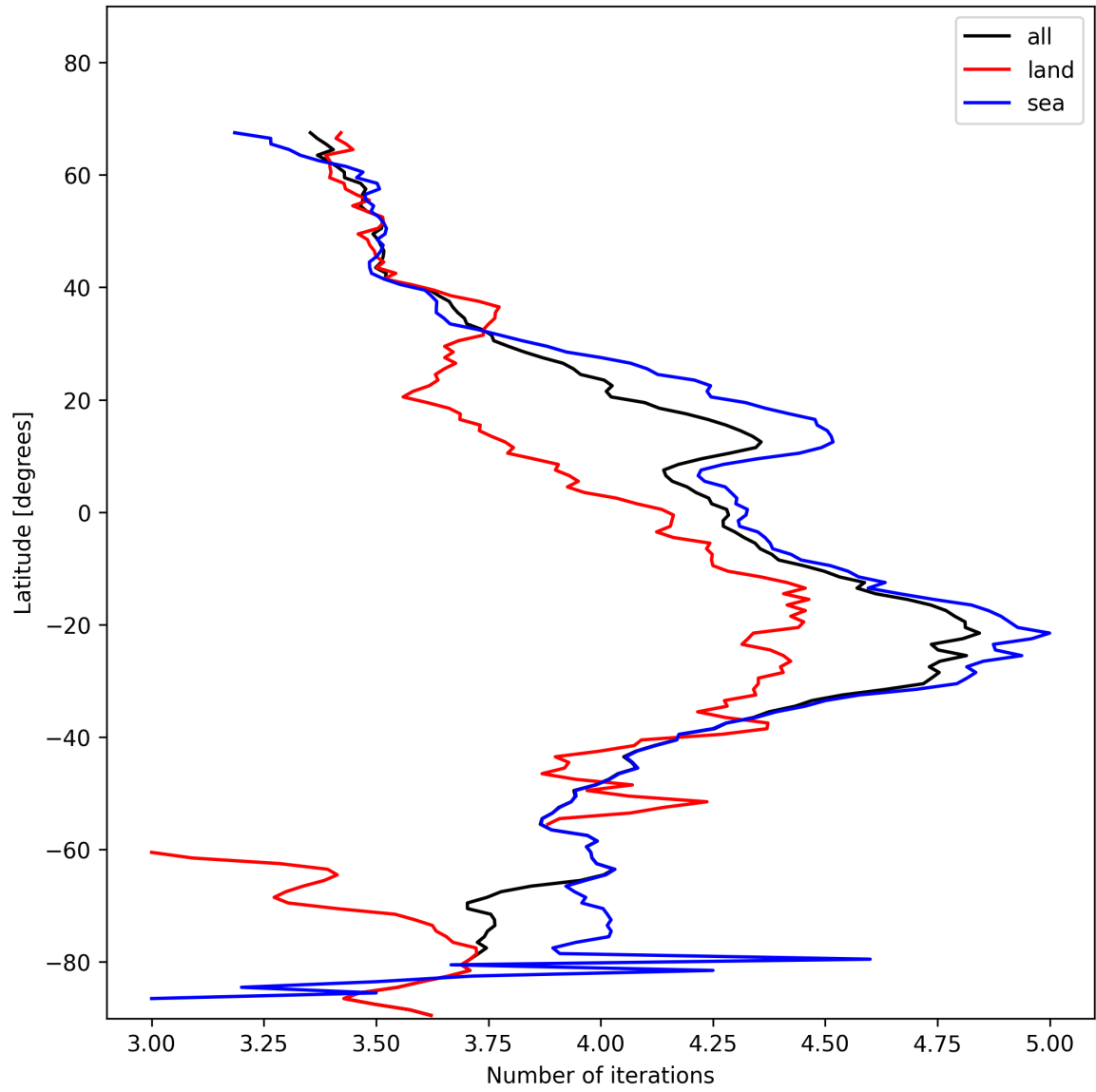
Figure 15: Zonal average of “Number of iterations” for 2025-01-17 to 2025-01-18.
