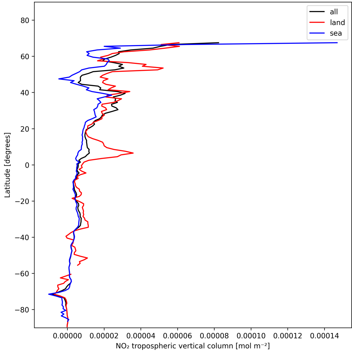
Figure 10: Zonal average of “NO 2 tropospheric vertical column” for 2025-01-17 to 2025-01-18.
