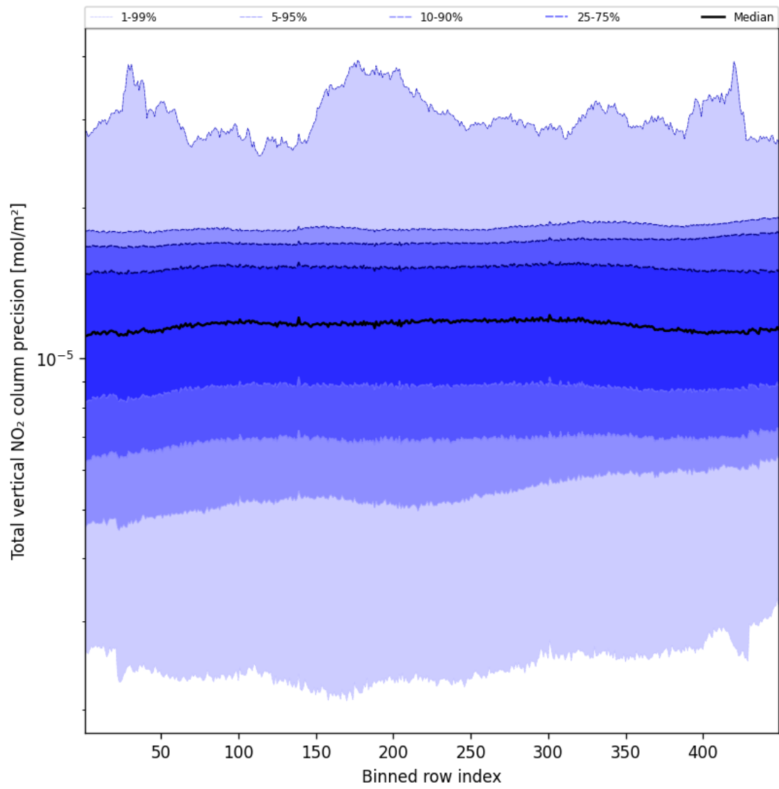
Figure 54: Along track statistics of “Total vertical NO 2 column precision” for 2025-01-17 to 2025-01-18
