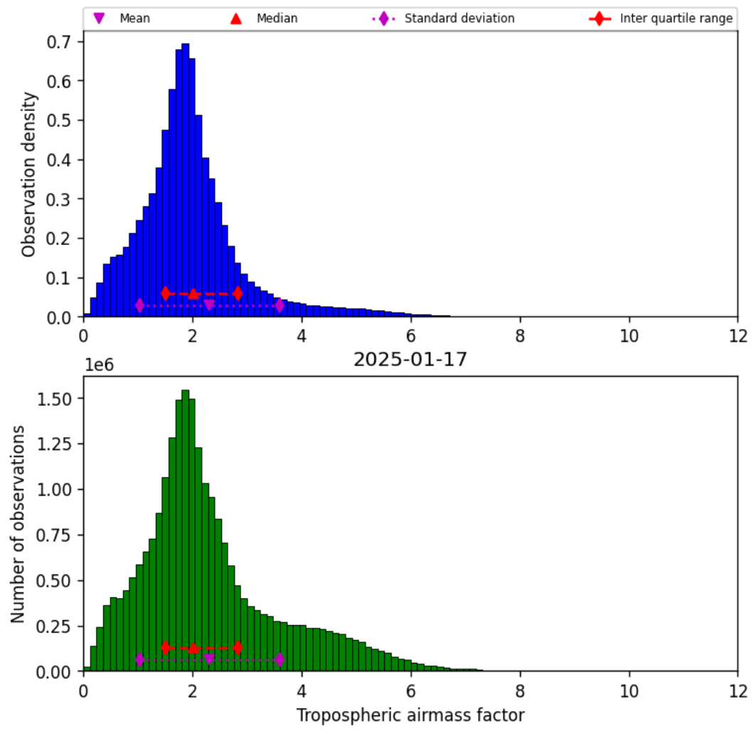
Figure 29: Histogram of “Tropospheric airmass factor” for 2025-01-17 to 2025-01-18
