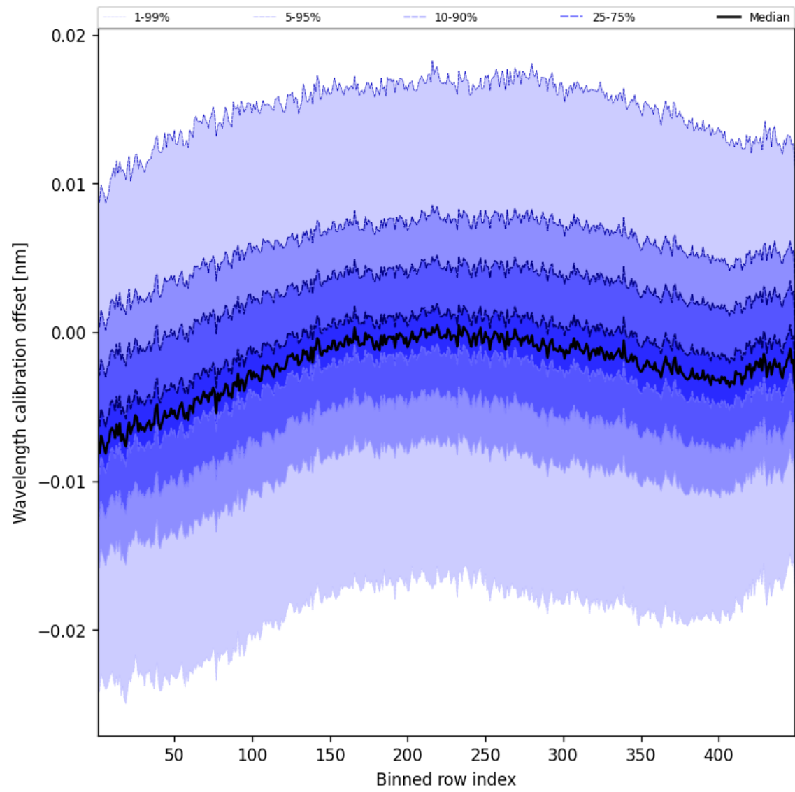
Figure 50: Along track statistics of “Wavelength calibration offset” for 2025-01-17 to 2025-01-18
