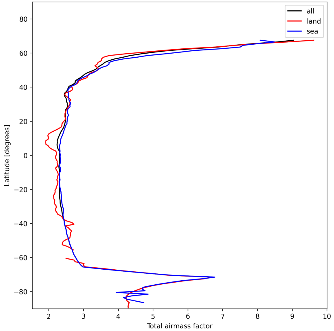
Figure 13: Zonal average of “Total airmass factor” for 2025-01-17 to 2025-01-18.
