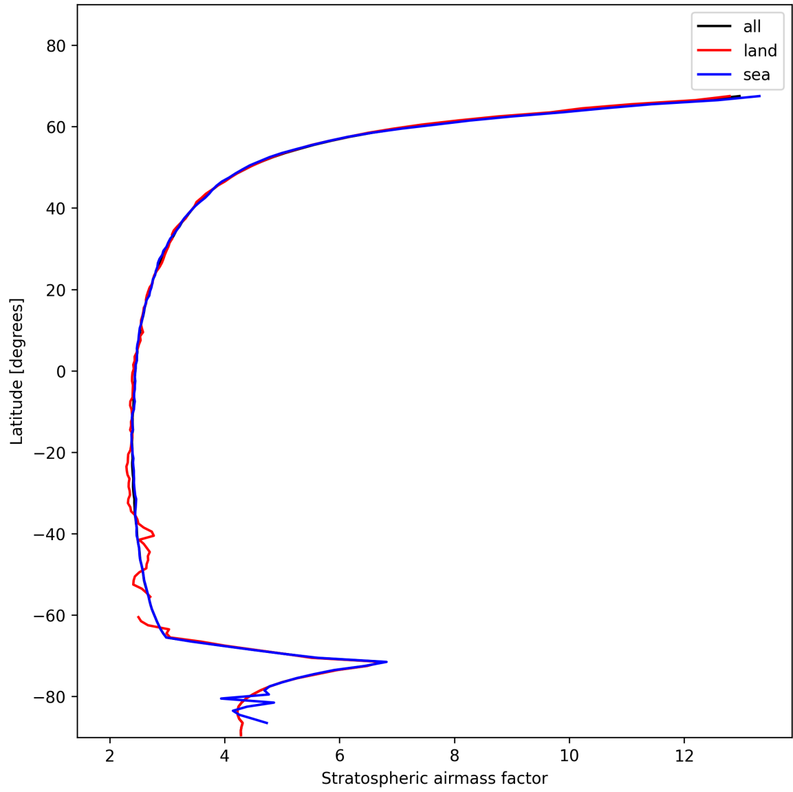
Figure 25: Zonal average of “Stratospheric airmass factor” for 2025-01-17 to 2025-01-18.
