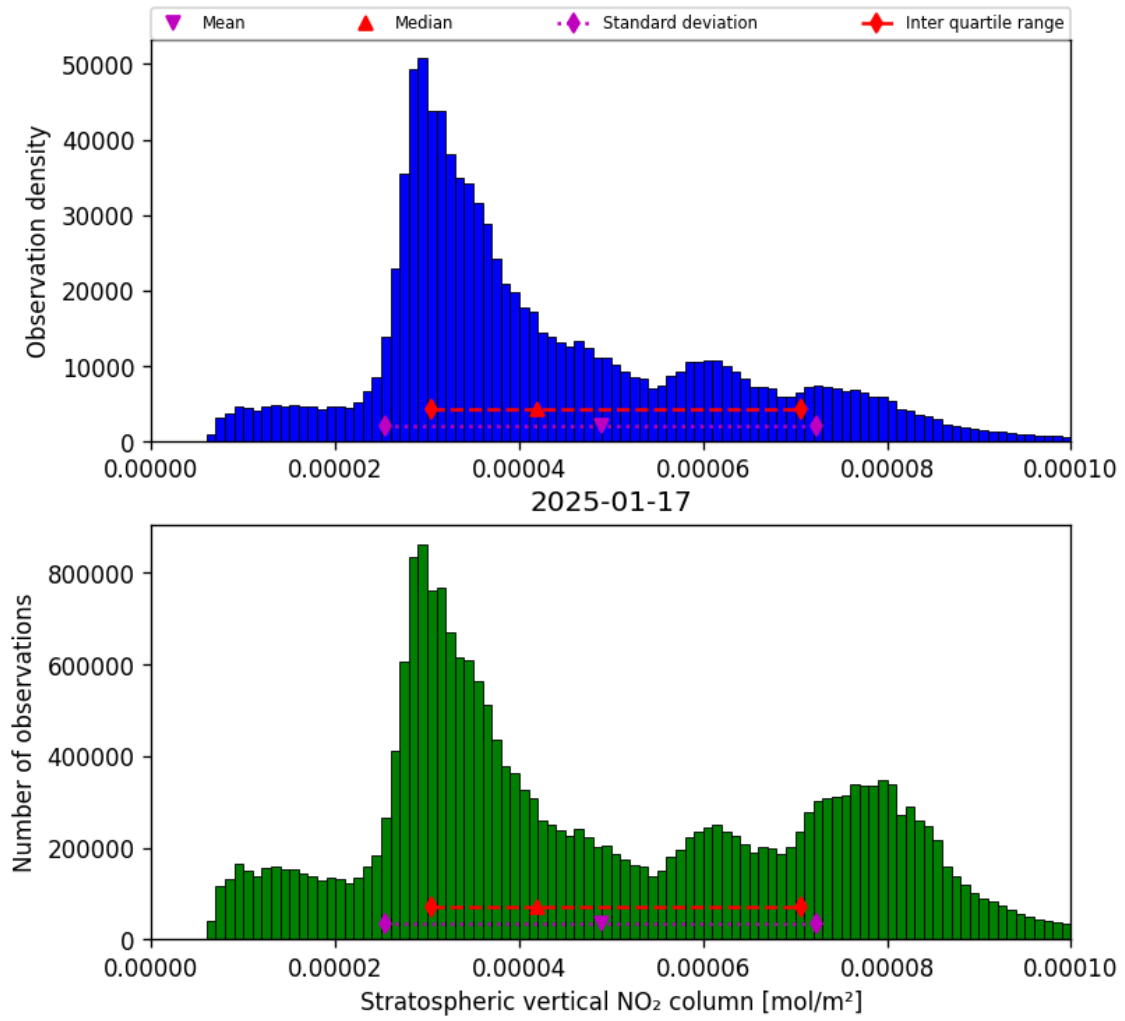
Figure 34: Histogram of “Stratospheric vertical NO 2 column” for 2025-01-17 to 2025-01-18
