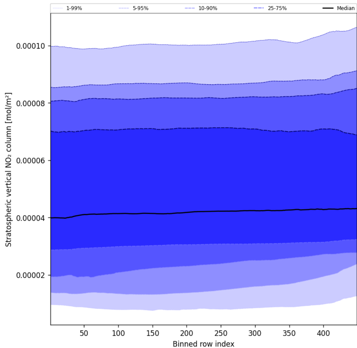
Figure 51: Along track statistics of “Stratospheric vertical NO 2 column” for 2025-01-17 to 2025-01-18
