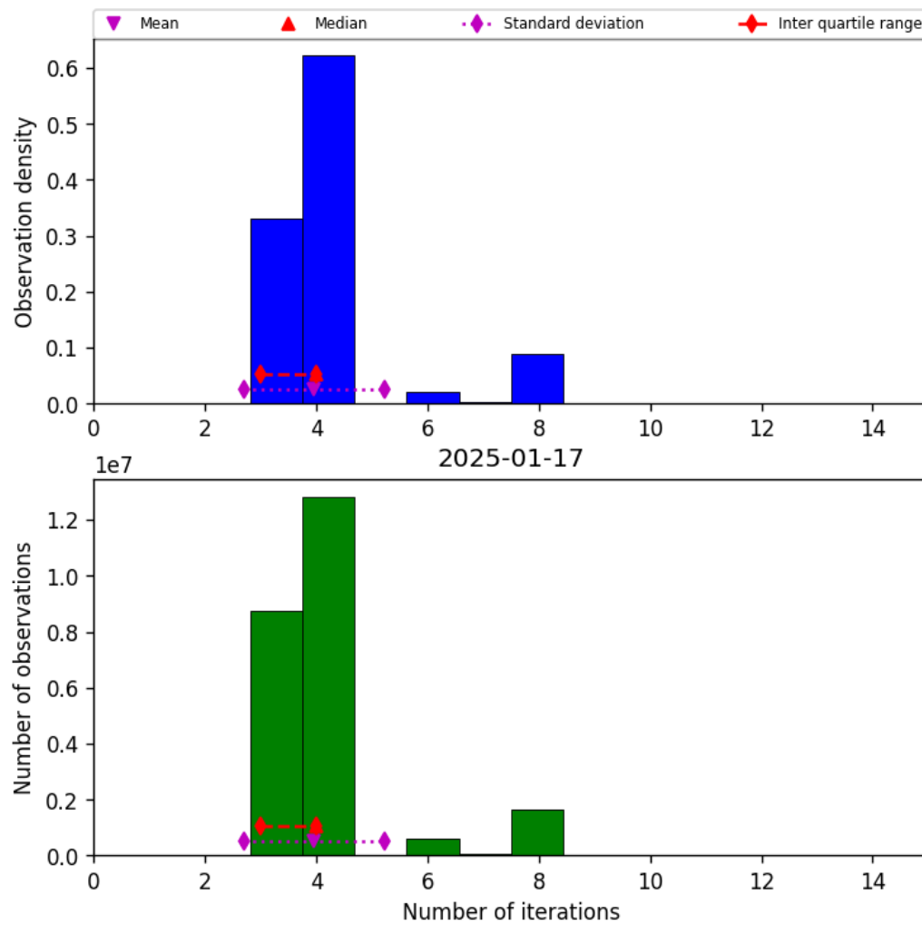
Figure 32: Histogram of “Number of iterations” for 2025-01-17 to 2025-01-18
