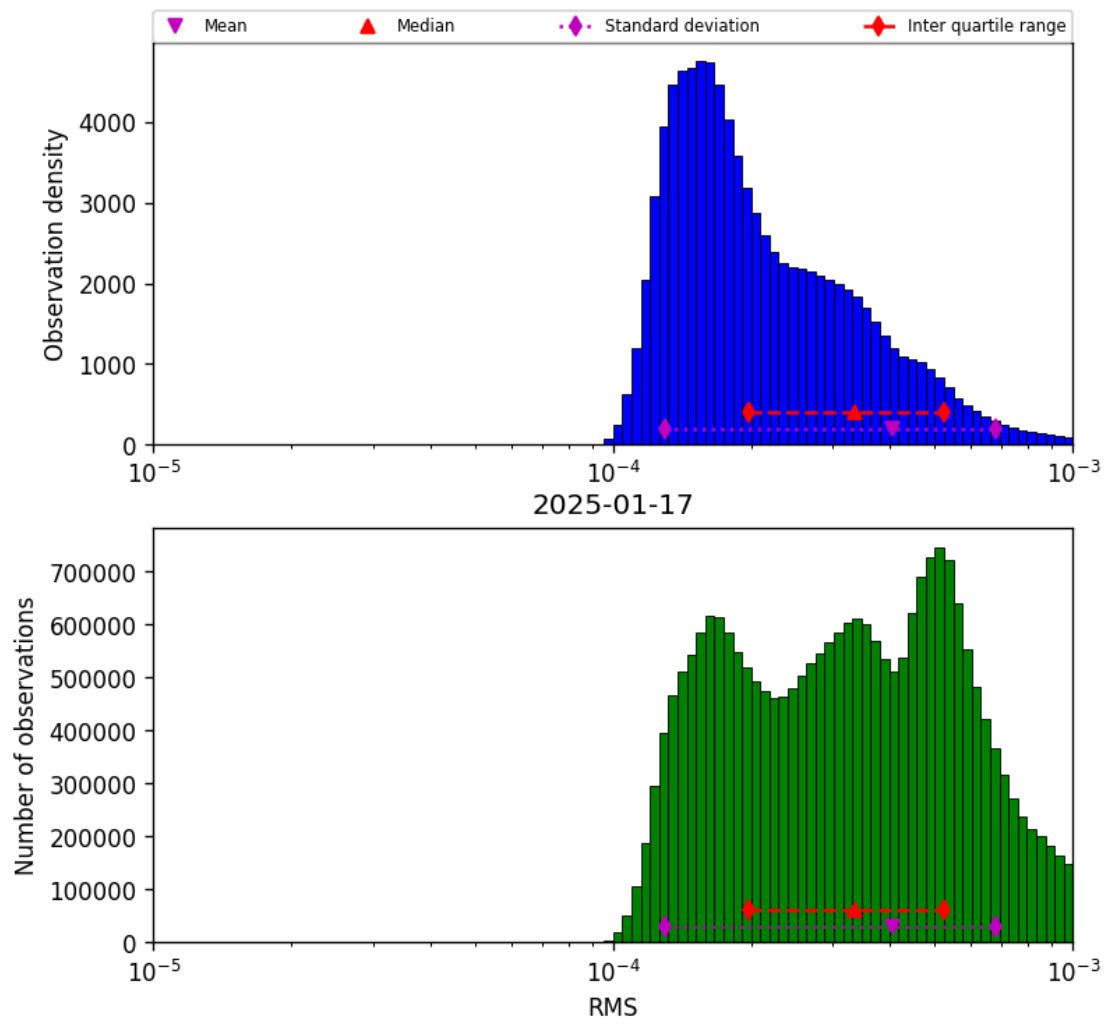
Figure 41: Histogram of “RMS” for 2025-01-17 to 2025-01-18
