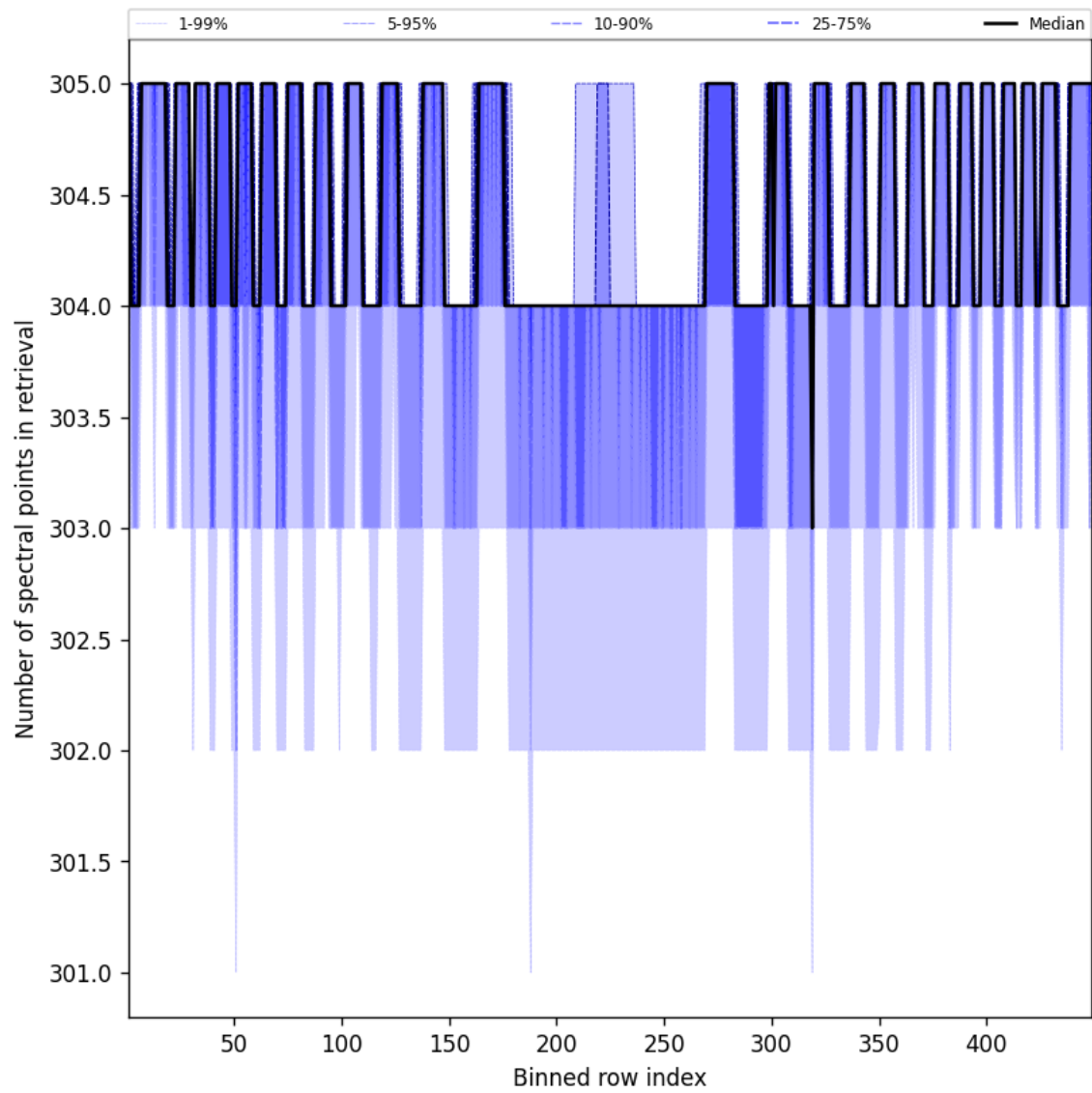
Figure 48: Along track statistics of “Number of spectral points in retrieval” for 2025-01-17 to 2025-01-18
