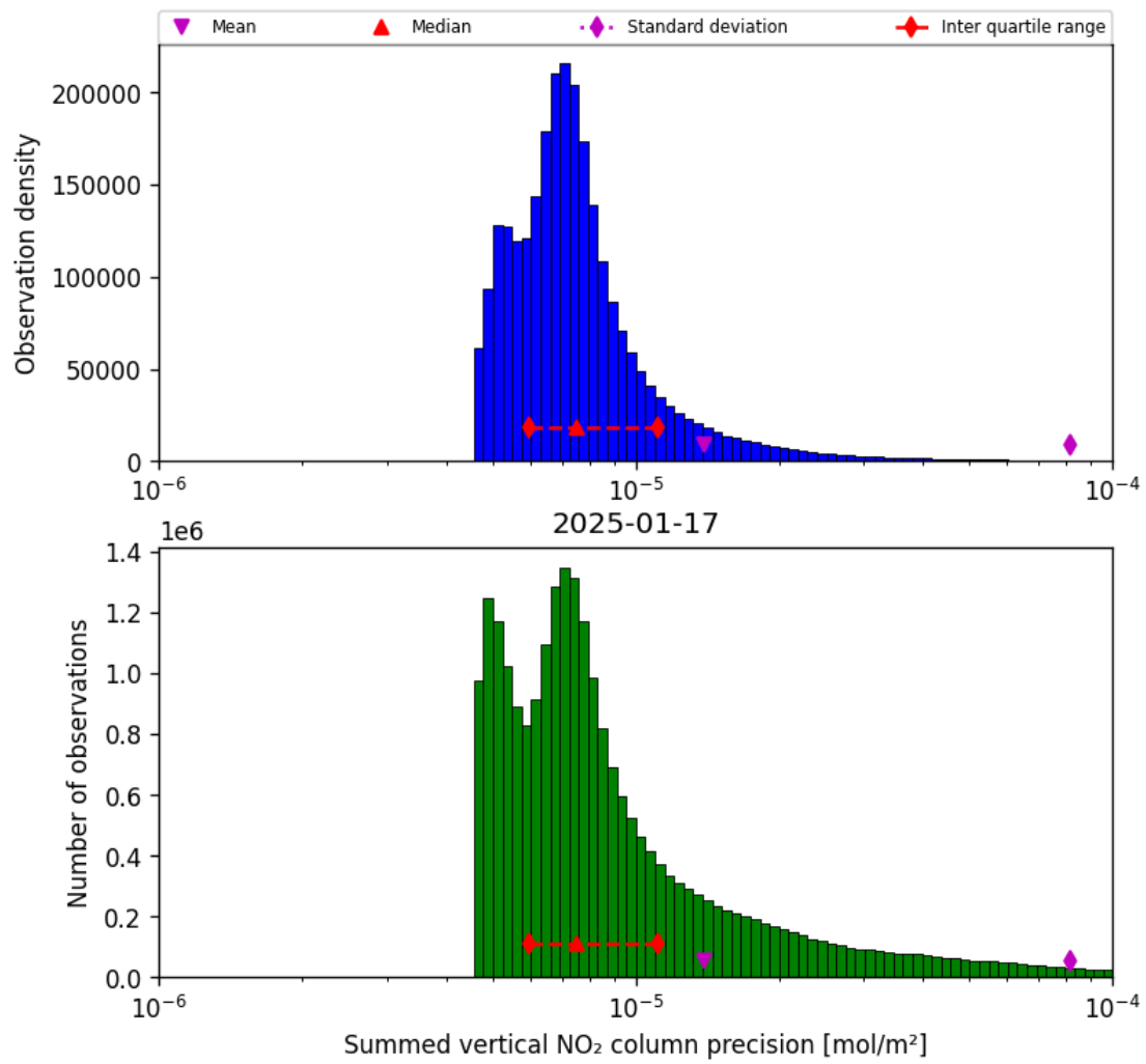
Figure 39: Histogram of "Summed vertical NO 2 column precision" for 2025-01-17 to 2025-01-18
