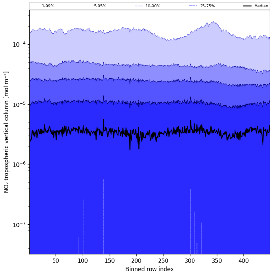
Figure 44: Along track statistics of “NO 2 tropospheric vertical column” for 2025-01-17 to 2025-01-18
