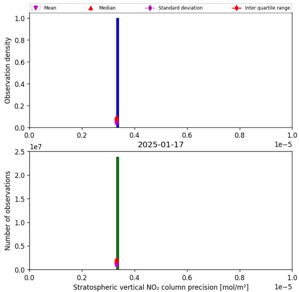
Figure 35: Histogram of “Stratospheric vertical NO 2 column precision” for 2025-01-17 to 2025-01-18
