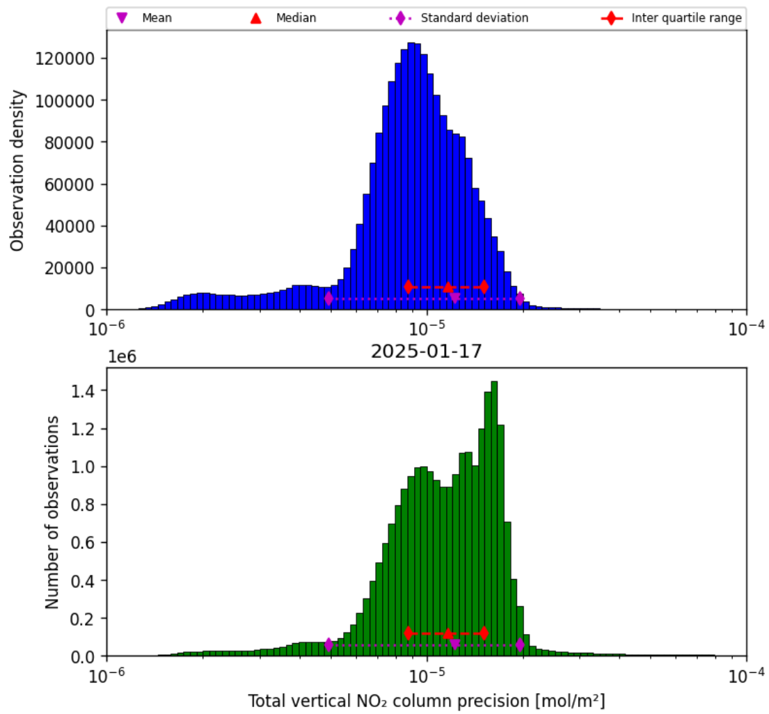
Figure 37: Histogram of “Total vertical NO 2 column precision” for 2025-01-17 to 2025-01-18
