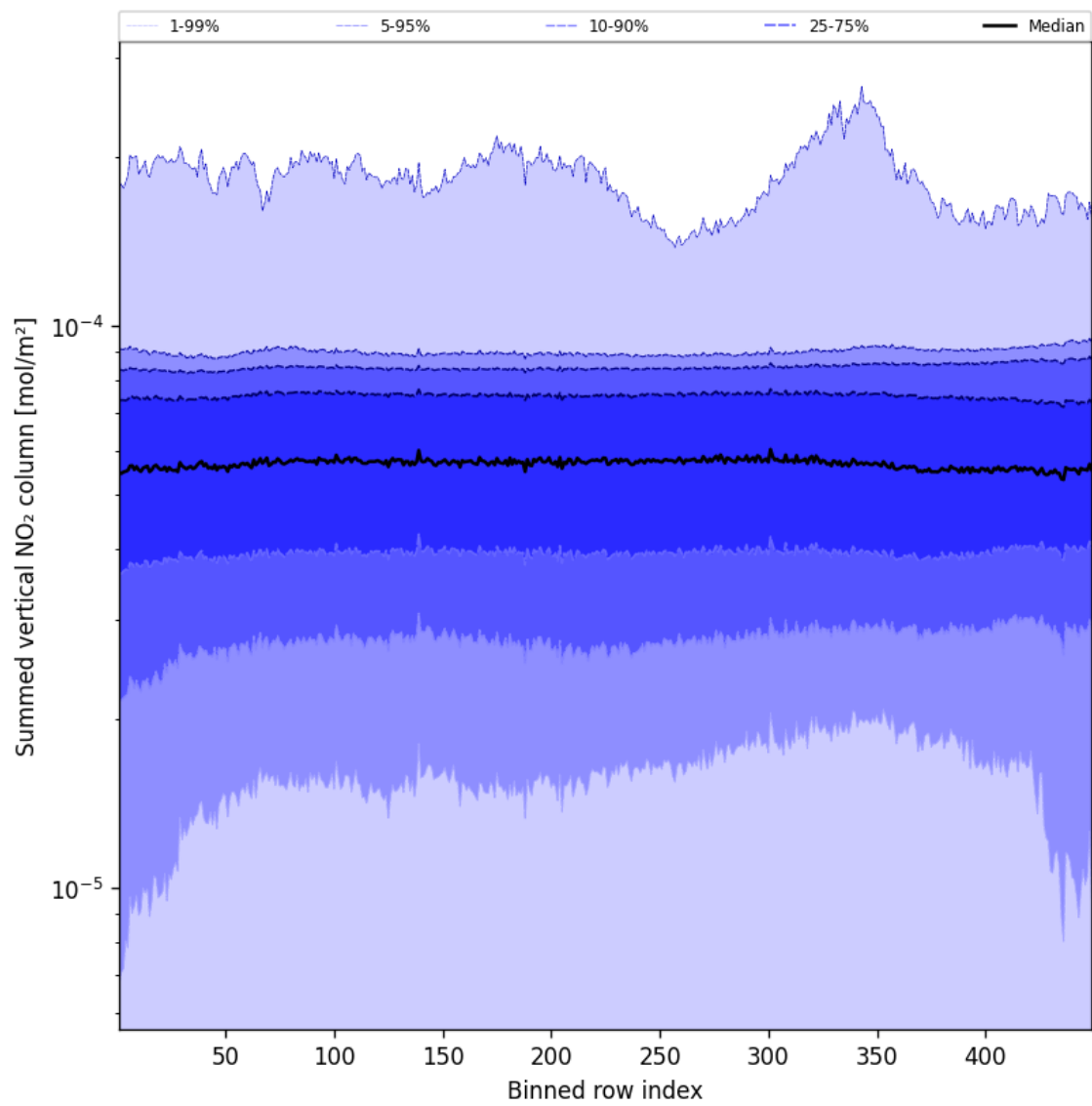
Figure 55: Along track statistics of “Summed vertical NO 2 column” for 2025-01-17 to 2025-01-18
