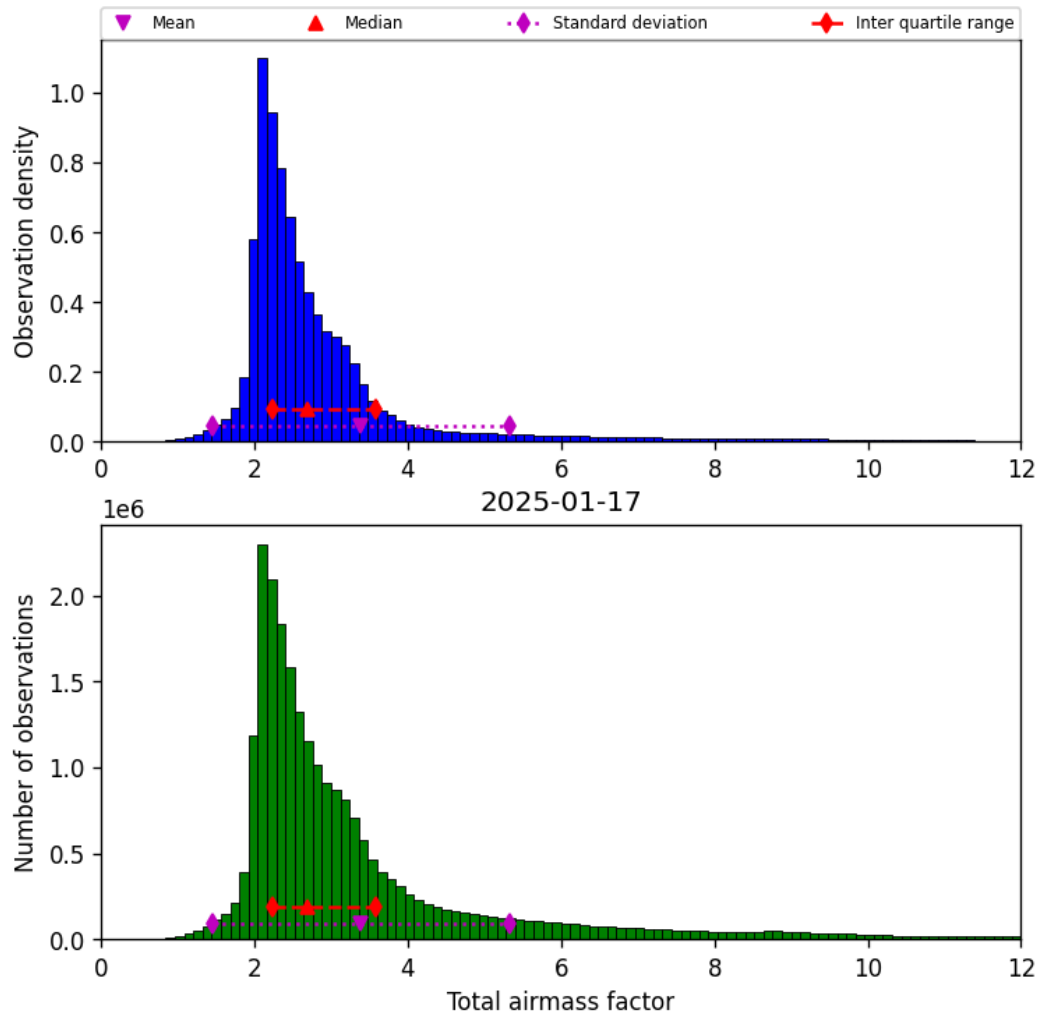
Figure 30: Histogram of “Total airmass factor” for 2025-01-17 to 2025-01-18
