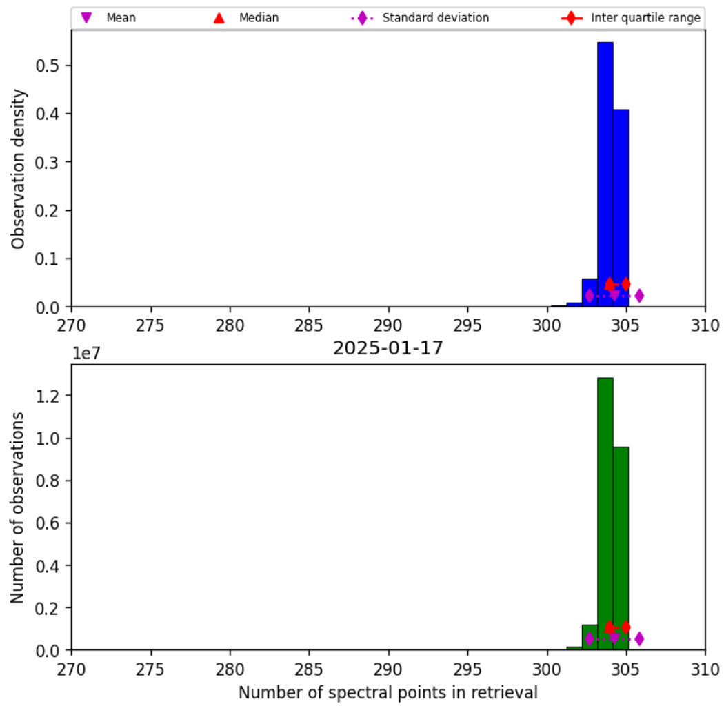
Figure 31: Histogram of “Number of spectral points in retrieval” for 2025-01-17 to 2025-01-18
