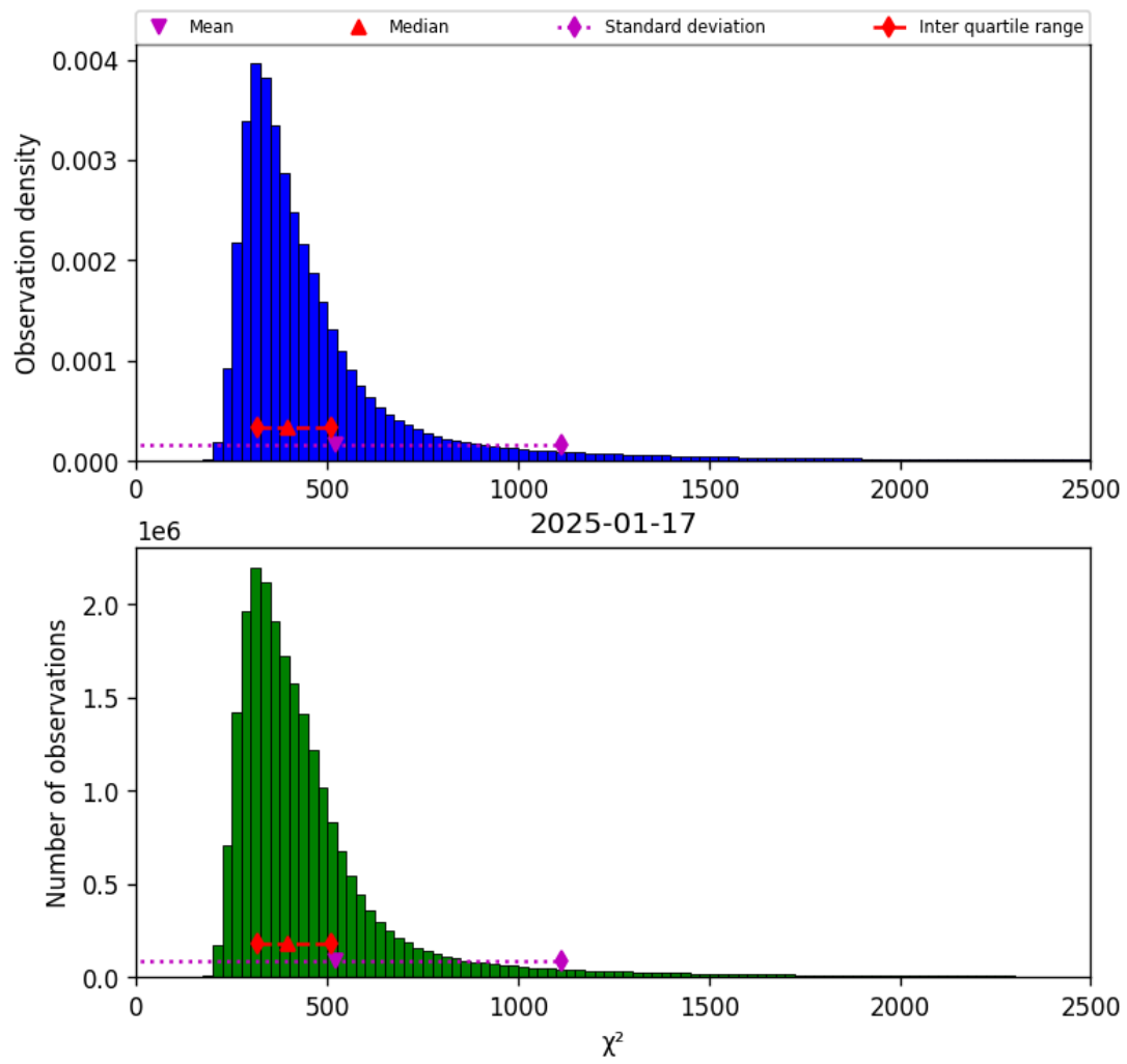
Figure 40: Histogram of “ \chi^2 ” for 2025-01-17 to 2025-01-18
