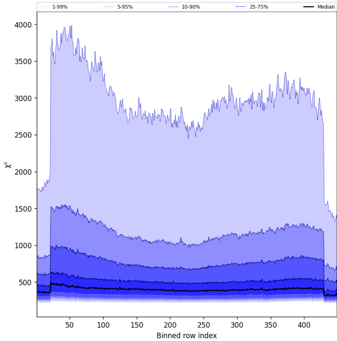
Figure 57: Along track statistics of “ \chi^2 ” for 2025-01-17 to 2025-01-18
