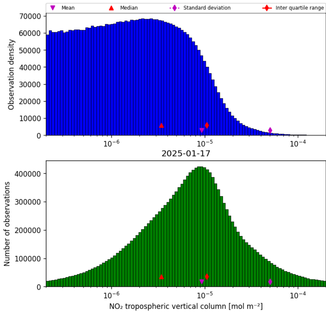
Figure 27: Histogram of “NO 2 tropospheric vertical column” for 2025-01-17 to 2025-01-18
