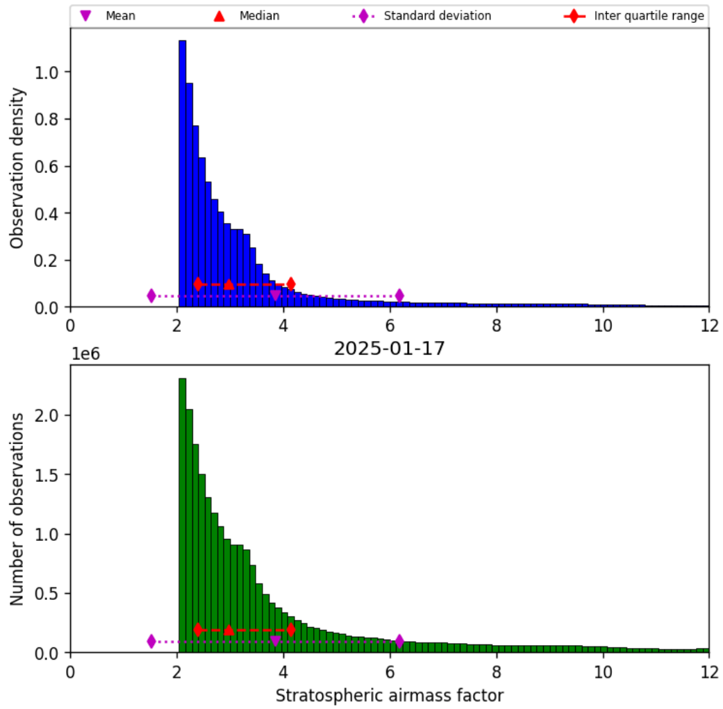
Figure 42: Histogram of “Stratospheric airmass factor” for 2025-01-17 to 2025-01-18
