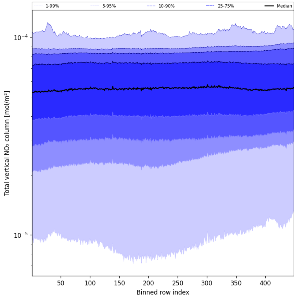
Figure 53: Along track statistics of “Total vertical NO 2 column” for 2025-01-17 to 2025-01-18
