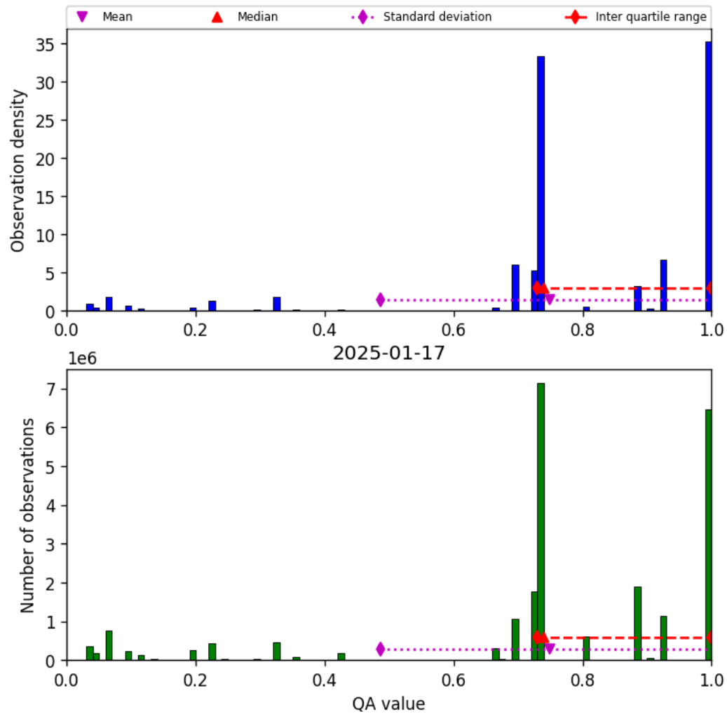
Figure 26: Histogram of “QA value” for 2025-01-17 to 2025-01-18
