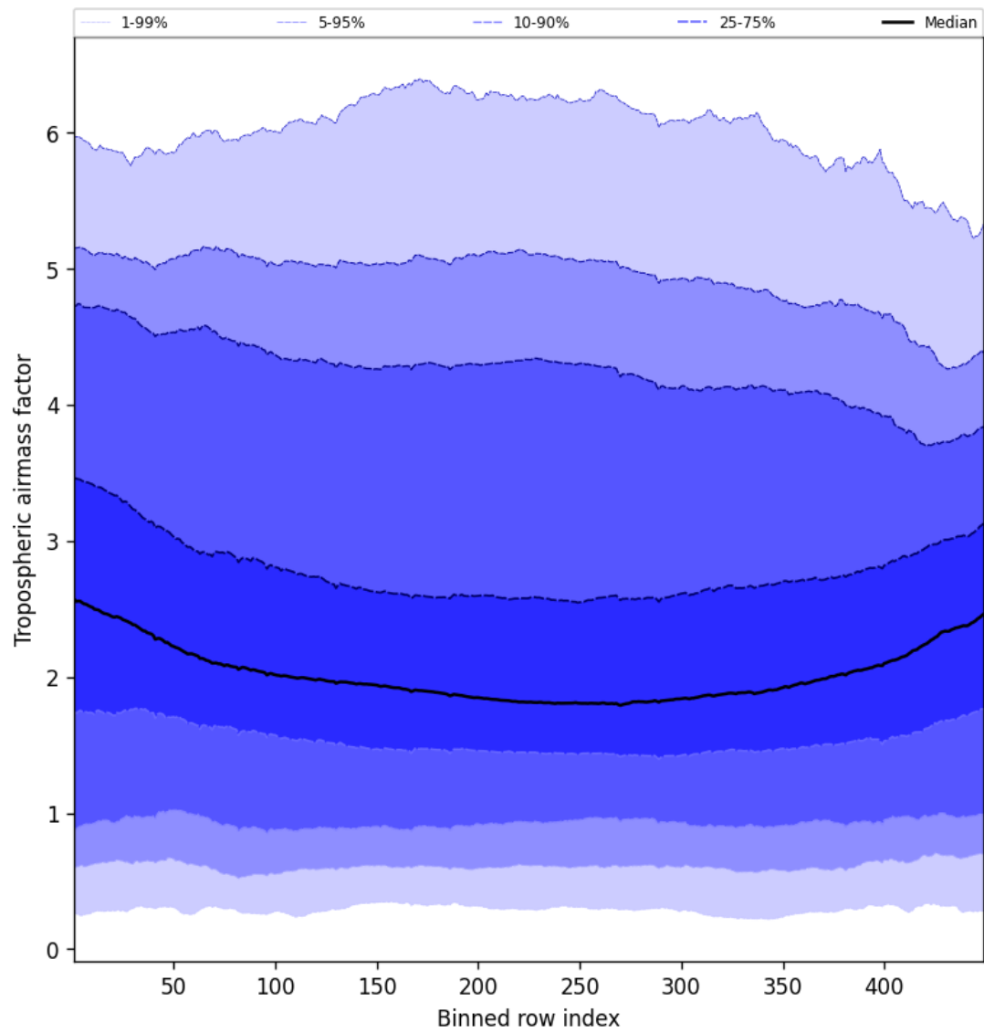
Figure 46: Along track statistics of “Tropospheric airmass factor” for 2025-01-17 to 2025-01-18
