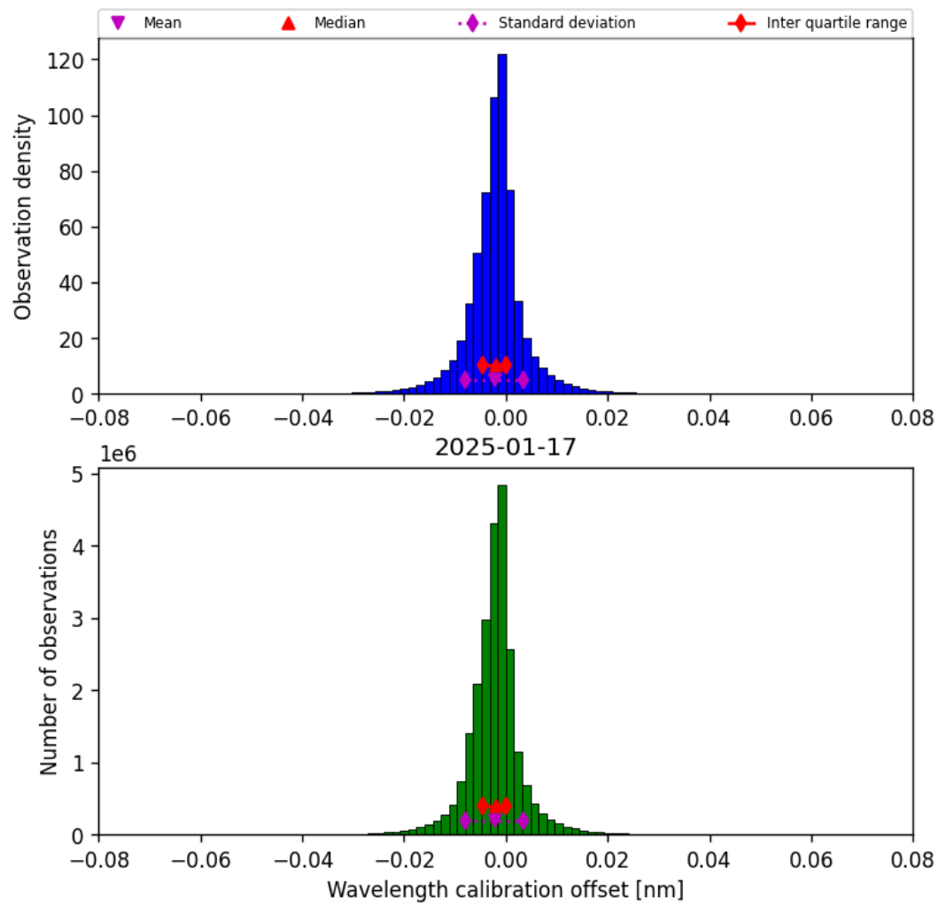
Figure 33: Histogram of “Wavelength calibration offset” for 2025-01-17 to 2025-01-18
