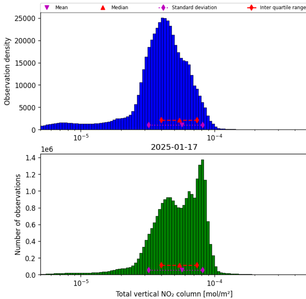
Figure 36: Histogram of "Total vertical NO 2 column" for 2025-01-17 to 2025-01-18
