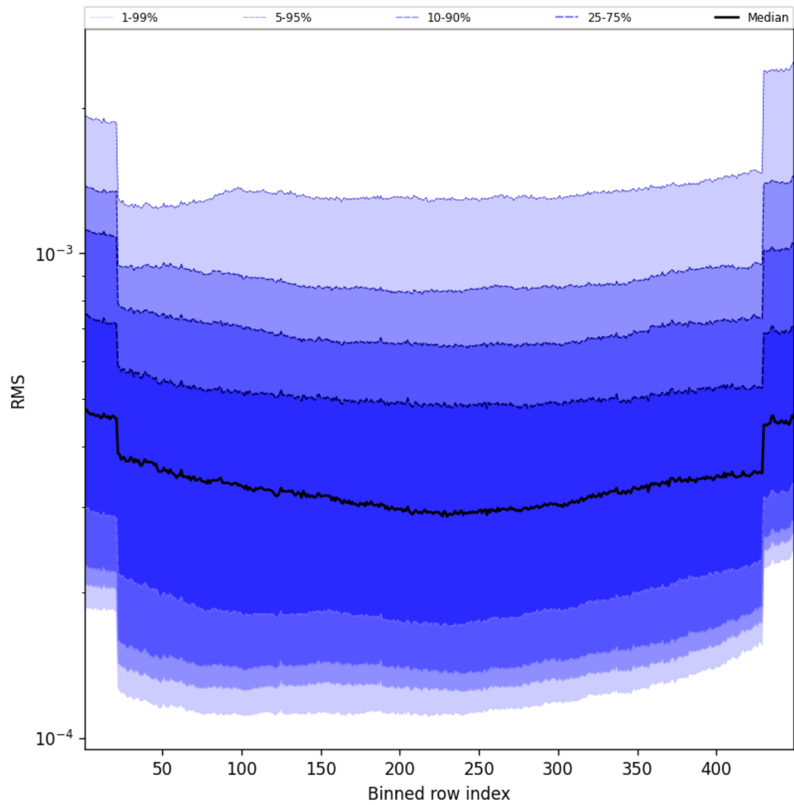
Figure 58: Along track statistics of “RMS” for 2025-01-17 to 2025-01-18
