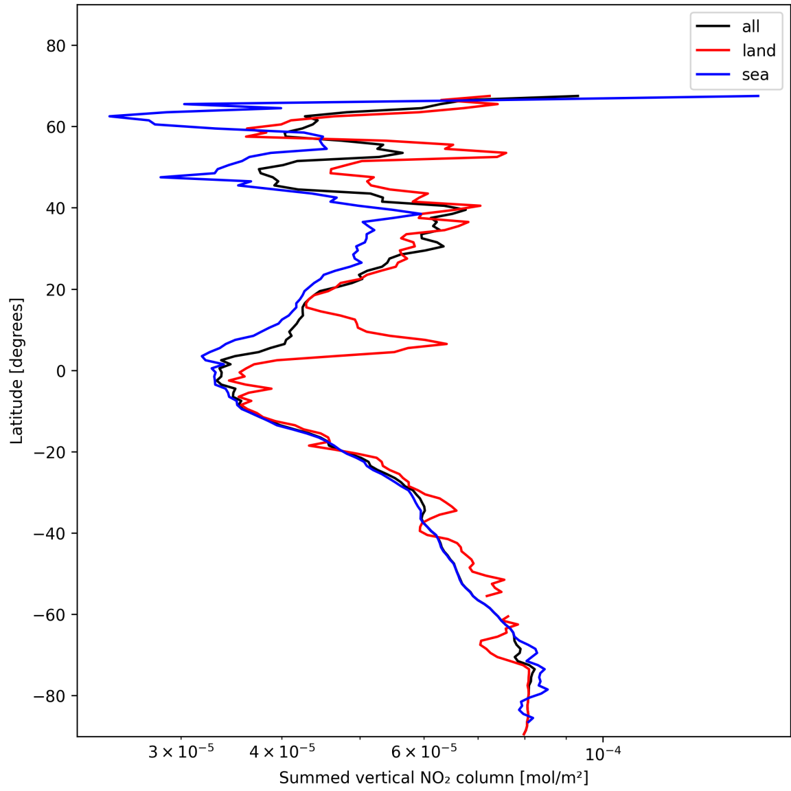
Figure 21: Zonal average of “Summed vertical NO 2 column” for 2025-01-17 to 2025-01-18.
