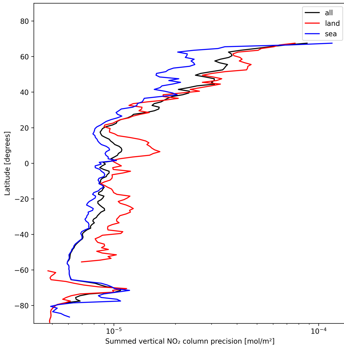
Figure 22: Zonal average of “Summed vertical NO 2 column precision” for 2025-01-17 to 2025-01-18.
