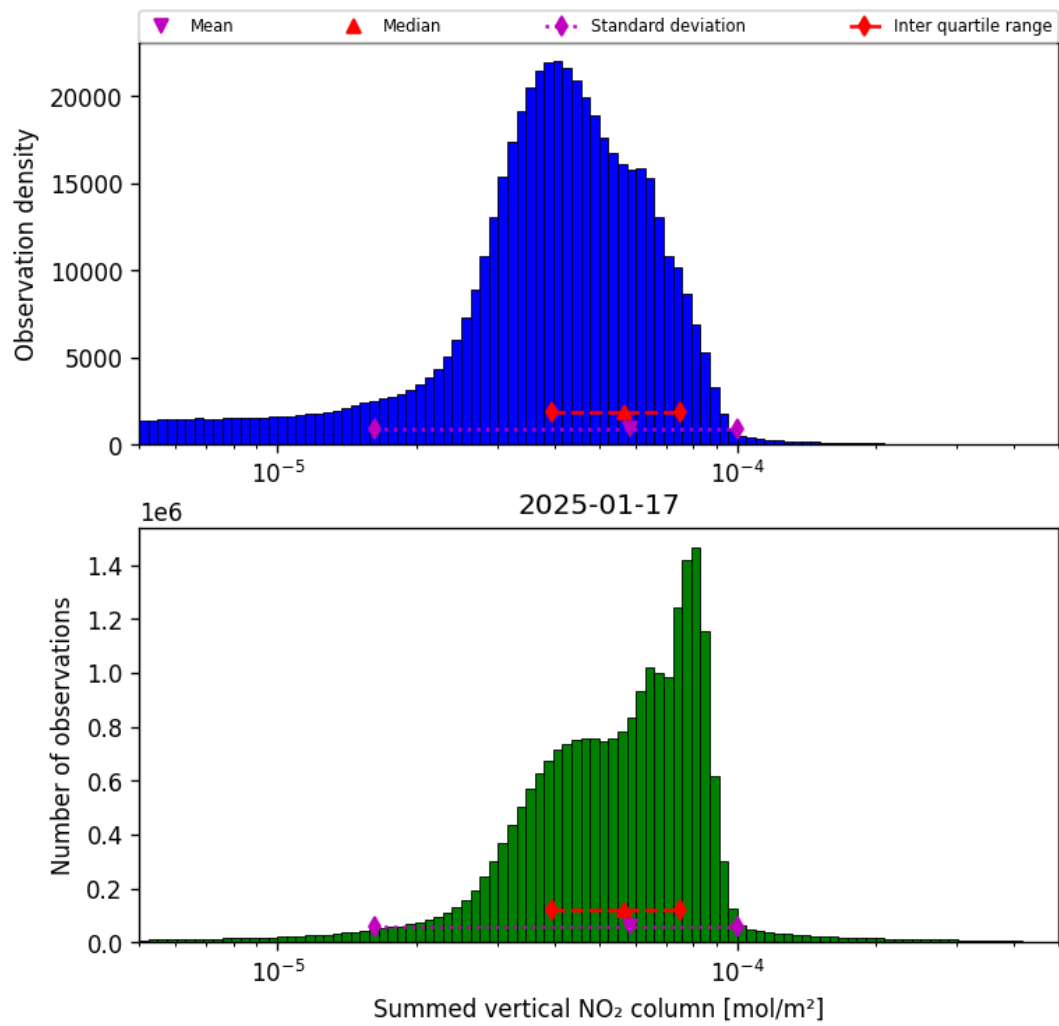
Figure 38: Histogram of “Summed vertical NO 2 column” for 2025-01-17 to 2025-01-18
