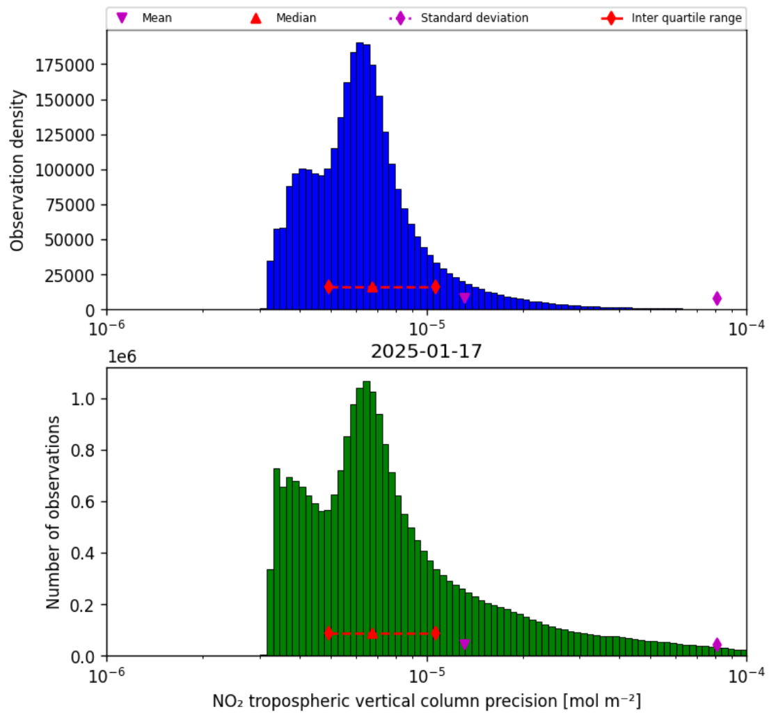
Figure 28: Histogram of “NO 2 tropospheric vertical column precision” for 2025-01-17 to 2025-01-18
