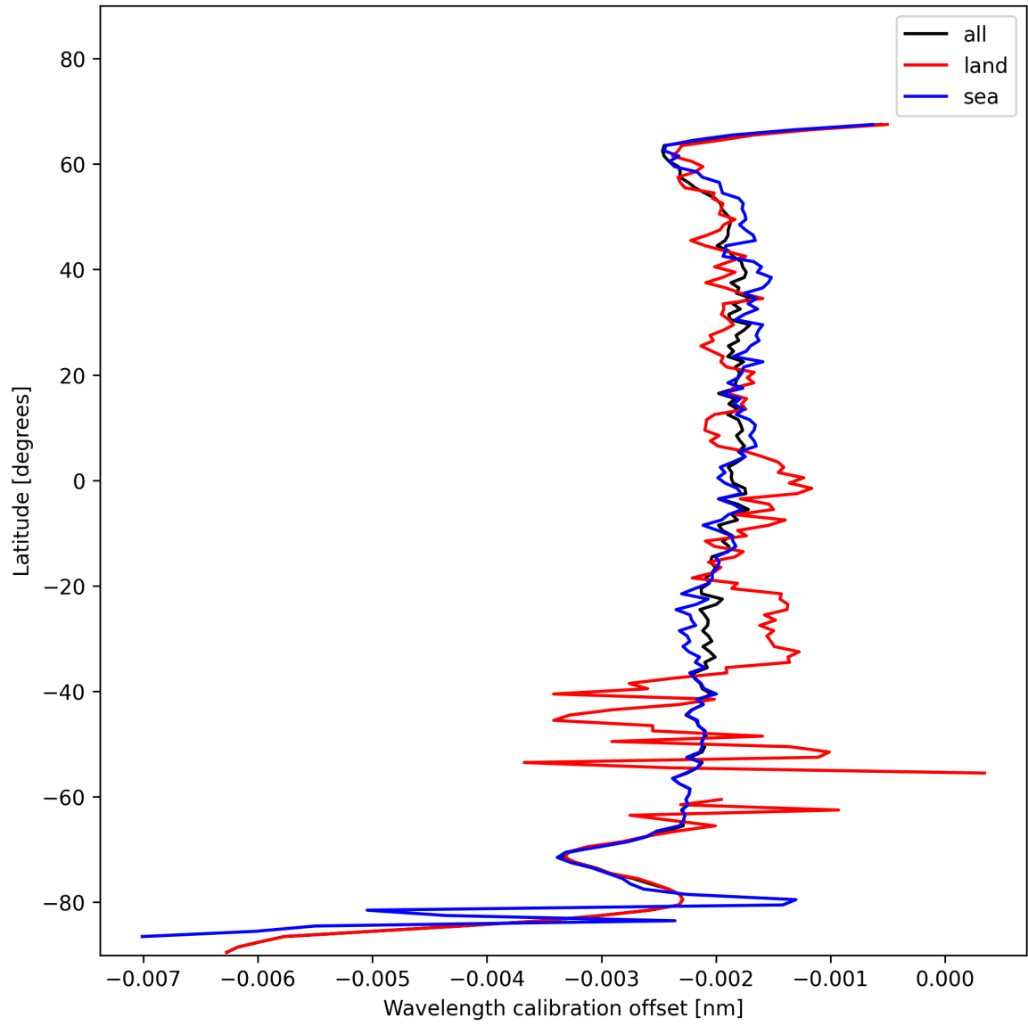
Figure 16: Zonal average of “Wavelength calibration offset” for 2025-01-17 to 2025-01-18.
