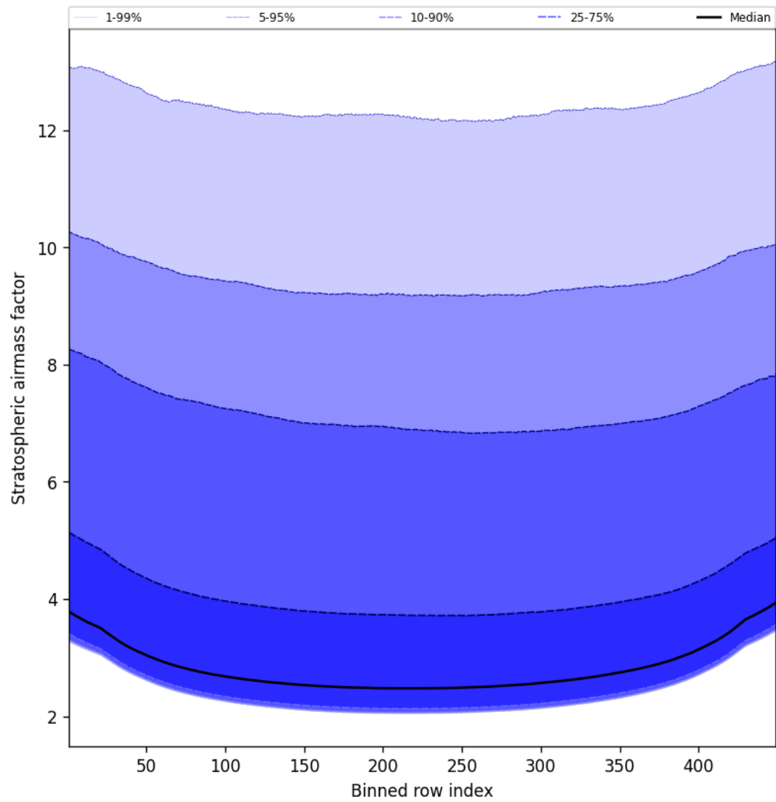
Figure 59: Along track statistics of “Stratospheric airmass factor” for 2025-01-17 to 2025-01-18
