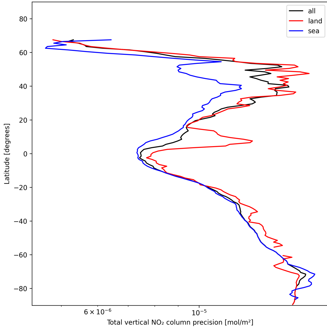
Figure 20: Zonal average of “Total vertical NO 2 column precision” for 2025-01-17 to 2025-01-18.
