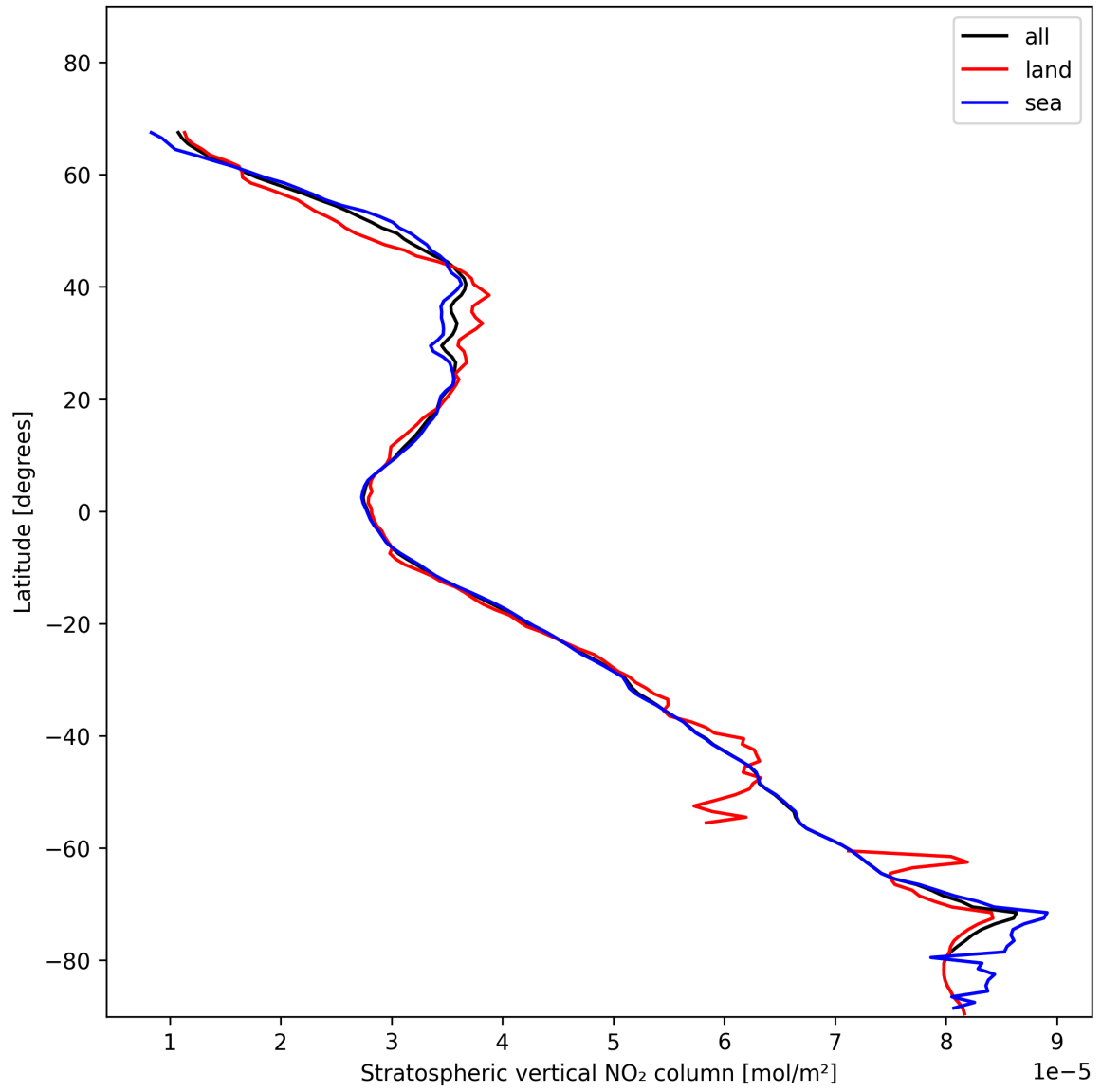
Figure 17: Zonal average of “Stratospheric vertical NO 2 column” for 2025-01-18 to 2025-01-19.
