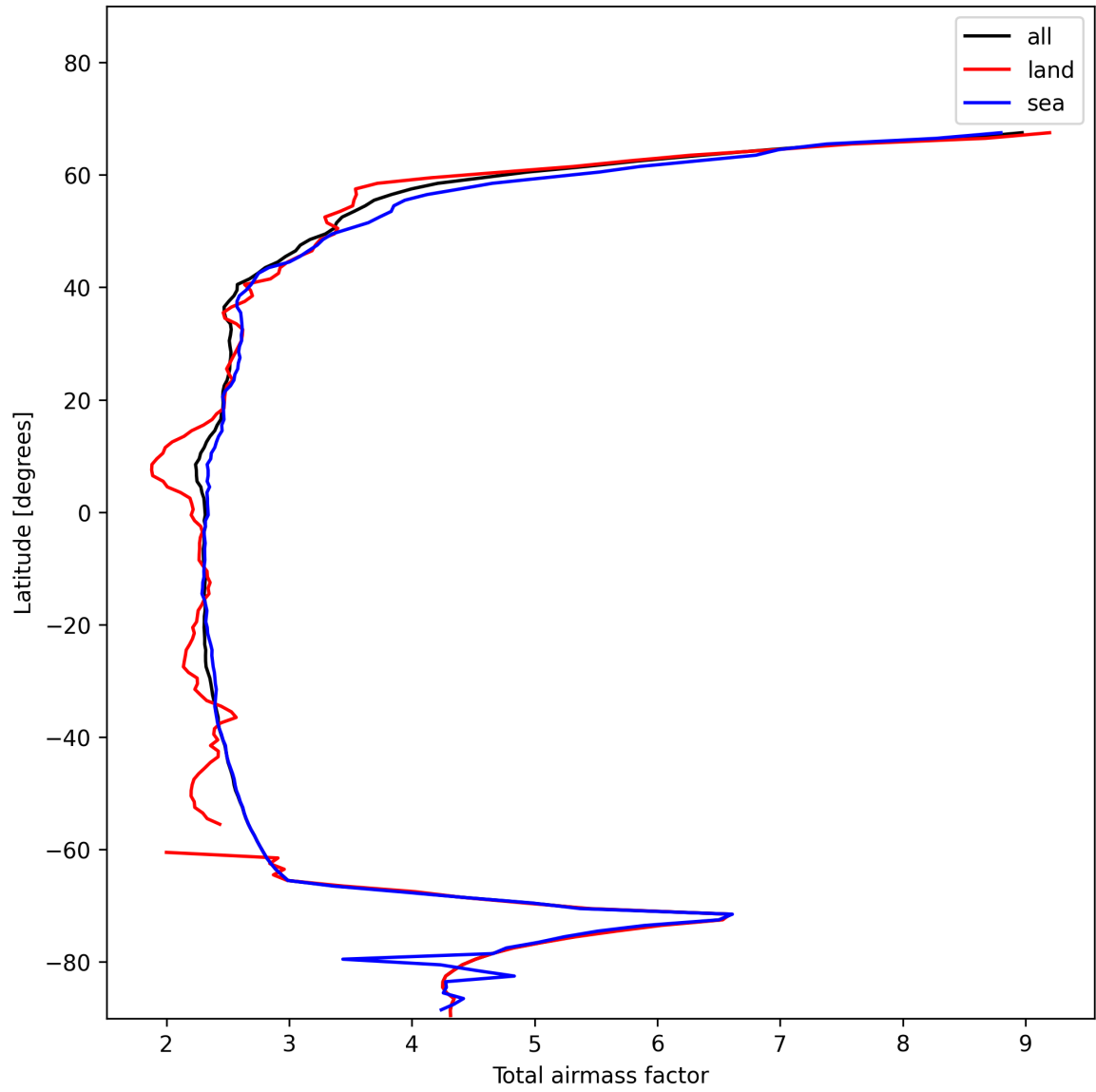
Figure 13: Zonal average of “Total airmass factor” for 2025-01-18 to 2025-01-19.
