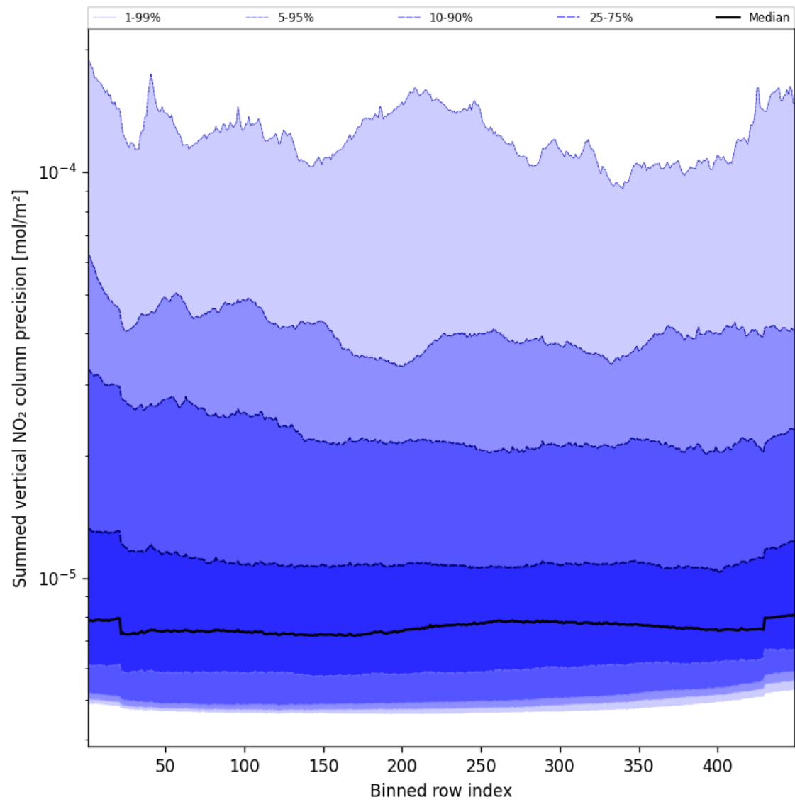
Figure 56: Along track statistics of “Summed vertical NO 2 column precision” for 2025-01-18 to 2025-01-19
