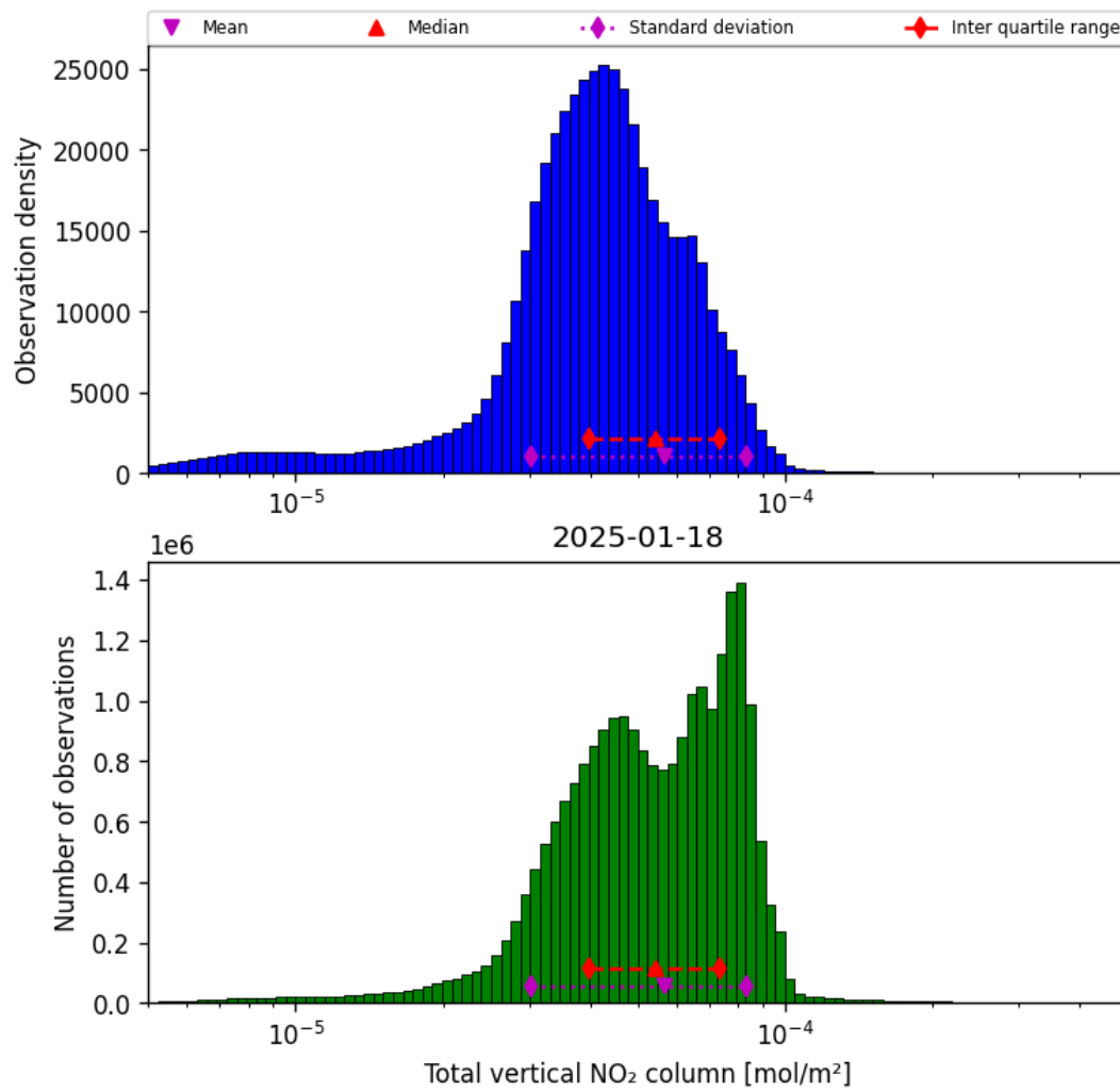
Figure 36: Histogram of “Total vertical NO 2 column” for 2025-01-18 to 2025-01-19
