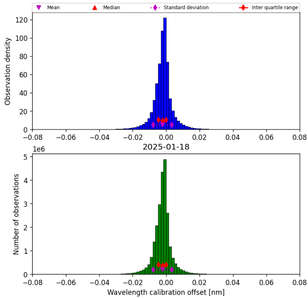
Figure 33: Histogram of “Wavelength calibration offset” for 2025-01-18 to 2025-01-19
