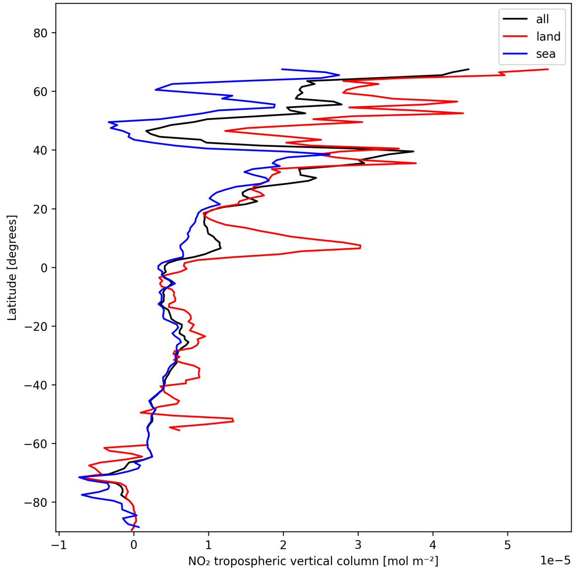
Figure 10: Zonal average of “NO 2 tropospheric vertical column” for 2025-01-18 to 2025-01-19.
