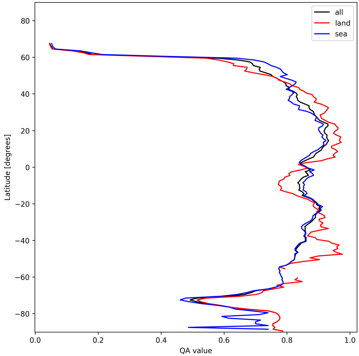
Figure 9: Zonal average of “QA value” for 2025-01-18 to 2025-01-19.
