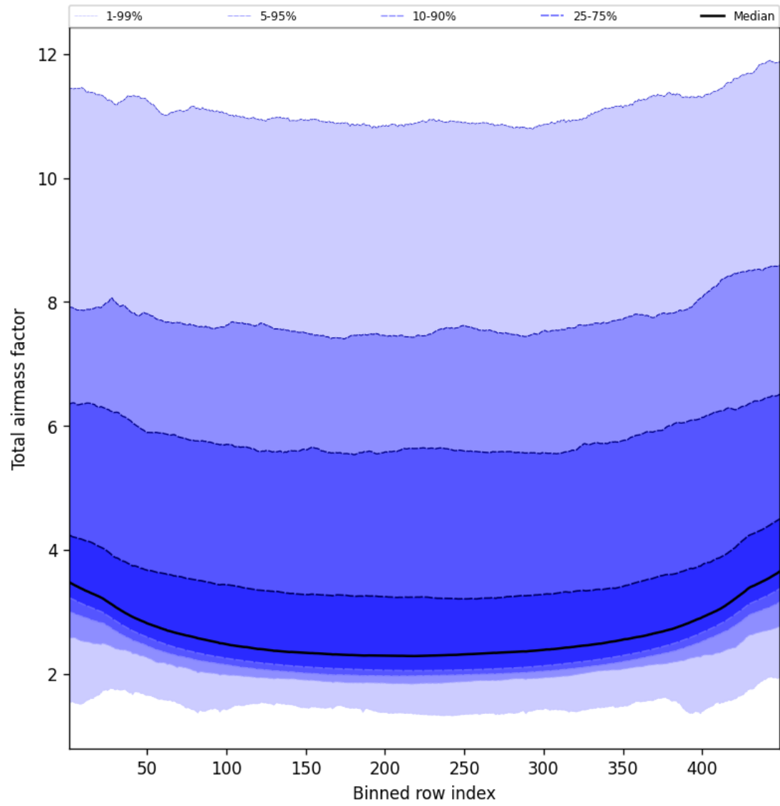
Figure 47: Along track statistics of “Total airmass factor” for 2025-01-18 to 2025-01-19
