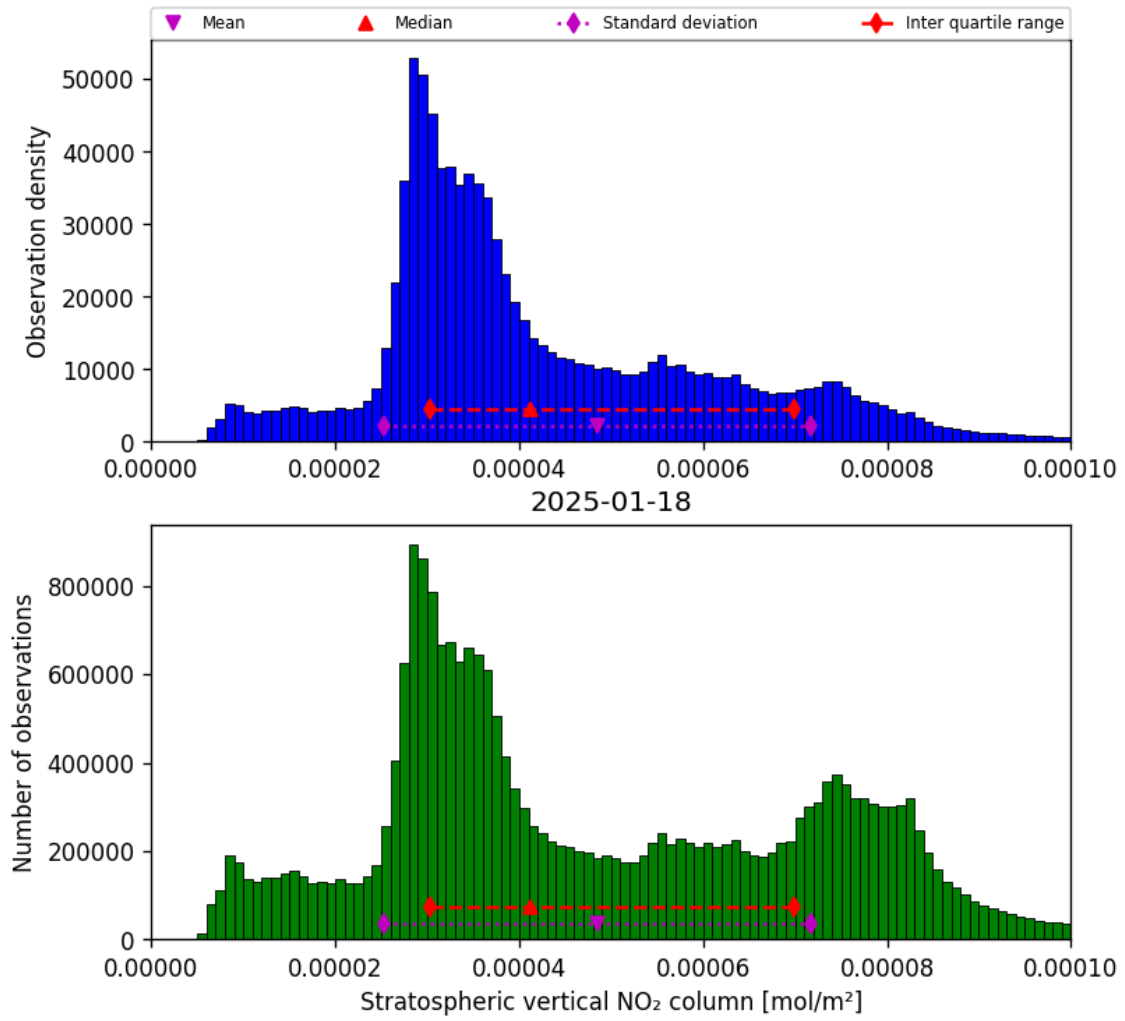
Figure 34: Histogram of “Stratospheric vertical NO 2 column” for 2025-01-18 to 2025-01-19
