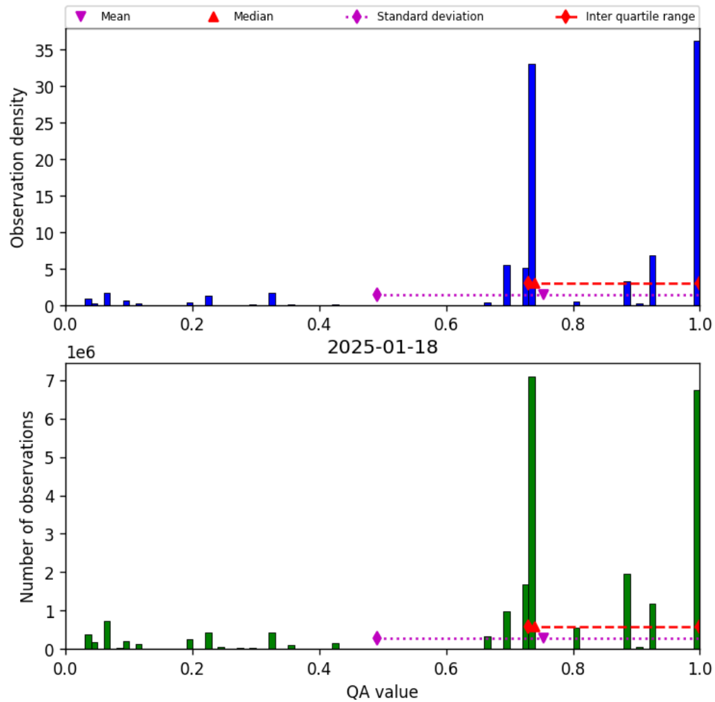
Figure 26: Histogram of “QA value” for 2025-01-18 to 2025-01-19
