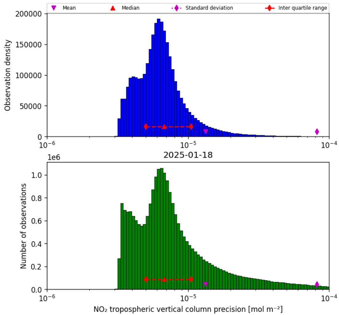
Figure 28: Histogram of “NO 2 tropospheric vertical column precision” for 2025-01-18 to 2025-01-19
