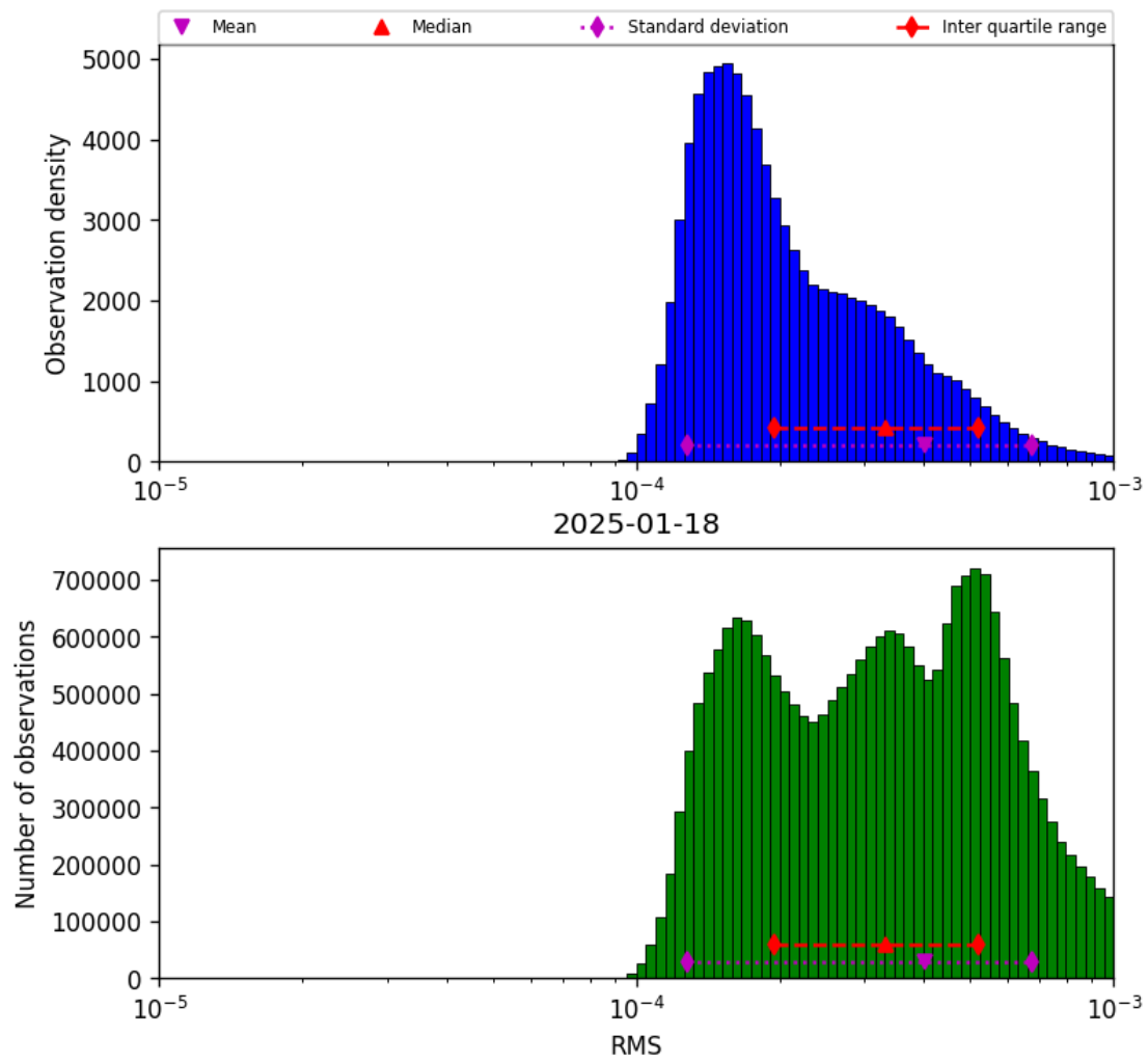
Figure 41: Histogram of “RMS” for 2025-01-18 to 2025-01-19
