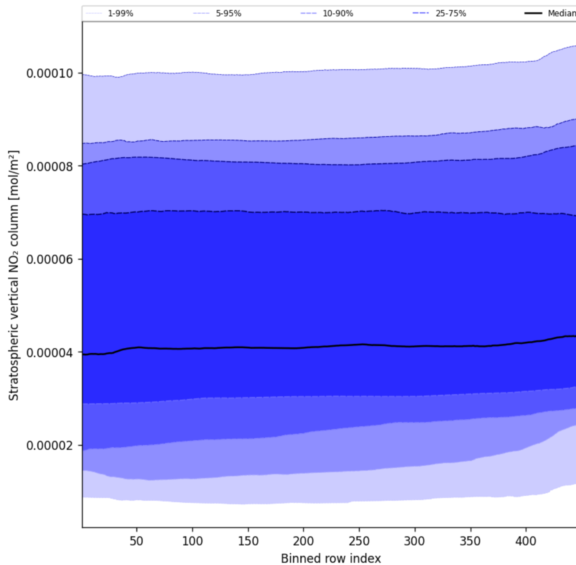
Figure 51: Along track statistics of “Stratospheric vertical NO 2 column” for 2025-01-18 to 2025-01-19
