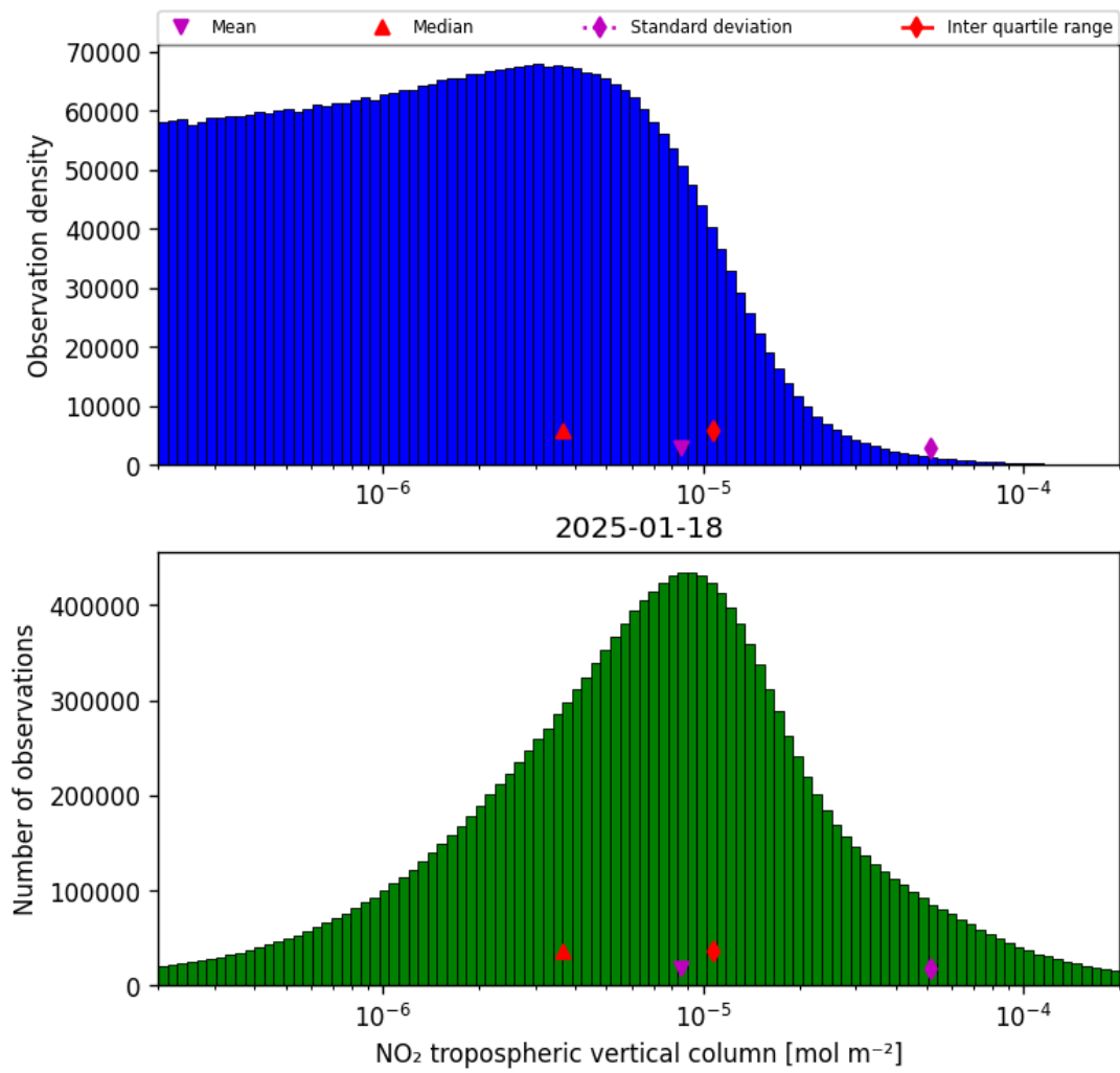
Figure 27: Histogram of “NO 2 tropospheric vertical column” for 2025-01-18 to 2025-01-19
