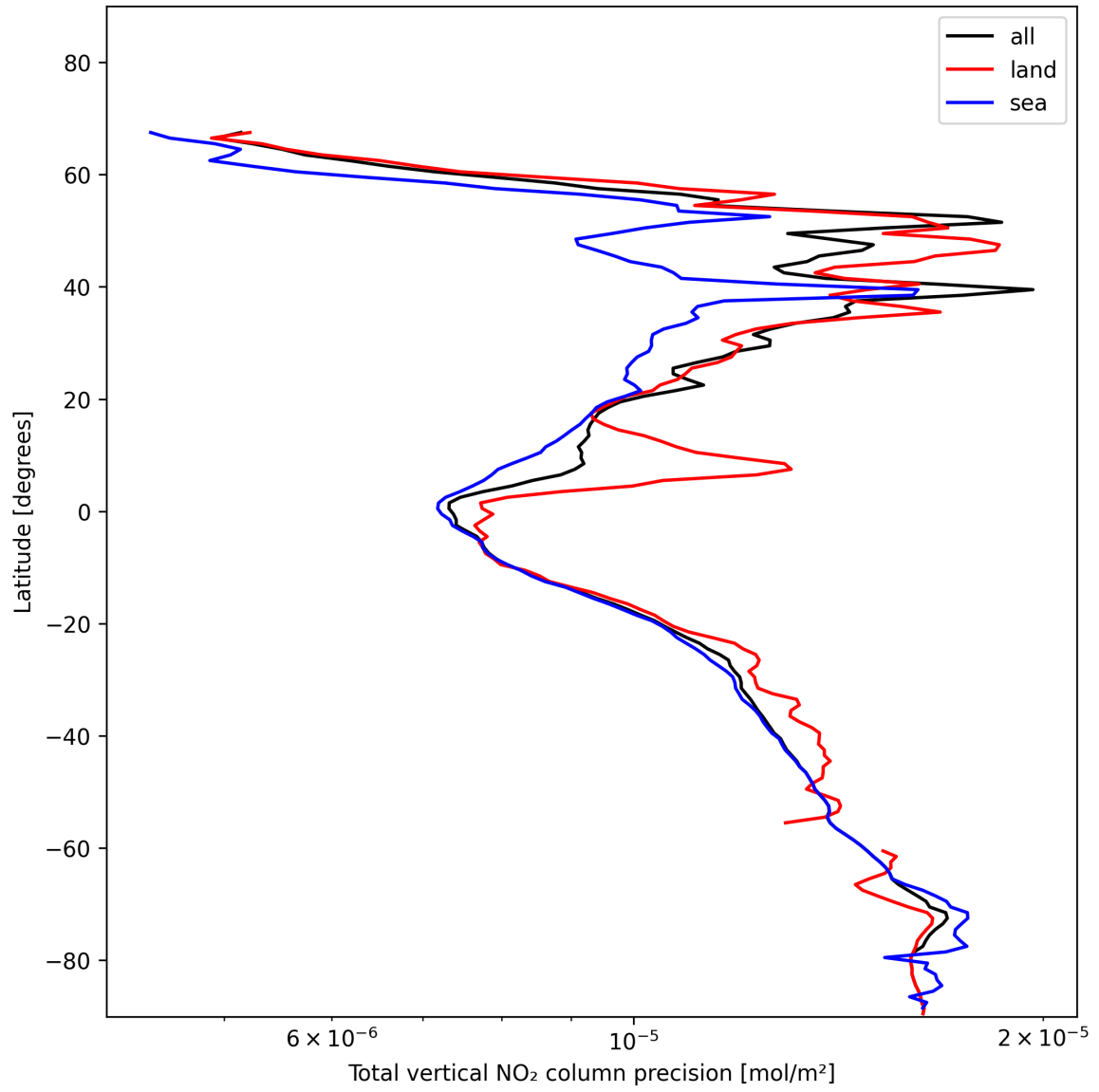
Figure 20: Zonal average of “Total vertical NO 2 column precision” for 2025-01-18 to 2025-01-19.
