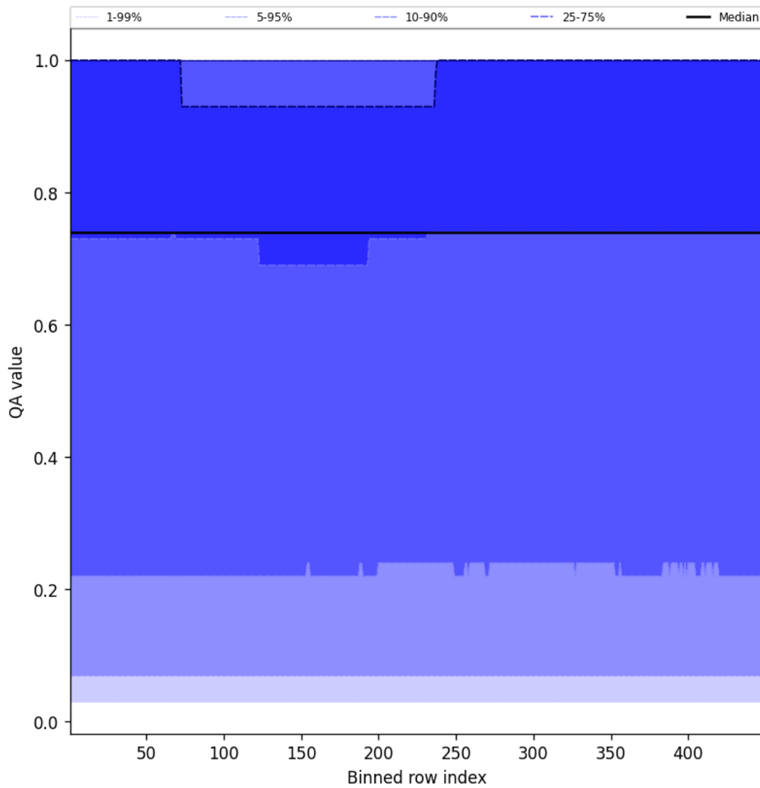
Figure 43: Along track statistics of “QA value” for 2025-01-18 to 2025-01-19
