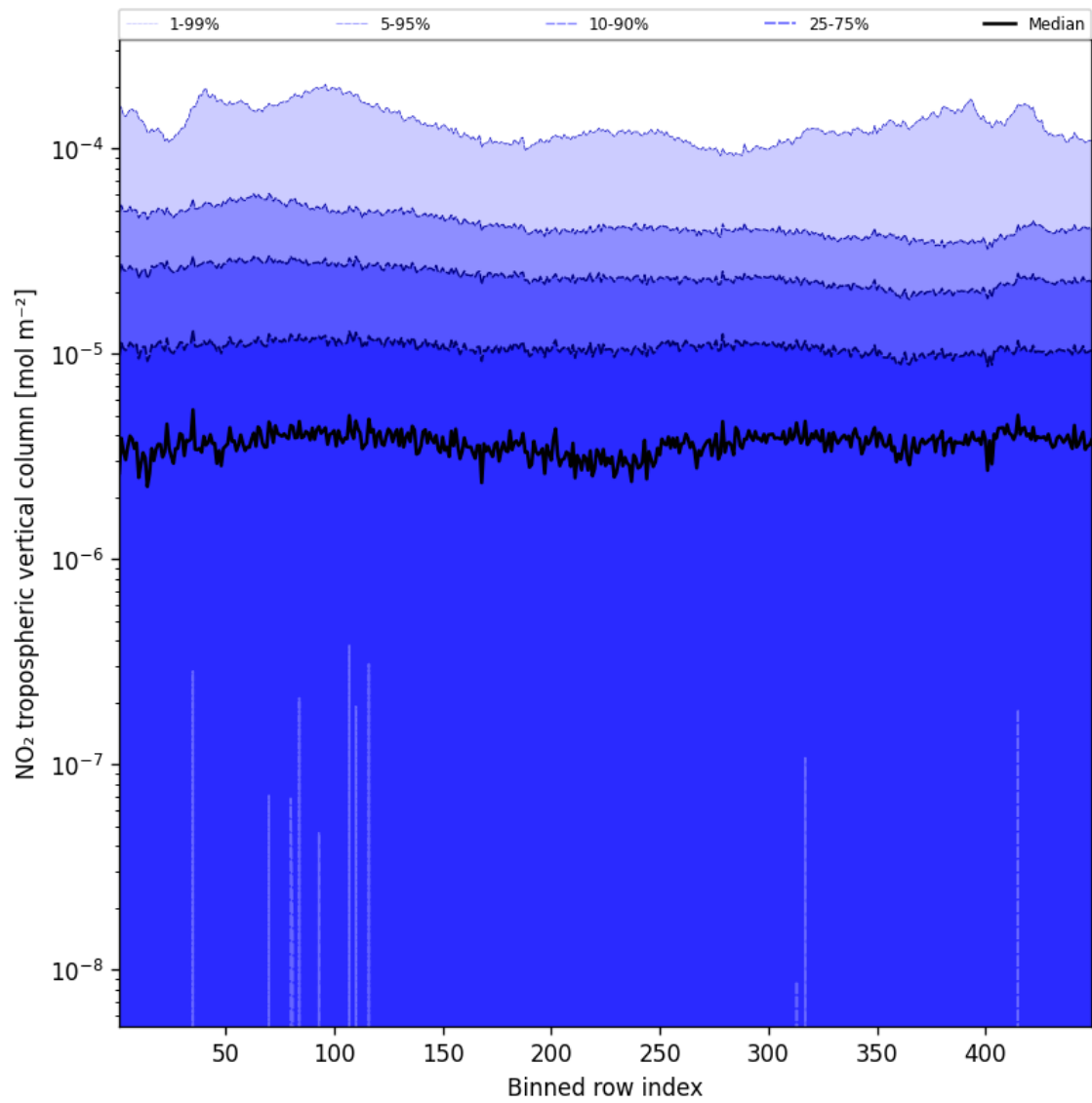
Figure 44: Along track statistics of “NO 2 tropospheric vertical column” for 2025-01-18 to 2025-01-19
