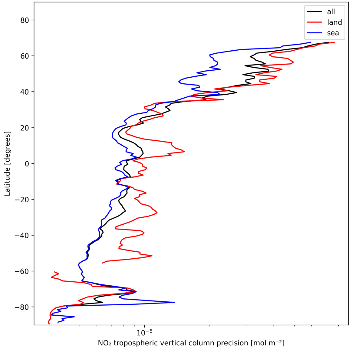
Figure 11: Zonal average of “NO 2 tropospheric vertical column precision” for 2025-01-18 to 2025-01-19.
