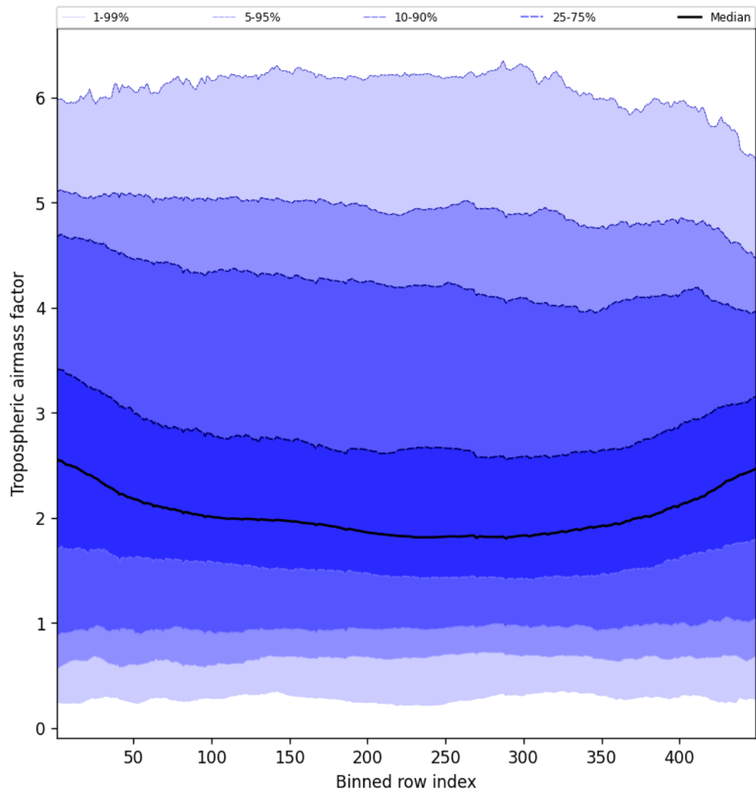
Figure 46: Along track statistics of “Tropospheric air mass factor” for 2025-01-18 to 2025-01-19
