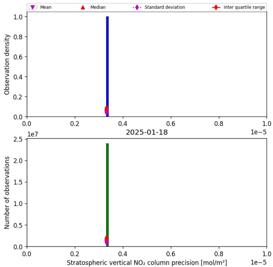
Figure 35: Histogram of “Stratospheric vertical NO 2 column precision” for 2025-01-18 to 2025-01-19
