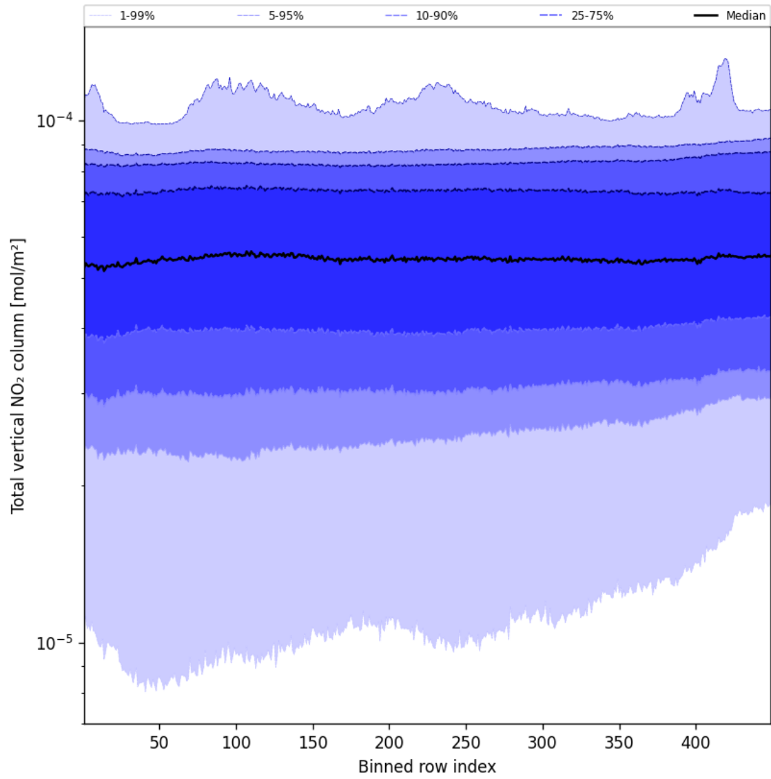
Figure 53: Along track statistics of “Total vertical NO 2 column” for 2025-01-18 to 2025-01-19
