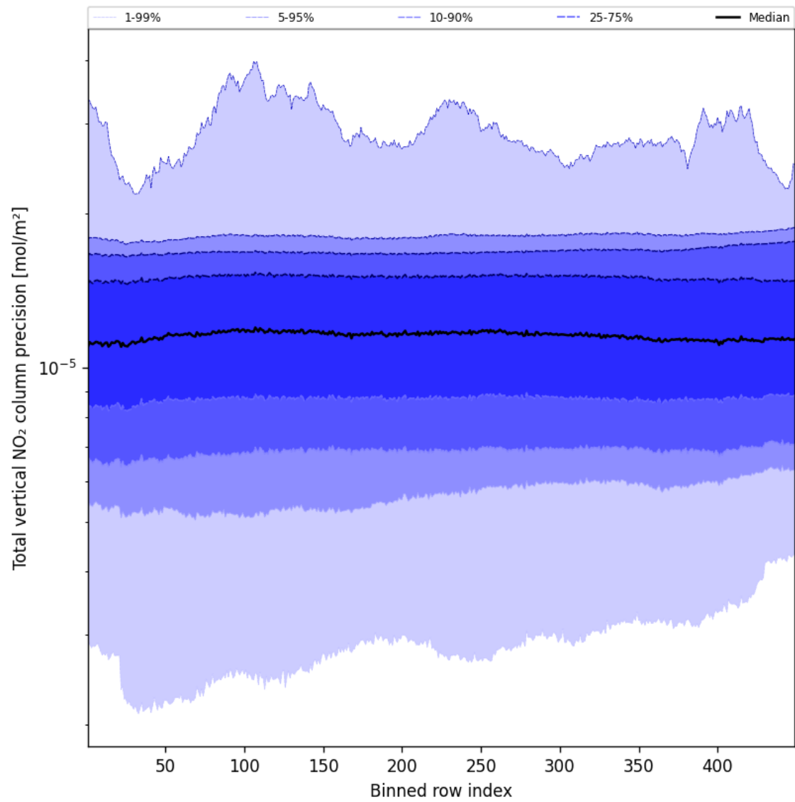
Figure 54: Along track statistics of “Total vertical NO 2 column precision” for 2025-01-18 to 2025-01-19
