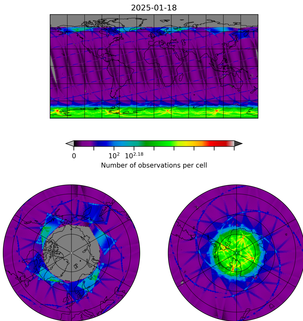
Figure 8: Map of the number of observations for 2025-01-18 to 2025-01-19
