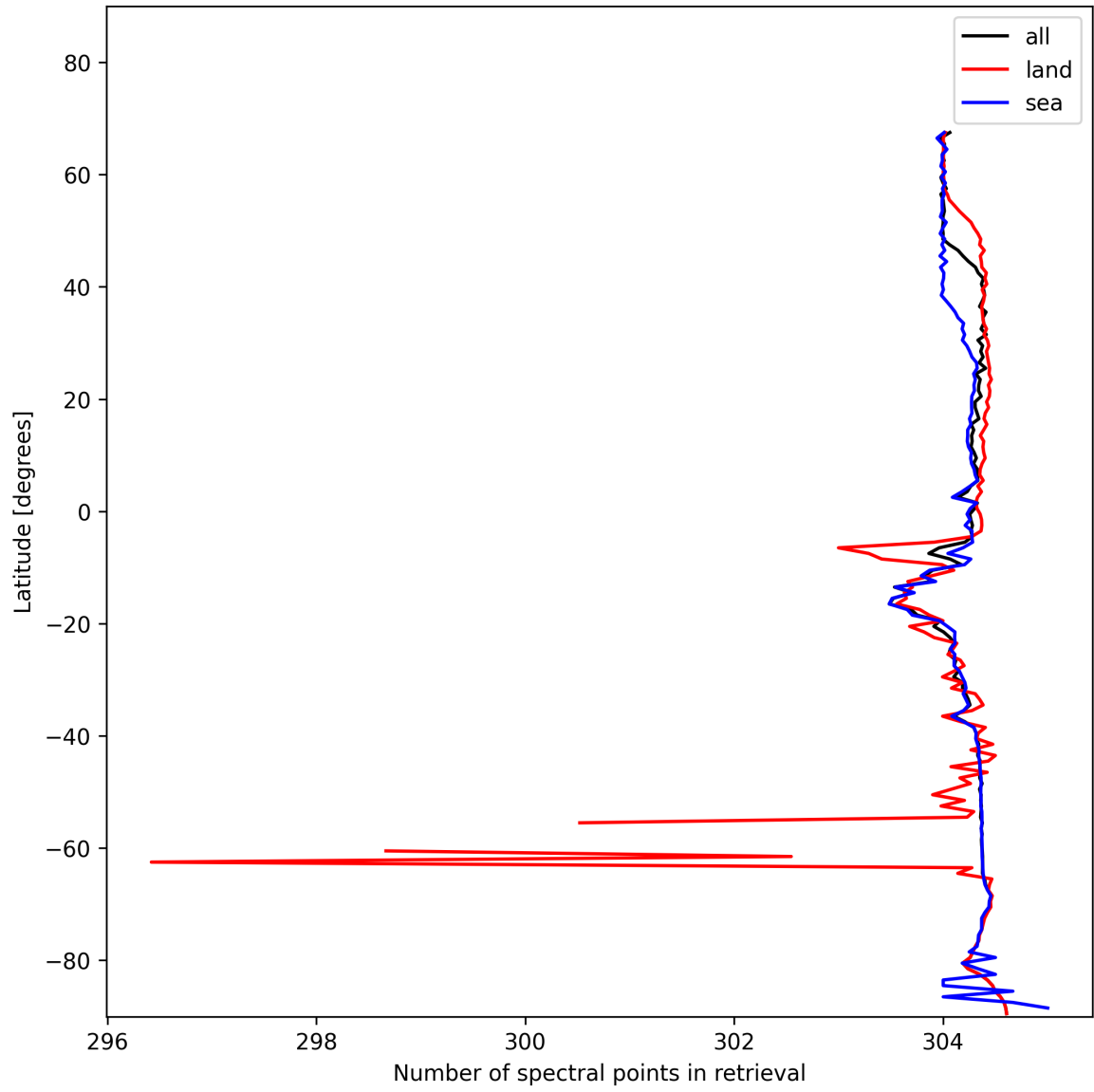
Figure 14: Zonal average of “Number of spectral points in retrieval” for 2025-01-18 to 2025-01-19.
