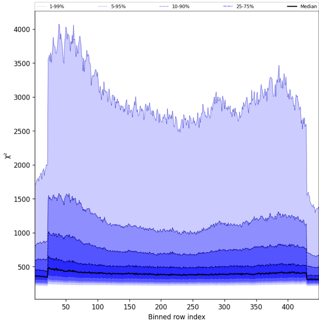
Figure 57: Along track statistics of “ \chi^2 ” for 2025-01-18 to 2025-01-19
