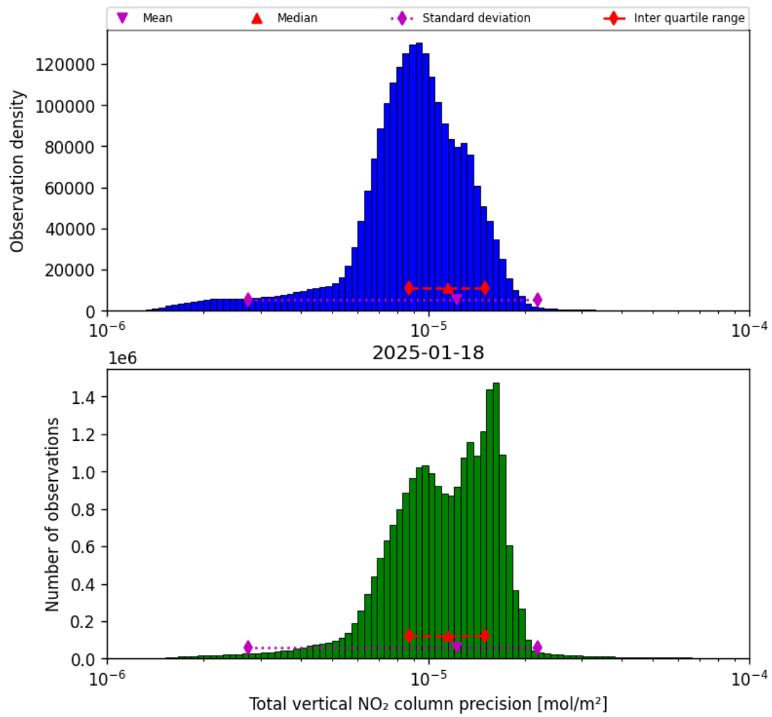
Figure 37: Histogram of “Total vertical NO 2 column precision” for 2025-01-18 to 2025-01-19
