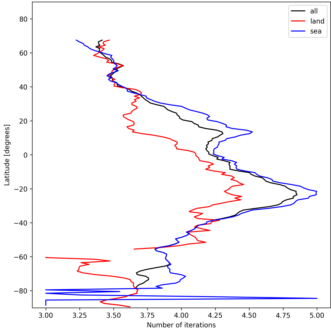
Figure 15: Zonal average of “Number of iterations” for 2025-01-18 to 2025-01-19.
