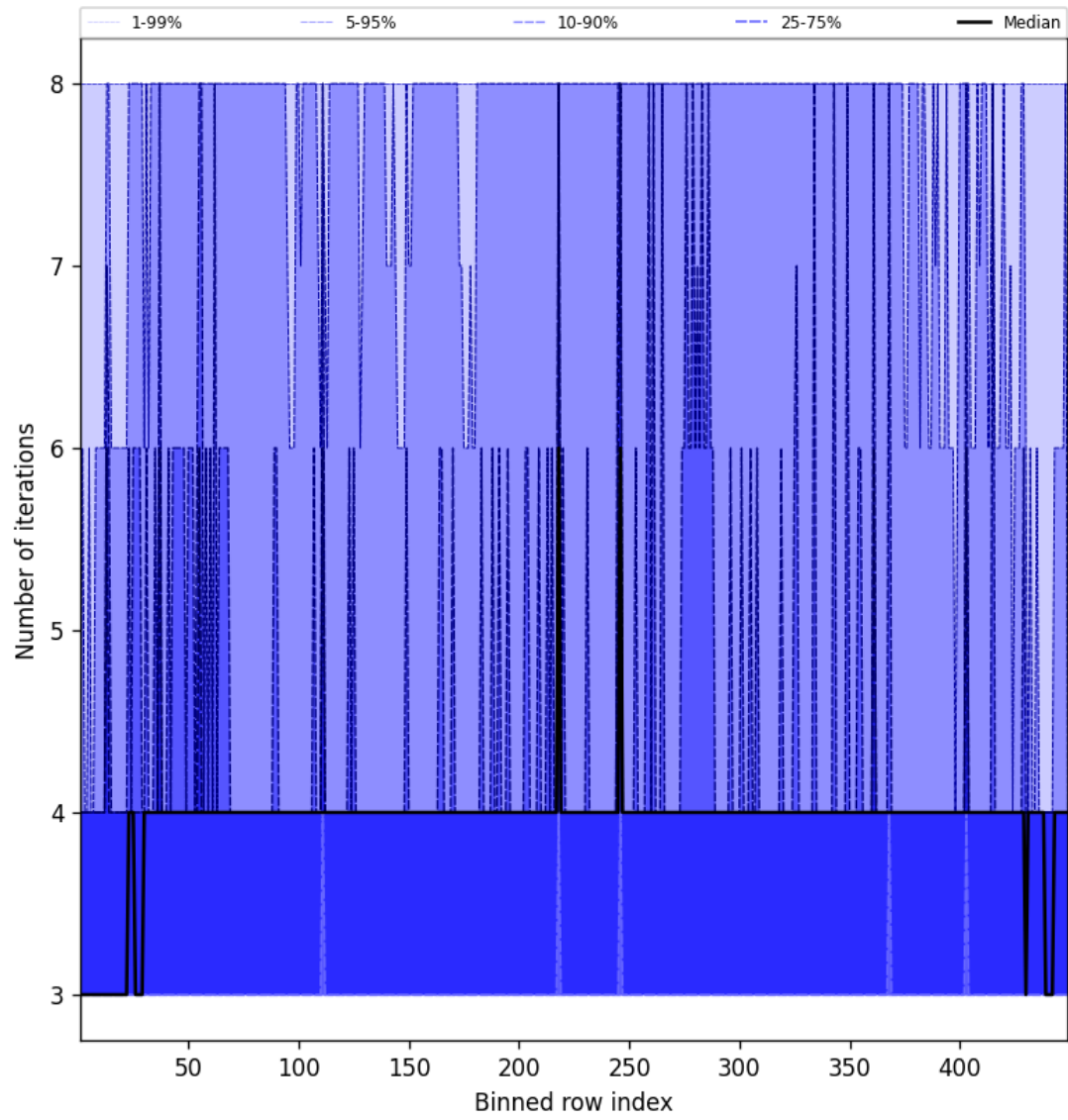
Figure 49: Along track statistics of “Number of iterations” for 2025-01-18 to 2025-01-19
