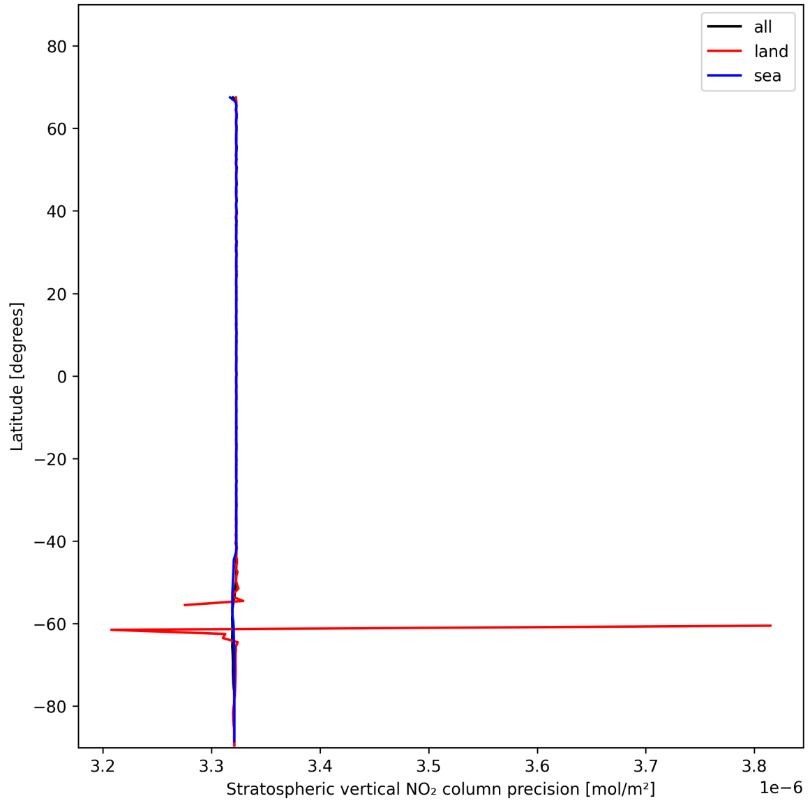
Figure 18: Zonal average of “Stratospheric vertical NO 2 column precision” for 2025-01-18 to 2025-01-19.
