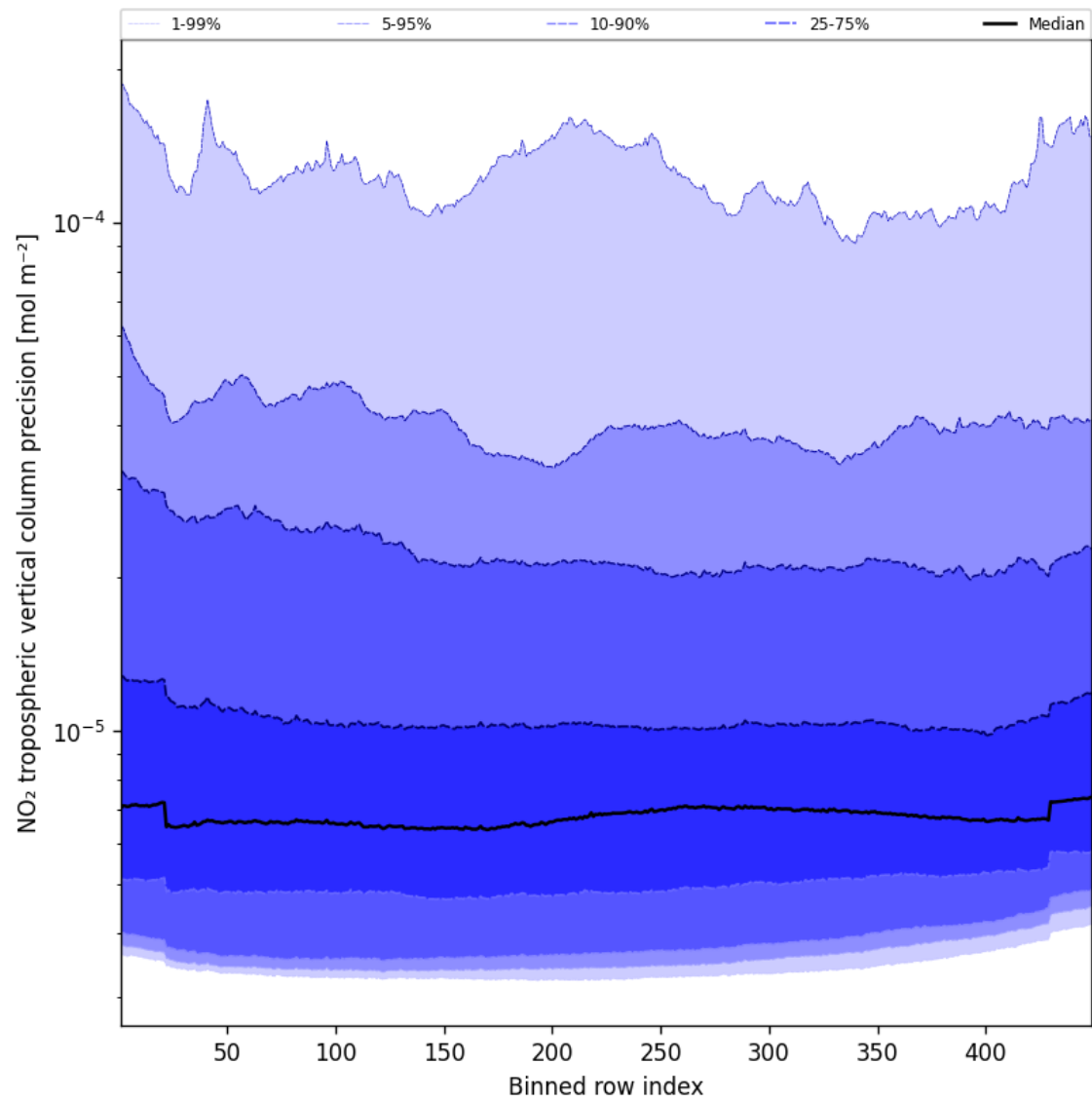
Figure 45: Along track statistics of “NO 2 tropospheric vertical column precision” for 2025-01-18 to 2025-01-19
