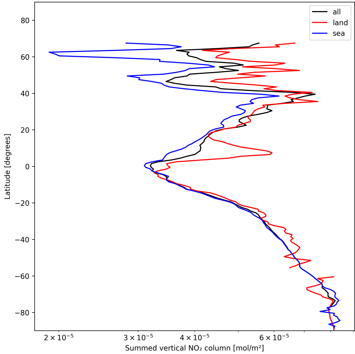
Figure 21: Zonal average of “Summed vertical NO 2 column” for 2025-01-18 to 2025-01-19.
