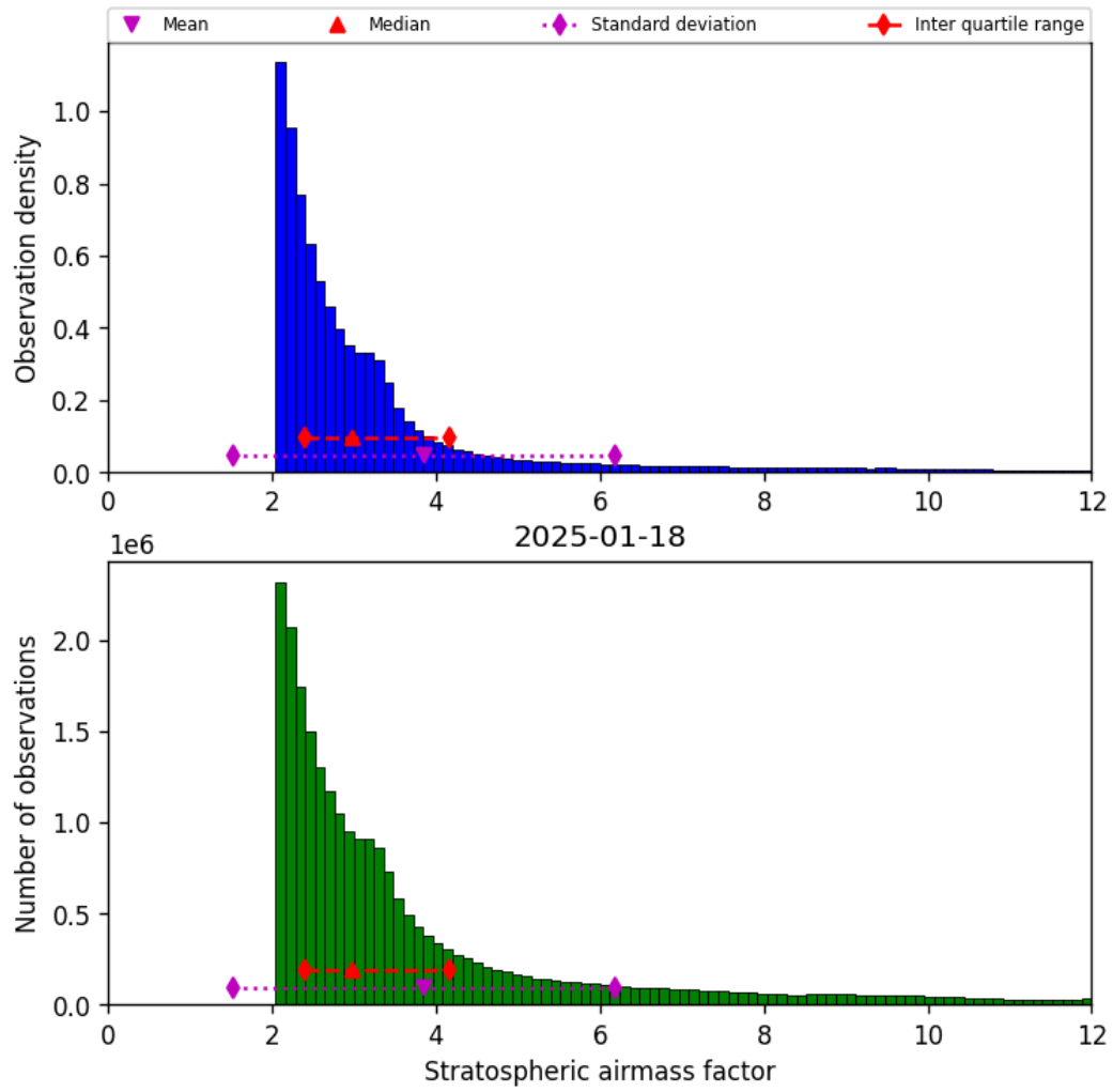
Figure 42: Histogram of “Stratospheric airmass factor” for 2025-01-18 to 2025-01-19
