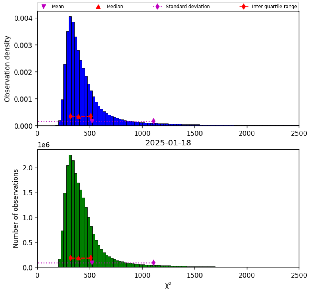
Figure 40: Histogram of “ \chi^2 ” for 2025-01-18 to 2025-01-19
