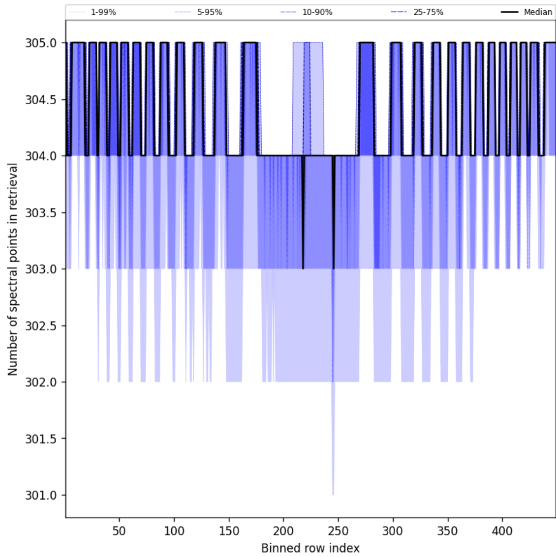
Figure 48: Along track statistics of “Number of spectral points in retrieval” for 2025-01-18 to 2025-01-19
