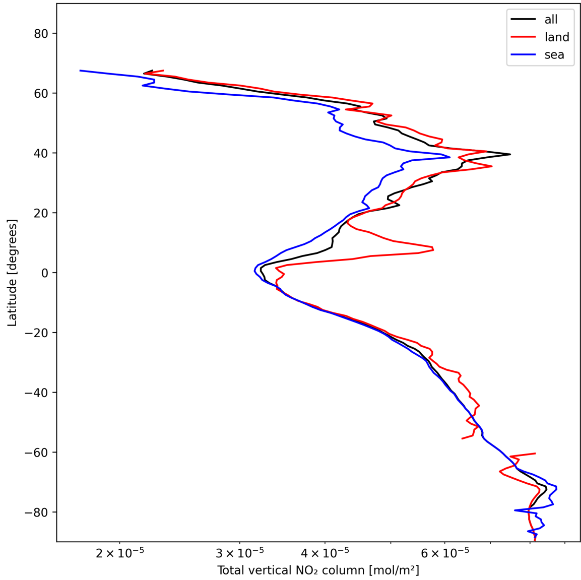
Figure 19: Zonal average of “Total vertical NO 2 column” for 2025-01-18 to 2025-01-19.
