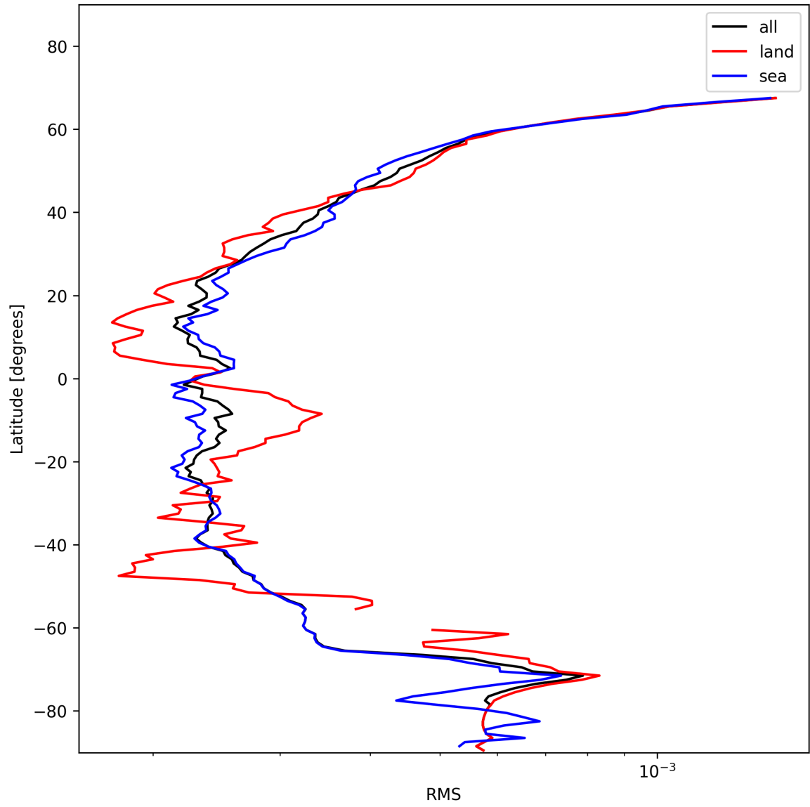
Figure 24: Zonal average of “RMS” for 2025-01-18 to 2025-01-19.
