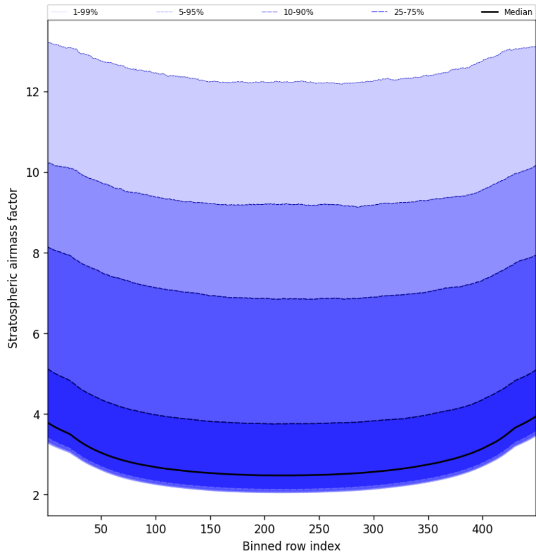
Figure 59: Along track statistics of “Stratospheric airmass factor” for 2025-01-18 to 2025-01-19
