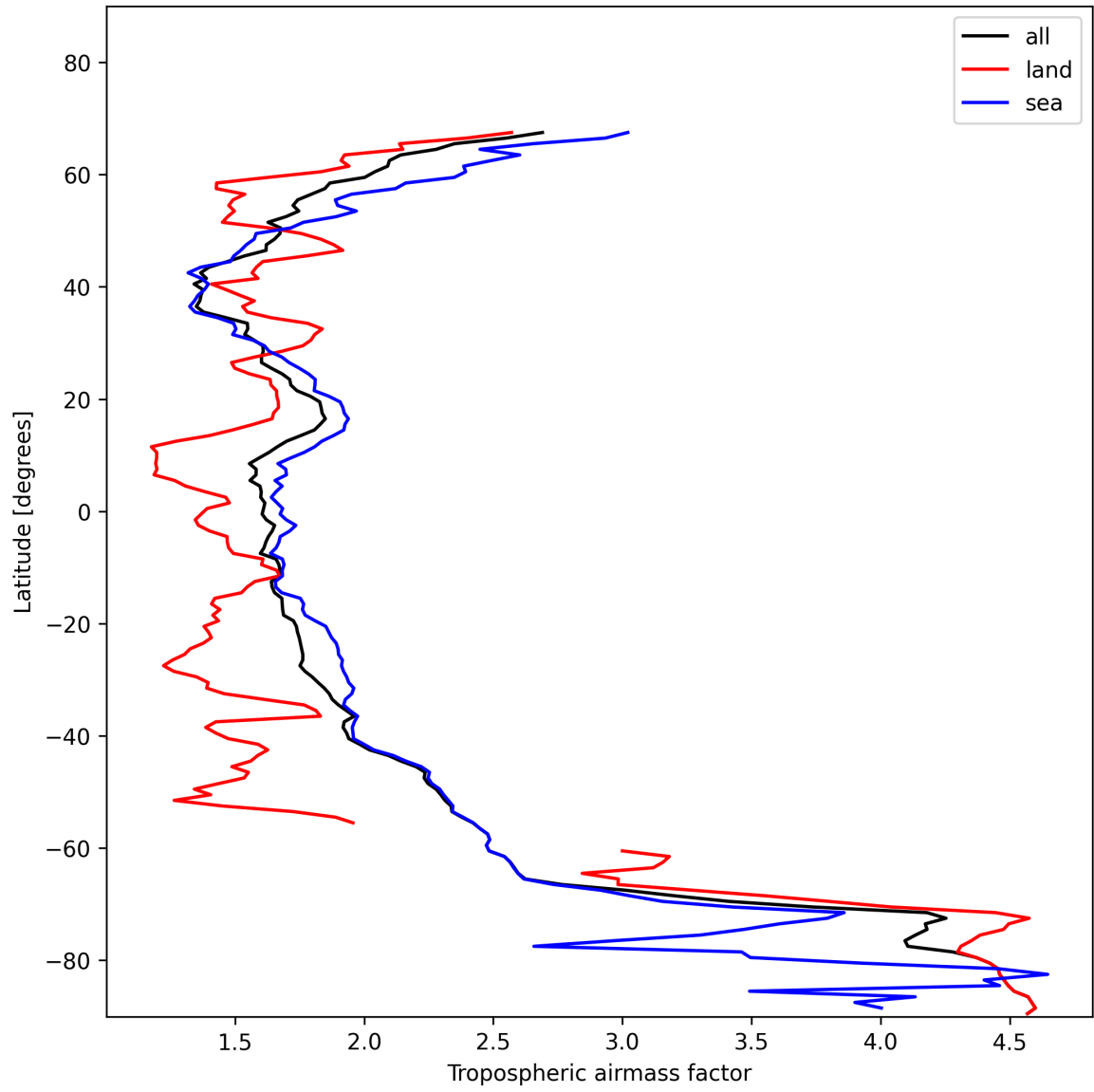
Figure 12: Zonal average of “Tropospheric airmass factor” for 2025-01-18 to 2025-01-19.
