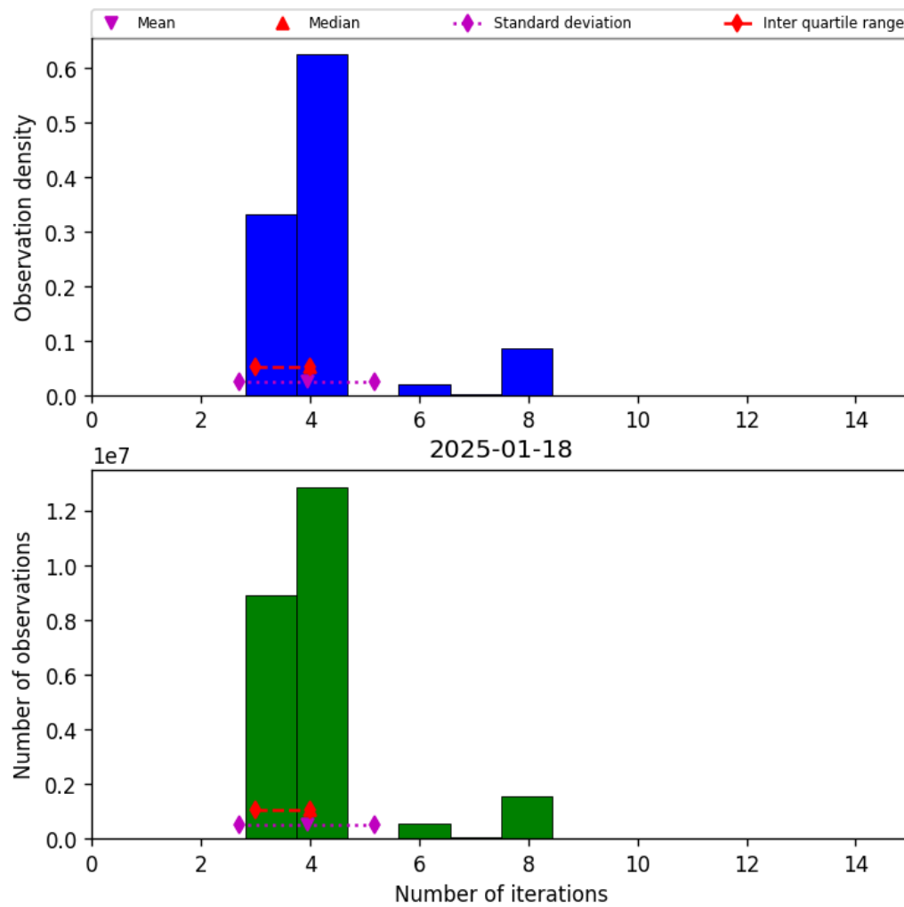
Figure 32: Histogram of “Number of iterations” for 2025-01-18 to 2025-01-19
