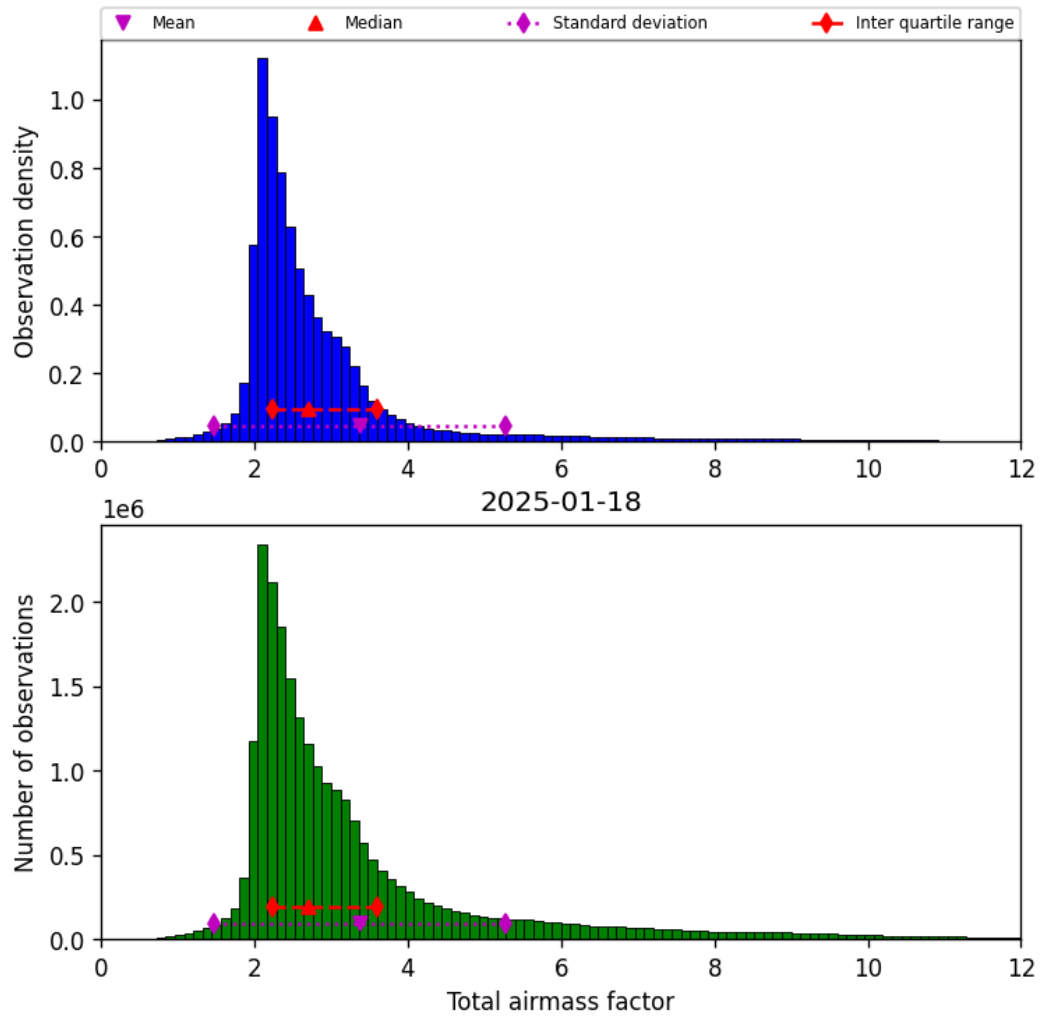
Figure 30: Histogram of “Total airmass factor” for 2025-01-18 to 2025-01-19
