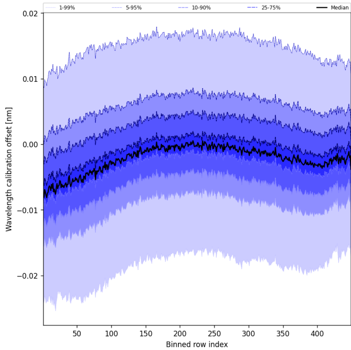
Figure 50: Along track statistics of “Wavelength calibration offset” for 2025-01-18 to 2025-01-19
