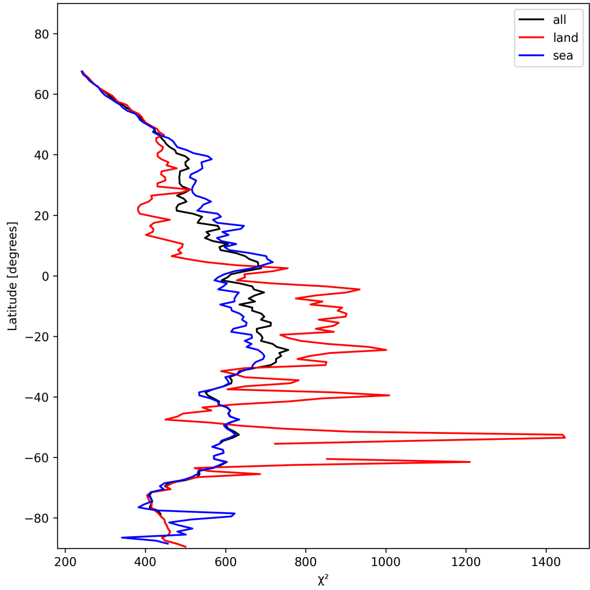
Figure 23: Zonal average of “ \chi^2 ” for 2025-01-18 to 2025-01-19.
