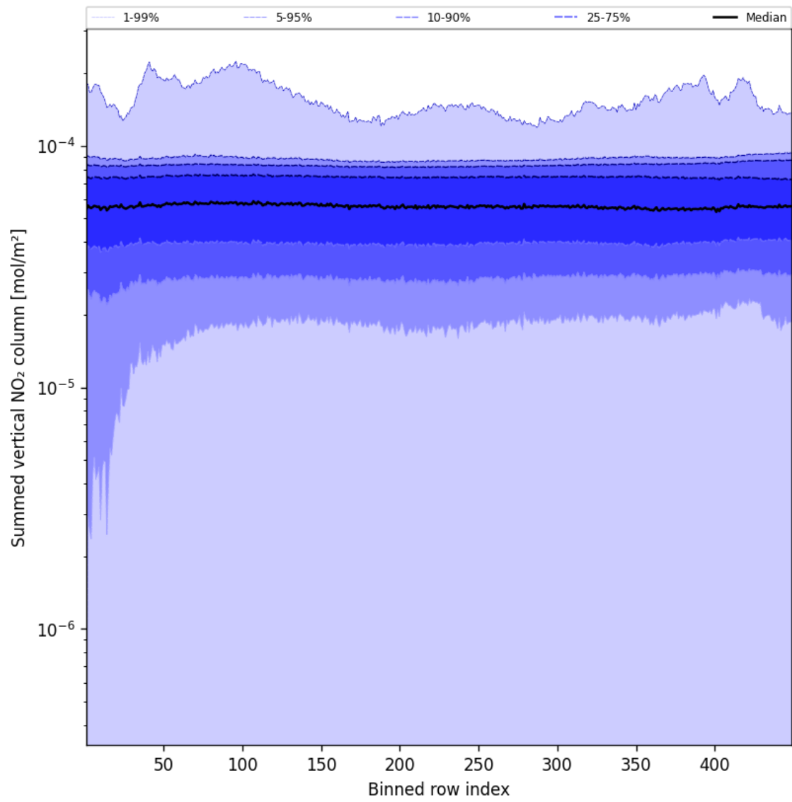
Figure 55: Along track statistics of “Summed vertical NO 2 column” for 2025-01-18 to 2025-01-19
