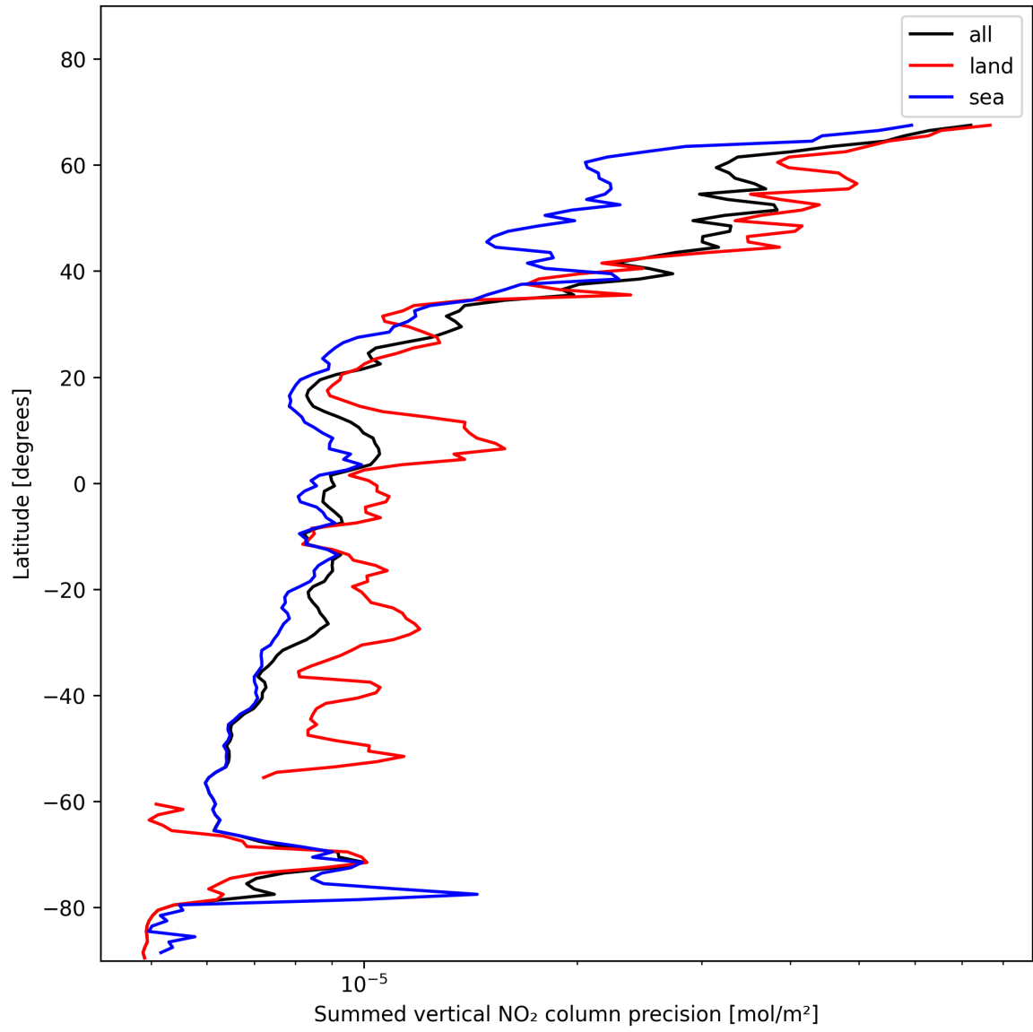
Figure 22: Zonal average of “Summed vertical NO 2 column precision” for 2025-01-18 to 2025-01-19.
