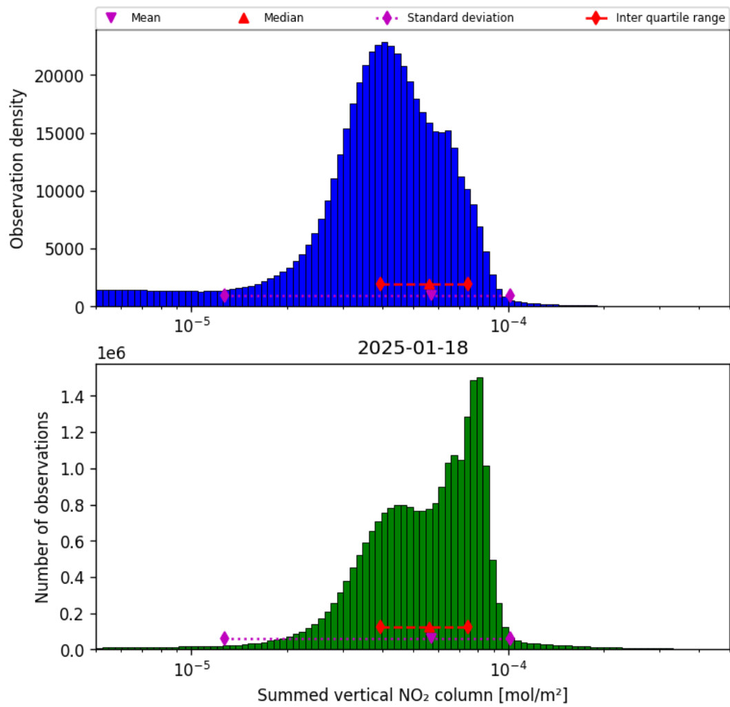
Figure 38: Histogram of “Summed vertical NO 2 column” for 2025-01-18 to 2025-01-19
