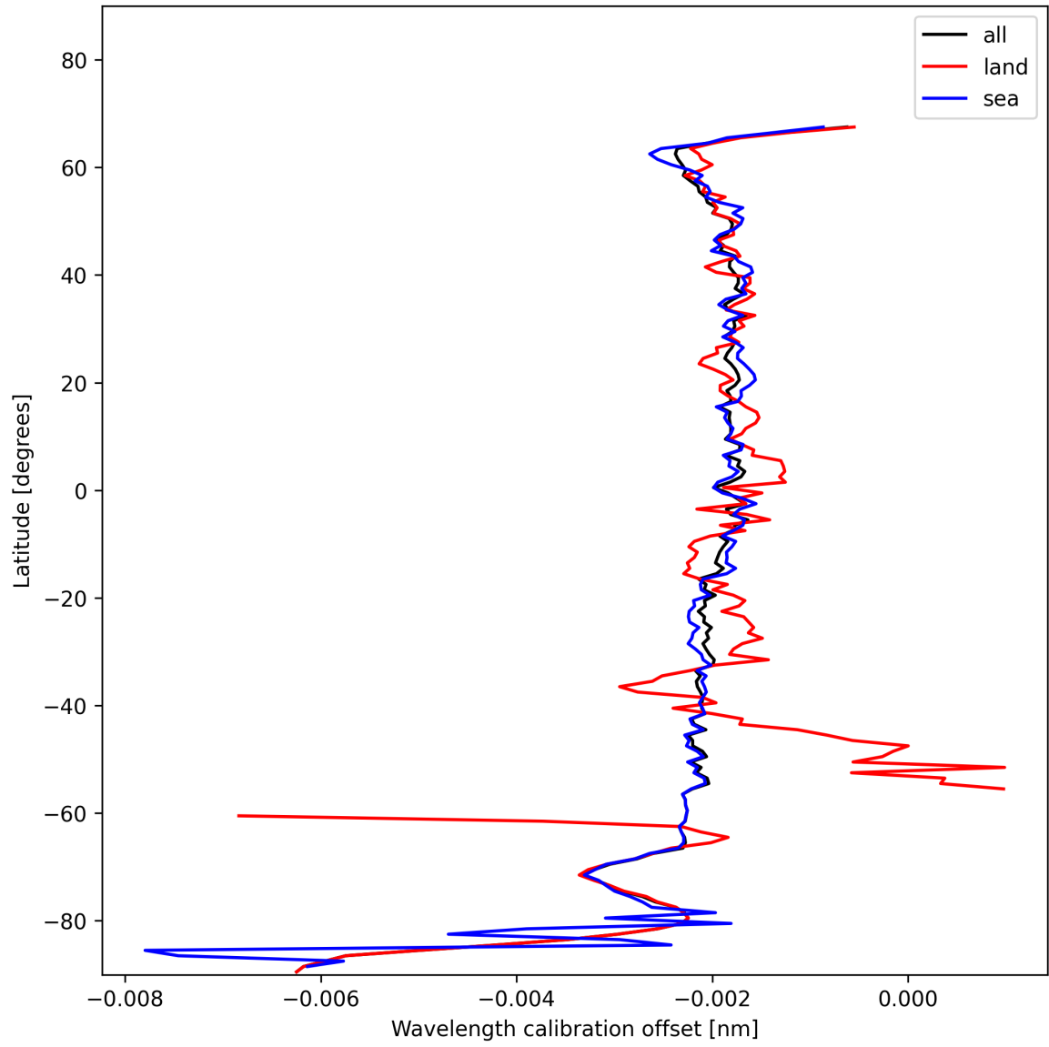
Figure 16: Zonal average of “Wavelength calibration offset” for 2025-01-18 to 2025-01-19.
