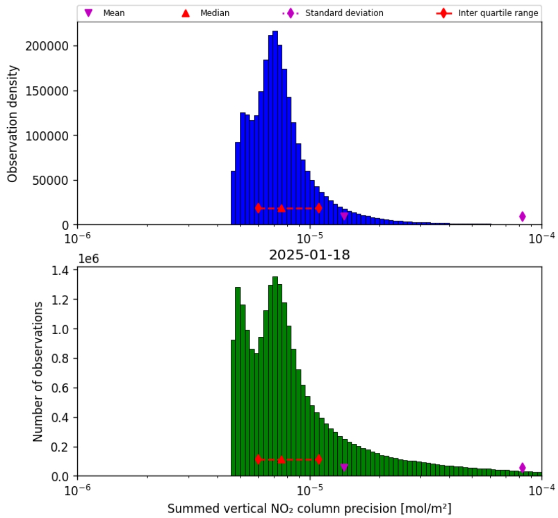
Figure 39: Histogram of “Summed vertical NO 2 column precision” for 2025-01-18 to 2025-01-19
