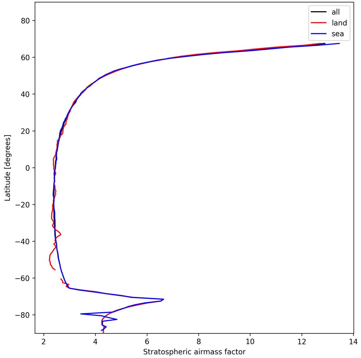
Figure 25: Zonal average of “Stratospheric air mass factor” for 2025-01-18 to 2025-01-19.
