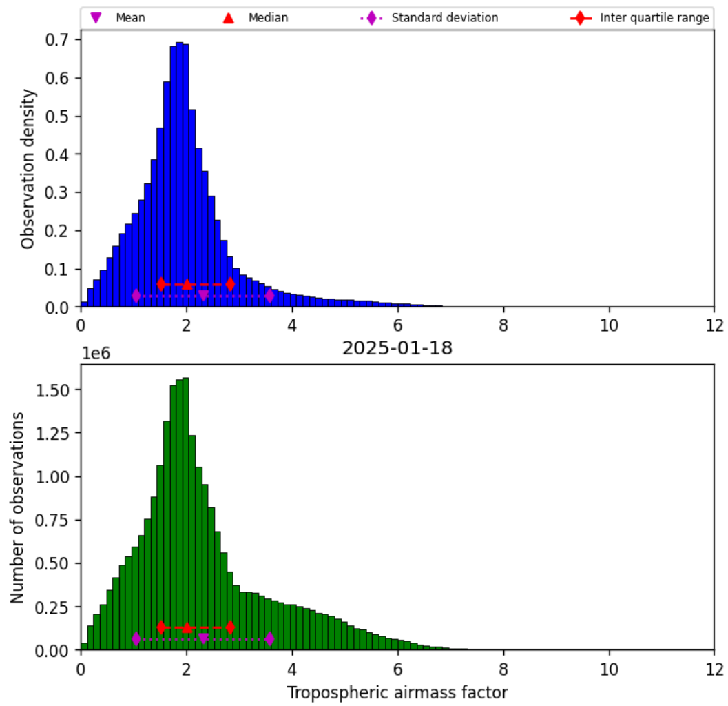
Figure 29: Histogram of “Tropospheric airmass factor” for 2025-01-18 to 2025-01-19
