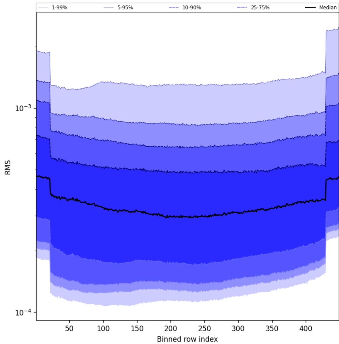
Figure 58: Along track statistics of “RMS” for 2025-01-18 to 2025-01-19
