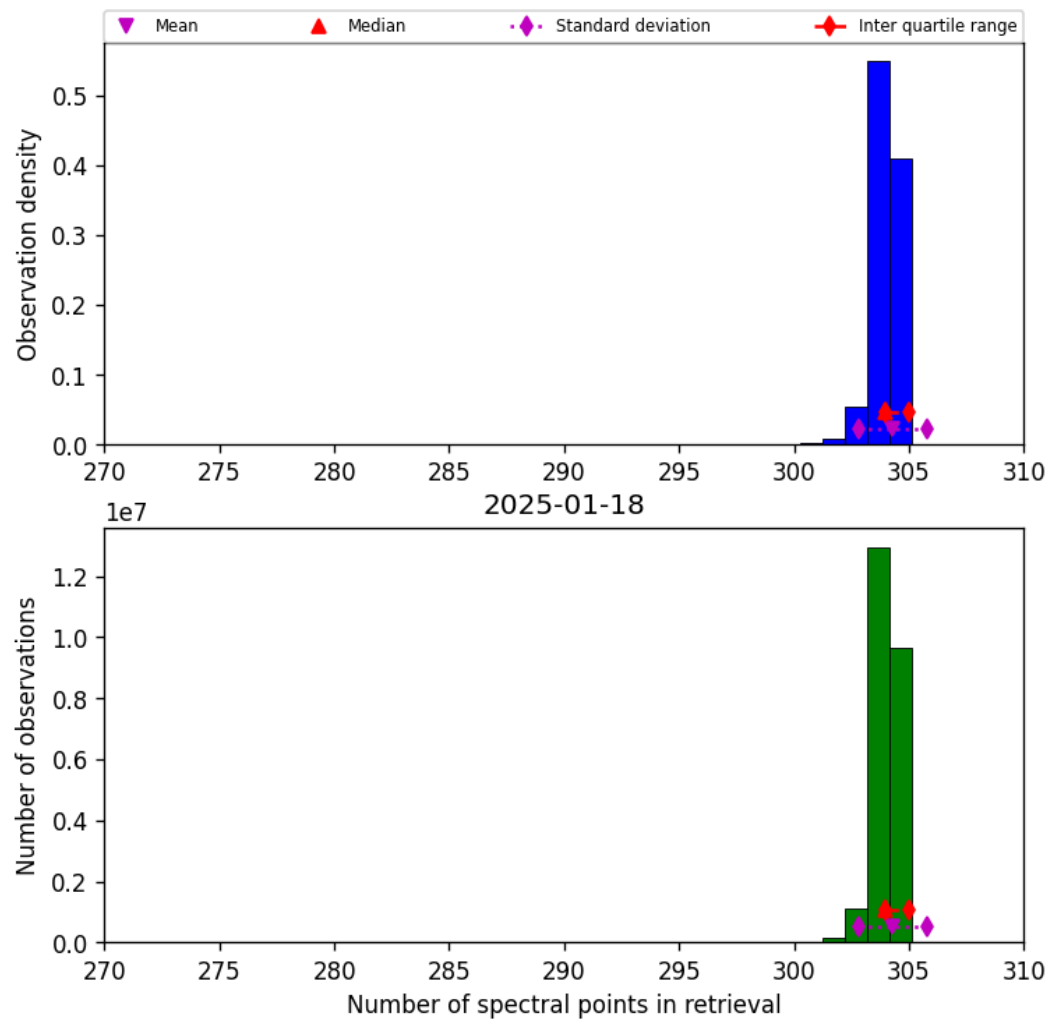
Figure 31: Histogram of “Number of spectral points in retrieval” for 2025-01-18 to 2025-01-19
