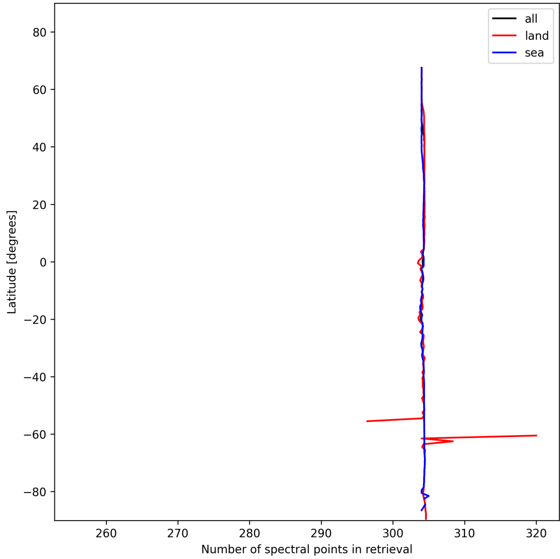
Figure 14: Zonal average of “Number of spectral points in retrieval” for 2025-01-19 to 2025-01-20.
