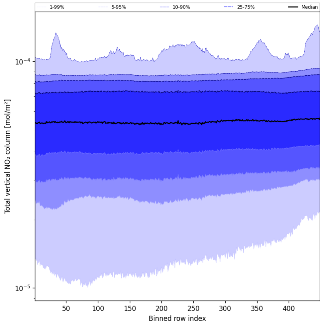
Figure 53: Along track statistics of “Total vertical NO 2 column” for 2025-01-19 to 2025-01-20
