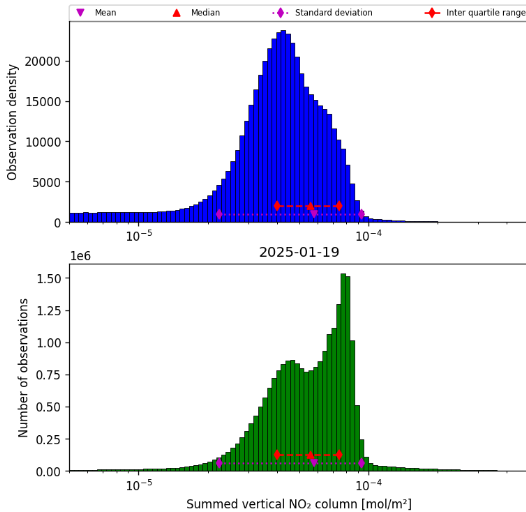
Figure 38: Histogram of “Summed vertical NO 2 column” for 2025-01-19 to 2025-01-20
