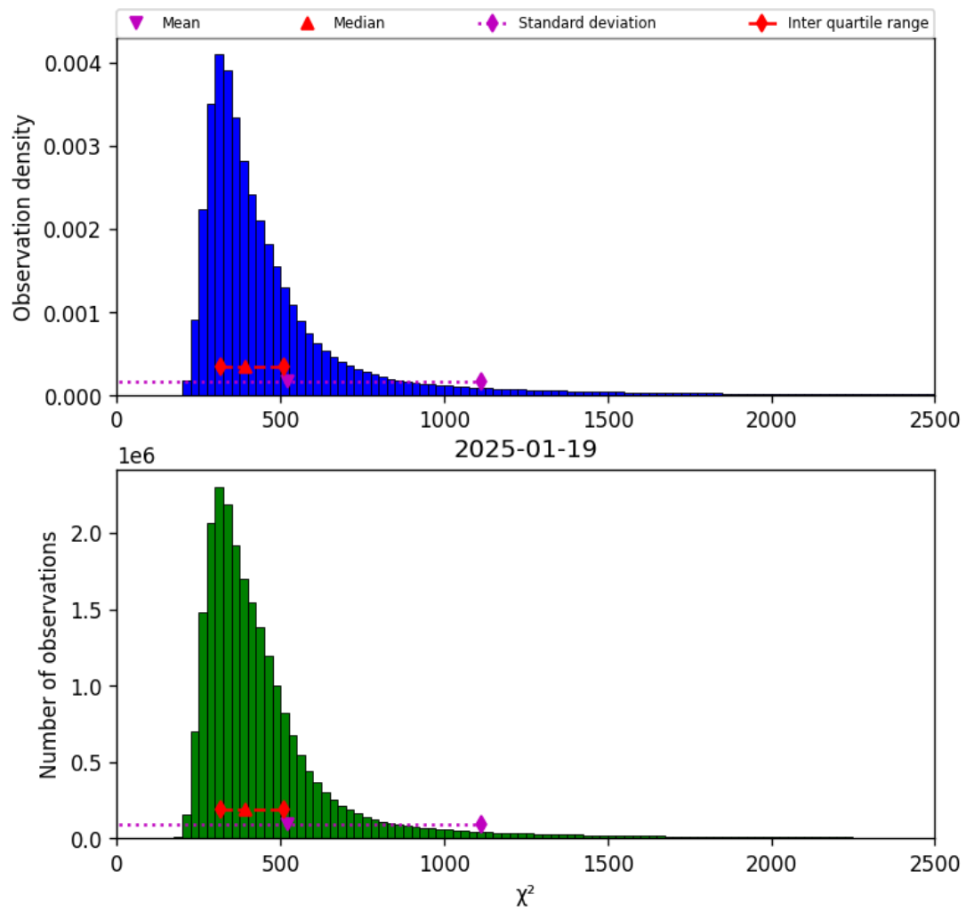
Figure 40: Histogram of “ \chi^2 ” for 2025-01-19 to 2025-01-20
