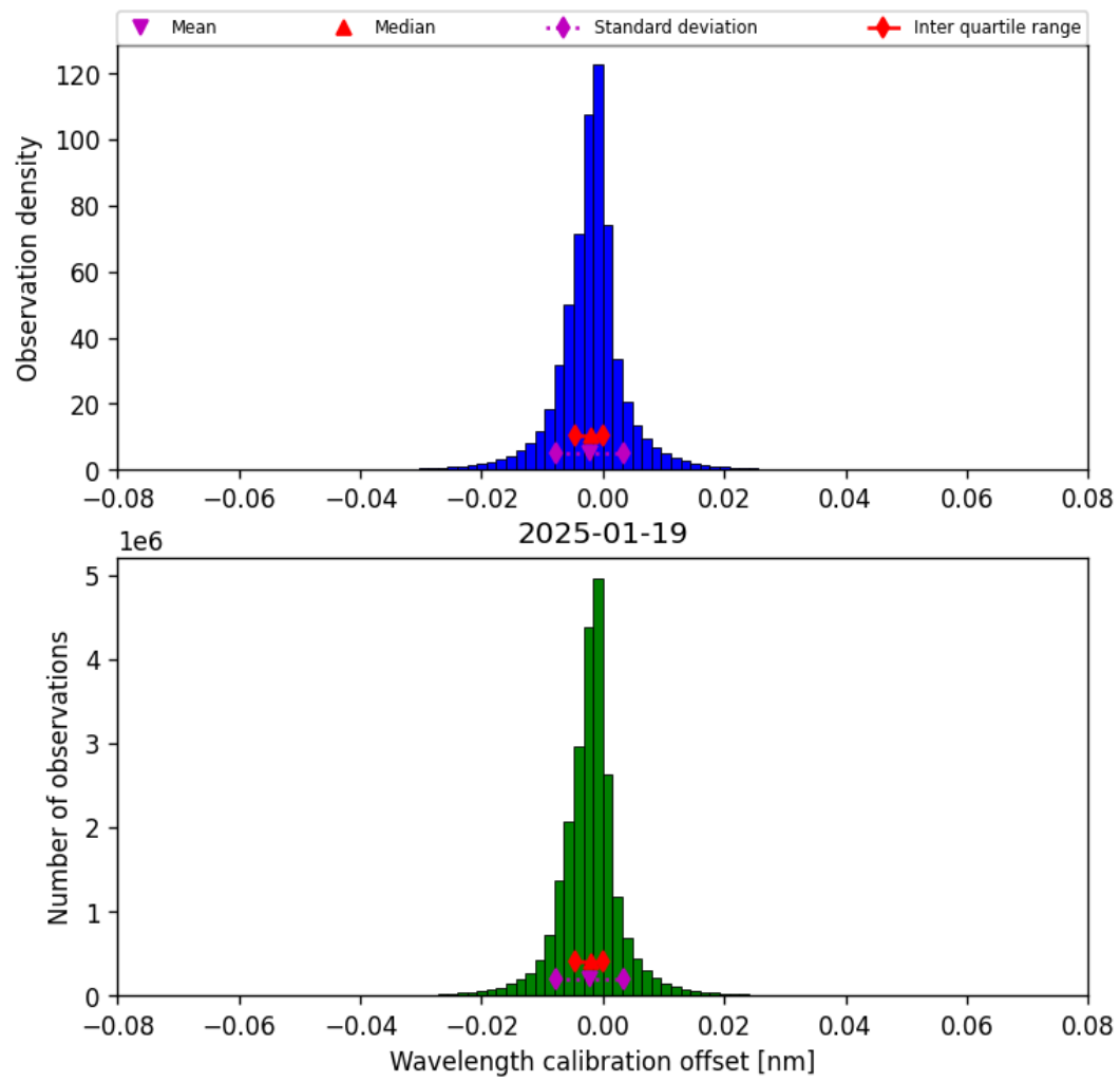
Figure 33: Histogram of “Wavelength calibration offset” for 2025-01-19 to 2025-01-20
