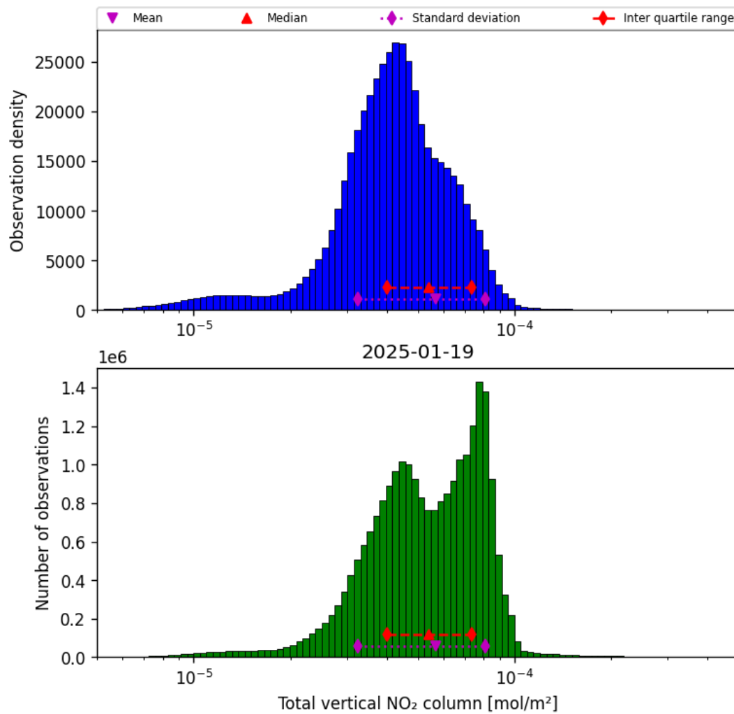
Figure 36: Histogram of “Total vertical NO 2 column” for 2025-01-19 to 2025-01-20
