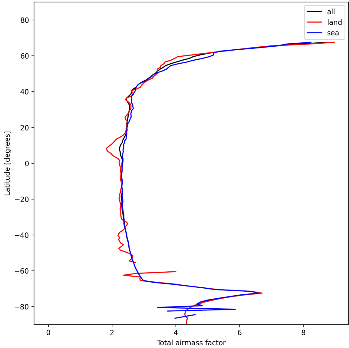
Figure 13: Zonal average of “Total airmass factor” for 2025-01-19 to 2025-01-20.
