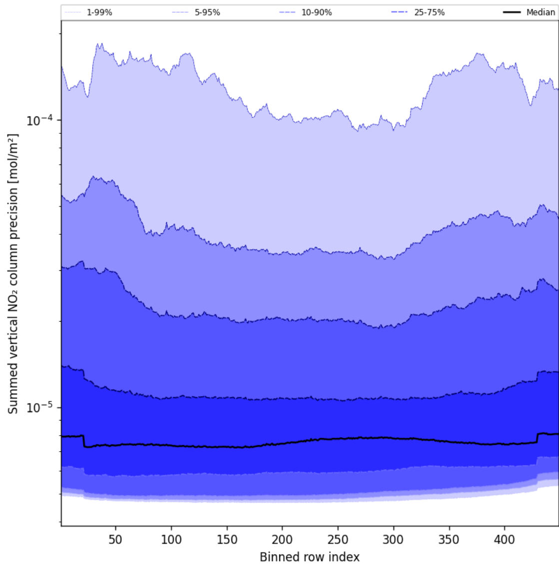
Figure 56: Along track statistics of “Summed vertical NO 2 column precision” for 2025-01-19 to 2025-01-20
