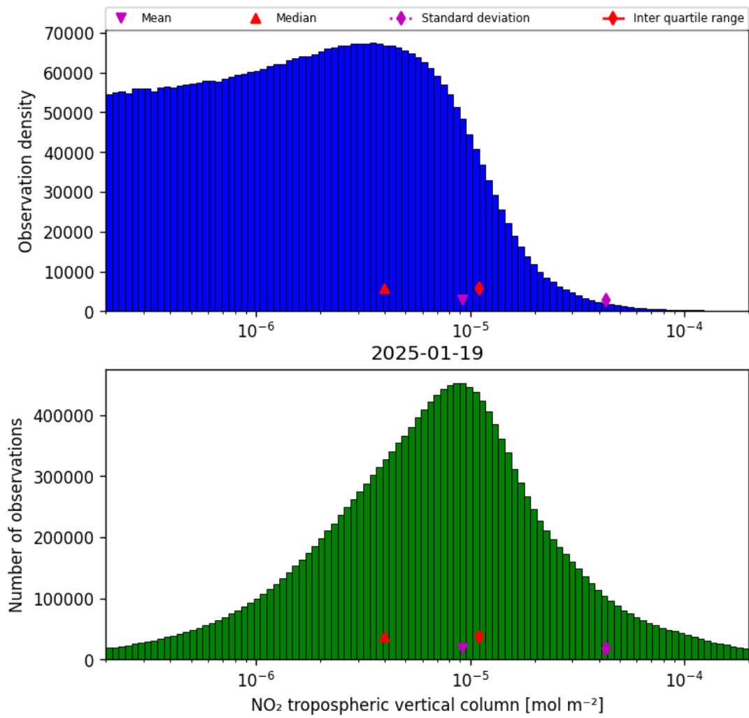
Figure 27: Histogram of “NO 2 tropospheric vertical column” for 2025-01-19 to 2025-01-20
