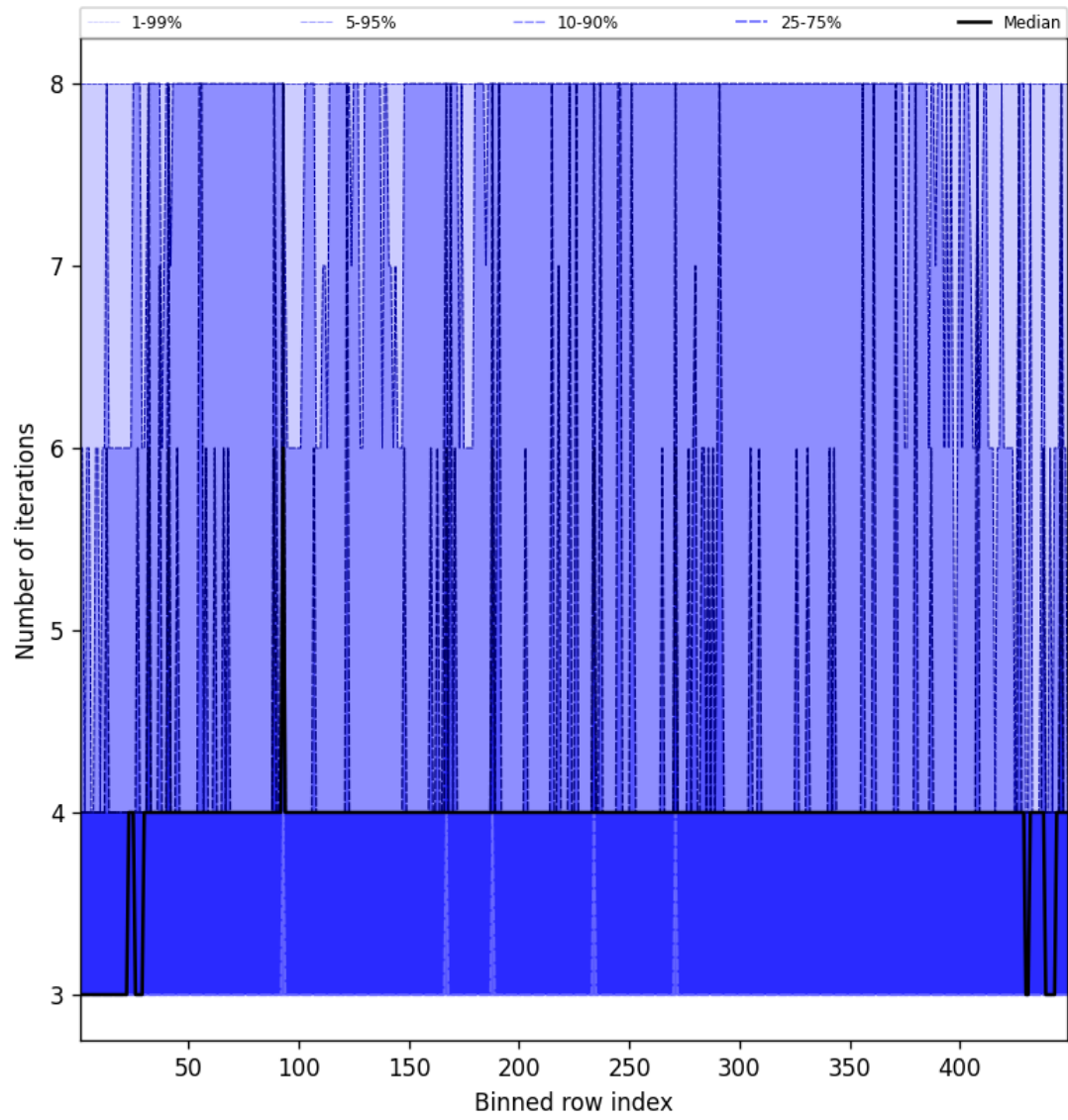
Figure 49: Along track statistics of “Number of iterations” for 2025-01-19 to 2025-01-20
