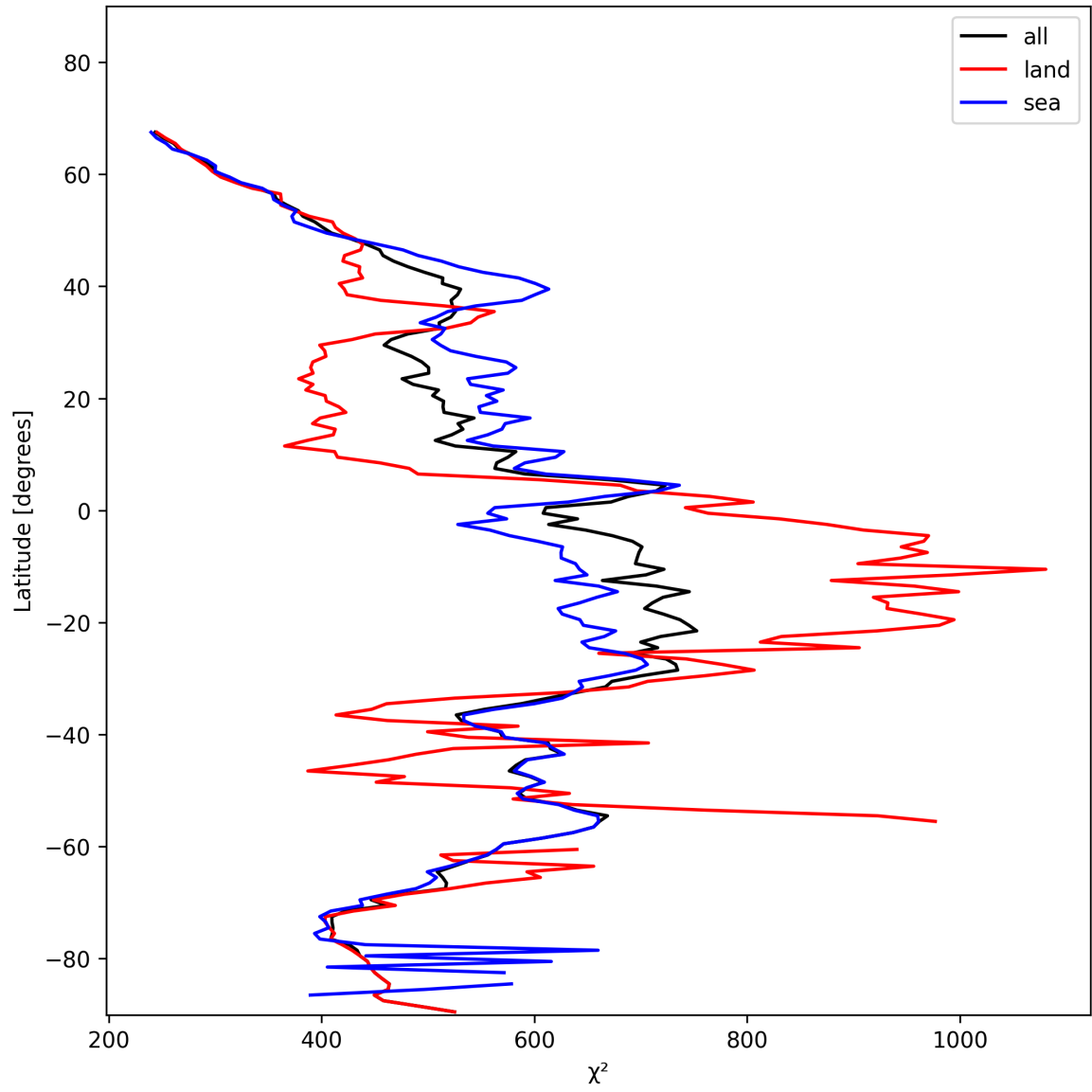
Figure 23: Zonal average of “ \chi^2 ” for 2025-01-19 to 2025-01-20.
