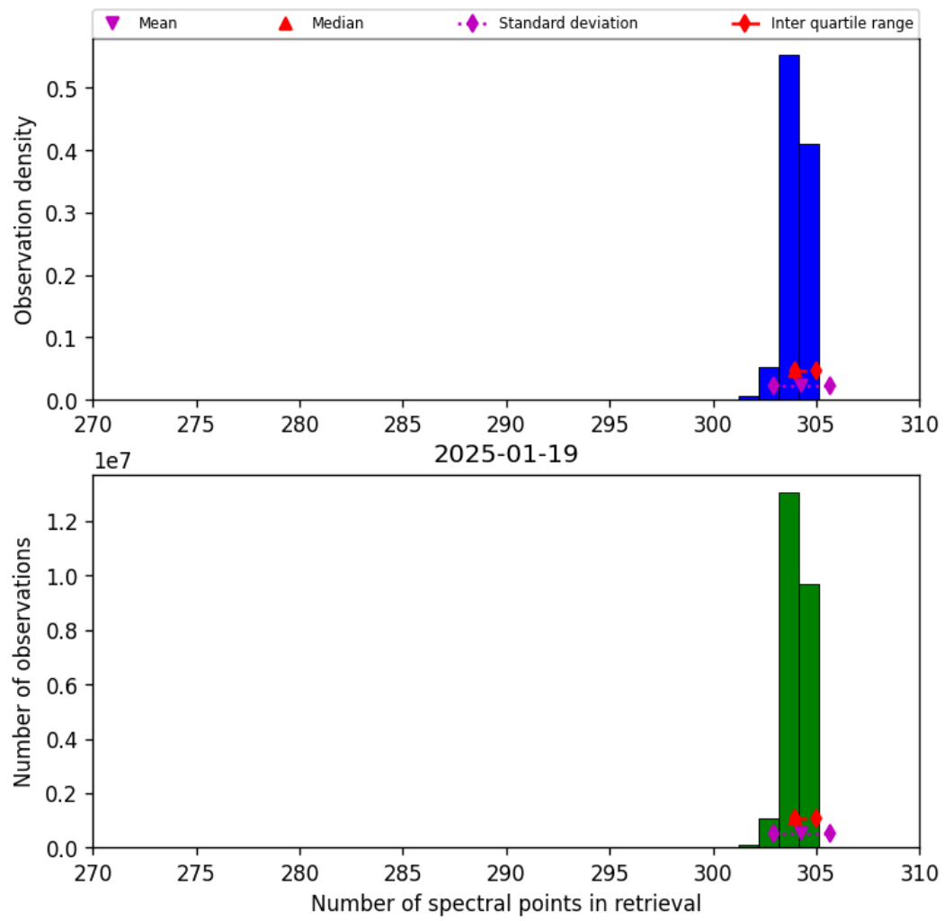
Figure 31: Histogram of “Number of spectral points in retrieval” for 2025-01-19 to 2025-01-20
