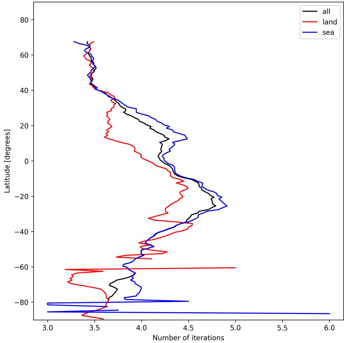
Figure 15: Zonal average of “Number of iterations” for 2025-01-19 to 2025-01-20.
