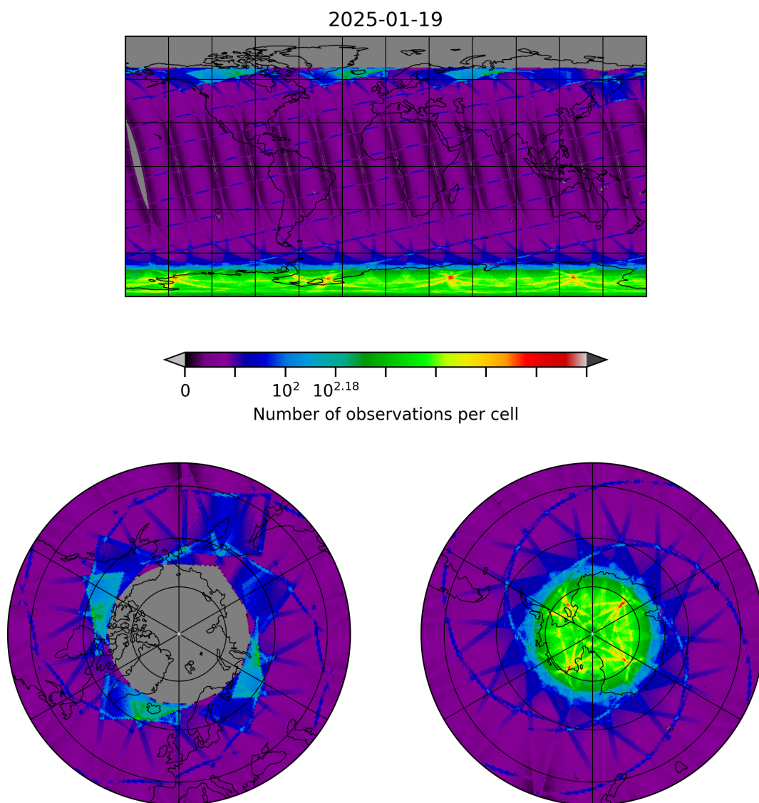
Figure 8: Map of the number of observations for 2025-01-19 to 2025-01-20
