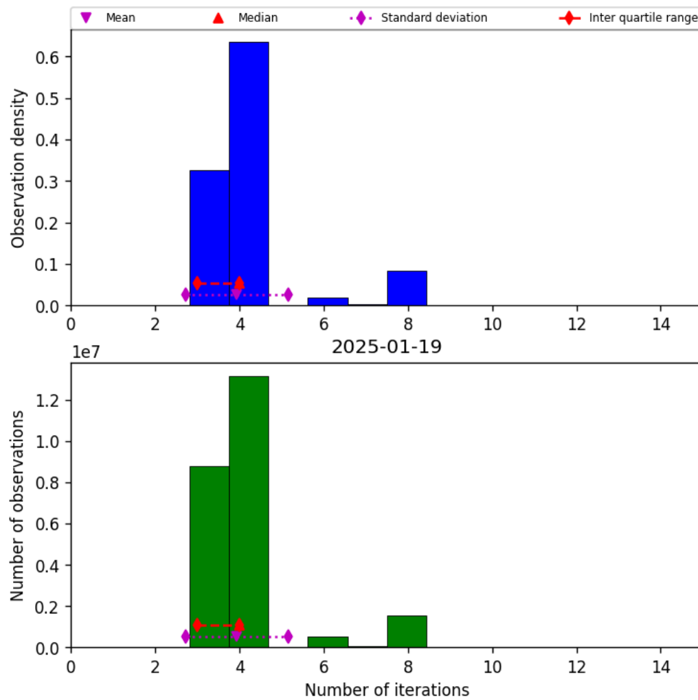
Figure 32: Histogram of “Number of iterations” for 2025-01-19 to 2025-01-20
