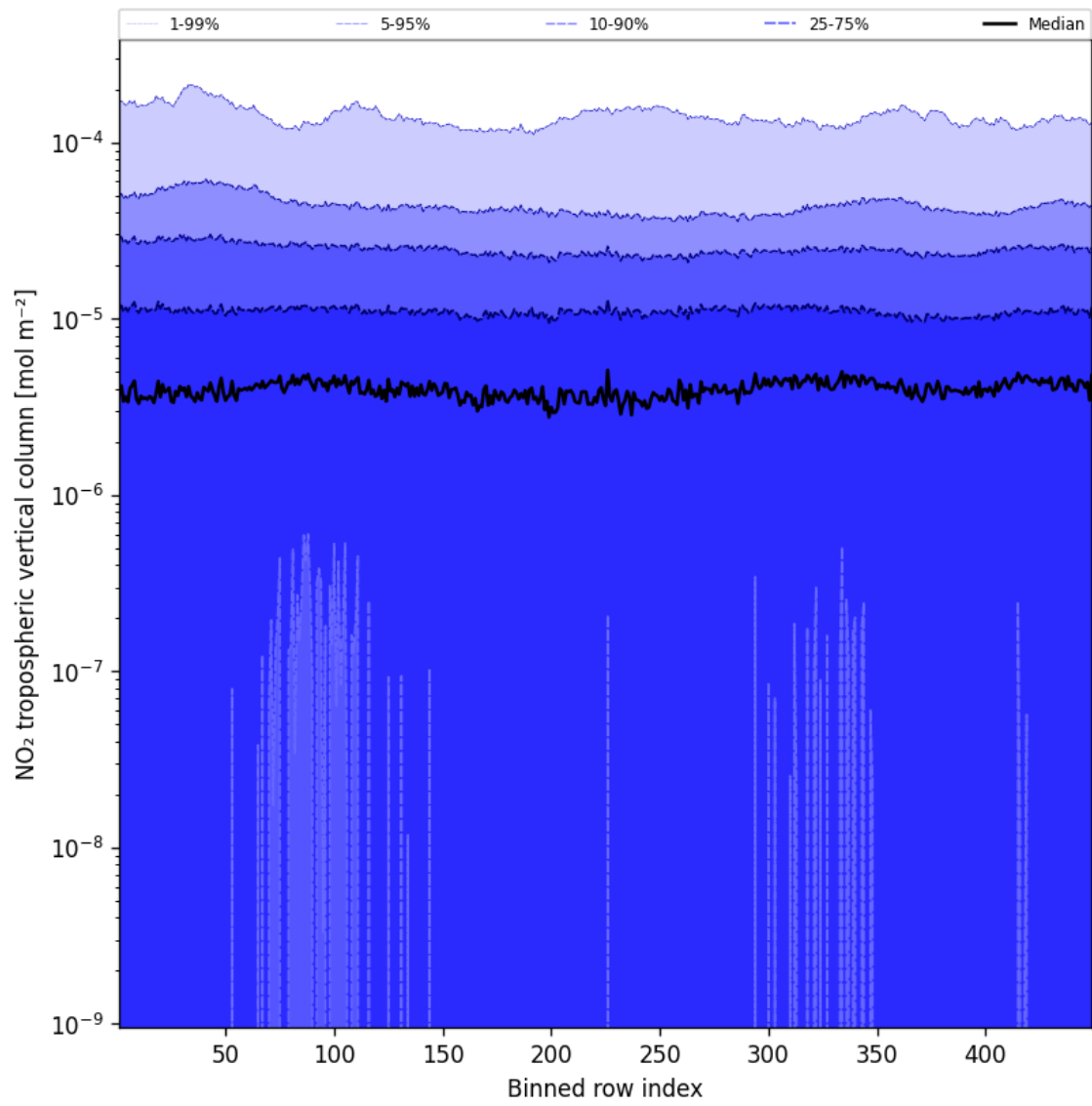
Figure 44: Along track statistics of “NO 2 tropospheric vertical column” for 2025-01-19 to 2025-01-20
