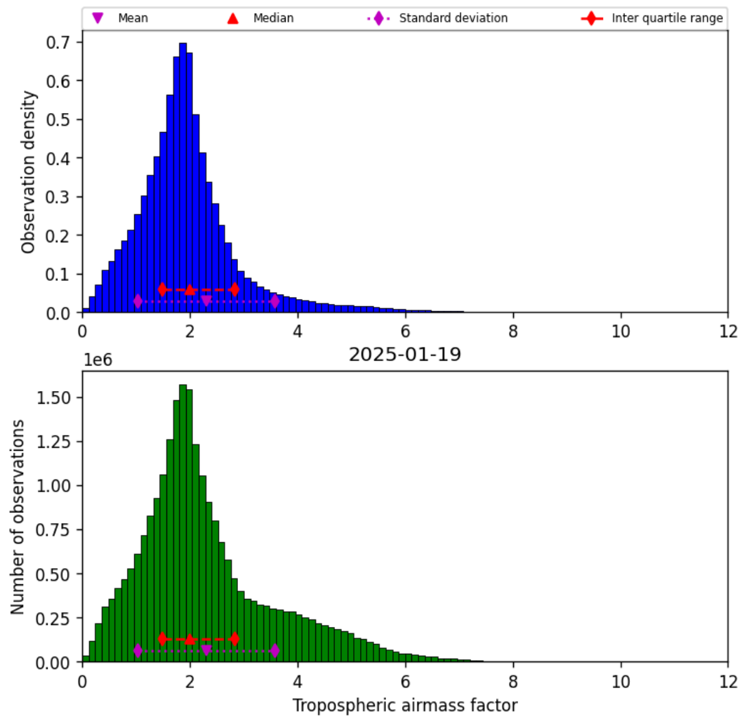
Figure 29: Histogram of “Tropospheric airmass factor” for 2025-01-19 to 2025-01-20
