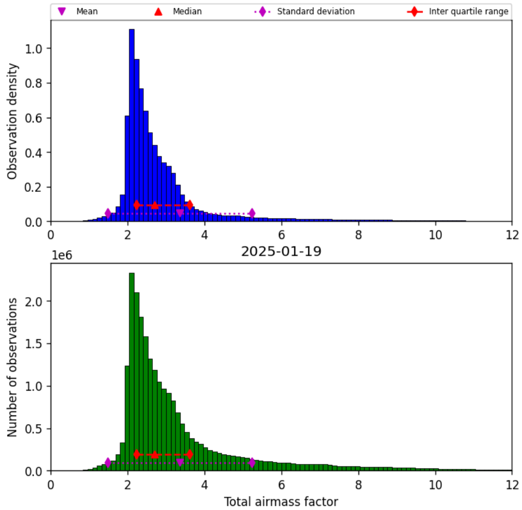
Figure 30: Histogram of “Total airmass factor” for 2025-01-19 to 2025-01-20
