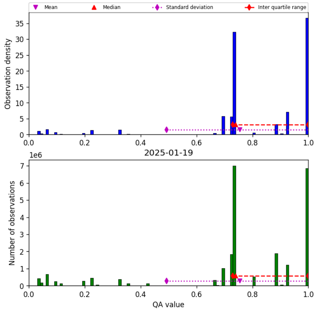
Figure 26: Histogram of “QA value” for 2025-01-19 to 2025-01-20
