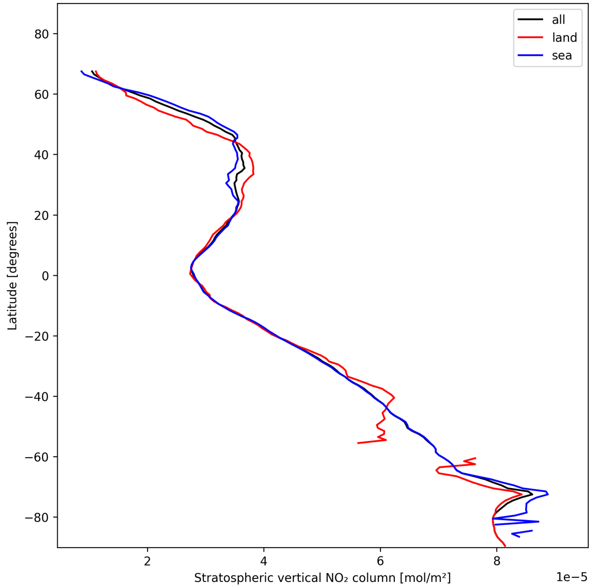
Figure 17: Zonal average of “Stratospheric vertical NO 2 column” for 2025-01-19 to 2025-01-20.
