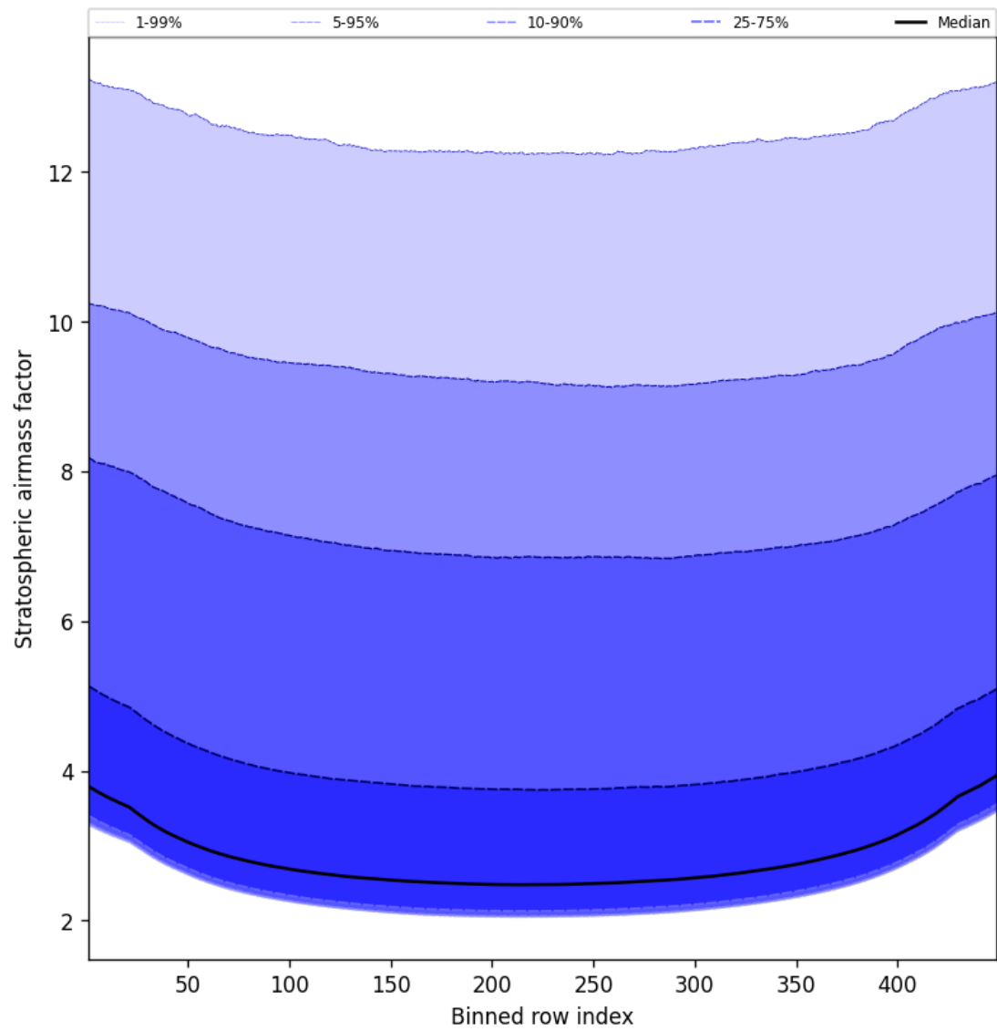
Figure 59: Along track statistics of “Stratospheric airmass factor” for 2025-01-19 to 2025-01-20
