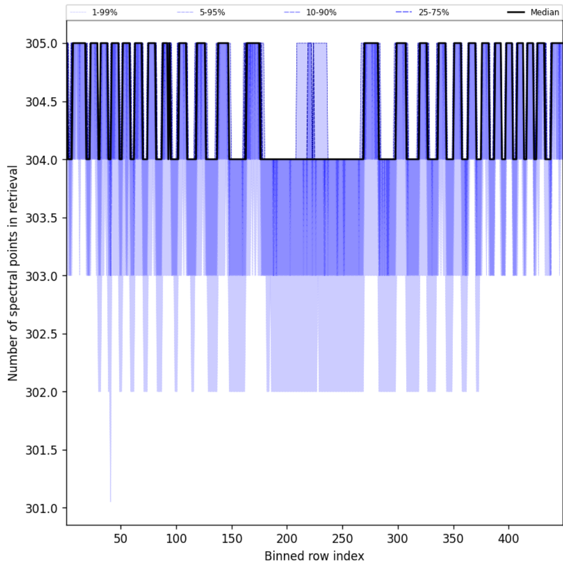
Figure 48: Along track statistics of “Number of spectral points in retrieval” for 2025-01-19 to 2025-01-20
