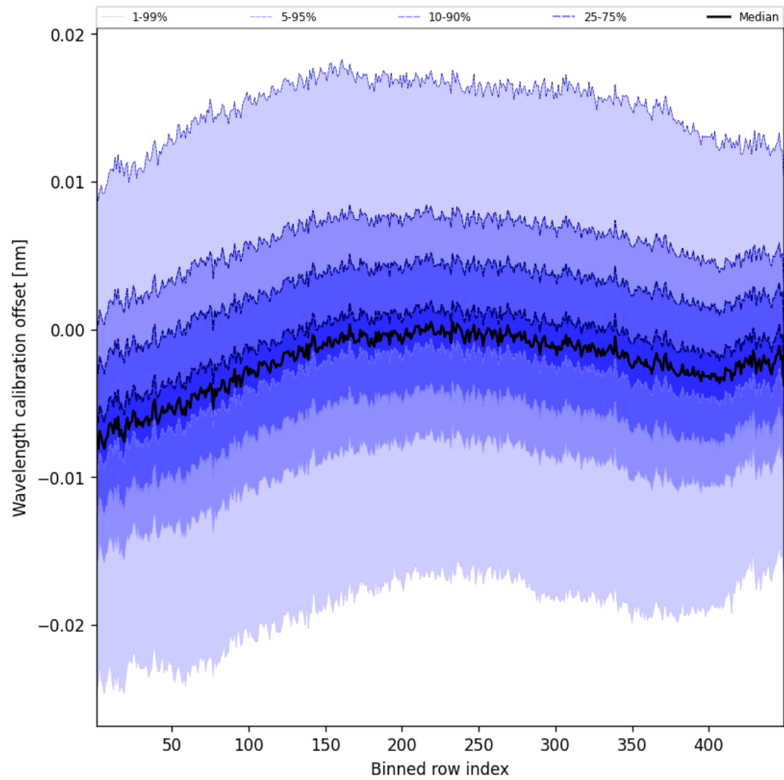
Figure 50: Along track statistics of “Wavelength calibration offset” for 2025-01-19 to 2025-01-20
