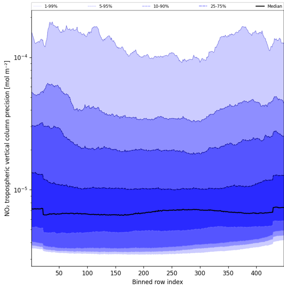
Figure 45: Along track statistics of “NO 2 tropospheric vertical column precision” for 2025-01-19 to 2025-01-20
