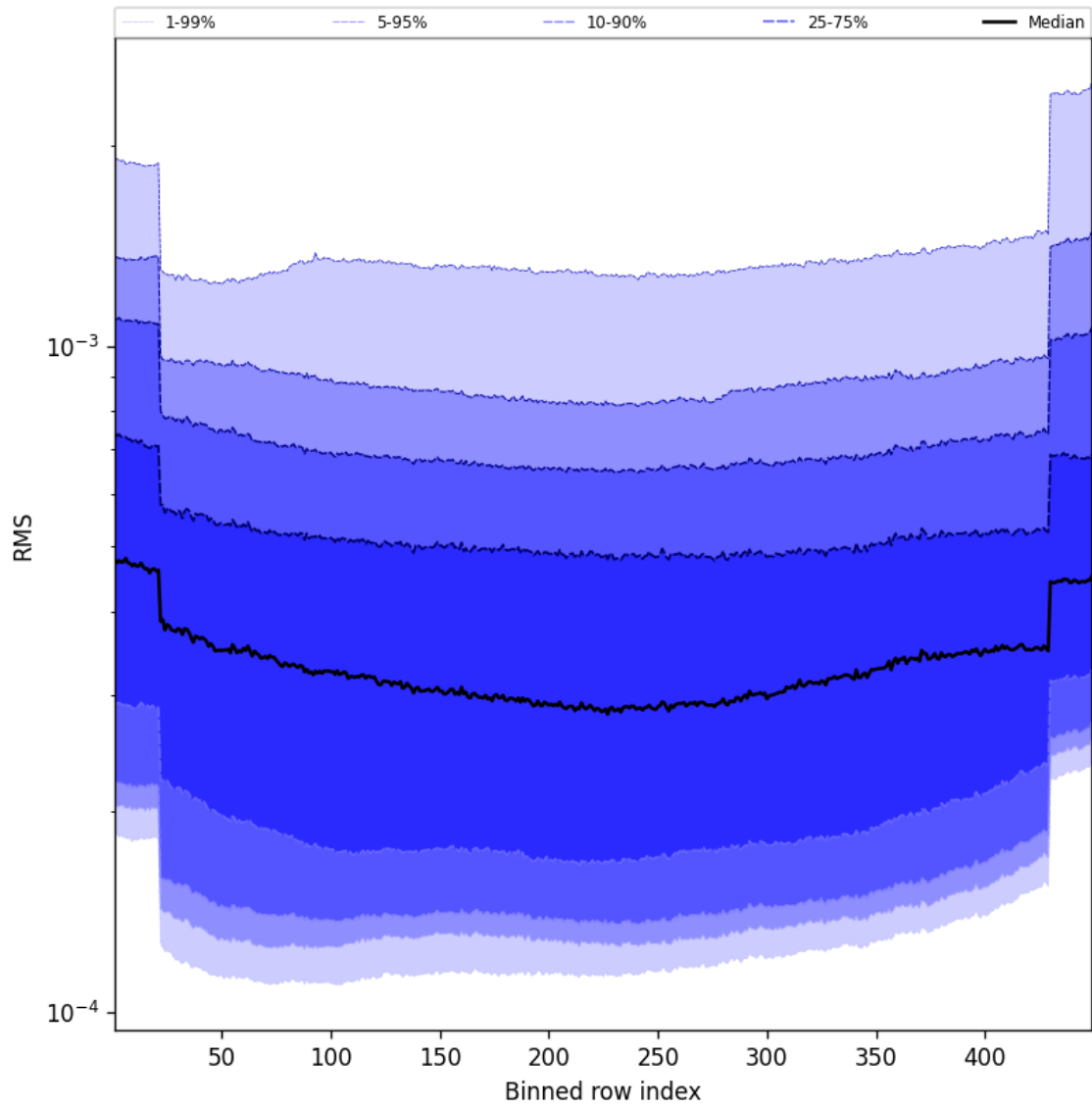
Figure 58: Along track statistics of “RMS” for 2025-01-19 to 2025-01-20
