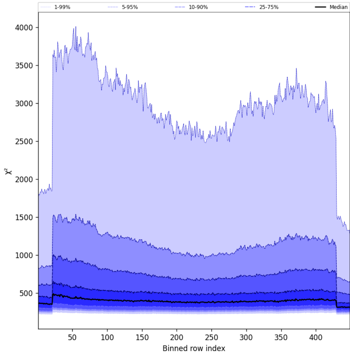
Figure 57: Along track statistics of “ \chi^2 ” for 2025-01-19 to 2025-01-20
