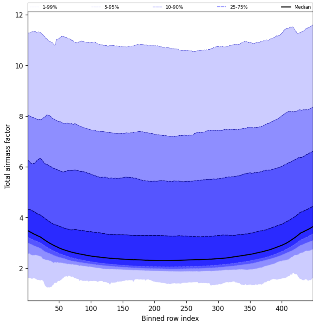
Figure 47: Along track statistics of “Total airmass factor” for 2025-01-19 to 2025-01-20
