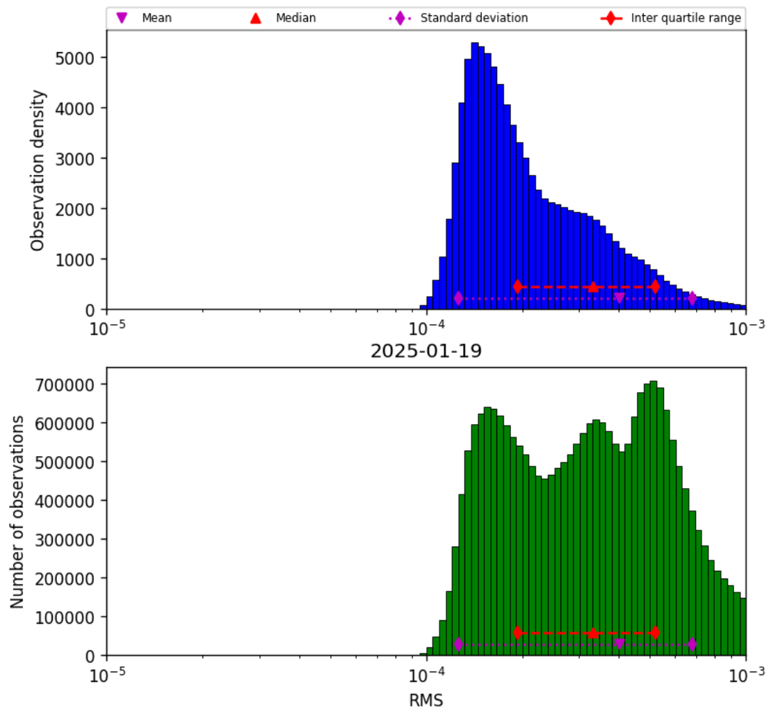
Figure 41: Histogram of “RMS” for 2025-01-19 to 2025-01-20
