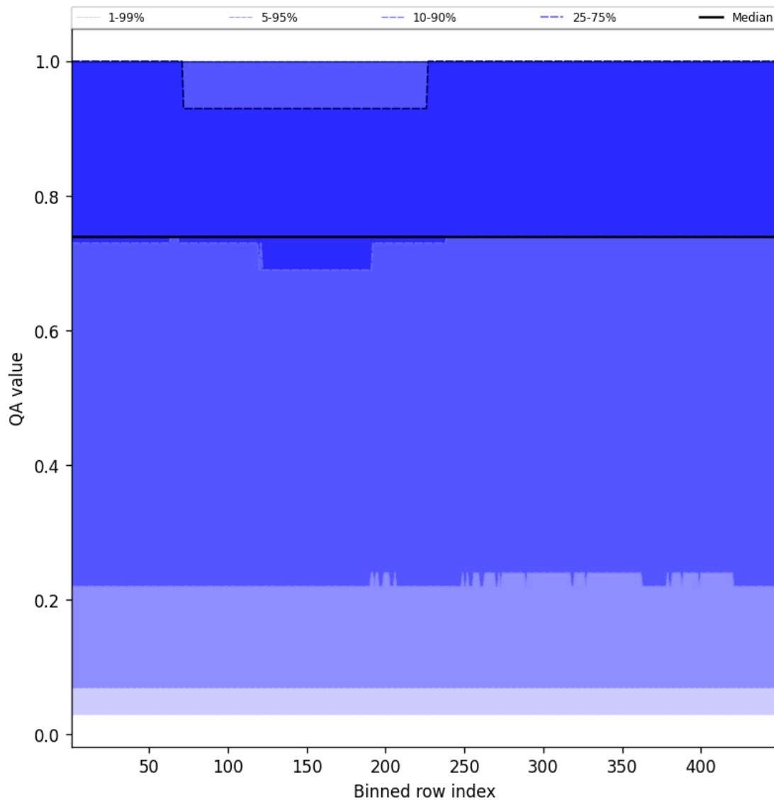
Figure 43: Along track statistics of "QA value" for 2025-01-19 to 2025-01-20
