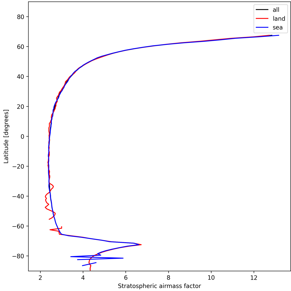
Figure 25: Zonal average of “Stratospheric air mass factor” for 2025-01-19 to 2025-01-20.
