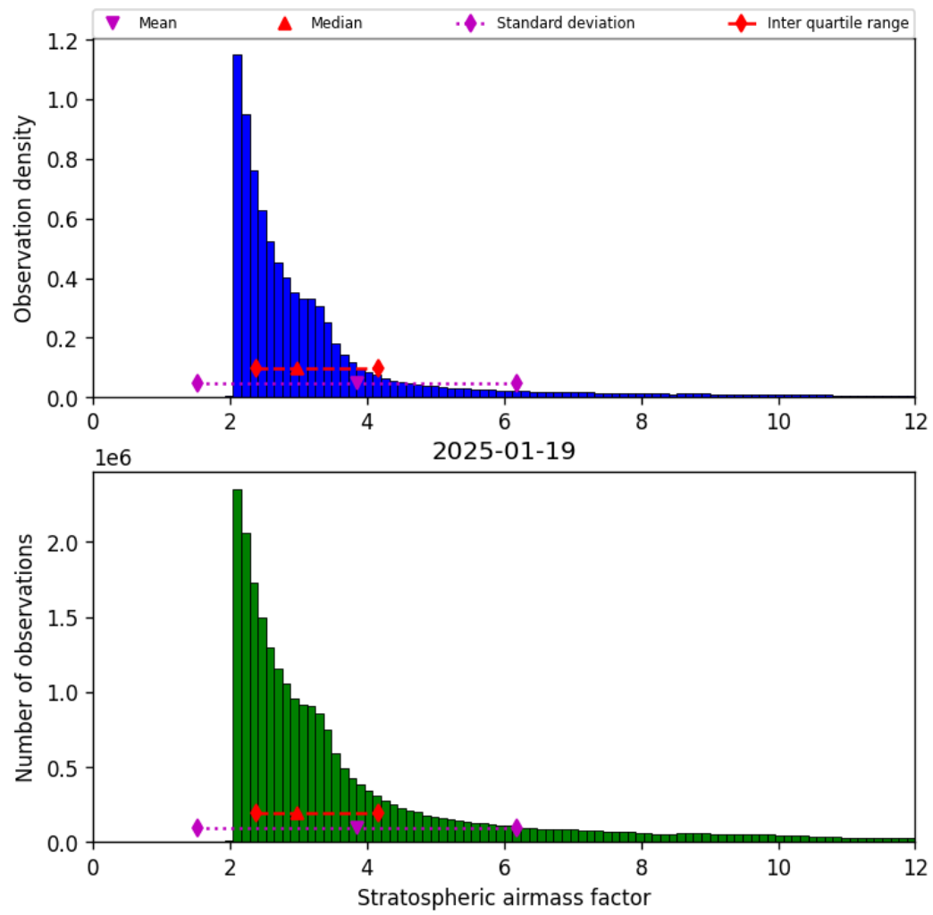
Figure 42: Histogram of “Stratospheric airmass factor” for 2025-01-19 to 2025-01-20
