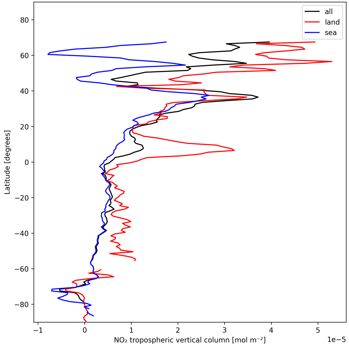
Figure 10: Zonal average of “NO 2 tropospheric vertical column” for 2025-01-19 to 2025-01-20.
