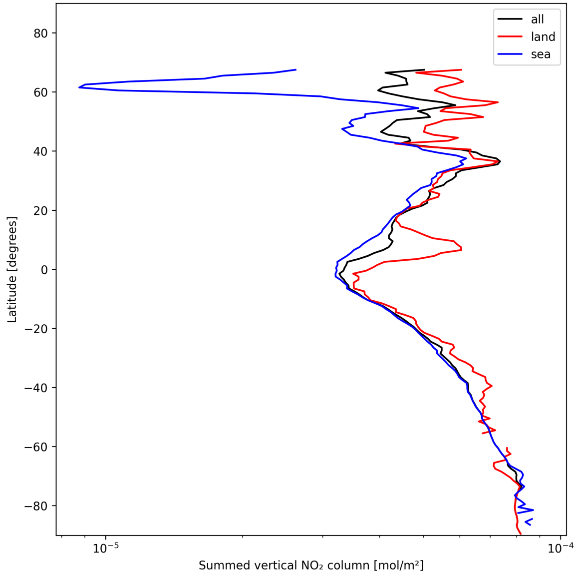
Figure 21: Zonal average of “Summed vertical NO 2 column” for 2025-01-19 to 2025-01-20.
