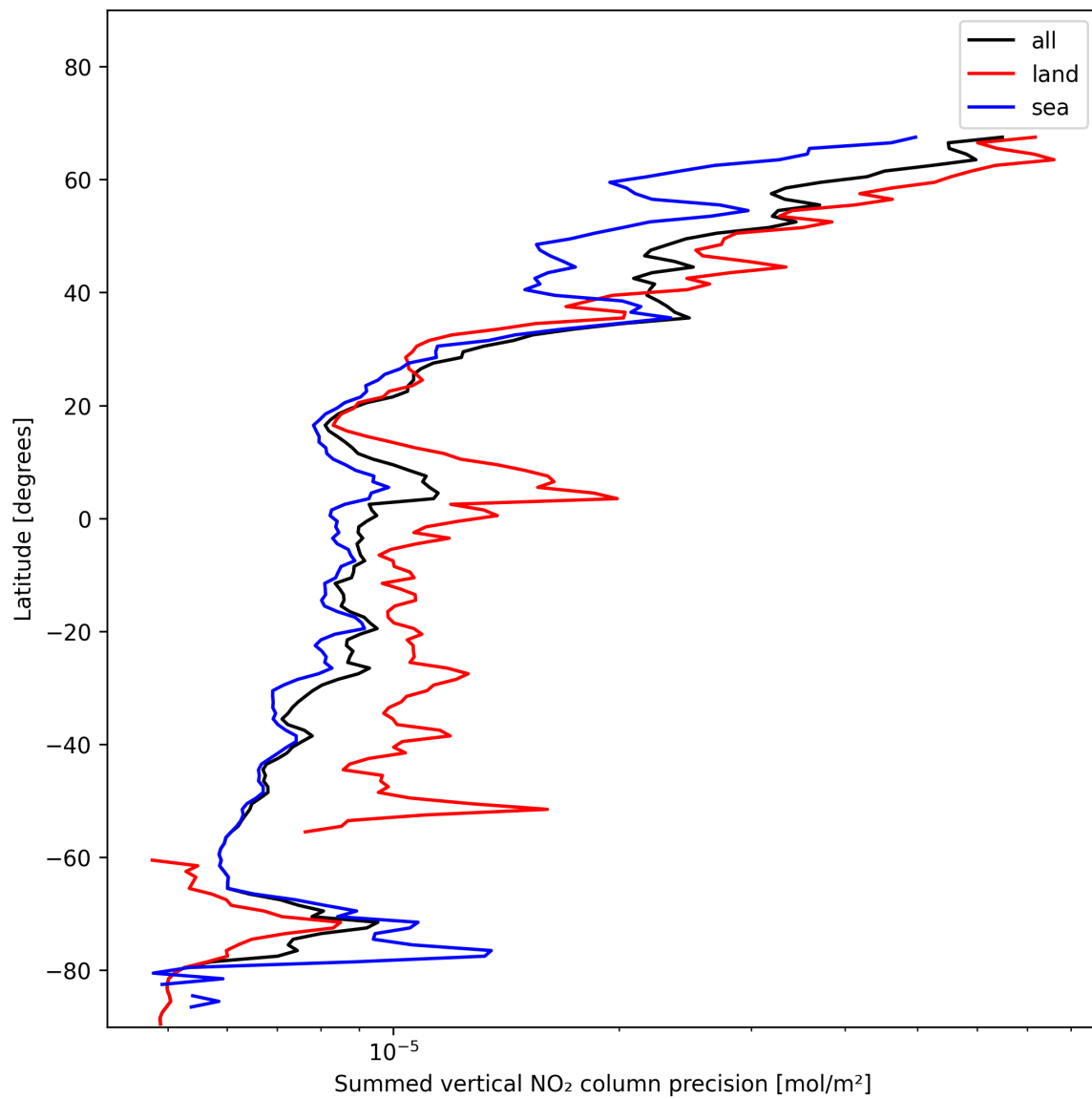
Figure 22: Zonal average of “Summed vertical NO 2 column precision” for 2025-01-19 to 2025-01-20.
