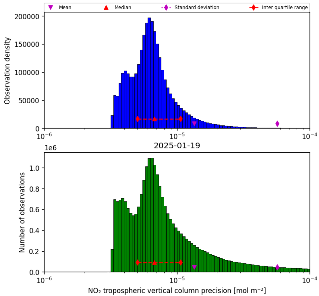
Figure 28: Histogram of “NO 2 tropospheric vertical column precision” for 2025-01-19 to 2025-01-20
