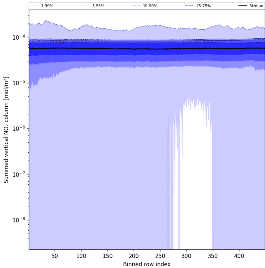
Figure 55: Along track statistics of “Summed vertical NO 2 column” for 2025-01-19 to 2025-01-20
