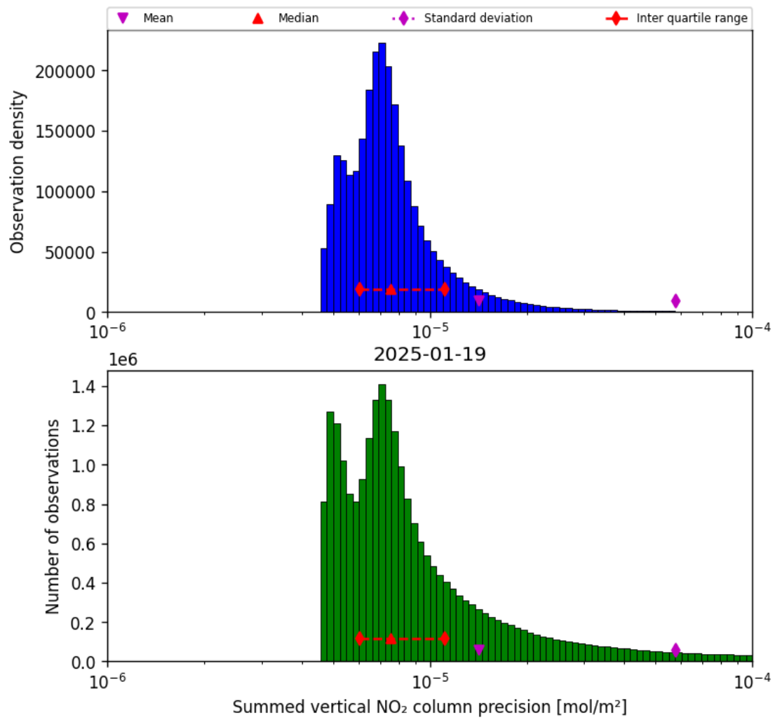
Figure 39: Histogram of "Summed vertical NO 2 column precision" for 2025-01-19 to 2025-01-20
