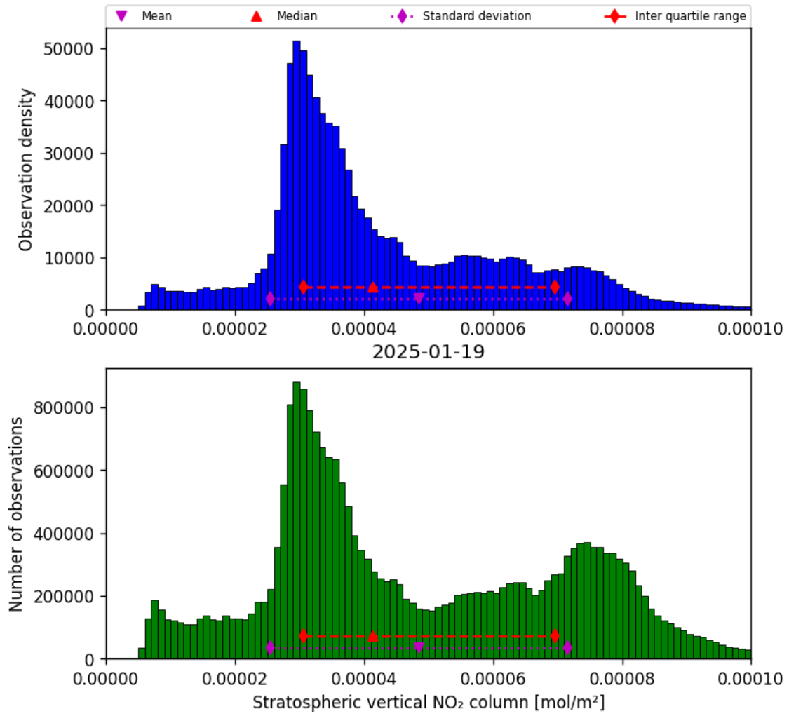
Figure 34: Histogram of “Stratospheric vertical NO 2 column” for 2025-01-19 to 2025-01-20
