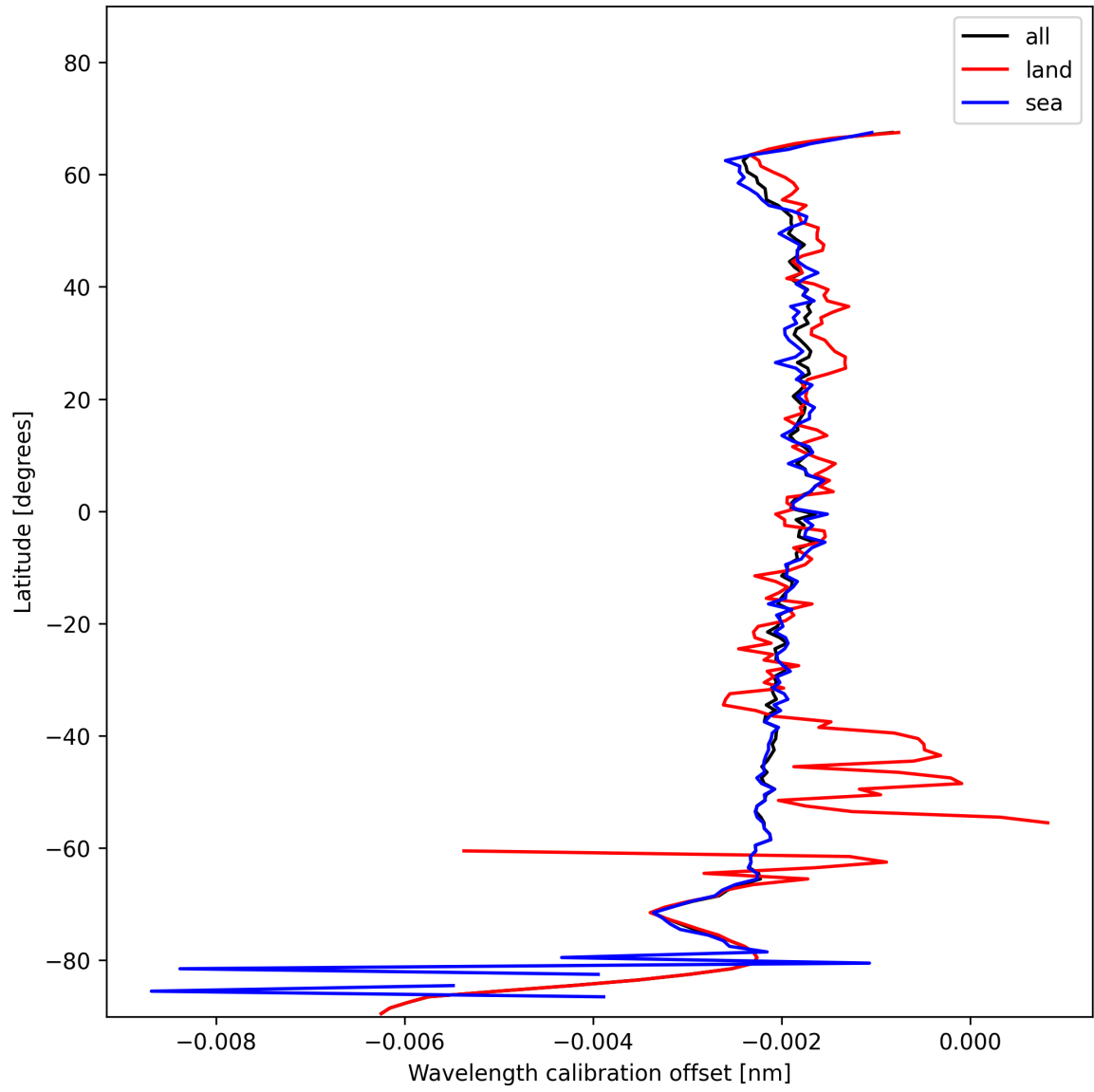
Figure 16: Zonal average of “Wavelength calibration offset” for 2025-01-19 to 2025-01-20.
