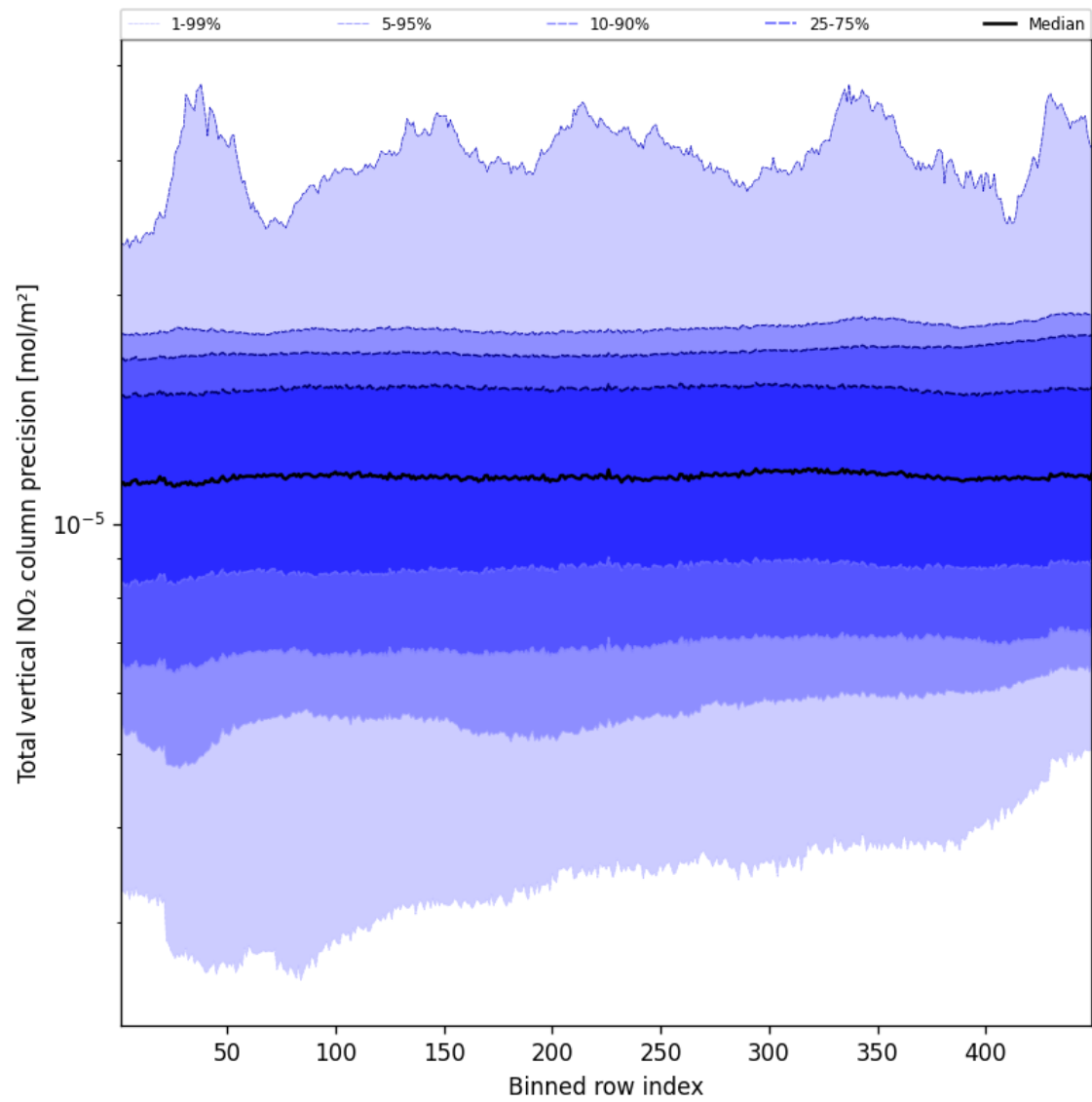
Figure 54: Along track statistics of “Total vertical NO 2 column precision” for 2025-01-19 to 2025-01-20
