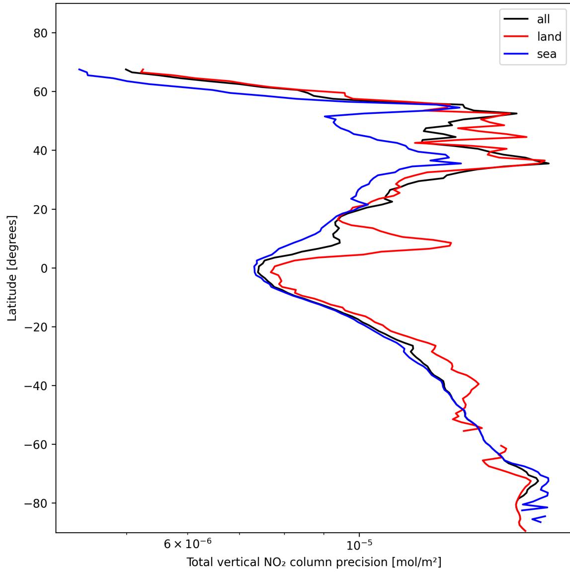
Figure 20: Zonal average of “Total vertical NO 2 column precision” for 2025-01-19 to 2025-01-20.
