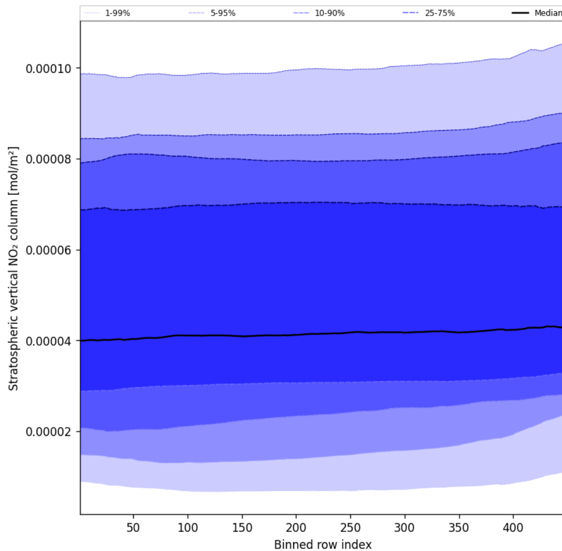
Figure 51: Along track statistics of “Stratospheric vertical NO 2 column” for 2025-01-19 to 2025-01-20
