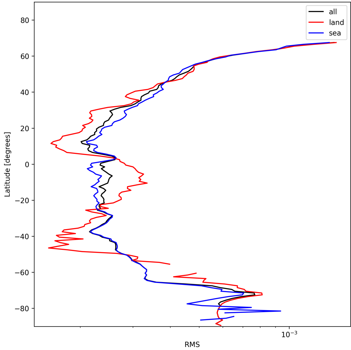
Figure 24: Zonal average of “RMS” for 2025-01-19 to 2025-01-20.
