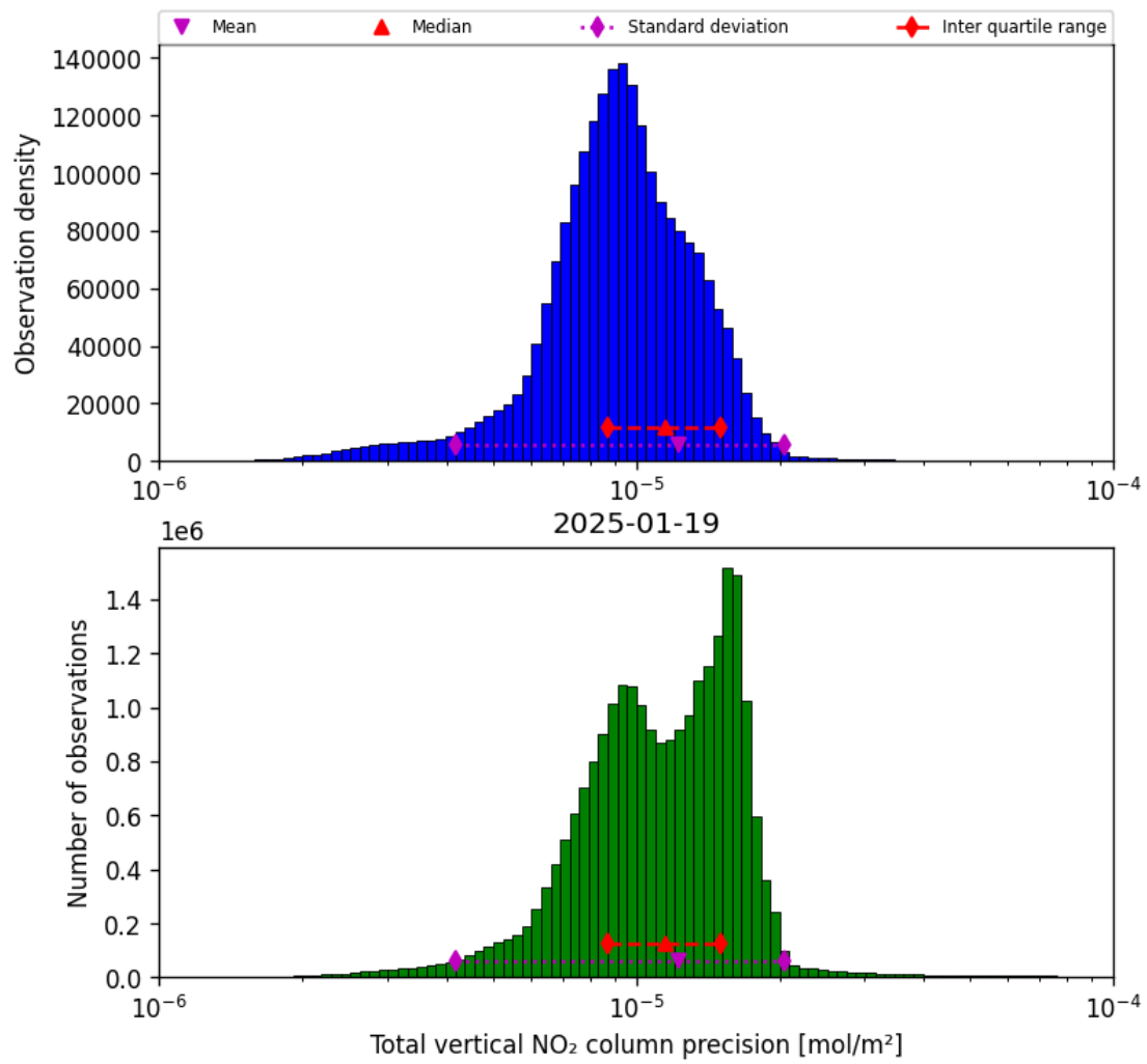
Figure 37: Histogram of “Total vertical NO 2 column precision” for 2025-01-19 to 2025-01-20
