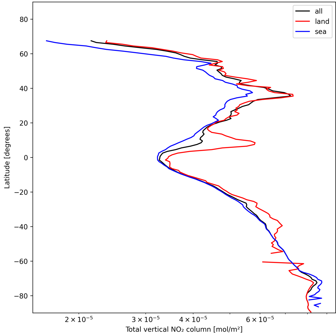
Figure 19: Zonal average of “Total vertical NO 2 column” for 2025-01-19 to 2025-01-20.
