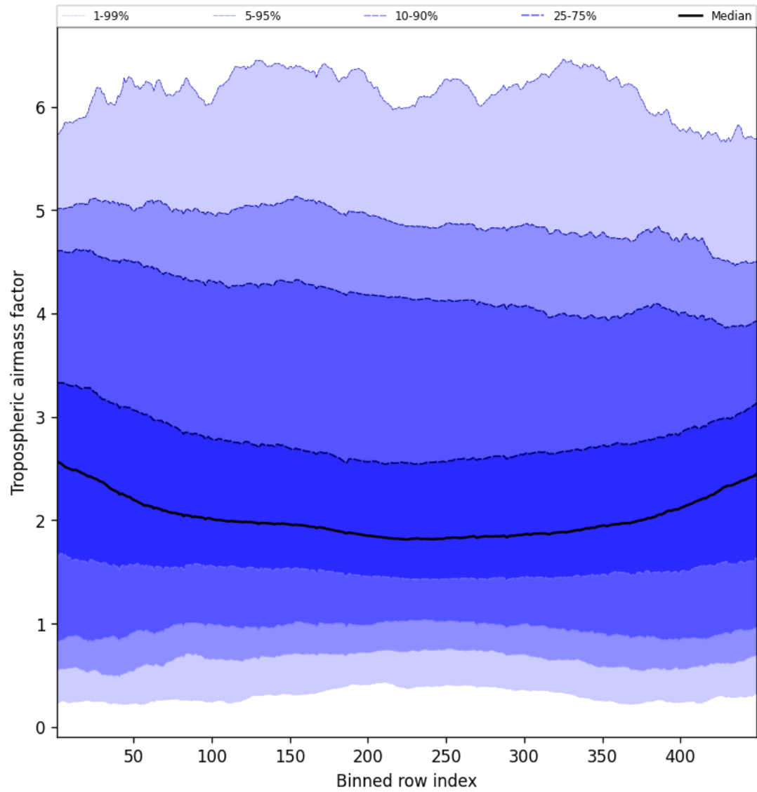
Figure 46: Along track statistics of “Tropospheric air mass factor” for 2025-01-19 to 2025-01-20
