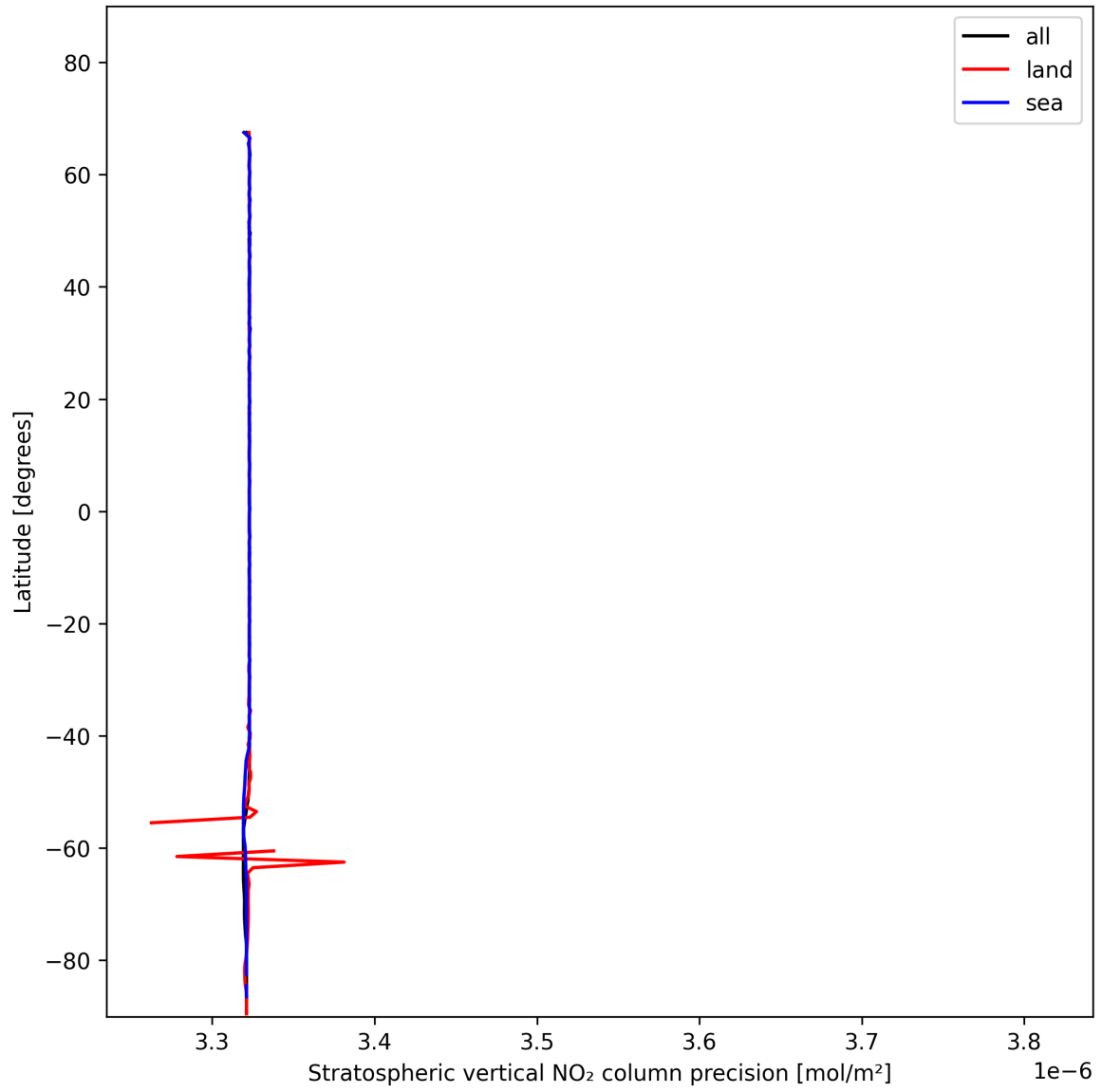
Figure 18: Zonal average of "Stratospheric vertical NO 2 column precision" for 2025-01-19 to 2025-01-20.
