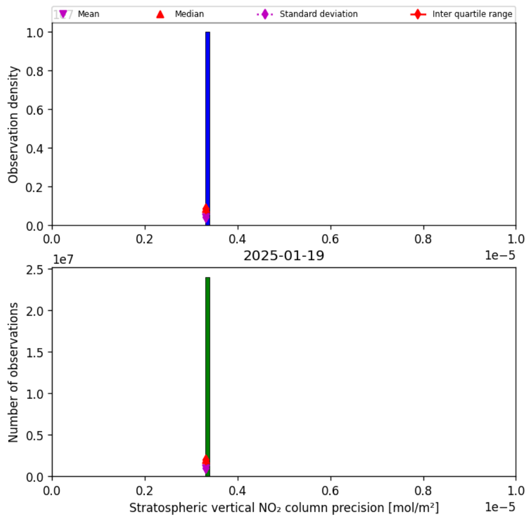
Figure 35: Histogram of “Stratospheric vertical NO 2 column precision” for 2025-01-19 to 2025-01-20
