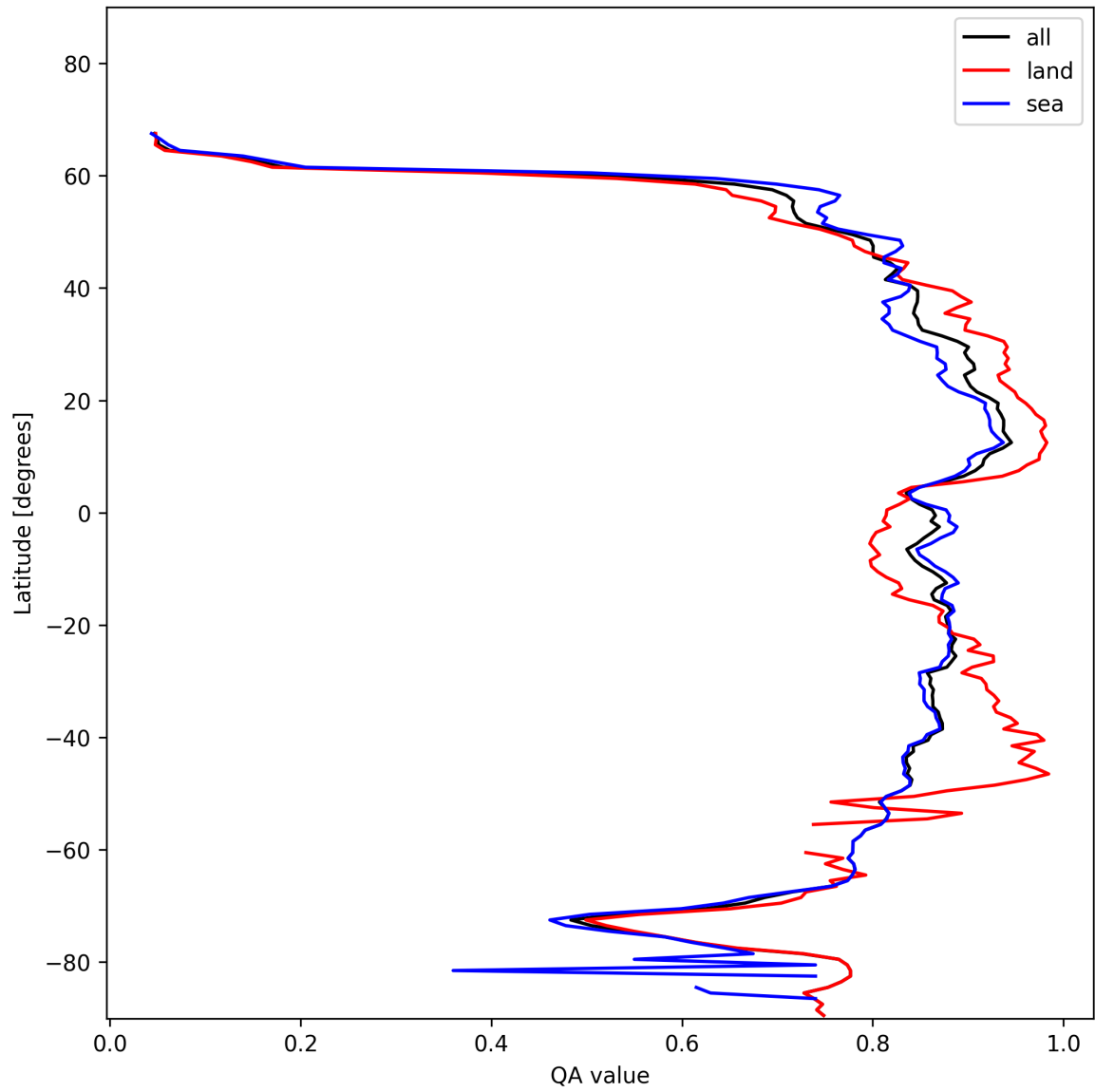
Figure 9: Zonal average of “QA value” for 2025-01-19 to 2025-01-20.
