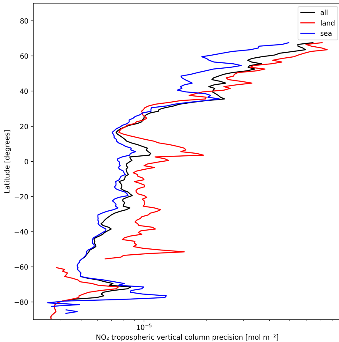
Figure 11: Zonal average of “NO 2 tropospheric vertical column precision” for 2025-01-19 to 2025-01-20.
