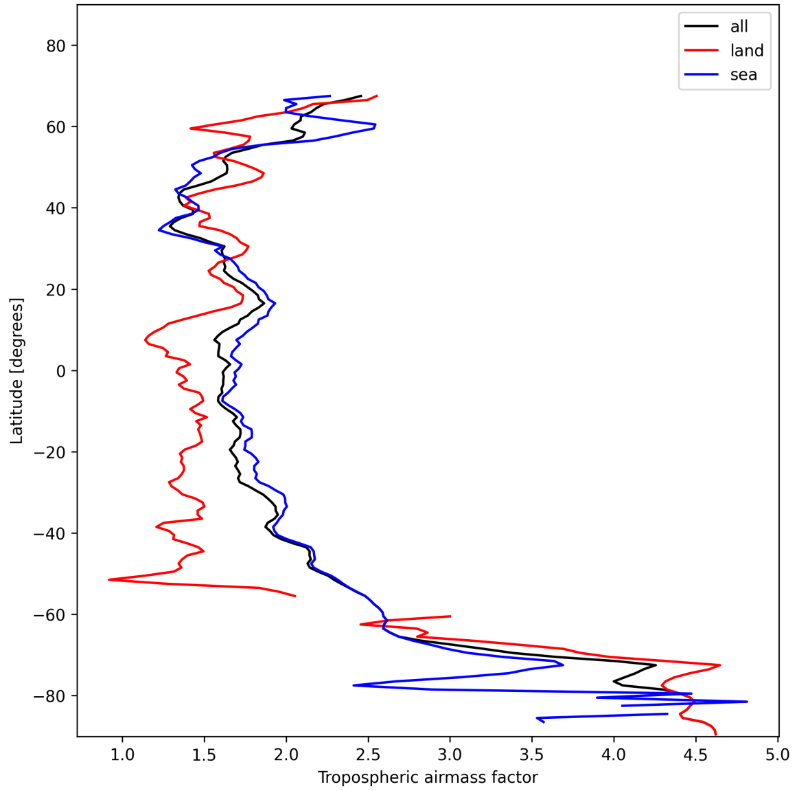
Figure 12: Zonal average of “Tropospheric airmass factor” for 2025-01-19 to 2025-01-20.
