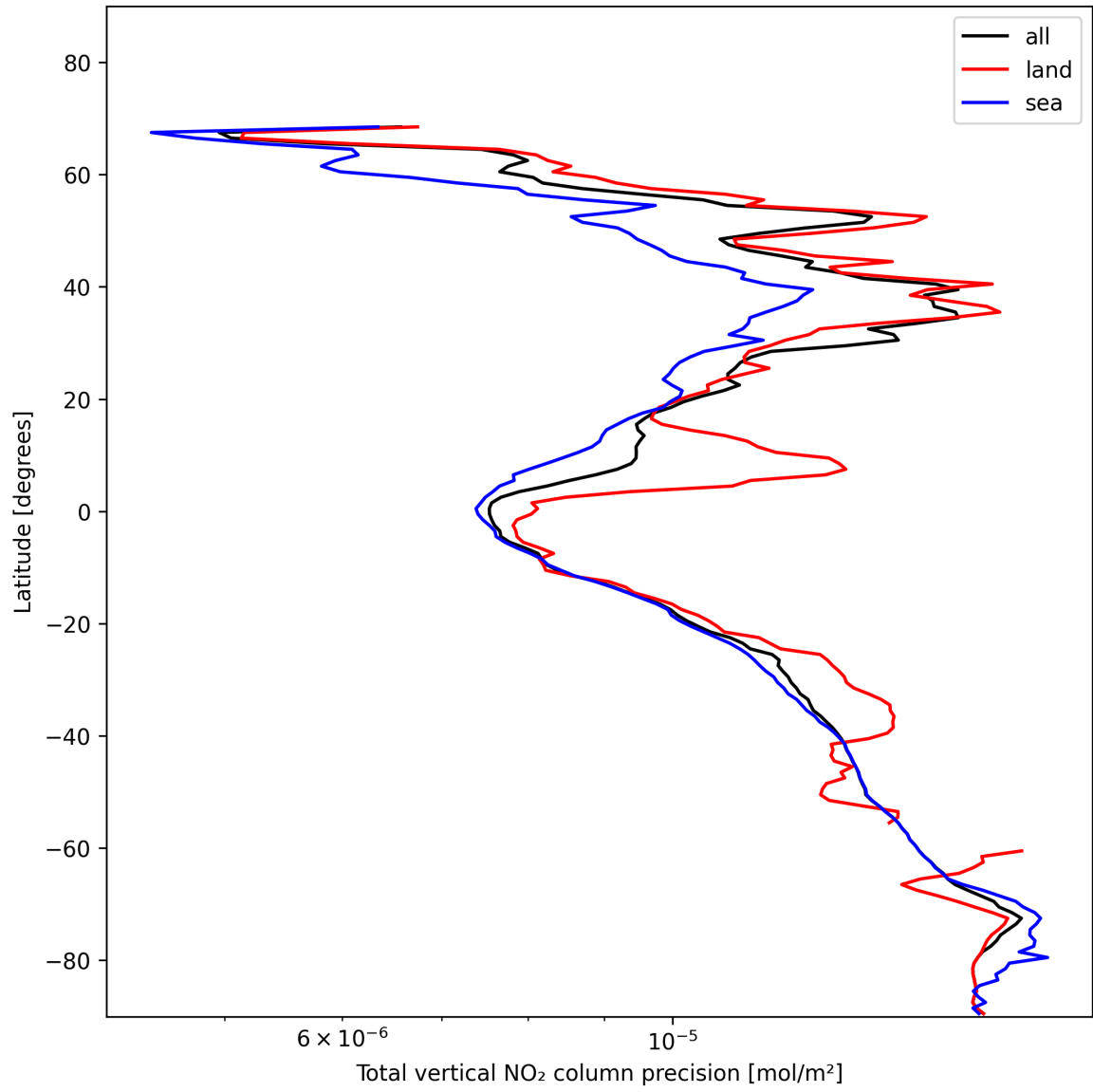
Figure 20: Zonal average of "Total vertical NO 2 column precision" for 2025-01-20 to 2025-01-21.
