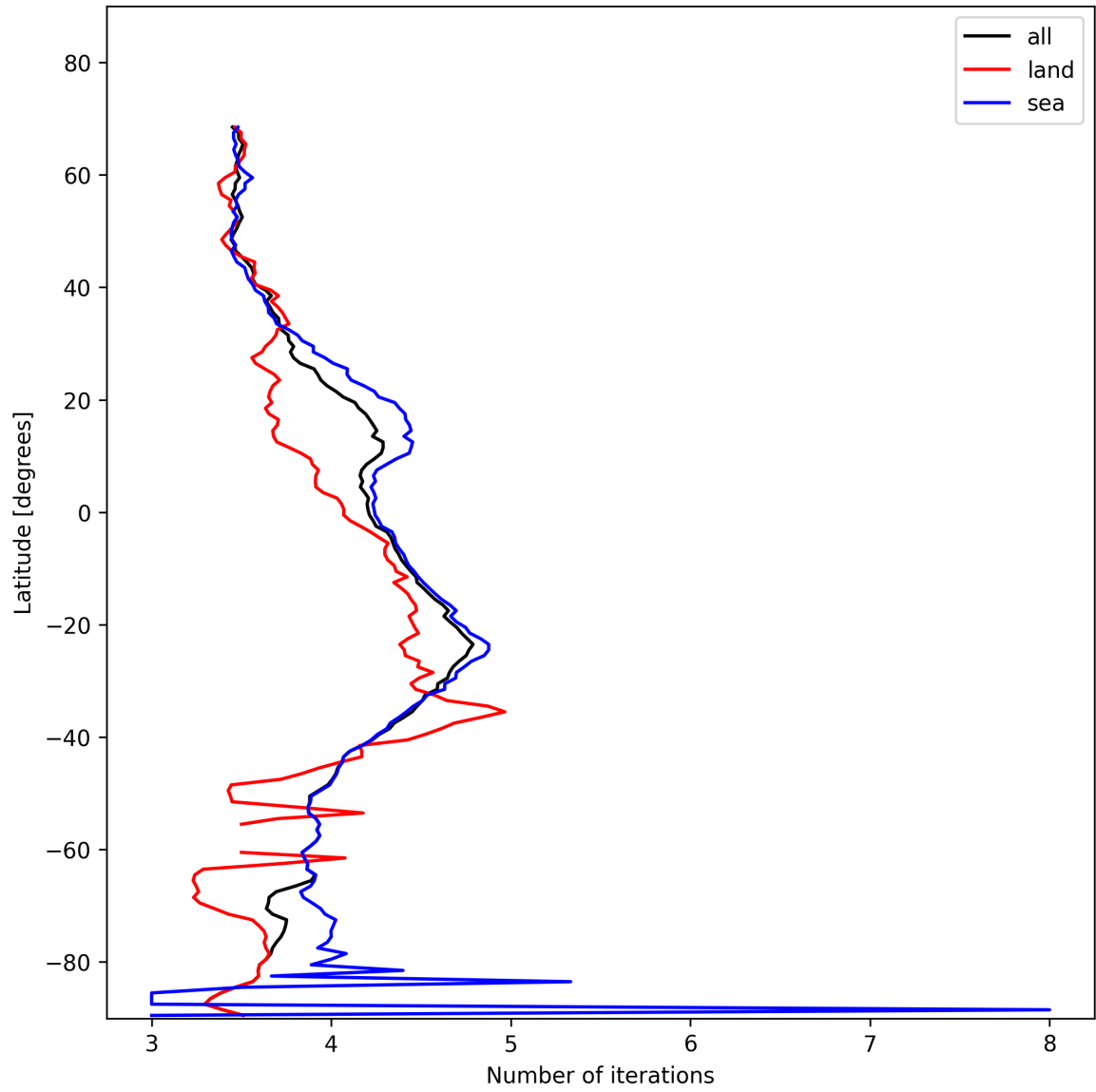
Figure 15: Zonal average of “Number of iterations” for 2025-01-20 to 2025-01-21.
