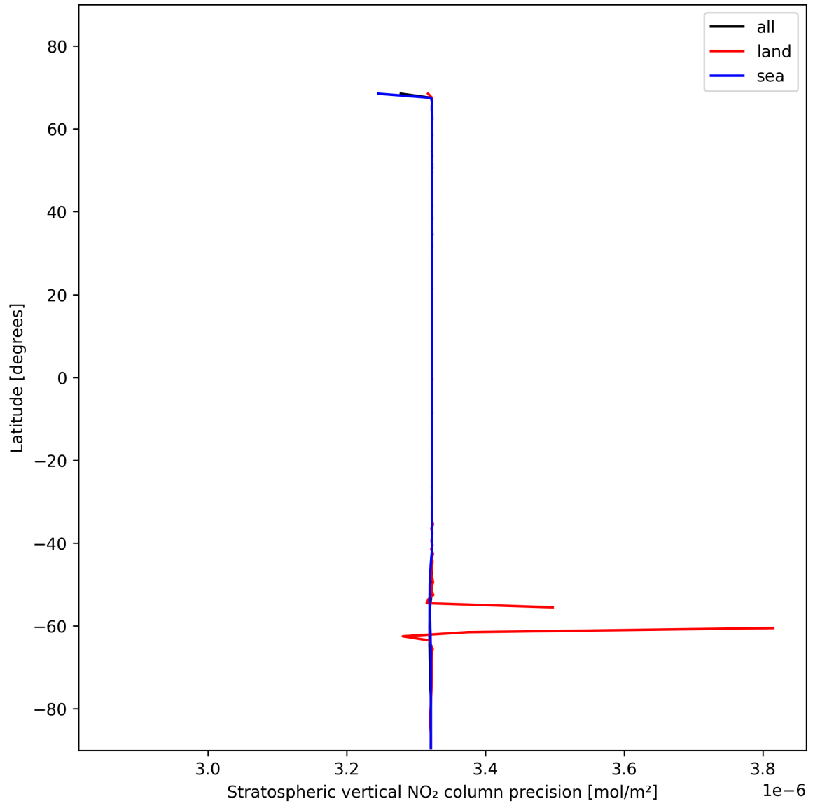
Figure 18: Zonal average of “Stratospheric vertical NO 2 column precision” for 2025-01-20 to 2025-01-21.
