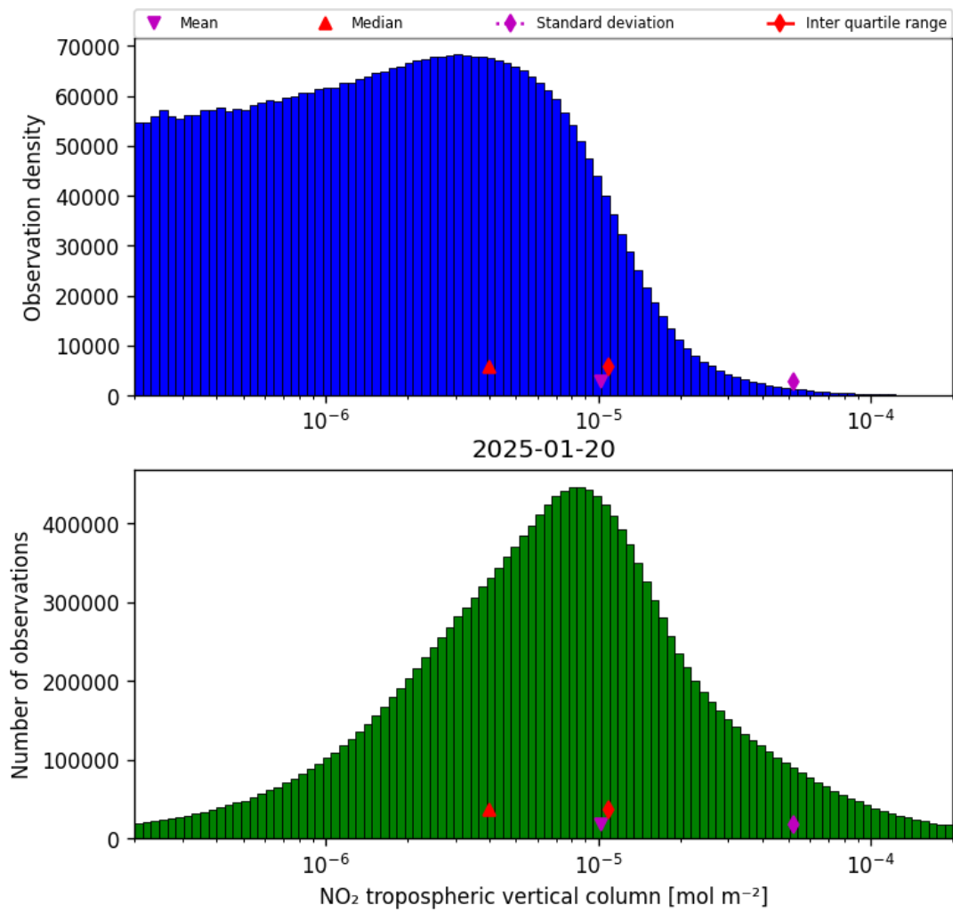
Figure 27: Histogram of “NO 2 tropospheric vertical column” for 2025-01-20 to 2025-01-21
