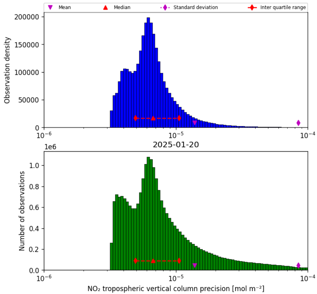
Figure 28: Histogram of “NO 2 tropospheric vertical column precision” for 2025-01-20 to 2025-01-21
