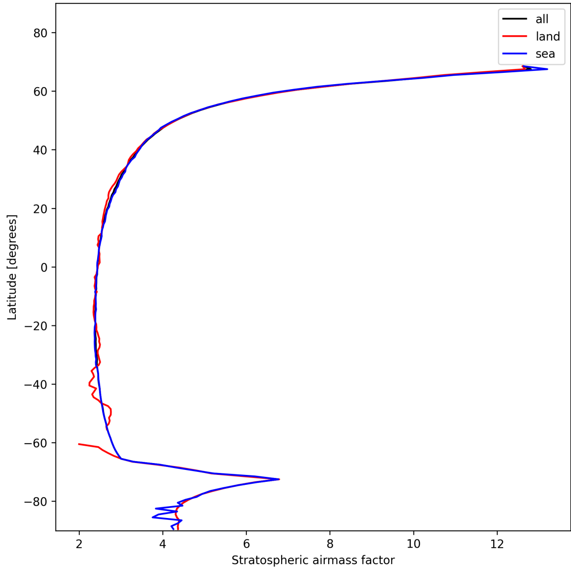
Figure 25: Zonal average of “Stratospheric airmass factor” for 2025-01-20 to 2025-01-21.
