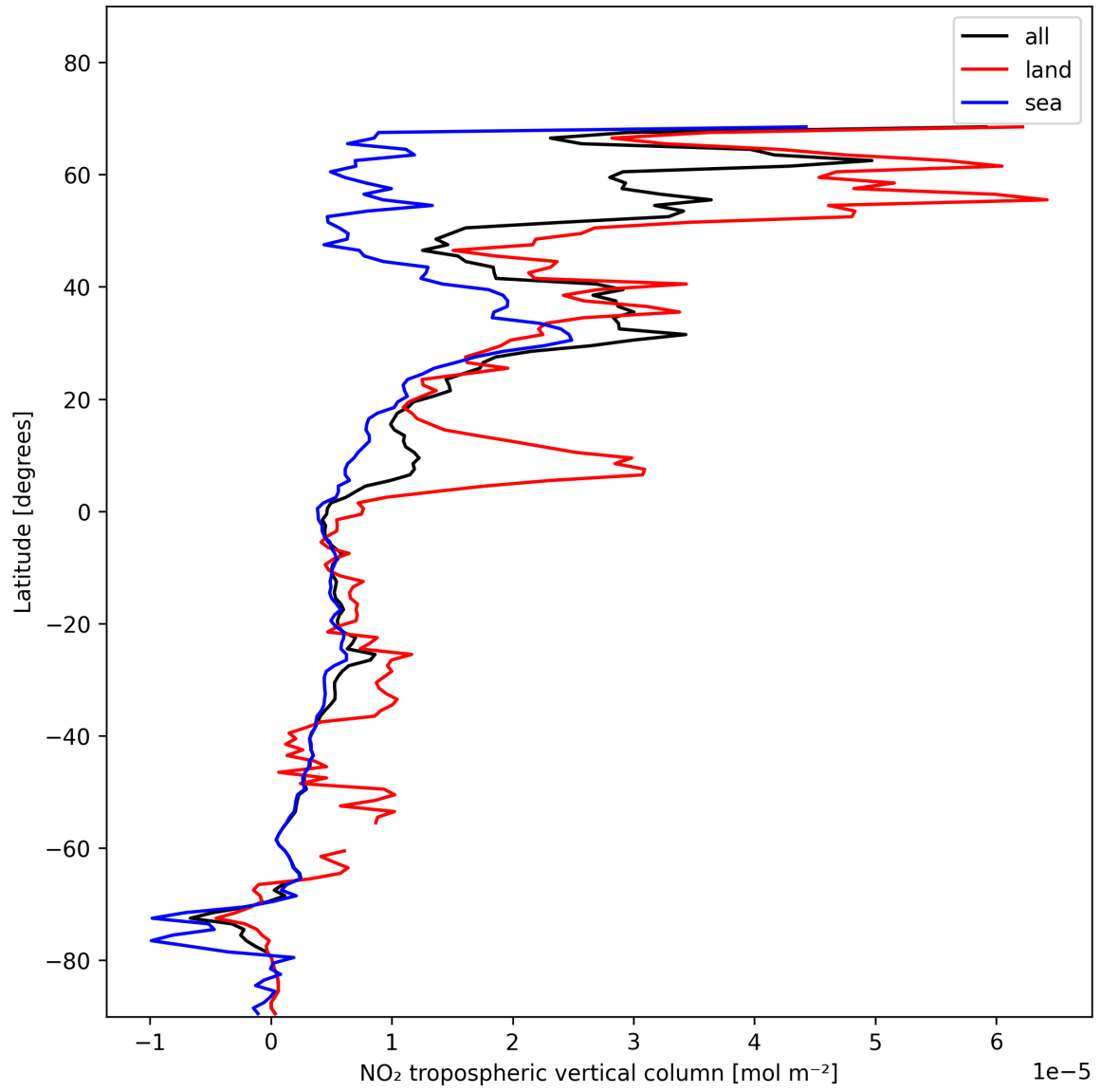
Figure 10: Zonal average of “NO 2 tropospheric vertical column” for 2025-01-20 to 2025-01-21.
