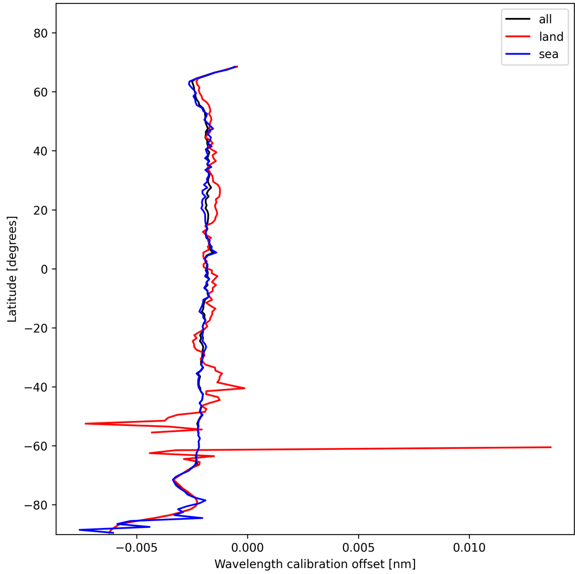
Figure 16: Zonal average of “Wavelength calibration offset” for 2025-01-20 to 2025-01-21.
