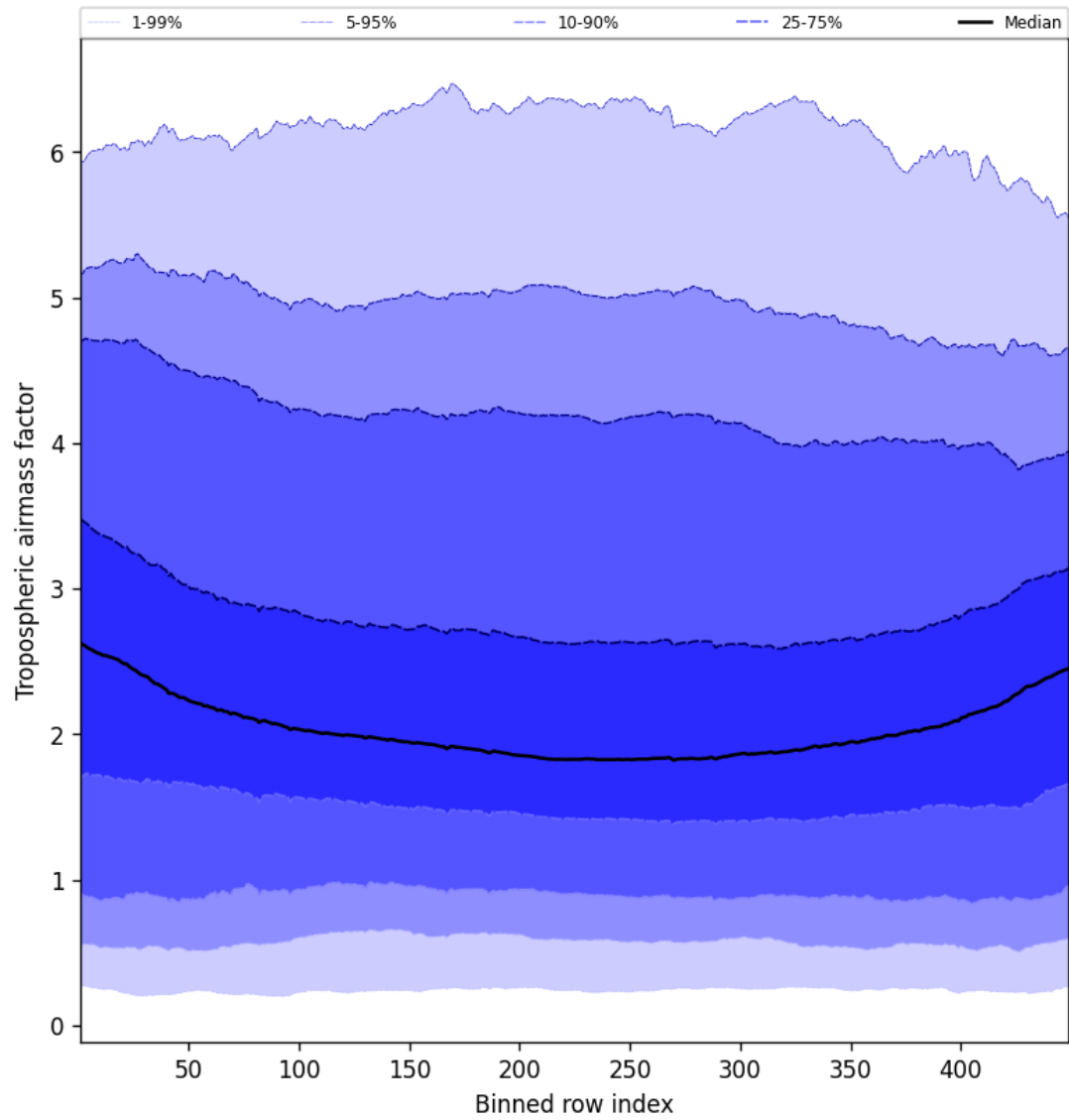
Figure 46: Along track statistics of “Tropospheric air mass factor” for 2025-01-20 to 2025-01-21
