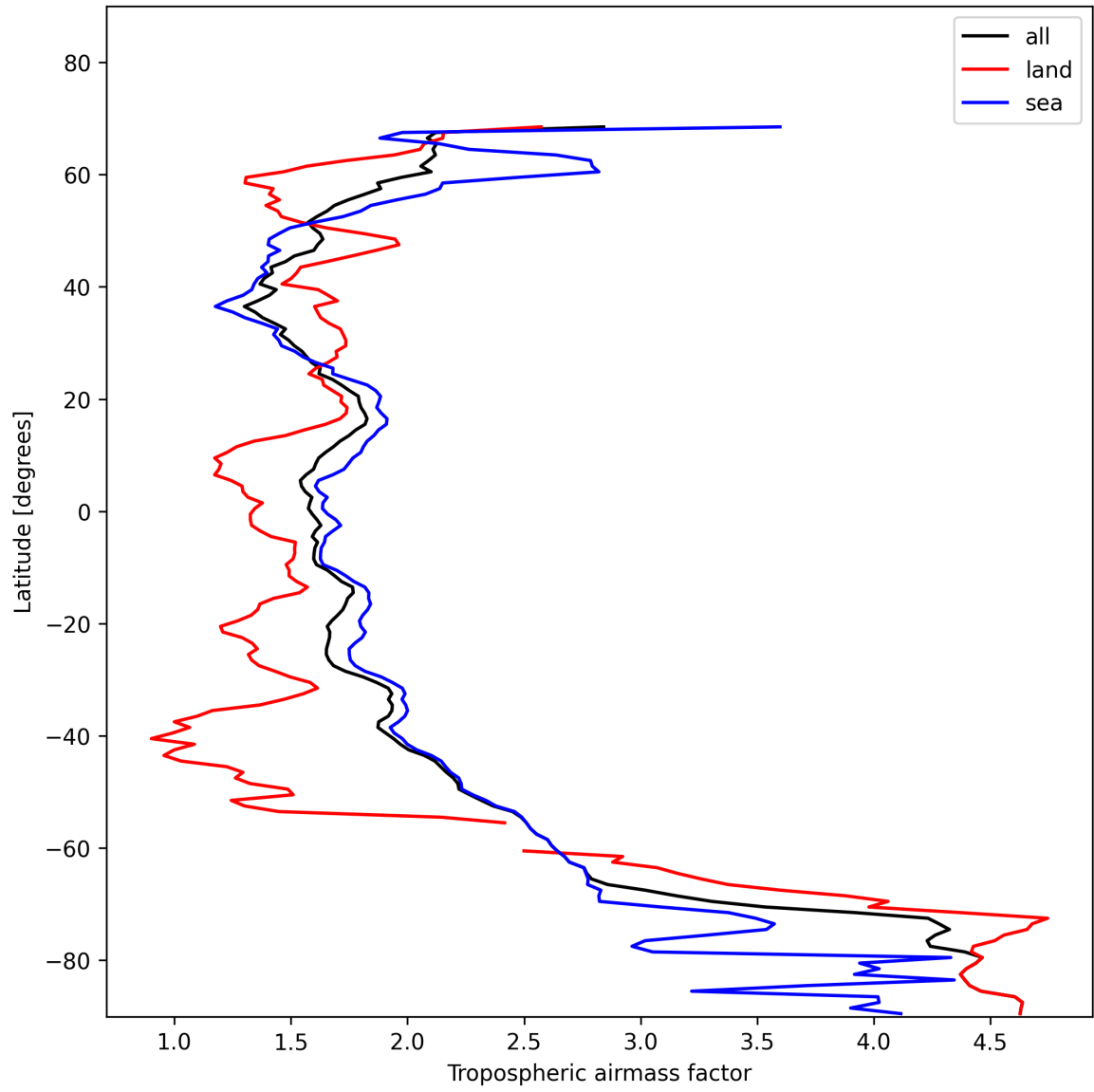
Figure 12: Zonal average of “Tropospheric air mass factor” for 2025-01-20 to 2025-01-21.
