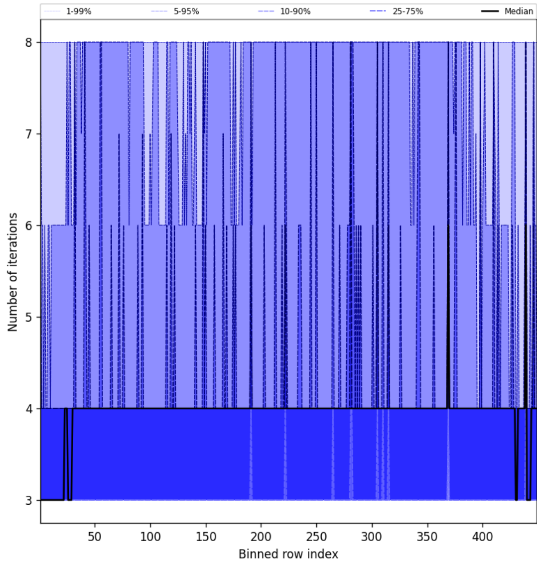
Figure 49: Along track statistics of “Number of iterations” for 2025-01-20 to 2025-01-21
