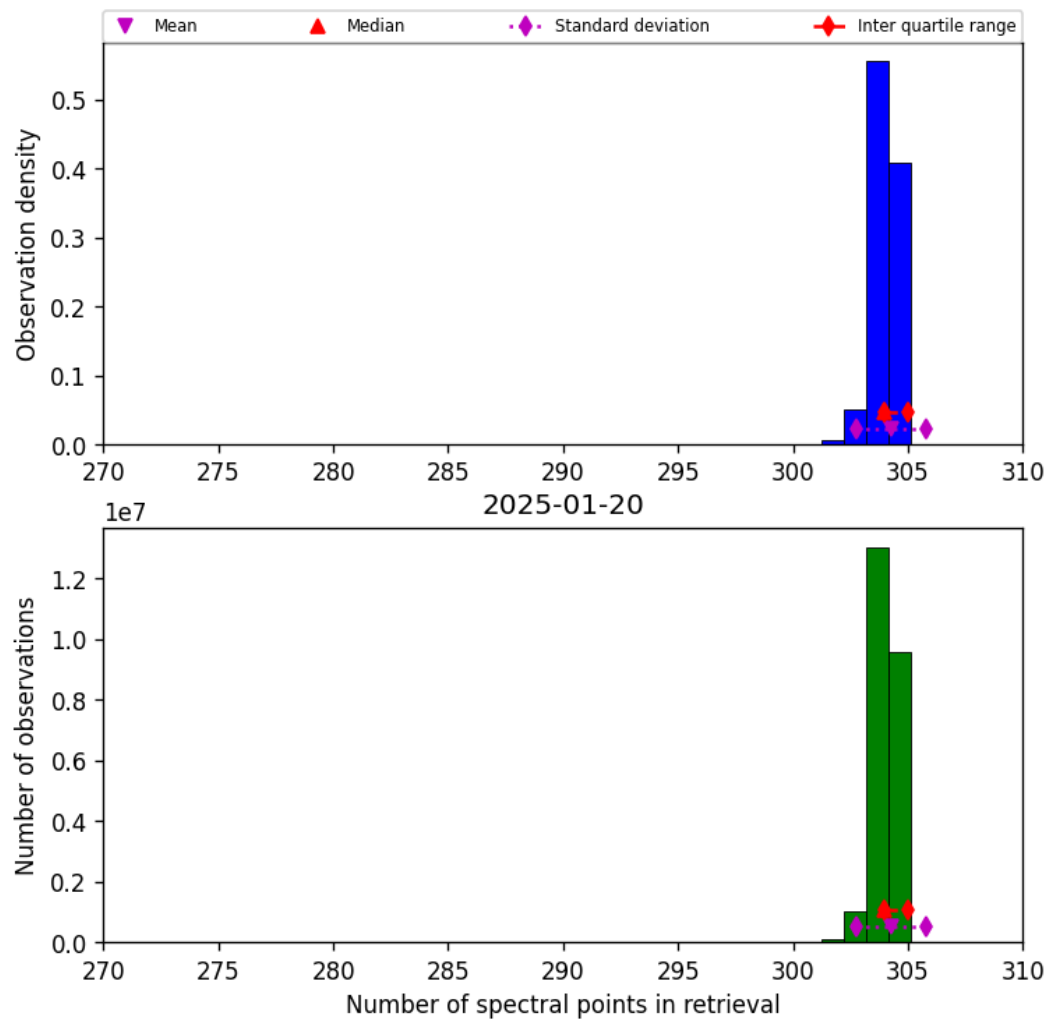
Figure 31: Histogram of “Number of spectral points in retrieval” for 2025-01-20 to 2025-01-21
