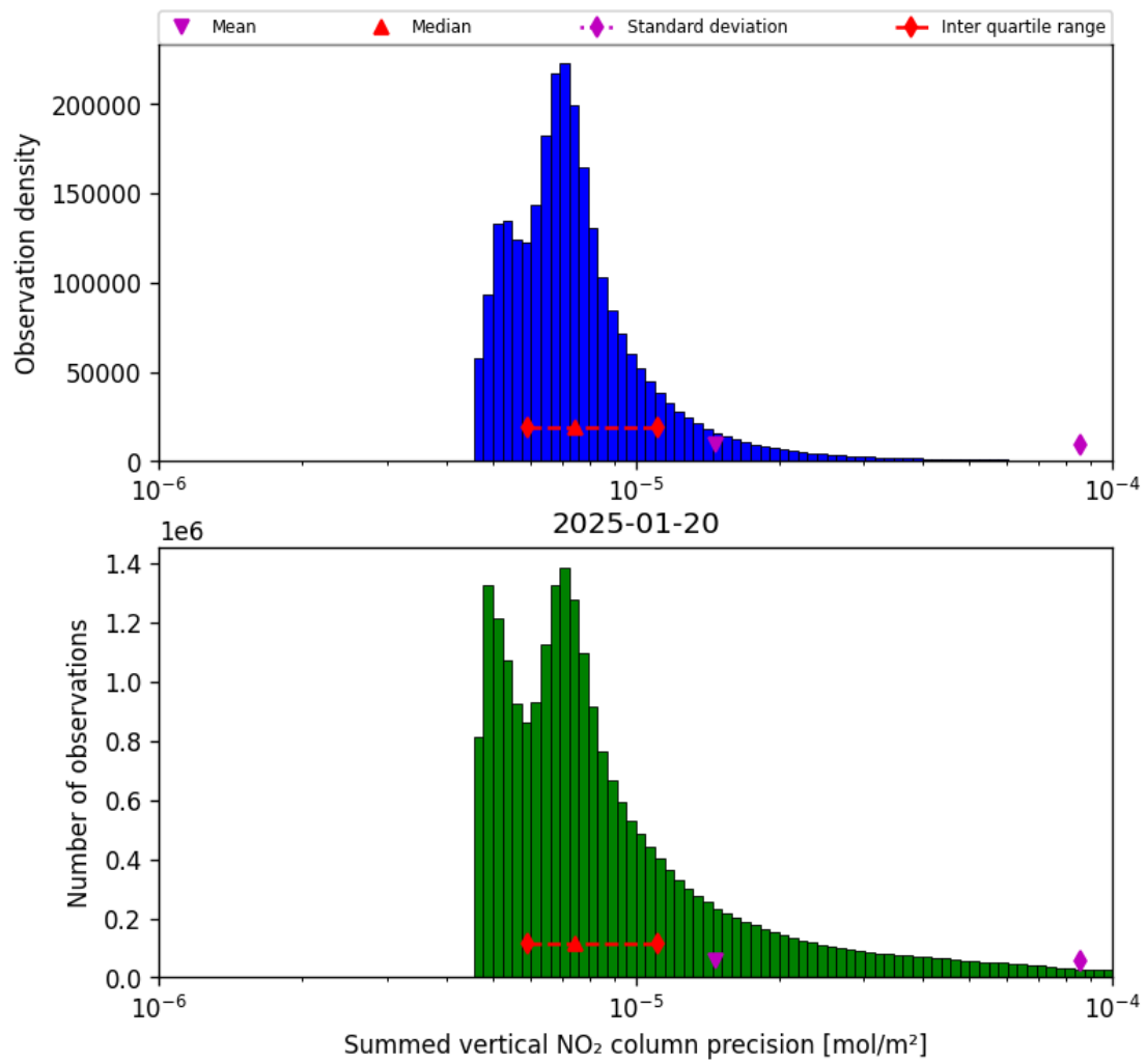
Figure 39: Histogram of “Summed vertical NO 2 column precision” for 2025-01-20 to 2025-01-21
