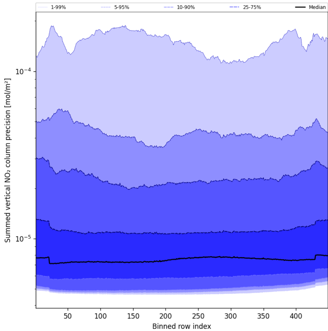
Figure 56: Along track statistics of “Summed vertical NO 2 column precision” for 2025-01-20 to 2025-01-21
