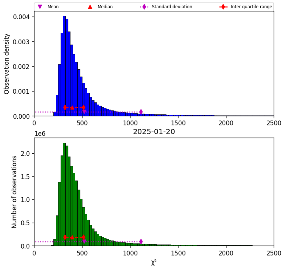
Figure 40: Histogram of “ \chi^2 ” for 2025-01-20 to 2025-01-21
