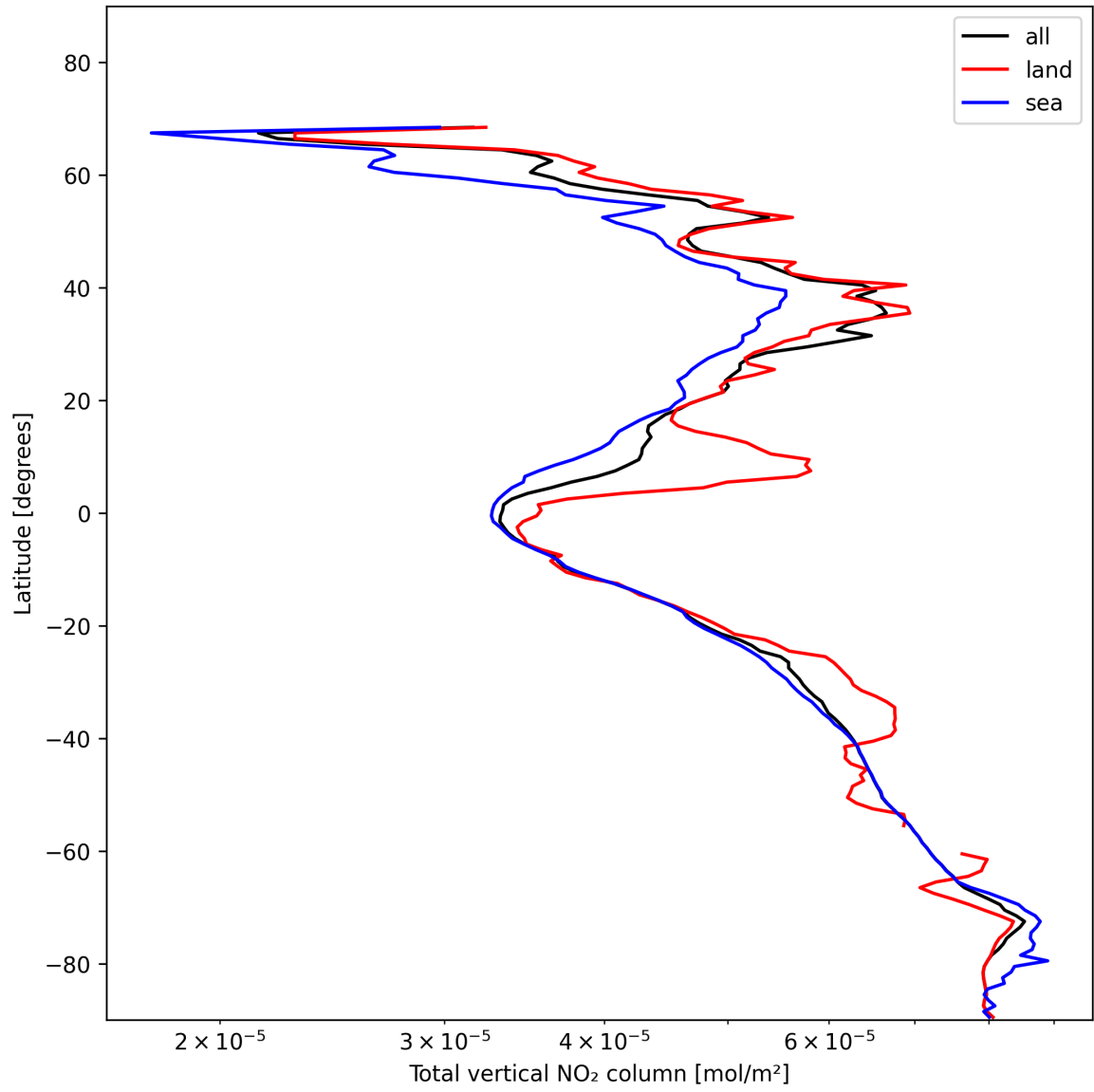
Figure 19: Zonal average of “Total vertical NO 2 column” for 2025-01-20 to 2025-01-21.
