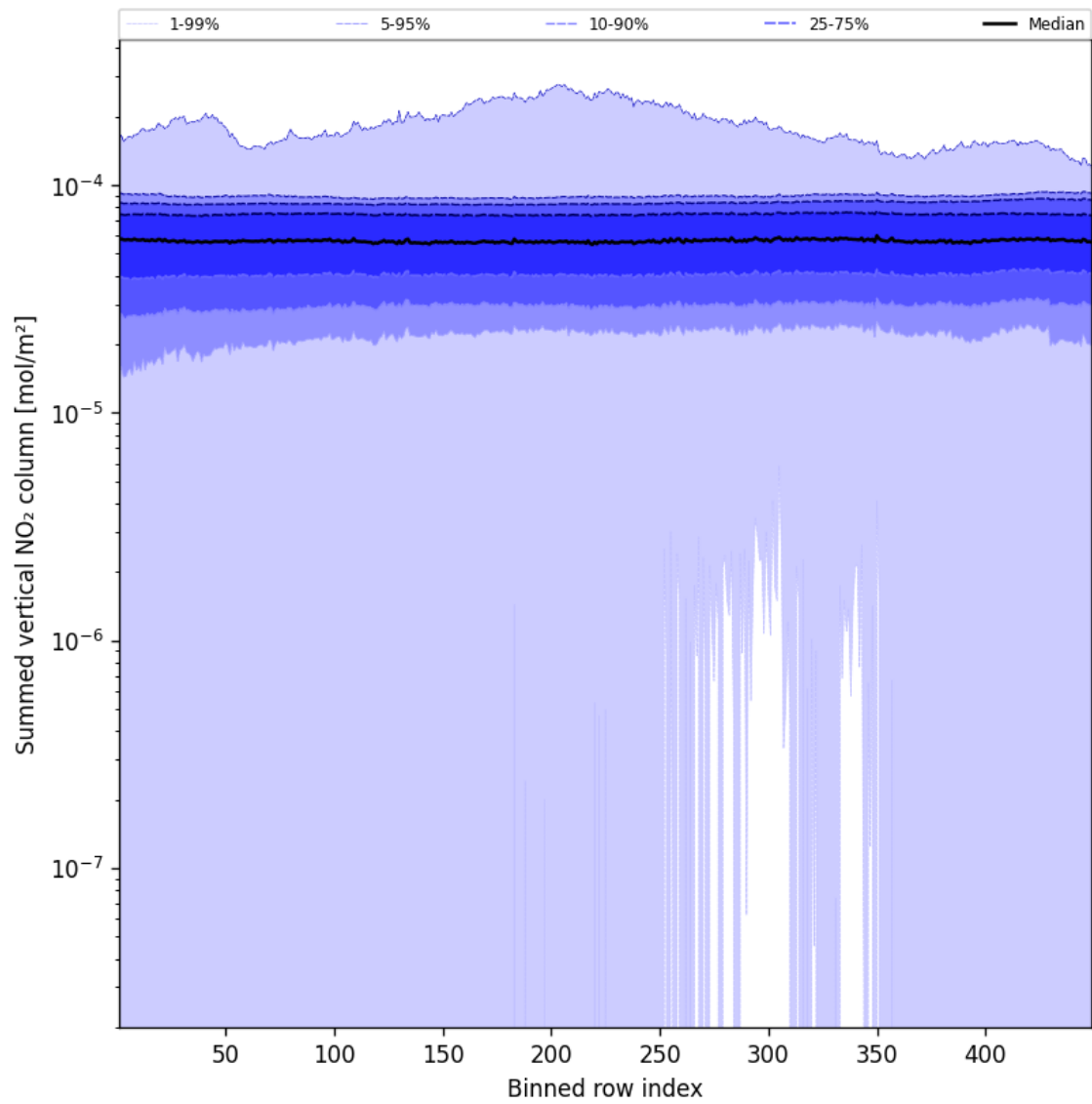
Figure 55: Along track statistics of “Summed vertical NO 2 column” for 2025-01-20 to 2025-01-21
