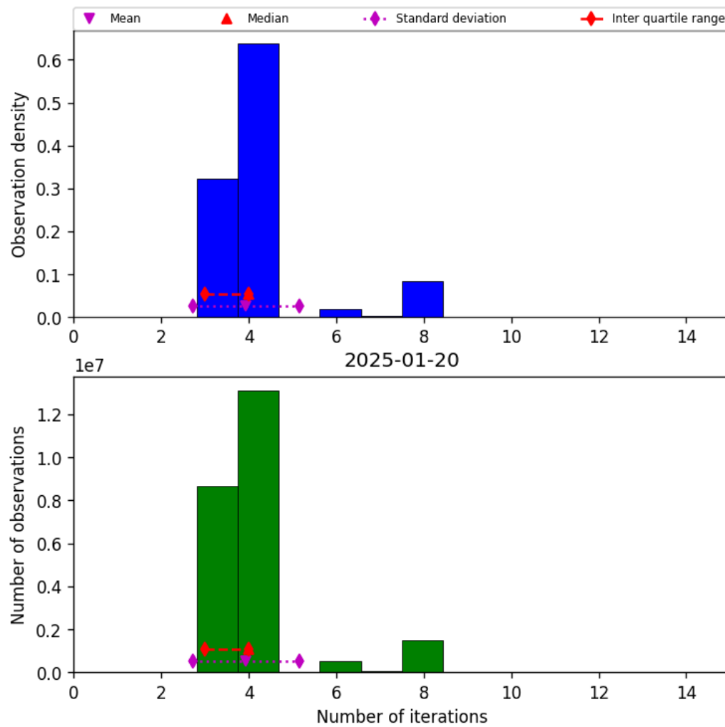
Figure 32: Histogram of “Number of iterations” for 2025-01-20 to 2025-01-21
