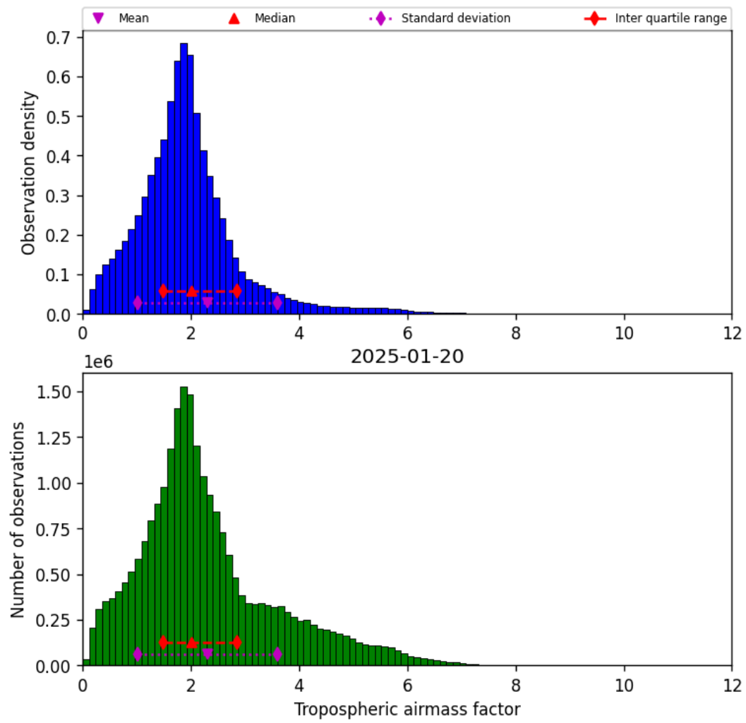
Figure 29: Histogram of “Tropospheric airmass factor” for 2025-01-20 to 2025-01-21
