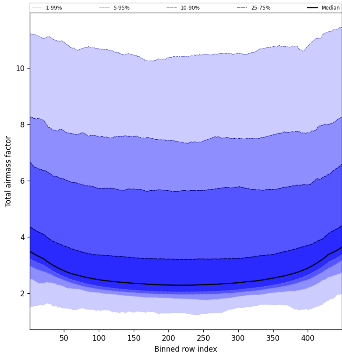
Figure 47: Along track statistics of “Total airmass factor” for 2025-01-20 to 2025-01-21
