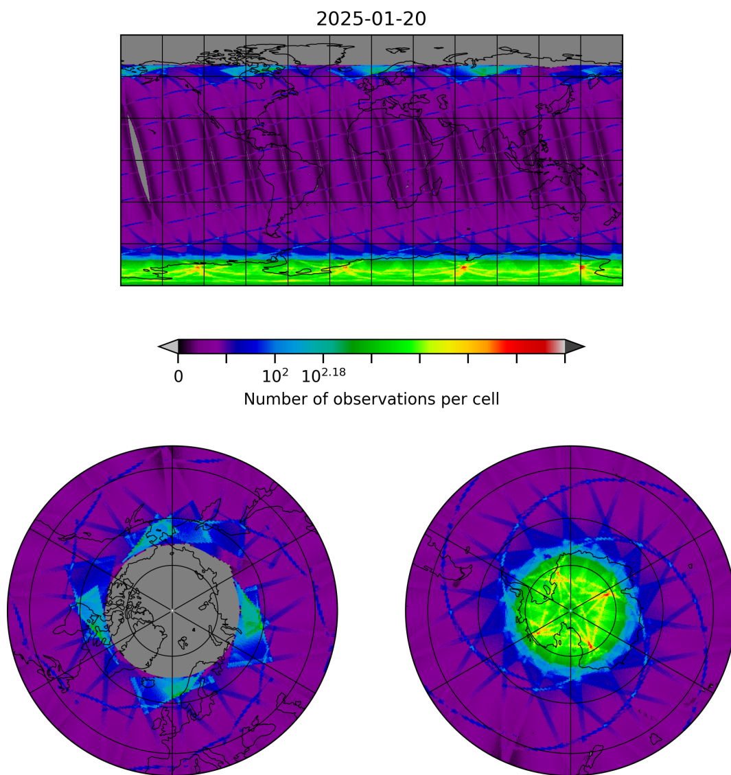
Figure 8: Map of the number of observations for 2025-01-20 to 2025-01-21
