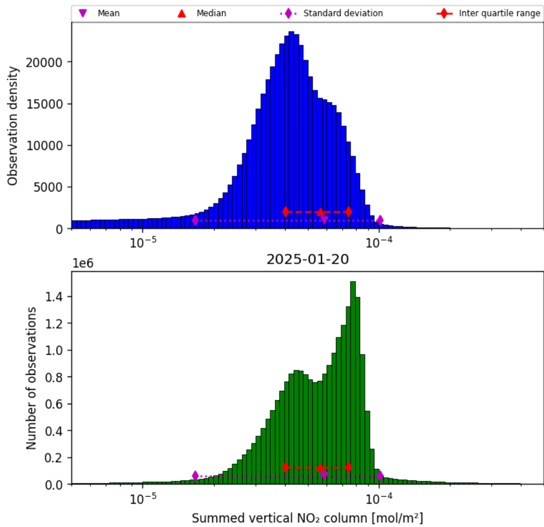
Figure 38: Histogram of “Summed vertical NO 2 column” for 2025-01-20 to 2025-01-21
