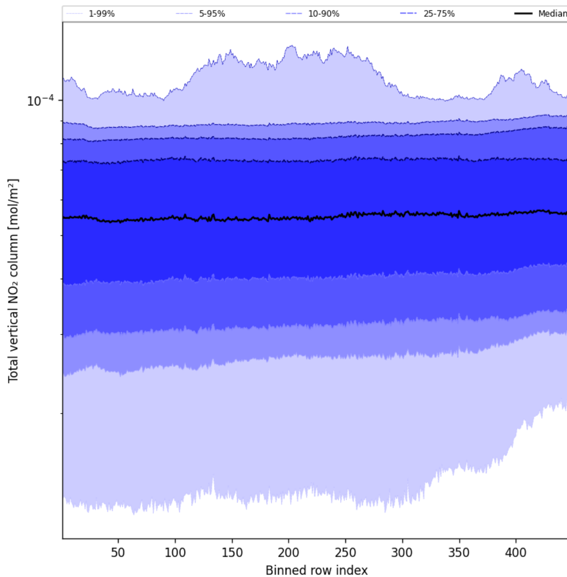
Figure 53: Along track statistics of “Total vertical NO 2 column” for 2025-01-20 to 2025-01-21
