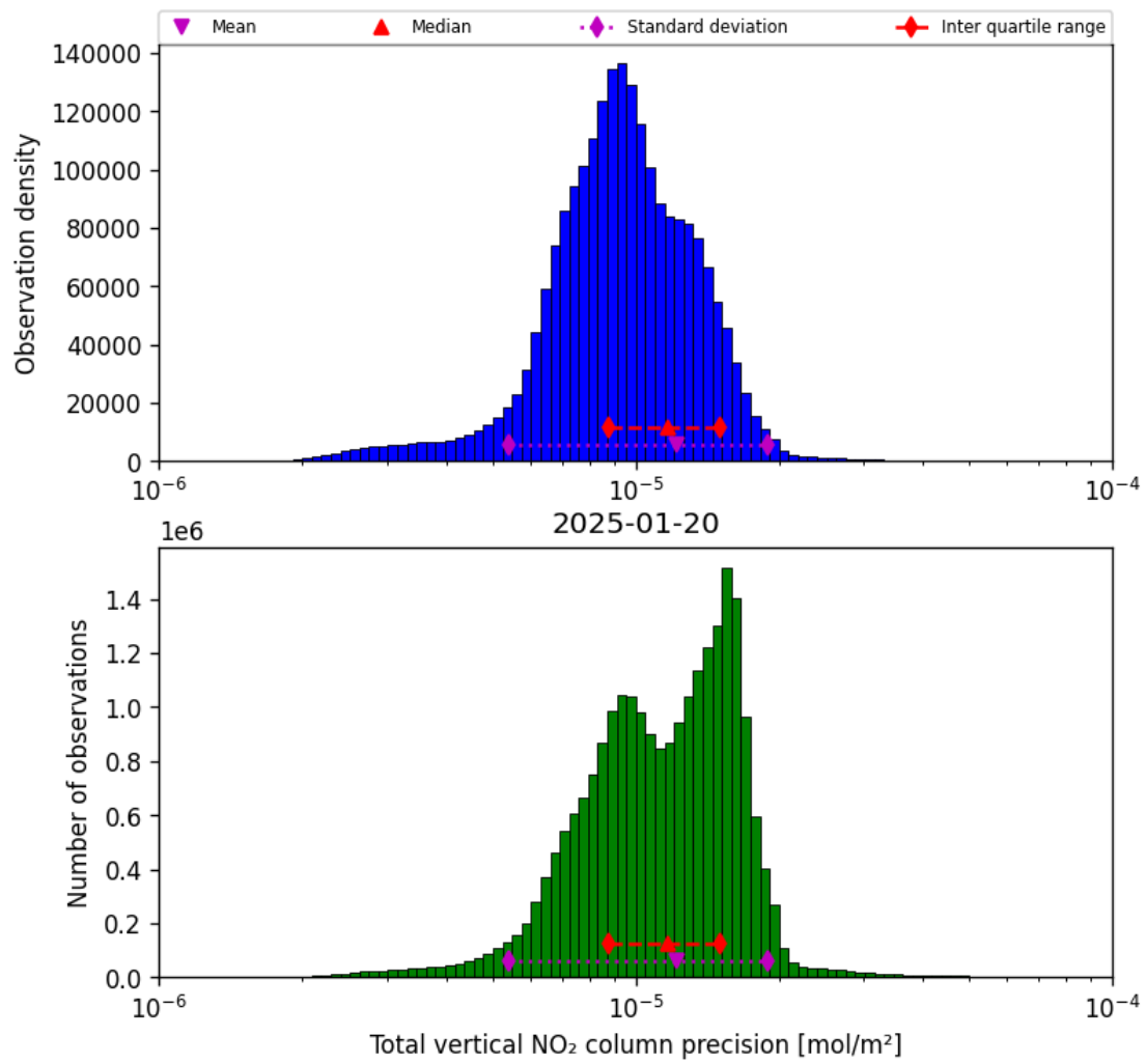
Figure 37: Histogram of “Total vertical NO 2 column precision” for 2025-01-20 to 2025-01-21
