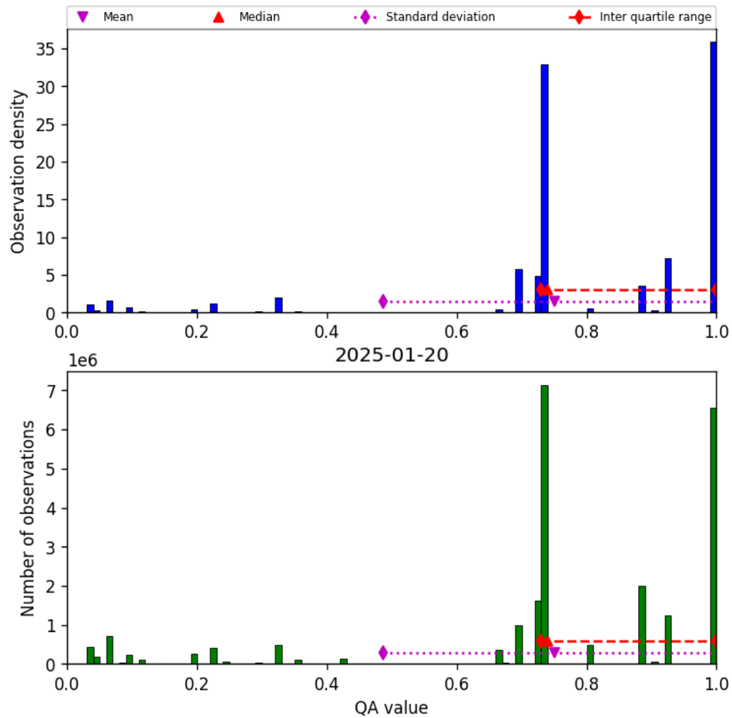
Figure 26: Histogram of “QA value” for 2025-01-20 to 2025-01-21
