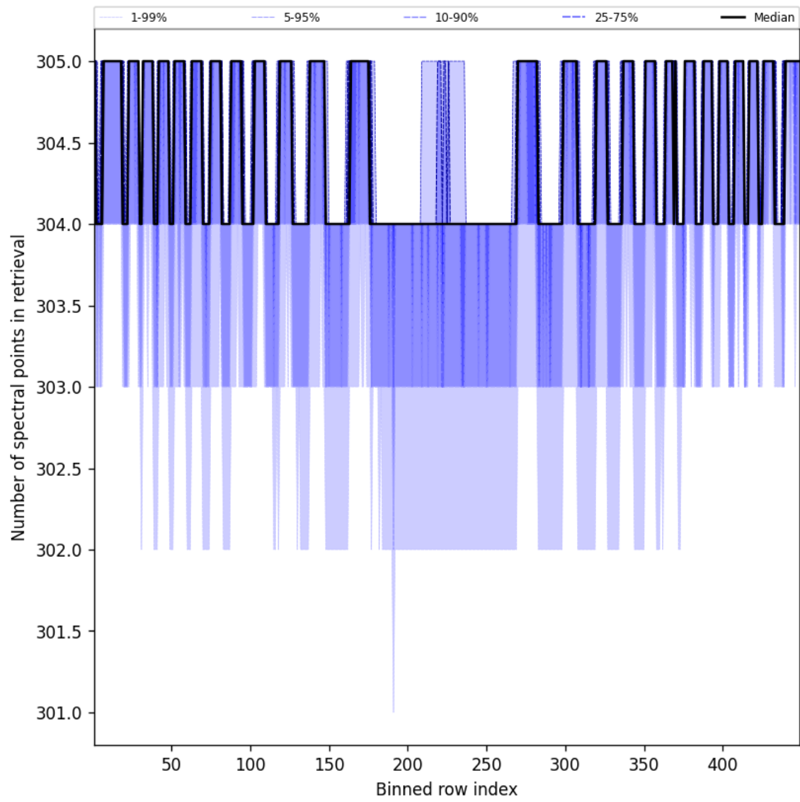
Figure 48: Along track statistics of “Number of spectral points in retrieval” for 2025-01-20 to 2025-01-21
