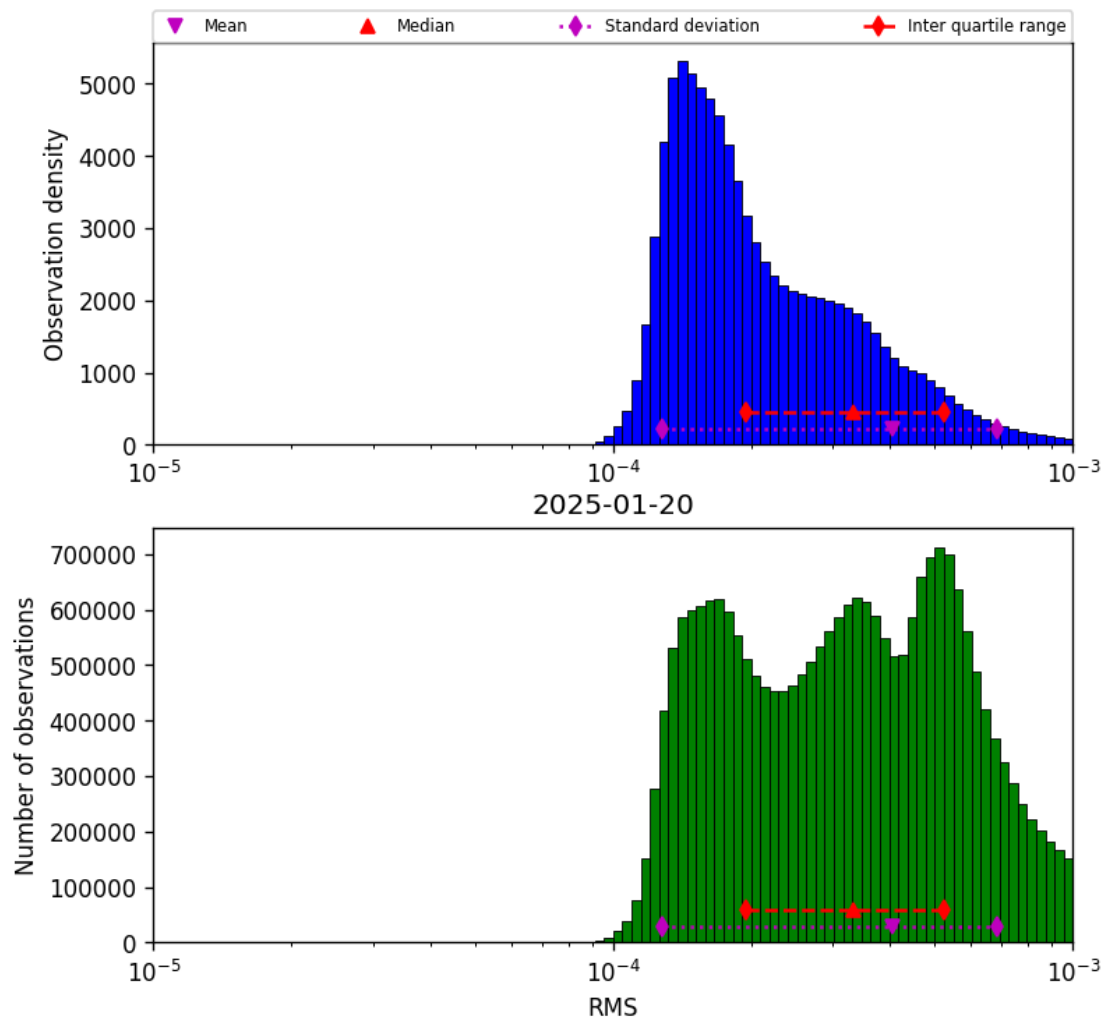
Figure 41: Histogram of “RMS” for 2025-01-20 to 2025-01-21
