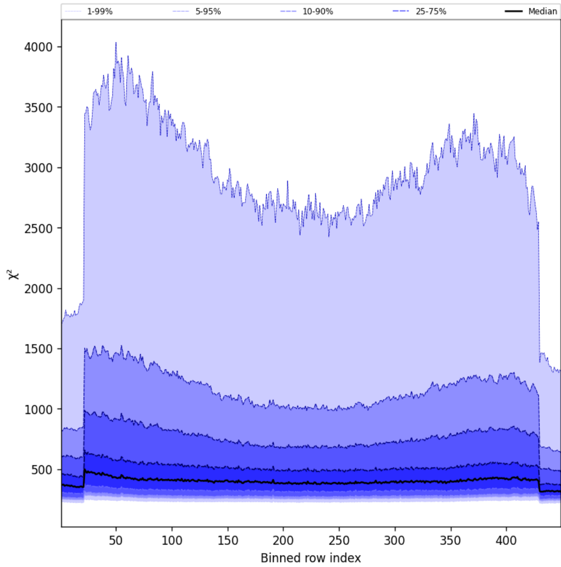
Figure 57: Along track statistics of “ \chi^2 ” for 2025-01-20 to 2025-01-21
