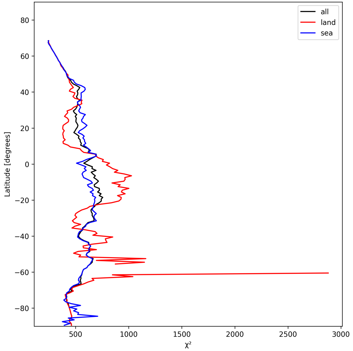
Figure 23: Zonal average of “ \chi^2 ” for 2025-01-20 to 2025-01-21.
