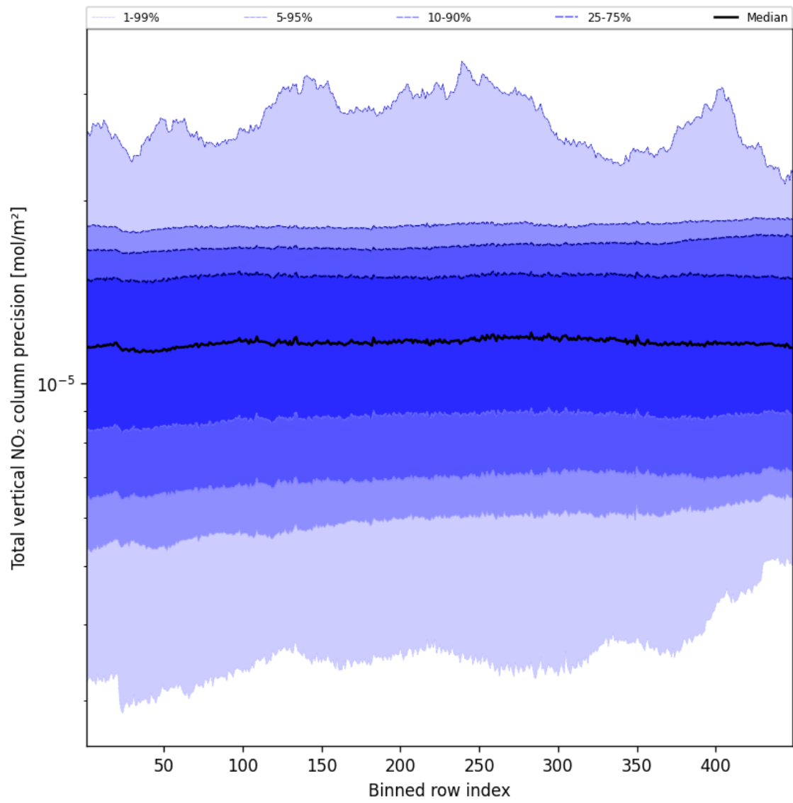
Figure 54: Along track statistics of “Total vertical NO 2 column precision” for 2025-01-20 to 2025-01-21
