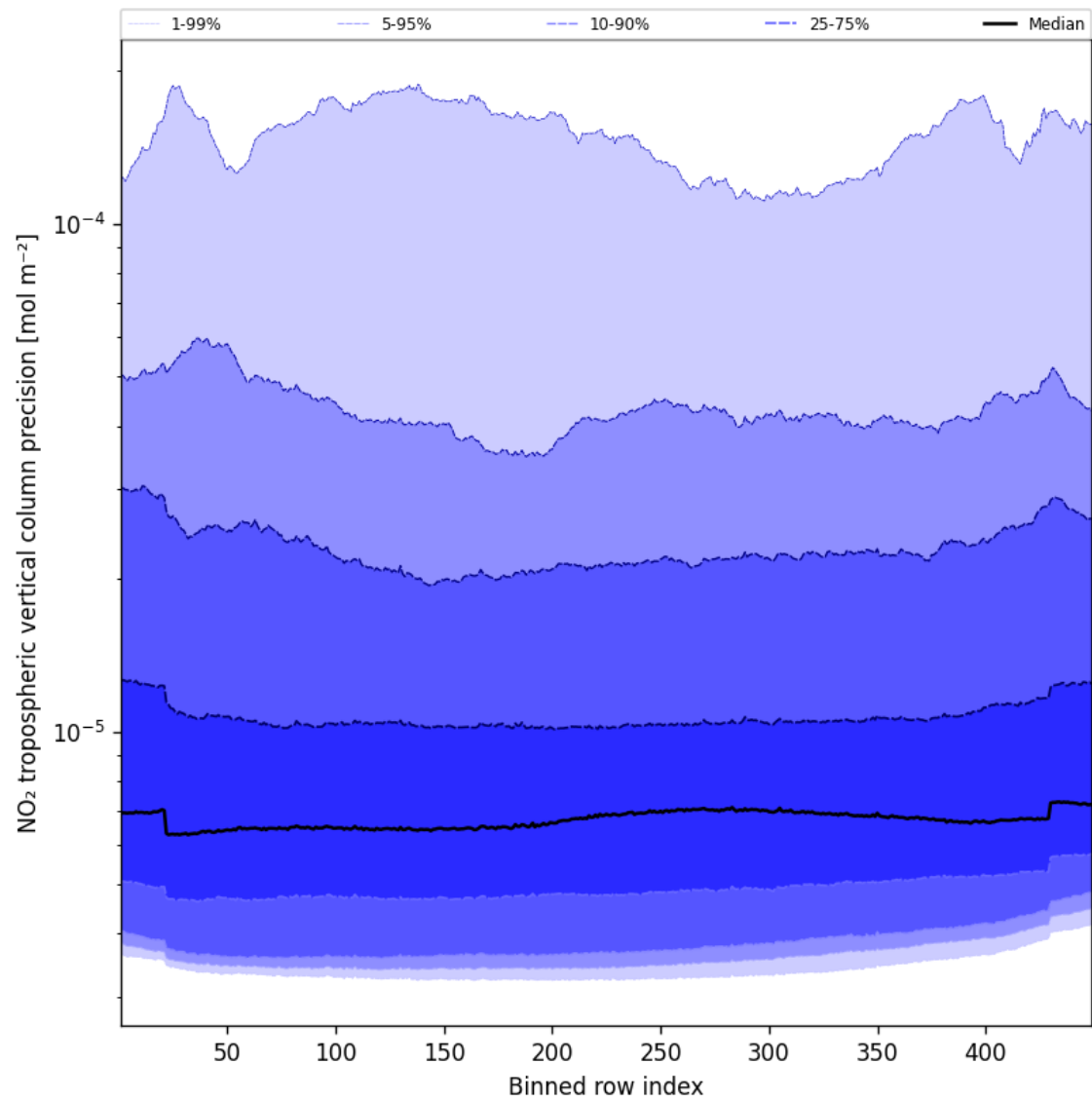
Figure 45: Along track statistics of “NO 2 tropospheric vertical column precision” for 2025-01-20 to 2025-01-21
