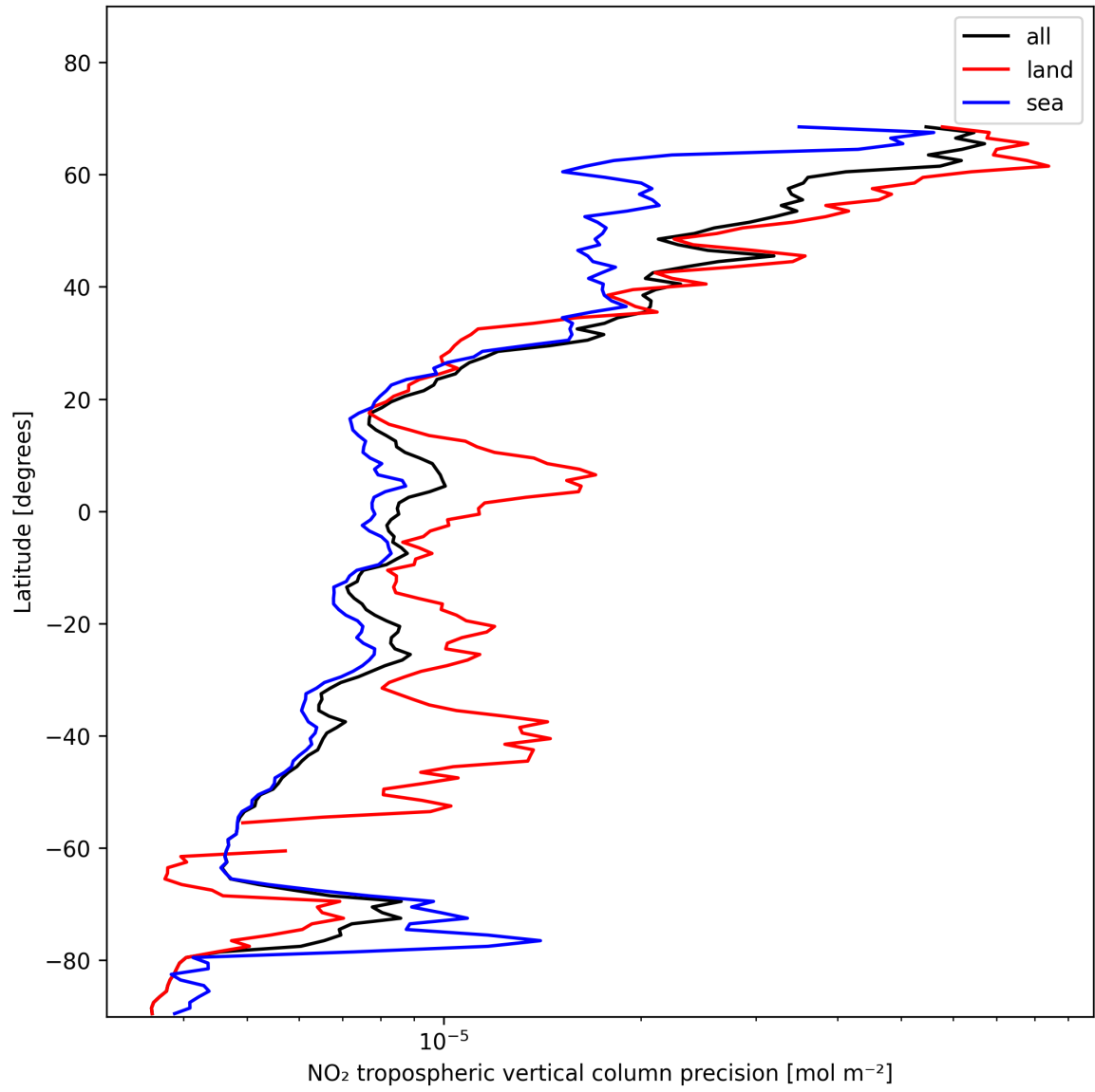
Figure 11: Zonal average of “NO 2 tropospheric vertical column precision” for 2025-01-20 to 2025-01-21.
