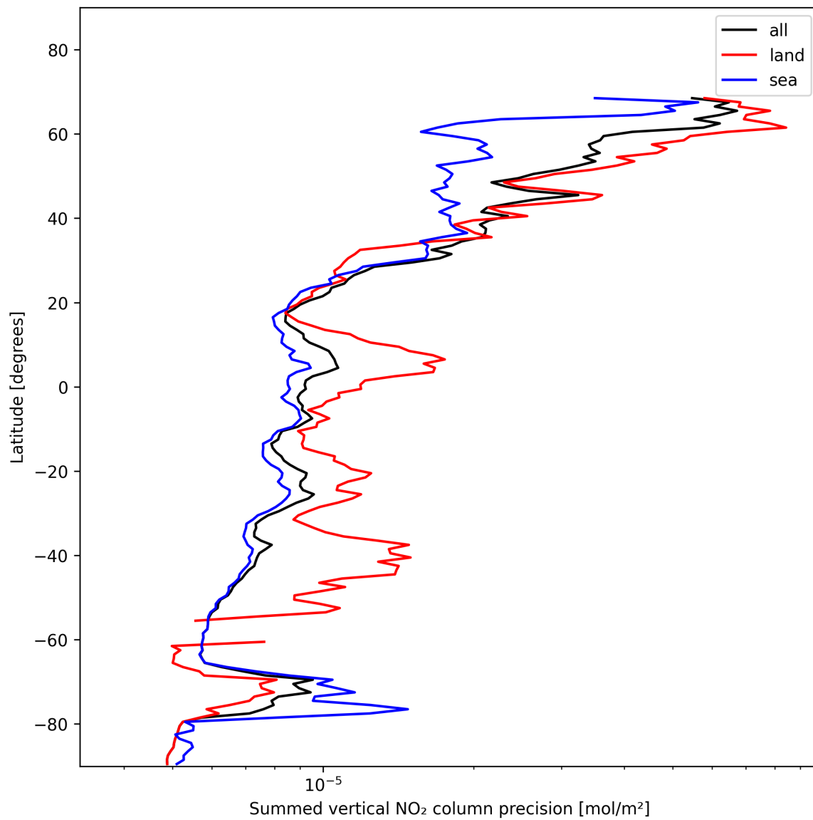
Figure 22: Zonal average of “Summed vertical NO 2 column precision” for 2025-01-20 to 2025-01-21.
