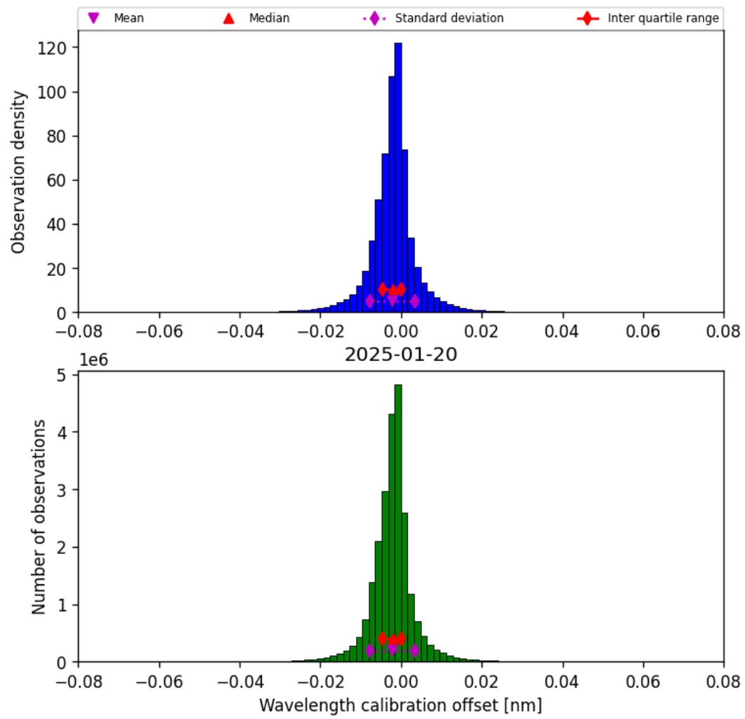
Figure 33: Histogram of “Wavelength calibration offset” for 2025-01-20 to 2025-01-21
