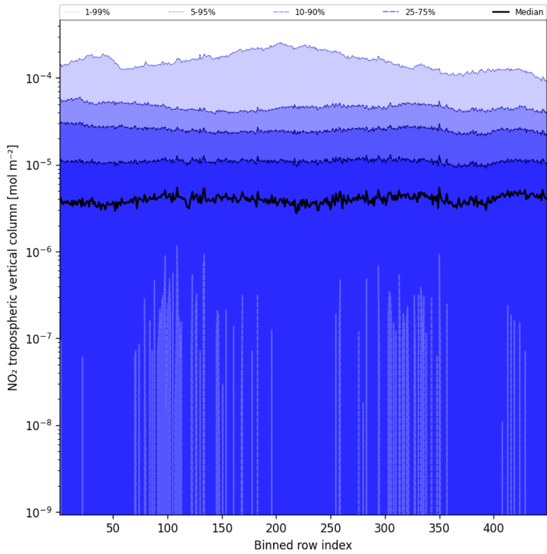
Figure 44: Along track statistics of “NO 2 tropospheric vertical column” for 2025-01-20 to 2025-01-21
