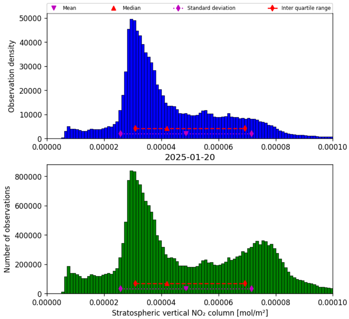
Figure 34: Histogram of “Stratospheric vertical NO 2 column” for 2025-01-20 to 2025-01-21
