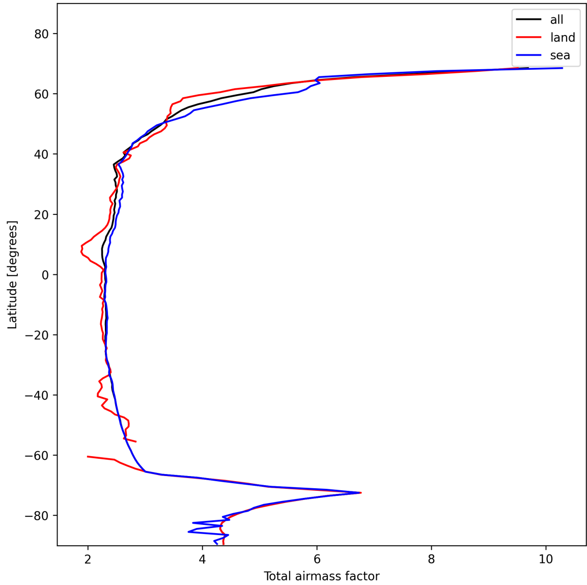
Figure 13: Zonal average of “Total airmass factor” for 2025-01-20 to 2025-01-21.
