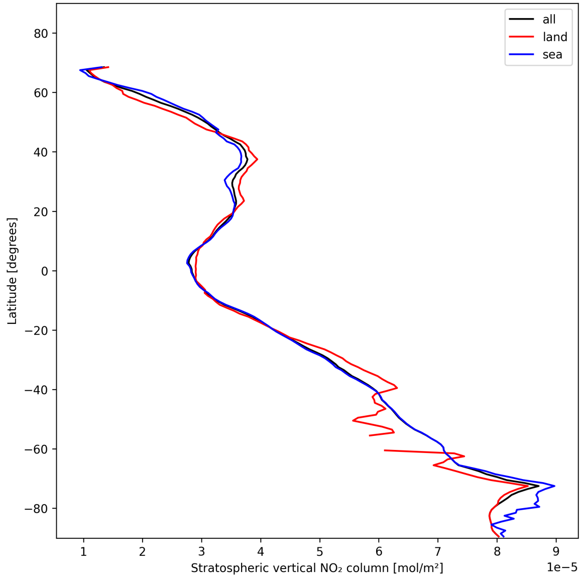
Figure 17: Zonal average of “Stratospheric vertical NO 2 column” for 2025-01-20 to 2025-01-21.
