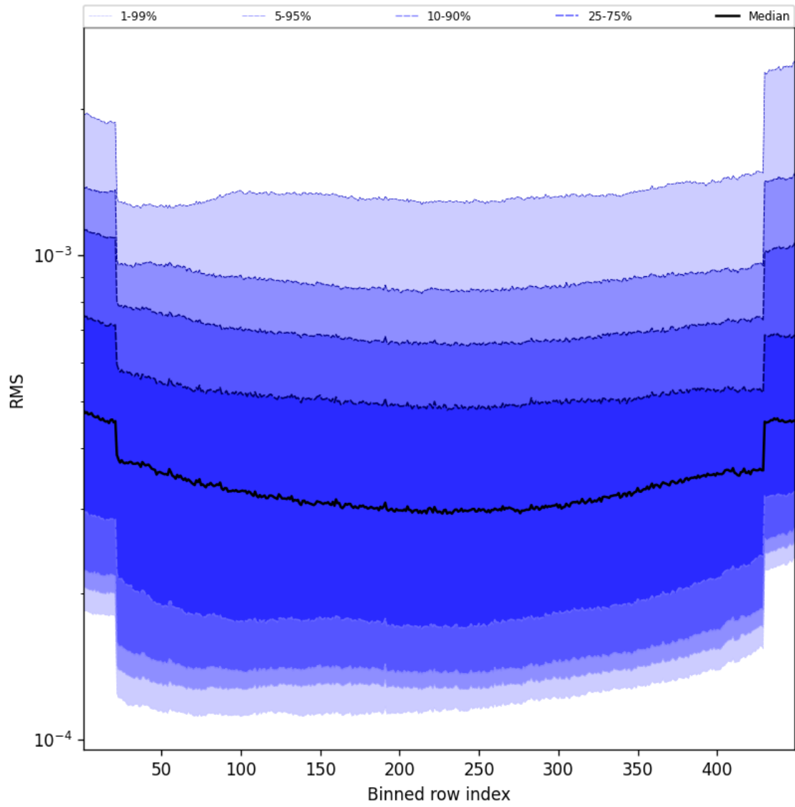
Figure 58: Along track statistics of “RMS” for 2025-01-20 to 2025-01-21
