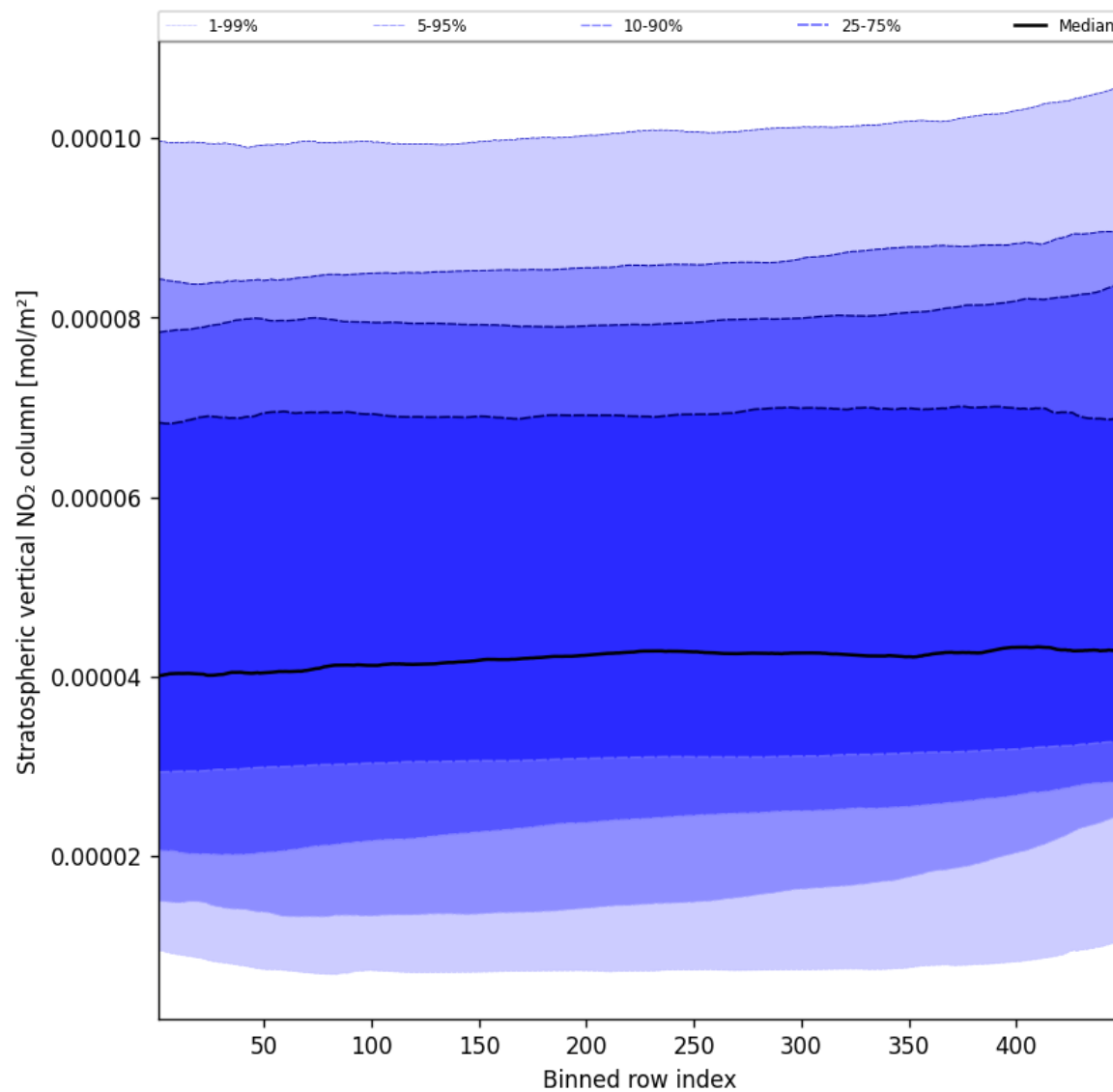
Figure 51: Along track statistics of “Stratospheric vertical NO 2 column” for 2025-01-20 to 2025-01-21
