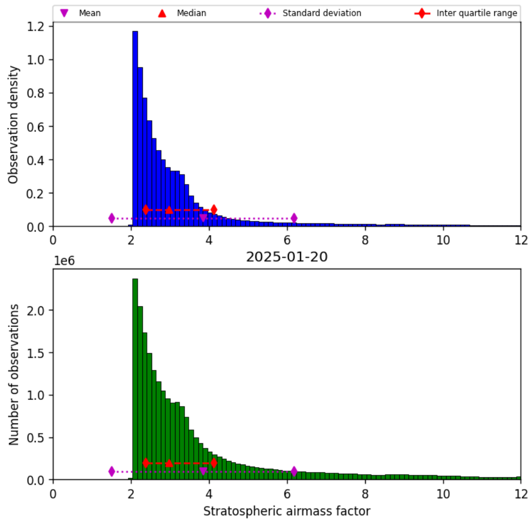
Figure 42: Histogram of “Stratospheric airmass factor” for 2025-01-20 to 2025-01-21
