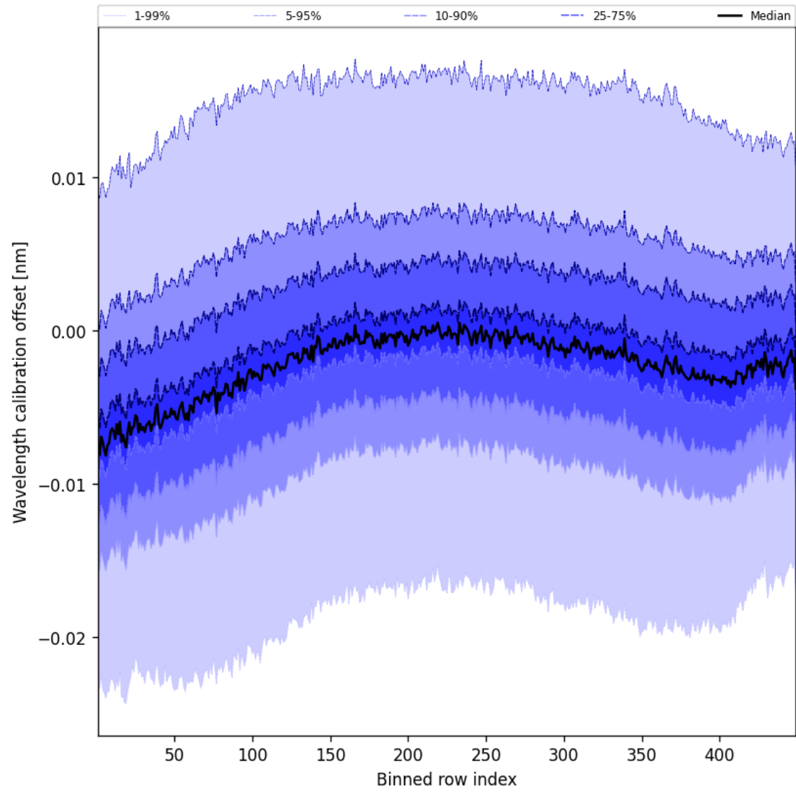
Figure 50: Along track statistics of “Wavelength calibration offset” for 2025-01-20 to 2025-01-21
