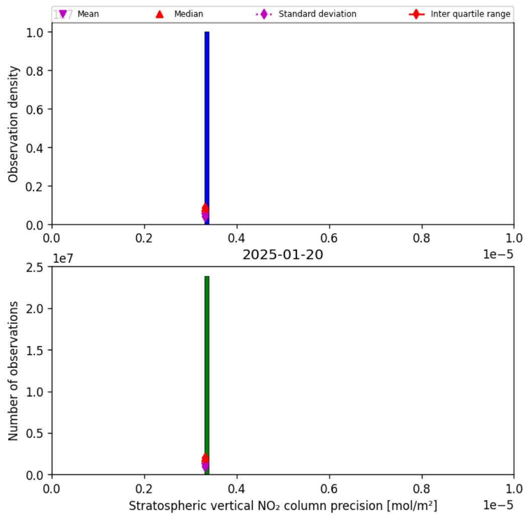
Figure 35: Histogram of “Stratospheric vertical NO 2 column precision” for 2025-01-20 to 2025-01-21
