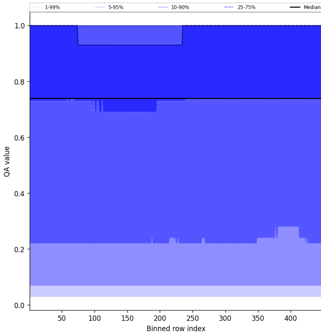
Figure 43: Along track statistics of “QA value” for 2025-01-20 to 2025-01-21
