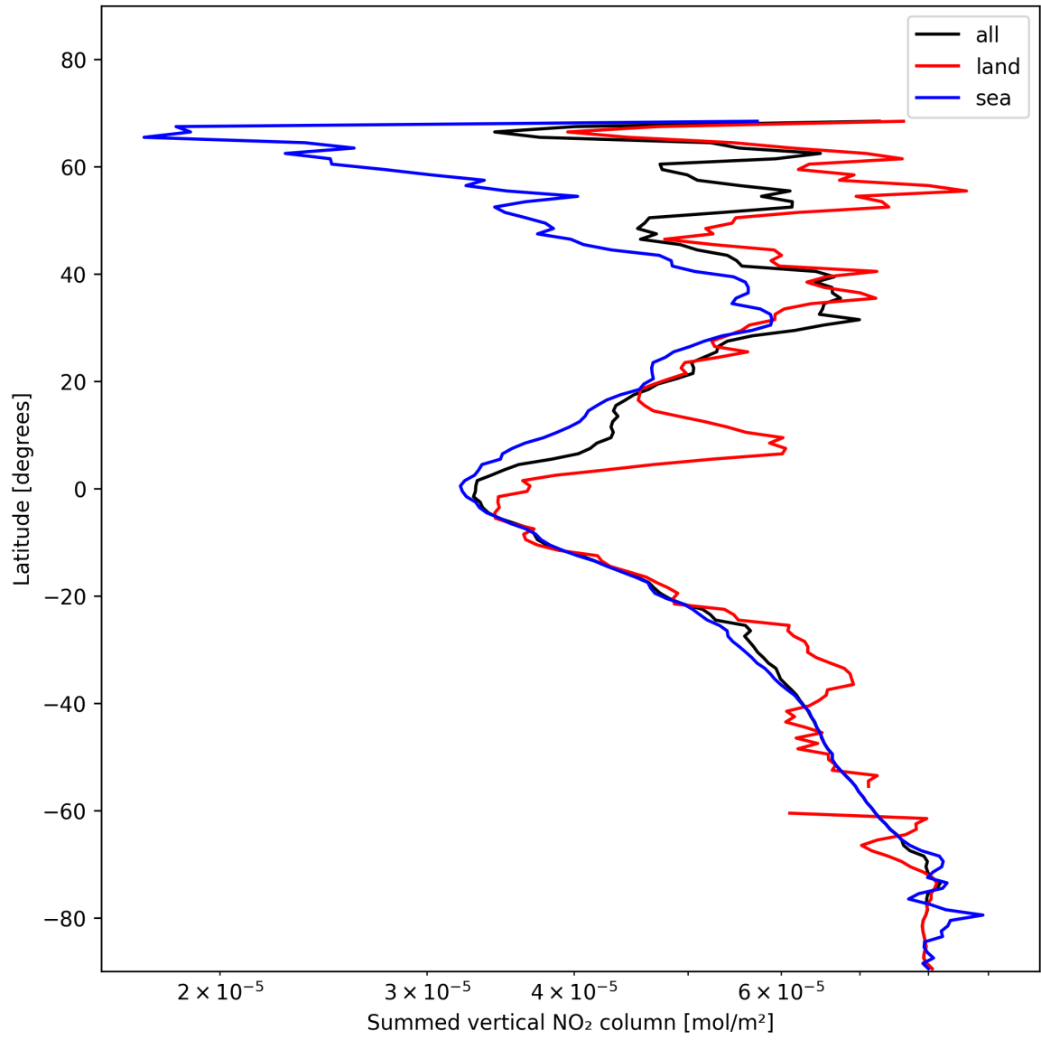
Figure 21: Zonal average of “Summed vertical NO 2 column” for 2025-01-20 to 2025-01-21.
