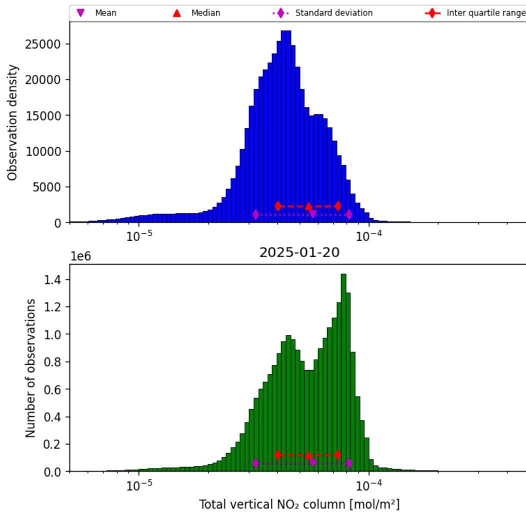
Figure 36: Histogram of “Total vertical NO 2 column” for 2025-01-20 to 2025-01-21
