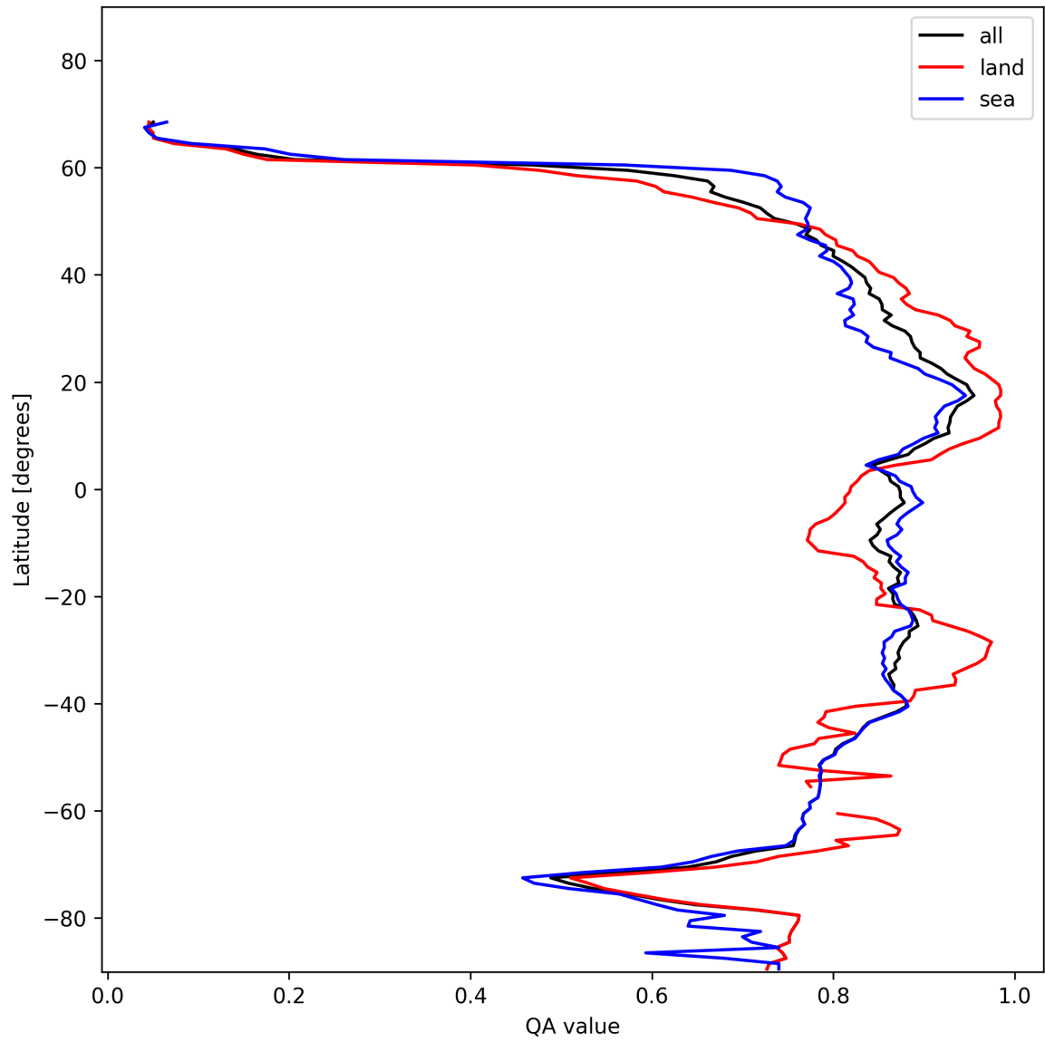
Figure 9: Zonal average of “QA value” for 2025-01-20 to 2025-01-21.
