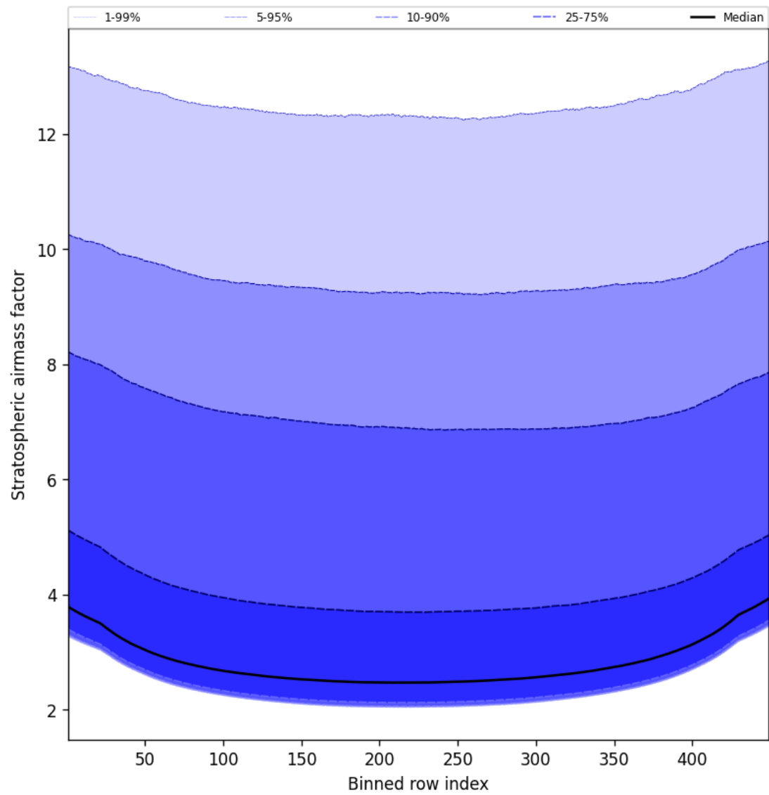
Figure 59: Along track statistics of “Stratospheric airmass factor” for 2025-01-20 to 2025-01-21
