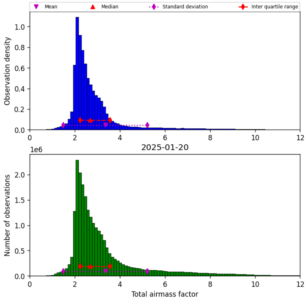
Figure 30: Histogram of “Total airmass factor” for 2025-01-20 to 2025-01-21
