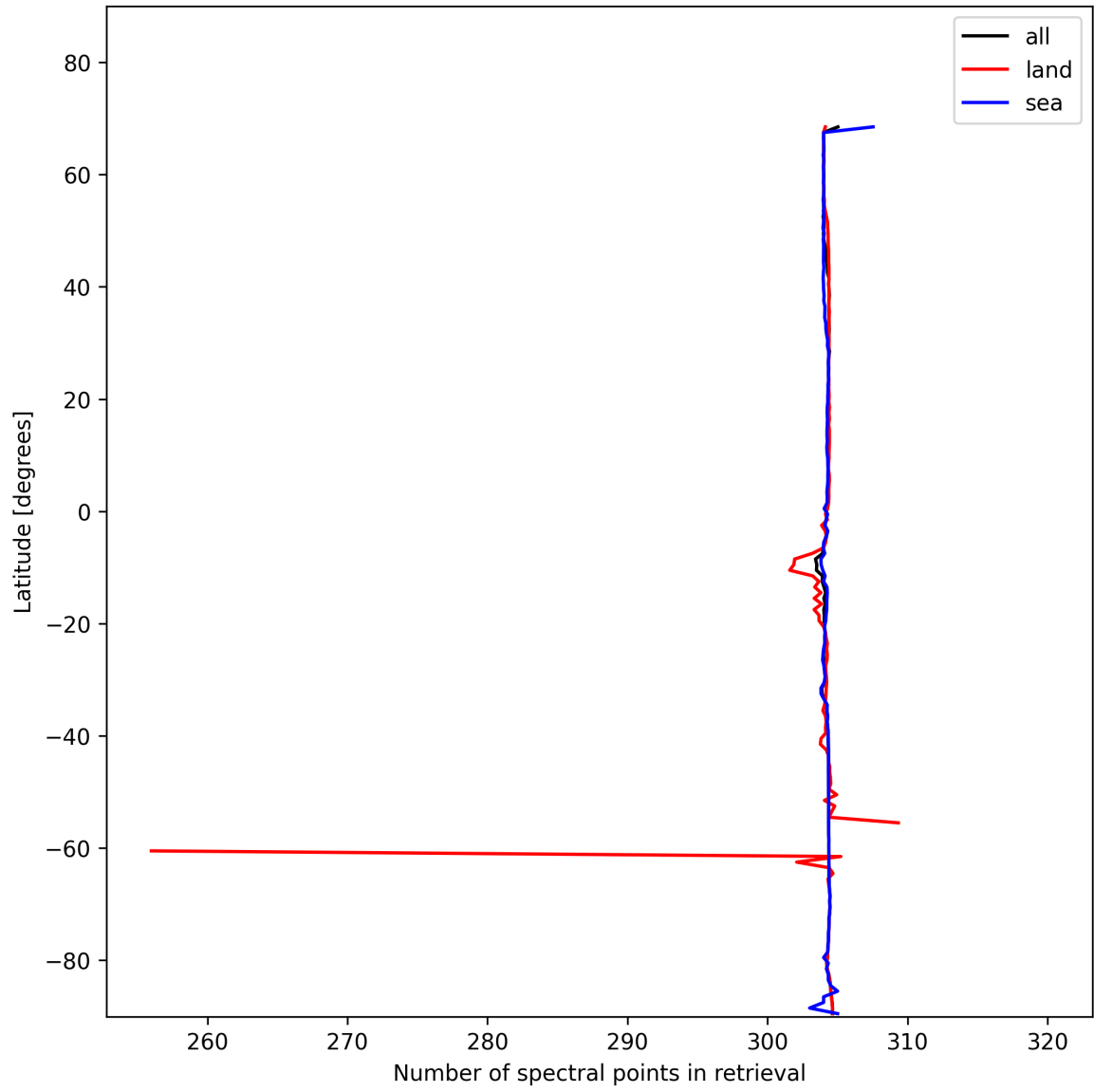
Figure 14: Zonal average of “Number of spectral points in retrieval” for 2025-01-20 to 2025-01-21.
