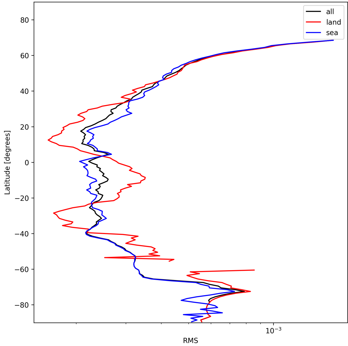
Figure 24: Zonal average of “RMS” for 2025-01-20 to 2025-01-21.
