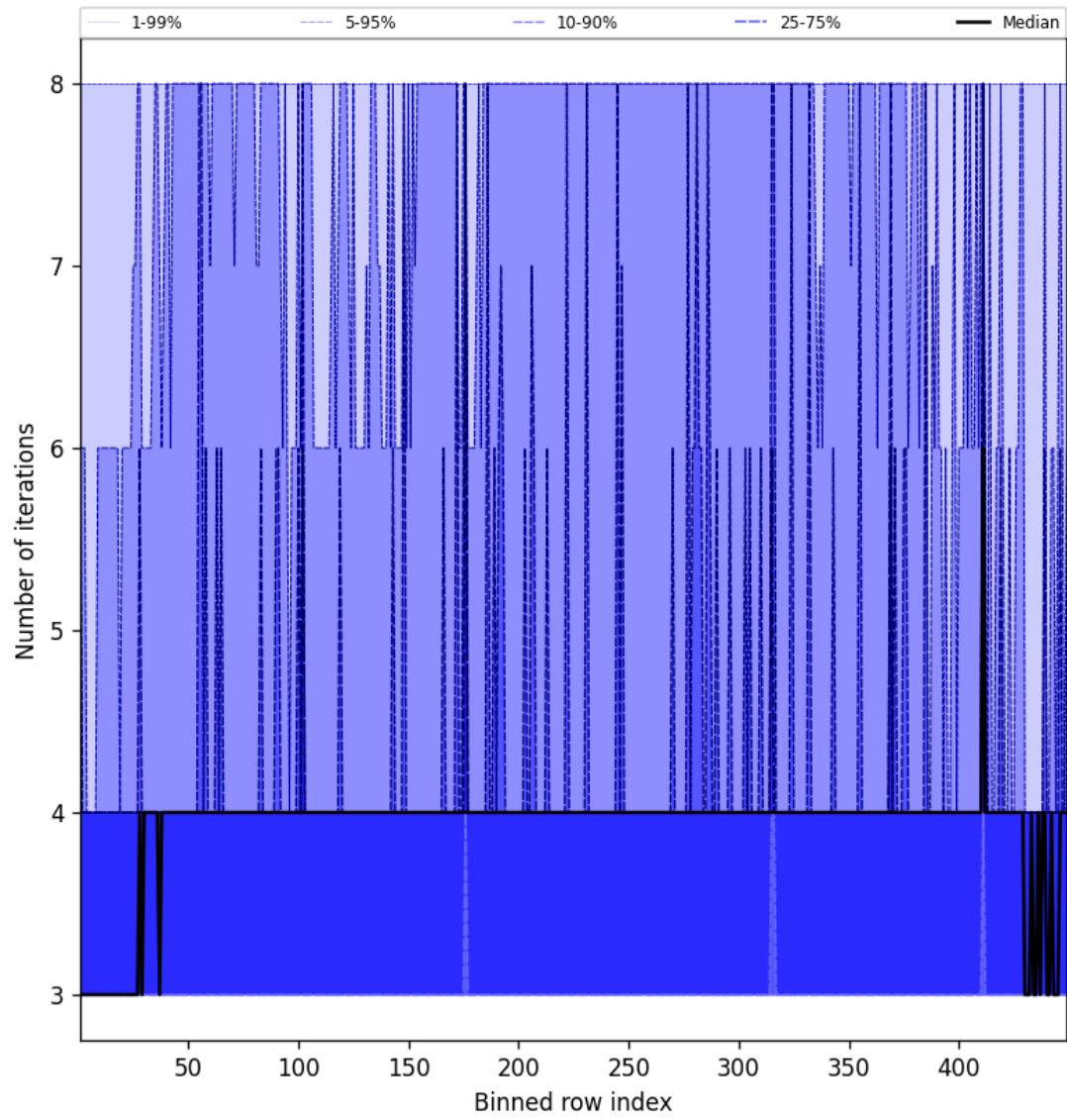
Figure 49: Along track statistics of “Number of iterations” for 2025-01-21 to 2025-01-21
