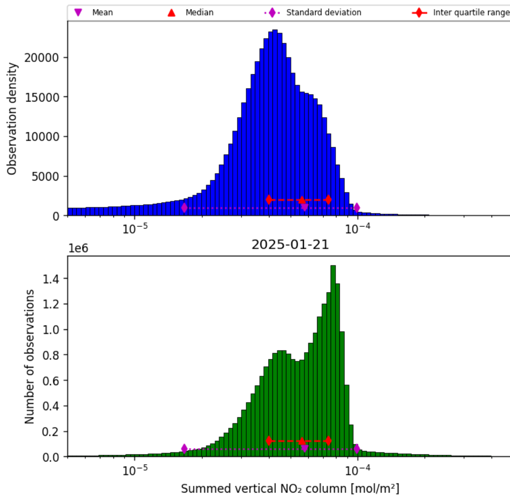
Figure 38: Histogram of "Summed vertical NO 2 column" for 2025-01-21 to 2025-01-21
