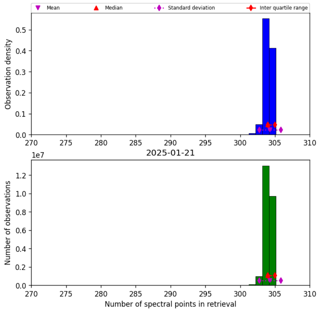
Figure 31: Histogram of “Number of spectral points in retrieval” for 2025-01-21 to 2025-01-21
