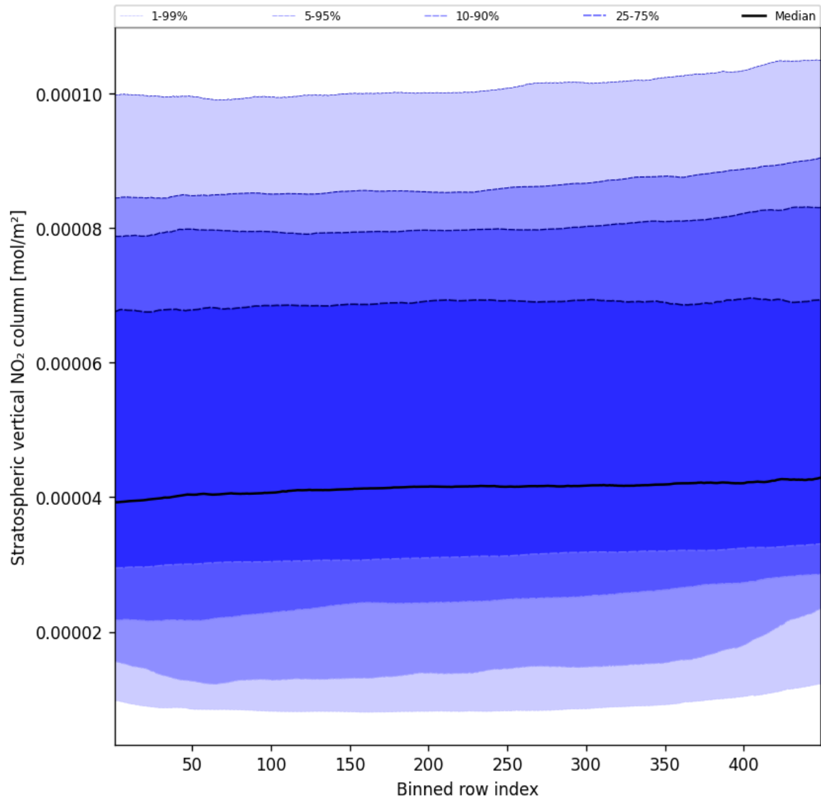
Figure 51: Along track statistics of “Stratospheric vertical NO 2 column” for 2025-01-21 to 2025-01-21
