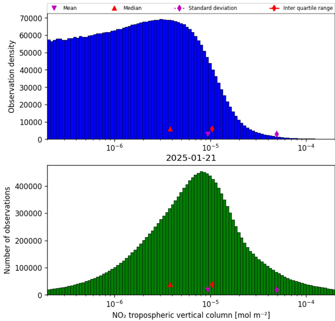
Figure 27: Histogram of “NO 2 tropospheric vertical column” for 2025-01-21 to 2025-01-21
