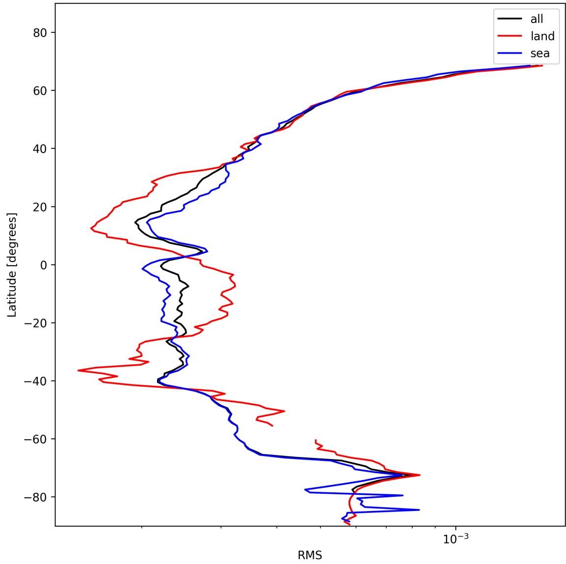
Figure 24: Zonal average of “RMS” for 2025-01-21 to 2025-01-21.
