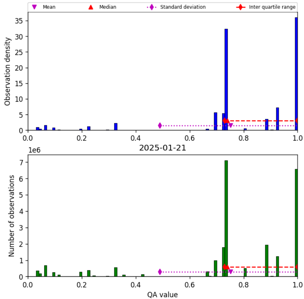
Figure 26: Histogram of “QA value” for 2025-01-21 to 2025-01-21
