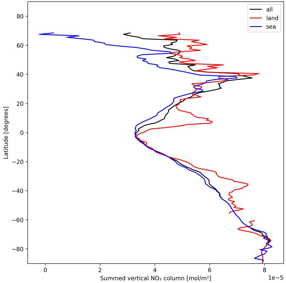
Figure 21: Zonal average of “Summed vertical NO 2 column” for 2025-01-21 to 2025-01-21.
