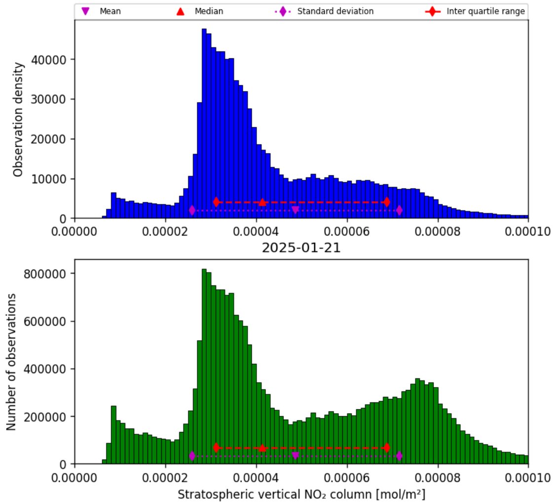
Figure 34: Histogram of “Stratospheric vertical NO 2 column” for 2025-01-21 to 2025-01-21
