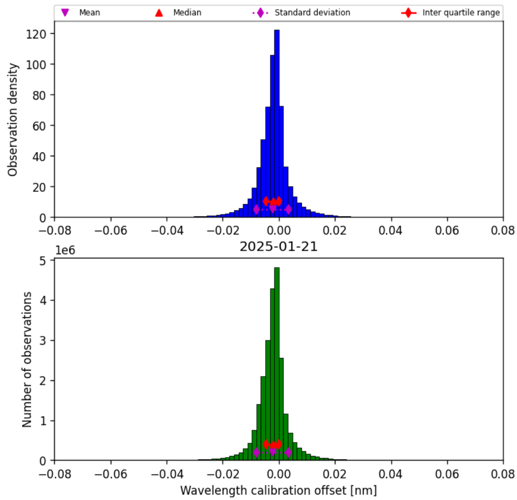
Figure 33: Histogram of “Wavelength calibration offset” for 2025-01-21 to 2025-01-21
