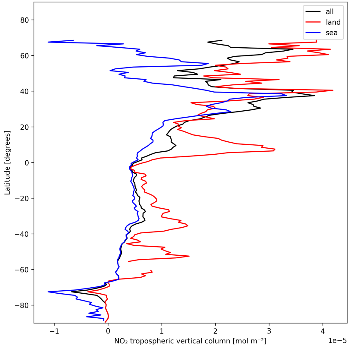
Figure 10: Zonal average of “NO 2 tropospheric vertical column” for 2025-01-21 to 2025-01-21.
