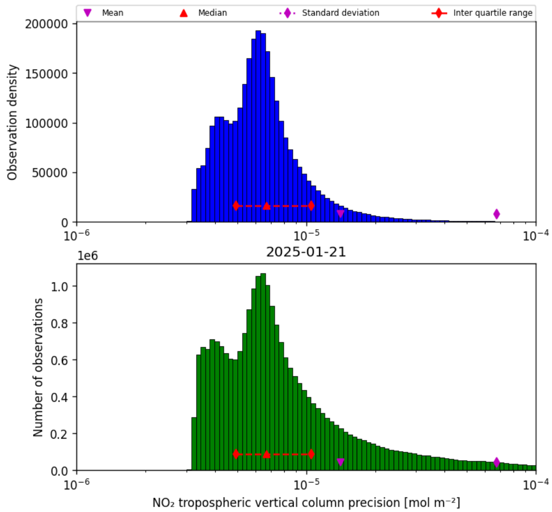
Figure 28: Histogram of “NO 2 tropospheric vertical column precision” for 2025-01-21 to 2025-01-21
