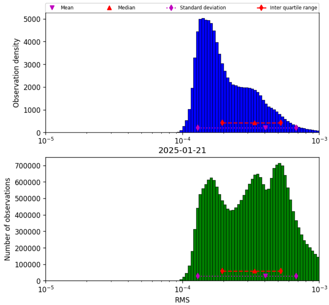
Figure 41: Histogram of “RMS” for 2025-01-21 to 2025-01-21
