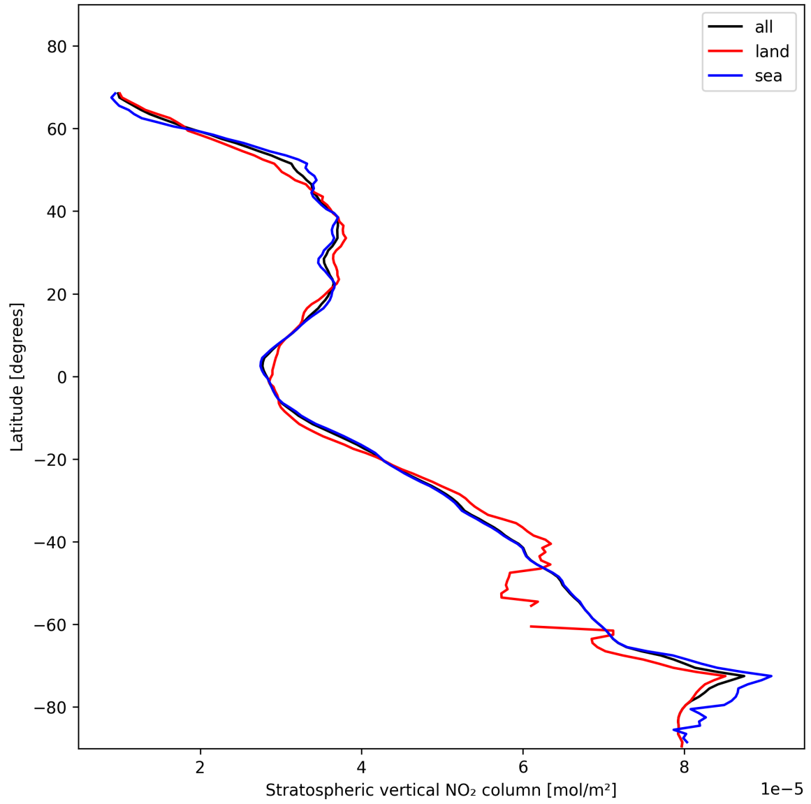
Figure 17: Zonal average of “Stratospheric vertical NO 2 column” for 2025-01-21 to 2025-01-21.
