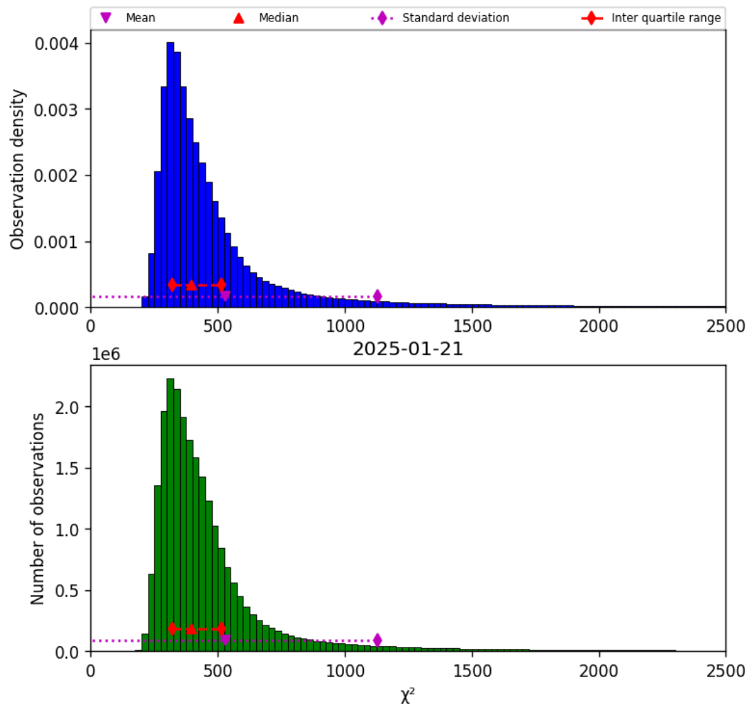
Figure 40: Histogram of " \chi^2 " for 2025-01-21 to 2025-01-21
