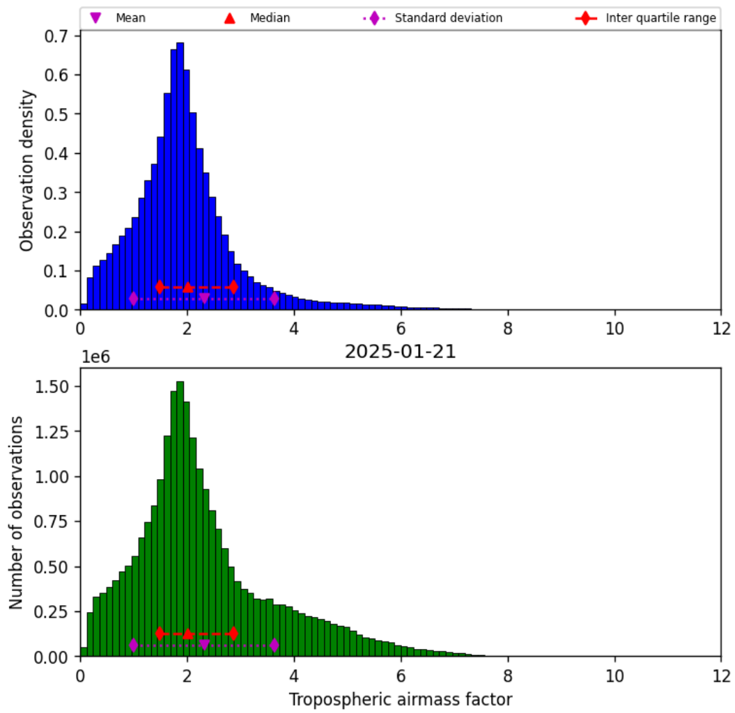
Figure 29: Histogram of “Tropospheric airmass factor” for 2025-01-21 to 2025-01-21
