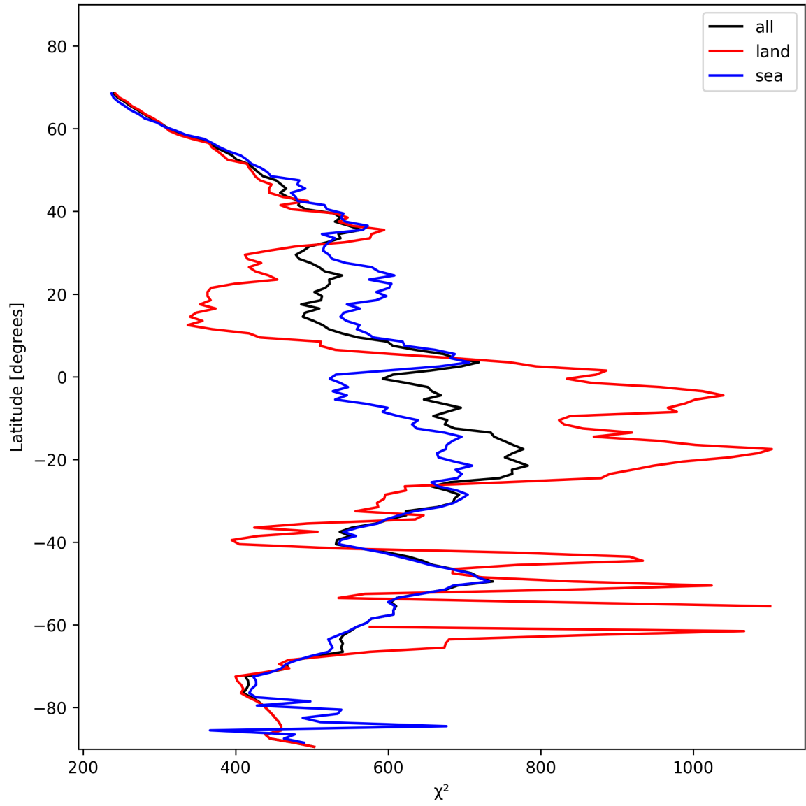
Figure 23: Zonal average of “ \chi^2 ” for 2025-01-21 to 2025-01-21.
