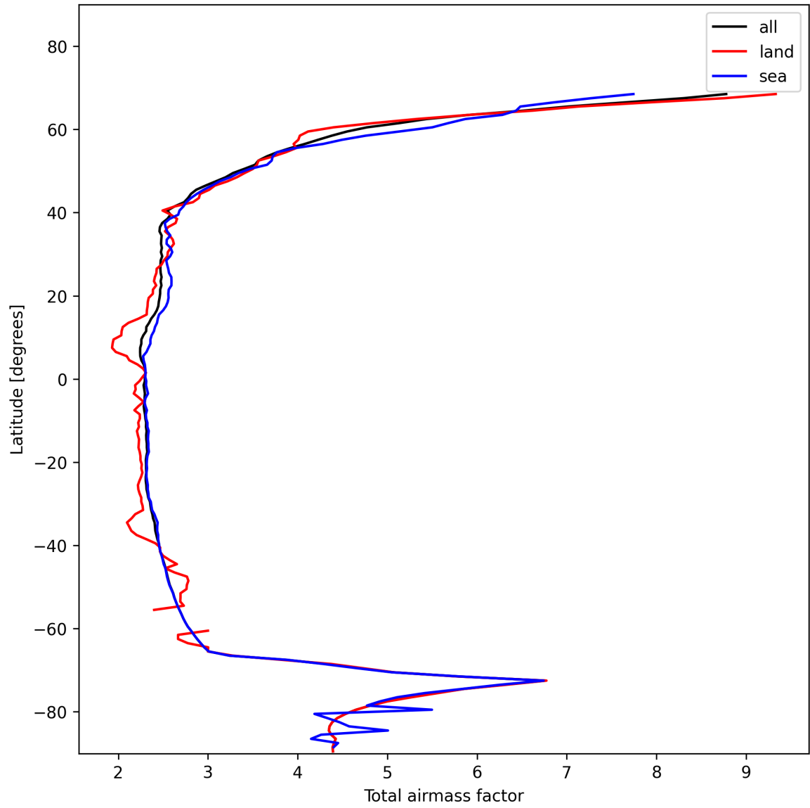
Figure 13: Zonal average of “Total airmass factor” for 2025-01-21 to 2025-01-21.
