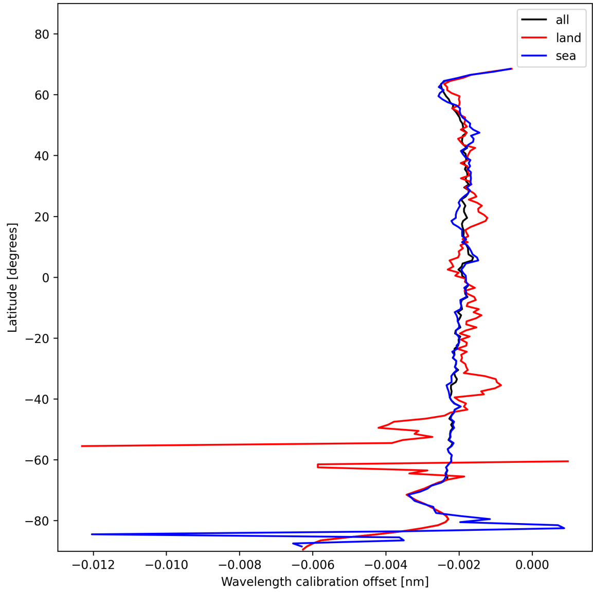
Figure 16: Zonal average of “Wavelength calibration offset” for 2025-01-21 to 2025-01-21.
