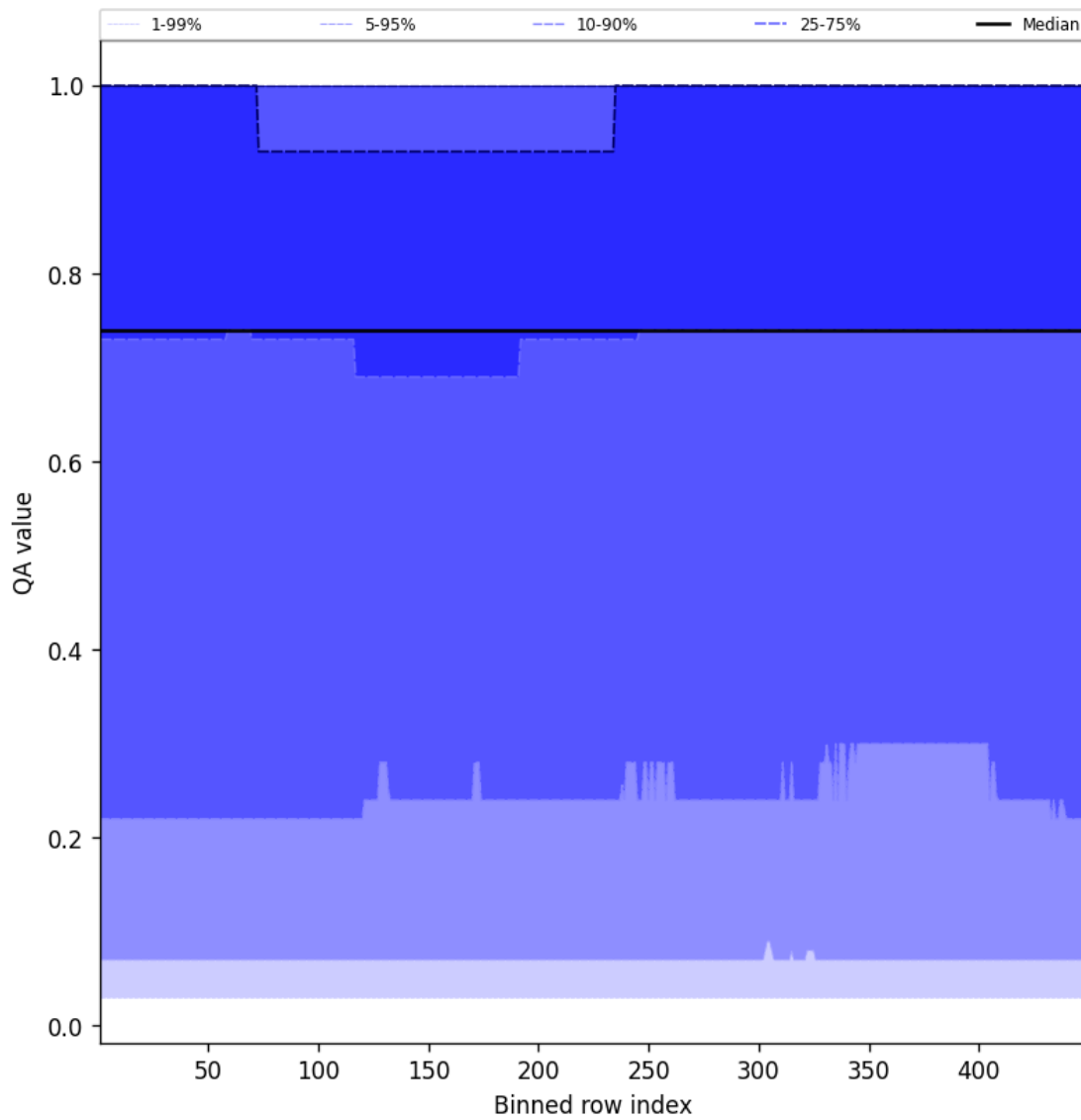
Figure 43: Along track statistics of “QA value” for 2025-01-21 to 2025-01-21
