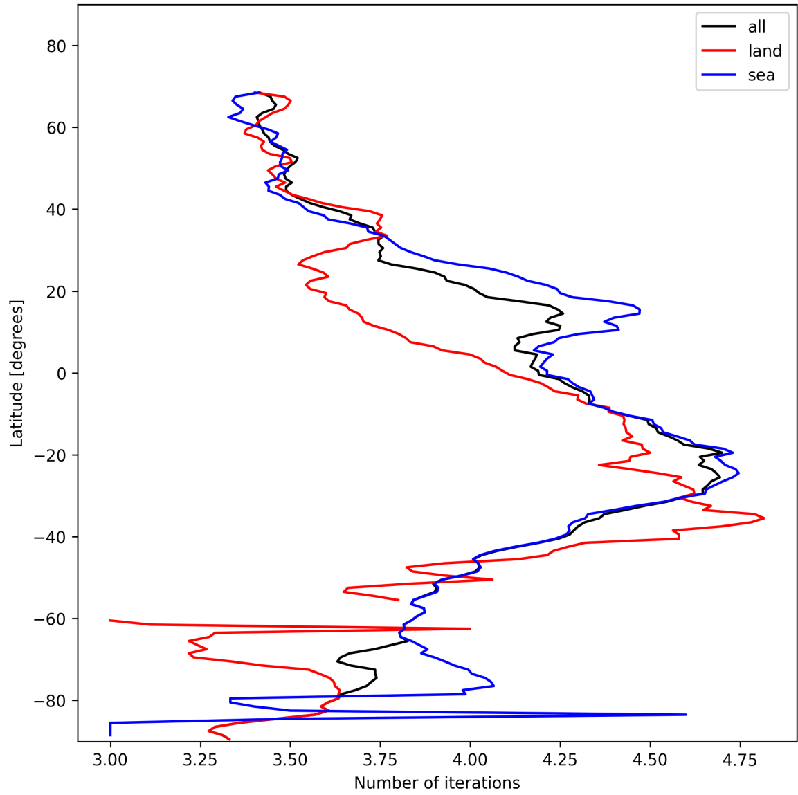
Figure 15: Zonal average of “Number of iterations” for 2025-01-21 to 2025-01-21.
