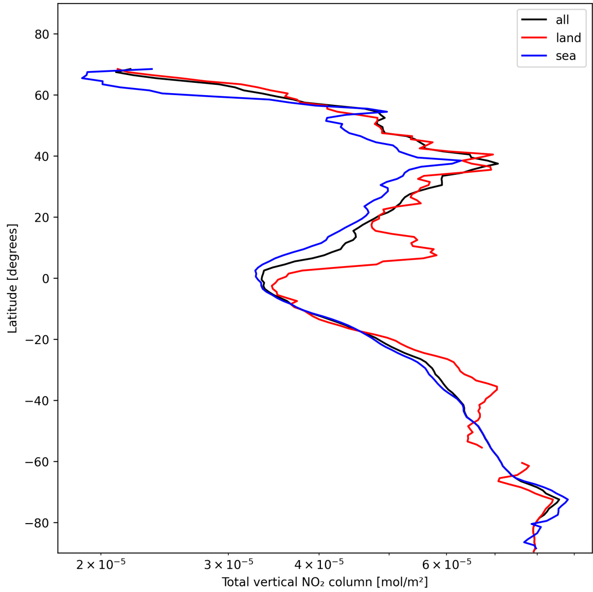
Figure 19: Zonal average of “Total vertical NO 2 column” for 2025-01-21 to 2025-01-21.
