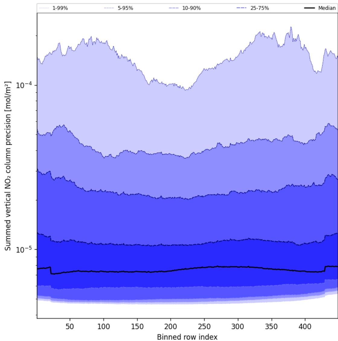
Figure 56: Along track statistics of “Summed vertical NO 2 column precision” for 2025-01-21 to 2025-01-21
