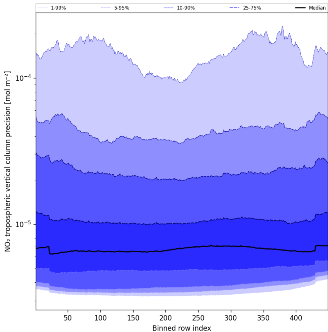
Figure 45: Along track statistics of “NO 2 tropospheric vertical column precision” for 2025-01-21 to 2025-01-21
