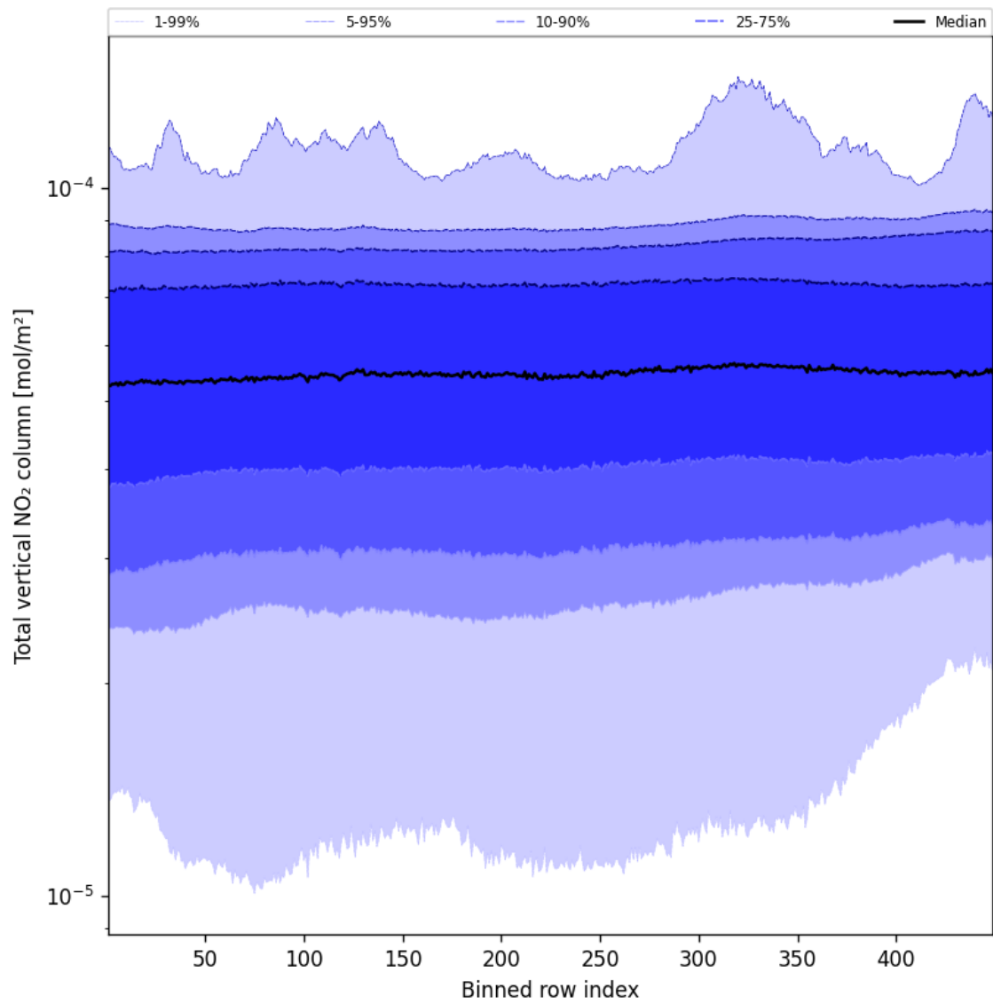
Figure 53: Along track statistics of “Total vertical NO 2 column” for 2025-01-21 to 2025-01-21
