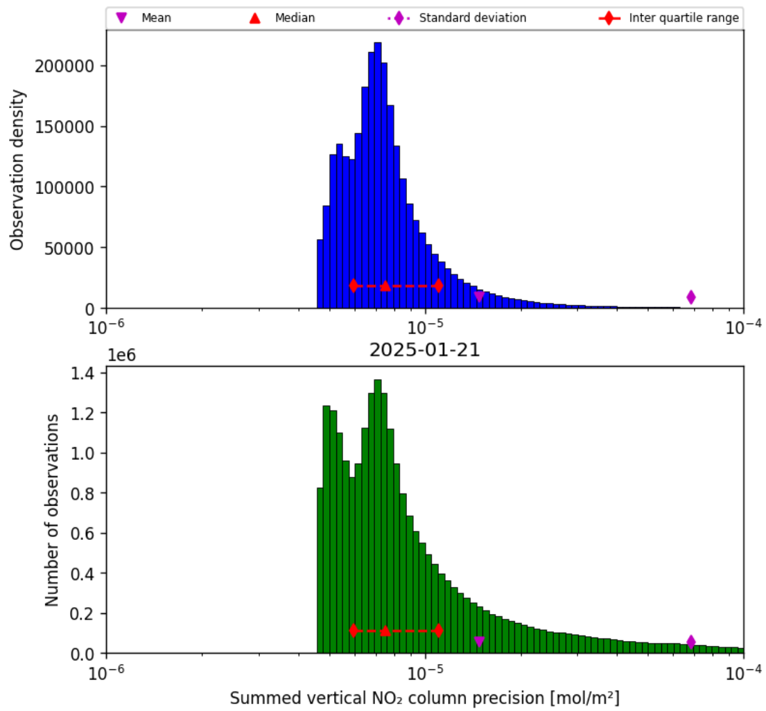
Figure 39: Histogram of "Summed vertical NO 2 column precision" for 2025-01-21 to 2025-01-21
