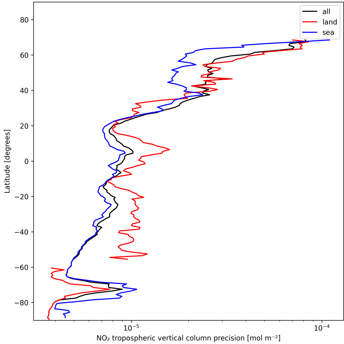
Figure 11: Zonal average of “NO 2 tropospheric vertical column precision” for 2025-01-21 to 2025-01-21.
