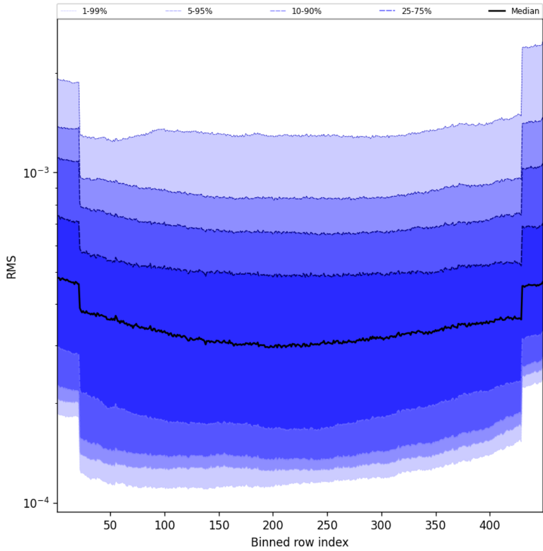
Figure 58: Along track statistics of “RMS” for 2025-01-21 to 2025-01-21
