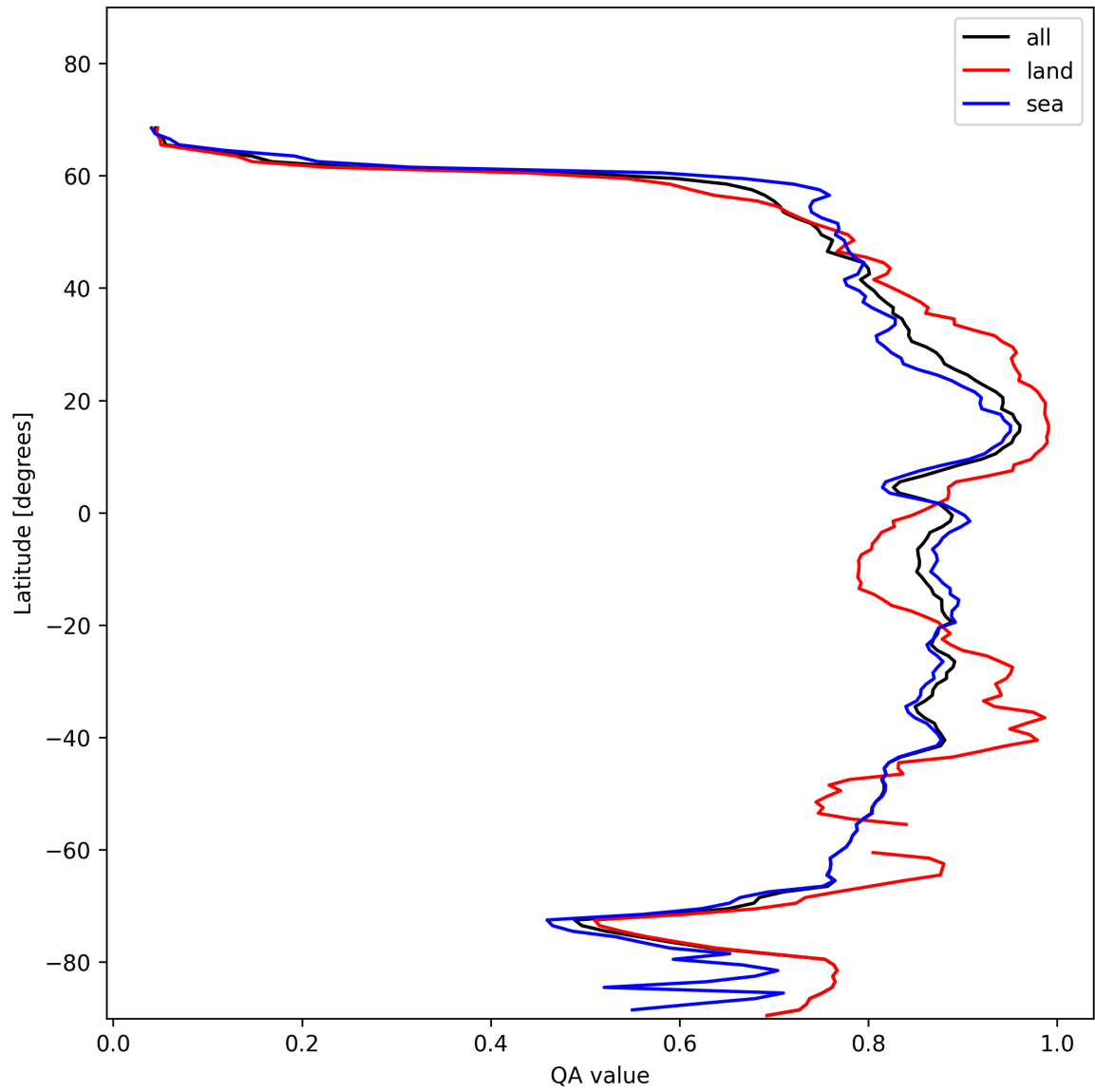
Figure 9: Zonal average of “QA value” for 2025-01-21 to 2025-01-21.
