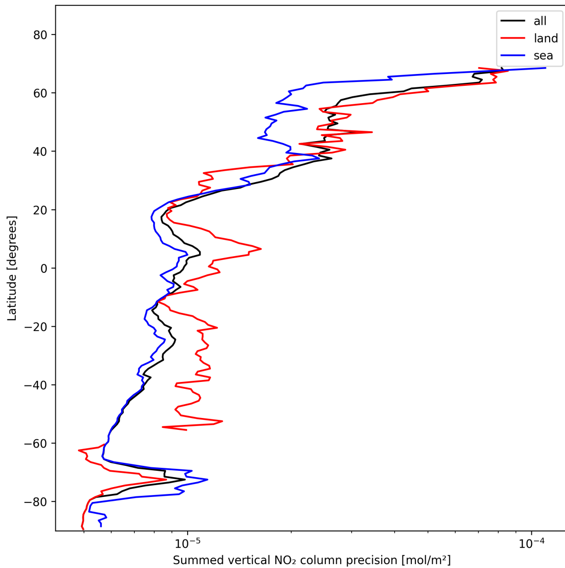
Figure 22: Zonal average of “Summed vertical NO 2 column precision” for 2025-01-21 to 2025-01-21.
