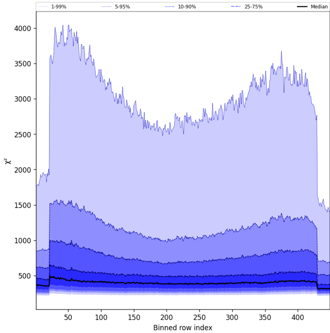
Figure 57: Along track statistics of “ \chi^2 ” for 2025-01-21 to 2025-01-21
