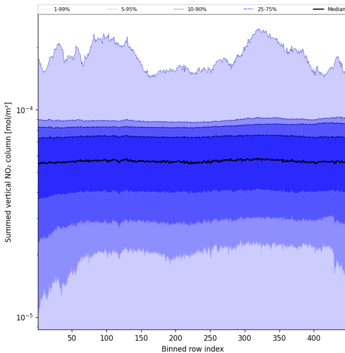
Figure 55: Along track statistics of “Summed vertical NO 2 column” for 2025-01-21 to 2025-01-21
