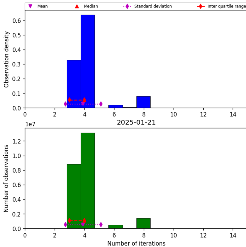
Figure 32: Histogram of “Number of iterations” for 2025-01-21 to 2025-01-21
