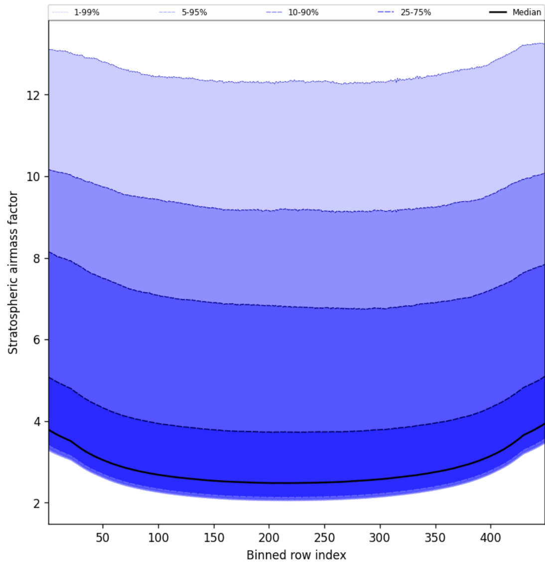
Figure 59: Along track statistics of “Stratospheric airmass factor” for 2025-01-21 to 2025-01-21
