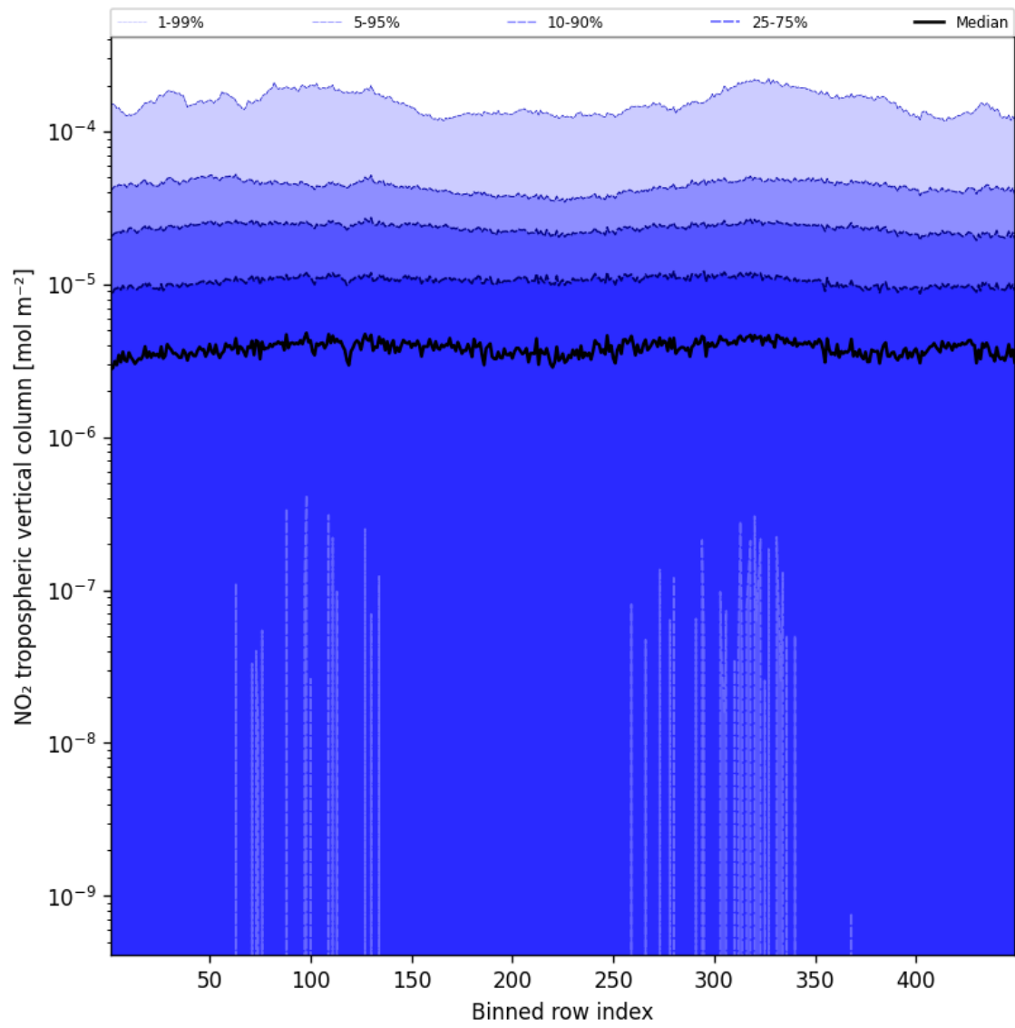
Figure 44: Along track statistics of “NO 2 tropospheric vertical column” for 2025-01-21 to 2025-01-21
