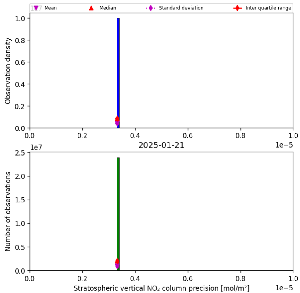
Figure 35: Histogram of “Stratospheric vertical NO 2 column precision” for 2025-01-21 to 2025-01-21
