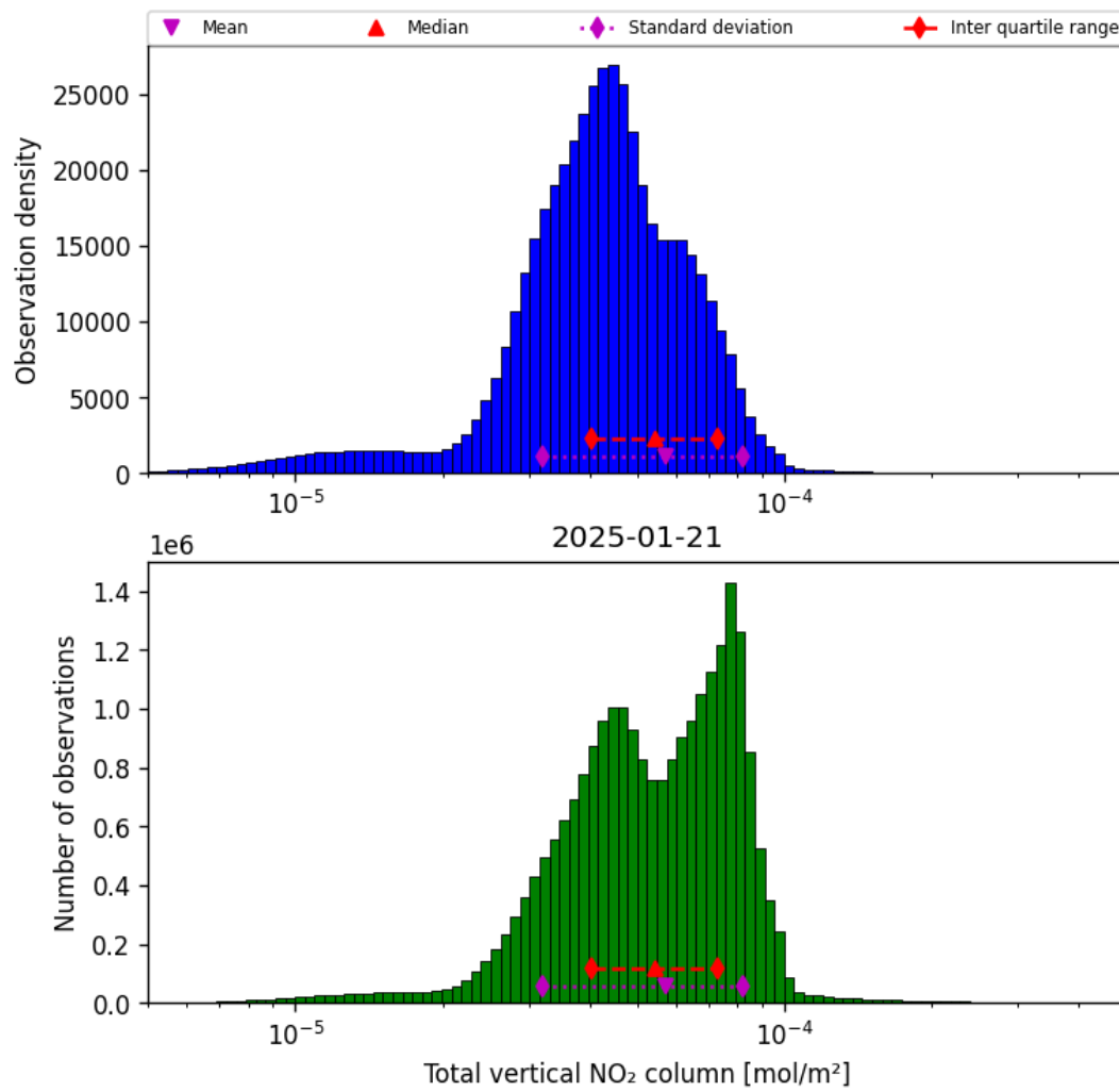
Figure 36: Histogram of “Total vertical NO 2 column” for 2025-01-21 to 2025-01-21
