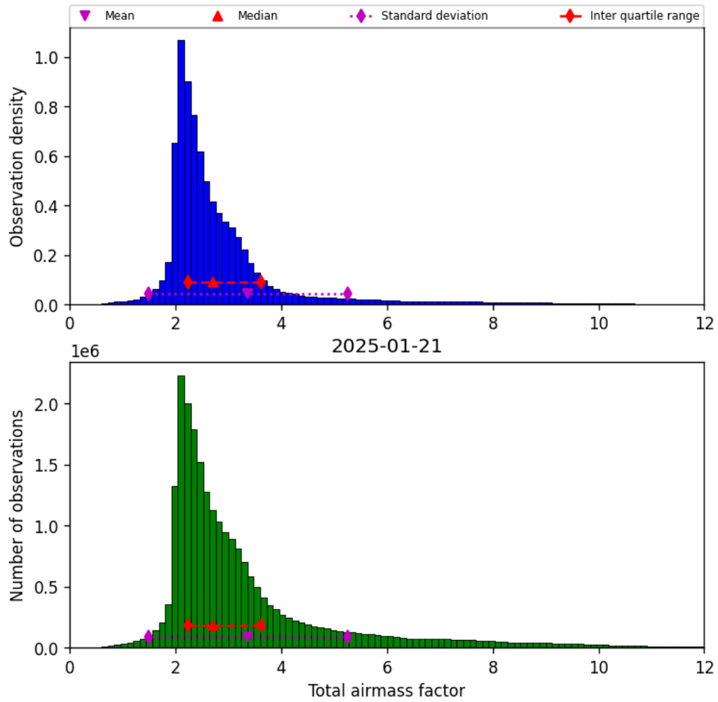
Figure 30: Histogram of “Total airmass factor” for 2025-01-21 to 2025-01-21
