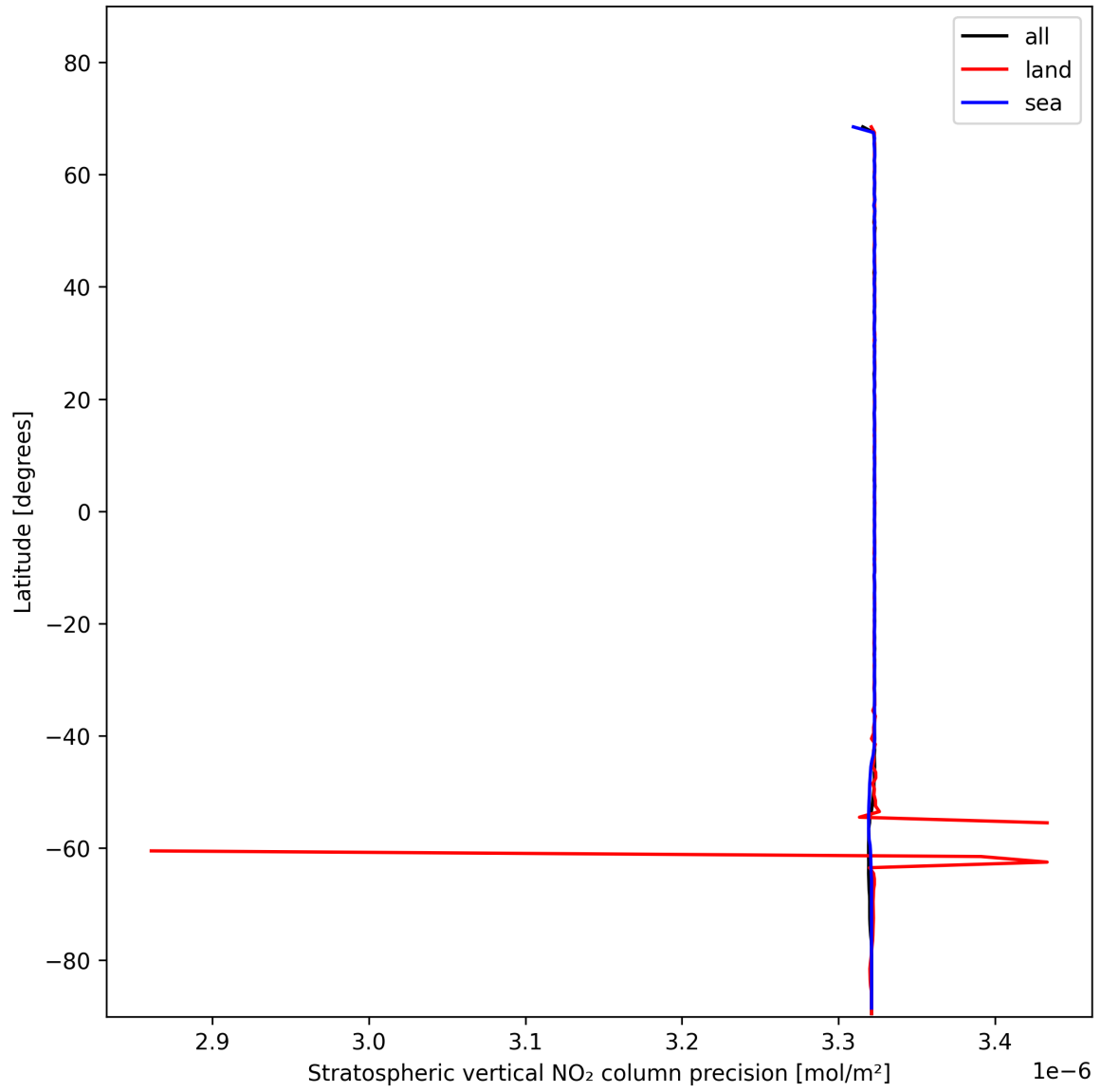
Figure 18: Zonal average of “Stratospheric vertical NO 2 column precision” for 2025-01-21 to 2025-01-21.
