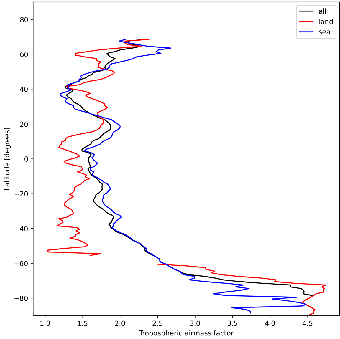
Figure 12: Zonal average of “Tropospheric airmass factor” for 2025-01-21 to 2025-01-21.
