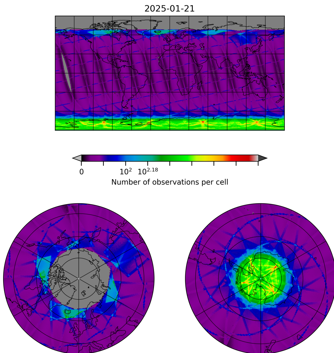
Figure 8: Map of the number of observations for 2025-01-21 to 2025-01-21
