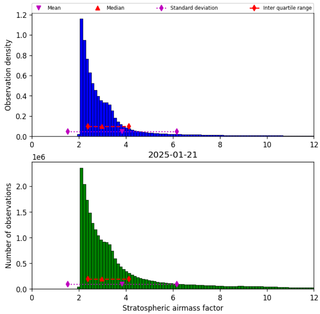
Figure 42: Histogram of “Stratospheric airmass factor” for 2025-01-21 to 2025-01-21
