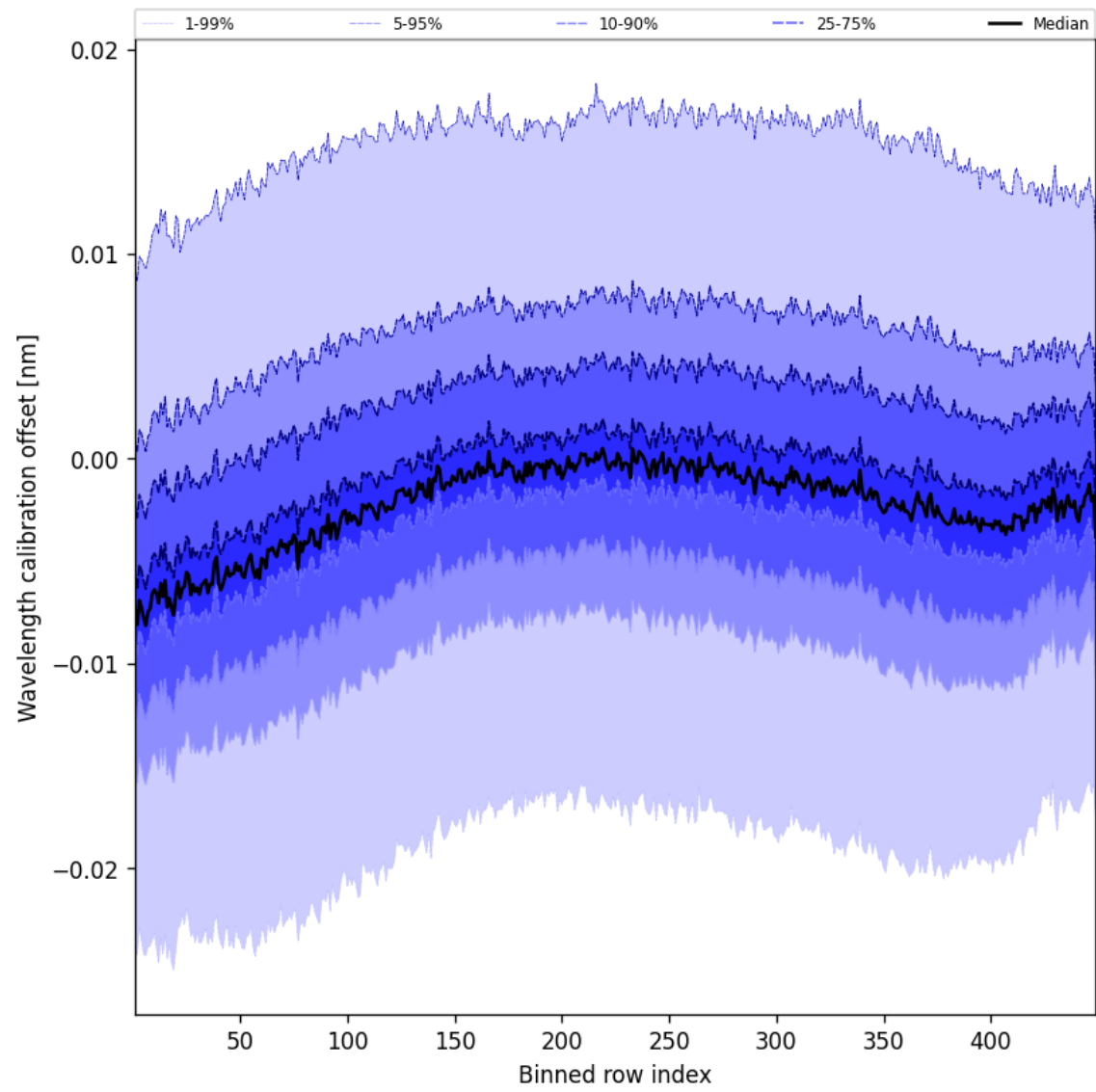
Figure 50: Along track statistics of “Wavelength calibration offset” for 2025-01-21 to 2025-01-21
