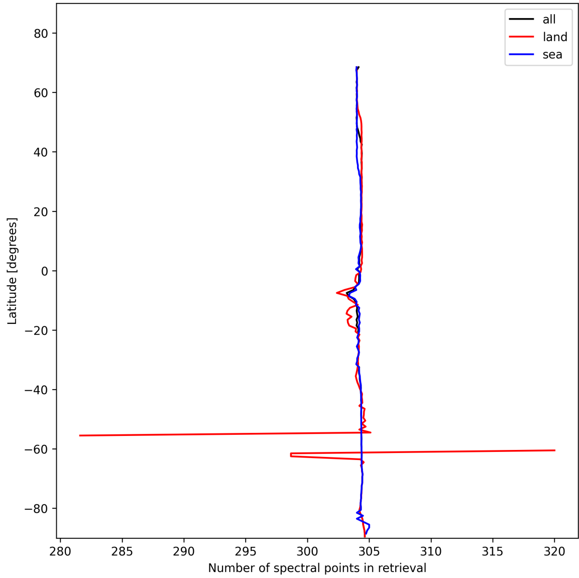
Figure 14: Zonal average of “Number of spectral points in retrieval” for 2025-01-21 to 2025-01-21.
