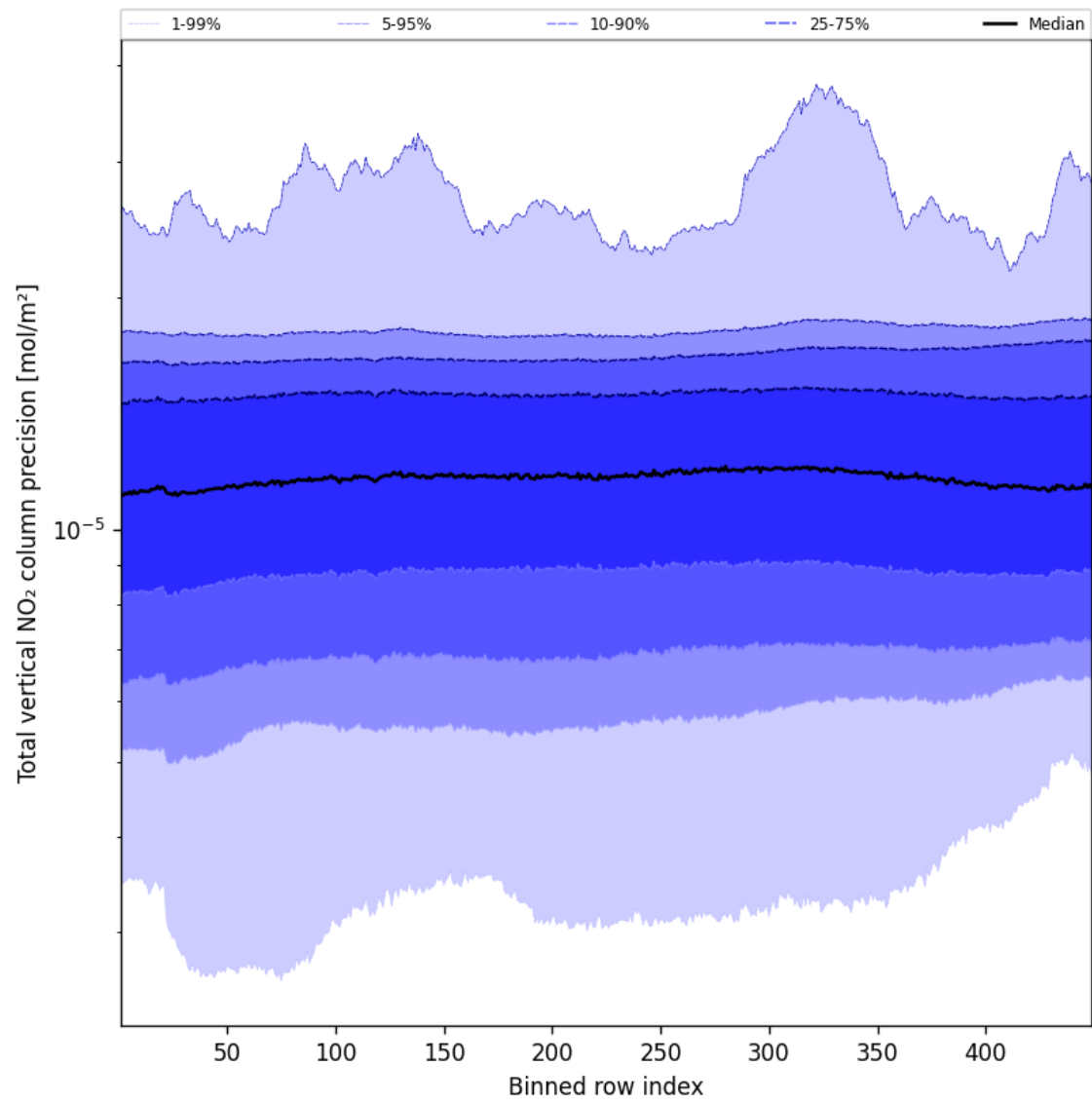
Figure 54: Along track statistics of “Total vertical NO 2 column precision” for 2025-01-21 to 2025-01-21
