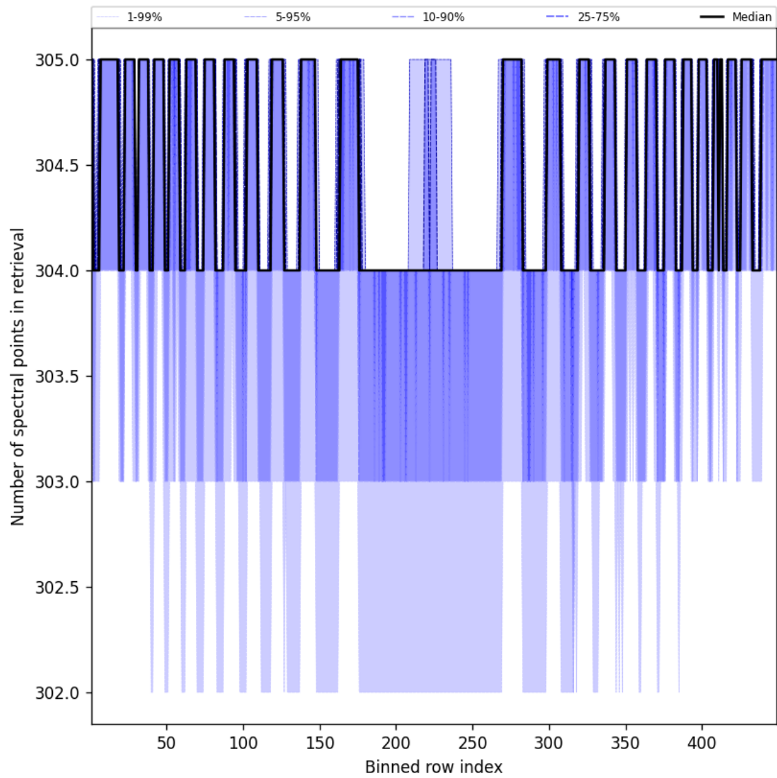
Figure 48: Along track statistics of “Number of spectral points in retrieval” for 2025-01-21 to 2025-01-21
