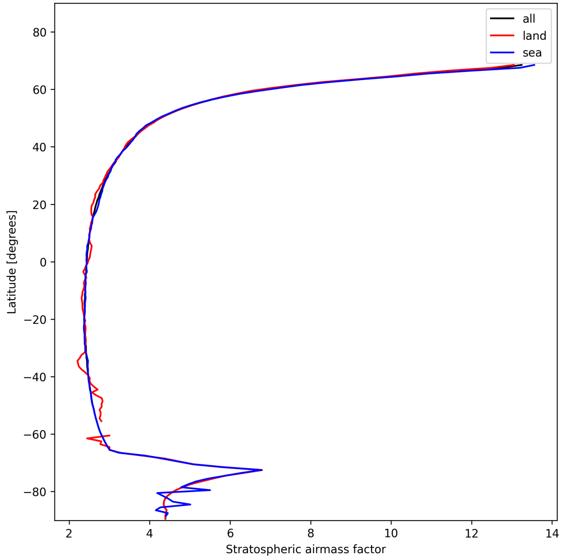
Figure 25: Zonal average of “Stratospheric airmass factor” for 2025-01-21 to 2025-01-21.
