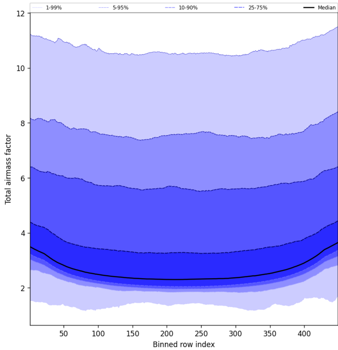
Figure 47: Along track statistics of “Total airmass factor” for 2025-01-21 to 2025-01-21
