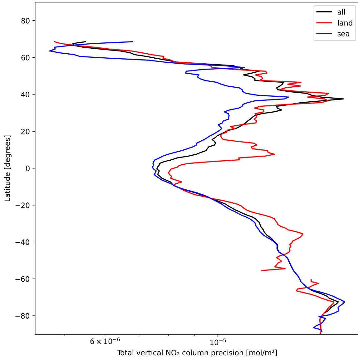
Figure 20: Zonal average of “Total vertical NO 2 column precision” for 2025-01-21 to 2025-01-21.
