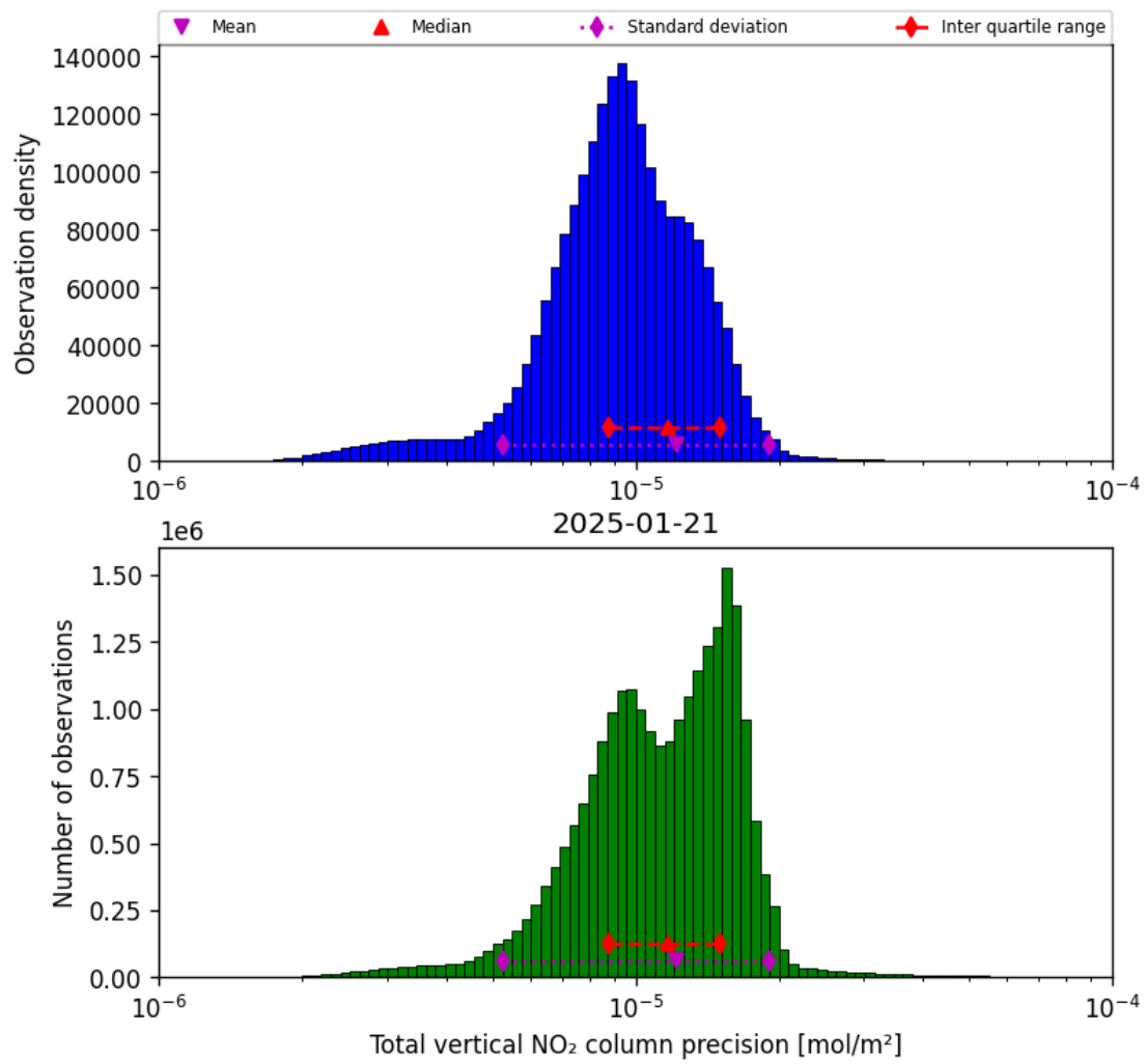
Figure 37: Histogram of "Total vertical NO 2 column precision" for 2025-01-21 to 2025-01-21
