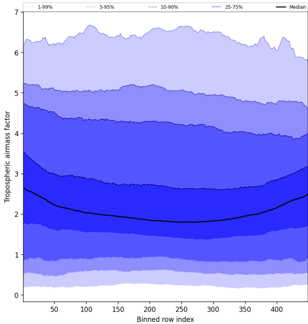
Figure 46: Along track statistics of “Tropospheric airmass factor” for 2025-01-21 to 2025-01-21
