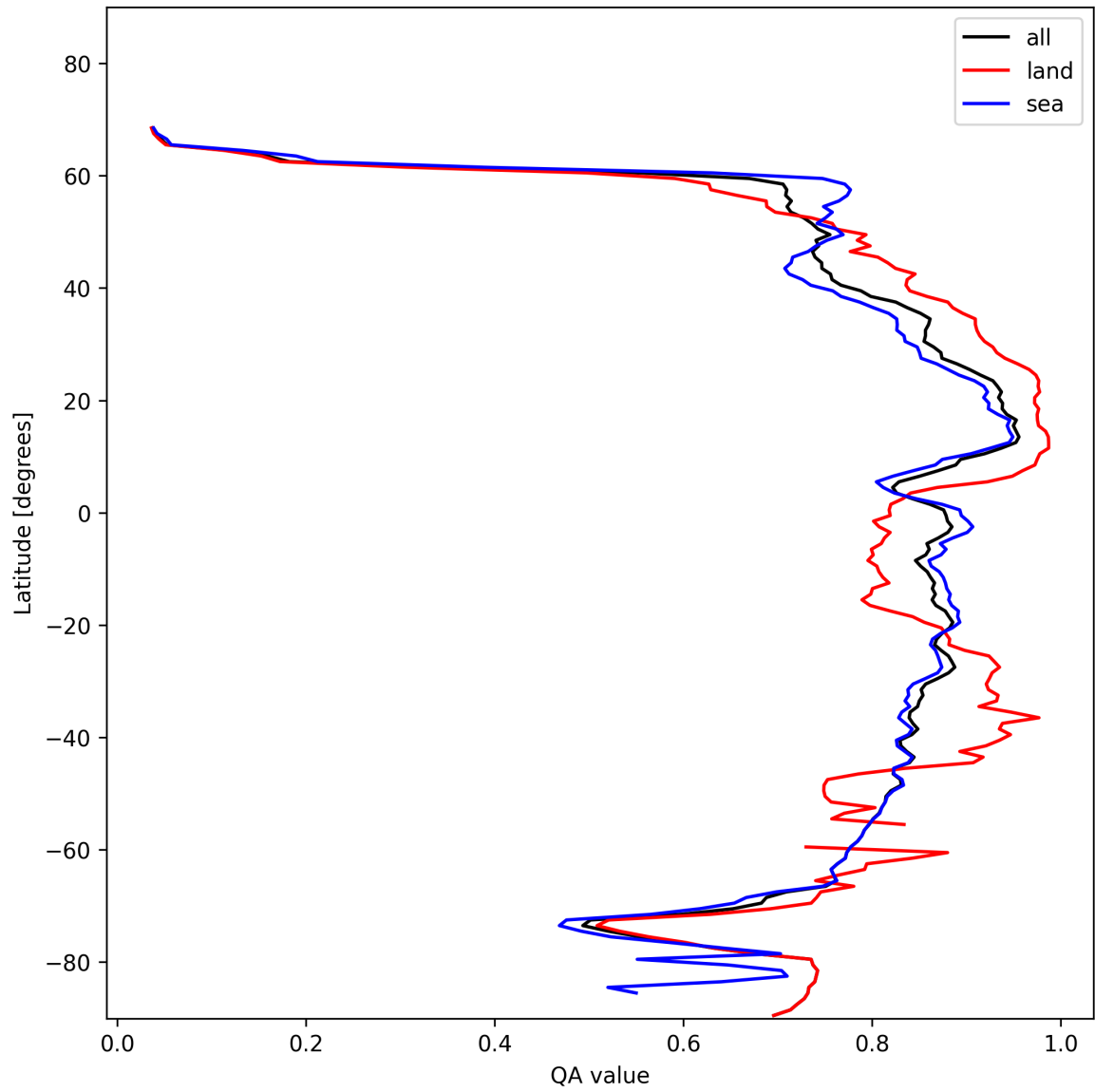
Figure 9: Zonal average of “QA value” for 2025-01-22 to 2025-01-23.
