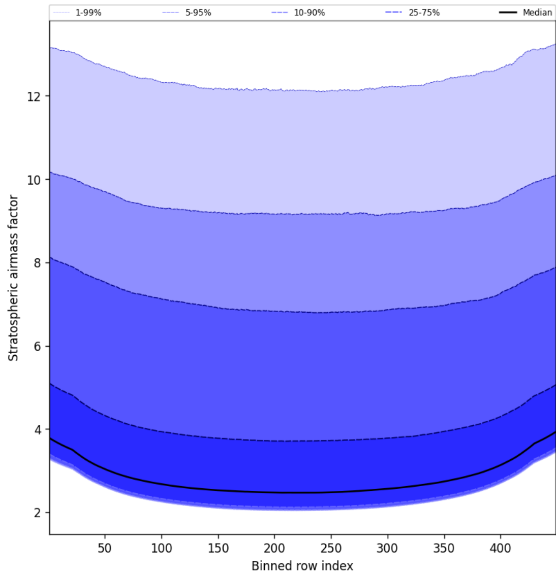
Figure 59: Along track statistics of “Stratospheric airmass factor” for 2025-01-22 to 2025-01-23
