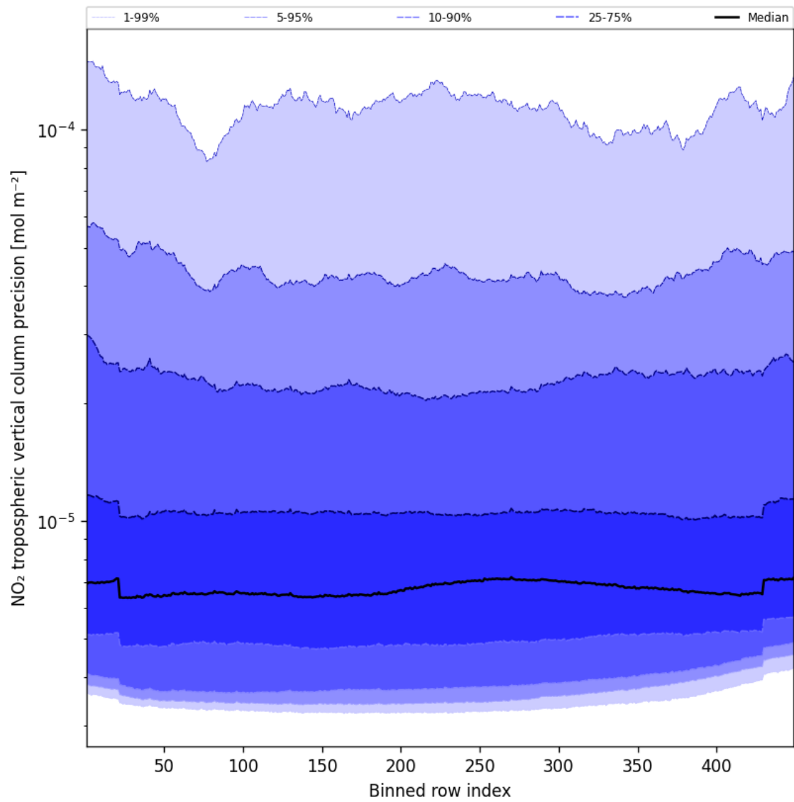
Figure 45: Along track statistics of “NO 2 tropospheric vertical column precision” for 2025-01-22 to 2025-01-23
