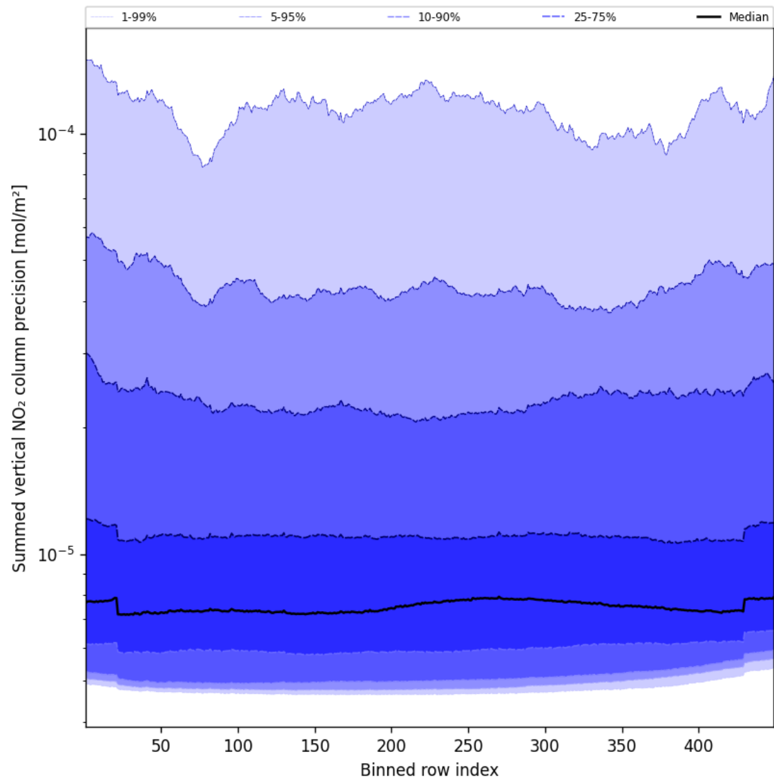
Figure 56: Along track statistics of “Summed vertical NO 2 column precision” for 2025-01-22 to 2025-01-23
