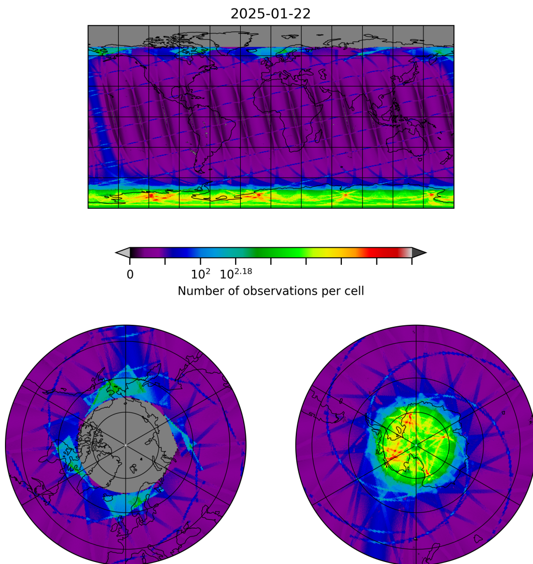
Figure 8: Map of the number of observations for 2025-01-22 to 2025-01-23
