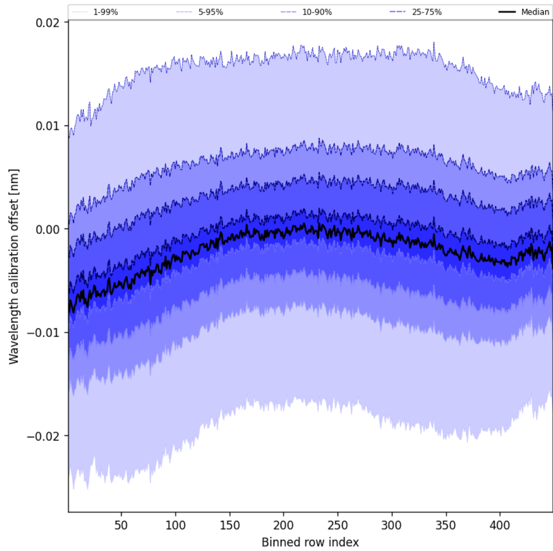
Figure 50: Along track statistics of “Wavelength calibration offset” for 2025-01-22 to 2025-01-23
