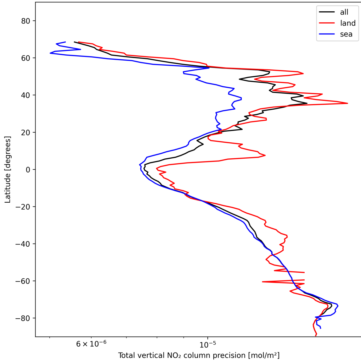
Figure 20: Zonal average of “Total vertical NO 2 column precision” for 2025-01-22 to 2025-01-23.
