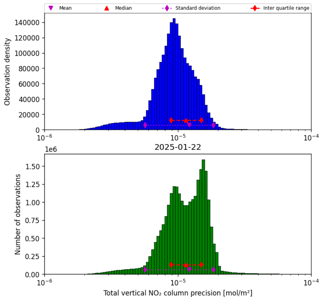
Figure 37: Histogram of “Total vertical NO 2 column precision” for 2025-01-22 to 2025-01-23
