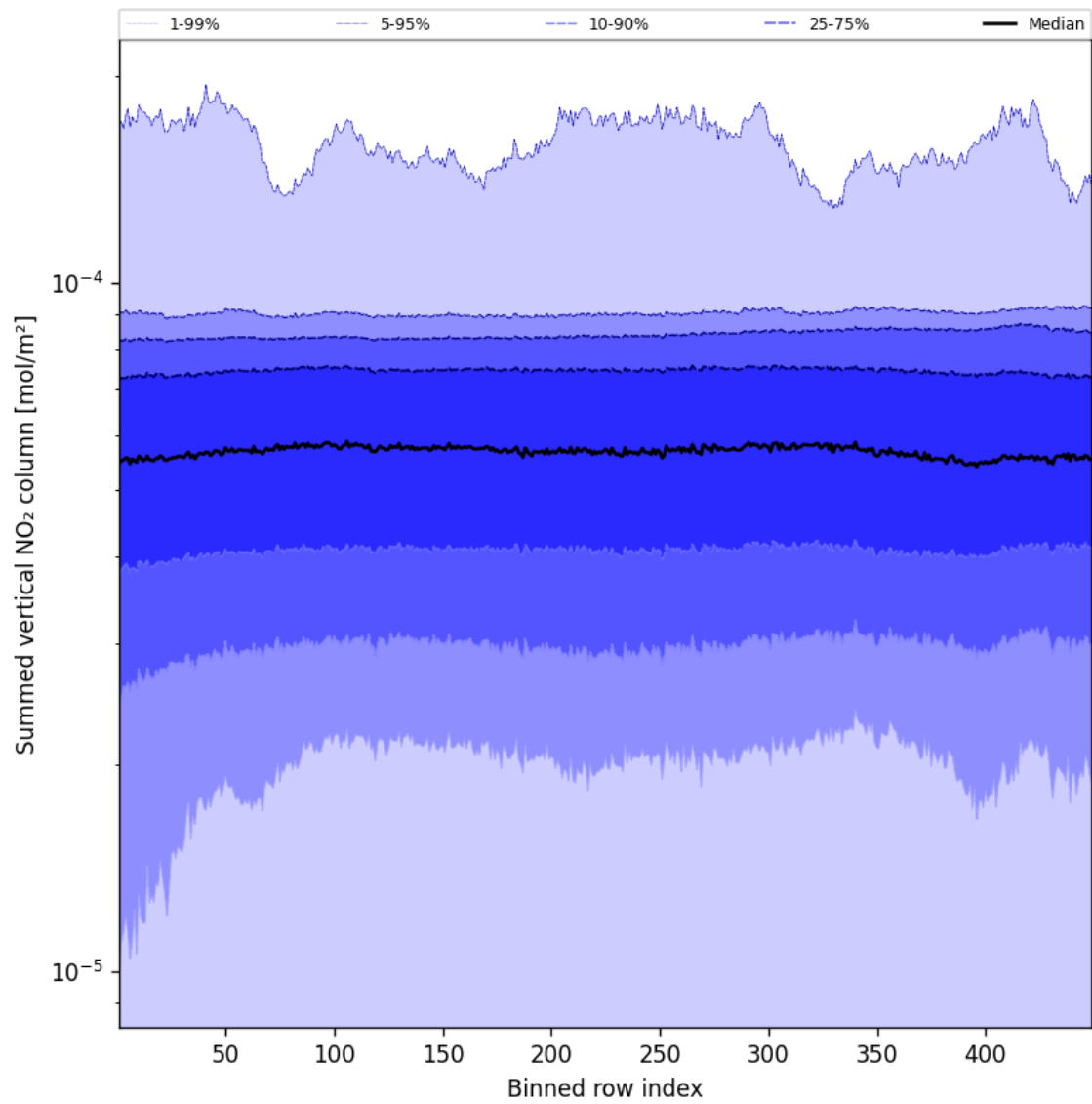
Figure 55: Along track statistics of “Summed vertical NO 2 column” for 2025-01-22 to 2025-01-23
