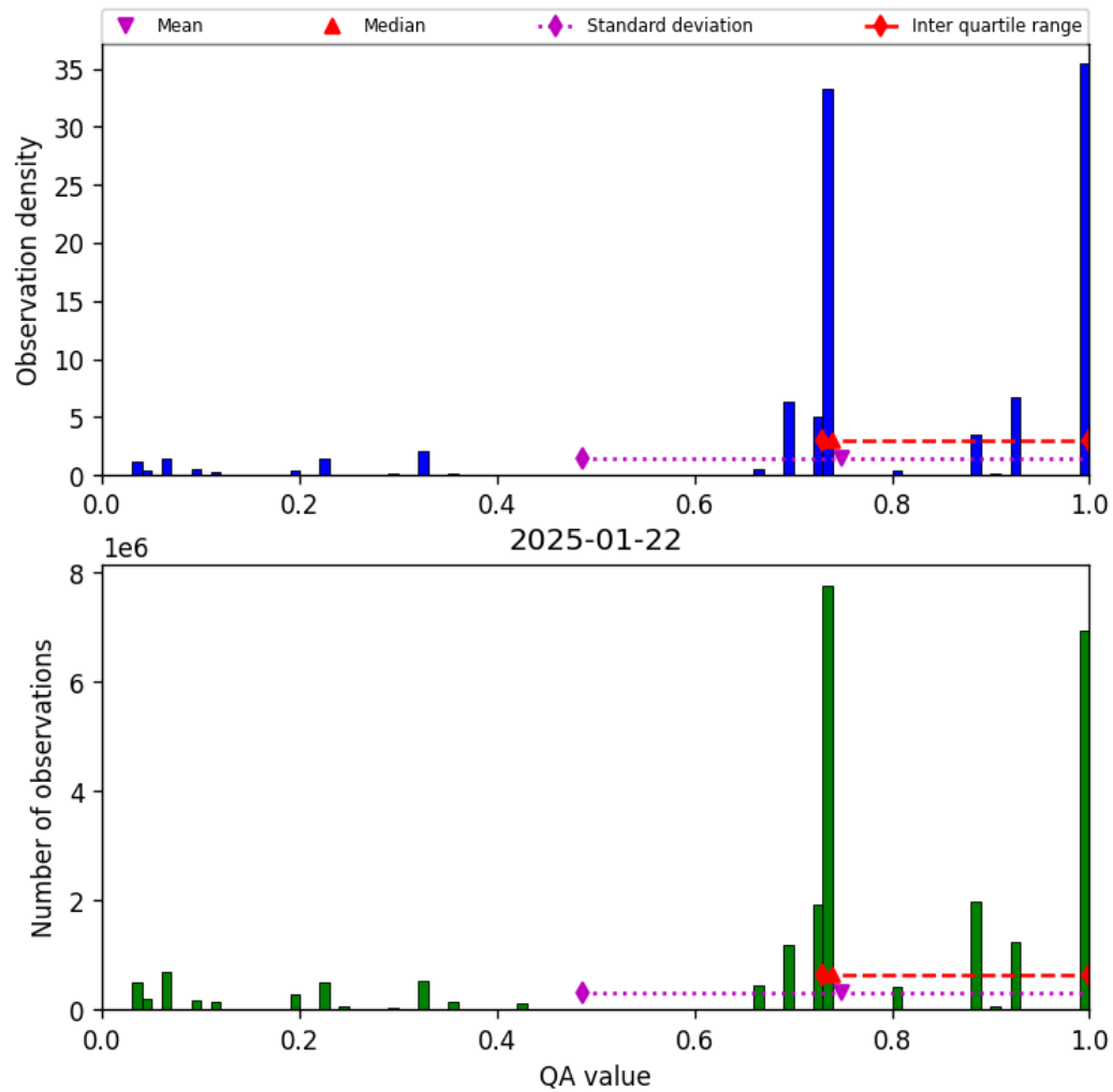
Figure 26: Histogram of “QA value” for 2025-01-22 to 2025-01-23
