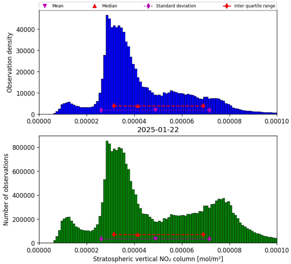
Figure 34: Histogram of “Stratospheric vertical NO 2 column” for 2025-01-22 to 2025-01-23
