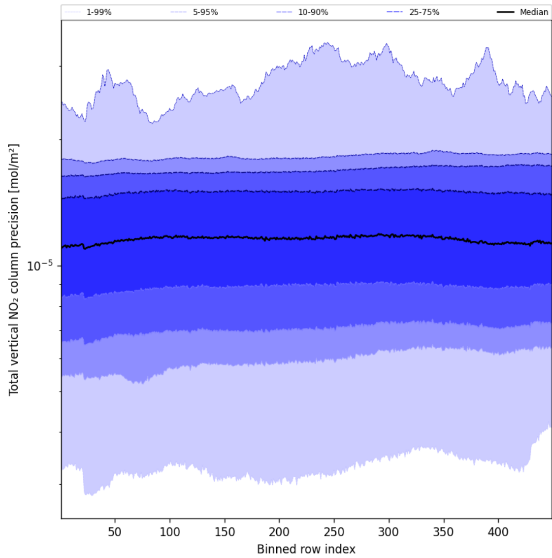
Figure 54: Along track statistics of “Total vertical NO 2 column precision” for 2025-01-22 to 2025-01-23
