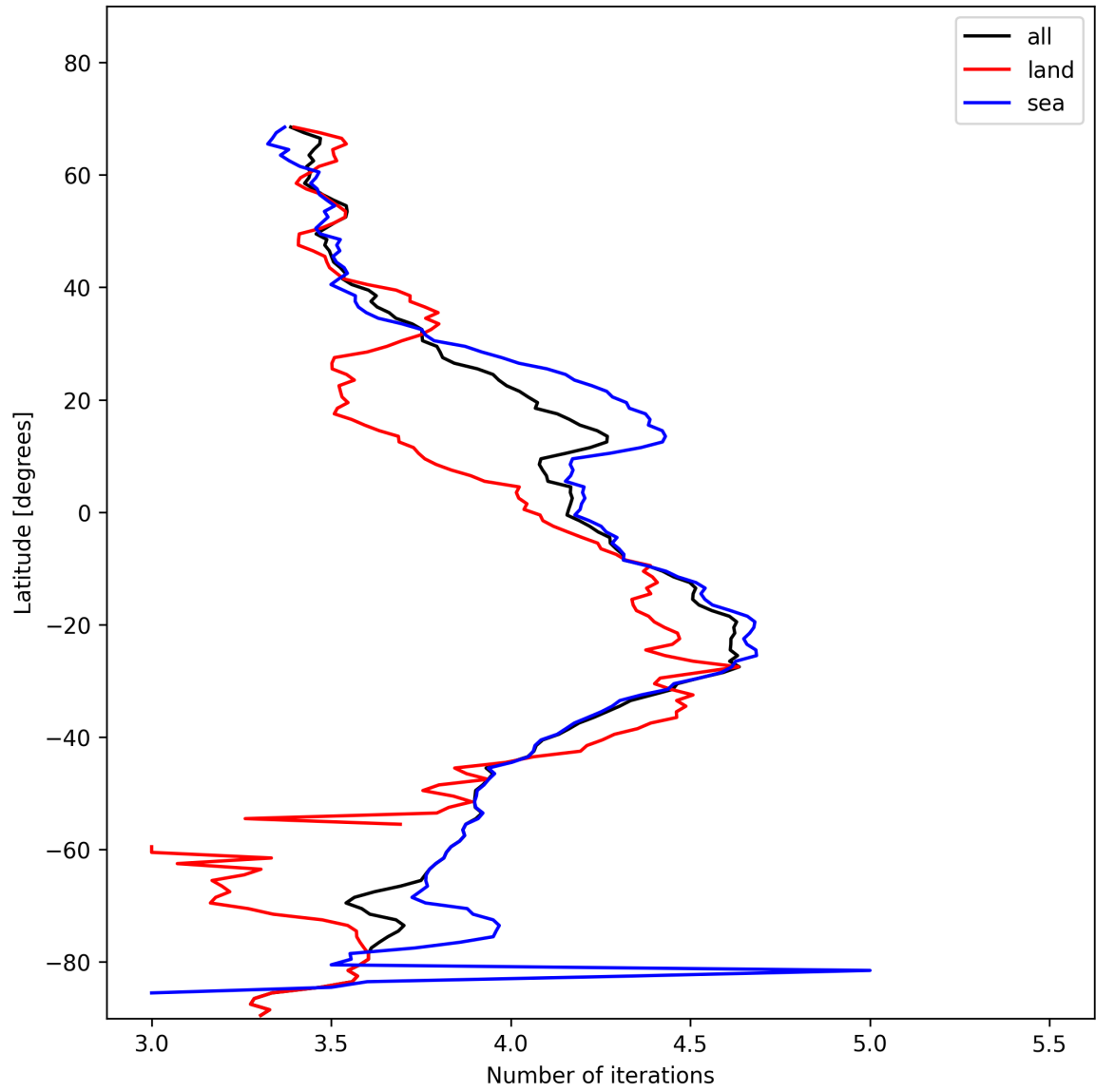
Figure 15: Zonal average of “Number of iterations” for 2025-01-22 to 2025-01-23.
