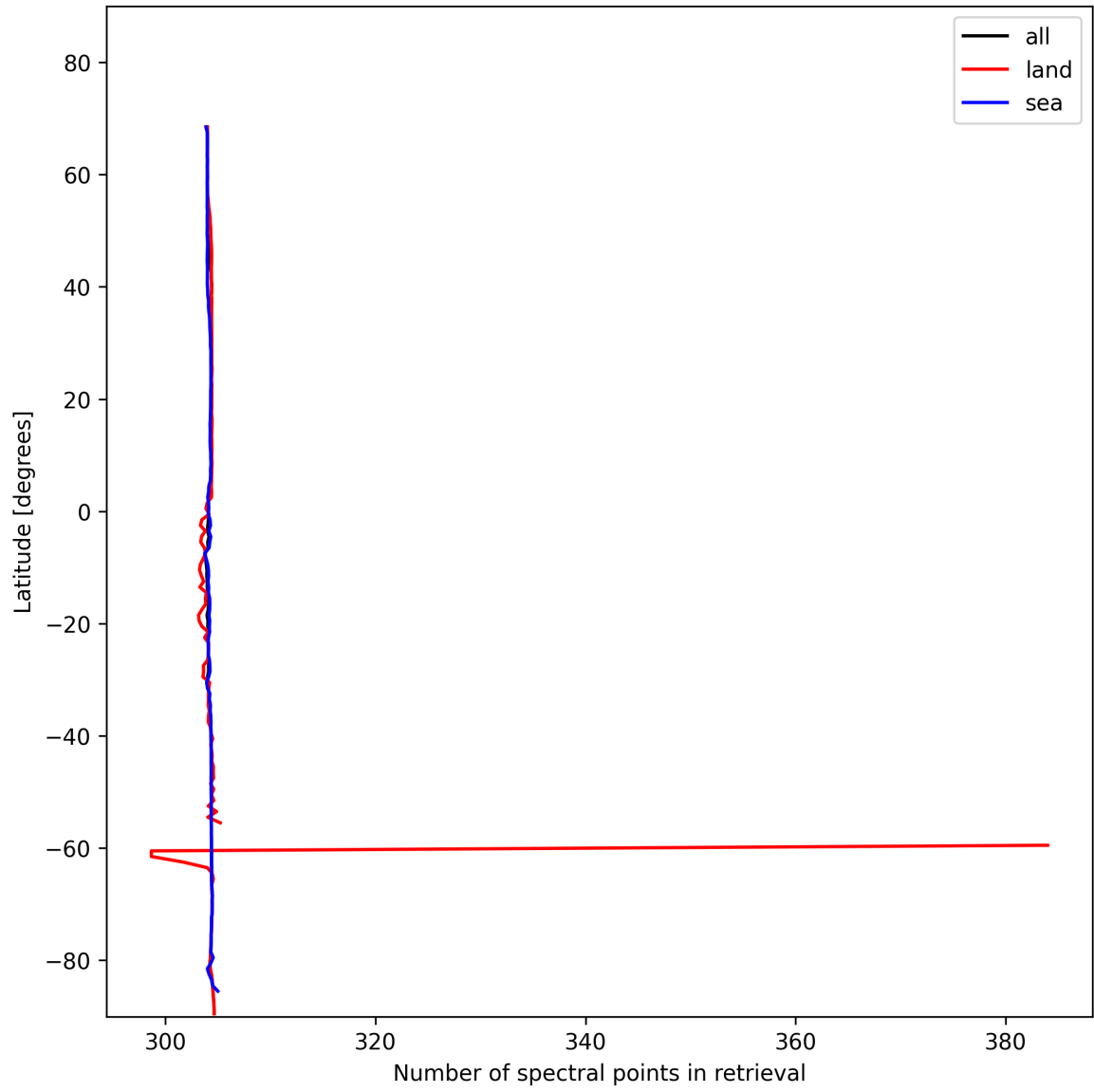
Figure 14: Zonal average of “Number of spectral points in retrieval” for 2025-01-22 to 2025-01-23.
