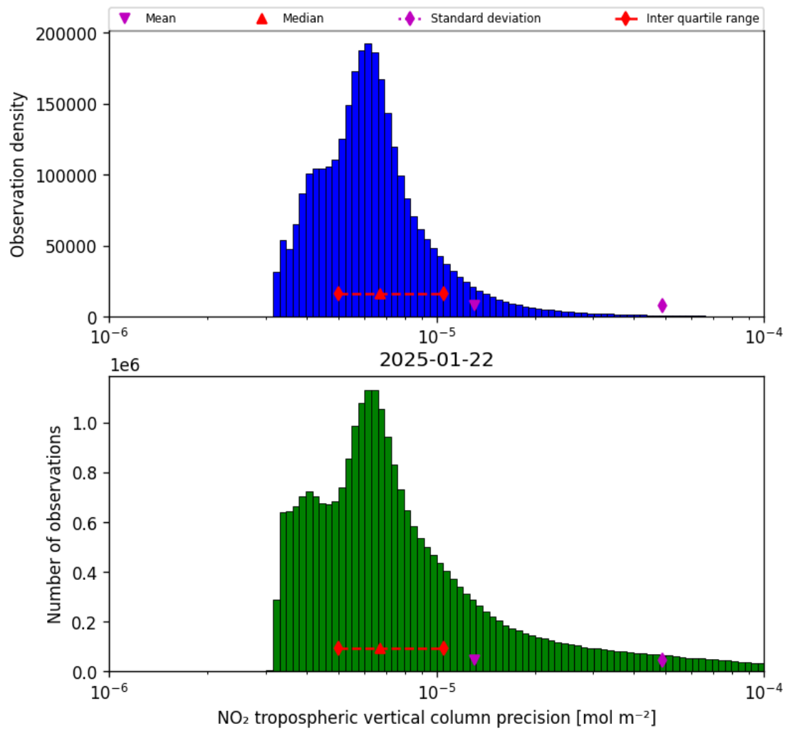
Figure 28: Histogram of “NO 2 tropospheric vertical column precision” for 2025-01-22 to 2025-01-23
