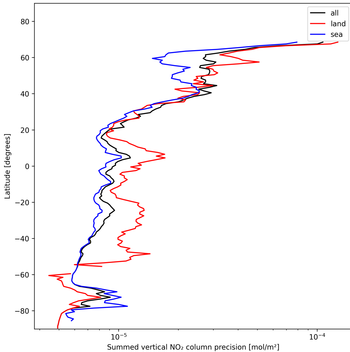
Figure 22: Zonal average of “Summed vertical NO 2 column precision” for 2025-01-22 to 2025-01-23.
