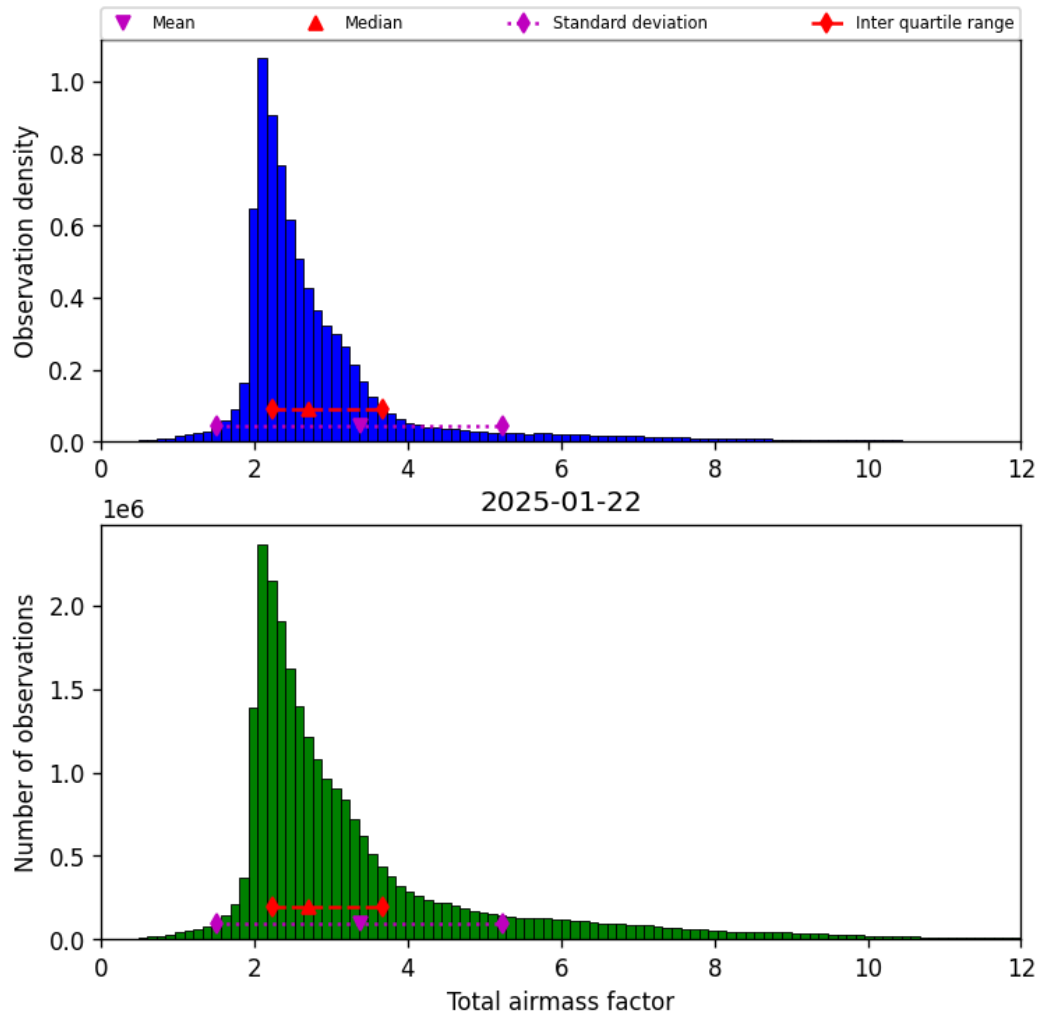
Figure 30: Histogram of “Total airmass factor” for 2025-01-22 to 2025-01-23
