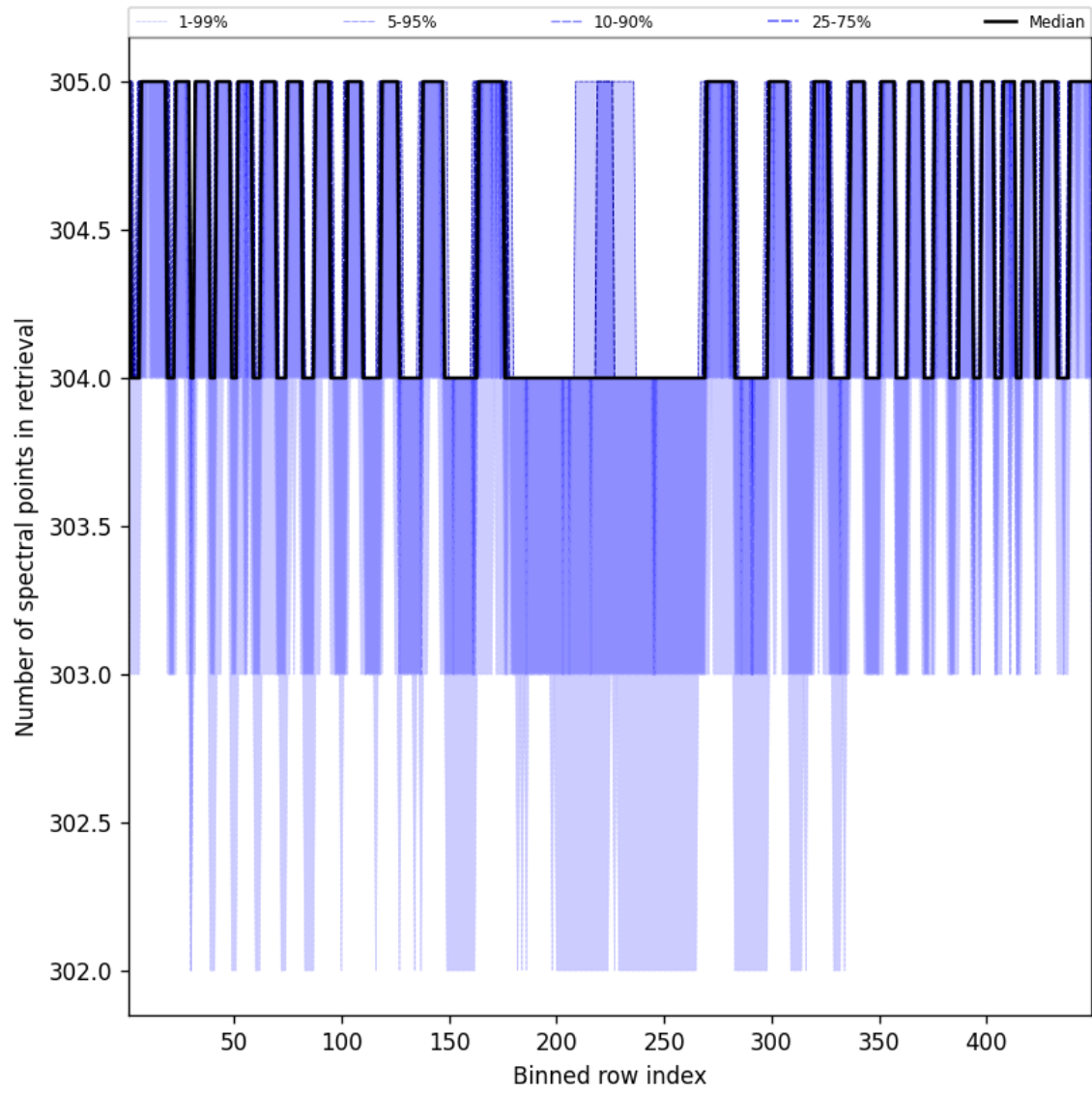
Figure 48: Along track statistics of “Number of spectral points in retrieval” for 2025-01-22 to 2025-01-23
