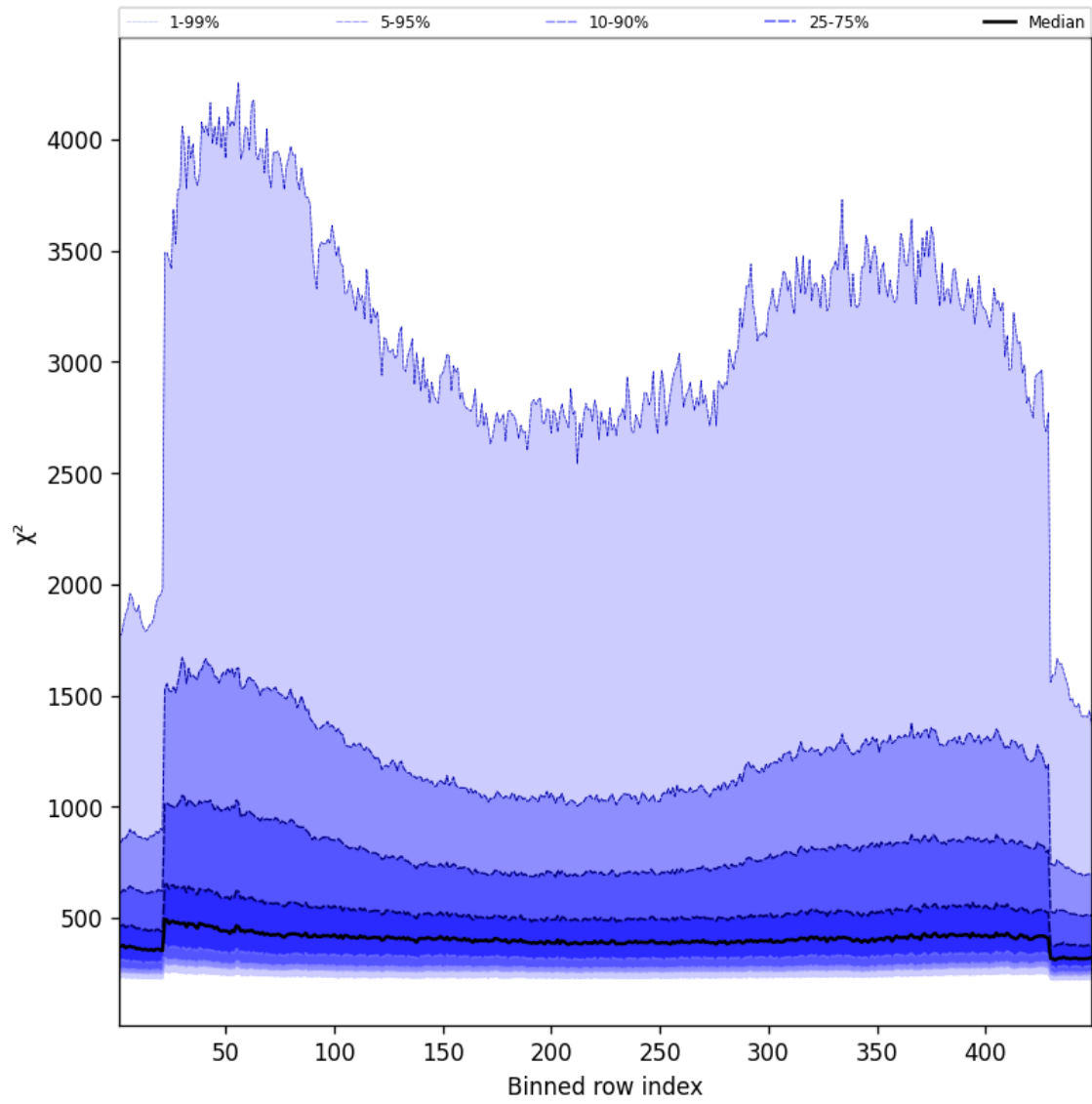
Figure 57: Along track statistics of “ \chi^2 ” for 2025-01-22 to 2025-01-23
