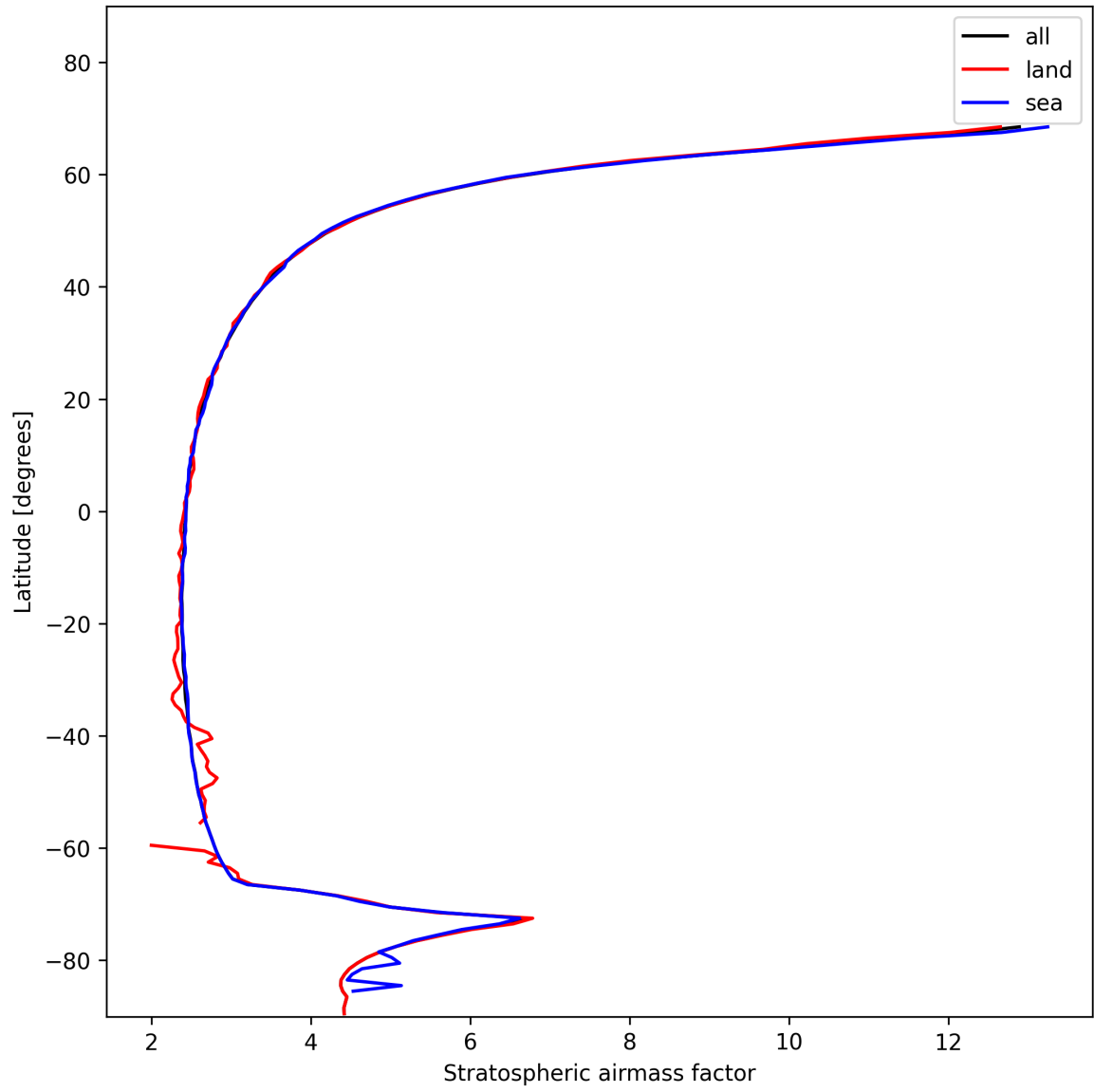
Figure 25: Zonal average of “Stratospheric airmass factor” for 2025-01-22 to 2025-01-23.
