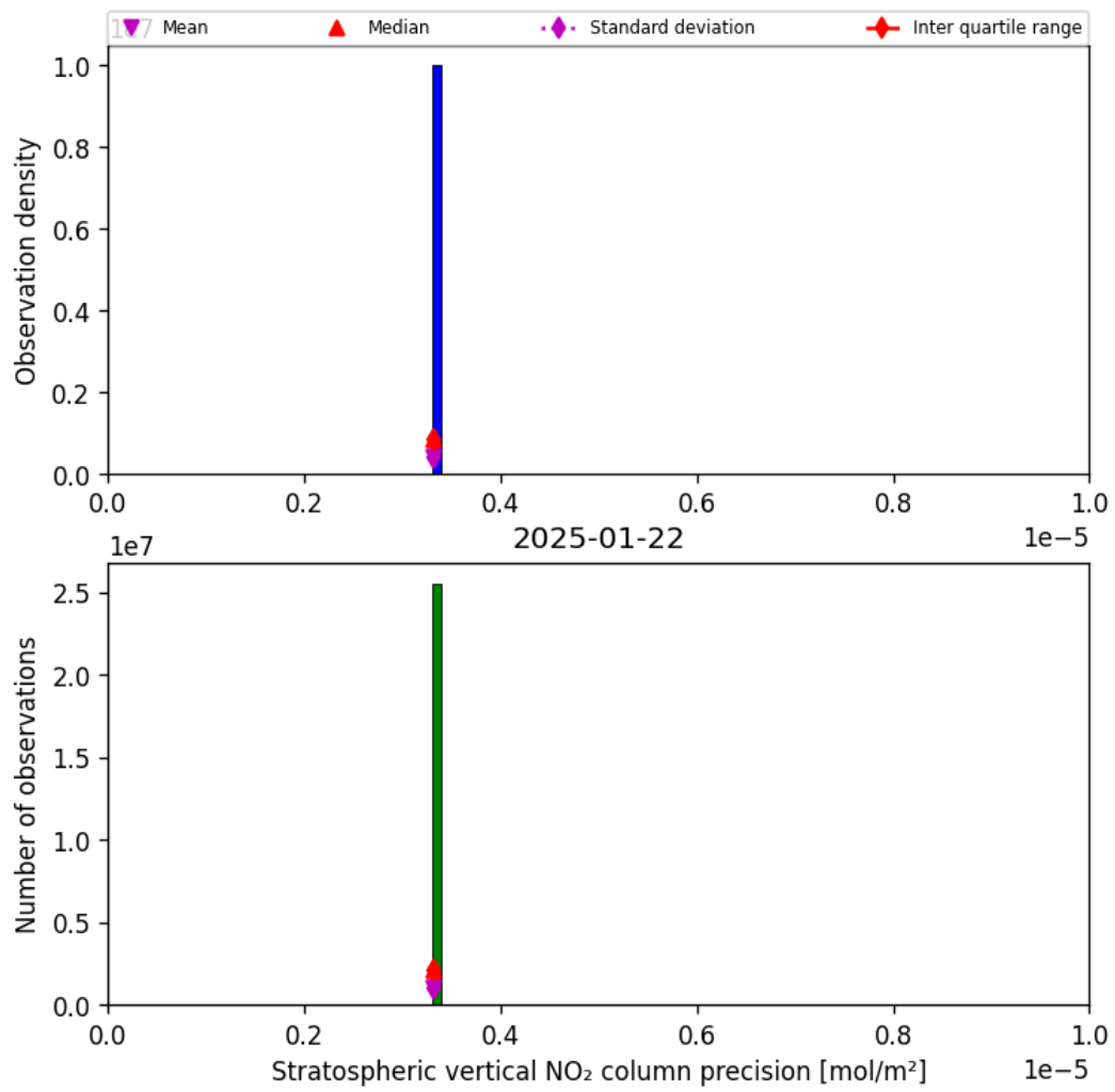
Figure 35: Histogram of “Stratospheric vertical NO 2 column precision” for 2025-01-22 to 2025-01-23
