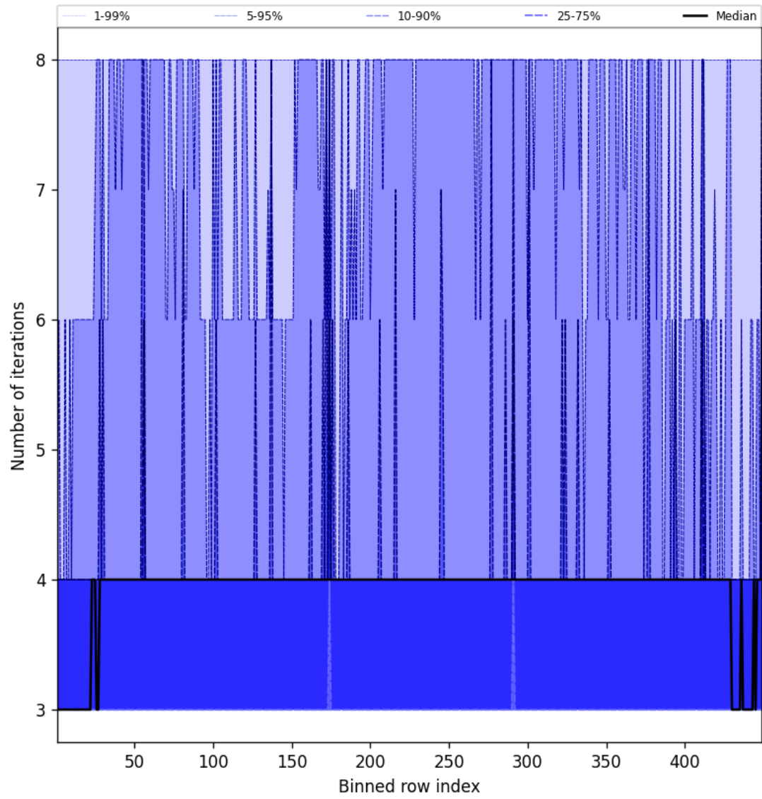
Figure 49: Along track statistics of “Number of iterations” for 2025-01-22 to 2025-01-23
