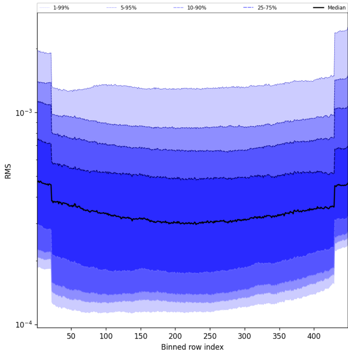
Figure 58: Along track statistics of “RMS” for 2025-01-22 to 2025-01-23
