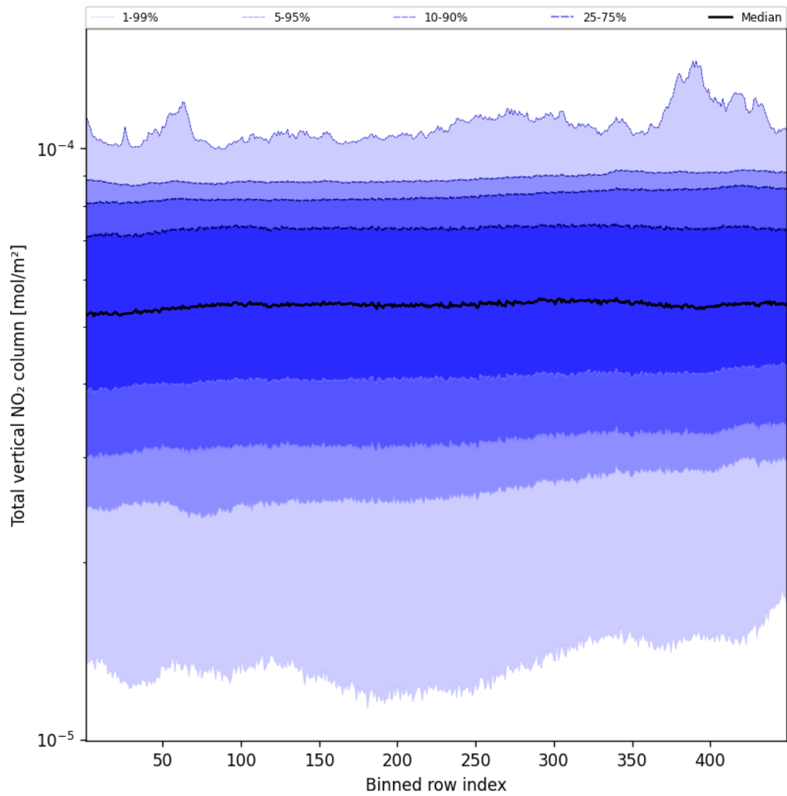
Figure 53: Along track statistics of “Total vertical NO 2 column” for 2025-01-22 to 2025-01-23
