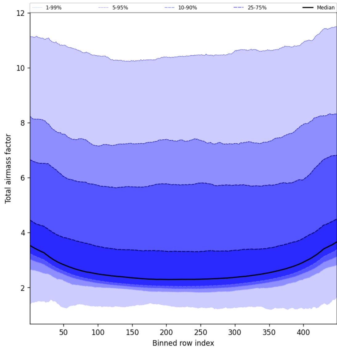
Figure 47: Along track statistics of “Total airmass factor” for 2025-01-22 to 2025-01-23
