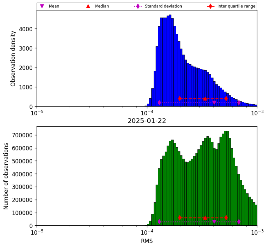
Figure 41: Histogram of “RMS” for 2025-01-22 to 2025-01-23
