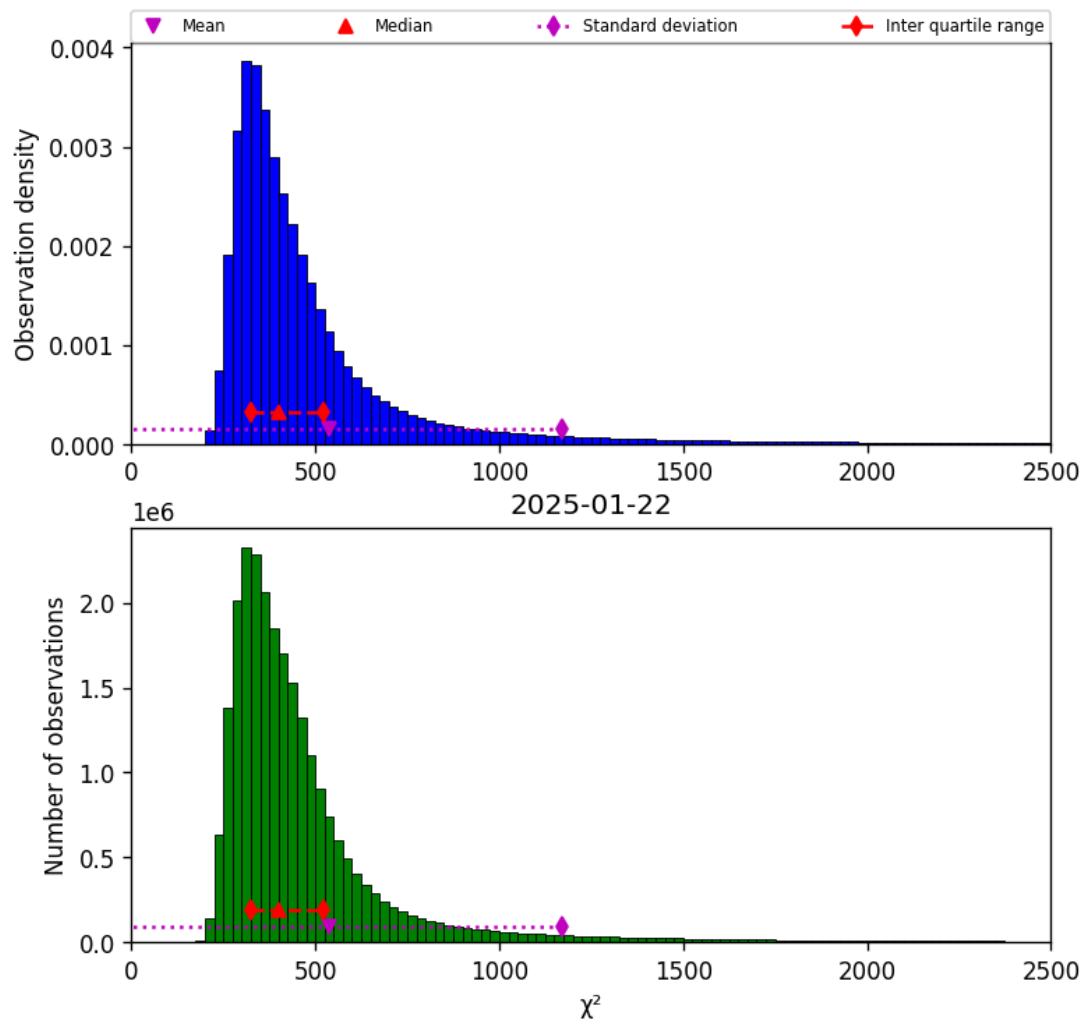
Figure 40: Histogram of “ \chi^2 ” for 2025-01-22 to 2025-01-23
