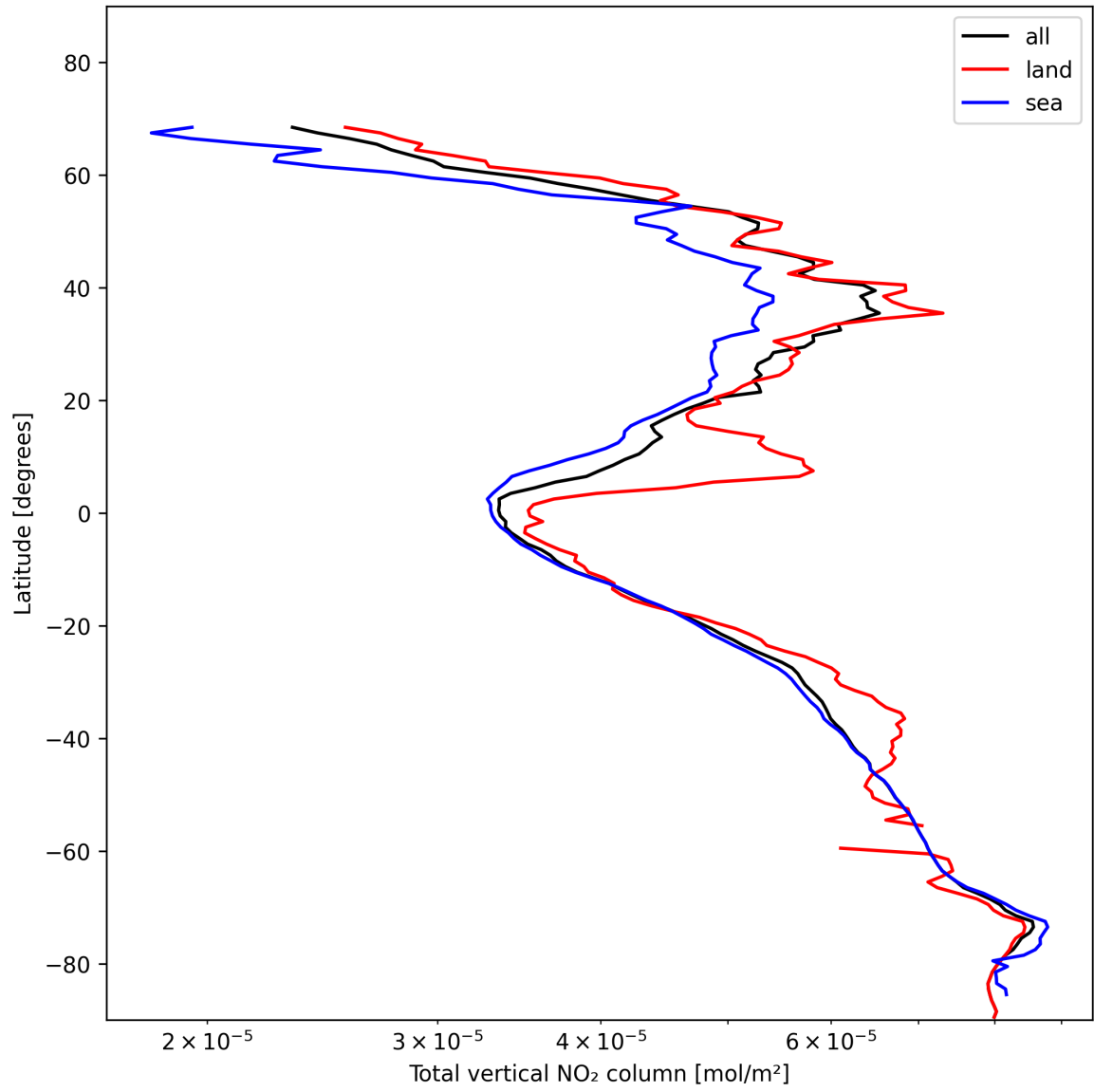
Figure 19: Zonal average of “Total vertical NO 2 column” for 2025-01-22 to 2025-01-23.
