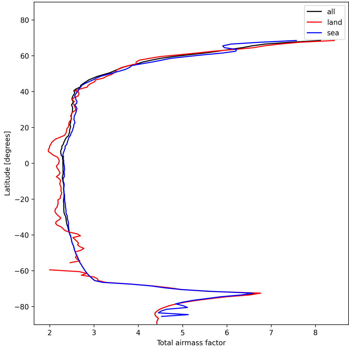
Figure 13: Zonal average of “Total airmass factor” for 2025-01-22 to 2025-01-23.
