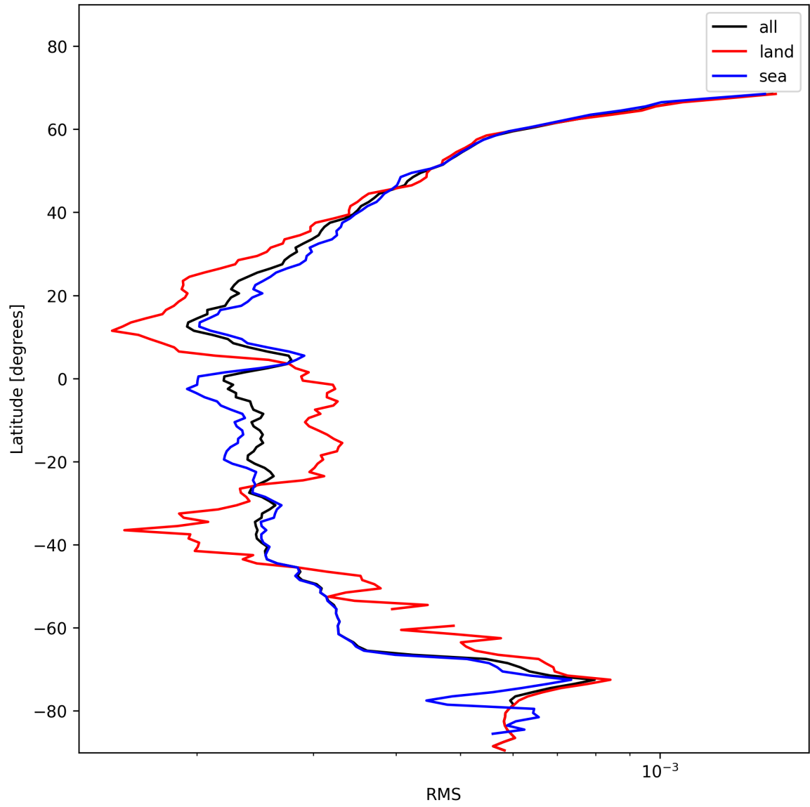
Figure 24: Zonal average of “RMS” for 2025-01-22 to 2025-01-23.
