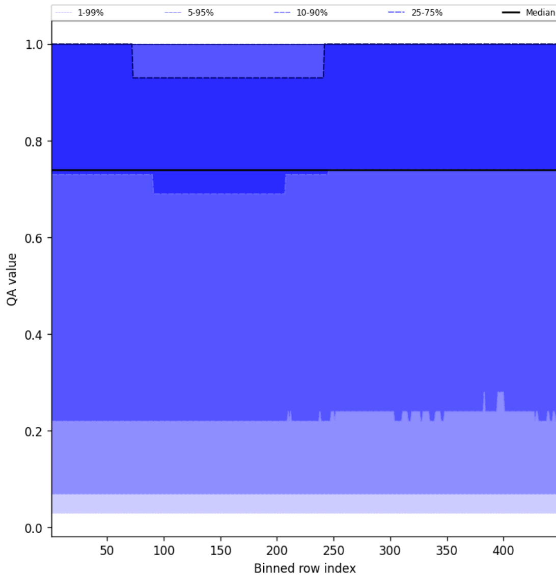
Figure 43: Along track statistics of “QA value” for 2025-01-22 to 2025-01-23
