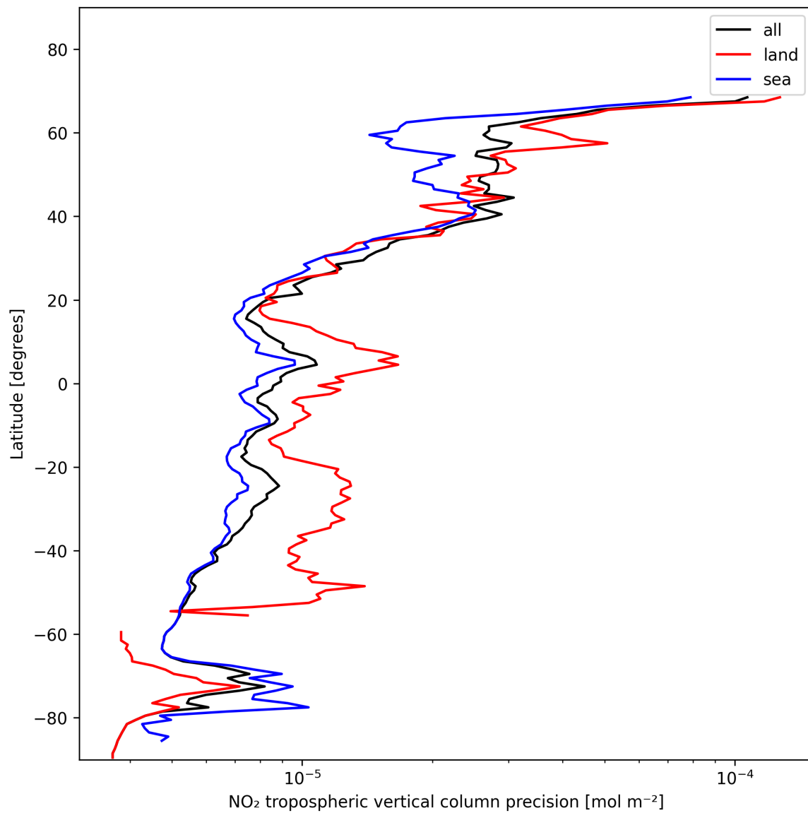
Figure 11: Zonal average of “NO 2 tropospheric vertical column precision” for 2025-01-22 to 2025-01-23.
