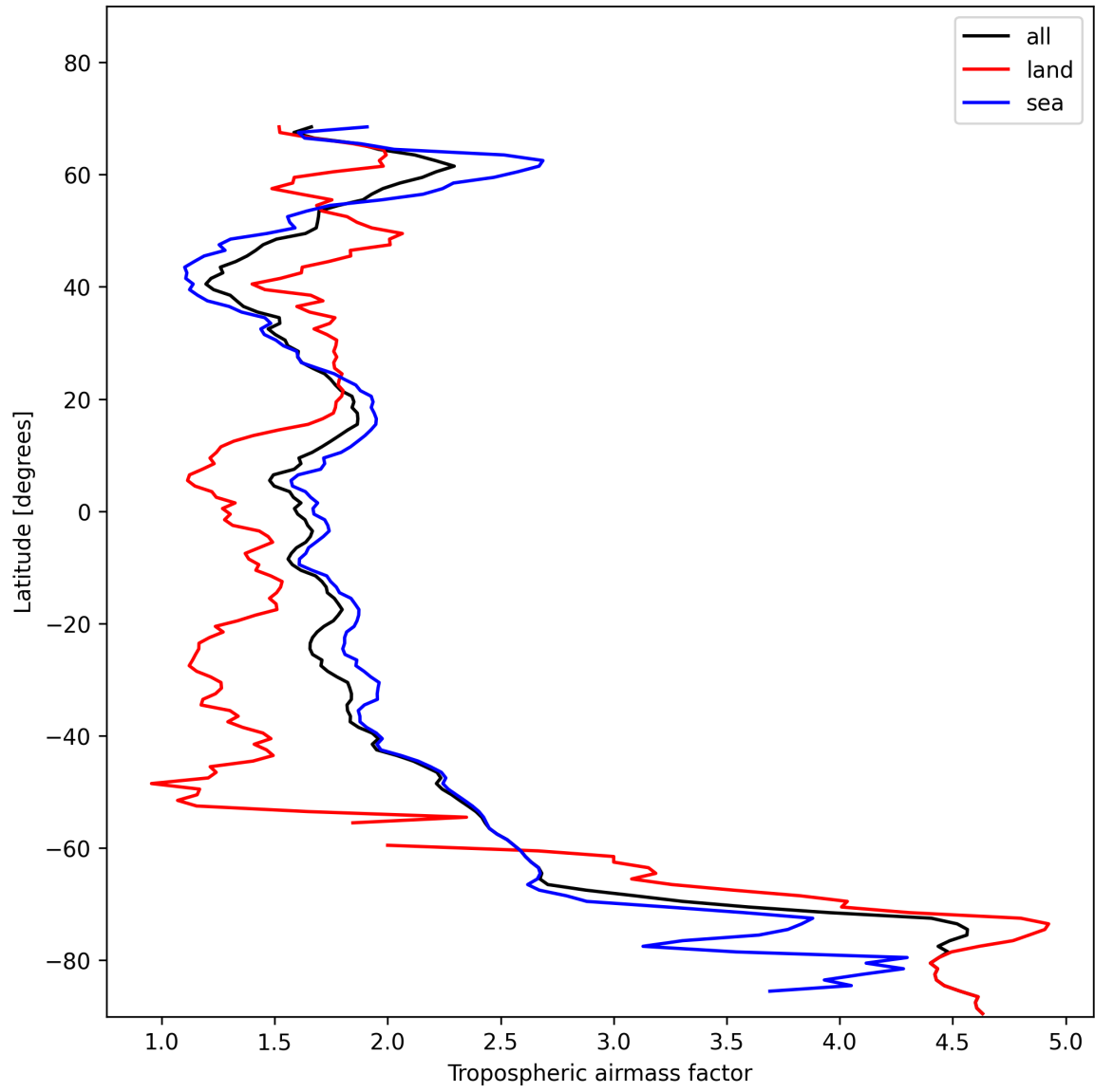
Figure 12: Zonal average of “Tropospheric air mass factor” for 2025-01-22 to 2025-01-23.
