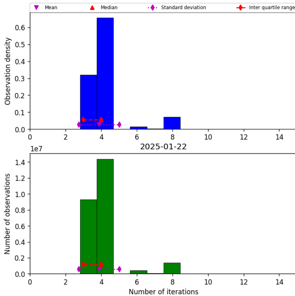
Figure 32: Histogram of “Number of iterations” for 2025-01-22 to 2025-01-23
