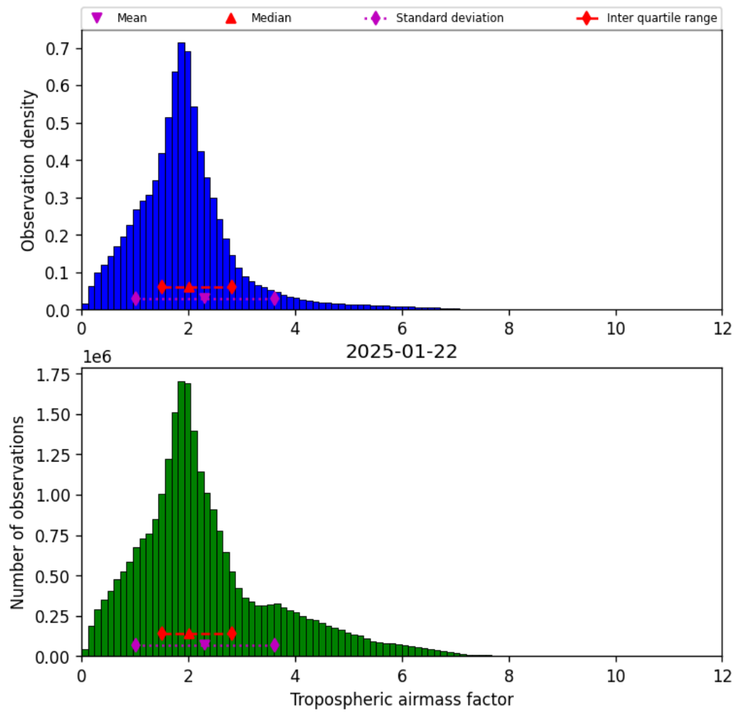
Figure 29: Histogram of “Tropospheric airmass factor” for 2025-01-22 to 2025-01-23
