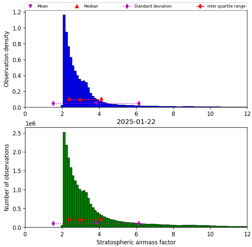
Figure 42: Histogram of “Stratospheric airmass factor” for 2025-01-22 to 2025-01-23
