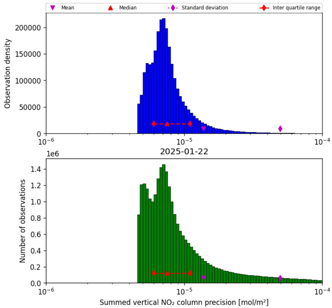
Figure 39: Histogram of "Summed vertical NO 2 column precision" for 2025-01-22 to 2025-01-23
