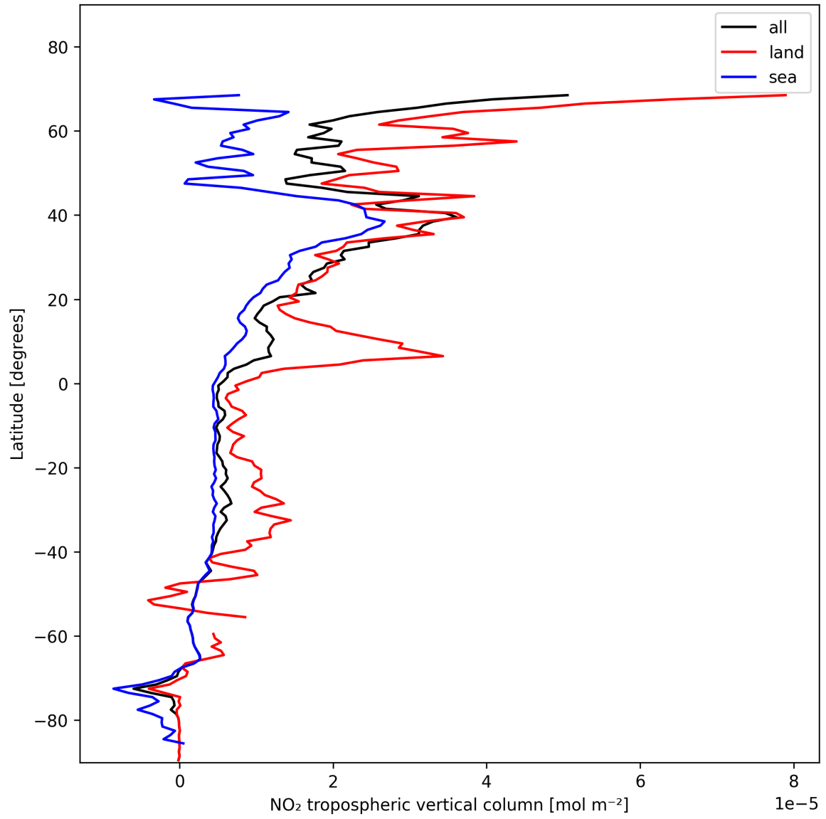
Figure 10: Zonal average of “NO 2 tropospheric vertical column” for 2025-01-22 to 2025-01-23.
