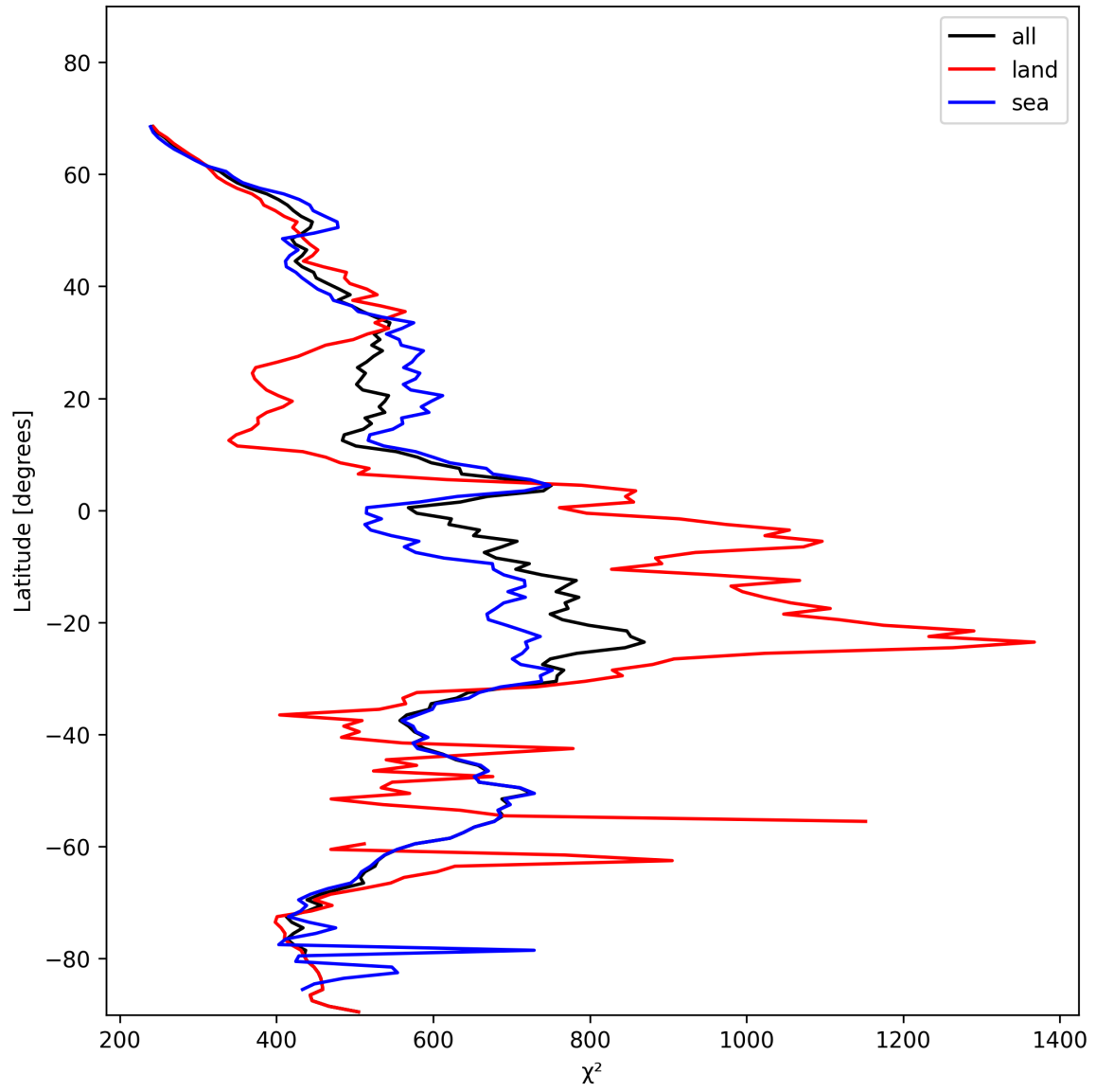
Figure 23: Zonal average of “ \chi^2 ” for 2025-01-22 to 2025-01-23.
