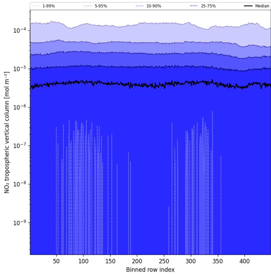
Figure 44: Along track statistics of “NO 2 tropospheric vertical column” for 2025-01-22 to 2025-01-23
