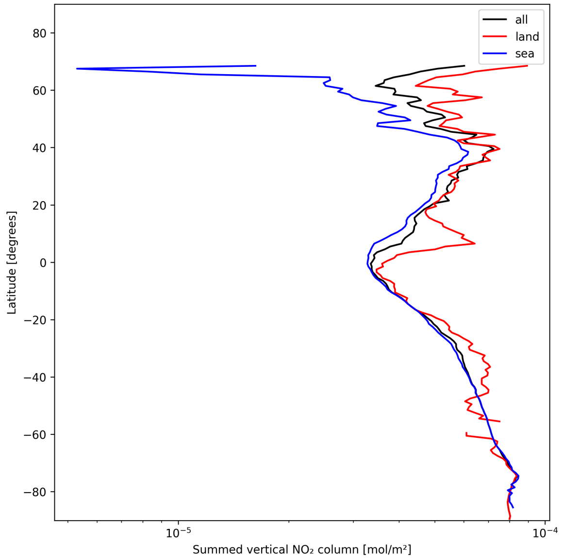
Figure 21: Zonal average of “Summed vertical NO 2 column” for 2025-01-22 to 2025-01-23.
