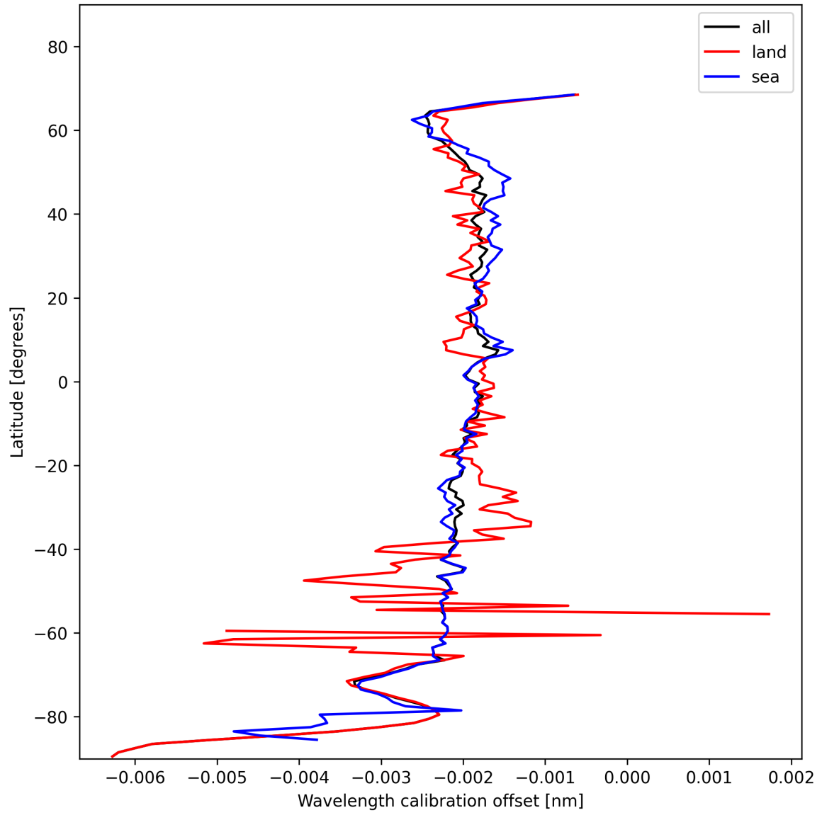
Figure 16: Zonal average of “Wavelength calibration offset” for 2025-01-22 to 2025-01-23.
