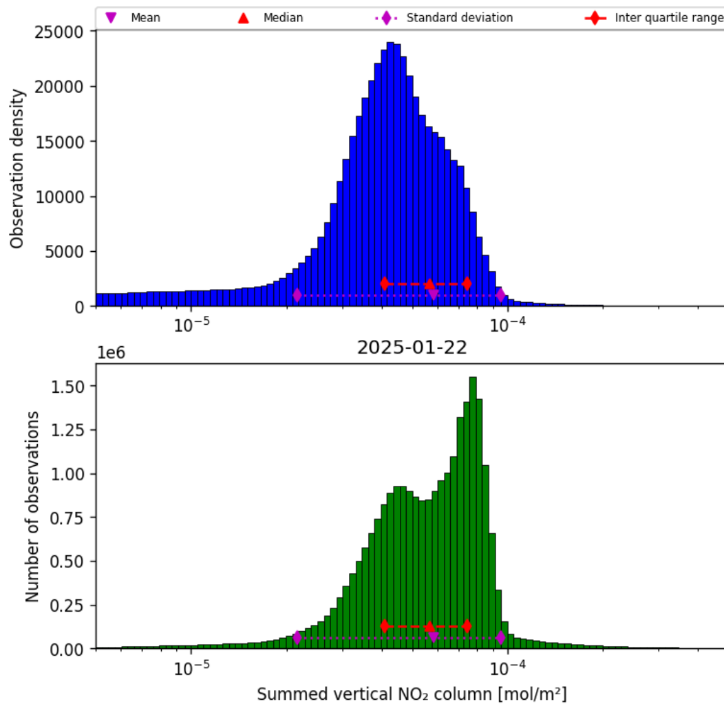
Figure 38: Histogram of “Summed vertical NO 2 column” for 2025-01-22 to 2025-01-23
