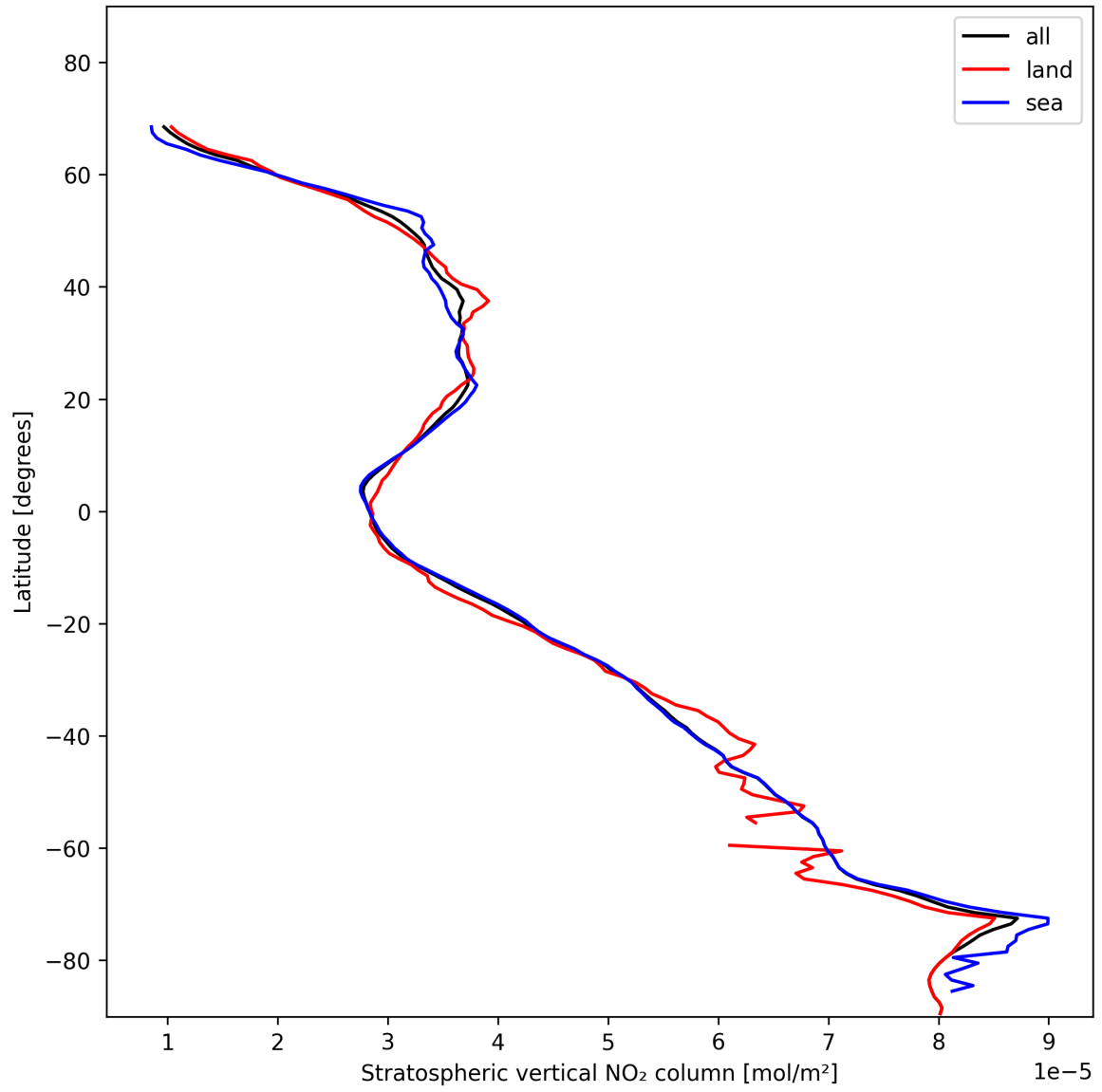
Figure 17: Zonal average of “Stratospheric vertical NO 2 column” for 2025-01-22 to 2025-01-23.
