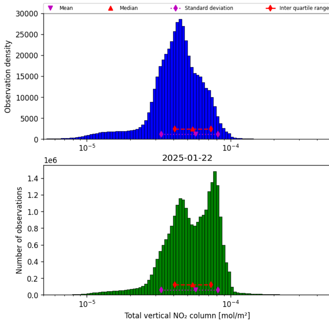
Figure 36: Histogram of “Total vertical NO 2 column” for 2025-01-22 to 2025-01-23
