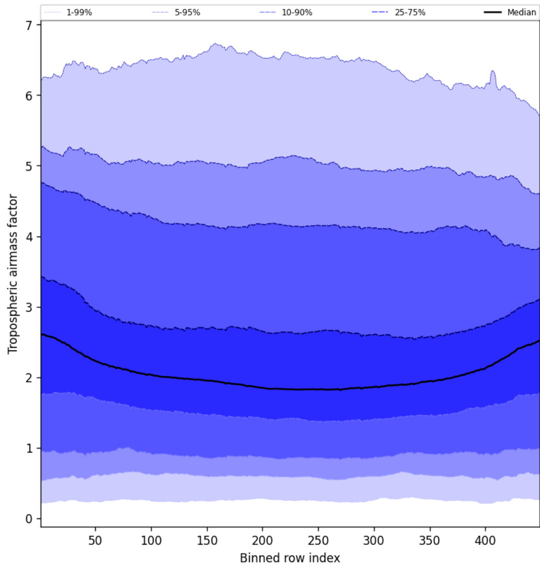
Figure 46: Along track statistics of “Tropospheric air mass factor” for 2025-01-22 to 2025-01-23
