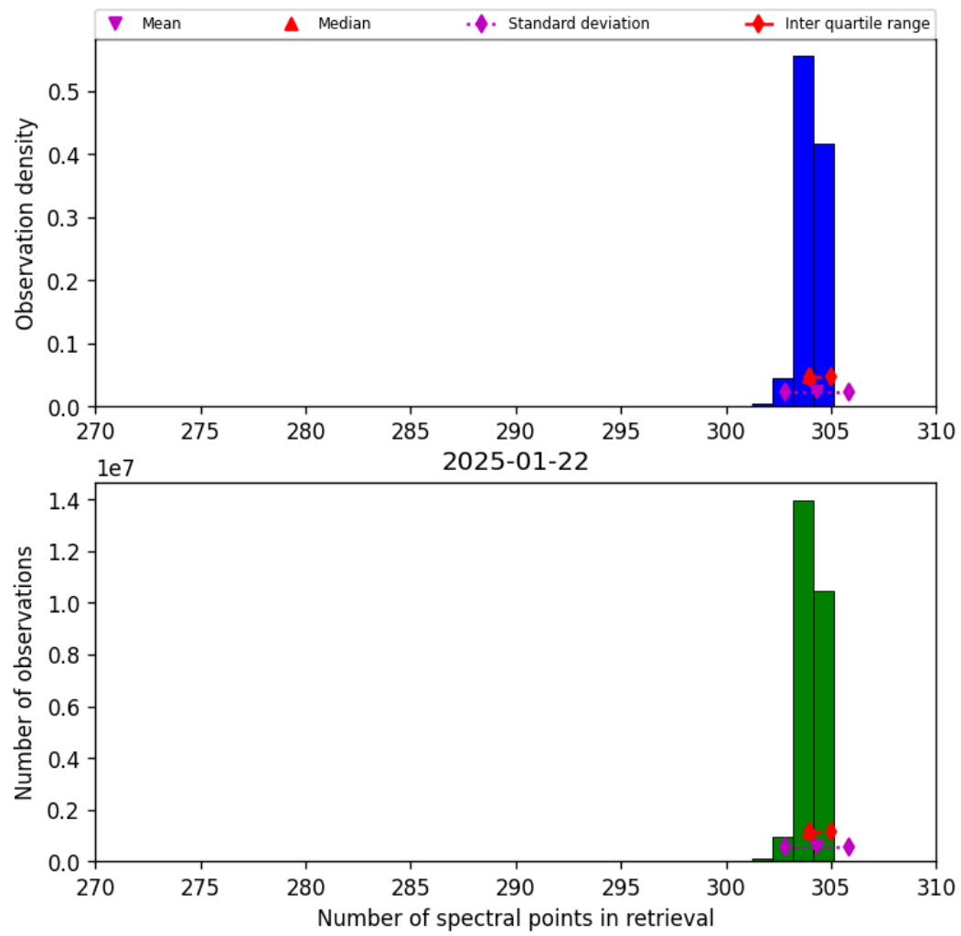
Figure 31: Histogram of “Number of spectral points in retrieval” for 2025-01-22 to 2025-01-23
