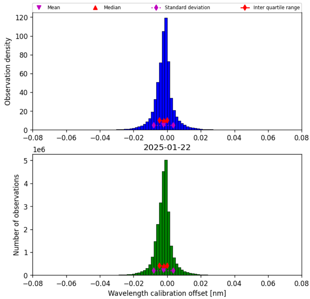
Figure 33: Histogram of “Wavelength calibration offset” for 2025-01-22 to 2025-01-23
