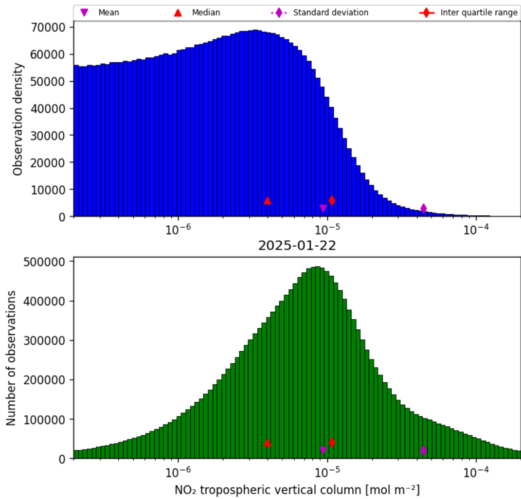
Figure 27: Histogram of “NO 2 tropospheric vertical column” for 2025-01-22 to 2025-01-23
