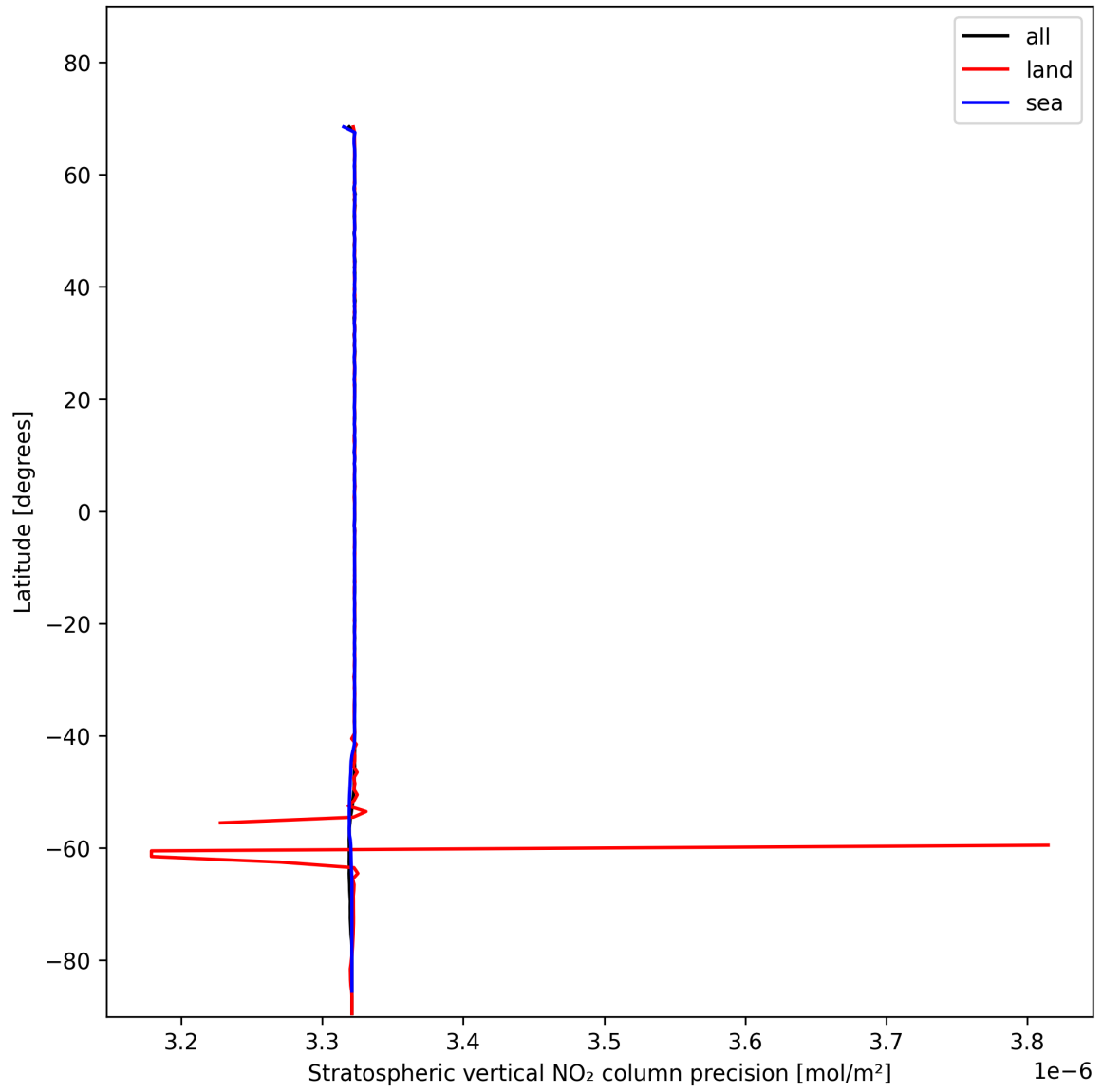
Figure 18: Zonal average of “Stratospheric vertical NO 2 column precision” for 2025-01-22 to 2025-01-23.
