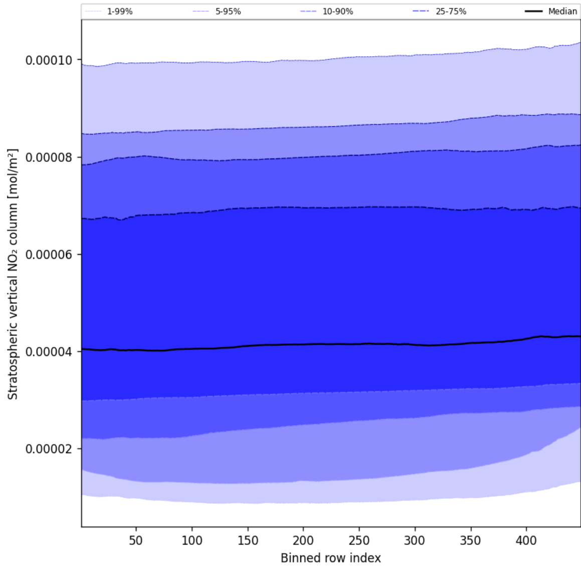
Figure 51: Along track statistics of “Stratospheric vertical NO 2 column” for 2025-01-22 to 2025-01-23
