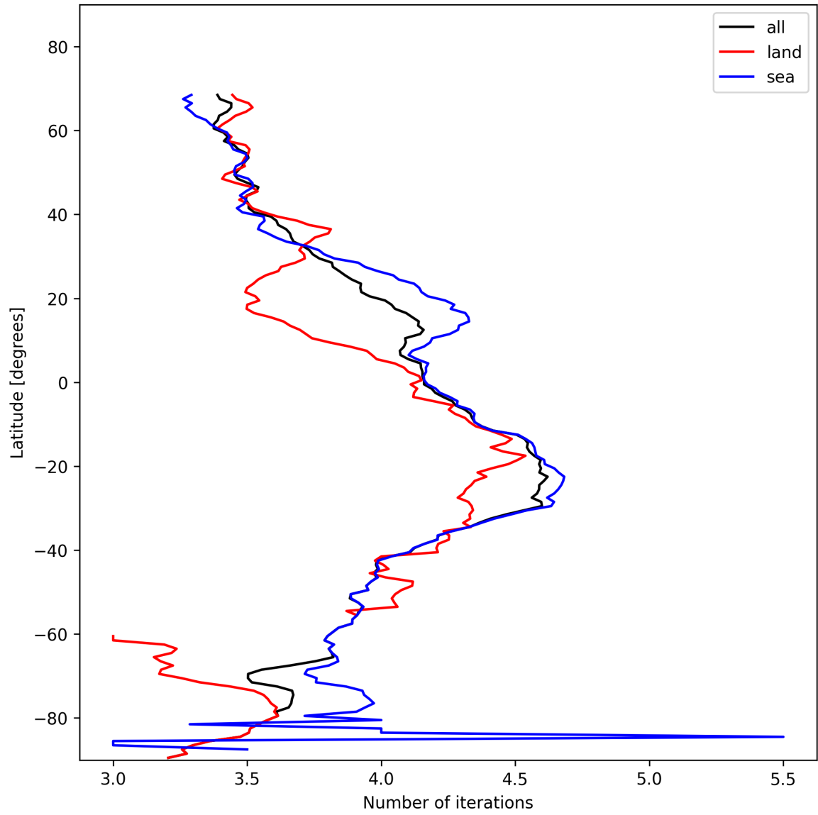
Figure 15: Zonal average of “Number of iterations” for 2025-01-23 to 2025-01-24.
