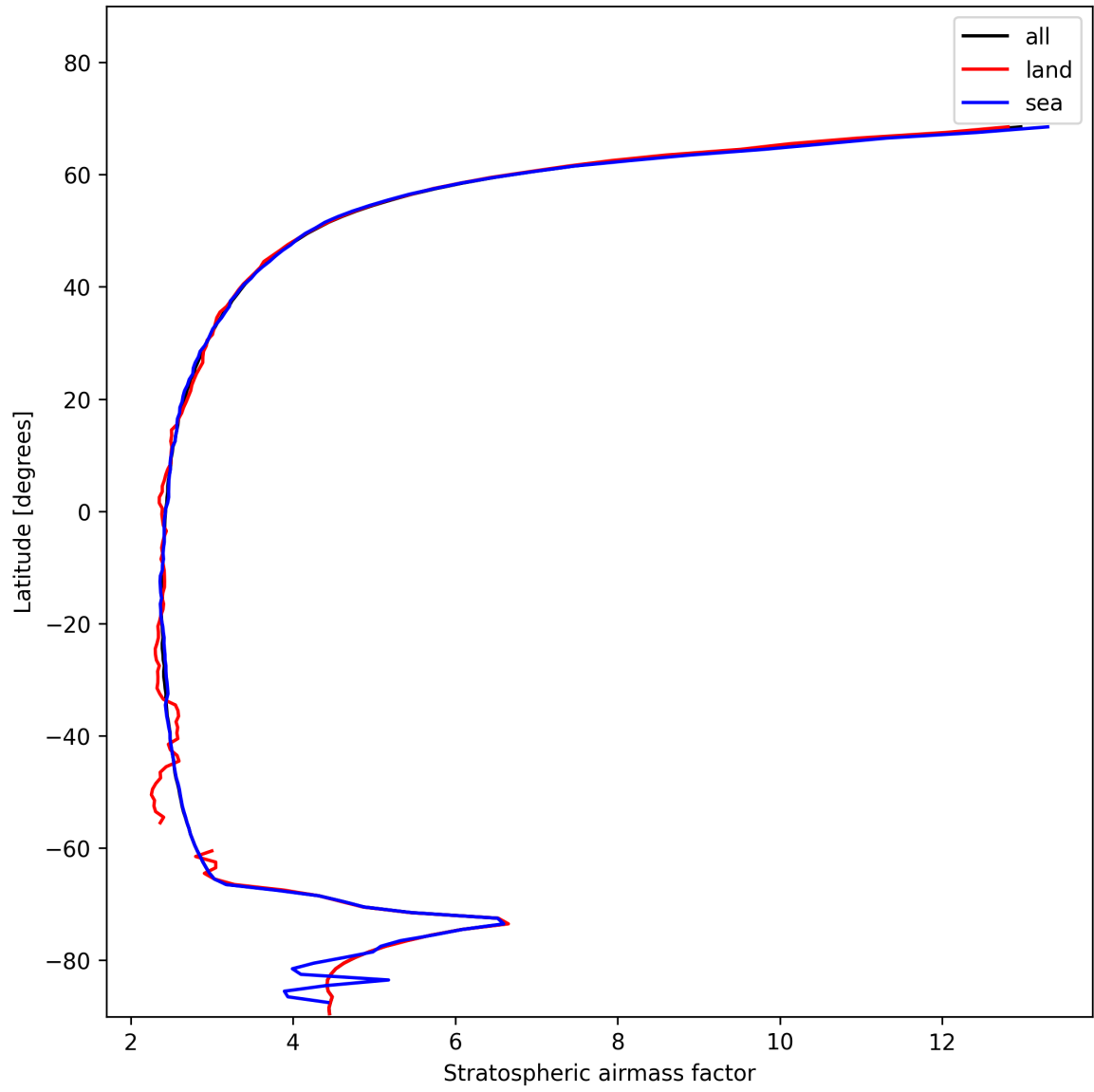
Figure 25: Zonal average of “Stratospheric airmass factor” for 2025-01-23 to 2025-01-24.
