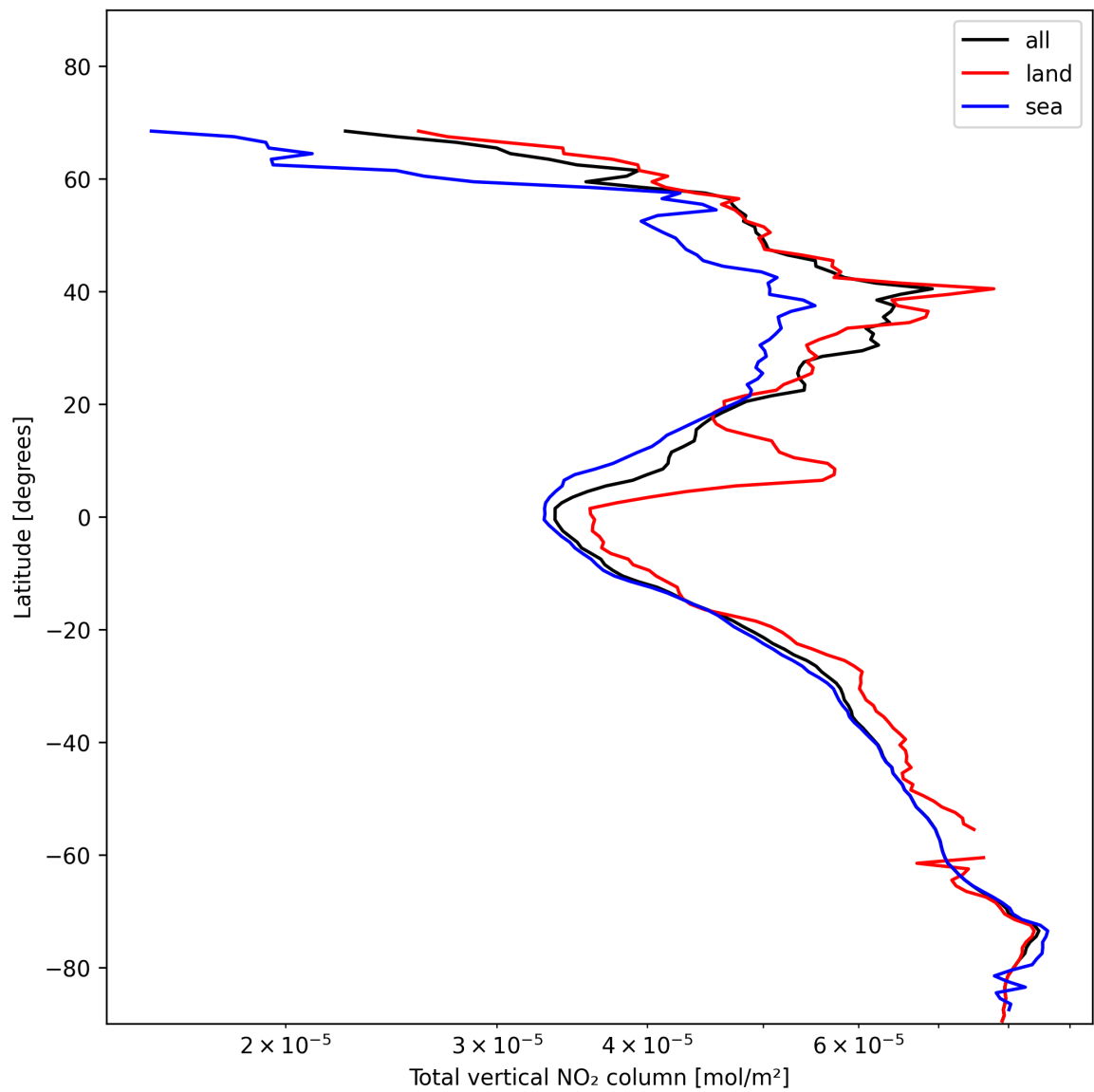
Figure 19: Zonal average of “Total vertical NO 2 column” for 2025-01-23 to 2025-01-24.
