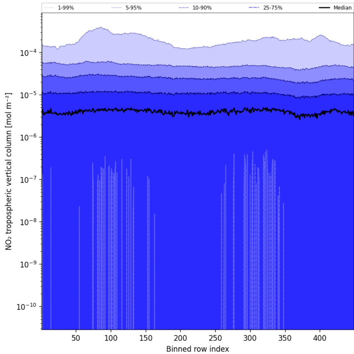
Figure 44: Along track statistics of “NO 2 tropospheric vertical column” for 2025-01-23 to 2025-01-24
