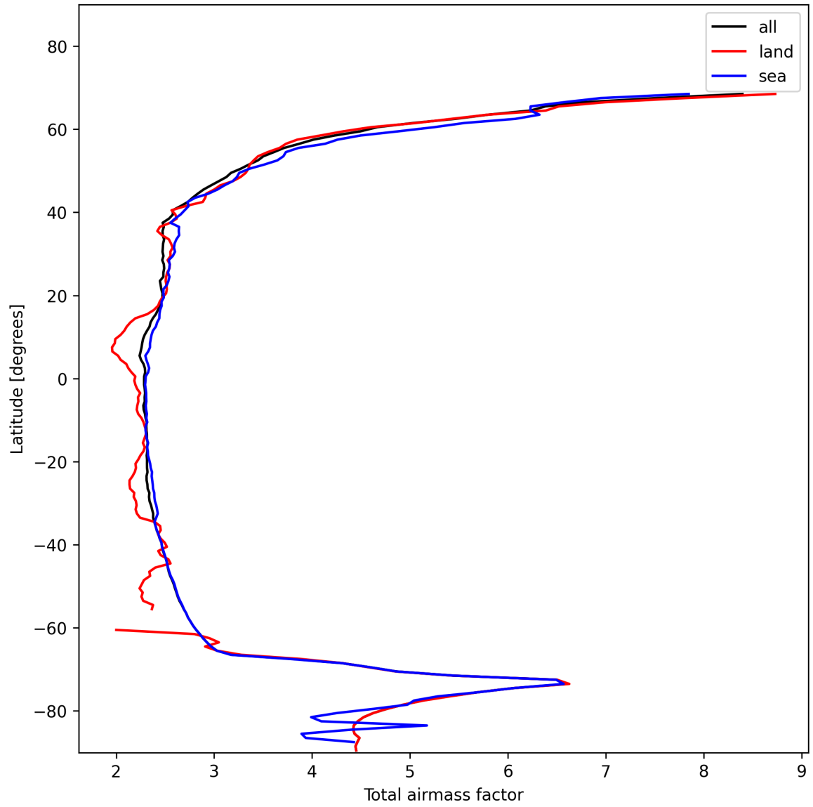
Figure 13: Zonal average of “Total airmass factor” for 2025-01-23 to 2025-01-24.
