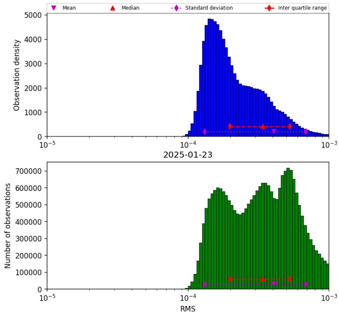
Figure 41: Histogram of “RMS” for 2025-01-23 to 2025-01-24
