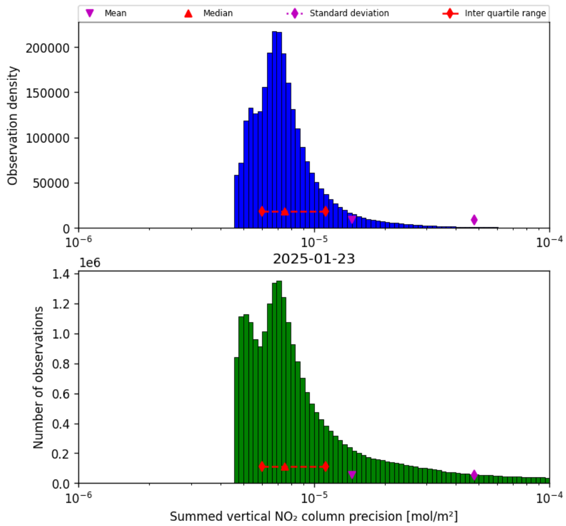
Figure 39: Histogram of “Summed vertical NO 2 column precision” for 2025-01-23 to 2025-01-24
