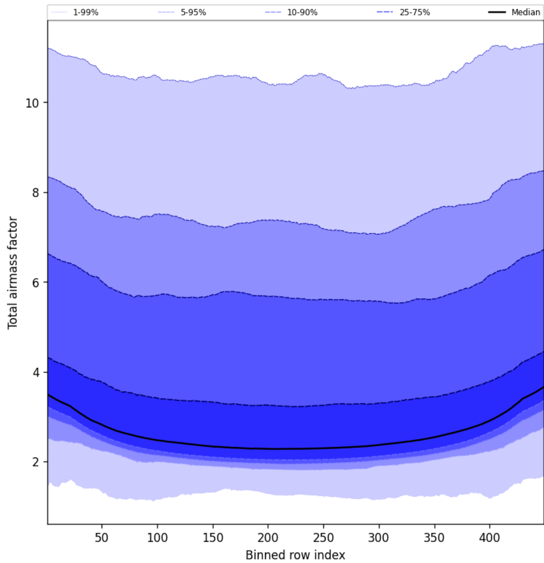
Figure 47: Along track statistics of “Total airmass factor” for 2025-01-23 to 2025-01-24
