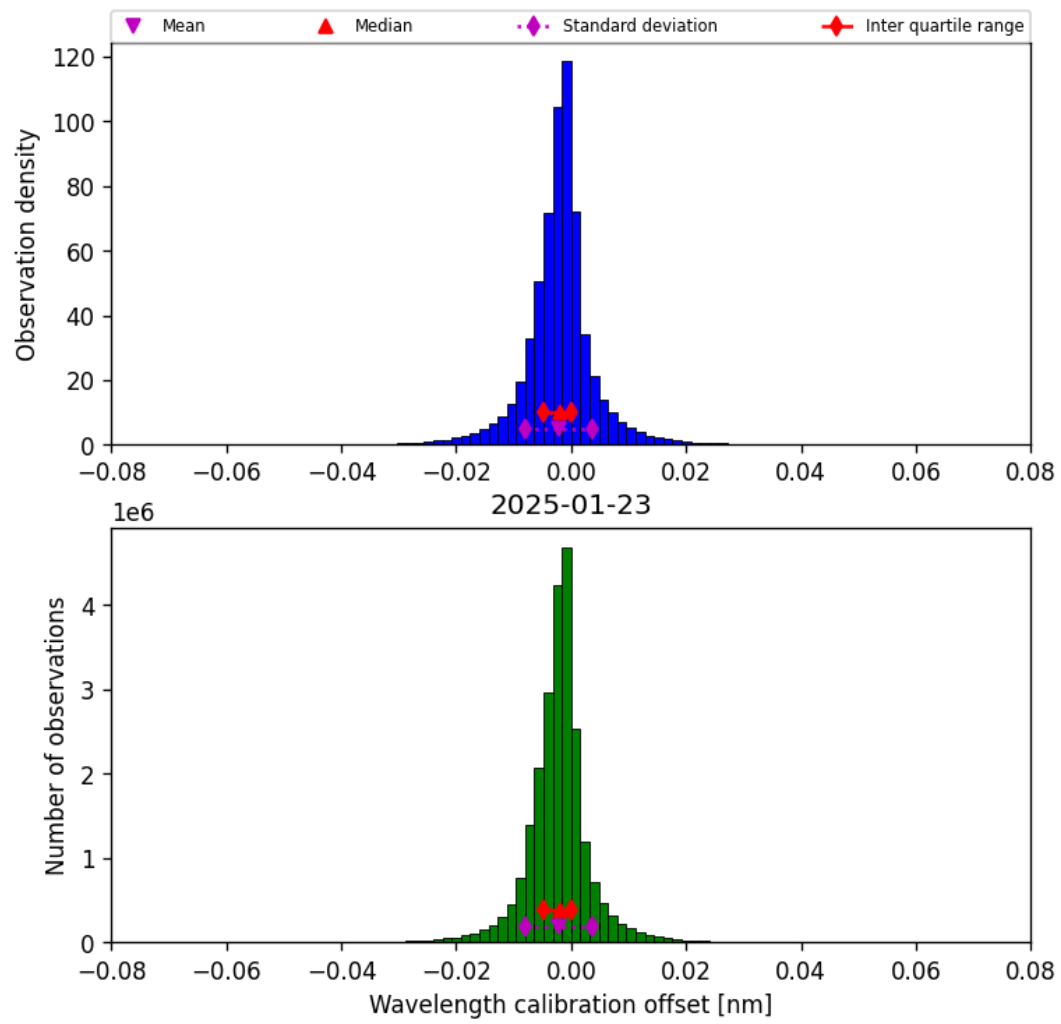
Figure 33: Histogram of “Wavelength calibration offset” for 2025-01-23 to 2025-01-24
