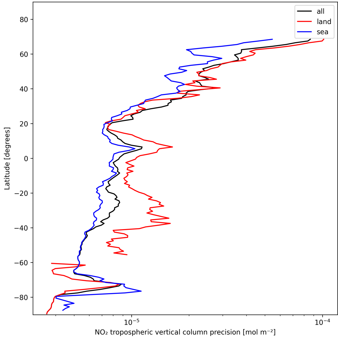
Figure 11: Zonal average of “NO 2 tropospheric vertical column precision” for 2025-01-23 to 2025-01-24.
