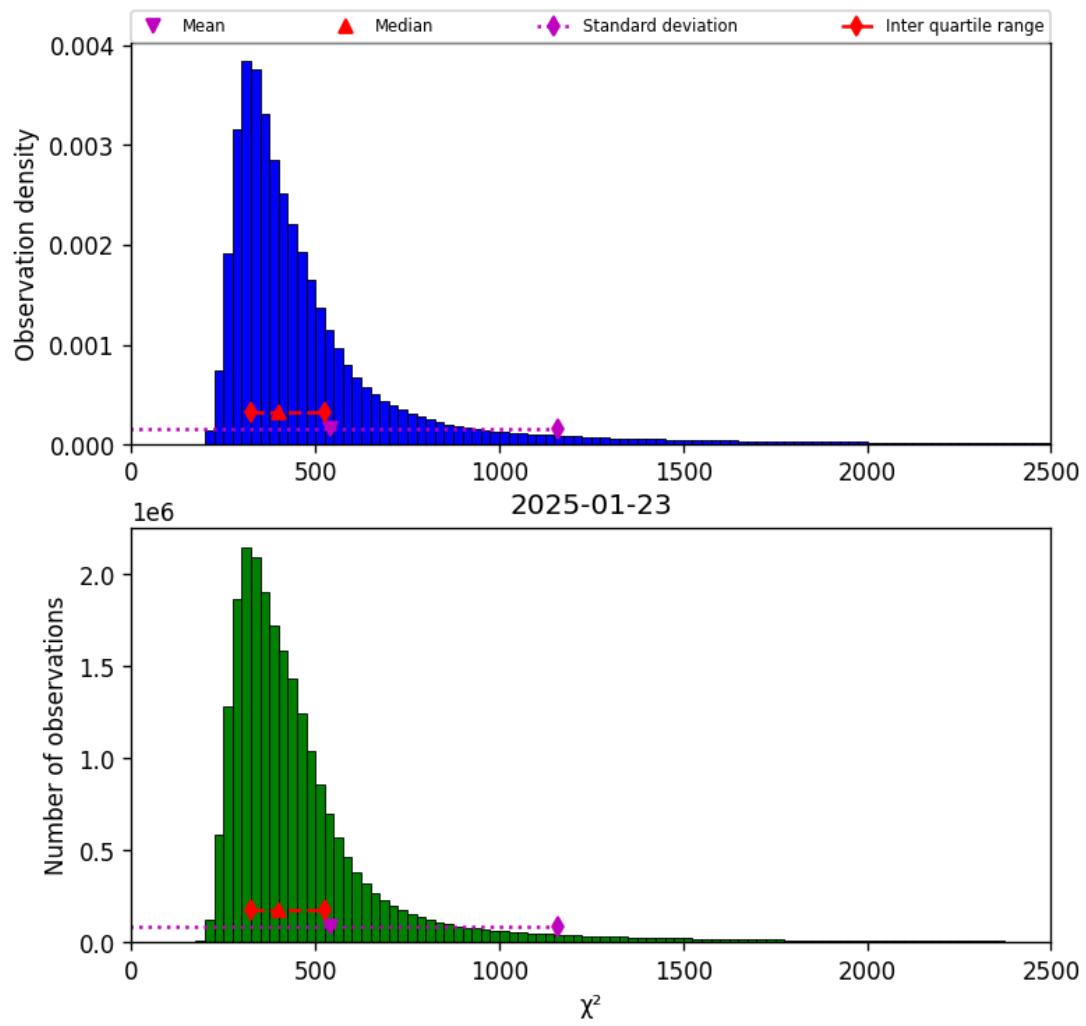
Figure 40: Histogram of “ \chi^2 ” for 2025-01-23 to 2025-01-24
