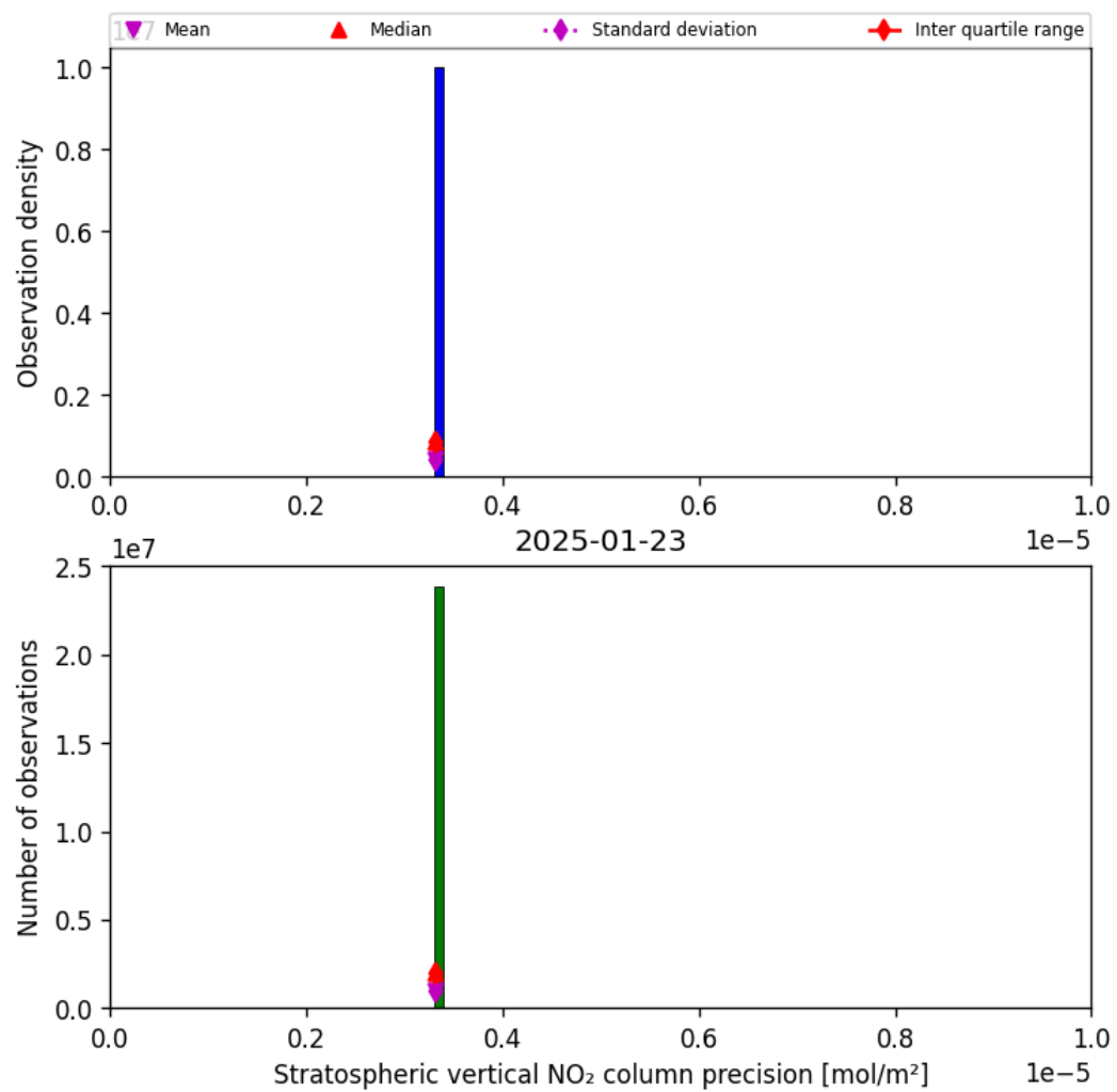
Figure 35: Histogram of “Stratospheric vertical NO 2 column precision” for 2025-01-23 to 2025-01-24
