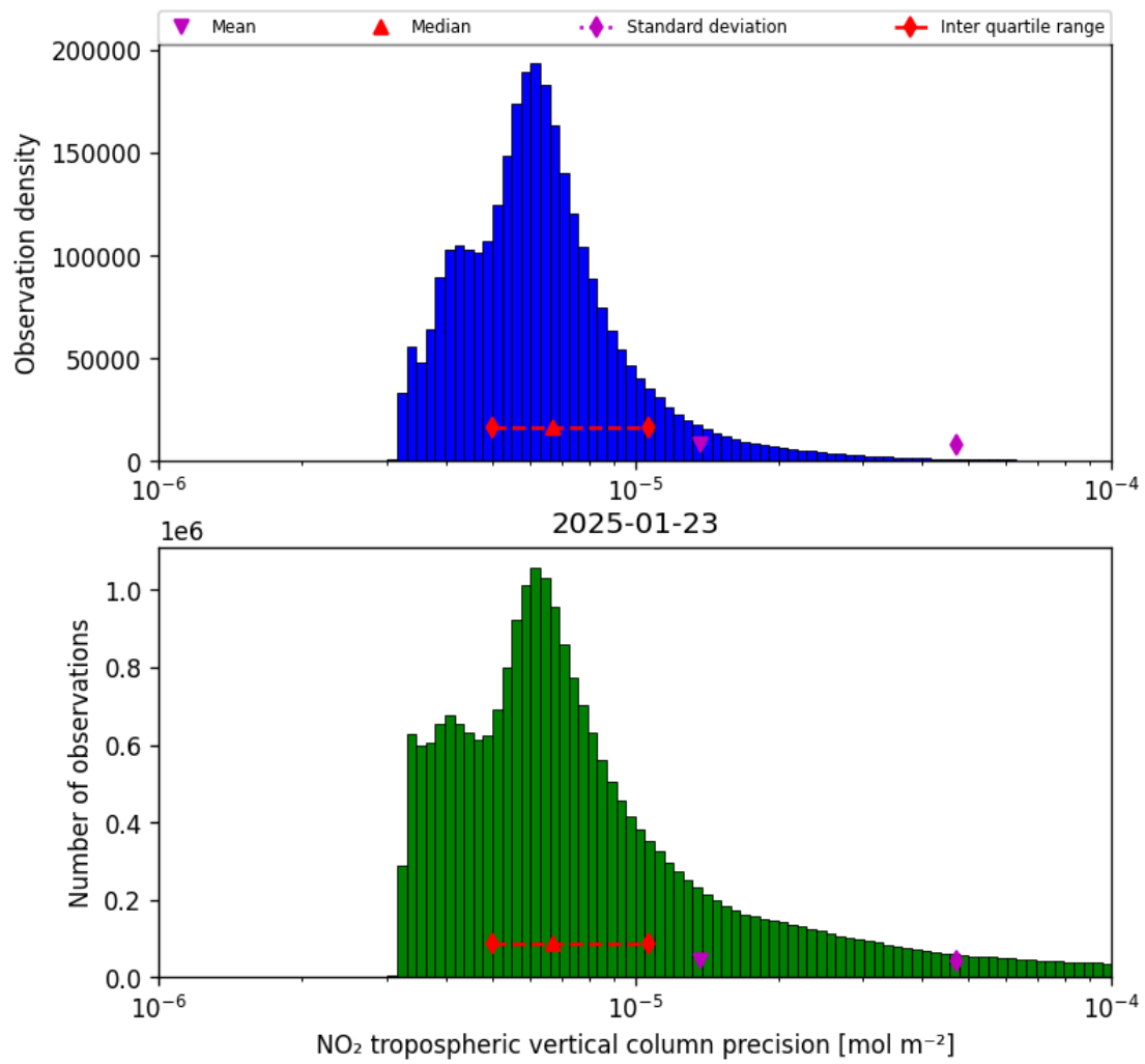
Figure 28: Histogram of “NO 2 tropospheric vertical column precision” for 2025-01-23 to 2025-01-24
