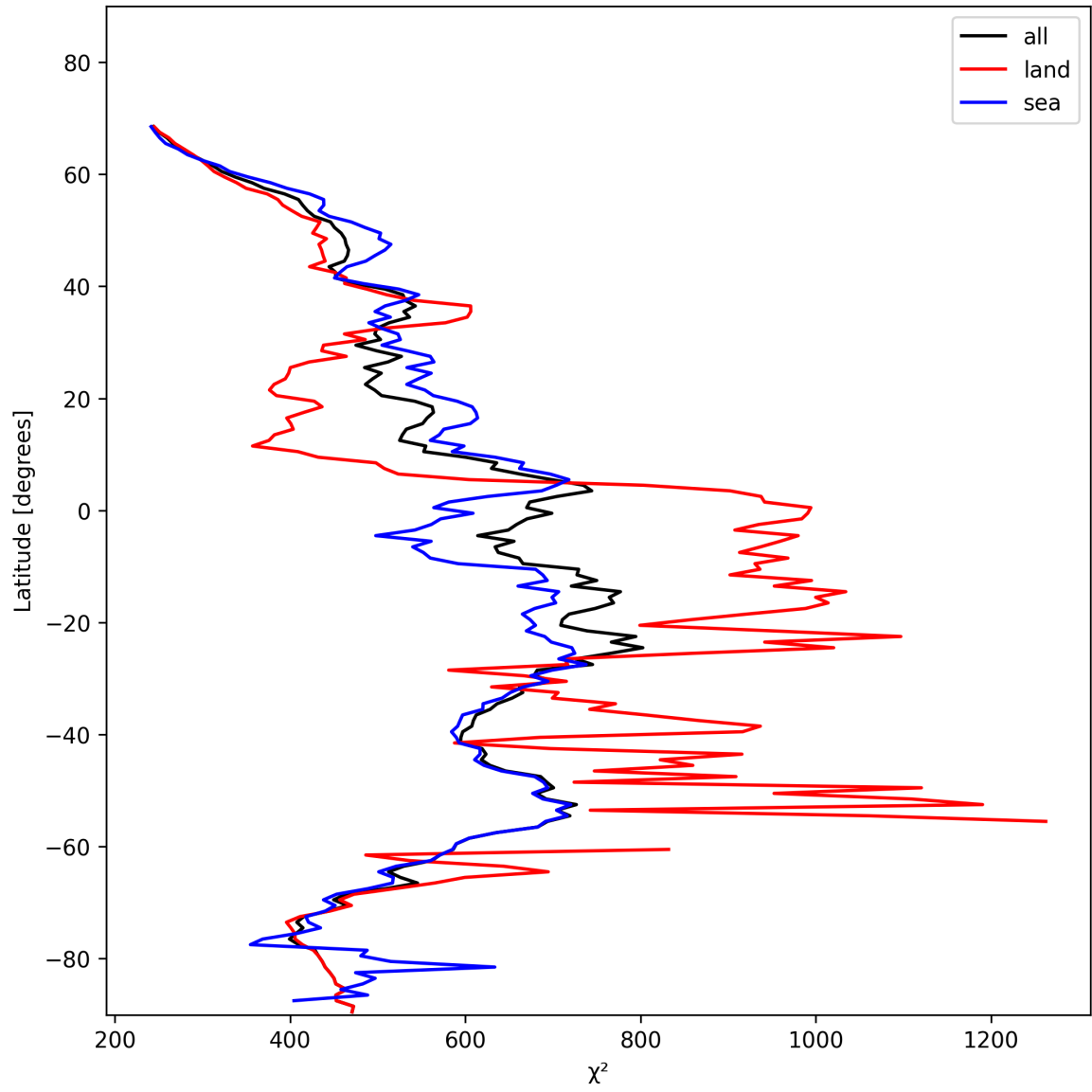
Figure 23: Zonal average of “ \chi^2 ” for 2025-01-23 to 2025-01-24.
