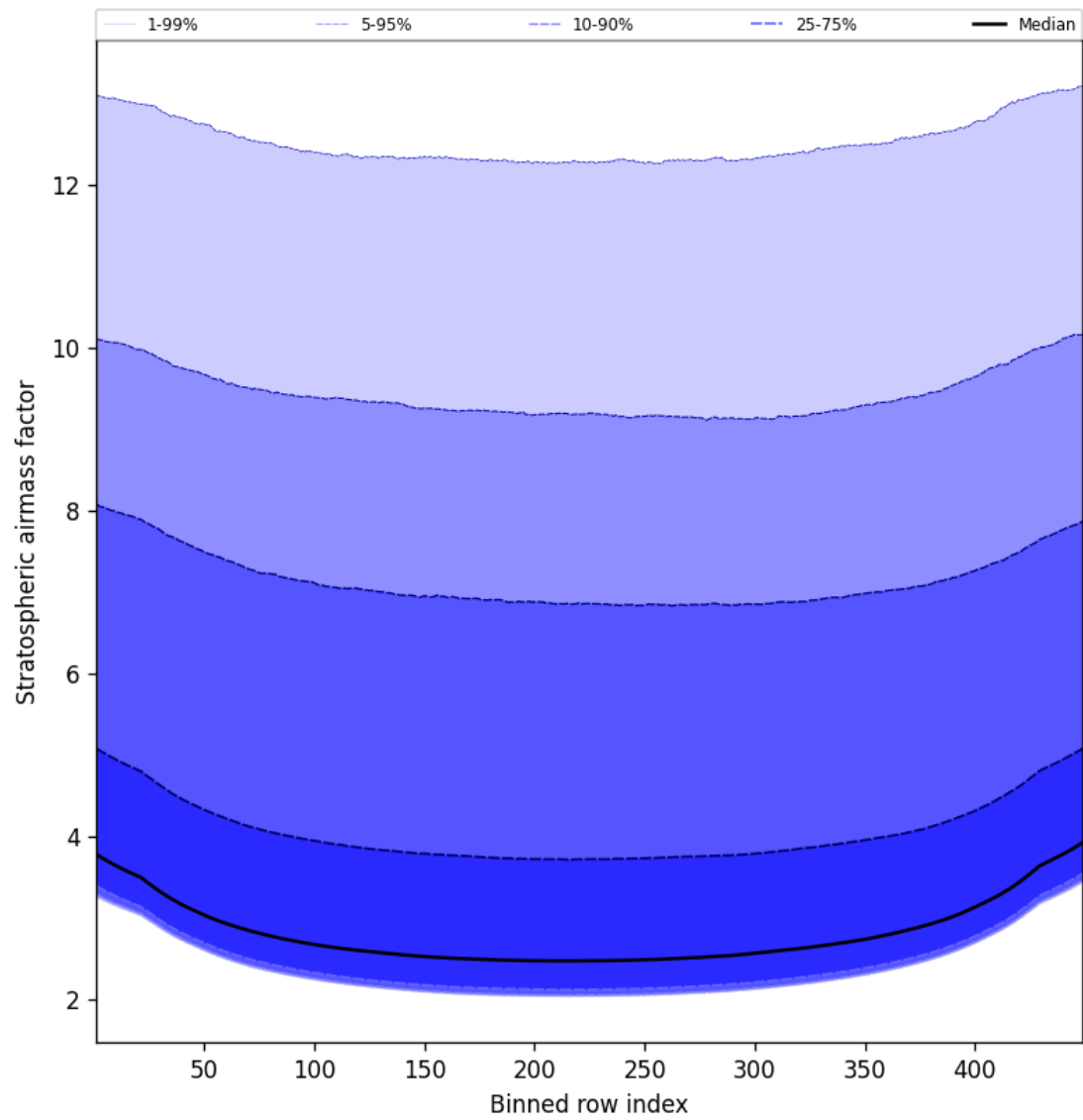
Figure 59: Along track statistics of “Stratospheric airmass factor” for 2025-01-23 to 2025-01-24
