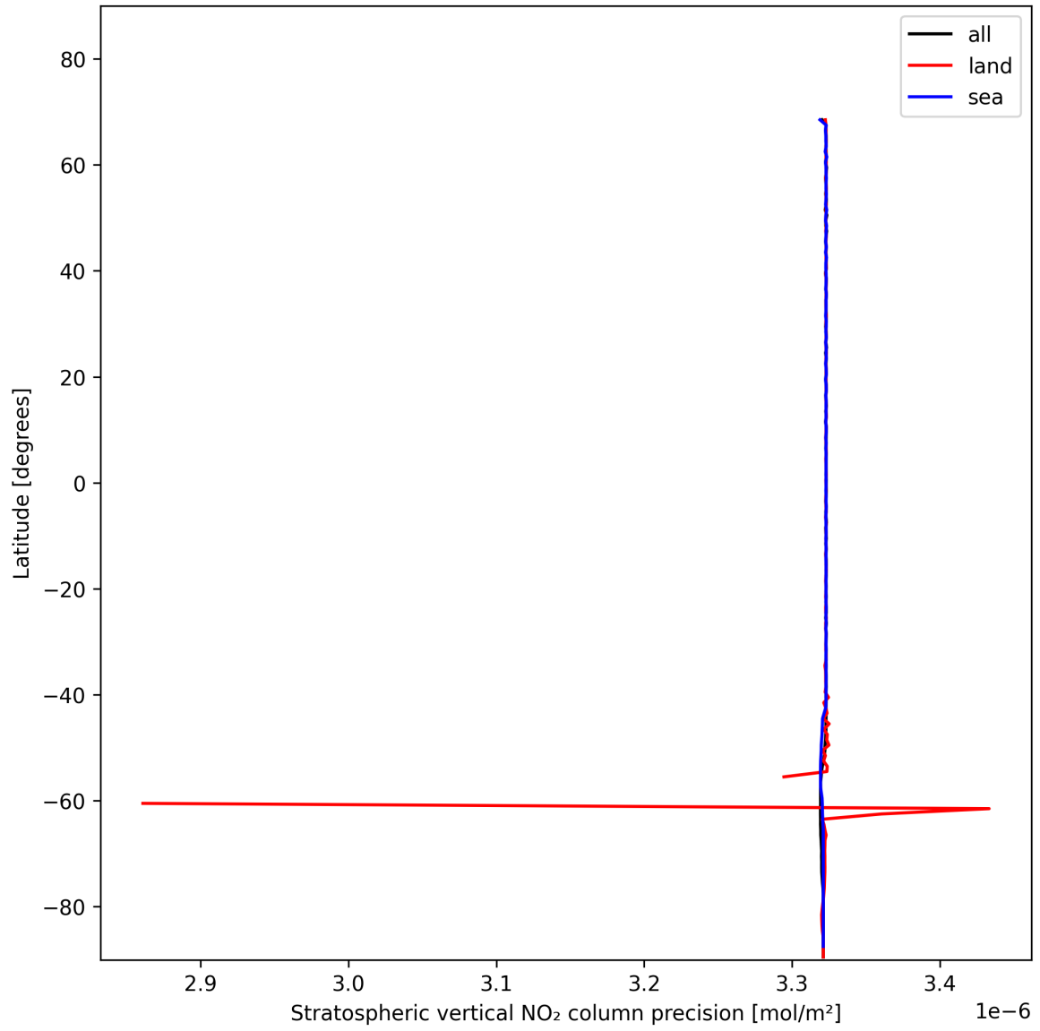
Figure 18: Zonal average of “Stratospheric vertical NO 2 column precision” for 2025-01-23 to 2025-01-24.
