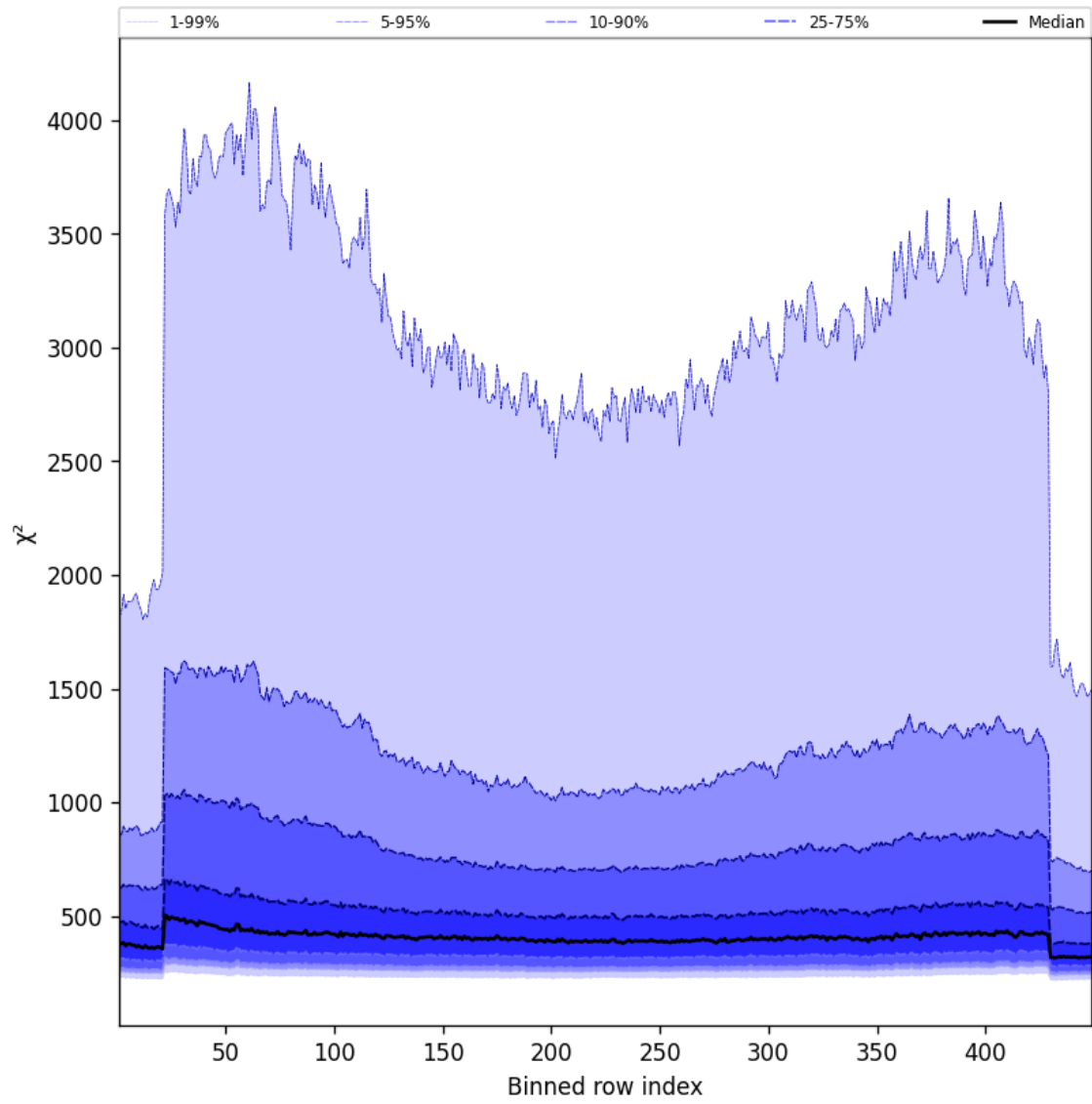
Figure 57: Along track statistics of “ \chi^2 ” for 2025-01-23 to 2025-01-24
