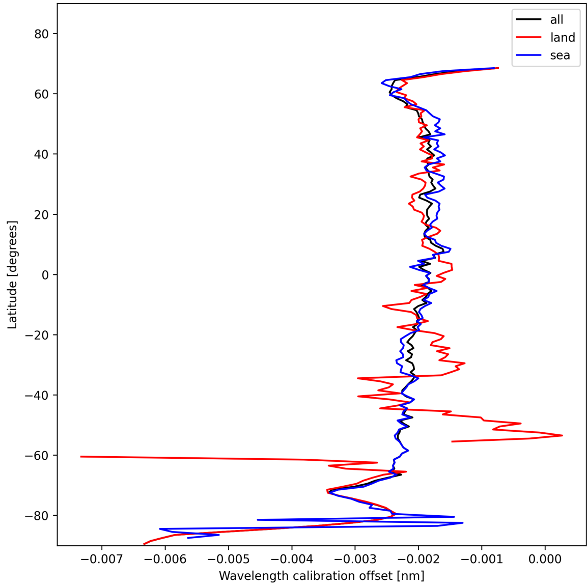
Figure 16: Zonal average of “Wavelength calibration offset” for 2025-01-23 to 2025-01-24.
