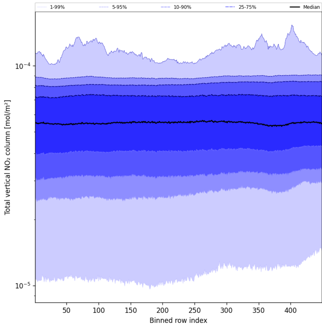
Figure 53: Along track statistics of “Total vertical NO 2 column” for 2025-01-23 to 2025-01-24
