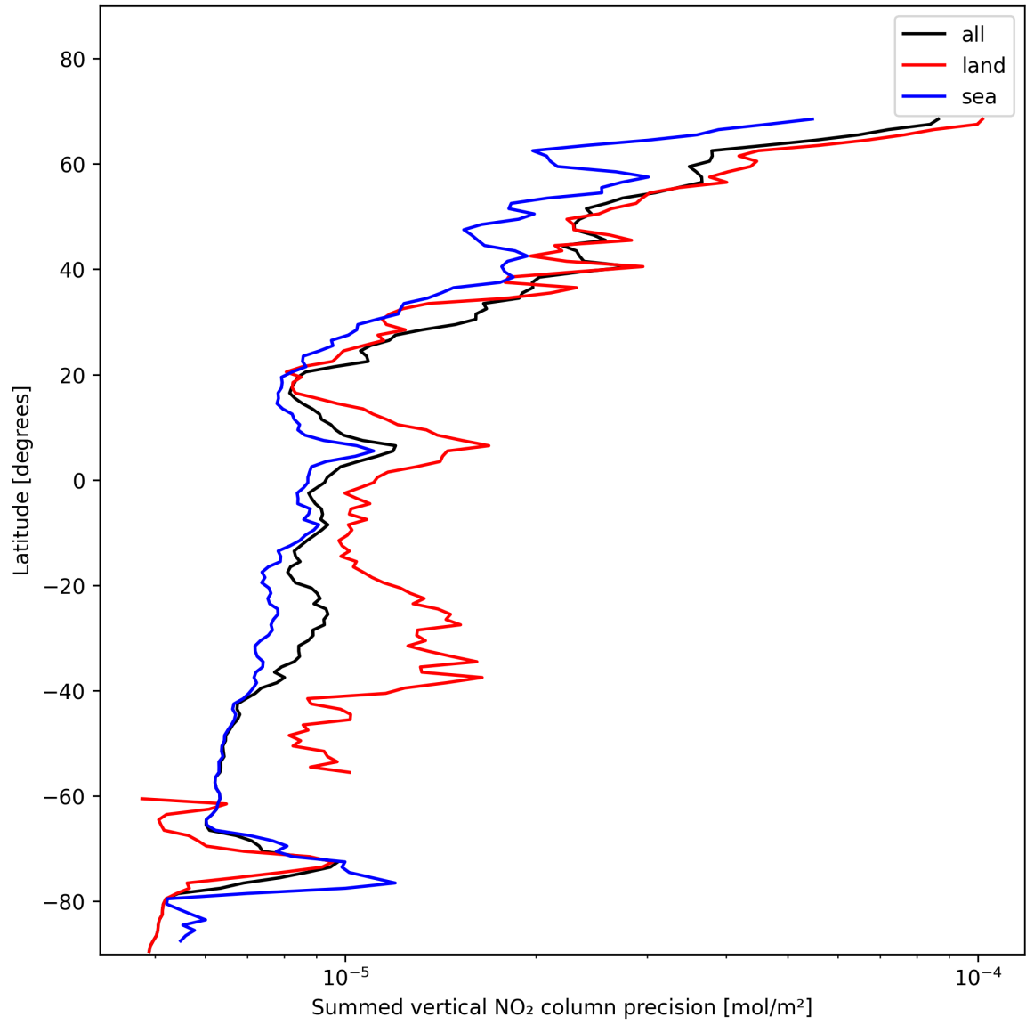
Figure 22: Zonal average of “Summed vertical NO 2 column precision” for 2025-01-23 to 2025-01-24.
