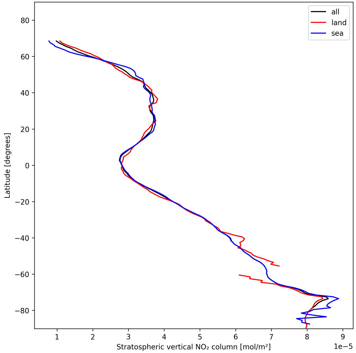
Figure 17: Zonal average of “Stratospheric vertical NO 2 column” for 2025-01-23 to 2025-01-24.
