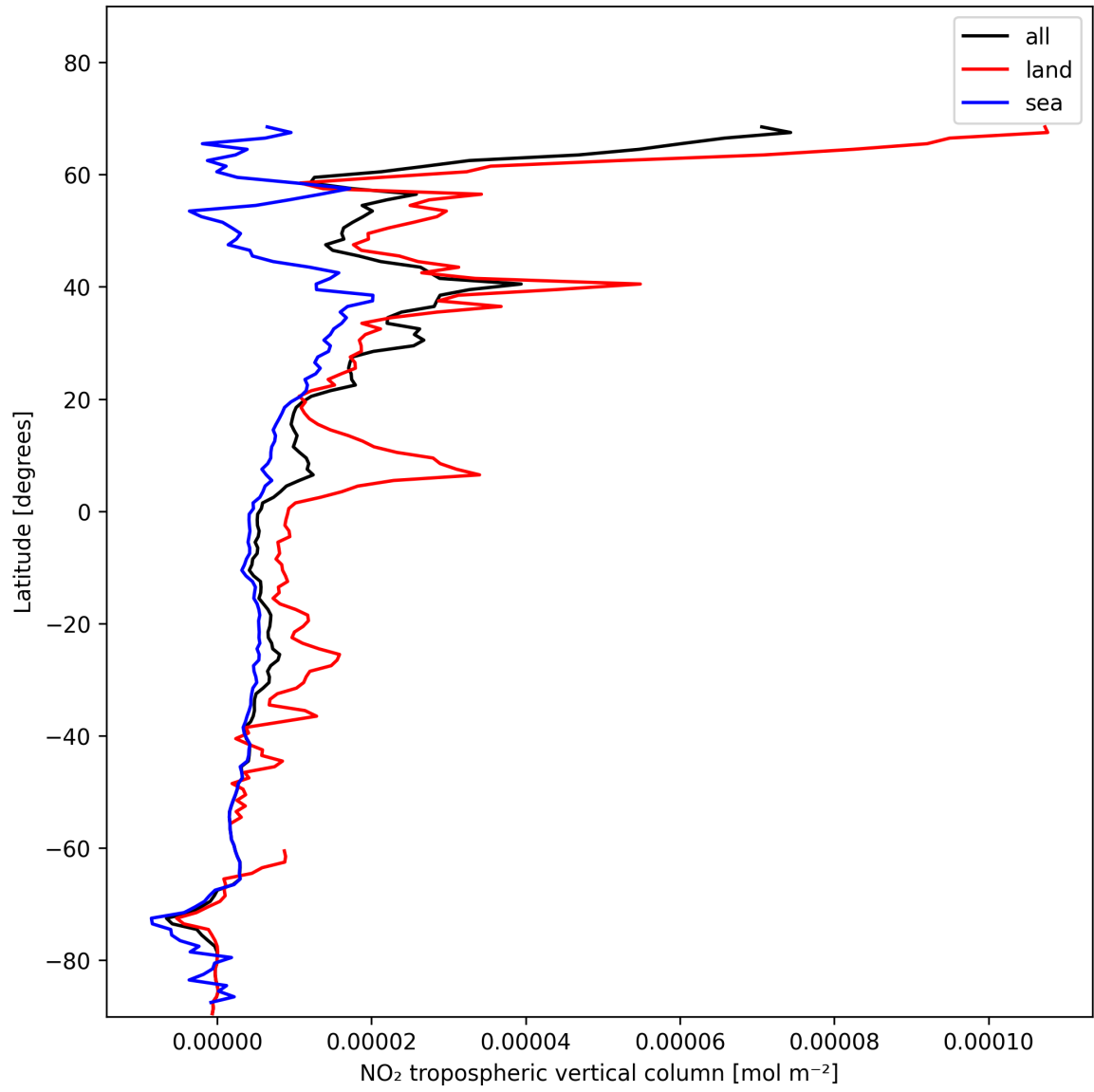
Figure 10: Zonal average of “NO 2 tropospheric vertical column” for 2025-01-23 to 2025-01-24.
