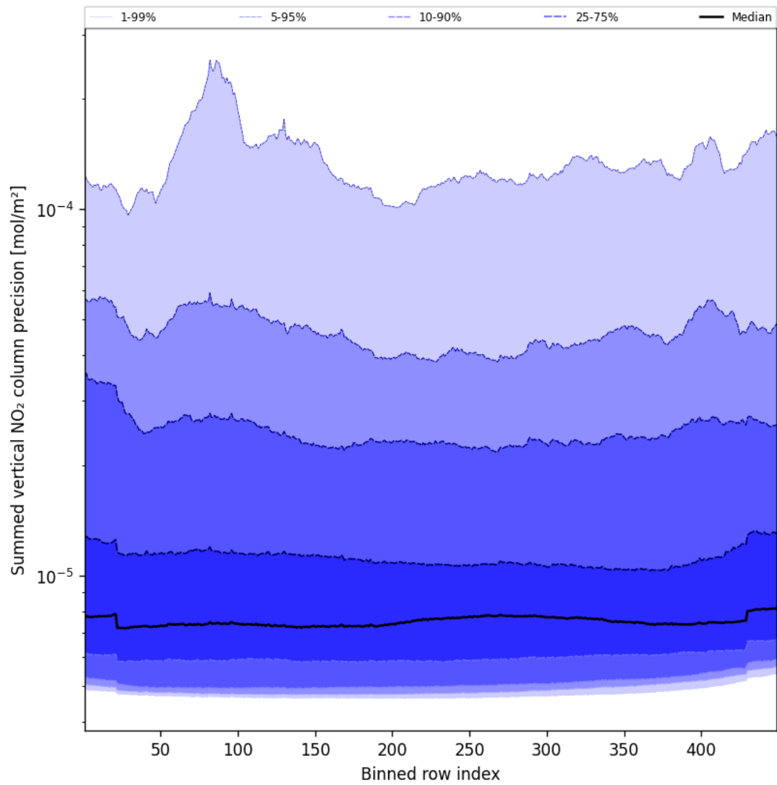
Figure 56: Along track statistics of “Summed vertical NO 2 column precision” for 2025-01-23 to 2025-01-24
