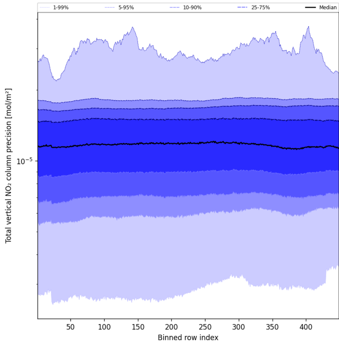
Figure 54: Along track statistics of “Total vertical NO 2 column precision” for 2025-01-23 to 2025-01-24
