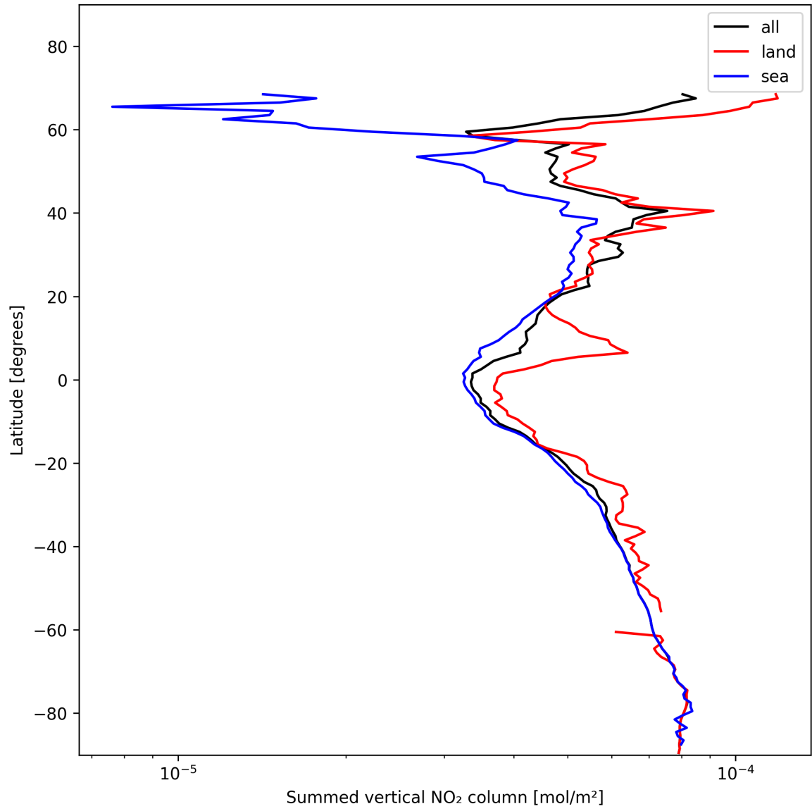
Figure 21: Zonal average of “Summed vertical NO 2 column” for 2025-01-23 to 2025-01-24.
