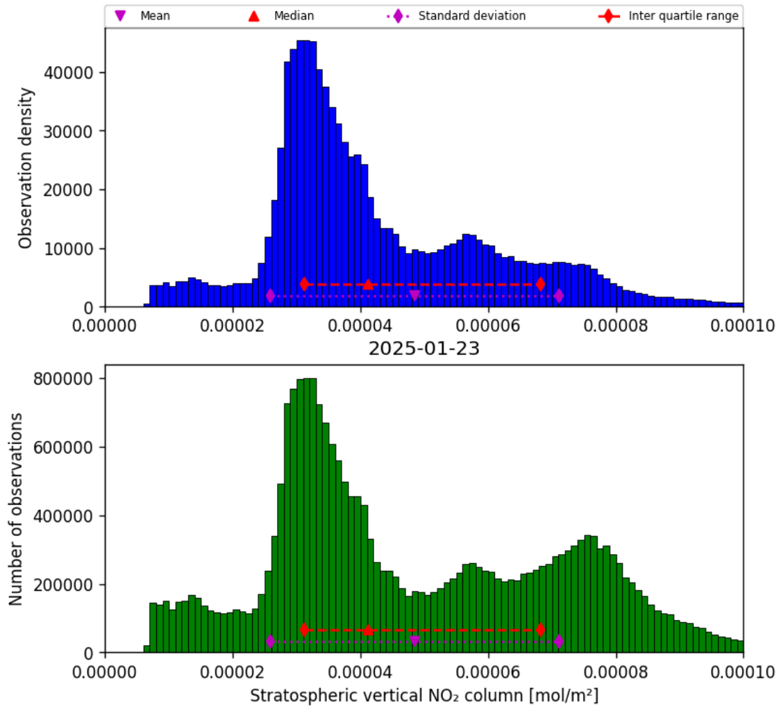
Figure 34: Histogram of “Stratospheric vertical NO 2 column” for 2025-01-23 to 2025-01-24
