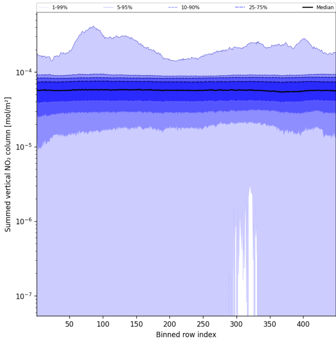
Figure 55: Along track statistics of “Summed vertical NO 2 column” for 2025-01-23 to 2025-01-24
