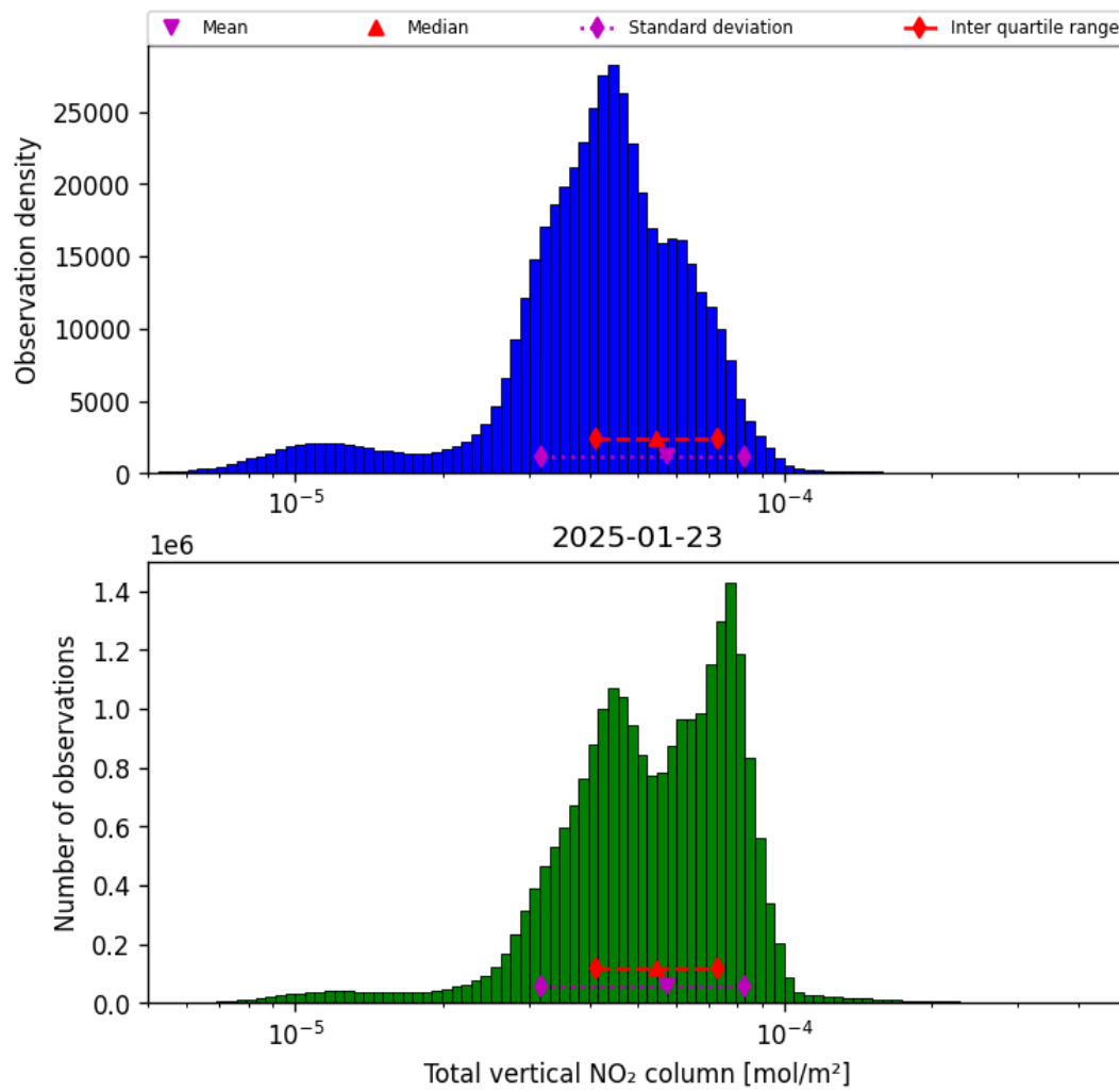
Figure 36: Histogram of “Total vertical NO 2 column” for 2025-01-23 to 2025-01-24
