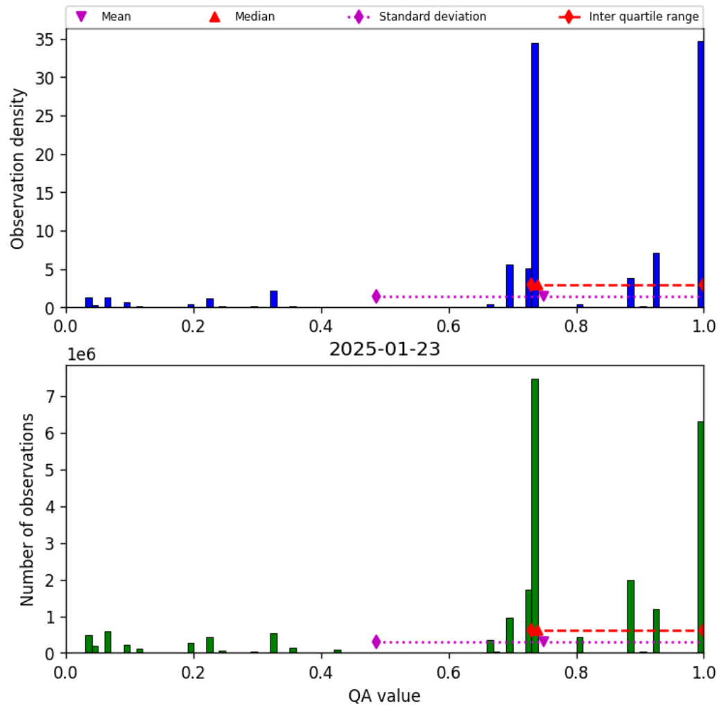
Figure 26: Histogram of “QA value” for 2025-01-23 to 2025-01-24
