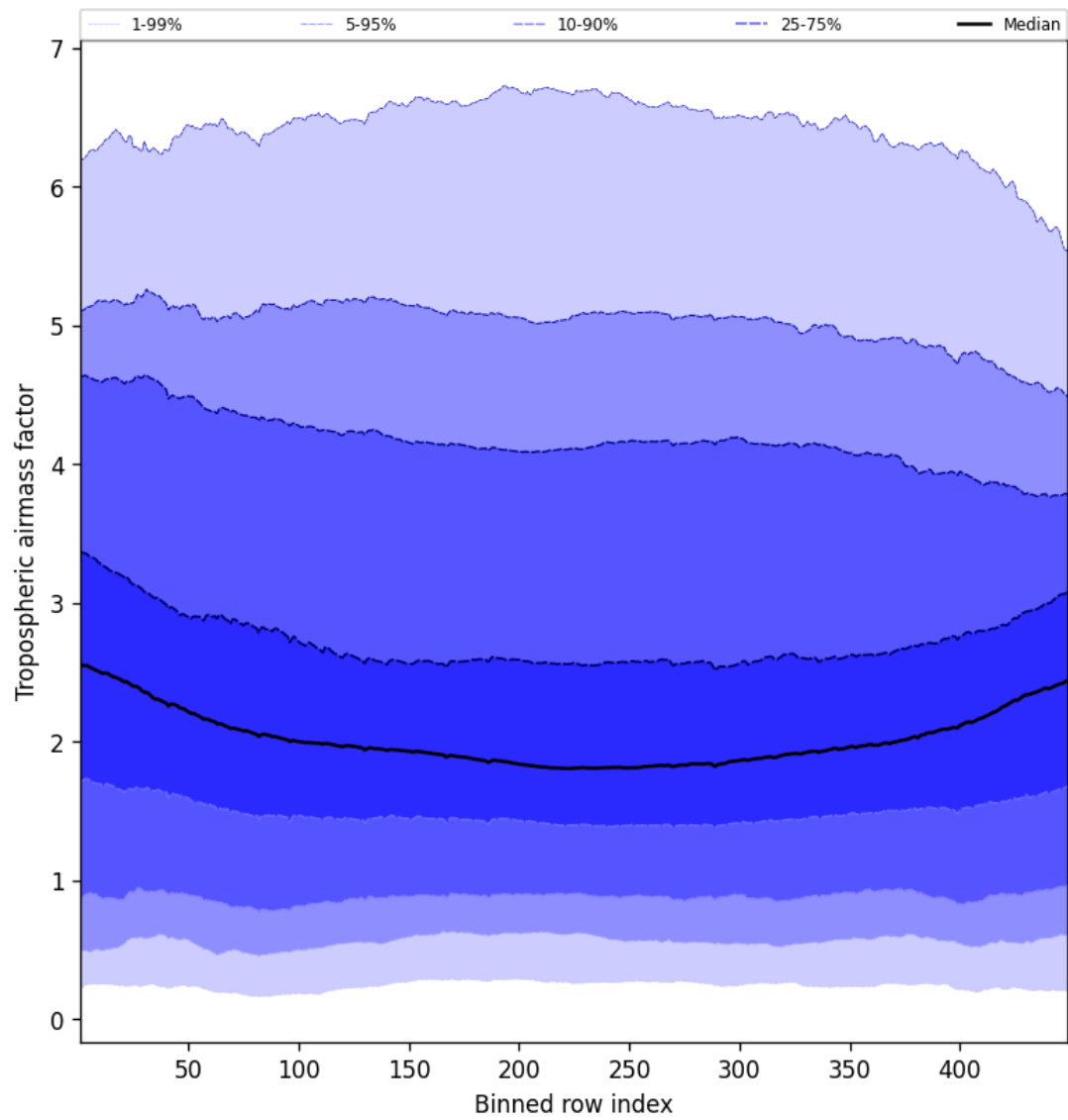
Figure 46: Along track statistics of “Tropospheric airmass factor” for 2025-01-23 to 2025-01-24
