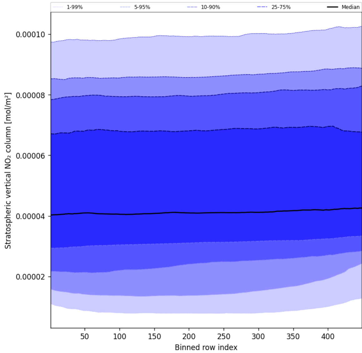
Figure 51: Along track statistics of “Stratospheric vertical NO 2 column” for 2025-01-23 to 2025-01-24
