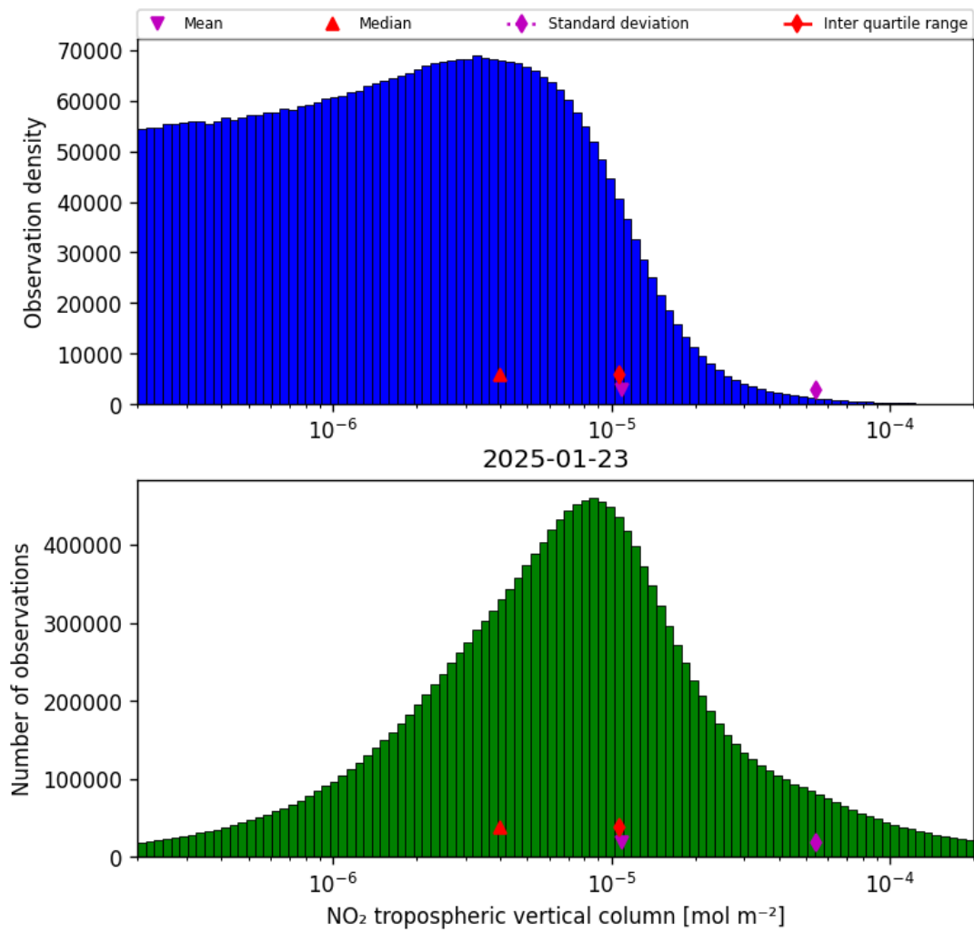
Figure 27: Histogram of “NO 2 tropospheric vertical column” for 2025-01-23 to 2025-01-24
