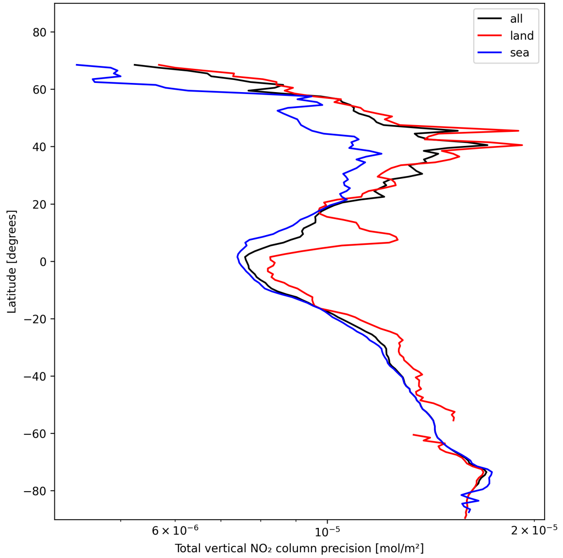
Figure 20: Zonal average of “Total vertical NO 2 column precision” for 2025-01-23 to 2025-01-24.
