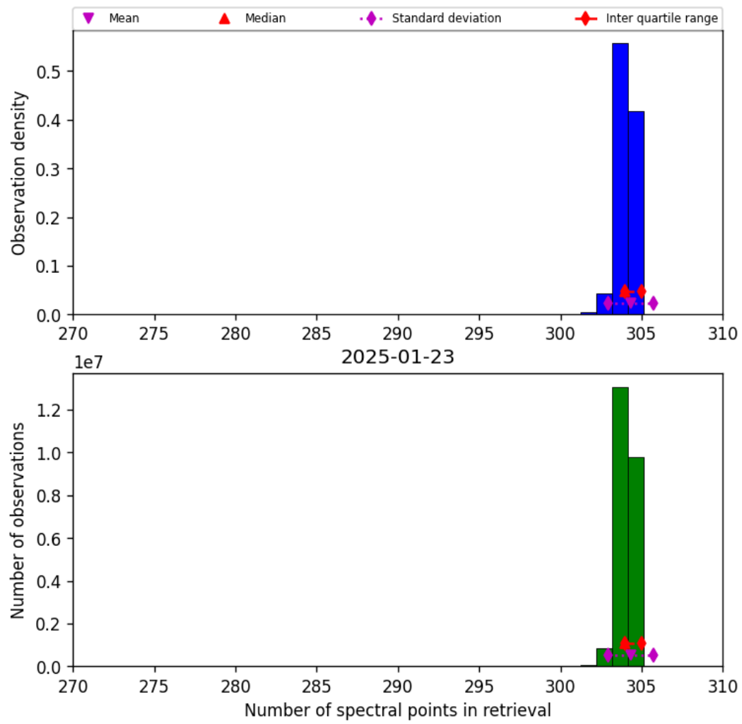
Figure 31: Histogram of “Number of spectral points in retrieval” for 2025-01-23 to 2025-01-24
