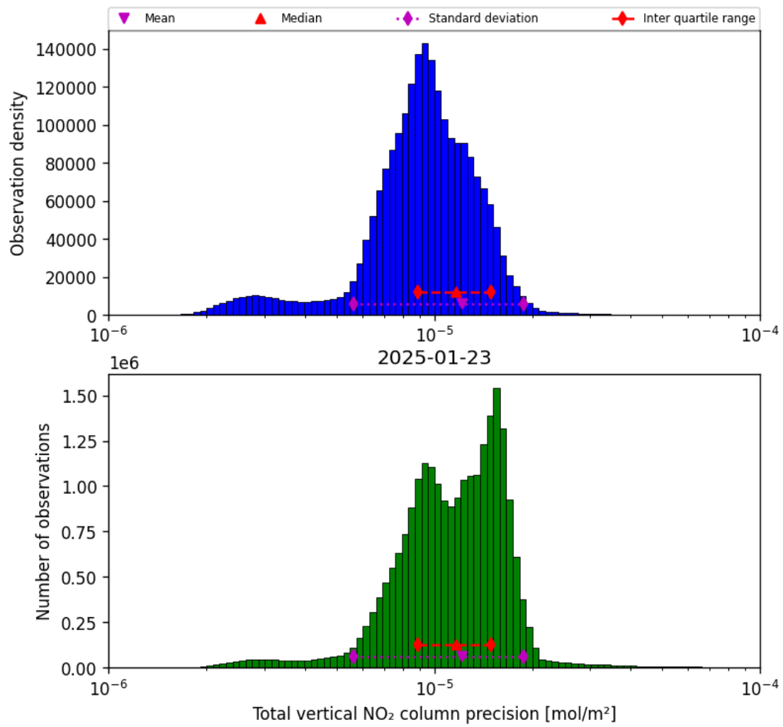
Figure 37: Histogram of “Total vertical NO 2 column precision” for 2025-01-23 to 2025-01-24
