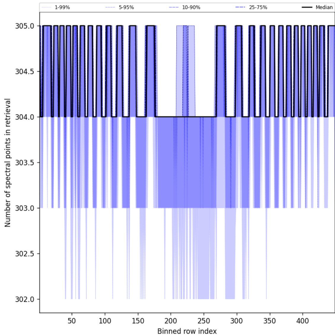
Figure 48: Along track statistics of “Number of spectral points in retrieval” for 2025-01-23 to 2025-01-24
