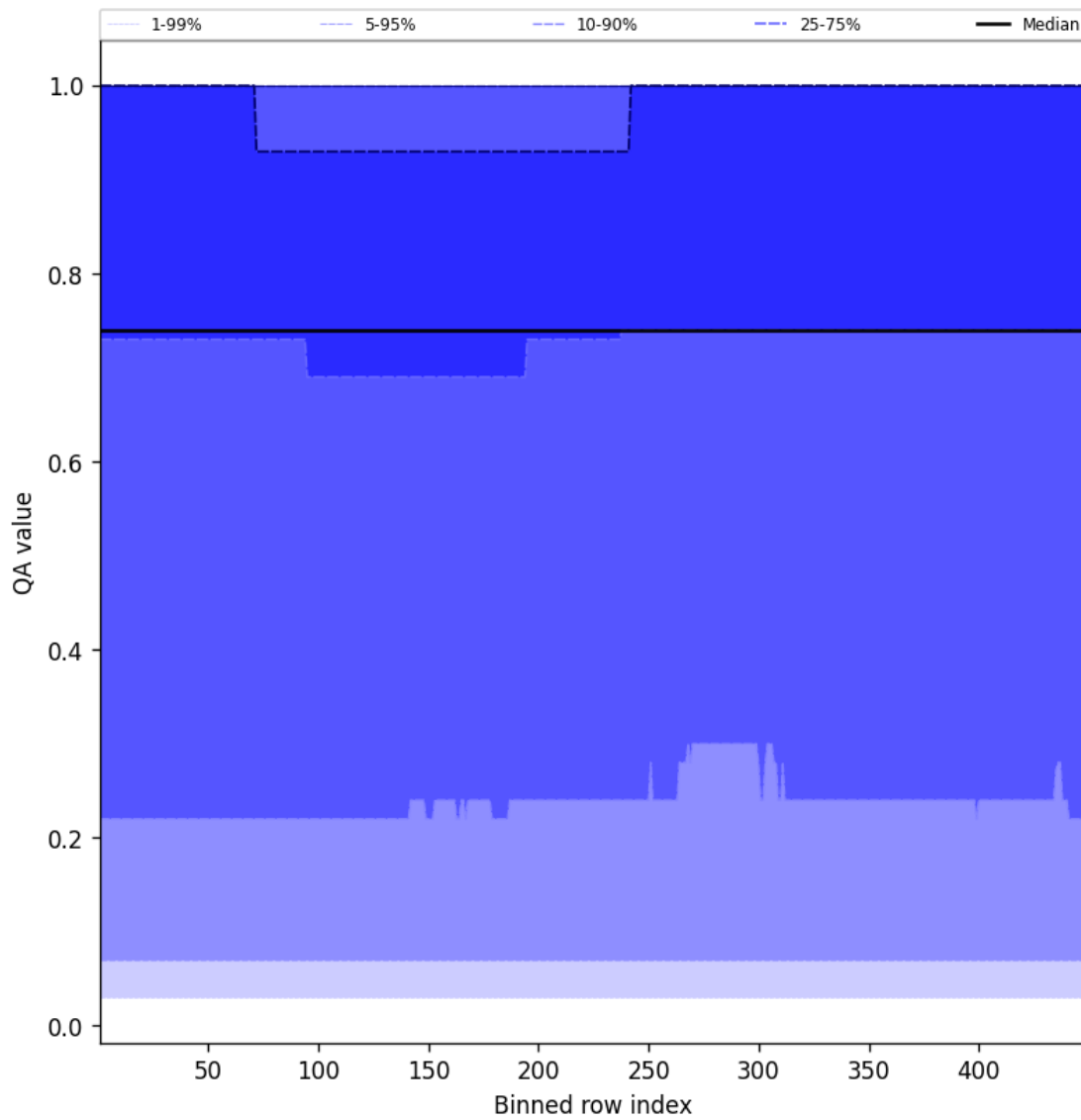
Figure 43: Along track statistics of “QA value” for 2025-01-23 to 2025-01-24
