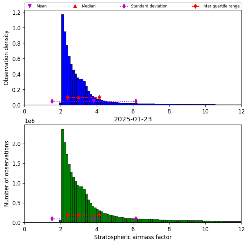
Figure 42: Histogram of “Stratospheric airmass factor” for 2025-01-23 to 2025-01-24
