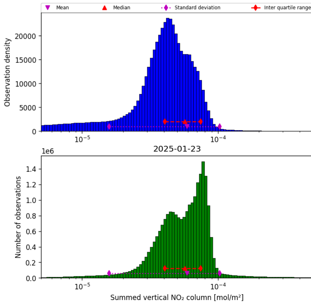
Figure 38: Histogram of “Summed vertical NO 2 column” for 2025-01-23 to 2025-01-24
