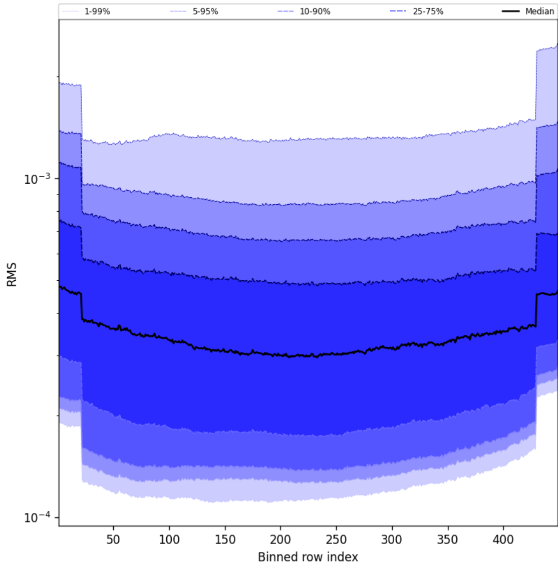
Figure 58: Along track statistics of “RMS” for 2025-01-23 to 2025-01-24
