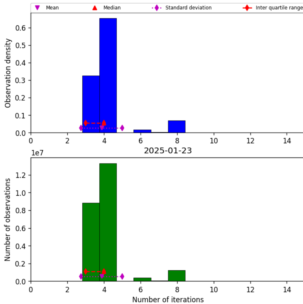
Figure 32: Histogram of “Number of iterations” for 2025-01-23 to 2025-01-24
