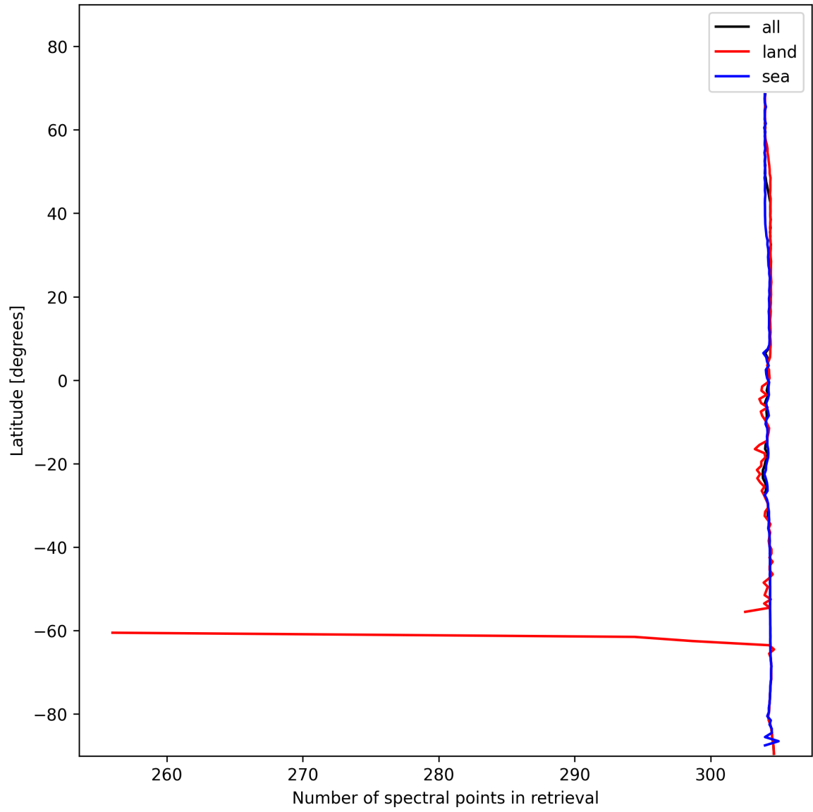
Figure 14: Zonal average of “Number of spectral points in retrieval” for 2025-01-23 to 2025-01-24.
