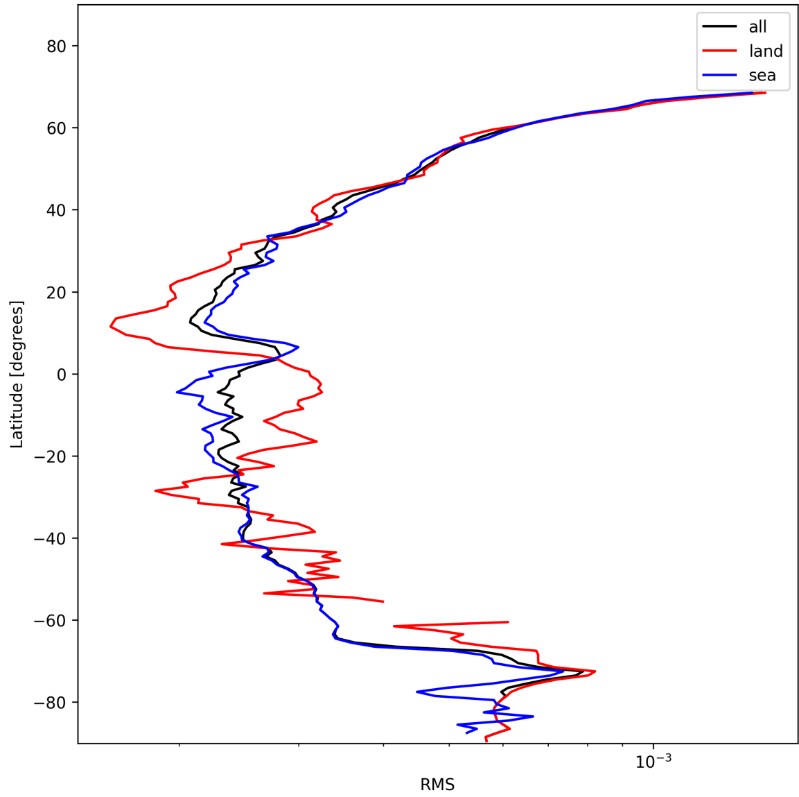
Figure 24: Zonal average of “RMS” for 2025-01-23 to 2025-01-24.
