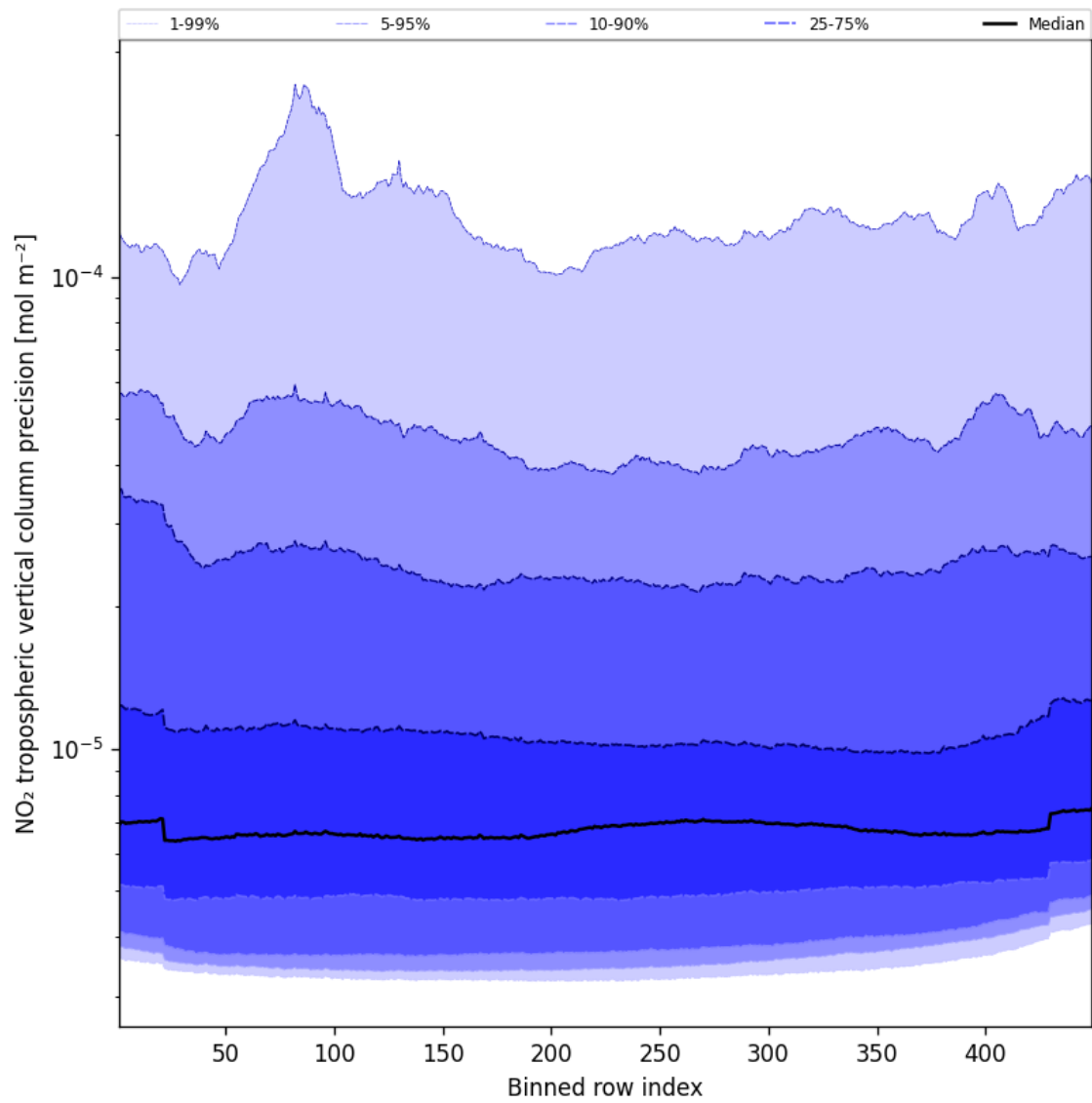
Figure 45: Along track statistics of “NO 2 tropospheric vertical column precision” for 2025-01-23 to 2025-01-24
