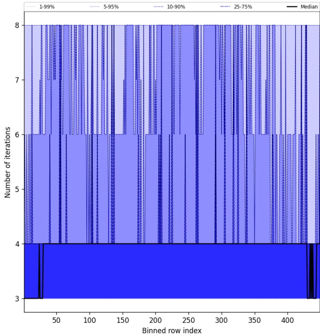
Figure 49: Along track statistics of “Number of iterations” for 2025-01-23 to 2025-01-24
