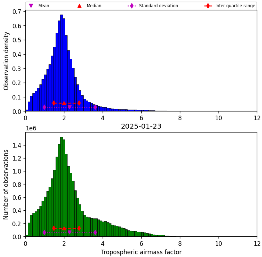
Figure 29: Histogram of “Tropospheric airmass factor” for 2025-01-23 to 2025-01-24
