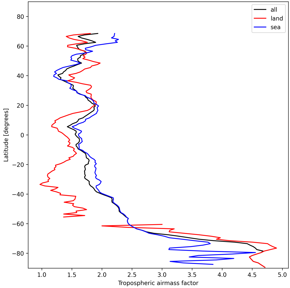
Figure 12: Zonal average of “Tropospheric airmass factor” for 2025-01-23 to 2025-01-24.
