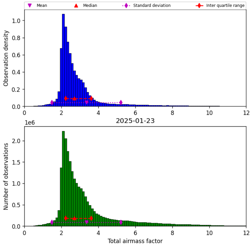
Figure 30: Histogram of “Total airmass factor” for 2025-01-23 to 2025-01-24
