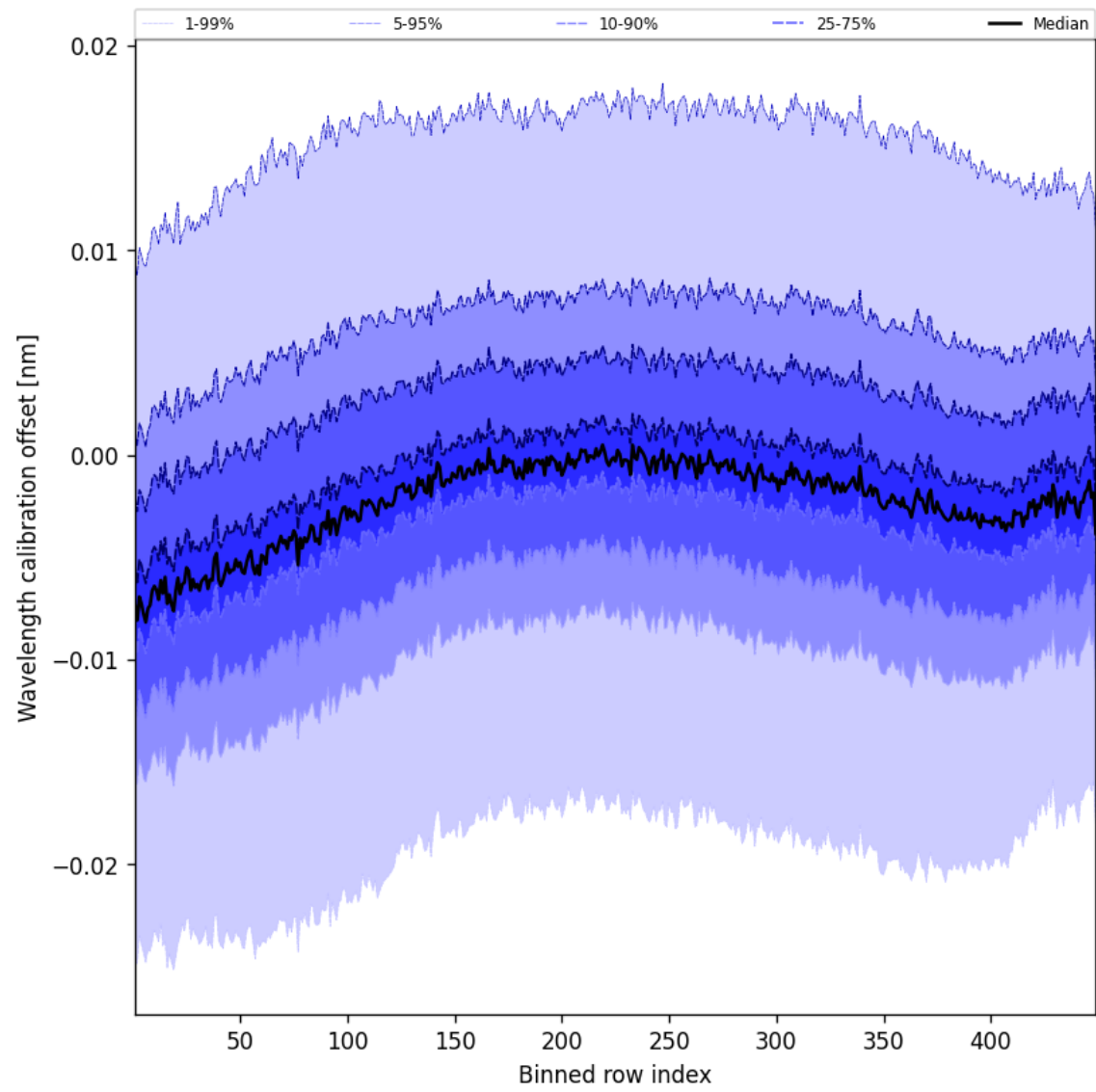
Figure 50: Along track statistics of “Wavelength calibration offset” for 2025-01-23 to 2025-01-24
