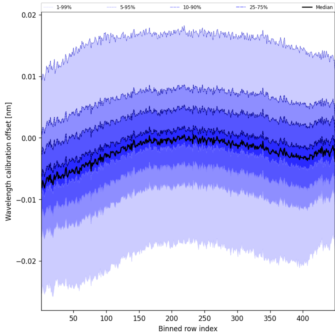
Figure 50: Along track statistics of “Wavelength calibration offset” for 2025-01-24 to 2025-01-25
