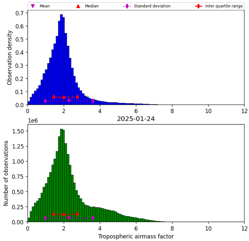
Figure 29: Histogram of “Tropospheric airmass factor” for 2025-01-24 to 2025-01-25
