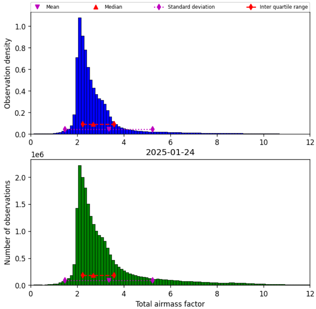
Figure 30: Histogram of “Total airmass factor” for 2025-01-24 to 2025-01-25
