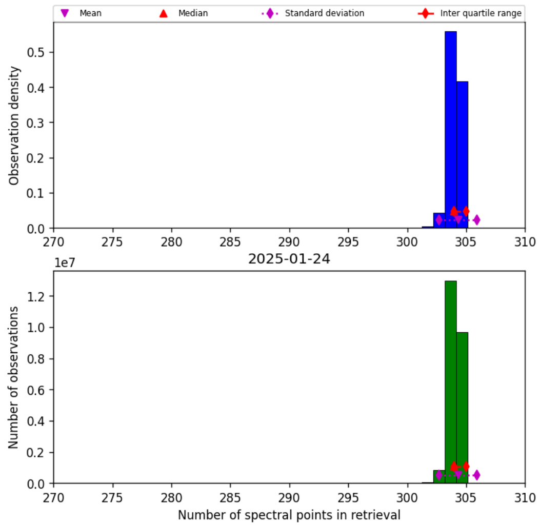
Figure 31: Histogram of “Number of spectral points in retrieval” for 2025-01-24 to 2025-01-25
