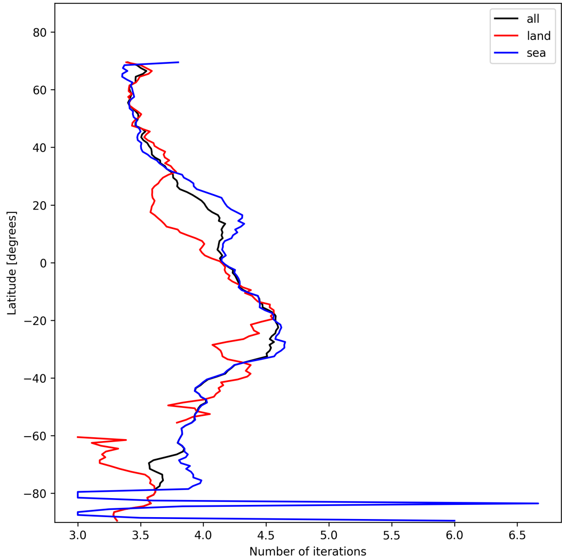
Figure 15: Zonal average of “Number of iterations” for 2025-01-24 to 2025-01-25.
