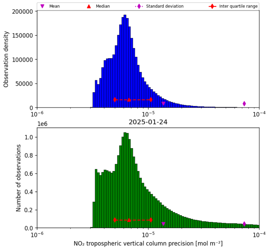
Figure 28: Histogram of “NO 2 tropospheric vertical column precision” for 2025-01-24 to 2025-01-25
