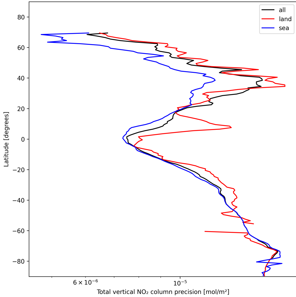
Figure 20: Zonal average of “Total vertical NO 2 column precision” for 2025-01-24 to 2025-01-25.
