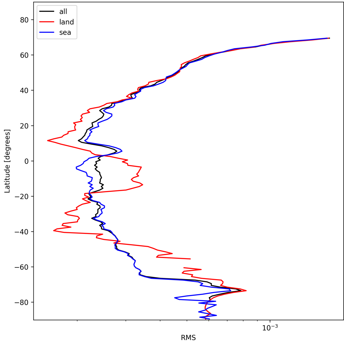
Figure 24: Zonal average of “RMS” for 2025-01-24 to 2025-01-25.
