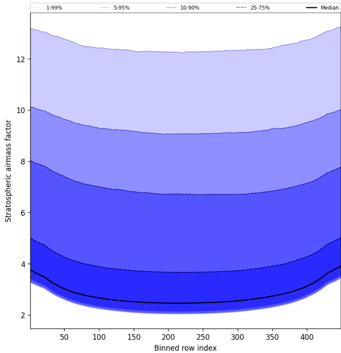
Figure 59: Along track statistics of “Stratospheric airmass factor” for 2025-01-24 to 2025-01-25
