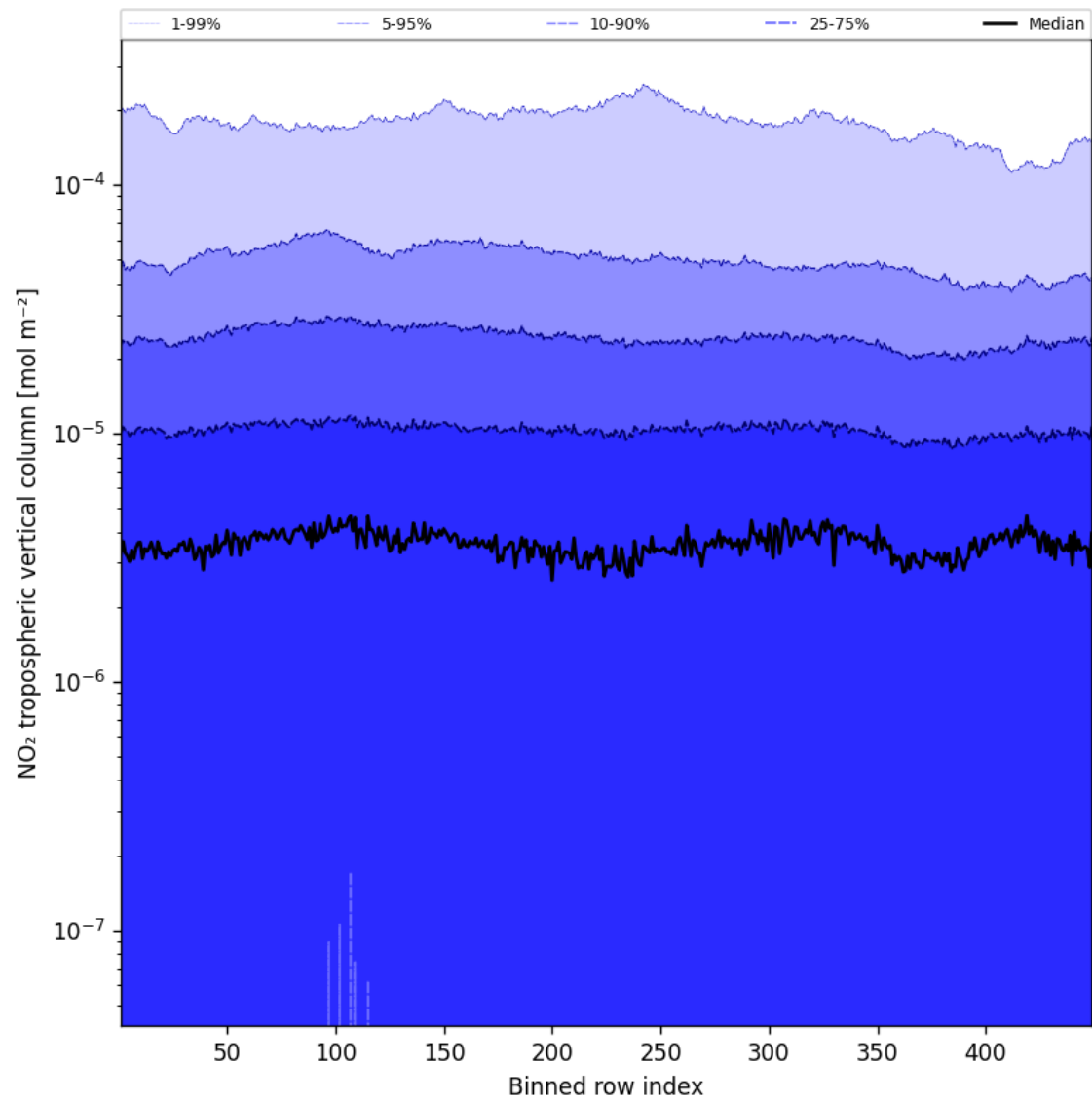
Figure 44: Along track statistics of “NO 2 tropospheric vertical column” for 2025-01-24 to 2025-01-25
