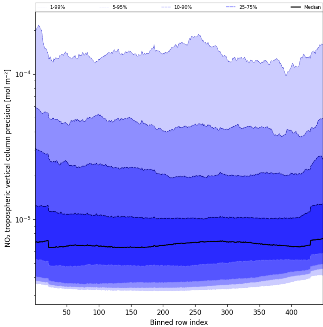
Figure 45: Along track statistics of “NO 2 tropospheric vertical column precision” for 2025-01-24 to 2025-01-25
