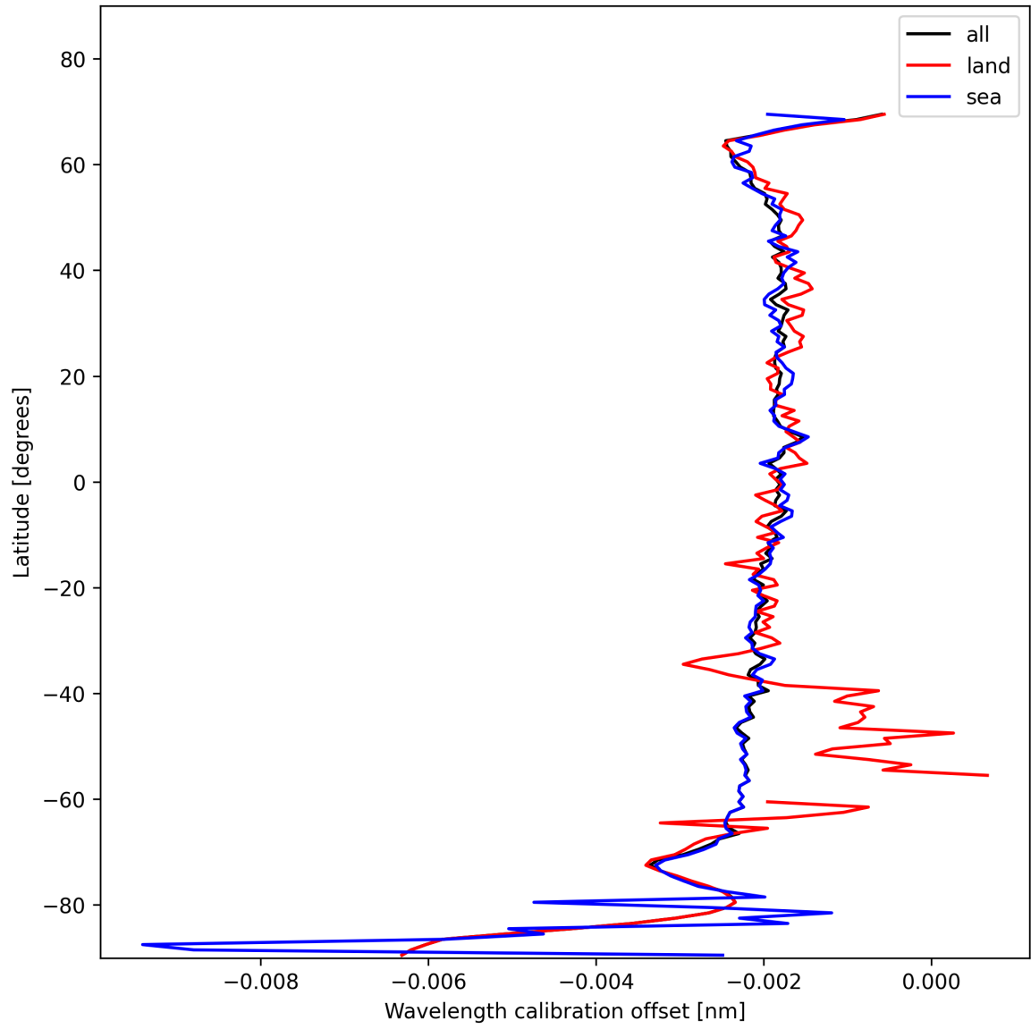
Figure 16: Zonal average of “Wavelength calibration offset” for 2025-01-24 to 2025-01-25.
