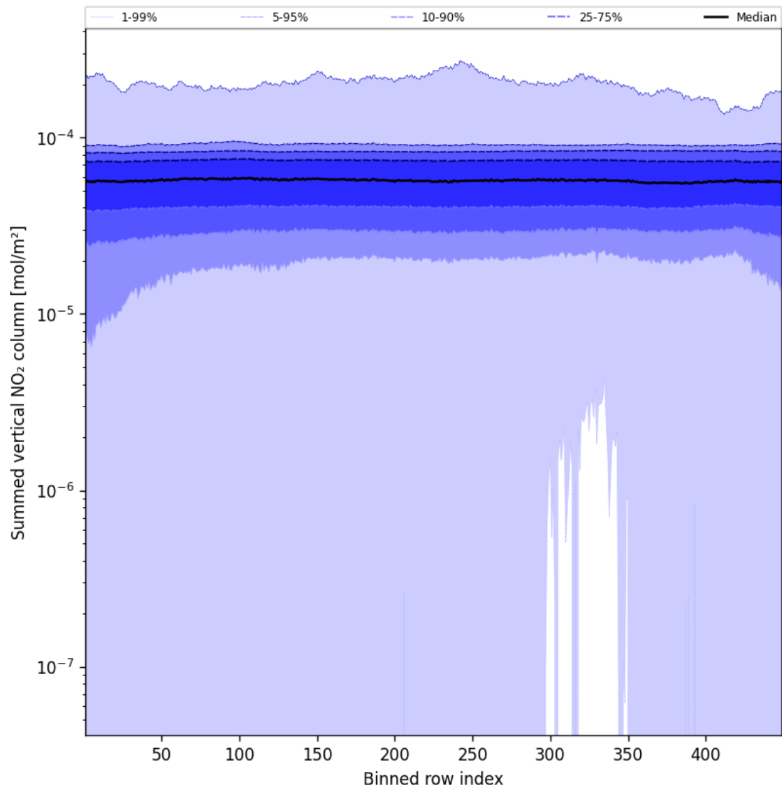
Figure 55: Along track statistics of “Summed vertical NO 2 column” for 2025-01-24 to 2025-01-25
