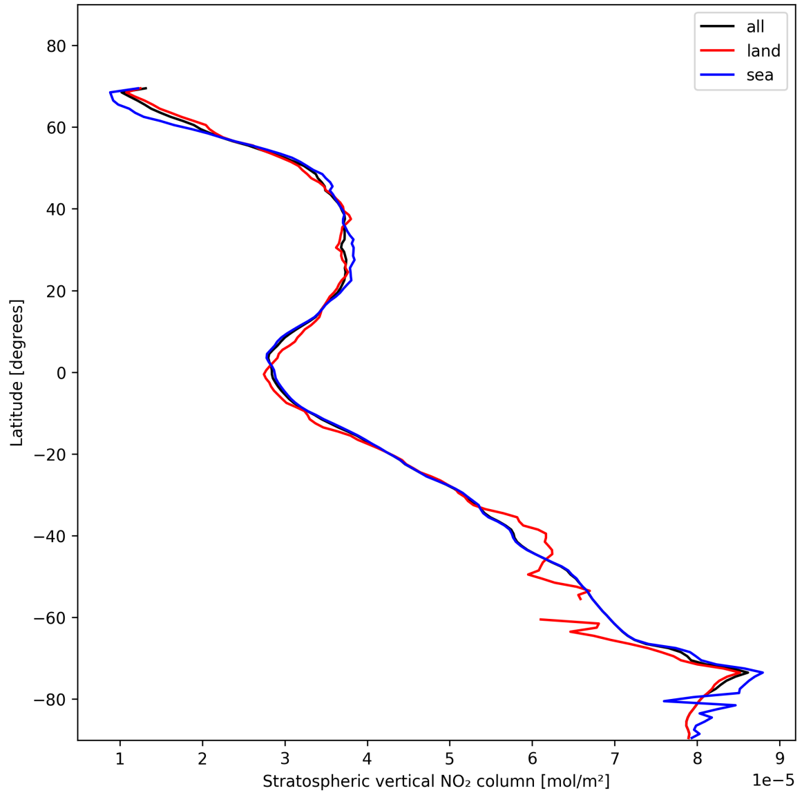
Figure 17: Zonal average of “Stratospheric vertical NO 2 column” for 2025-01-24 to 2025-01-25.
