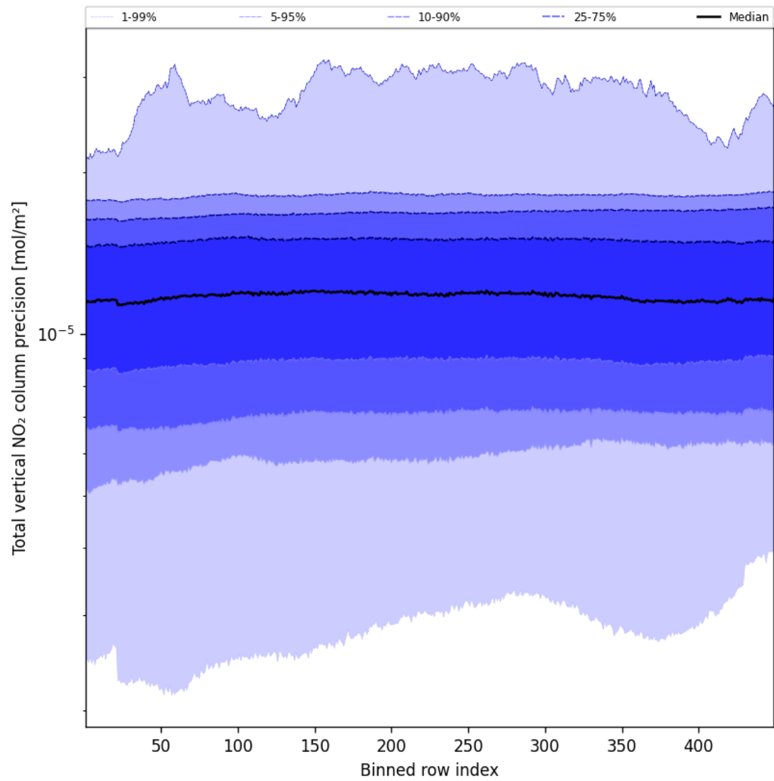
Figure 54: Along track statistics of “Total vertical NO 2 column precision” for 2025-01-24 to 2025-01-25
