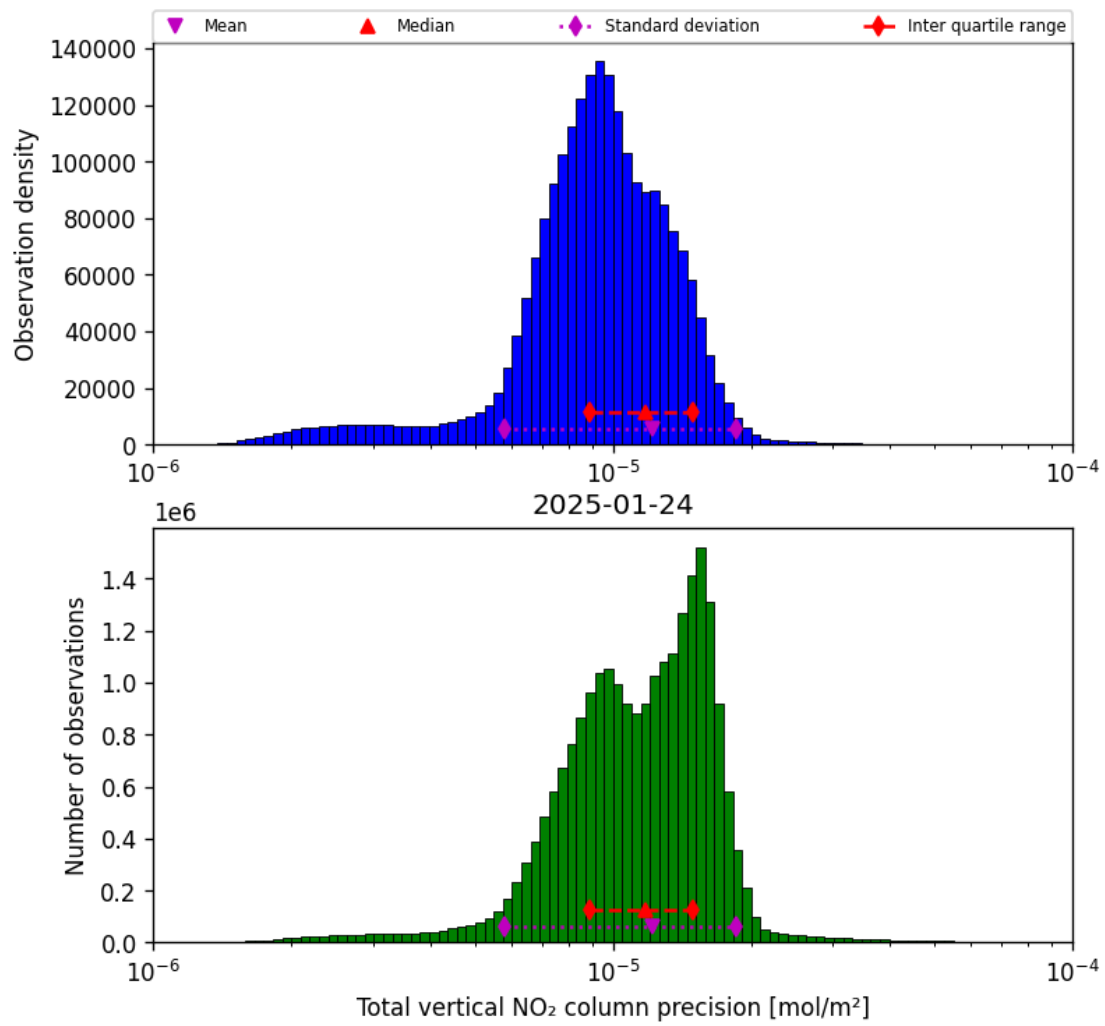
Figure 37: Histogram of “Total vertical NO 2 column precision” for 2025-01-24 to 2025-01-25
