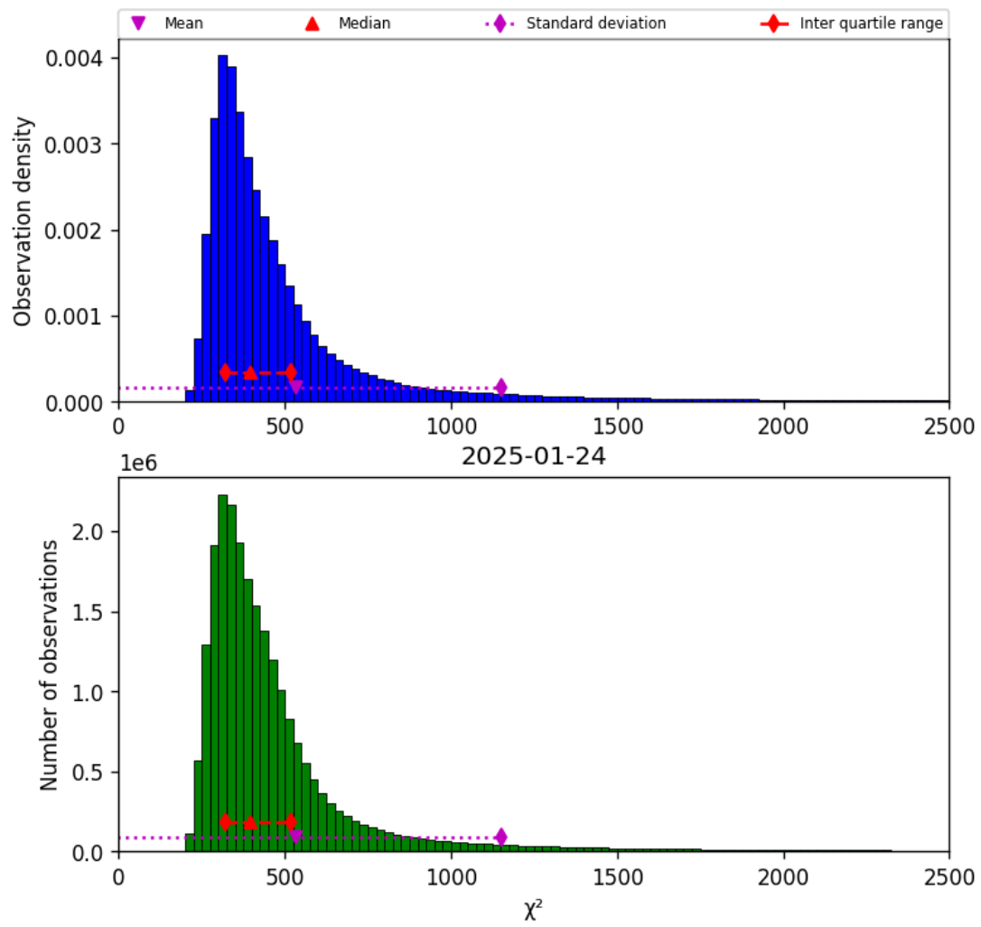
Figure 40: Histogram of “ \chi^2 ” for 2025-01-24 to 2025-01-25
