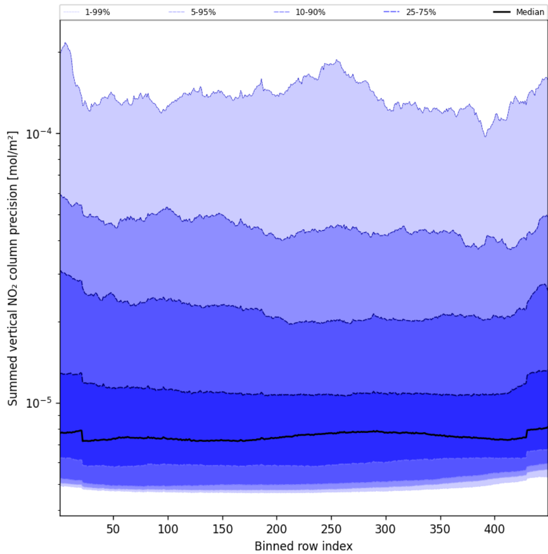
Figure 56: Along track statistics of “Summed vertical NO 2 column precision” for 2025-01-24 to 2025-01-25
