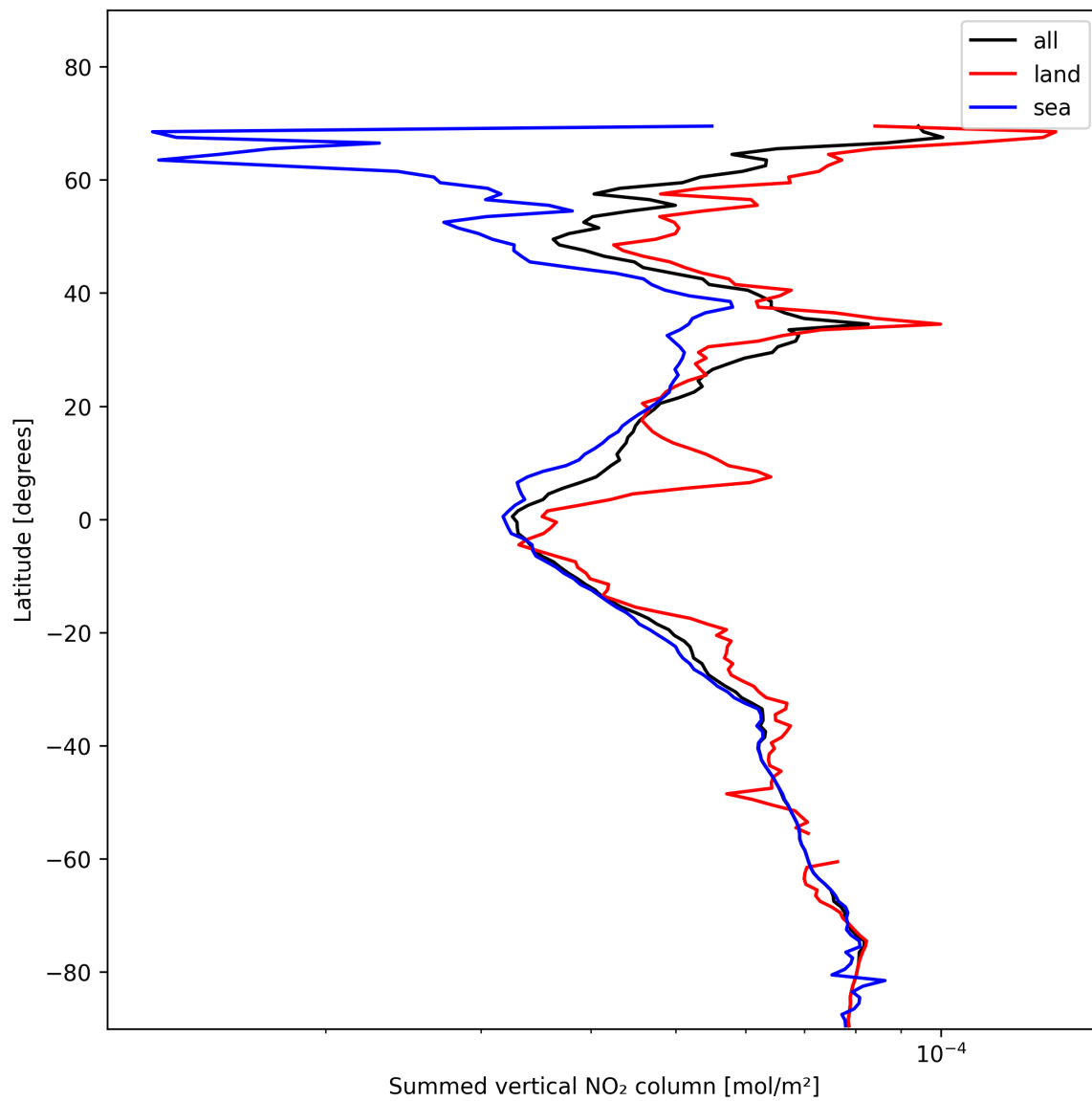
Figure 21: Zonal average of “Summed vertical NO 2 column” for 2025-01-24 to 2025-01-25.
