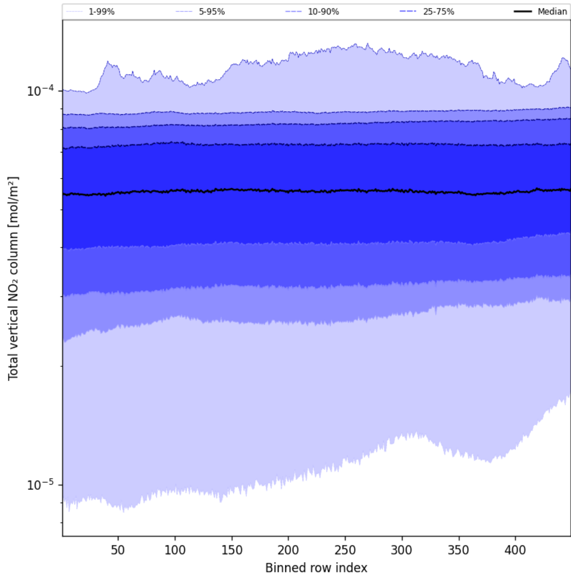
Figure 53: Along track statistics of “Total vertical NO 2 column” for 2025-01-24 to 2025-01-25
