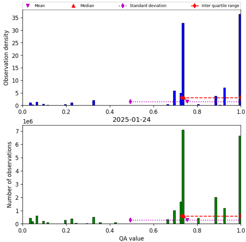
Figure 26: Histogram of “QA value” for 2025-01-24 to 2025-01-25
