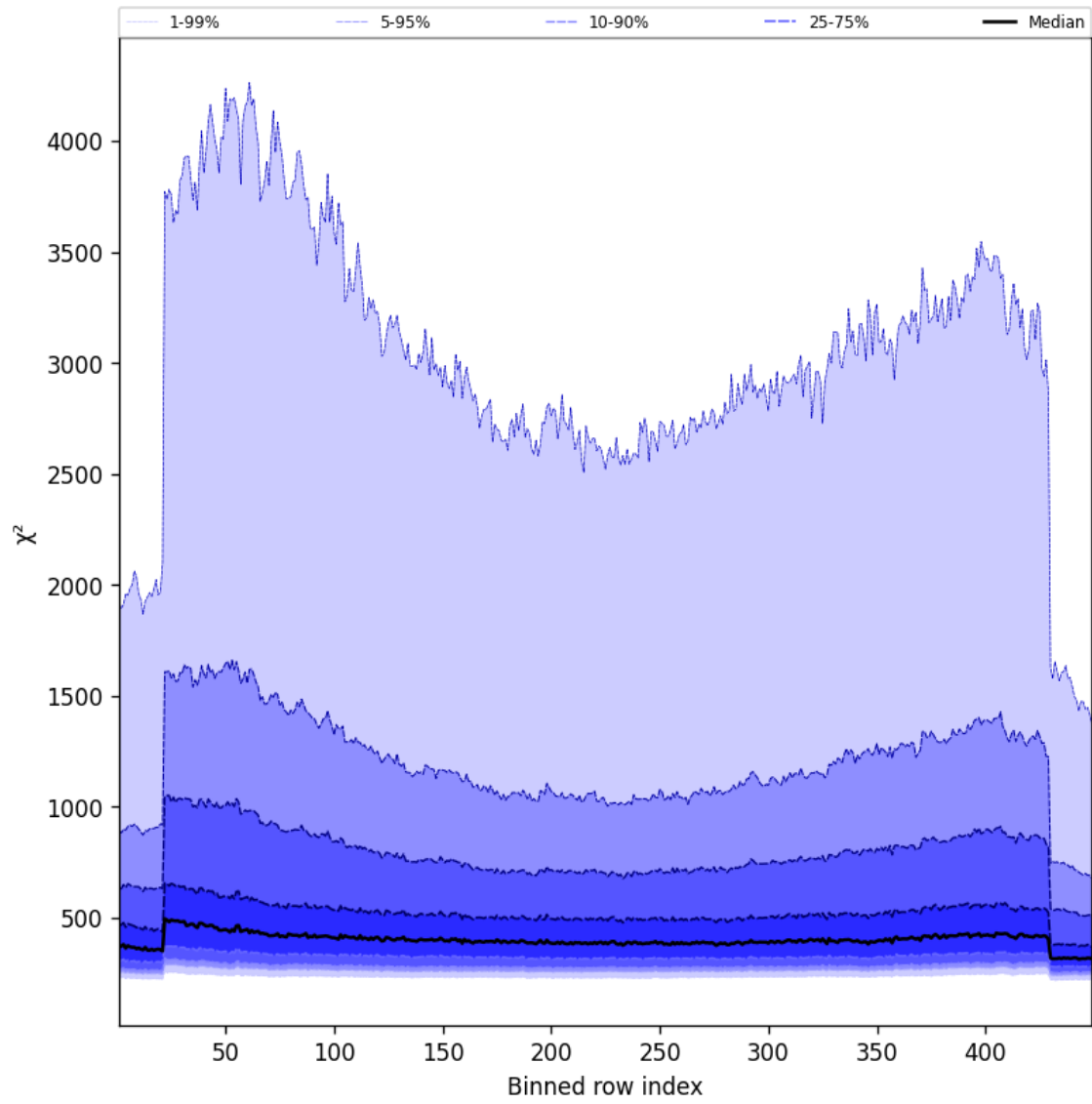
Figure 57: Along track statistics of “ \chi^2 ” for 2025-01-24 to 2025-01-25
