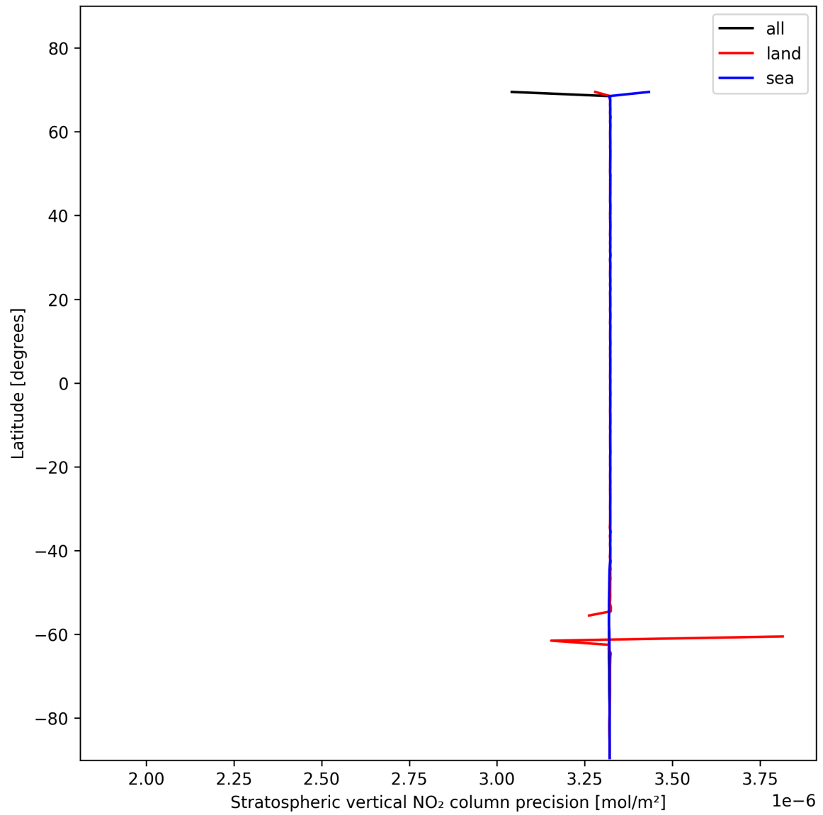
Figure 18: Zonal average of “Stratospheric vertical NO 2 column precision” for 2025-01-24 to 2025-01-25.
