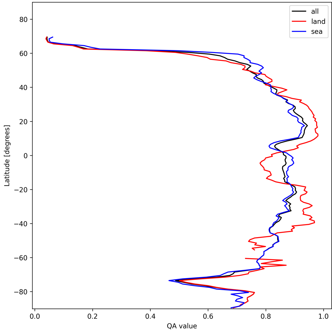
Figure 9: Zonal average of “QA value” for 2025-01-24 to 2025-01-25.
