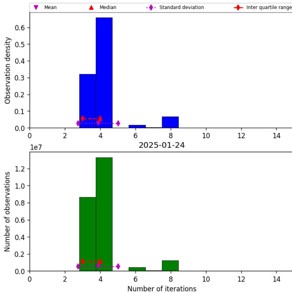
Figure 32: Histogram of “Number of iterations” for 2025-01-24 to 2025-01-25
