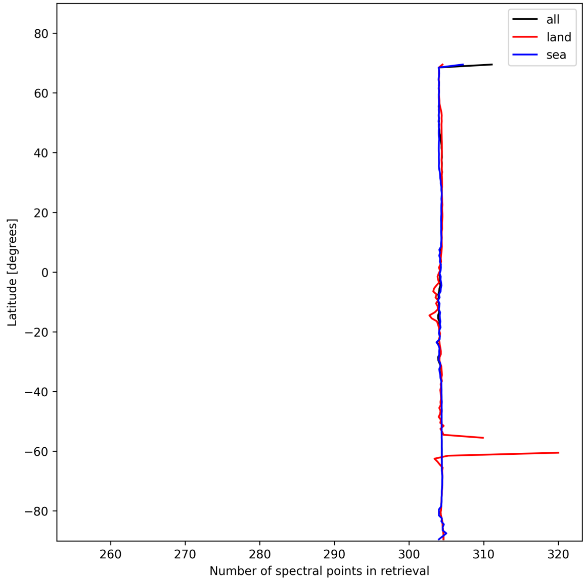
Figure 14: Zonal average of “Number of spectral points in retrieval” for 2025-01-24 to 2025-01-25.
