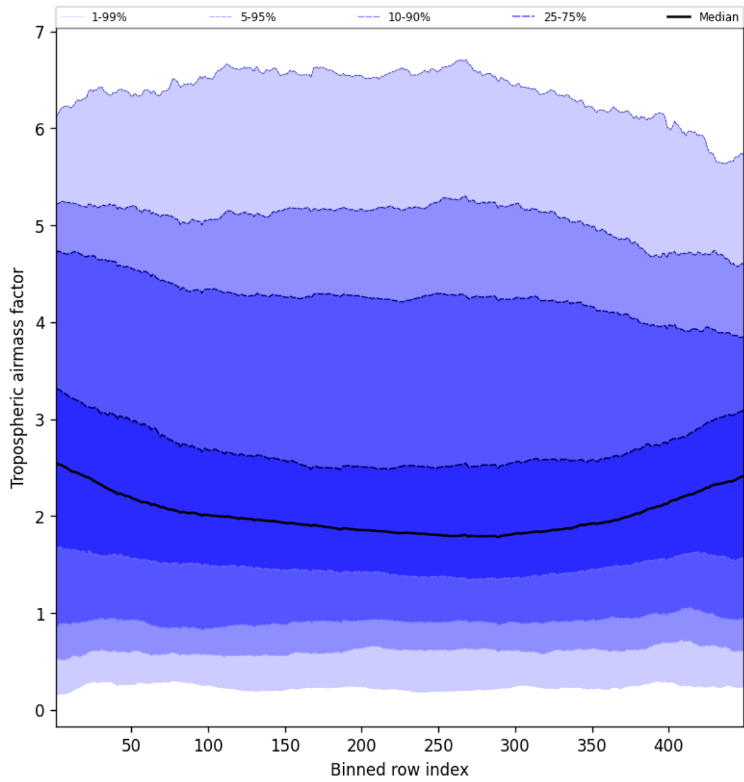
Figure 46: Along track statistics of “Tropospheric airmass factor” for 2025-01-24 to 2025-01-25
