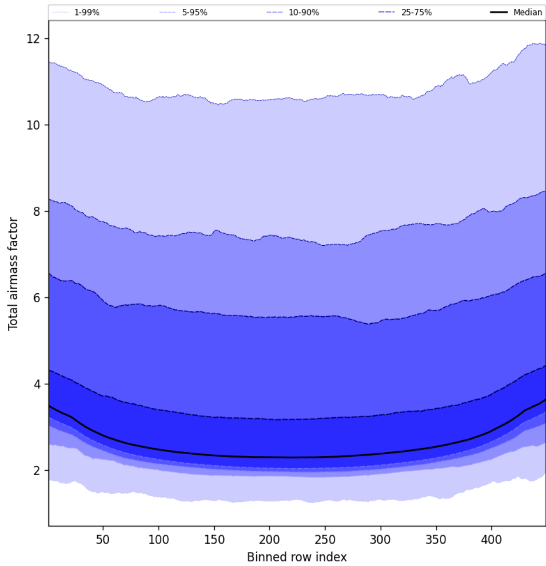
Figure 47: Along track statistics of “Total airmass factor” for 2025-01-24 to 2025-01-25
