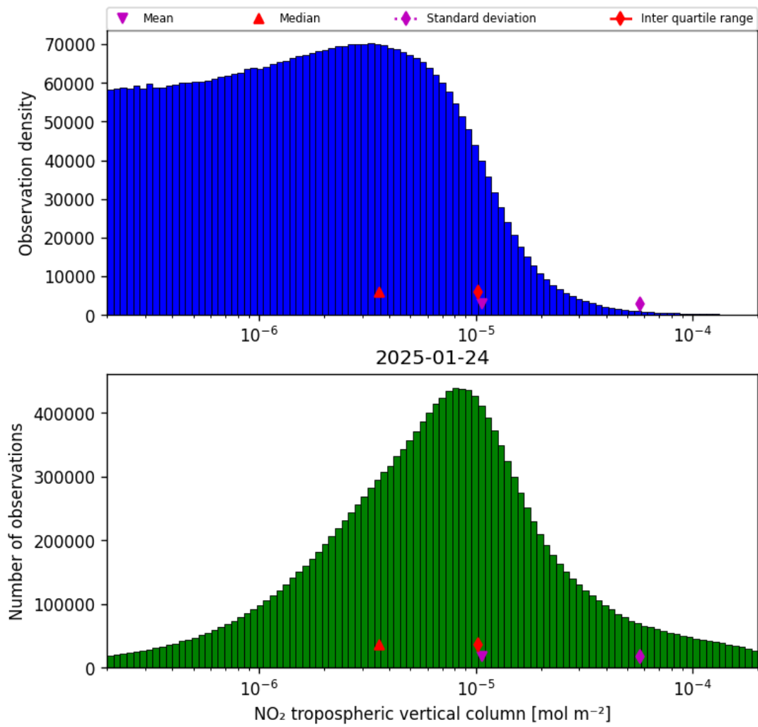
Figure 27: Histogram of “NO 2 tropospheric vertical column” for 2025-01-24 to 2025-01-25
