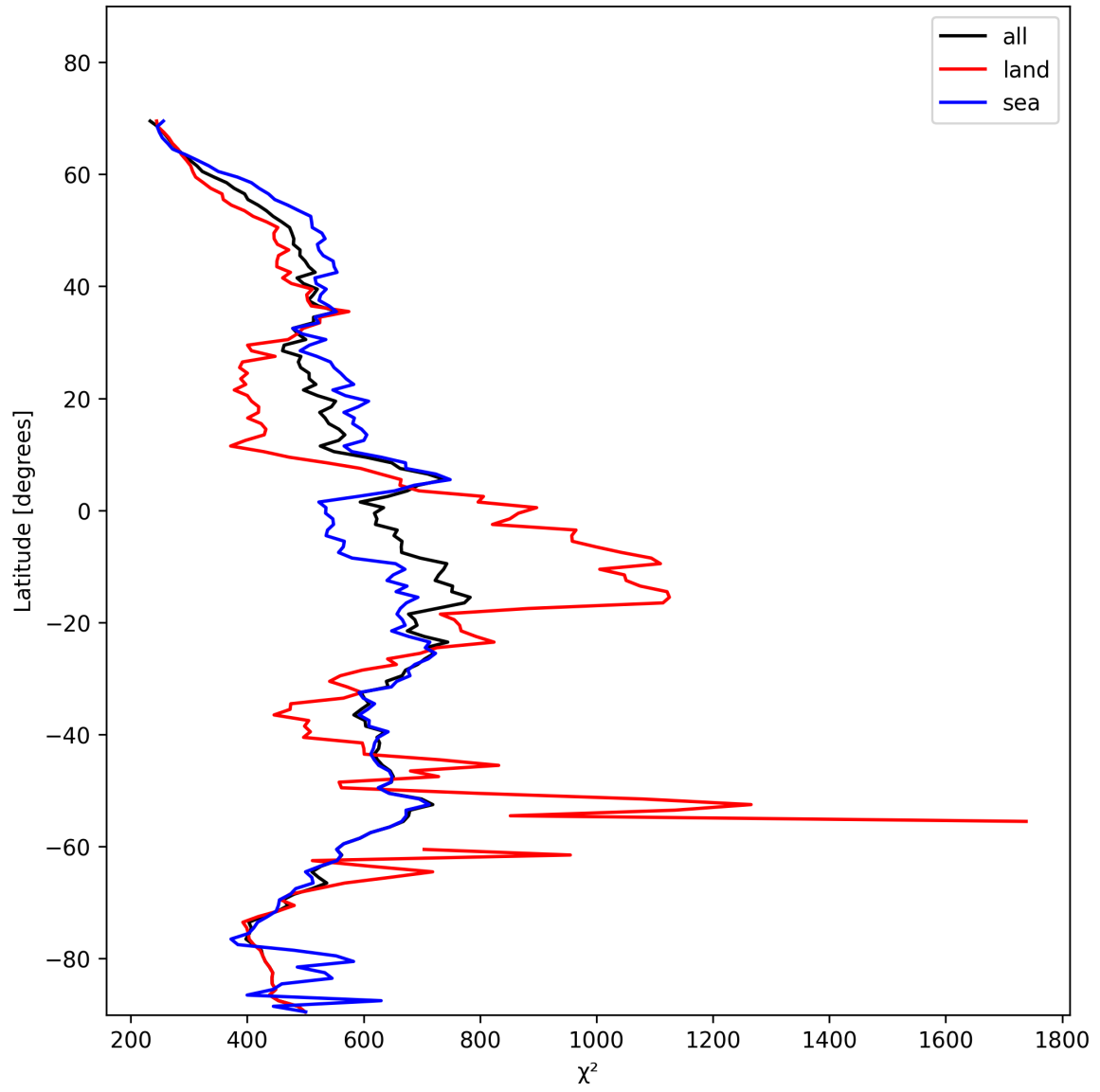
Figure 23: Zonal average of “ \chi^2 ” for 2025-01-24 to 2025-01-25.
