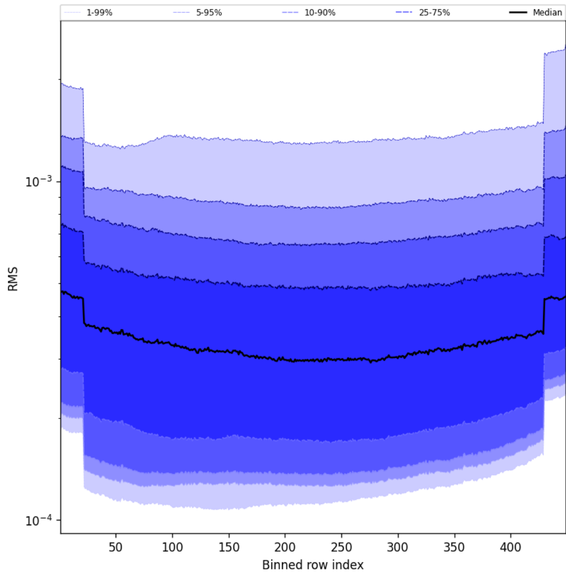
Figure 58: Along track statistics of “RMS” for 2025-01-24 to 2025-01-25
