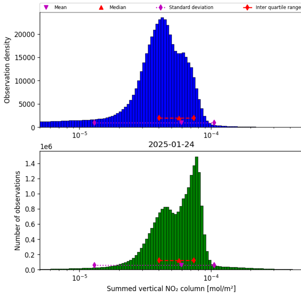
Figure 38: Histogram of “Summed vertical NO 2 column” for 2025-01-24 to 2025-01-25
