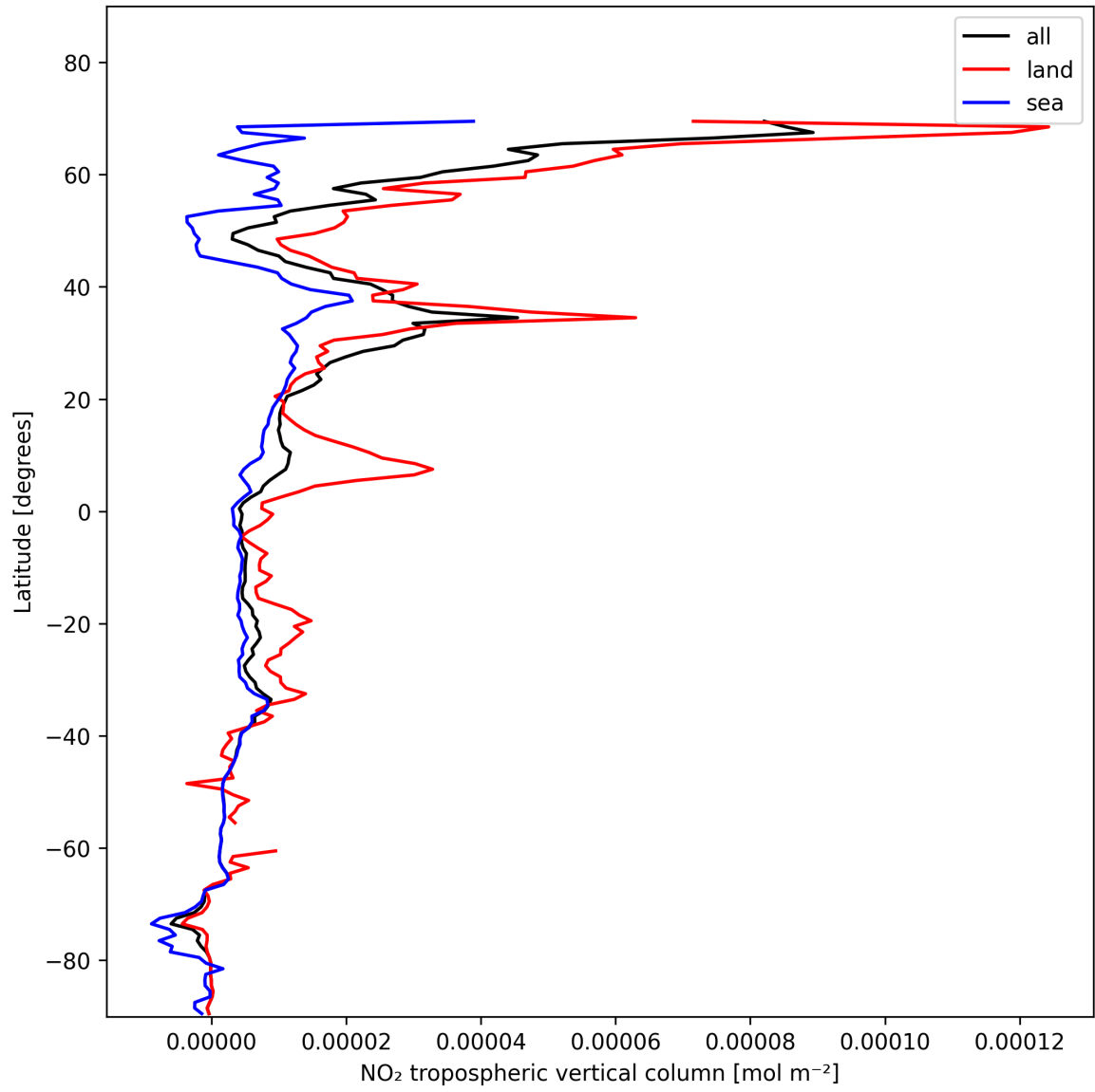
Figure 10: Zonal average of “NO 2 tropospheric vertical column” for 2025-01-24 to 2025-01-25.
