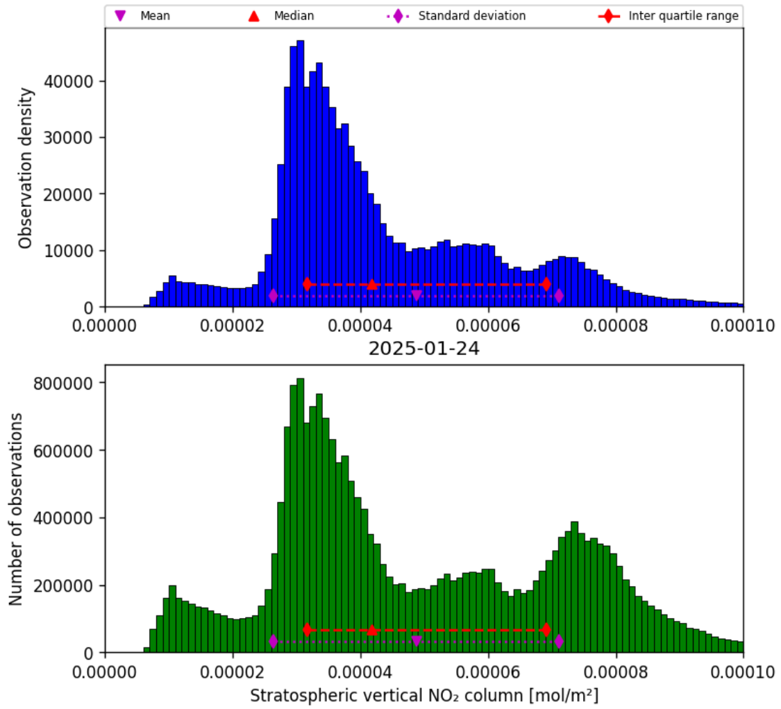
Figure 34: Histogram of “Stratospheric vertical NO 2 column” for 2025-01-24 to 2025-01-25
