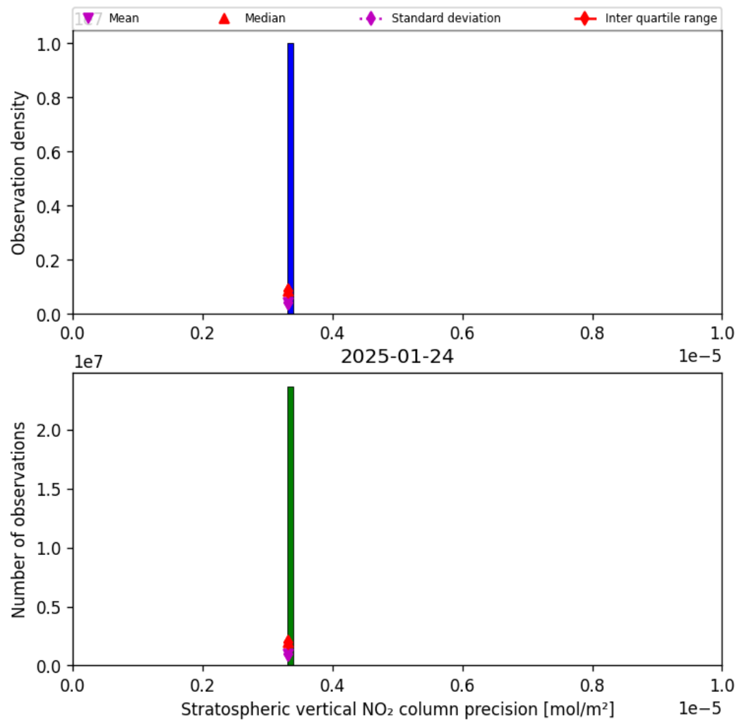
Figure 35: Histogram of “Stratospheric vertical NO 2 column precision” for 2025-01-24 to 2025-01-25
