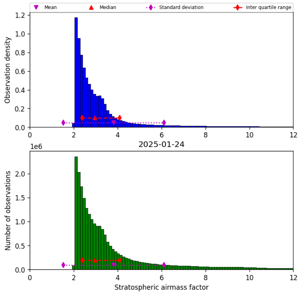
Figure 42: Histogram of “Stratospheric airmass factor” for 2025-01-24 to 2025-01-25
