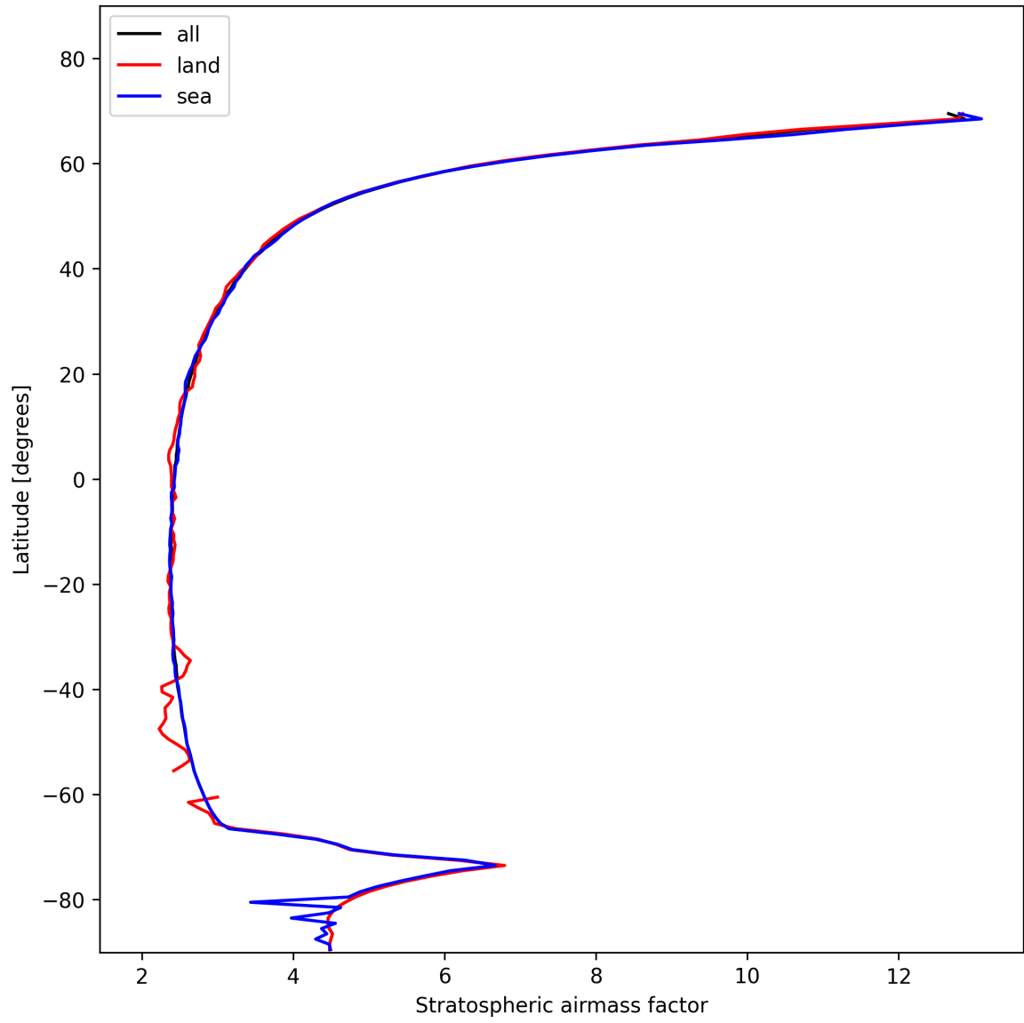
Figure 25: Zonal average of “Stratospheric airmass factor” for 2025-01-24 to 2025-01-25.
