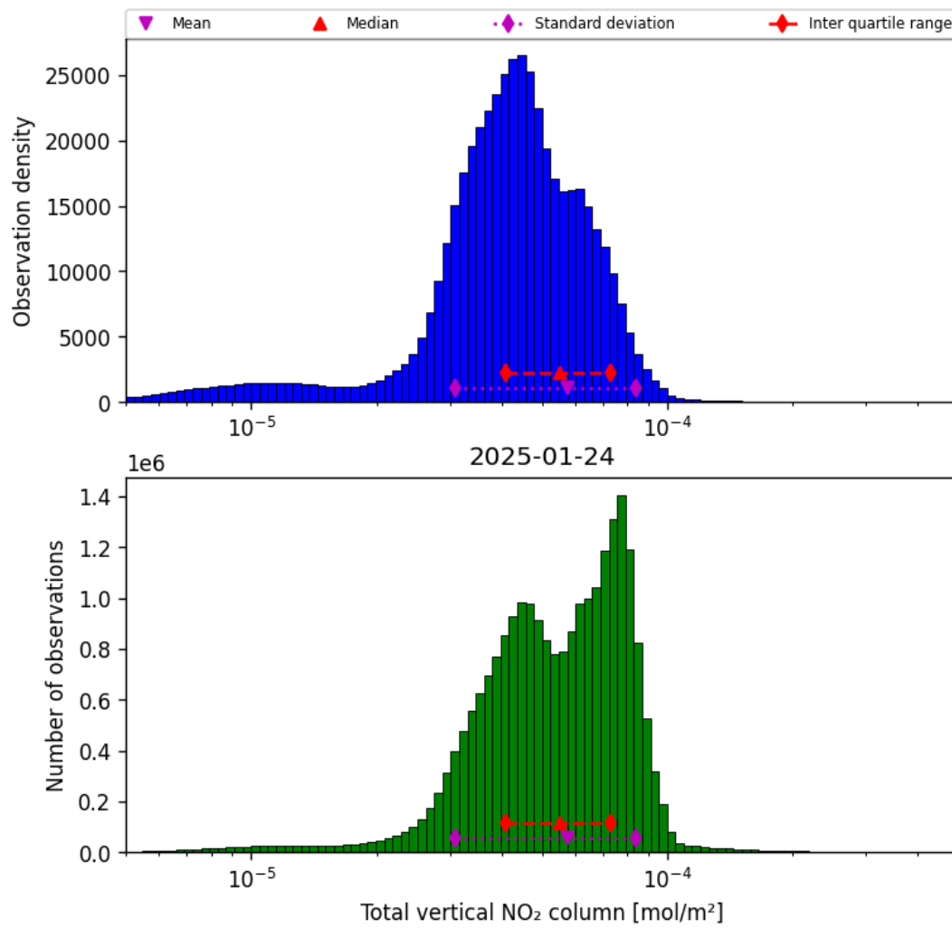
Figure 36: Histogram of “Total vertical NO 2 column” for 2025-01-24 to 2025-01-25
