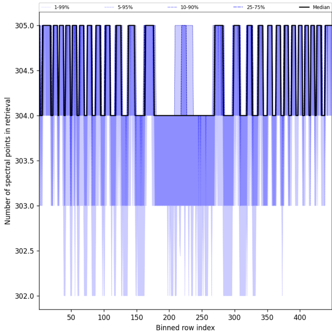
Figure 48: Along track statistics of “Number of spectral points in retrieval” for 2025-01-24 to 2025-01-25
