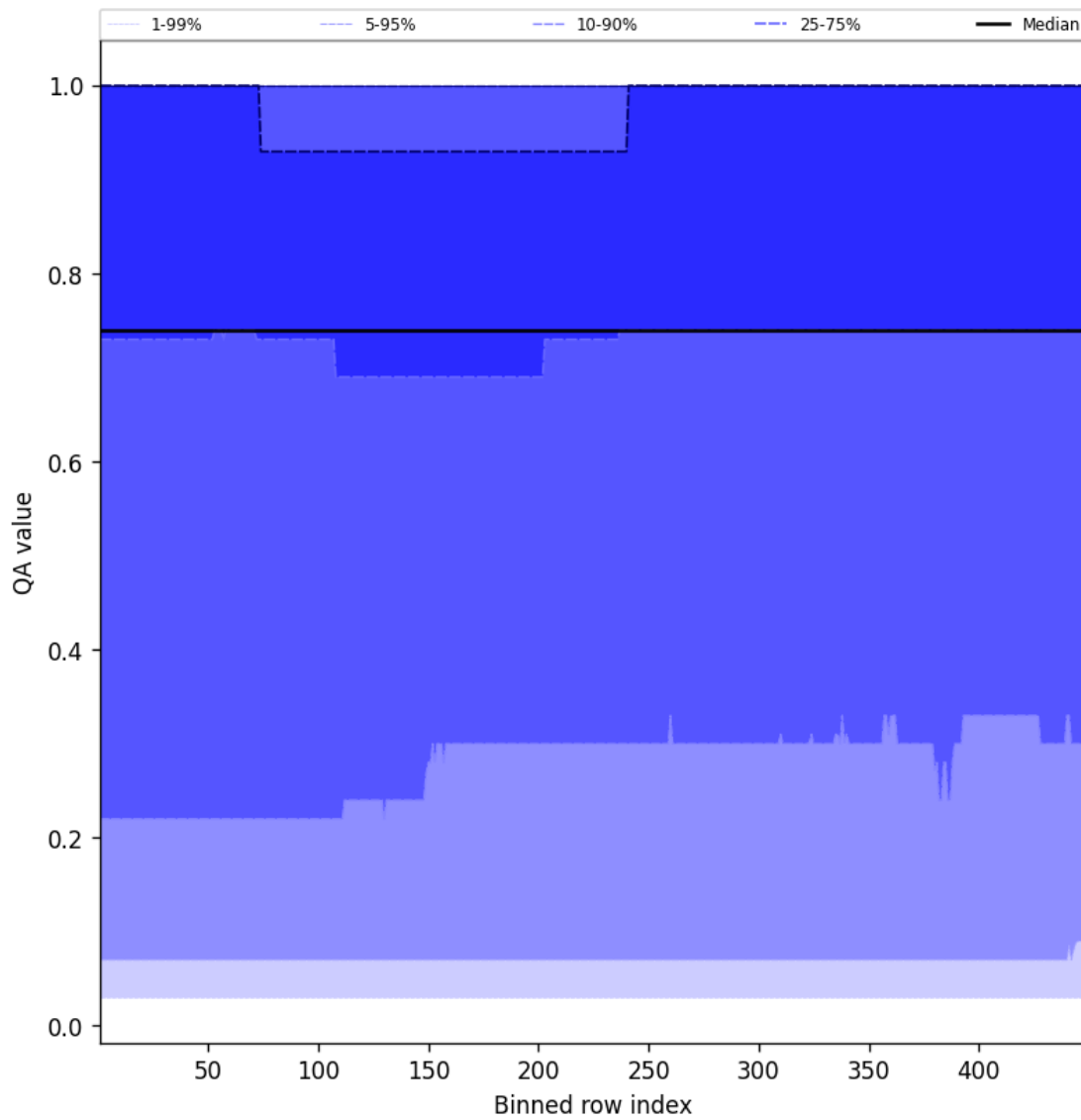
Figure 43: Along track statistics of “QA value” for 2025-01-24 to 2025-01-25
