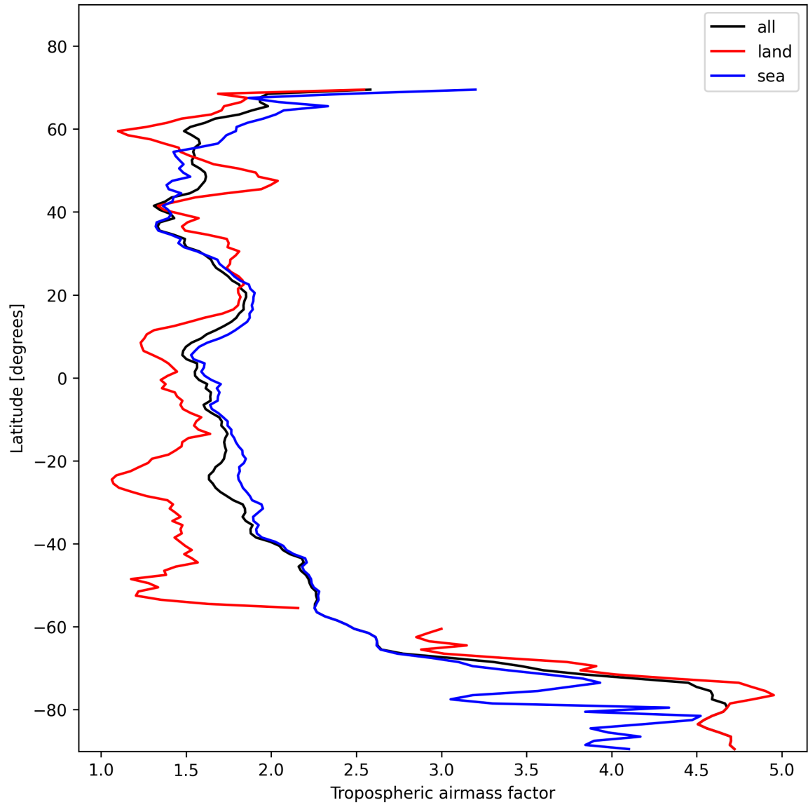
Figure 12: Zonal average of “Tropospheric airmass factor” for 2025-01-24 to 2025-01-25.
