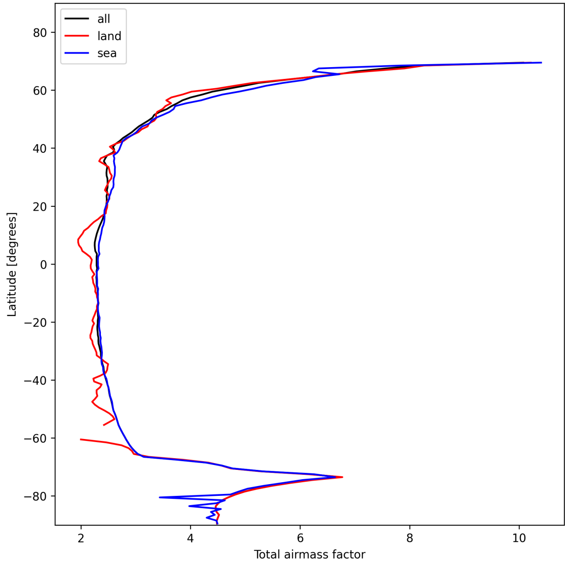
Figure 13: Zonal average of “Total airmass factor” for 2025-01-24 to 2025-01-25.
