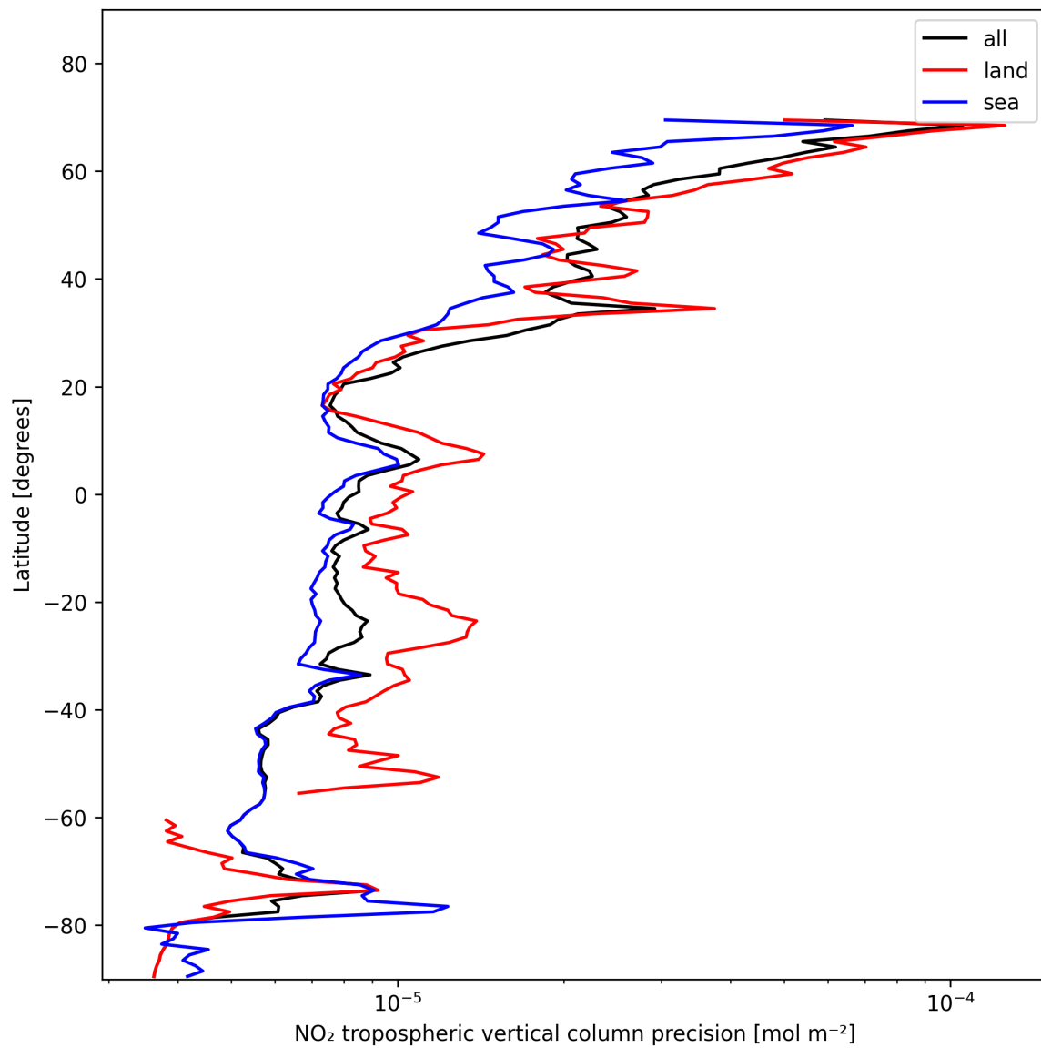
Figure 11: Zonal average of “NO 2 tropospheric vertical column precision” for 2025-01-24 to 2025-01-25.
