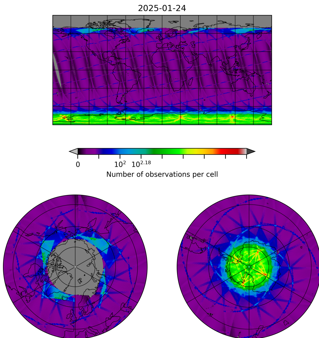
Figure 8: Map of the number of observations for 2025-01-24 to 2025-01-25
