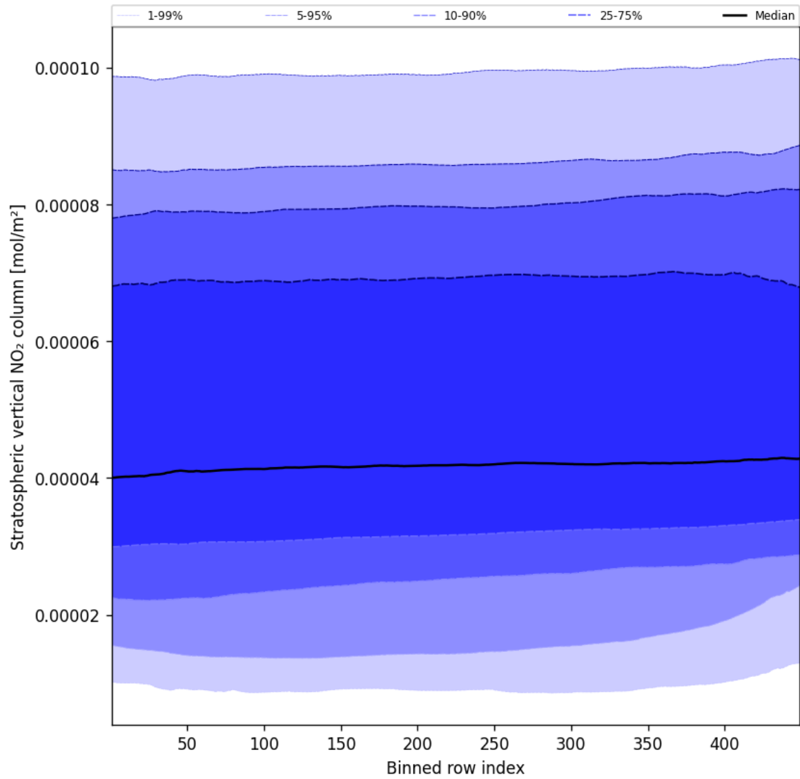
Figure 51: Along track statistics of “Stratospheric vertical NO 2 column” for 2025-01-24 to 2025-01-25
