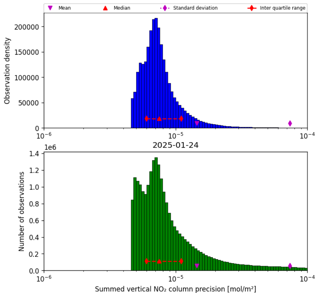
Figure 39: Histogram of “Summed vertical NO 2 column precision” for 2025-01-24 to 2025-01-25
