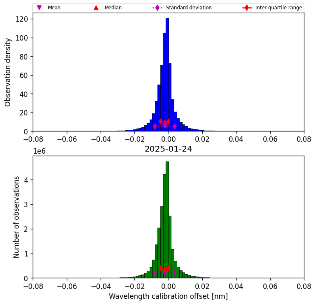
Figure 33: Histogram of “Wavelength calibration offset” for 2025-01-24 to 2025-01-25
