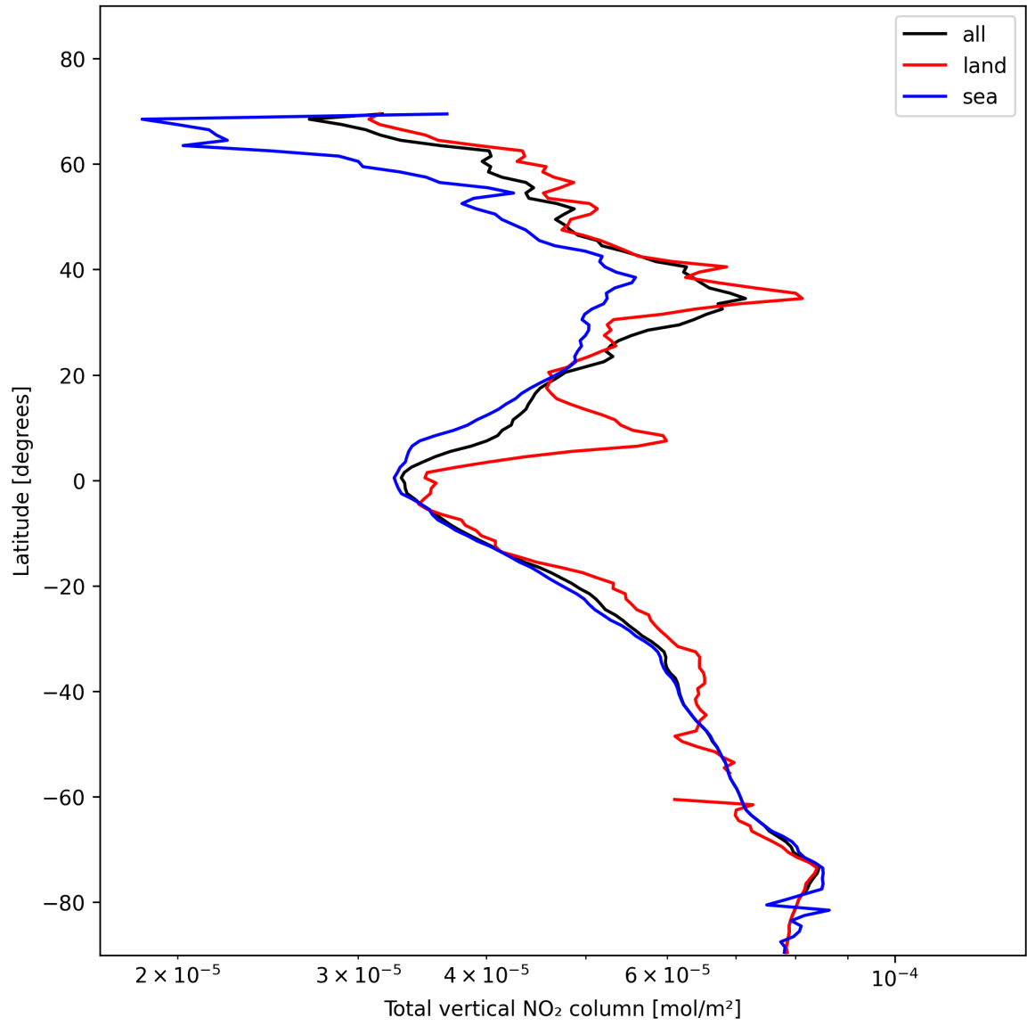
Figure 19: Zonal average of “Total vertical NO 2 column” for 2025-01-24 to 2025-01-25.
