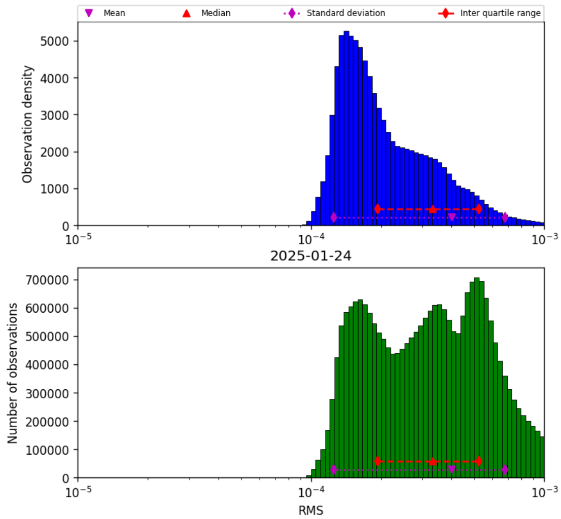
Figure 41: Histogram of “RMS” for 2025-01-24 to 2025-01-25
