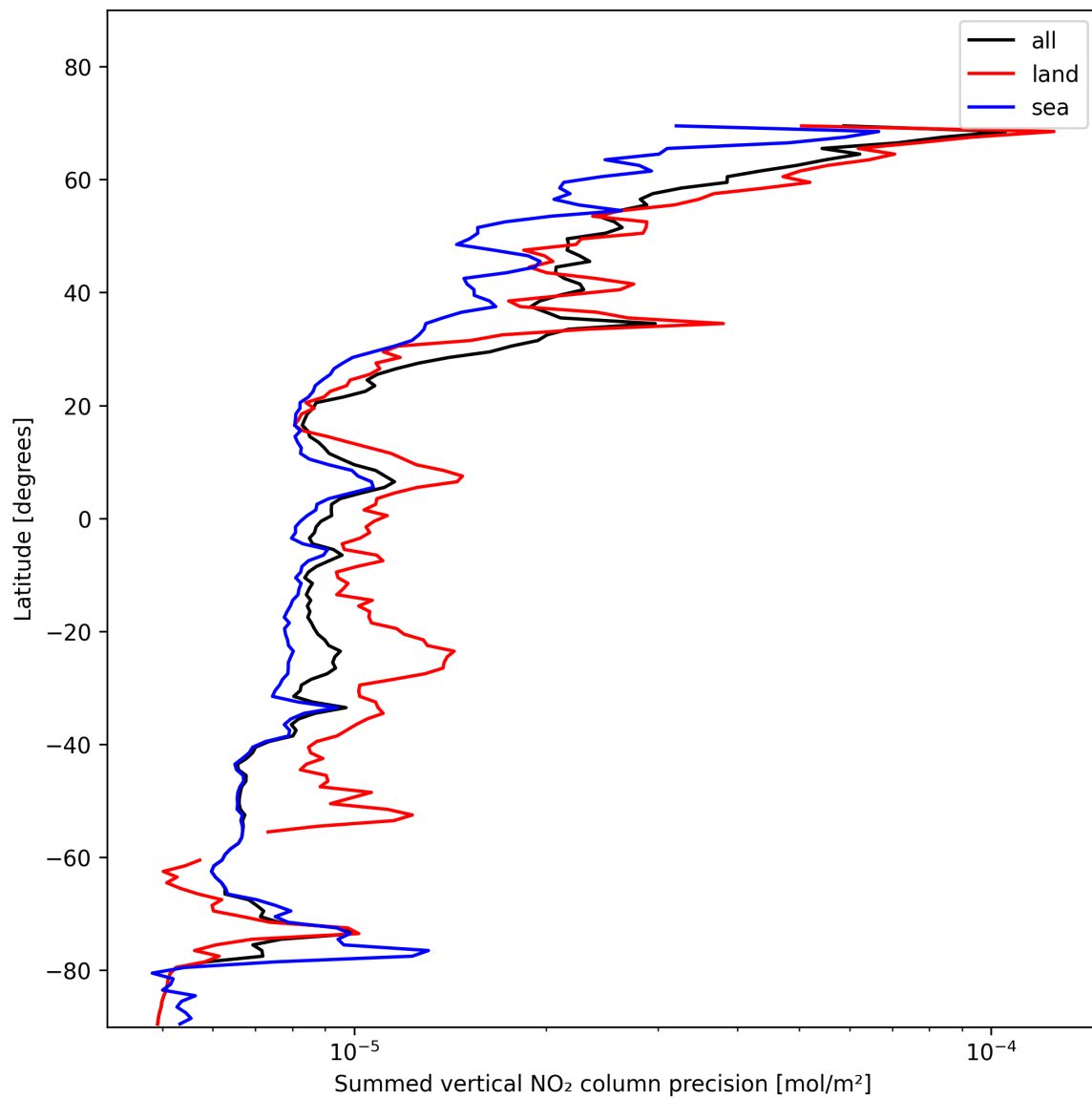
Figure 22: Zonal average of “Summed vertical NO 2 column precision” for 2025-01-24 to 2025-01-25.
