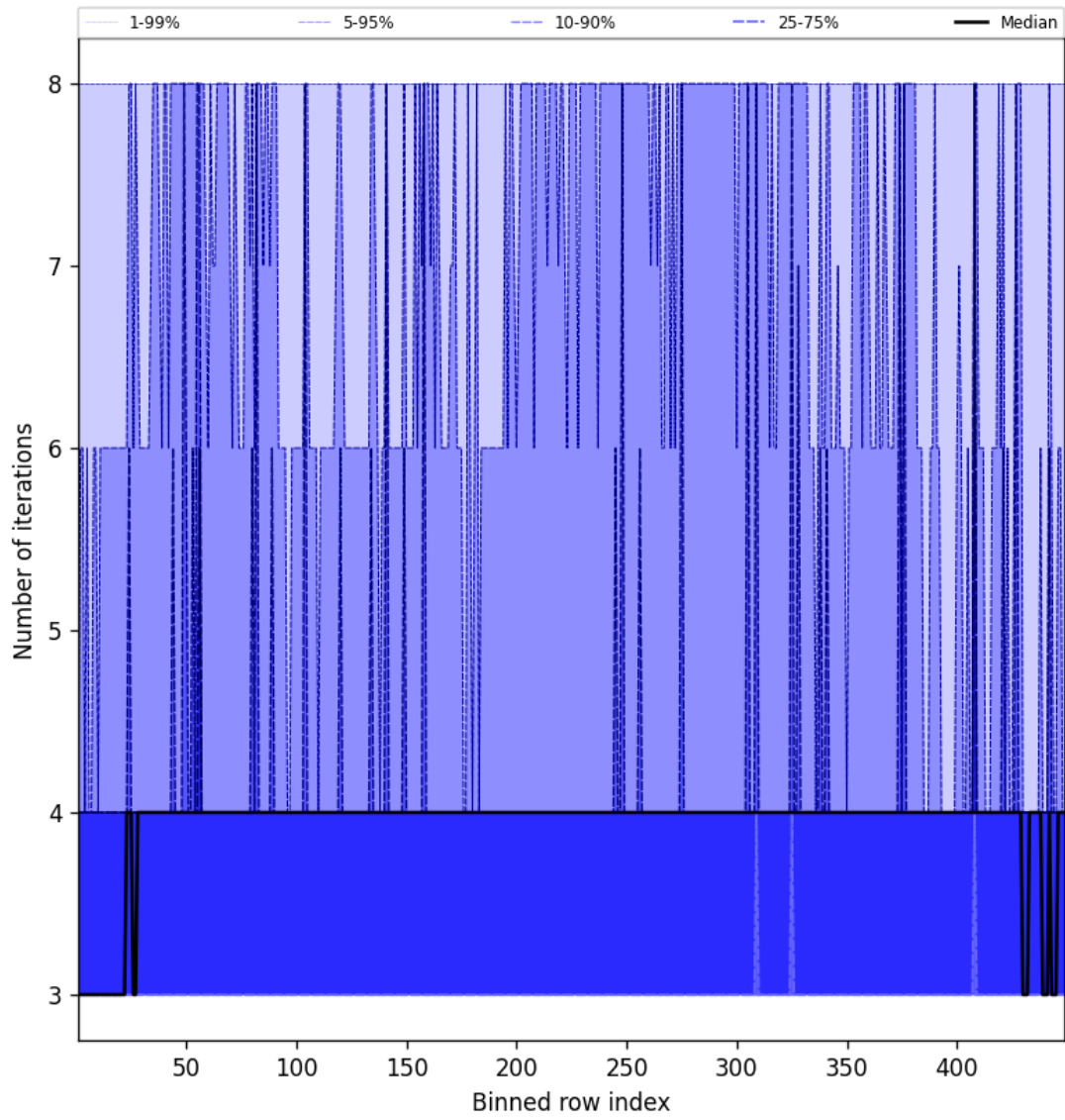
Figure 49: Along track statistics of “Number of iterations” for 2025-01-24 to 2025-01-25
