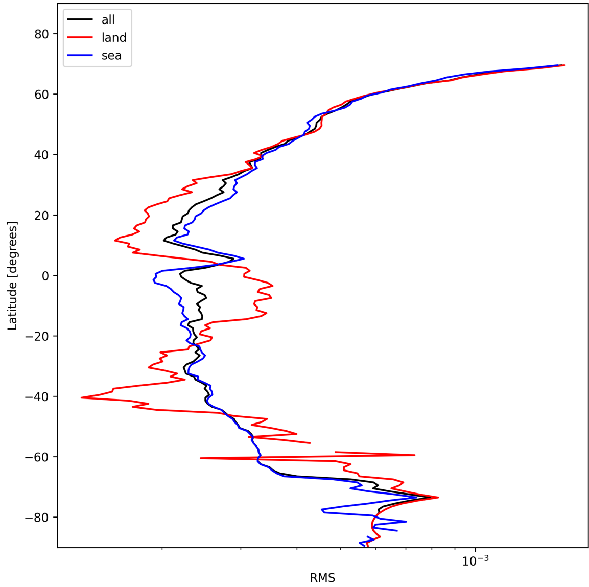
Figure 24: Zonal average of “RMS” for 2025-01-25 to 2025-01-26.
