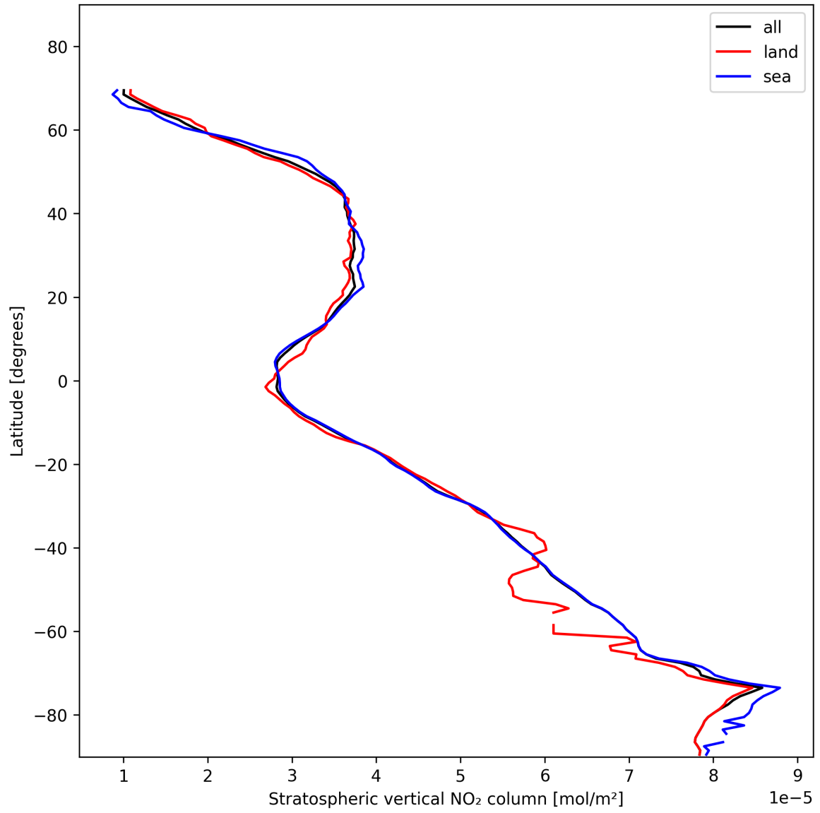
Figure 17: Zonal average of “Stratospheric vertical NO 2 column” for 2025-01-25 to 2025-01-26.
