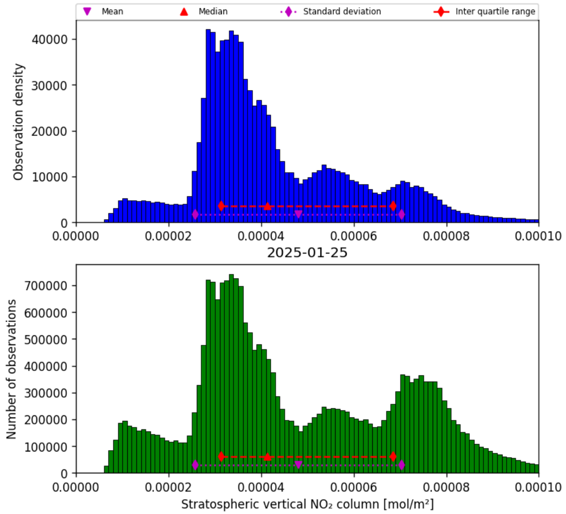
Figure 34: Histogram of “Stratospheric vertical NO 2 column” for 2025-01-25 to 2025-01-26
