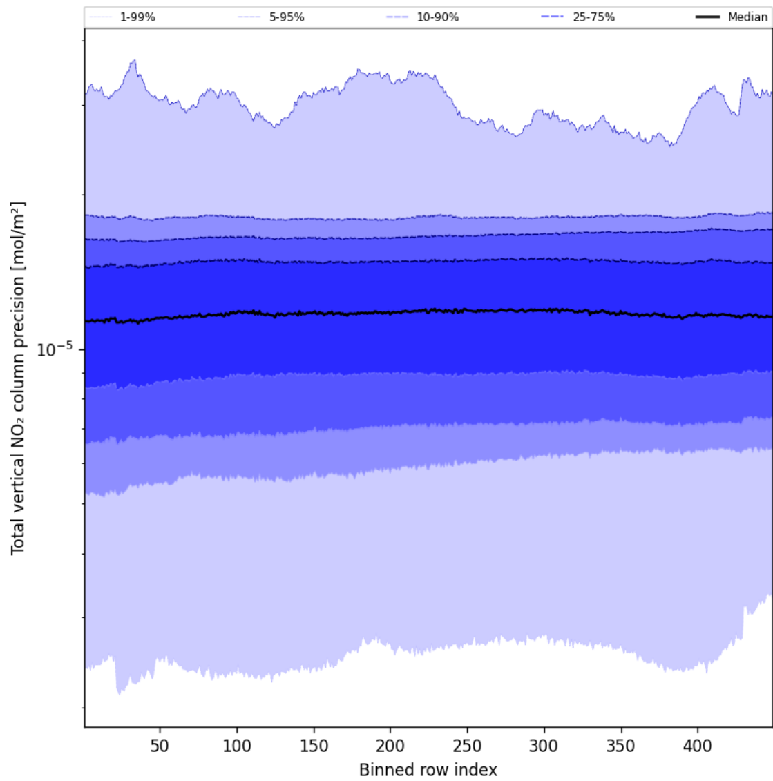
Figure 54: Along track statistics of “Total vertical NO 2 column precision” for 2025-01-25 to 2025-01-26
