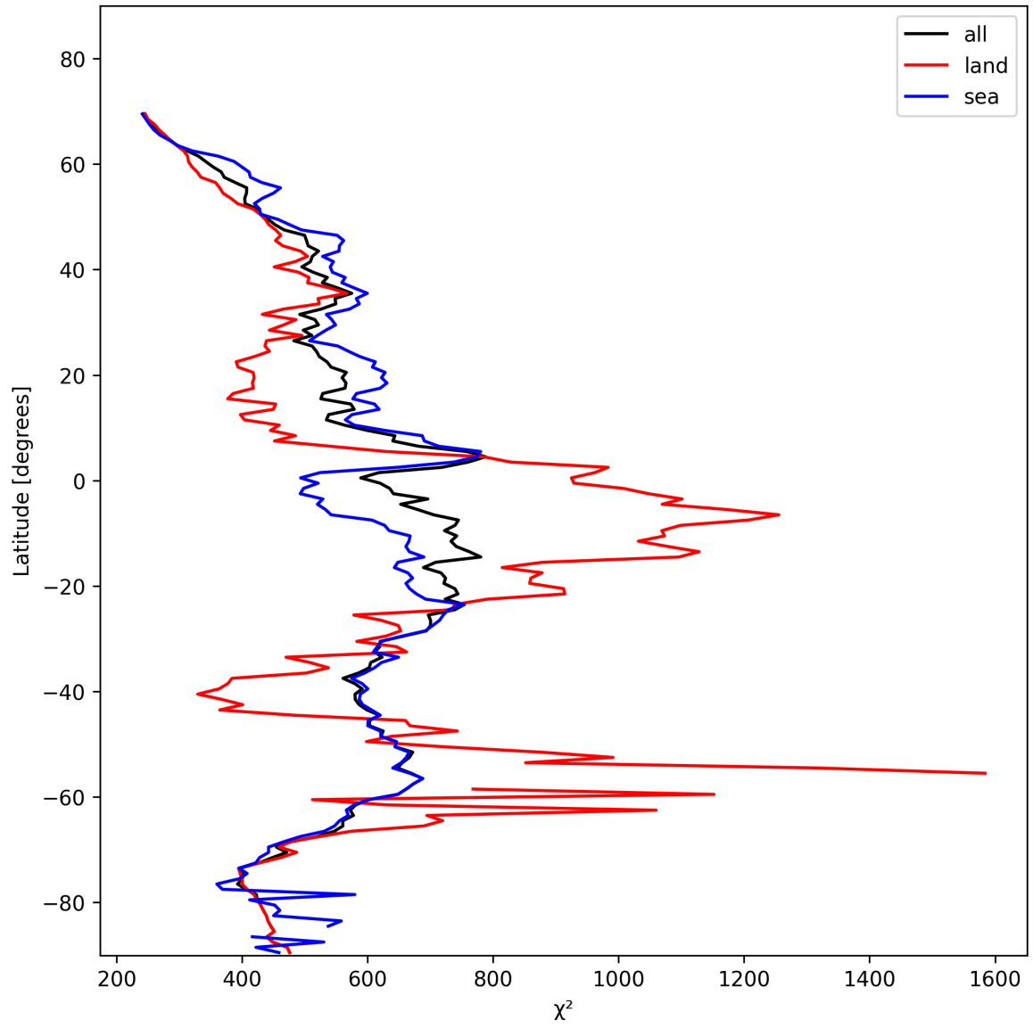
Figure 23: Zonal average of “ \chi^2 ” for 2025-01-25 to 2025-01-26.
