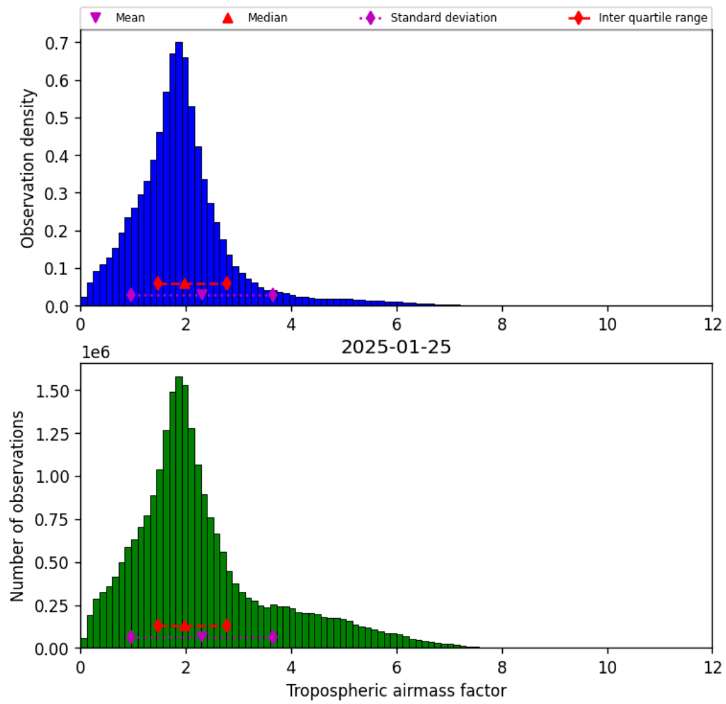
Figure 29: Histogram of “Tropospheric airmass factor” for 2025-01-25 to 2025-01-26
