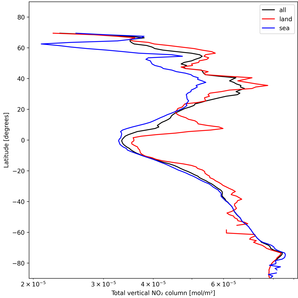
Figure 19: Zonal average of “Total vertical NO 2 column” for 2025-01-25 to 2025-01-26.
