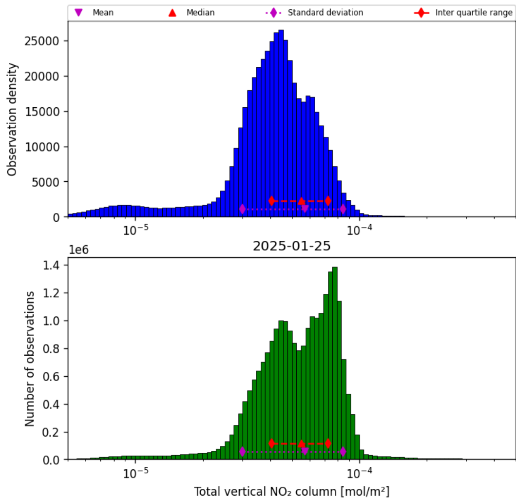
Figure 36: Histogram of “Total vertical NO 2 column” for 2025-01-25 to 2025-01-26
