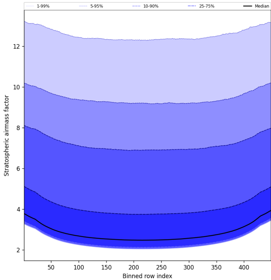
Figure 59: Along track statistics of “Stratospheric airmass factor” for 2025-01-25 to 2025-01-26
