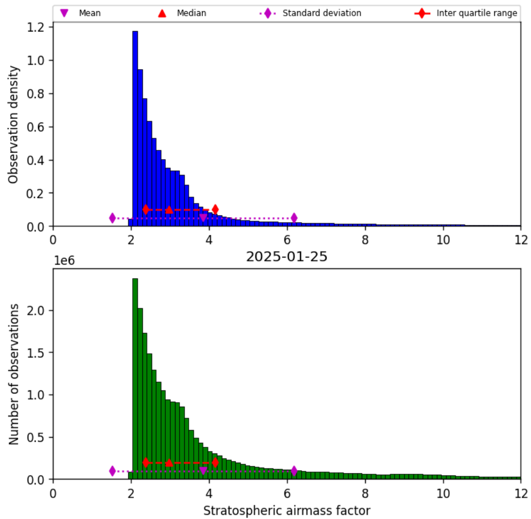
Figure 42: Histogram of “Stratospheric airmass factor” for 2025-01-25 to 2025-01-26
