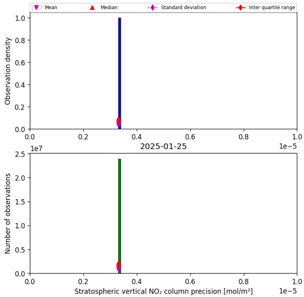
Figure 35: Histogram of “Stratospheric vertical NO 2 column precision” for 2025-01-25 to 2025-01-26
