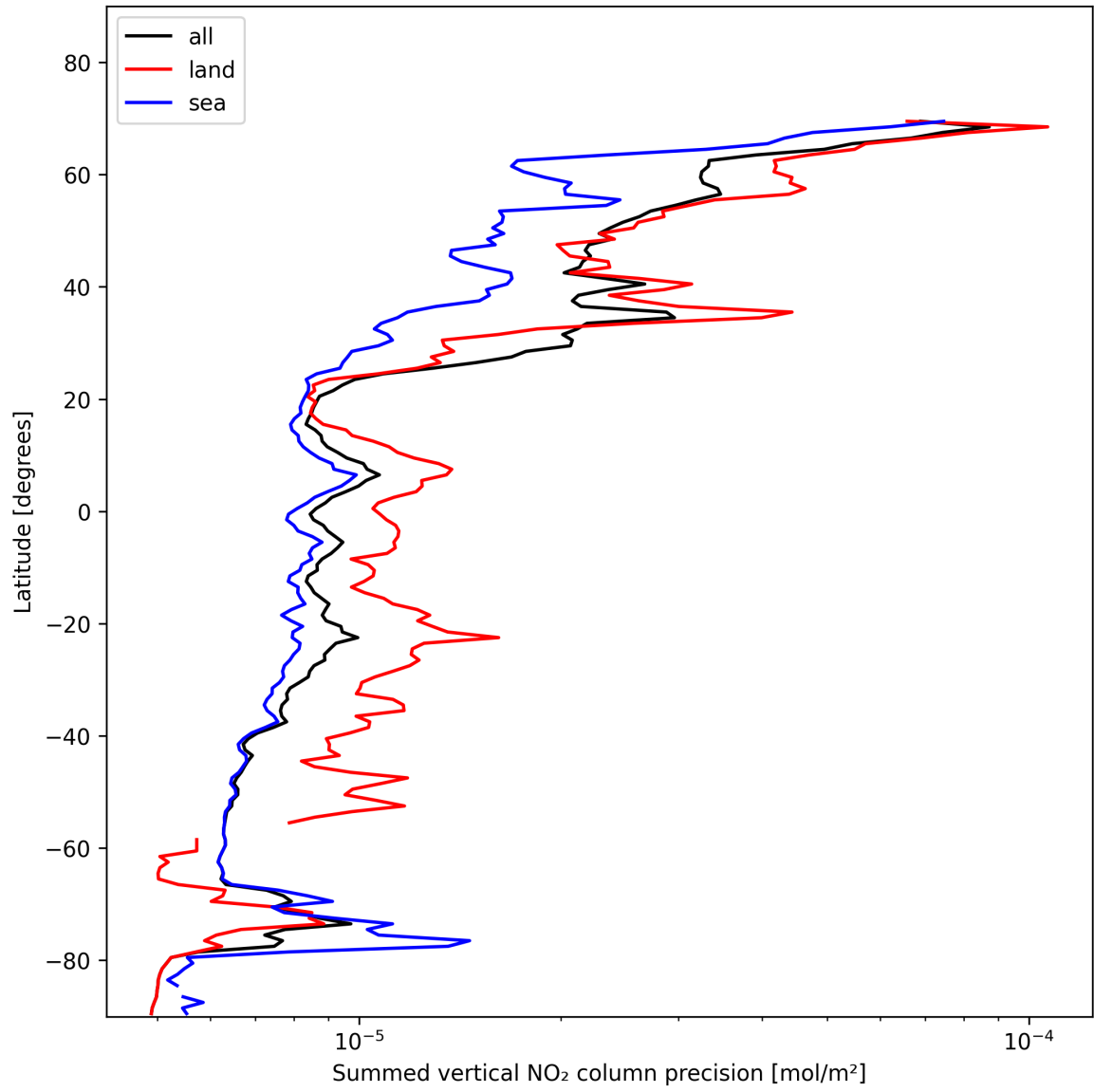
Figure 22: Zonal average of “Summed vertical NO 2 column precision” for 2025-01-25 to 2025-01-26.
