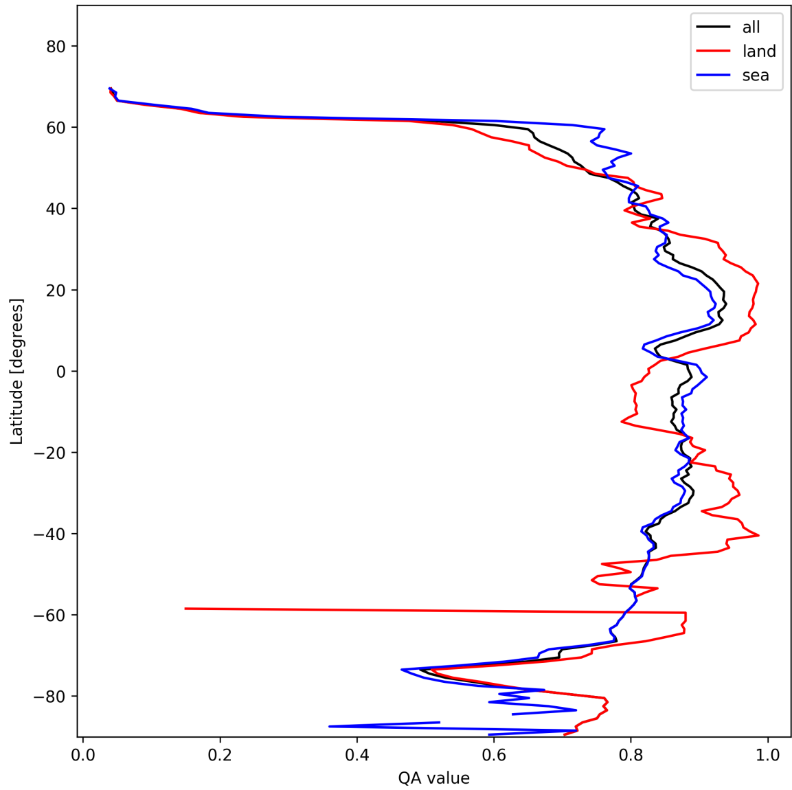
Figure 9: Zonal average of “QA value” for 2025-01-25 to 2025-01-26.
