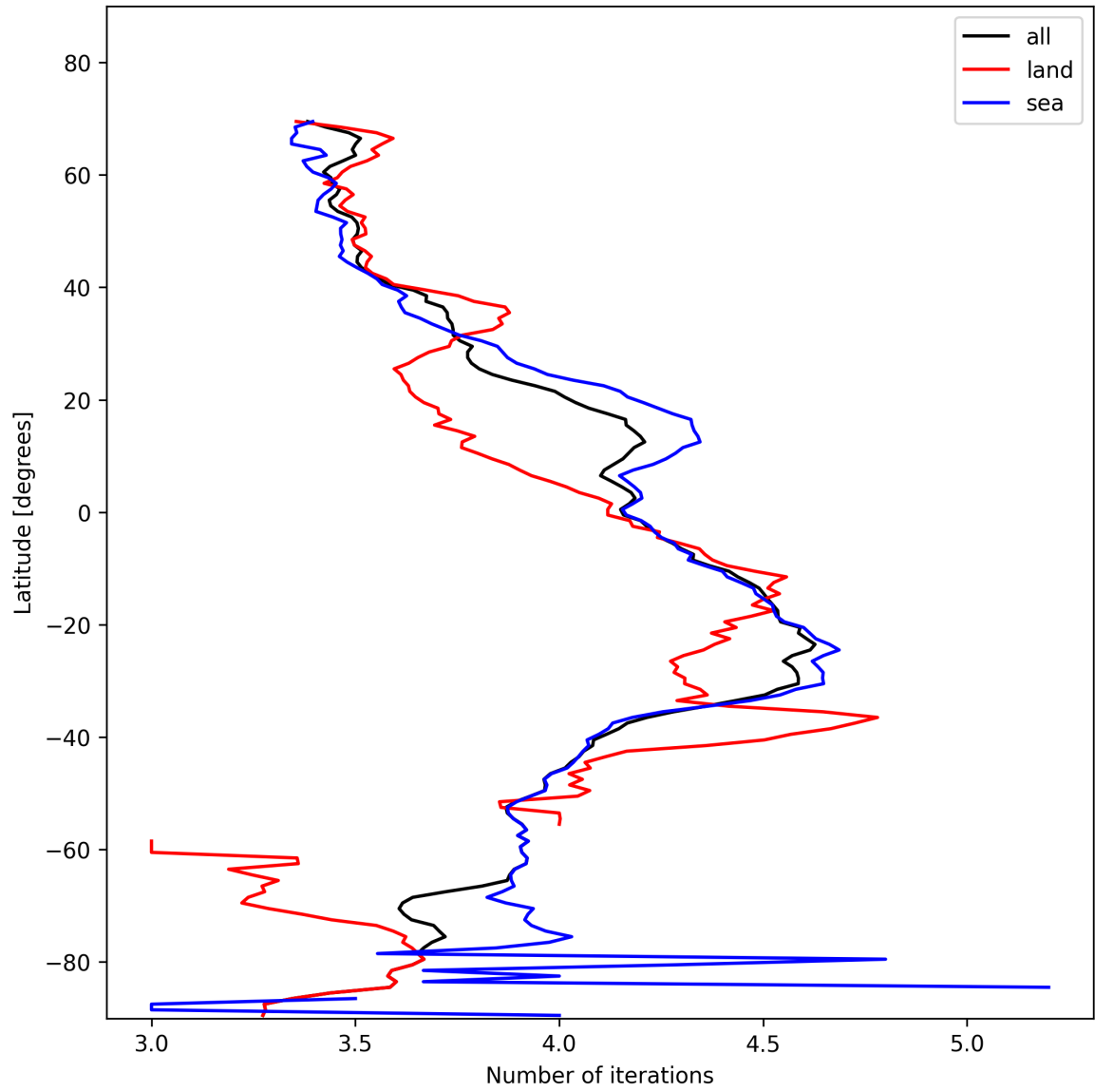
Figure 15: Zonal average of “Number of iterations” for 2025-01-25 to 2025-01-26.
