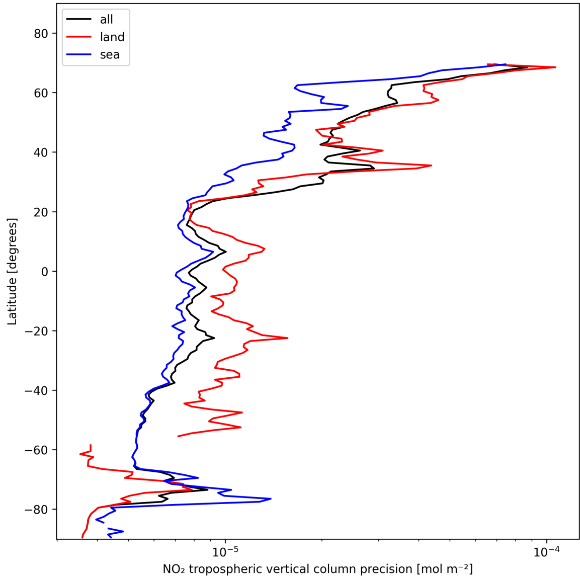
Figure 11: Zonal average of “NO 2 tropospheric vertical column precision” for 2025-01-25 to 2025-01-26.
