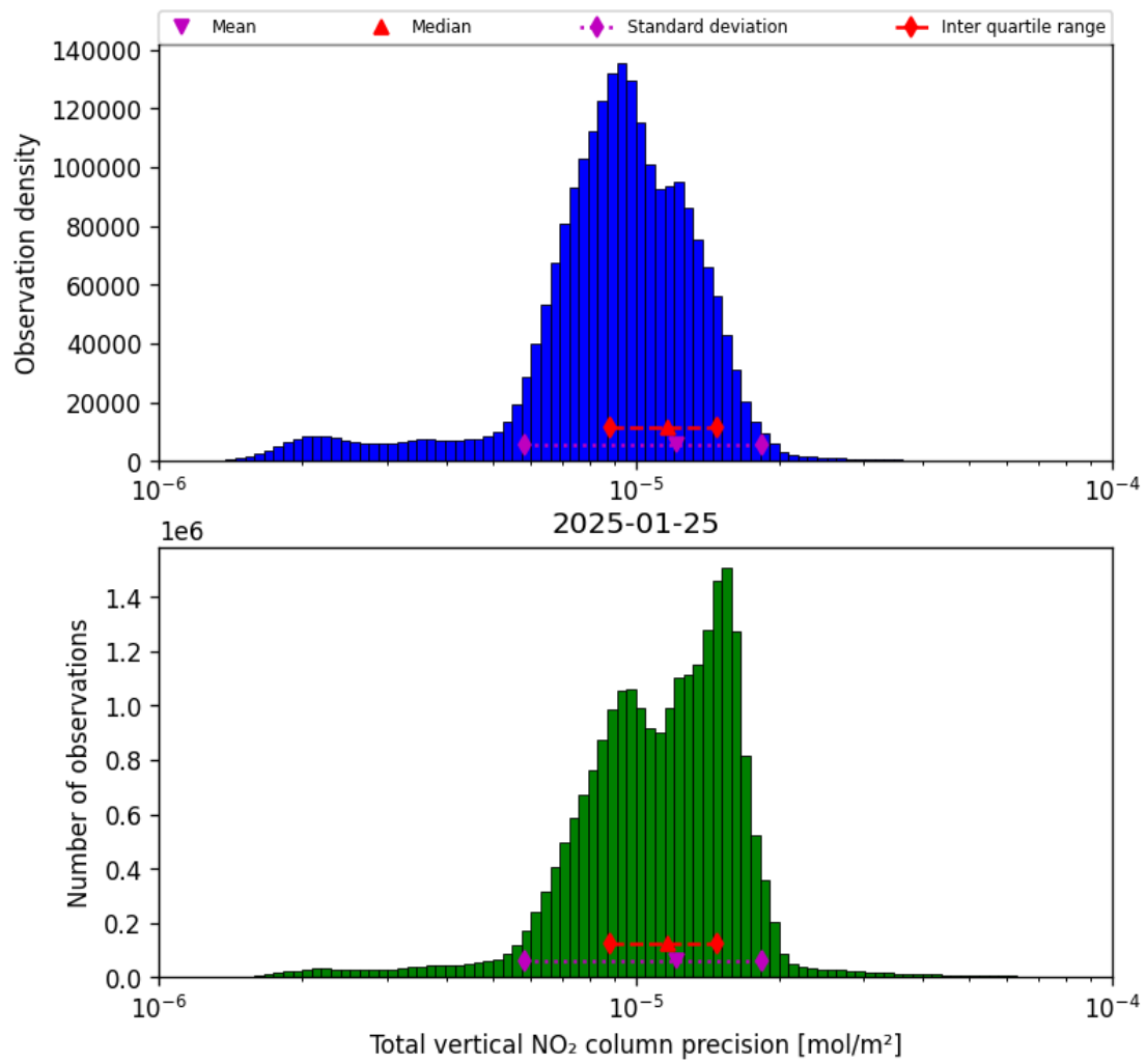
Figure 37: Histogram of “Total vertical NO 2 column precision” for 2025-01-25 to 2025-01-26
