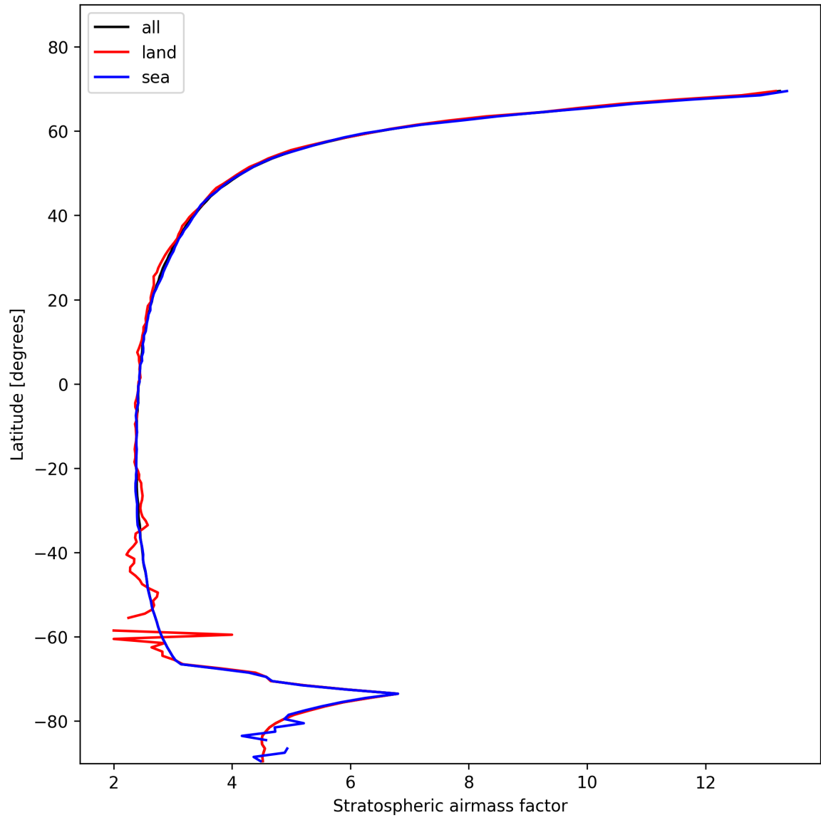
Figure 25: Zonal average of “Stratospheric air mass factor” for 2025-01-25 to 2025-01-26.
