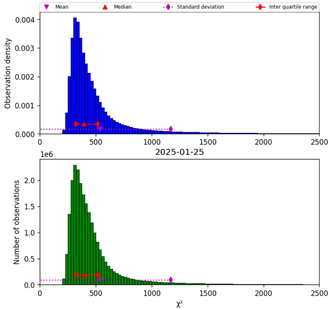
Figure 40: Histogram of “ \chi^2 ” for 2025-01-25 to 2025-01-26
