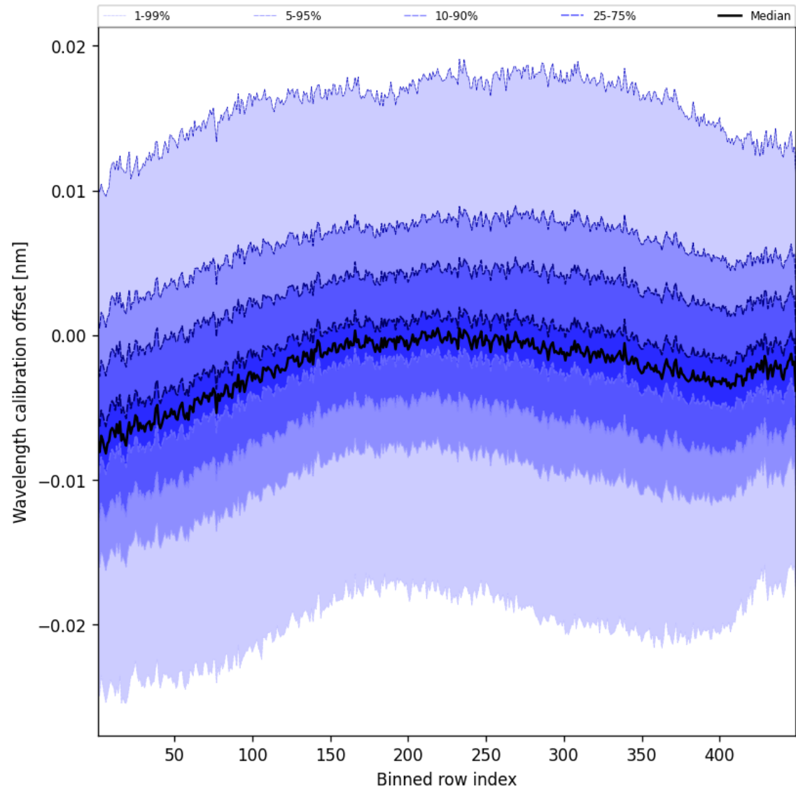
Figure 50: Along track statistics of “Wavelength calibration offset” for 2025-01-25 to 2025-01-26
