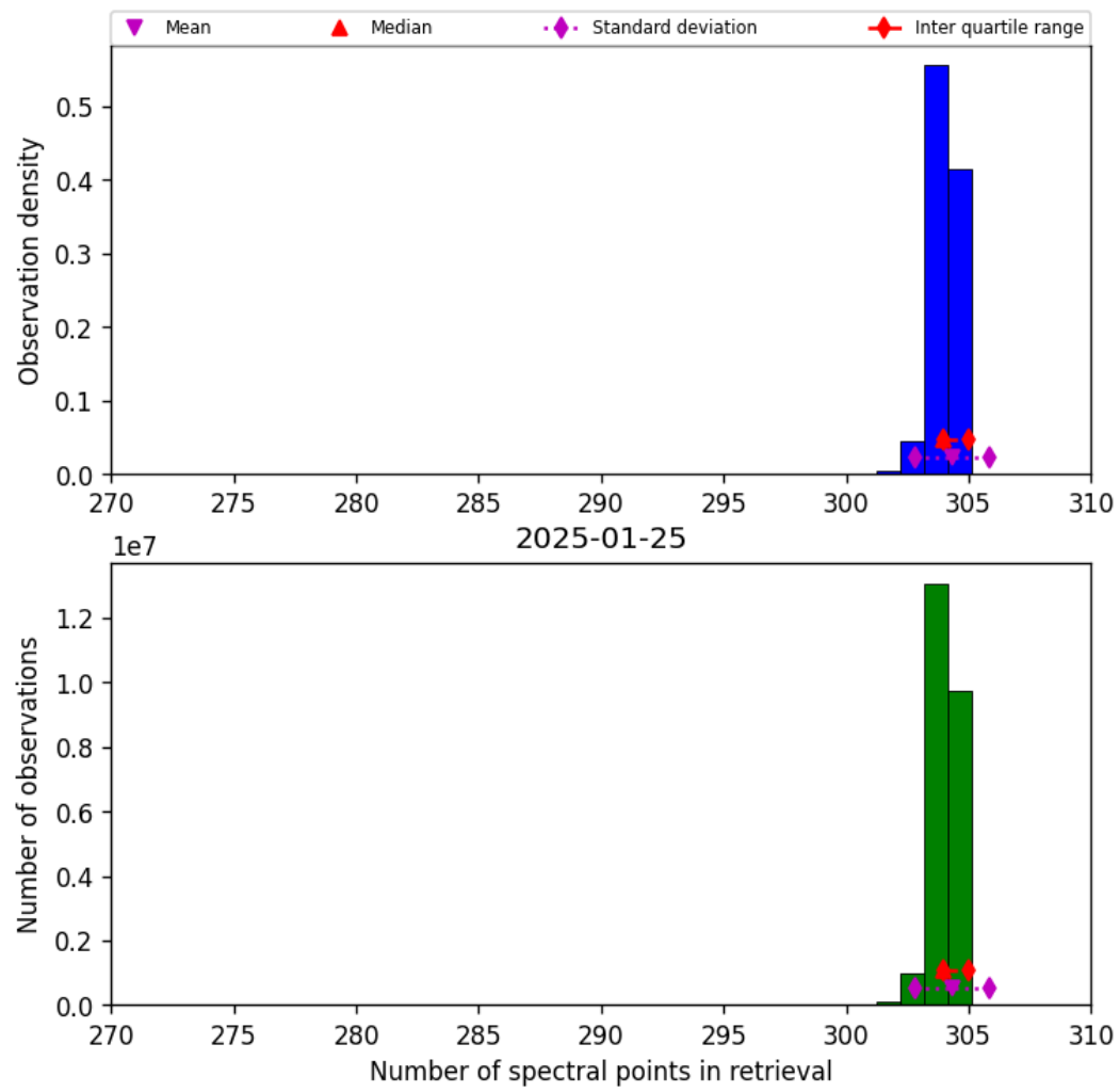
Figure 31: Histogram of “Number of spectral points in retrieval” for 2025-01-25 to 2025-01-26
