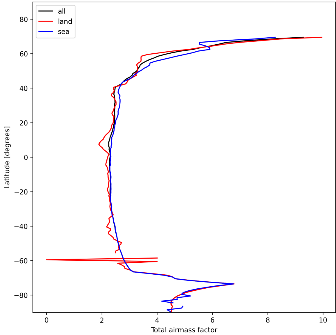
Figure 13: Zonal average of “Total airmass factor” for 2025-01-25 to 2025-01-26.
