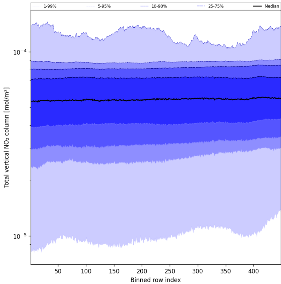
Figure 53: Along track statistics of “Total vertical NO 2 column” for 2025-01-25 to 2025-01-26
