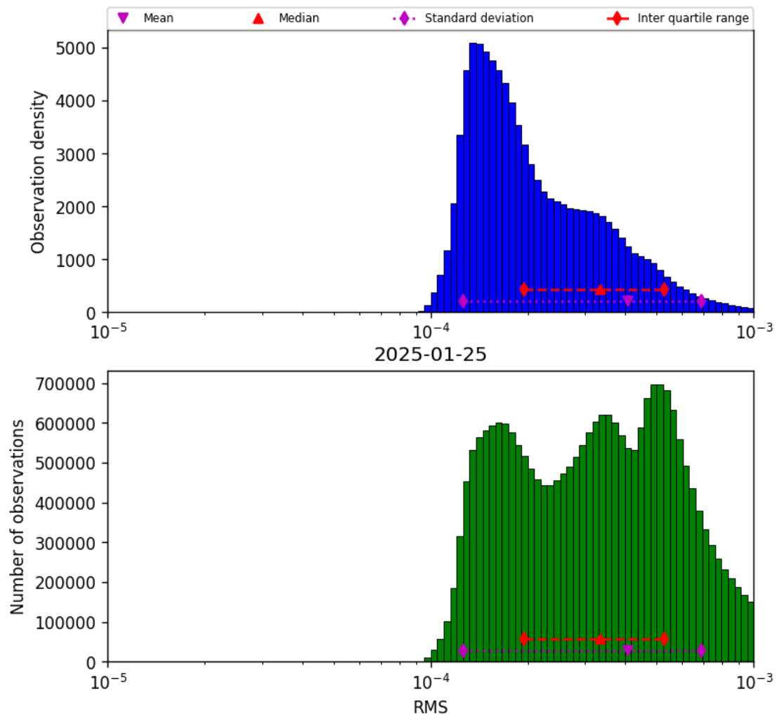
Figure 41: Histogram of “RMS” for 2025-01-25 to 2025-01-26
