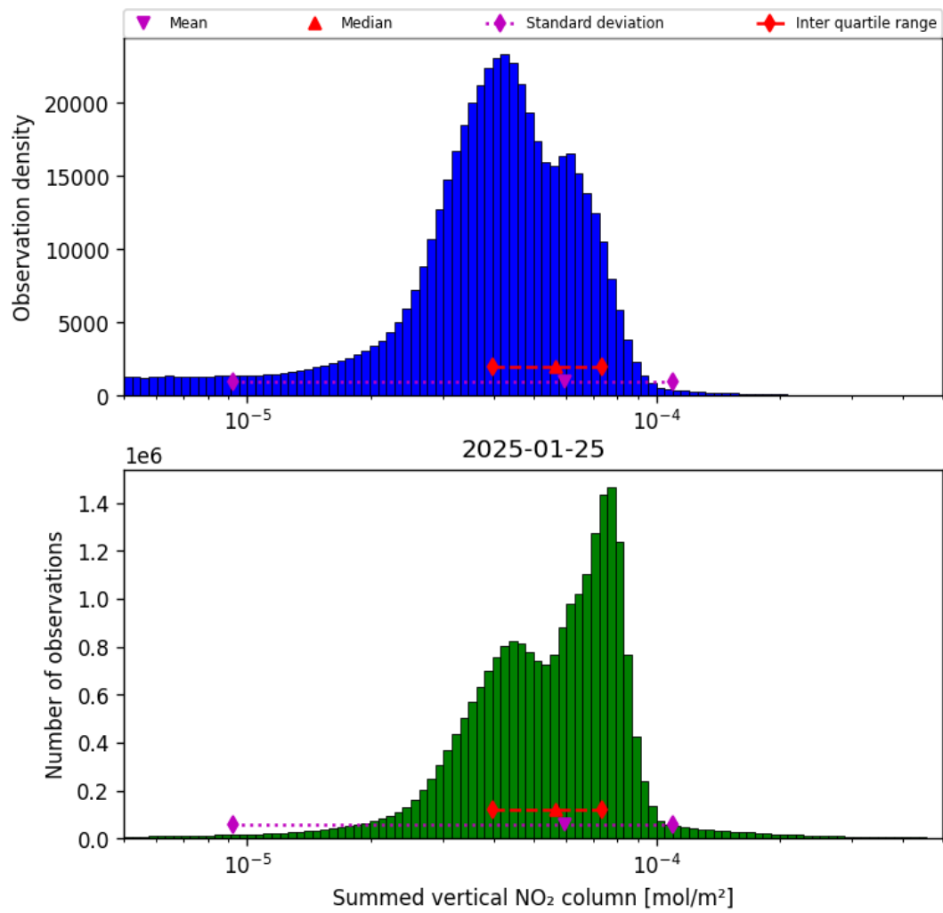
Figure 38: Histogram of “Summed vertical NO 2 column” for 2025-01-25 to 2025-01-26
