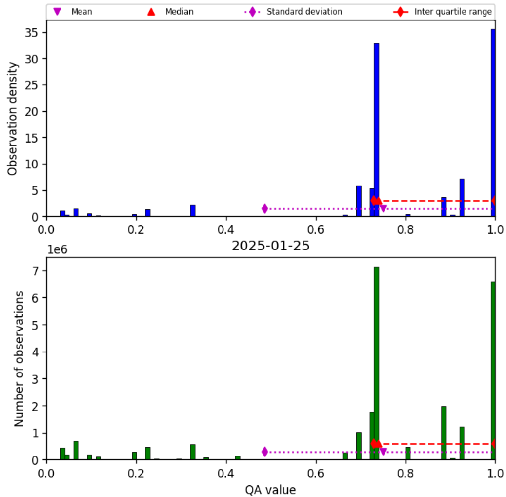
Figure 26: Histogram of “QA value” for 2025-01-25 to 2025-01-26
