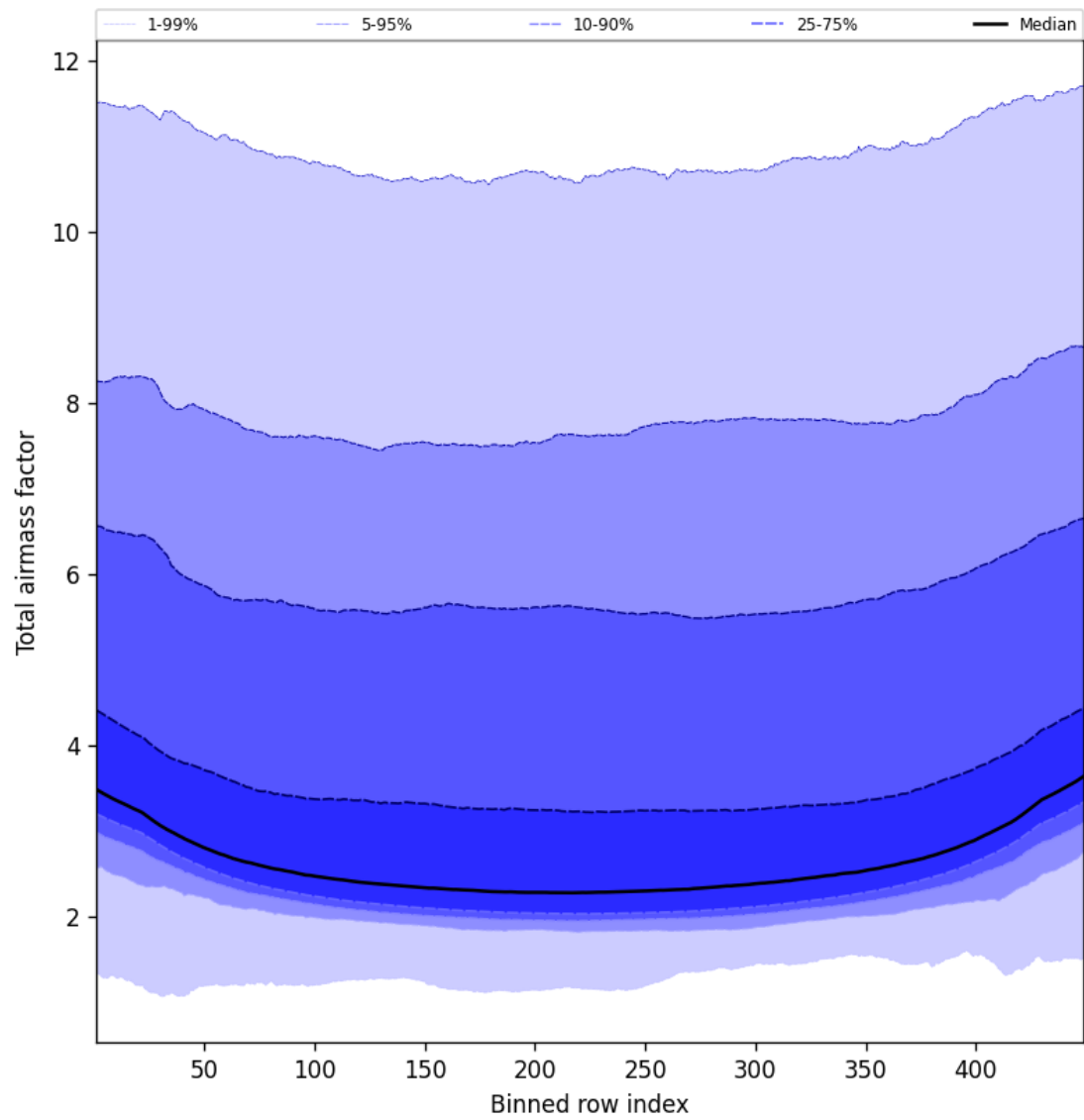
Figure 47: Along track statistics of “Total airmass factor” for 2025-01-25 to 2025-01-26
