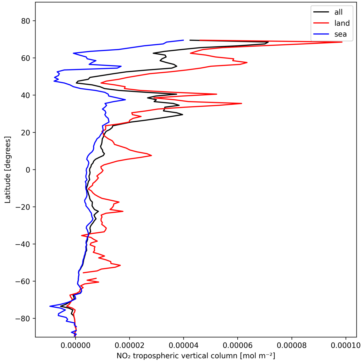
Figure 10: Zonal average of “NO 2 tropospheric vertical column” for 2025-01-25 to 2025-01-26.
