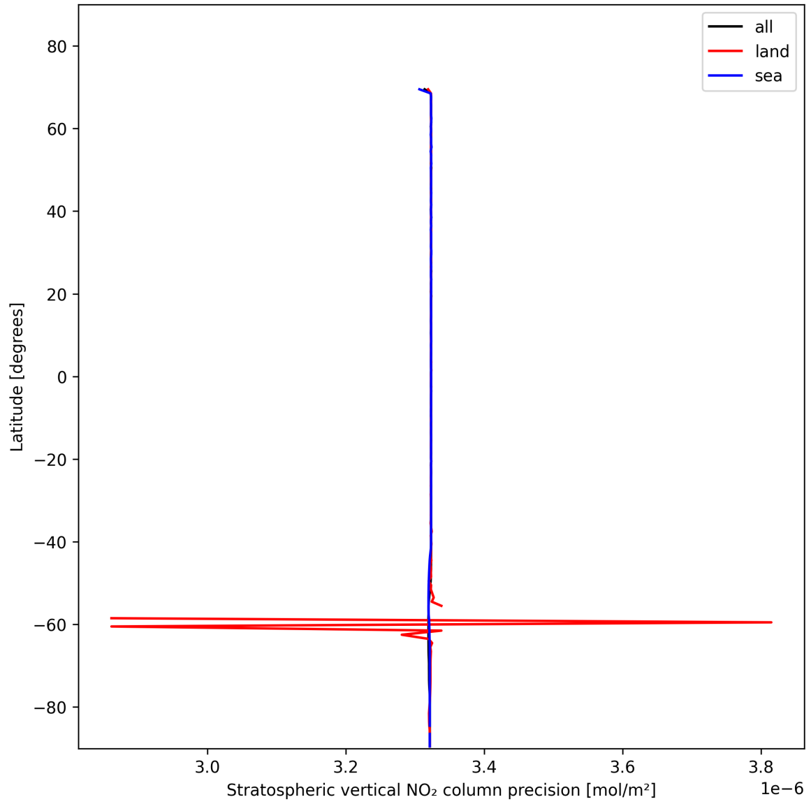
Figure 18: Zonal average of “Stratospheric vertical NO 2 column precision” for 2025-01-25 to 2025-01-26.
