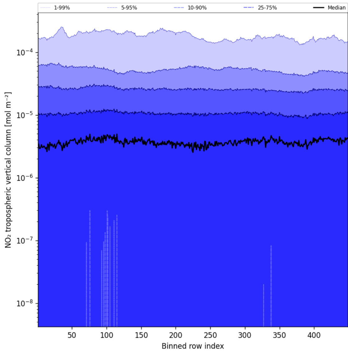
Figure 44: Along track statistics of “NO 2 tropospheric vertical column” for 2025-01-25 to 2025-01-26
