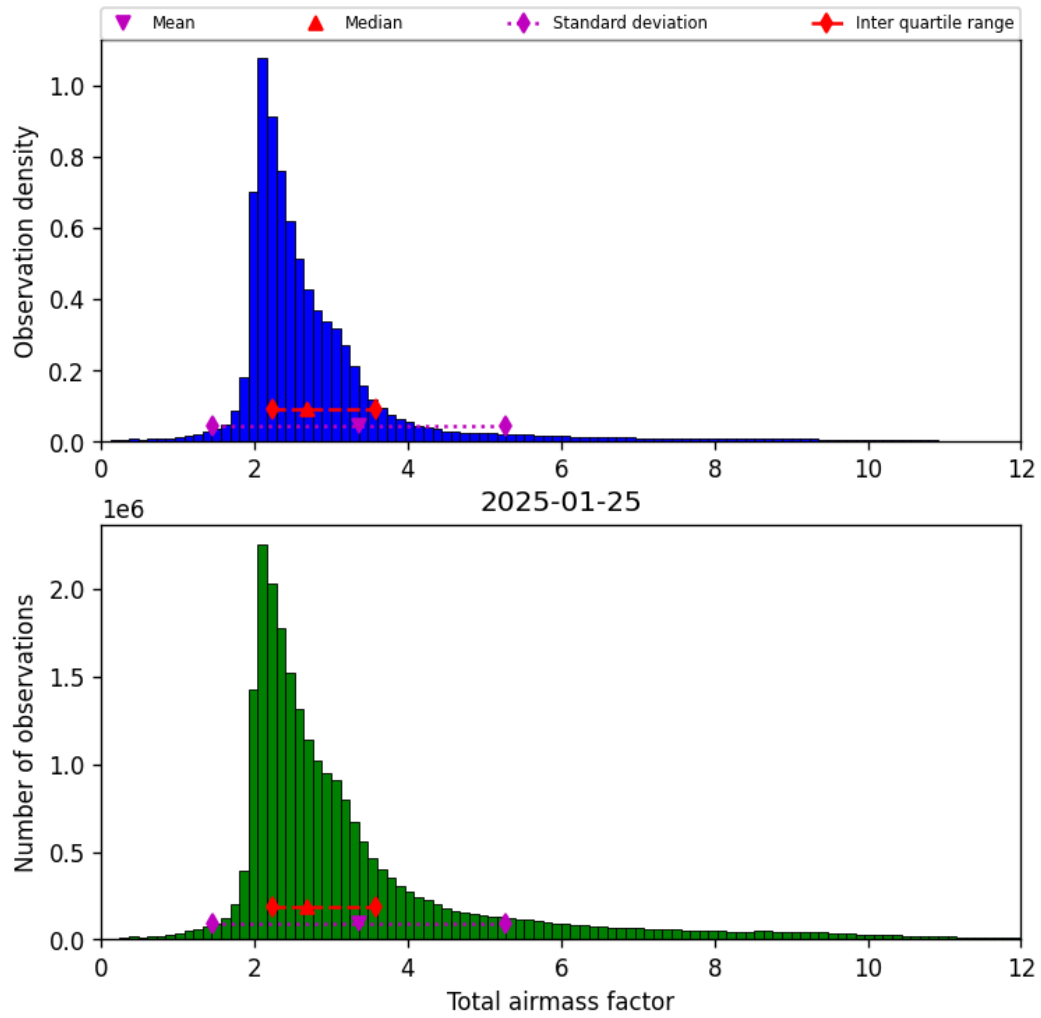
Figure 30: Histogram of “Total airmass factor” for 2025-01-25 to 2025-01-26
