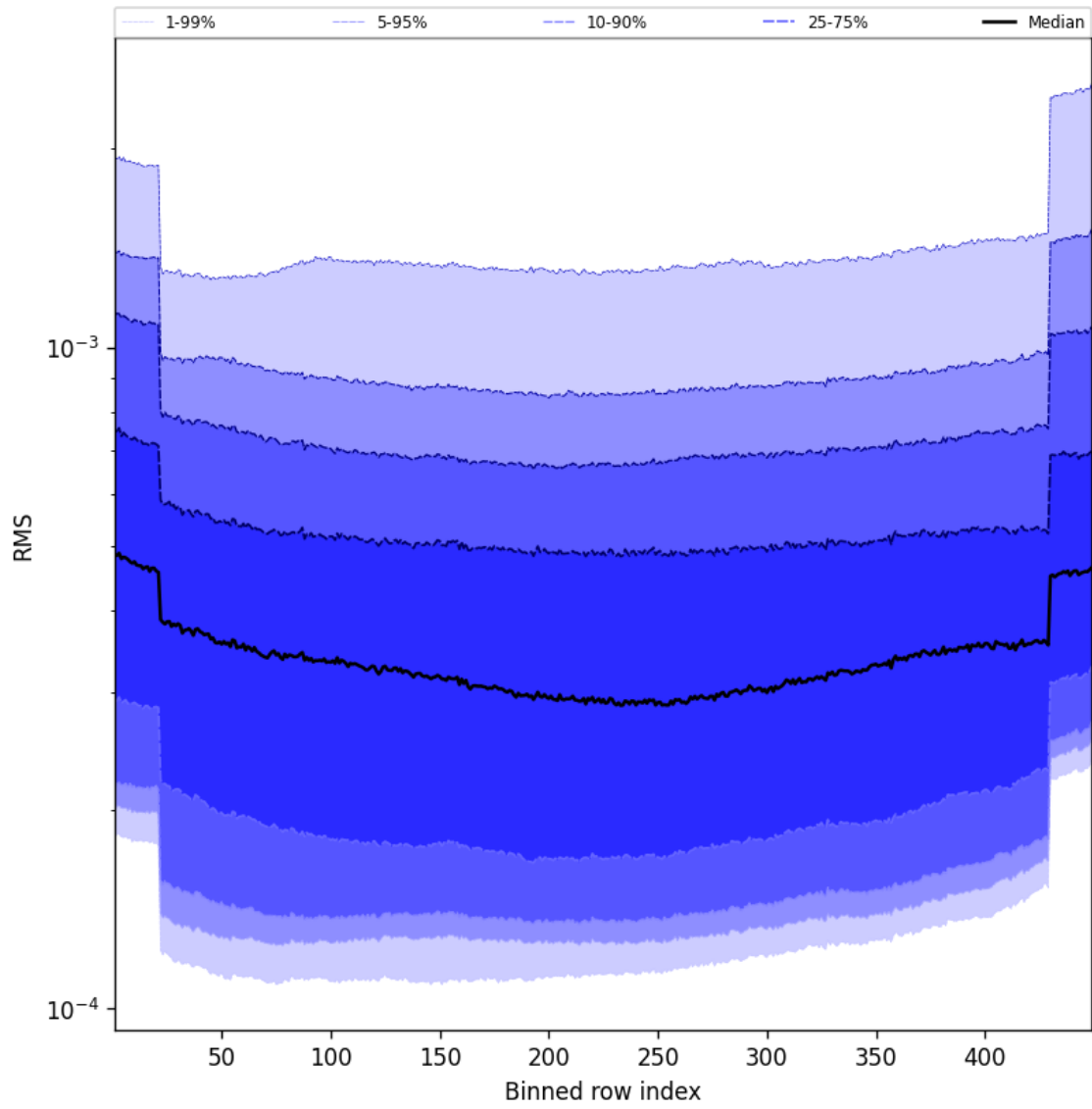
Figure 58: Along track statistics of “RMS” for 2025-01-25 to 2025-01-26
