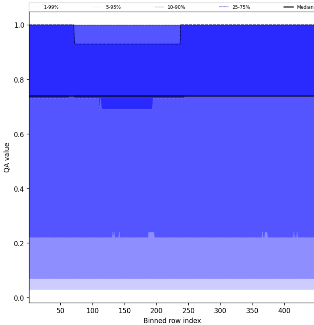
Figure 43: Along track statistics of “QA value” for 2025-01-25 to 2025-01-26
