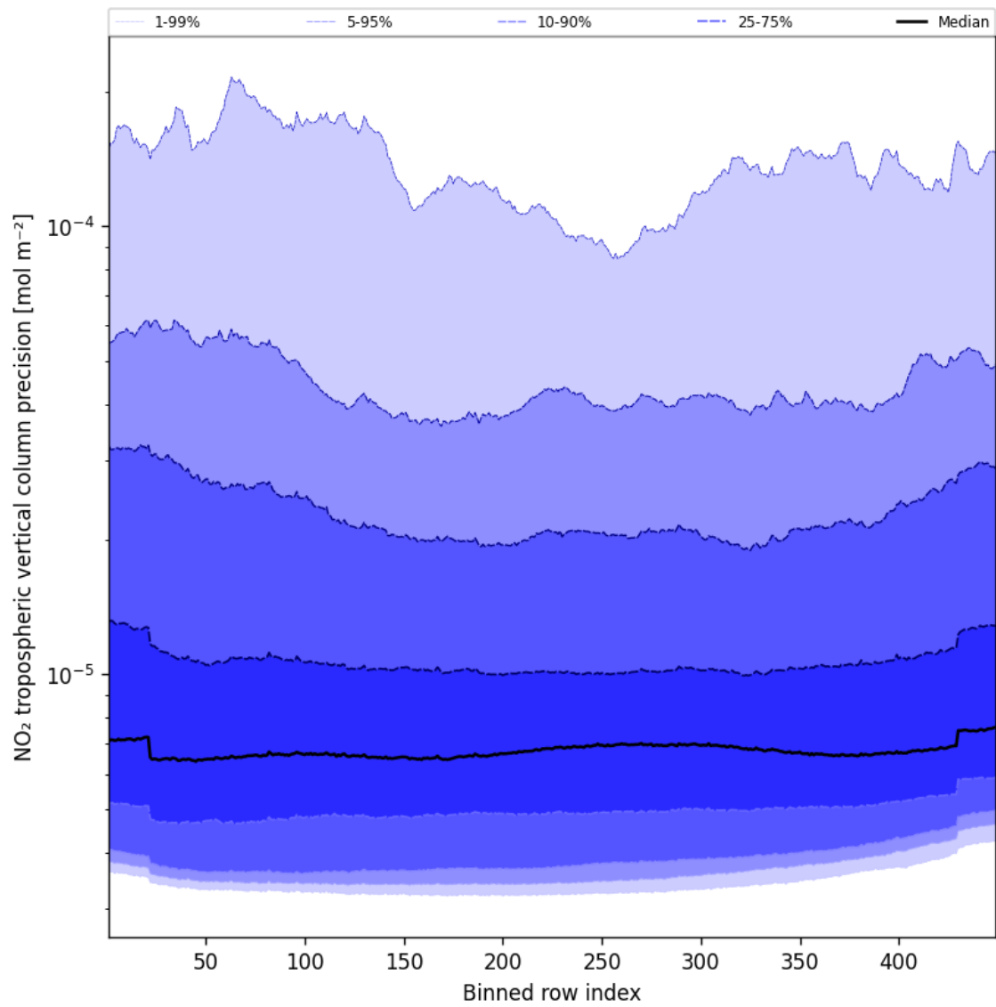
Figure 45: Along track statistics of “NO 2 tropospheric vertical column precision” for 2025-01-25 to 2025-01-26
