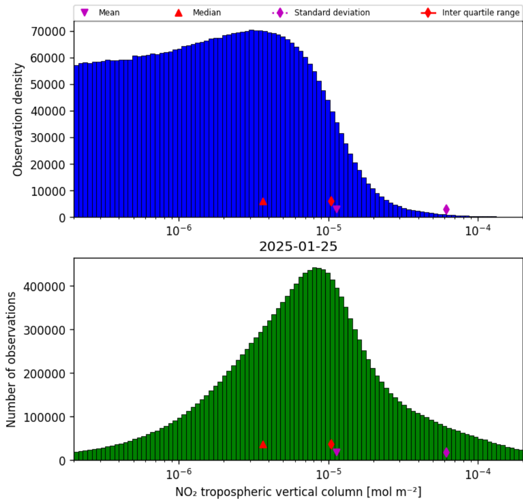
Figure 27: Histogram of “NO 2 tropospheric vertical column” for 2025-01-25 to 2025-01-26
