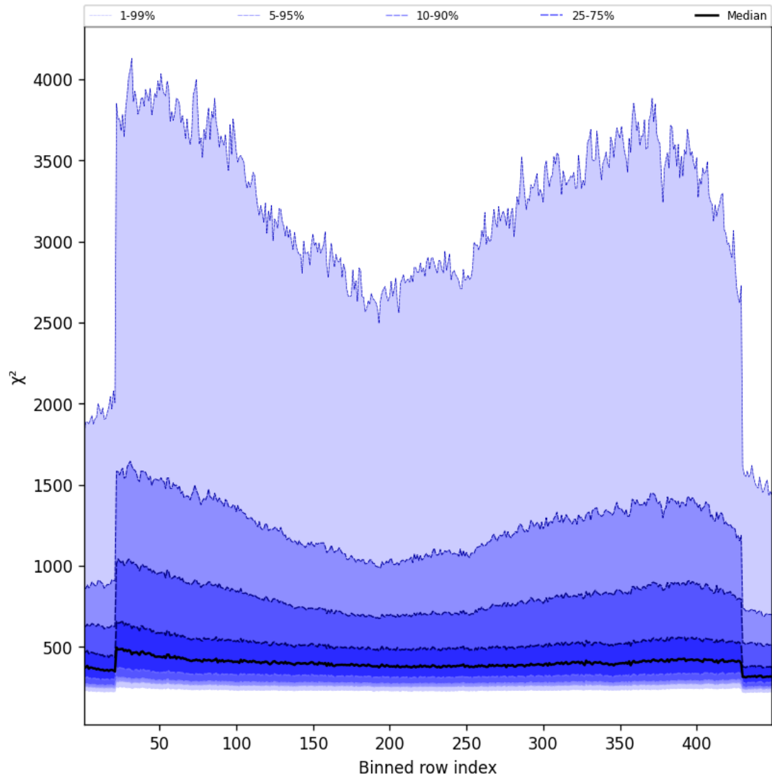
Figure 57: Along track statistics of “ \chi^2 ” for 2025-01-25 to 2025-01-26
