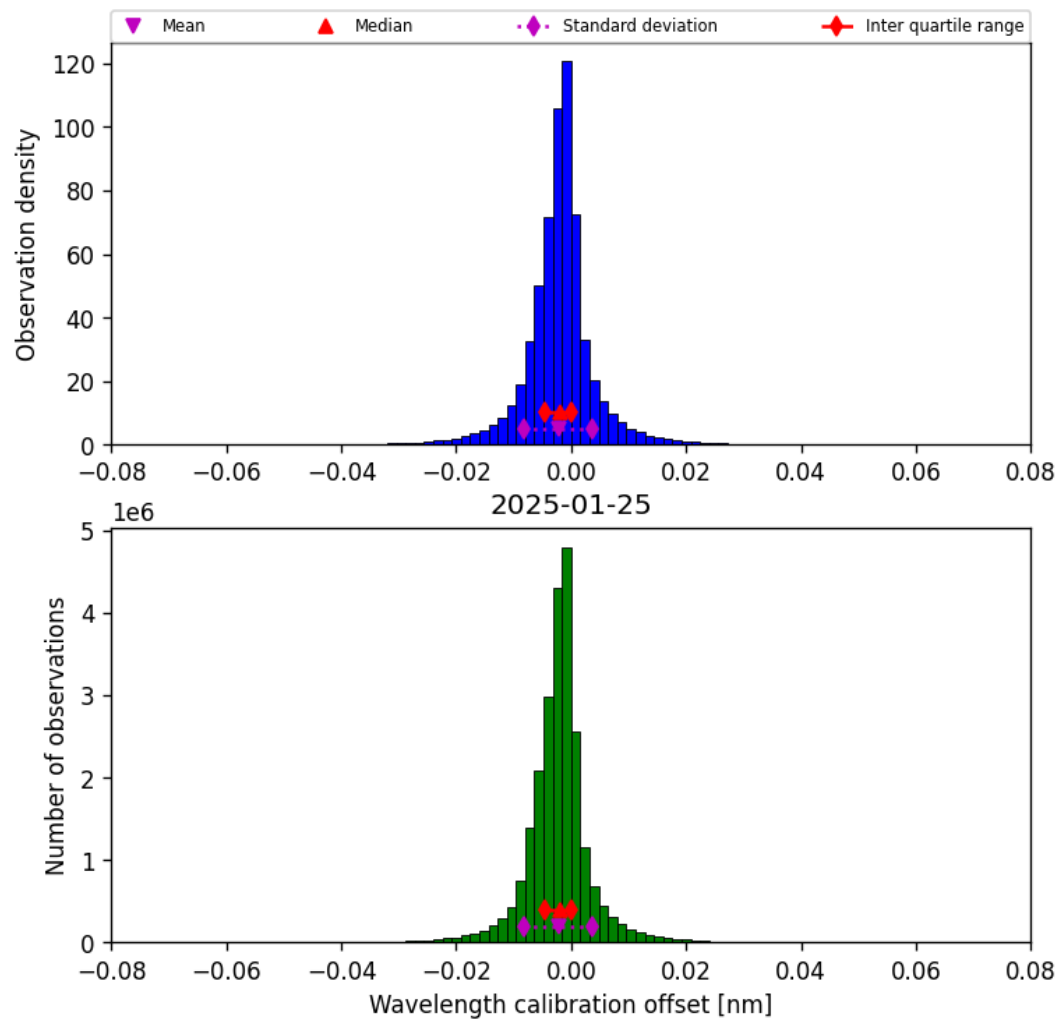
Figure 33: Histogram of “Wavelength calibration offset” for 2025-01-25 to 2025-01-26
