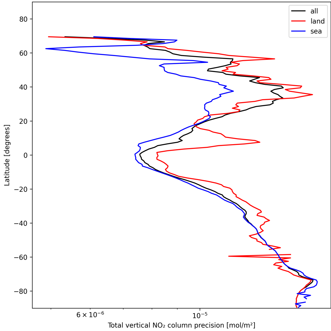
Figure 20: Zonal average of “Total vertical NO 2 column precision” for 2025-01-25 to 2025-01-26.
