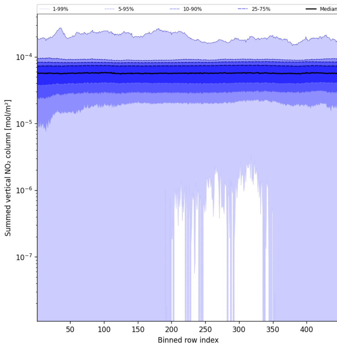
Figure 55: Along track statistics of “Summed vertical NO 2 column” for 2025-01-25 to 2025-01-26
