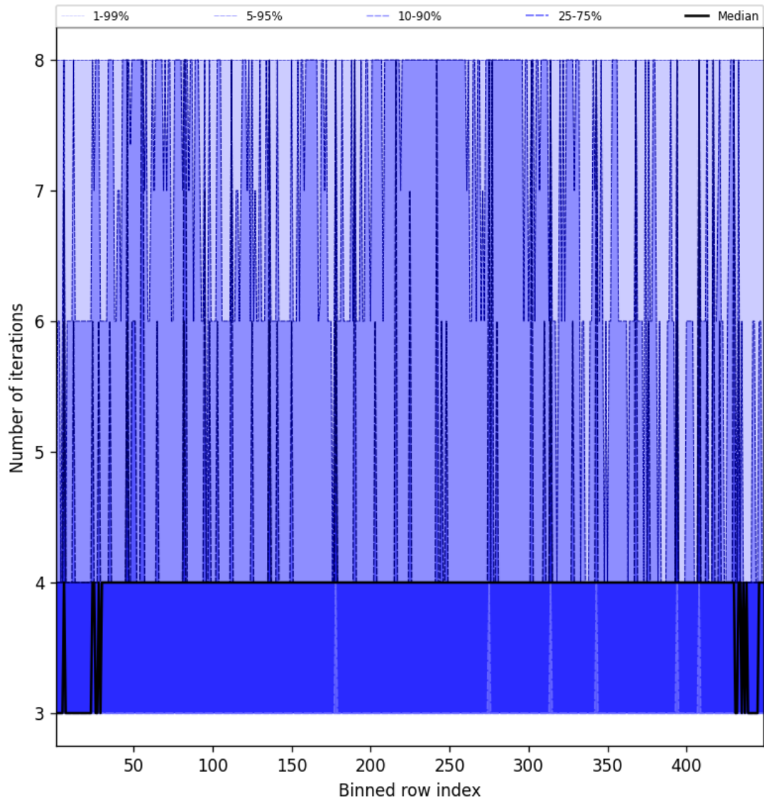
Figure 49: Along track statistics of “Number of iterations” for 2025-01-25 to 2025-01-26
