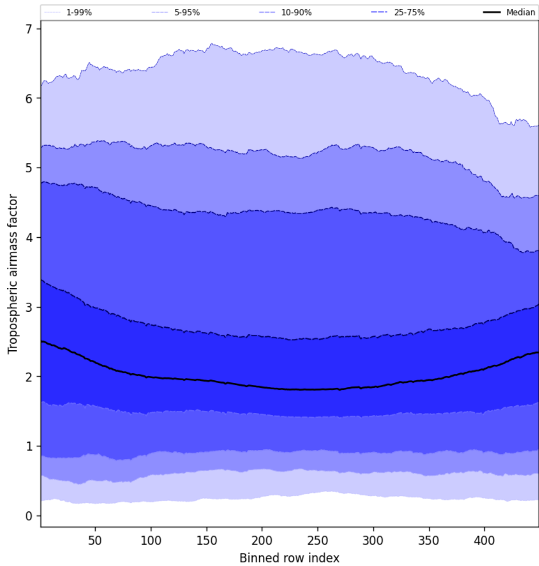
Figure 46: Along track statistics of “Tropospheric air mass factor” for 2025-01-25 to 2025-01-26
