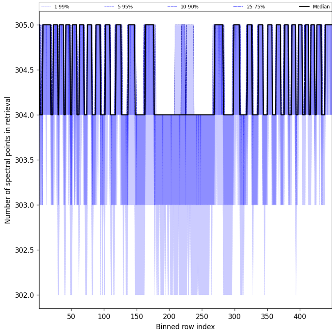
Figure 48: Along track statistics of “Number of spectral points in retrieval” for 2025-01-25 to 2025-01-26
