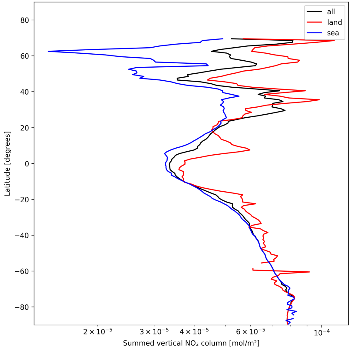
Figure 21: Zonal average of “Summed vertical NO 2 column” for 2025-01-25 to 2025-01-26.
