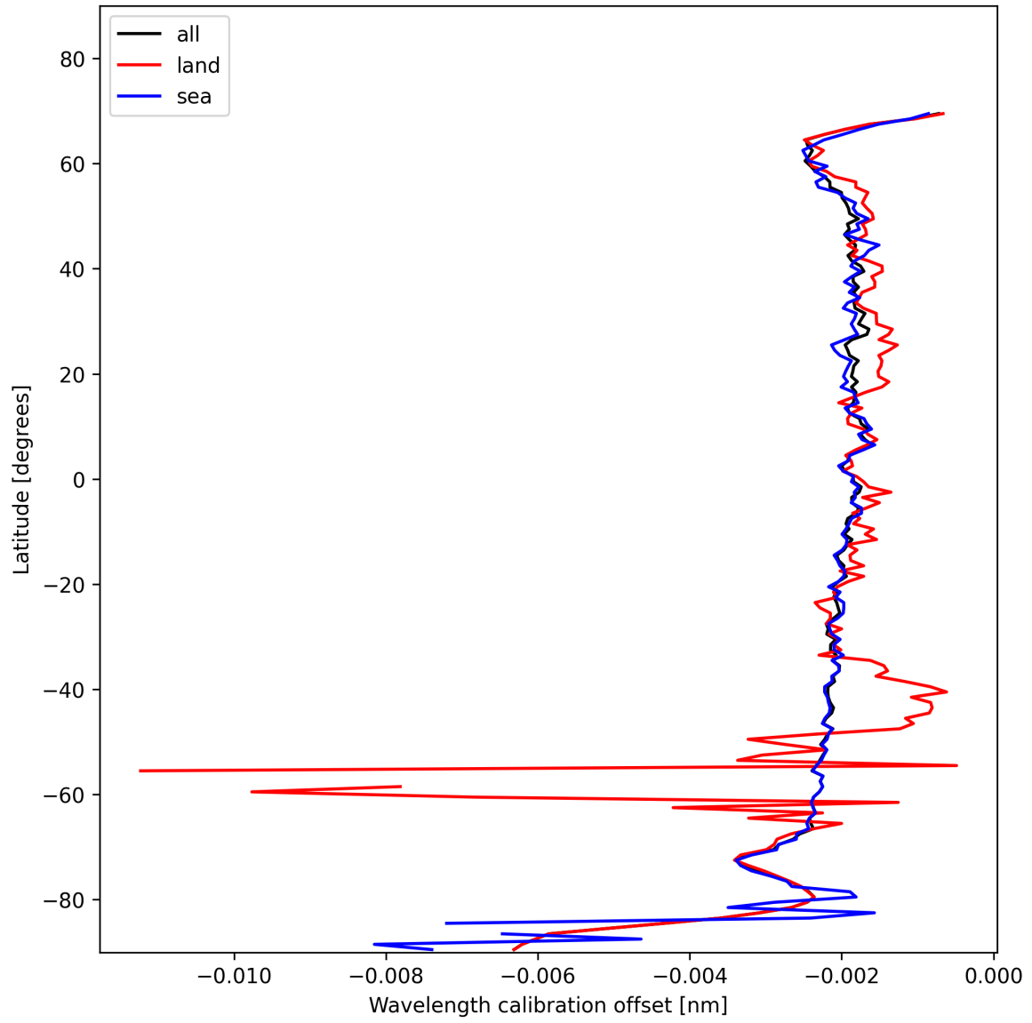
Figure 16: Zonal average of “Wavelength calibration offset” for 2025-01-25 to 2025-01-26.
