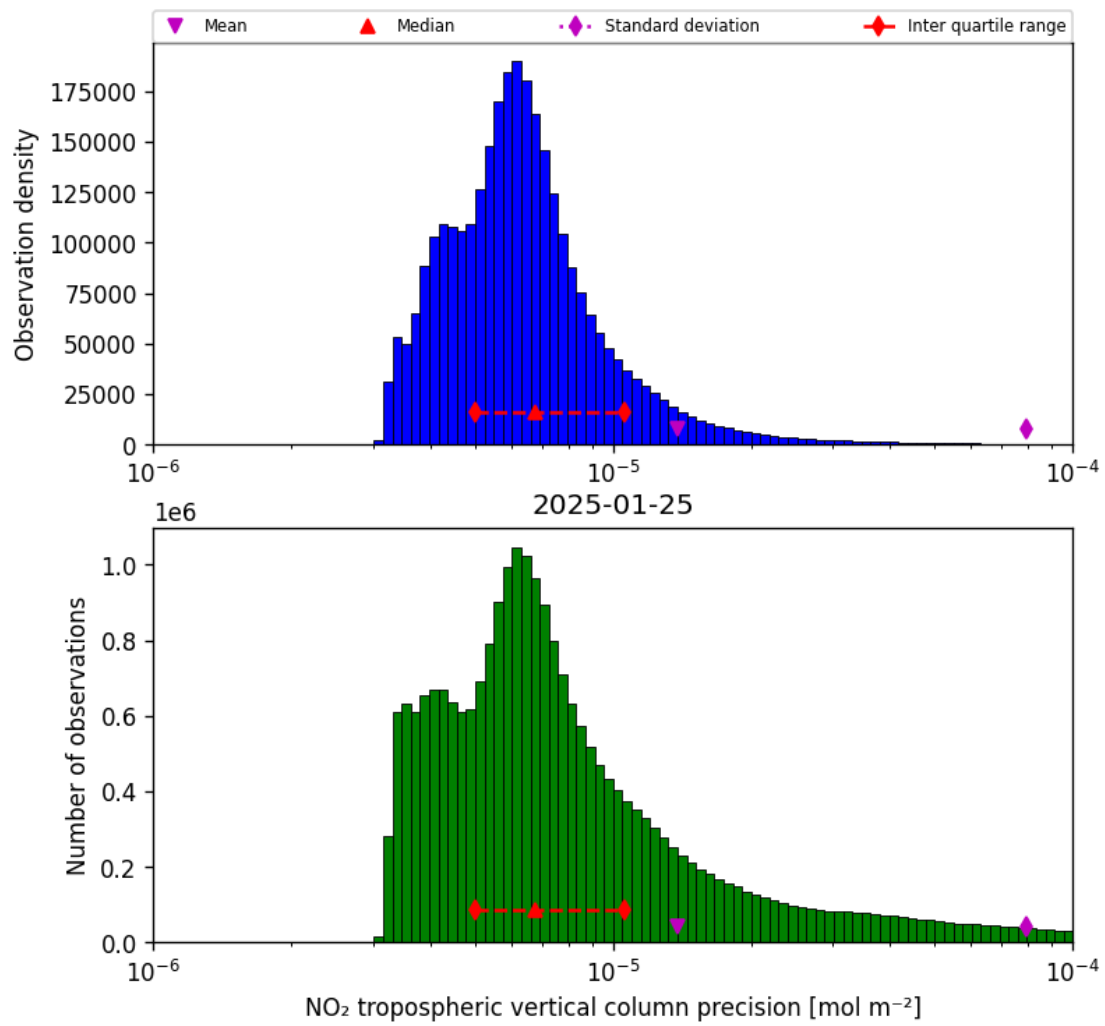
Figure 28: Histogram of "NO 2 tropospheric vertical column precision" for 2025-01-25 to 2025-01-26
