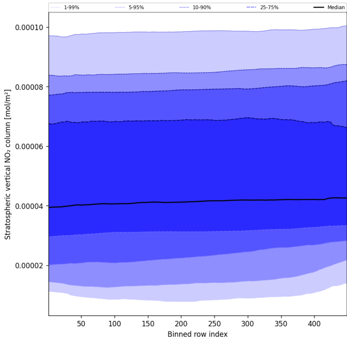
Figure 51: Along track statistics of “Stratospheric vertical NO 2 column” for 2025-01-25 to 2025-01-26
