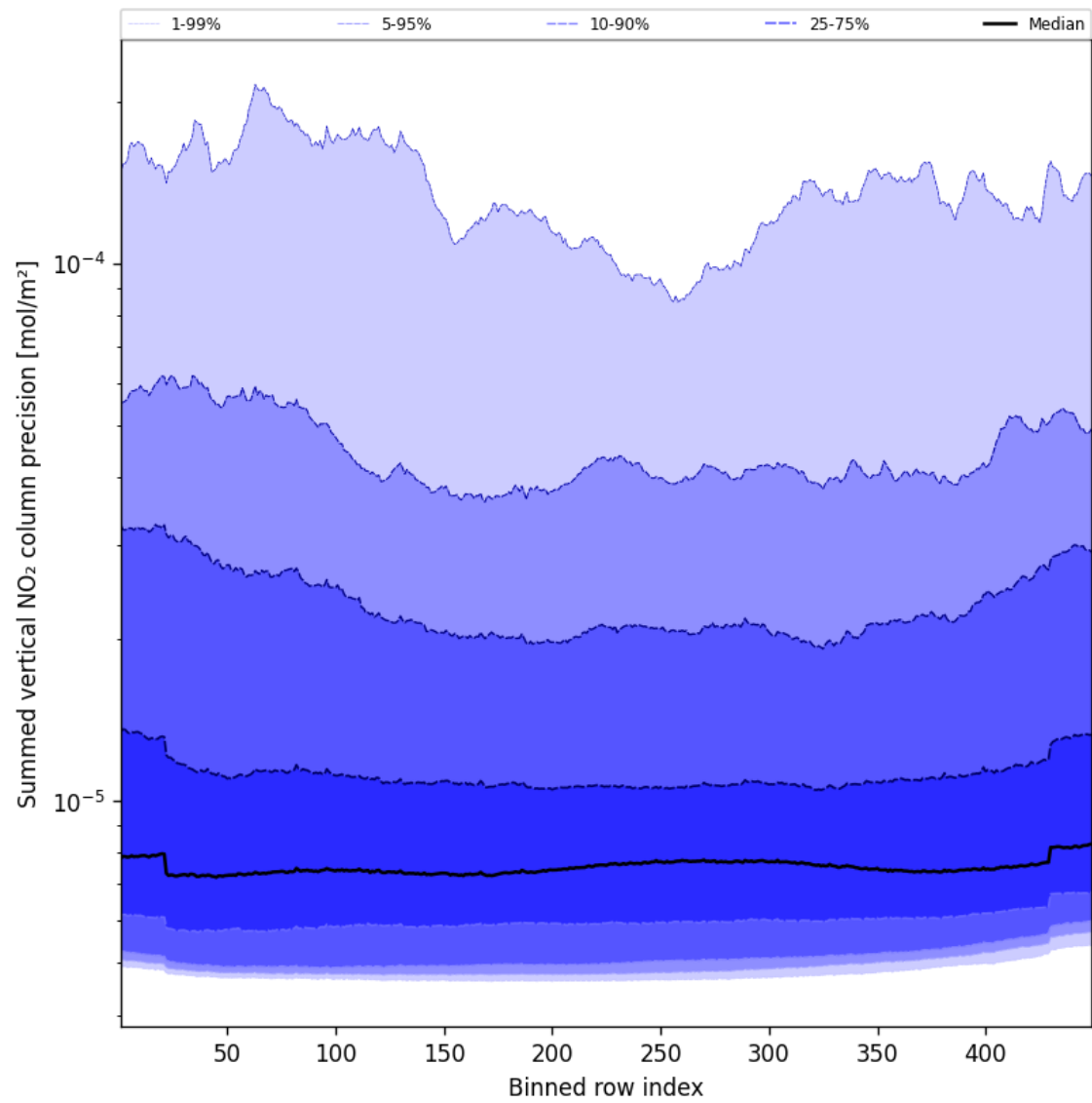
Figure 56: Along track statistics of “Summed vertical NO 2 column precision” for 2025-01-25 to 2025-01-26
