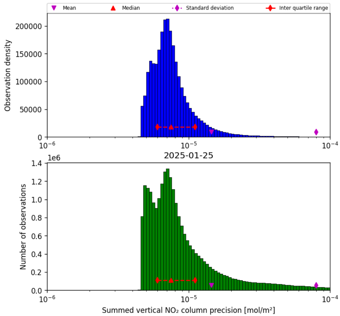
Figure 39: Histogram of “Summed vertical NO 2 column precision” for 2025-01-25 to 2025-01-26
