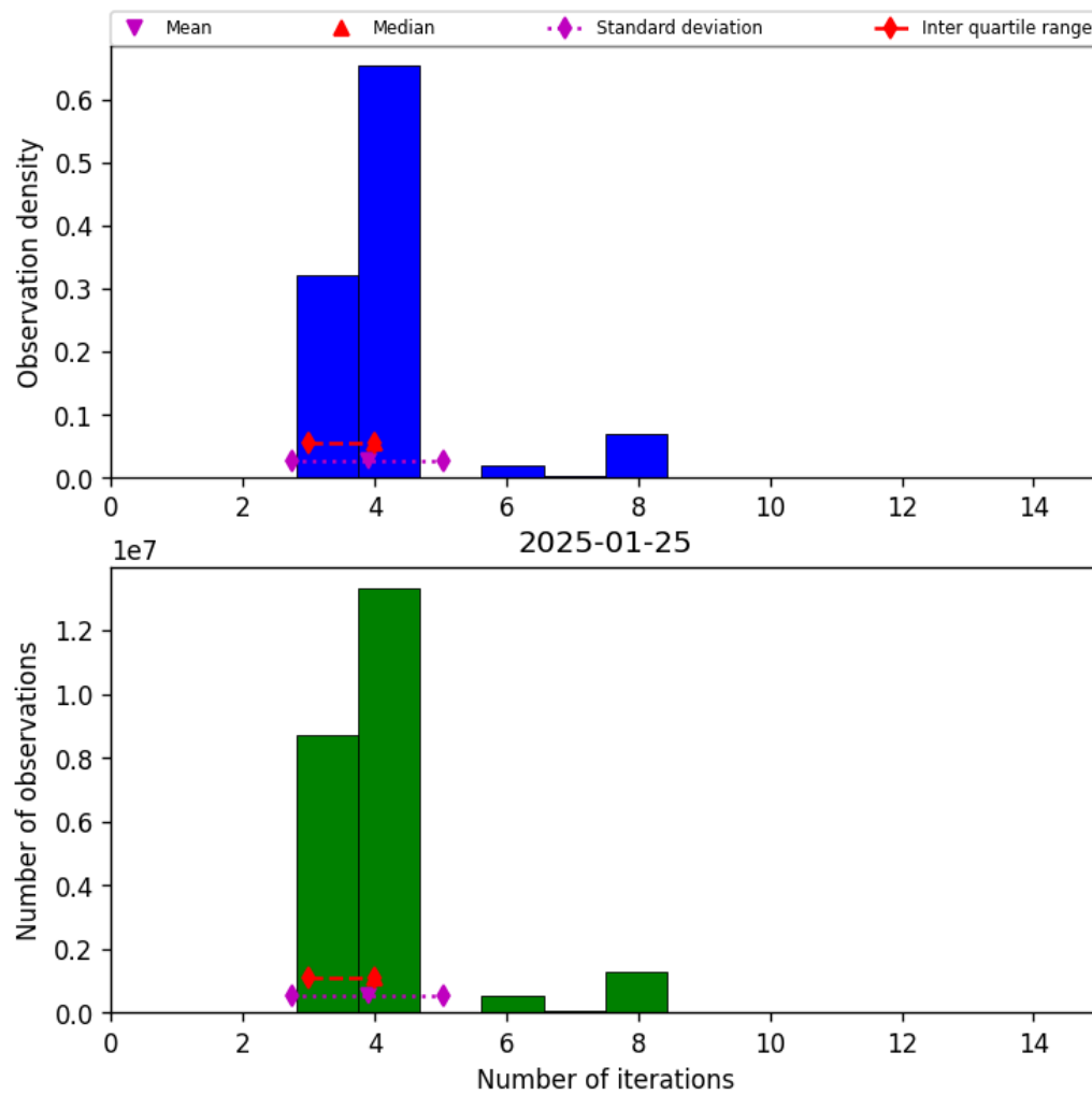
Figure 32: Histogram of “Number of iterations” for 2025-01-25 to 2025-01-26
