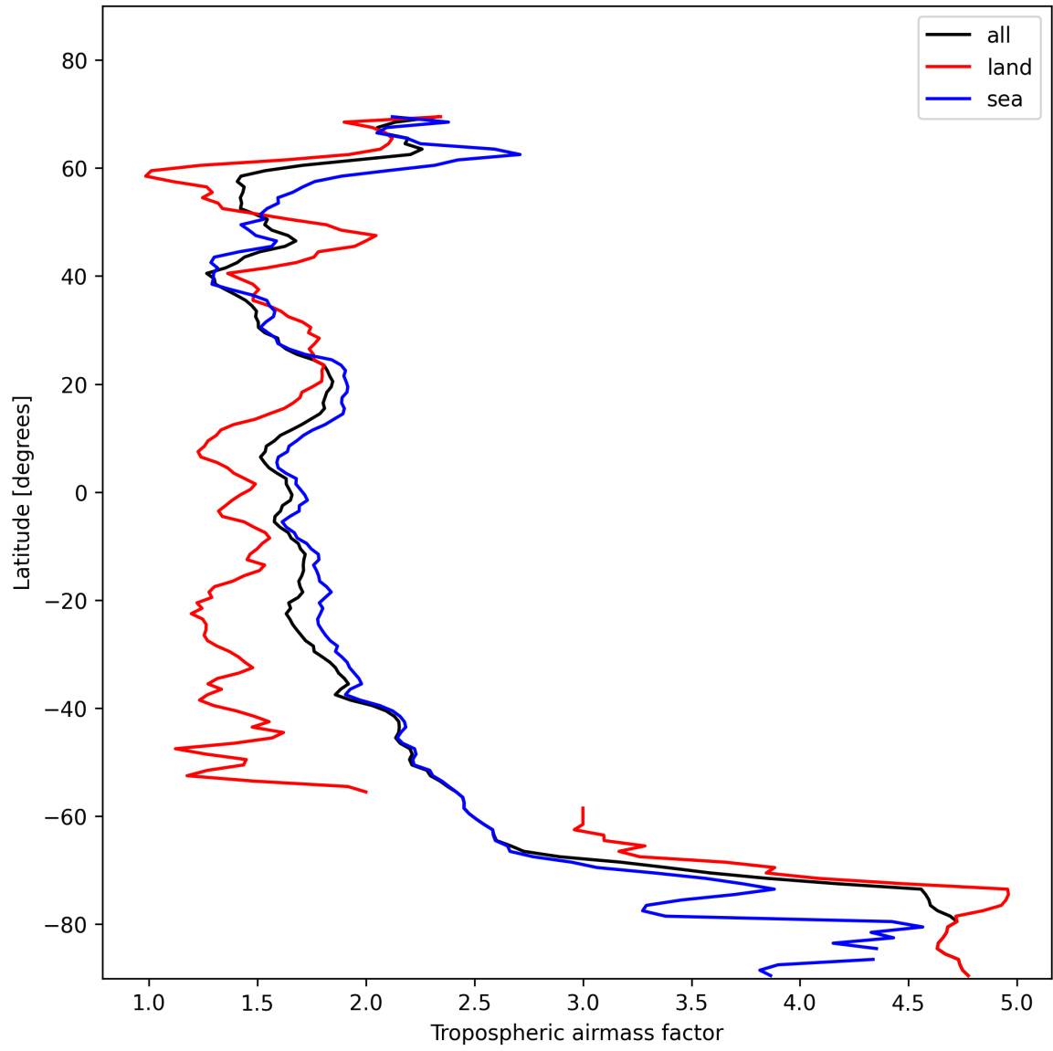
Figure 12: Zonal average of “Tropospheric airmass factor” for 2025-01-25 to 2025-01-26.
