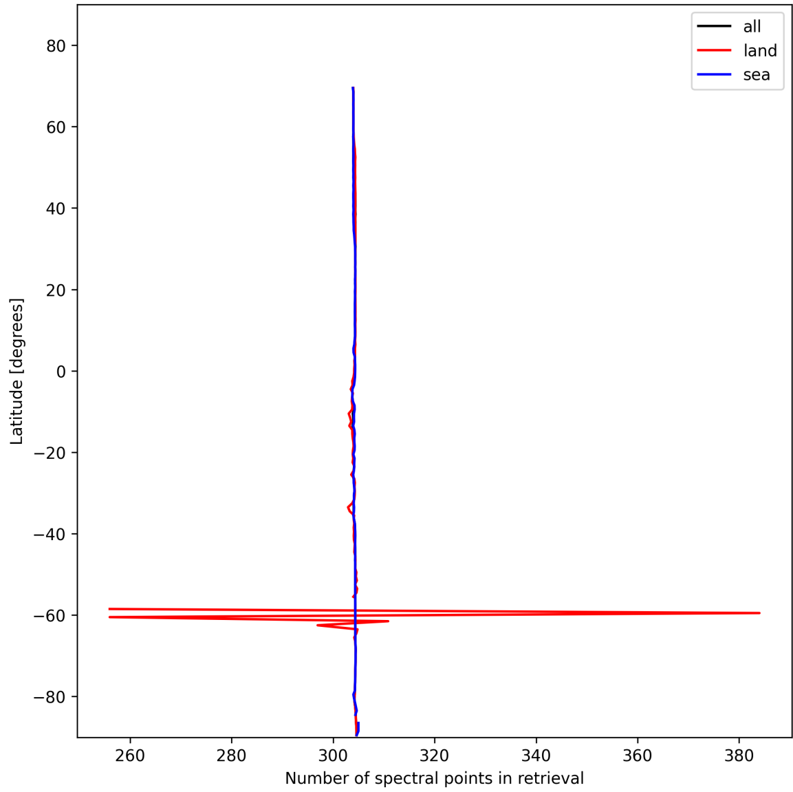
Figure 14: Zonal average of “Number of spectral points in retrieval” for 2025-01-25 to 2025-01-26.
