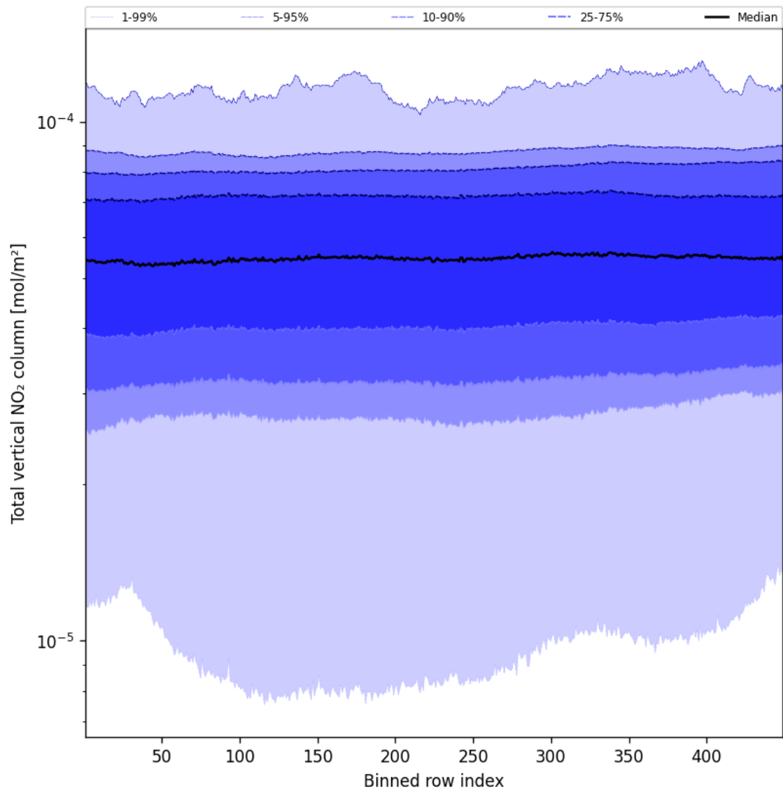
Figure 53: Along track statistics of “Total vertical NO 2 column” for 2025-01-26 to 2025-01-26
