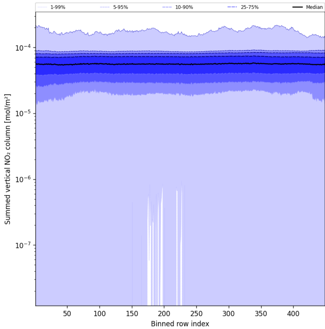
Figure 55: Along track statistics of “Summed vertical NO 2 column” for 2025-01-26 to 2025-01-26
