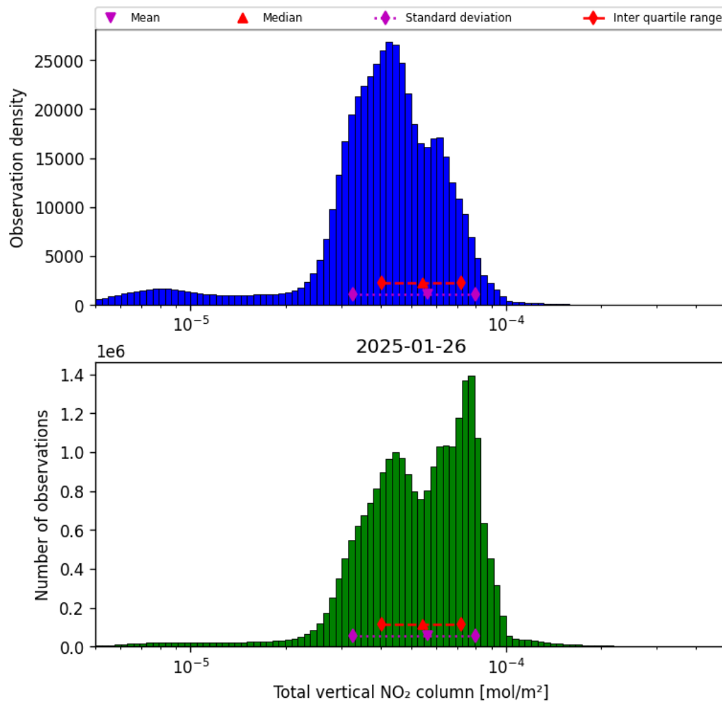
Figure 36: Histogram of “Total vertical NO 2 column” for 2025-01-26 to 2025-01-26
