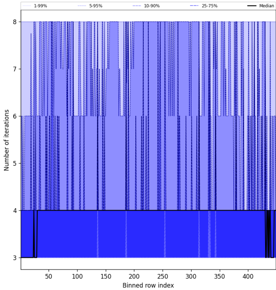
Figure 49: Along track statistics of “Number of iterations” for 2025-01-26 to 2025-01-26
