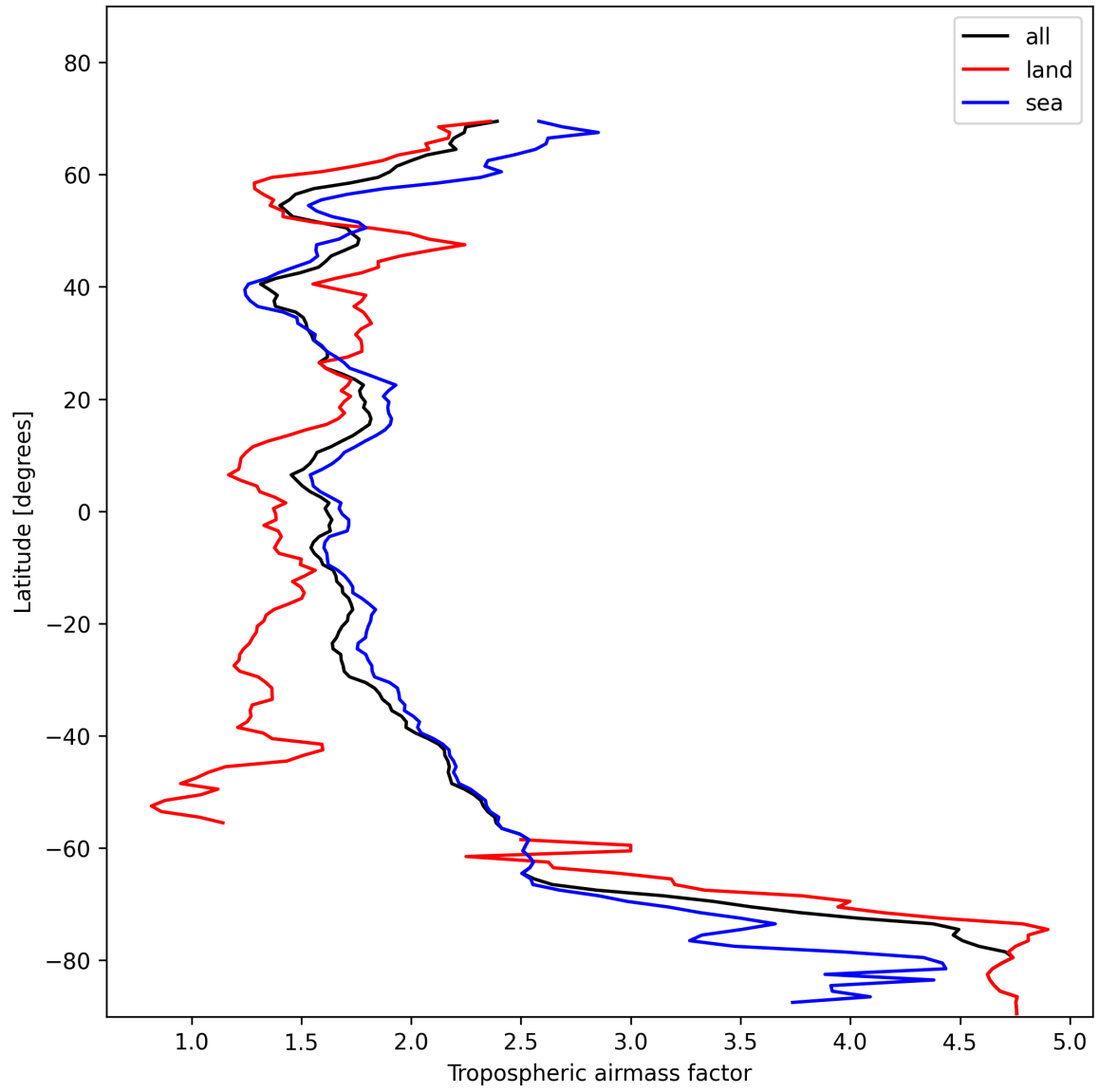
Figure 12: Zonal average of “Tropospheric airmass factor” for 2025-01-26 to 2025-01-26.
