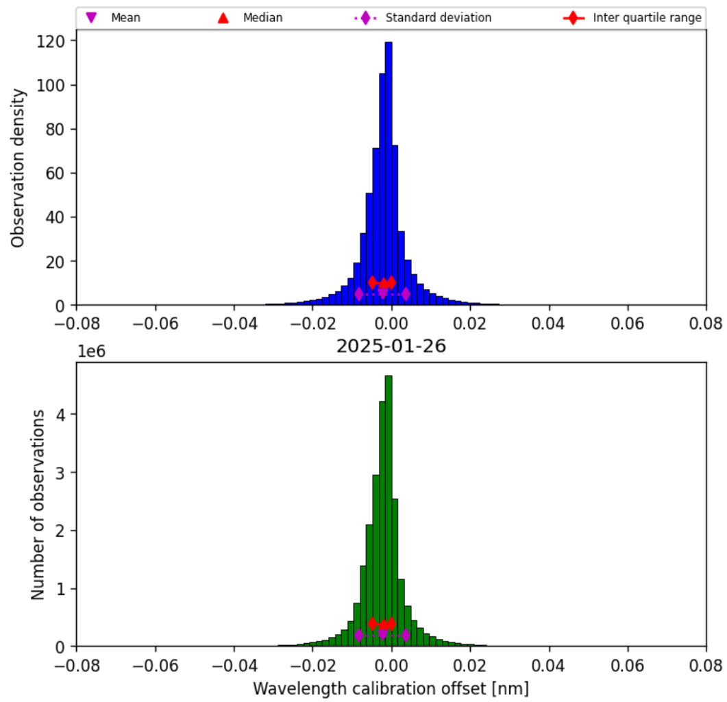
Figure 33: Histogram of “Wavelength calibration offset” for 2025-01-26 to 2025-01-26
