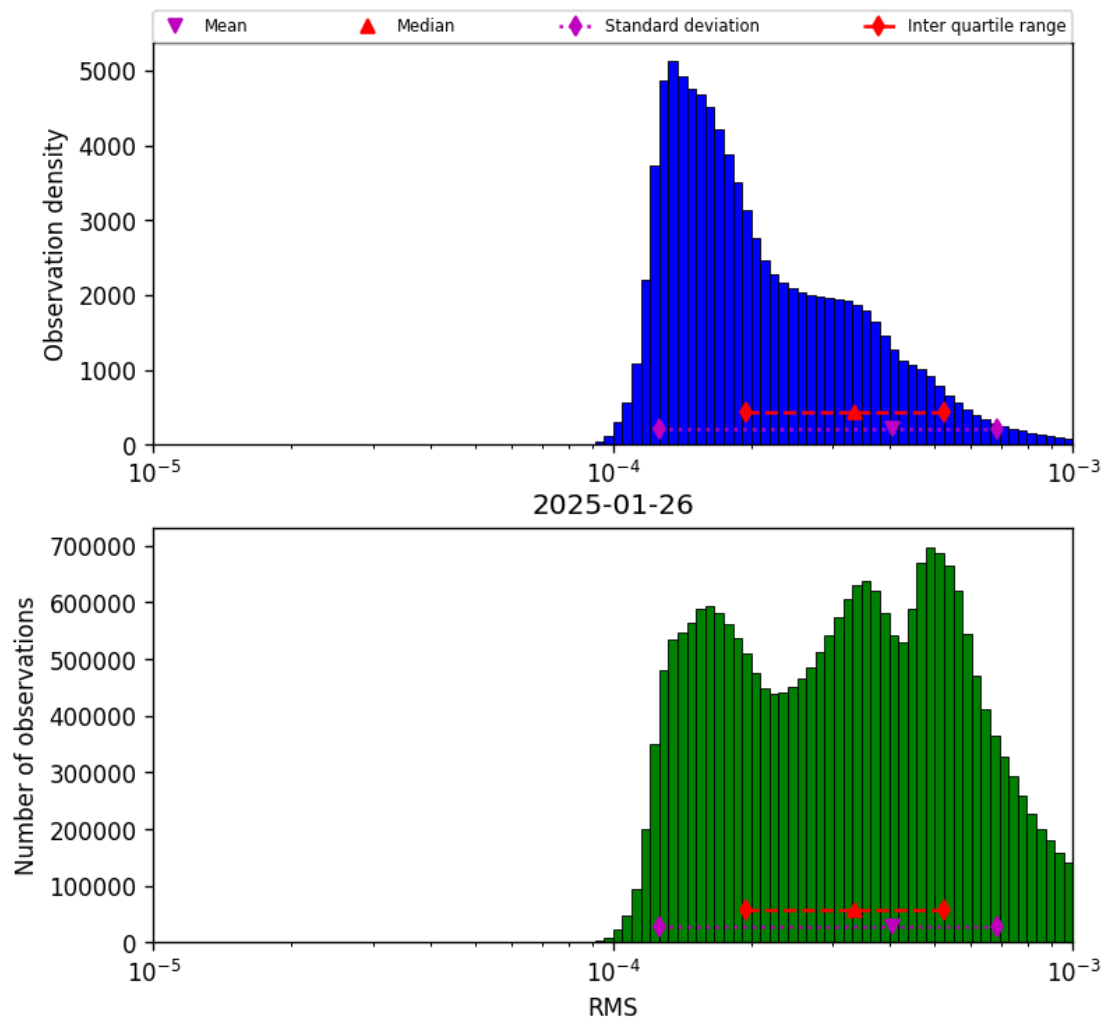
Figure 41: Histogram of “RMS” for 2025-01-26 to 2025-01-26
