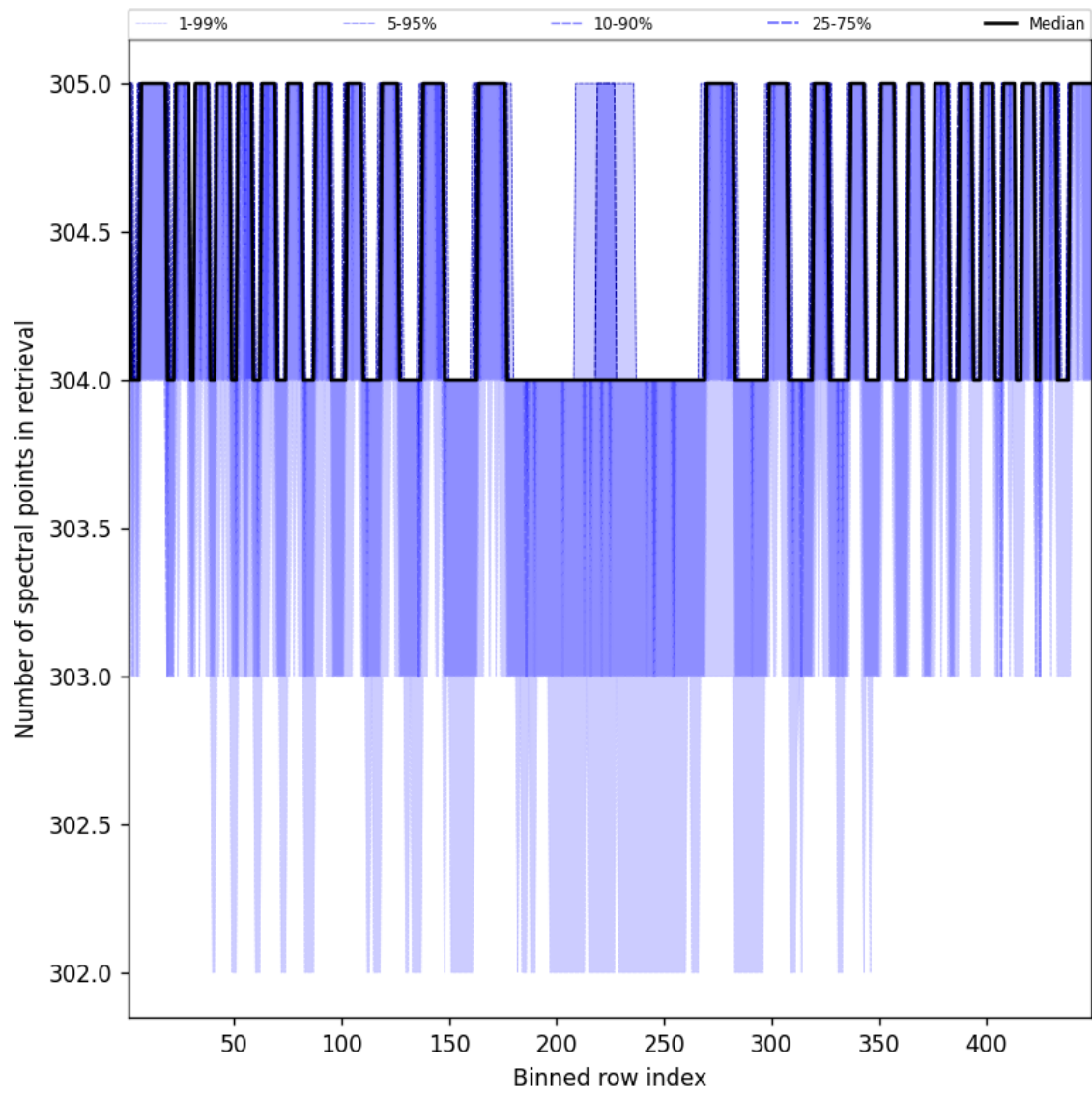
Figure 48: Along track statistics of “Number of spectral points in retrieval” for 2025-01-26 to 2025-01-26
