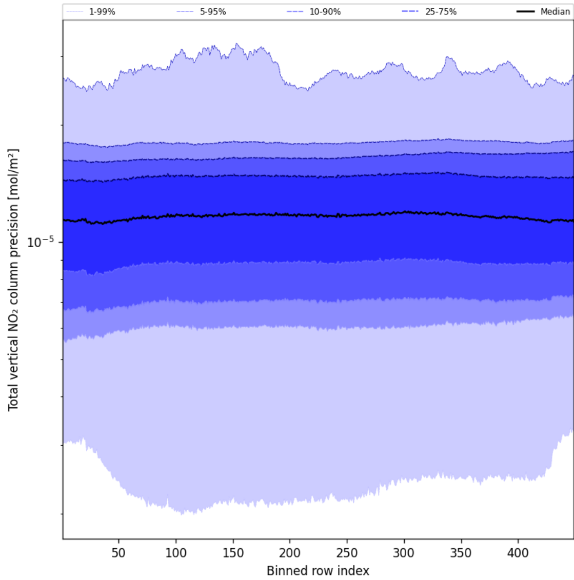
Figure 54: Along track statistics of “Total vertical NO 2 column precision” for 2025-01-26 to 2025-01-26
