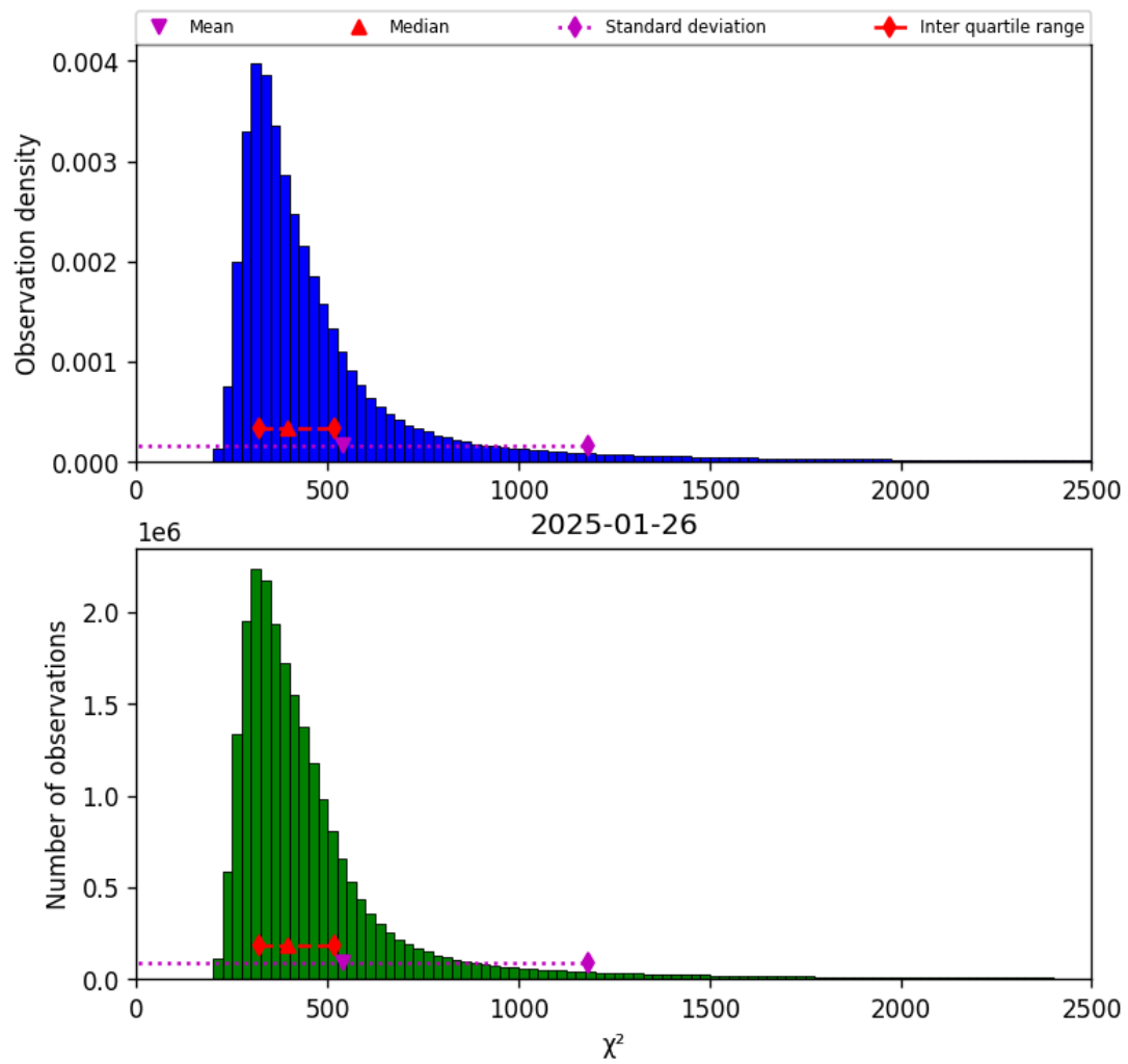
Figure 40: Histogram of “ \chi^2 ” for 2025-01-26 to 2025-01-26
