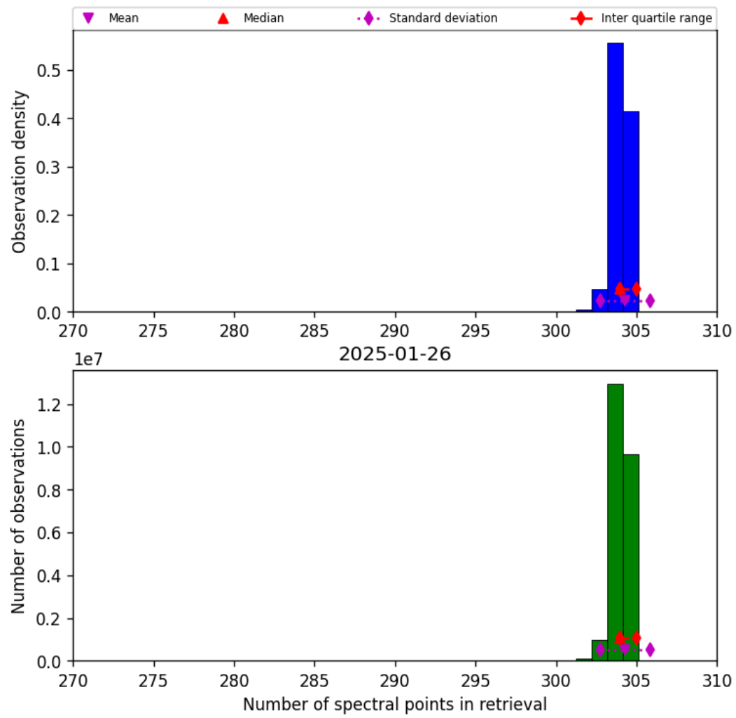
Figure 31: Histogram of “Number of spectral points in retrieval” for 2025-01-26 to 2025-01-26
