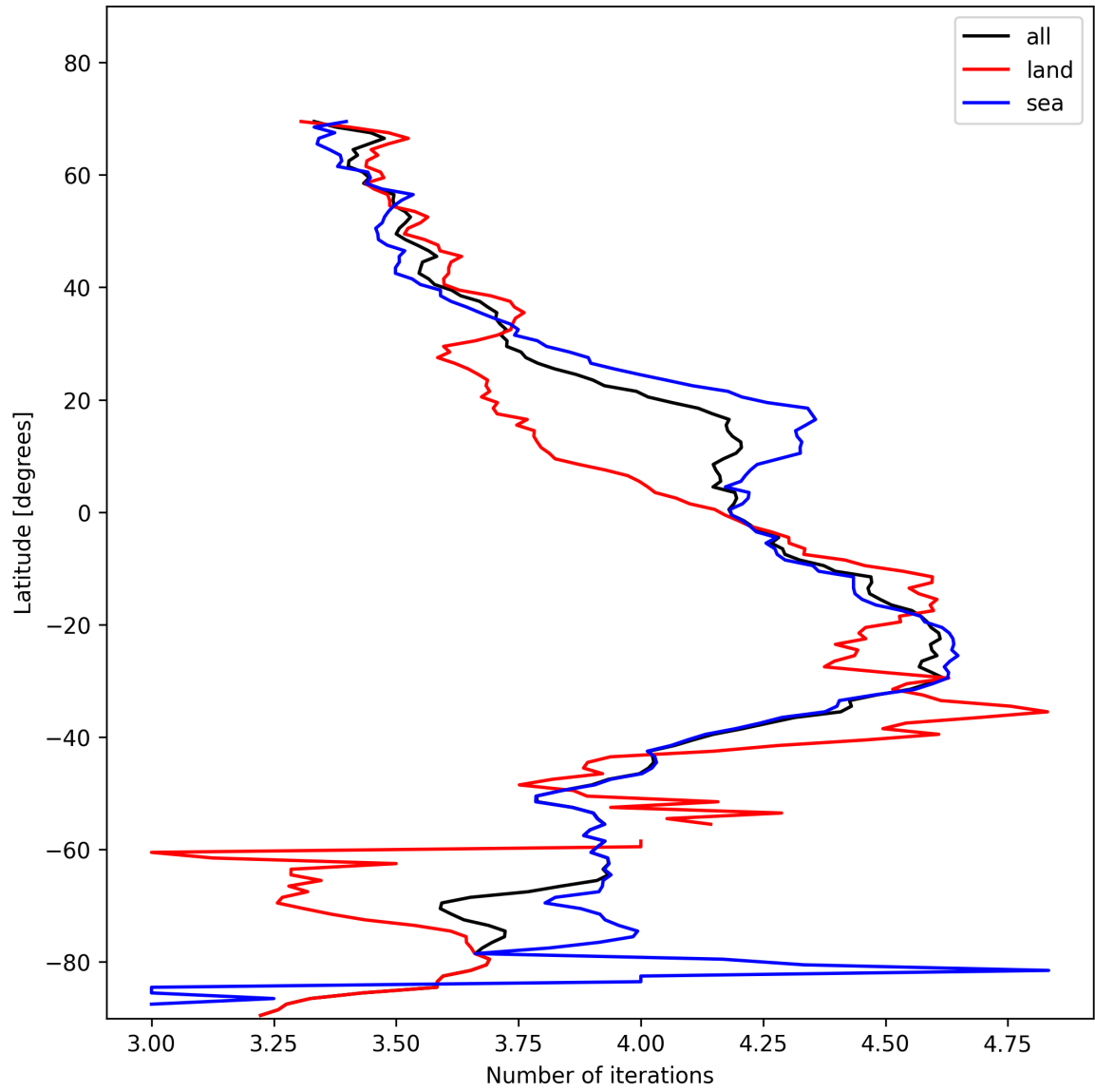
Figure 15: Zonal average of “Number of iterations” for 2025-01-26 to 2025-01-26.
