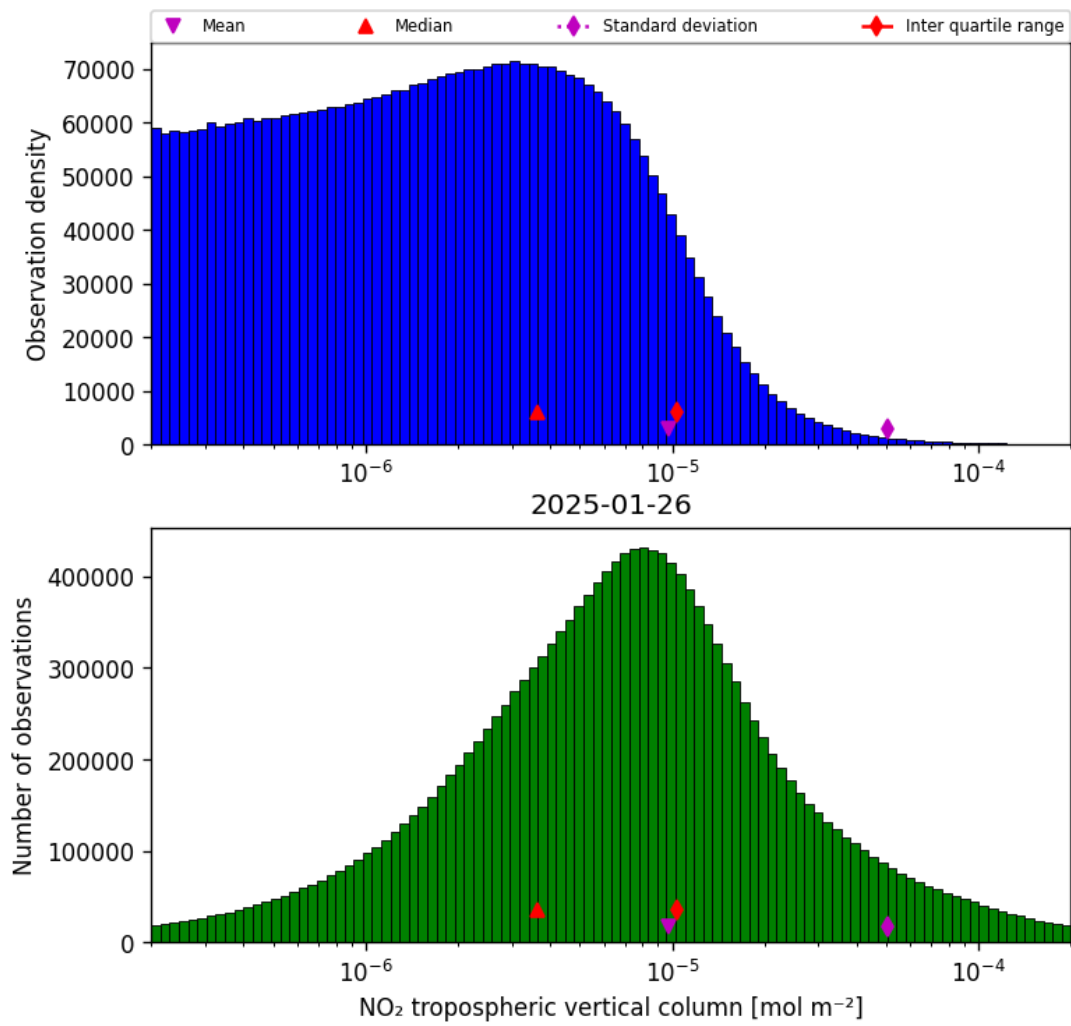
Figure 27: Histogram of “NO 2 tropospheric vertical column” for 2025-01-26 to 2025-01-26
