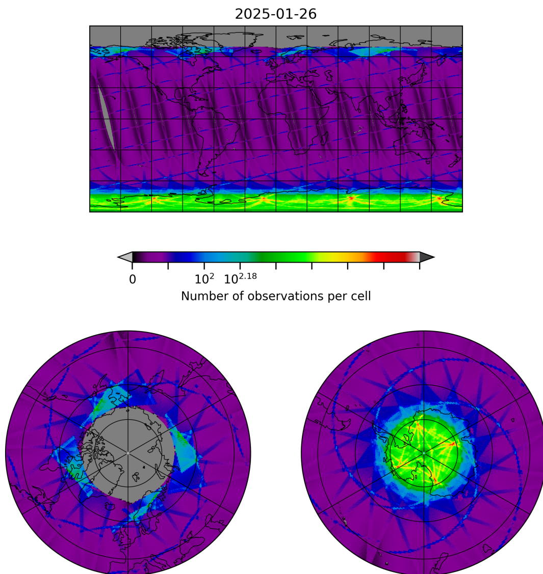
Figure 8: Map of the number of observations for 2025-01-26 to 2025-01-26
