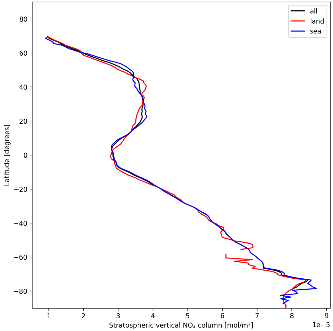
Figure 17: Zonal average of “Stratospheric vertical NO 2 column” for 2025-01-26 to 2025-01-26.
