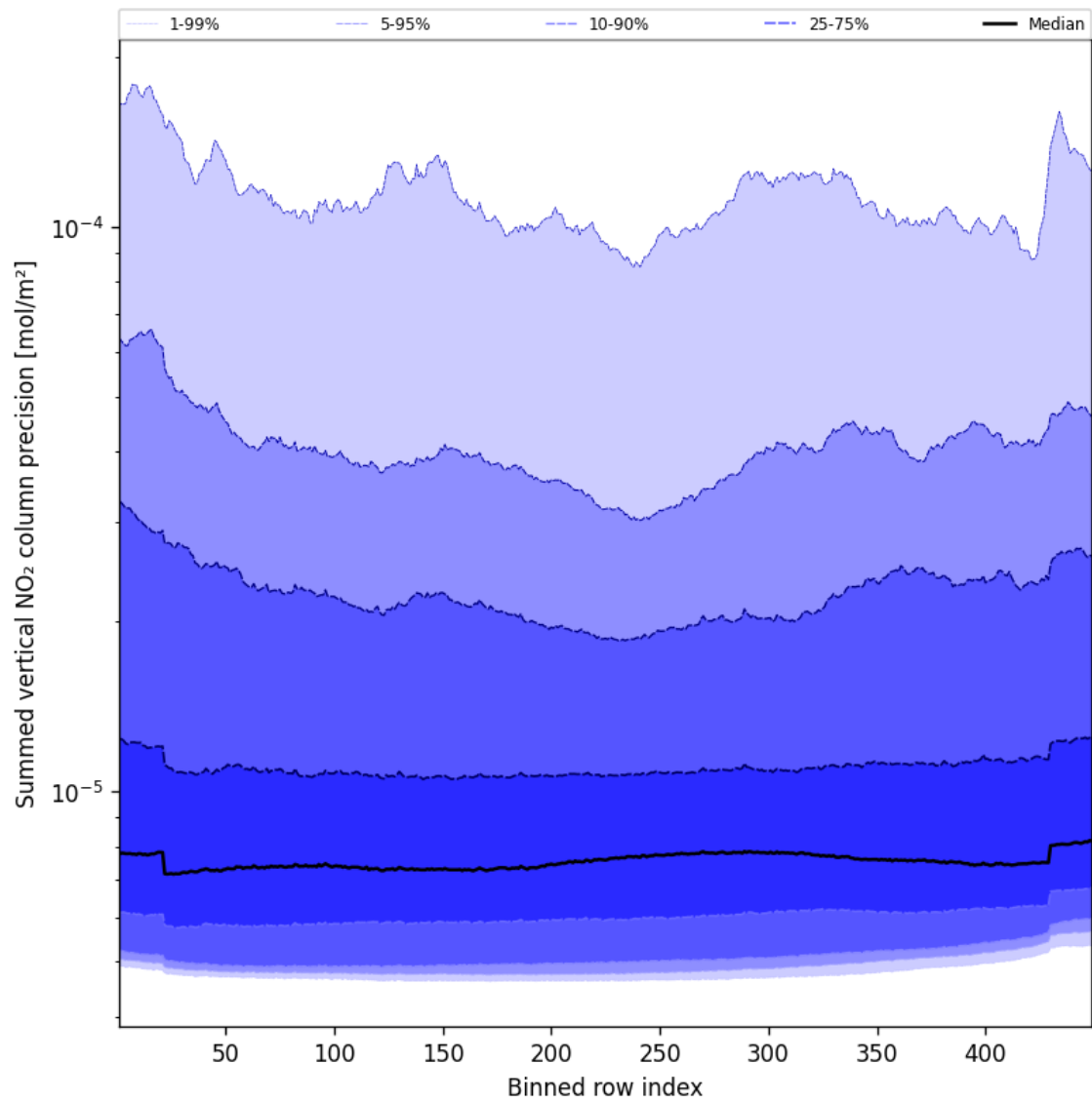
Figure 56: Along track statistics of “Summed vertical NO 2 column precision” for 2025-01-26 to 2025-01-26
