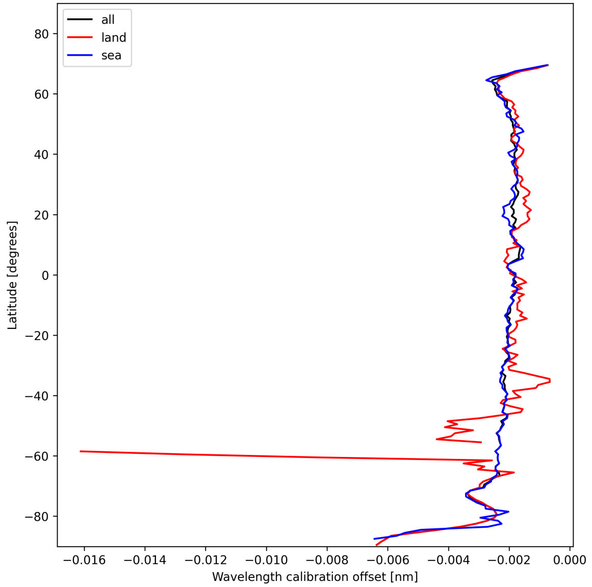
Figure 16: Zonal average of “Wavelength calibration offset” for 2025-01-26 to 2025-01-26.
