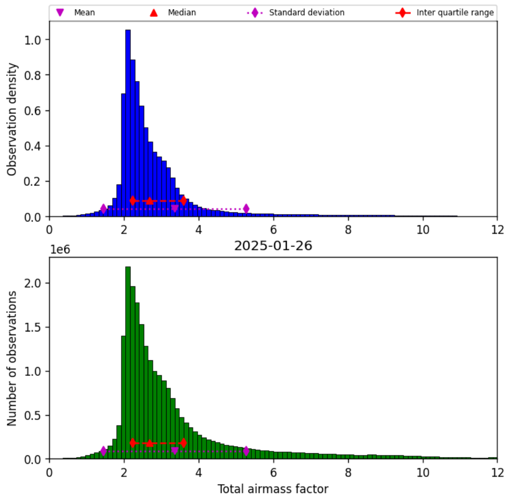
Figure 30: Histogram of “Total airmass factor” for 2025-01-26 to 2025-01-26
