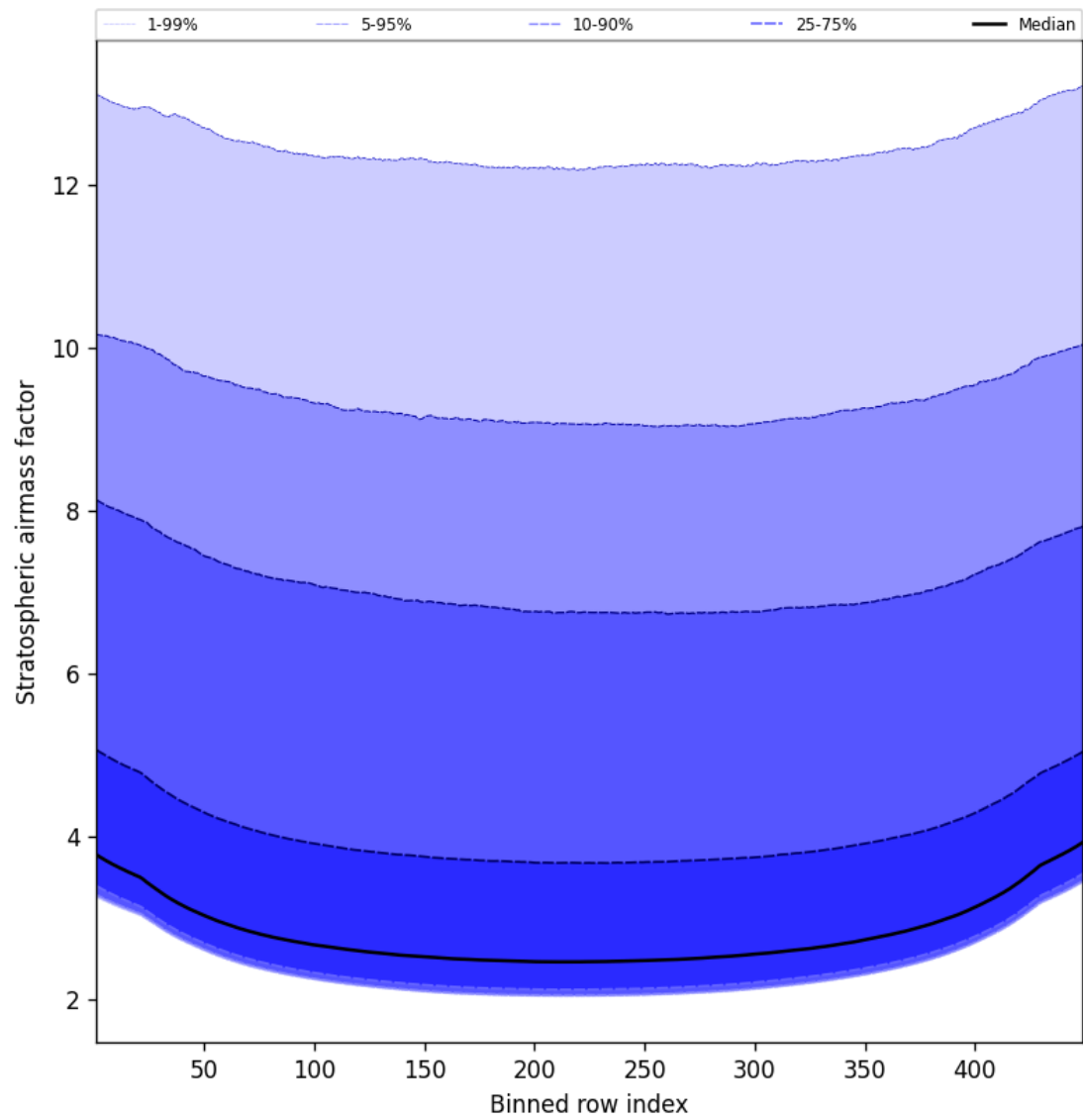
Figure 59: Along track statistics of “Stratospheric airmass factor” for 2025-01-26 to 2025-01-26
