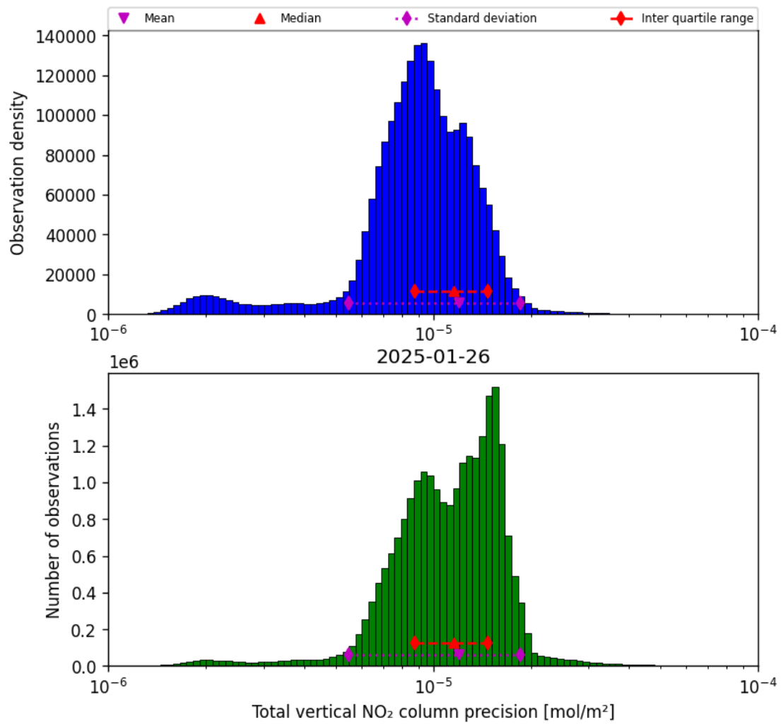
Figure 37: Histogram of "Total vertical NO 2 column precision" for 2025-01-26 to 2025-01-26
