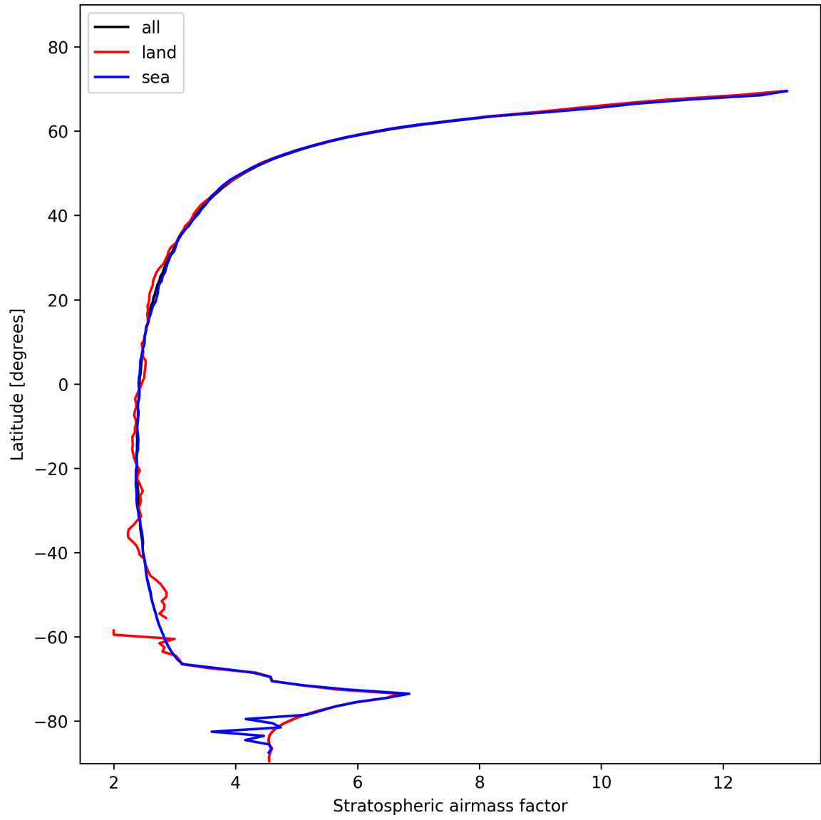
Figure 25: Zonal average of “Stratospheric airmass factor” for 2025-01-26 to 2025-01-26.
