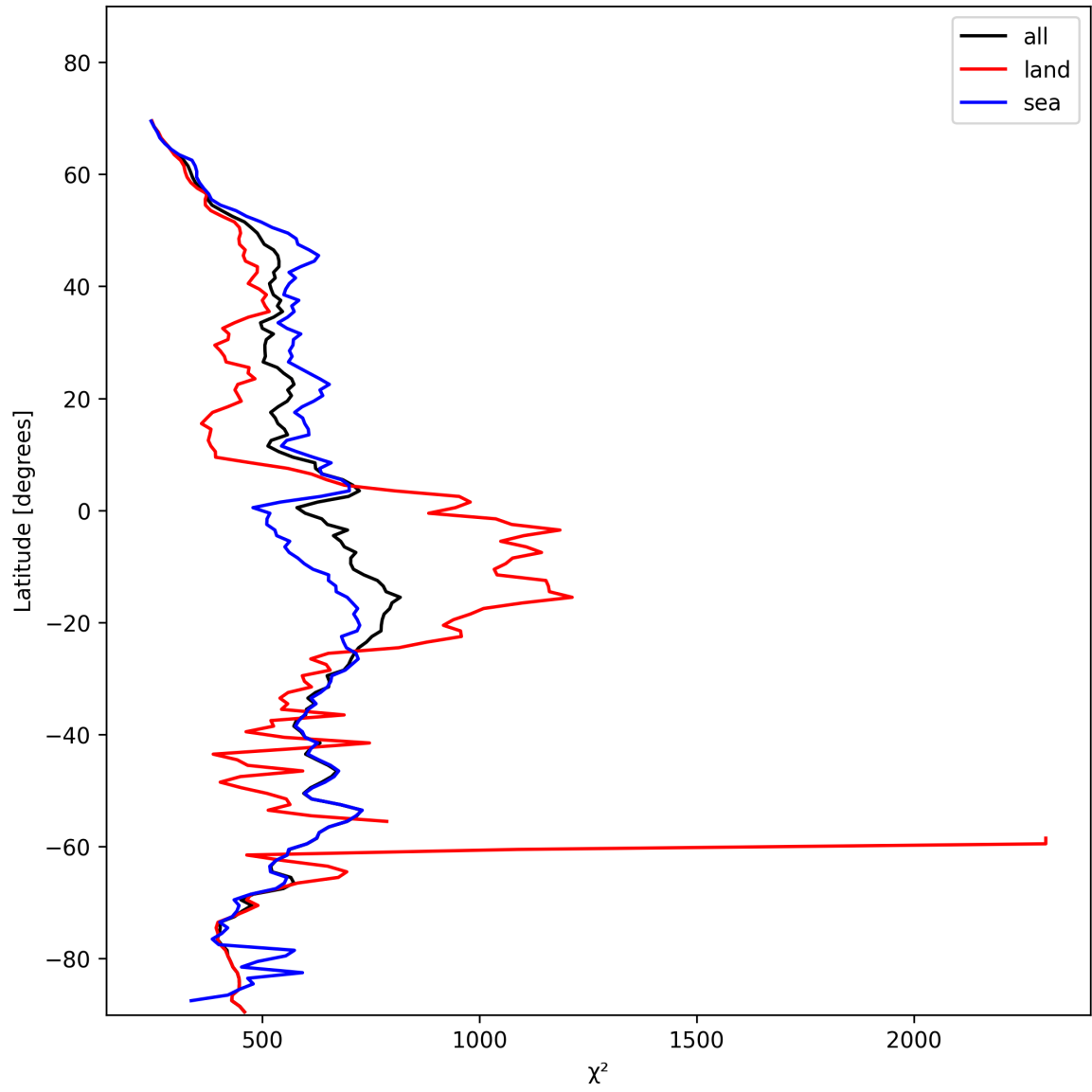
Figure 23: Zonal average of “ \chi^2 ” for 2025-01-26 to 2025-01-26.
