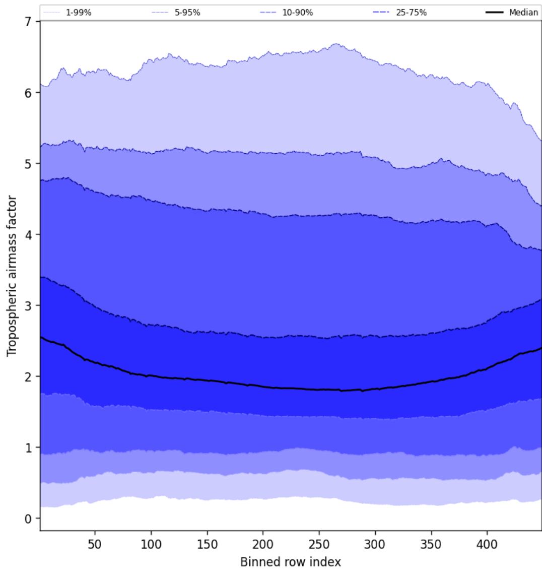
Figure 46: Along track statistics of “Tropospheric airmass factor” for 2025-01-26 to 2025-01-26
