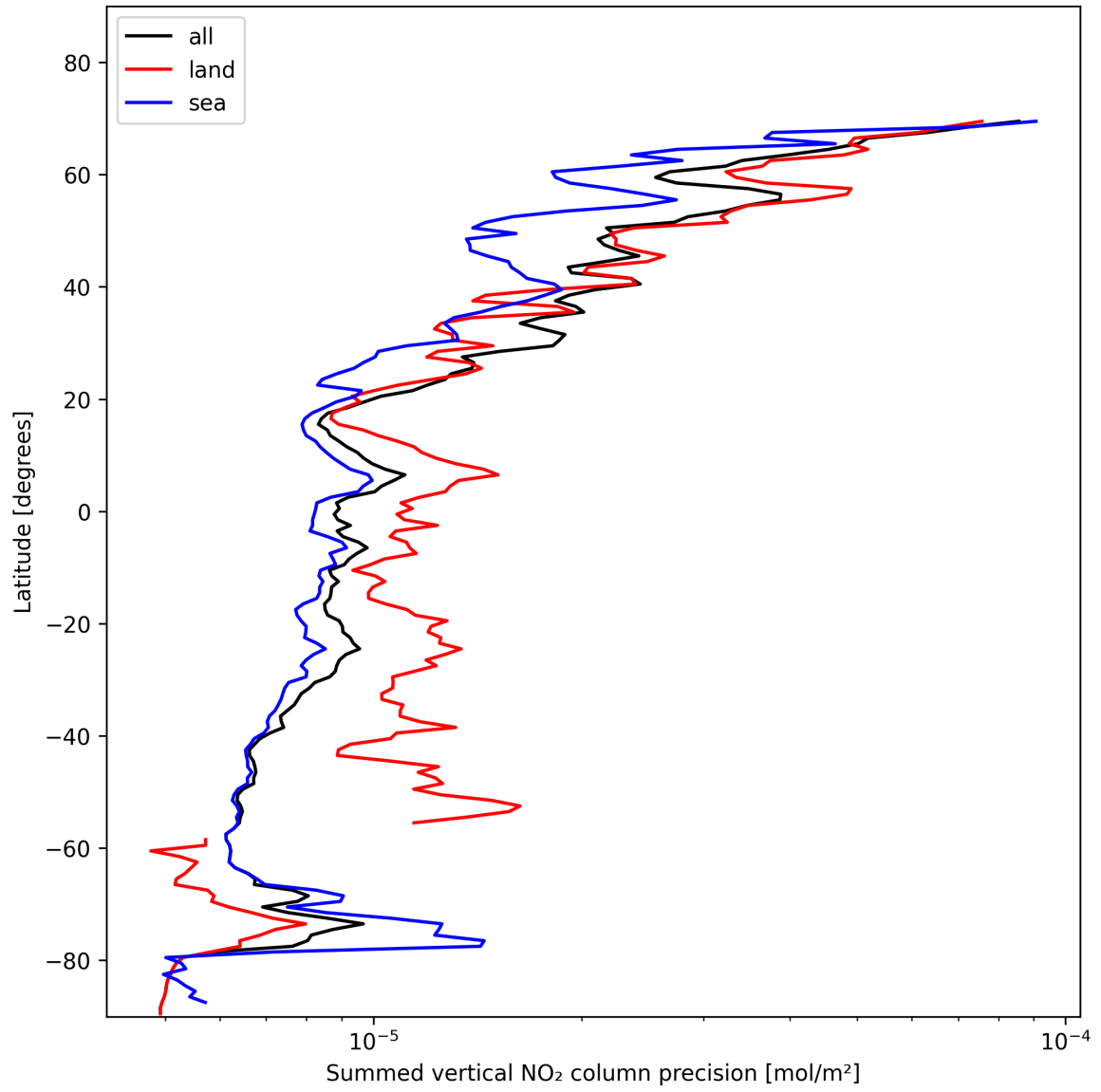
Figure 22: Zonal average of “Summed vertical NO 2 column precision” for 2025-01-26 to 2025-01-26.
