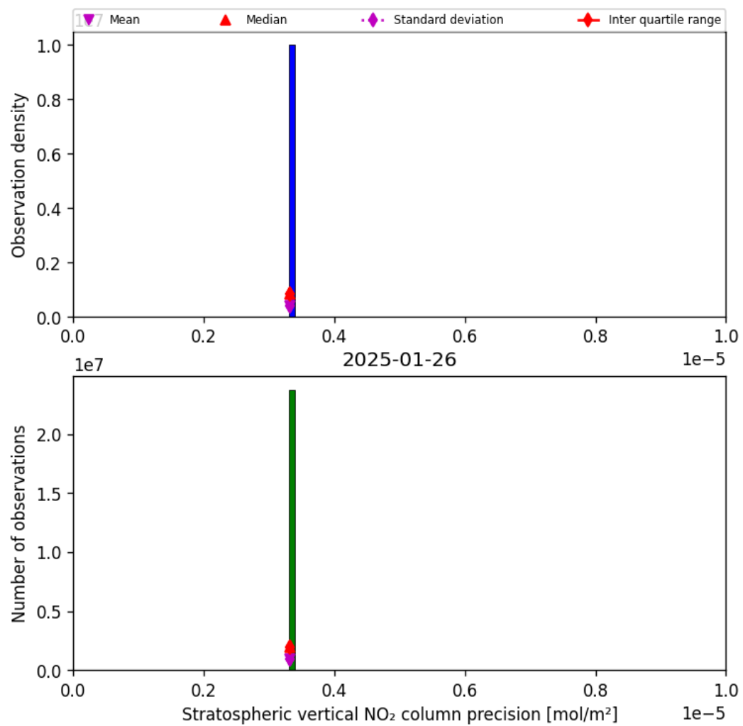
Figure 35: Histogram of “Stratospheric vertical NO 2 column precision” for 2025-01-26 to 2025-01-26
