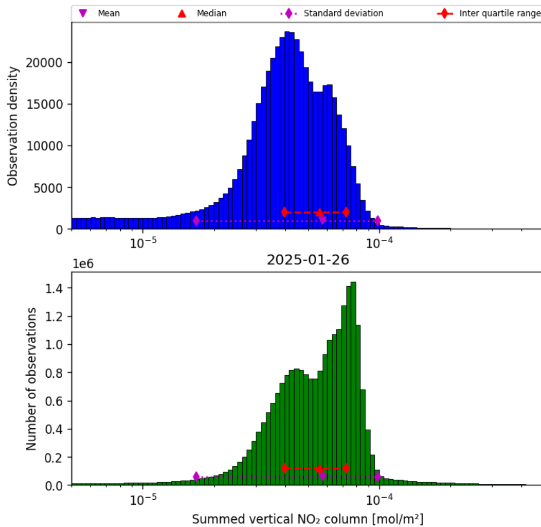
Figure 38: Histogram of “Summed vertical NO 2 column” for 2025-01-26 to 2025-01-26
