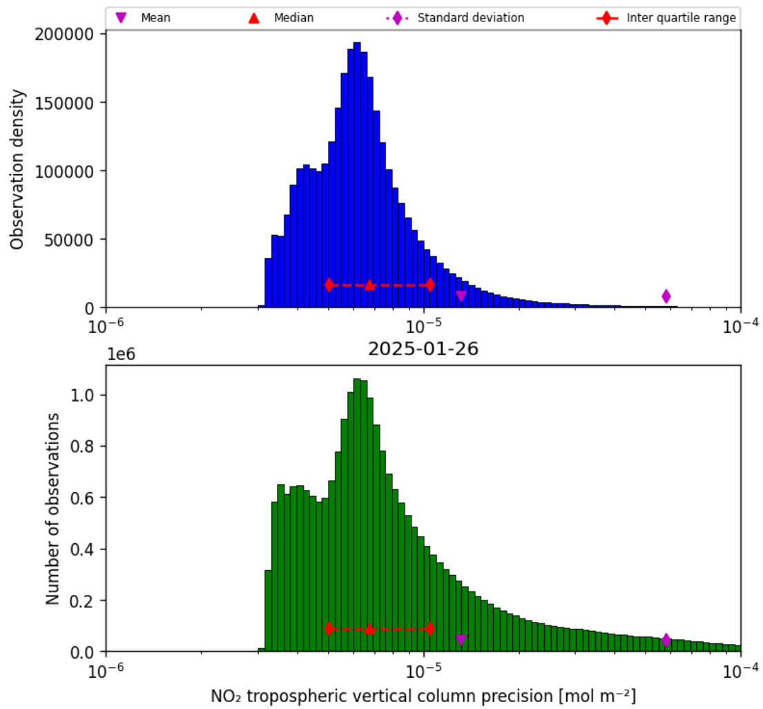
Figure 28: Histogram of "NO 2 tropospheric vertical column precision" for 2025-01-26 to 2025-01-26
