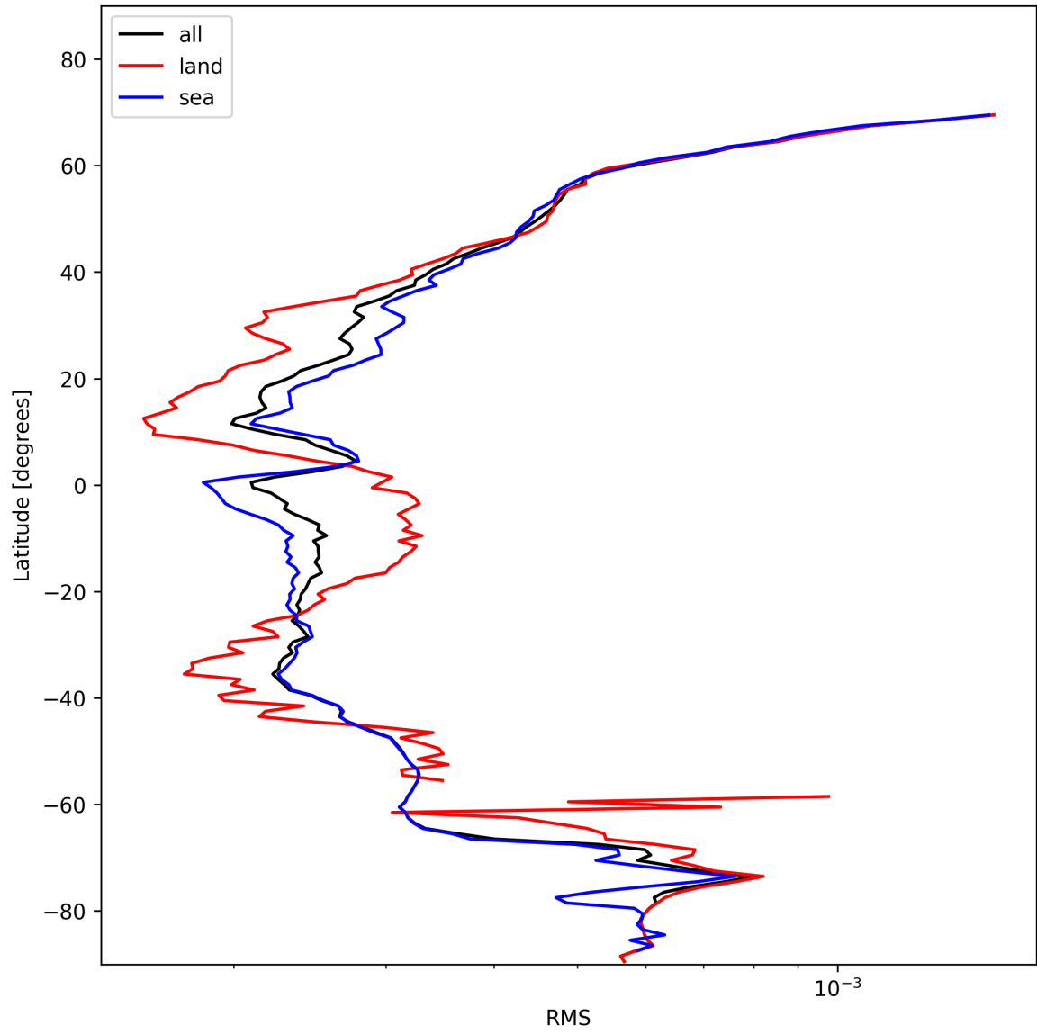
Figure 24: Zonal average of “RMS” for 2025-01-26 to 2025-01-26.
