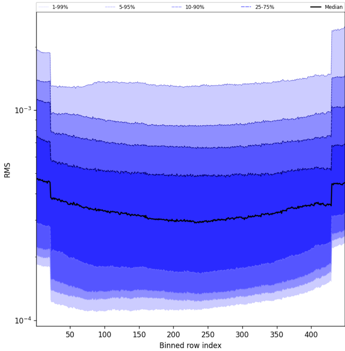
Figure 58: Along track statistics of “RMS” for 2025-01-26 to 2025-01-26
