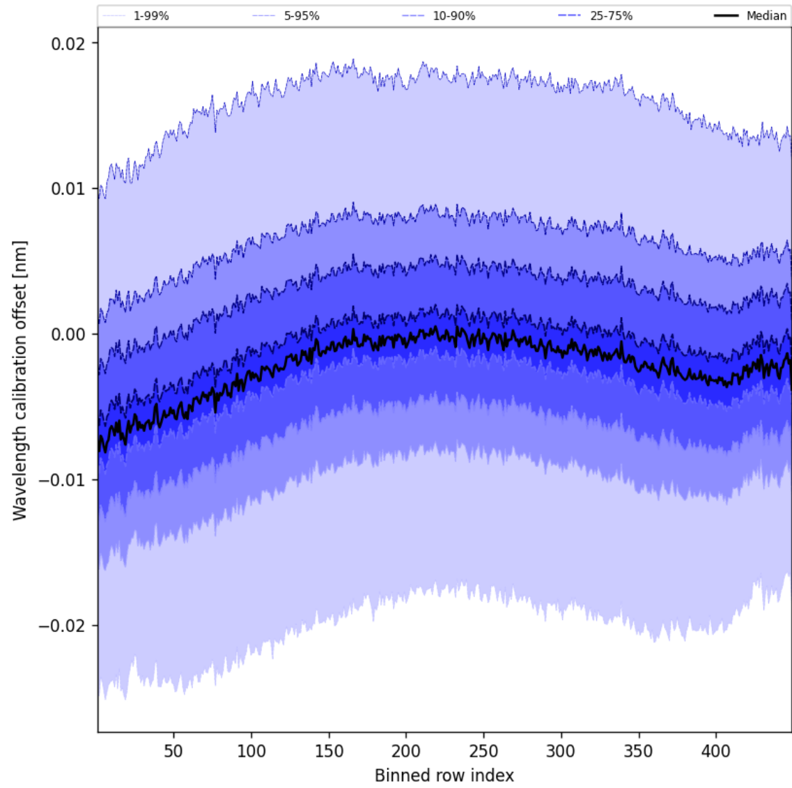
Figure 50: Along track statistics of “Wavelength calibration offset” for 2025-01-26 to 2025-01-26
