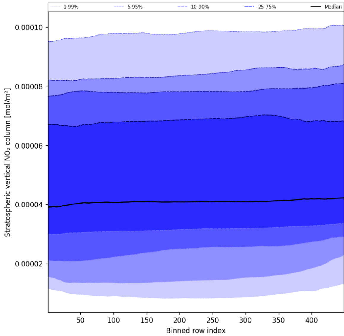
Figure 51: Along track statistics of “Stratospheric vertical NO 2 column” for 2025-01-26 to 2025-01-26
