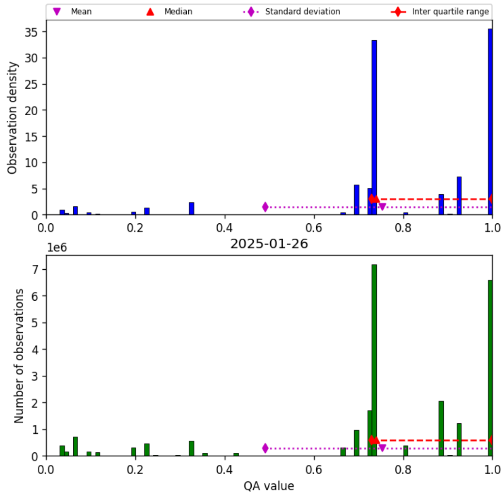
Figure 26: Histogram of “QA value” for 2025-01-26 to 2025-01-26
