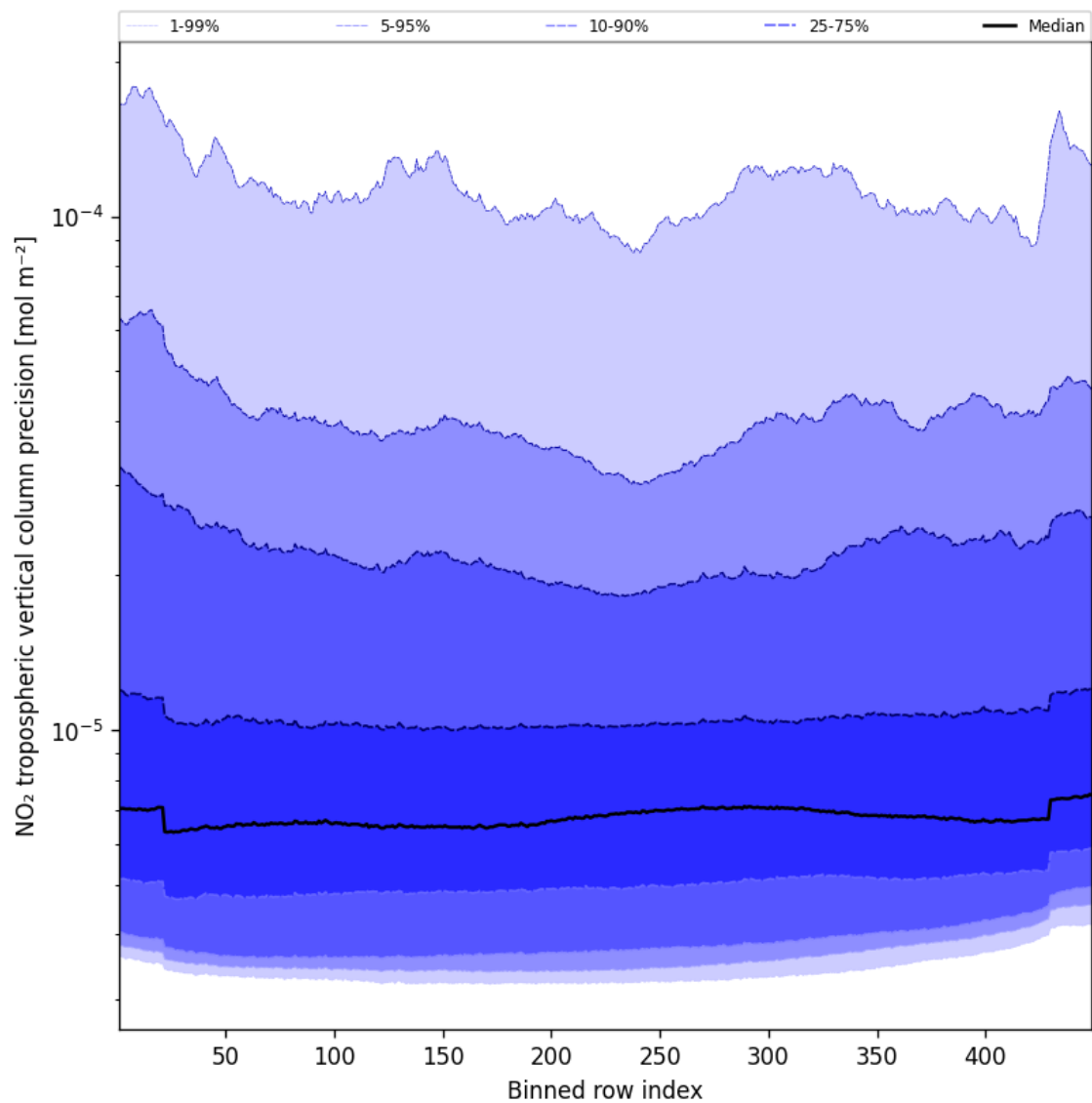
Figure 45: Along track statistics of “NO 2 tropospheric vertical column precision” for 2025-01-26 to 2025-01-26
