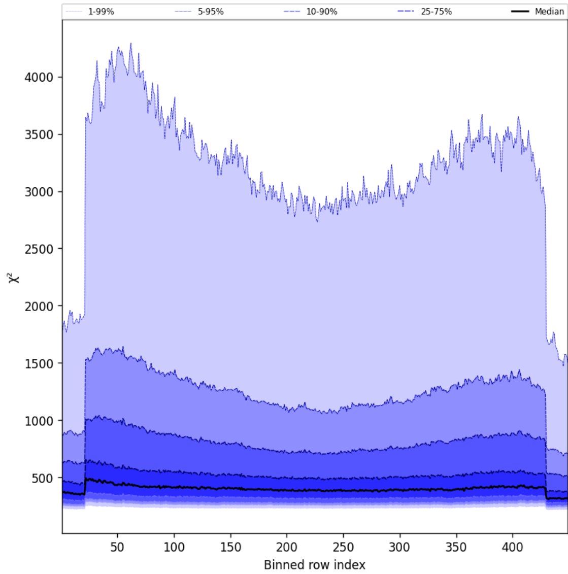
Figure 57: Along track statistics of “ \chi^2 ” for 2025-01-26 to 2025-01-26
