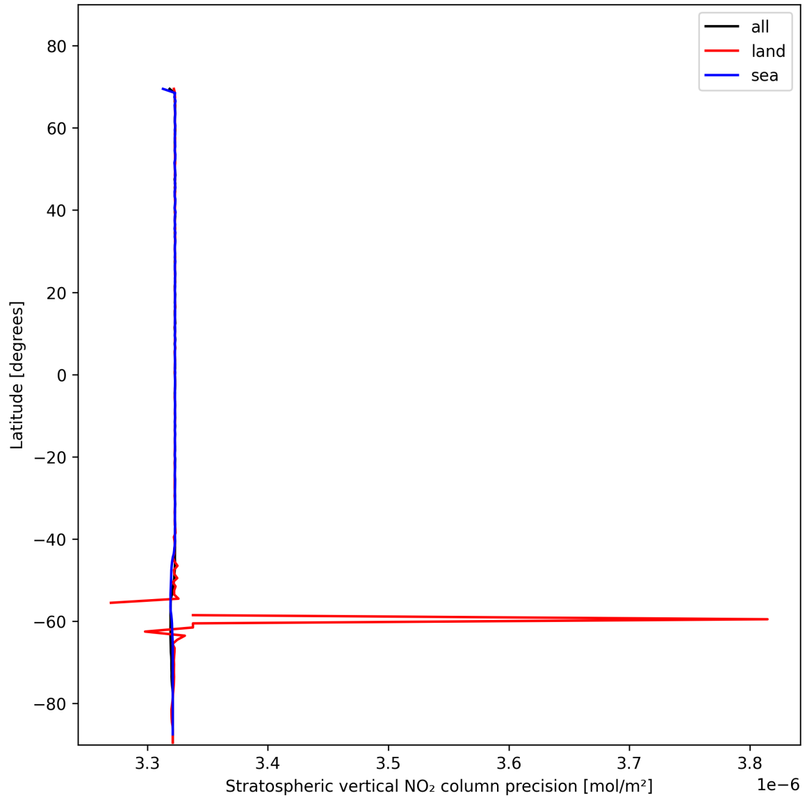
Figure 18: Zonal average of “Stratospheric vertical NO 2 column precision” for 2025-01-26 to 2025-01-26.
