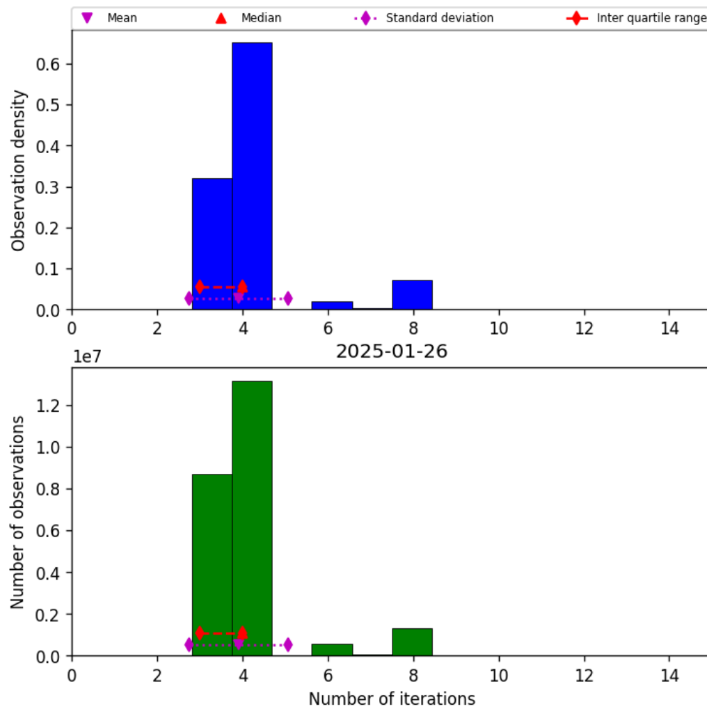
Figure 32: Histogram of “Number of iterations” for 2025-01-26 to 2025-01-26
