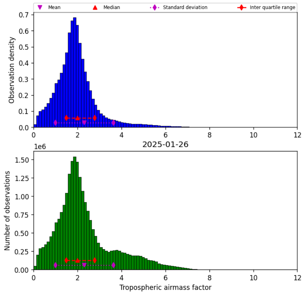
Figure 29: Histogram of “Tropospheric airmass factor” for 2025-01-26 to 2025-01-26
