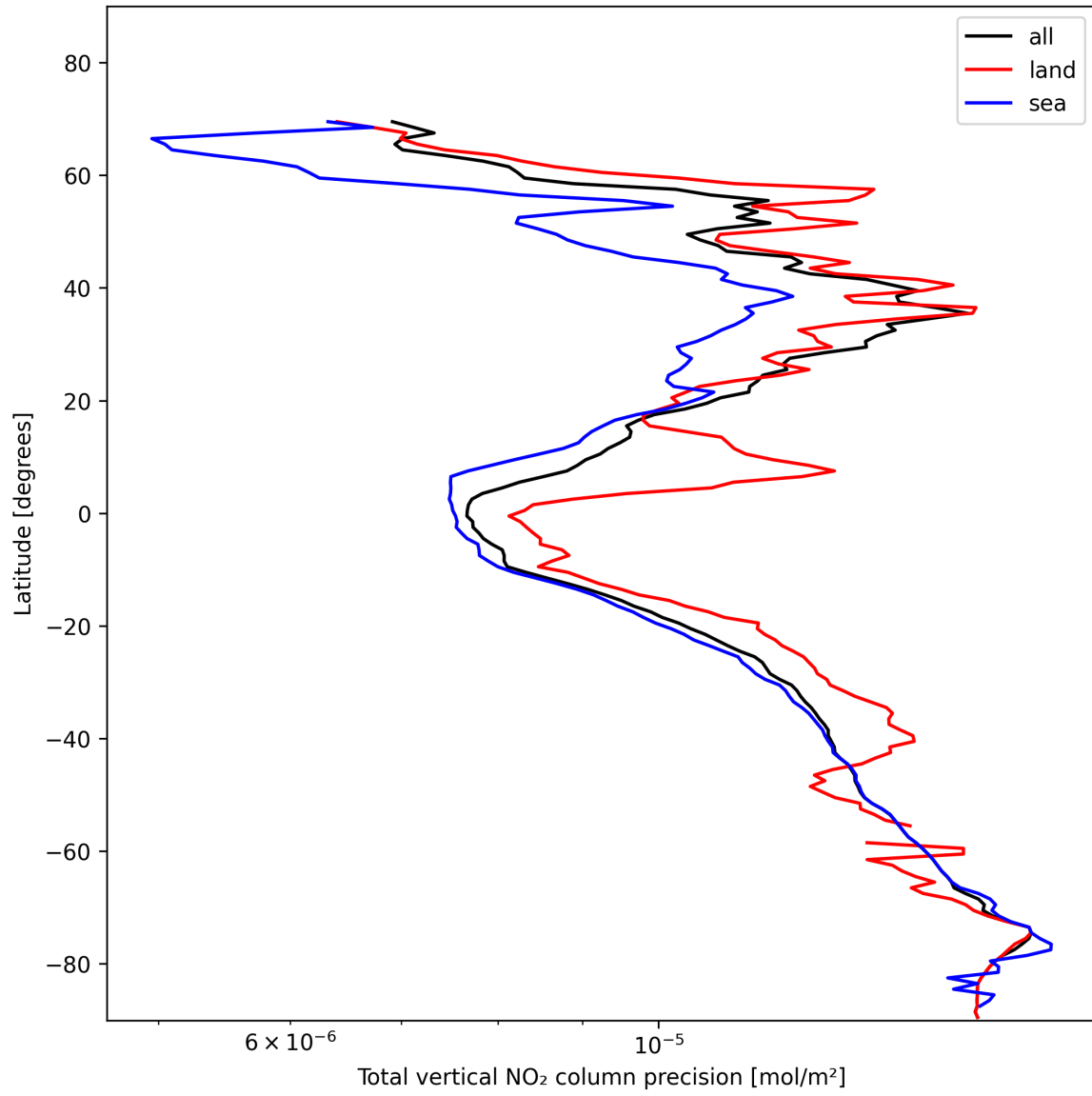
Figure 20: Zonal average of “Total vertical NO 2 column precision” for 2025-01-26 to 2025-01-26.
