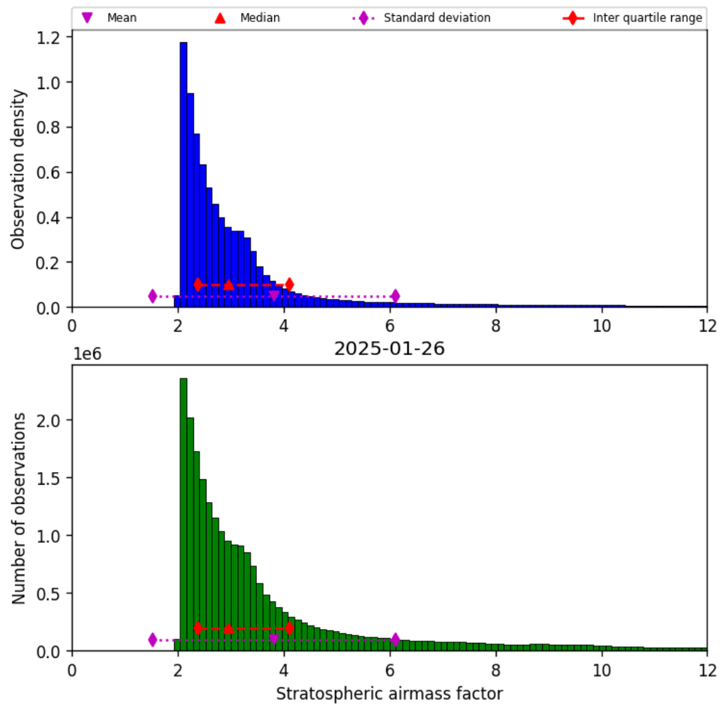
Figure 42: Histogram of “Stratospheric airmass factor” for 2025-01-26 to 2025-01-26
