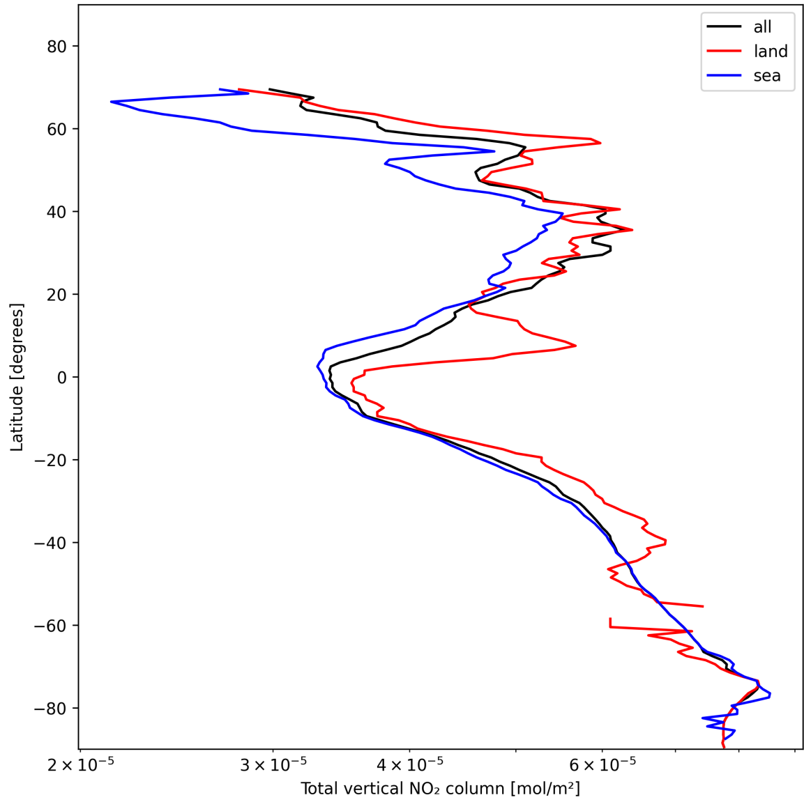
Figure 19: Zonal average of “Total vertical NO 2 column” for 2025-01-26 to 2025-01-26.
