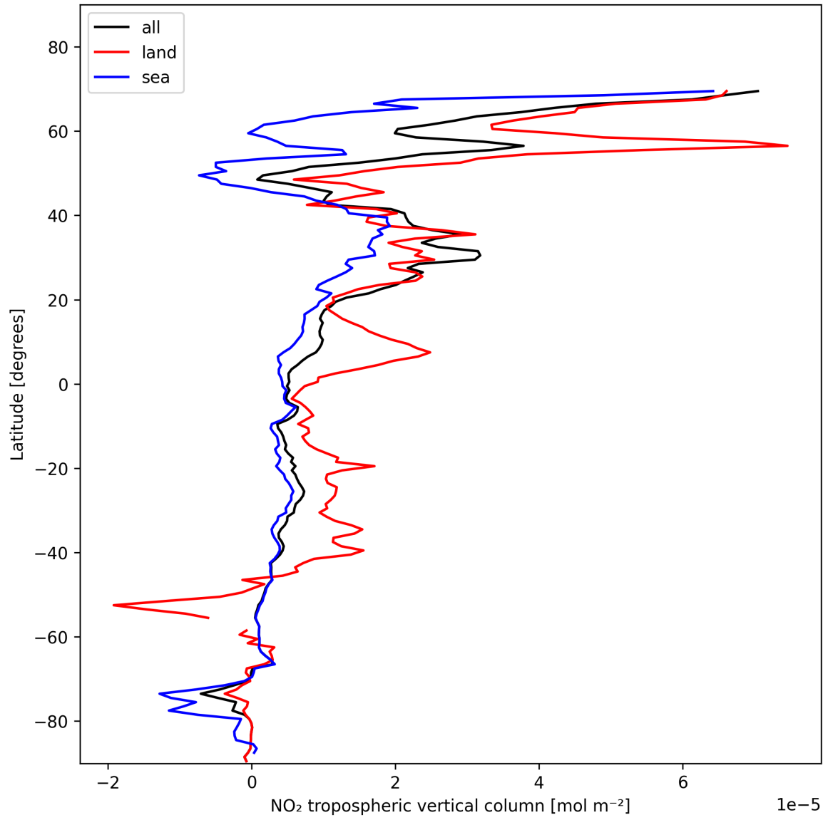
Figure 10: Zonal average of “NO 2 tropospheric vertical column” for 2025-01-26 to 2025-01-26.
