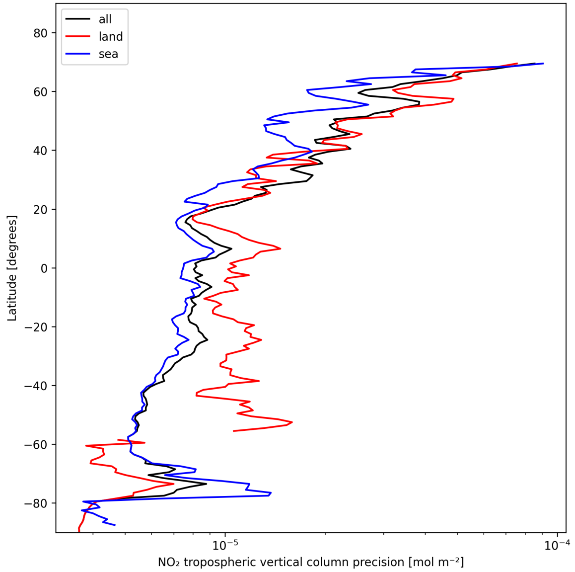
Figure 11: Zonal average of “NO 2 tropospheric vertical column precision” for 2025-01-26 to 2025-01-26.
