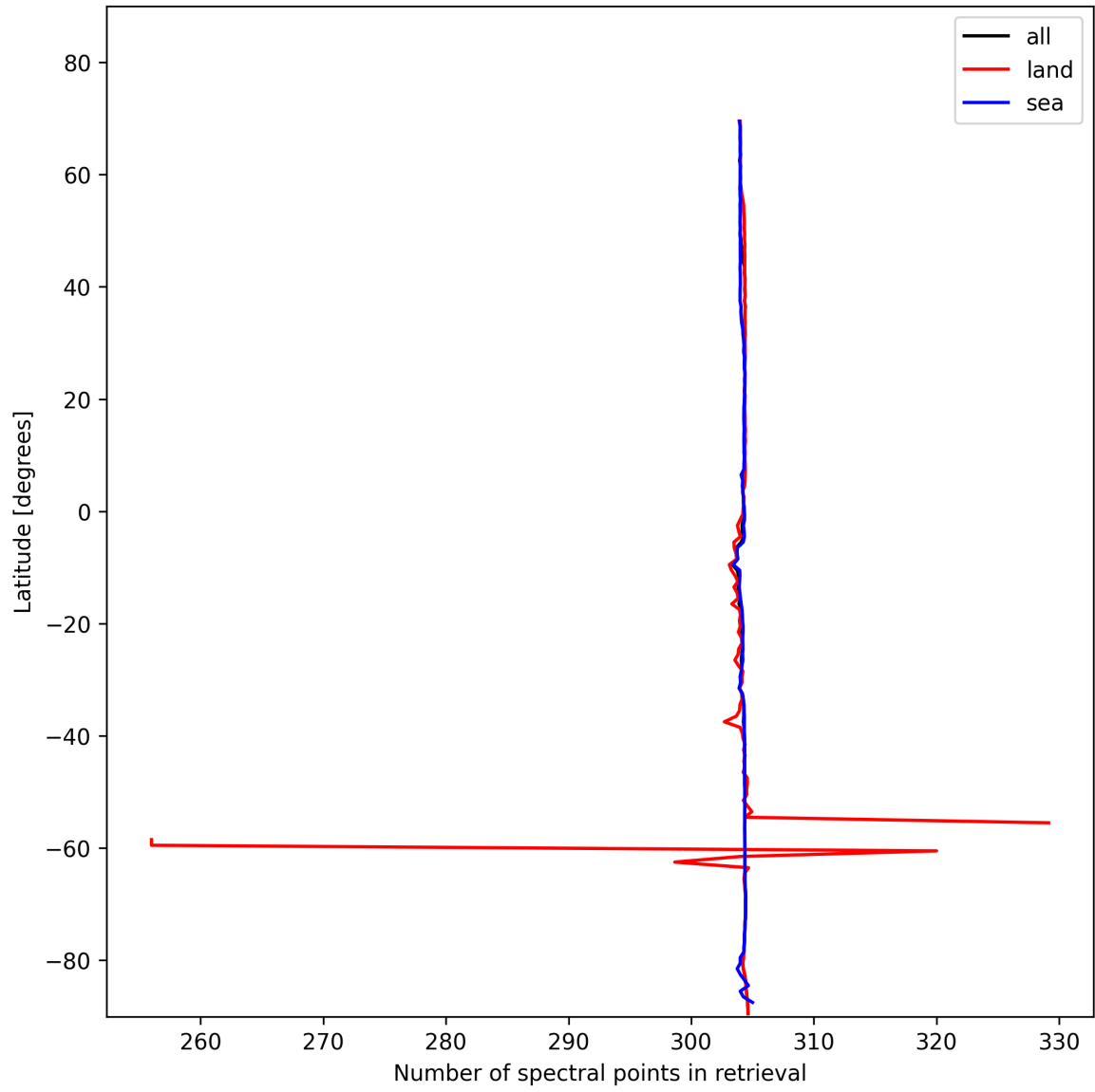
Figure 14: Zonal average of “Number of spectral points in retrieval” for 2025-01-26 to 2025-01-26.
