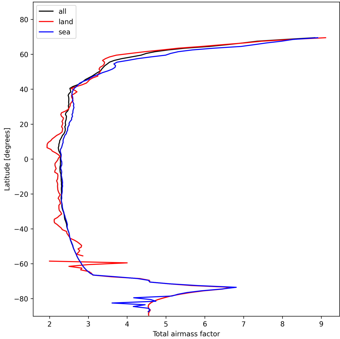
Figure 13: Zonal average of “Total airmass factor” for 2025-01-26 to 2025-01-26.
