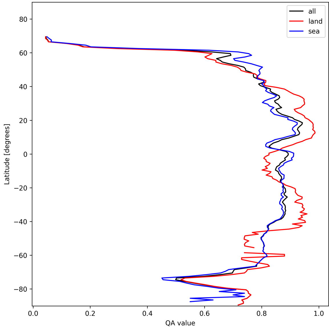
Figure 9: Zonal average of “QA value” for 2025-01-26 to 2025-01-26.
