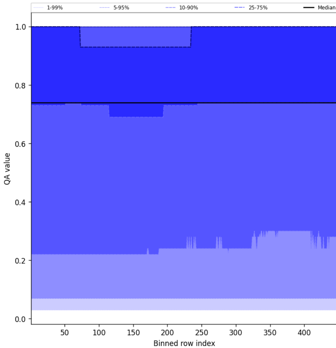
Figure 43: Along track statistics of “QA value” for 2025-01-26 to 2025-01-26
