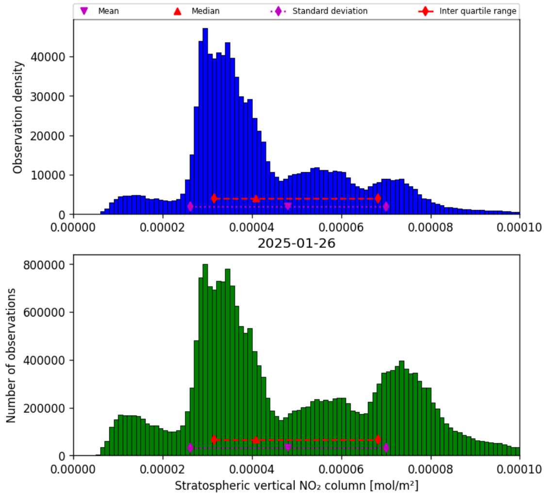
Figure 34: Histogram of “Stratospheric vertical NO 2 column” for 2025-01-26 to 2025-01-26
