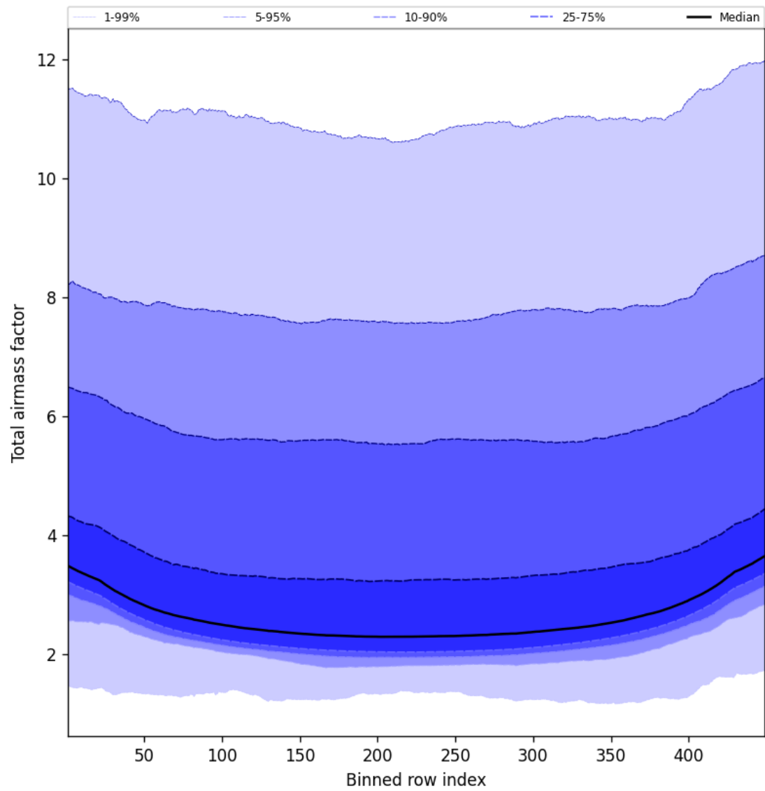
Figure 47: Along track statistics of “Total airmass factor” for 2025-01-26 to 2025-01-26
