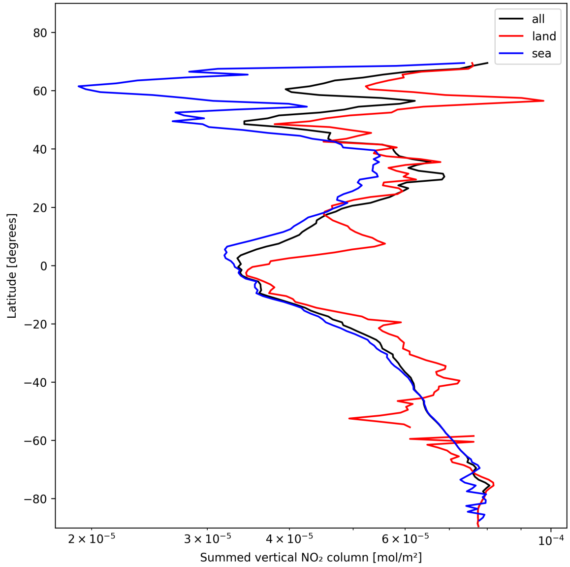
Figure 21: Zonal average of “Summed vertical NO 2 column” for 2025-01-26 to 2025-01-26.
