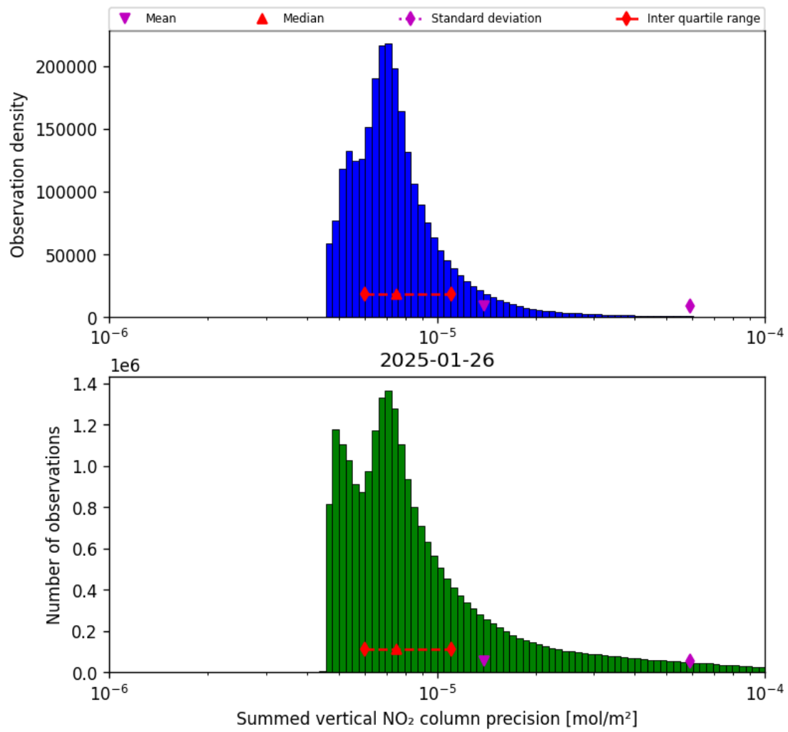
Figure 39: Histogram of "Summed vertical NO 2 column precision" for 2025-01-26 to 2025-01-26
