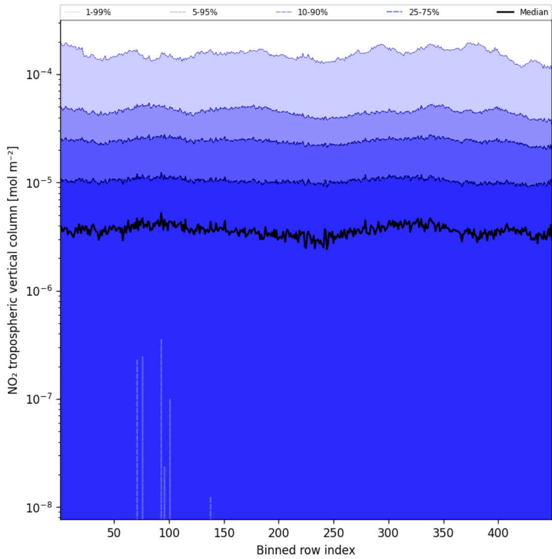
Figure 44: Along track statistics of “NO 2 tropospheric vertical column” for 2025-01-26 to 2025-01-26
