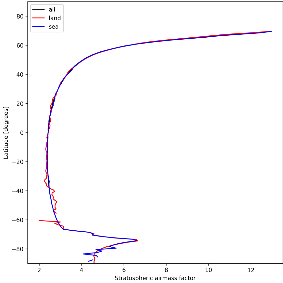
Figure 25: Zonal average of “Stratospheric airmass factor” for 2025-01-27 to 2025-01-28.
