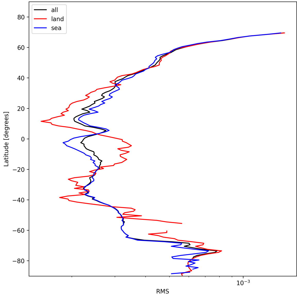
Figure 24: Zonal average of “RMS” for 2025-01-27 to 2025-01-28.
