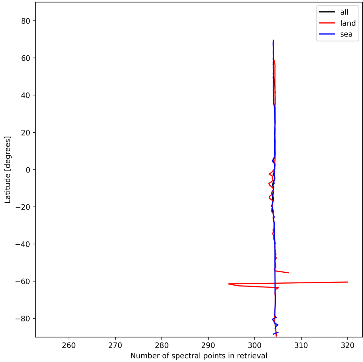
Figure 14: Zonal average of “Number of spectral points in retrieval” for 2025-01-27 to 2025-01-28.
