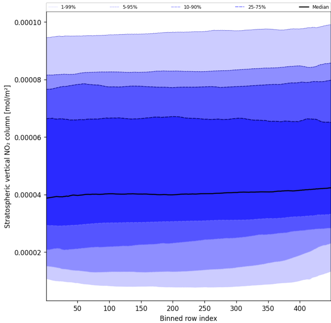
Figure 51: Along track statistics of “Stratospheric vertical NO 2 column” for 2025-01-27 to 2025-01-28
