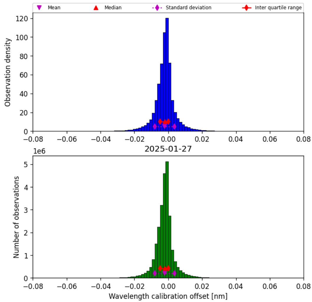
Figure 33: Histogram of “Wavelength calibration offset” for 2025-01-27 to 2025-01-28
