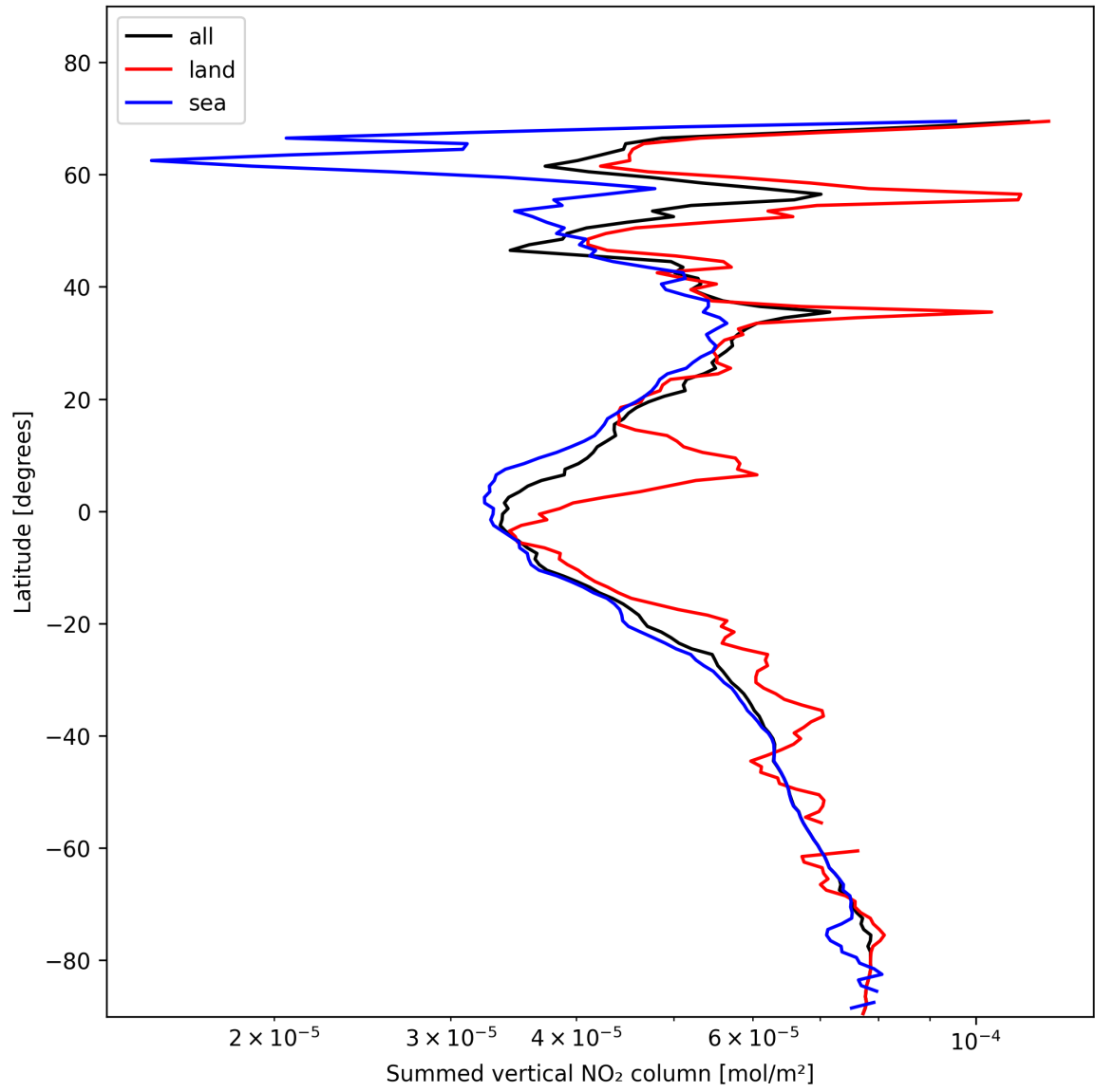
Figure 21: Zonal average of “Summed vertical NO 2 column” for 2025-01-27 to 2025-01-28.
