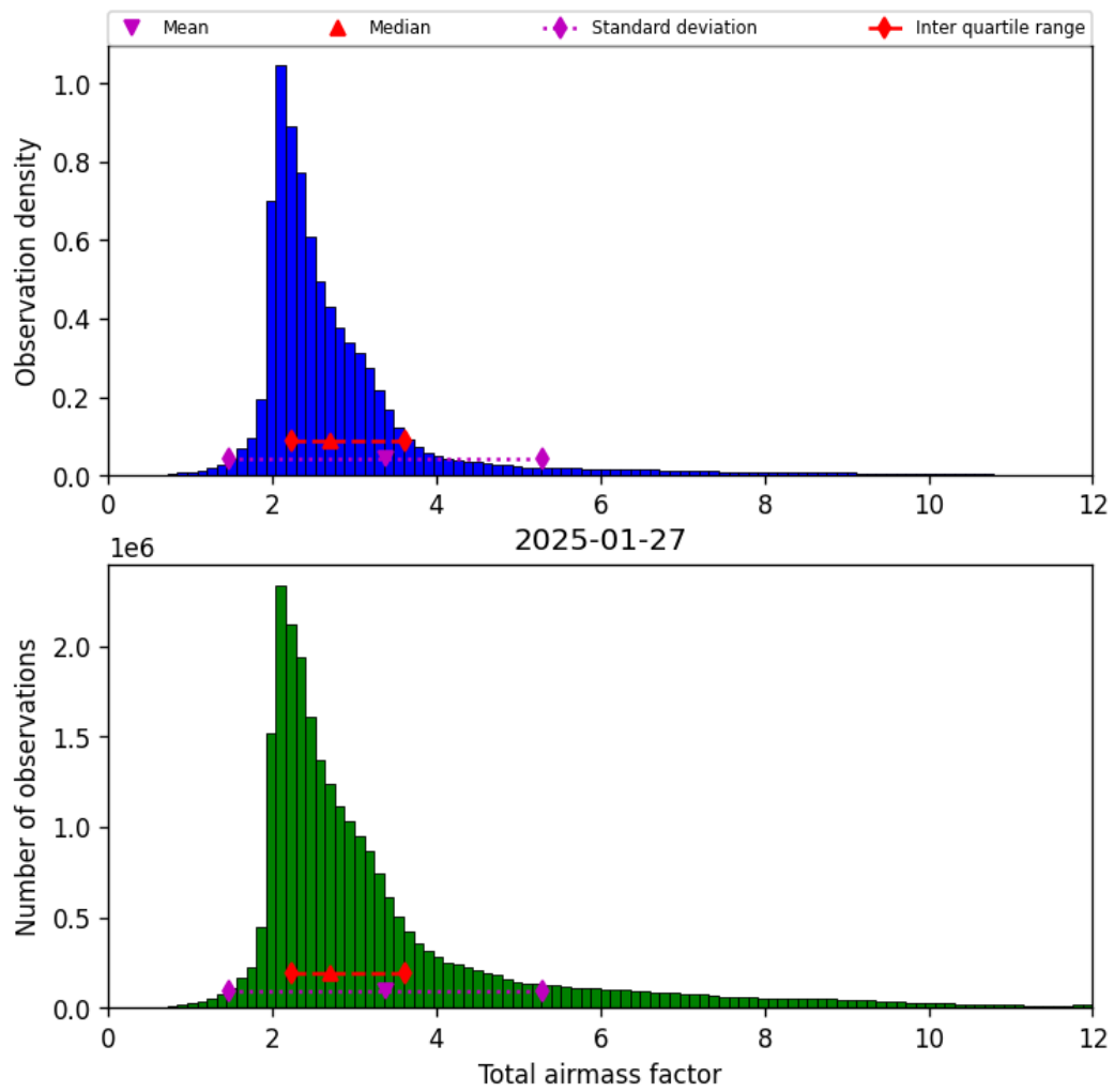
Figure 30: Histogram of “Total airmass factor” for 2025-01-27 to 2025-01-28
