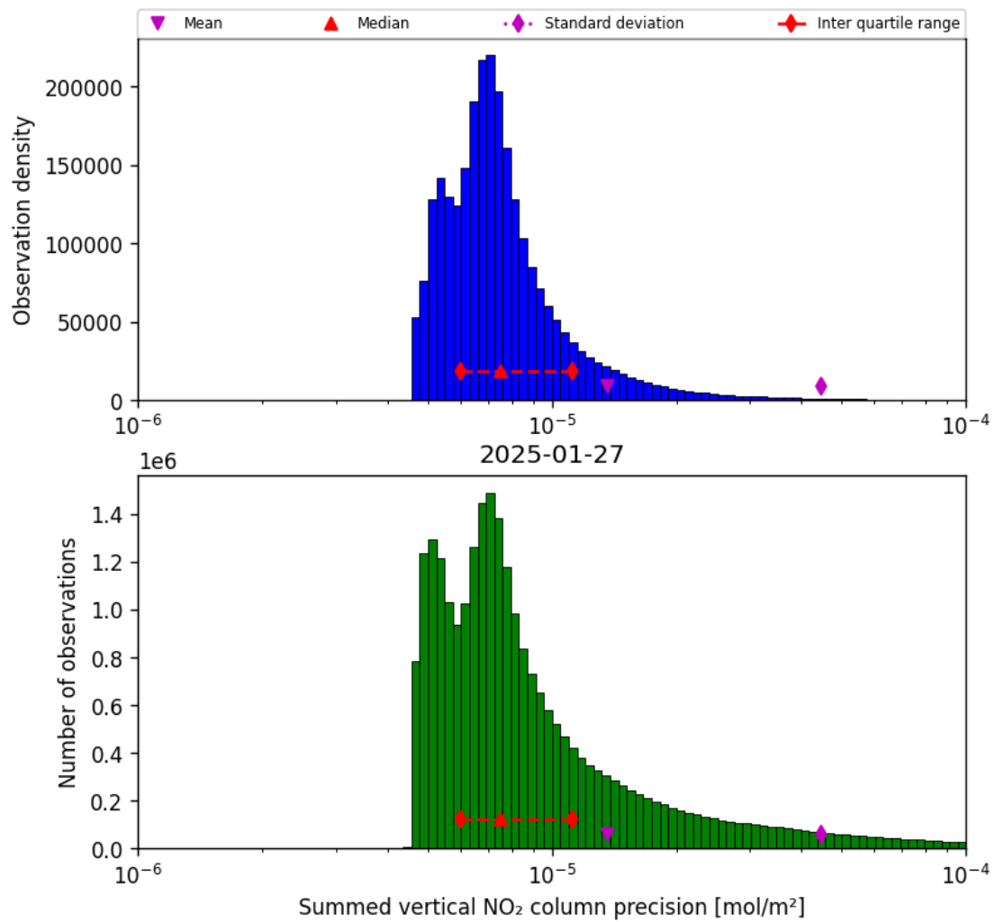
Figure 39: Histogram of “Summed vertical NO 2 column precision” for 2025-01-27 to 2025-01-28
