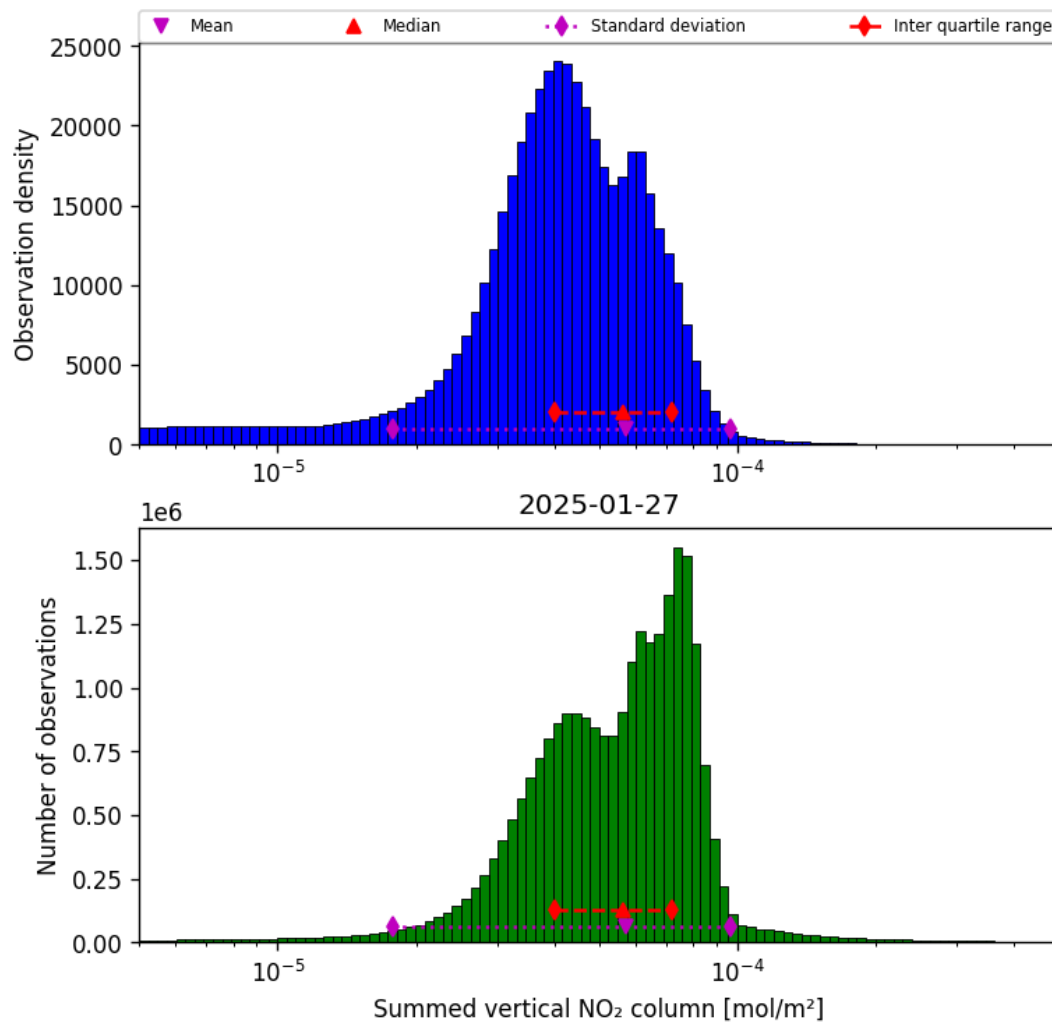
Figure 38: Histogram of “Summed vertical NO 2 column” for 2025-01-27 to 2025-01-28
