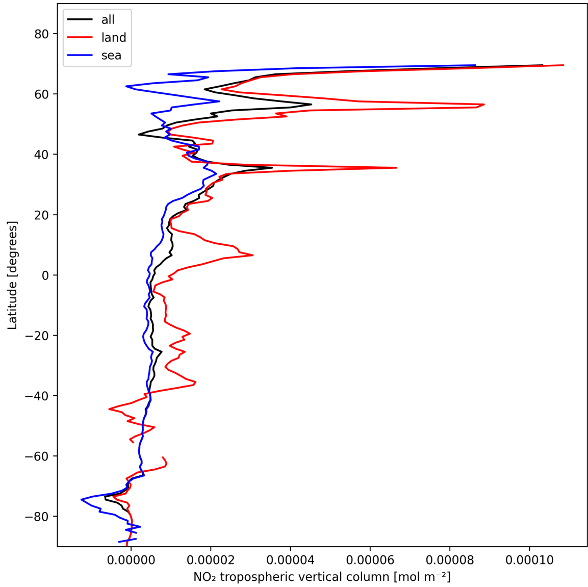
Figure 10: Zonal average of “NO 2 tropospheric vertical column” for 2025-01-27 to 2025-01-28.
