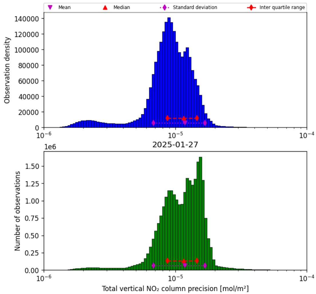
Figure 37: Histogram of “Total vertical NO 2 column precision” for 2025-01-27 to 2025-01-28
