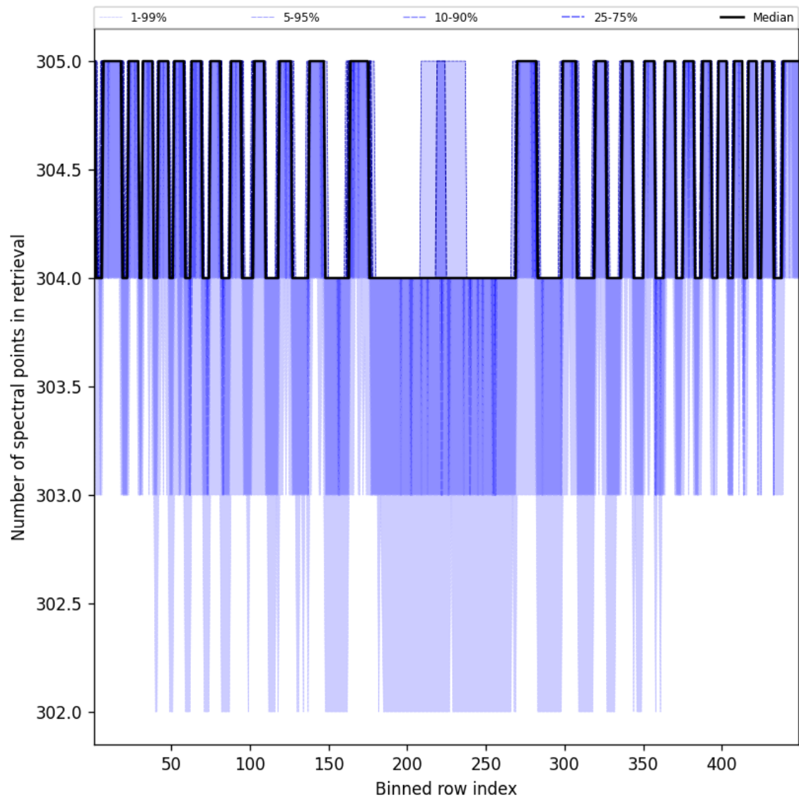
Figure 48: Along track statistics of “Number of spectral points in retrieval” for 2025-01-27 to 2025-01-28
