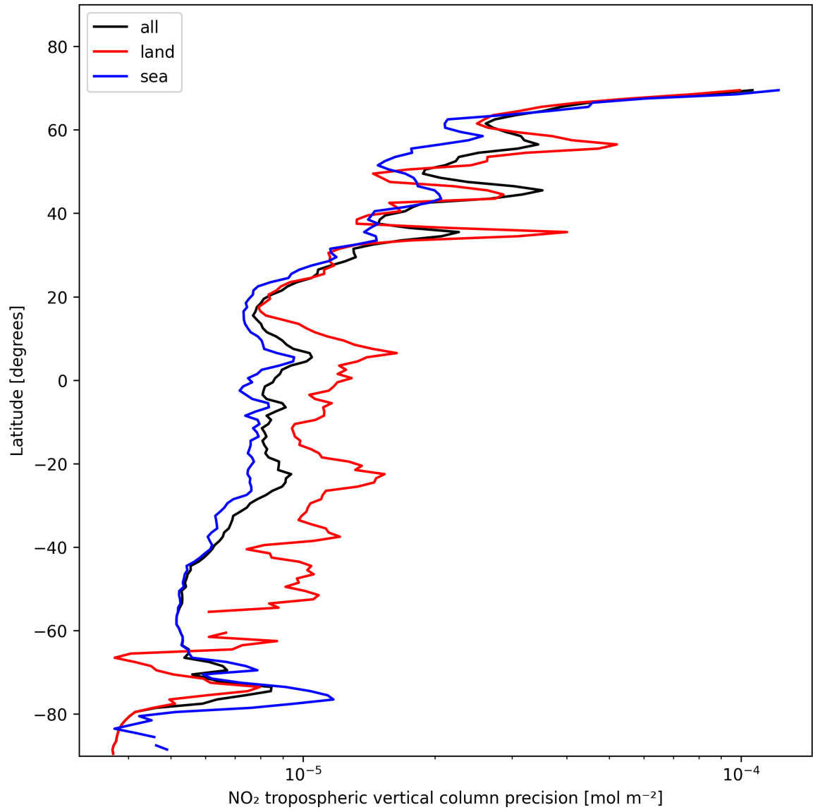
Figure 11: Zonal average of “NO 2 tropospheric vertical column precision” for 2025-01-27 to 2025-01-28.
