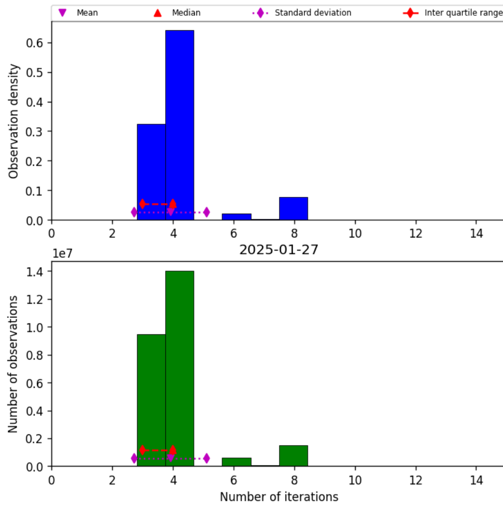
Figure 32: Histogram of “Number of iterations” for 2025-01-27 to 2025-01-28
