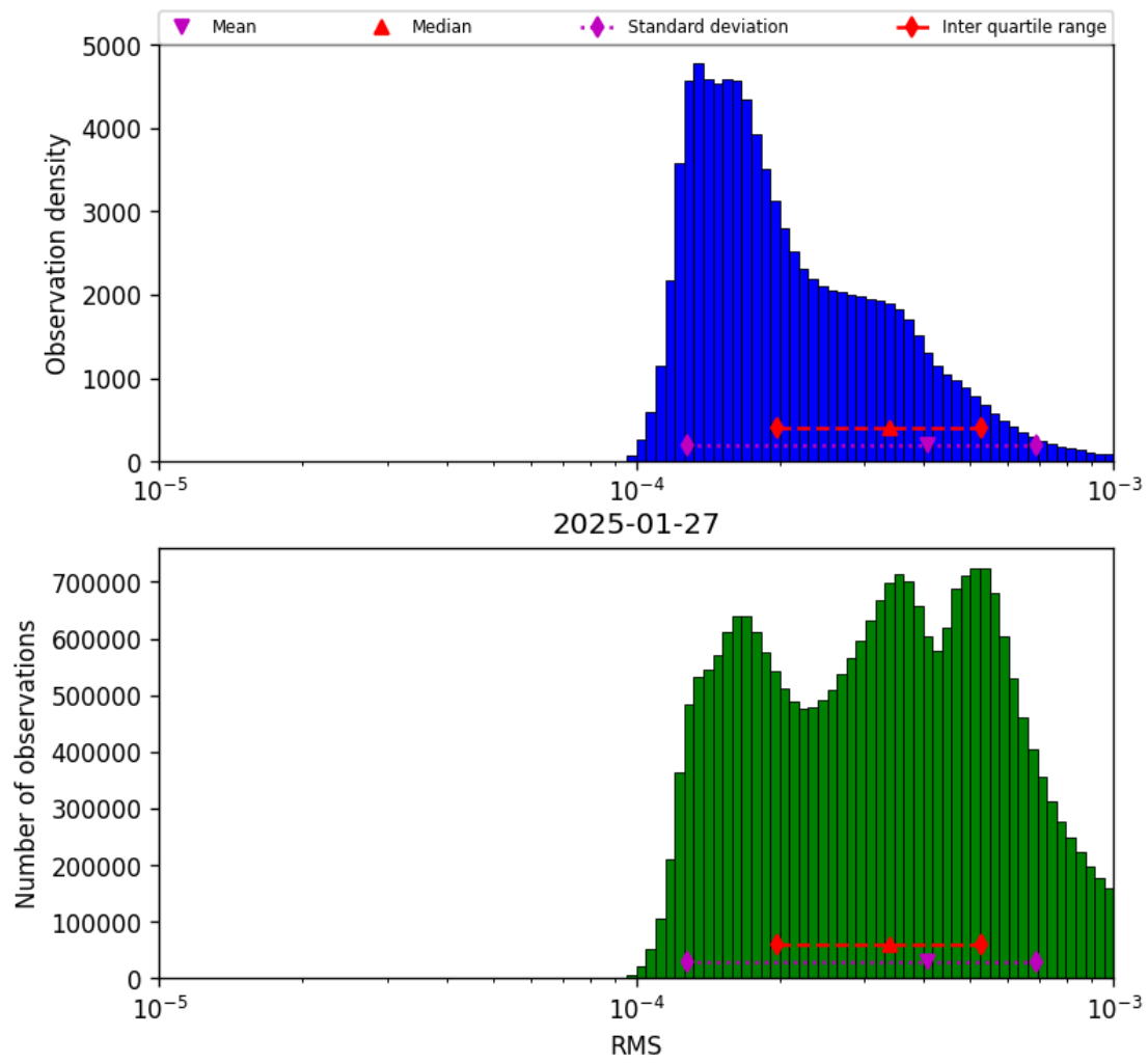
Figure 41: Histogram of “RMS” for 2025-01-27 to 2025-01-28
