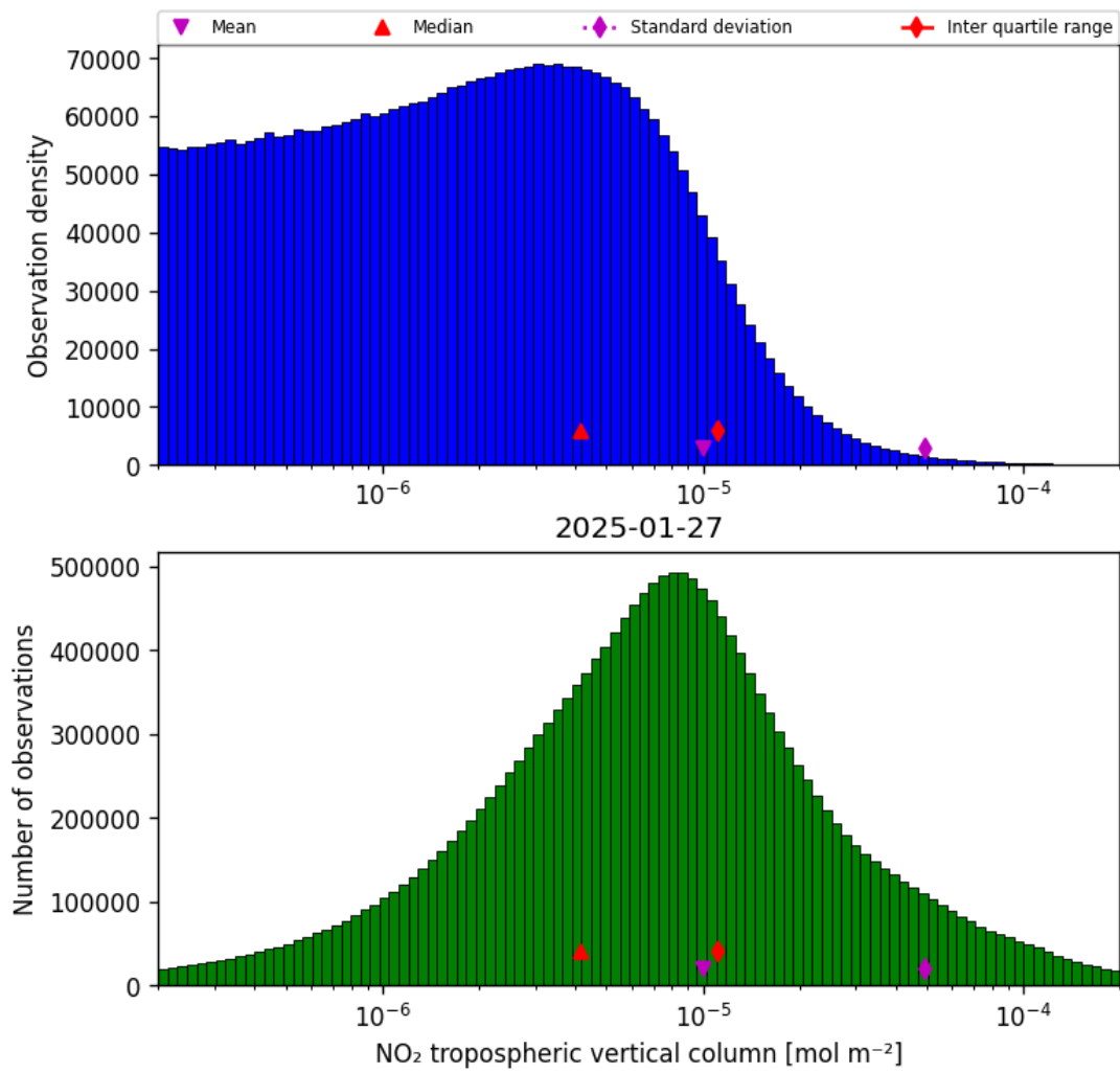
Figure 27: Histogram of “NO 2 tropospheric vertical column” for 2025-01-27 to 2025-01-28
