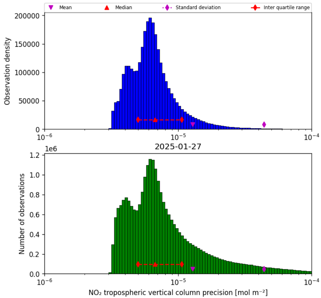
Figure 28: Histogram of “NO 2 tropospheric vertical column precision” for 2025-01-27 to 2025-01-28
