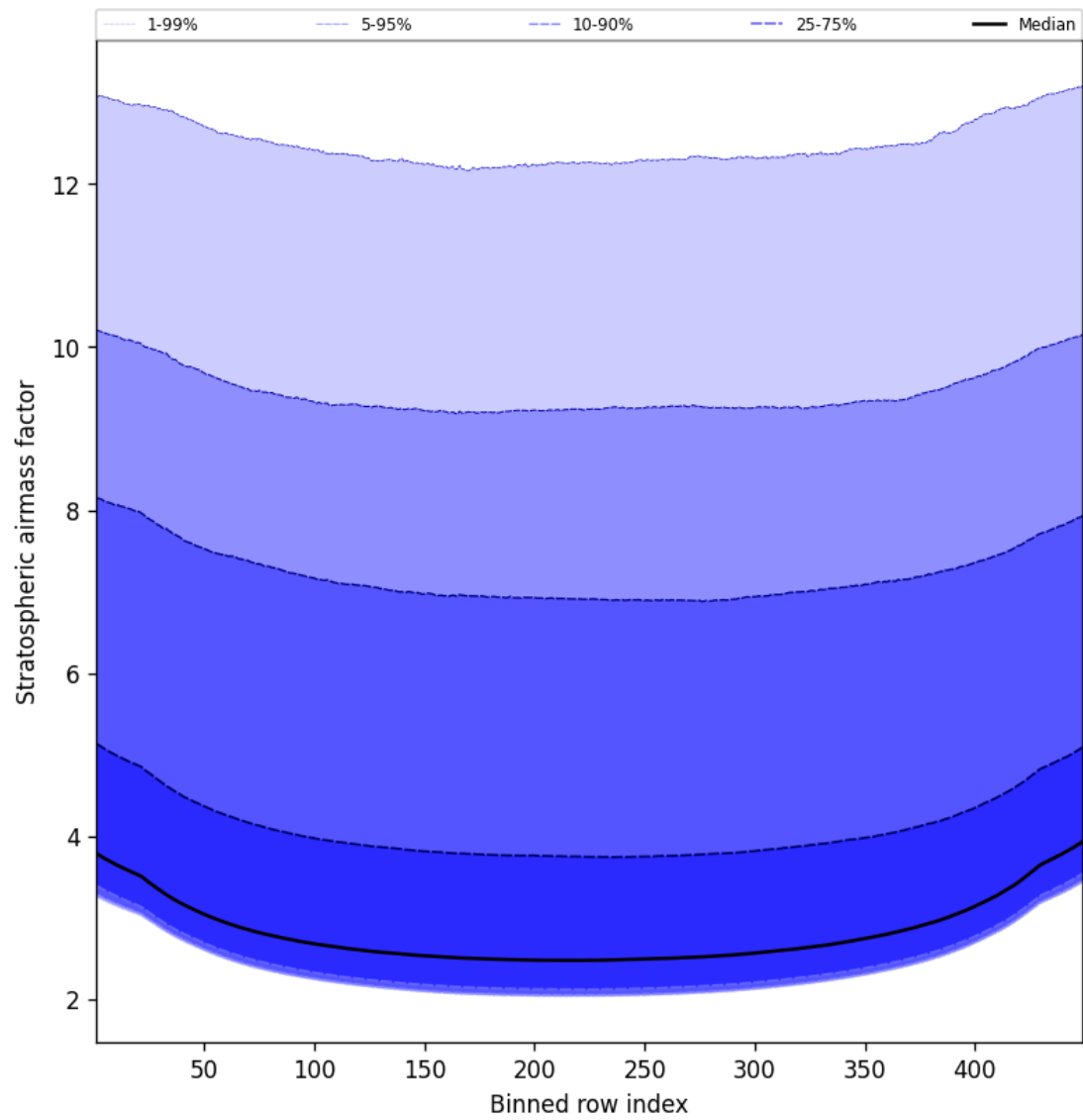
Figure 59: Along track statistics of “Stratospheric airmass factor” for 2025-01-27 to 2025-01-28
