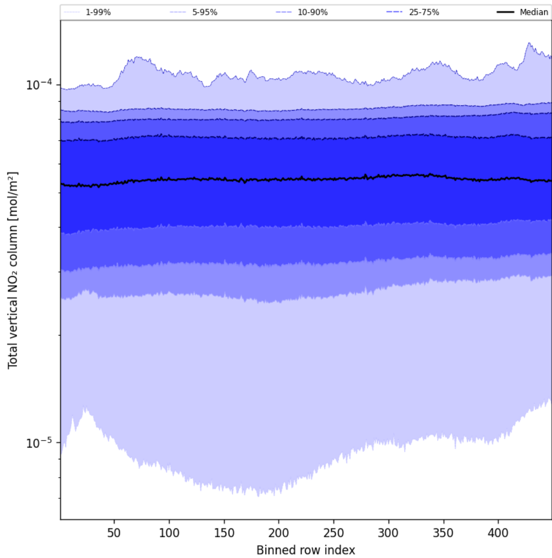
Figure 53: Along track statistics of “Total vertical NO 2 column” for 2025-01-27 to 2025-01-28
