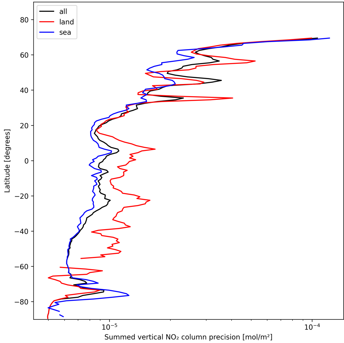
Figure 22: Zonal average of “Summed vertical NO 2 column precision” for 2025-01-27 to 2025-01-28.
