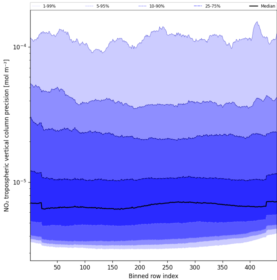
Figure 45: Along track statistics of “NO 2 tropospheric vertical column precision” for 2025-01-27 to 2025-01-28
