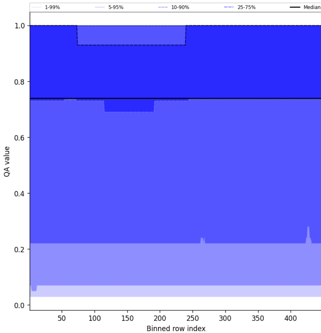
Figure 43: Along track statistics of “QA value” for 2025-01-27 to 2025-01-28
