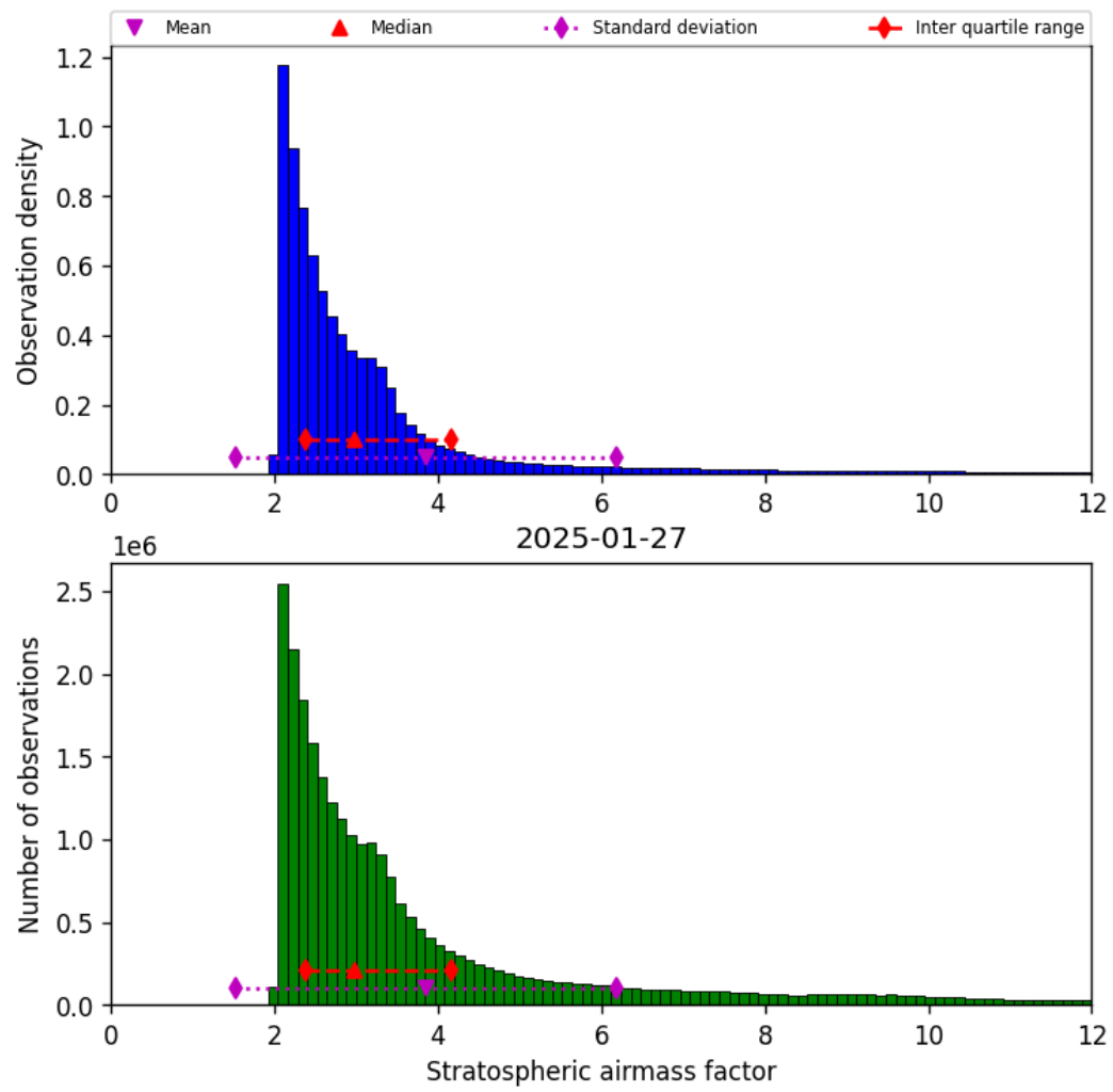
Figure 42: Histogram of “Stratospheric airmass factor” for 2025-01-27 to 2025-01-28
