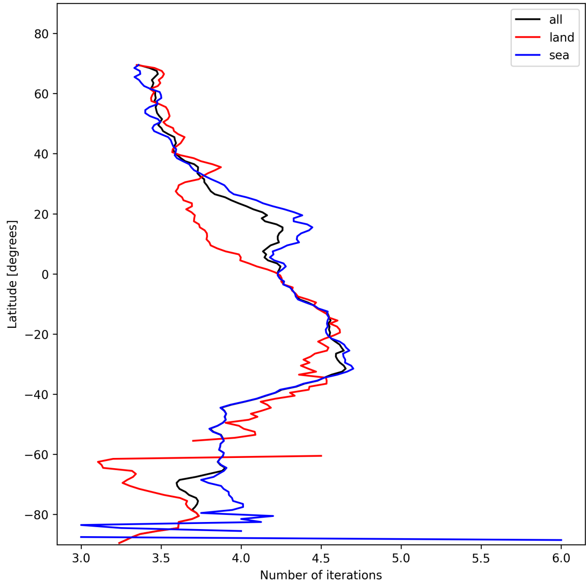
Figure 15: Zonal average of “Number of iterations” for 2025-01-27 to 2025-01-28.
