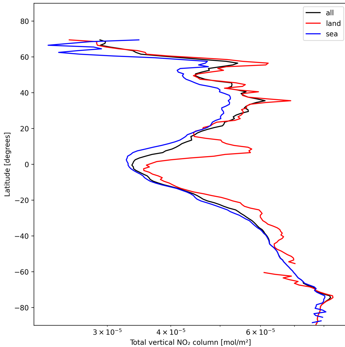
Figure 19: Zonal average of “Total vertical NO 2 column” for 2025-01-27 to 2025-01-28.
