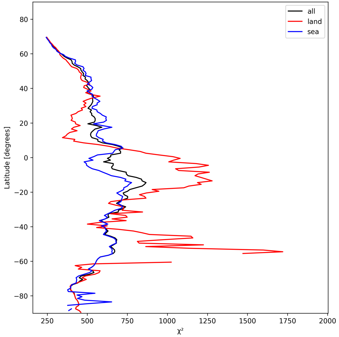
Figure 23: Zonal average of “ \chi^2 ” for 2025-01-27 to 2025-01-28.
