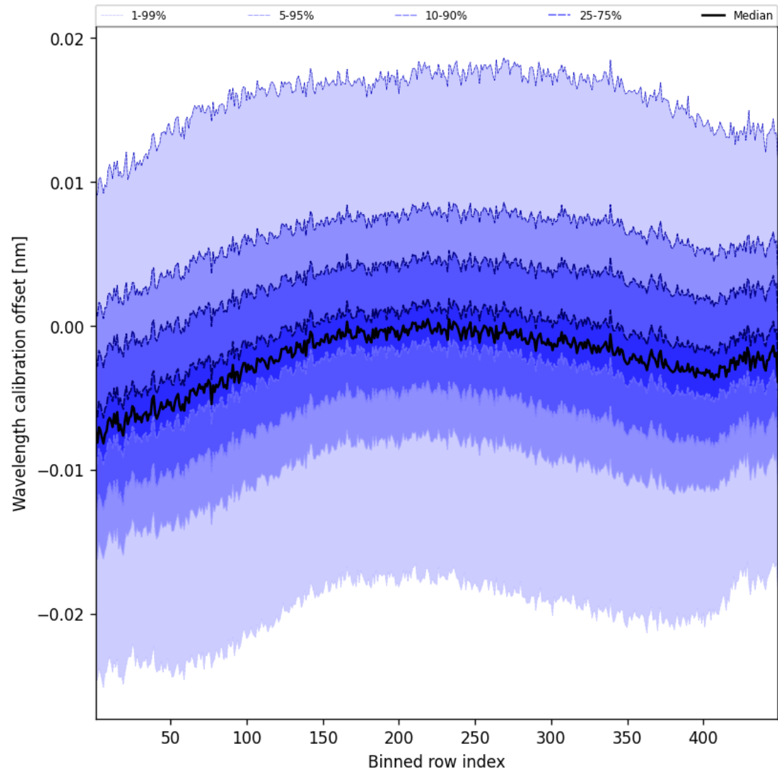
Figure 50: Along track statistics of “Wavelength calibration offset” for 2025-01-27 to 2025-01-28
