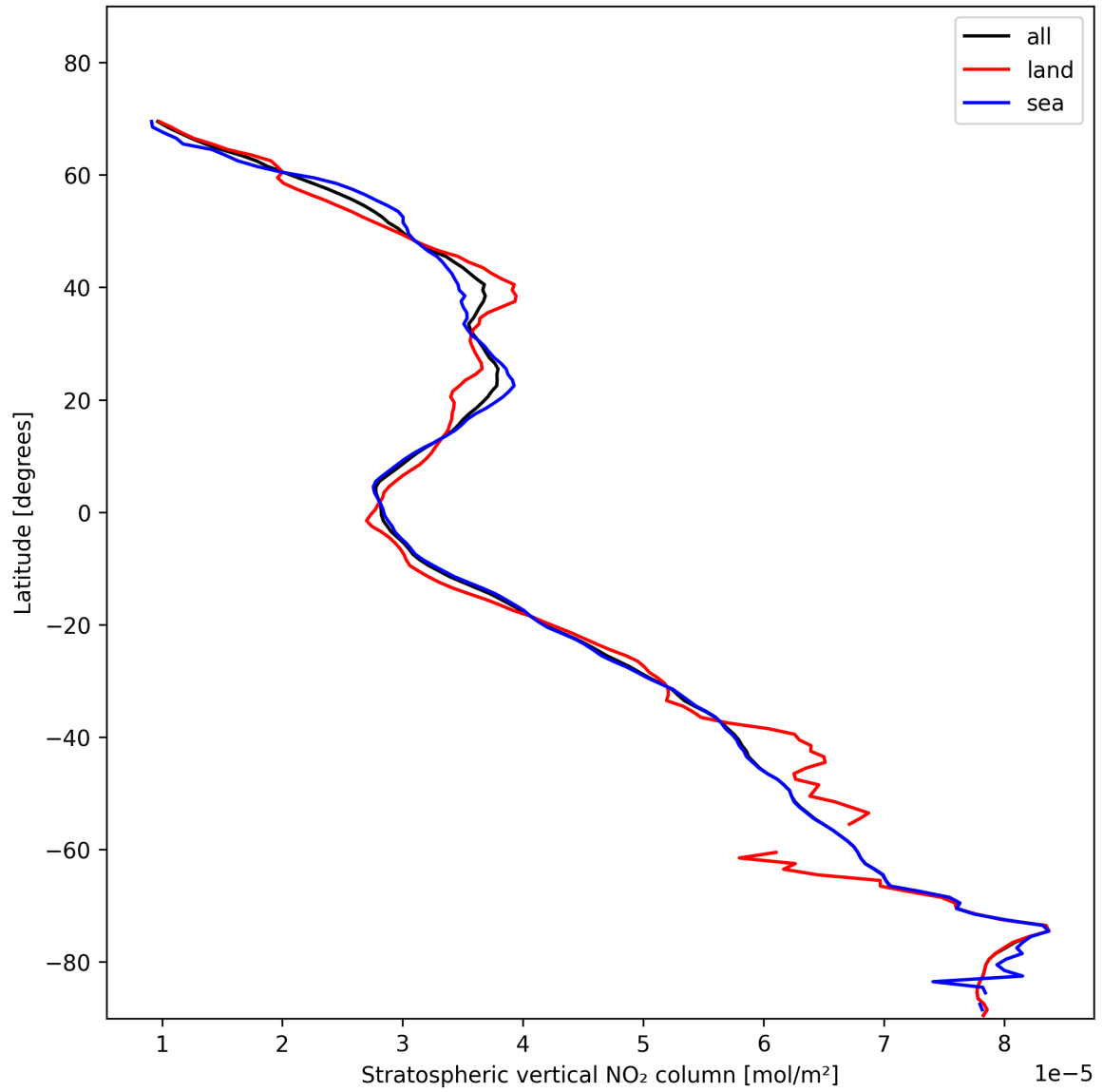
Figure 17: Zonal average of “Stratospheric vertical NO 2 column” for 2025-01-27 to 2025-01-28.
