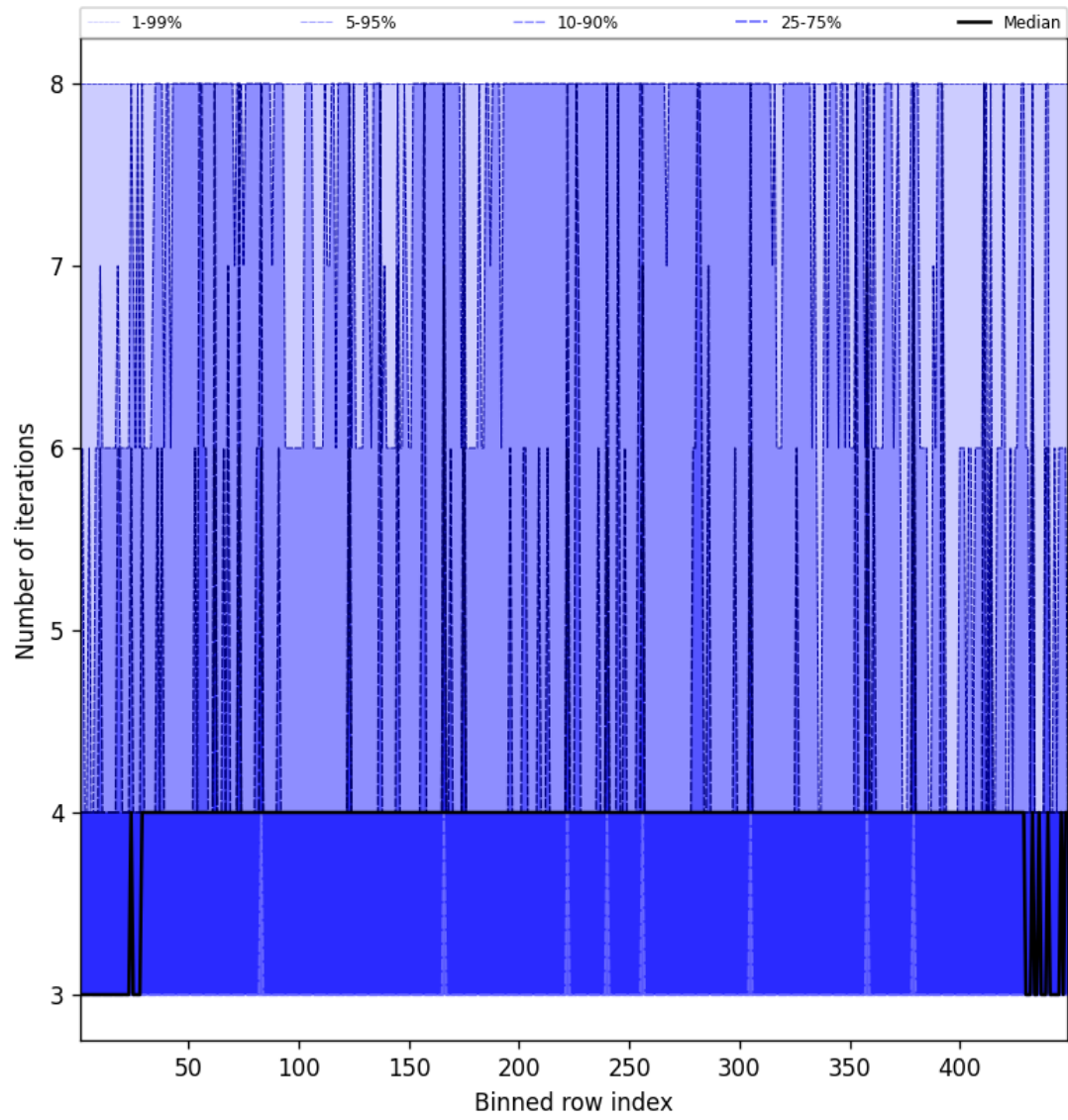
Figure 49: Along track statistics of “Number of iterations” for 2025-01-27 to 2025-01-28
