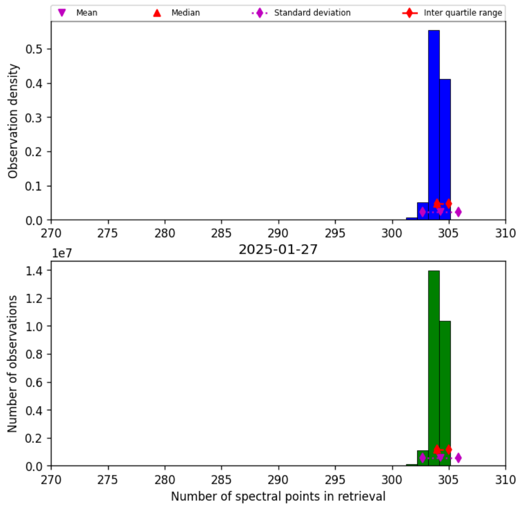
Figure 31: Histogram of “Number of spectral points in retrieval” for 2025-01-27 to 2025-01-28
