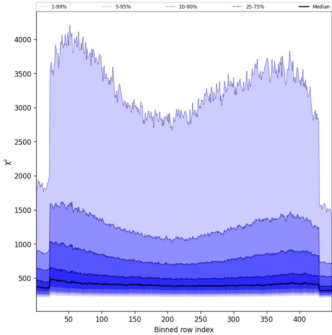
Figure 57: Along track statistics of “ \chi^2 ” for 2025-01-27 to 2025-01-28
