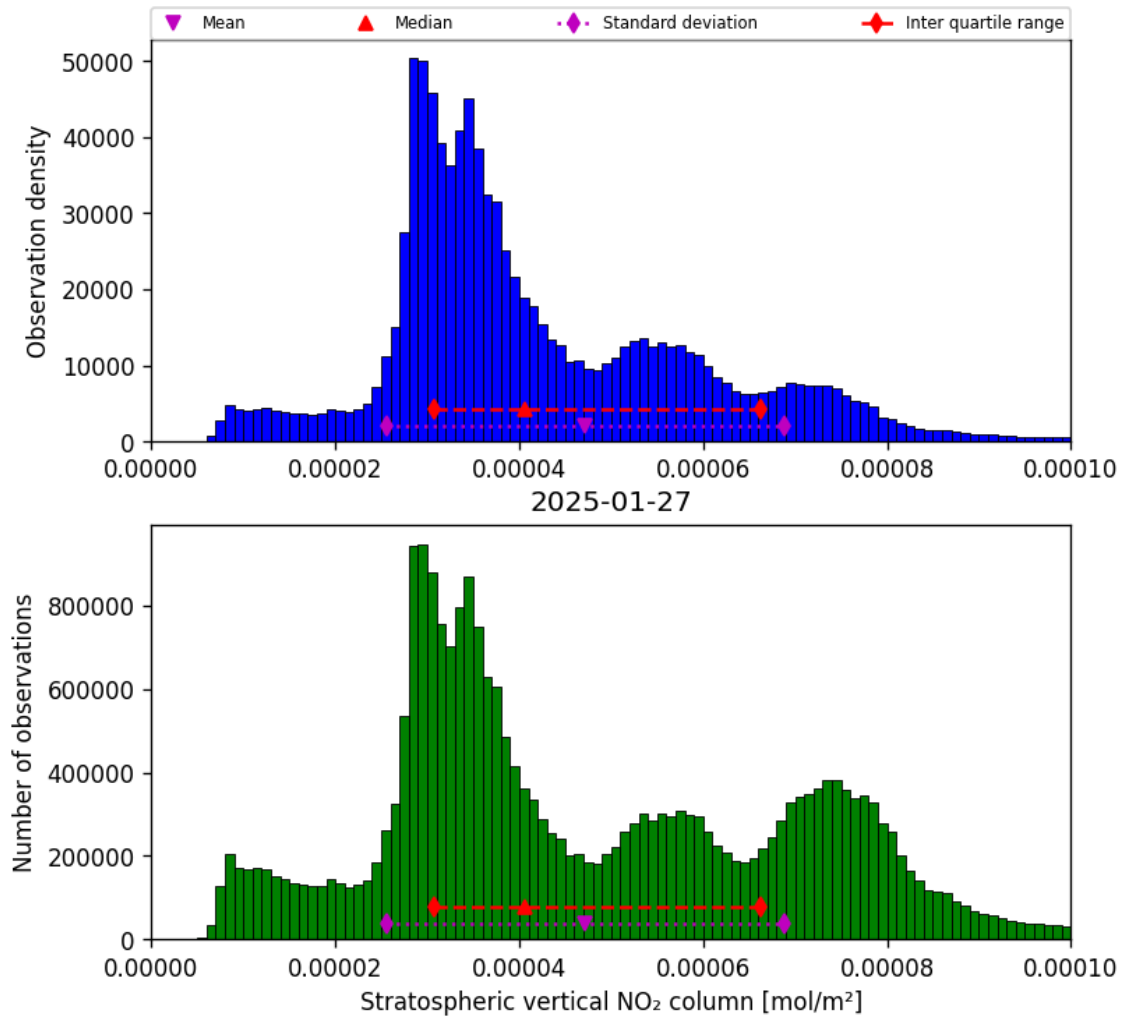
Figure 34: Histogram of “Stratospheric vertical NO 2 column” for 2025-01-27 to 2025-01-28
