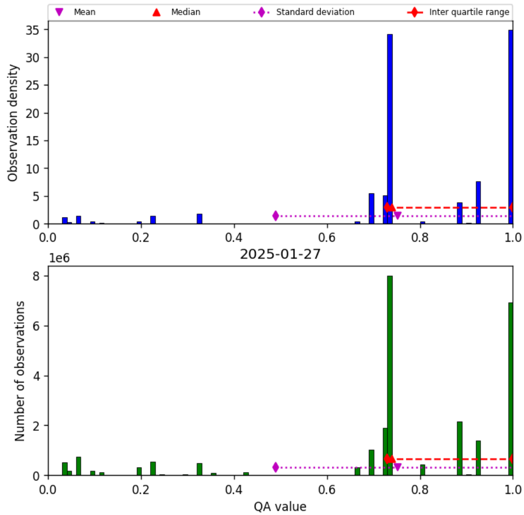
Figure 26: Histogram of “QA value” for 2025-01-27 to 2025-01-28
