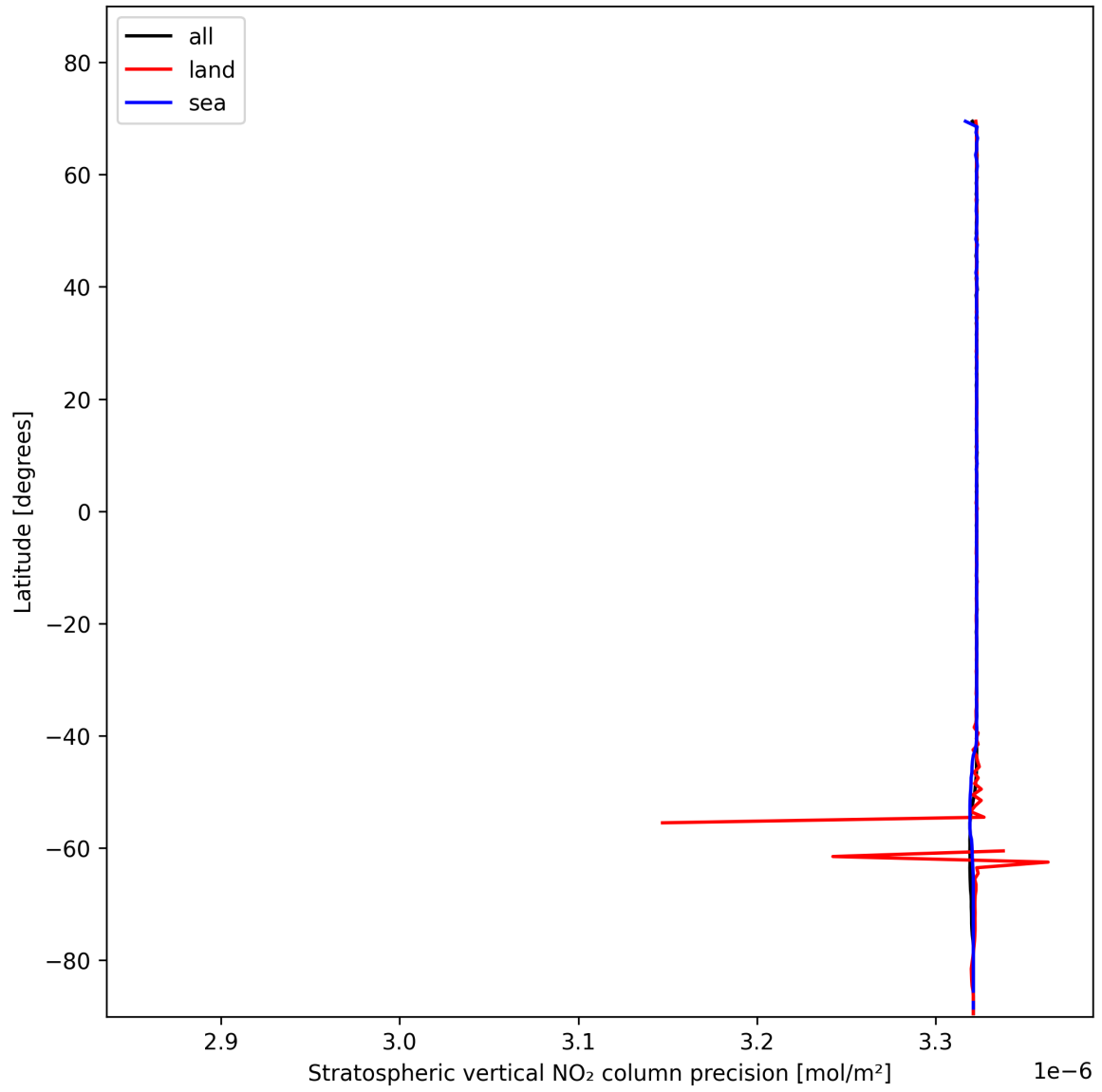
Figure 18: Zonal average of "Stratospheric vertical NO 2 column precision" for 2025-01-27 to 2025-01-28.
