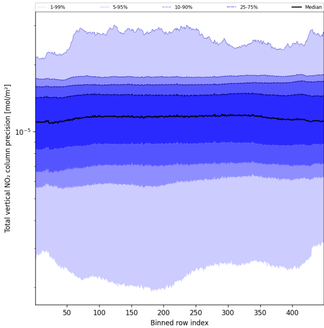
Figure 54: Along track statistics of “Total vertical NO 2 column precision” for 2025-01-27 to 2025-01-28
