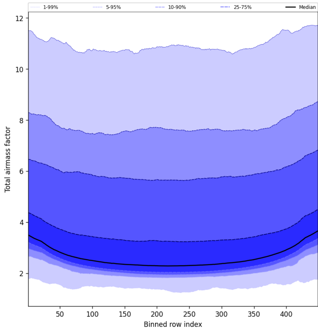
Figure 47: Along track statistics of “Total airmass factor” for 2025-01-27 to 2025-01-28
