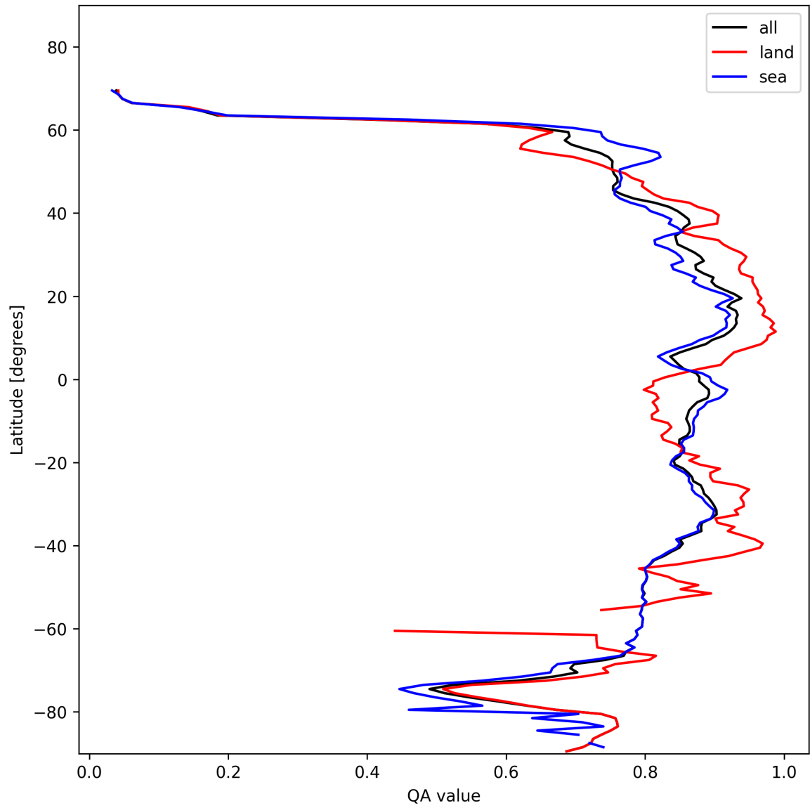
Figure 9: Zonal average of “QA value” for 2025-01-27 to 2025-01-28.
