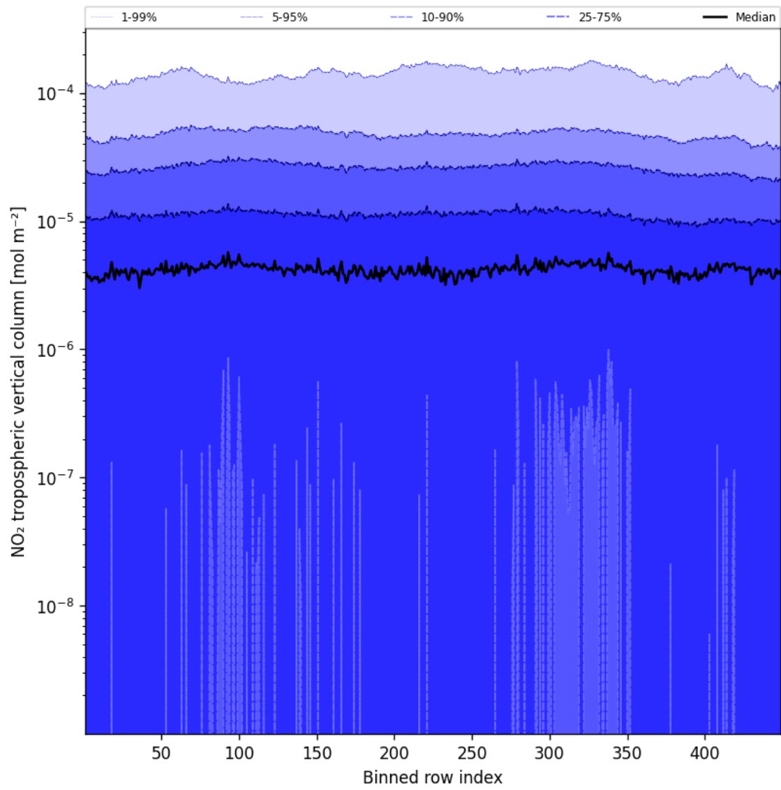
Figure 44: Along track statistics of “NO 2 tropospheric vertical column” for 2025-01-27 to 2025-01-28
