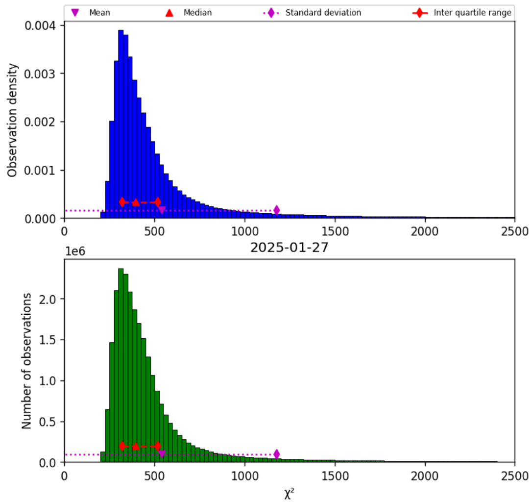
Figure 40: Histogram of “ \chi^2 ” for 2025-01-27 to 2025-01-28
