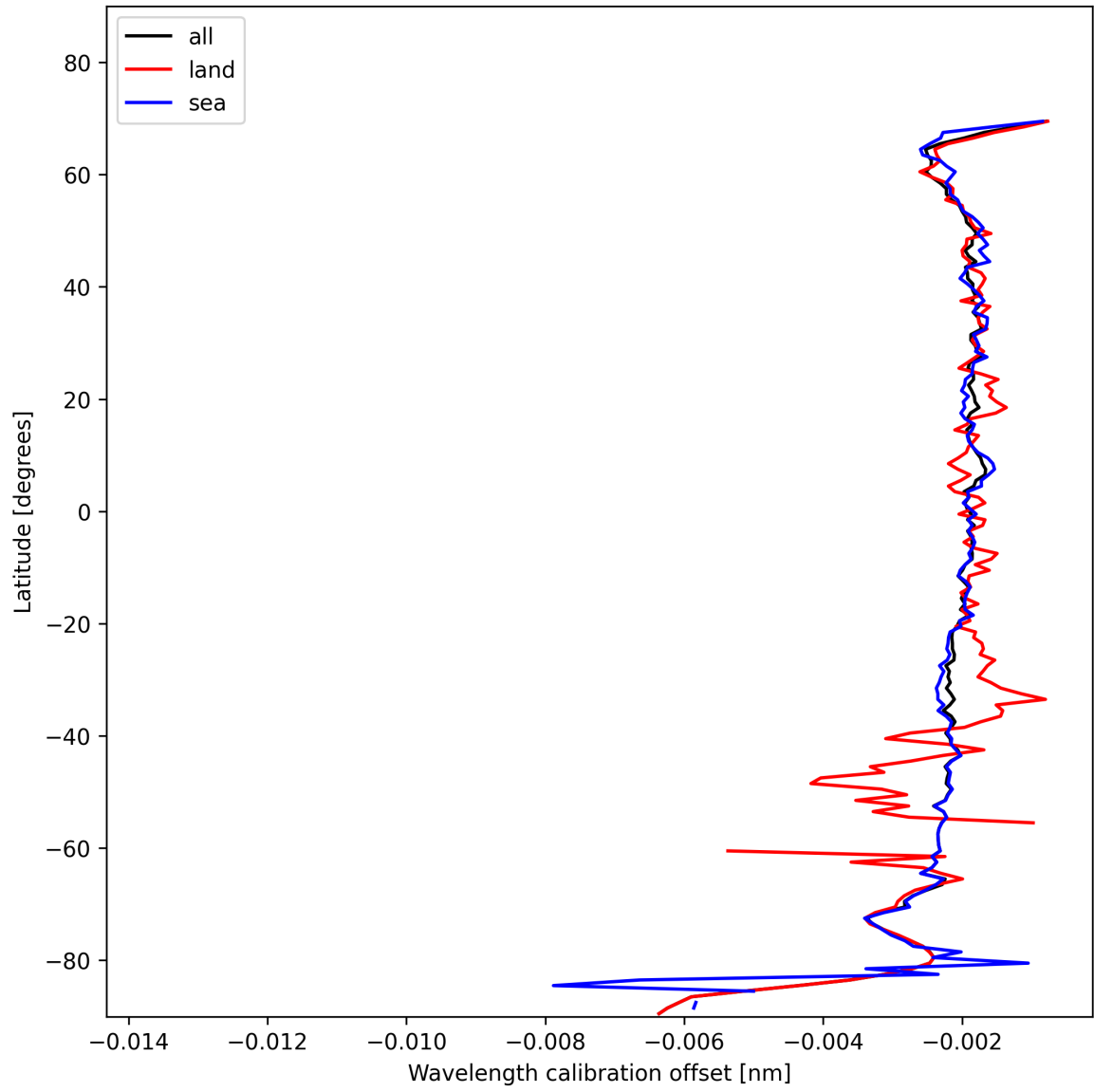
Figure 16: Zonal average of “Wavelength calibration offset” for 2025-01-27 to 2025-01-28.
