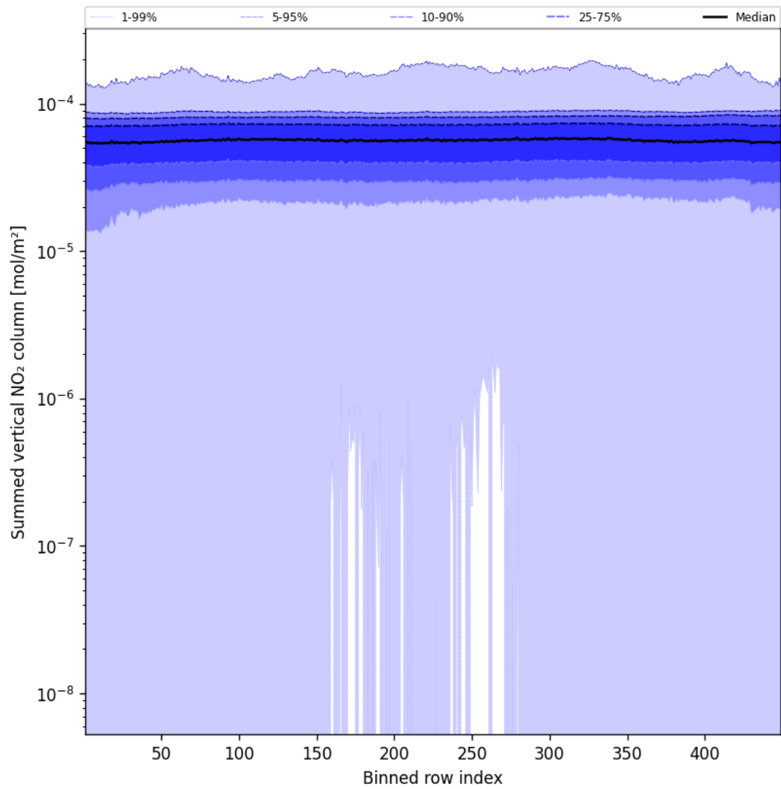
Figure 55: Along track statistics of “Summed vertical NO 2 column” for 2025-01-27 to 2025-01-28
