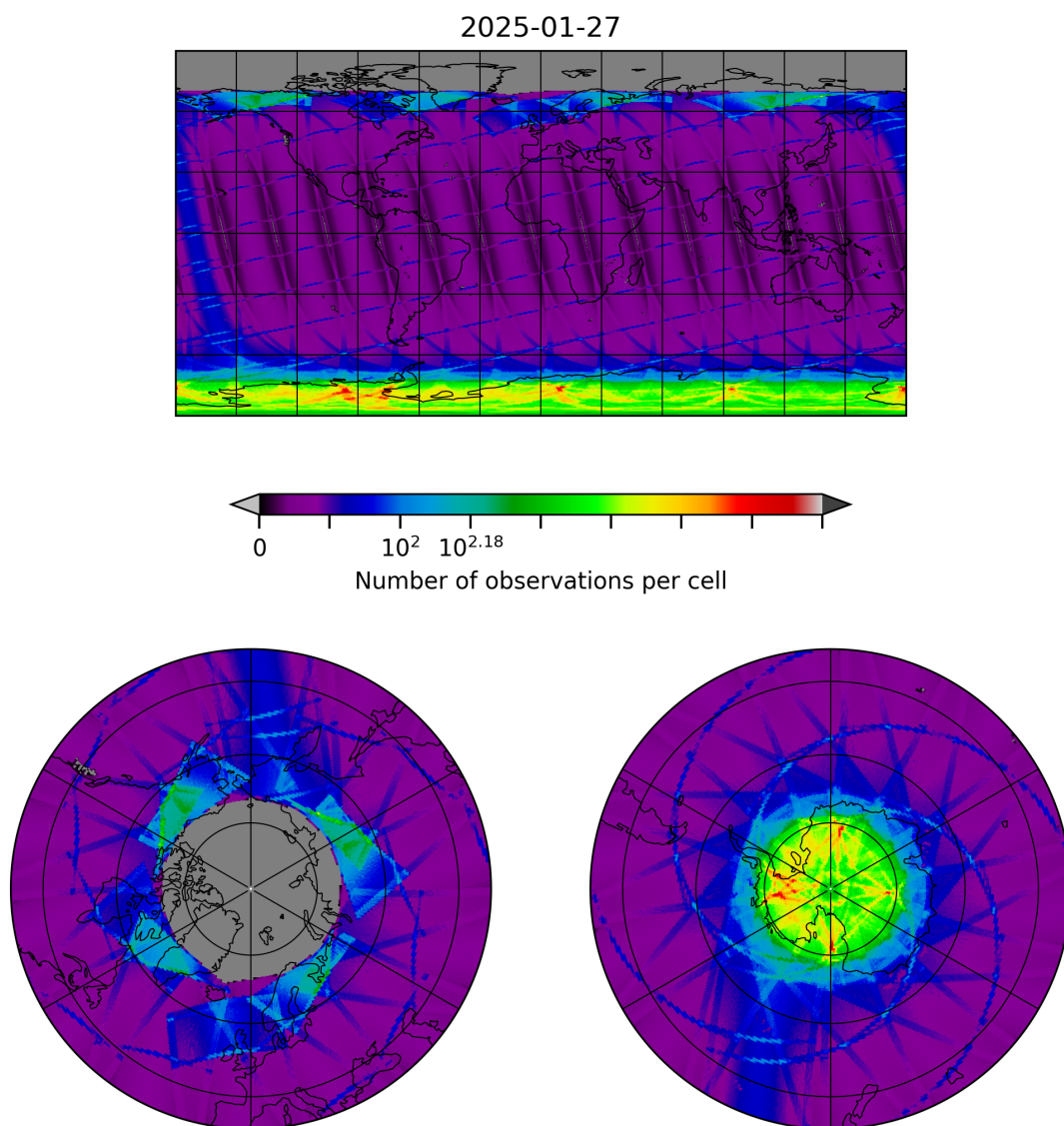
Figure 8: Map of the number of observations for 2025-01-27 to 2025-01-28
