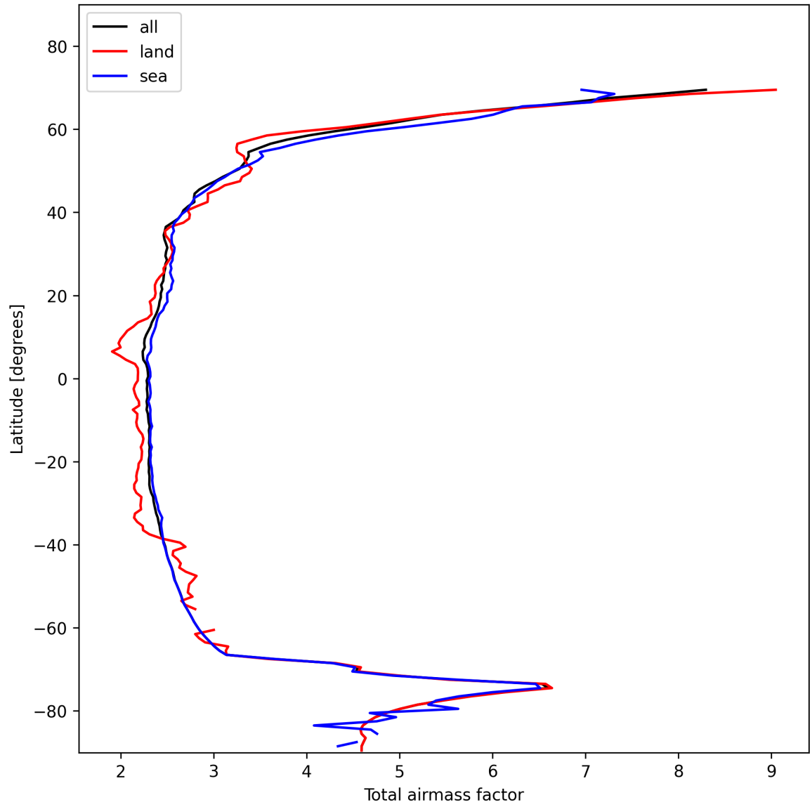
Figure 13: Zonal average of “Total airmass factor” for 2025-01-27 to 2025-01-28.
