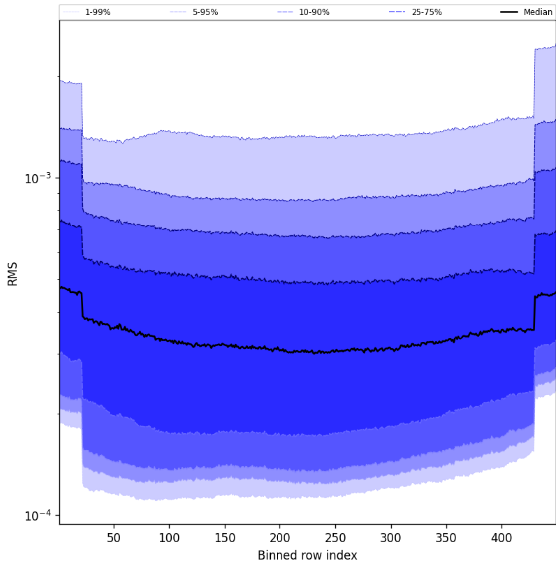
Figure 58: Along track statistics of “RMS” for 2025-01-27 to 2025-01-28
