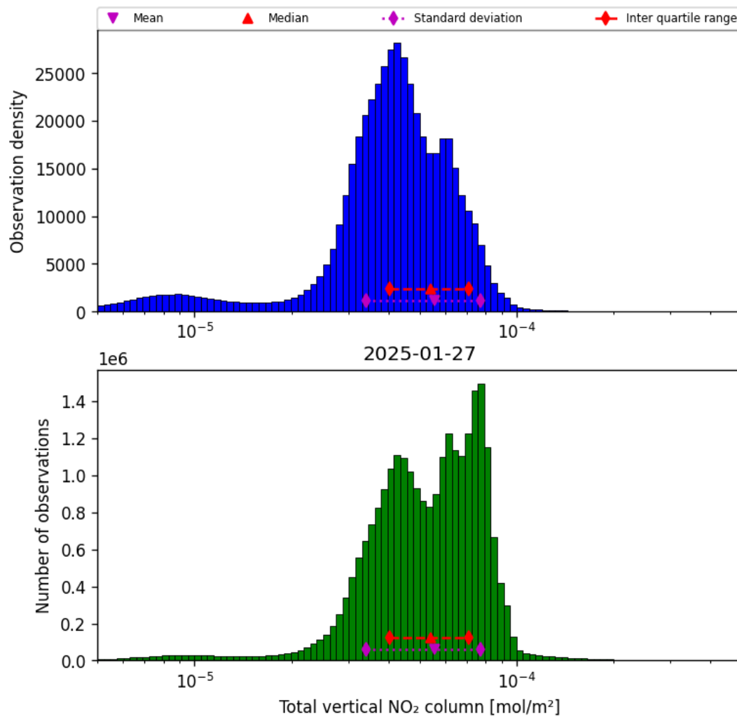
Figure 36: Histogram of “Total vertical NO 2 column” for 2025-01-27 to 2025-01-28
