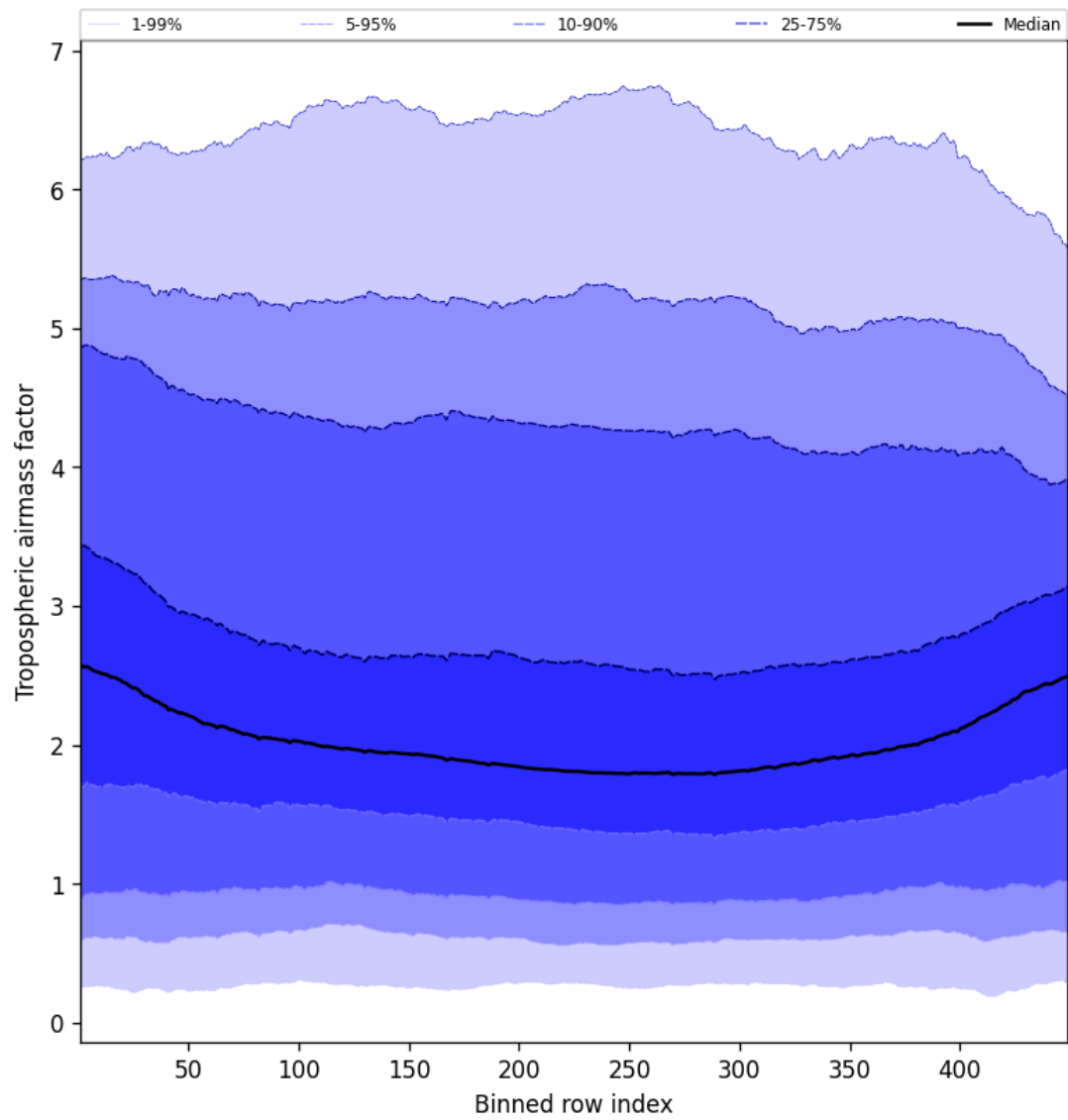
Figure 46: Along track statistics of “Tropospheric airmass factor” for 2025-01-27 to 2025-01-28
