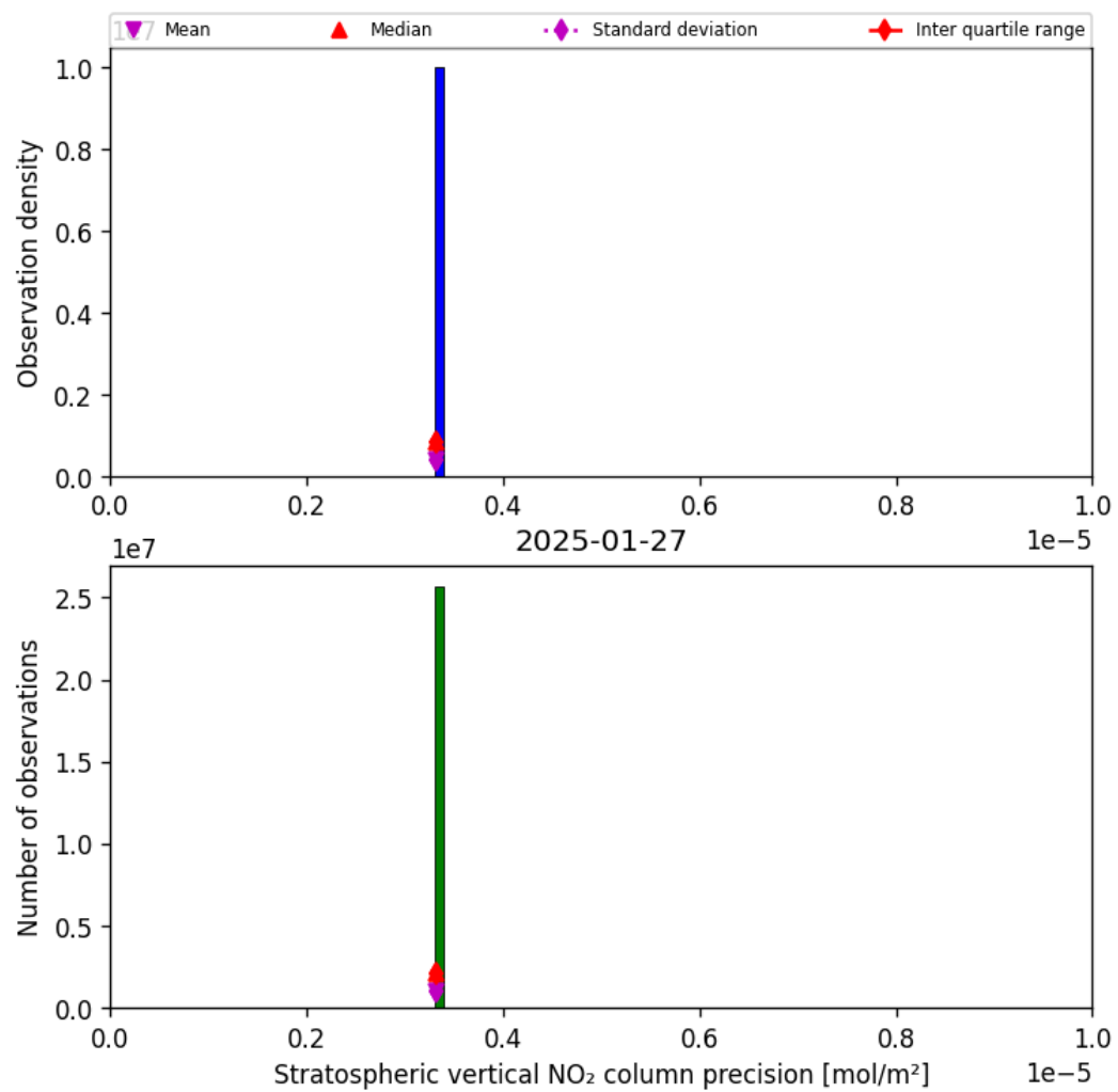
Figure 35: Histogram of “Stratospheric vertical NO 2 column precision” for 2025-01-27 to 2025-01-28
