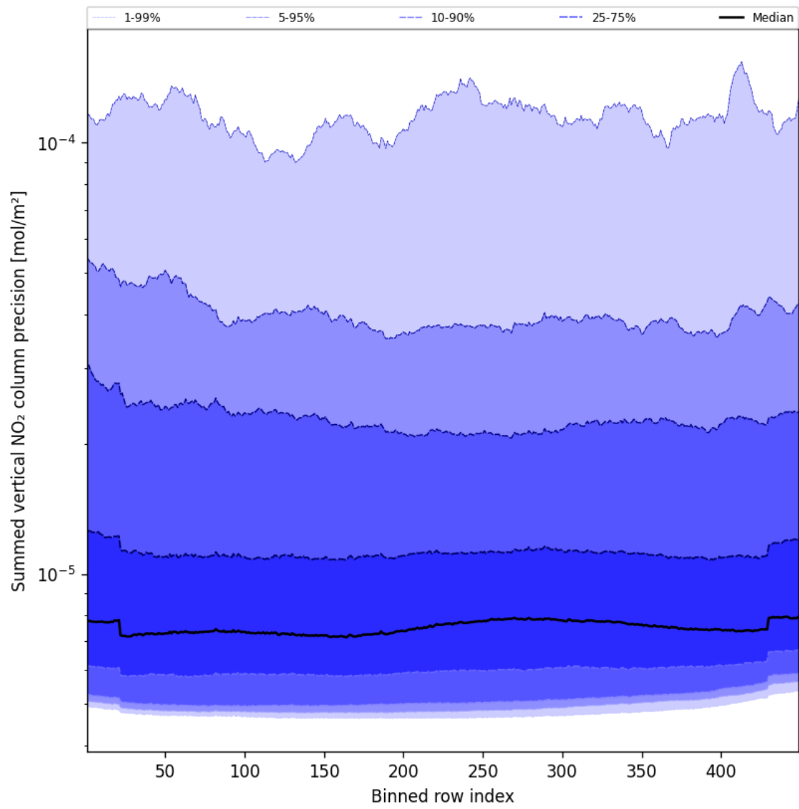
Figure 56: Along track statistics of “Summed vertical NO 2 column precision” for 2025-01-27 to 2025-01-28
