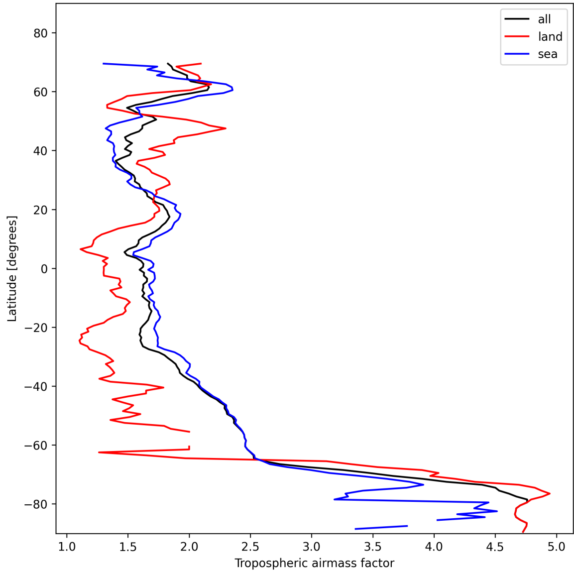
Figure 12: Zonal average of “Tropospheric airmass factor” for 2025-01-27 to 2025-01-28.
