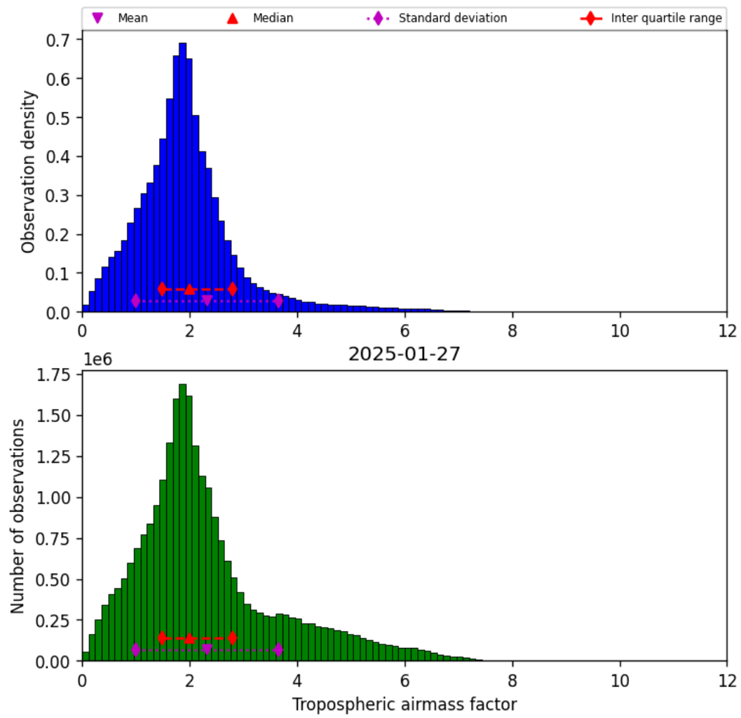
Figure 29: Histogram of “Tropospheric airmass factor” for 2025-01-27 to 2025-01-28
