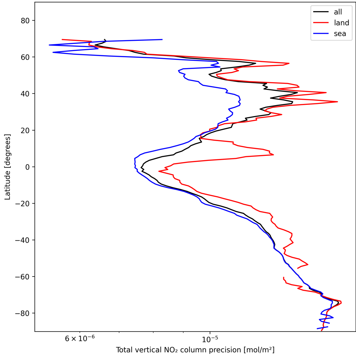
Figure 20: Zonal average of “Total vertical NO 2 column precision” for 2025-01-27 to 2025-01-28.
