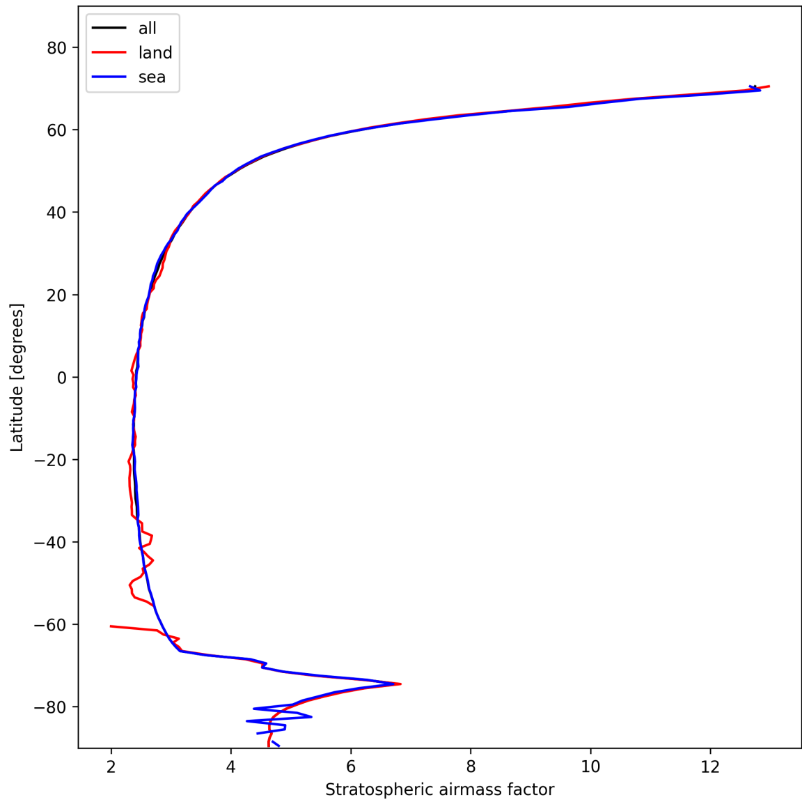
Figure 25: Zonal average of “Stratospheric air mass factor” for 2025-01-28 to 2025-01-29.
