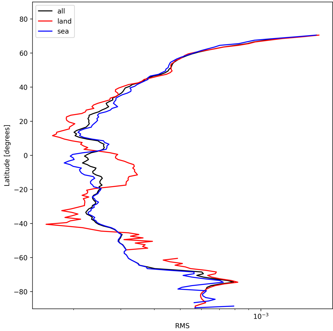
Figure 24: Zonal average of “RMS” for 2025-01-28 to 2025-01-29.
