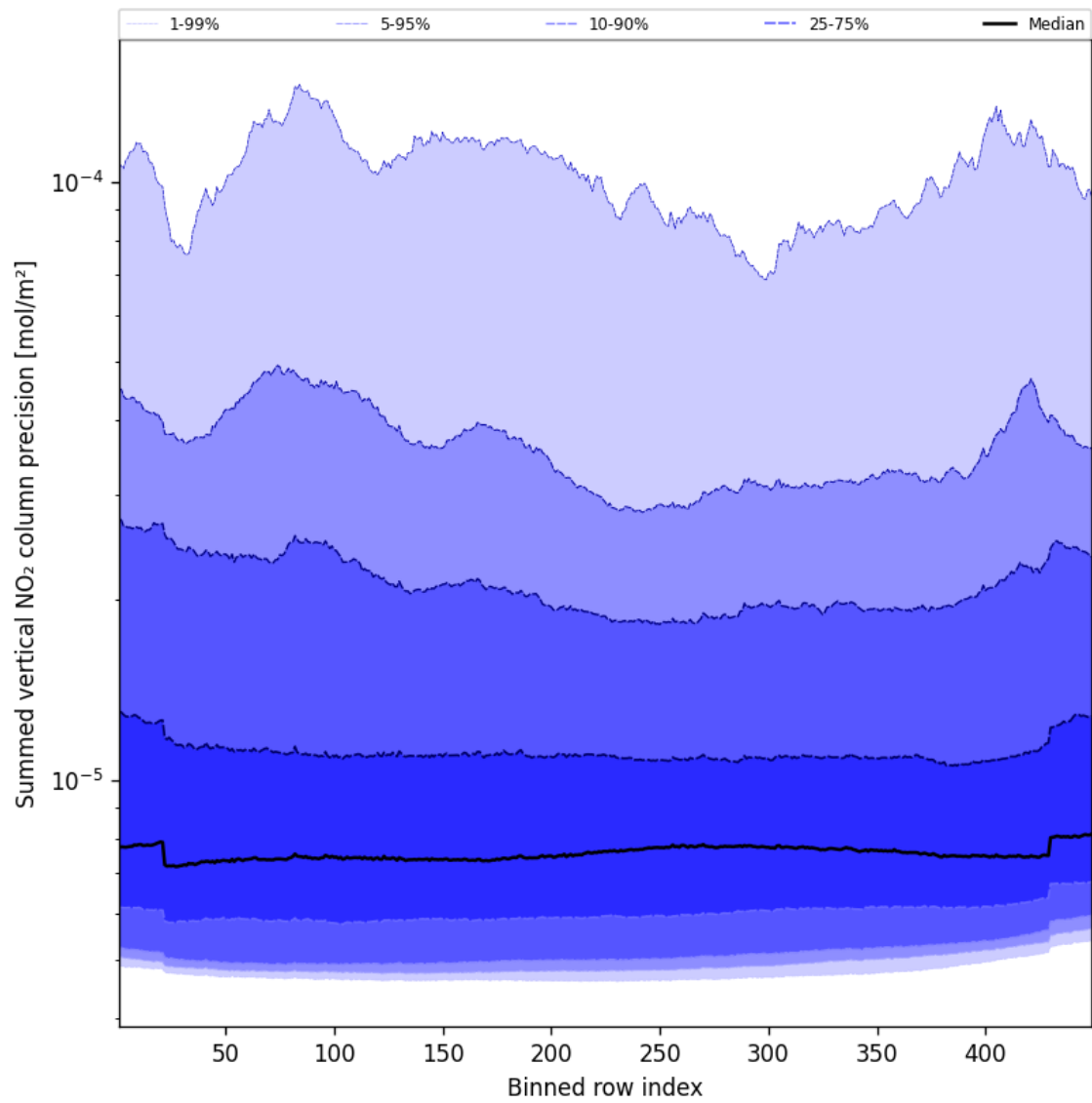
Figure 56: Along track statistics of “Summed vertical NO 2 column precision” for 2025-01-28 to 2025-01-29
