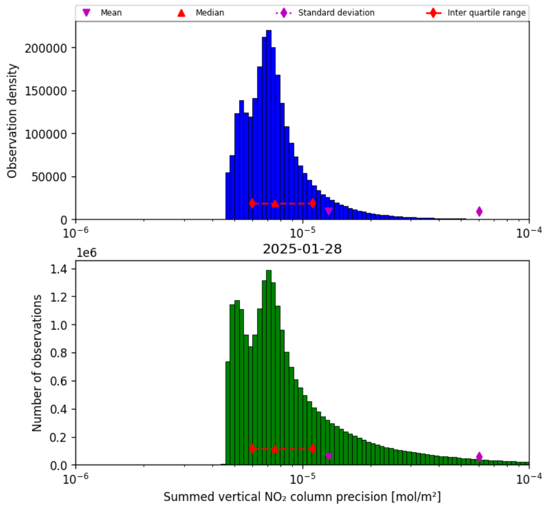
Figure 39: Histogram of "Summed vertical NO 2 column precision" for 2025-01-28 to 2025-01-29
