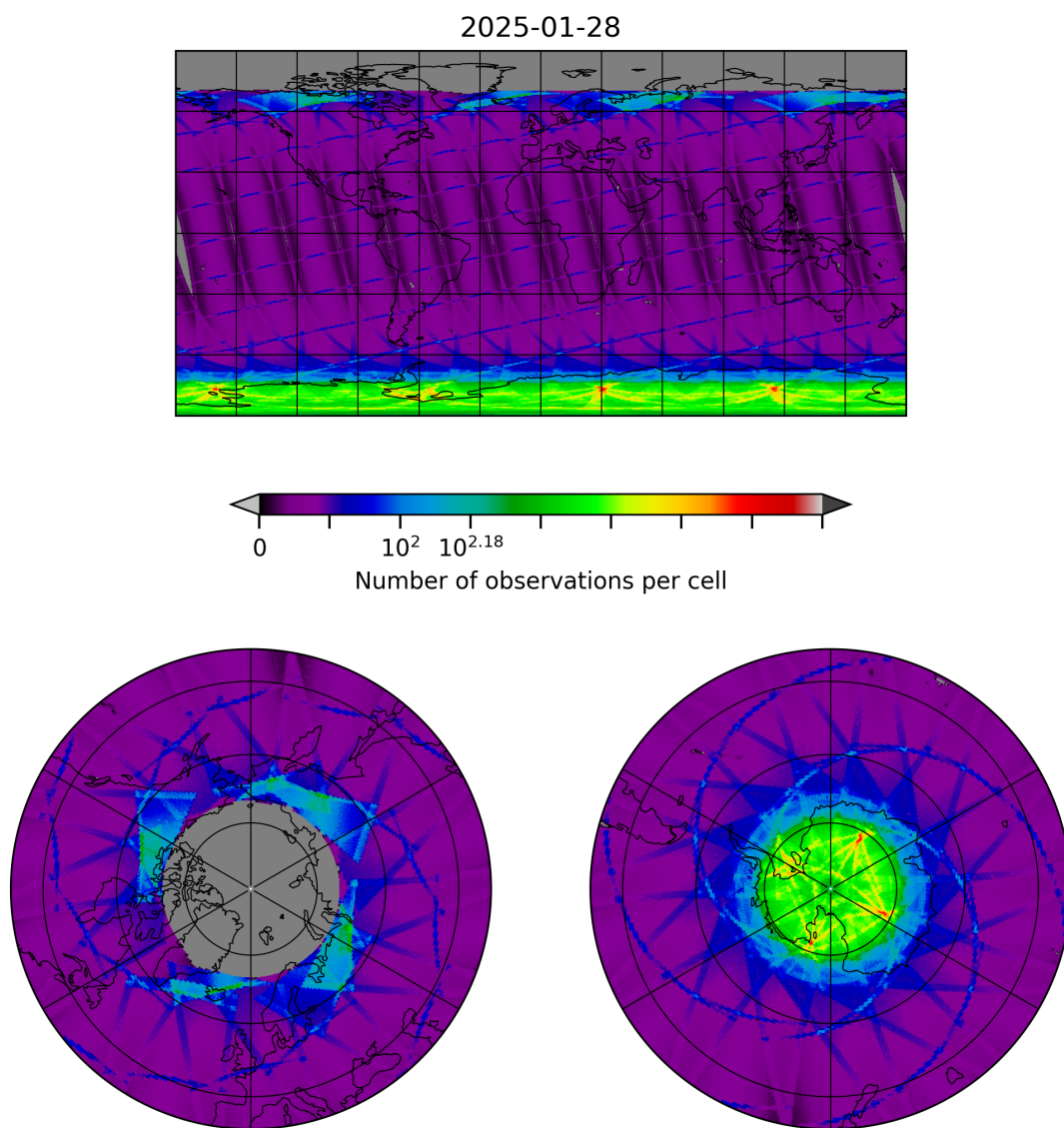
Figure 8: Map of the number of observations for 2025-01-28 to 2025-01-29
