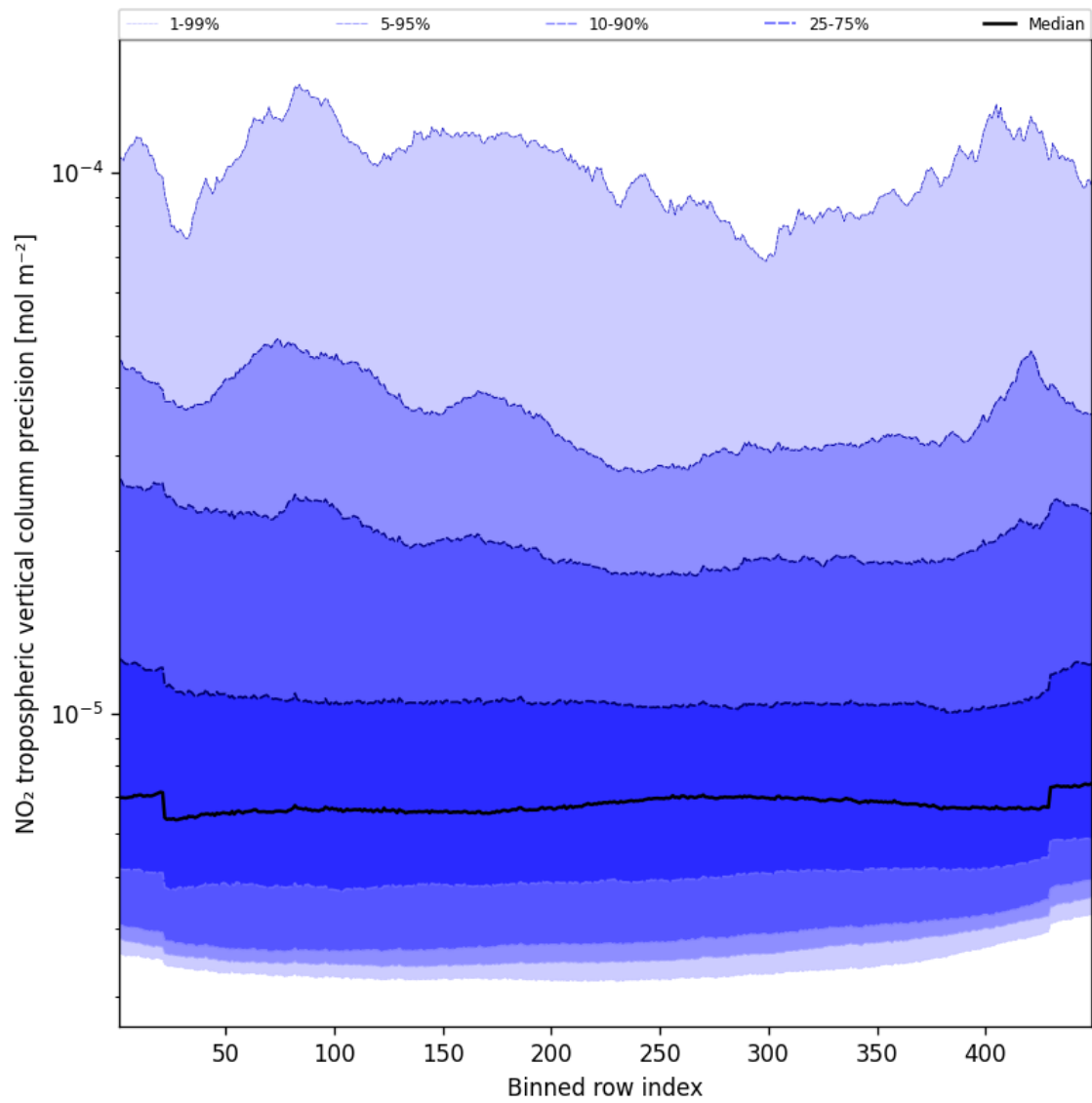
Figure 45: Along track statistics of “NO 2 tropospheric vertical column precision” for 2025-01-28 to 2025-01-29
