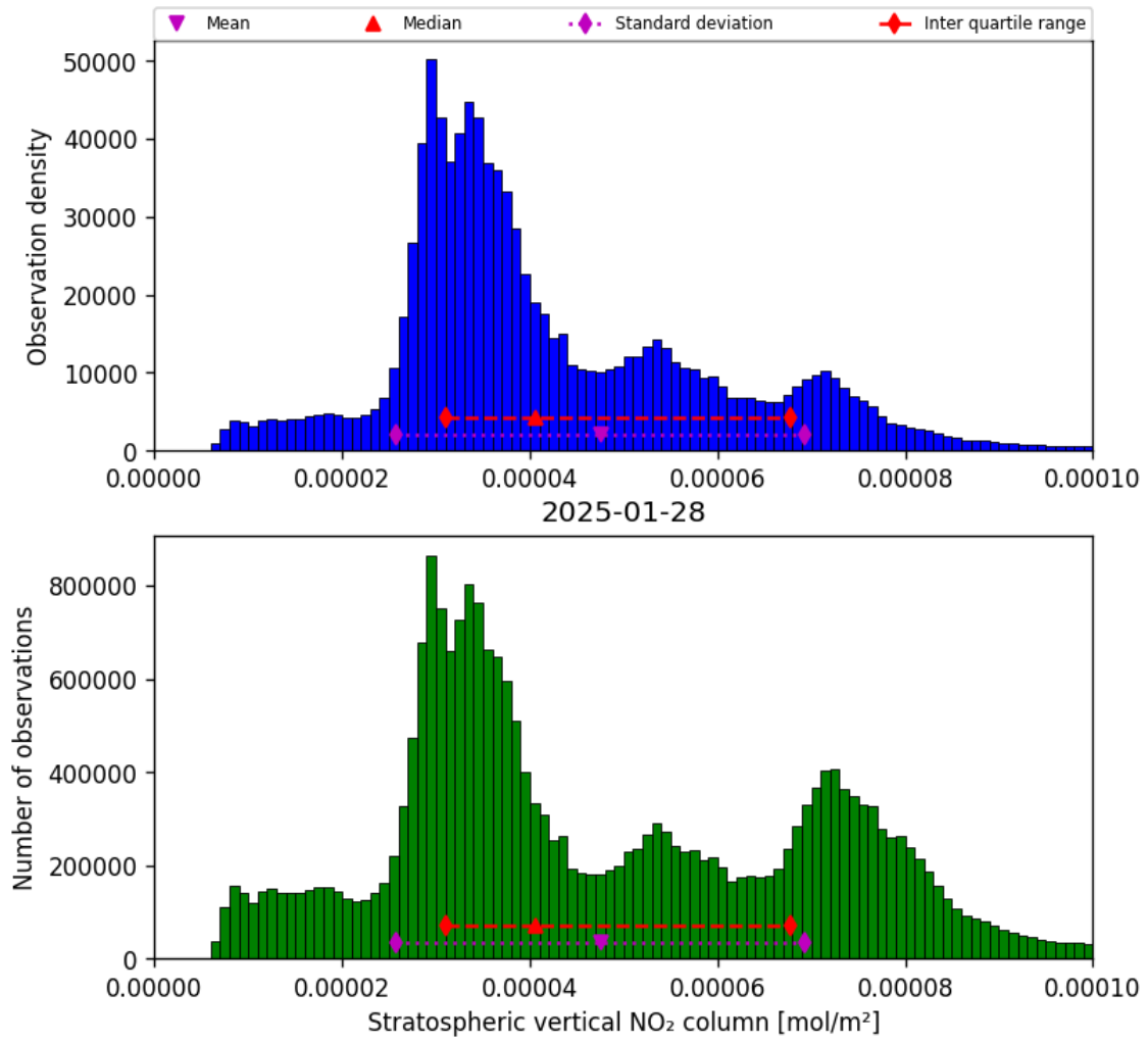
Figure 34: Histogram of “Stratospheric vertical NO 2 column” for 2025-01-28 to 2025-01-29
