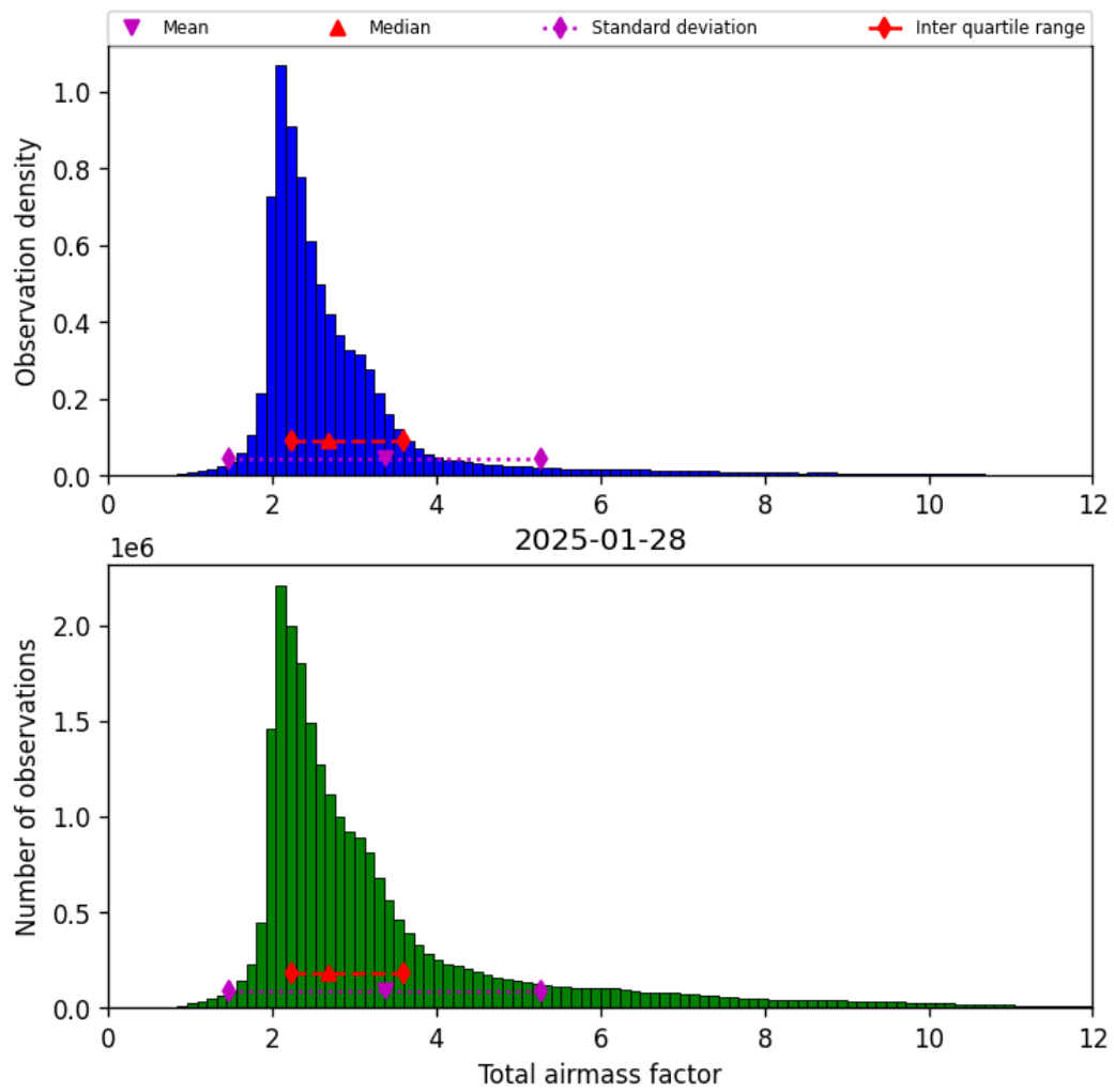
Figure 30: Histogram of “Total airmass factor” for 2025-01-28 to 2025-01-29
