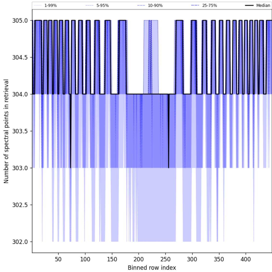
Figure 48: Along track statistics of “Number of spectral points in retrieval” for 2025-01-28 to 2025-01-29
