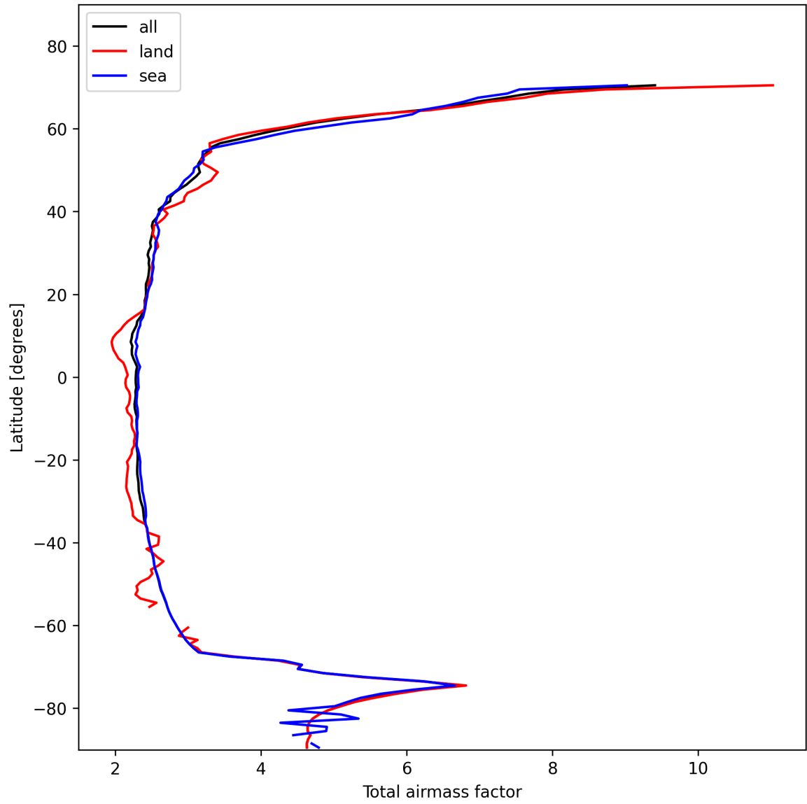
Figure 13: Zonal average of “Total airmass factor” for 2025-01-28 to 2025-01-29.
