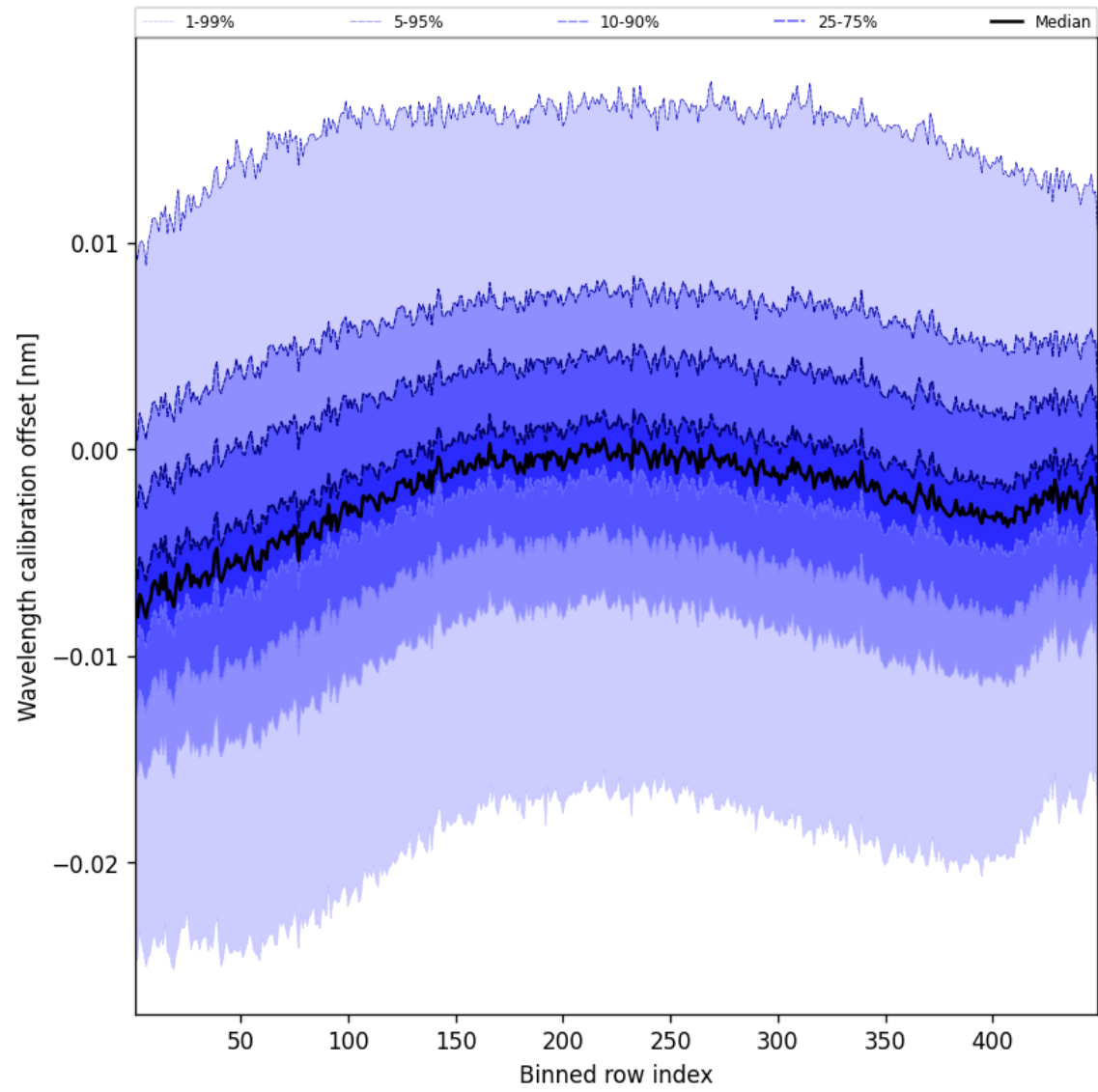
Figure 50: Along track statistics of “Wavelength calibration offset” for 2025-01-28 to 2025-01-29
