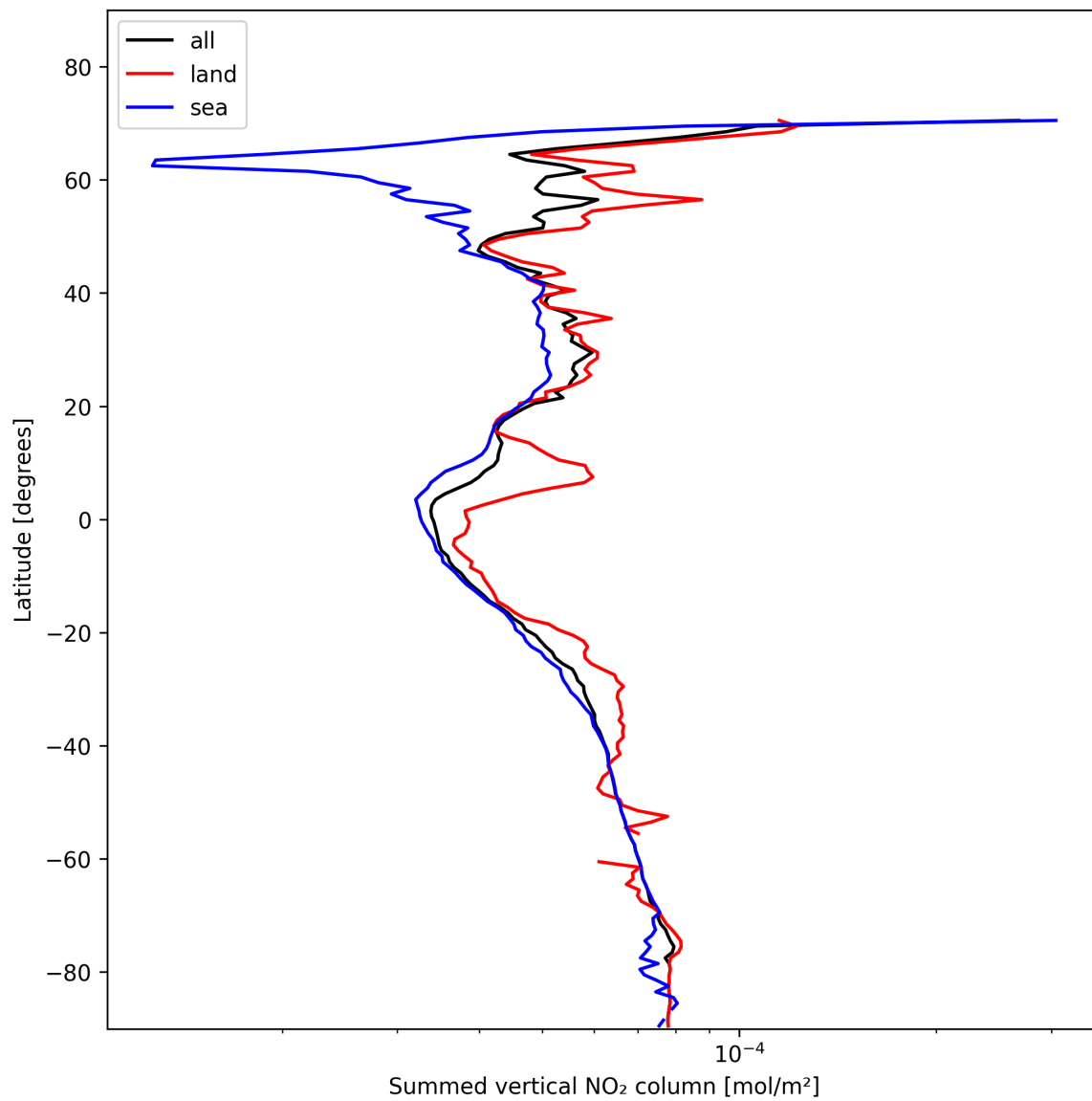
Figure 21: Zonal average of “Summed vertical NO 2 column” for 2025-01-28 to 2025-01-29.
