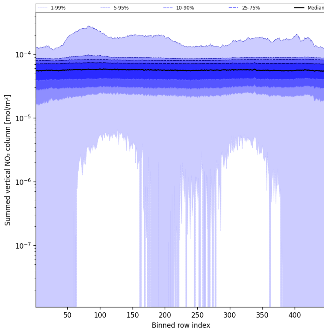
Figure 55: Along track statistics of “Summed vertical NO 2 column” for 2025-01-28 to 2025-01-29
