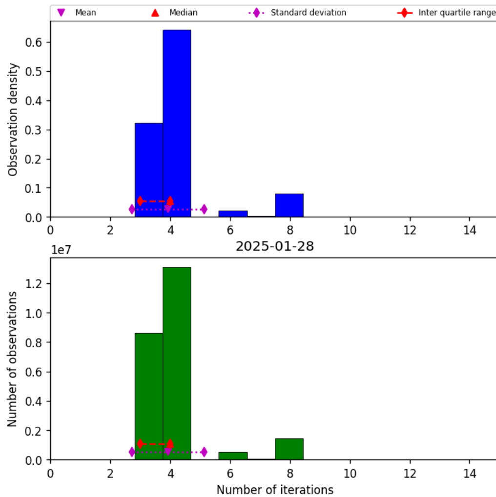
Figure 32: Histogram of “Number of iterations” for 2025-01-28 to 2025-01-29
