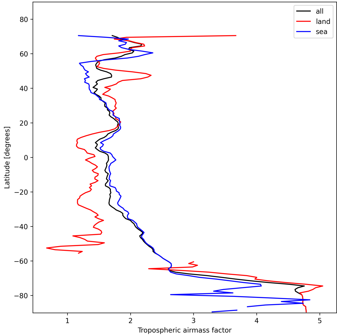
Figure 12: Zonal average of “Tropospheric airmass factor” for 2025-01-28 to 2025-01-29.
