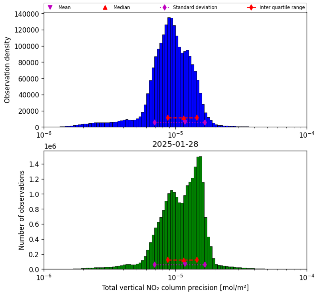
Figure 37: Histogram of “Total vertical NO 2 column precision” for 2025-01-28 to 2025-01-29
