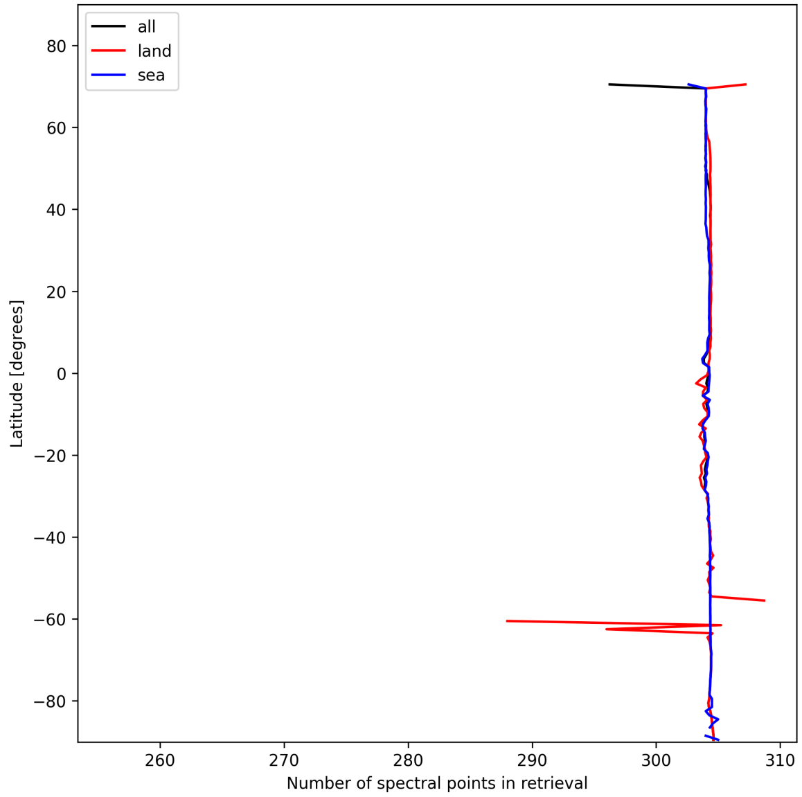
Figure 14: Zonal average of “Number of spectral points in retrieval” for 2025-01-28 to 2025-01-29.
