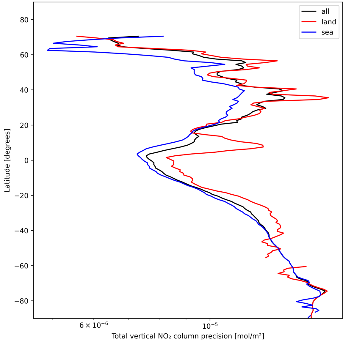
Figure 20: Zonal average of “Total vertical NO 2 column precision” for 2025-01-28 to 2025-01-29.
