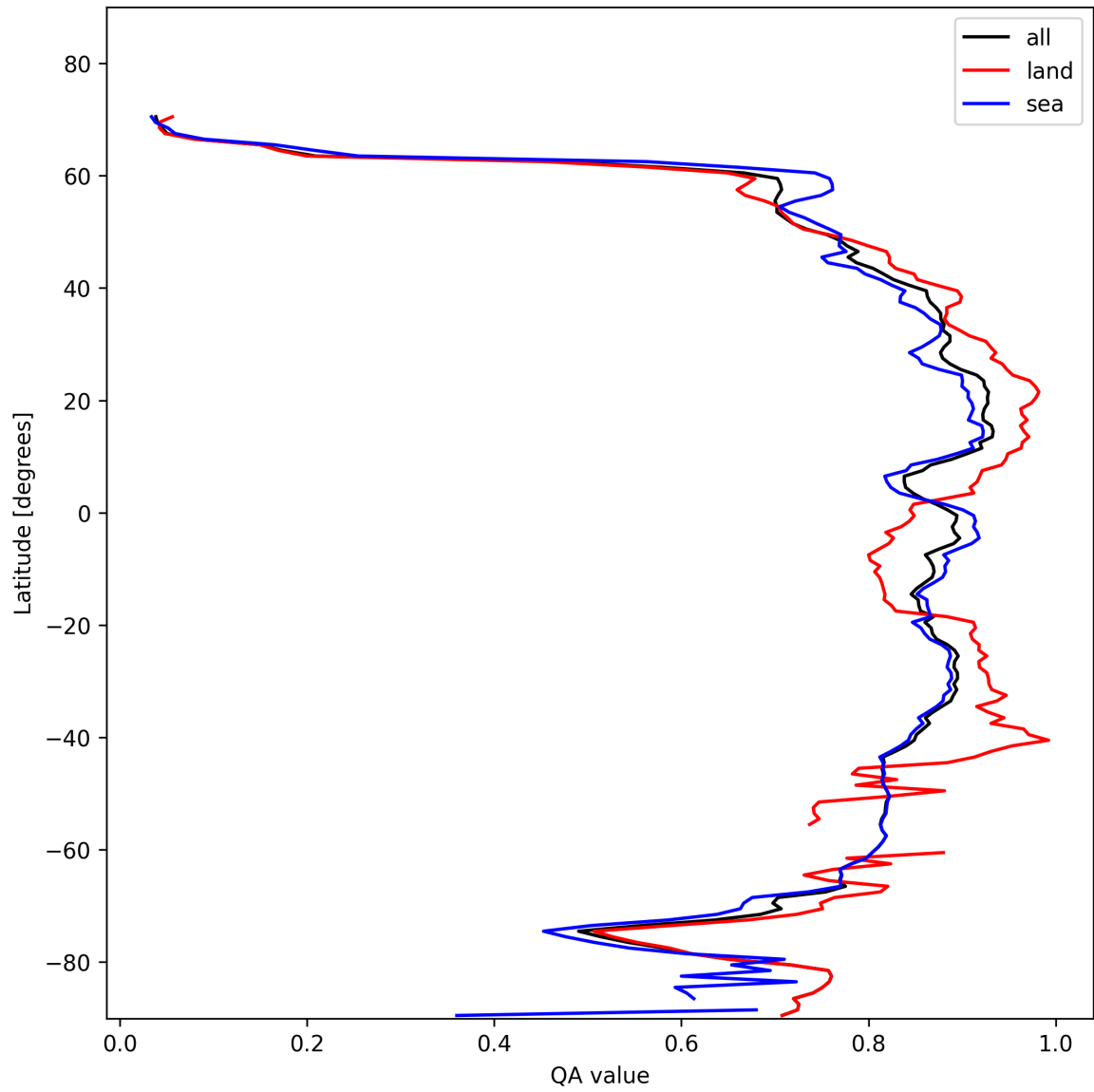
Figure 9: Zonal average of “QA value” for 2025-01-28 to 2025-01-29.
