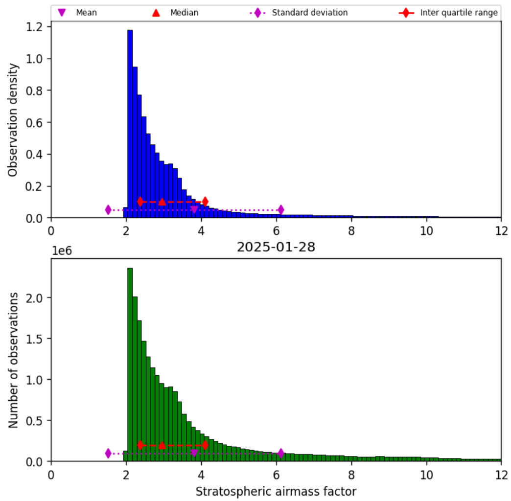
Figure 42: Histogram of “Stratospheric airmass factor” for 2025-01-28 to 2025-01-29
