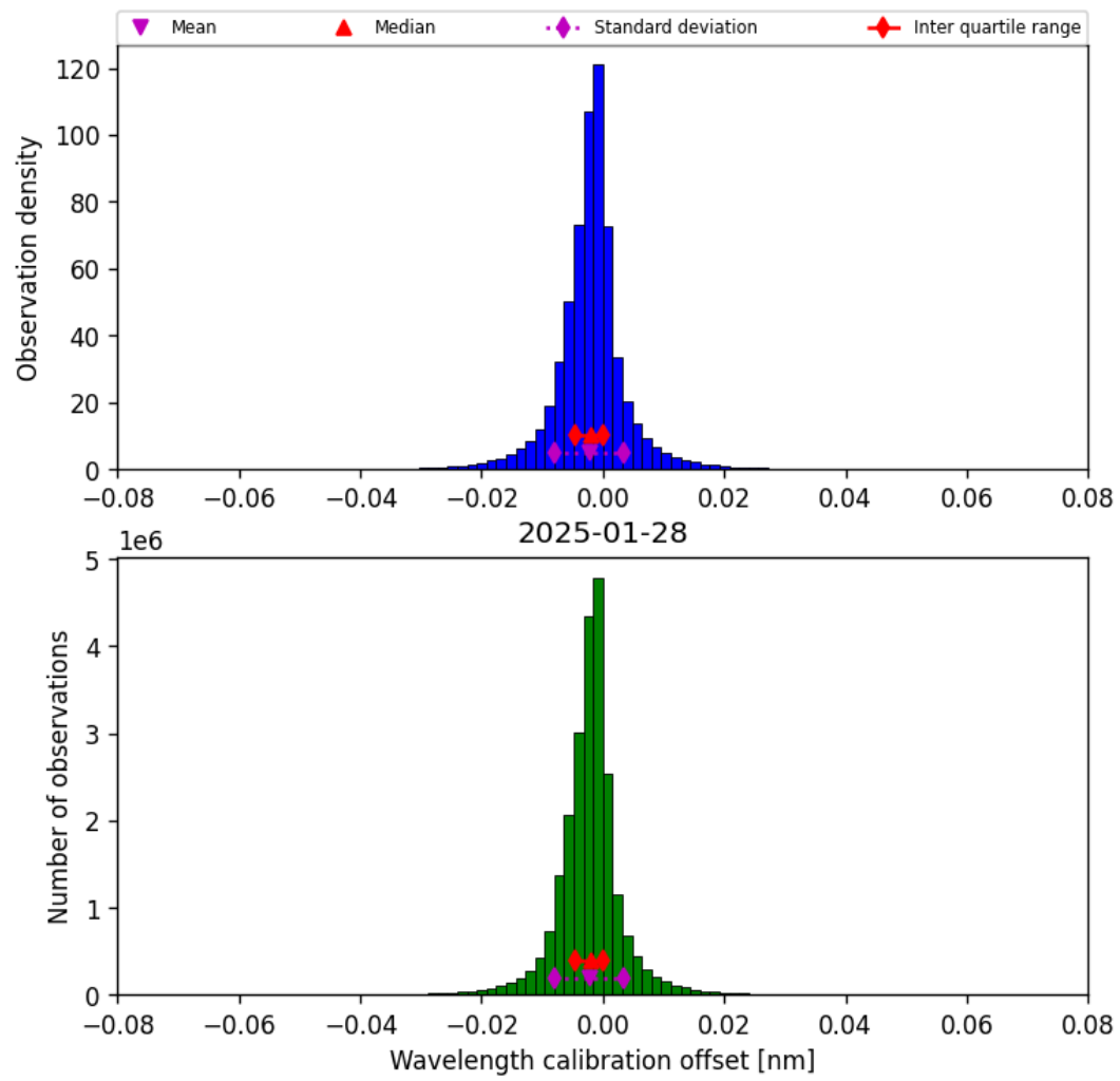
Figure 33: Histogram of “Wavelength calibration offset” for 2025-01-28 to 2025-01-29
