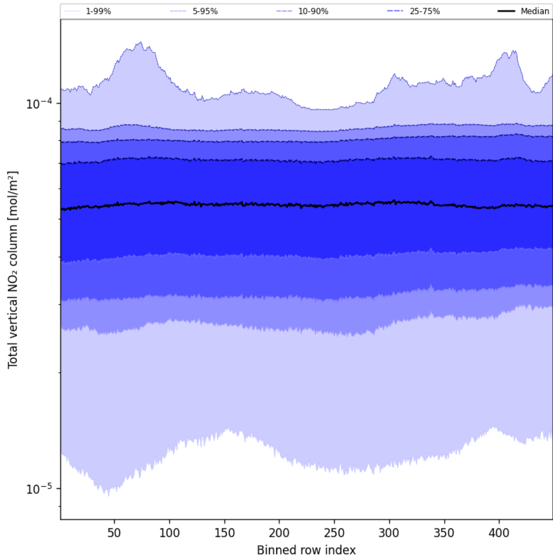
Figure 53: Along track statistics of “Total vertical NO 2 column” for 2025-01-28 to 2025-01-29
