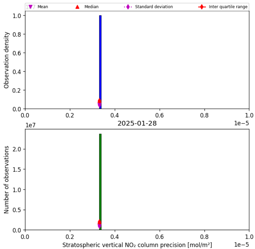
Figure 35: Histogram of “Stratospheric vertical NO 2 column precision” for 2025-01-28 to 2025-01-29
