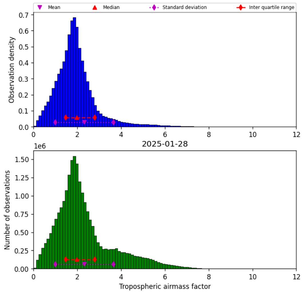
Figure 29: Histogram of “Tropospheric airmass factor” for 2025-01-28 to 2025-01-29
