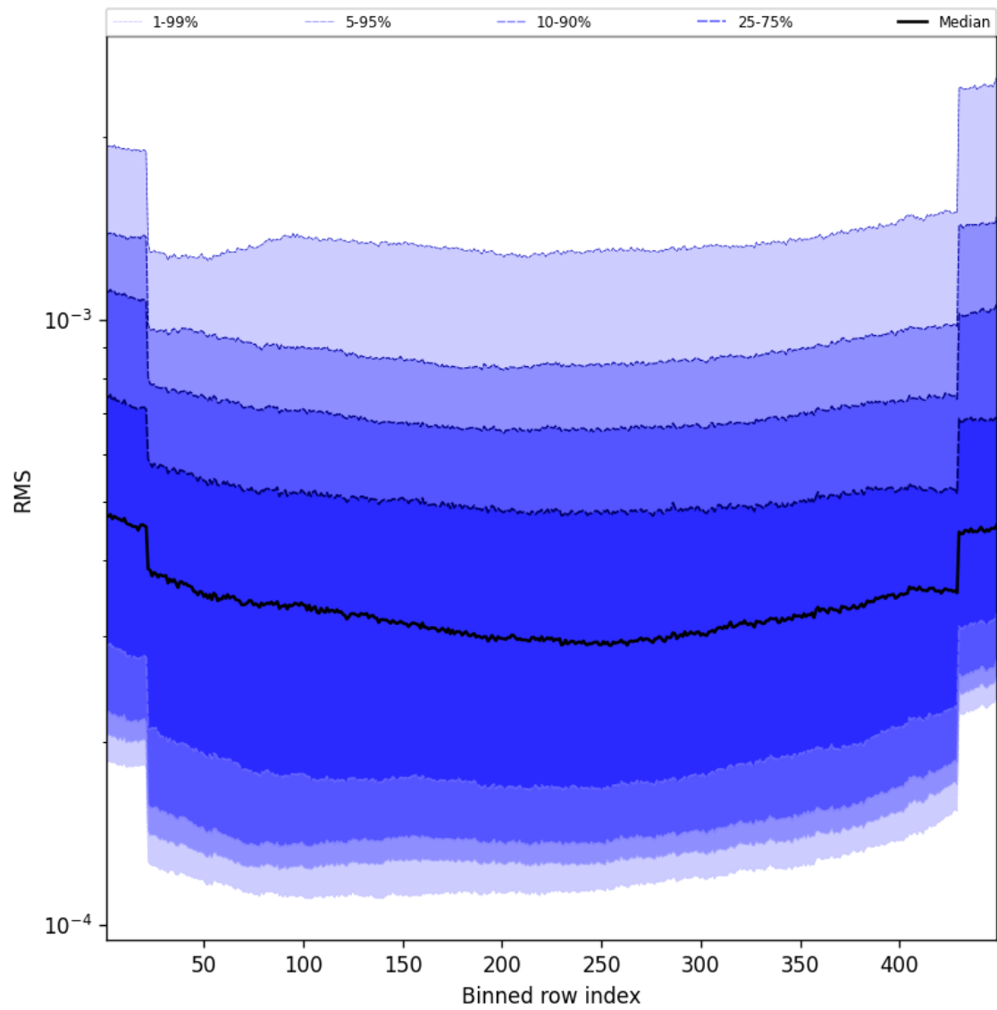
Figure 58: Along track statistics of “RMS” for 2025-01-28 to 2025-01-29
