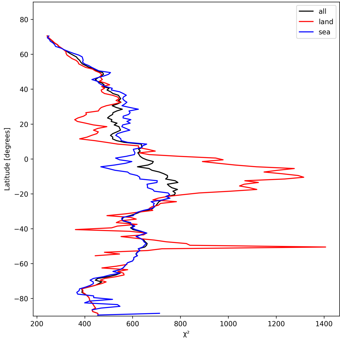
Figure 23: Zonal average of “ \chi^2 ” for 2025-01-28 to 2025-01-29.
