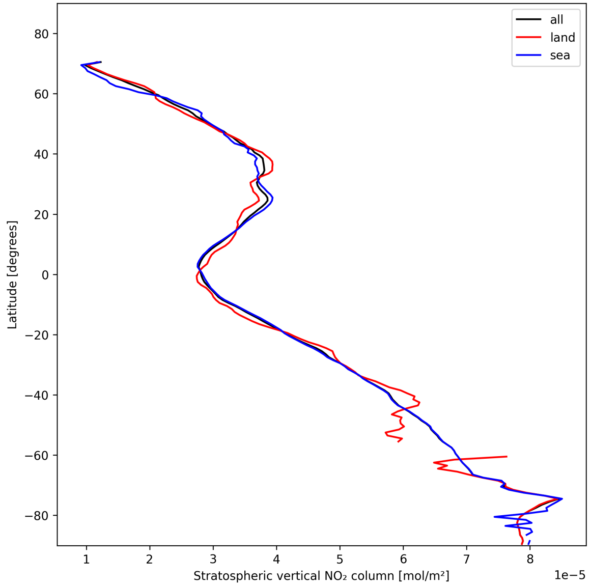
Figure 17: Zonal average of “Stratospheric vertical NO 2 column” for 2025-01-28 to 2025-01-29.
