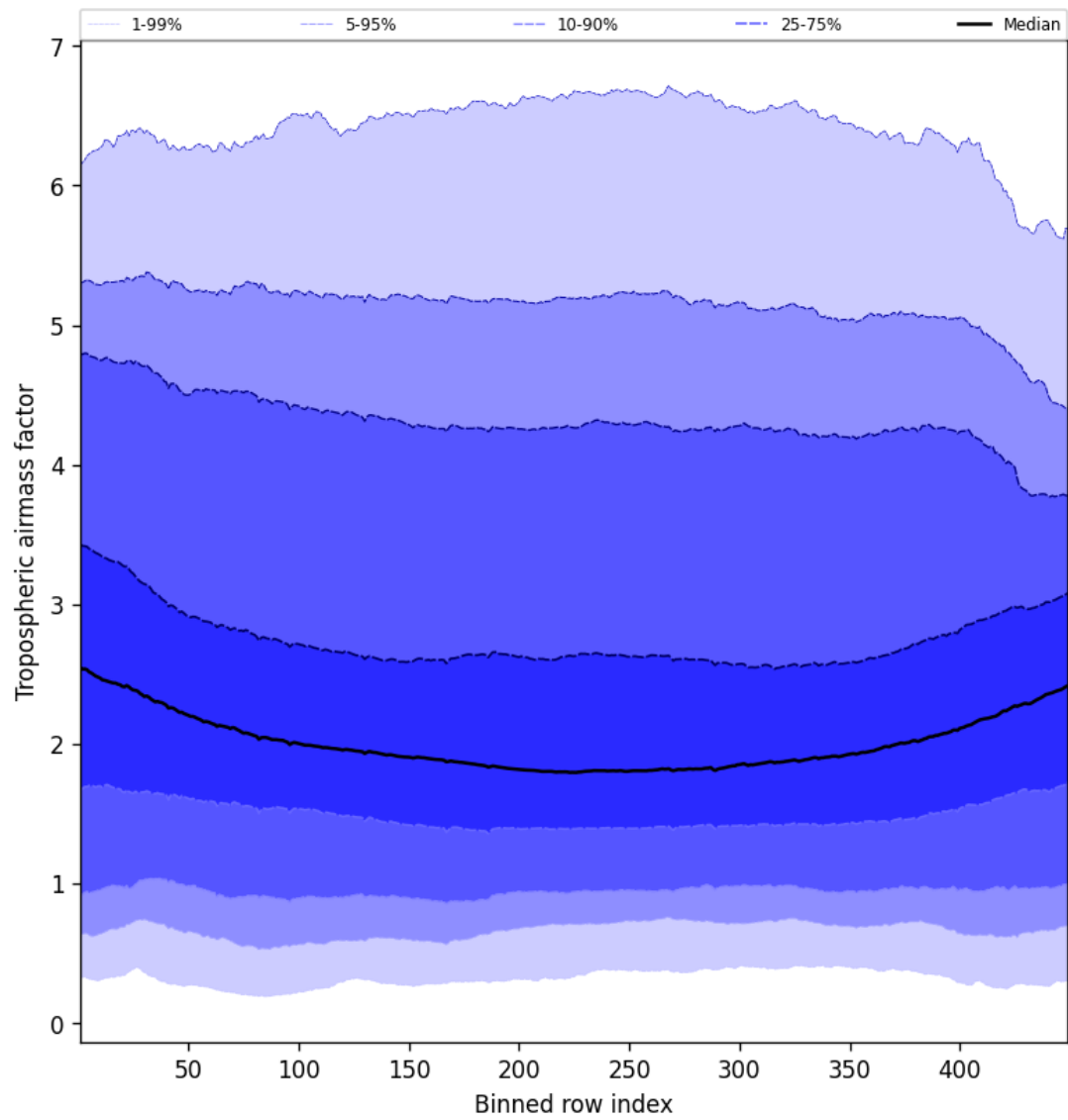
Figure 46: Along track statistics of “Tropospheric airmass factor” for 2025-01-28 to 2025-01-29
