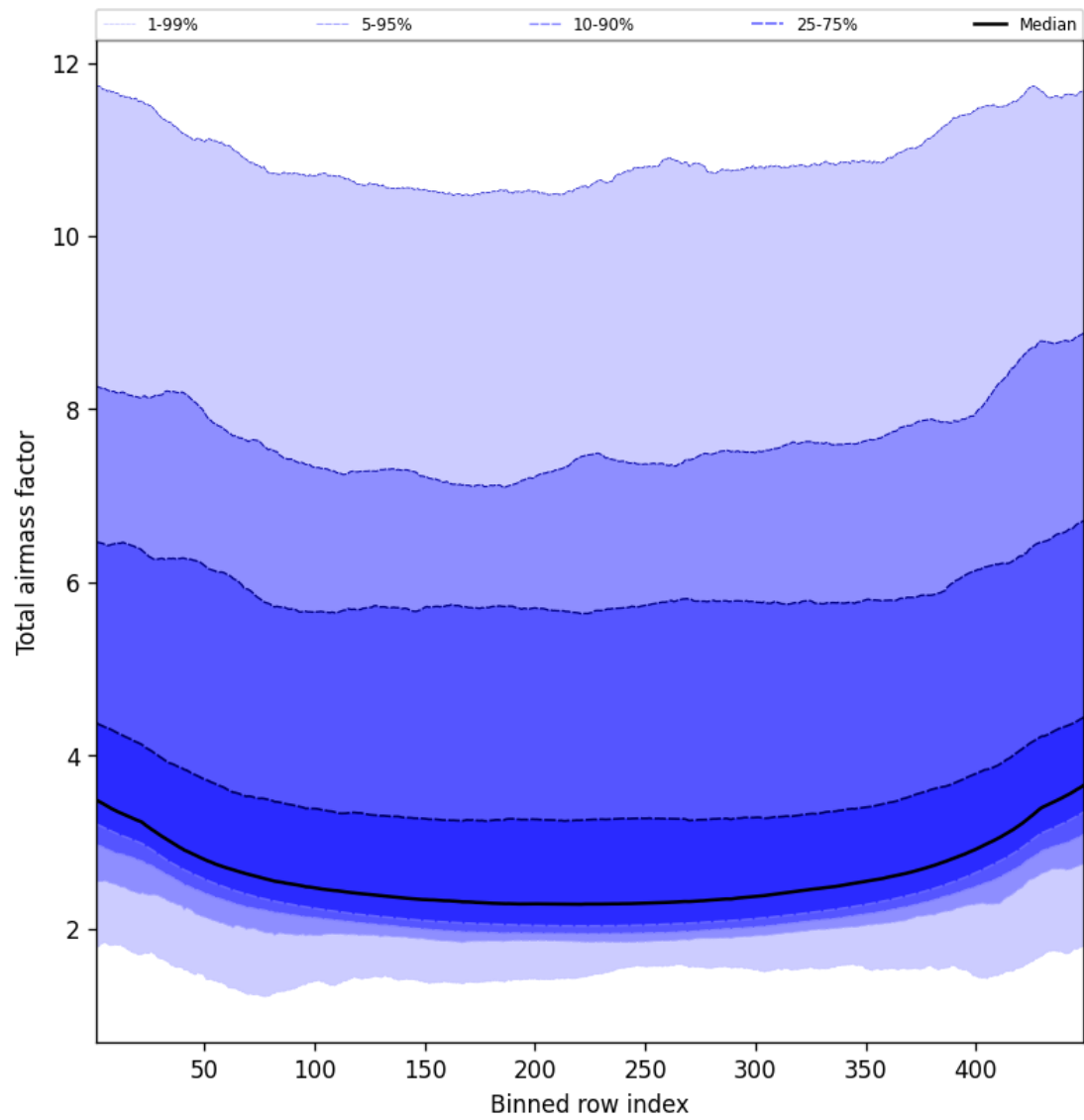
Figure 47: Along track statistics of “Total airmass factor” for 2025-01-28 to 2025-01-29
