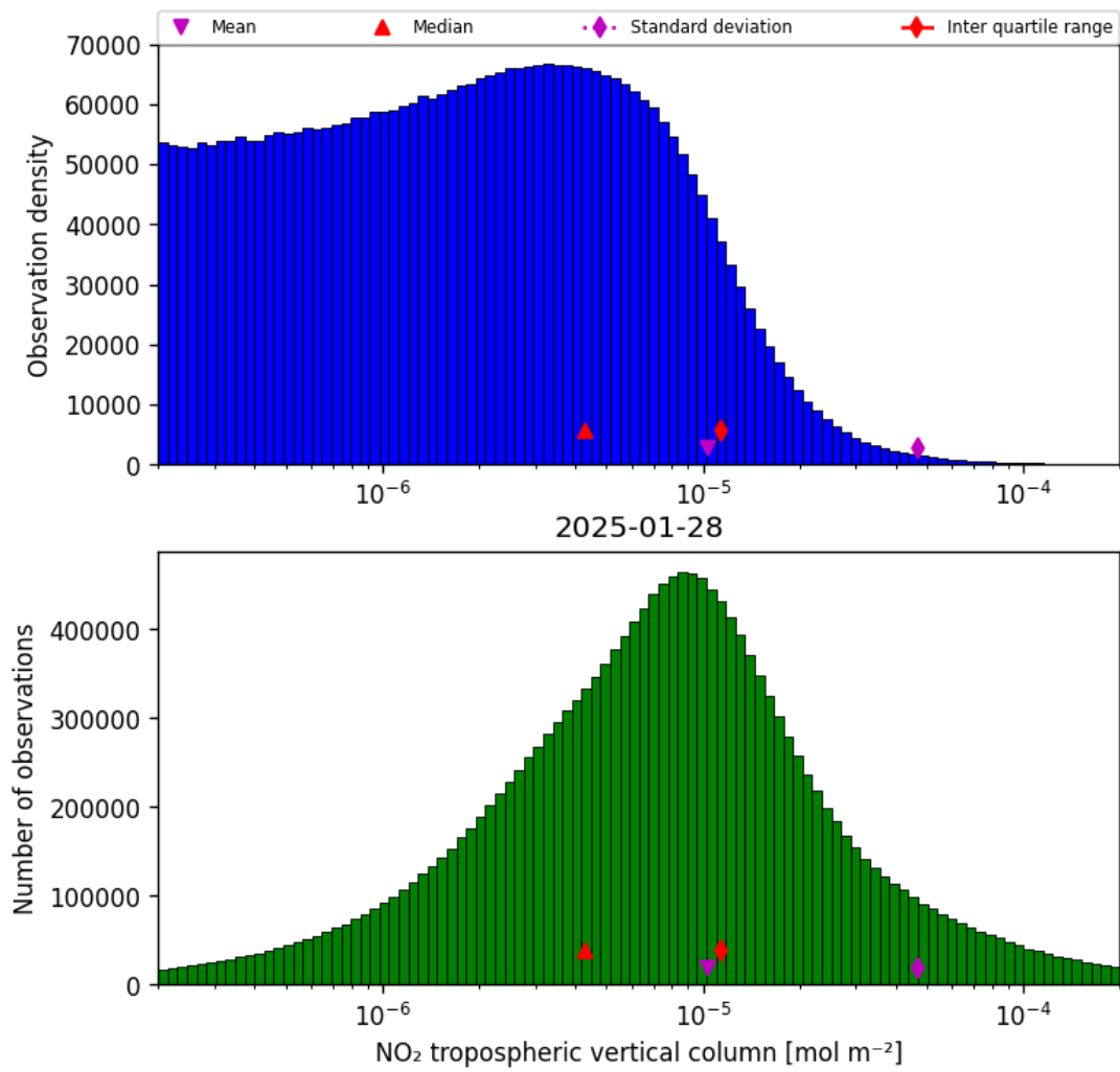
Figure 27: Histogram of “NO 2 tropospheric vertical column” for 2025-01-28 to 2025-01-29
