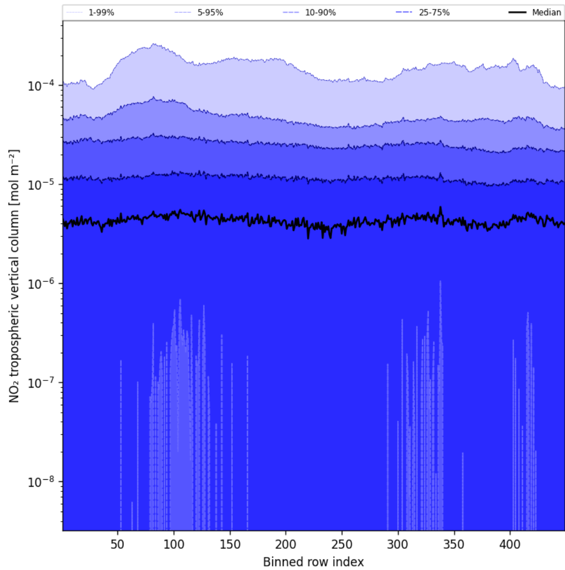
Figure 44: Along track statistics of “NO 2 tropospheric vertical column” for 2025-01-28 to 2025-01-29
