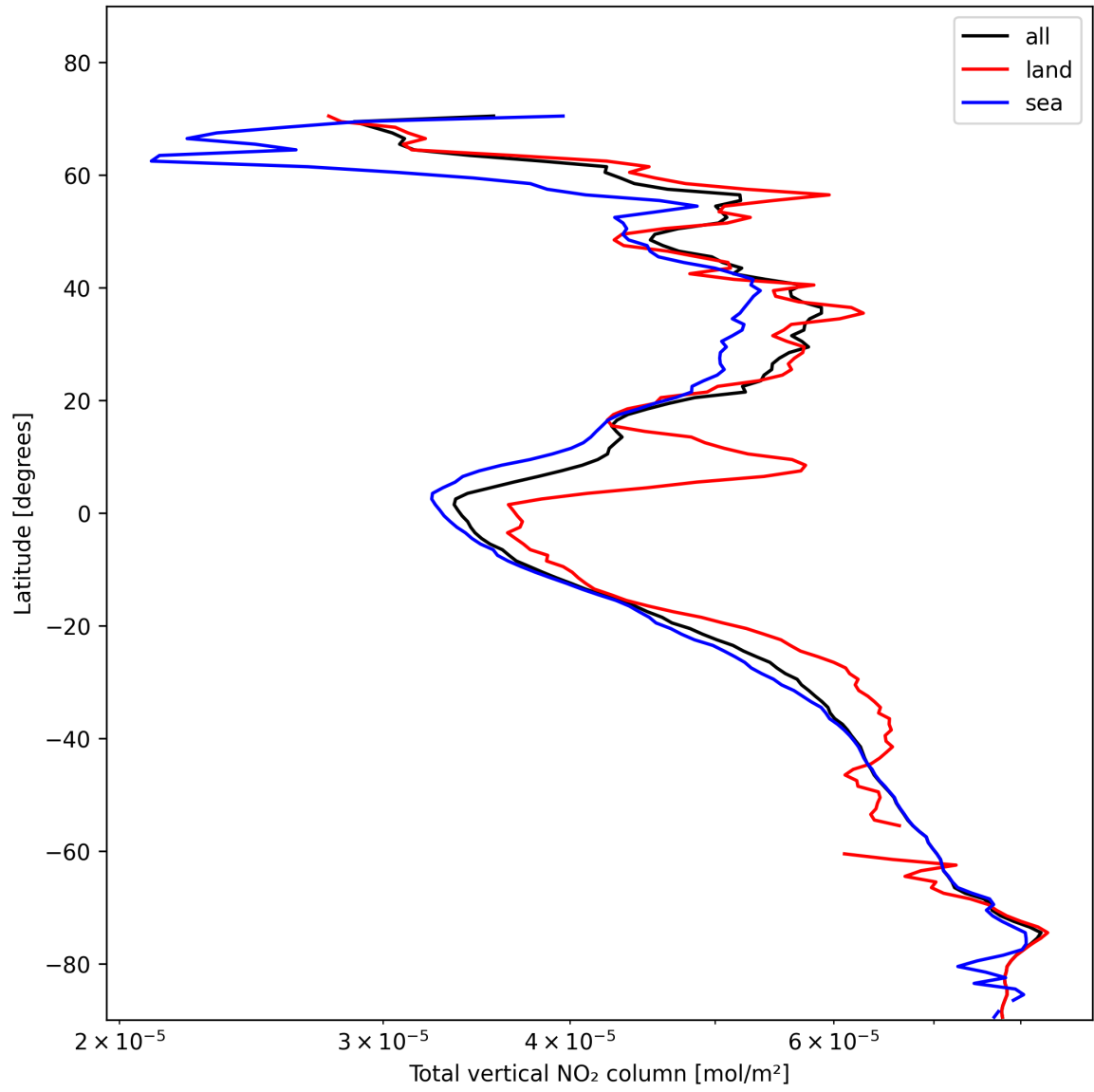
Figure 19: Zonal average of “Total vertical NO 2 column” for 2025-01-28 to 2025-01-29.
