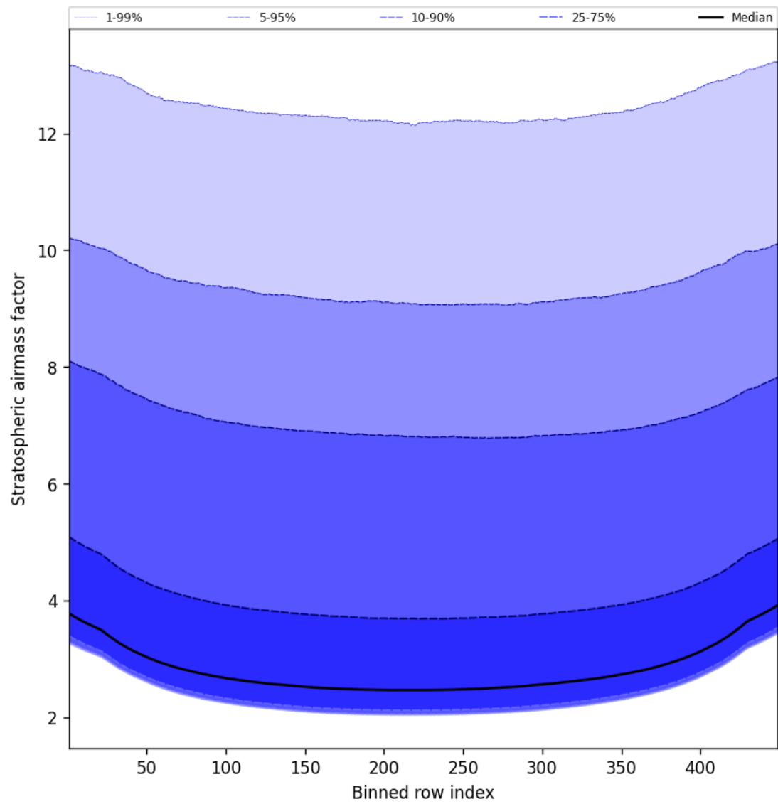
Figure 59: Along track statistics of “Stratospheric airmass factor” for 2025-01-28 to 2025-01-29
