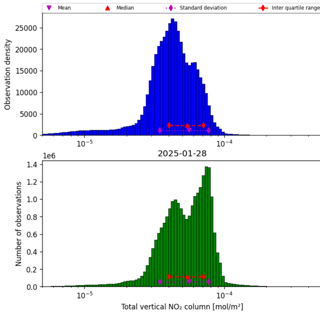
Figure 36: Histogram of “Total vertical NO 2 column” for 2025-01-28 to 2025-01-29
