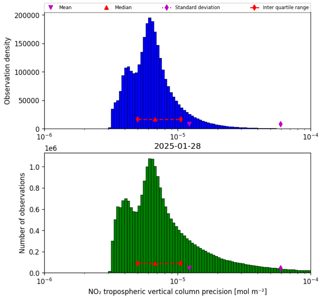
Figure 28: Histogram of “NO 2 tropospheric vertical column precision” for 2025-01-28 to 2025-01-29
