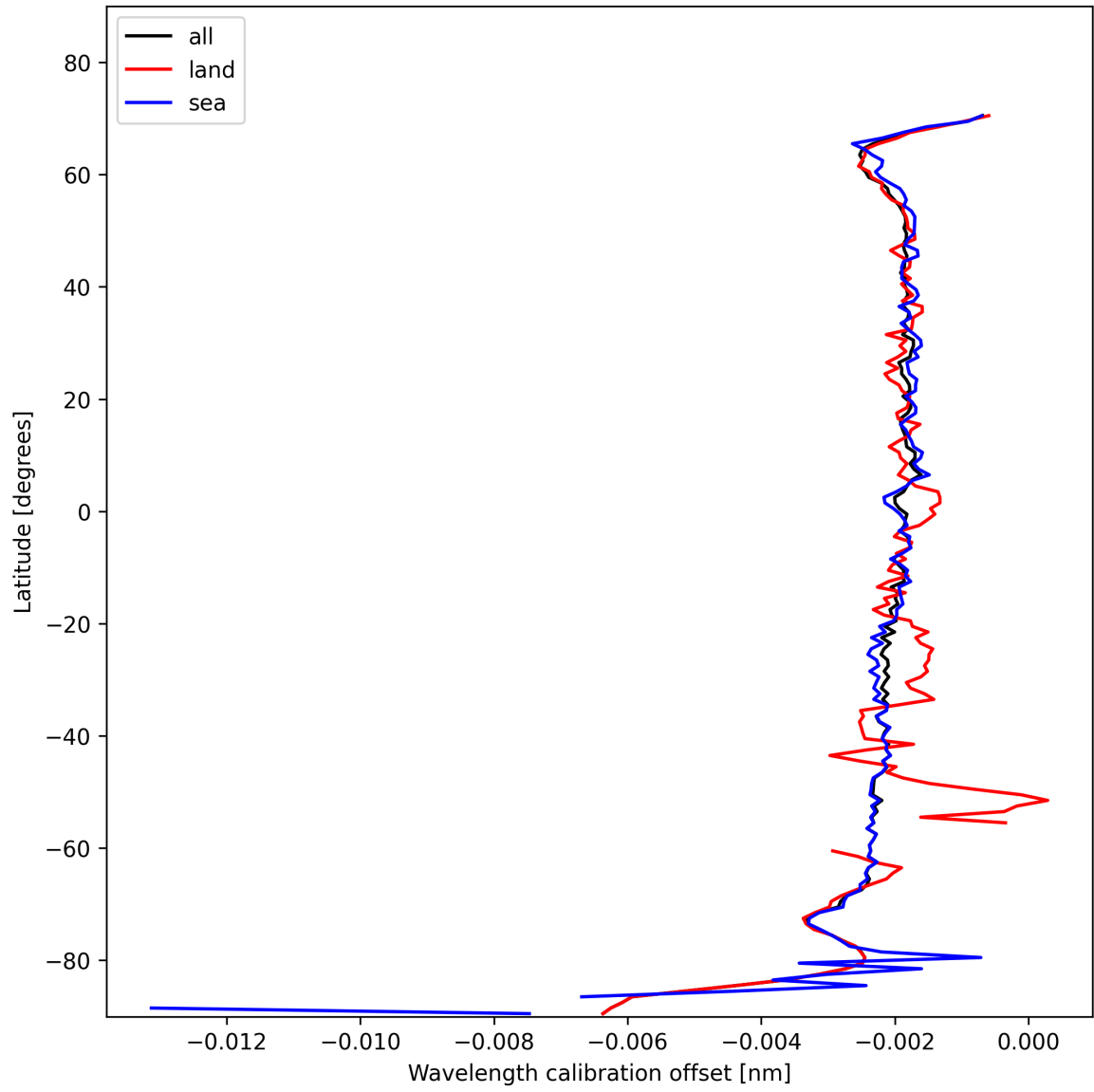
Figure 16: Zonal average of “Wavelength calibration offset” for 2025-01-28 to 2025-01-29.
