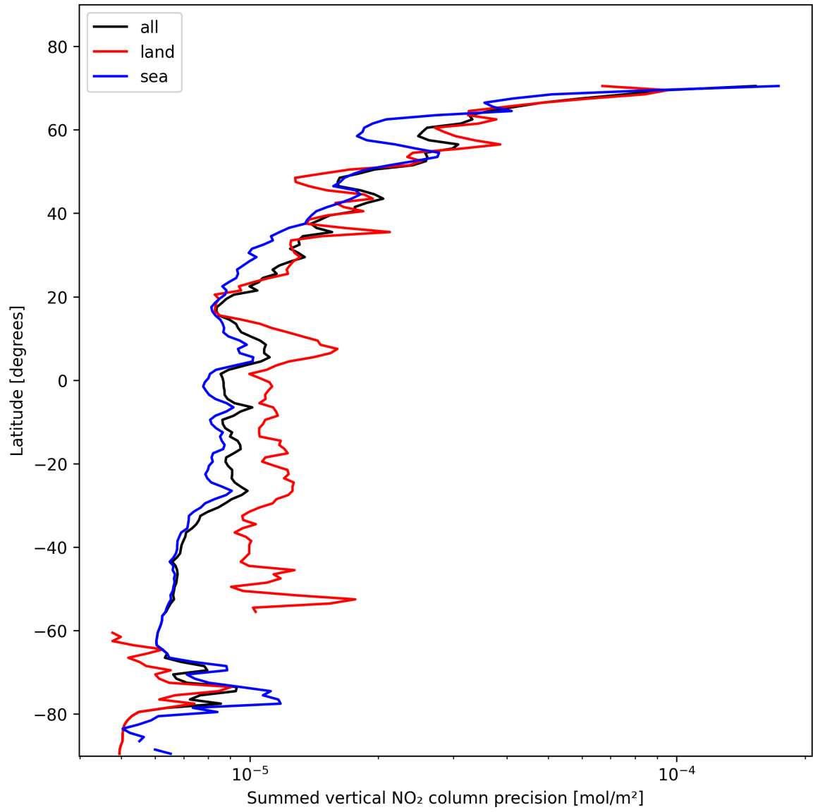
Figure 22: Zonal average of “Summed vertical NO 2 column precision” for 2025-01-28 to 2025-01-29.
