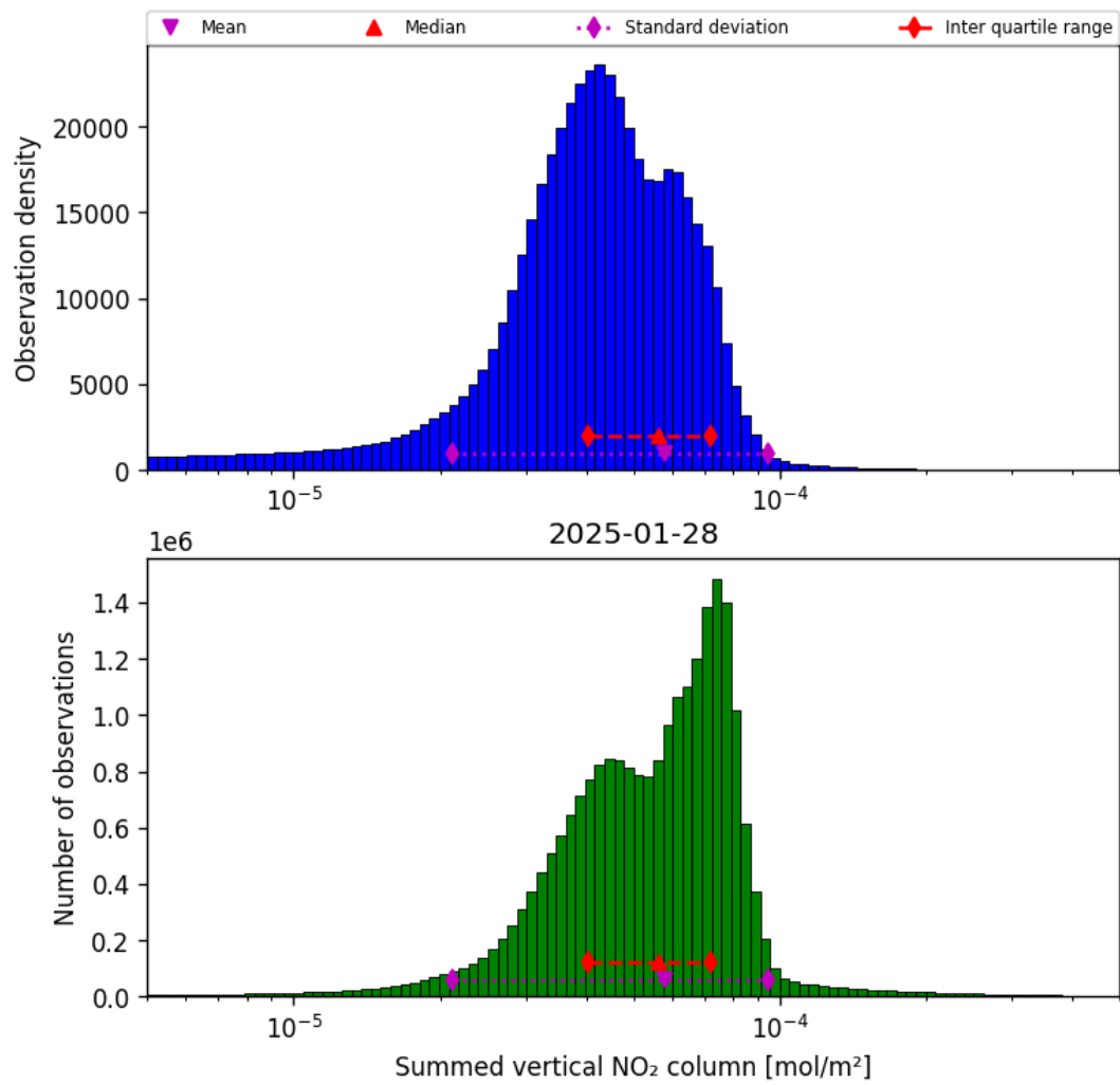
Figure 38: Histogram of “Summed vertical NO 2 column” for 2025-01-28 to 2025-01-29
