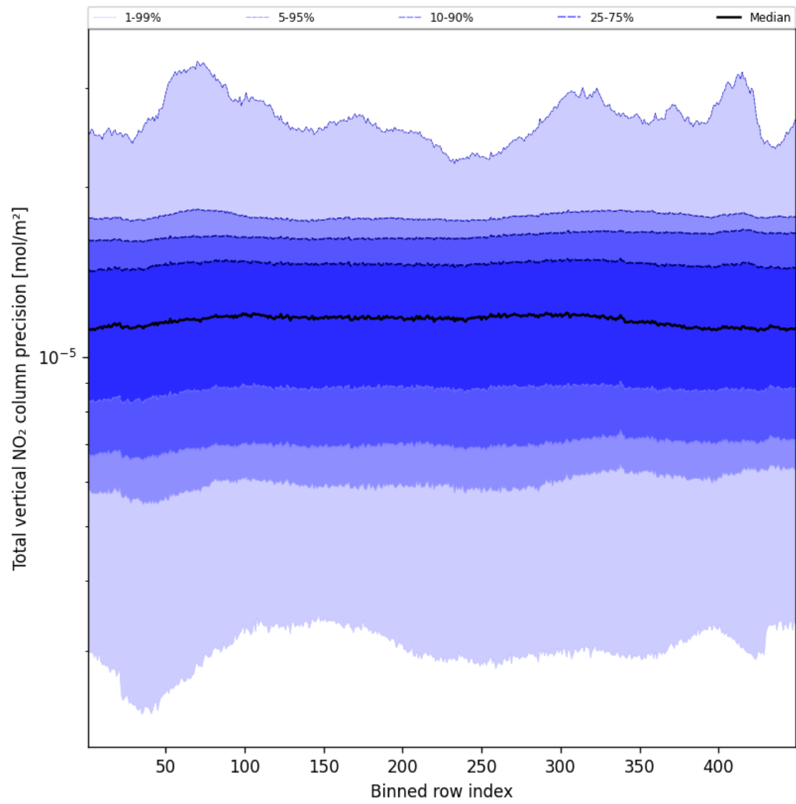
Figure 54: Along track statistics of “Total vertical NO 2 column precision” for 2025-01-28 to 2025-01-29
