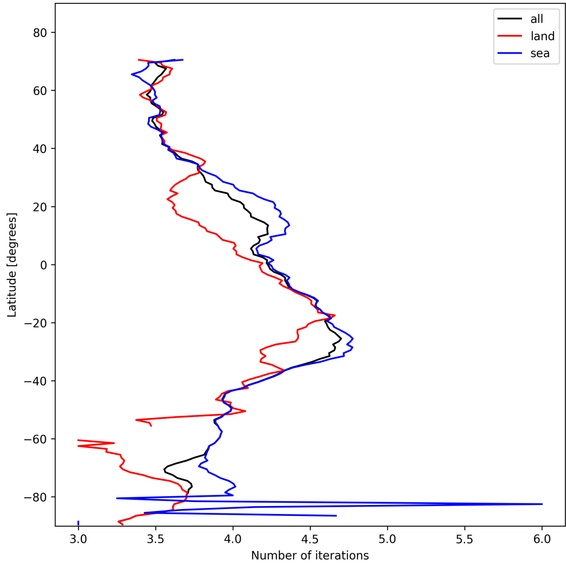
Figure 15: Zonal average of “Number of iterations” for 2025-01-28 to 2025-01-29.
