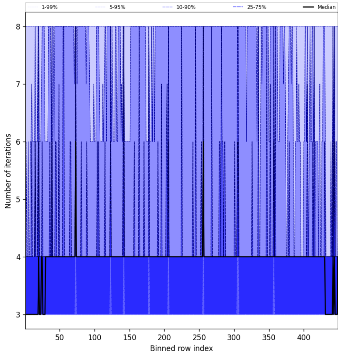
Figure 49: Along track statistics of “Number of iterations” for 2025-01-28 to 2025-01-29
