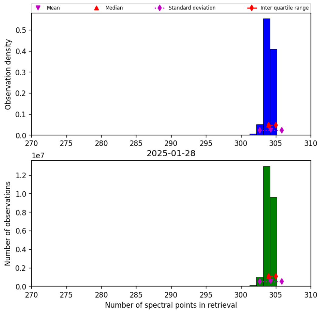
Figure 31: Histogram of “Number of spectral points in retrieval” for 2025-01-28 to 2025-01-29
