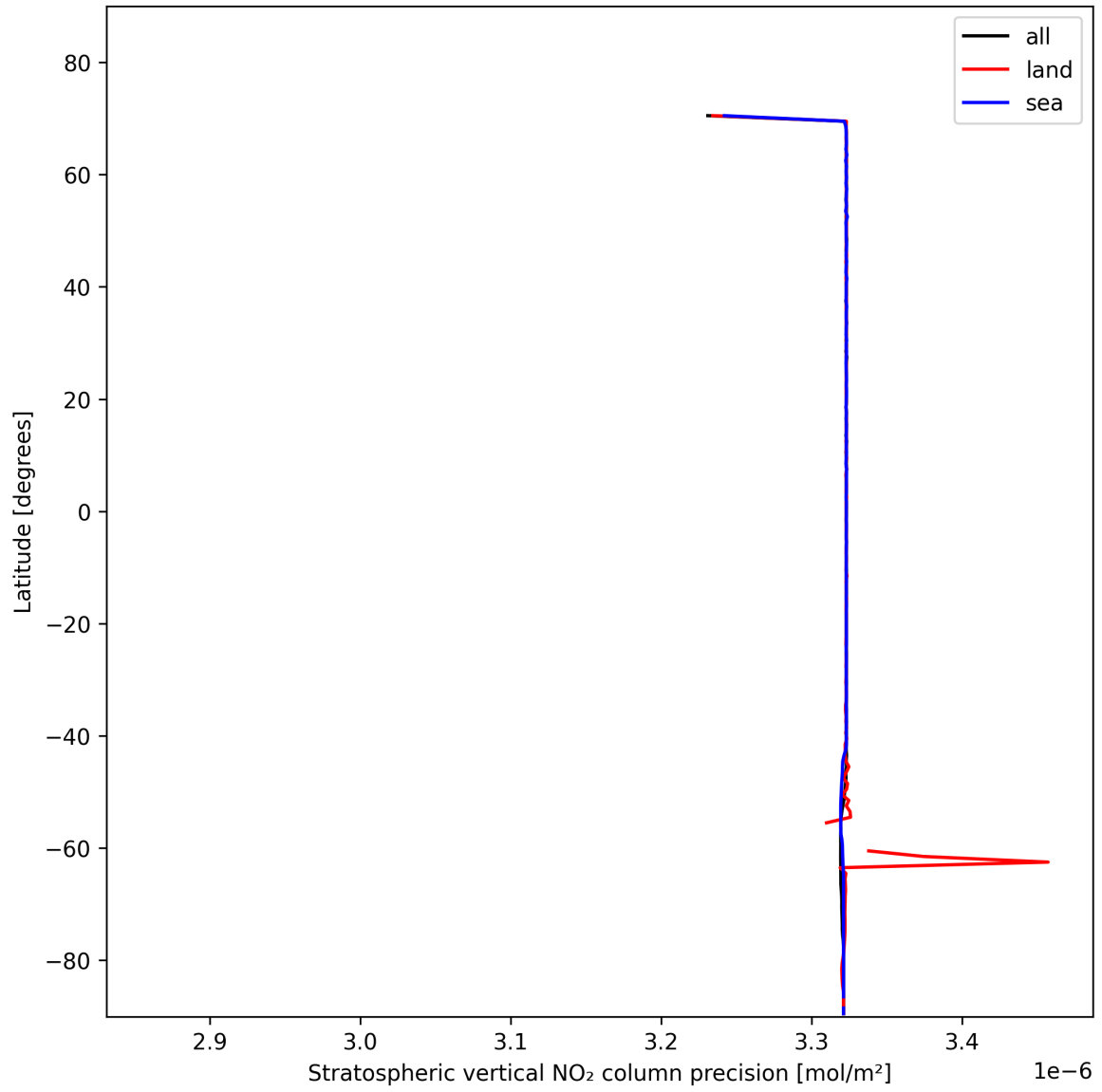
Figure 18: Zonal average of "Stratospheric vertical NO 2 column precision" for 2025-01-28 to 2025-01-29.
