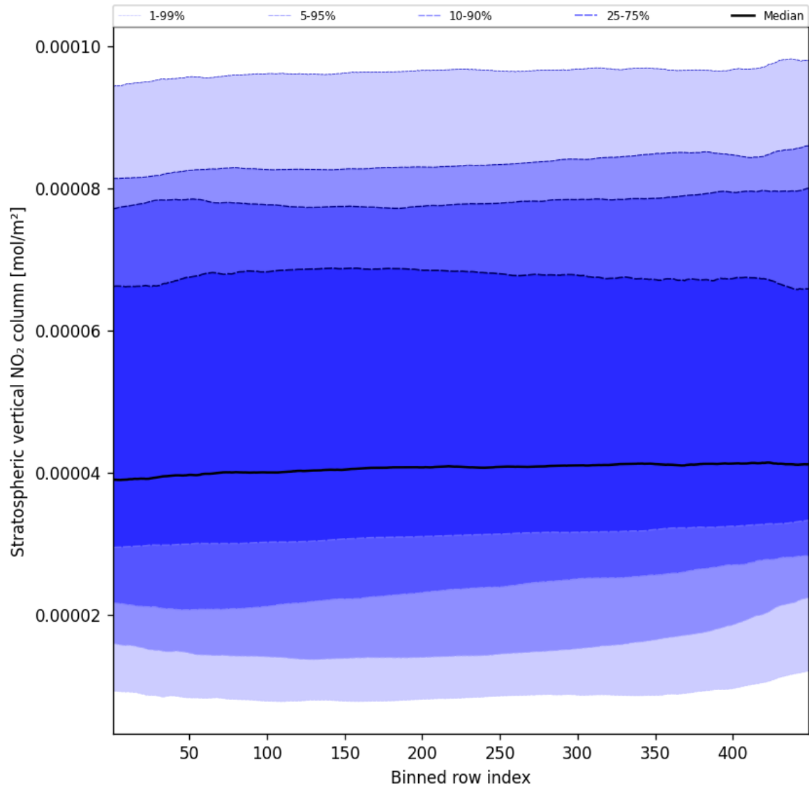
Figure 51: Along track statistics of “Stratospheric vertical NO 2 column” for 2025-01-28 to 2025-01-29
