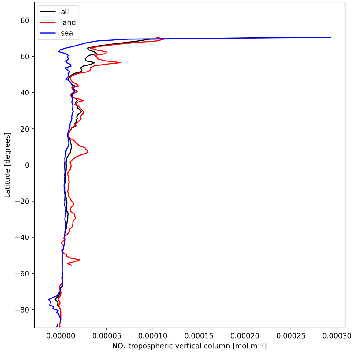
Figure 10: Zonal average of “NO 2 tropospheric vertical column” for 2025-01-28 to 2025-01-29.
