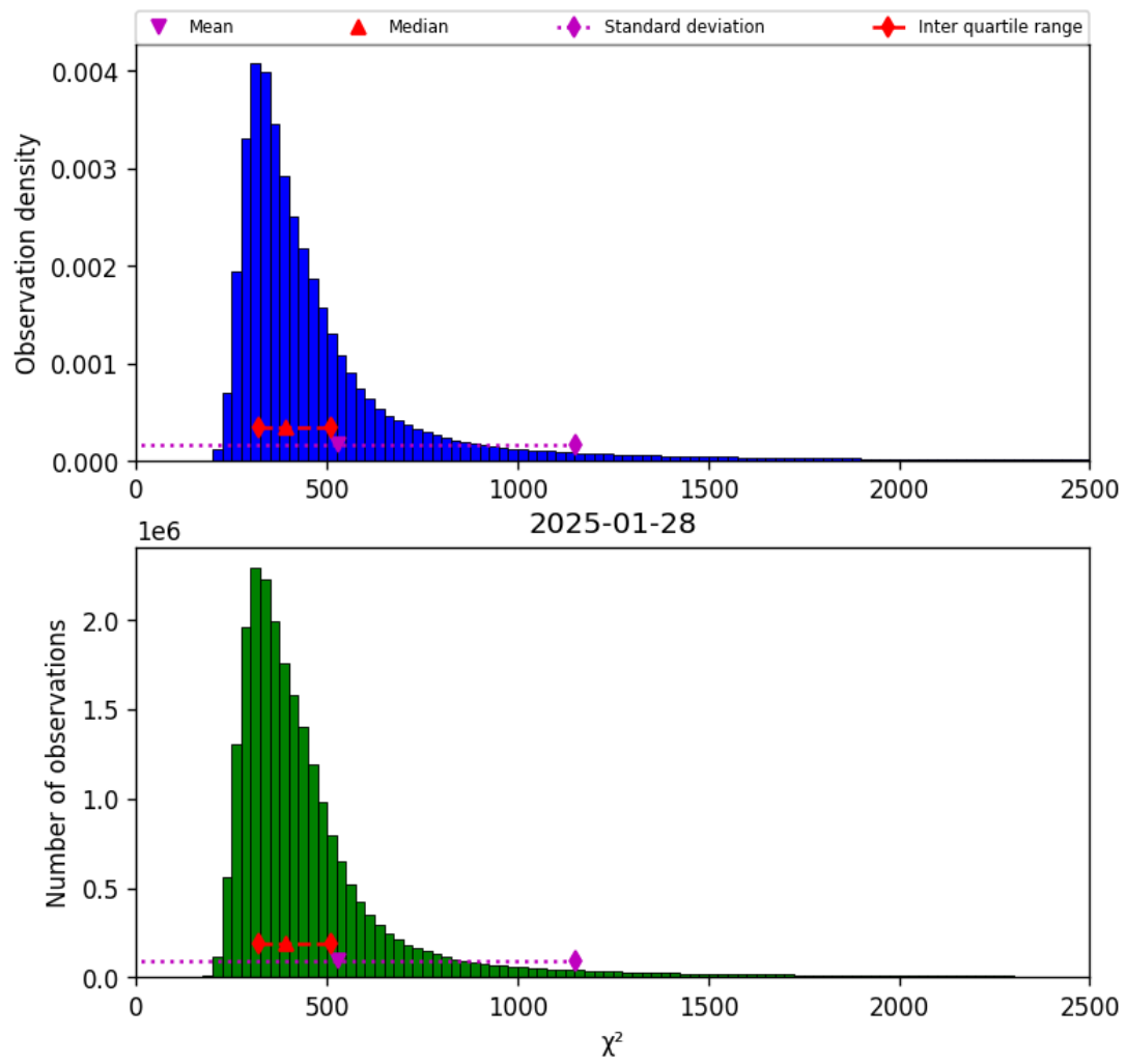
Figure 40: Histogram of “ \chi^2 ” for 2025-01-28 to 2025-01-29
