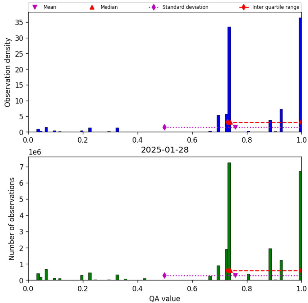
Figure 26: Histogram of “QA value” for 2025-01-28 to 2025-01-29
