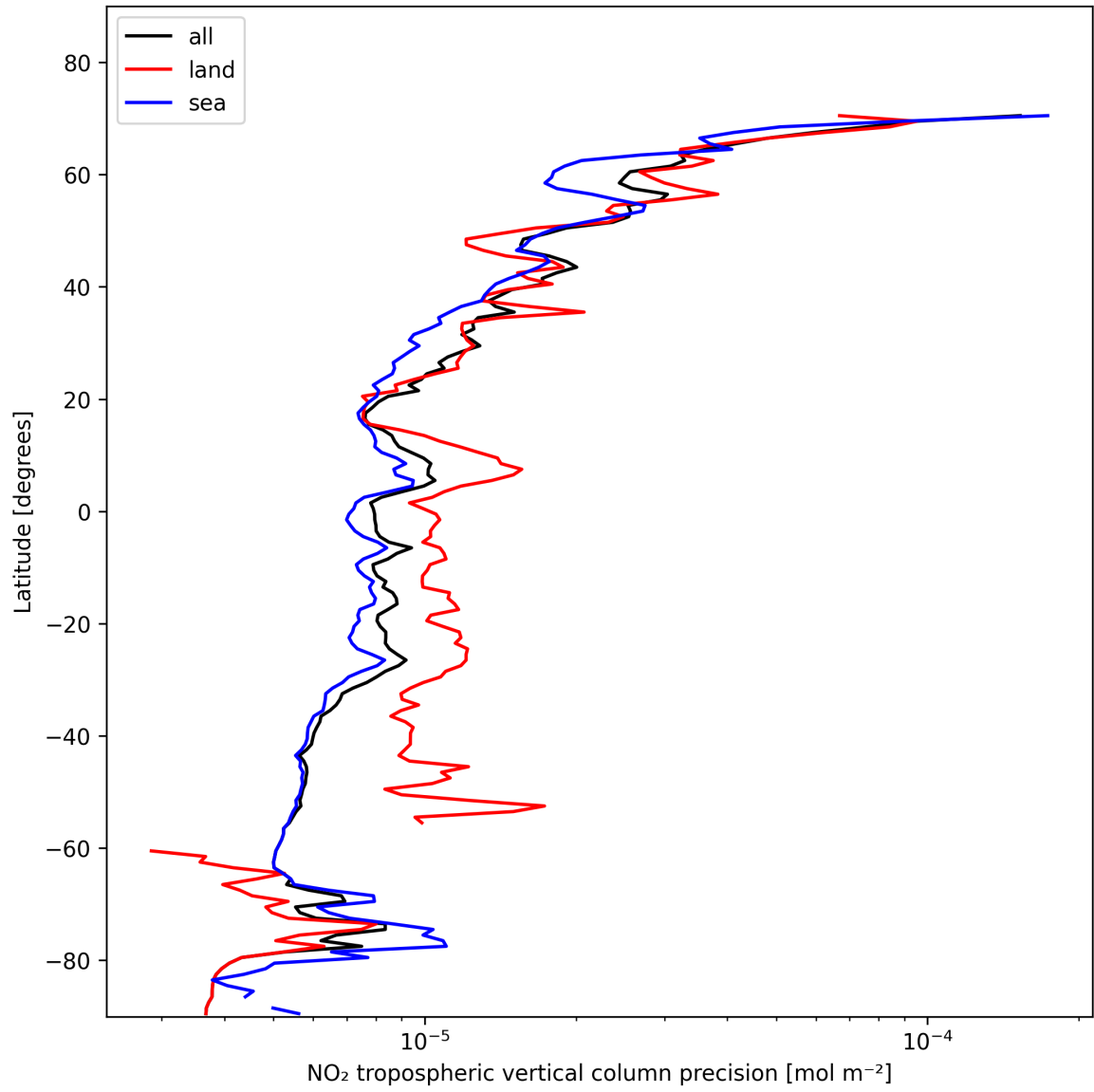
Figure 11: Zonal average of “NO 2 tropospheric vertical column precision” for 2025-01-28 to 2025-01-29.
