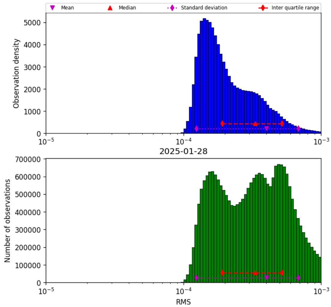
Figure 41: Histogram of “RMS” for 2025-01-28 to 2025-01-29
