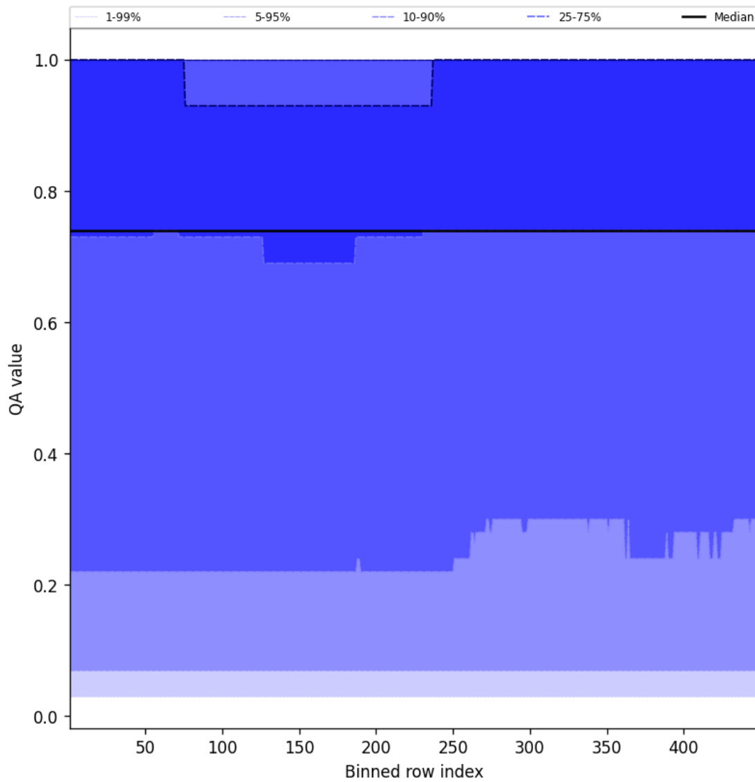
Figure 43: Along track statistics of “QA value” for 2025-01-28 to 2025-01-29
