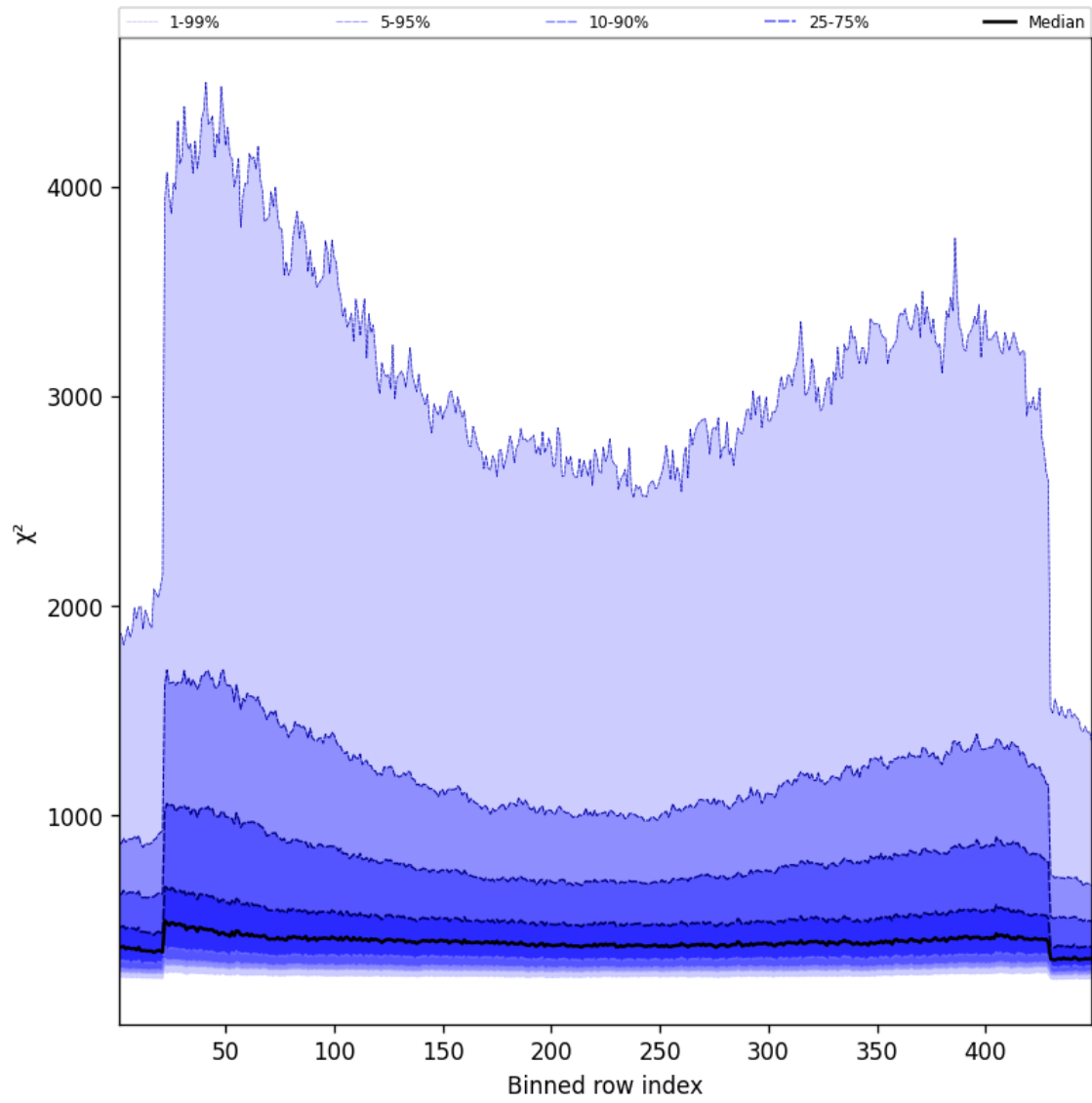
Figure 57: Along track statistics of “ \chi^2 ” for 2025-01-28 to 2025-01-29
