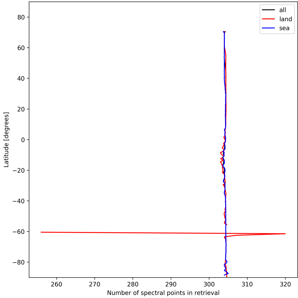
Figure 14: Zonal average of “Number of spectral points in retrieval” for 2025-01-29 to 2025-01-30.
