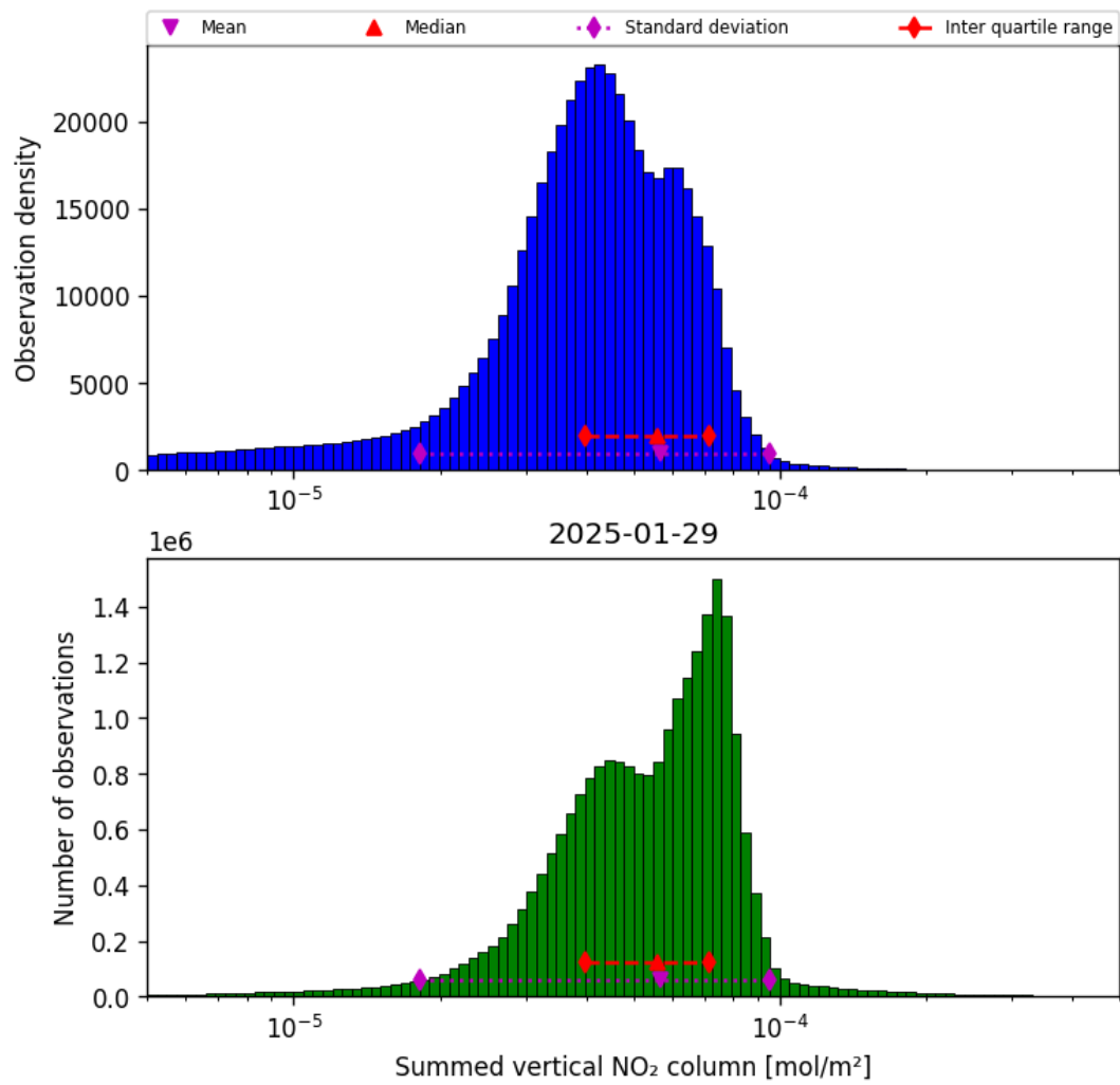
Figure 38: Histogram of “Summed vertical NO 2 column” for 2025-01-29 to 2025-01-30
