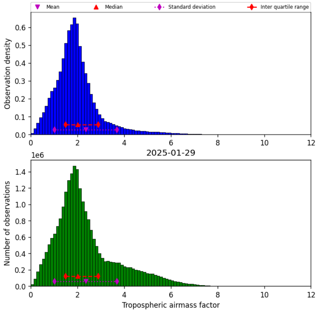
Figure 29: Histogram of “Tropospheric airmass factor” for 2025-01-29 to 2025-01-30
