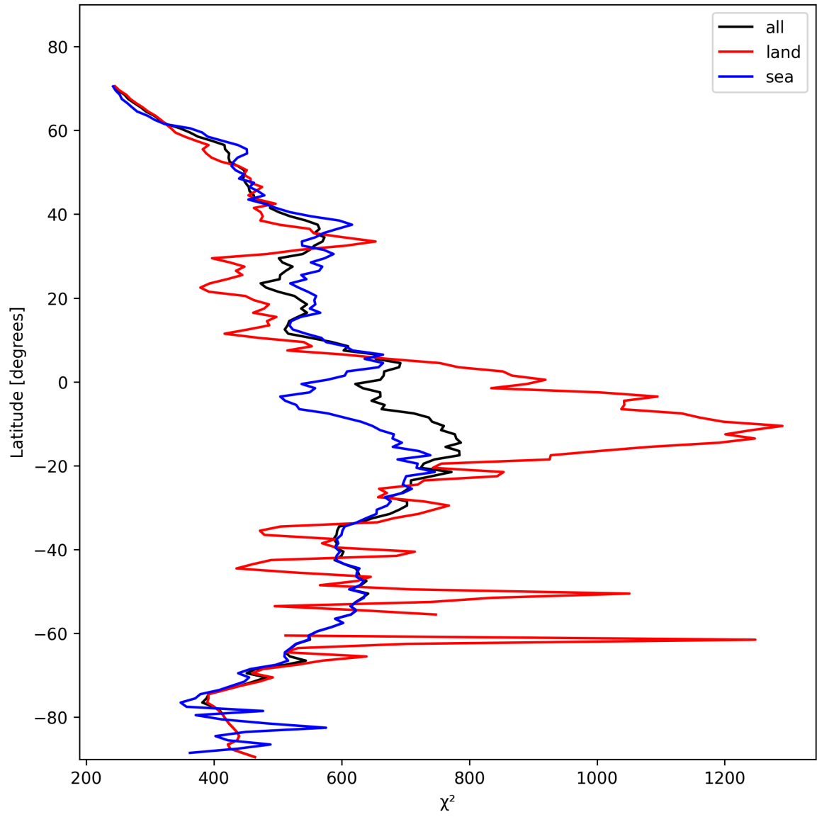
Figure 23: Zonal average of “ \chi^2 ” for 2025-01-29 to 2025-01-30.
