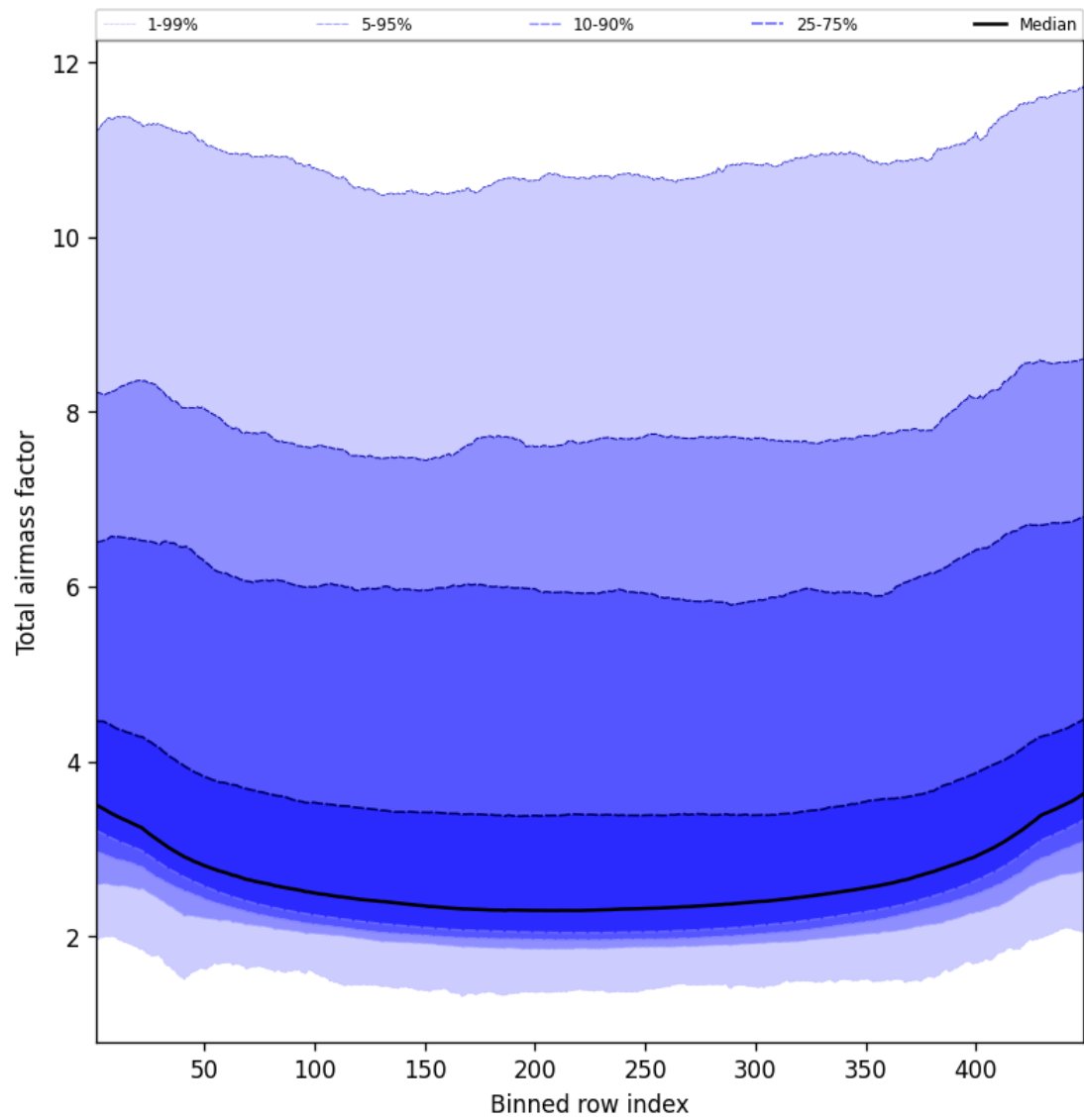
Figure 47: Along track statistics of “Total airmass factor” for 2025-01-29 to 2025-01-30
