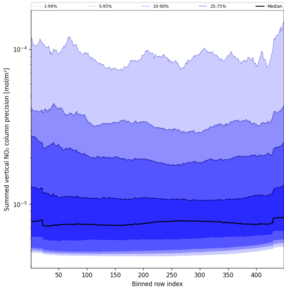
Figure 56: Along track statistics of “Summed vertical NO 2 column precision” for 2025-01-29 to 2025-01-30
