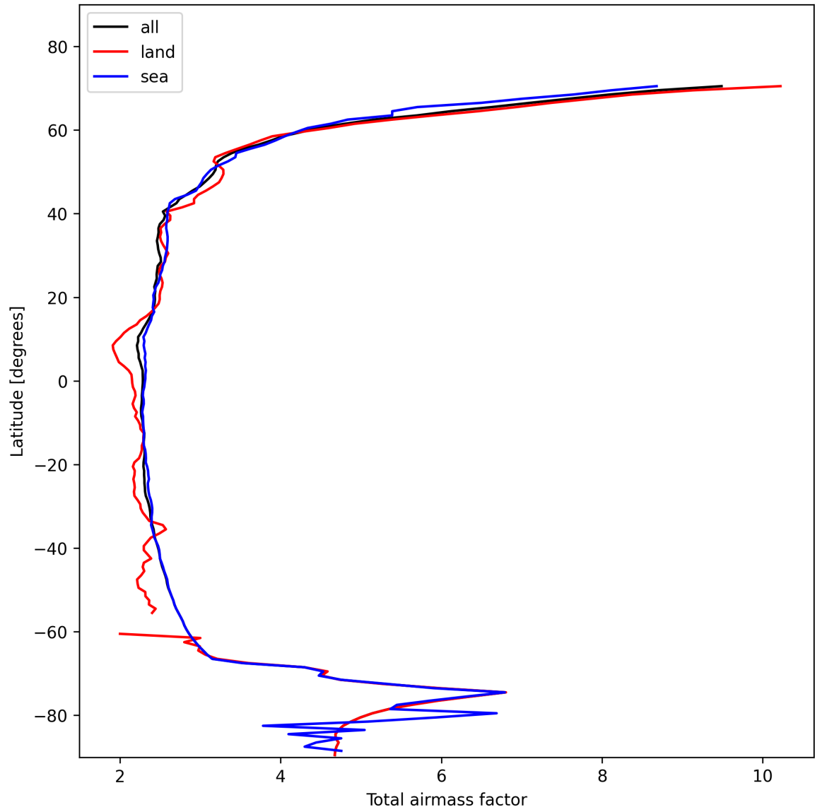
Figure 13: Zonal average of “Total airmass factor” for 2025-01-29 to 2025-01-30.
