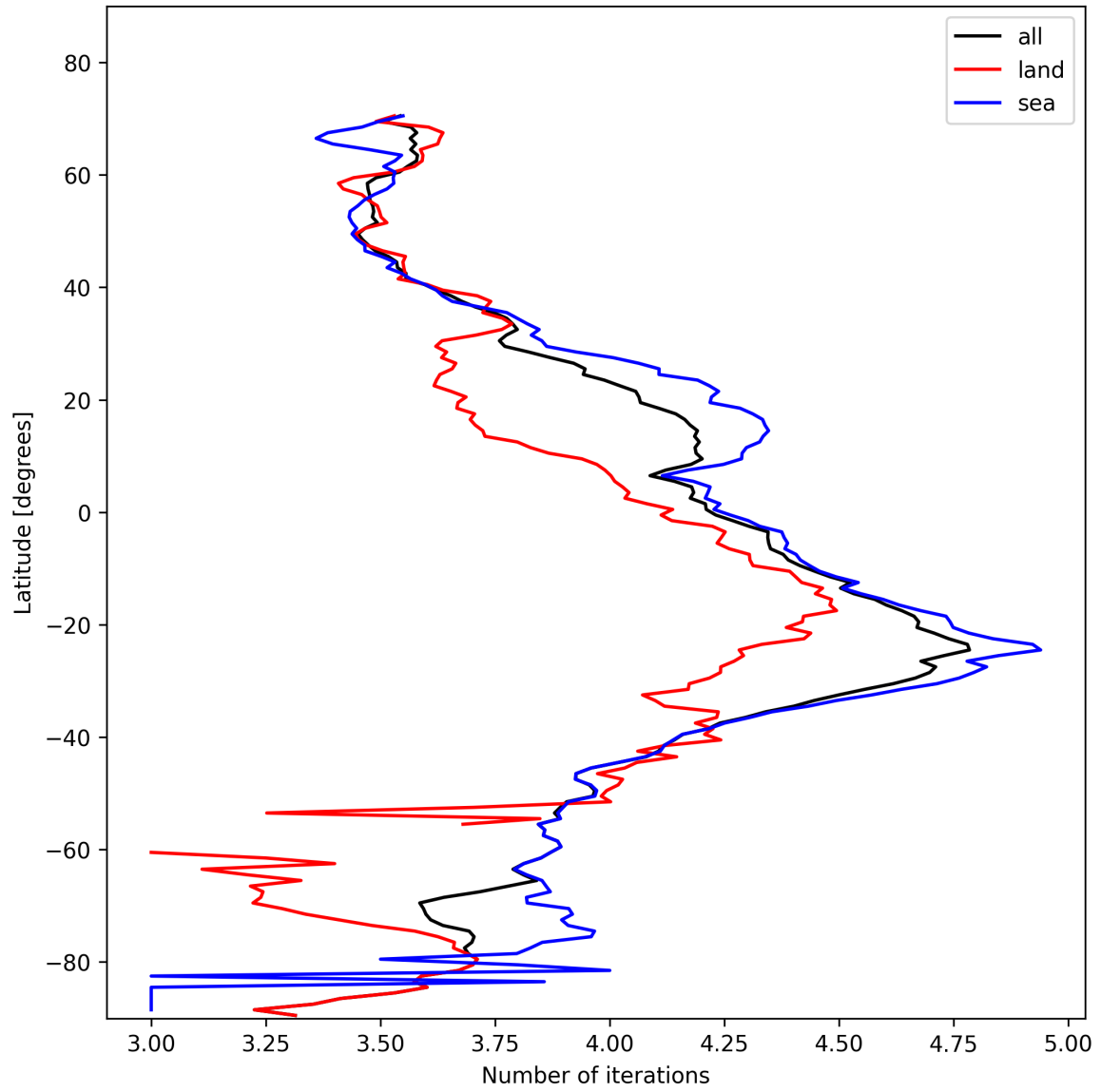
Figure 15: Zonal average of “Number of iterations” for 2025-01-29 to 2025-01-30.
