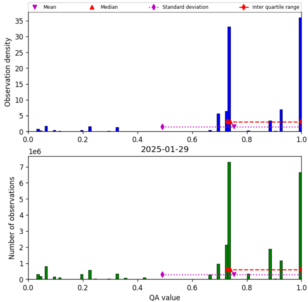
Figure 26: Histogram of “QA value” for 2025-01-29 to 2025-01-30
