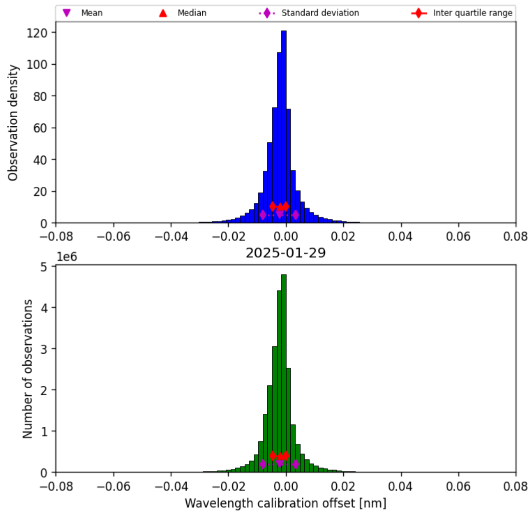
Figure 33: Histogram of “Wavelength calibration offset” for 2025-01-29 to 2025-01-30
