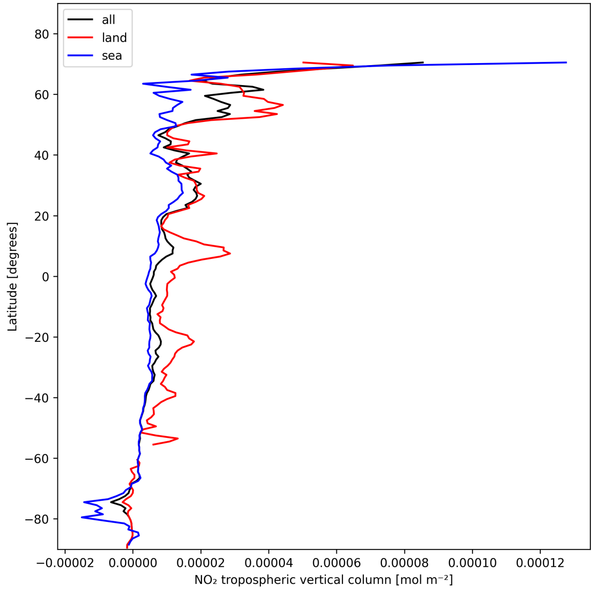
Figure 10: Zonal average of “NO 2 tropospheric vertical column” for 2025-01-29 to 2025-01-30.
