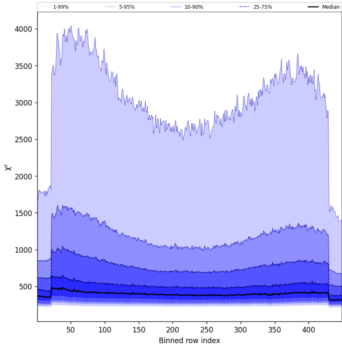
Figure 57: Along track statistics of “ \chi^2 ” for 2025-01-29 to 2025-01-30
