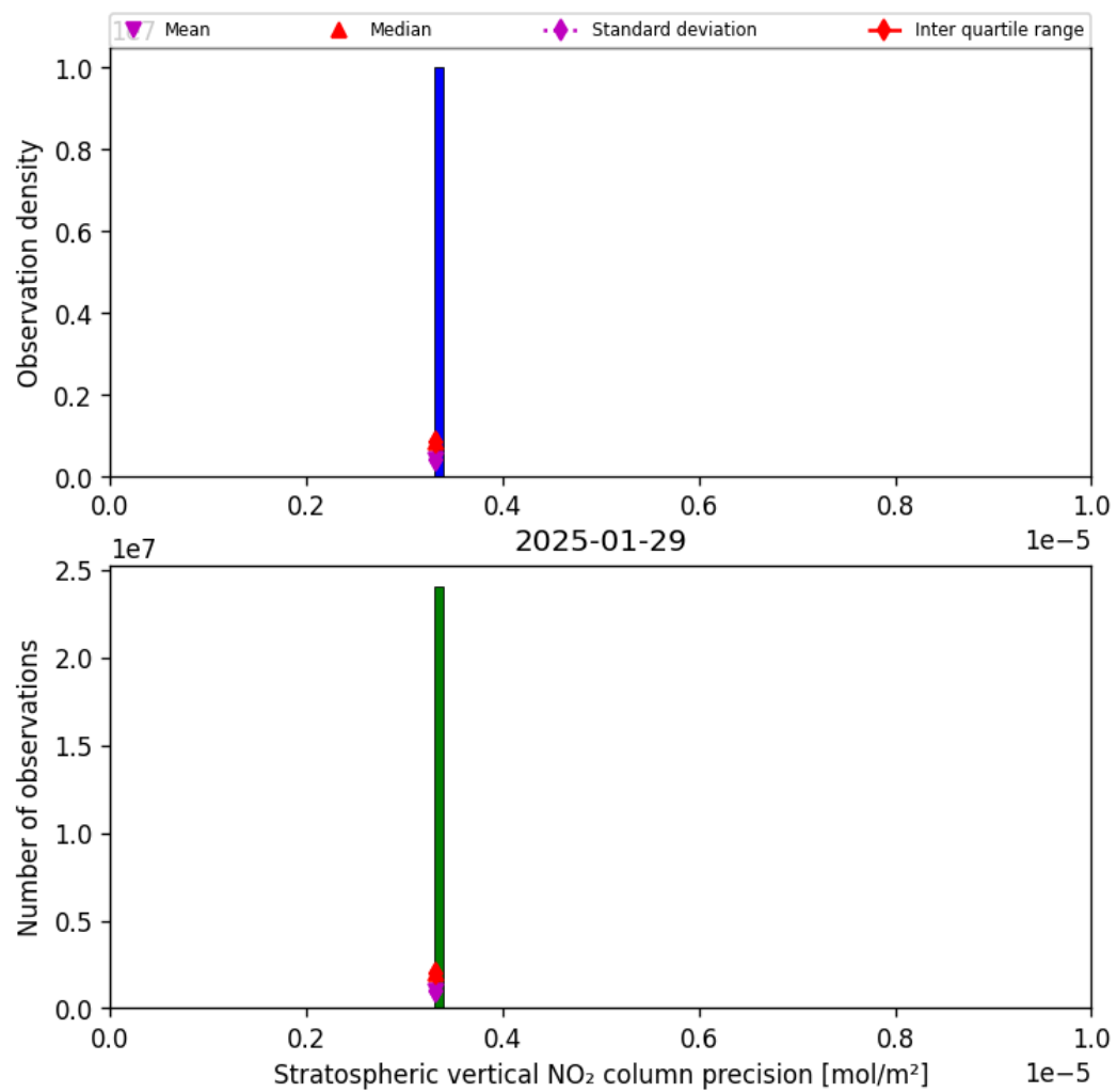
Figure 35: Histogram of “Stratospheric vertical NO 2 column precision” for 2025-01-29 to 2025-01-30
