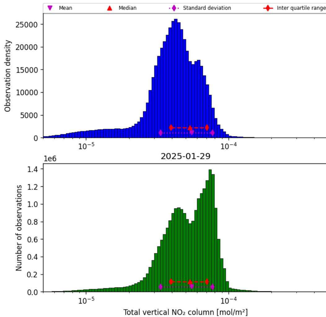
Figure 36: Histogram of “Total vertical NO 2 column” for 2025-01-29 to 2025-01-30
