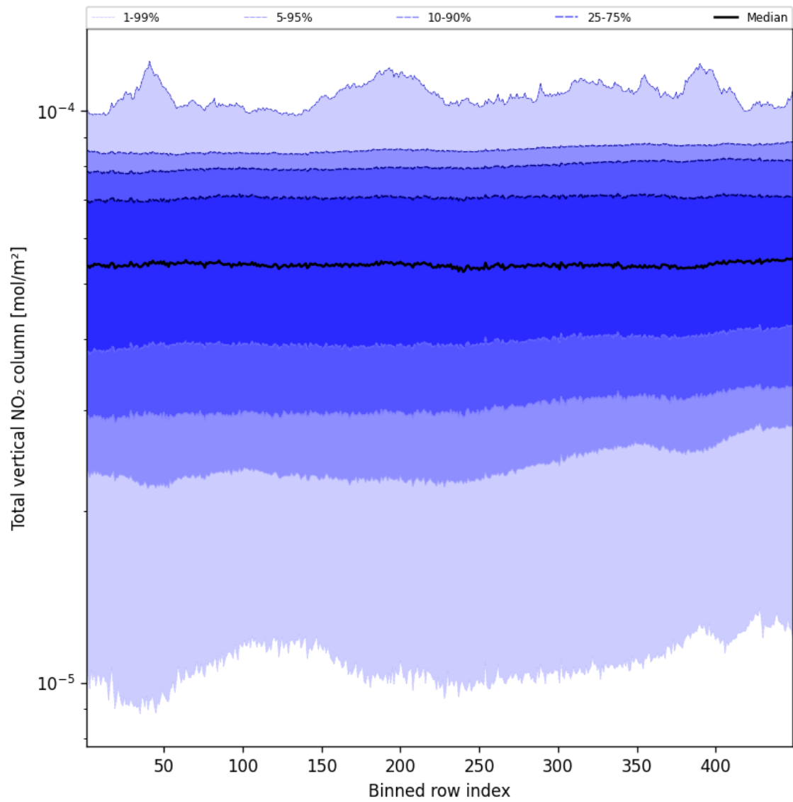
Figure 53: Along track statistics of “Total vertical NO 2 column” for 2025-01-29 to 2025-01-30
