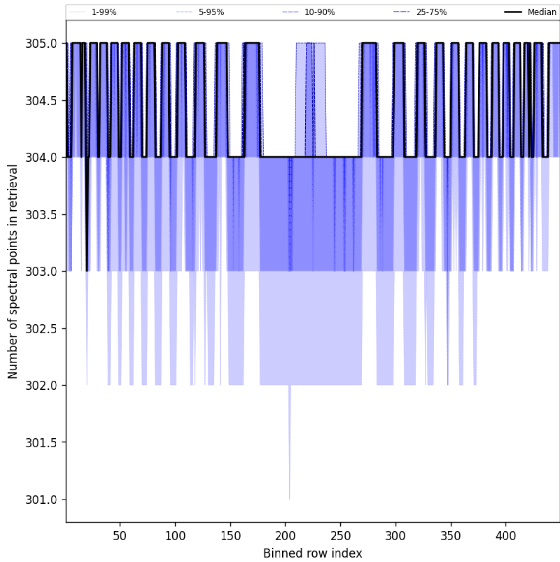
Figure 48: Along track statistics of “Number of spectral points in retrieval” for 2025-01-29 to 2025-01-30
