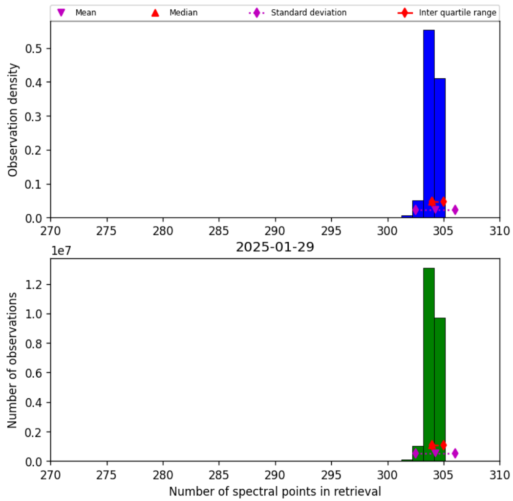
Figure 31: Histogram of “Number of spectral points in retrieval” for 2025-01-29 to 2025-01-30
