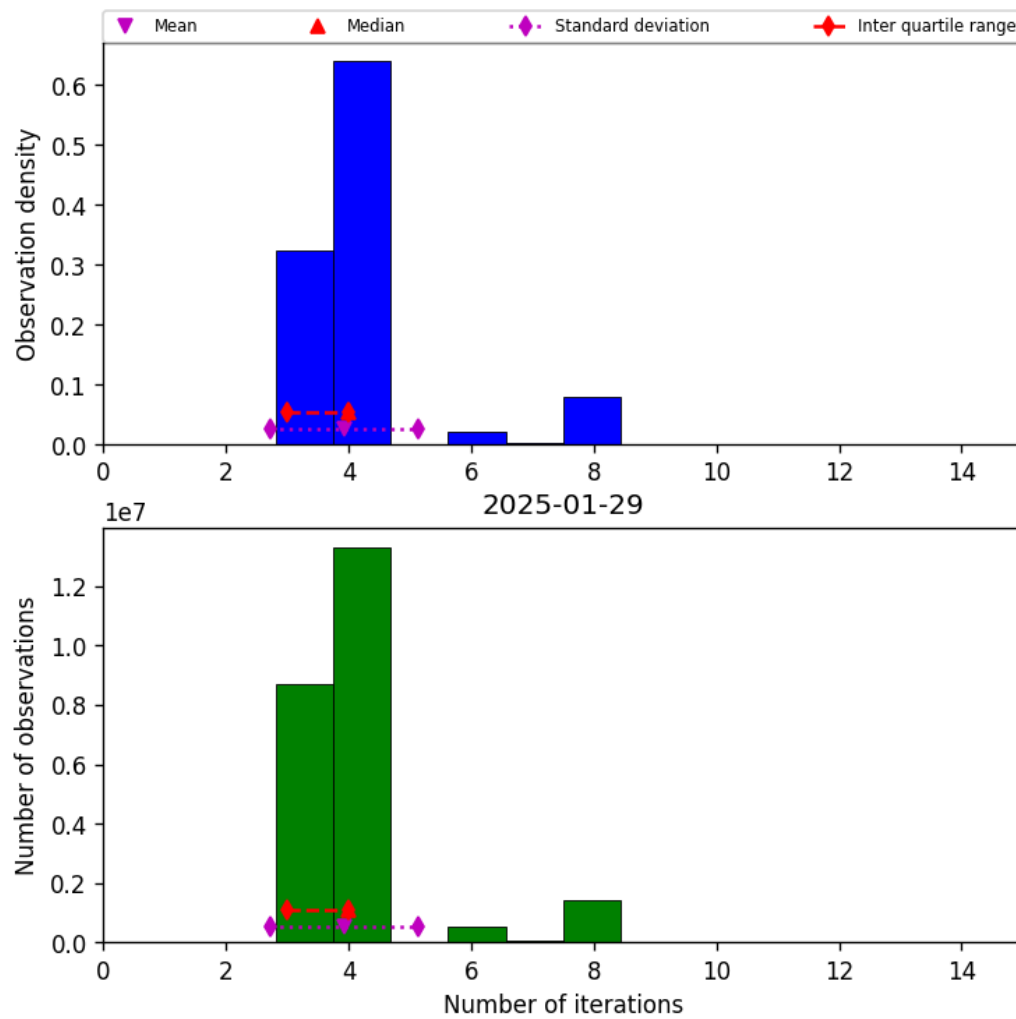
Figure 32: Histogram of “Number of iterations” for 2025-01-29 to 2025-01-30
