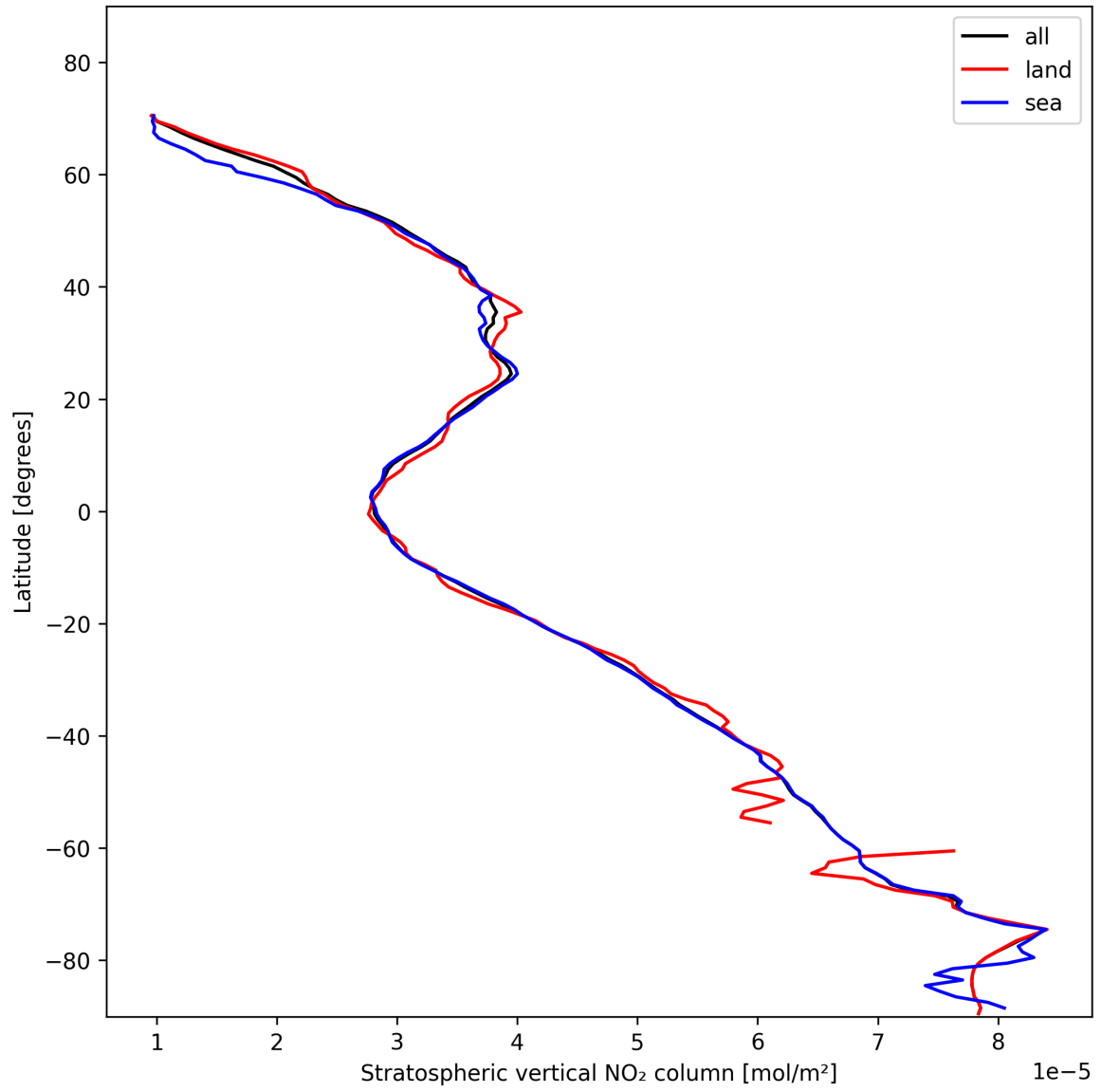
Figure 17: Zonal average of “Stratospheric vertical NO 2 column” for 2025-01-29 to 2025-01-30.
