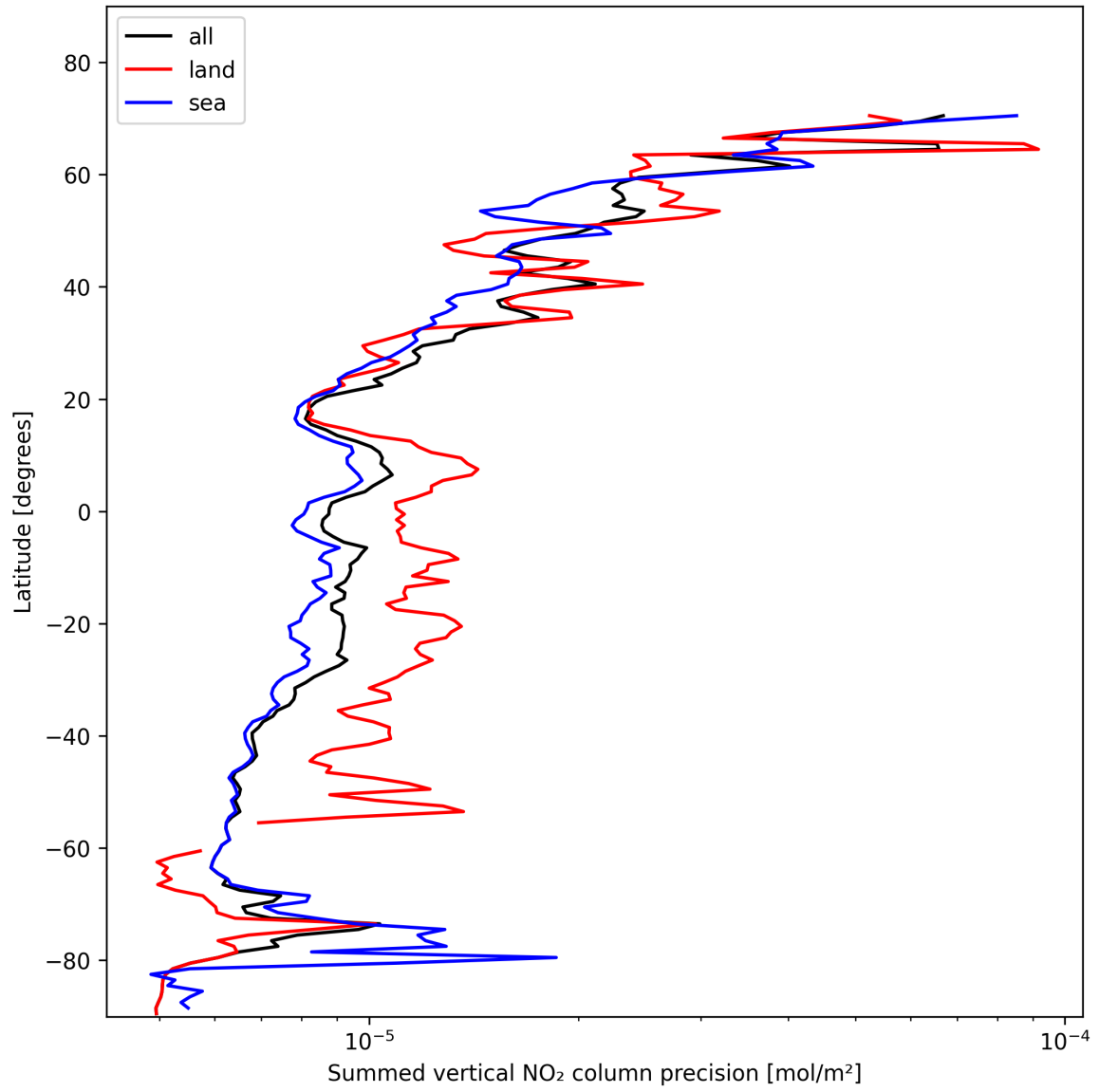
Figure 22: Zonal average of “Summed vertical NO 2 column precision” for 2025-01-29 to 2025-01-30.
