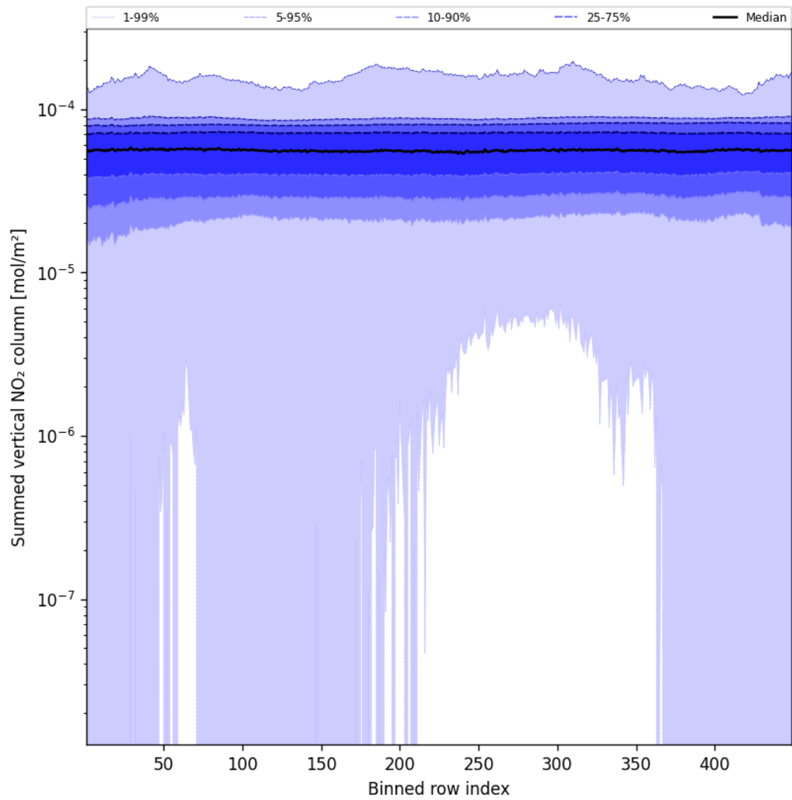
Figure 55: Along track statistics of “Summed vertical NO 2 column” for 2025-01-29 to 2025-01-30
