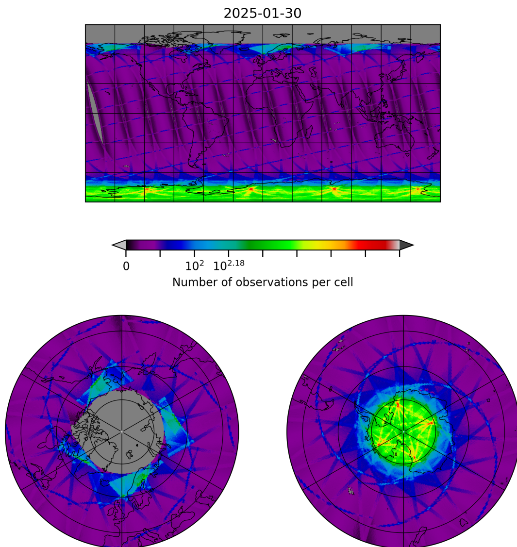
Figure 8: Map of the number of observations for 2025-01-30 to 2025-01-31
