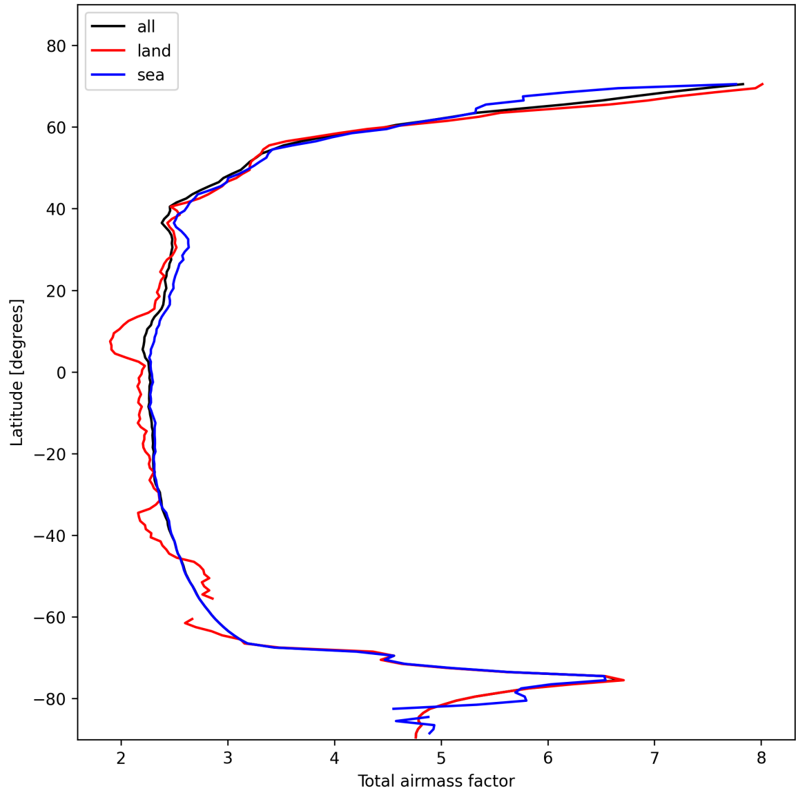
Figure 13: Zonal average of “Total airmass factor” for 2025-01-31 to 2025-01-31.
