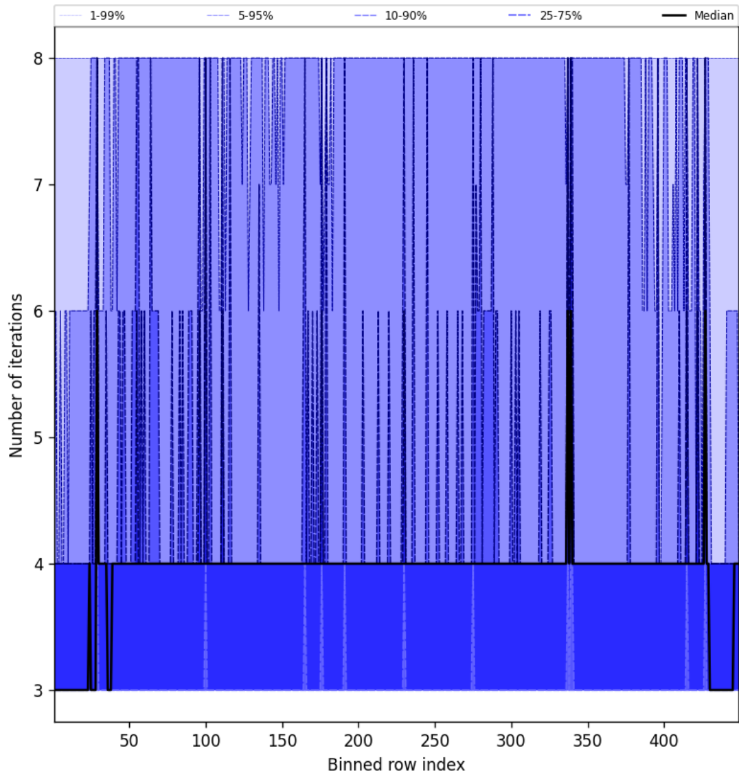
Figure 49: Along track statistics of “Number of iterations” for 2025-01-31 to 2025-01-31
