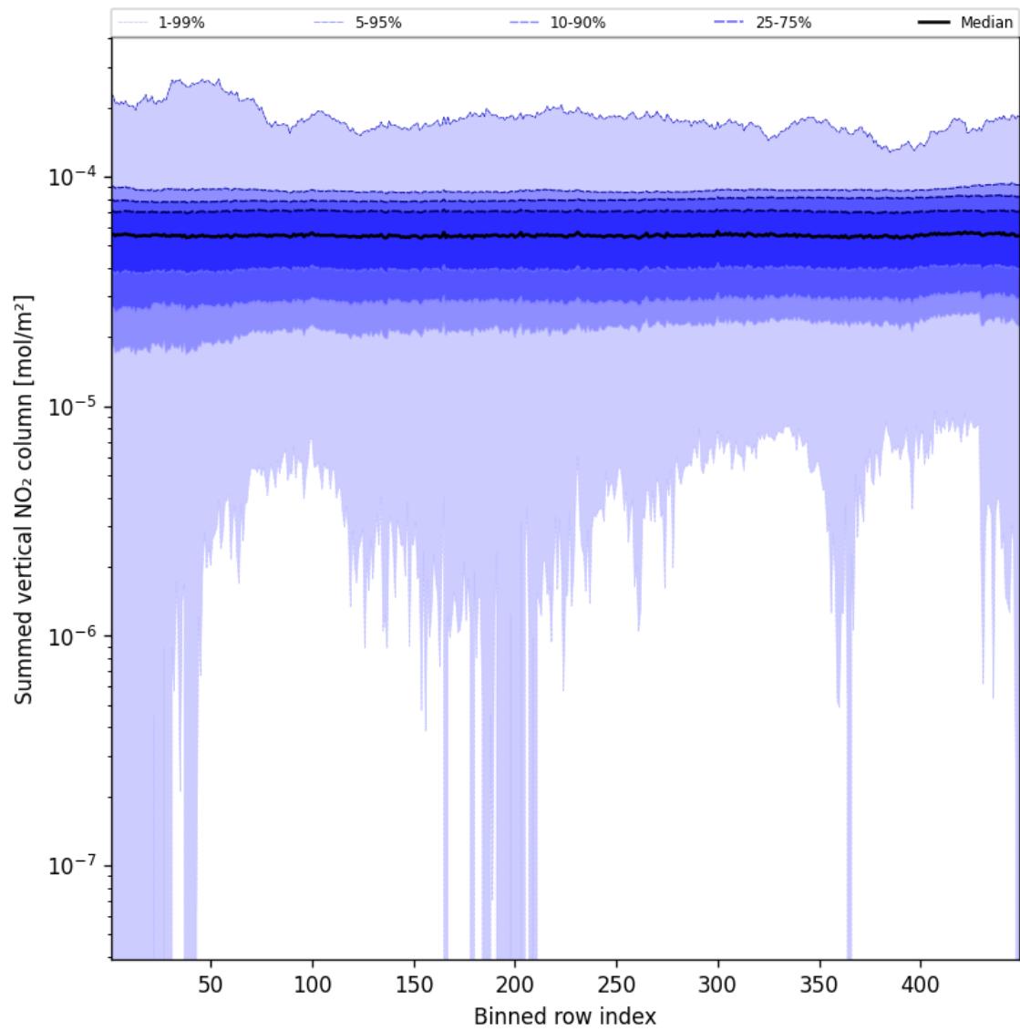
Figure 55: Along track statistics of “Summed vertical NO 2 column” for 2025-01-31 to 2025-01-31
