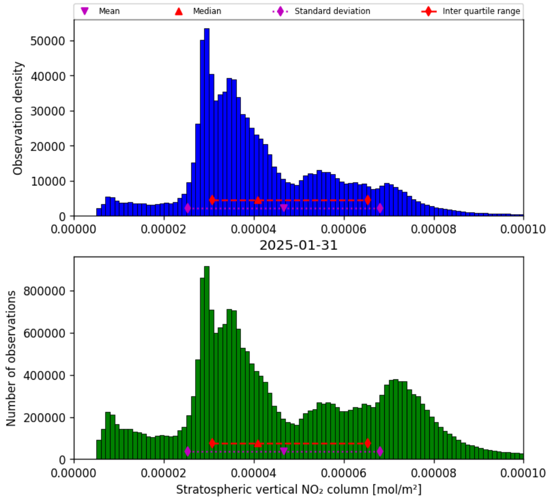
Figure 34: Histogram of “Stratospheric vertical NO 2 column” for 2025-01-31 to 2025-01-31
