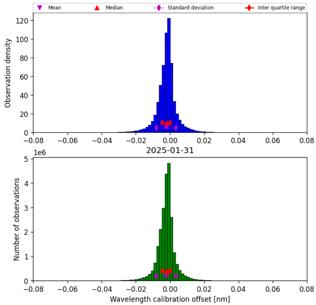
Figure 33: Histogram of “Wavelength calibration offset” for 2025-01-31 to 2025-01-31
