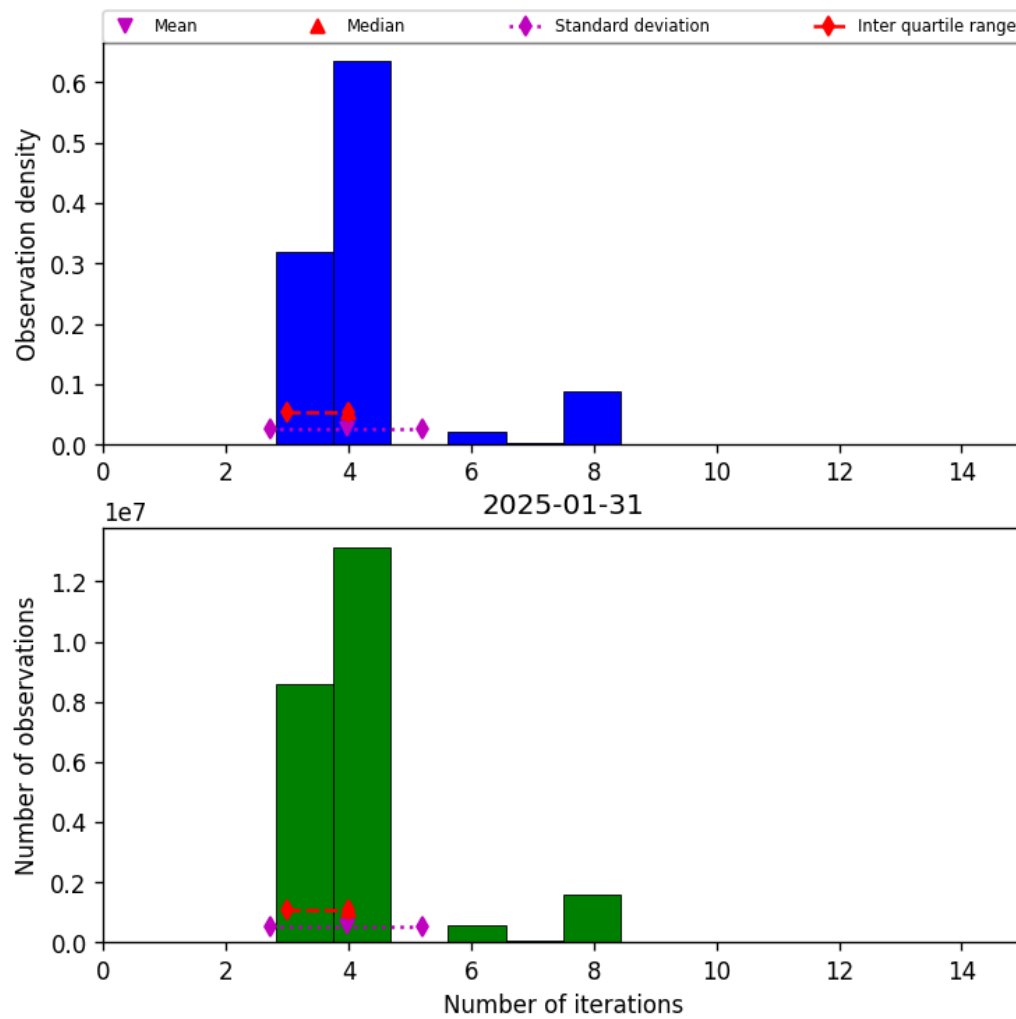
Figure 32: Histogram of “Number of iterations” for 2025-01-31 to 2025-01-31
