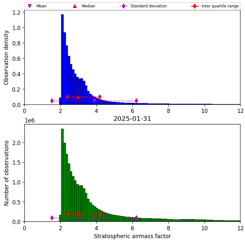
Figure 42: Histogram of “Stratospheric airmass factor” for 2025-01-31 to 2025-01-31
