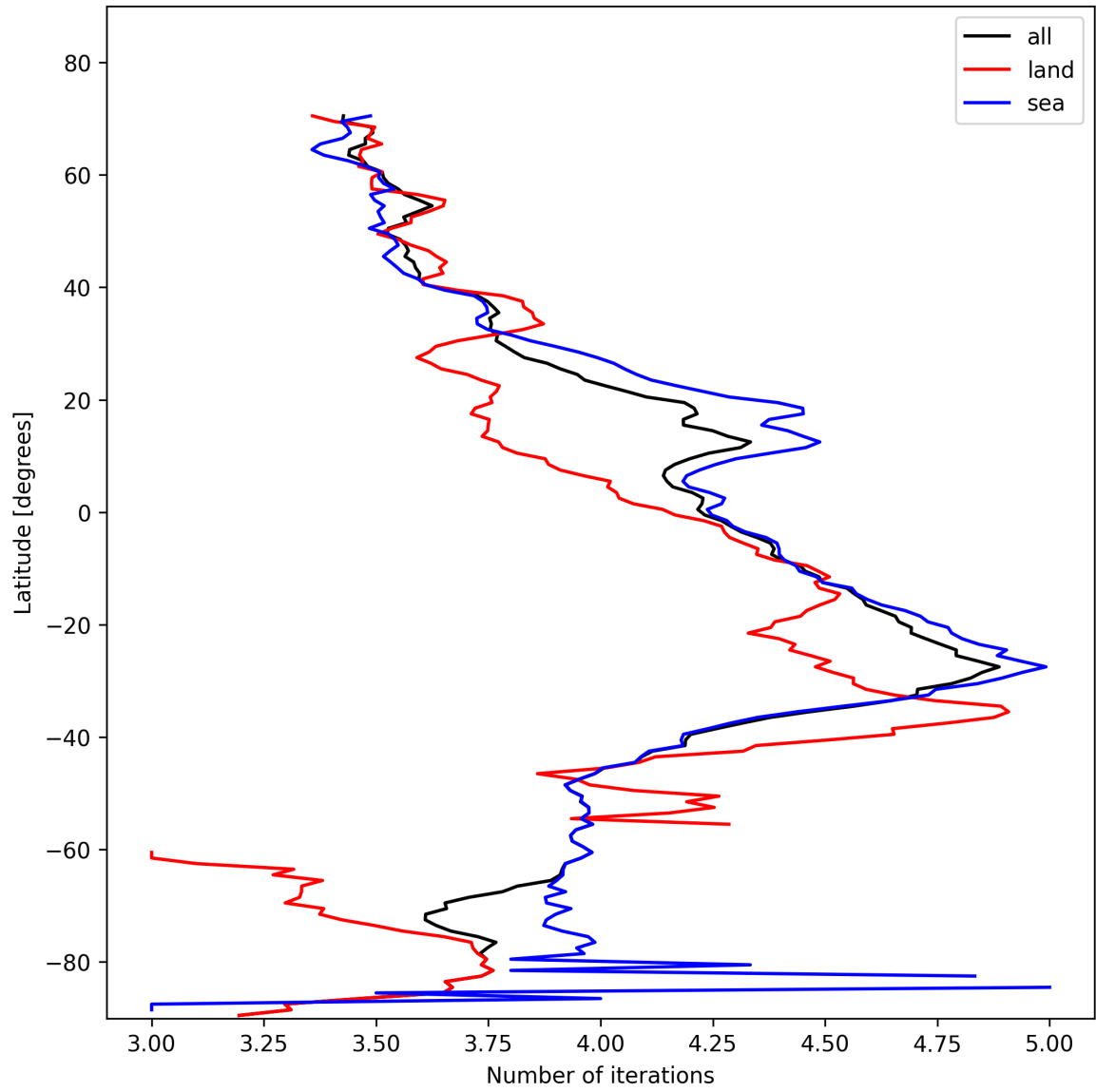
Figure 15: Zonal average of “Number of iterations” for 2025-01-31 to 2025-01-31.
