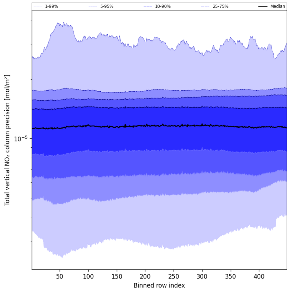
Figure 54: Along track statistics of “Total vertical NO 2 column precision” for 2025-01-31 to 2025-01-31
