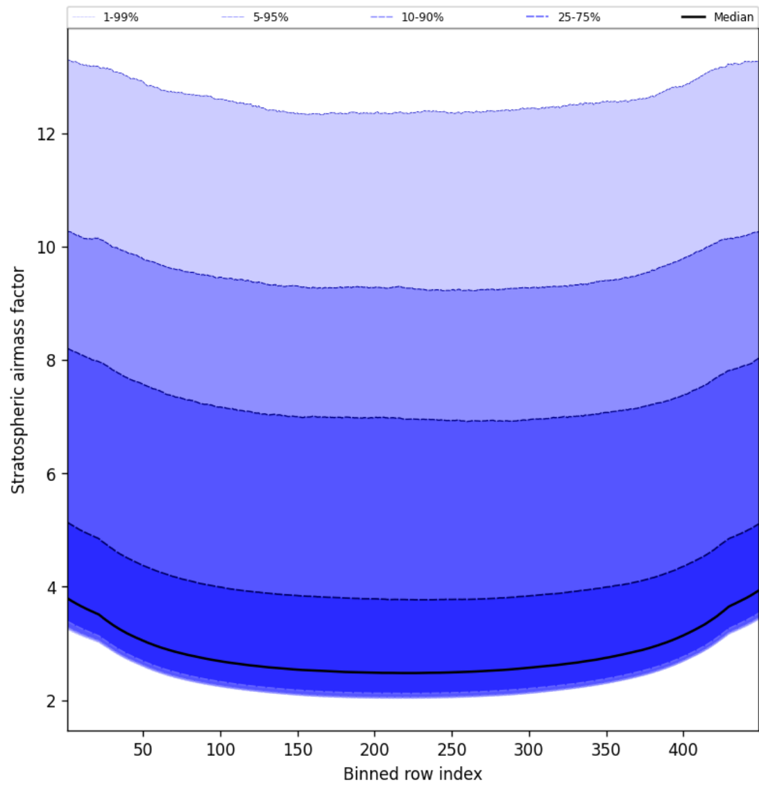
Figure 59: Along track statistics of “Stratospheric airmass factor” for 2025-01-31 to 2025-01-31
