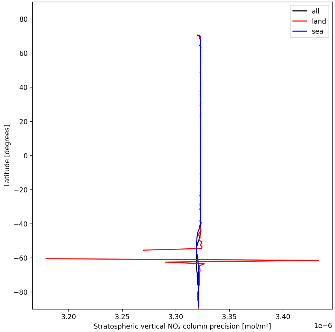
Figure 18: Zonal average of "Stratospheric vertical NO 2 column precision" for 2025-01-31 to 2025-01-31.
