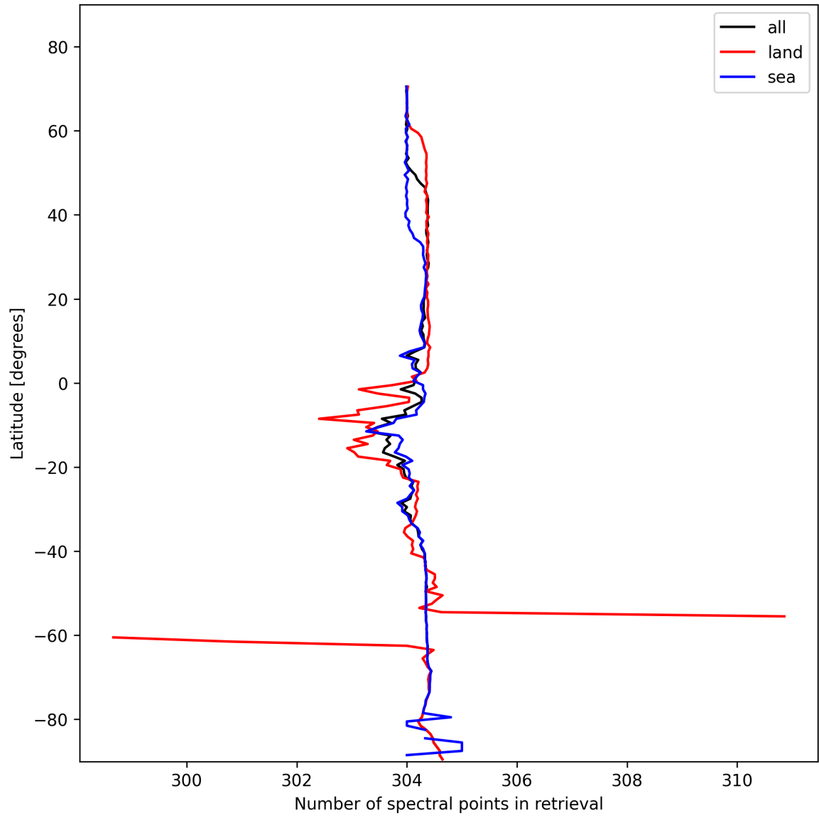
Figure 14: Zonal average of “Number of spectral points in retrieval” for 2025-01-31 to 2025-01-31.
