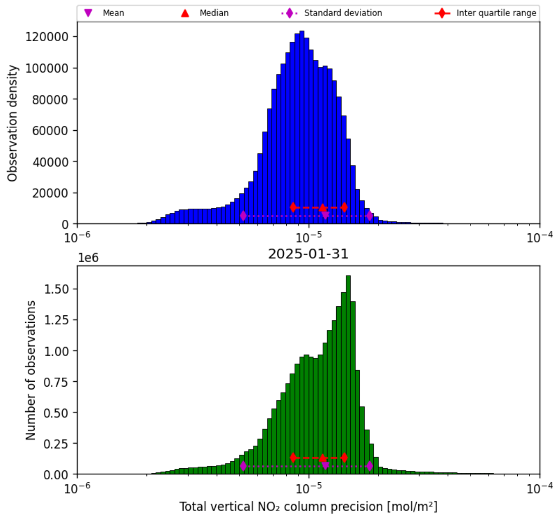
Figure 37: Histogram of "Total vertical NO 2 column precision" for 2025-01-31 to 2025-01-31
