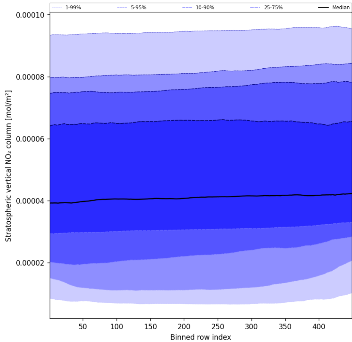
Figure 51: Along track statistics of “Stratospheric vertical NO 2 column” for 2025-01-31 to 2025-01-31
