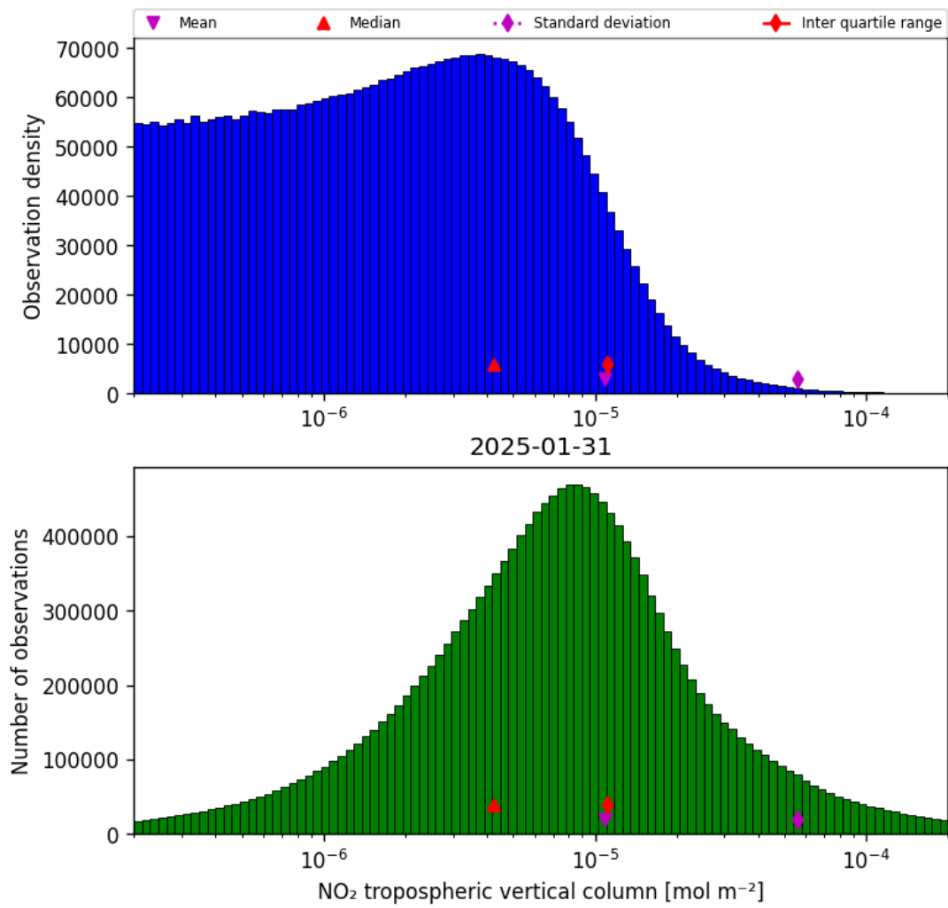
Figure 27: Histogram of “NO 2 tropospheric vertical column” for 2025-01-31 to 2025-01-31
