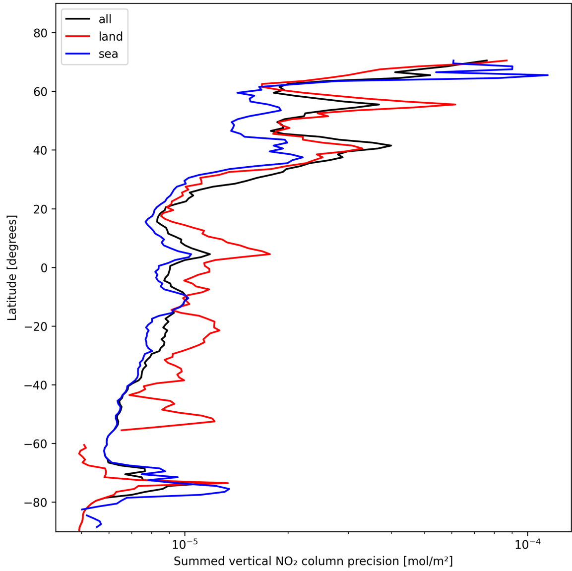
Figure 22: Zonal average of “Summed vertical NO 2 column precision” for 2025-01-31 to 2025-01-31.
