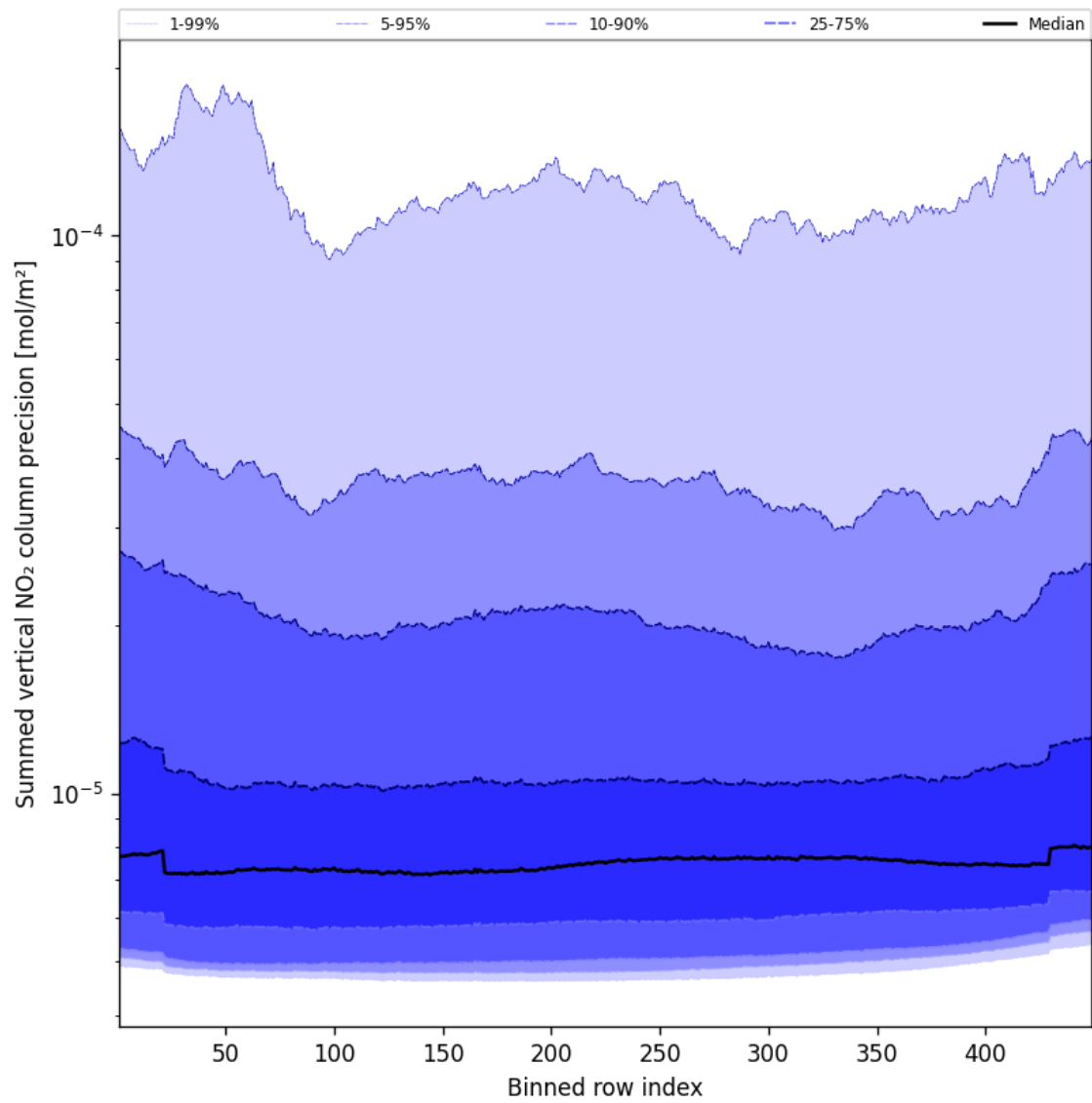
Figure 56: Along track statistics of “Summed vertical NO 2 column precision” for 2025-01-31 to 2025-01-31
