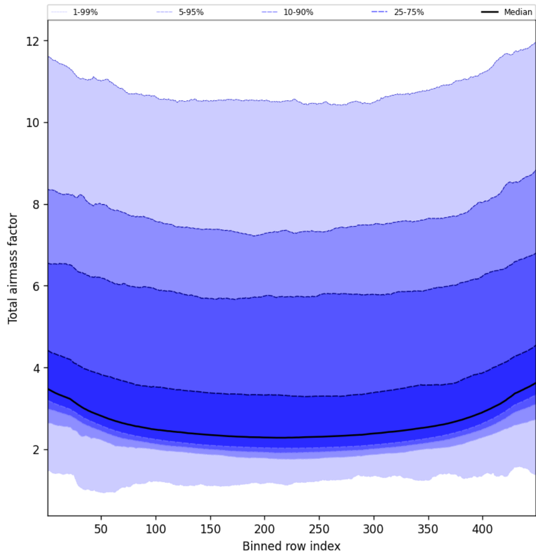
Figure 47: Along track statistics of “Total airmass factor” for 2025-01-31 to 2025-01-31
