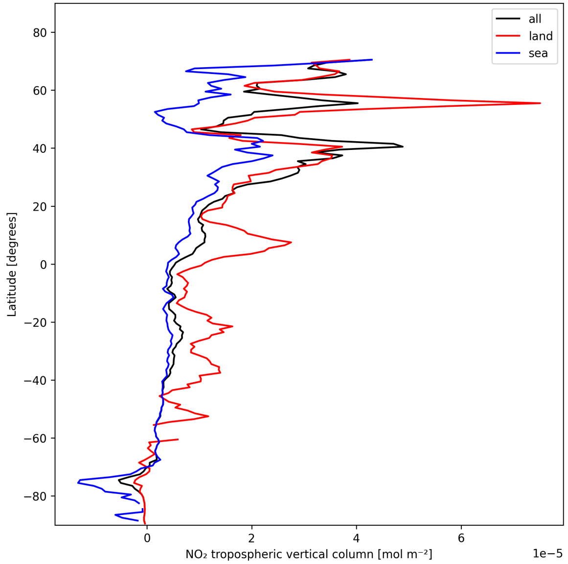
Figure 10: Zonal average of “NO 2 tropospheric vertical column” for 2025-01-31 to 2025-01-31.
