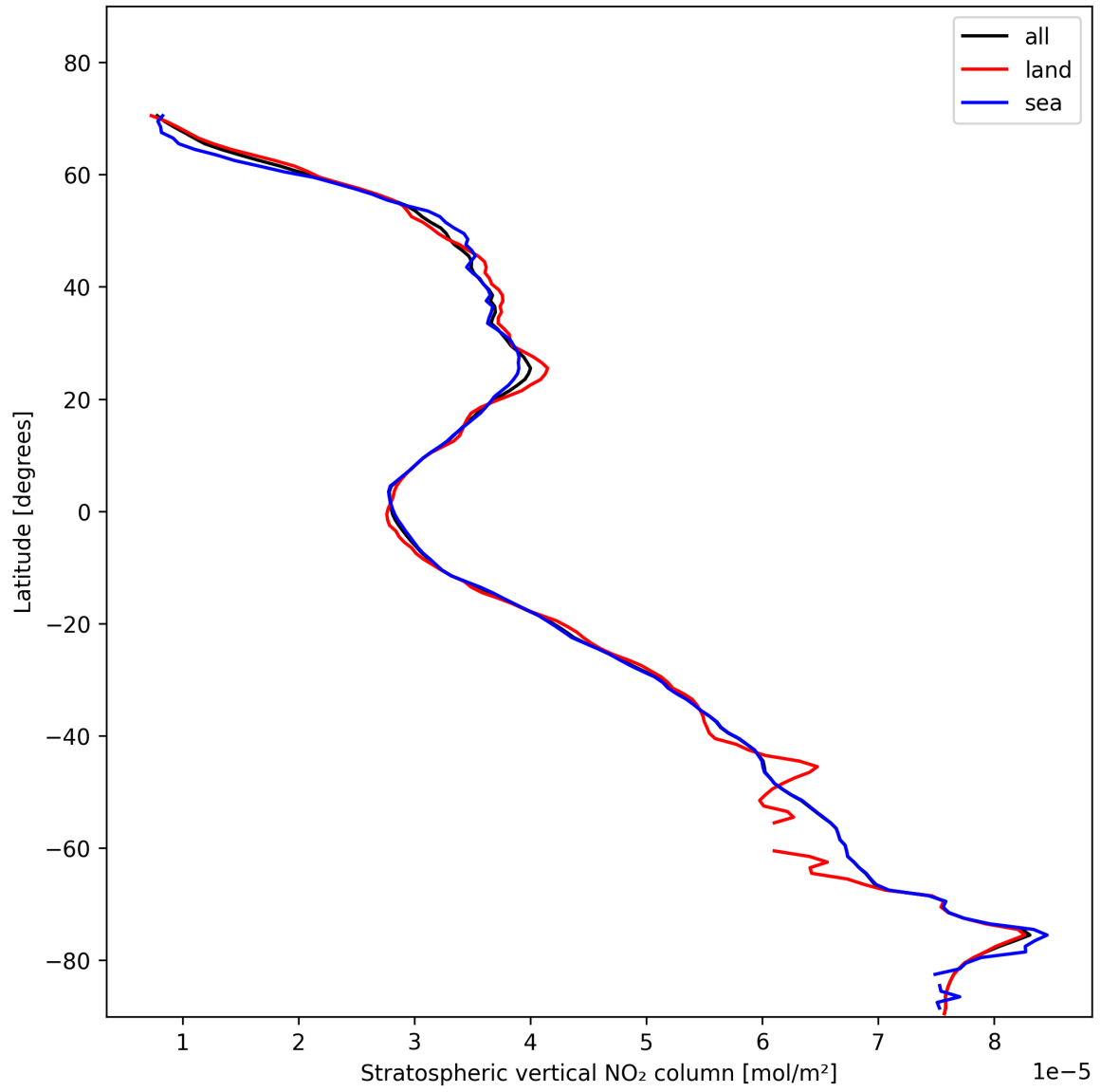
Figure 17: Zonal average of “Stratospheric vertical NO 2 column” for 2025-01-31 to 2025-01-31.
