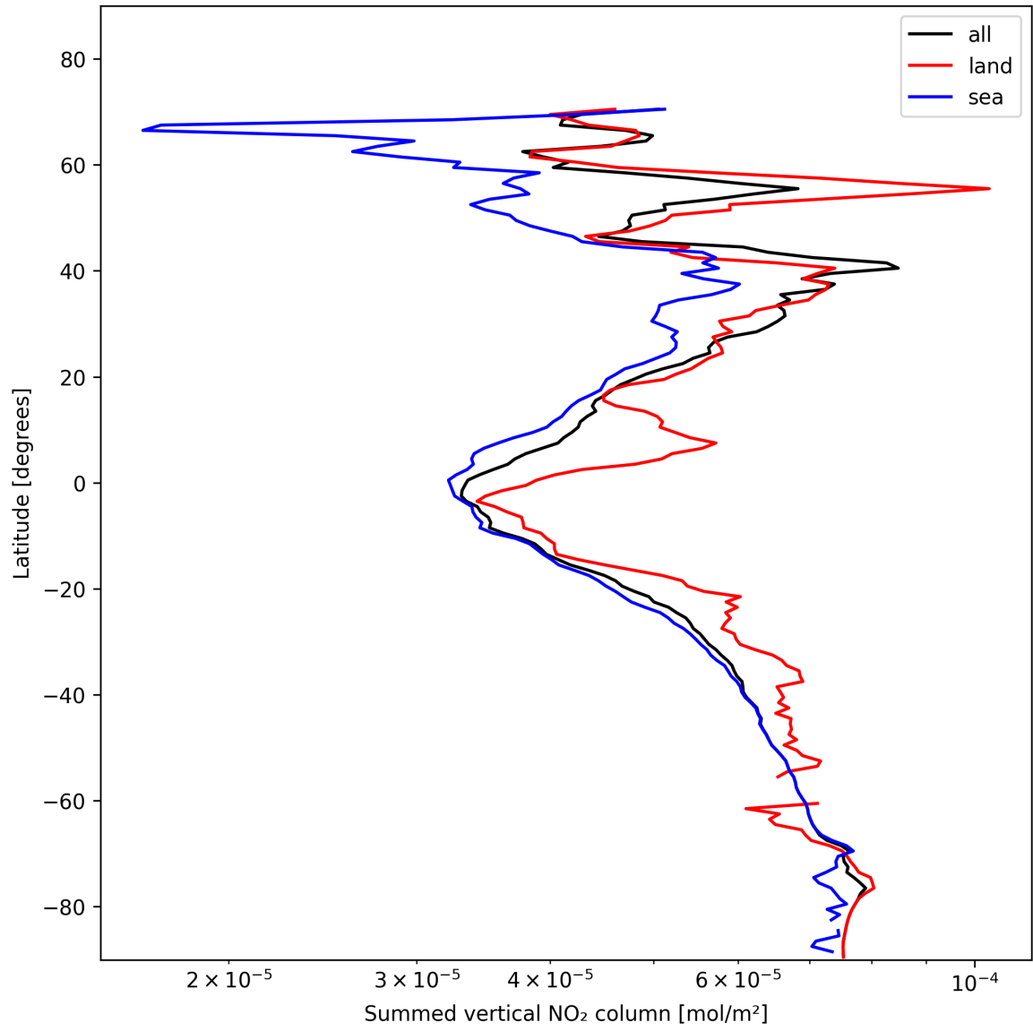
Figure 21: Zonal average of “Summed vertical NO 2 column” for 2025-01-31 to 2025-01-31.
