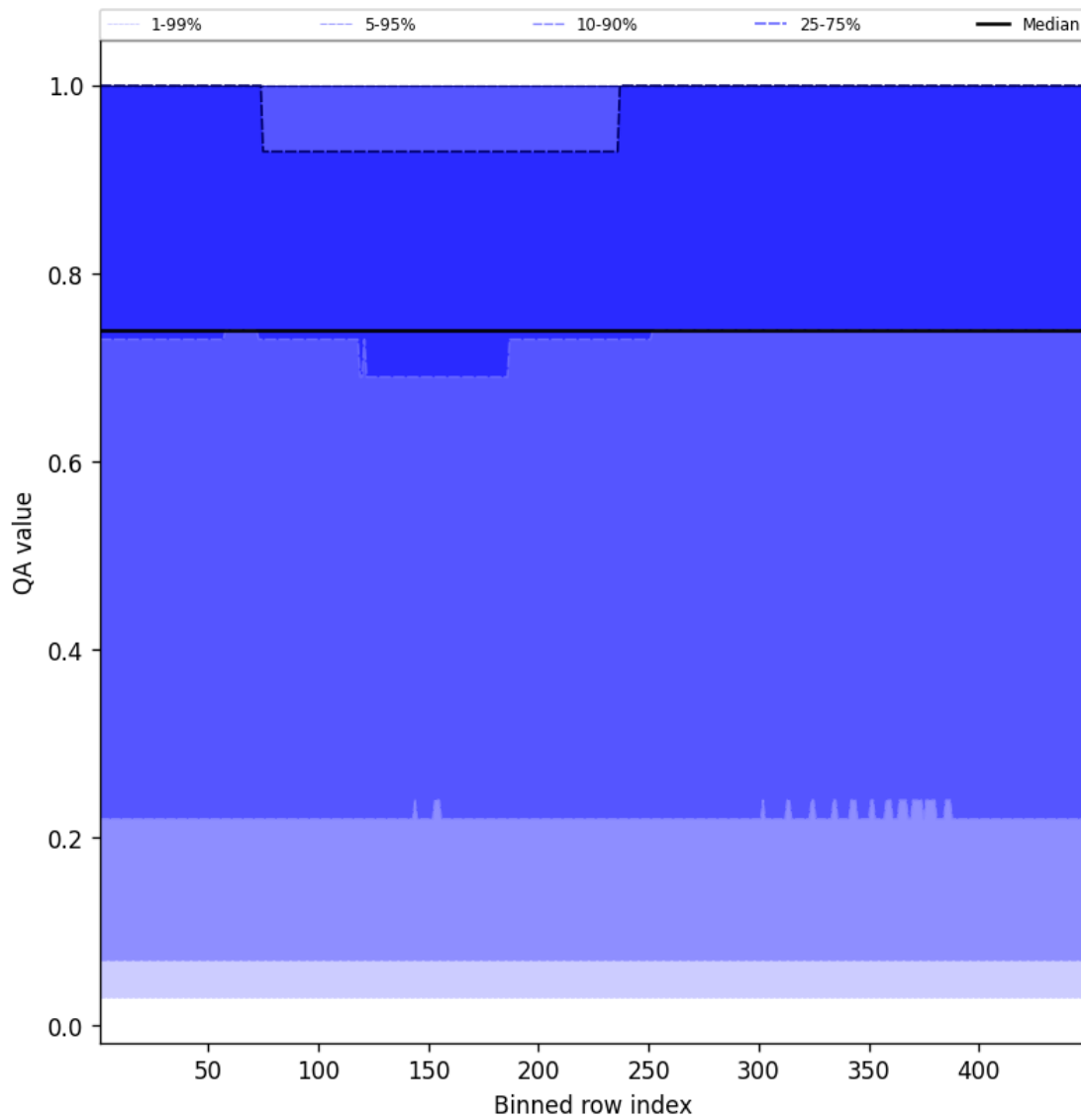
Figure 43: Along track statistics of “QA value” for 2025-01-31 to 2025-01-31
