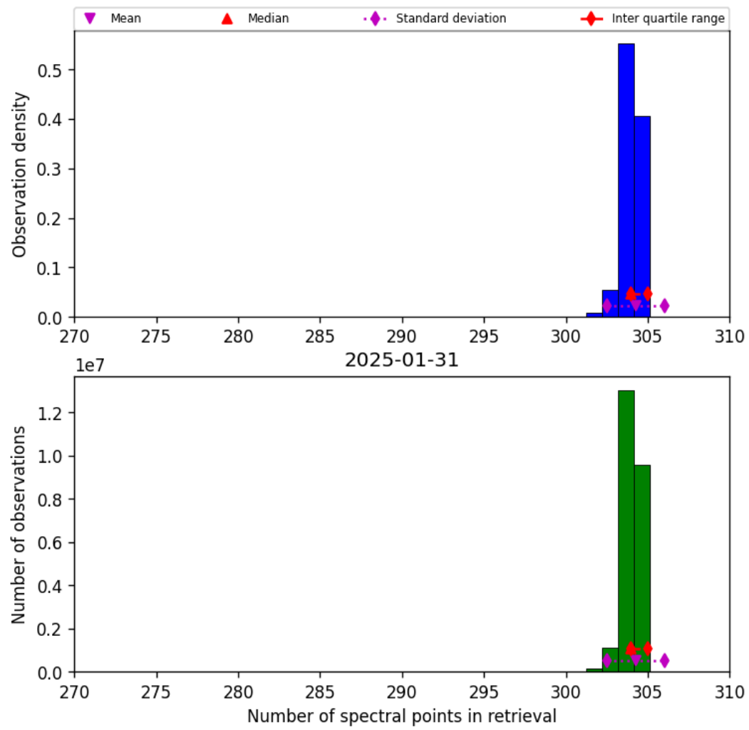
Figure 31: Histogram of “Number of spectral points in retrieval” for 2025-01-31 to 2025-01-31
