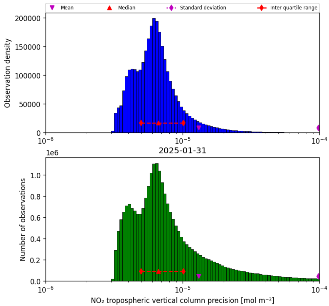
Figure 28: Histogram of "NO 2 tropospheric vertical column precision" for 2025-01-31 to 2025-01-31
