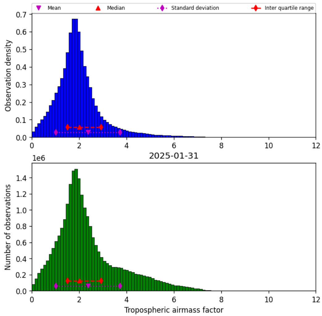
Figure 29: Histogram of “Tropospheric airmass factor” for 2025-01-31 to 2025-01-31
