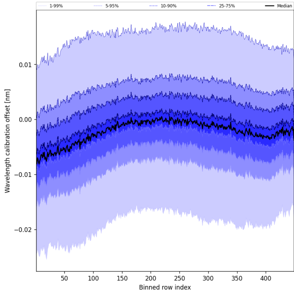
Figure 50: Along track statistics of “Wavelength calibration offset” for 2025-01-31 to 2025-01-31
