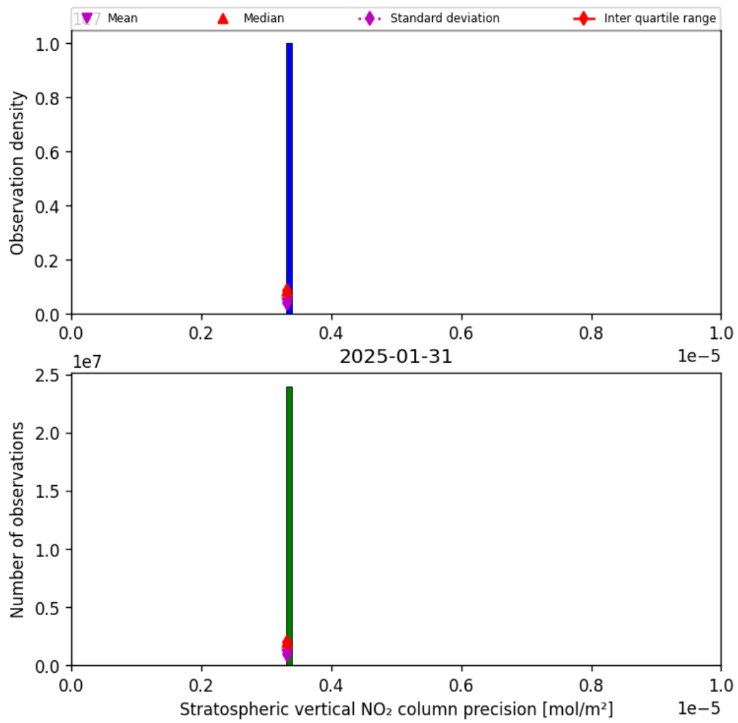
Figure 35: Histogram of “Stratospheric vertical NO 2 column precision” for 2025-01-31 to 2025-01-31
