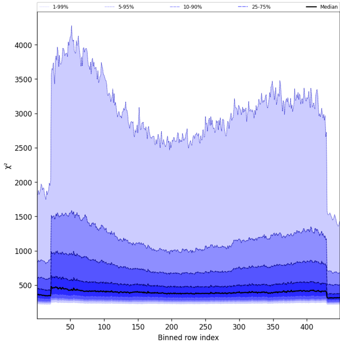
Figure 57: Along track statistics of “ \chi^2 ” for 2025-01-31 to 2025-01-31
