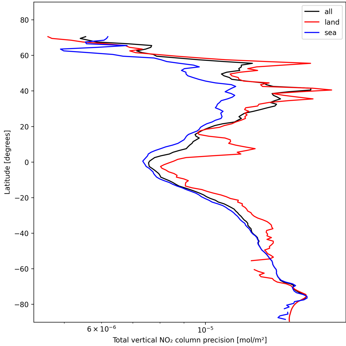
Figure 20: Zonal average of “Total vertical NO 2 column precision” for 2025-01-31 to 2025-01-31.
