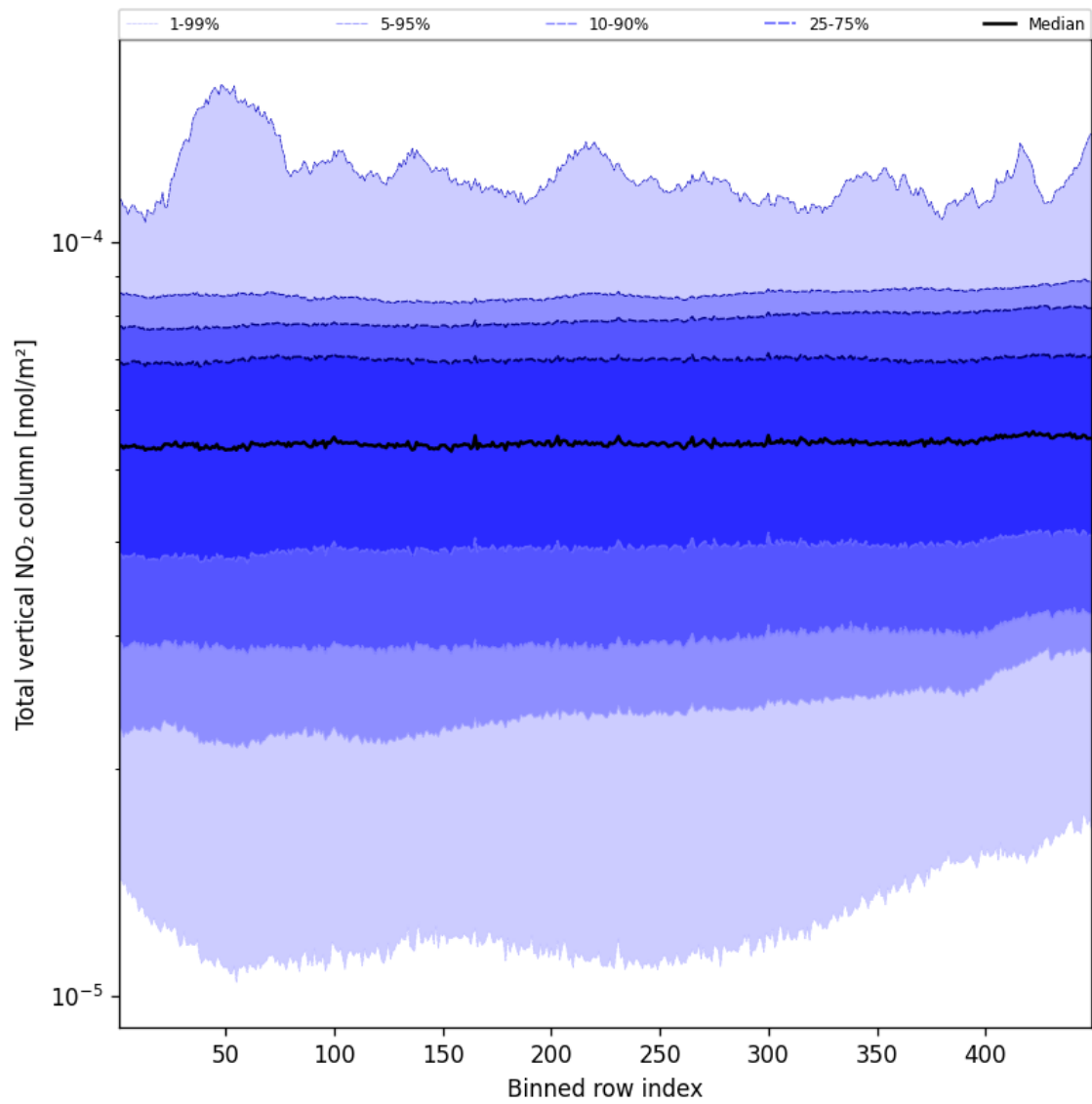
Figure 53: Along track statistics of “Total vertical NO 2 column” for 2025-01-31 to 2025-01-31
