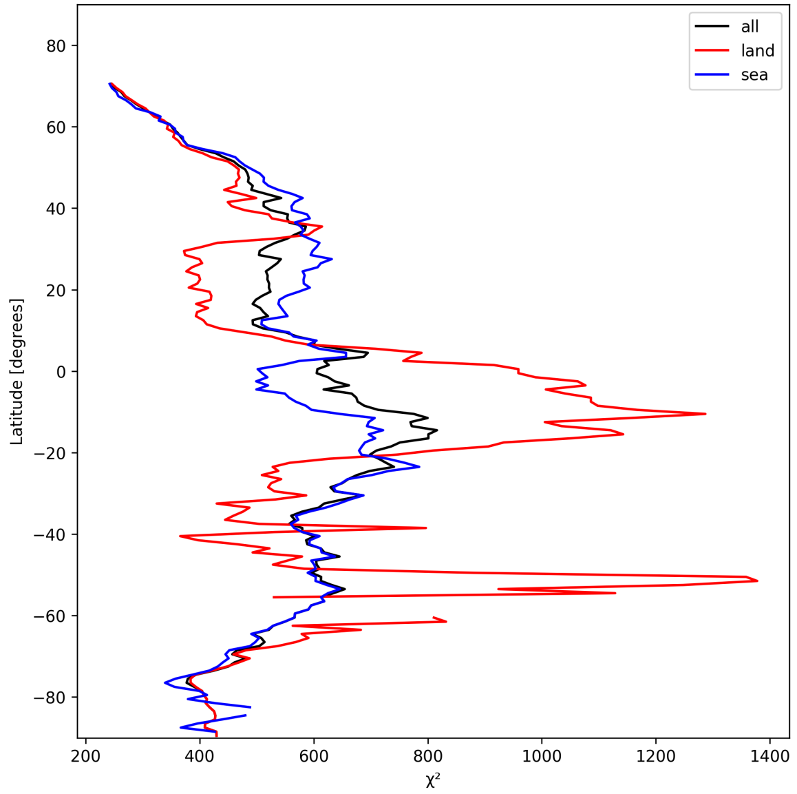
Figure 23: Zonal average of “ \chi^2 ” for 2025-01-31 to 2025-01-31.
