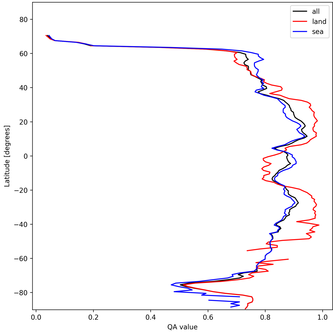
Figure 9: Zonal average of “QA value” for 2025-01-31 to 2025-01-31.
