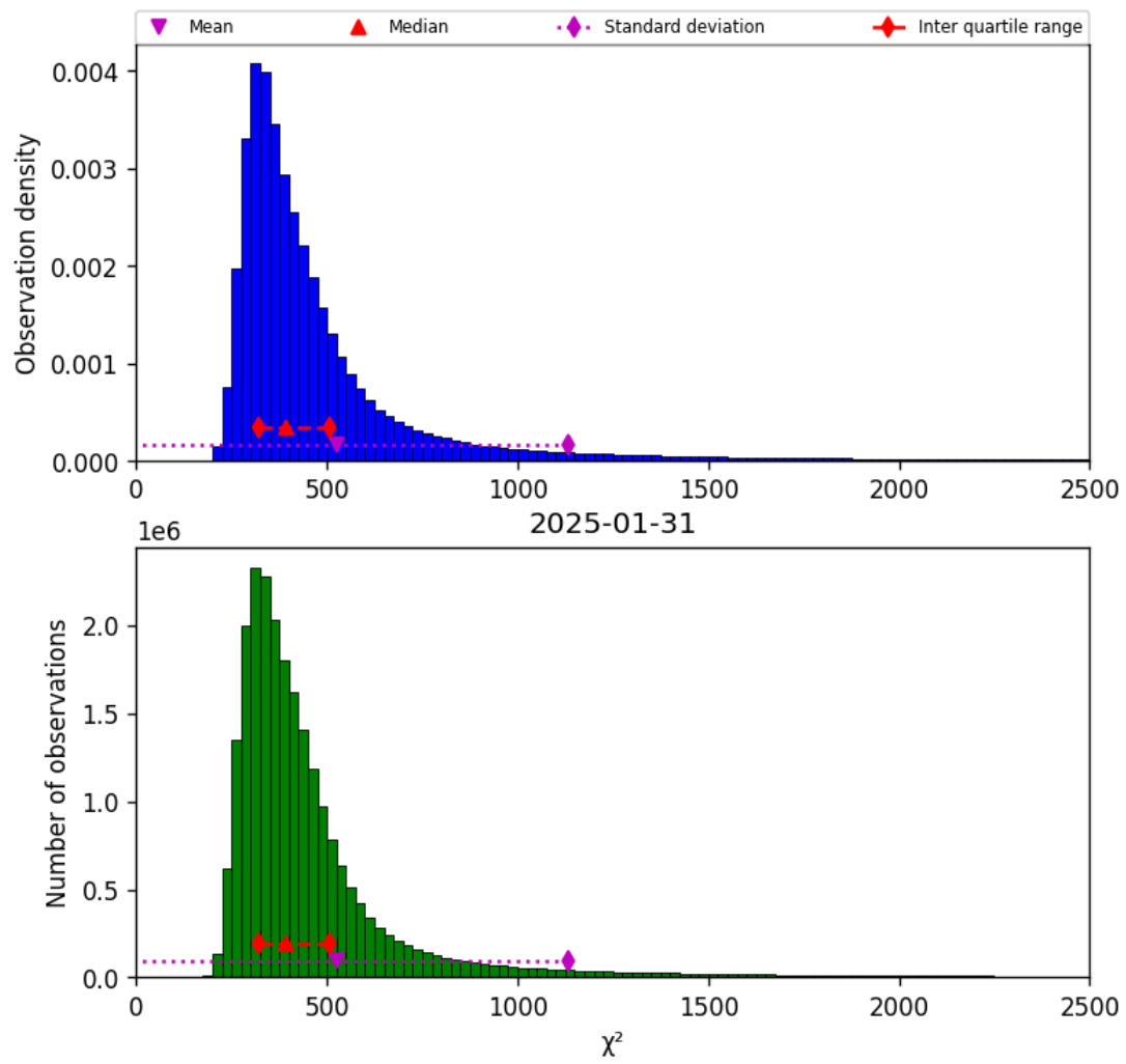
Figure 40: Histogram of “ \chi^2 ” for 2025-01-31 to 2025-01-31
