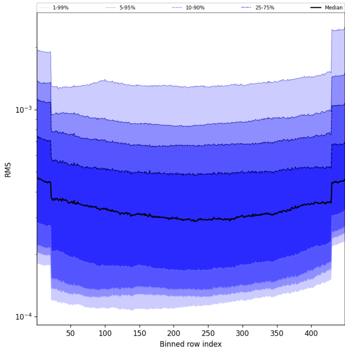
Figure 58: Along track statistics of “RMS” for 2025-01-31 to 2025-01-31
