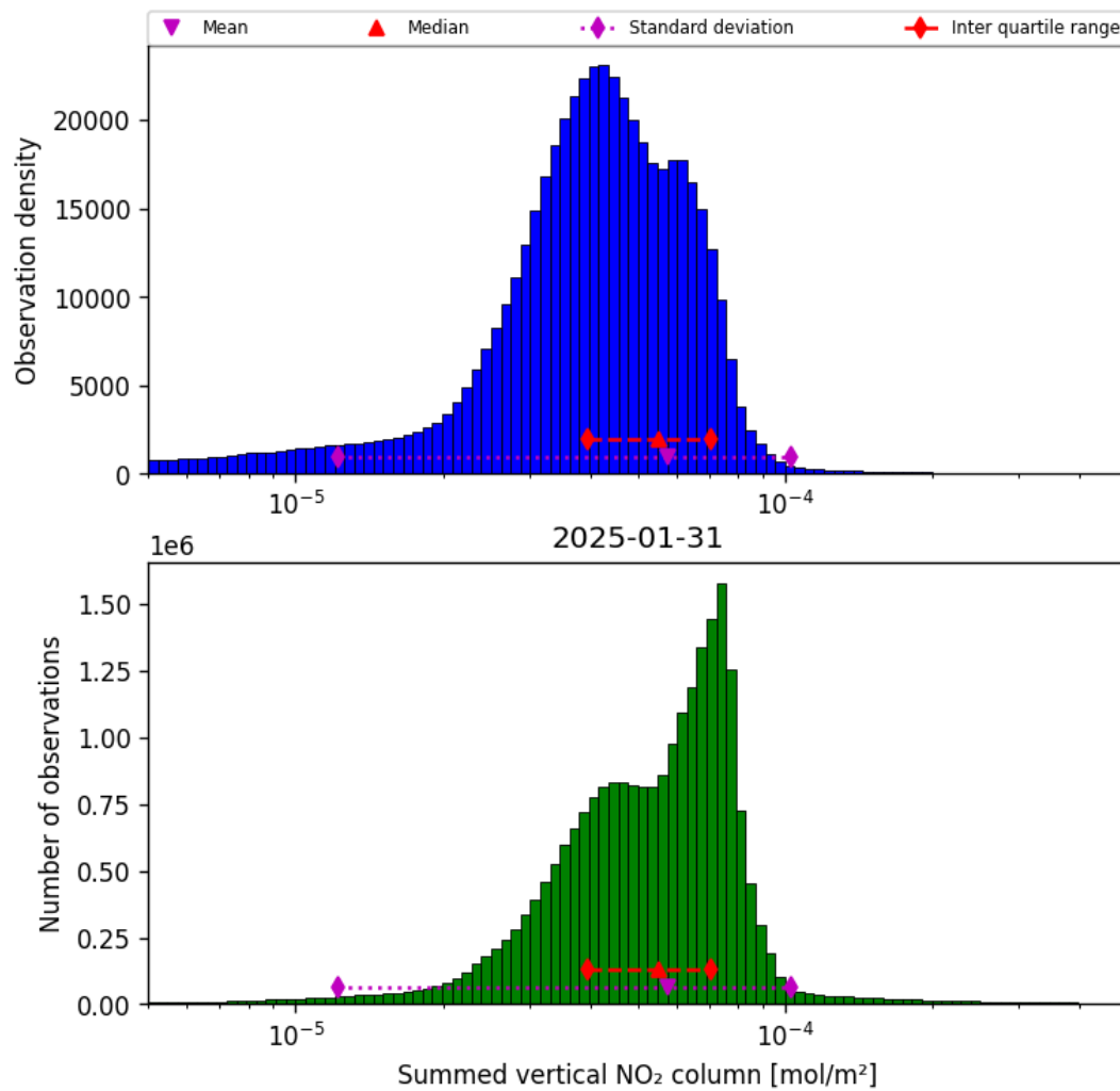
Figure 38: Histogram of "Summed vertical NO 2 column" for 2025-01-31 to 2025-01-31
