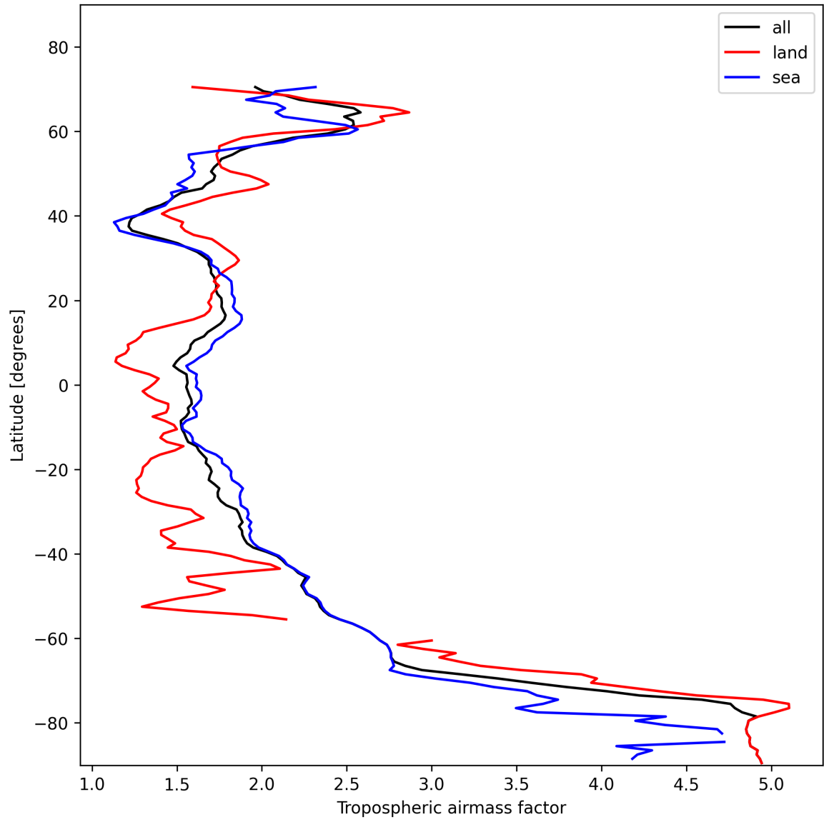
Figure 12: Zonal average of “Tropospheric airmass factor” for 2025-01-31 to 2025-01-31.
