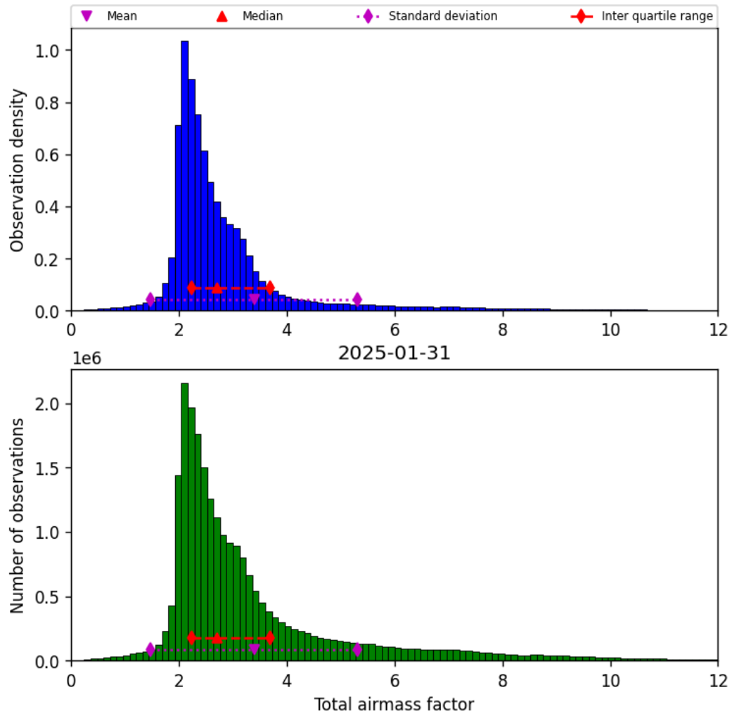
Figure 30: Histogram of “Total airmass factor” for 2025-01-31 to 2025-01-31
