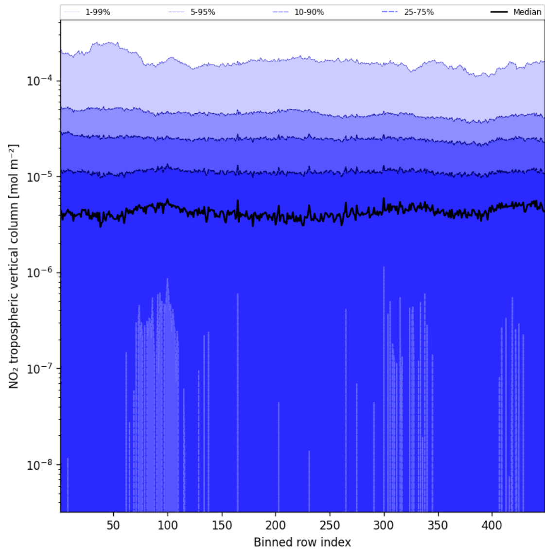
Figure 44: Along track statistics of “NO 2 tropospheric vertical column” for 2025-01-31 to 2025-01-31
