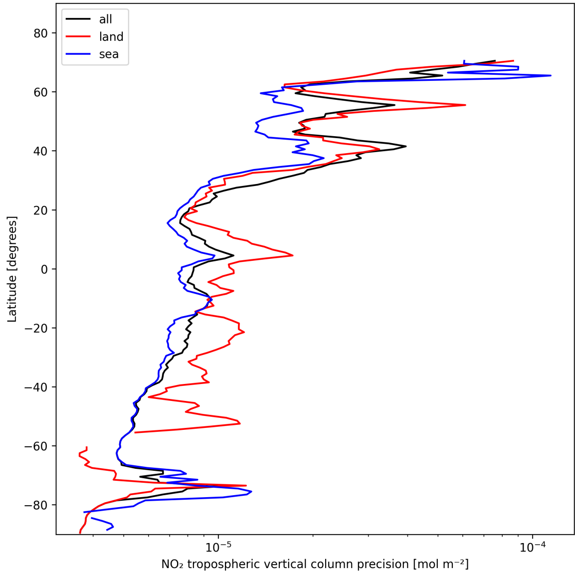
Figure 11: Zonal average of “NO 2 tropospheric vertical column precision” for 2025-01-31 to 2025-01-31.
