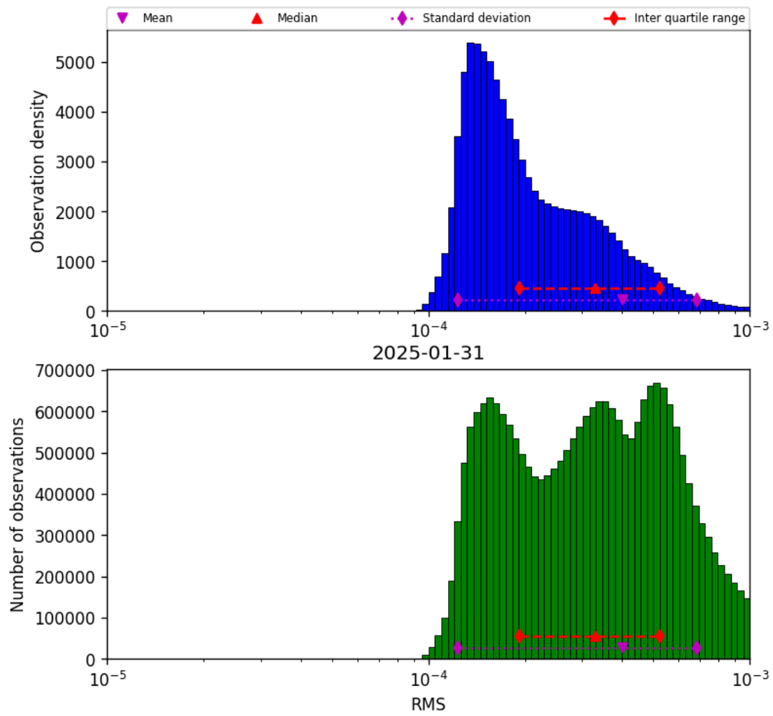
Figure 41: Histogram of “RMS” for 2025-01-31 to 2025-01-31
