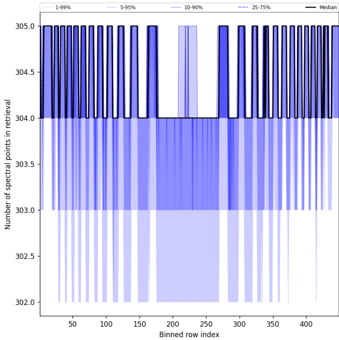
Figure 48: Along track statistics of “Number of spectral points in retrieval” for 2025-01-31 to 2025-01-31
