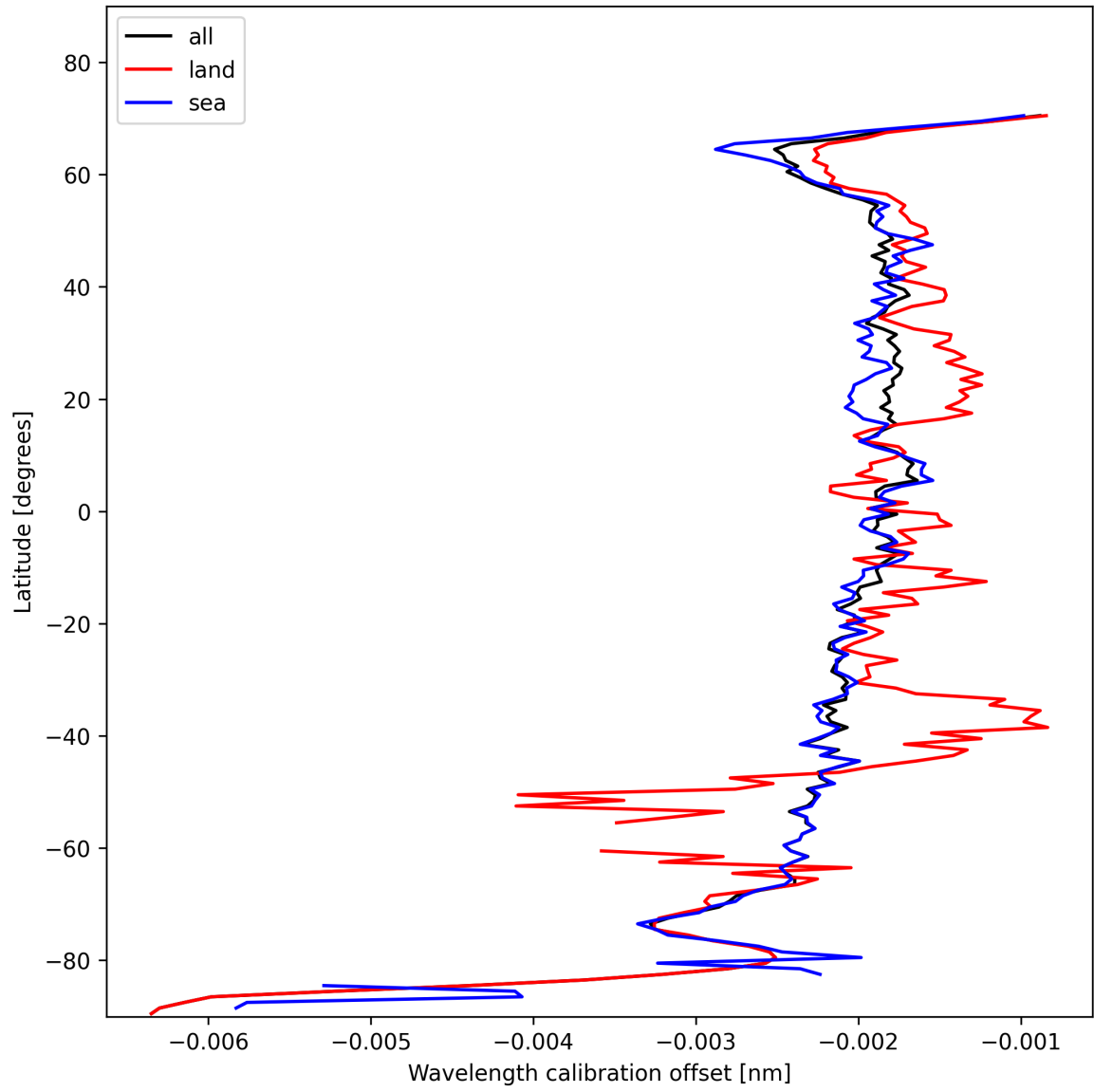
Figure 16: Zonal average of “Wavelength calibration offset” for 2025-01-31 to 2025-01-31.
