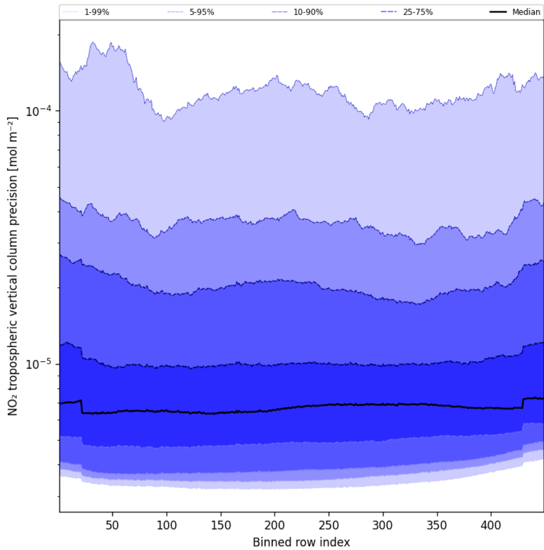
Figure 45: Along track statistics of “NO 2 tropospheric vertical column precision” for 2025-01-31 to 2025-01-31
