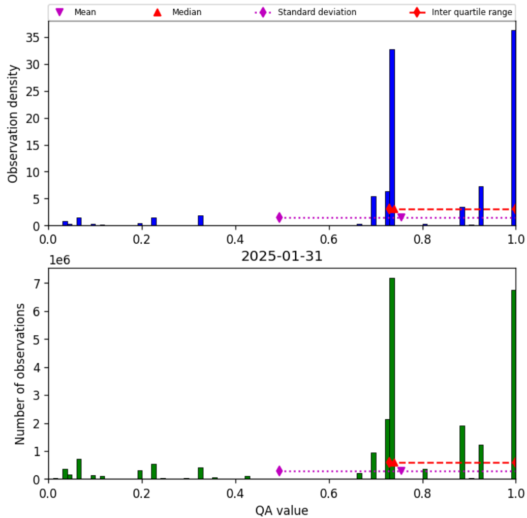
Figure 26: Histogram of “QA value” for 2025-01-31 to 2025-01-31
