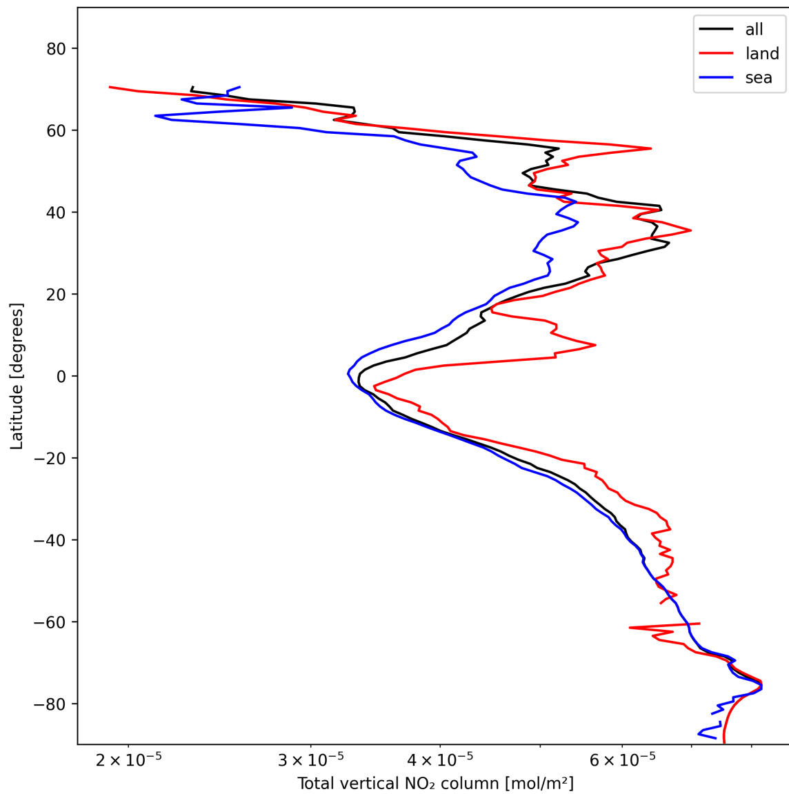
Figure 19: Zonal average of “Total vertical NO 2 column” for 2025-01-31 to 2025-01-31.
