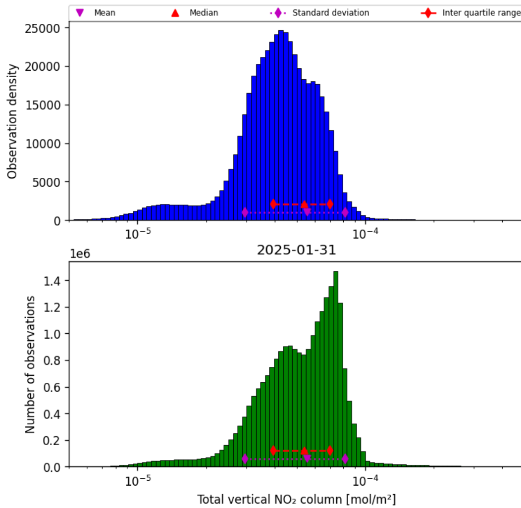
Figure 36: Histogram of "Total vertical NO 2 column" for 2025-01-31 to 2025-01-31
