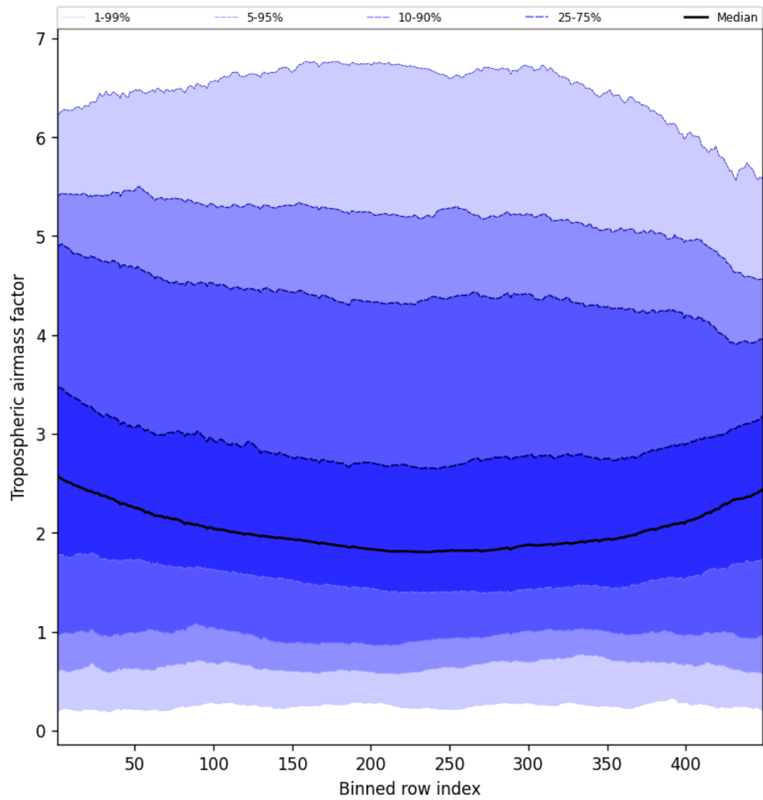
Figure 46: Along track statistics of “Tropospheric airmass factor” for 2025-01-31 to 2025-01-31
