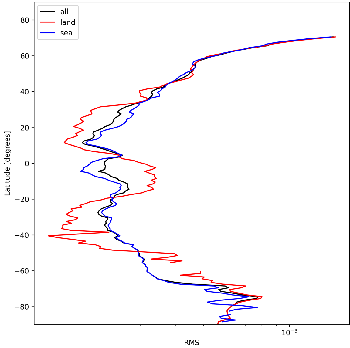
Figure 24: Zonal average of “RMS” for 2025-01-31 to 2025-01-31.
