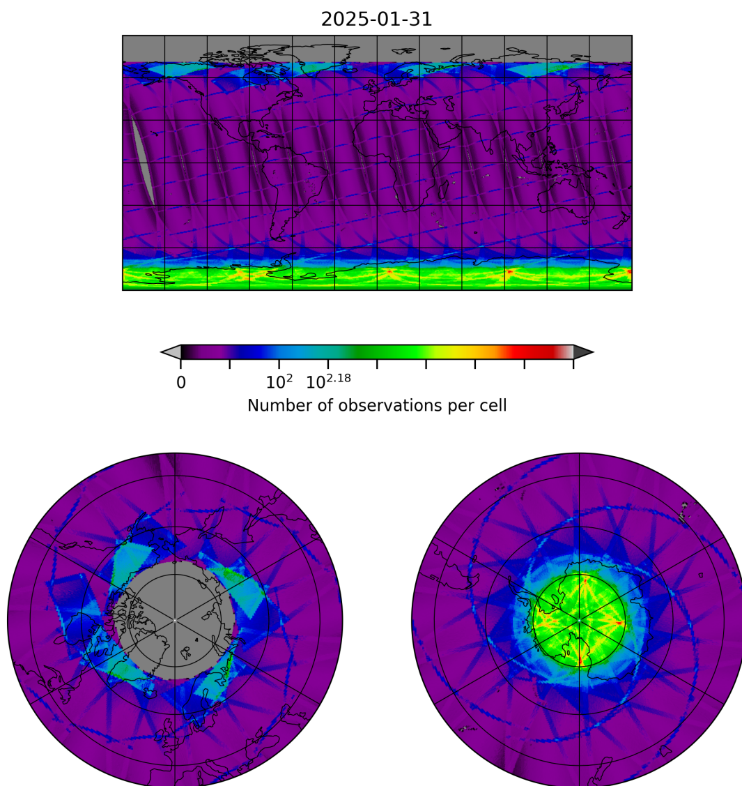
Figure 8: Map of the number of observations for 2025-01-31 to 2025-01-31
