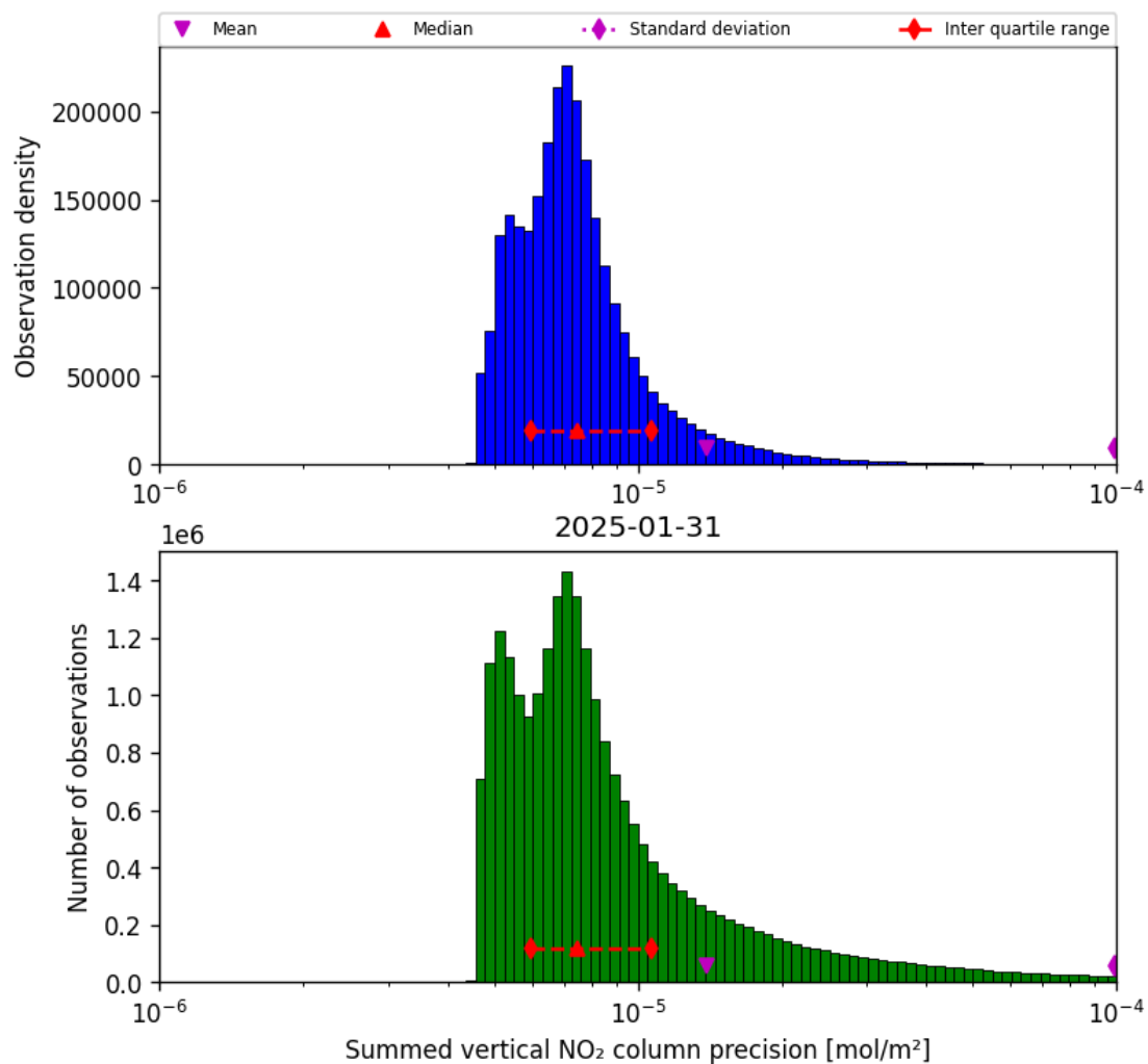
Figure 39: Histogram of “Summed vertical NO 2 column precision” for 2025-01-31 to 2025-01-31
