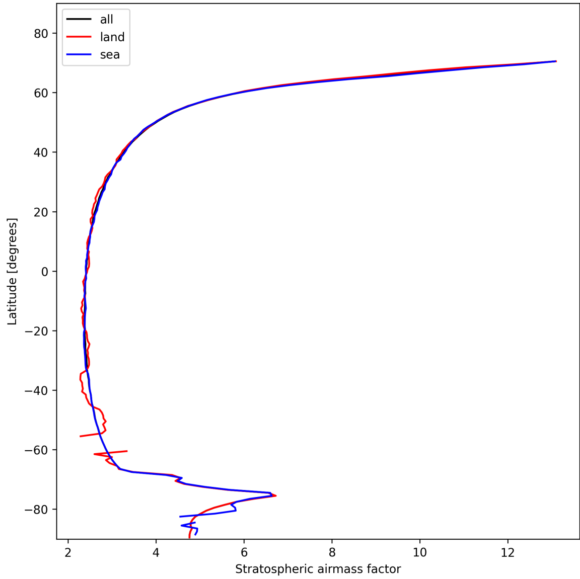
Figure 25: Zonal average of “Stratospheric air mass factor” for 2025-01-31 to 2025-01-31.
