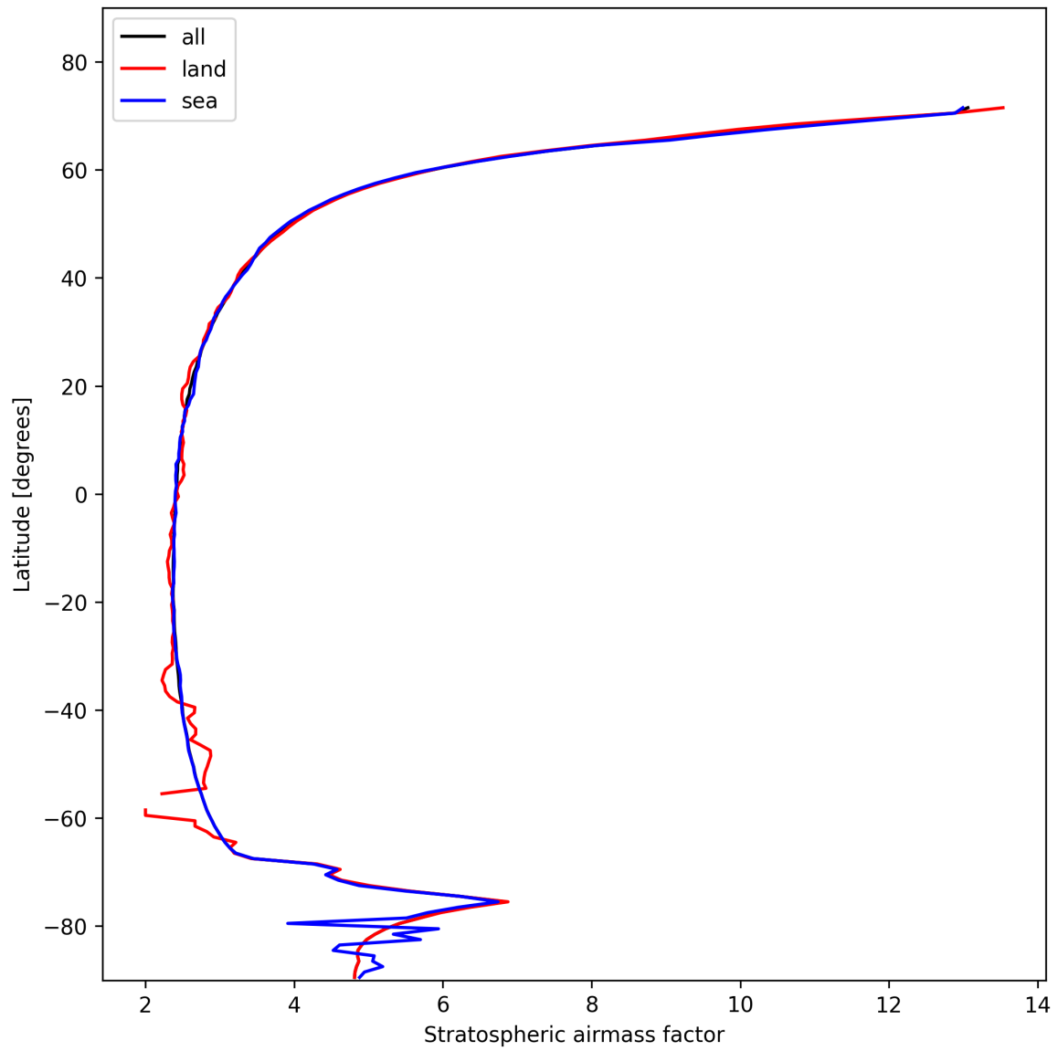
Figure 25: Zonal average of “Stratospheric airmass factor” for 2025-02-01 to 2025-02-02.
