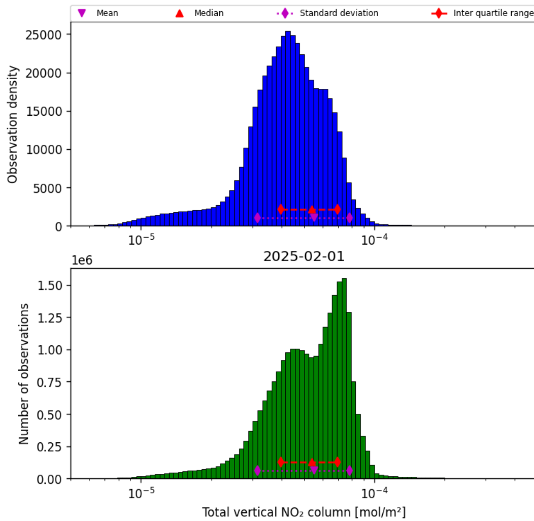
Figure 36: Histogram of “Total vertical NO 2 column” for 2025-02-01 to 2025-02-02
