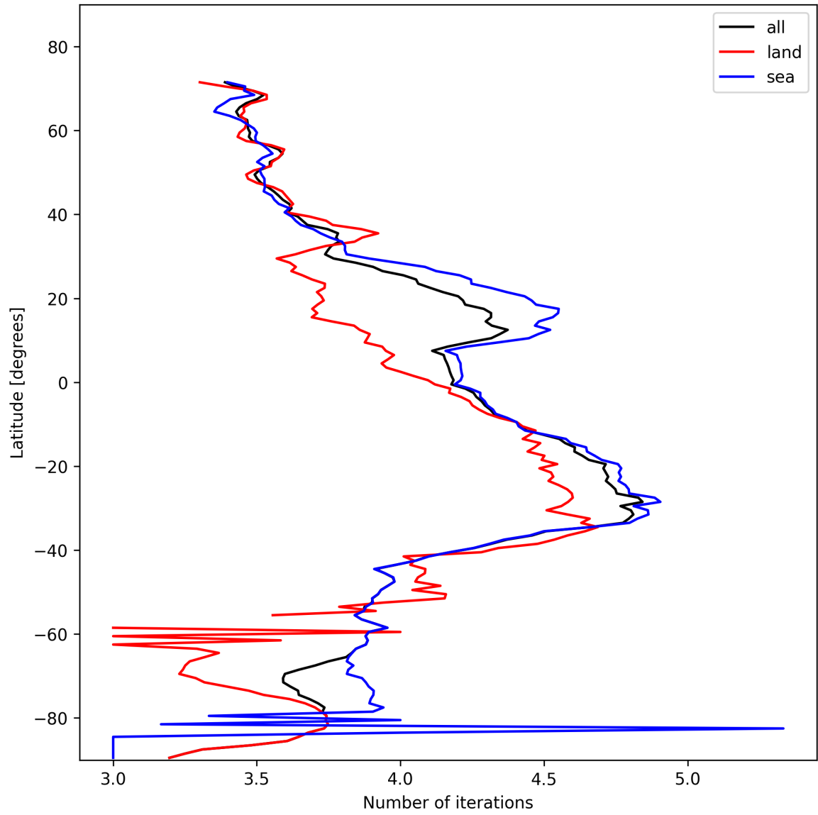
Figure 15: Zonal average of “Number of iterations” for 2025-02-01 to 2025-02-02.
