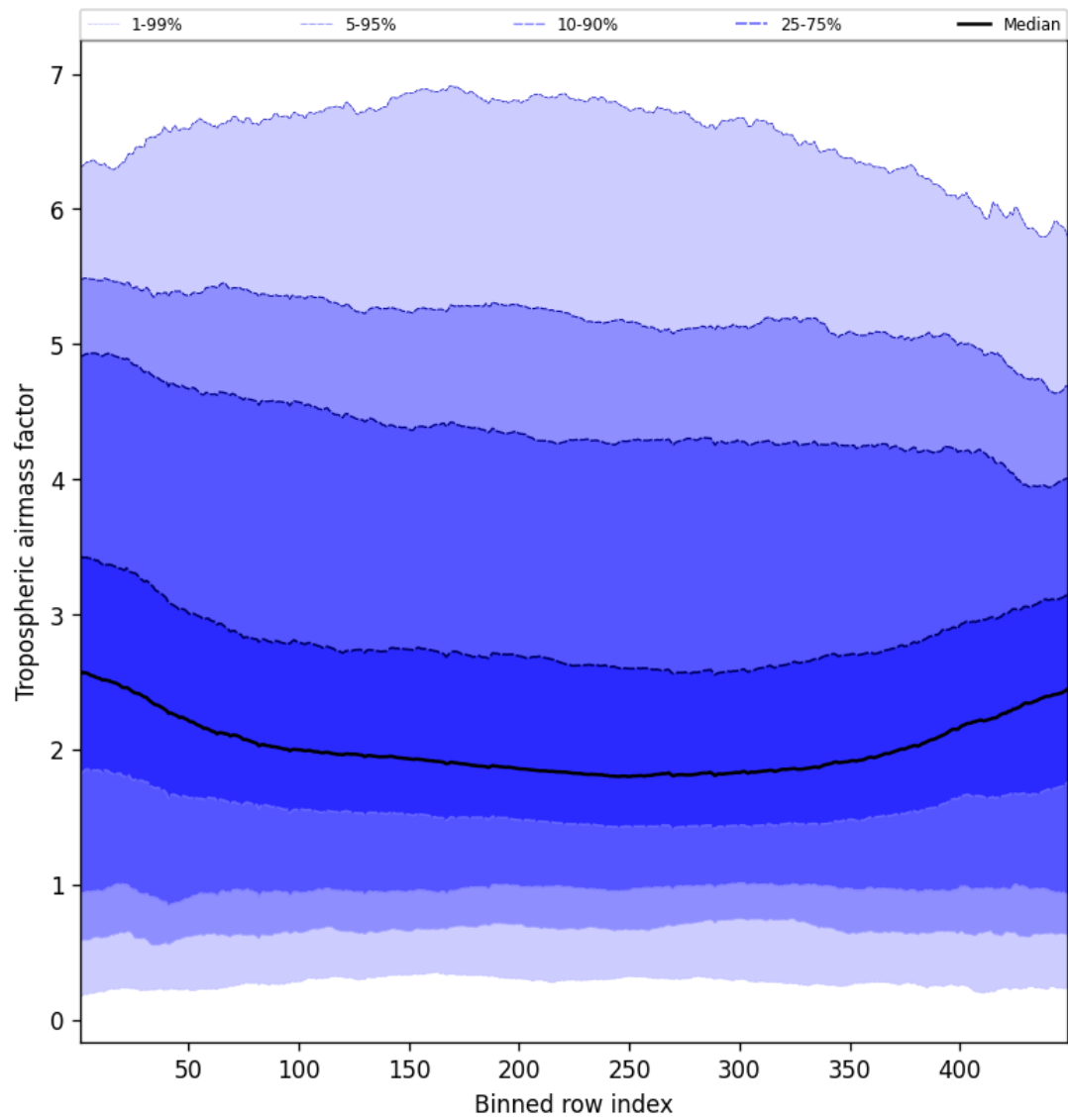
Figure 46: Along track statistics of “Tropospheric air mass factor” for 2025-02-01 to 2025-02-02
