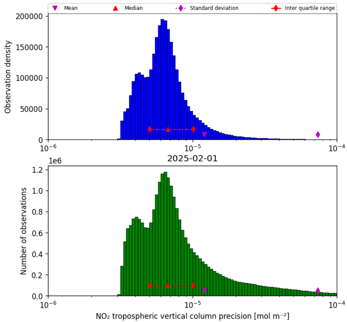
Figure 28: Histogram of “NO 2 tropospheric vertical column precision” for 2025-02-01 to 2025-02-02
