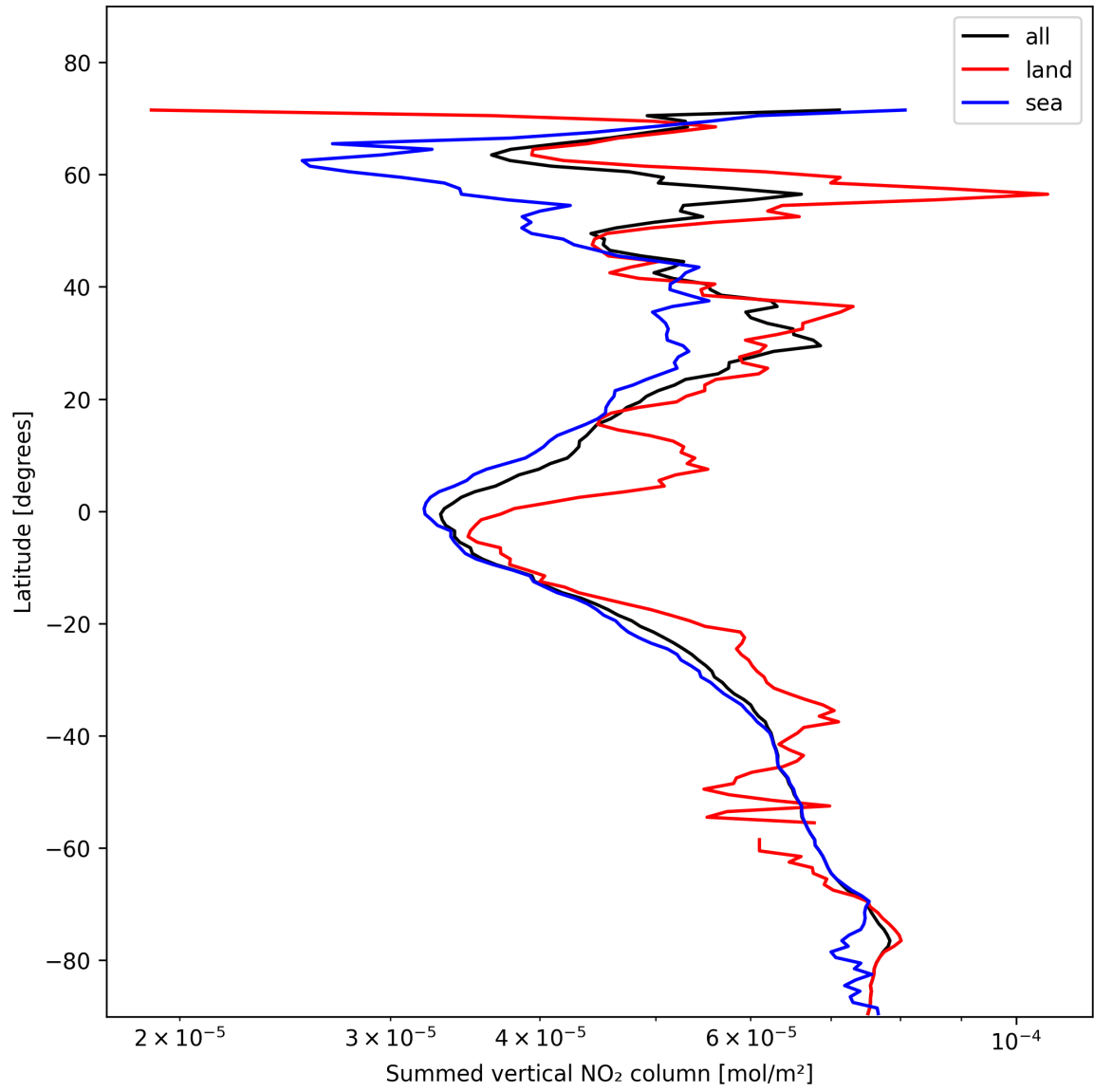
Figure 21: Zonal average of “Summed vertical NO 2 column” for 2025-02-01 to 2025-02-02.
