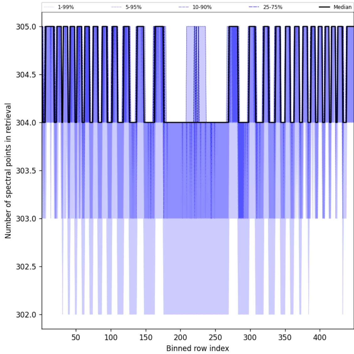
Figure 48: Along track statistics of “Number of spectral points in retrieval” for 2025-02-01 to 2025-02-02
