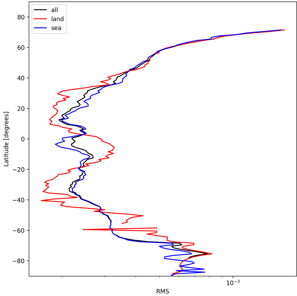
Figure 24: Zonal average of “RMS” for 2025-02-01 to 2025-02-02.
