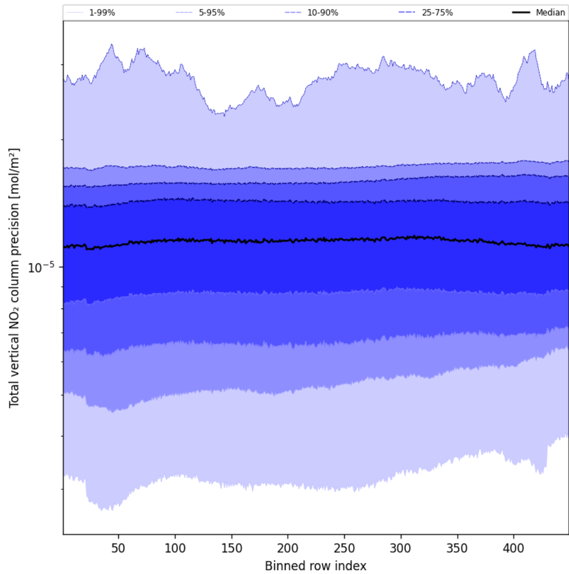
Figure 54: Along track statistics of “Total vertical NO 2 column precision” for 2025-02-01 to 2025-02-02
