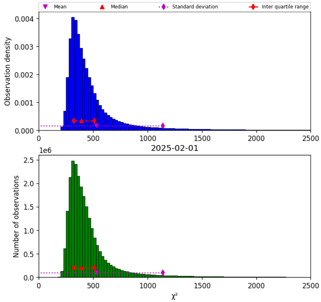
Figure 40: Histogram of “ \chi^2 ” for 2025-02-01 to 2025-02-02
