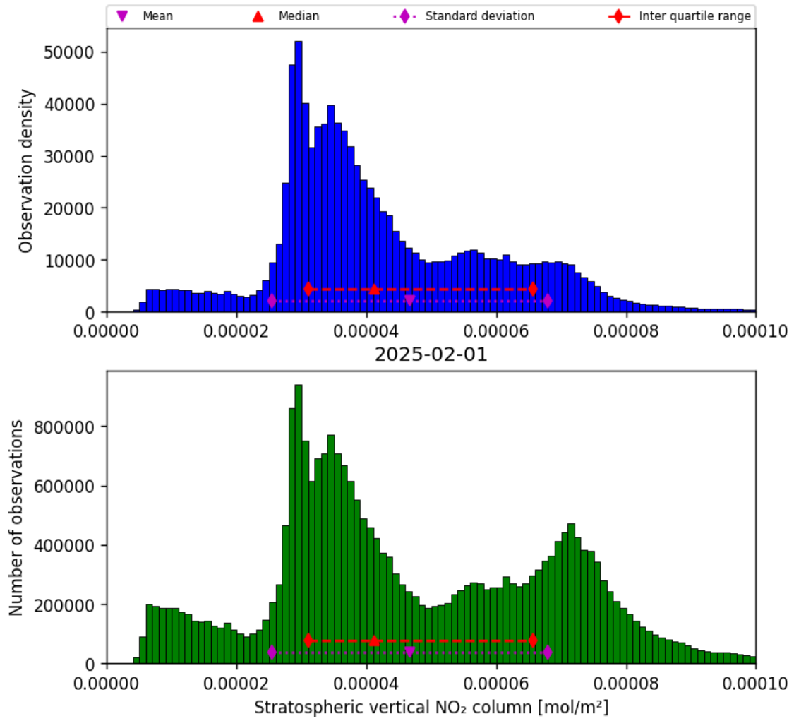
Figure 34: Histogram of “Stratospheric vertical NO 2 column” for 2025-02-01 to 2025-02-02
