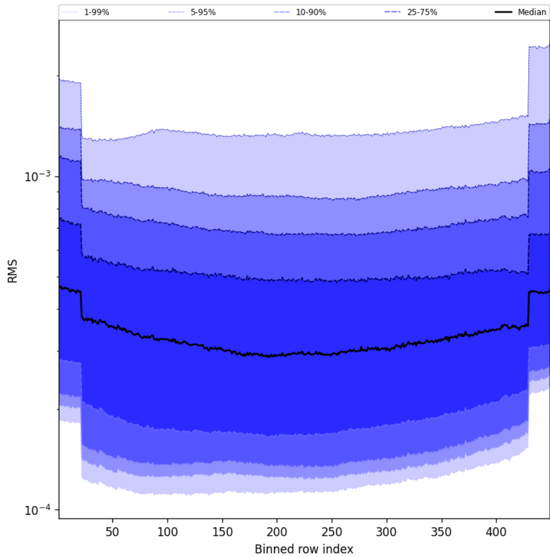
Figure 58: Along track statistics of “RMS” for 2025-02-01 to 2025-02-02
