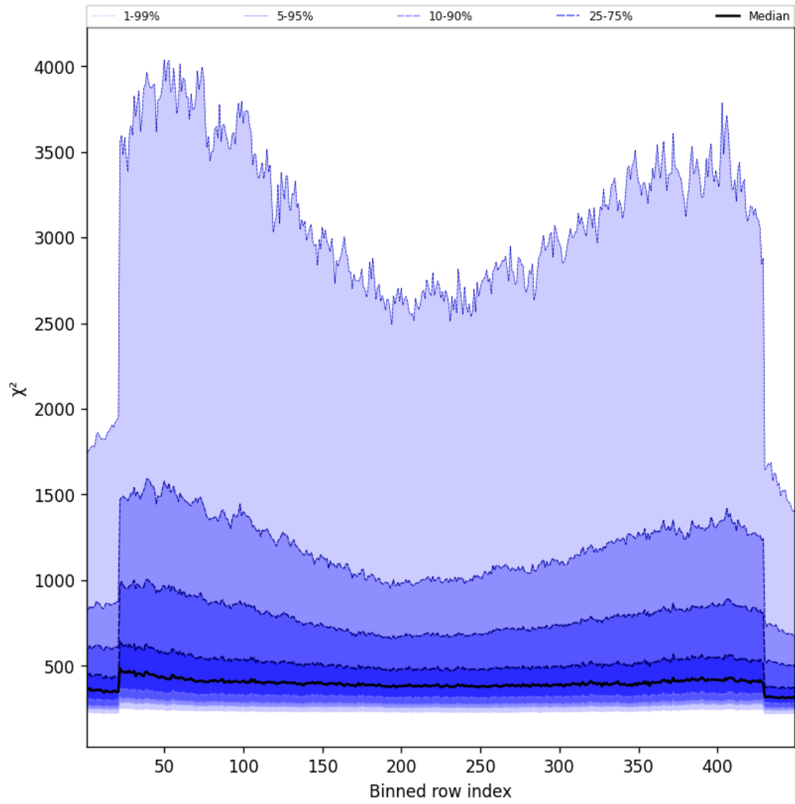
Figure 57: Along track statistics of “ \chi^2 ” for 2025-02-01 to 2025-02-02
