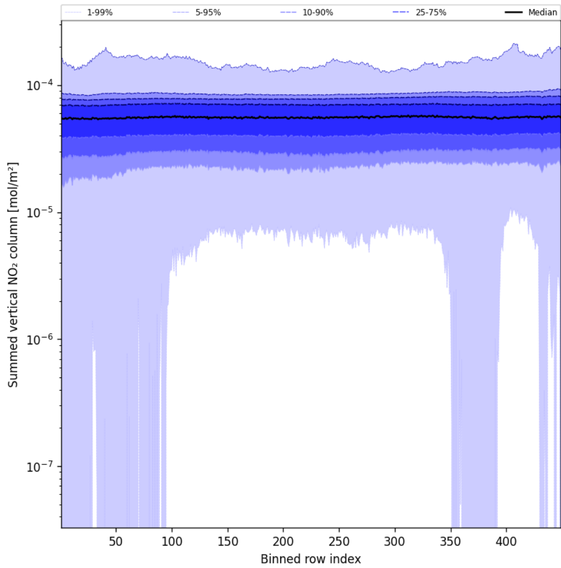
Figure 55: Along track statistics of “Summed vertical NO 2 column” for 2025-02-01 to 2025-02-02
