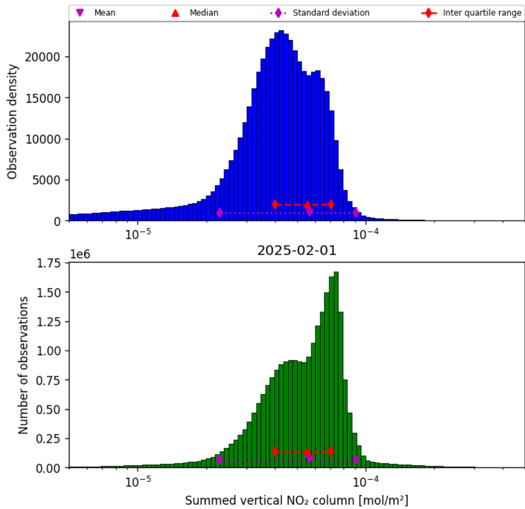
Figure 38: Histogram of “Summed vertical NO 2 column” for 2025-02-01 to 2025-02-02
