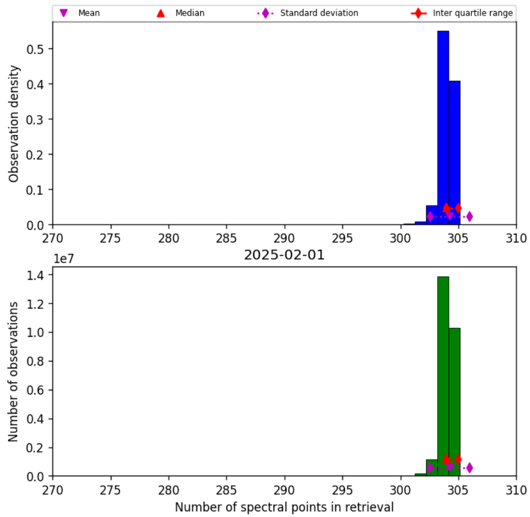
Figure 31: Histogram of “Number of spectral points in retrieval” for 2025-02-01 to 2025-02-02
