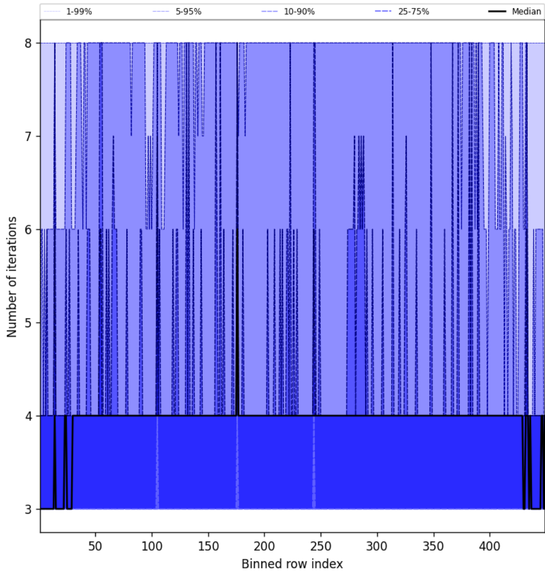
Figure 49: Along track statistics of “Number of iterations” for 2025-02-01 to 2025-02-02
