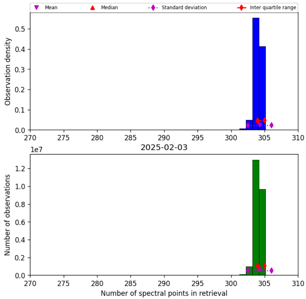
Figure 31: Histogram of “Number of spectral points in retrieval” for 2025-02-03 to 2025-02-04
