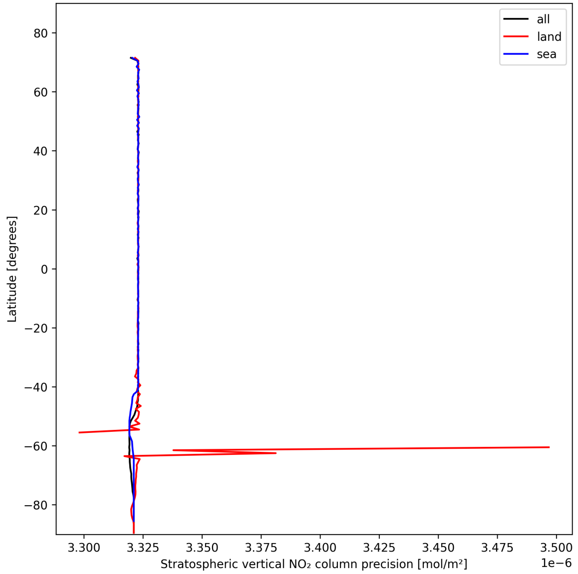
Figure 18: Zonal average of "Stratospheric vertical NO 2 column precision" for 2025-02-03 to 2025-02-04.
