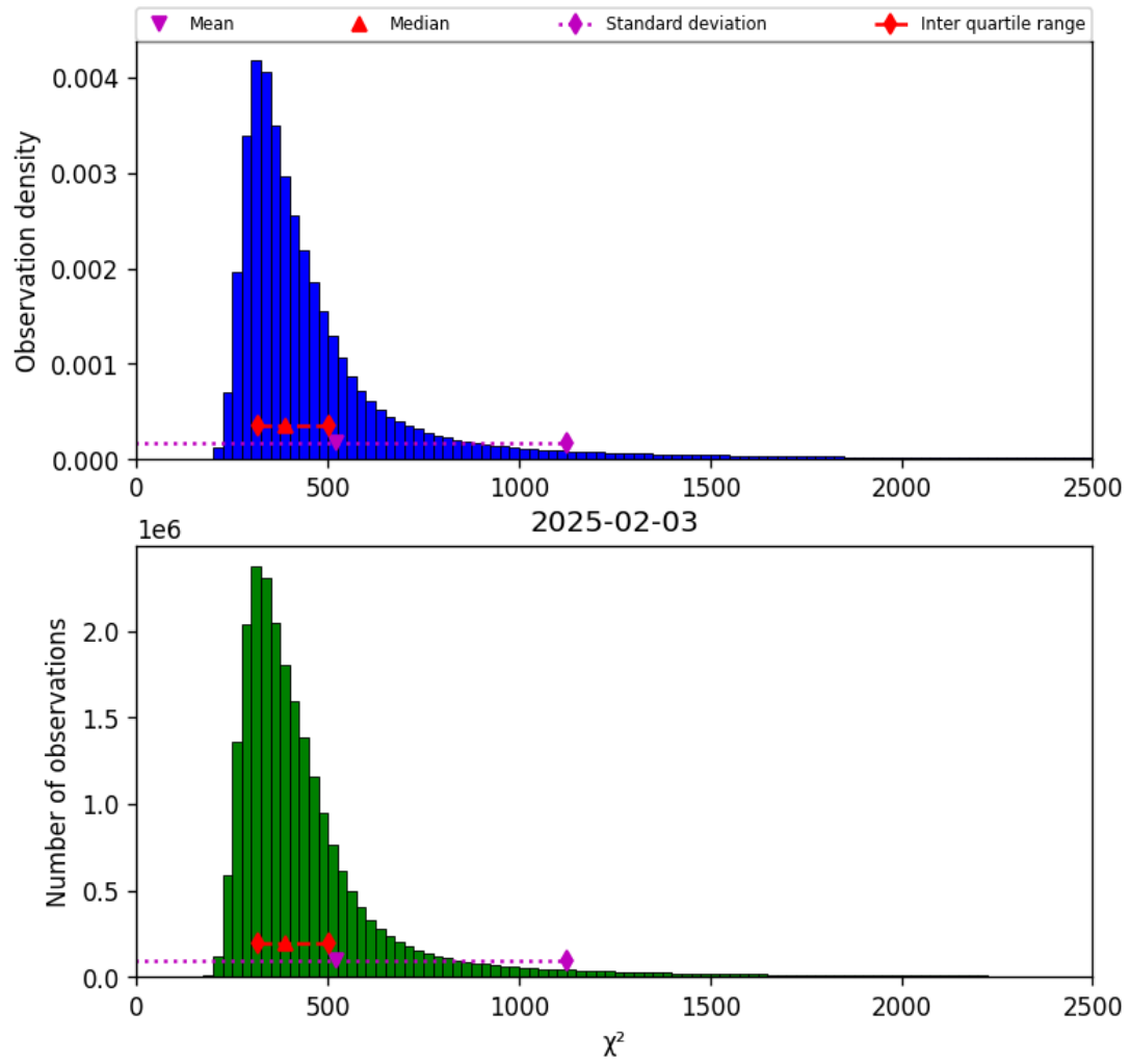
Figure 40: Histogram of “ \chi^2 ” for 2025-02-03 to 2025-02-04
