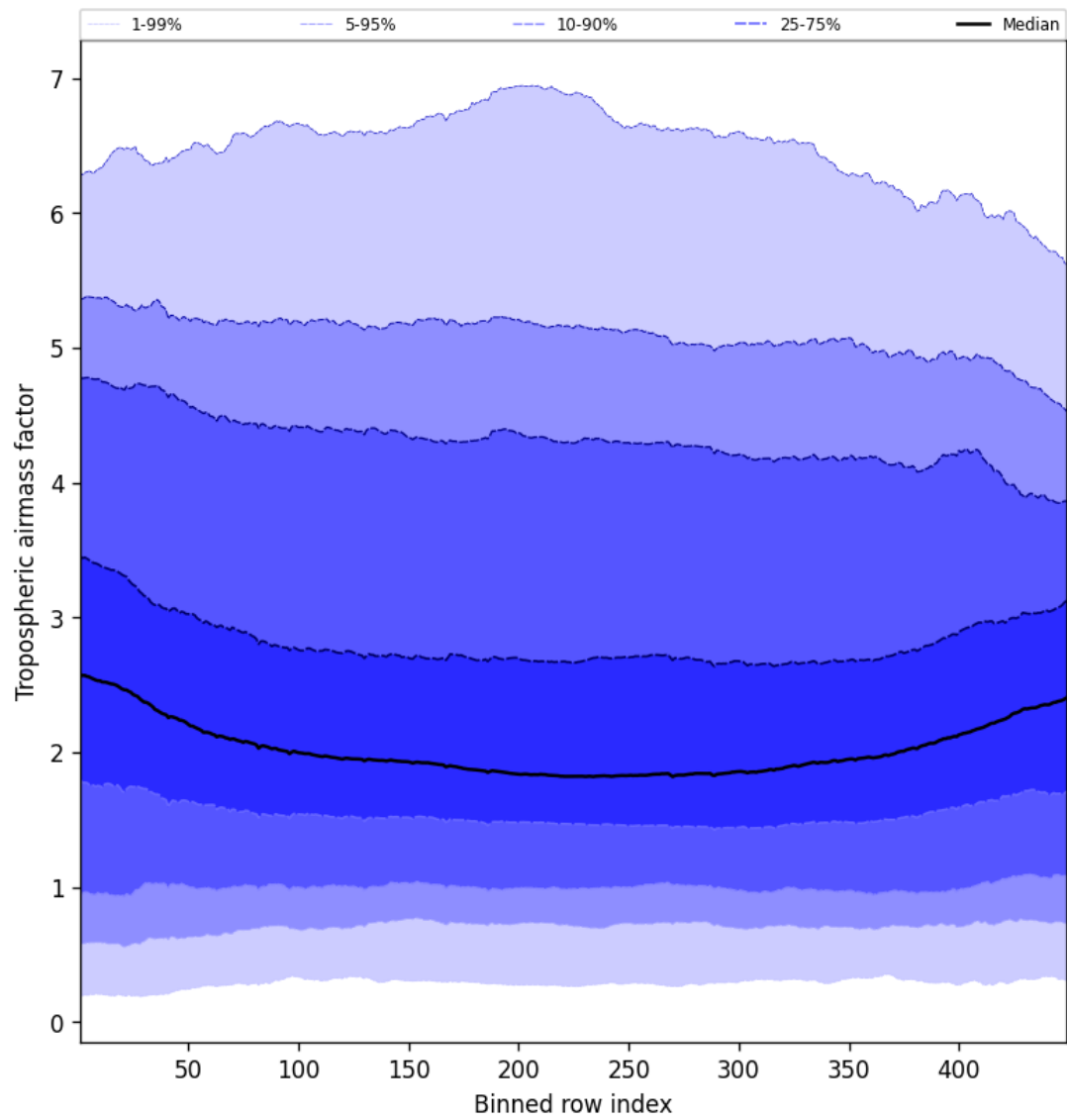
Figure 46: Along track statistics of “Tropospheric airmass factor” for 2025-02-03 to 2025-02-04
