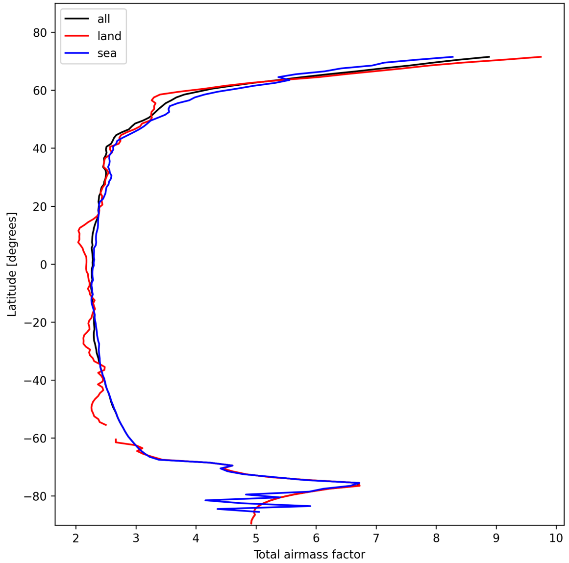
Figure 13: Zonal average of “Total airmass factor” for 2025-02-03 to 2025-02-04.
