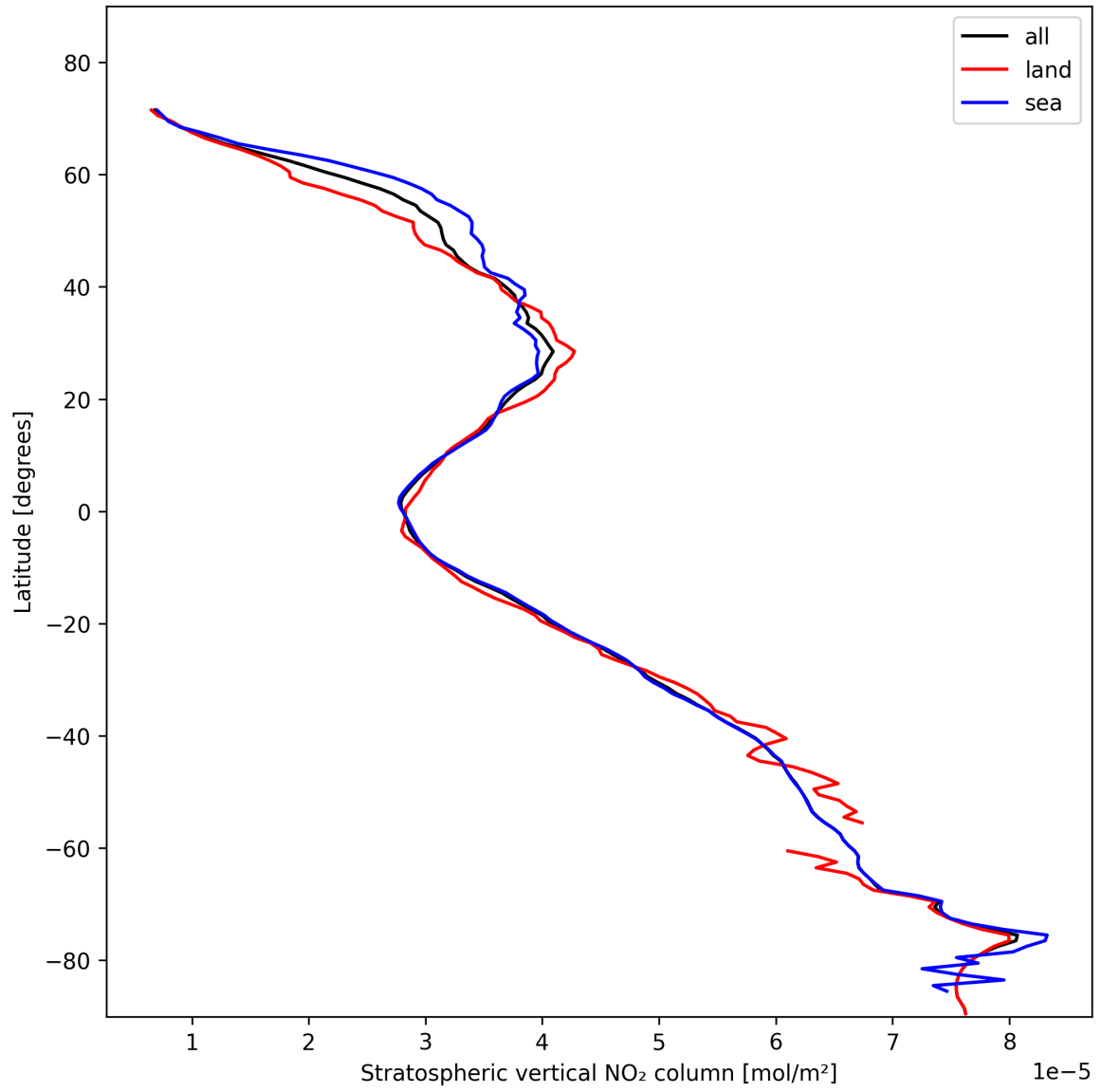
Figure 17: Zonal average of “Stratospheric vertical NO 2 column” for 2025-02-03 to 2025-02-04.
