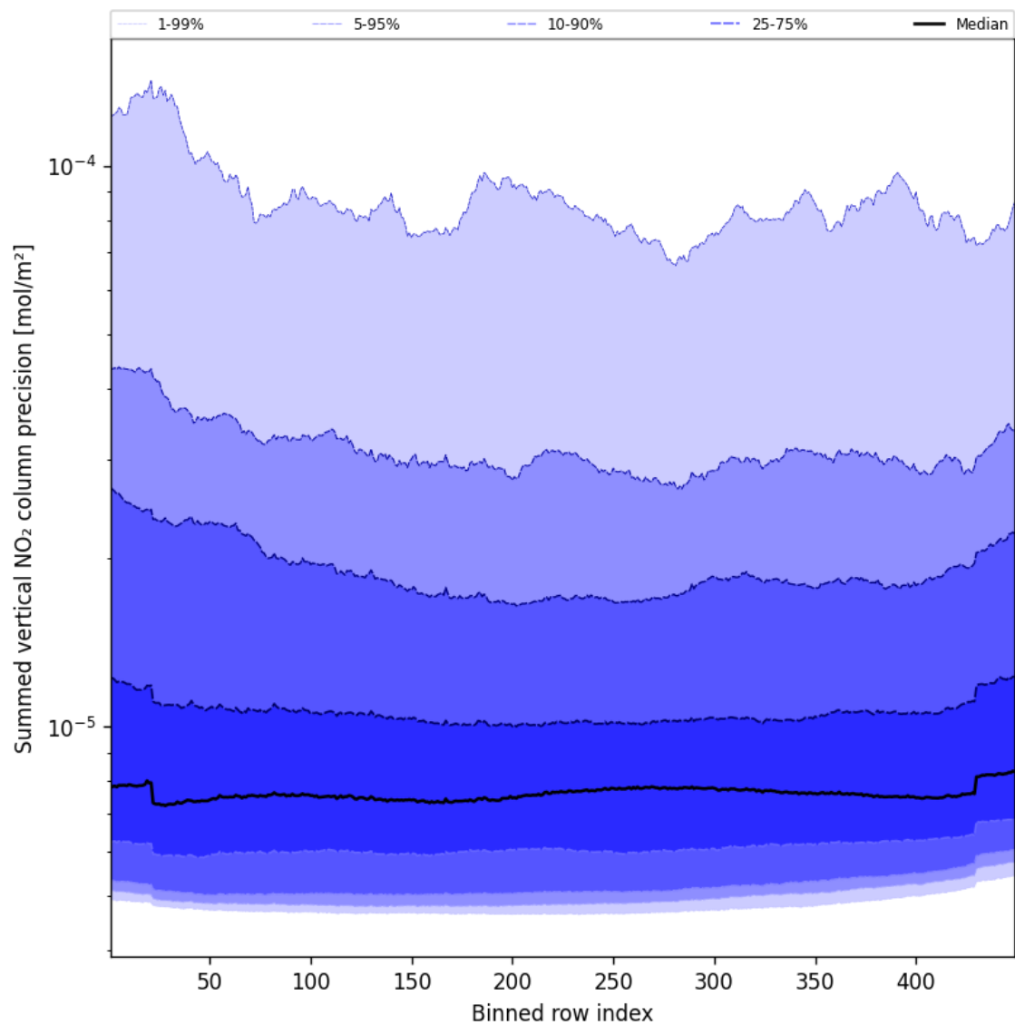
Figure 56: Along track statistics of “Summed vertical NO 2 column precision” for 2025-02-03 to 2025-02-04
