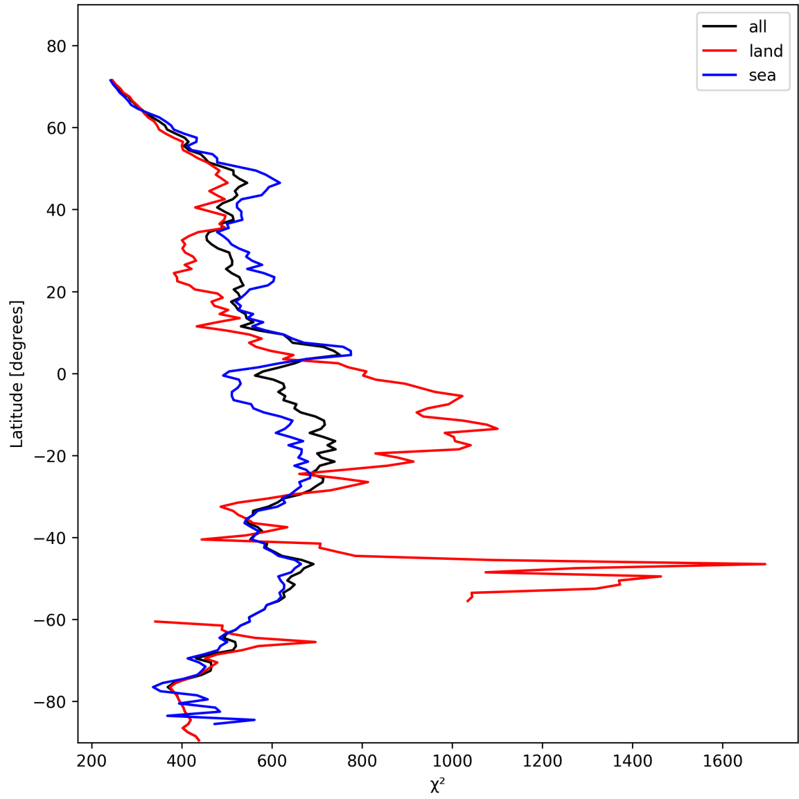
Figure 23: Zonal average of “ \chi^2 ” for 2025-02-03 to 2025-02-04.
