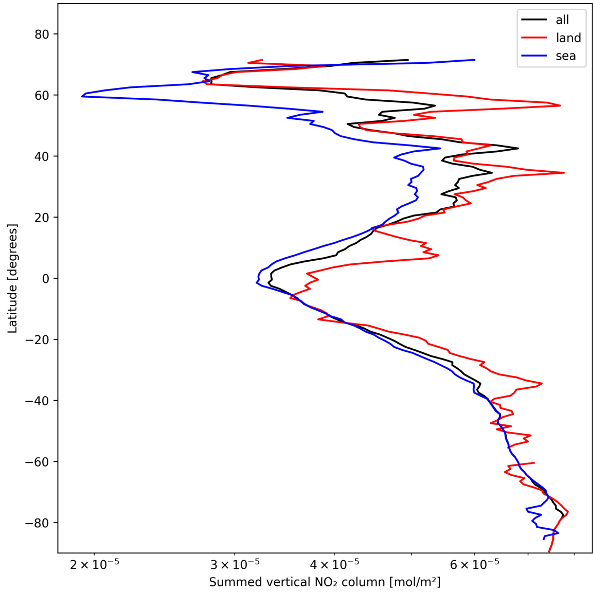
Figure 21: Zonal average of “Summed vertical NO 2 column” for 2025-02-03 to 2025-02-04.
