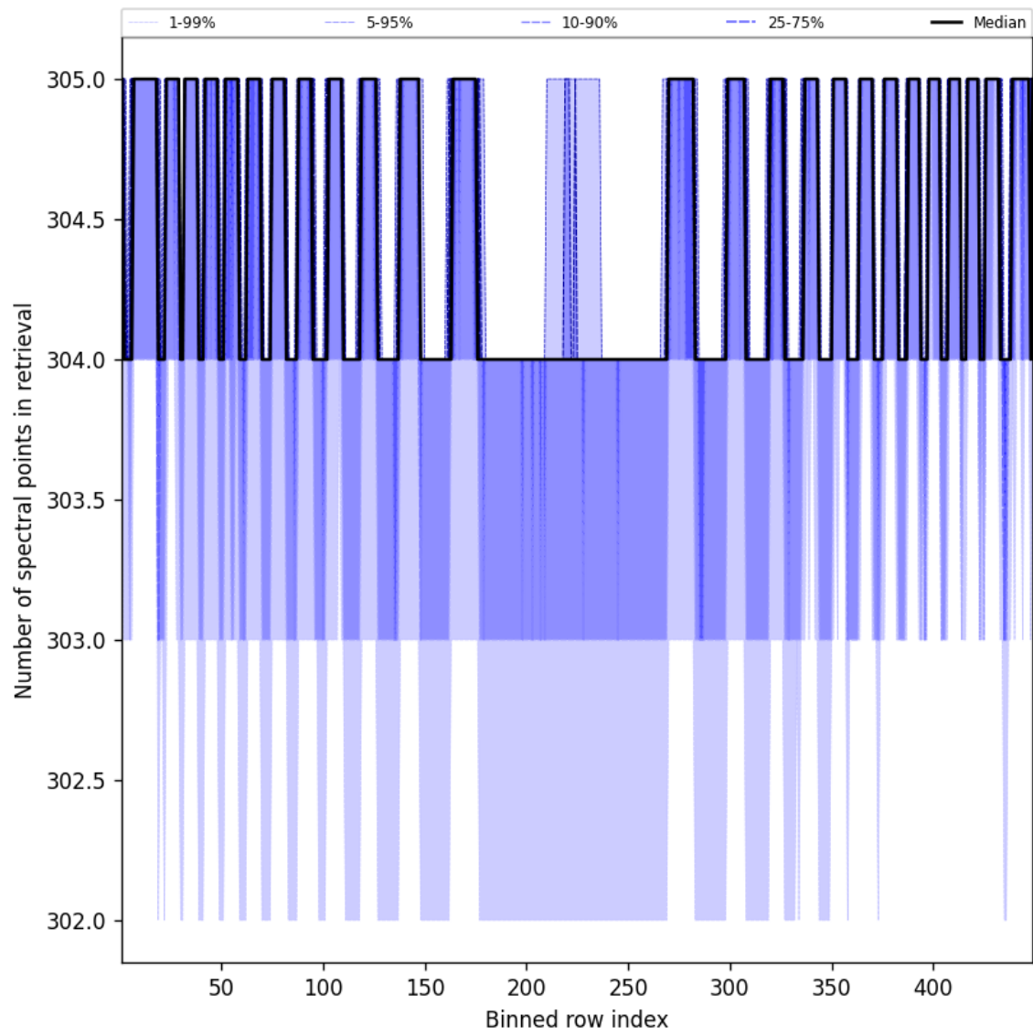
Figure 48: Along track statistics of “Number of spectral points in retrieval” for 2025-02-03 to 2025-02-04
