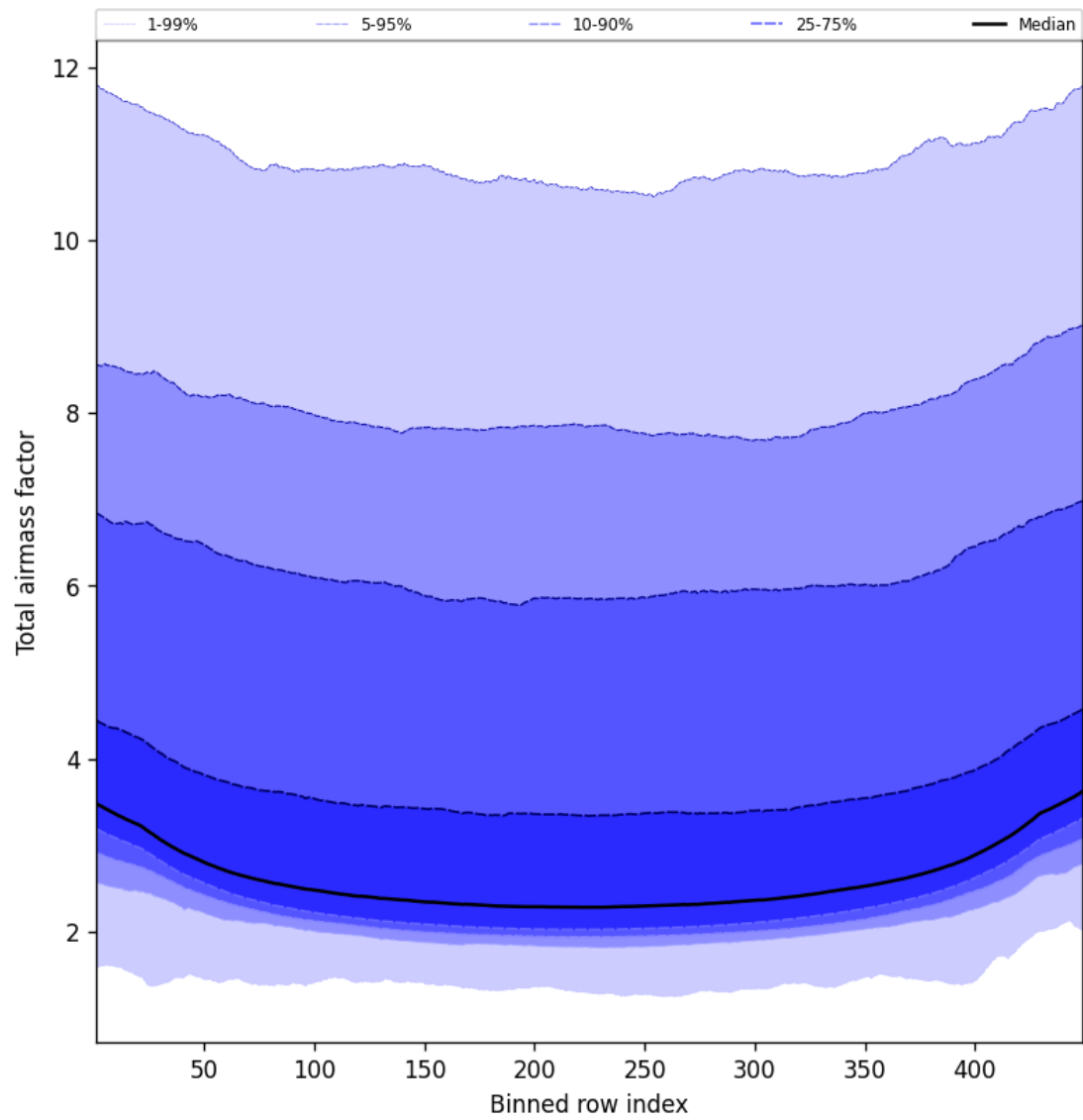
Figure 47: Along track statistics of “Total airmass factor” for 2025-02-03 to 2025-02-04
