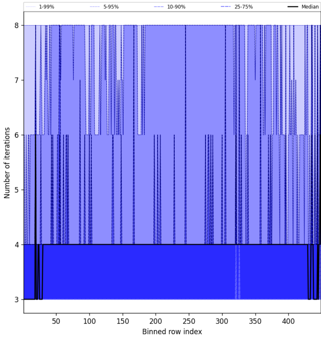
Figure 49: Along track statistics of “Number of iterations” for 2025-02-03 to 2025-02-04
