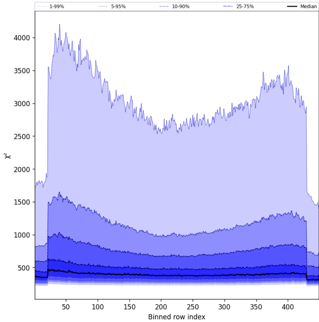
Figure 57: Along track statistics of “ \chi^2 ” for 2025-02-03 to 2025-02-04
