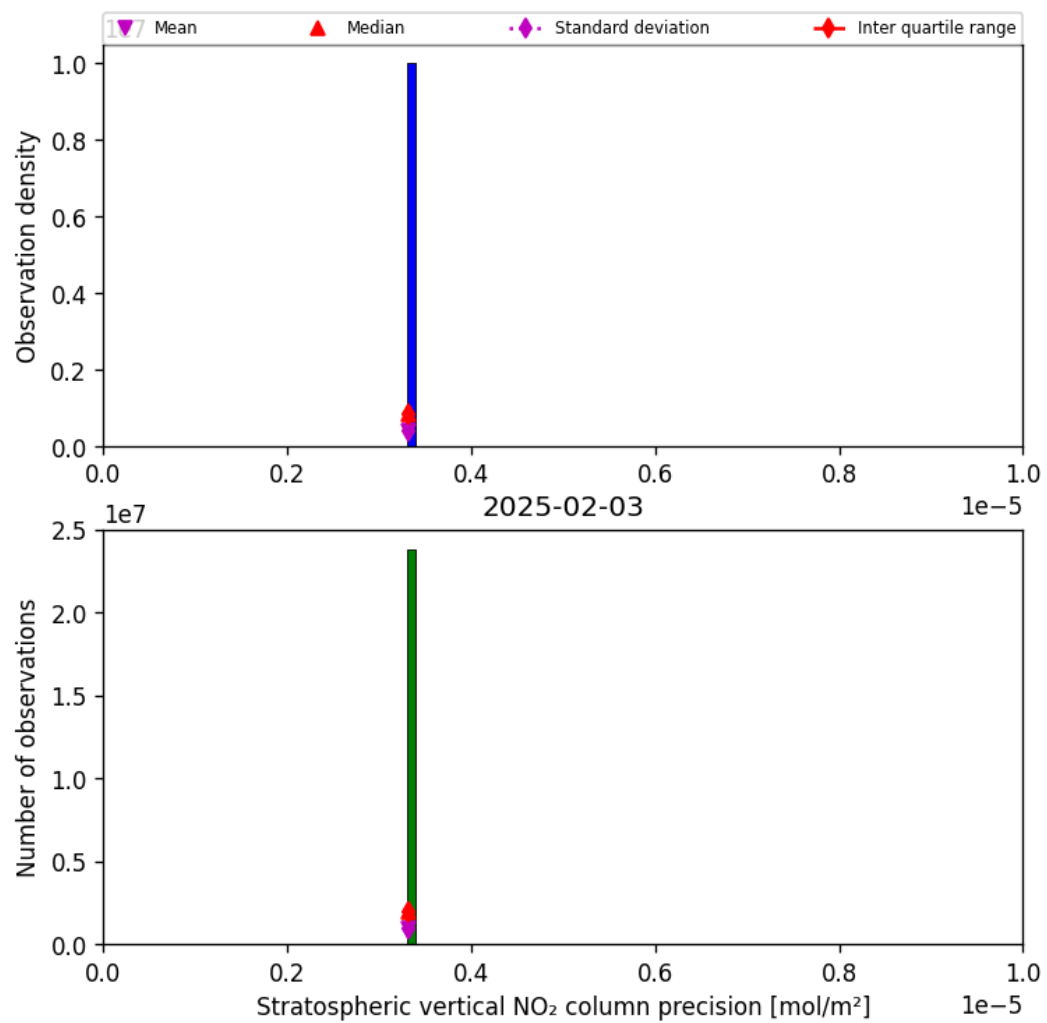
Figure 35: Histogram of “Stratospheric vertical NO 2 column precision” for 2025-02-03 to 2025-02-04
