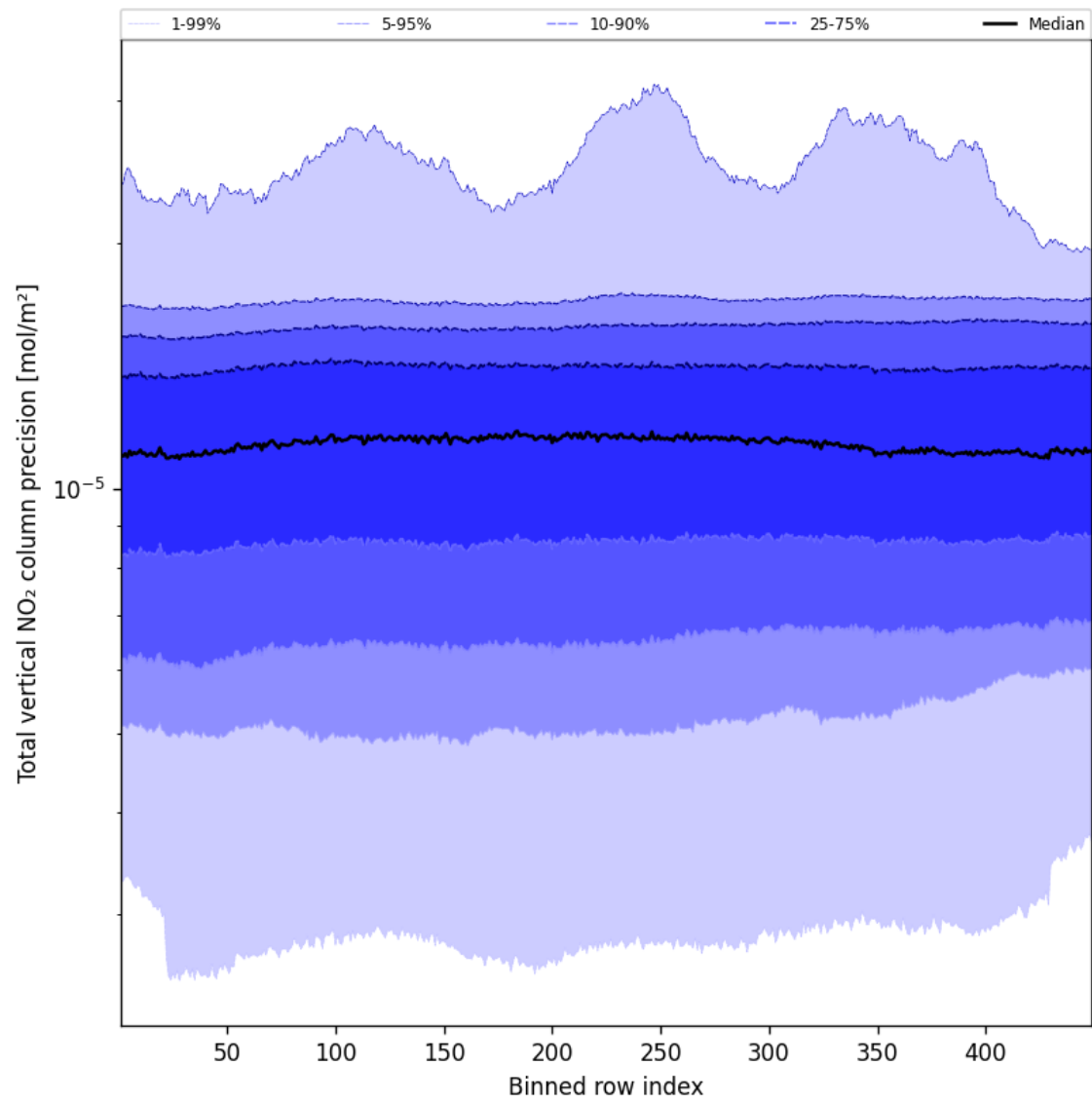
Figure 54: Along track statistics of “Total vertical NO 2 column precision” for 2025-02-03 to 2025-02-04
