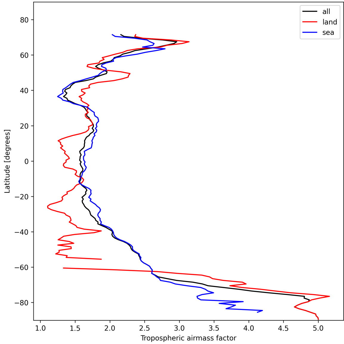
Figure 12: Zonal average of “Tropospheric airmass factor” for 2025-02-03 to 2025-02-04.
