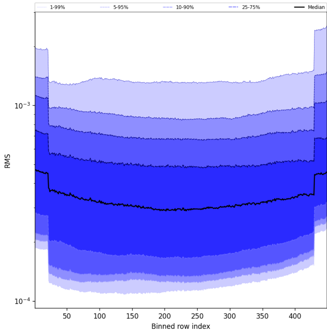
Figure 58: Along track statistics of “RMS” for 2025-02-03 to 2025-02-04
