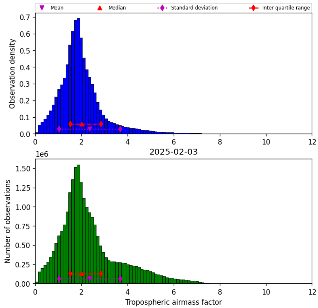
Figure 29: Histogram of “Tropospheric airmass factor” for 2025-02-03 to 2025-02-04
