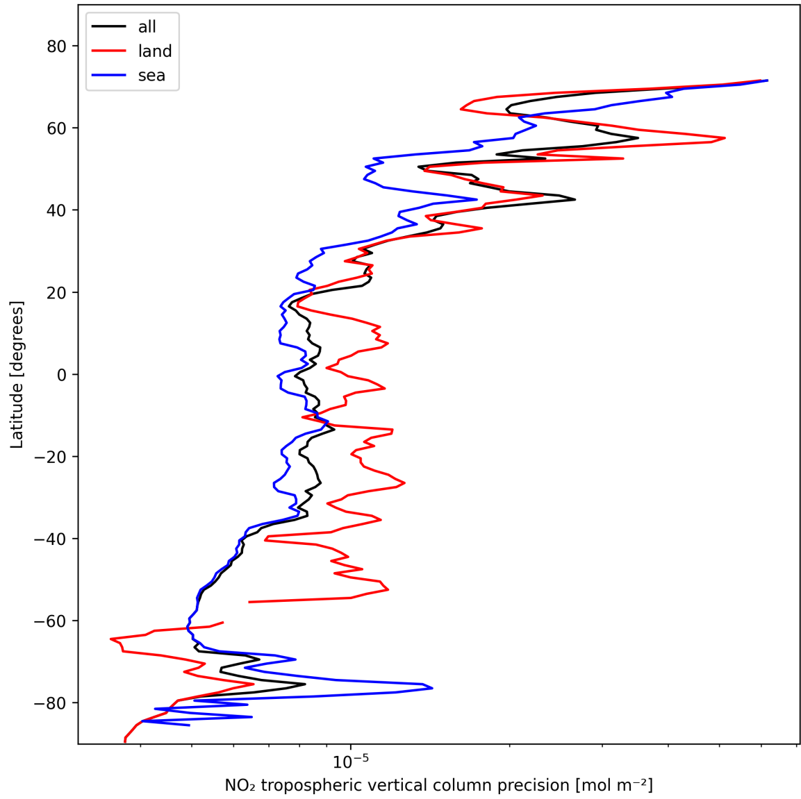
Figure 11: Zonal average of "NO 2 tropospheric vertical column precision" for 2025-02-03 to 2025-02-04.
