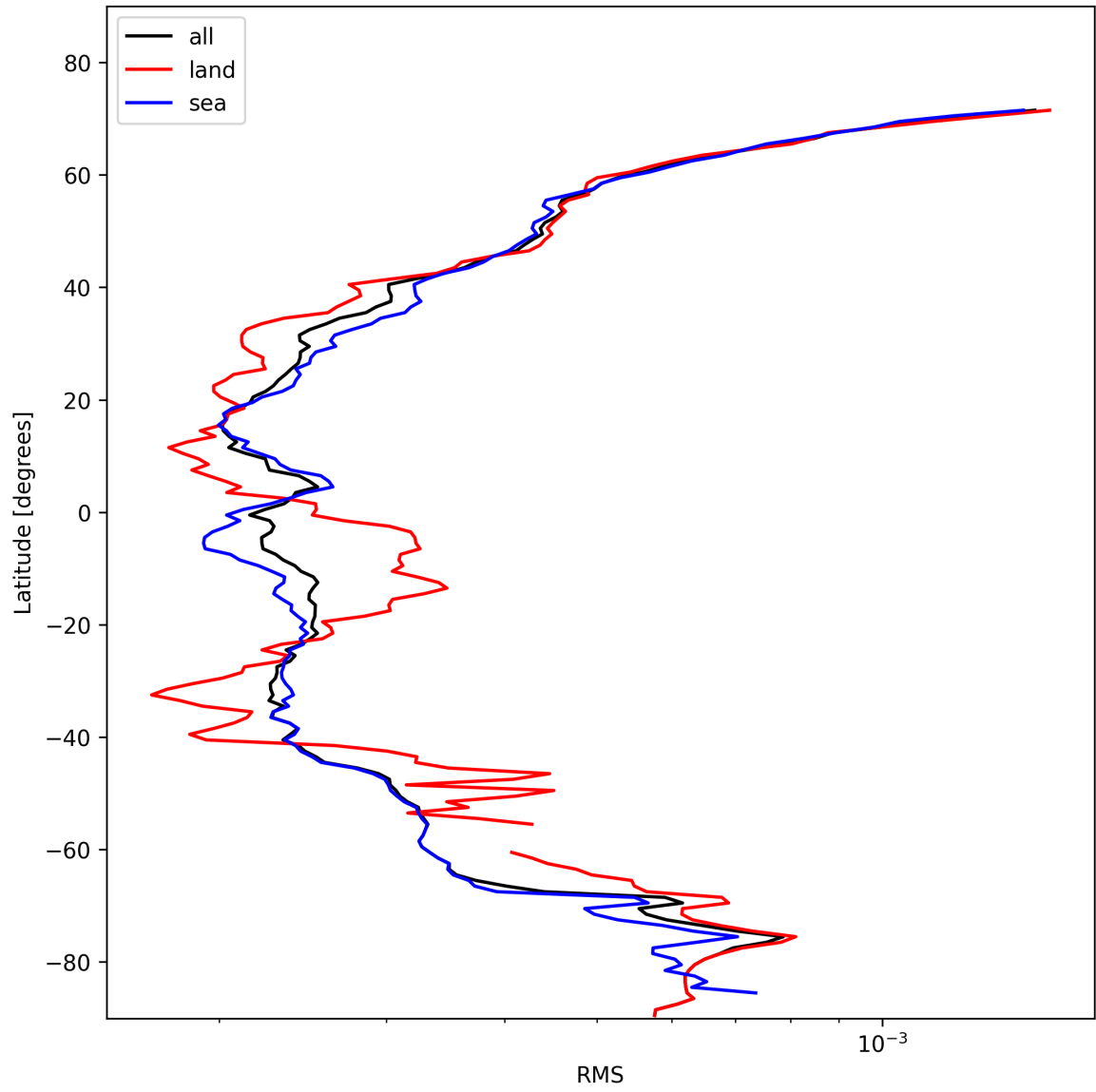
Figure 24: Zonal average of “RMS” for 2025-02-03 to 2025-02-04.
