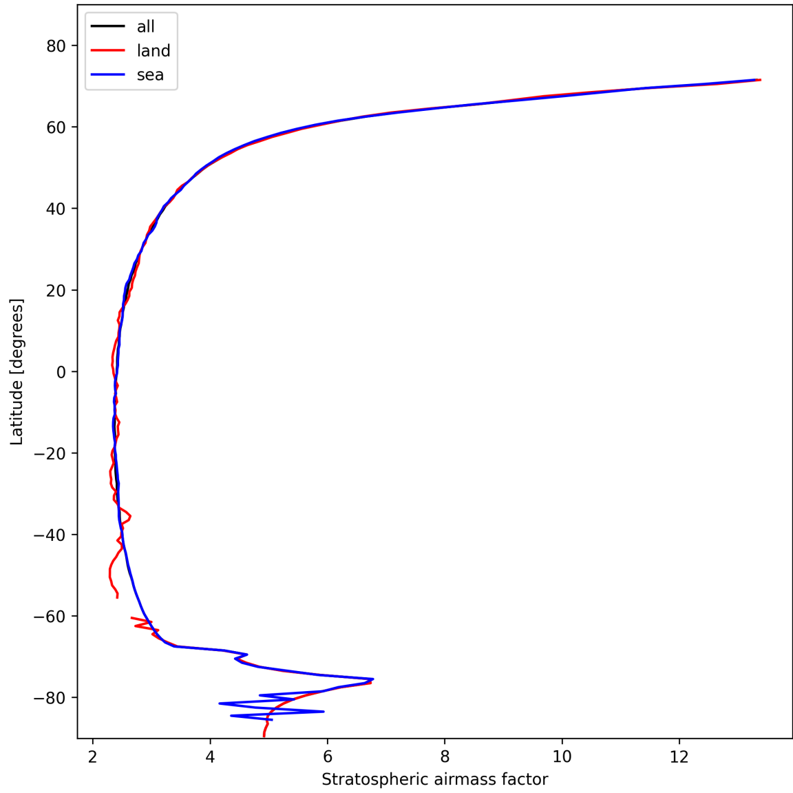
Figure 25: Zonal average of “Stratospheric air mass factor” for 2025-02-03 to 2025-02-04.
