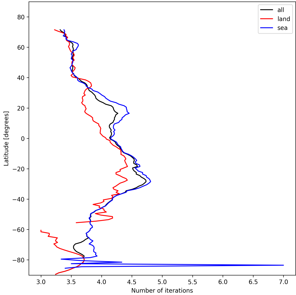
Figure 15: Zonal average of “Number of iterations” for 2025-02-03 to 2025-02-04.
