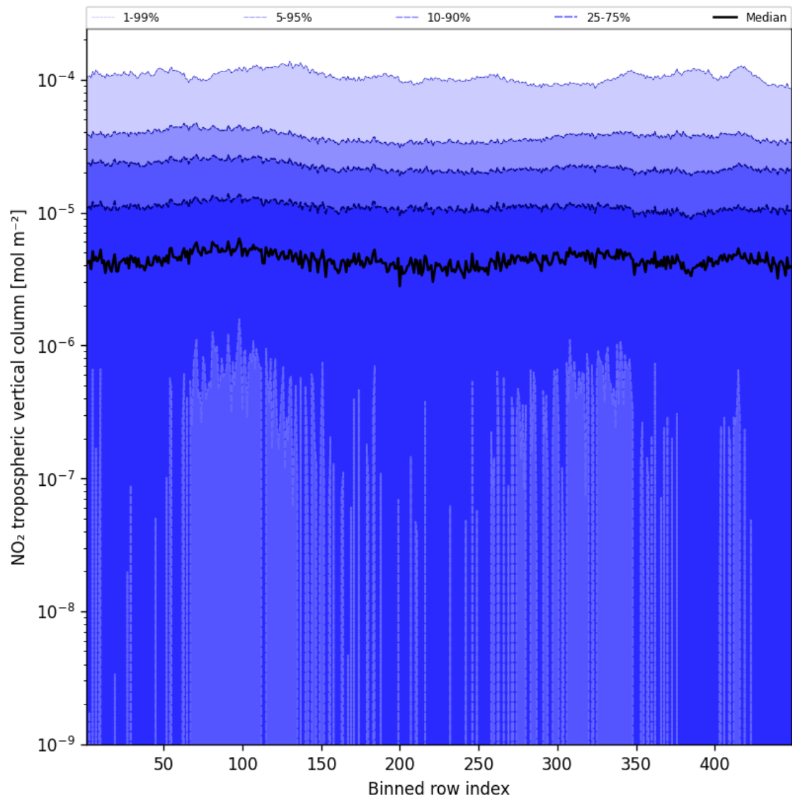
Figure 44: Along track statistics of “NO 2 tropospheric vertical column” for 2025-02-03 to 2025-02-04
