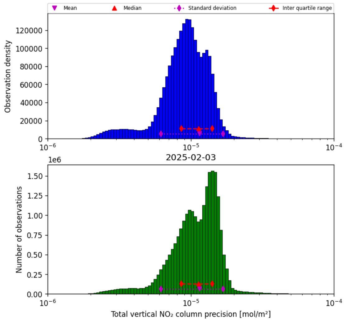
Figure 37: Histogram of “Total vertical NO 2 column precision” for 2025-02-03 to 2025-02-04
