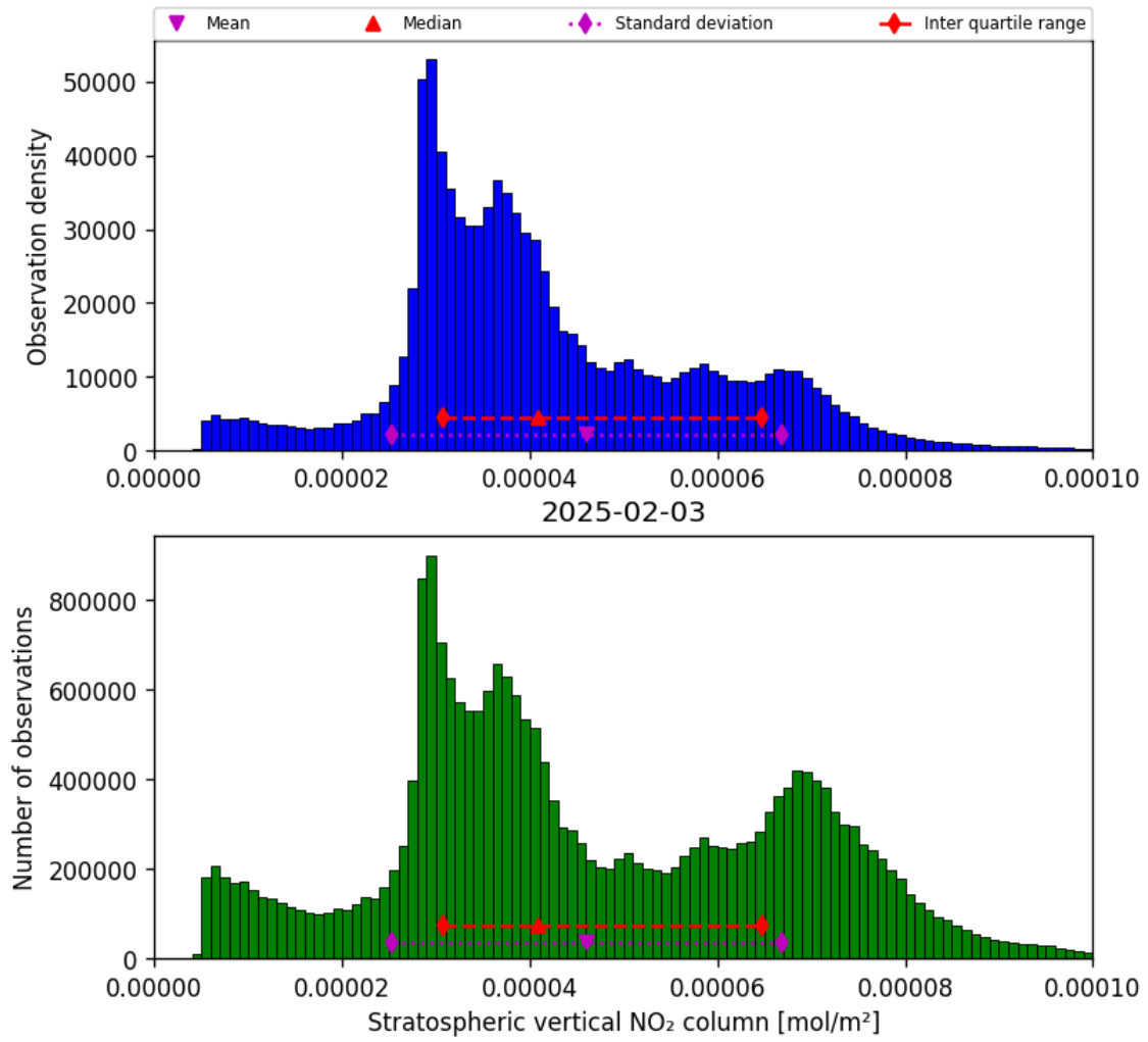
Figure 34: Histogram of “Stratospheric vertical NO 2 column” for 2025-02-03 to 2025-02-04
