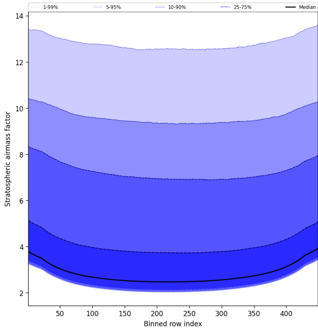
Figure 59: Along track statistics of “Stratospheric airmass factor” for 2025-02-03 to 2025-02-04
