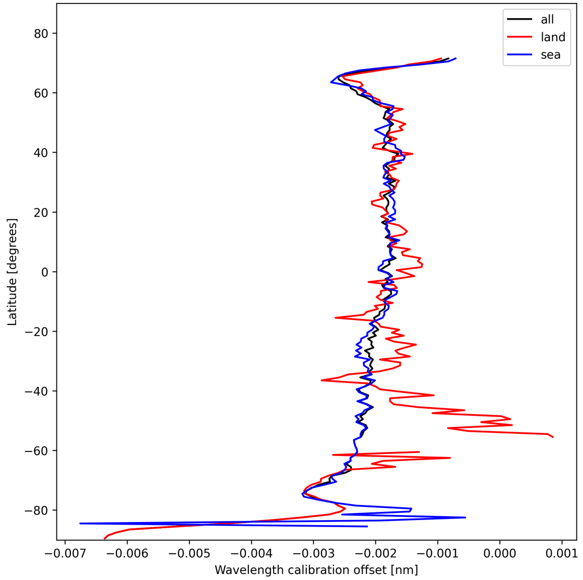
Figure 16: Zonal average of “Wavelength calibration offset” for 2025-02-03 to 2025-02-04.
