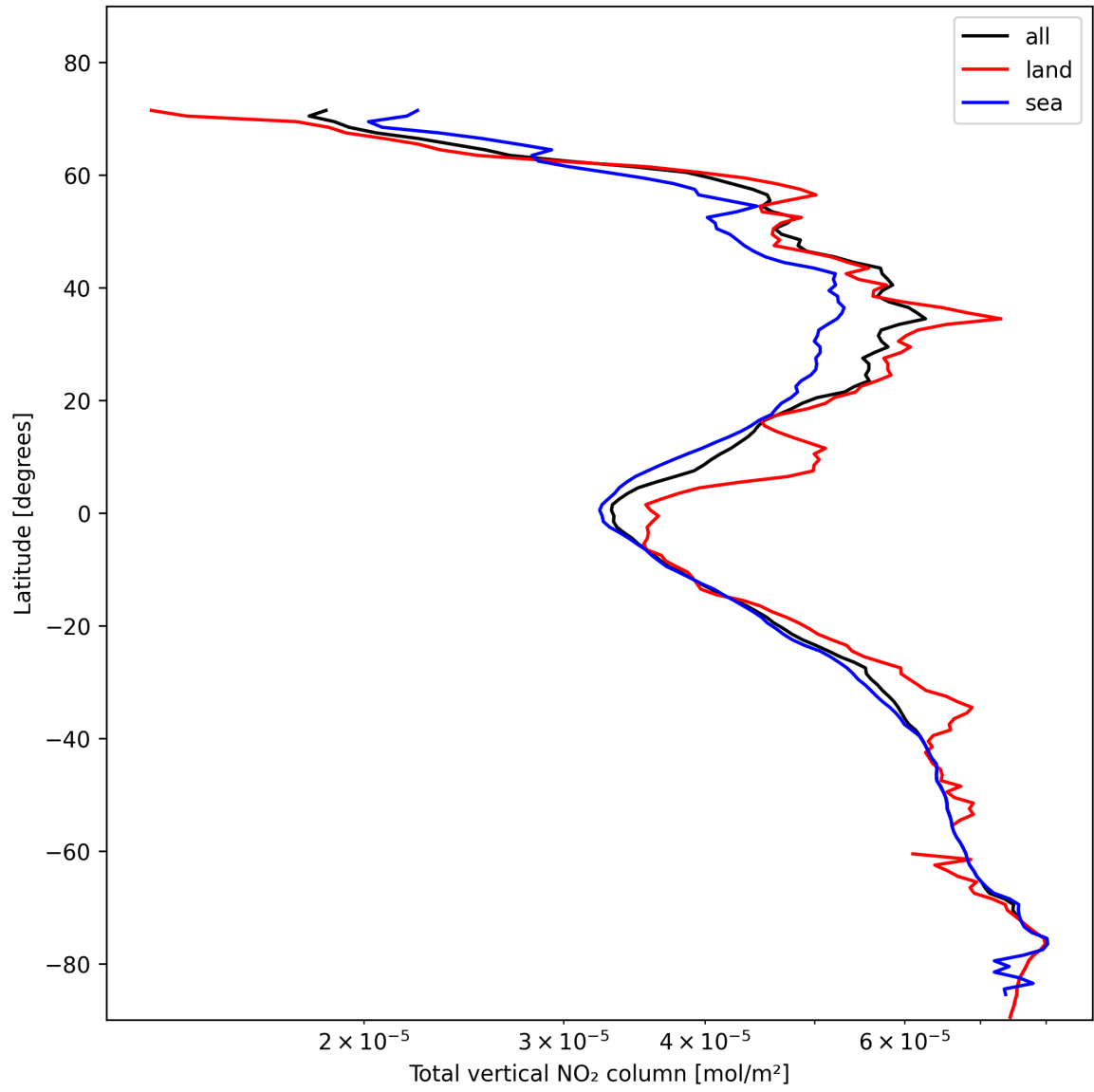
Figure 19: Zonal average of “Total vertical NO 2 column” for 2025-02-03 to 2025-02-04.
