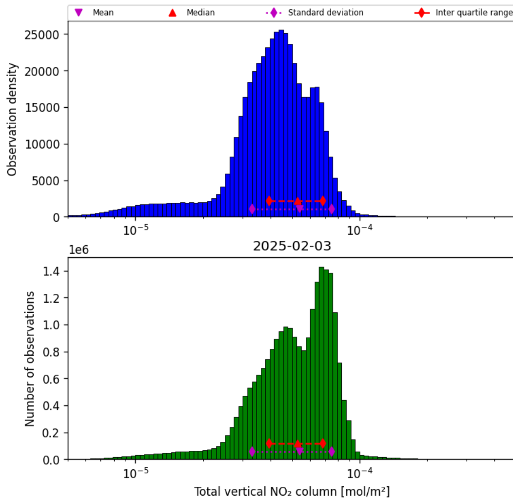
Figure 36: Histogram of “Total vertical NO 2 column” for 2025-02-03 to 2025-02-04
