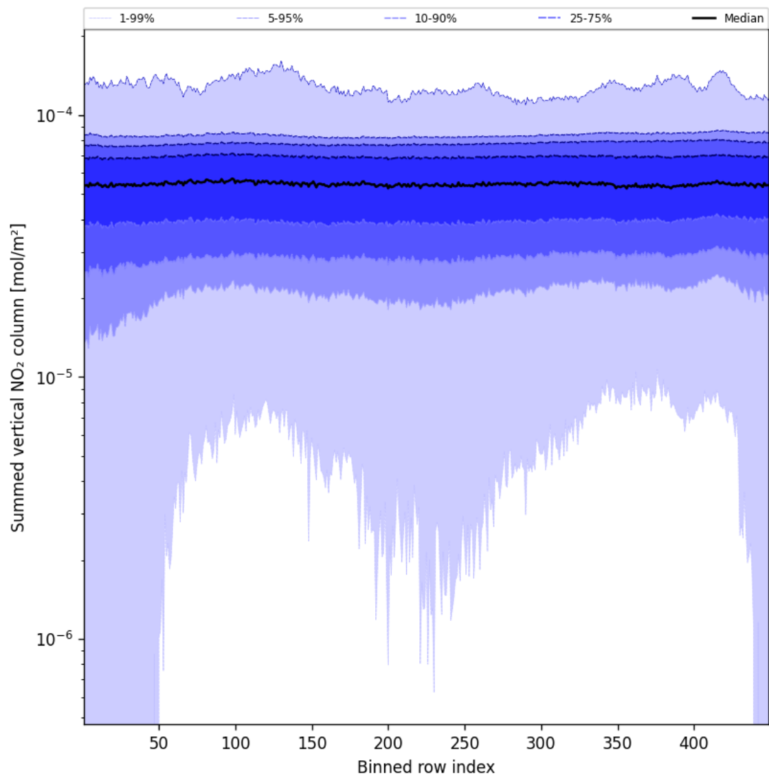
Figure 55: Along track statistics of “Summed vertical NO 2 column” for 2025-02-03 to 2025-02-04
