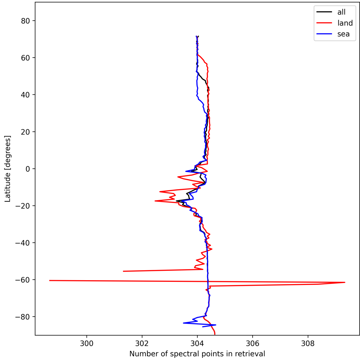
Figure 14: Zonal average of “Number of spectral points in retrieval” for 2025-02-03 to 2025-02-04.
