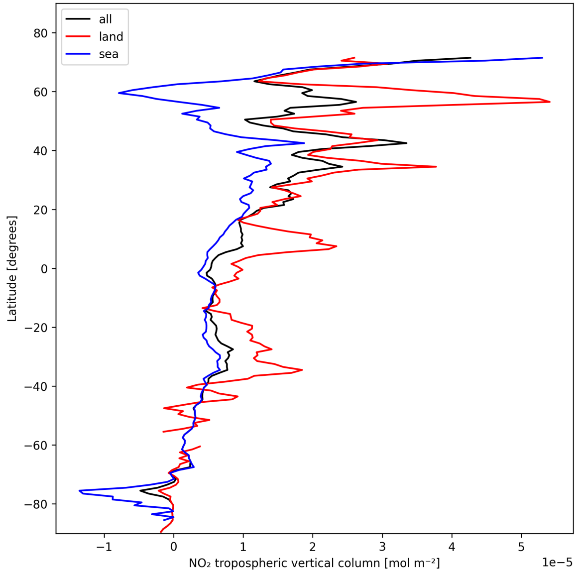
Figure 10: Zonal average of “NO 2 tropospheric vertical column” for 2025-02-03 to 2025-02-04.
