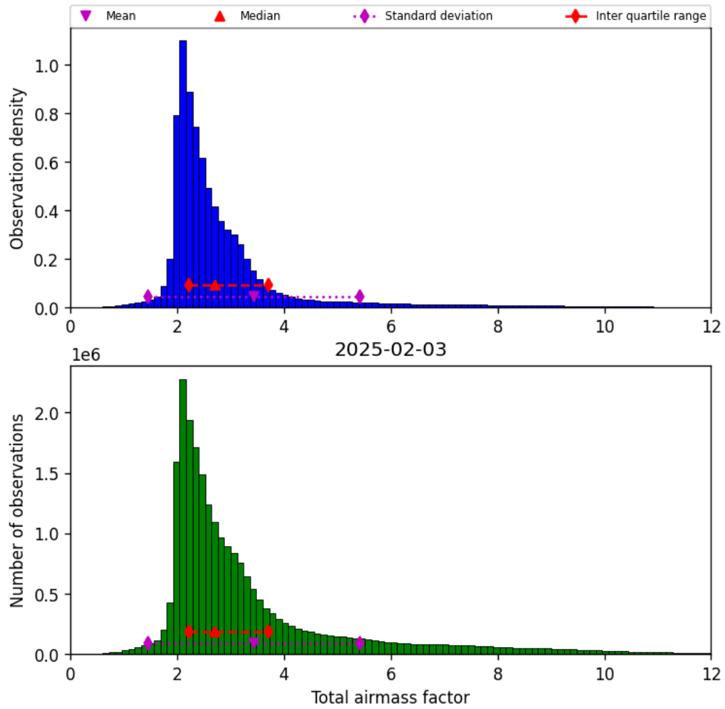
Figure 30: Histogram of “Total airmass factor” for 2025-02-03 to 2025-02-04
