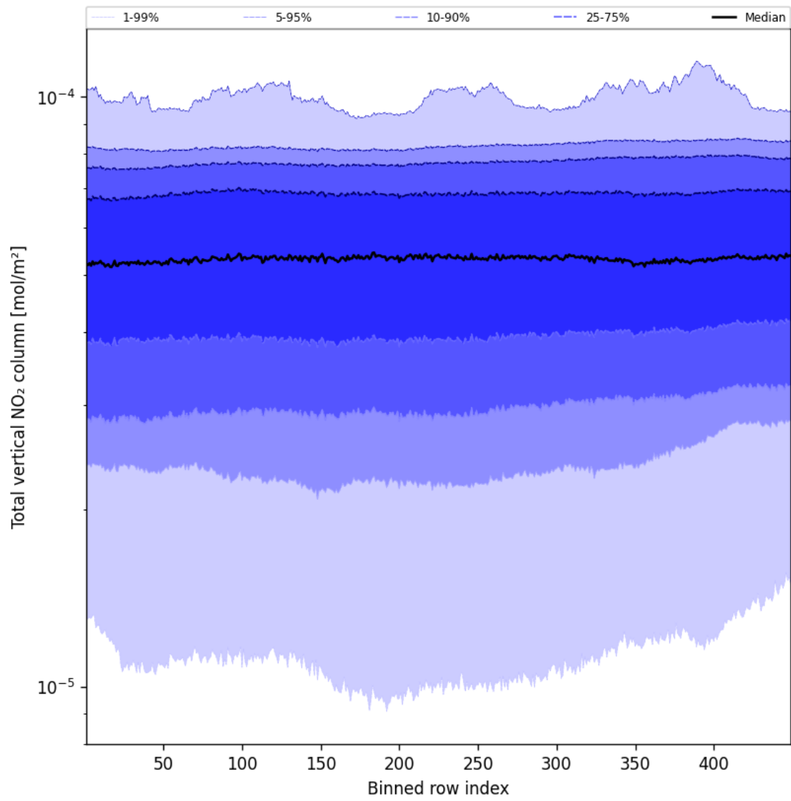
Figure 53: Along track statistics of “Total vertical NO 2 column” for 2025-02-03 to 2025-02-04
