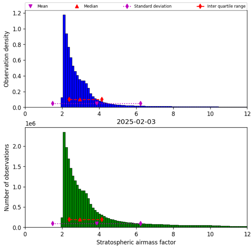
Figure 42: Histogram of “Stratospheric airmass factor” for 2025-02-03 to 2025-02-04
