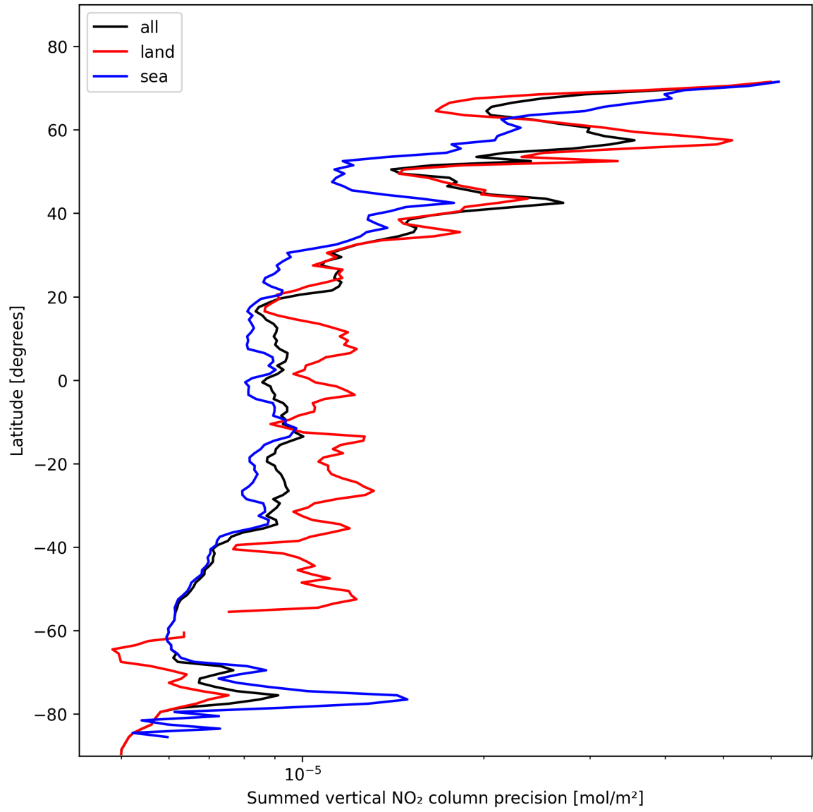
Figure 22: Zonal average of “Summed vertical NO 2 column precision” for 2025-02-03 to 2025-02-04.
