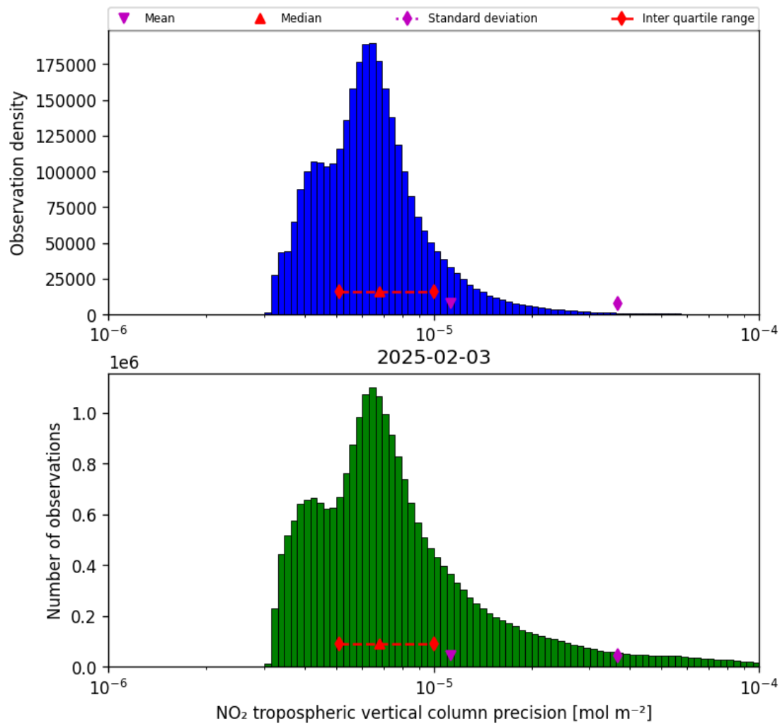
Figure 28: Histogram of “NO 2 tropospheric vertical column precision” for 2025-02-03 to 2025-02-04
