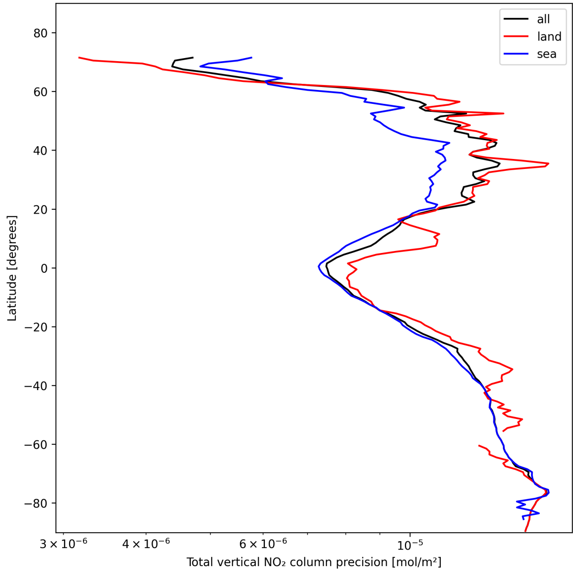
Figure 20: Zonal average of “Total vertical NO 2 column precision” for 2025-02-03 to 2025-02-04.
