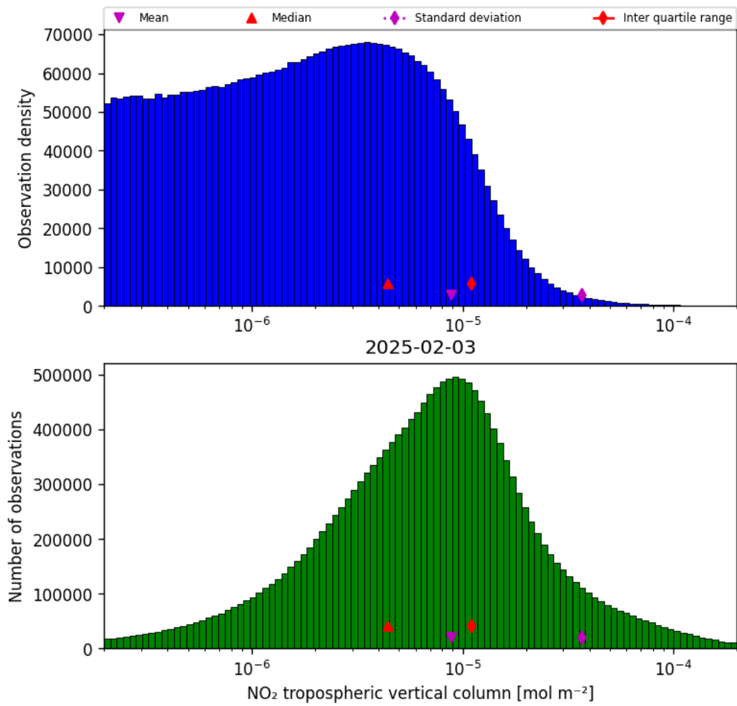
Figure 27: Histogram of “NO 2 tropospheric vertical column” for 2025-02-03 to 2025-02-04
