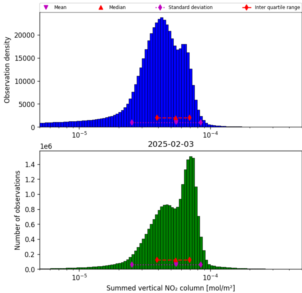
Figure 38: Histogram of “Summed vertical NO 2 column” for 2025-02-03 to 2025-02-04
