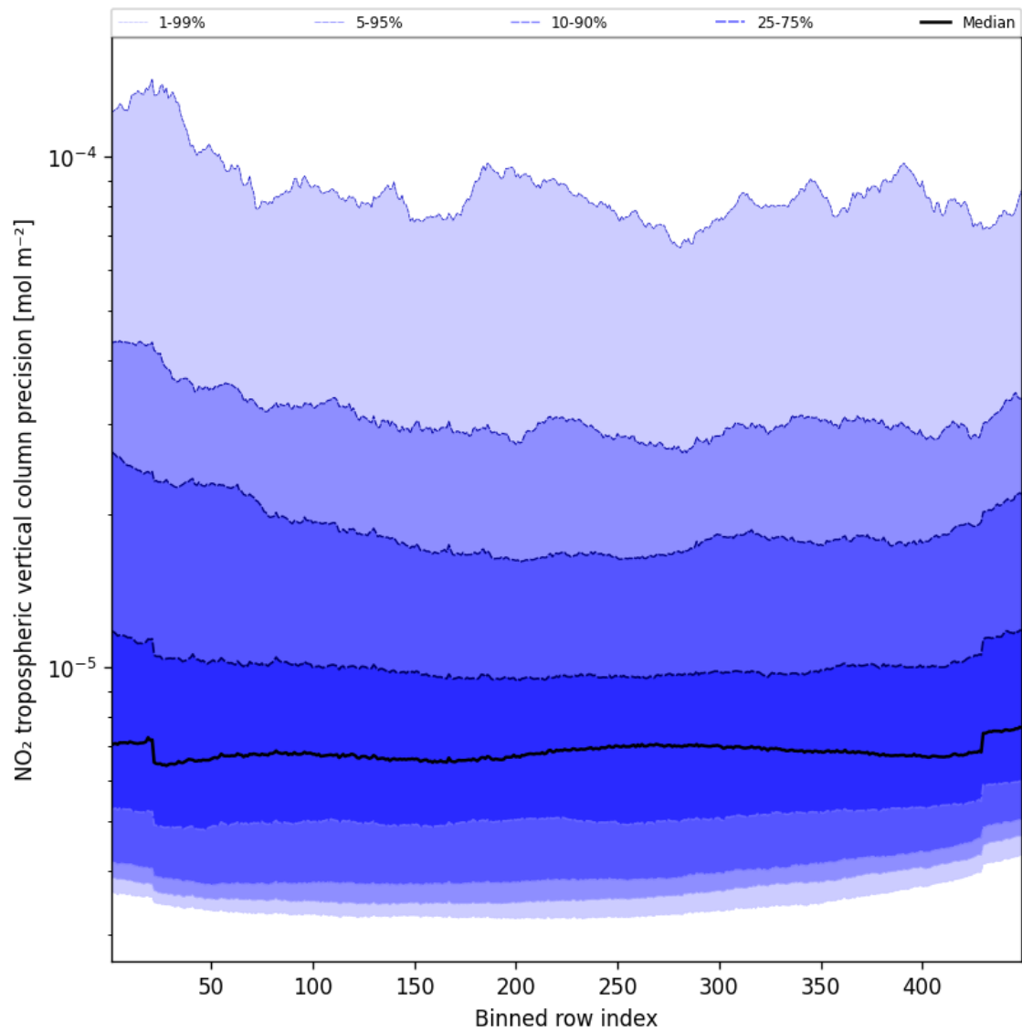
Figure 45: Along track statistics of “NO 2 tropospheric vertical column precision” for 2025-02-03 to 2025-02-04
