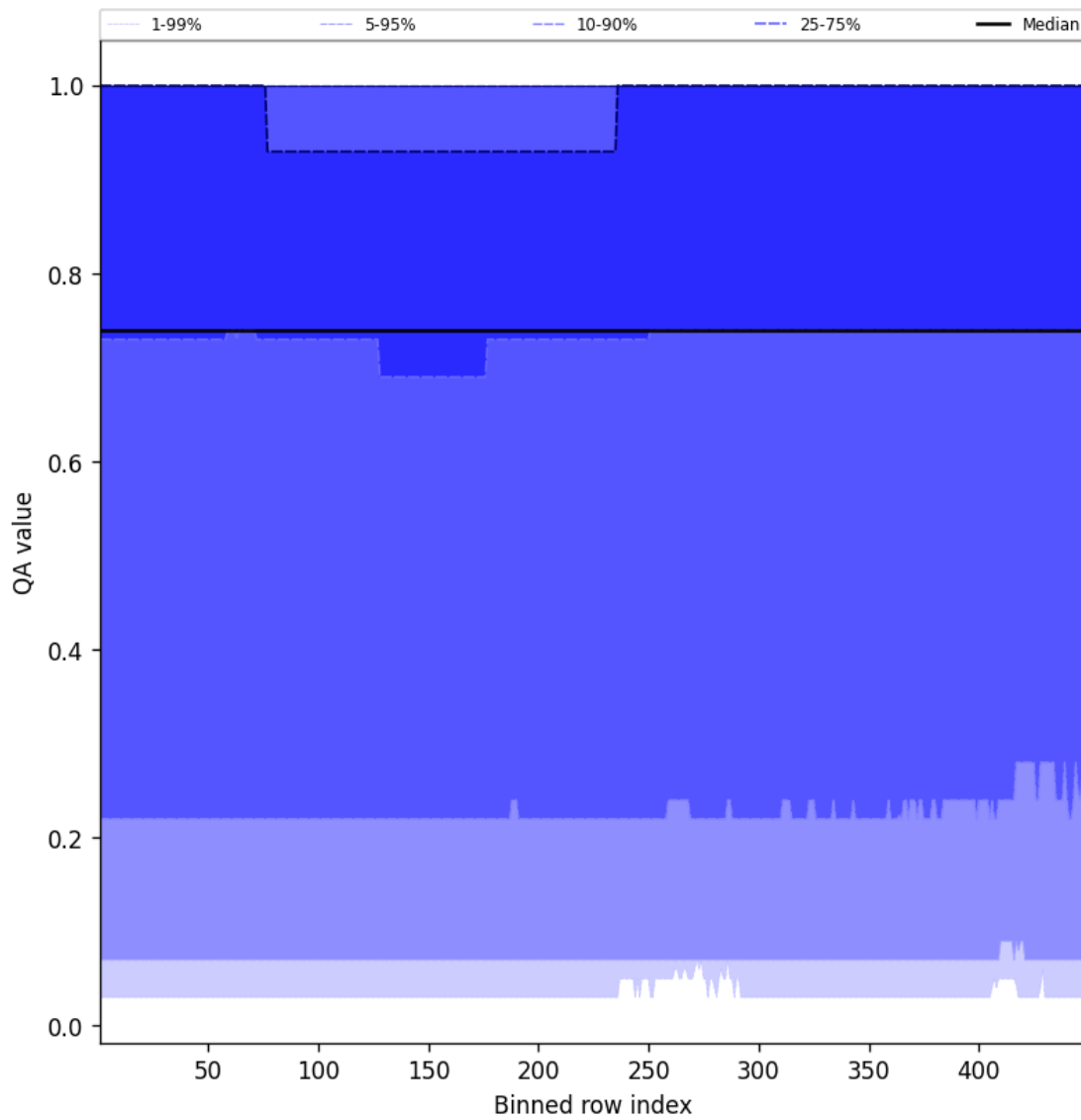
Figure 43: Along track statistics of “QA value” for 2025-02-03 to 2025-02-04
