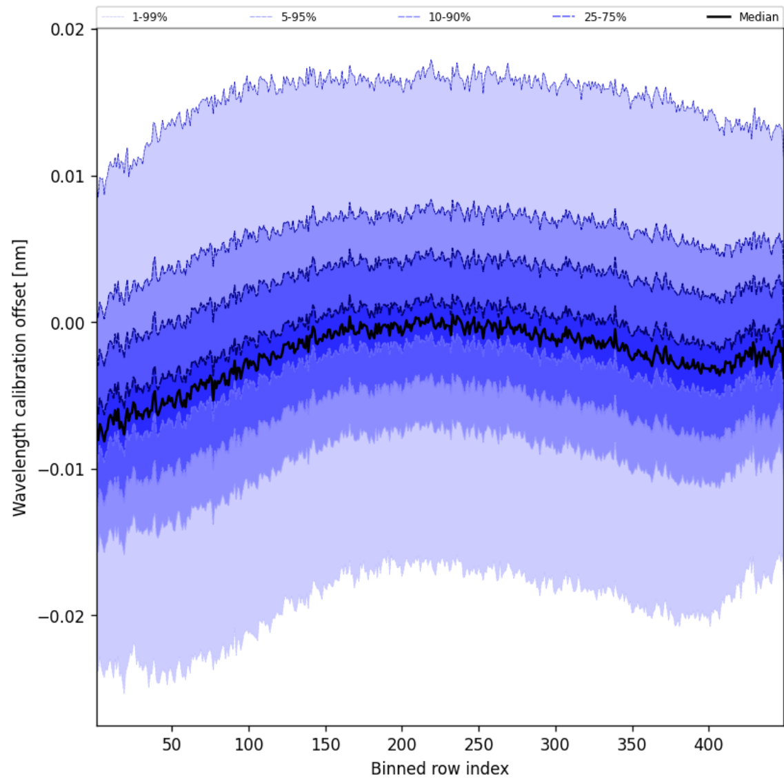
Figure 50: Along track statistics of “Wavelength calibration offset” for 2025-02-03 to 2025-02-04
