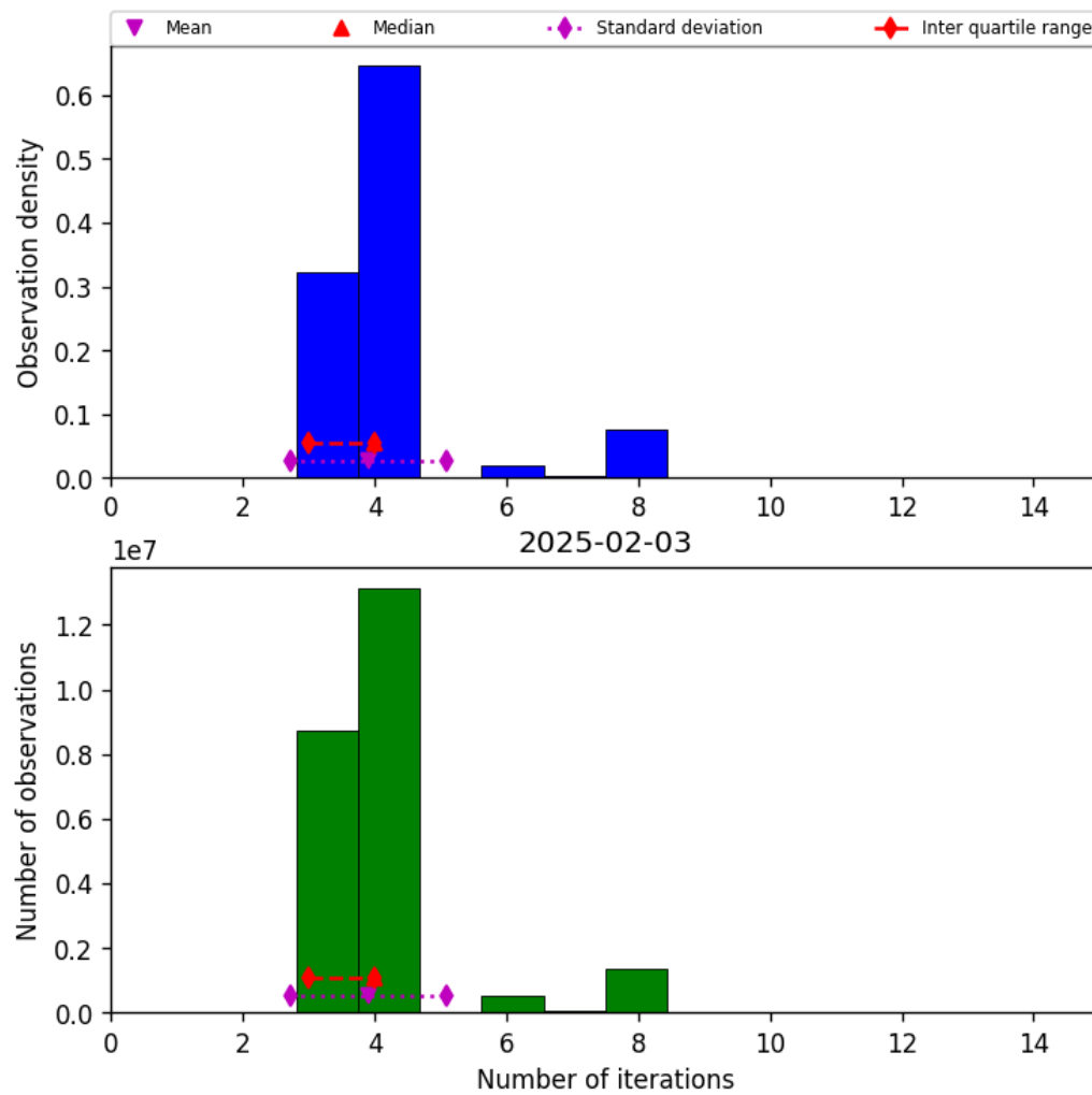
Figure 32: Histogram of “Number of iterations” for 2025-02-03 to 2025-02-04
