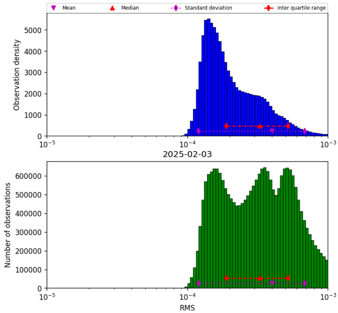
Figure 41: Histogram of “RMS” for 2025-02-03 to 2025-02-04
