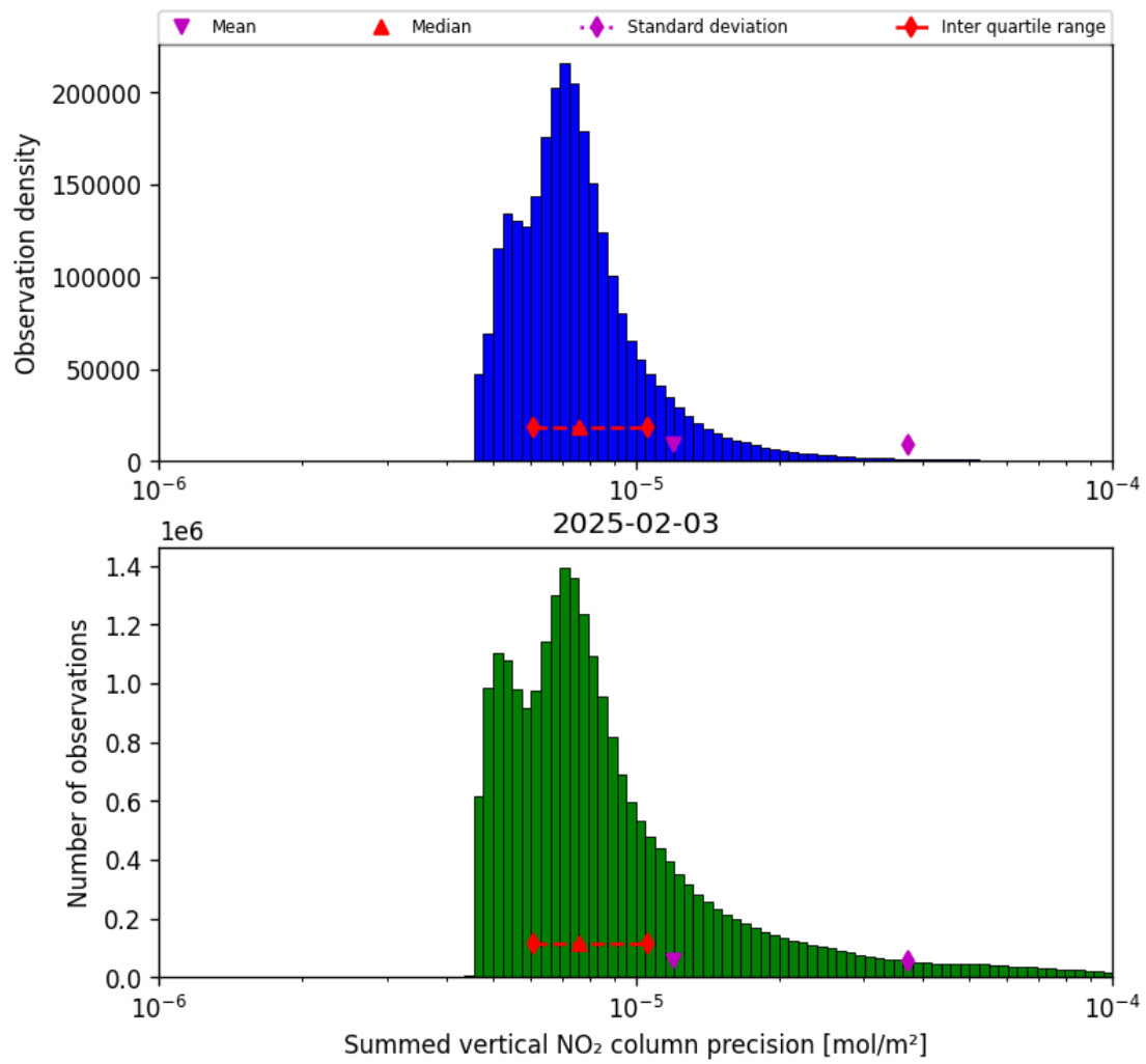
Figure 39: Histogram of "Summed vertical NO 2 column precision" for 2025-02-03 to 2025-02-04
