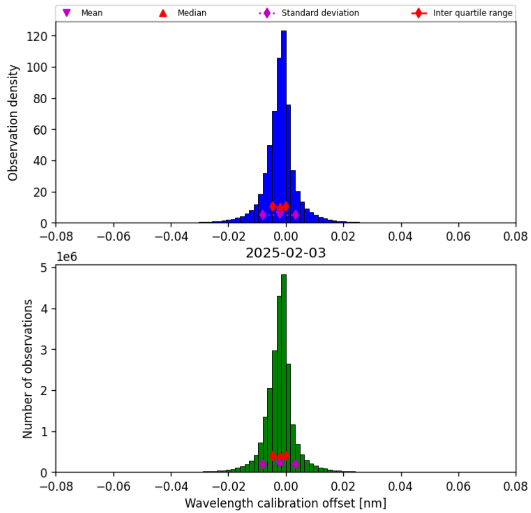
Figure 33: Histogram of “Wavelength calibration offset” for 2025-02-03 to 2025-02-04
