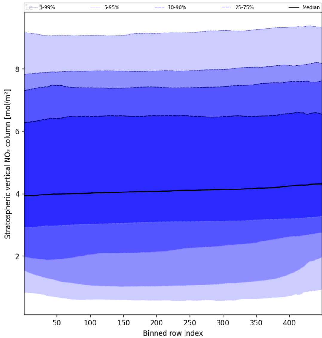
Figure 51: Along track statistics of “Stratospheric vertical NO 2 column” for 2025-02-03 to 2025-02-04
