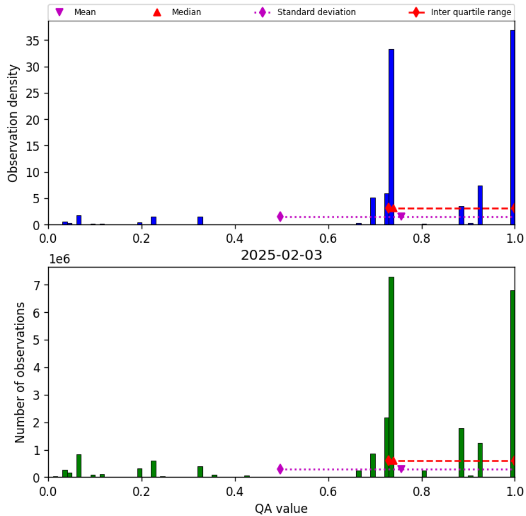
Figure 26: Histogram of “QA value” for 2025-02-03 to 2025-02-04
