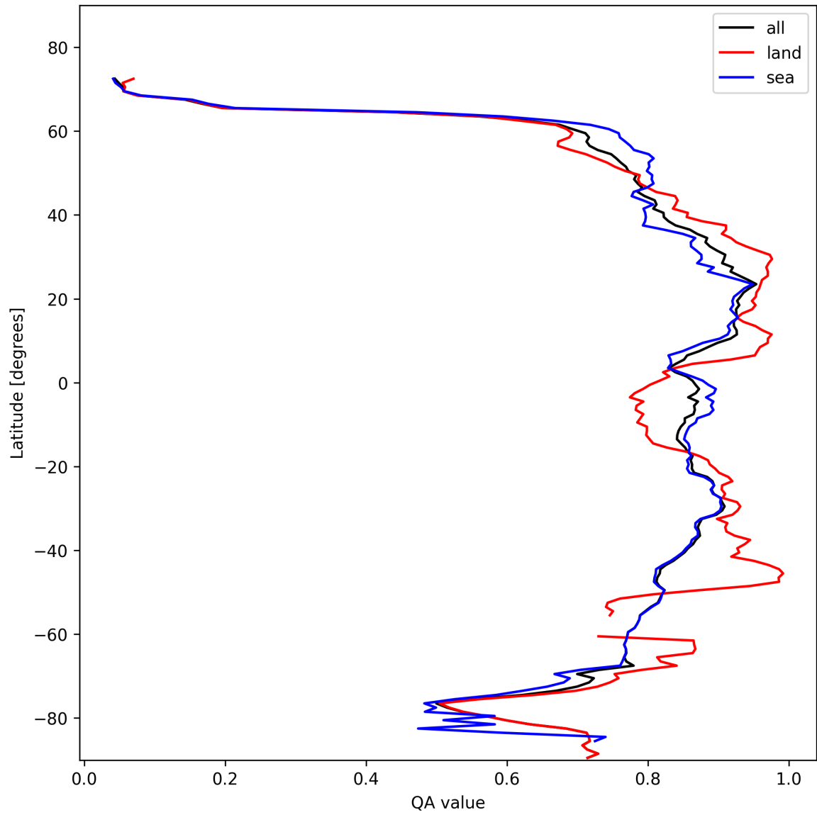
Figure 9: Zonal average of “QA value” for 2025-02-04 to 2025-02-05.
