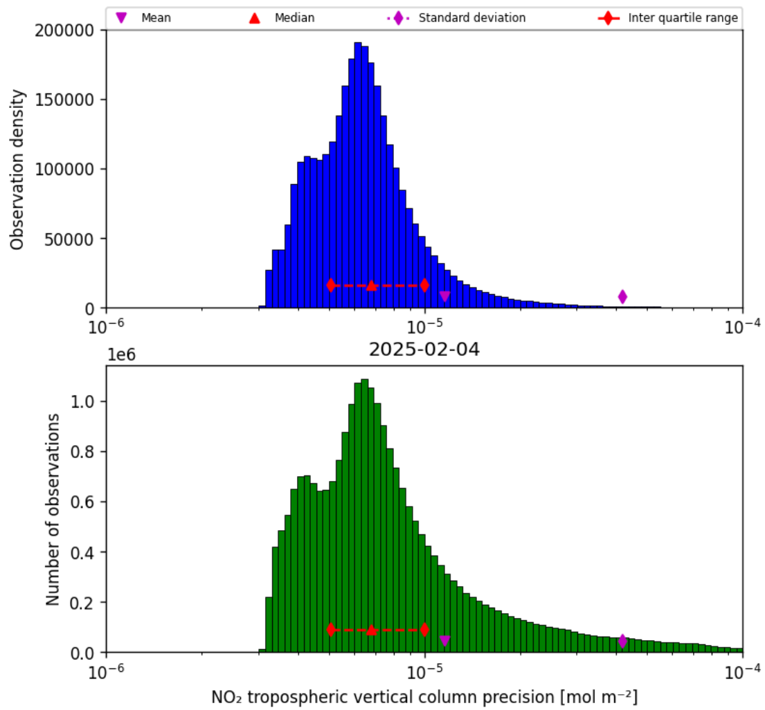
Figure 28: Histogram of “NO 2 tropospheric vertical column precision” for 2025-02-04 to 2025-02-05
