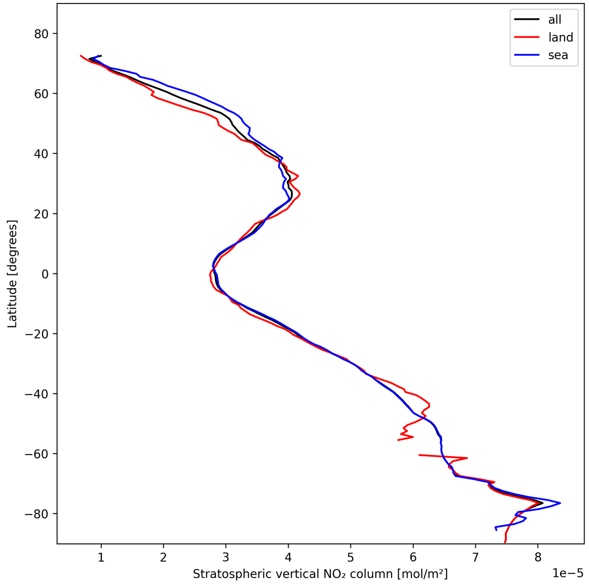
Figure 17: Zonal average of “Stratospheric vertical NO 2 column” for 2025-02-04 to 2025-02-05.
