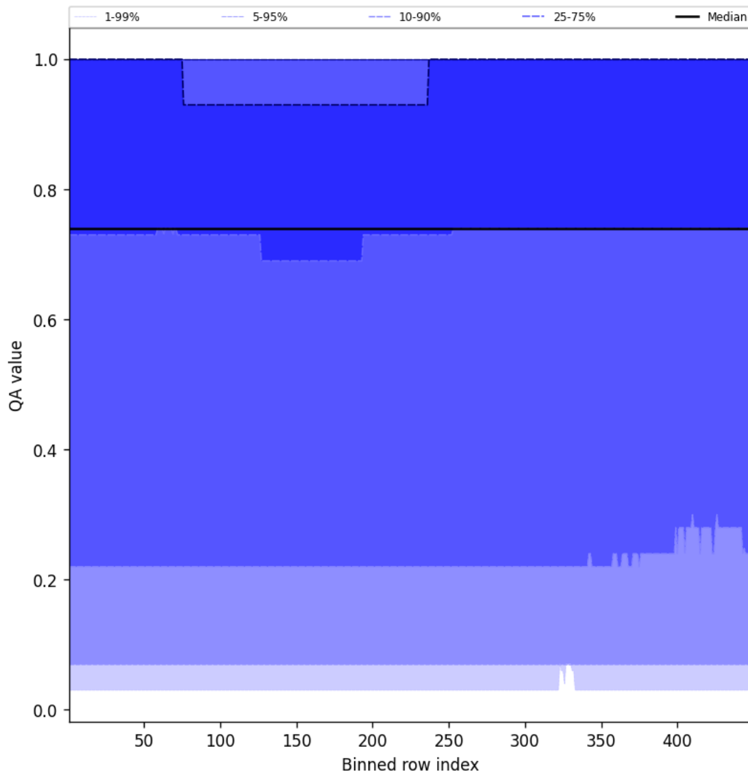
Figure 43: Along track statistics of “QA value” for 2025-02-04 to 2025-02-05
