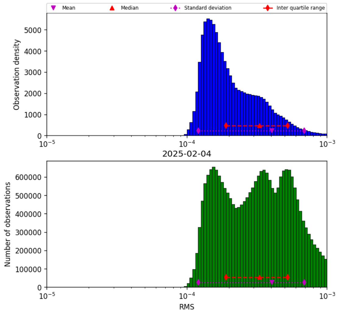
Figure 41: Histogram of “RMS” for 2025-02-04 to 2025-02-05
