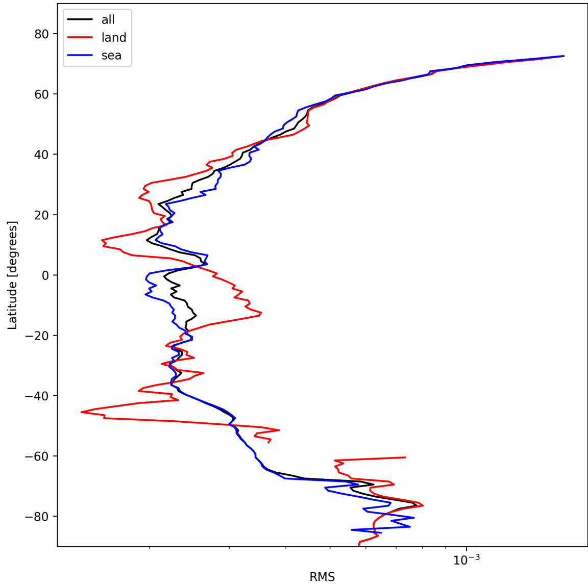
Figure 24: Zonal average of “RMS” for 2025-02-04 to 2025-02-05.
