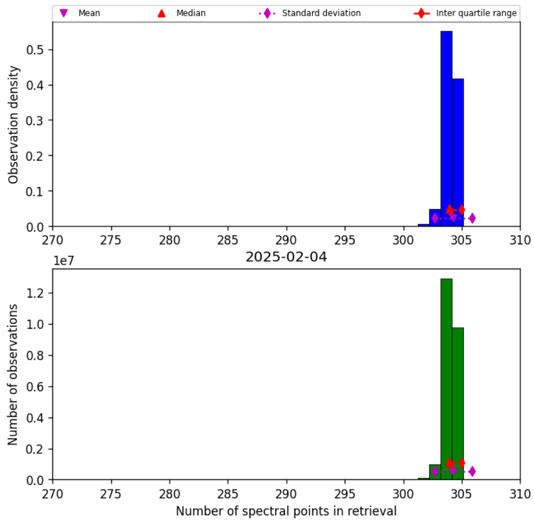
Figure 31: Histogram of “Number of spectral points in retrieval” for 2025-02-04 to 2025-02-05
