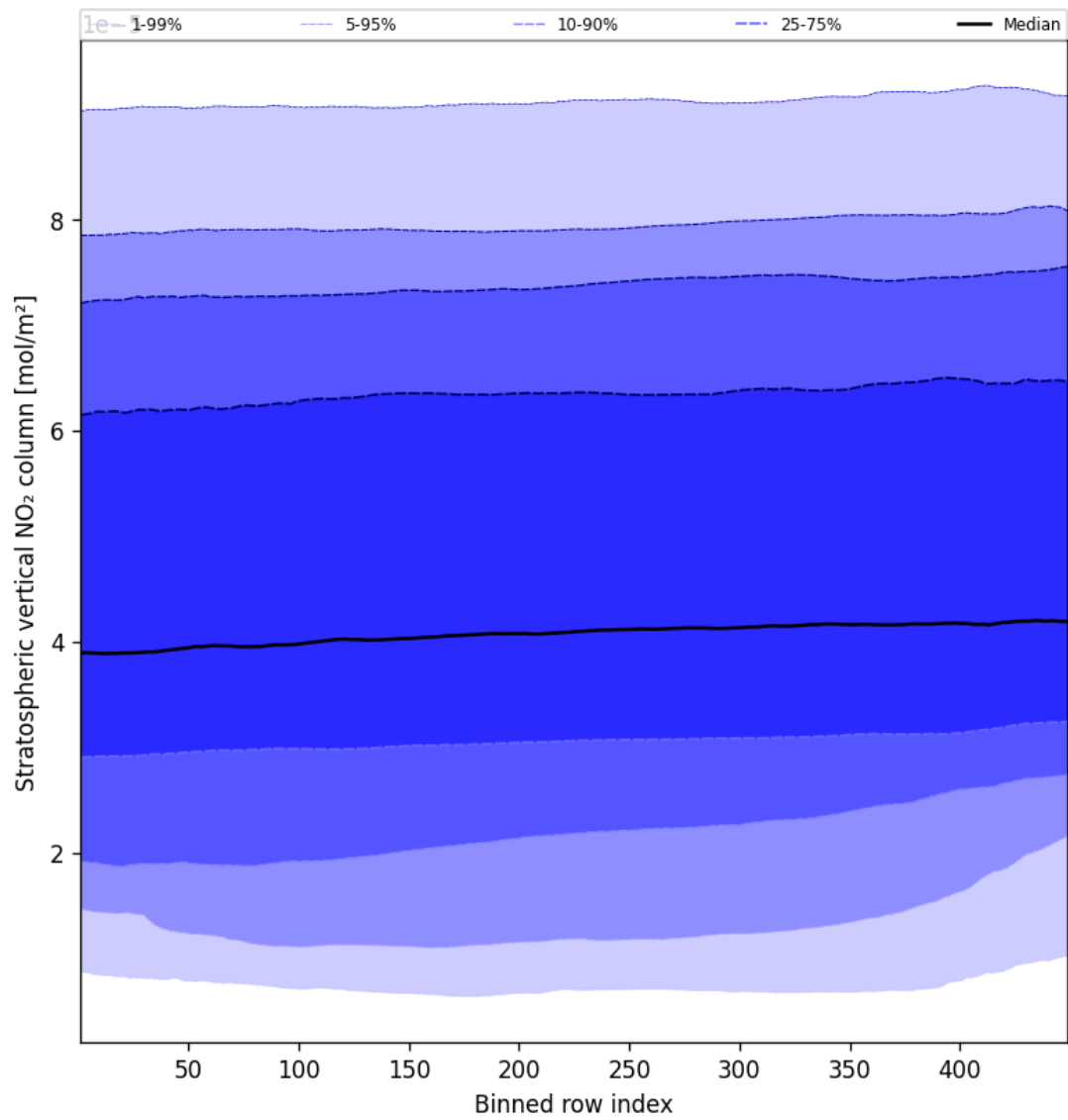
Figure 51: Along track statistics of “Stratospheric vertical NO 2 column” for 2025-02-04 to 2025-02-05
