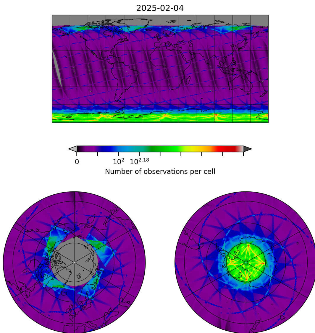
Figure 8: Map of the number of observations for 2025-02-04 to 2025-02-05
