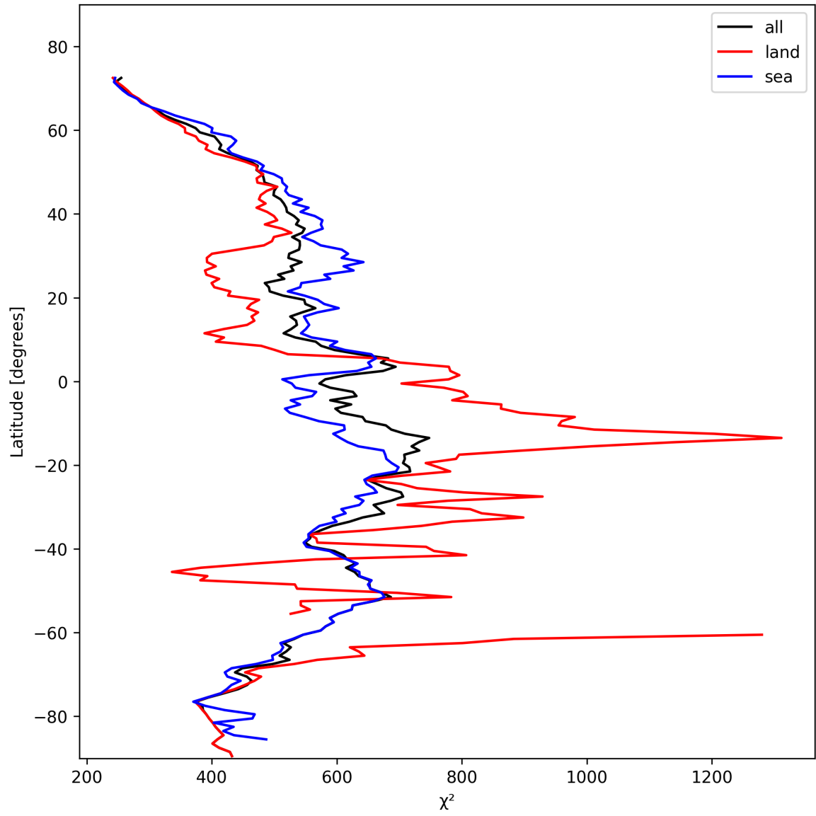
Figure 23: Zonal average of “ \chi^2 ” for 2025-02-04 to 2025-02-05.
