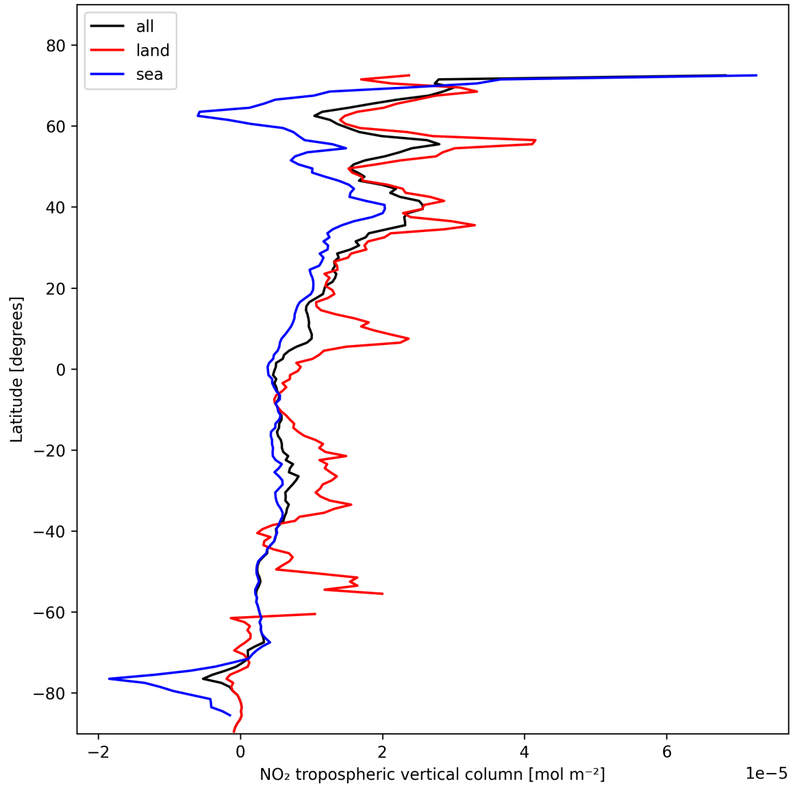
Figure 10: Zonal average of “NO 2 tropospheric vertical column” for 2025-02-04 to 2025-02-05.
