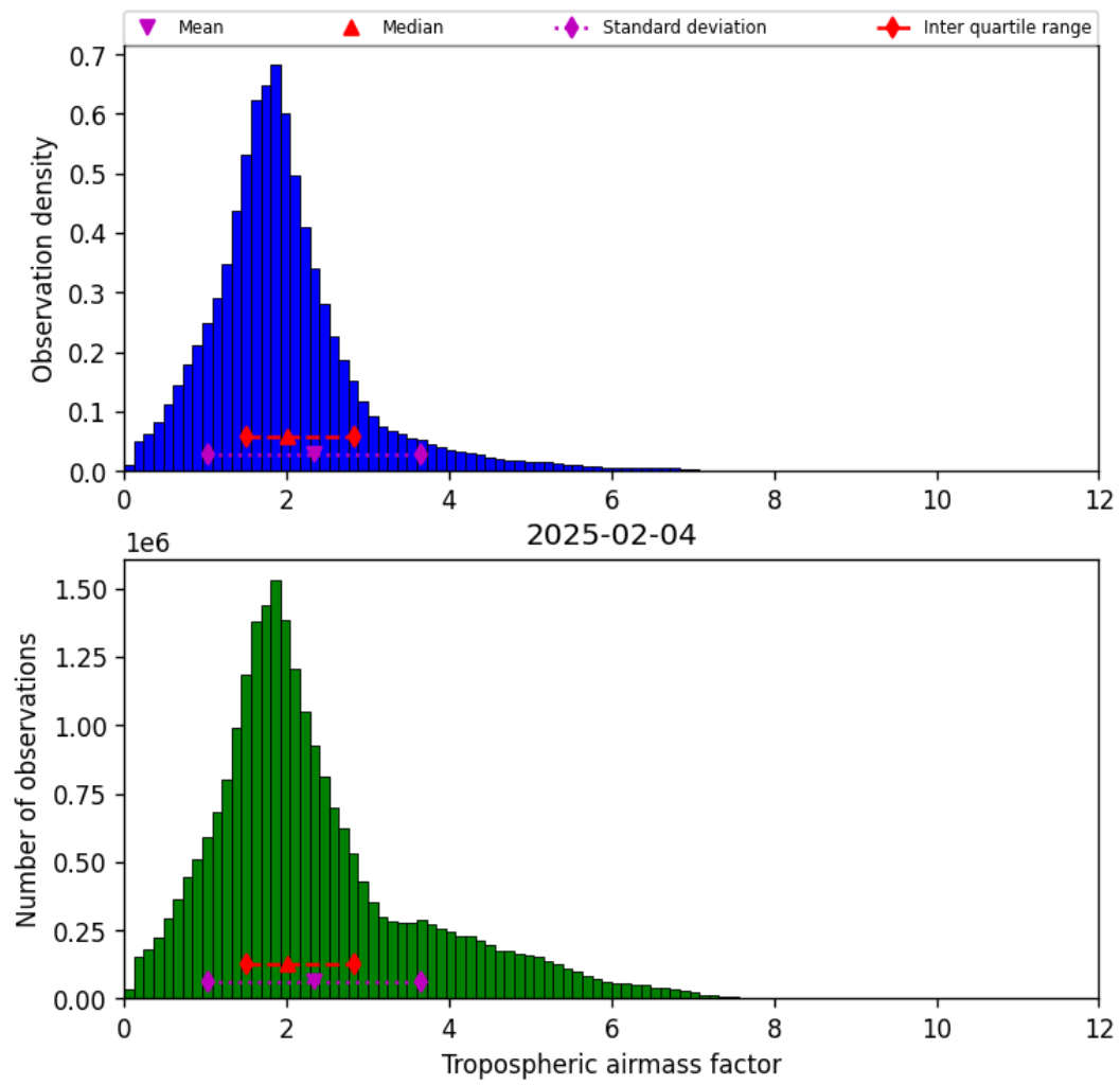
Figure 29: Histogram of “Tropospheric airmass factor” for 2025-02-04 to 2025-02-05
