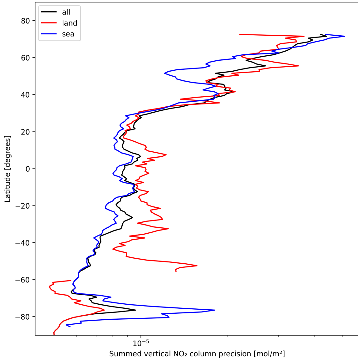
Figure 22: Zonal average of “Summed vertical NO 2 column precision” for 2025-02-04 to 2025-02-05.
