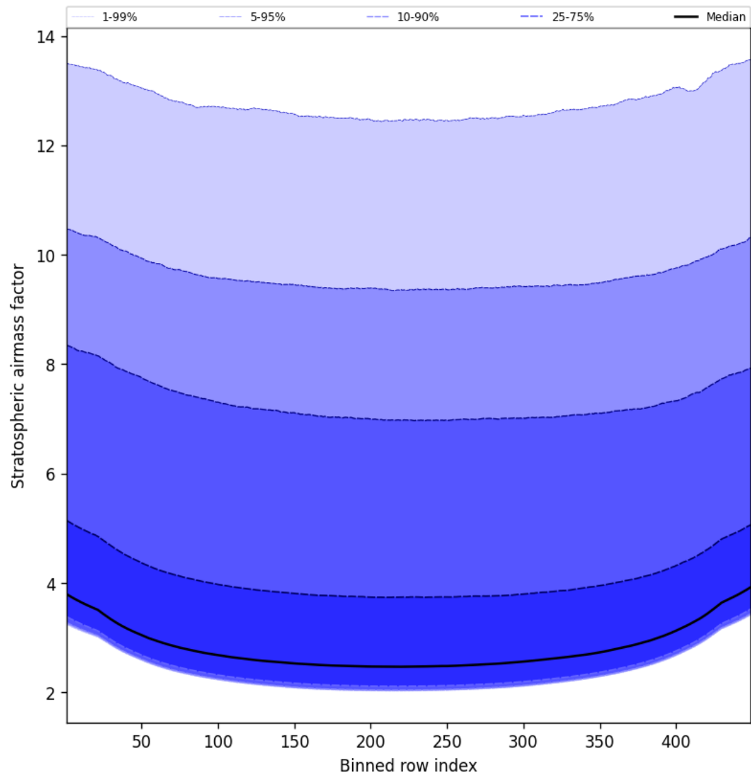
Figure 59: Along track statistics of “Stratospheric airmass factor” for 2025-02-04 to 2025-02-05
