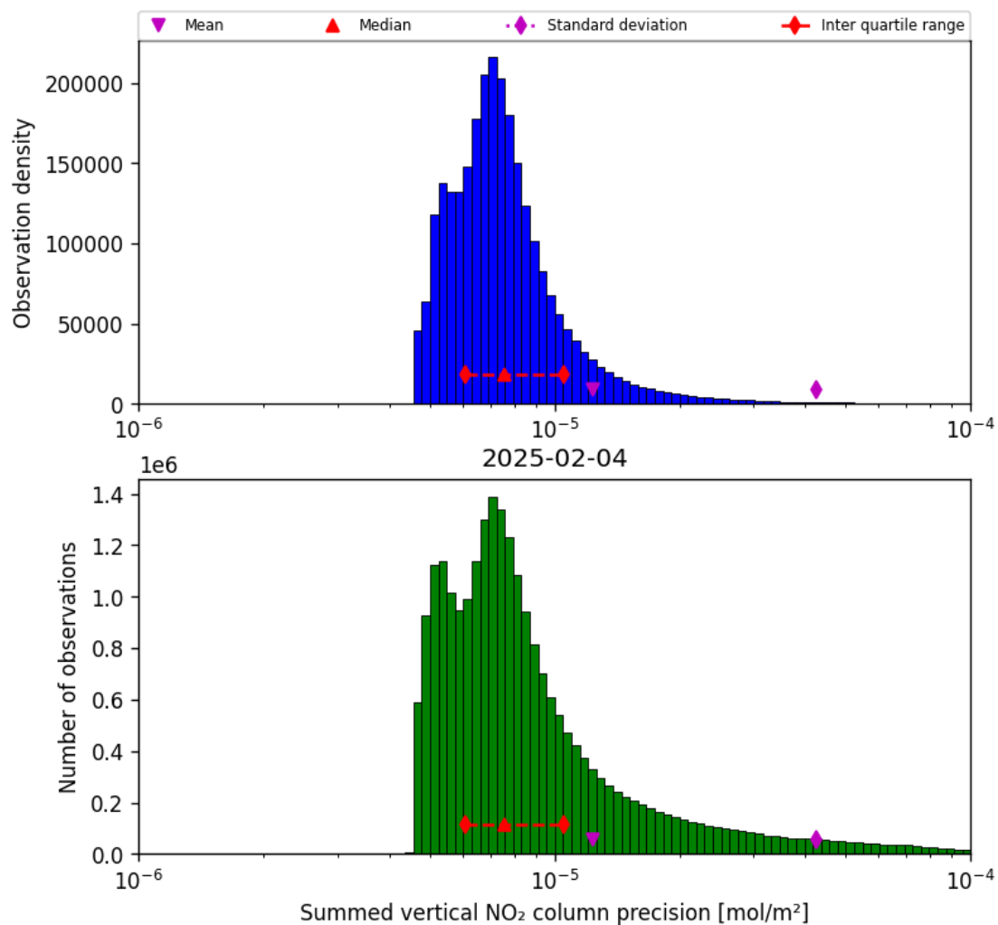
Figure 39: Histogram of “Summed vertical NO 2 column precision” for 2025-02-04 to 2025-02-05
