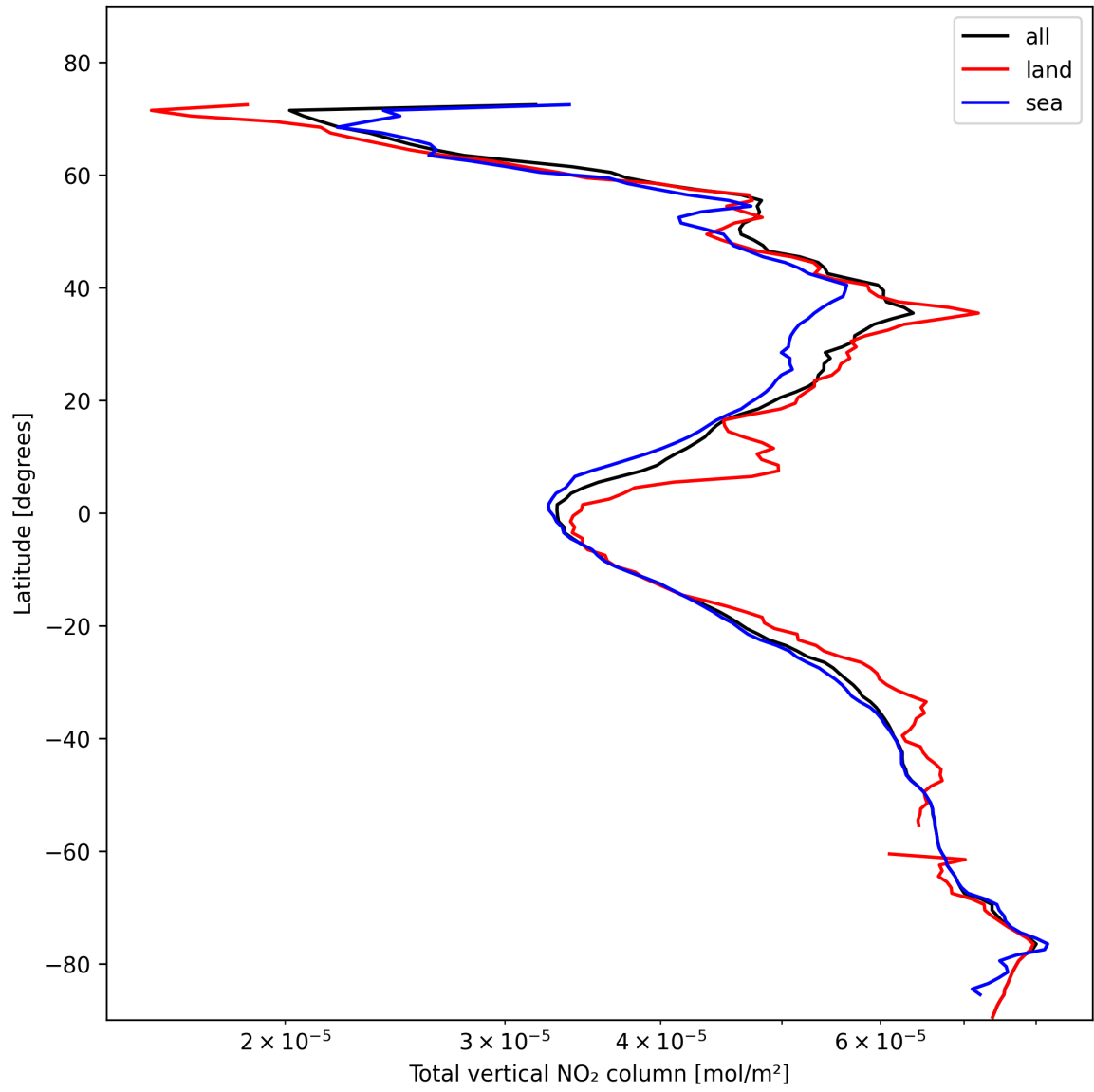
Figure 19: Zonal average of “Total vertical NO 2 column” for 2025-02-04 to 2025-02-05.
