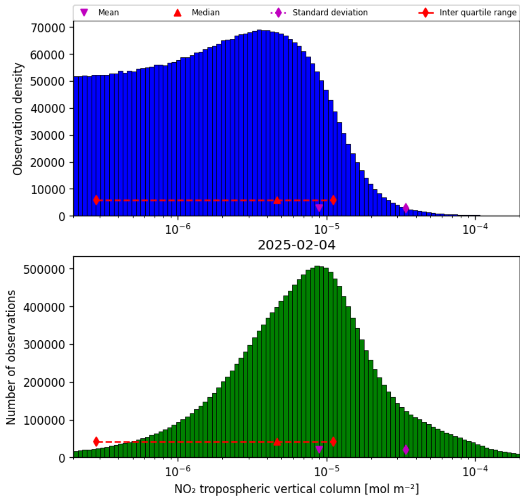
Figure 27: Histogram of “NO 2 tropospheric vertical column” for 2025-02-04 to 2025-02-05
