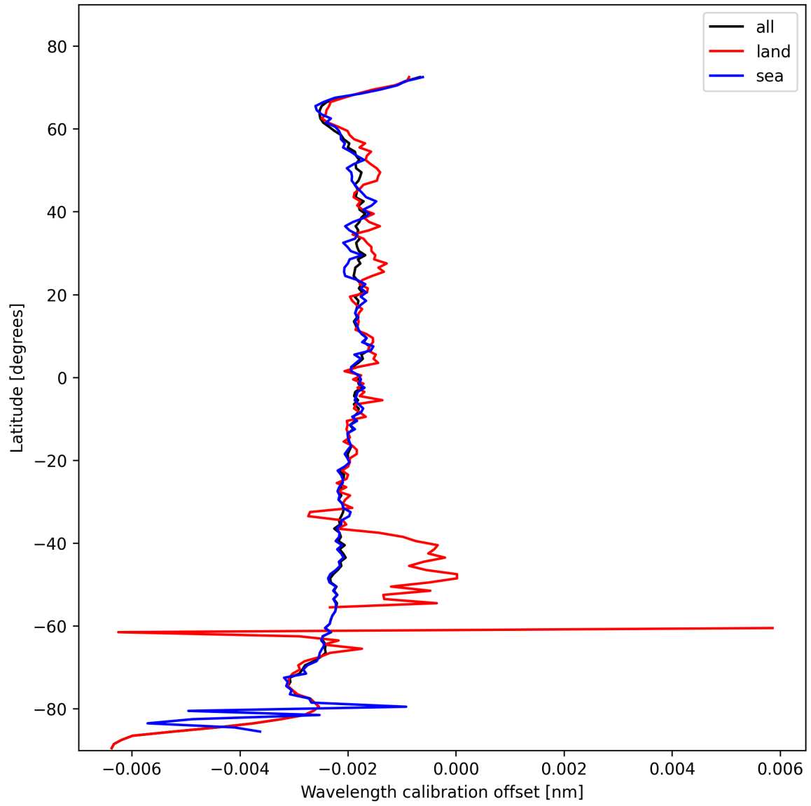
Figure 16: Zonal average of “Wavelength calibration offset” for 2025-02-04 to 2025-02-05.
