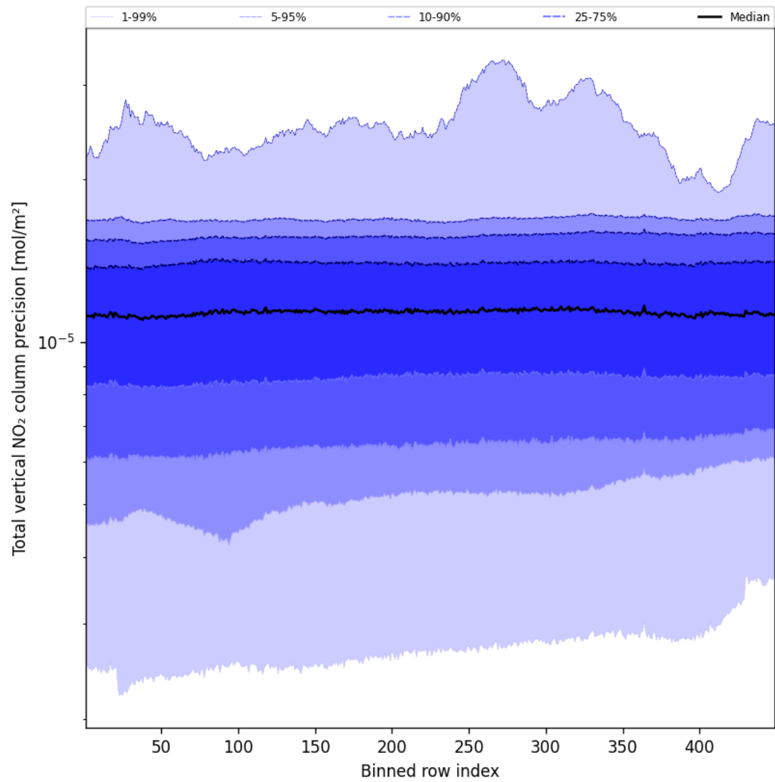
Figure 54: Along track statistics of “Total vertical NO 2 column precision” for 2025-02-04 to 2025-02-05
