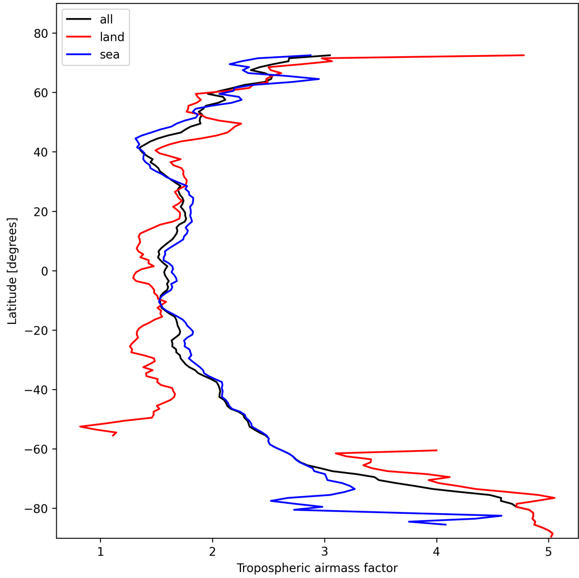
Figure 12: Zonal average of “Tropospheric airmass factor” for 2025-02-04 to 2025-02-05.
