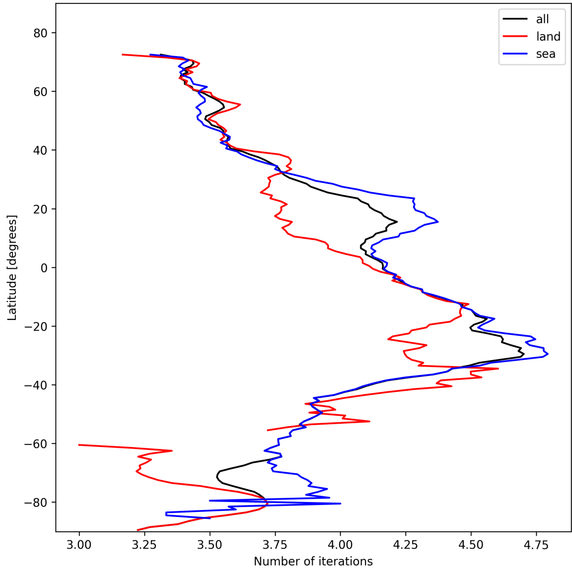
Figure 15: Zonal average of “Number of iterations” for 2025-02-04 to 2025-02-05.
