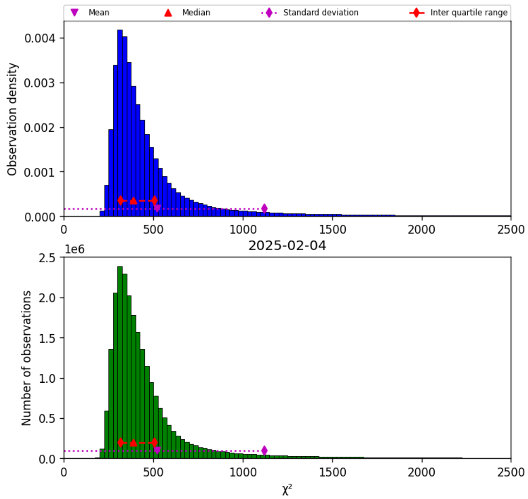
Figure 40: Histogram of “ \chi^2 ” for 2025-02-04 to 2025-02-05
