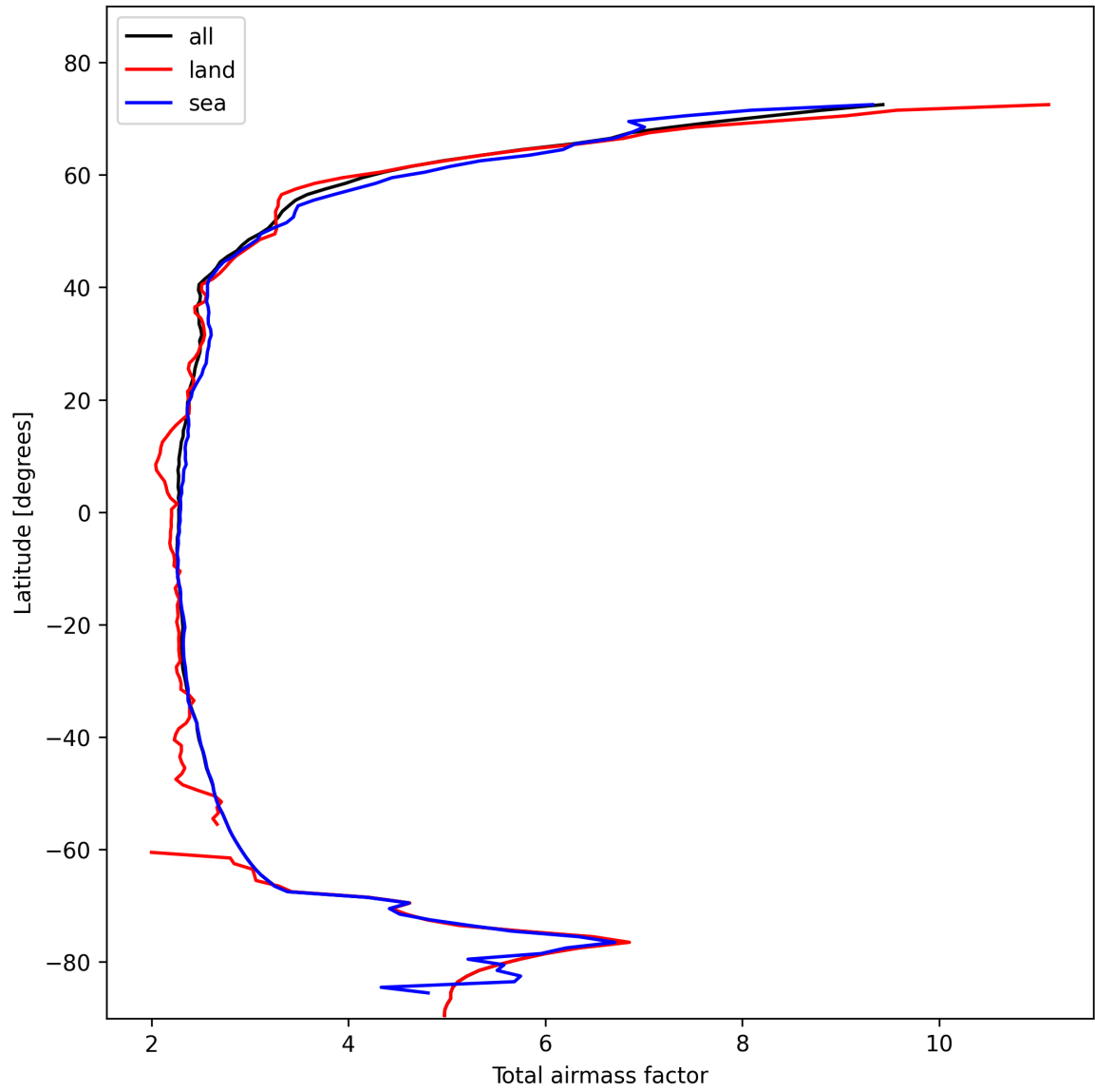
Figure 13: Zonal average of “Total airmass factor” for 2025-02-04 to 2025-02-05.
