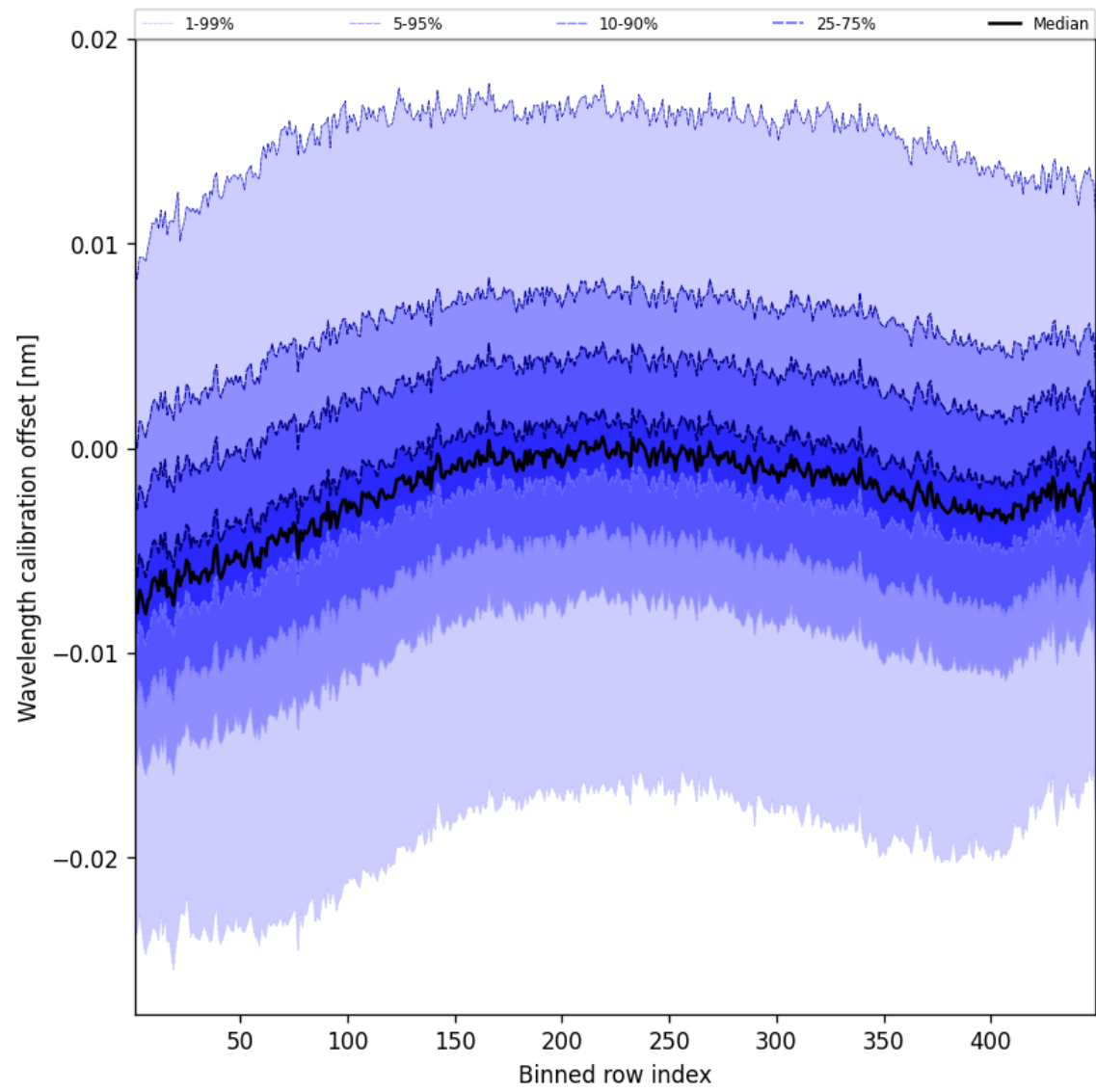
Figure 50: Along track statistics of “Wavelength calibration offset” for 2025-02-04 to 2025-02-05
