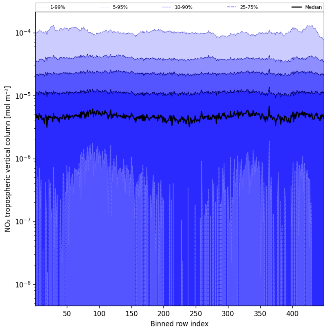
Figure 44: Along track statistics of “NO 2 tropospheric vertical column” for 2025-02-04 to 2025-02-05
