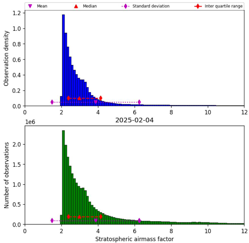
Figure 42: Histogram of “Stratospheric airmass factor” for 2025-02-04 to 2025-02-05
