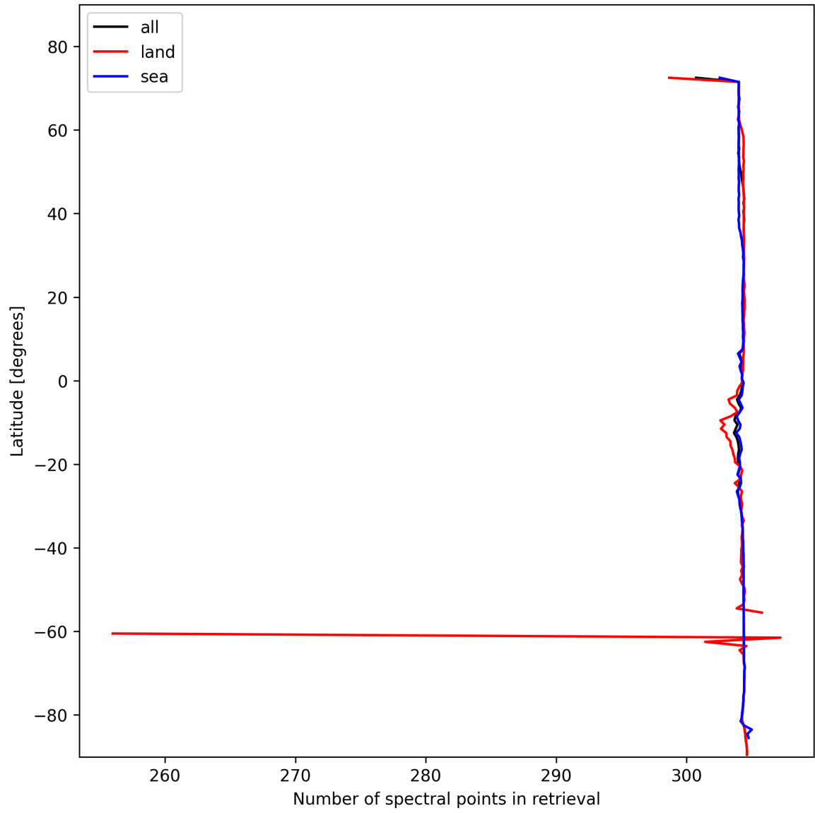
Figure 14: Zonal average of “Number of spectral points in retrieval” for 2025-02-04 to 2025-02-05.
