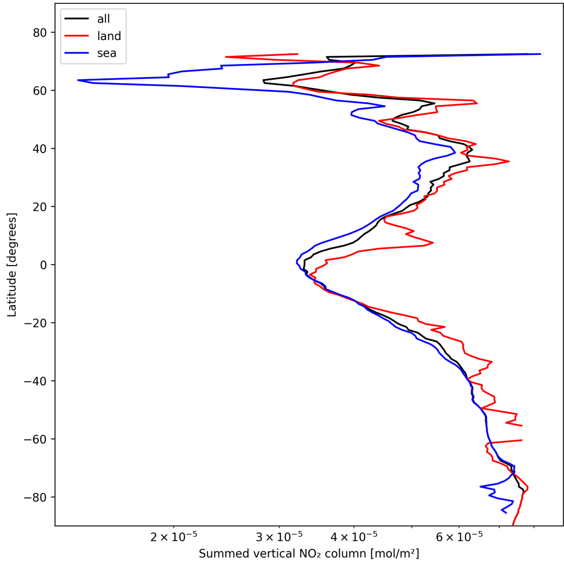
Figure 21: Zonal average of “Summed vertical NO 2 column” for 2025-02-04 to 2025-02-05.
