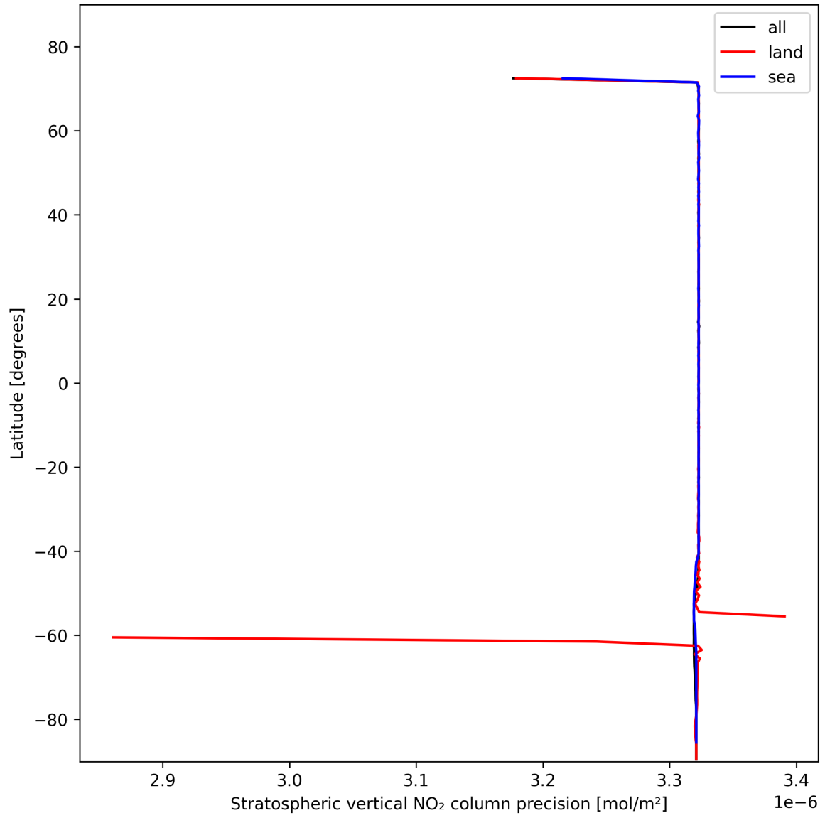
Figure 18: Zonal average of “Stratospheric vertical NO 2 column precision” for 2025-02-04 to 2025-02-05.
