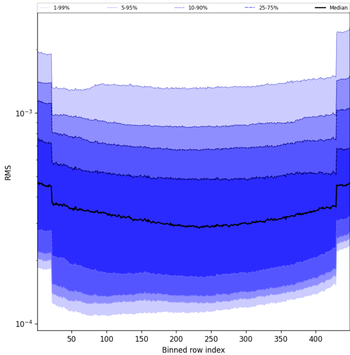
Figure 58: Along track statistics of “RMS” for 2025-02-04 to 2025-02-05
