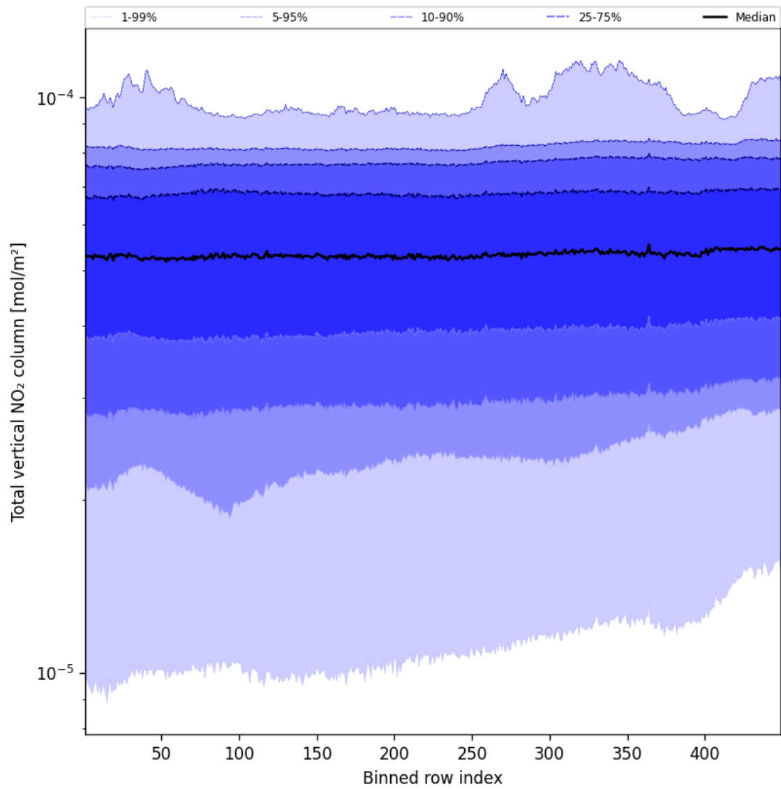
Figure 53: Along track statistics of “Total vertical NO 2 column” for 2025-02-04 to 2025-02-05
