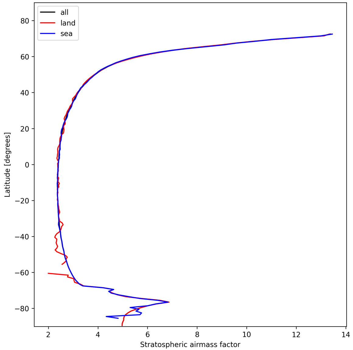
Figure 25: Zonal average of “Stratospheric air mass factor” for 2025-02-04 to 2025-02-05.
