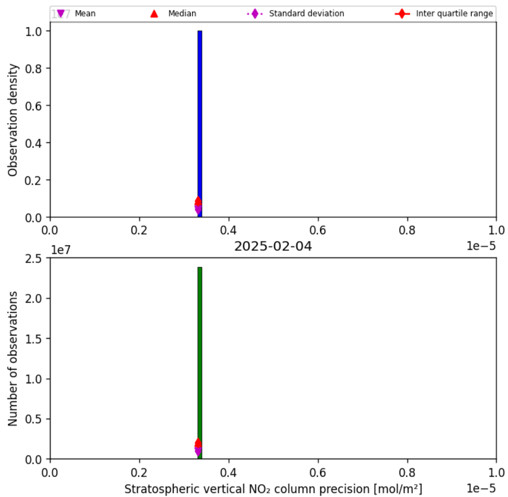
Figure 35: Histogram of “Stratospheric vertical NO 2 column precision” for 2025-02-04 to 2025-02-05
