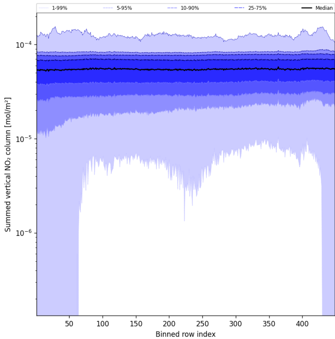
Figure 55: Along track statistics of “Summed vertical NO 2 column” for 2025-02-04 to 2025-02-05
