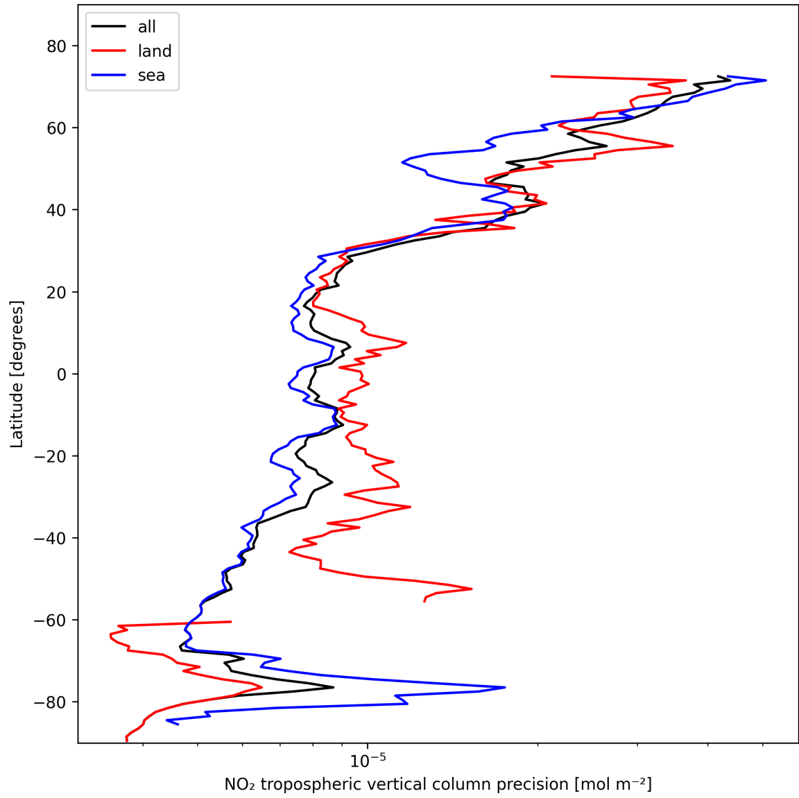
Figure 11: Zonal average of “NO 2 tropospheric vertical column precision” for 2025-02-04 to 2025-02-05.
