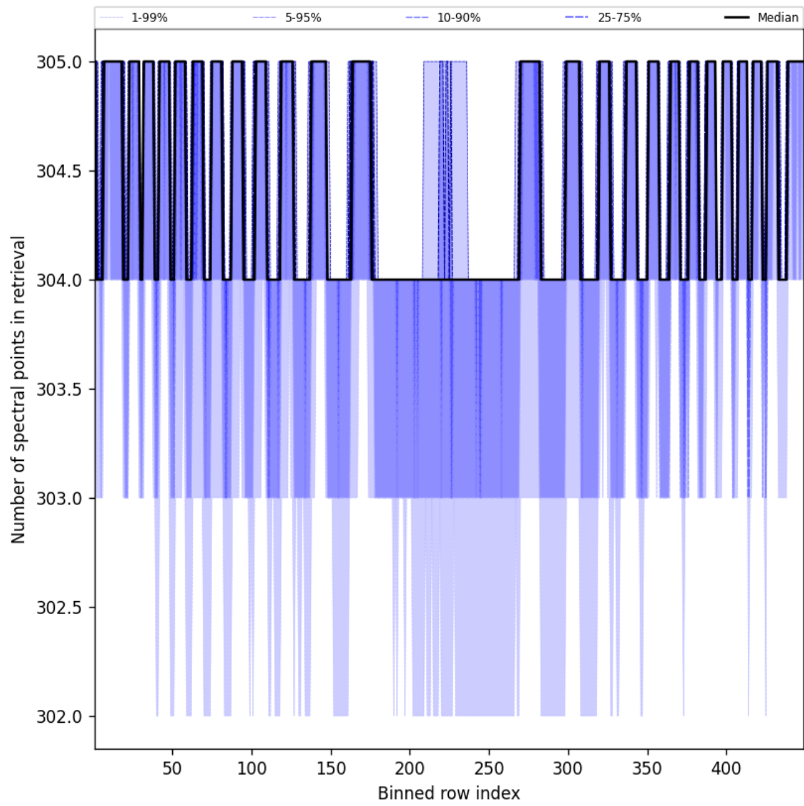
Figure 48: Along track statistics of “Number of spectral points in retrieval” for 2025-02-04 to 2025-02-05
