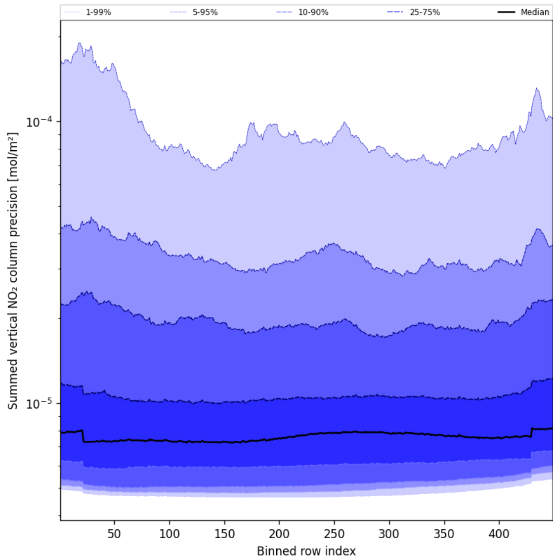
Figure 56: Along track statistics of “Summed vertical NO 2 column precision” for 2025-02-04 to 2025-02-05
