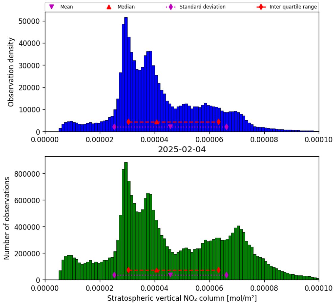
Figure 34: Histogram of “Stratospheric vertical NO 2 column” for 2025-02-04 to 2025-02-05
