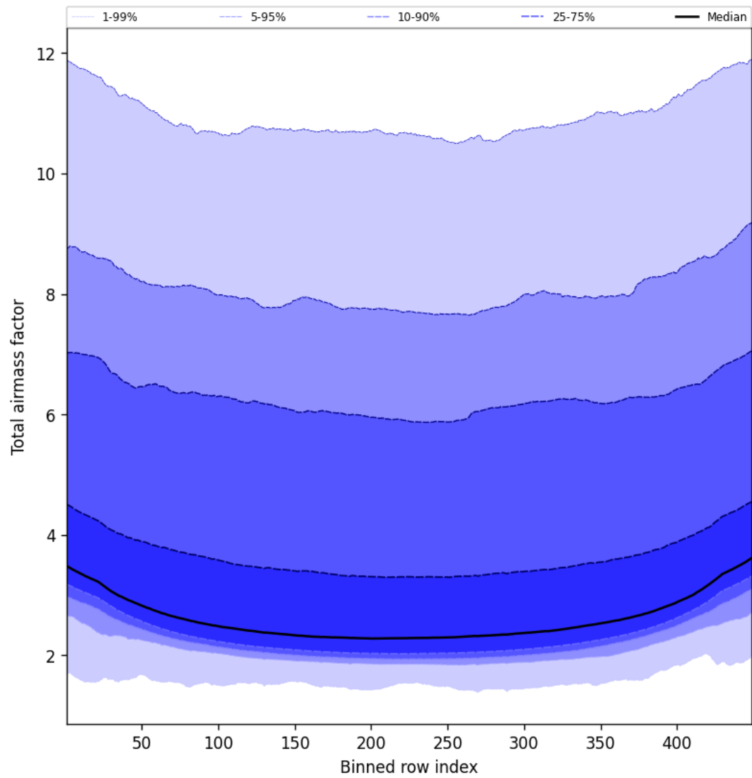
Figure 47: Along track statistics of “Total airmass factor” for 2025-02-04 to 2025-02-05
