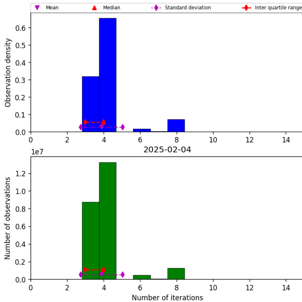
Figure 32: Histogram of “Number of iterations” for 2025-02-04 to 2025-02-05
