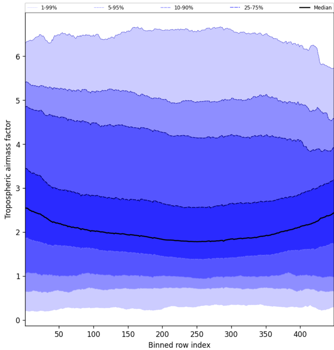
Figure 46: Along track statistics of “Tropospheric air mass factor” for 2025-02-04 to 2025-02-05
