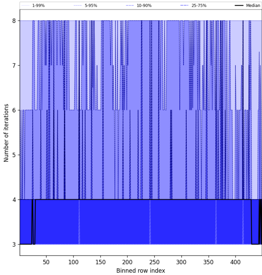
Figure 49: Along track statistics of “Number of iterations” for 2025-02-04 to 2025-02-05
