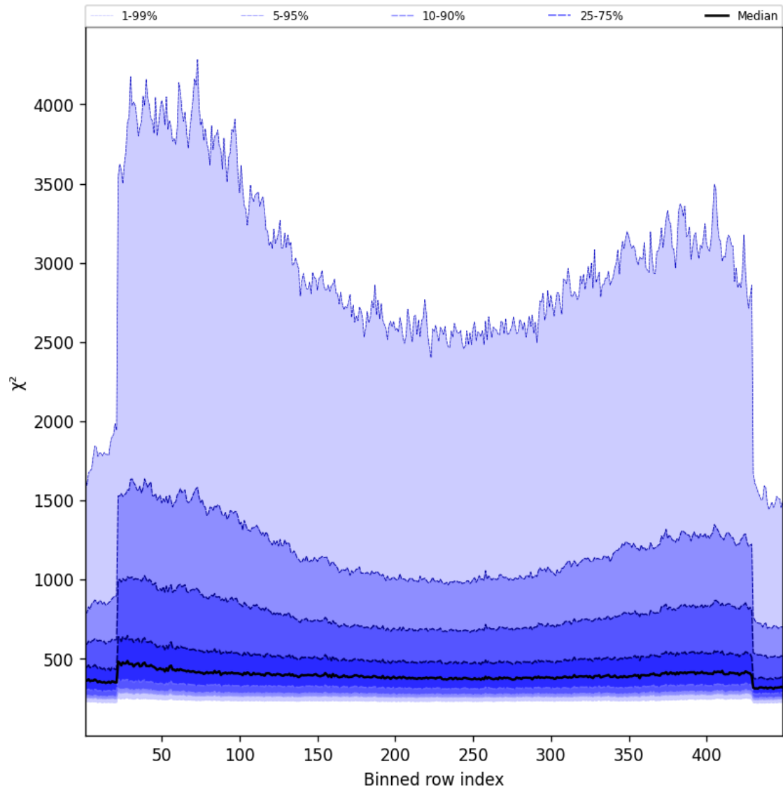
Figure 57: Along track statistics of “ \chi^2 ” for 2025-02-04 to 2025-02-05
