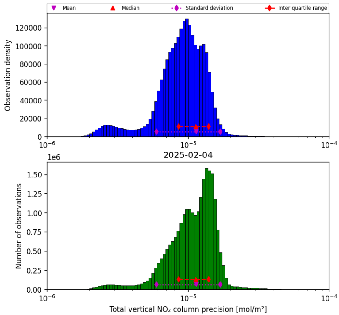
Figure 37: Histogram of “Total vertical NO 2 column precision” for 2025-02-04 to 2025-02-05
