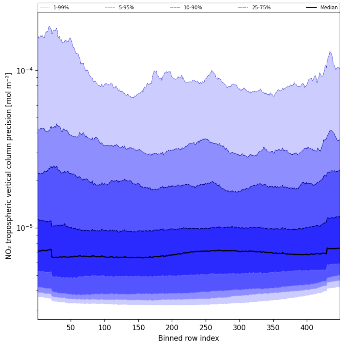
Figure 45: Along track statistics of “NO 2 tropospheric vertical column precision” for 2025-02-04 to 2025-02-05
