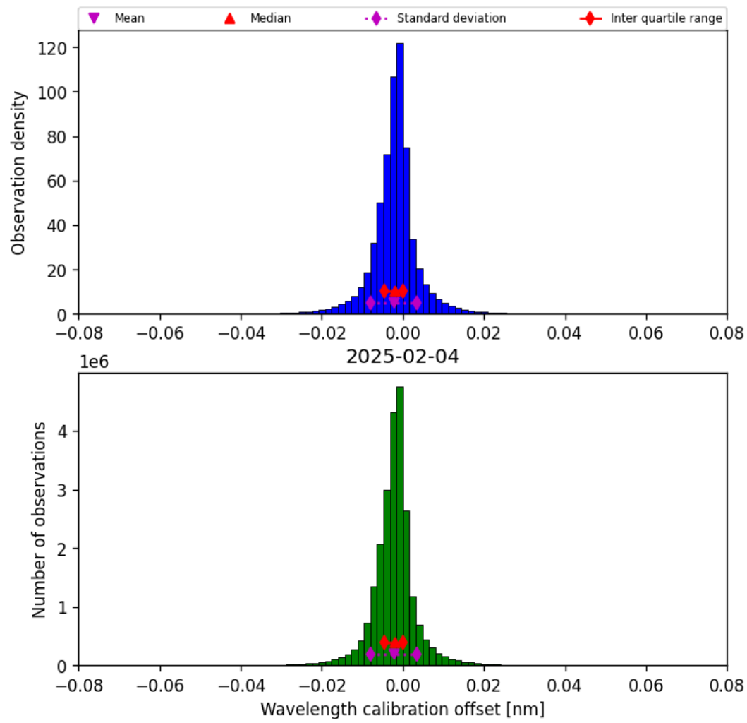
Figure 33: Histogram of “Wavelength calibration offset” for 2025-02-04 to 2025-02-05
