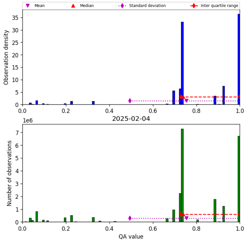
Figure 26: Histogram of “QA value” for 2025-02-04 to 2025-02-05
