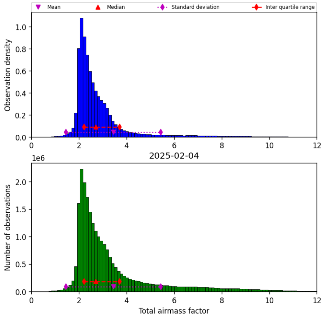
Figure 30: Histogram of “Total airmass factor” for 2025-02-04 to 2025-02-05
