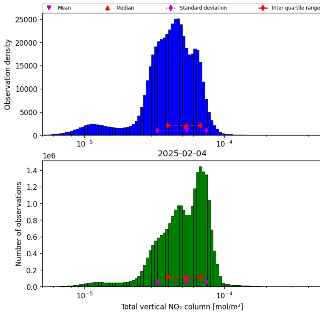
Figure 36: Histogram of “Total vertical NO 2 column” for 2025-02-04 to 2025-02-05
