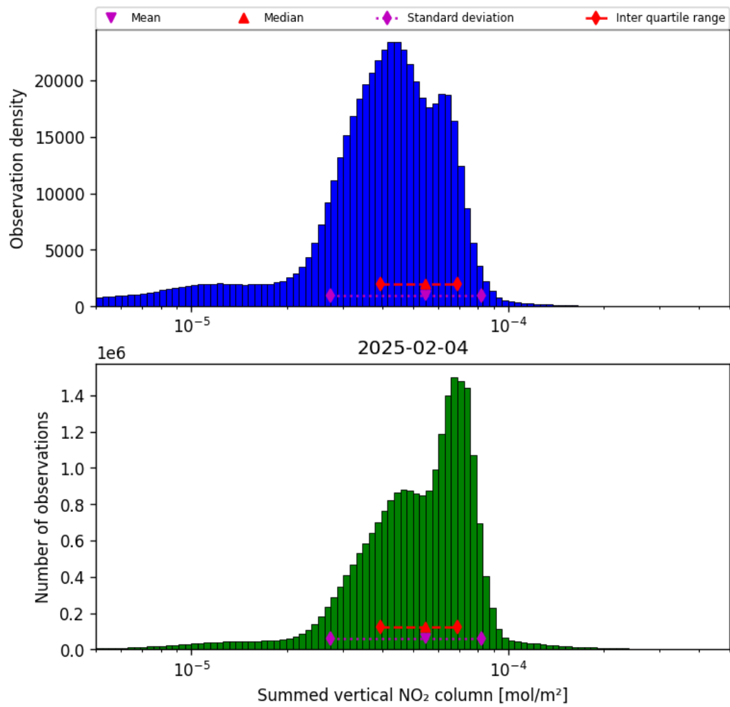
Figure 38: Histogram of “Summed vertical NO 2 column” for 2025-02-04 to 2025-02-05
