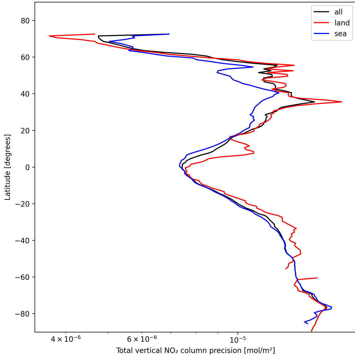
Figure 20: Zonal average of “Total vertical NO 2 column precision” for 2025-02-04 to 2025-02-05.
