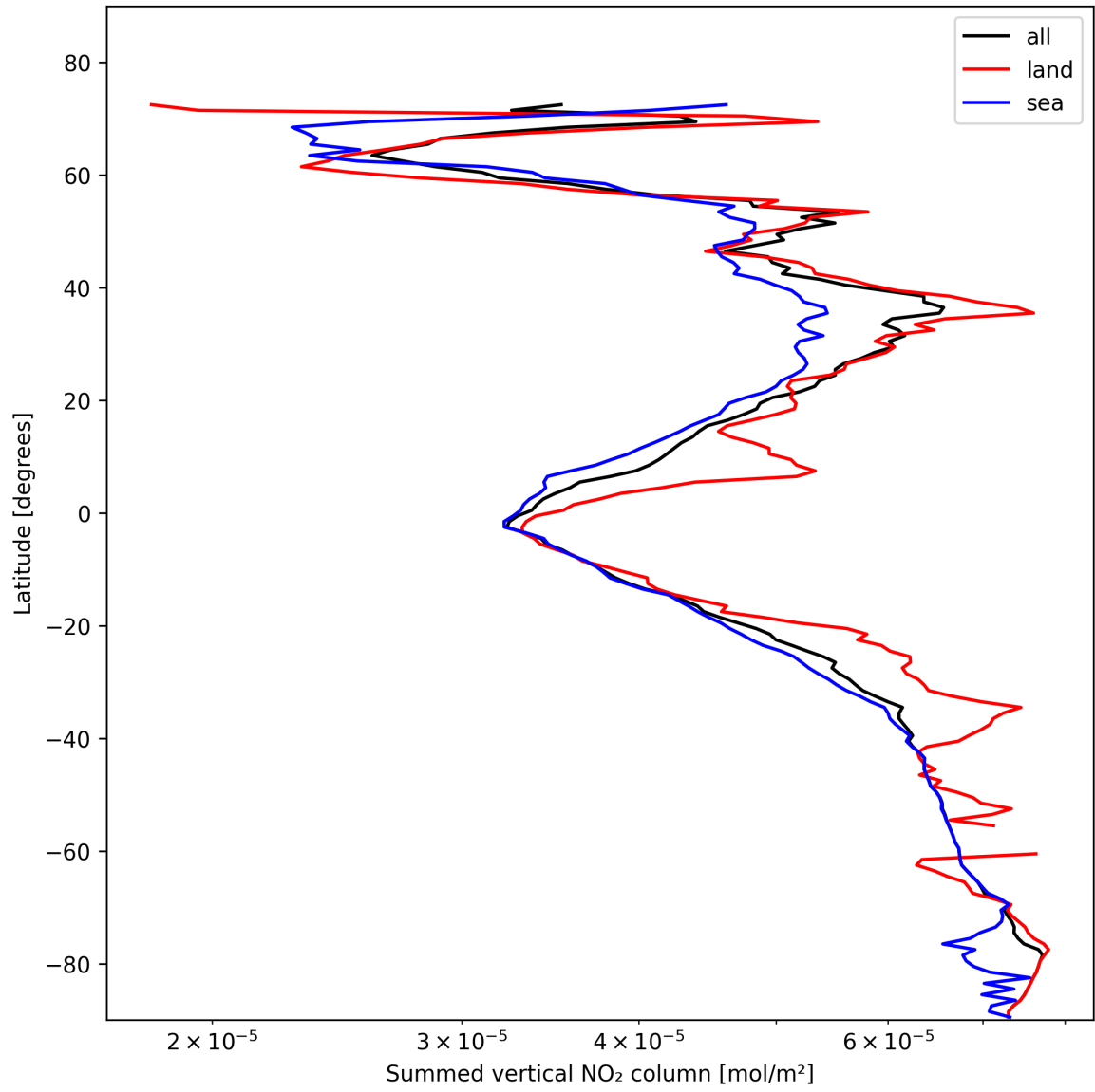
Figure 21: Zonal average of “Summed vertical NO 2 column” for 2025-02-05 to 2025-02-06.
