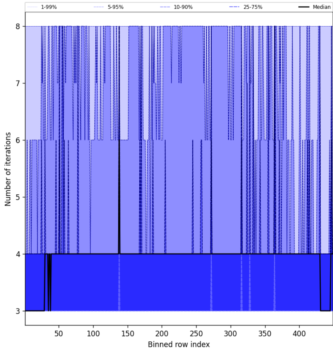
Figure 49: Along track statistics of “Number of iterations” for 2025-02-05 to 2025-02-06
