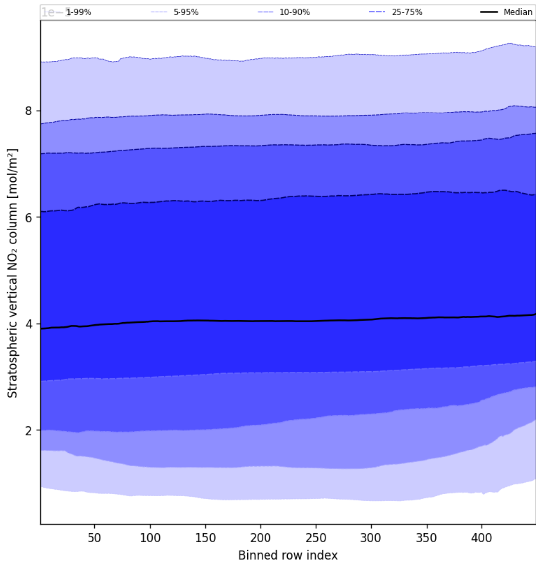
Figure 51: Along track statistics of “Stratospheric vertical NO 2 column” for 2025-02-05 to 2025-02-06
