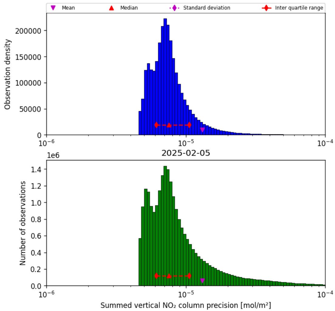
Figure 39: Histogram of "Summed vertical NO 2 column precision" for 2025-02-05 to 2025-02-06
