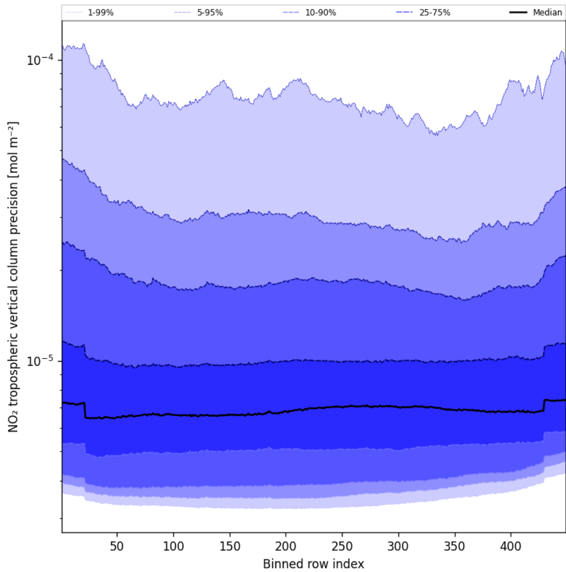
Figure 45: Along track statistics of “NO 2 tropospheric vertical column precision” for 2025-02-05 to 2025-02-06
