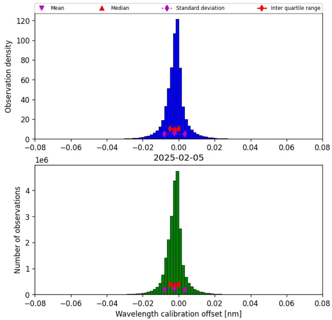
Figure 33: Histogram of “Wavelength calibration offset” for 2025-02-05 to 2025-02-06
