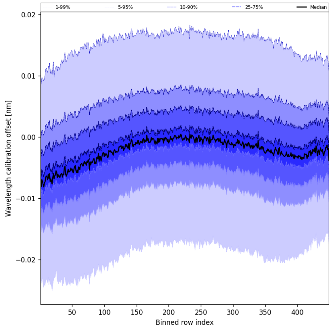
Figure 50: Along track statistics of “Wavelength calibration offset” for 2025-02-05 to 2025-02-06
