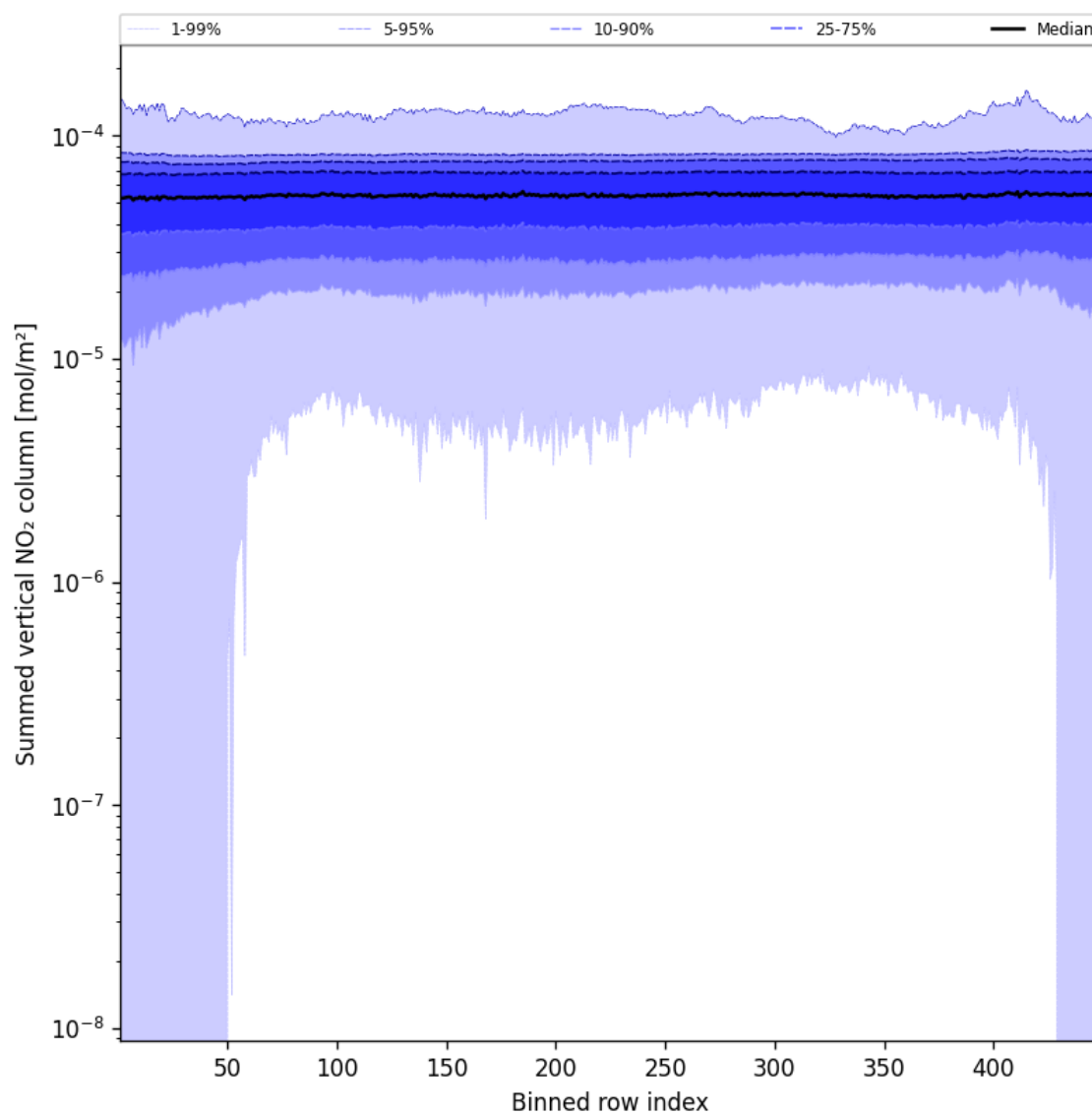
Figure 55: Along track statistics of “Summed vertical NO 2 column” for 2025-02-05 to 2025-02-06
