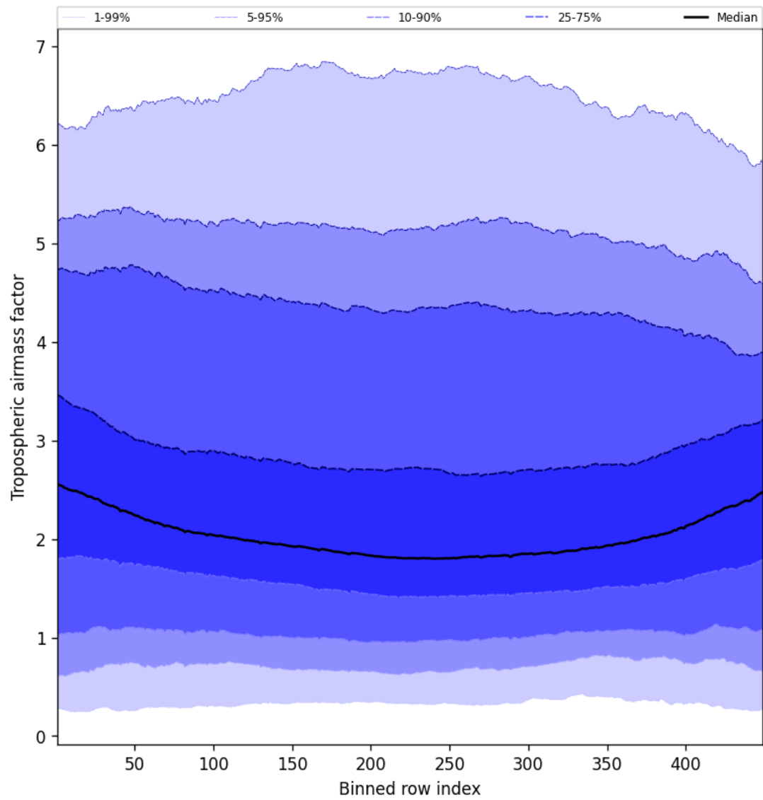
Figure 46: Along track statistics of “Tropospheric airmass factor” for 2025-02-05 to 2025-02-06
