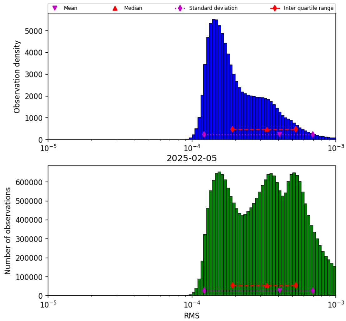
Figure 41: Histogram of “RMS” for 2025-02-05 to 2025-02-06
