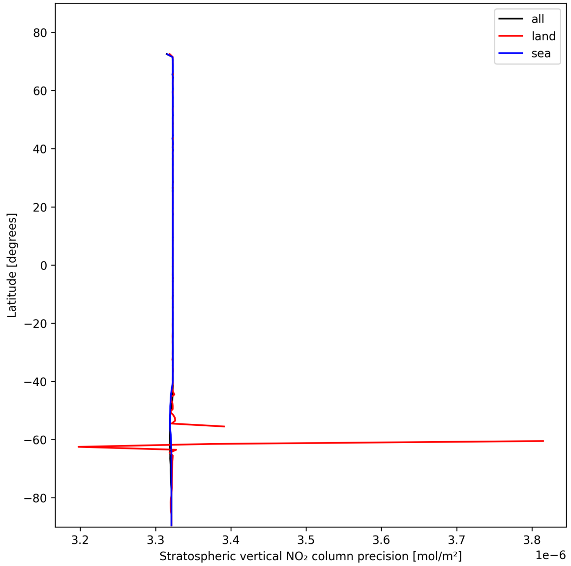
Figure 18: Zonal average of “Stratospheric vertical NO 2 column precision” for 2025-02-05 to 2025-02-06.
