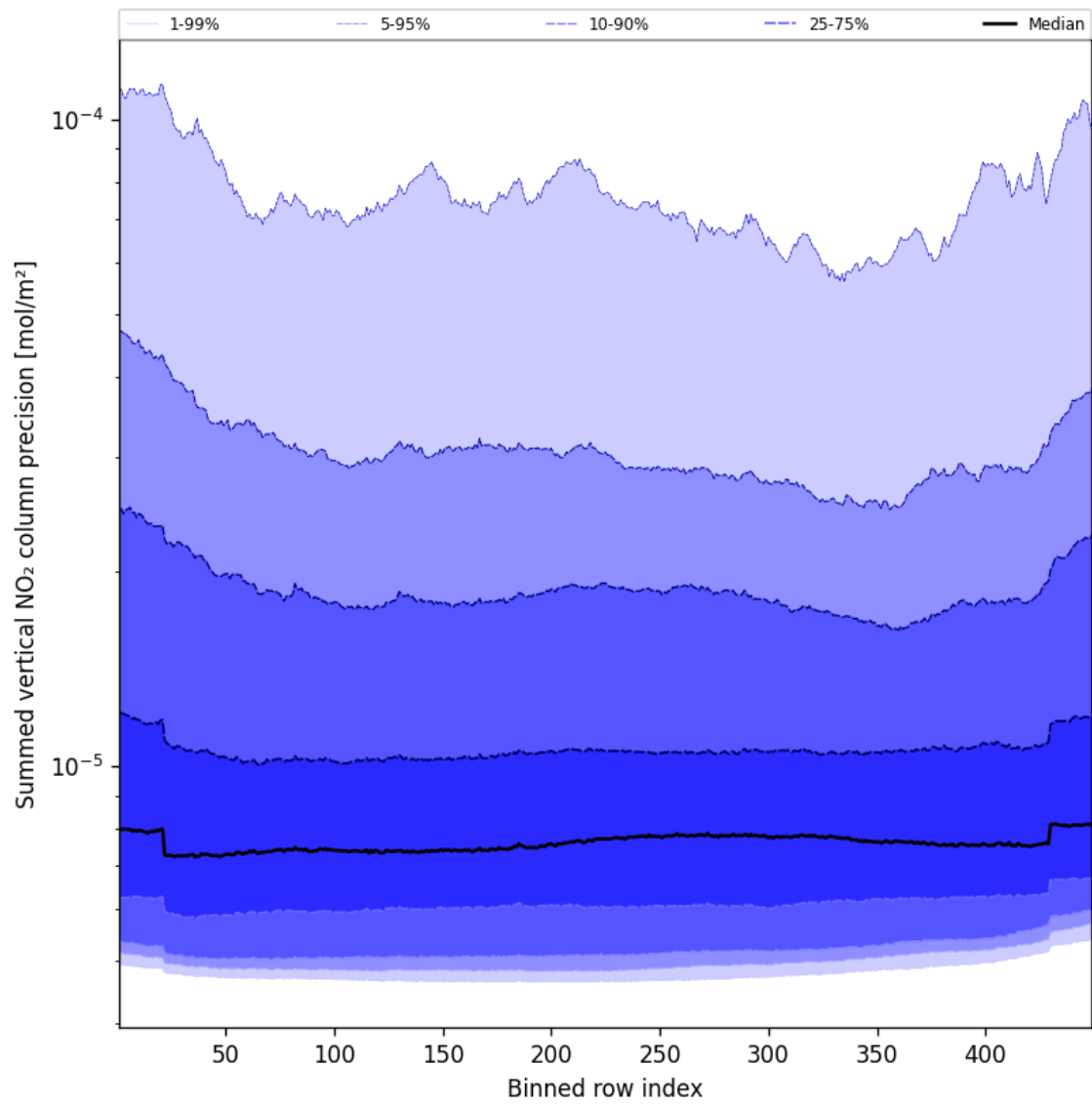
Figure 56: Along track statistics of “Summed vertical NO 2 column precision” for 2025-02-05 to 2025-02-06
