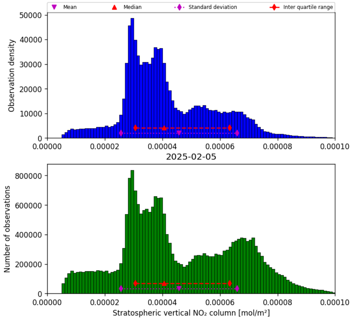
Figure 34: Histogram of “Stratospheric vertical NO 2 column” for 2025-02-05 to 2025-02-06
