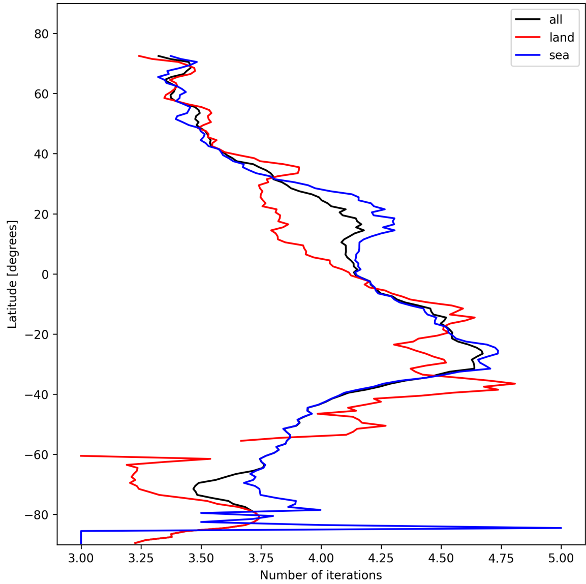
Figure 15: Zonal average of “Number of iterations” for 2025-02-05 to 2025-02-06.
