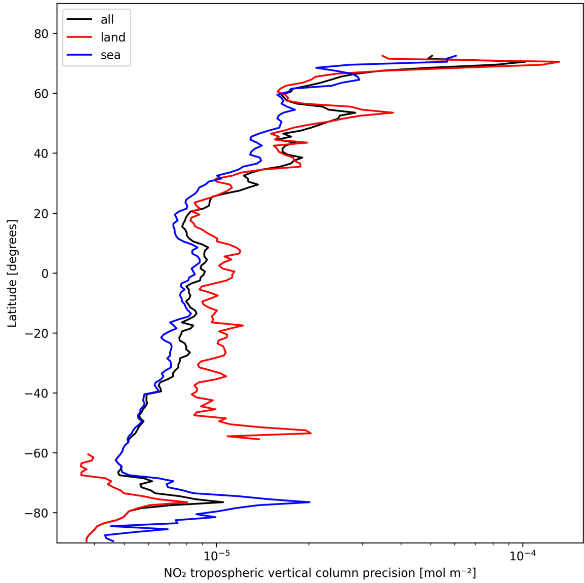
Figure 11: Zonal average of “NO 2 tropospheric vertical column precision” for 2025-02-05 to 2025-02-06.
