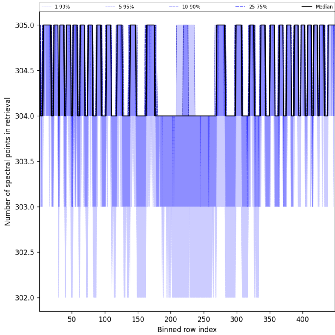
Figure 48: Along track statistics of “Number of spectral points in retrieval” for 2025-02-05 to 2025-02-06
