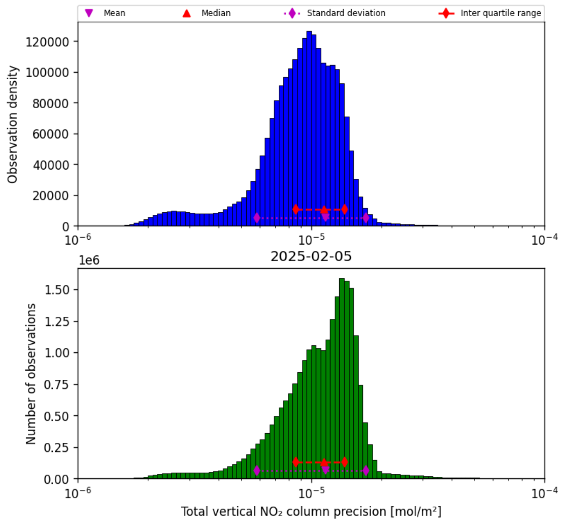
Figure 37: Histogram of “Total vertical NO 2 column precision” for 2025-02-05 to 2025-02-06
