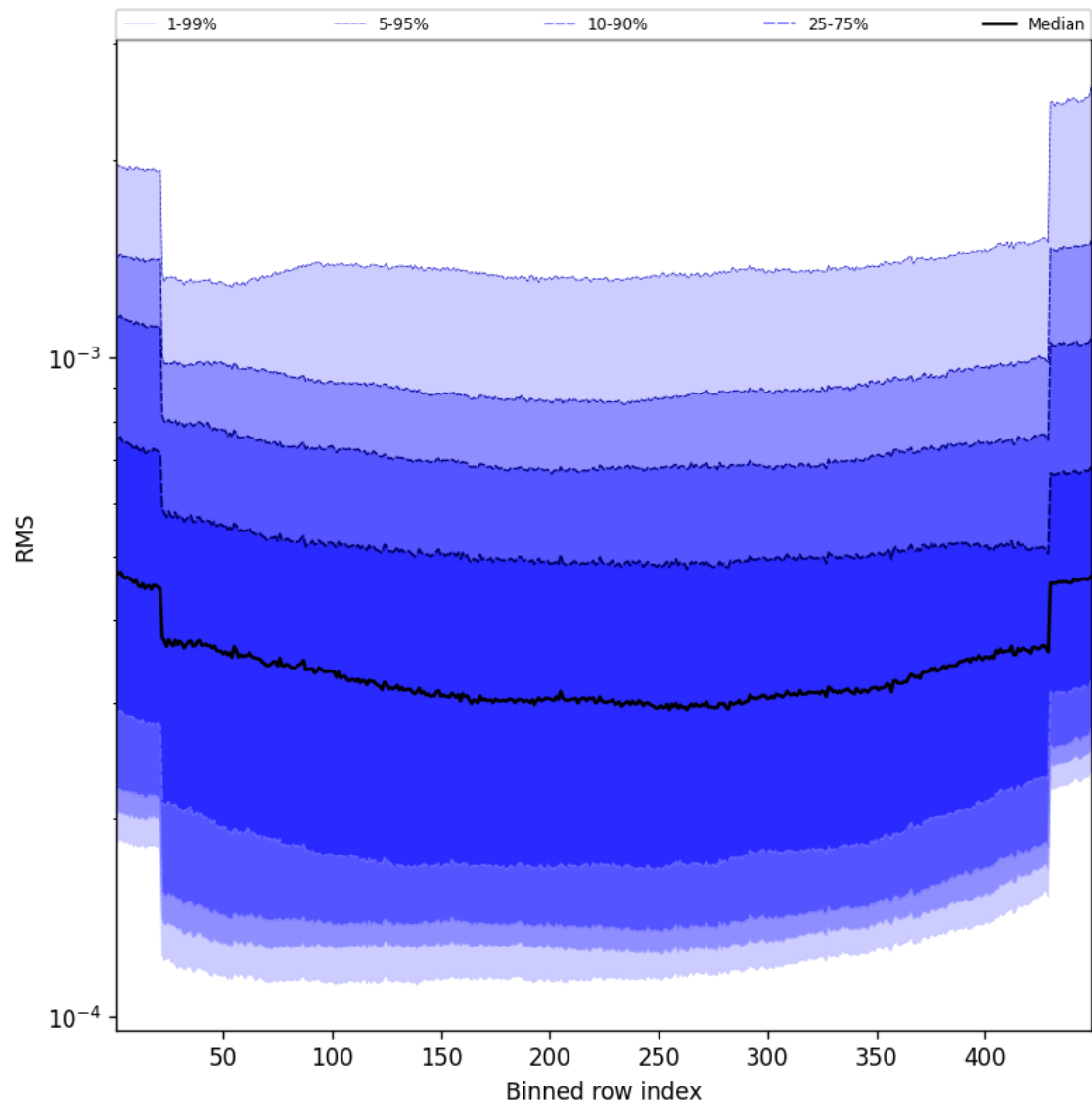
Figure 58: Along track statistics of “RMS” for 2025-02-05 to 2025-02-06
