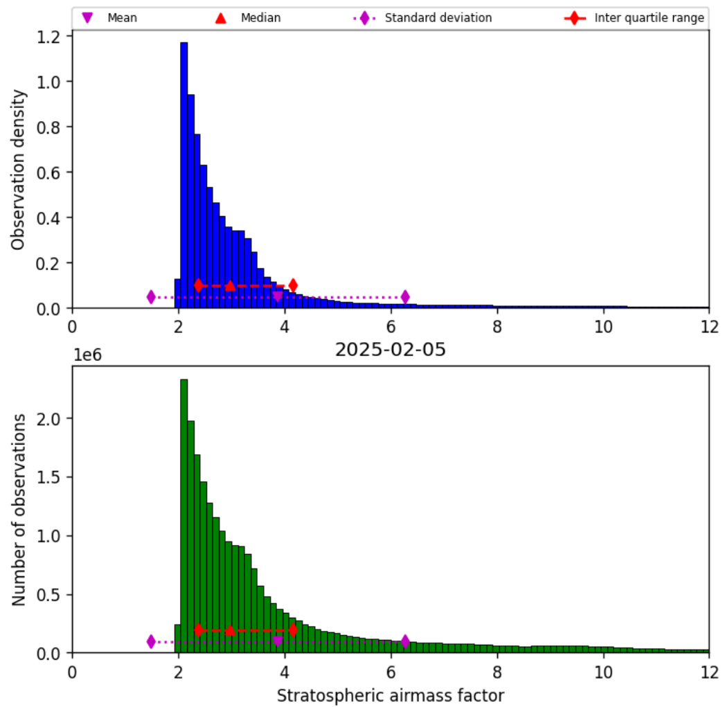
Figure 42: Histogram of “Stratospheric airmass factor” for 2025-02-05 to 2025-02-06
