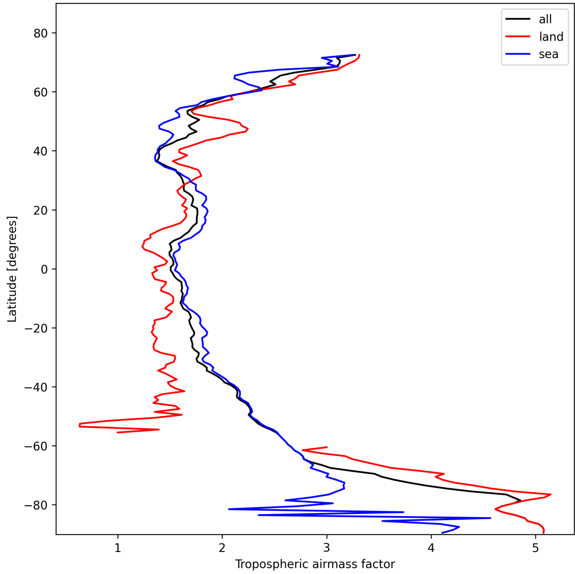
Figure 12: Zonal average of “Tropospheric airmass factor” for 2025-02-05 to 2025-02-06.
