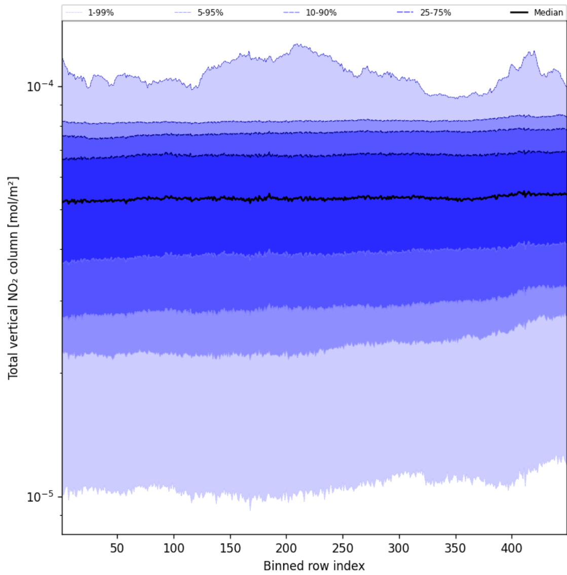
Figure 53: Along track statistics of “Total vertical NO 2 column” for 2025-02-05 to 2025-02-06
