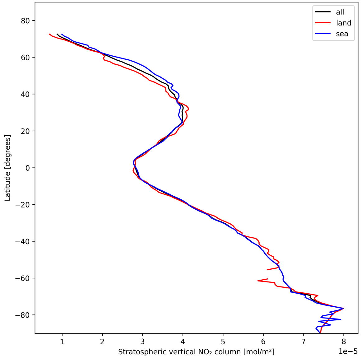
Figure 17: Zonal average of “Stratospheric vertical NO 2 column” for 2025-02-05 to 2025-02-06.
