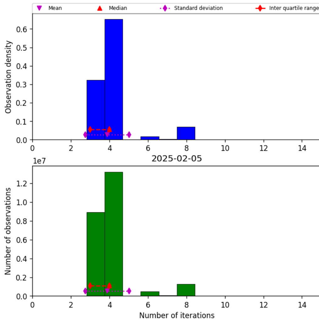
Figure 32: Histogram of “Number of iterations” for 2025-02-05 to 2025-02-06
