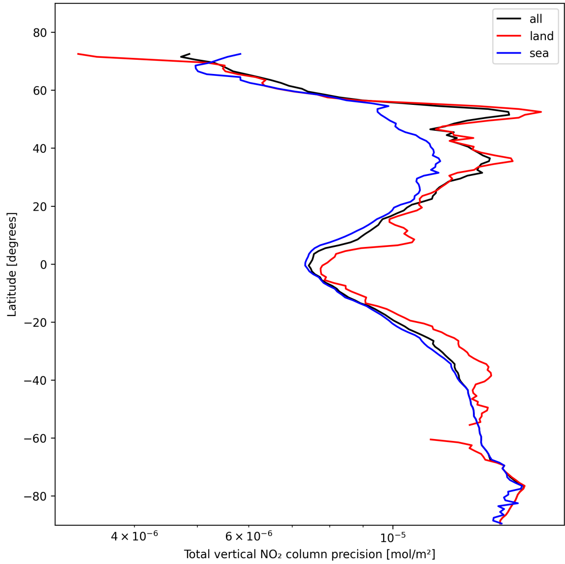
Figure 20: Zonal average of “Total vertical NO 2 column precision” for 2025-02-05 to 2025-02-06.
