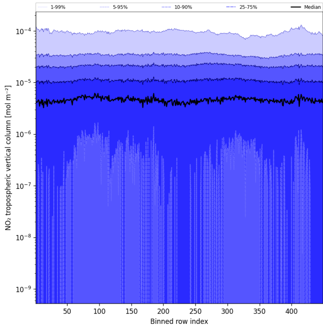
Figure 44: Along track statistics of “NO 2 tropospheric vertical column” for 2025-02-05 to 2025-02-06
