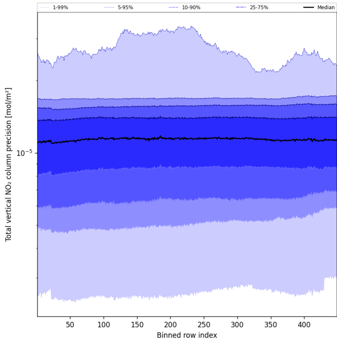
Figure 54: Along track statistics of “Total vertical NO 2 column precision” for 2025-02-05 to 2025-02-06
