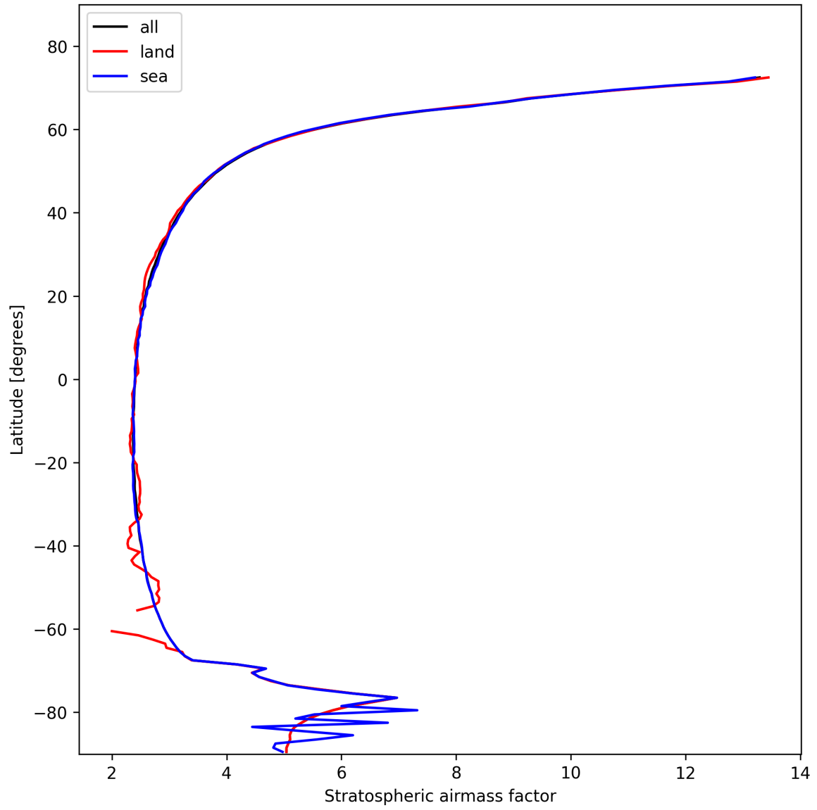
Figure 25: Zonal average of “Stratospheric airmass factor” for 2025-02-05 to 2025-02-06.
