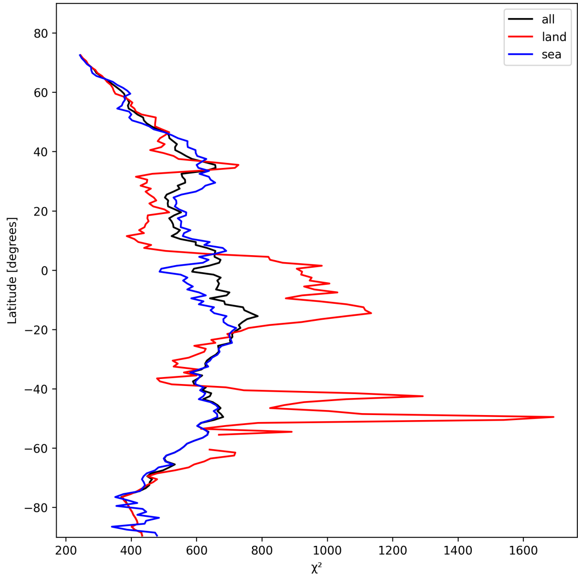
Figure 23: Zonal average of “ \chi^2 ” for 2025-02-05 to 2025-02-06.
