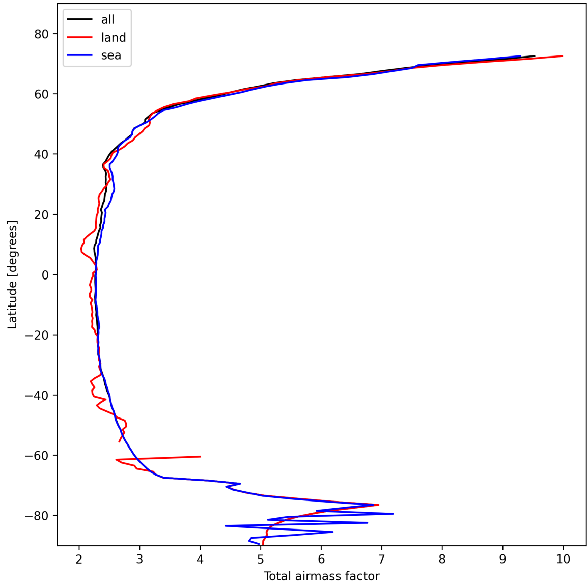
Figure 13: Zonal average of “Total airmass factor” for 2025-02-05 to 2025-02-06.
