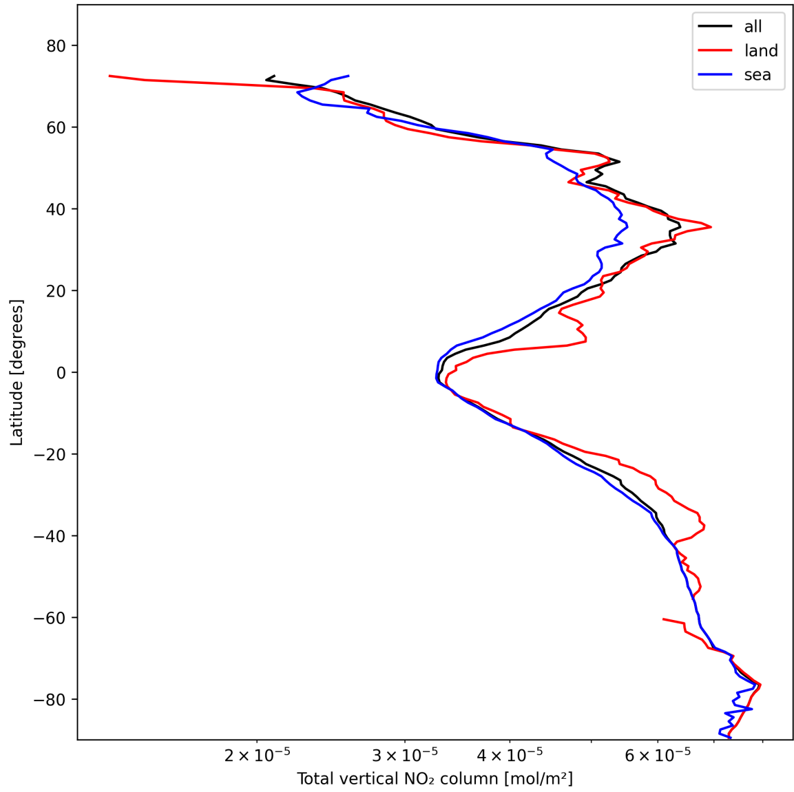
Figure 19: Zonal average of “Total vertical NO 2 column” for 2025-02-05 to 2025-02-06.
