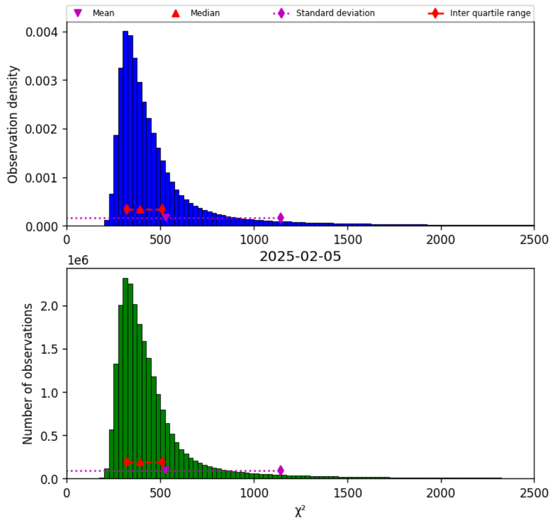
Figure 40: Histogram of “ \chi^2 ” for 2025-02-05 to 2025-02-06
