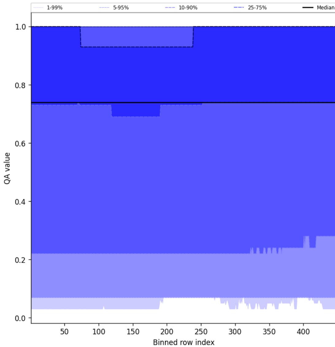
Figure 43: Along track statistics of “QA value” for 2025-02-05 to 2025-02-06
