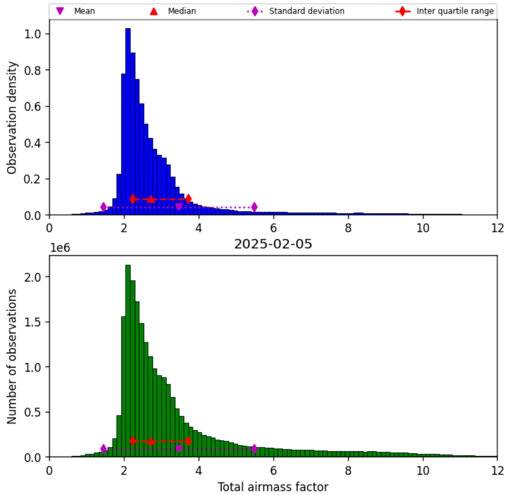
Figure 30: Histogram of “Total airmass factor” for 2025-02-05 to 2025-02-06
