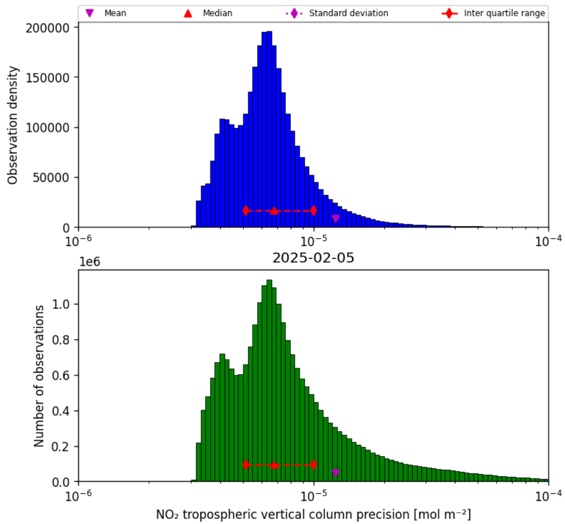
Figure 28: Histogram of “NO 2 tropospheric vertical column precision” for 2025-02-05 to 2025-02-06
