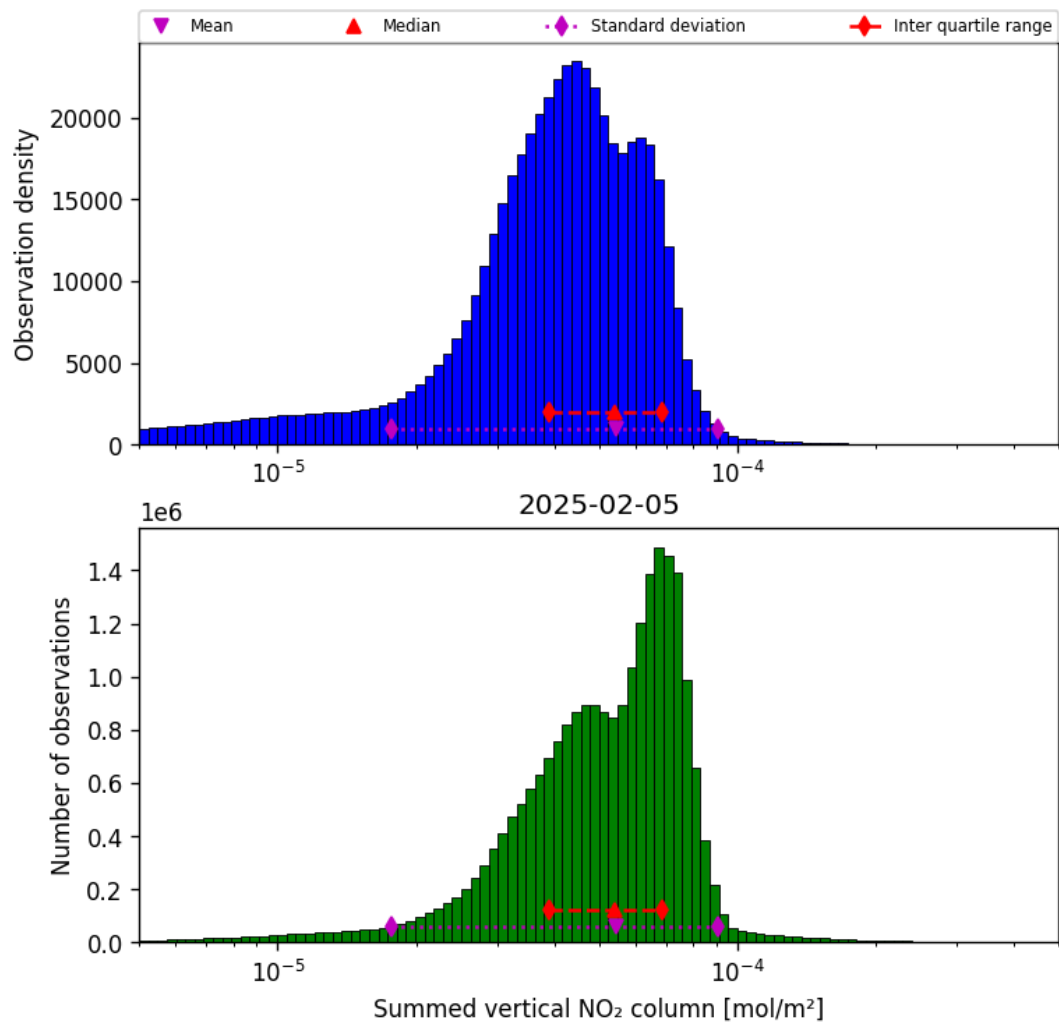
Figure 38: Histogram of “Summed vertical NO 2 column” for 2025-02-05 to 2025-02-06
