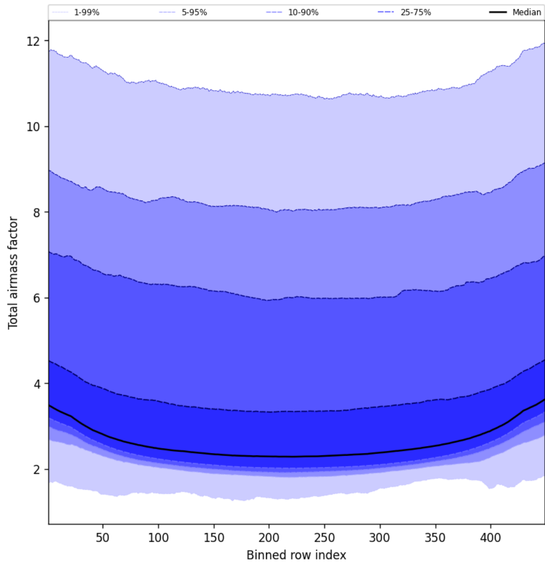
Figure 47: Along track statistics of “Total airmass factor” for 2025-02-05 to 2025-02-06
