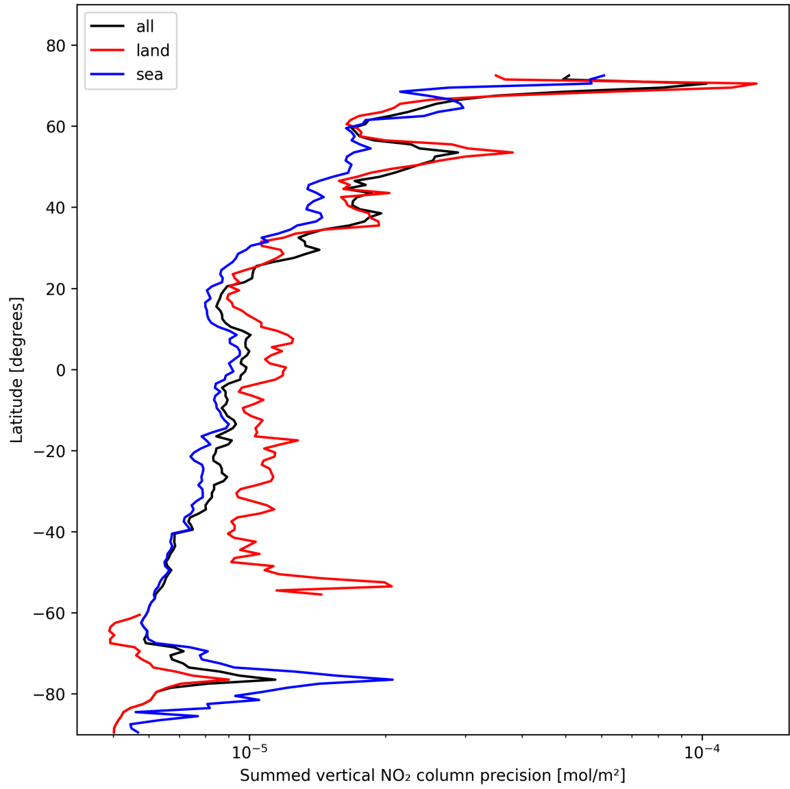
Figure 22: Zonal average of “Summed vertical NO 2 column precision” for 2025-02-05 to 2025-02-06.
