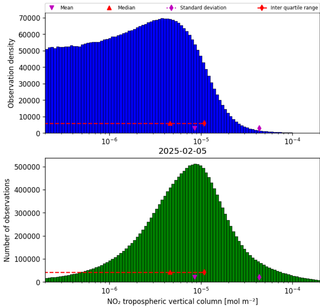
Figure 27: Histogram of “NO 2 tropospheric vertical column” for 2025-02-05 to 2025-02-06
