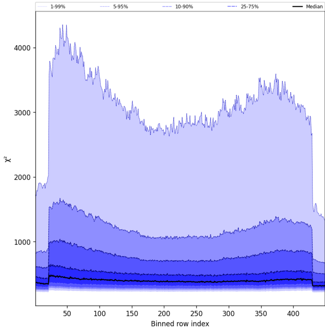
Figure 57: Along track statistics of “ \chi^2 ” for 2025-02-05 to 2025-02-06
