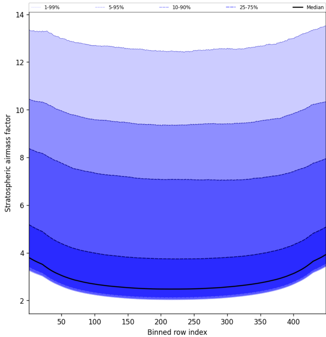
Figure 59: Along track statistics of “Stratospheric airmass factor” for 2025-02-05 to 2025-02-06
