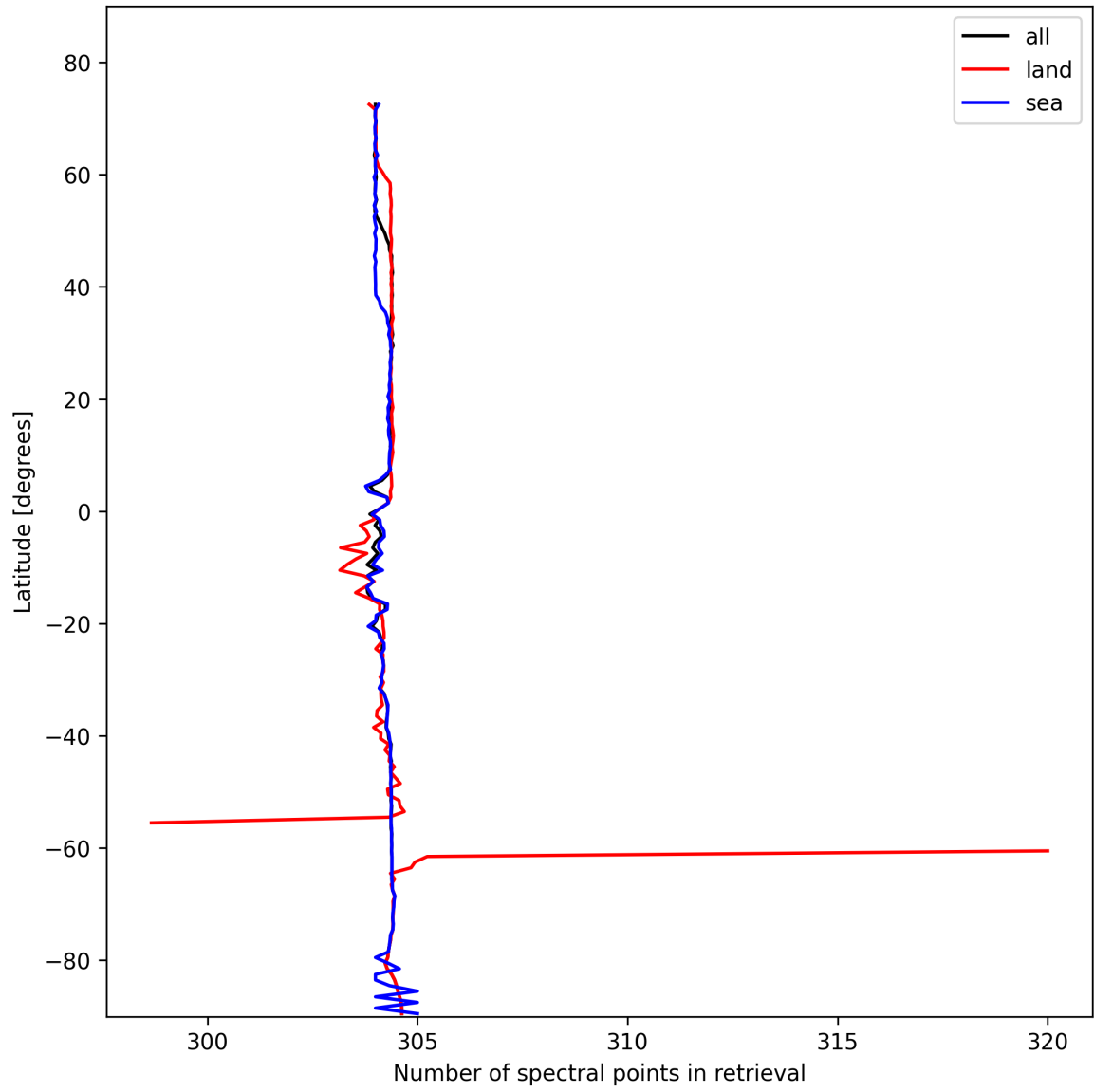
Figure 14: Zonal average of “Number of spectral points in retrieval” for 2025-02-05 to 2025-02-06.
