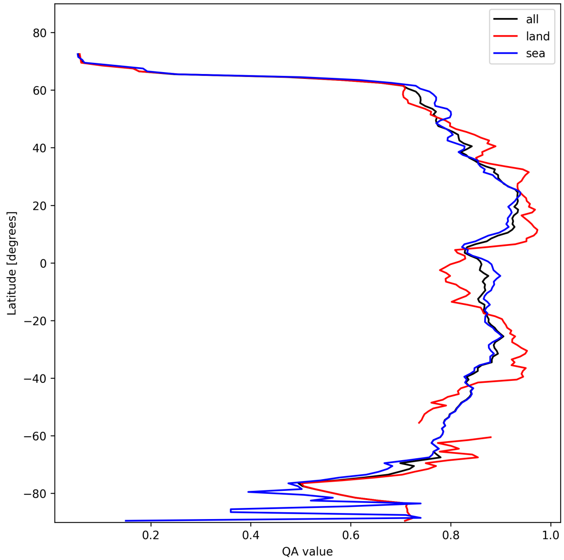
Figure 9: Zonal average of “QA value” for 2025-02-05 to 2025-02-06.
