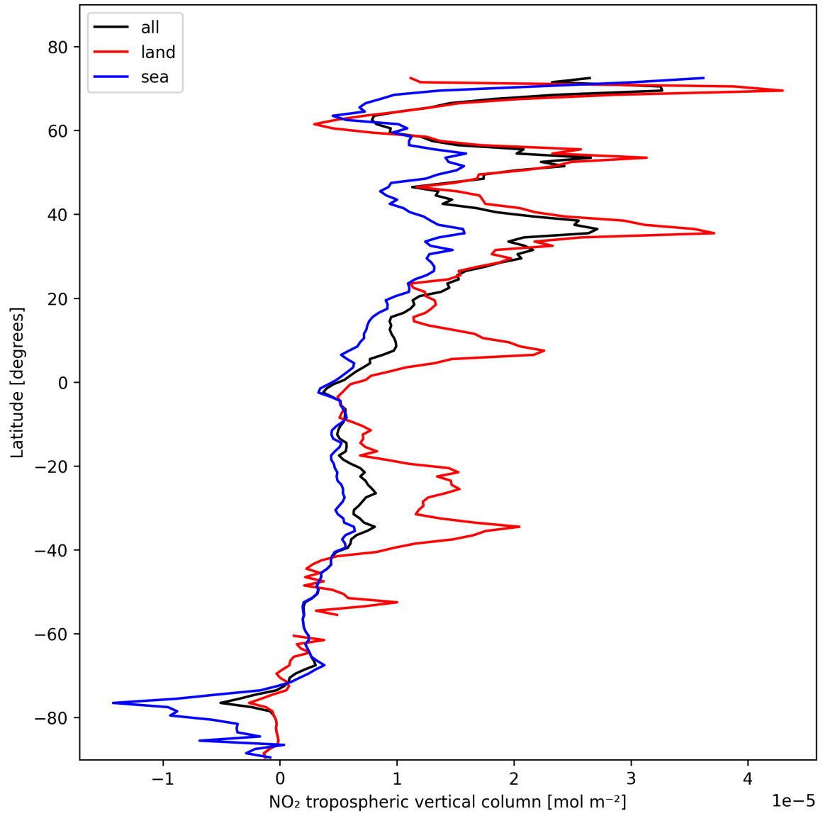
Figure 10: Zonal average of “NO 2 tropospheric vertical column” for 2025-02-05 to 2025-02-06.
