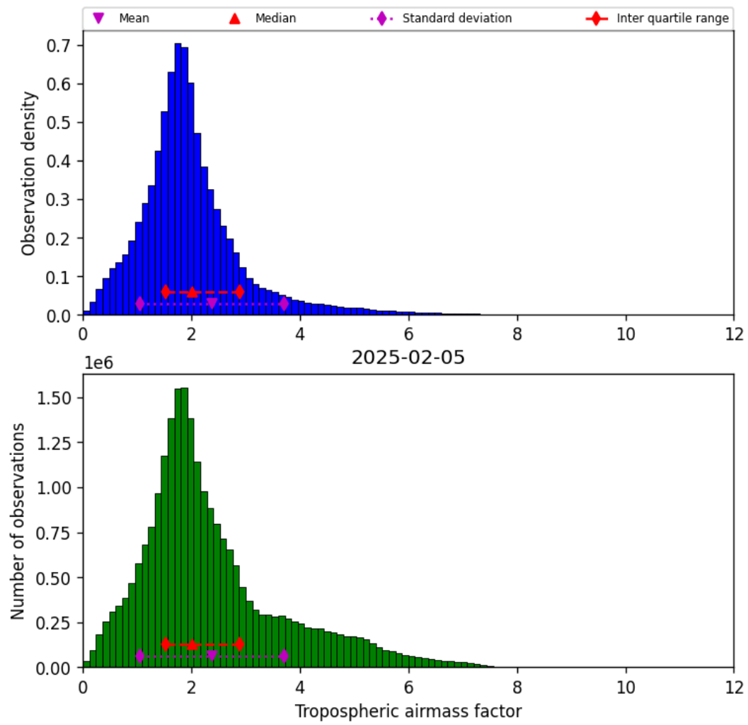
Figure 29: Histogram of “Tropospheric airmass factor” for 2025-02-05 to 2025-02-06
