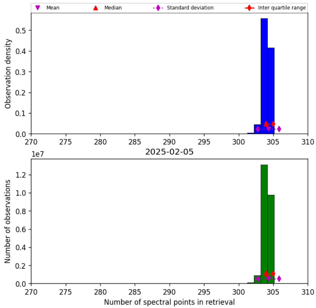
Figure 31: Histogram of “Number of spectral points in retrieval” for 2025-02-05 to 2025-02-06
