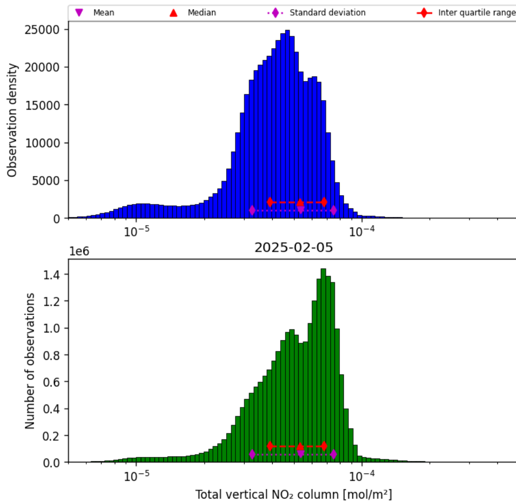
Figure 36: Histogram of “Total vertical NO 2 column” for 2025-02-05 to 2025-02-06
