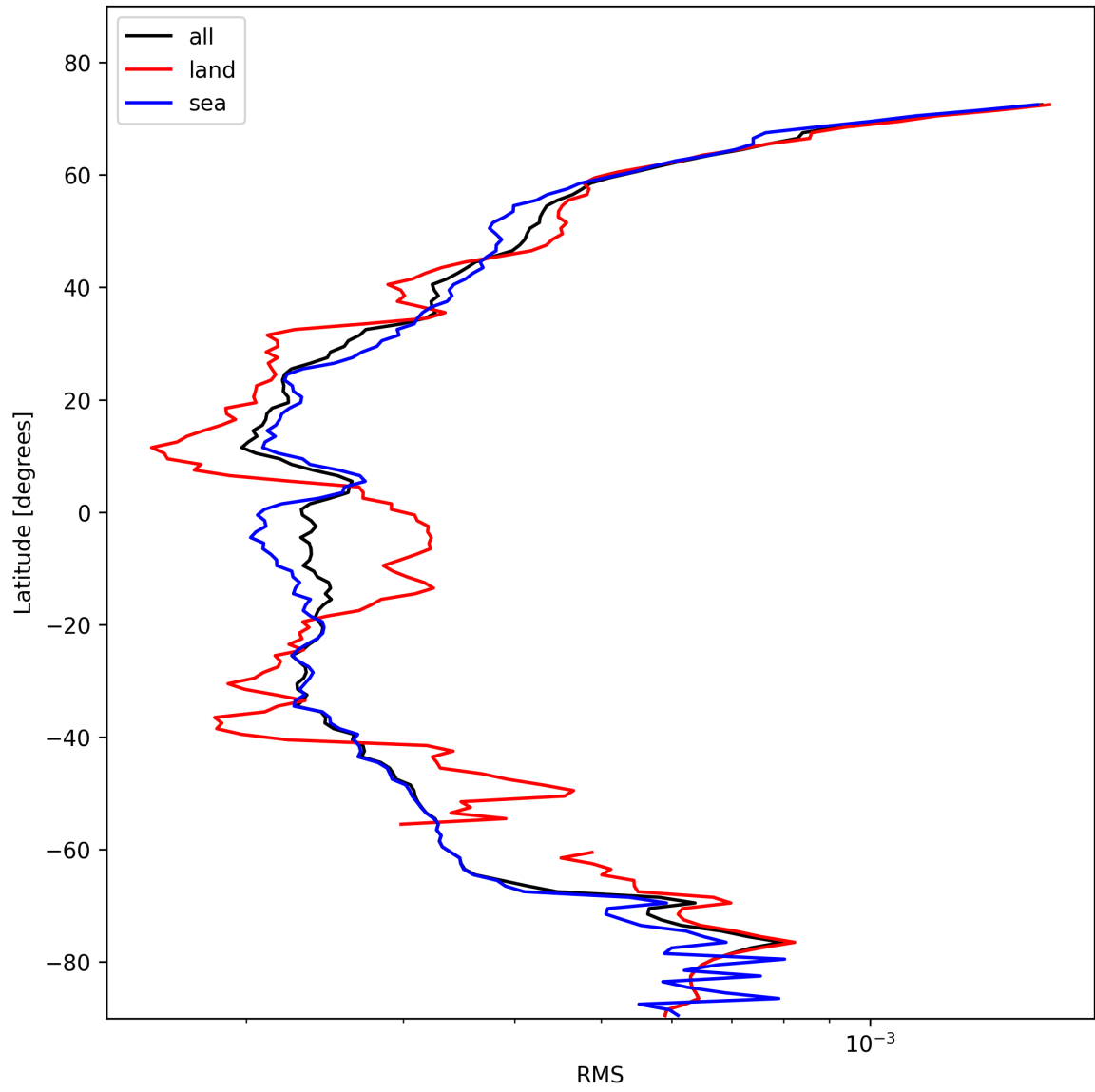
Figure 24: Zonal average of “RMS” for 2025-02-05 to 2025-02-06.
