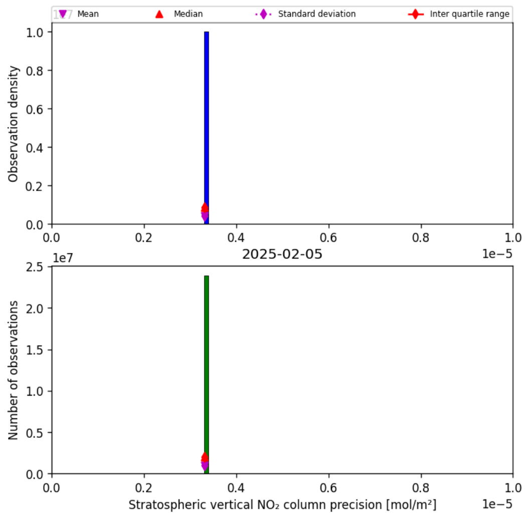
Figure 35: Histogram of “Stratospheric vertical NO 2 column precision” for 2025-02-05 to 2025-02-06
