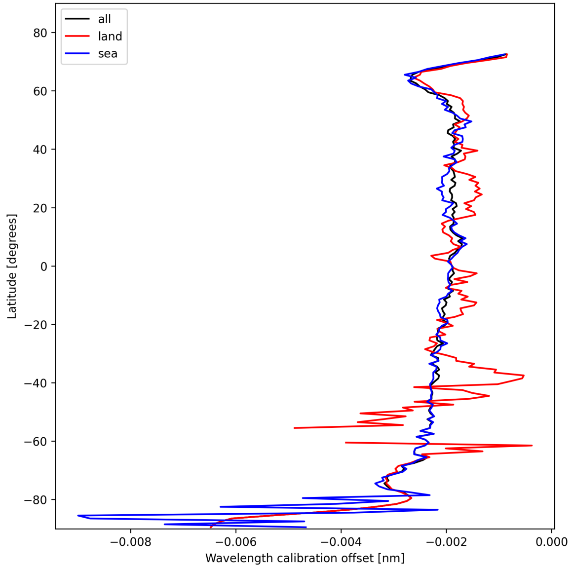
Figure 16: Zonal average of “Wavelength calibration offset” for 2025-02-05 to 2025-02-06.
