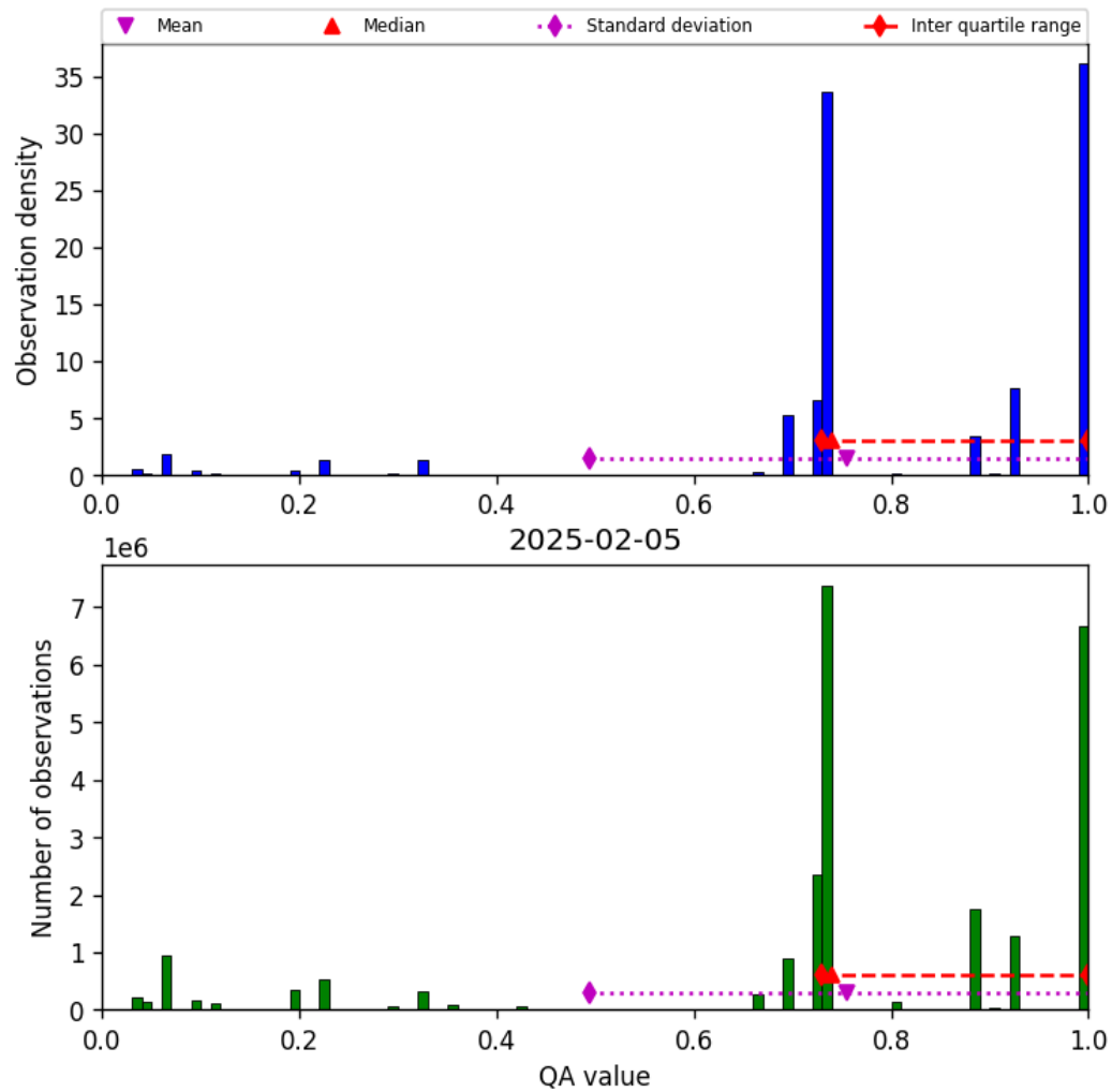
Figure 26: Histogram of “QA value” for 2025-02-05 to 2025-02-06
