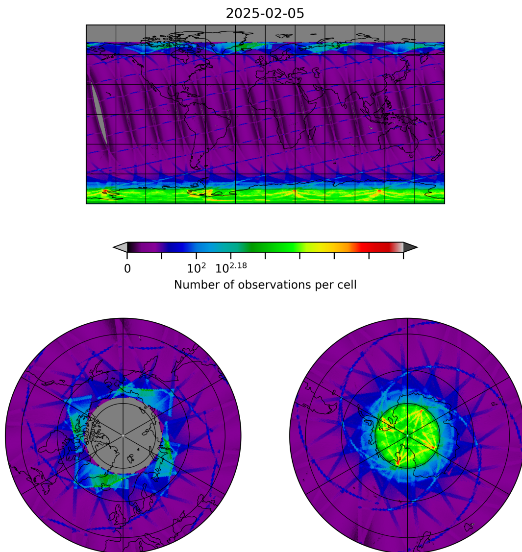
Figure 8: Map of the number of observations for 2025-02-05 to 2025-02-06
