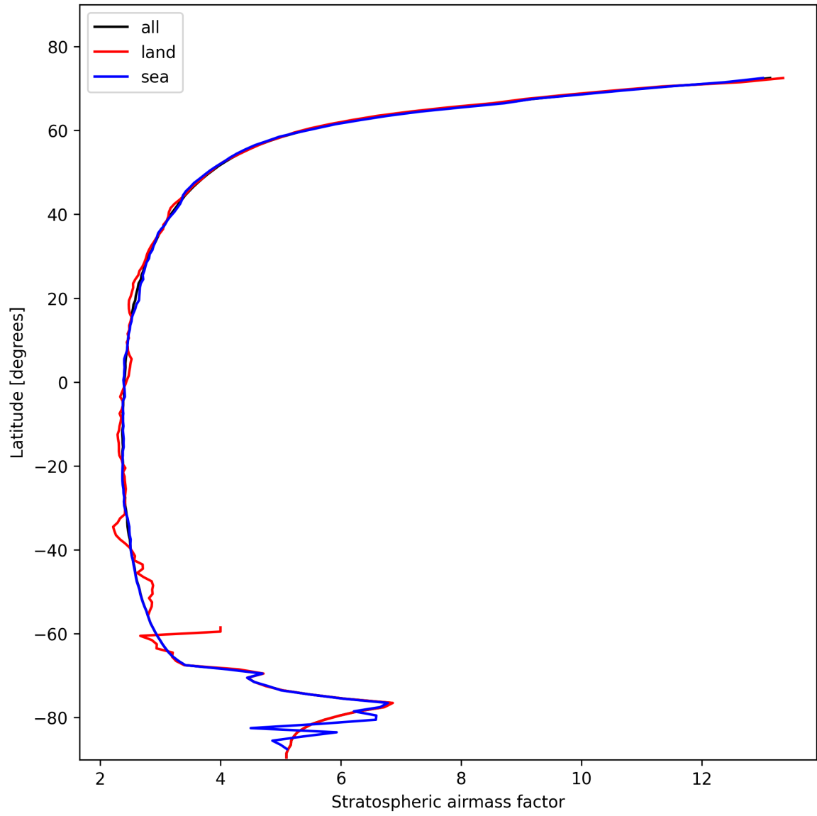
Figure 25: Zonal average of “Stratospheric airmass factor” for 2025-02-06 to 2025-02-06.
