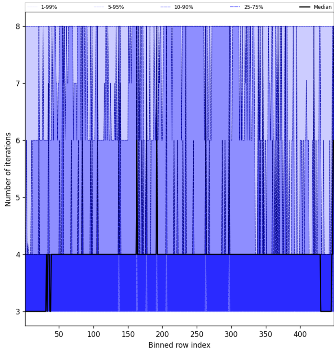
Figure 49: Along track statistics of “Number of iterations” for 2025-02-06 to 2025-02-06
