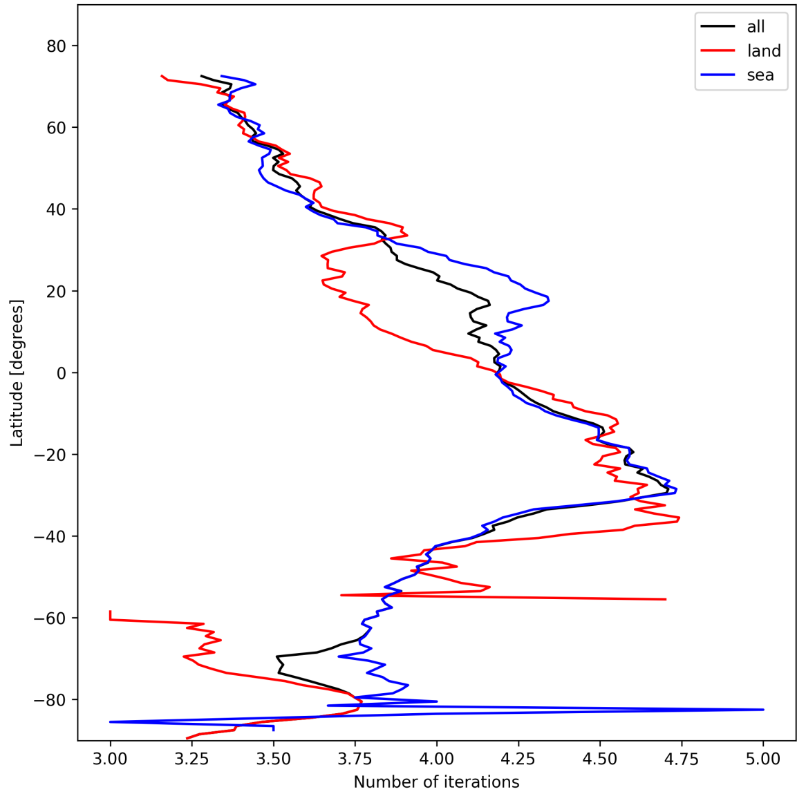
Figure 15: Zonal average of “Number of iterations” for 2025-02-06 to 2025-02-06.
