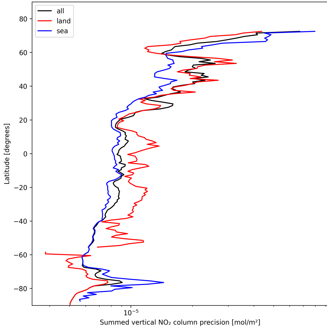
Figure 22: Zonal average of “Summed vertical NO 2 column precision” for 2025-02-06 to 2025-02-06.
