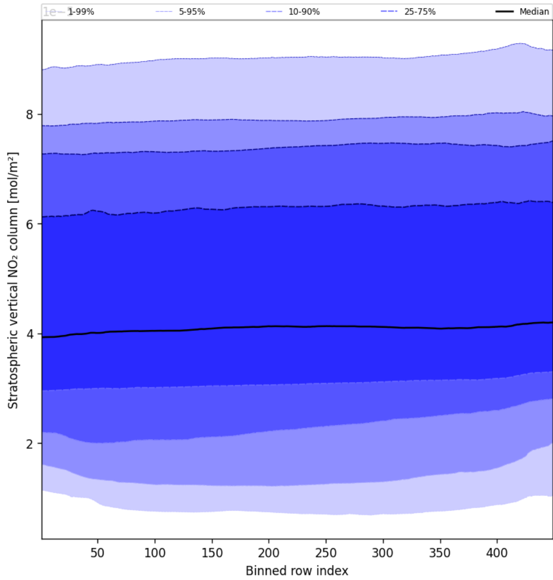
Figure 51: Along track statistics of “Stratospheric vertical NO 2 column” for 2025-02-06 to 2025-02-06
