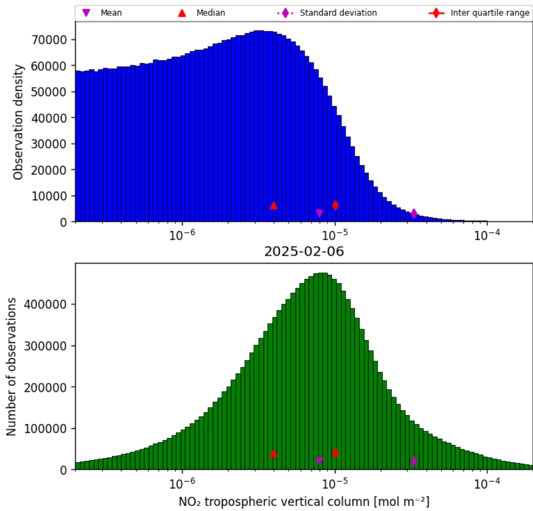
Figure 27: Histogram of “NO 2 tropospheric vertical column” for 2025-02-06 to 2025-02-06
