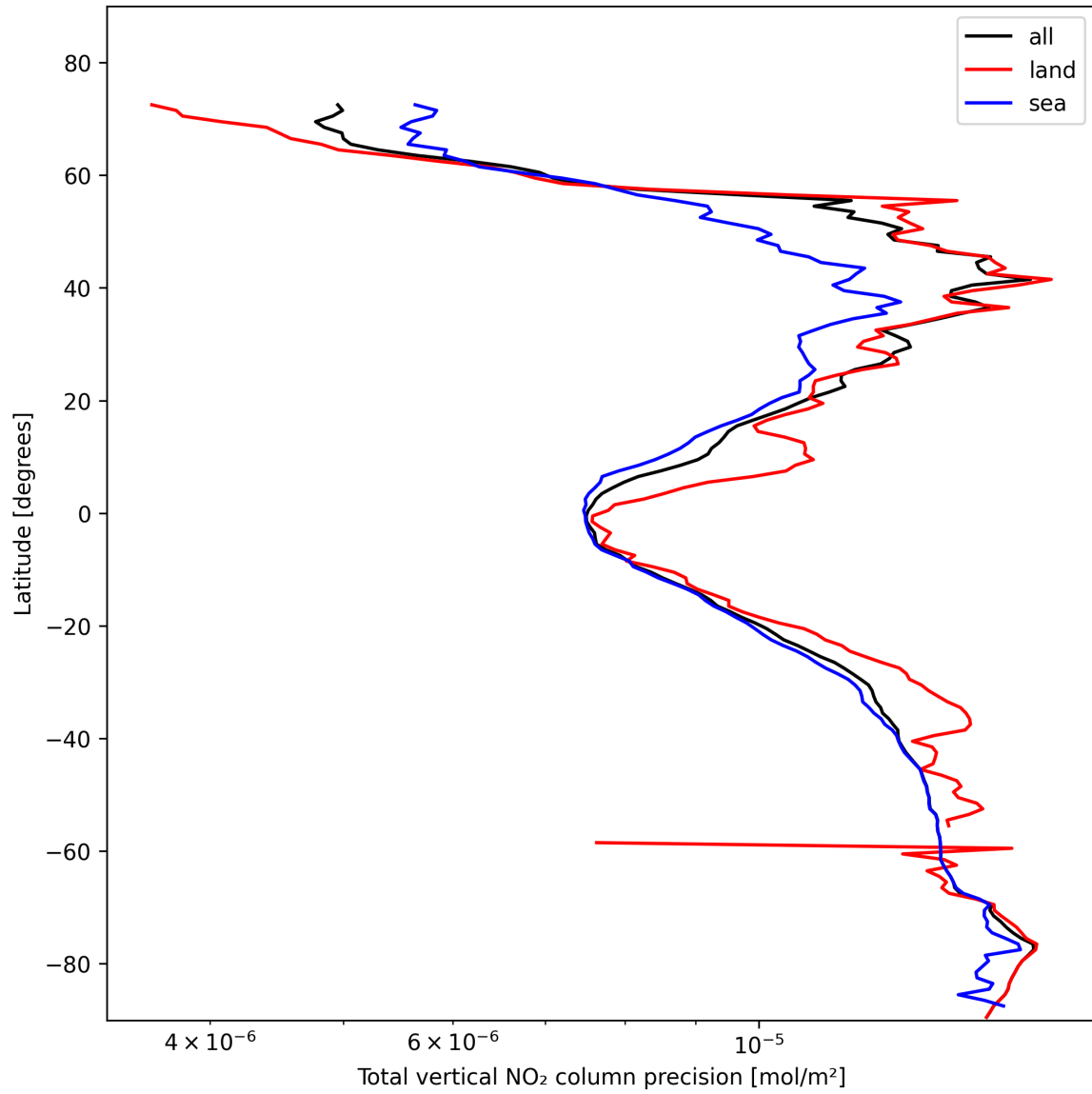
Figure 20: Zonal average of “Total vertical NO 2 column precision” for 2025-02-06 to 2025-02-06.
