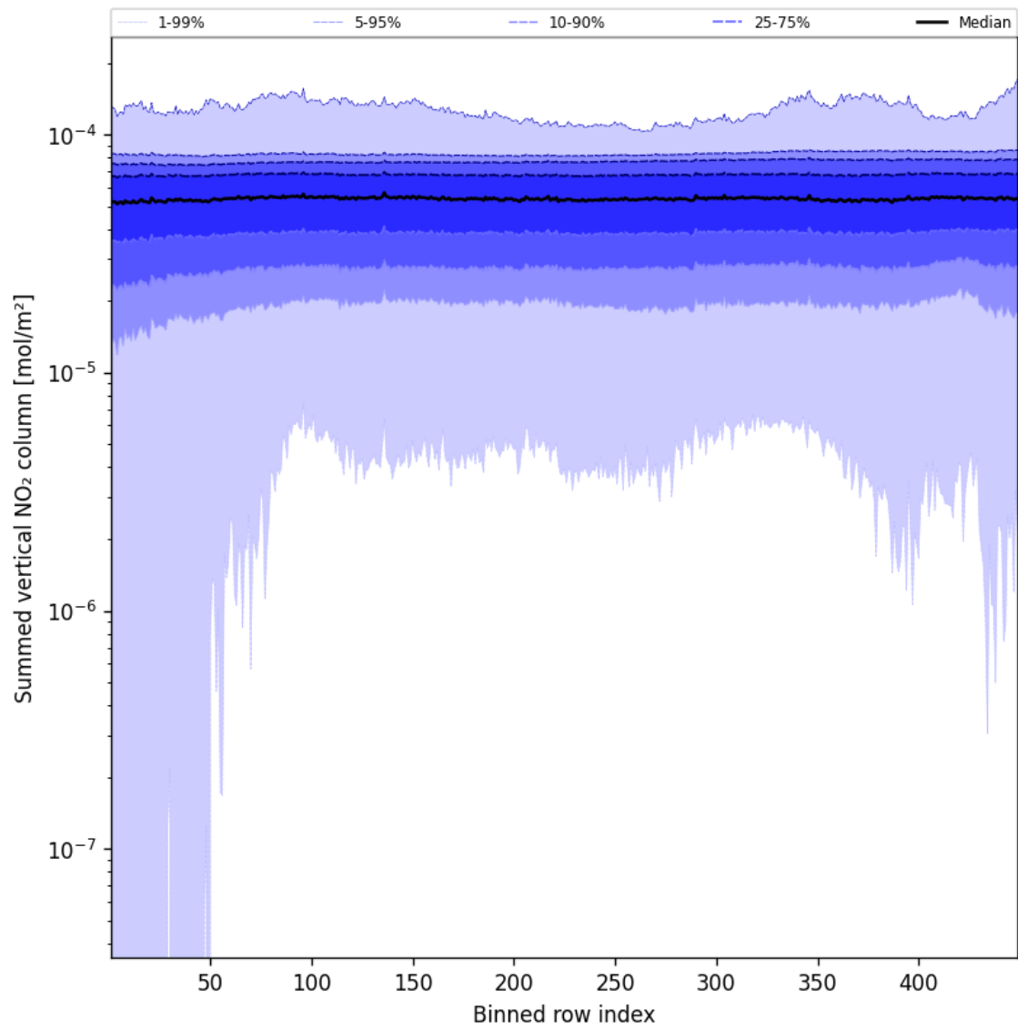
Figure 55: Along track statistics of “Summed vertical NO 2 column” for 2025-02-06 to 2025-02-06
