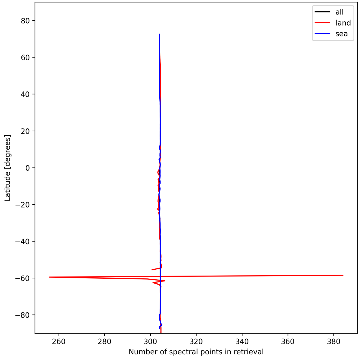
Figure 14: Zonal average of “Number of spectral points in retrieval” for 2025-02-06 to 2025-02-06.
