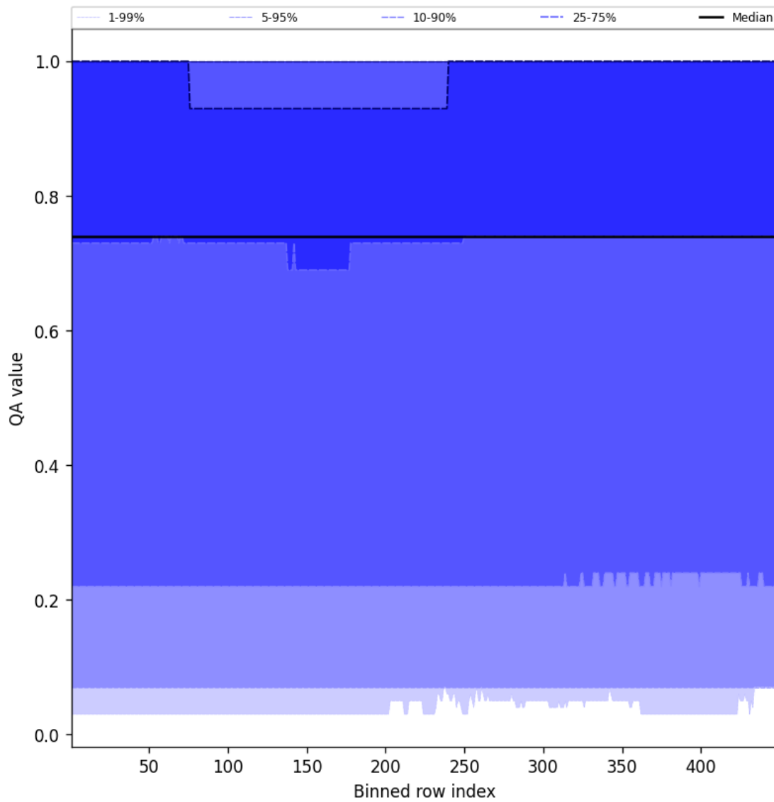
Figure 43: Along track statistics of "QA value" for 2025-02-06 to 2025-02-06
