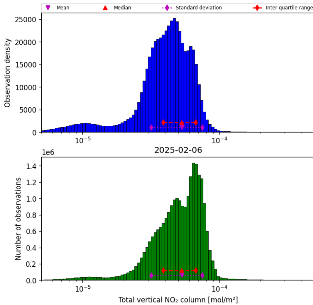
Figure 36: Histogram of "Total vertical NO 2 column" for 2025-02-06 to 2025-02-06
