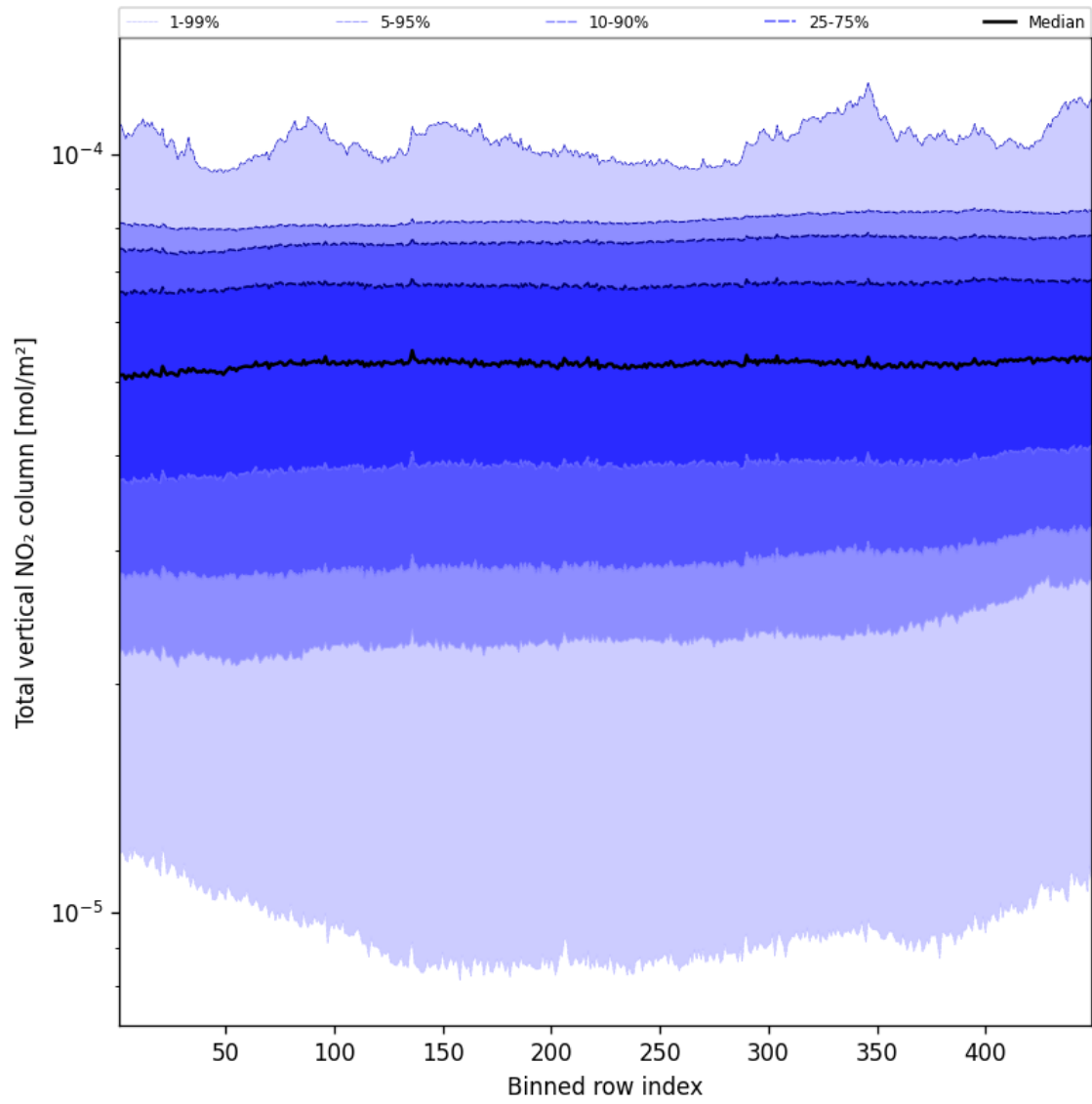
Figure 53: Along track statistics of “Total vertical NO 2 column” for 2025-02-06 to 2025-02-06
