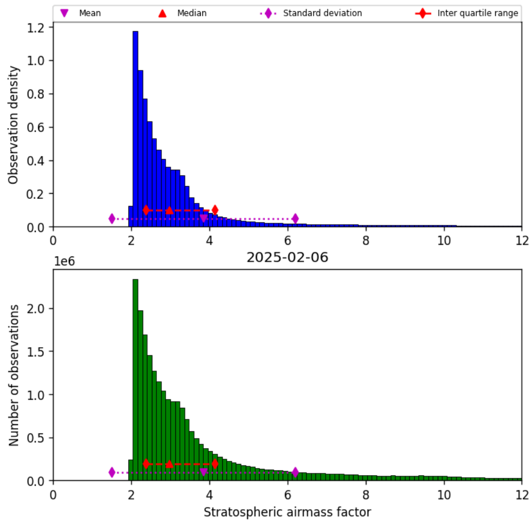
Figure 42: Histogram of “Stratospheric airmass factor” for 2025-02-06 to 2025-02-06
