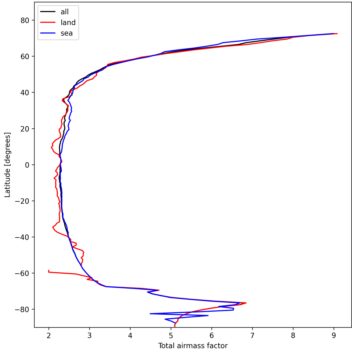
Figure 13: Zonal average of “Total airmass factor” for 2025-02-06 to 2025-02-06.
