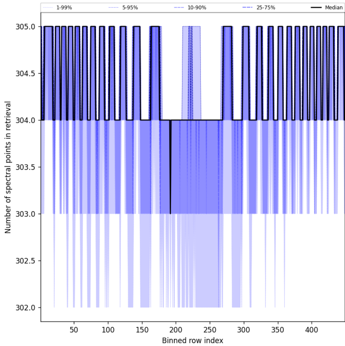
Figure 48: Along track statistics of “Number of spectral points in retrieval” for 2025-02-06 to 2025-02-06
