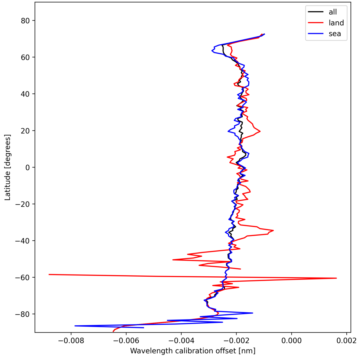
Figure 16: Zonal average of “Wavelength calibration offset” for 2025-02-06 to 2025-02-06.
