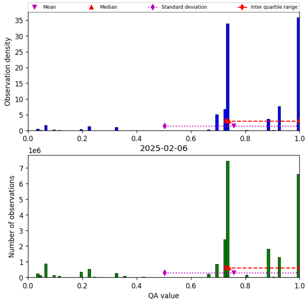
Figure 26: Histogram of “QA value” for 2025-02-06 to 2025-02-06
