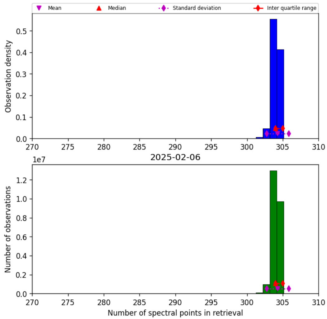
Figure 31: Histogram of “Number of spectral points in retrieval” for 2025-02-06 to 2025-02-06
