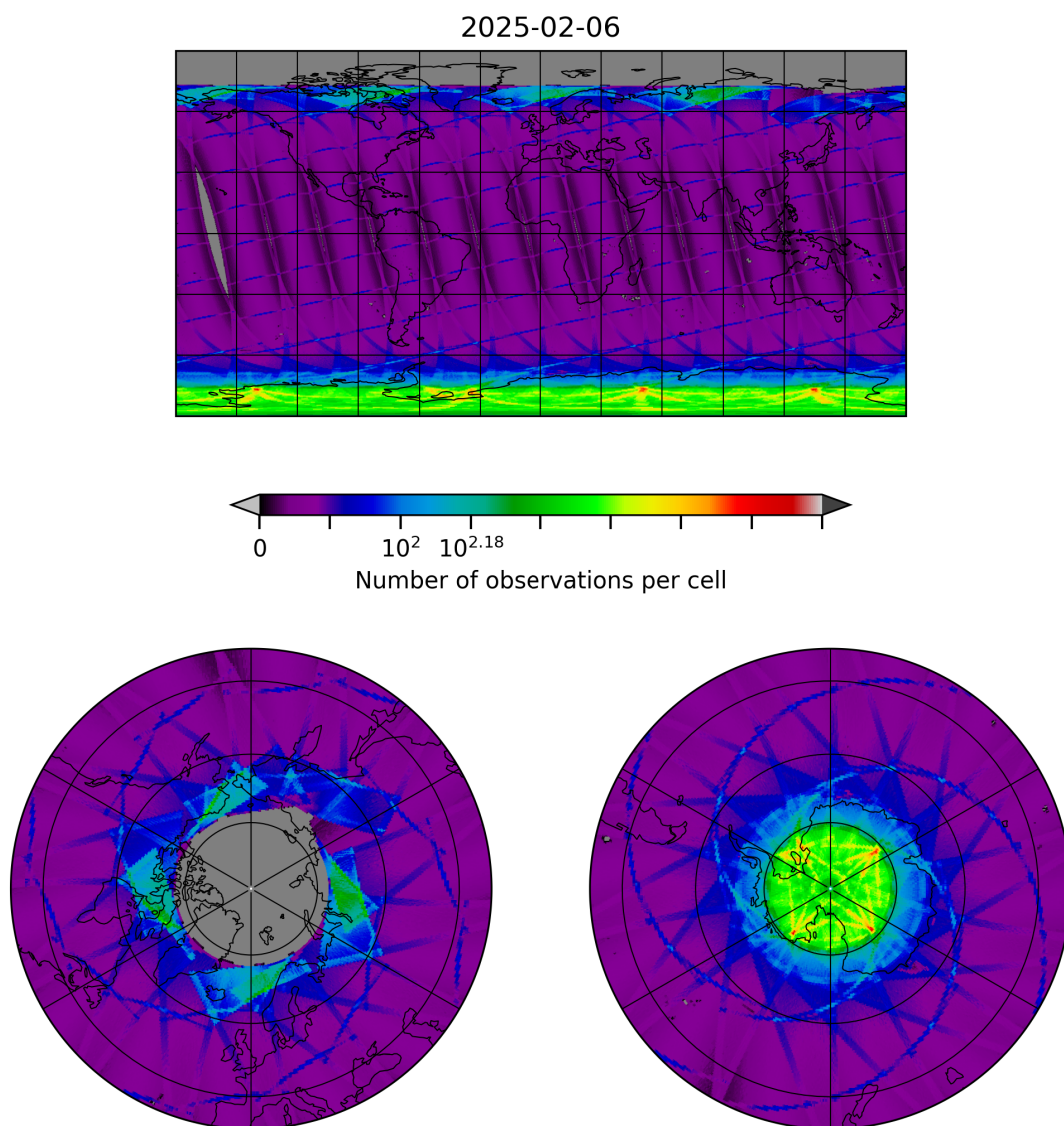
Figure 8: Map of the number of observations for 2025-02-06 to 2025-02-06
