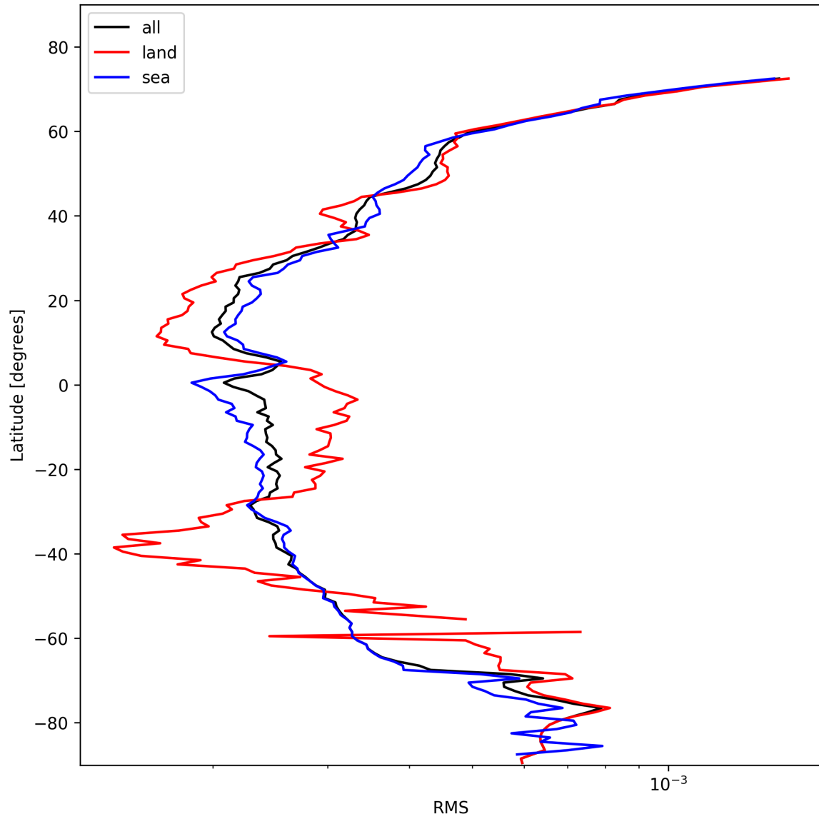
Figure 24: Zonal average of “RMS” for 2025-02-06 to 2025-02-06.
