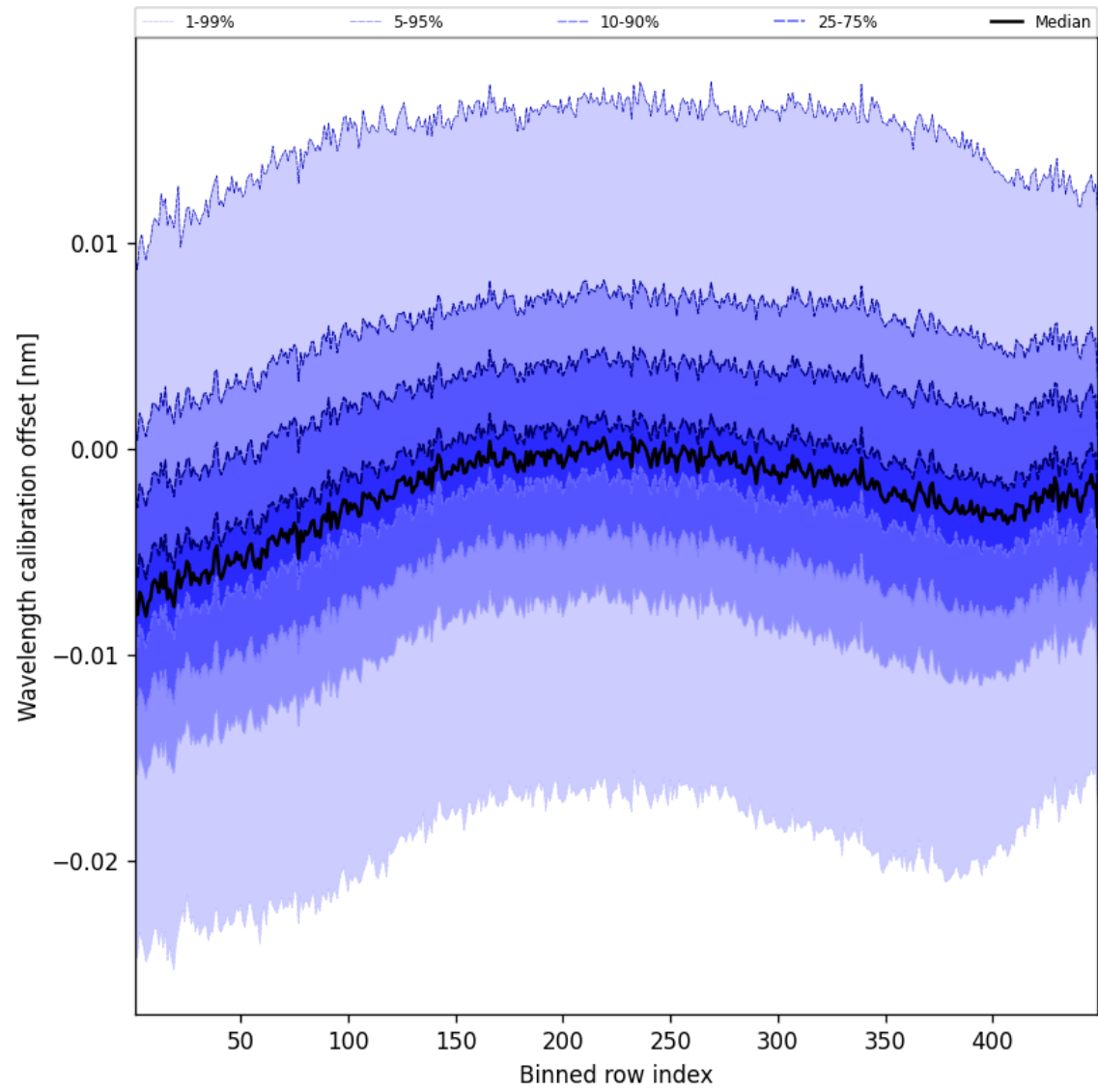
Figure 50: Along track statistics of “Wavelength calibration offset” for 2025-02-06 to 2025-02-06
