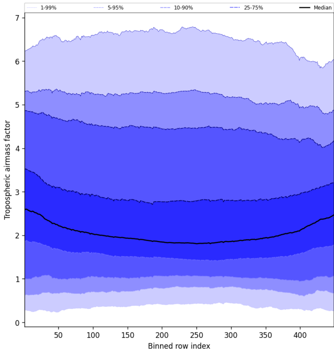
Figure 46: Along track statistics of “Tropospheric airmass factor” for 2025-02-06 to 2025-02-06
