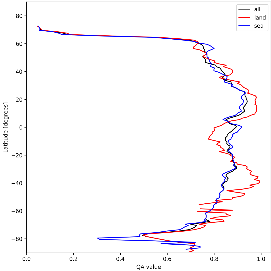
Figure 9: Zonal average of “QA value” for 2025-02-06 to 2025-02-06.
