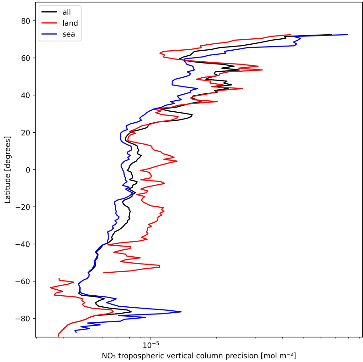
Figure 11: Zonal average of “NO 2 tropospheric vertical column precision” for 2025-02-06 to 2025-02-06.
