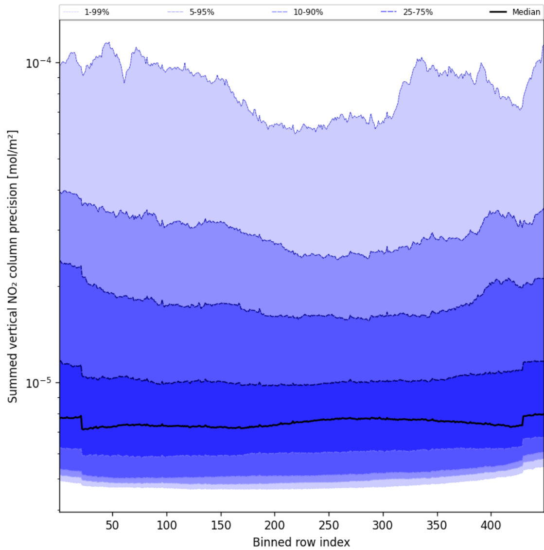
Figure 56: Along track statistics of “Summed vertical NO 2 column precision” for 2025-02-06 to 2025-02-06
