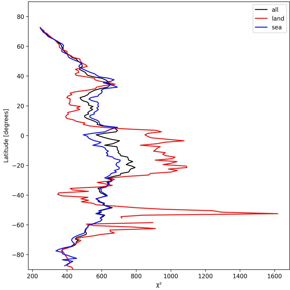
Figure 23: Zonal average of “ \chi^2 ” for 2025-02-06 to 2025-02-06.
