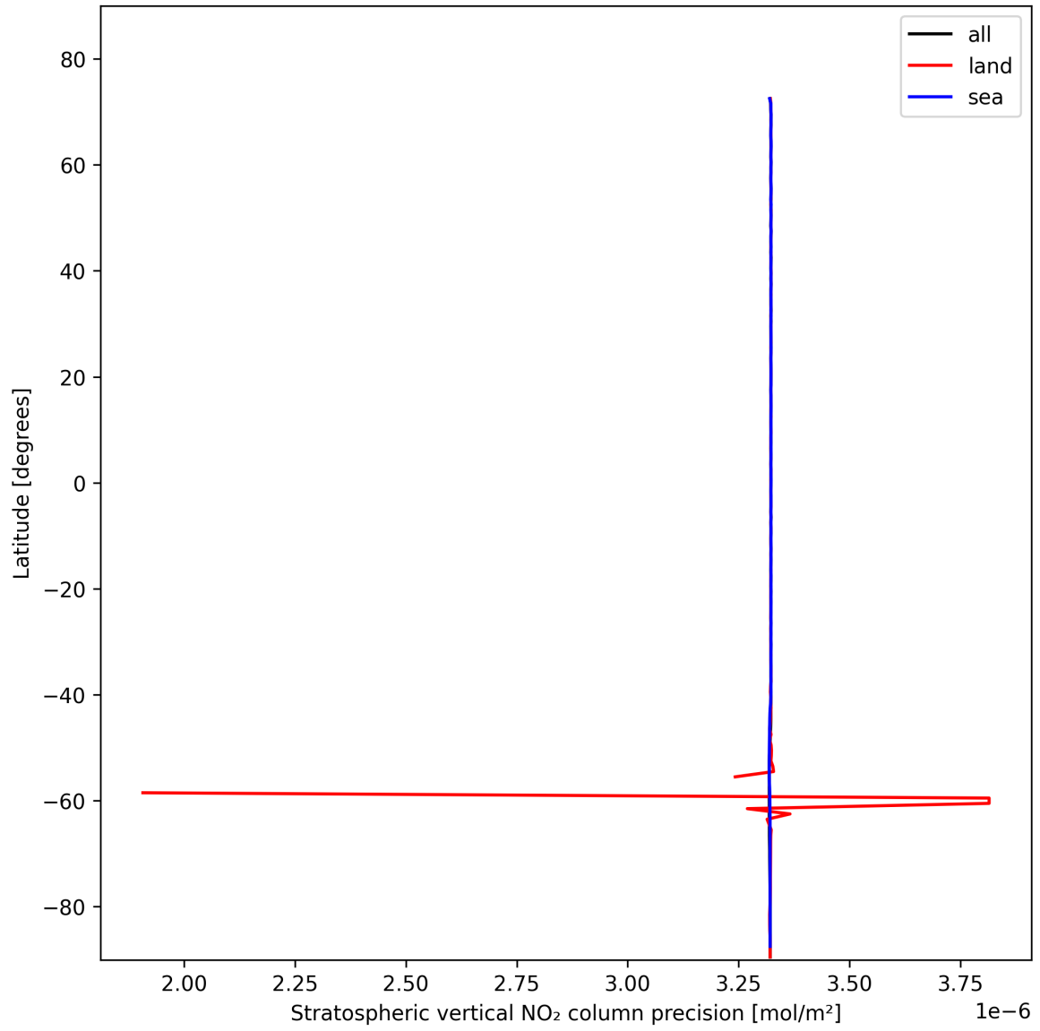
Figure 18: Zonal average of “Stratospheric vertical NO 2 column precision” for 2025-02-06 to 2025-02-06.
