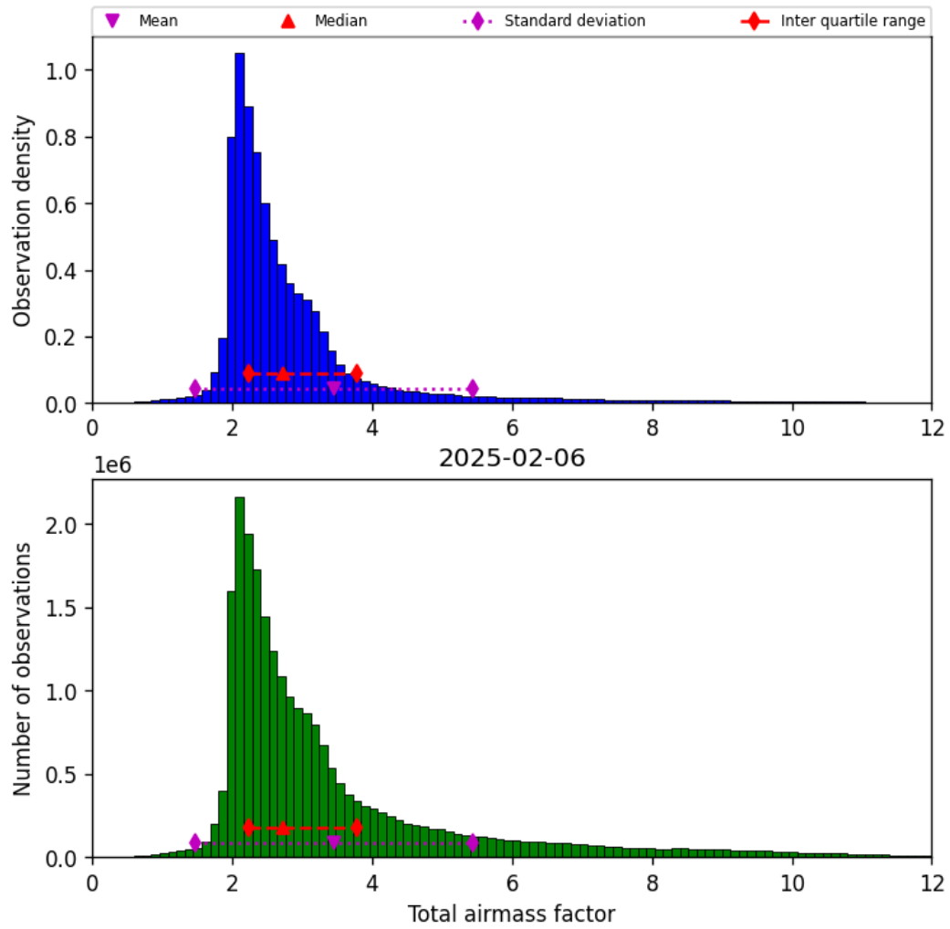
Figure 30: Histogram of “Total airmass factor” for 2025-02-06 to 2025-02-06
