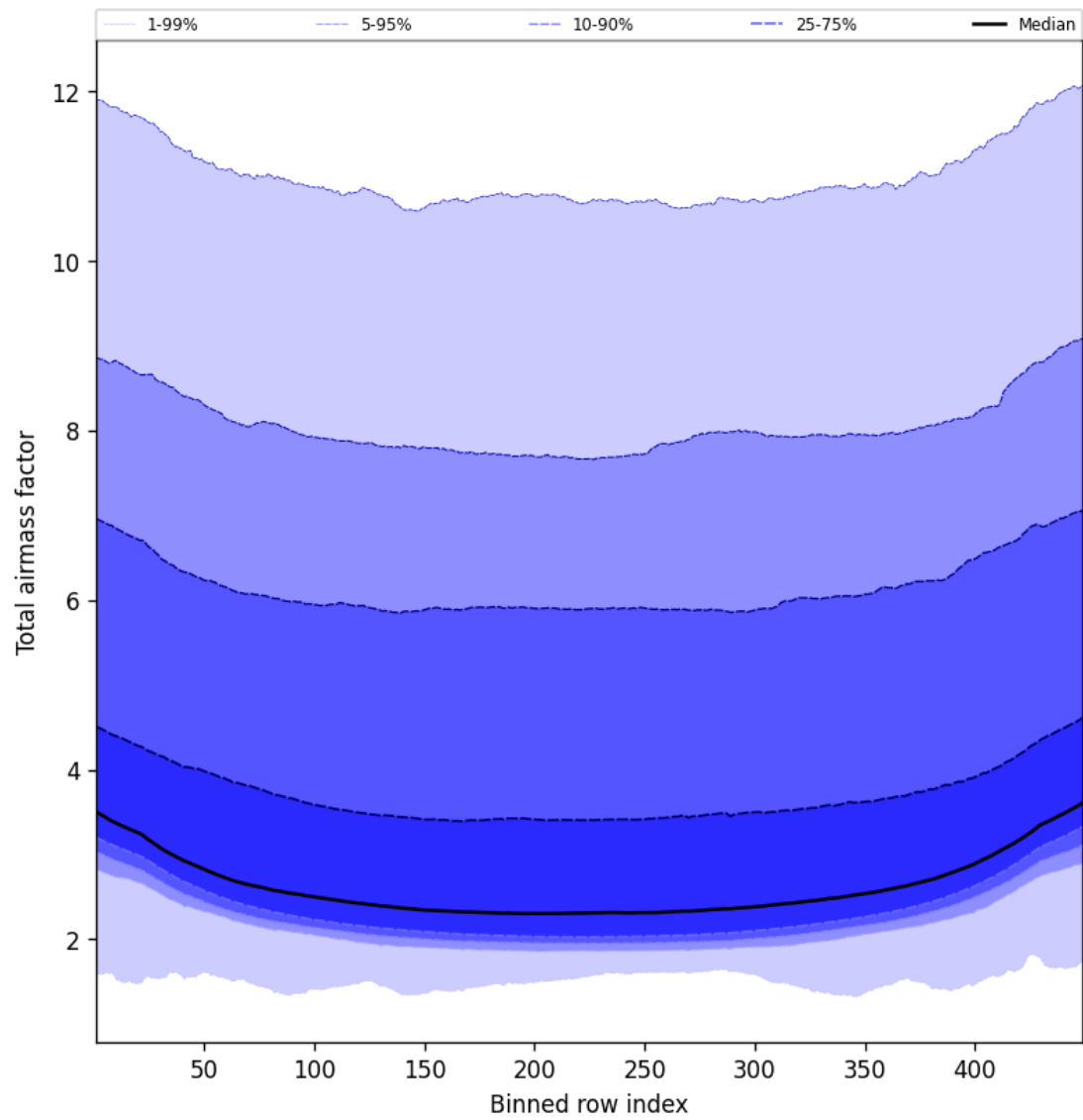
Figure 47: Along track statistics of “Total airmass factor” for 2025-02-06 to 2025-02-06
