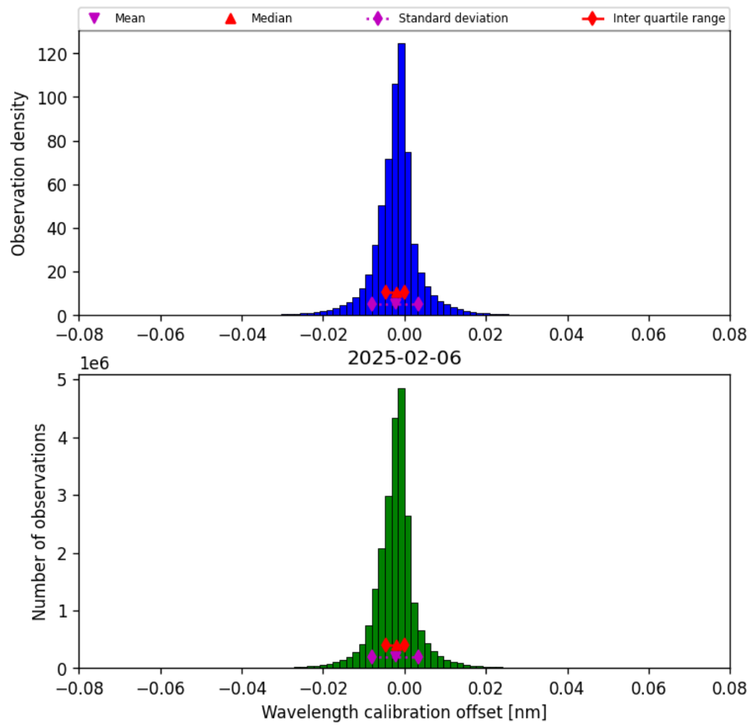
Figure 33: Histogram of “Wavelength calibration offset” for 2025-02-06 to 2025-02-06
