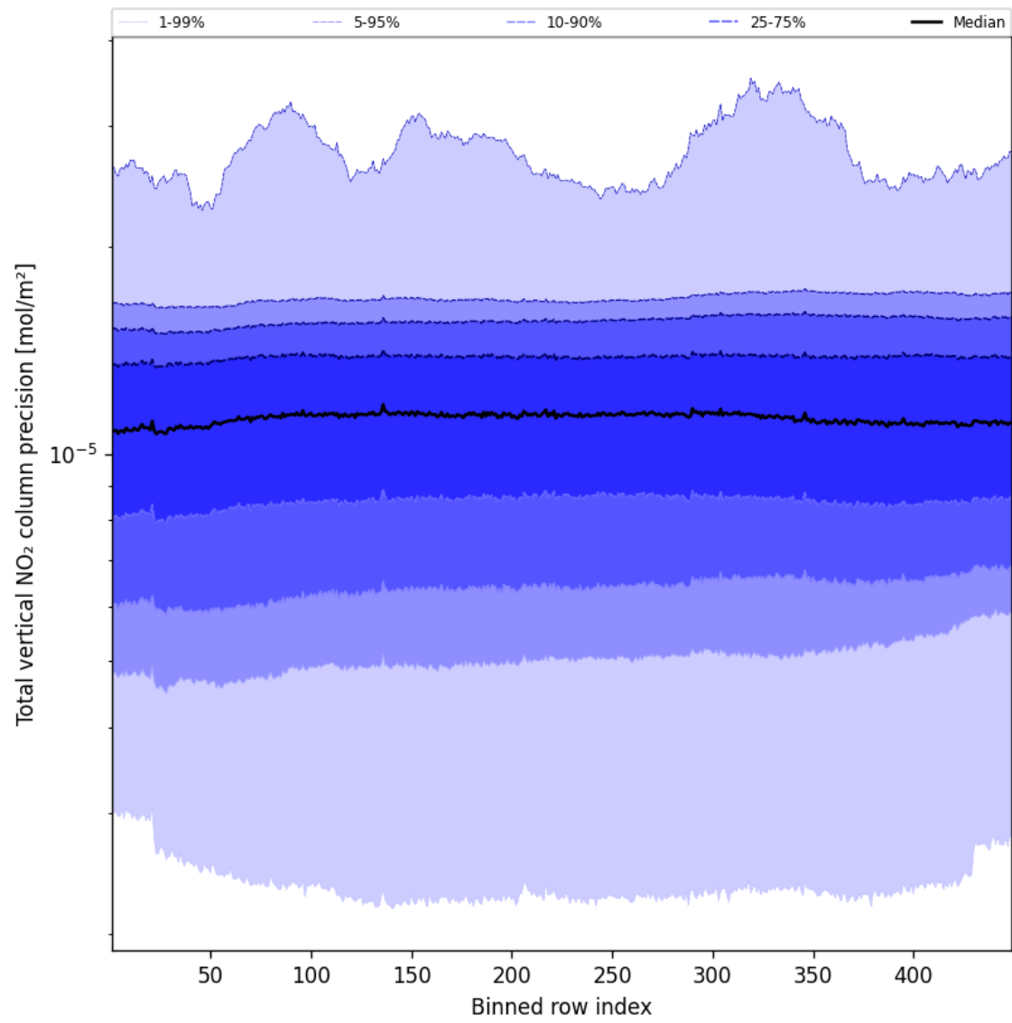
Figure 54: Along track statistics of “Total vertical NO 2 column precision” for 2025-02-06 to 2025-02-06
