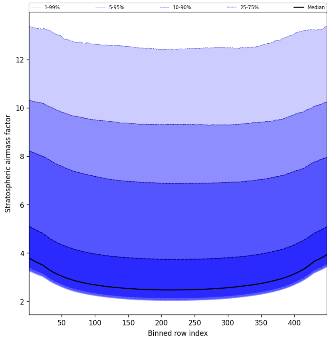
Figure 59: Along track statistics of “Stratospheric airmass factor” for 2025-02-06 to 2025-02-06
