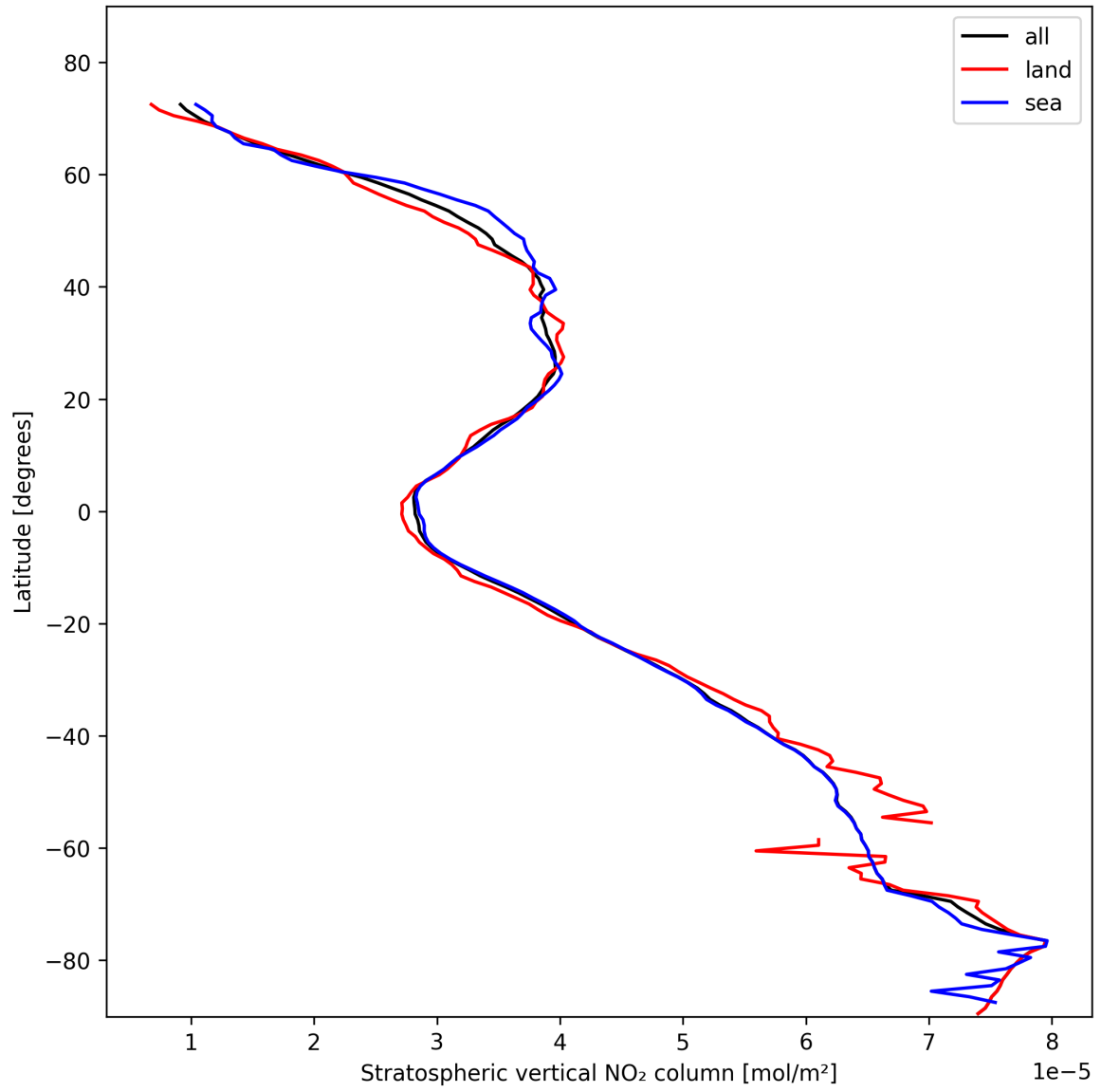
Figure 17: Zonal average of “Stratospheric vertical NO 2 column” for 2025-02-06 to 2025-02-06.
