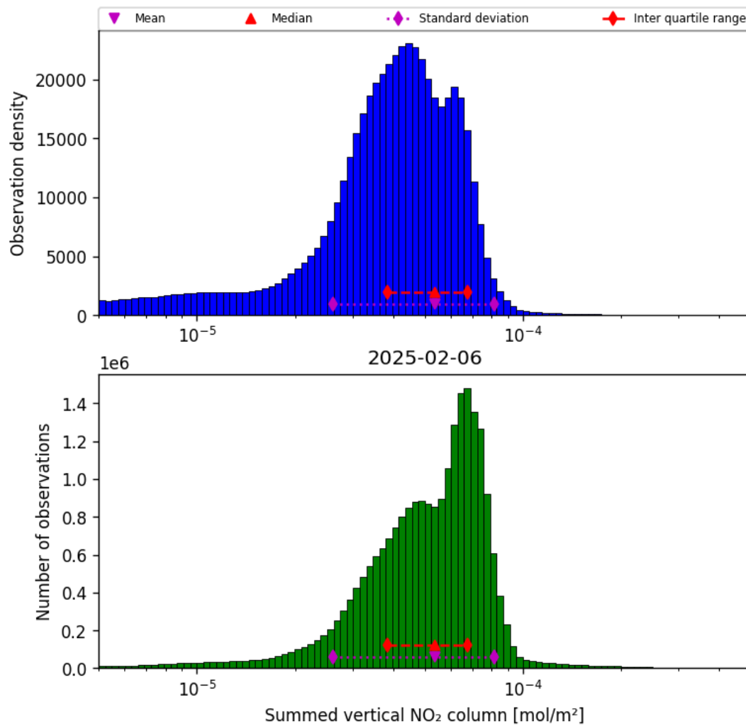
Figure 38: Histogram of “Summed vertical NO 2 column” for 2025-02-06 to 2025-02-06
