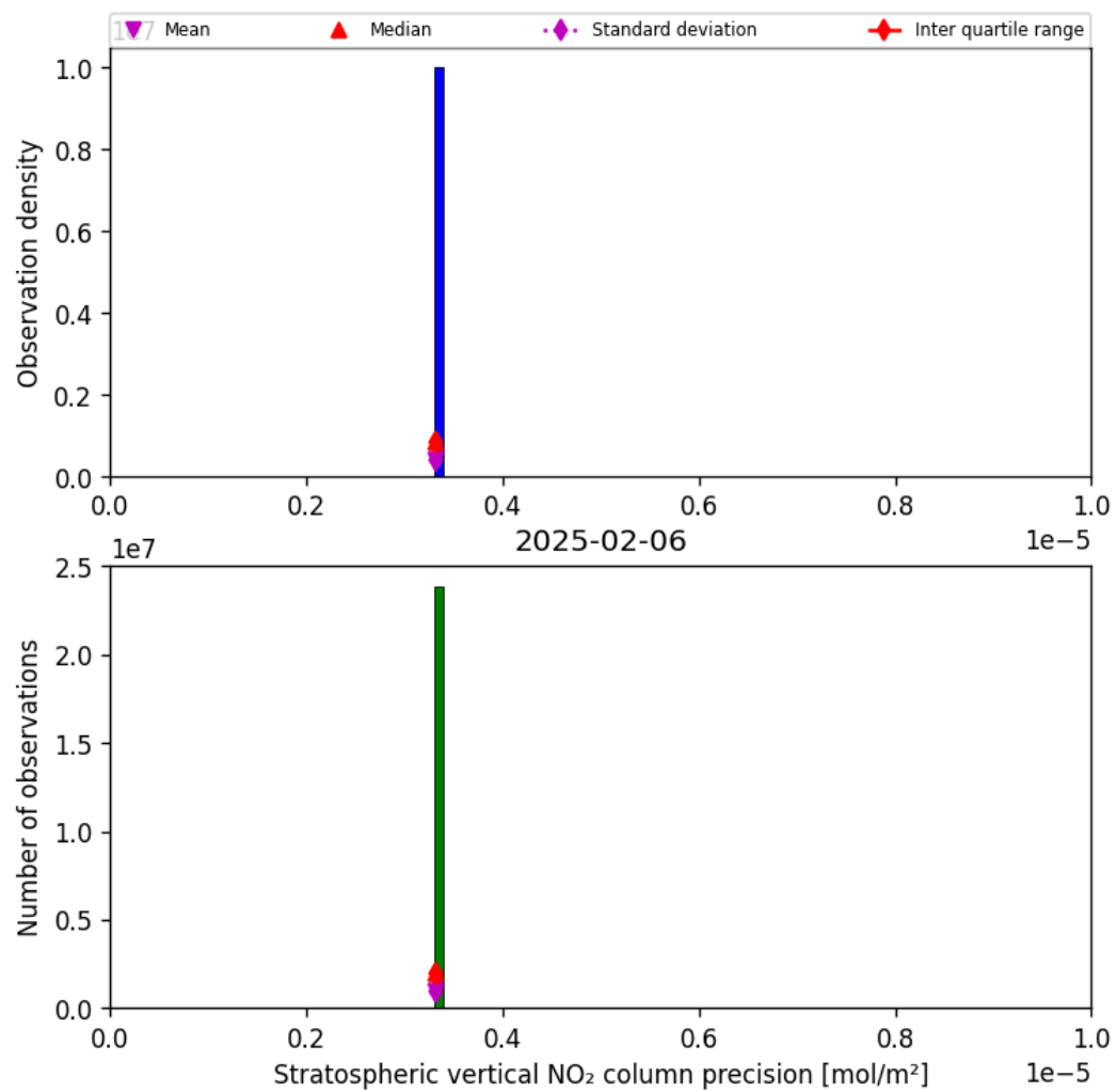
Figure 35: Histogram of “Stratospheric vertical NO 2 column precision” for 2025-02-06 to 2025-02-06
