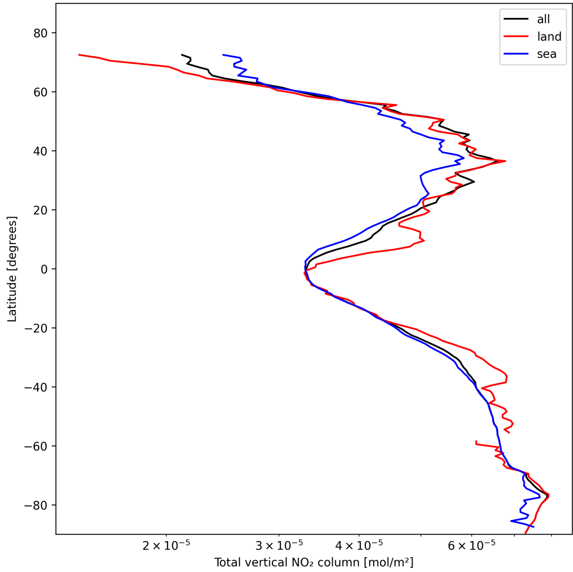
Figure 19: Zonal average of “Total vertical NO 2 column” for 2025-02-06 to 2025-02-06.
