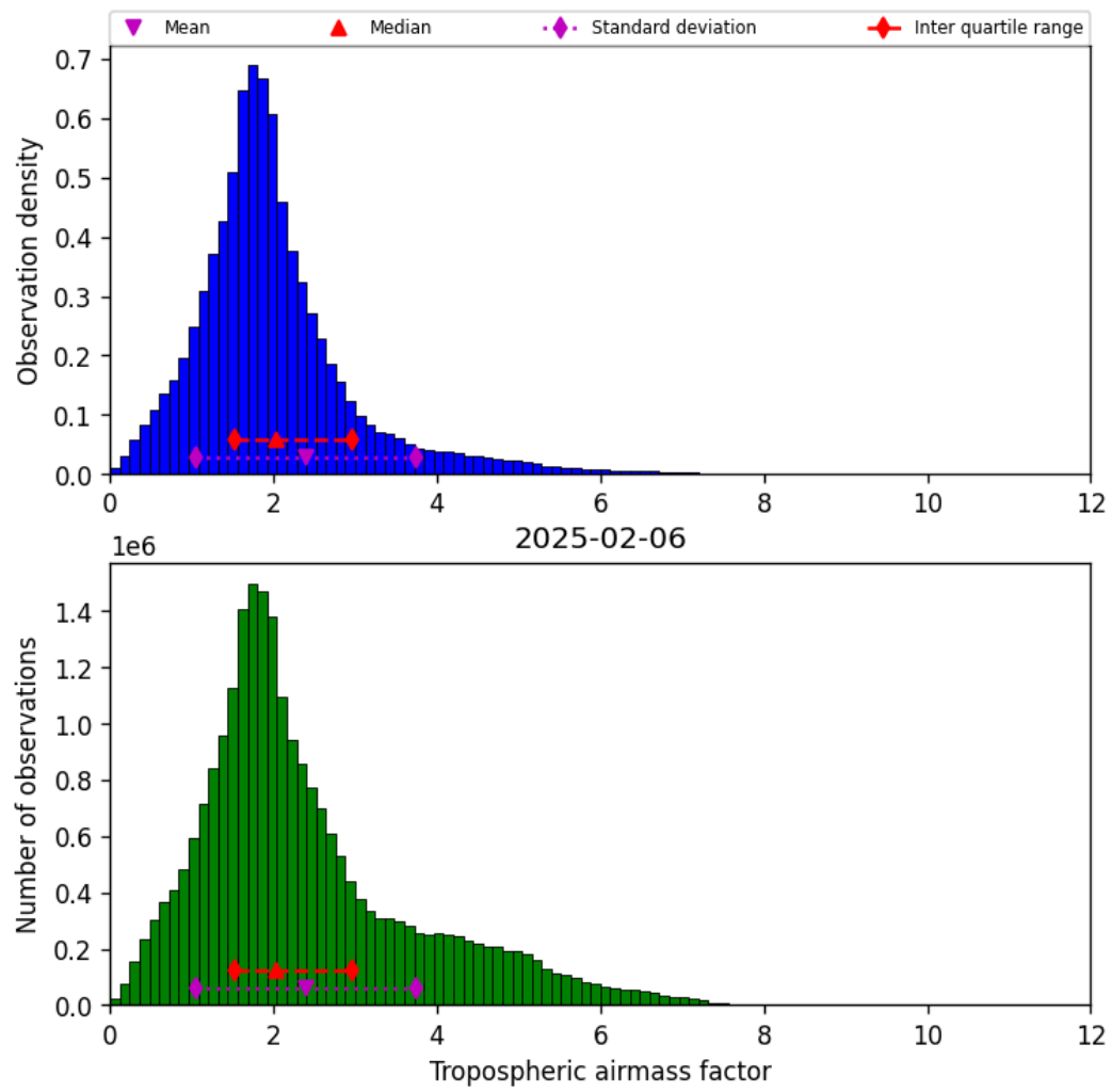
Figure 29: Histogram of “Tropospheric airmass factor” for 2025-02-06 to 2025-02-06
