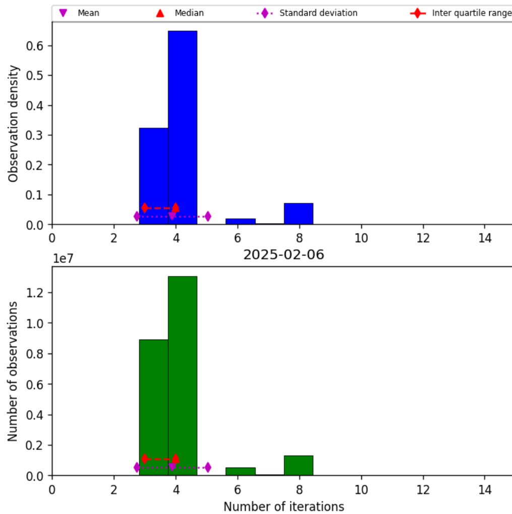
Figure 32: Histogram of “Number of iterations” for 2025-02-06 to 2025-02-06
