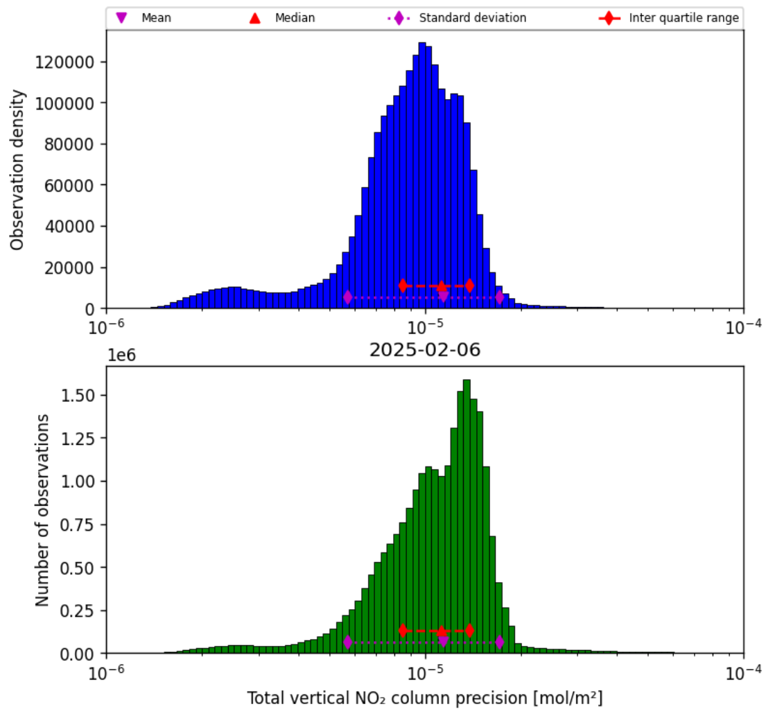
Figure 37: Histogram of “Total vertical NO 2 column precision” for 2025-02-06 to 2025-02-06
