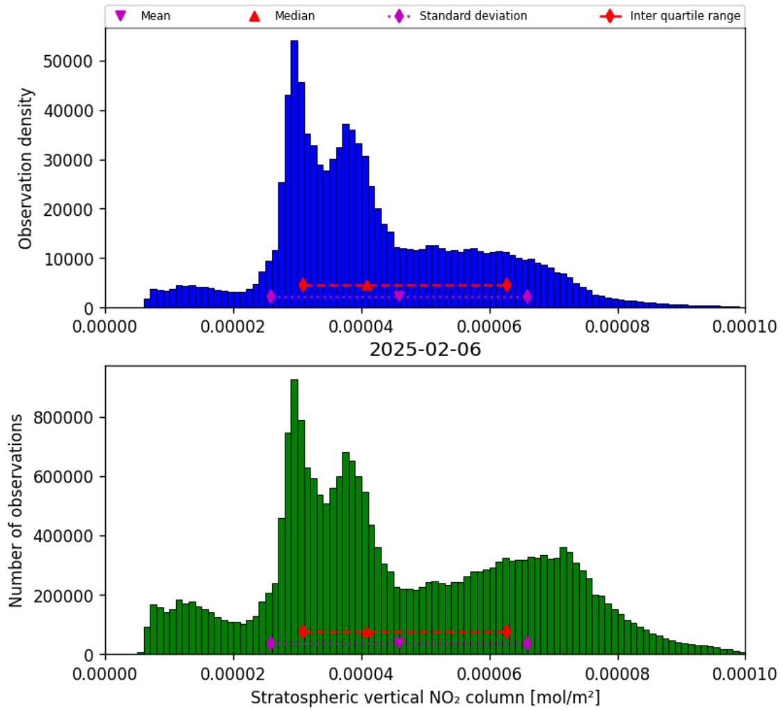
Figure 34: Histogram of “Stratospheric vertical NO 2 column” for 2025-02-06 to 2025-02-06
