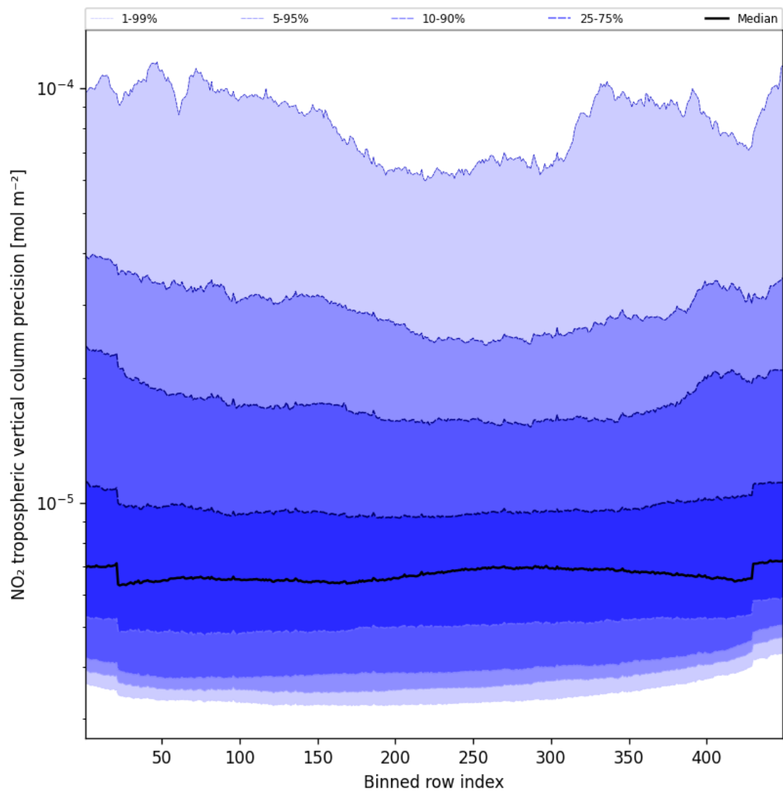
Figure 45: Along track statistics of “NO 2 tropospheric vertical column precision” for 2025-02-06 to 2025-02-06
