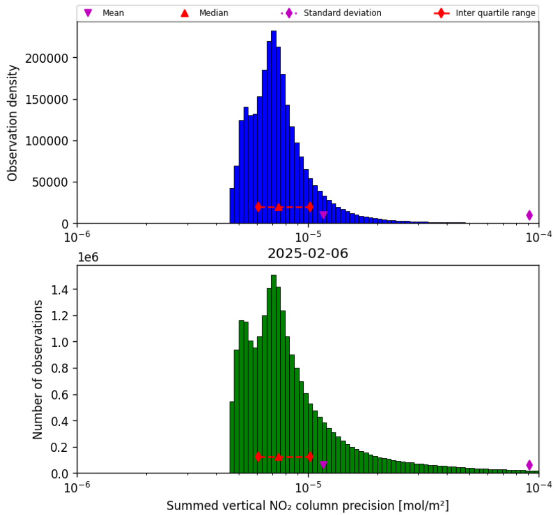
Figure 39: Histogram of "Summed vertical NO 2 column precision" for 2025-02-06 to 2025-02-06
