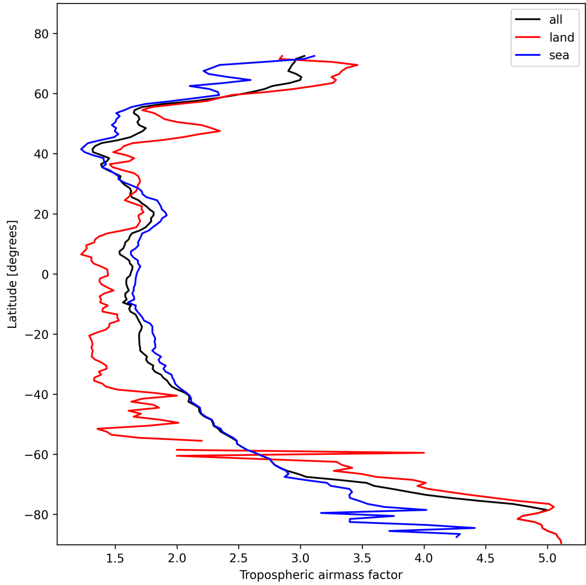
Figure 12: Zonal average of “Tropospheric airmass factor” for 2025-02-06 to 2025-02-06.
