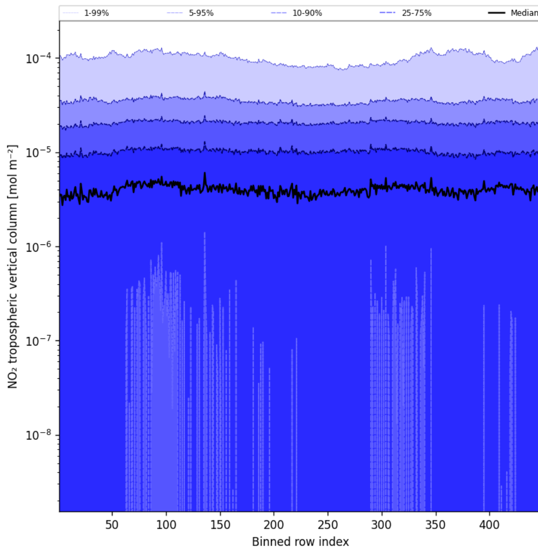
Figure 44: Along track statistics of “NO 2 tropospheric vertical column” for 2025-02-06 to 2025-02-06
