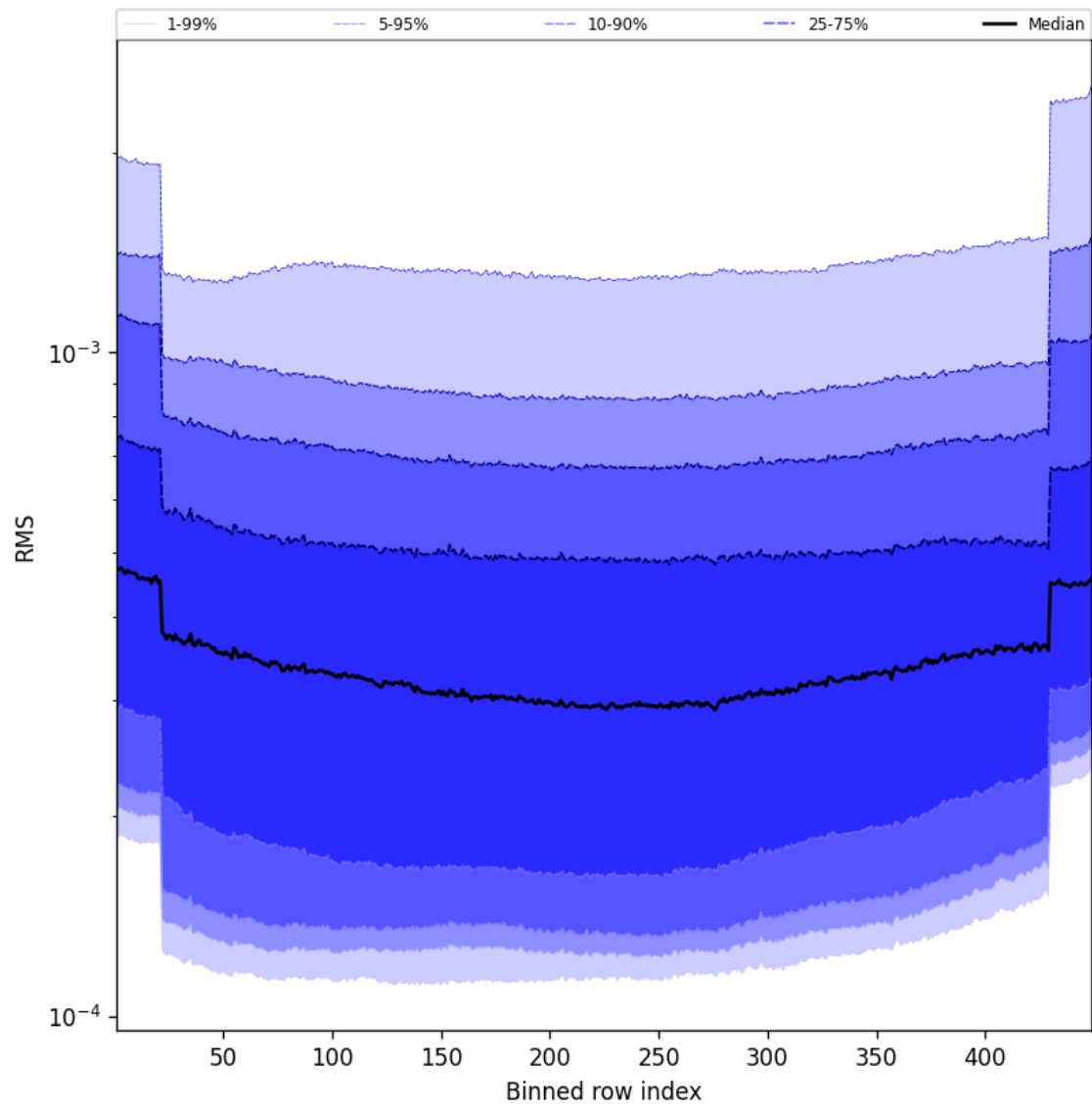
Figure 58: Along track statistics of “RMS” for 2025-02-06 to 2025-02-06
