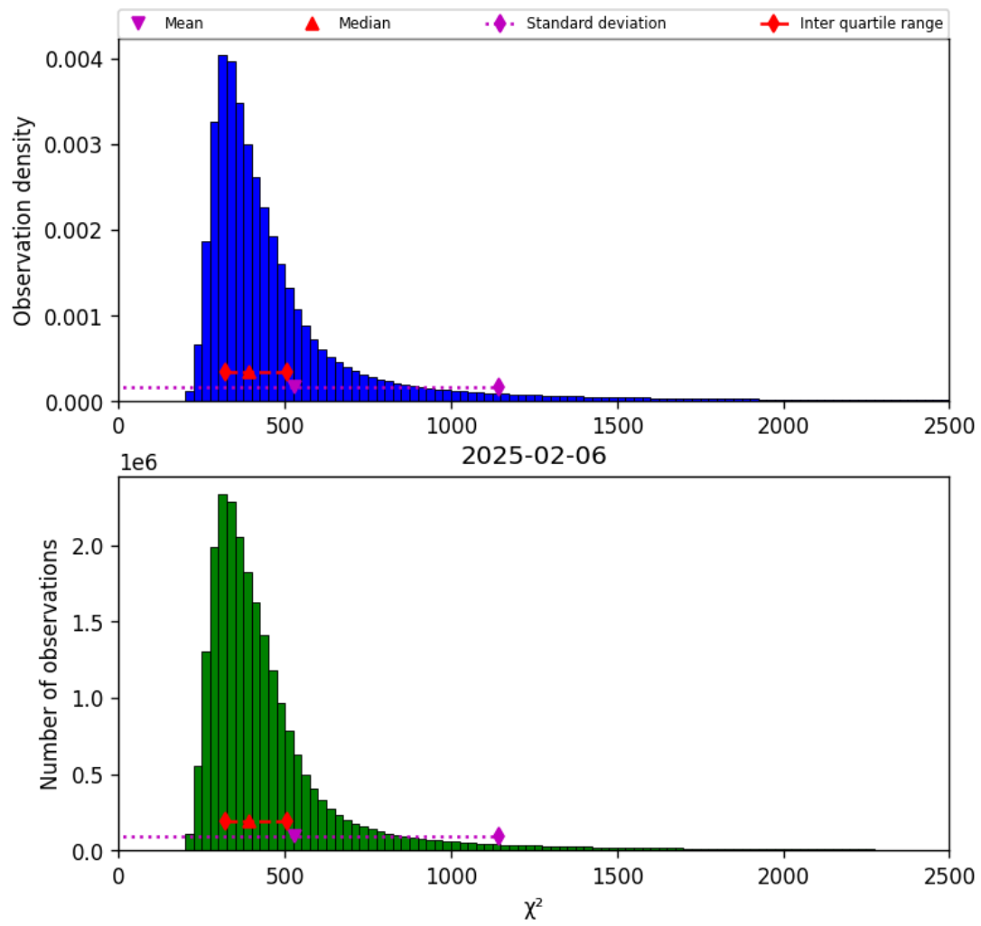
Figure 40: Histogram of “ \chi^2 ” for 2025-02-06 to 2025-02-06
