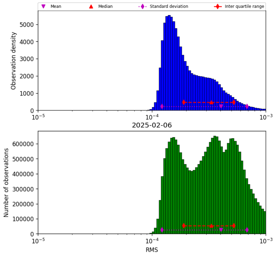
Figure 41: Histogram of “RMS” for 2025-02-06 to 2025-02-06
