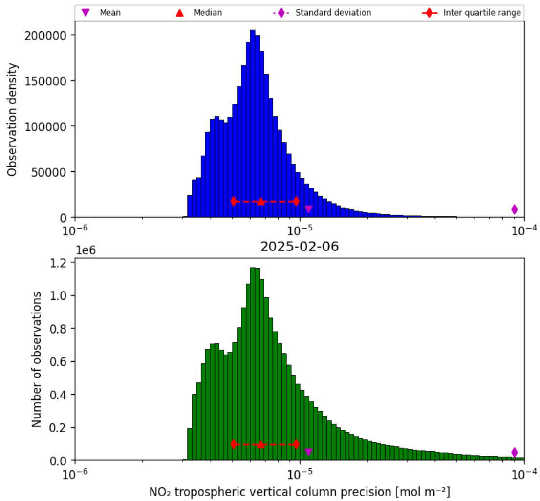
Figure 28: Histogram of "NO 2 tropospheric vertical column precision" for 2025-02-06 to 2025-02-06
