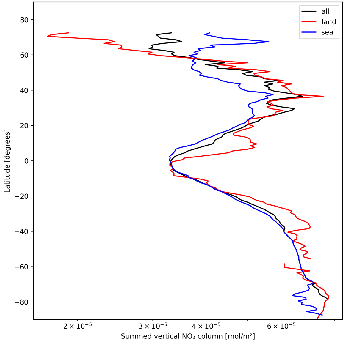
Figure 21: Zonal average of “Summed vertical NO 2 column” for 2025-02-06 to 2025-02-06.
