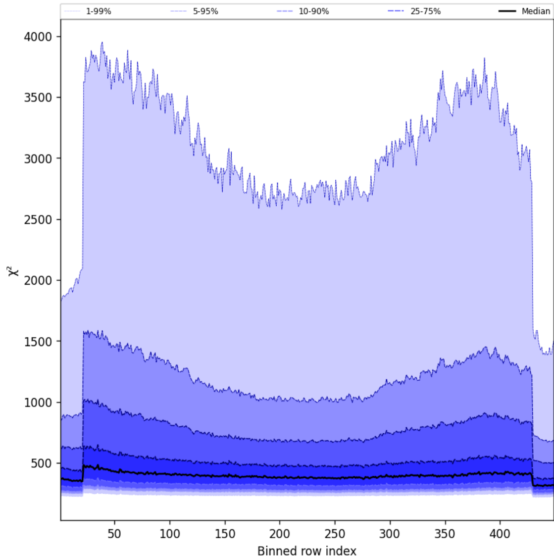
Figure 57: Along track statistics of “ \chi^2 ” for 2025-02-06 to 2025-02-06
