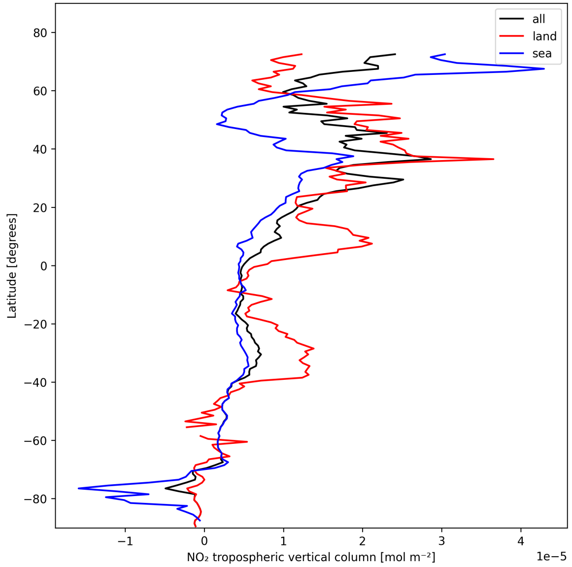
Figure 10: Zonal average of “NO 2 tropospheric vertical column” for 2025-02-06 to 2025-02-06.
