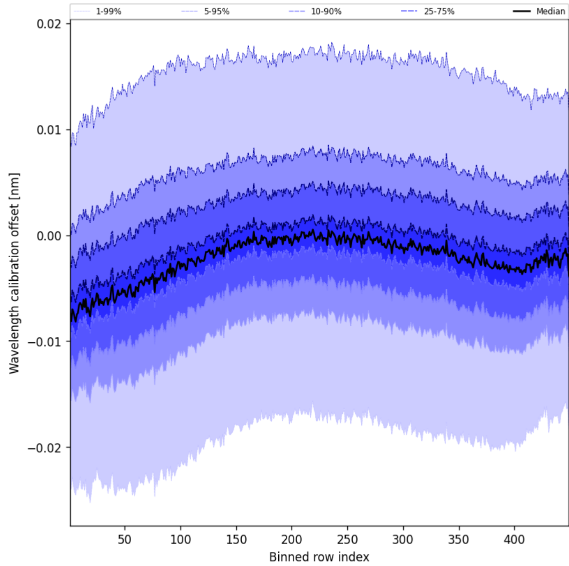
Figure 50: Along track statistics of “Wavelength calibration offset” for 2025-02-07 to 2025-02-08
