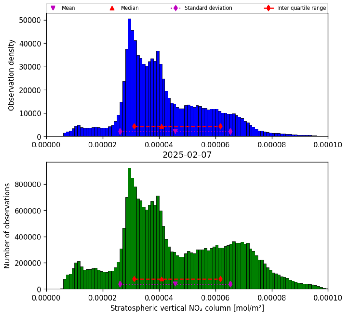
Figure 34: Histogram of “Stratospheric vertical NO 2 column” for 2025-02-07 to 2025-02-08
