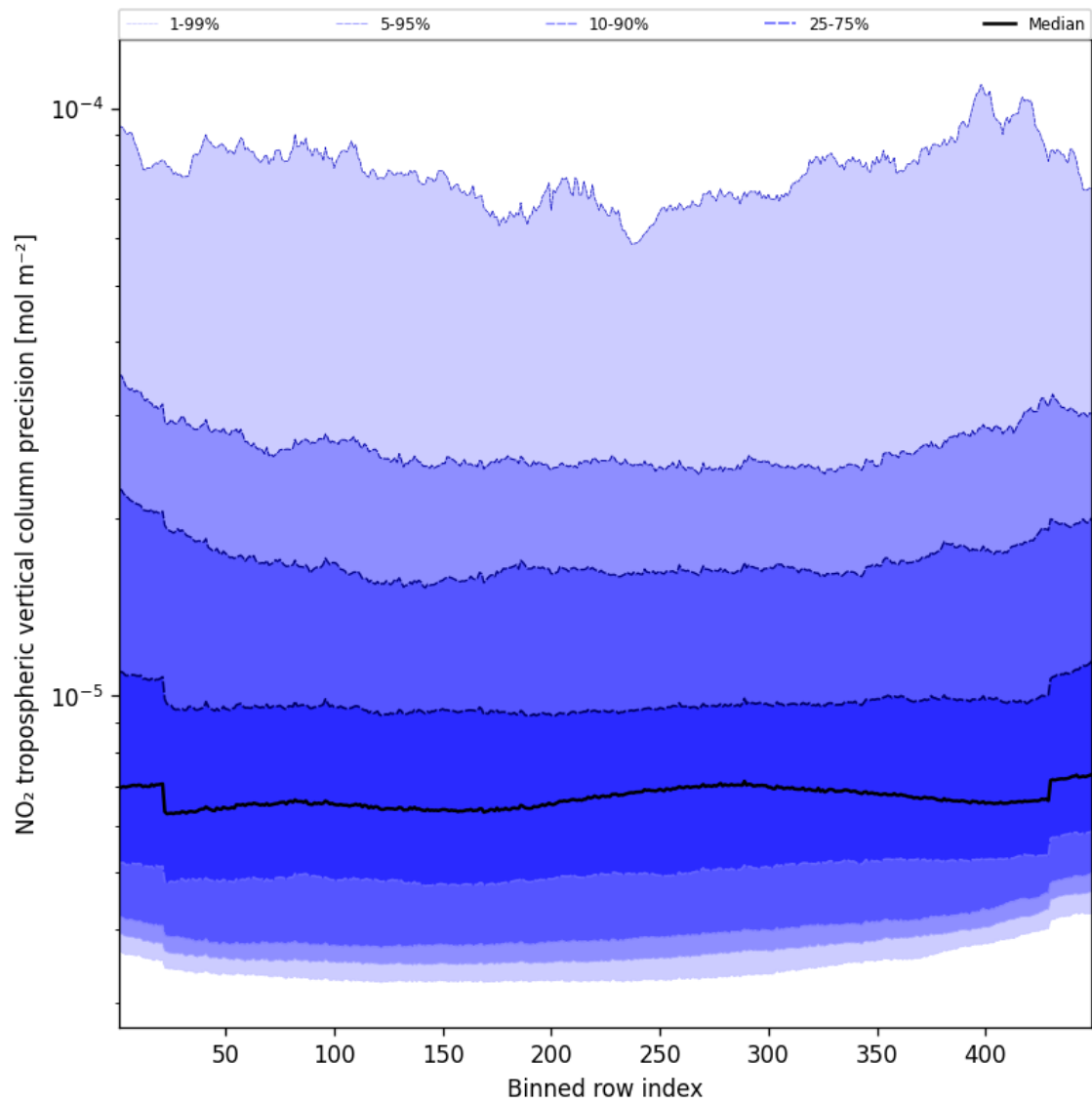
Figure 45: Along track statistics of “NO 2 tropospheric vertical column precision” for 2025-02-07 to 2025-02-08
