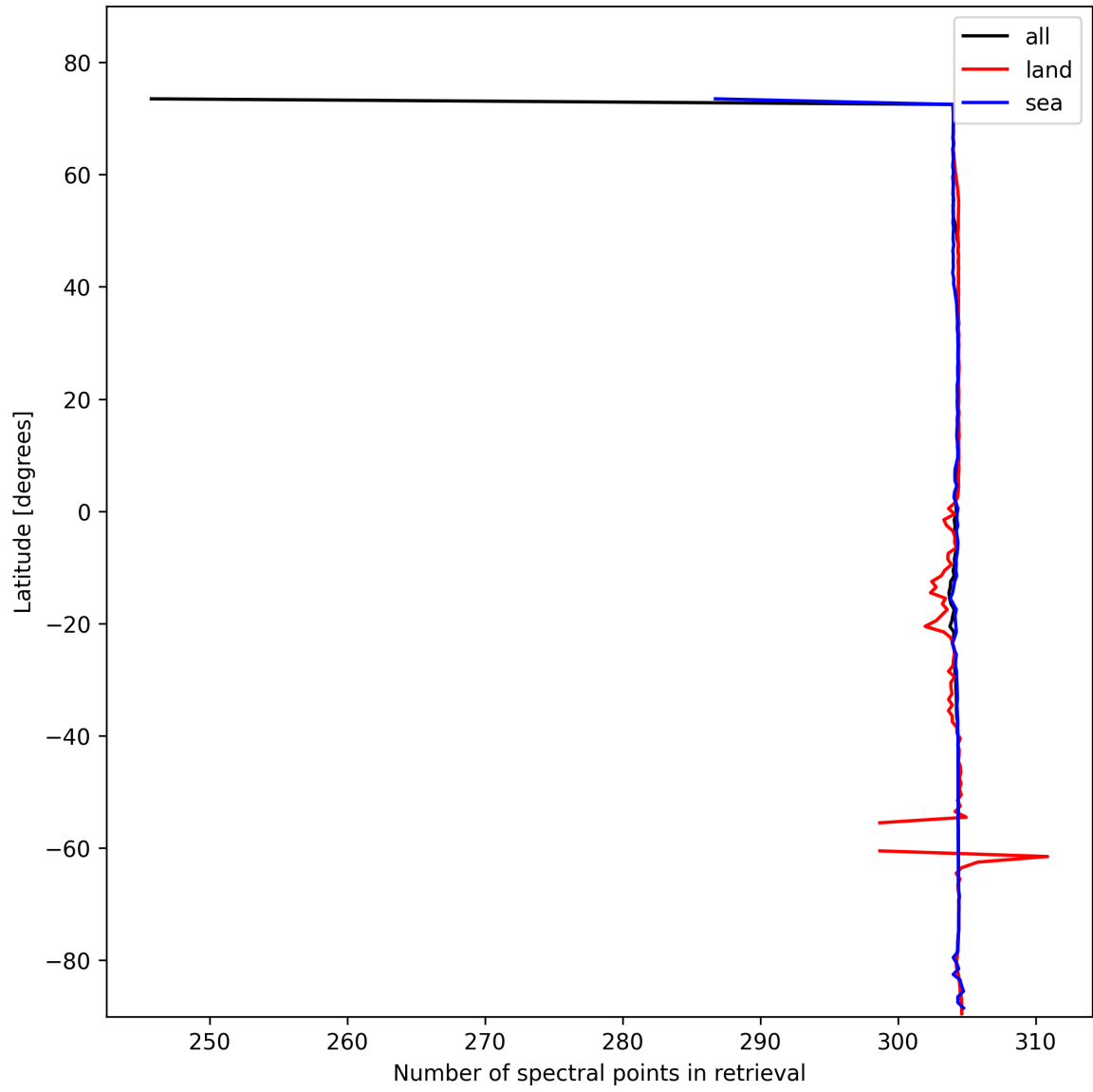
Figure 14: Zonal average of “Number of spectral points in retrieval” for 2025-02-07 to 2025-02-08.
