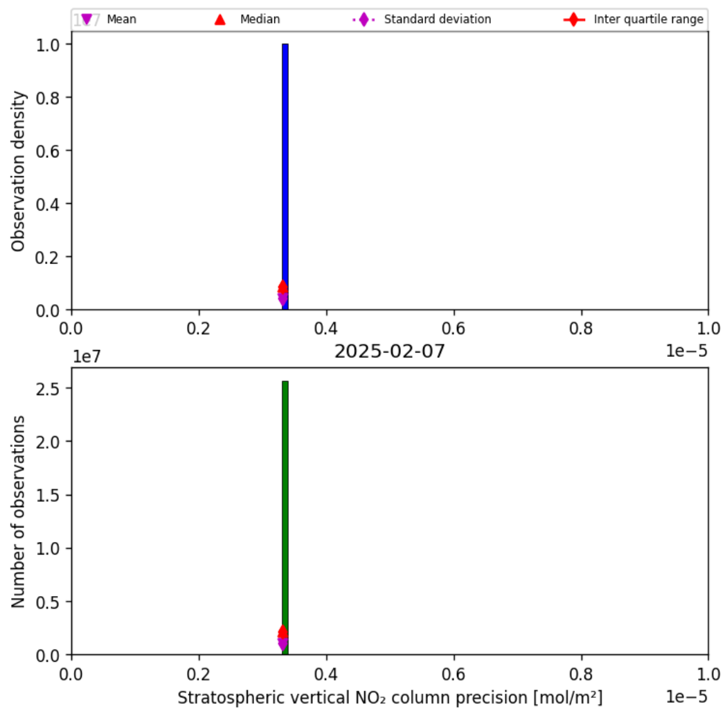
Figure 35: Histogram of “Stratospheric vertical NO 2 column precision” for 2025-02-07 to 2025-02-08
