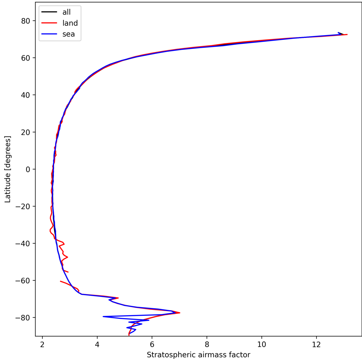
Figure 25: Zonal average of “Stratospheric airmass factor” for 2025-02-07 to 2025-02-08.
