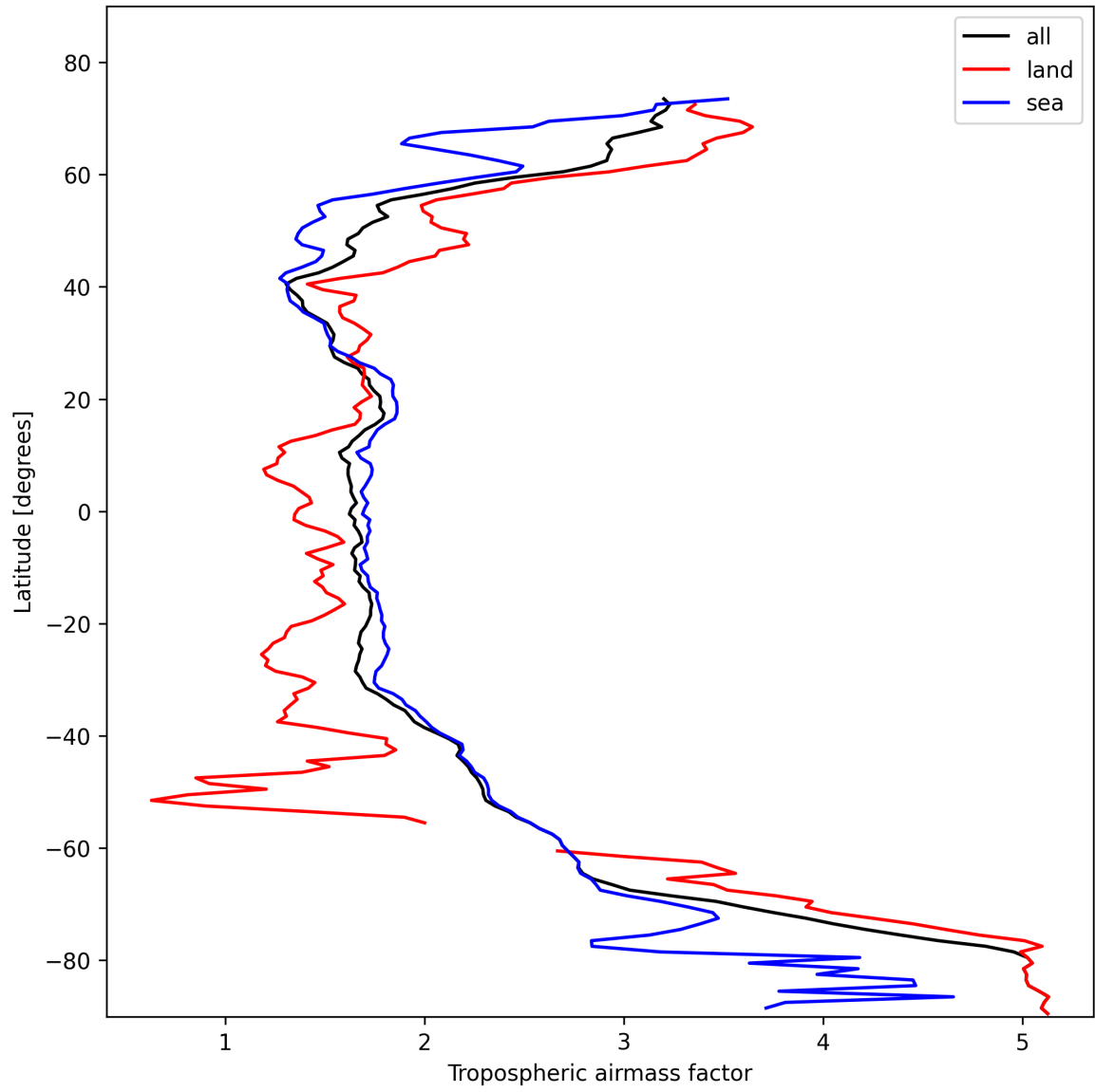
Figure 12: Zonal average of “Tropospheric airmass factor” for 2025-02-07 to 2025-02-08.
