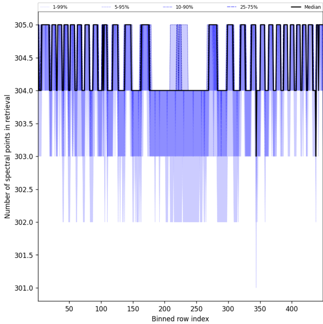
Figure 48: Along track statistics of “Number of spectral points in retrieval” for 2025-02-07 to 2025-02-08
