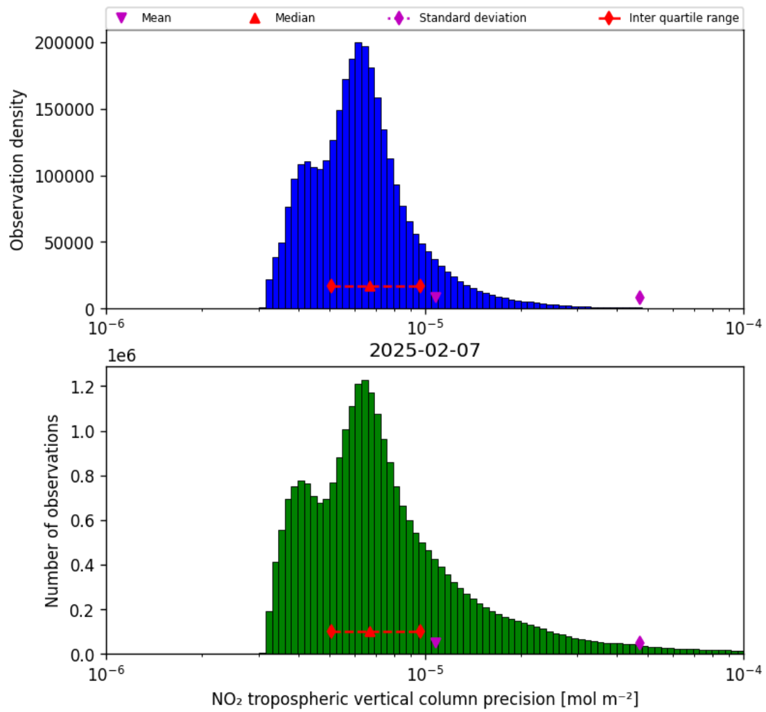
Figure 28: Histogram of “NO 2 tropospheric vertical column precision” for 2025-02-07 to 2025-02-08
