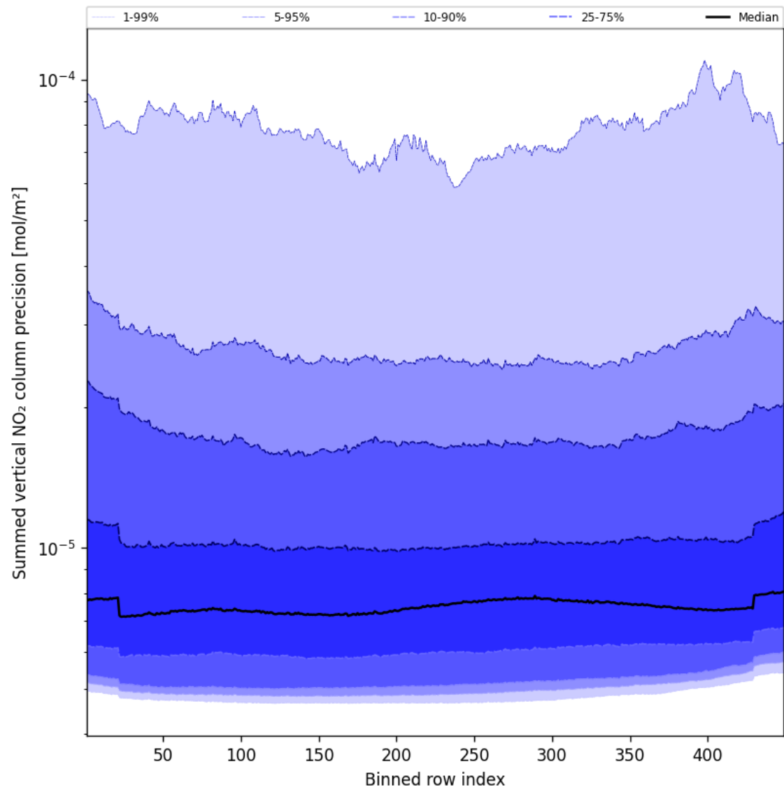
Figure 56: Along track statistics of “Summed vertical NO 2 column precision” for 2025-02-07 to 2025-02-08
