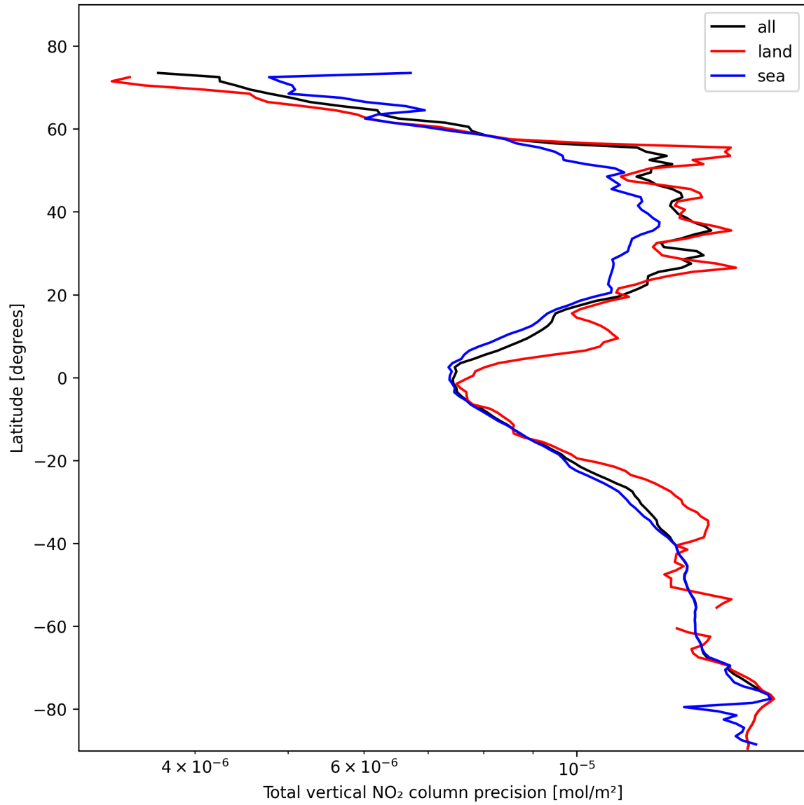
Figure 20: Zonal average of “Total vertical NO 2 column precision” for 2025-02-07 to 2025-02-08.
