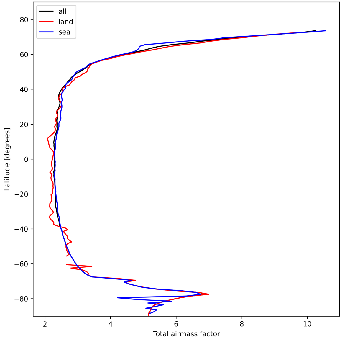
Figure 13: Zonal average of “Total airmass factor” for 2025-02-07 to 2025-02-08.
