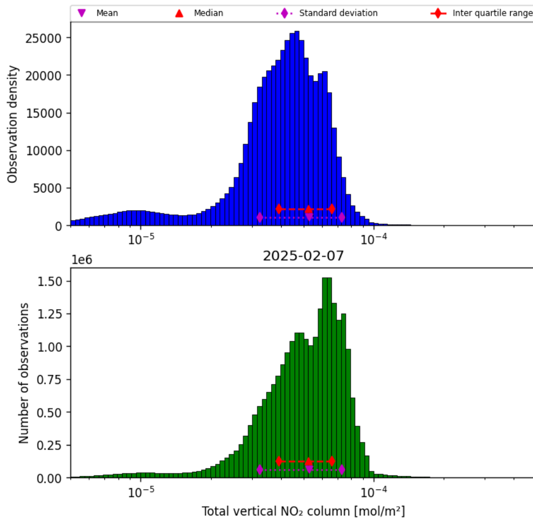
Figure 36: Histogram of “Total vertical NO 2 column” for 2025-02-07 to 2025-02-08
