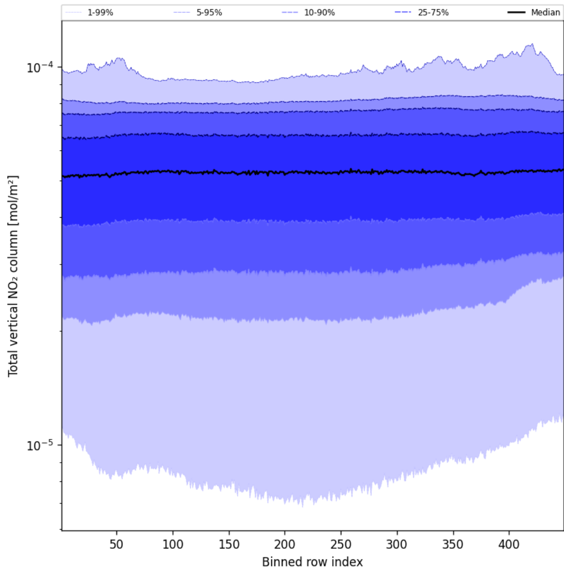
Figure 53: Along track statistics of “Total vertical NO 2 column” for 2025-02-07 to 2025-02-08
