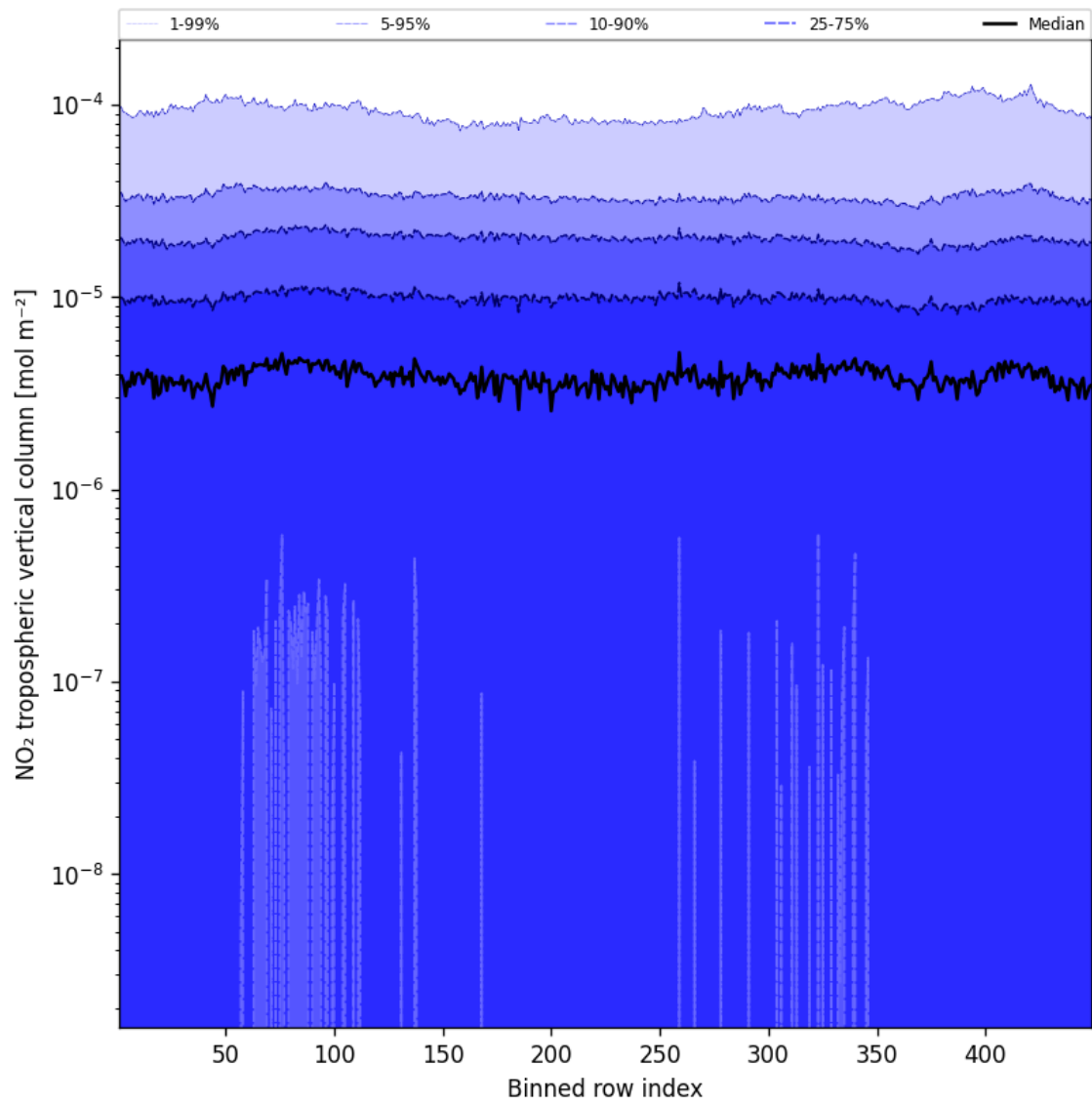
Figure 44: Along track statistics of “NO 2 tropospheric vertical column” for 2025-02-07 to 2025-02-08
