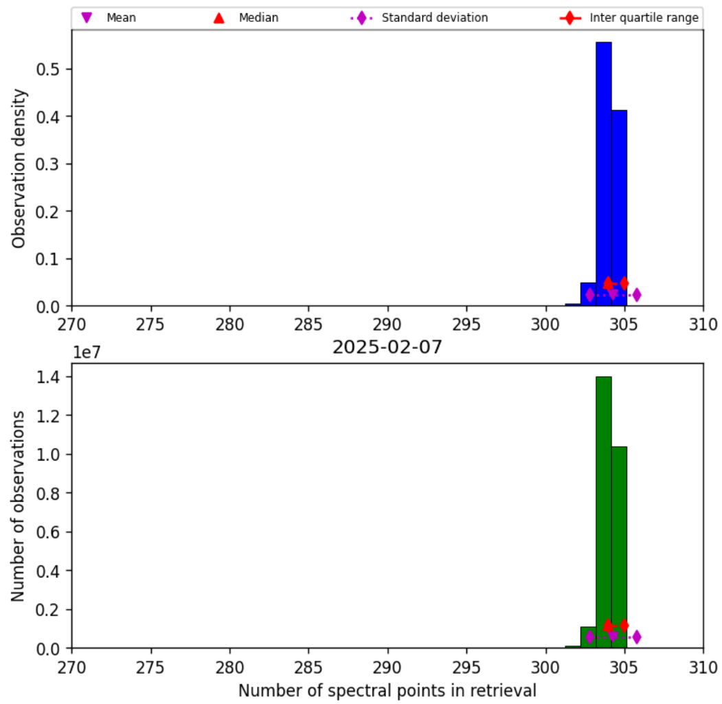
Figure 31: Histogram of “Number of spectral points in retrieval” for 2025-02-07 to 2025-02-08
