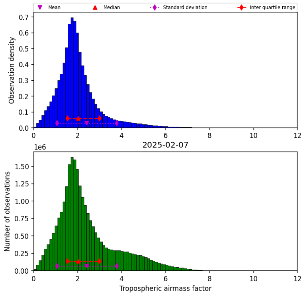
Figure 29: Histogram of “Tropospheric airmass factor” for 2025-02-07 to 2025-02-08
