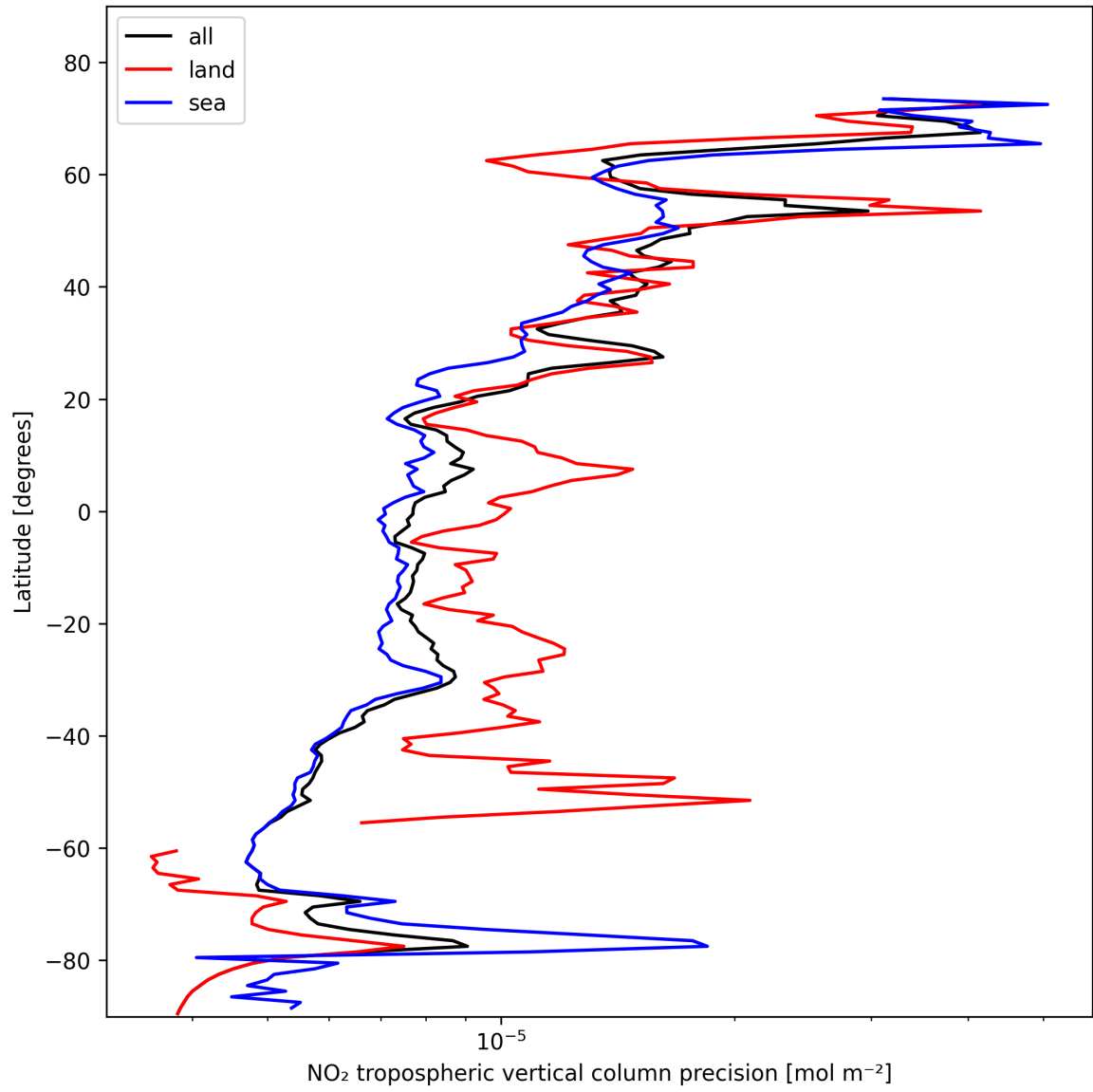
Figure 11: Zonal average of “NO 2 tropospheric vertical column precision” for 2025-02-07 to 2025-02-08.
