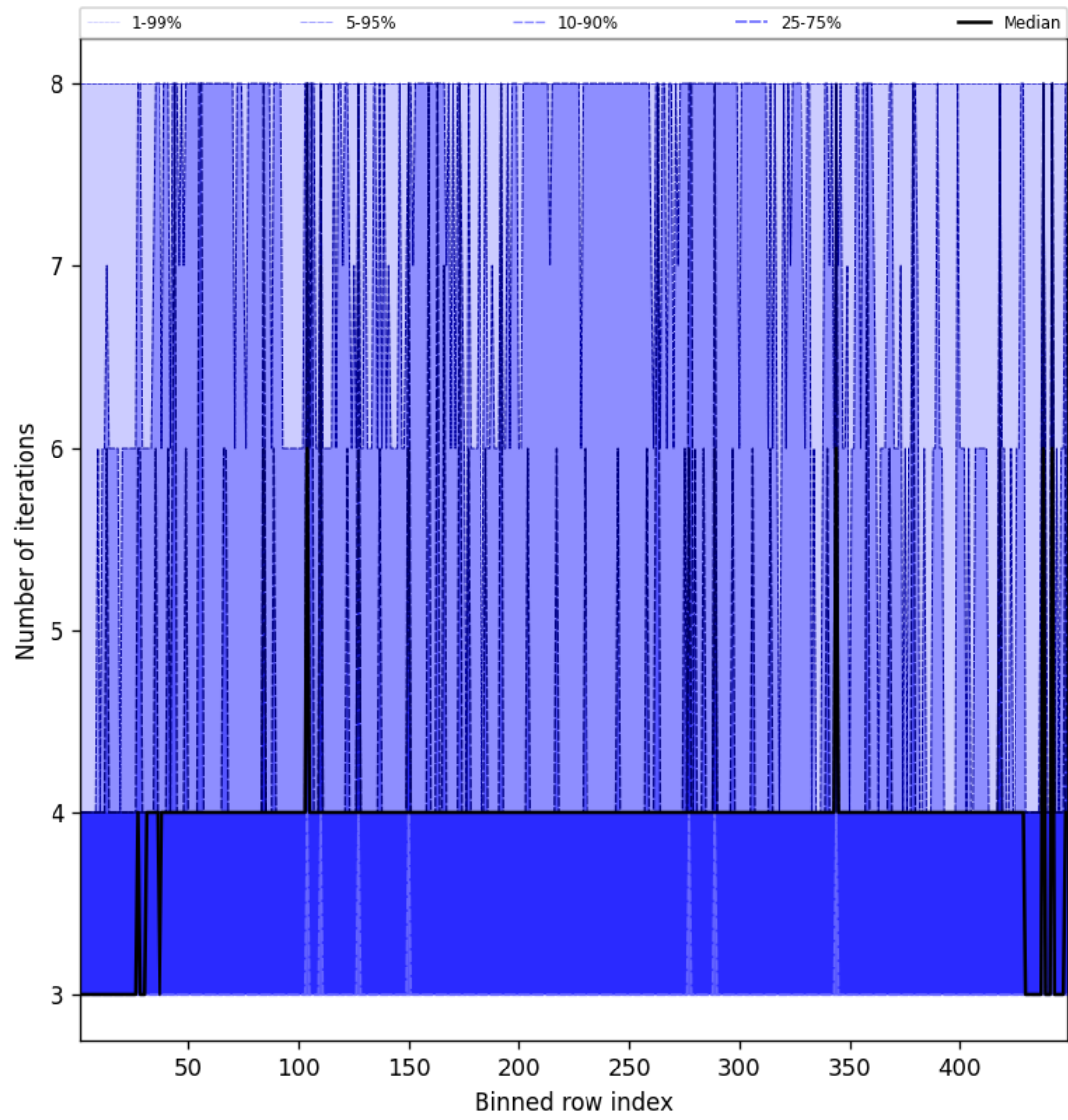
Figure 49: Along track statistics of “Number of iterations” for 2025-02-07 to 2025-02-08
