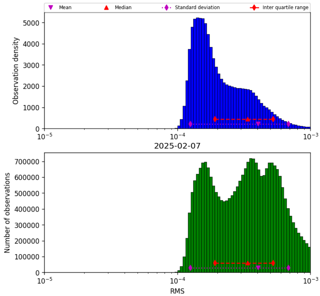
Figure 41: Histogram of “RMS” for 2025-02-07 to 2025-02-08
