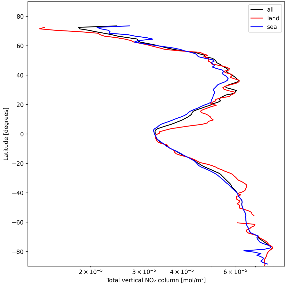
Figure 19: Zonal average of “Total vertical NO 2 column” for 2025-02-07 to 2025-02-08.
