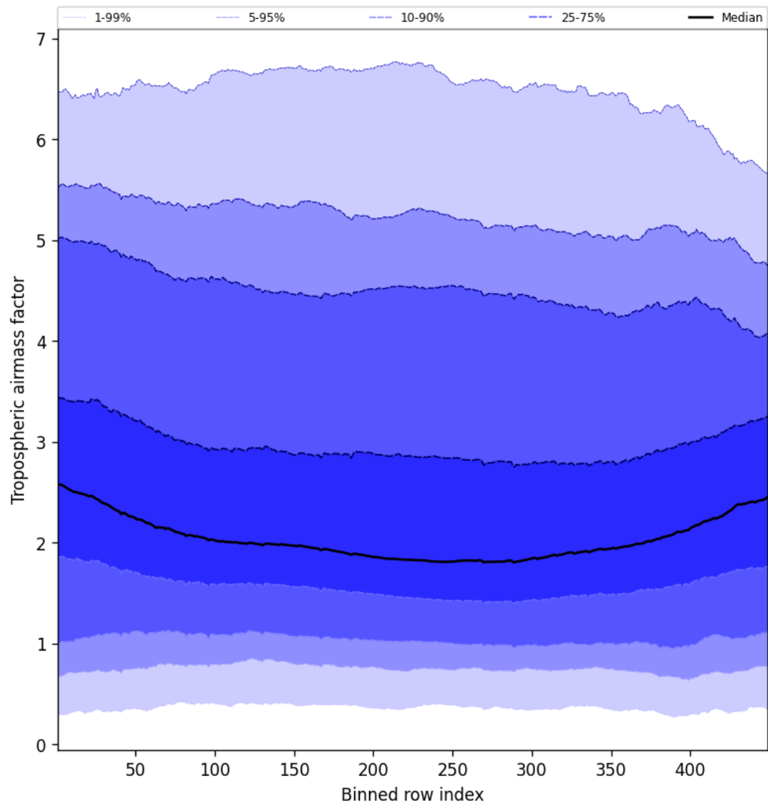
Figure 46: Along track statistics of “Tropospheric air mass factor” for 2025-02-07 to 2025-02-08
