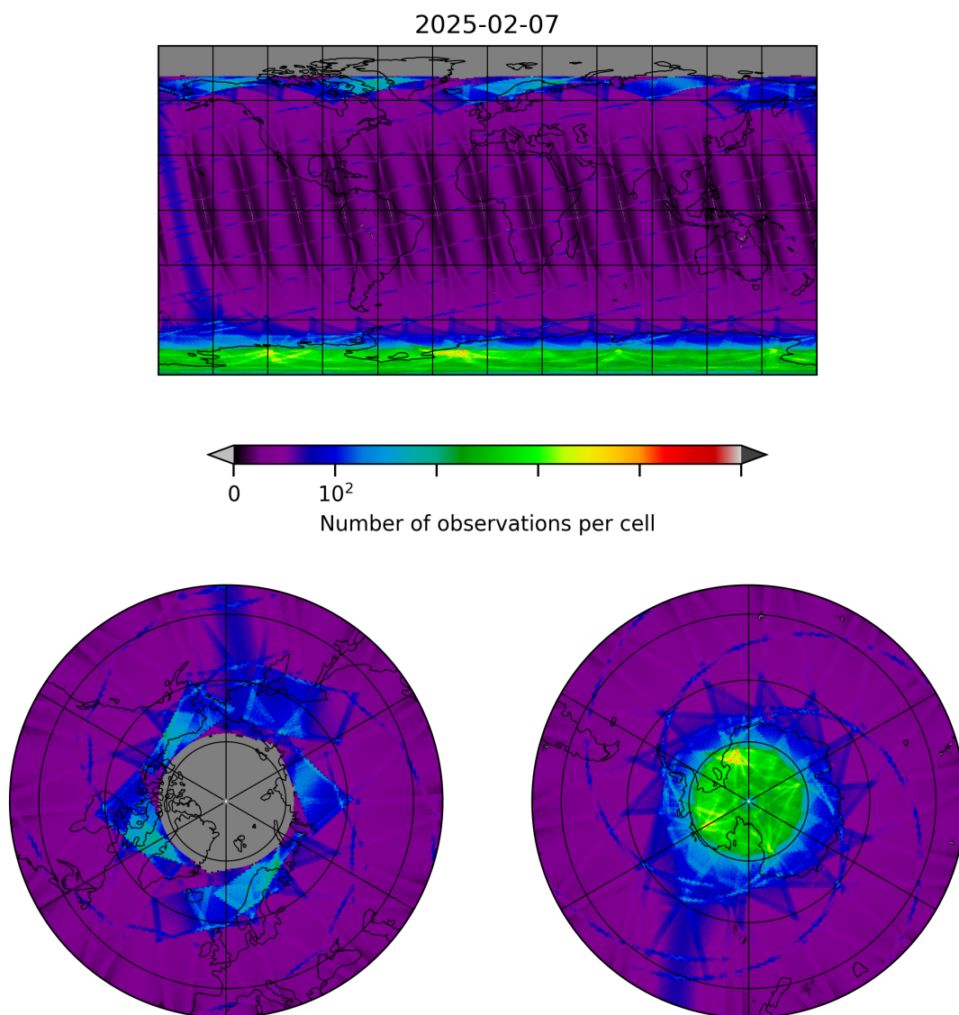
Figure 8: Map of the number of observations for 2025-02-07 to 2025-02-08
