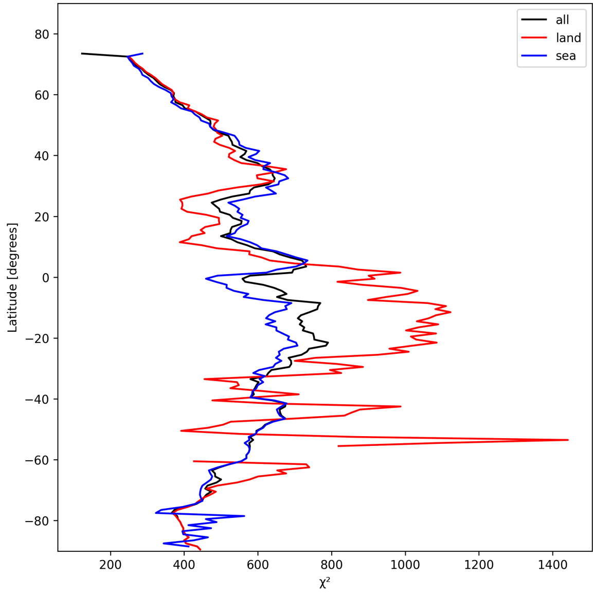
Figure 23: Zonal average of “ \chi^2 ” for 2025-02-07 to 2025-02-08.
