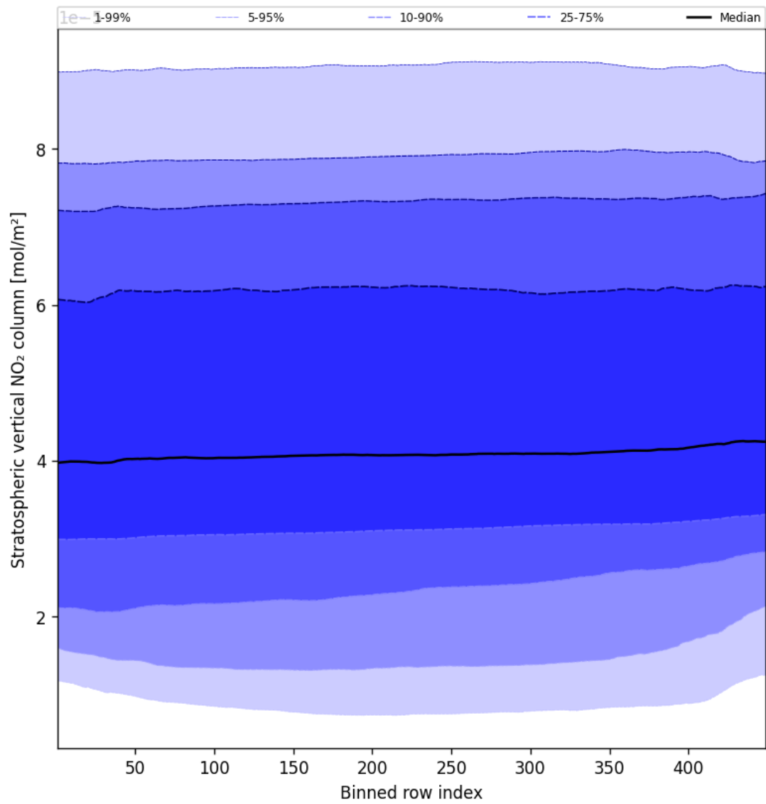
Figure 51: Along track statistics of “Stratospheric vertical NO 2 column” for 2025-02-07 to 2025-02-08
