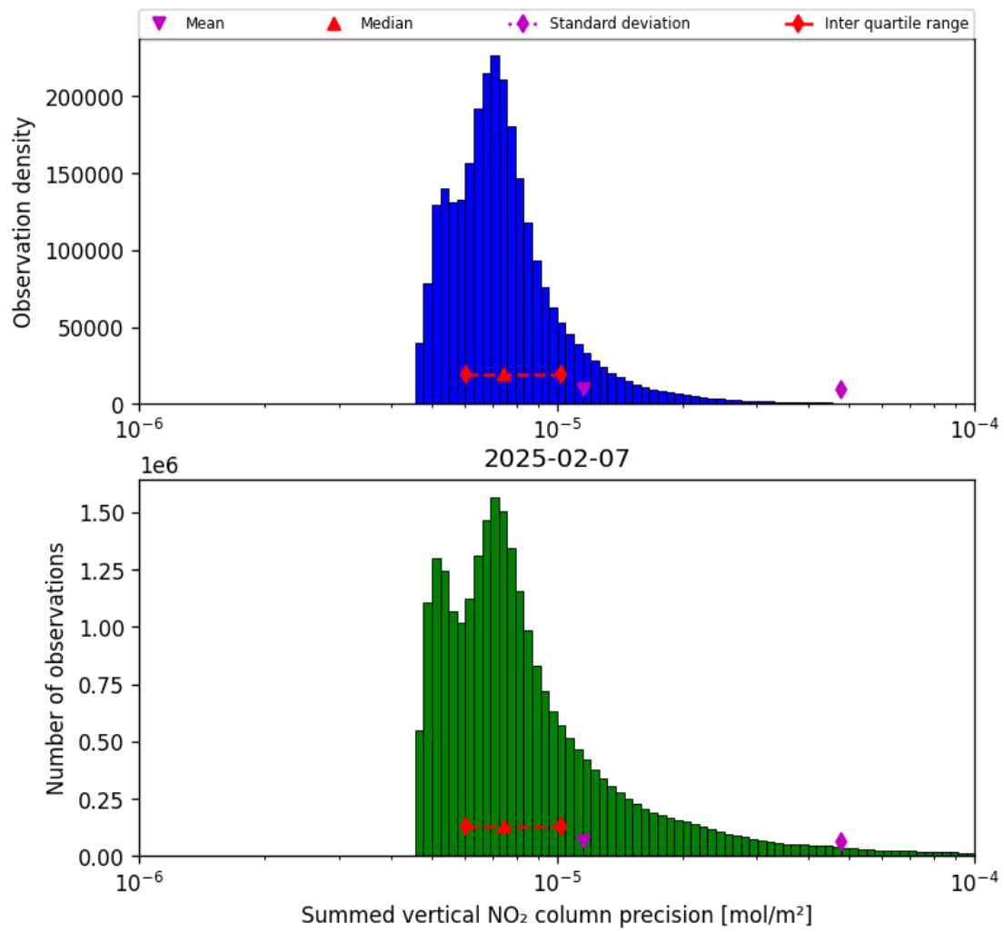
Figure 39: Histogram of “Summed vertical NO 2 column precision” for 2025-02-07 to 2025-02-08
