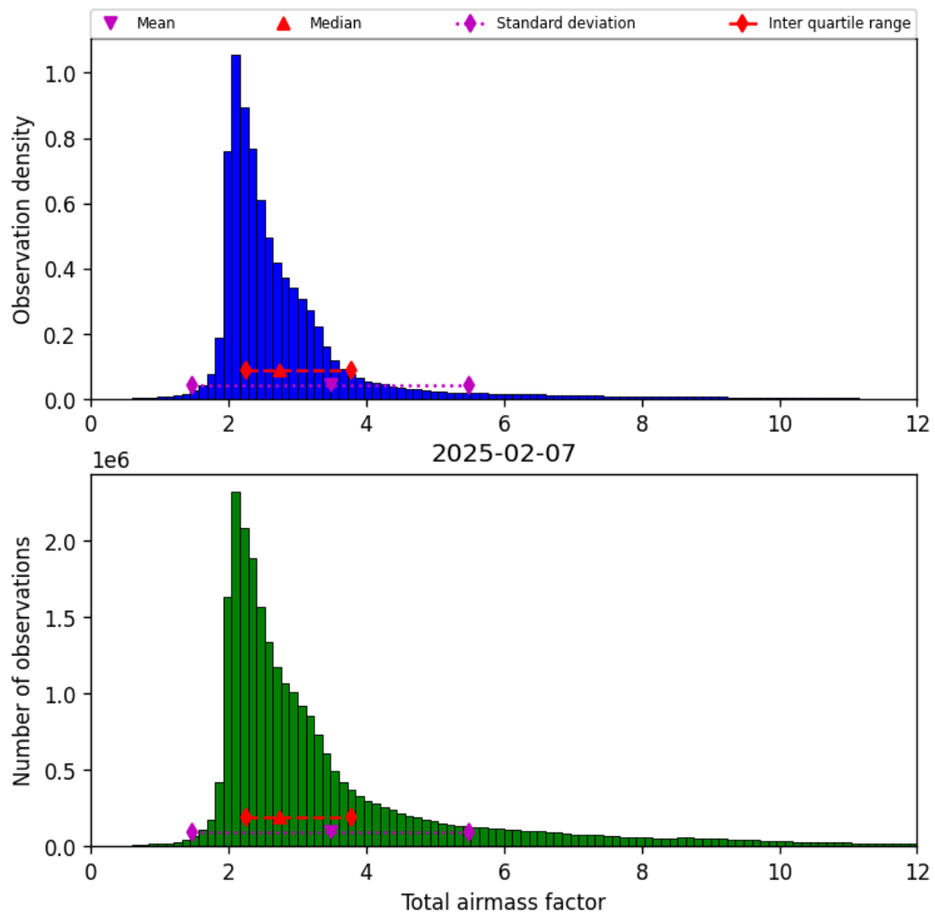
Figure 30: Histogram of “Total airmass factor” for 2025-02-07 to 2025-02-08
