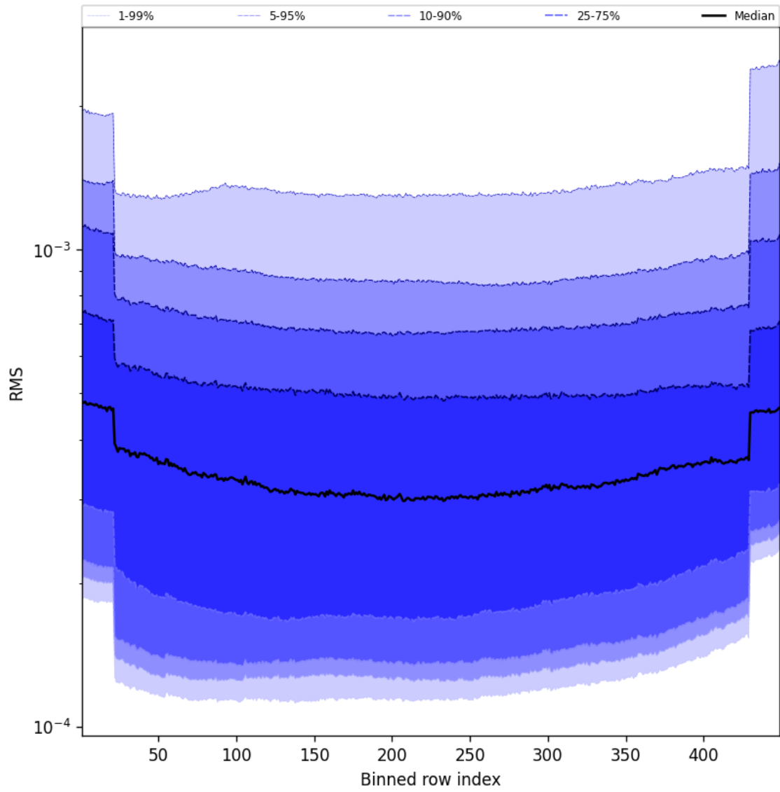
Figure 58: Along track statistics of “RMS” for 2025-02-07 to 2025-02-08
