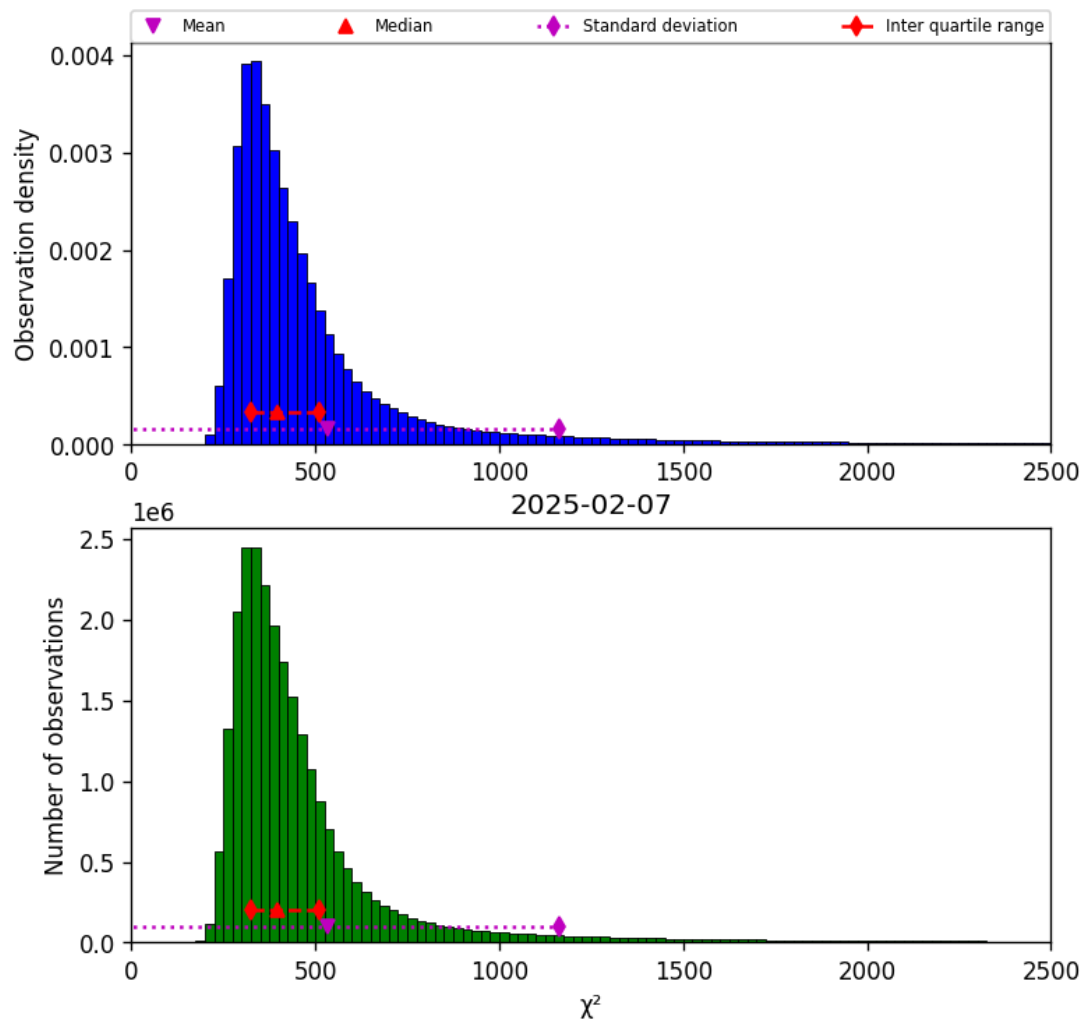
Figure 40: Histogram of “ \chi^2 ” for 2025-02-07 to 2025-02-08
