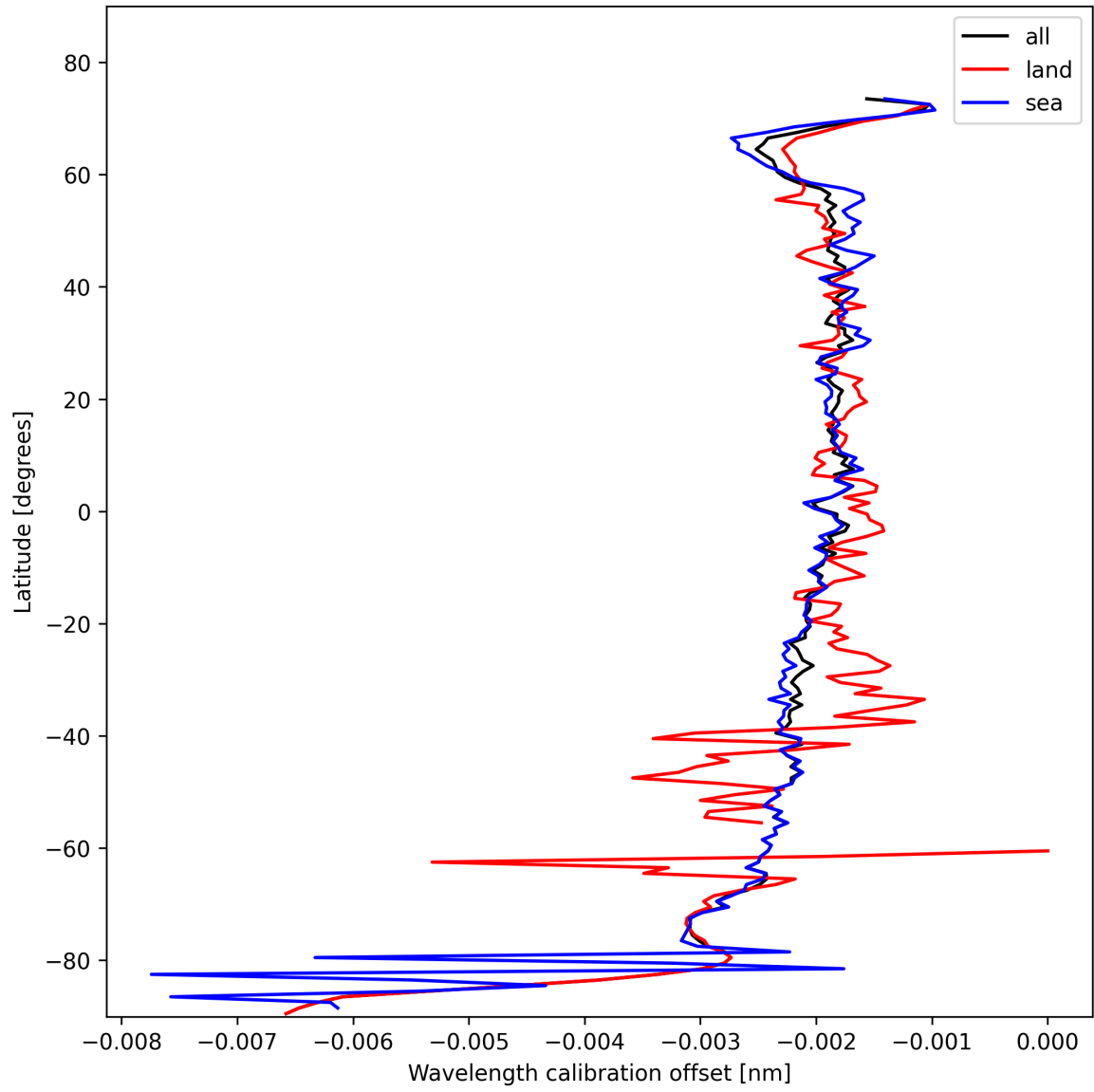
Figure 16: Zonal average of “Wavelength calibration offset” for 2025-02-07 to 2025-02-08.
