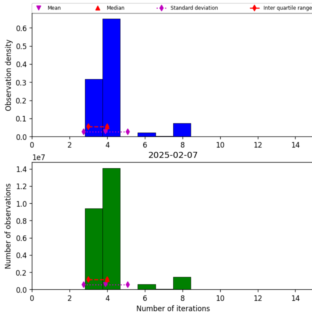
Figure 32: Histogram of “Number of iterations” for 2025-02-07 to 2025-02-08
