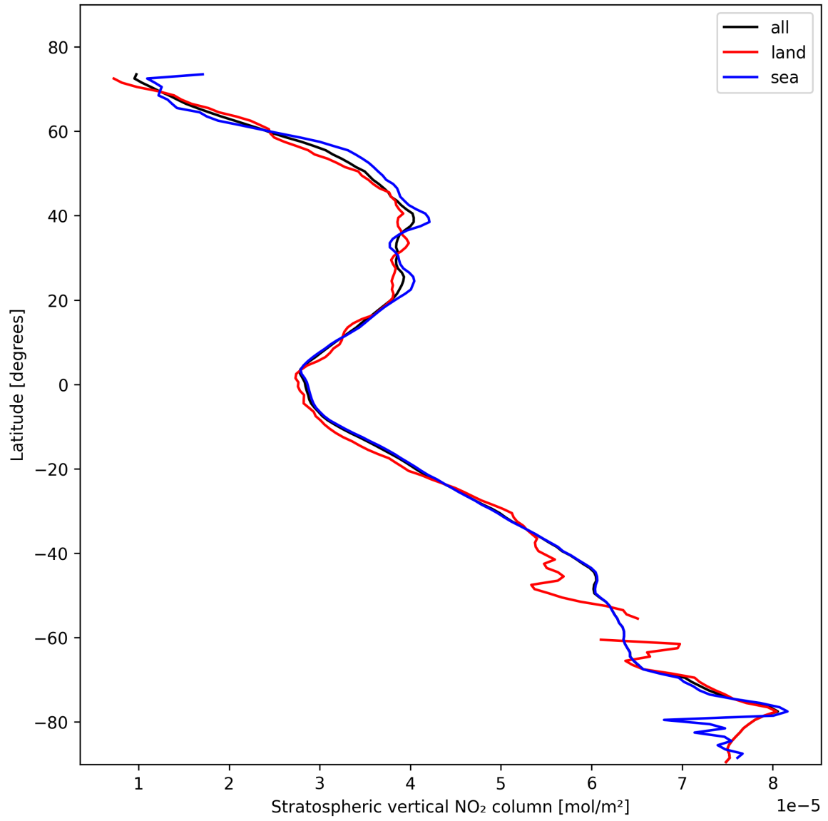
Figure 17: Zonal average of “Stratospheric vertical NO 2 column” for 2025-02-07 to 2025-02-08.
