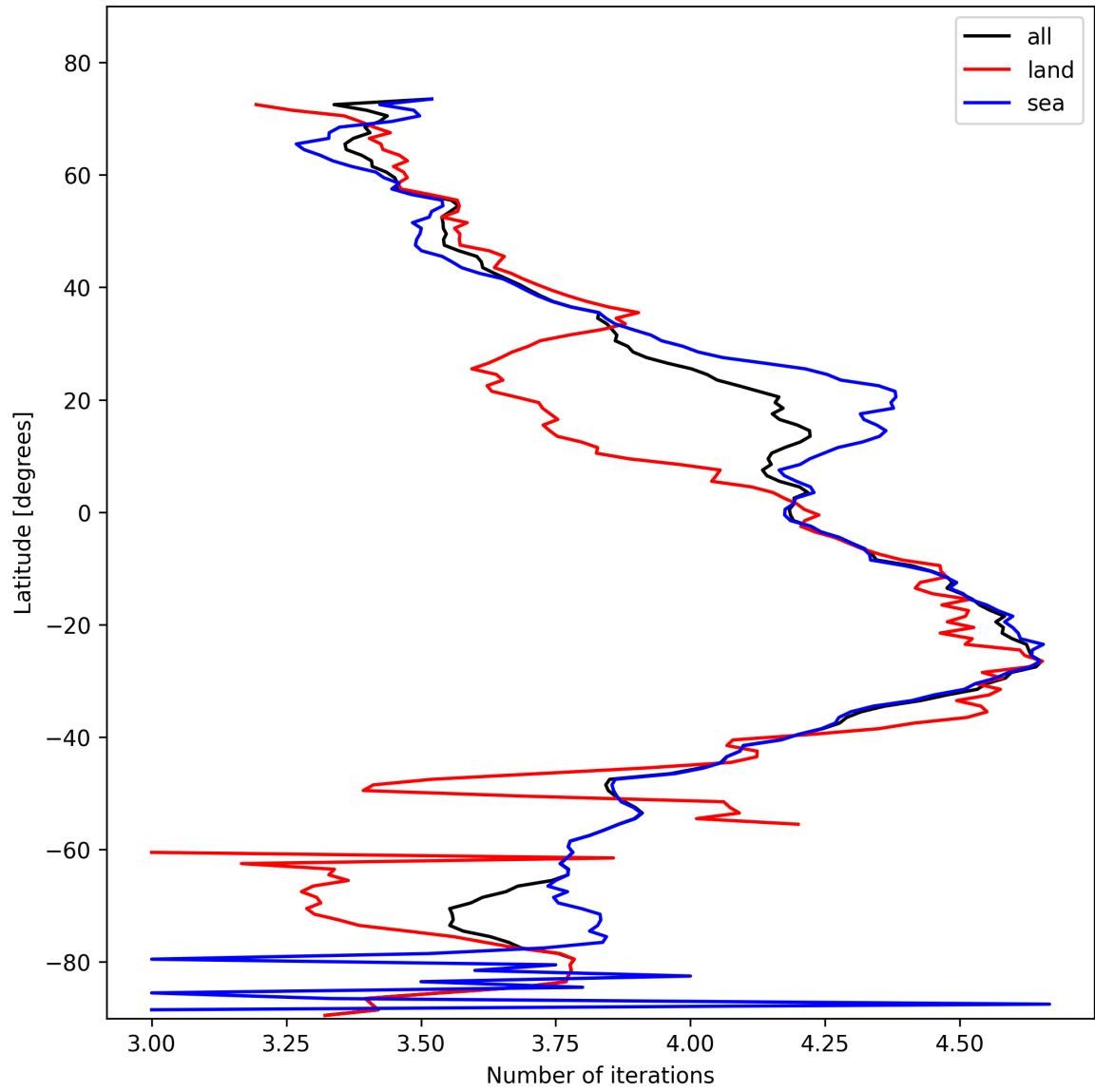
Figure 15: Zonal average of “Number of iterations” for 2025-02-07 to 2025-02-08.
