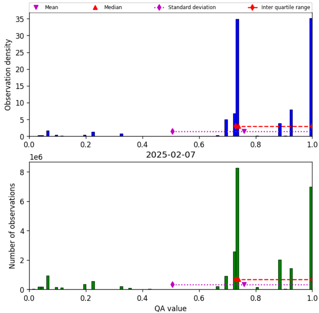
Figure 26: Histogram of “QA value” for 2025-02-07 to 2025-02-08
