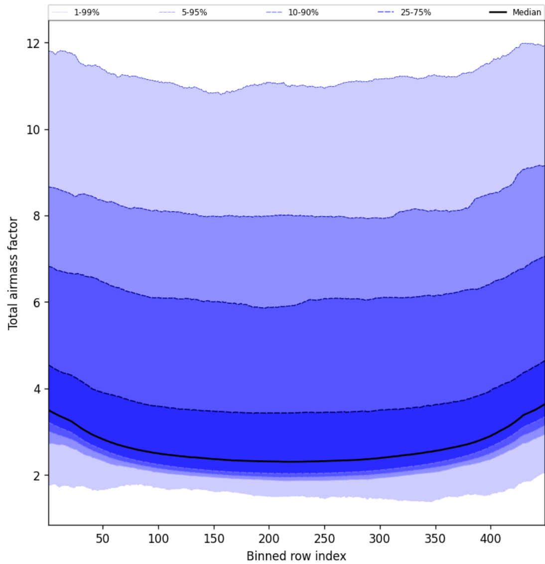
Figure 47: Along track statistics of “Total airmass factor” for 2025-02-07 to 2025-02-08
