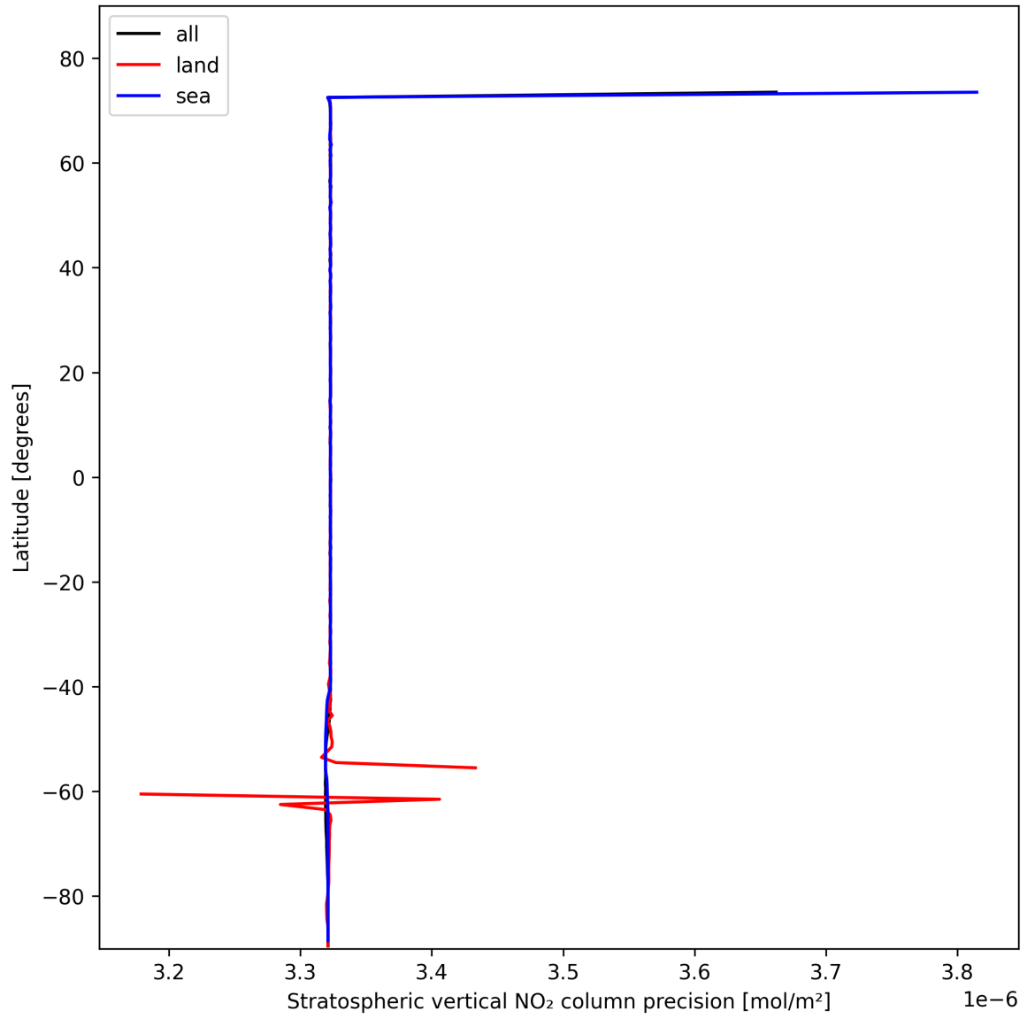
Figure 18: Zonal average of “Stratospheric vertical NO 2 column precision” for 2025-02-07 to 2025-02-08.
