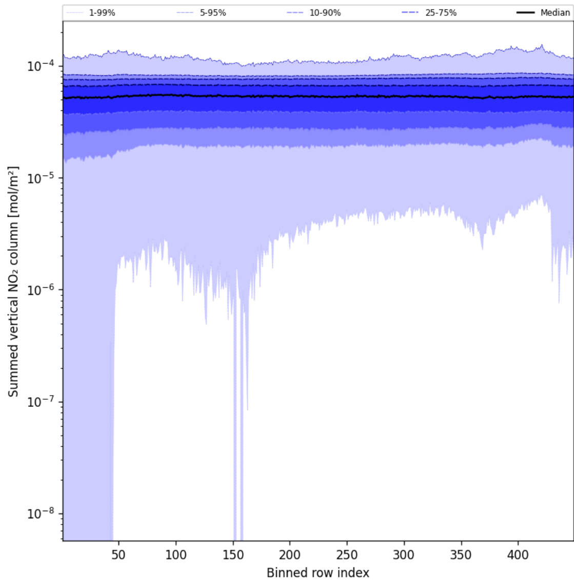
Figure 55: Along track statistics of “Summed vertical NO 2 column” for 2025-02-07 to 2025-02-08
