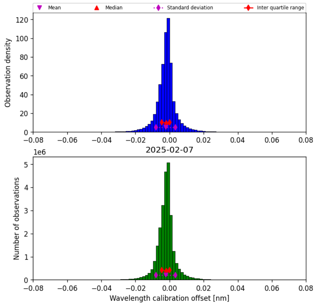
Figure 33: Histogram of “Wavelength calibration offset” for 2025-02-07 to 2025-02-08
