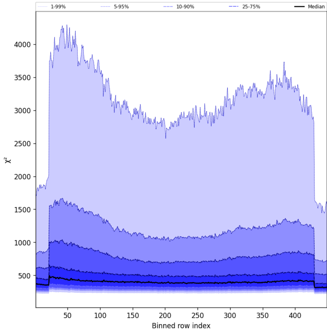
Figure 57: Along track statistics of “ \chi^2 ” for 2025-02-07 to 2025-02-08
