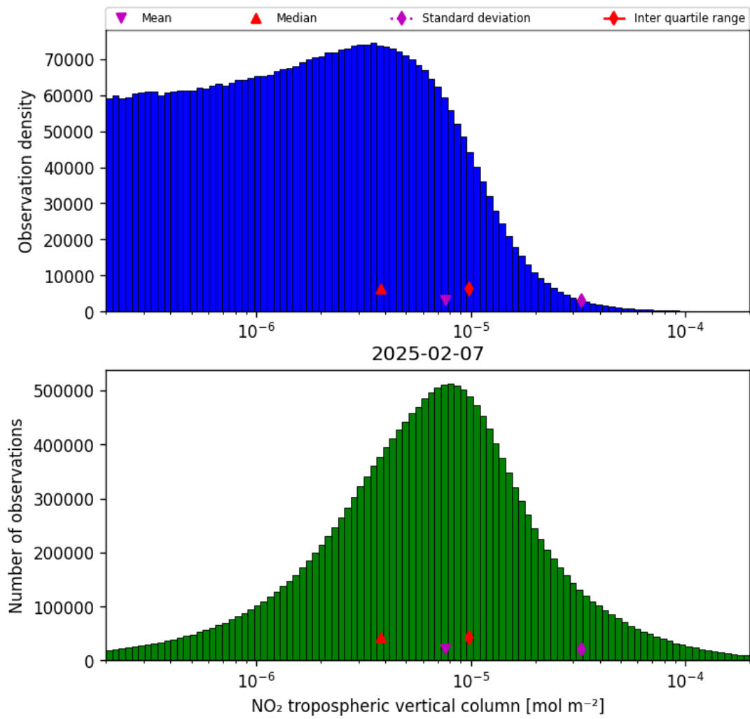
Figure 27: Histogram of “NO 2 tropospheric vertical column” for 2025-02-07 to 2025-02-08
