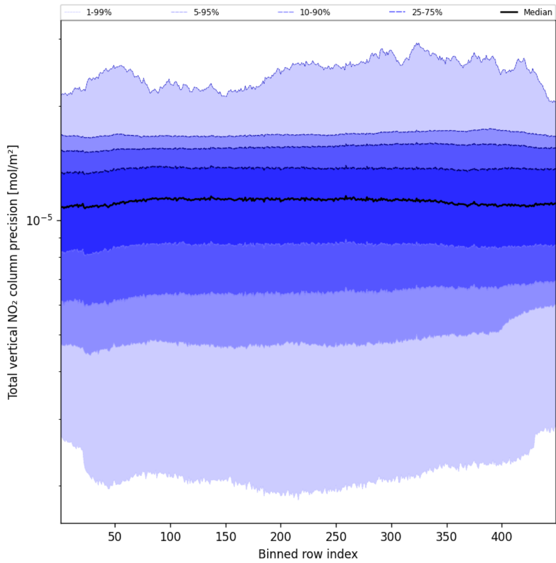
Figure 54: Along track statistics of “Total vertical NO 2 column precision” for 2025-02-07 to 2025-02-08
