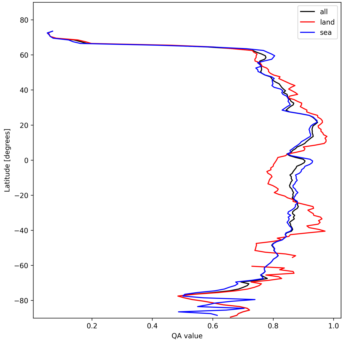
Figure 9: Zonal average of “QA value” for 2025-02-07 to 2025-02-08.
