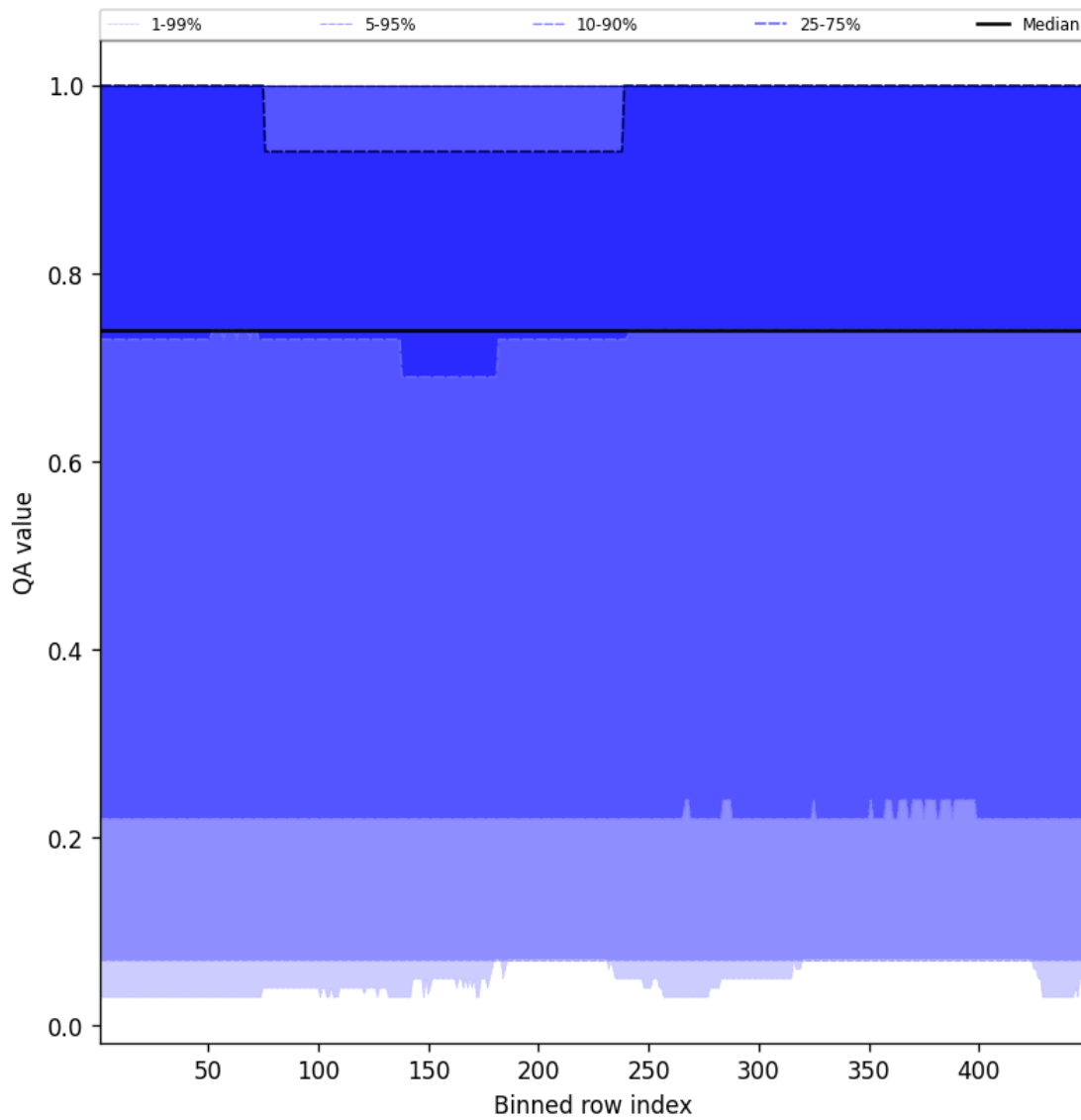
Figure 43: Along track statistics of “QA value” for 2025-02-07 to 2025-02-08
