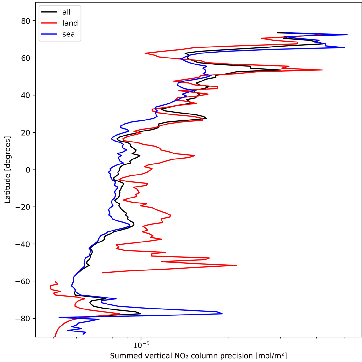
Figure 22: Zonal average of “Summed vertical NO 2 column precision” for 2025-02-07 to 2025-02-08.
