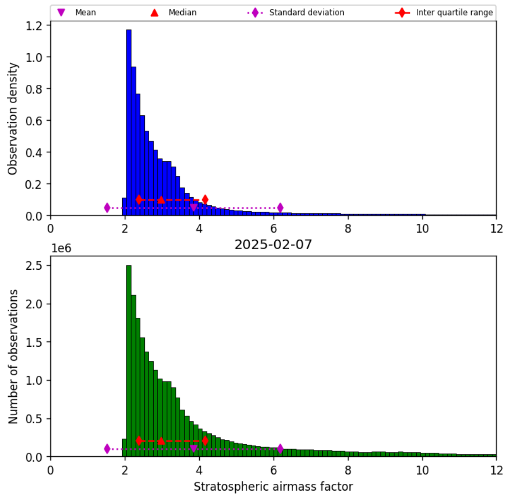
Figure 42: Histogram of “Stratospheric airmass factor” for 2025-02-07 to 2025-02-08
