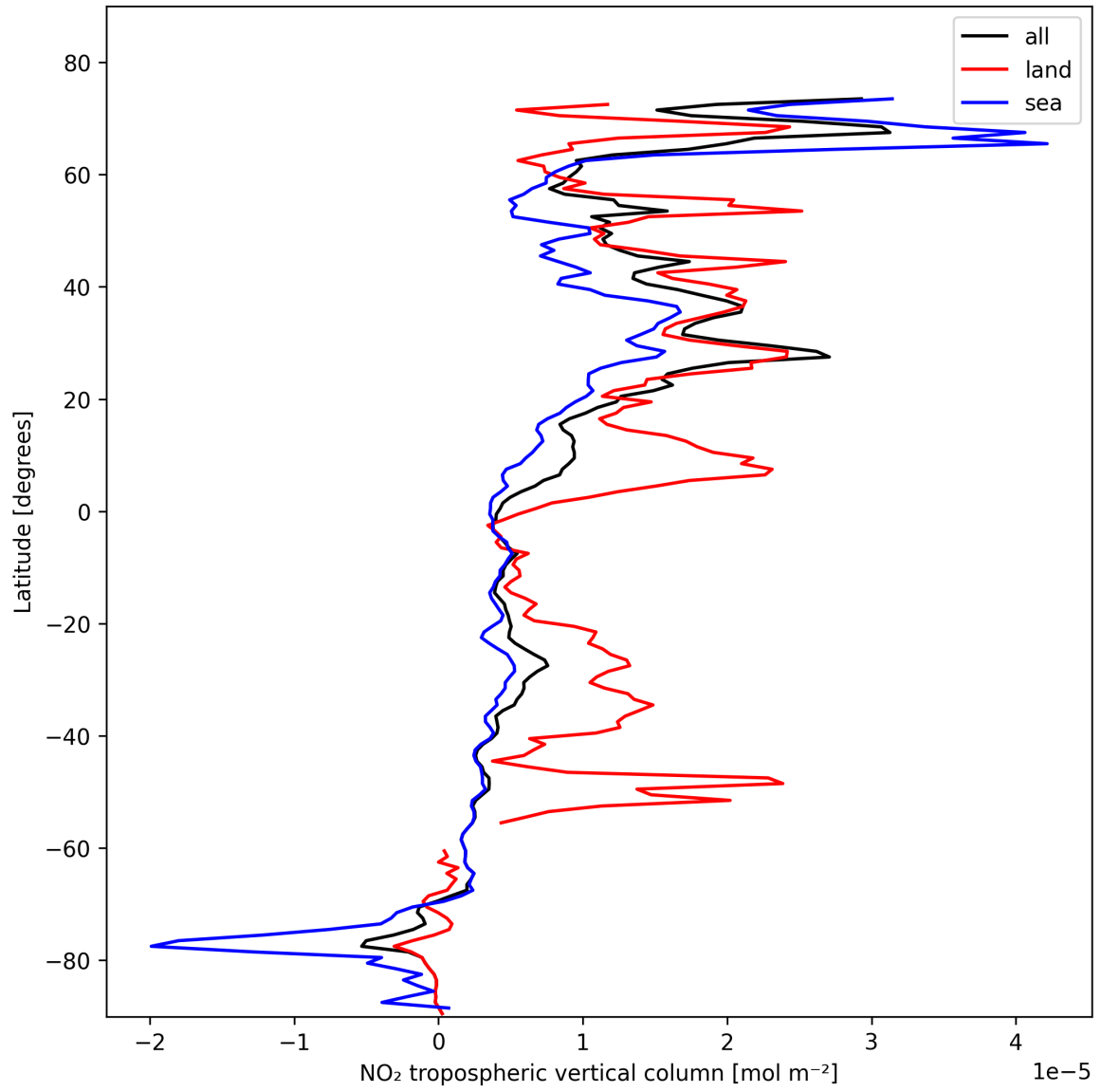
Figure 10: Zonal average of “NO 2 tropospheric vertical column” for 2025-02-07 to 2025-02-08.
