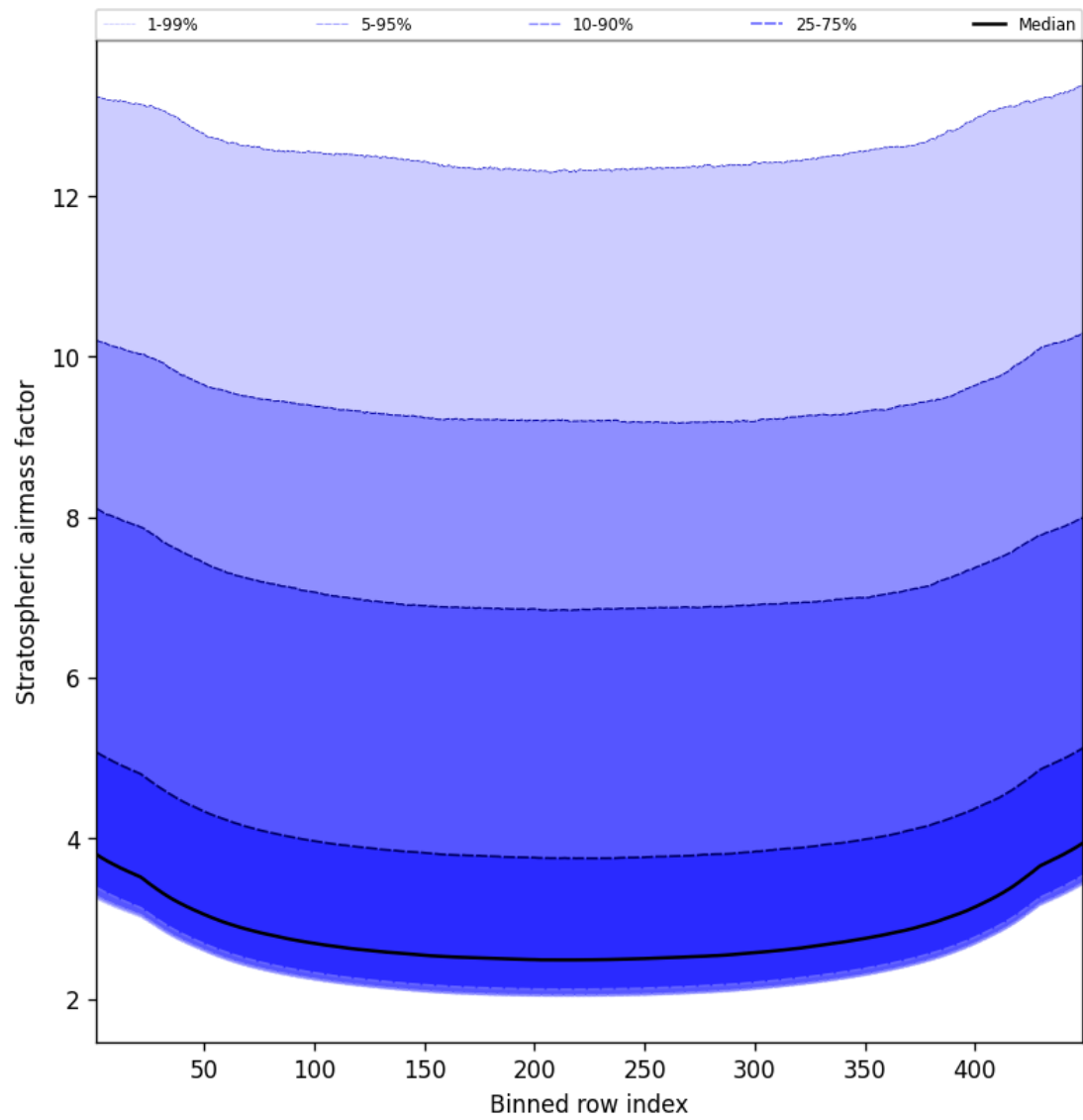
Figure 59: Along track statistics of “Stratospheric airmass factor” for 2025-02-07 to 2025-02-08
