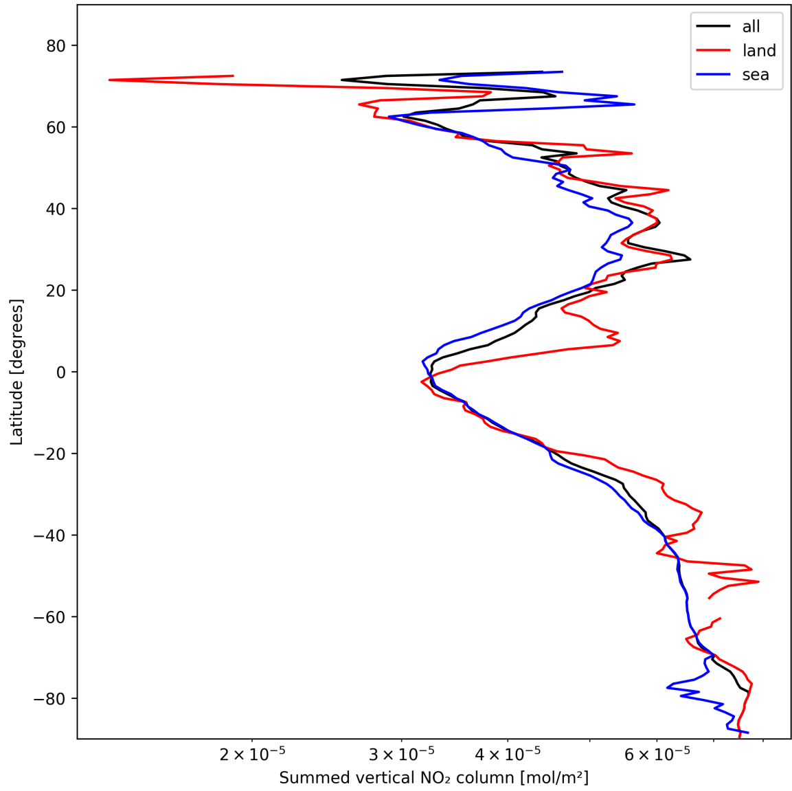
Figure 21: Zonal average of “Summed vertical NO 2 column” for 2025-02-07 to 2025-02-08.
