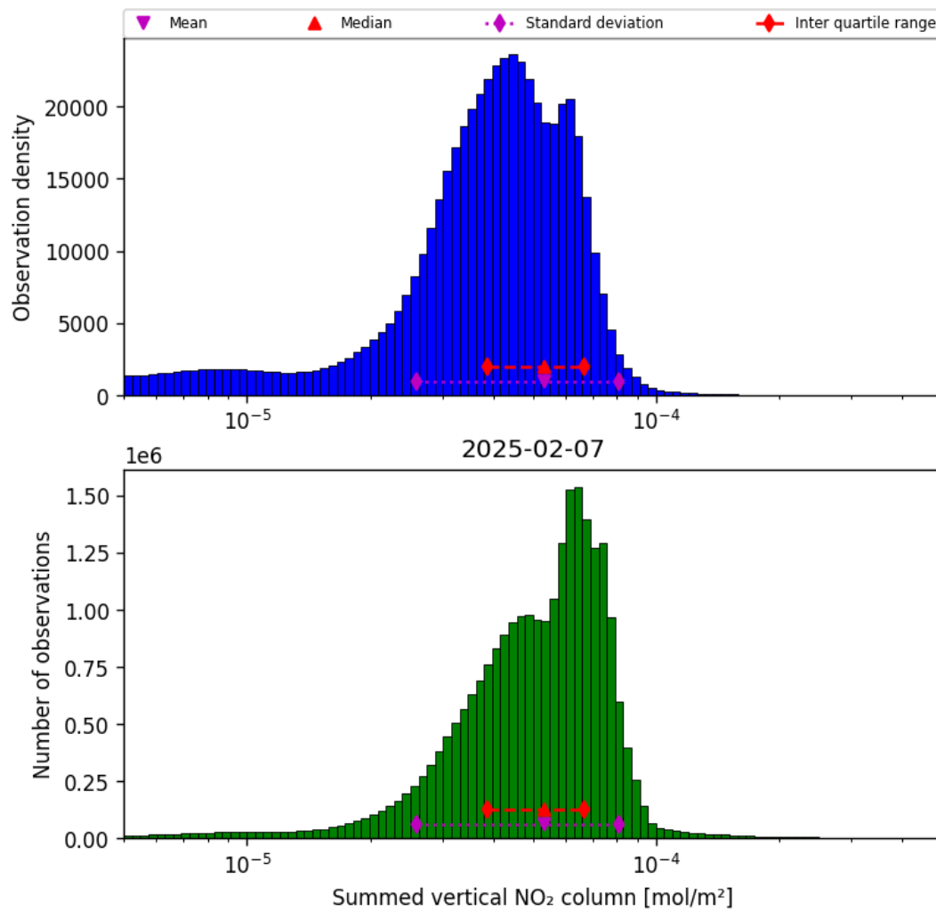
Figure 38: Histogram of “Summed vertical NO 2 column” for 2025-02-07 to 2025-02-08
