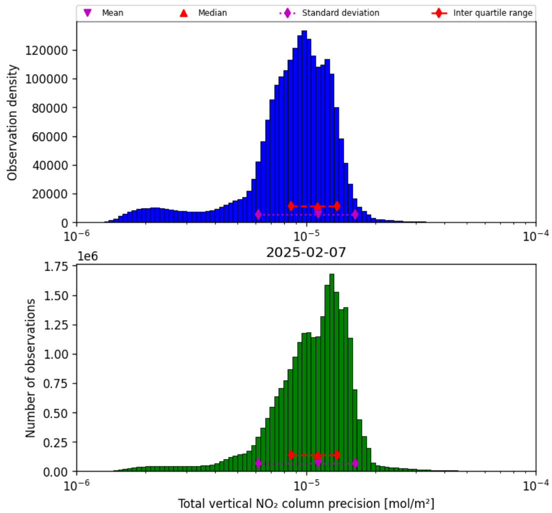
Figure 37: Histogram of “Total vertical NO 2 column precision” for 2025-02-07 to 2025-02-08
