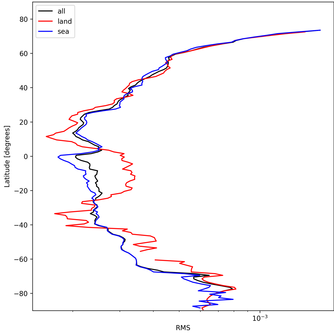
Figure 24: Zonal average of “RMS” for 2025-02-07 to 2025-02-08.
