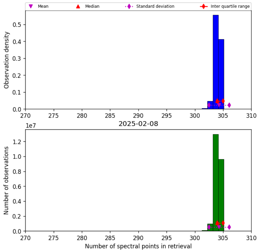
Figure 31: Histogram of “Number of spectral points in retrieval” for 2025-02-08 to 2025-02-09
