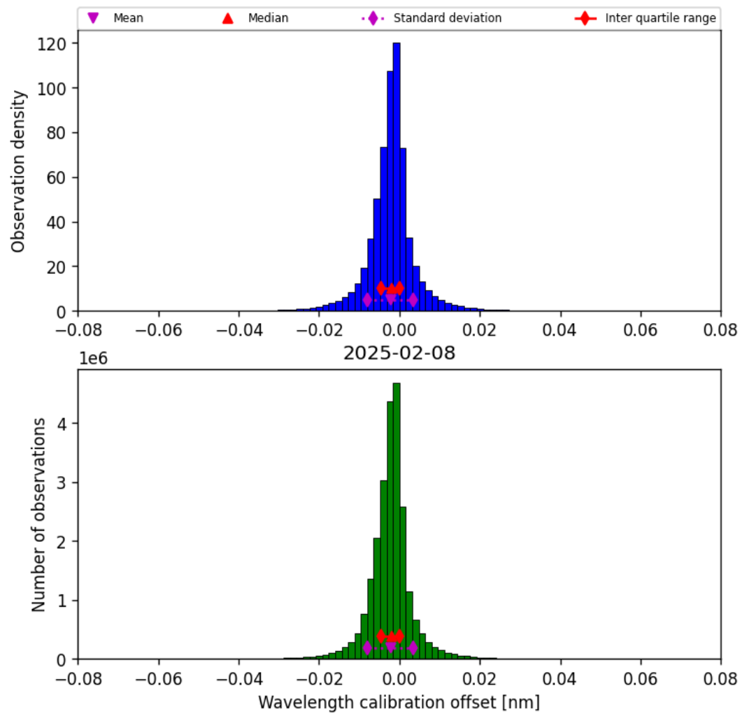
Figure 33: Histogram of “Wavelength calibration offset” for 2025-02-08 to 2025-02-09
