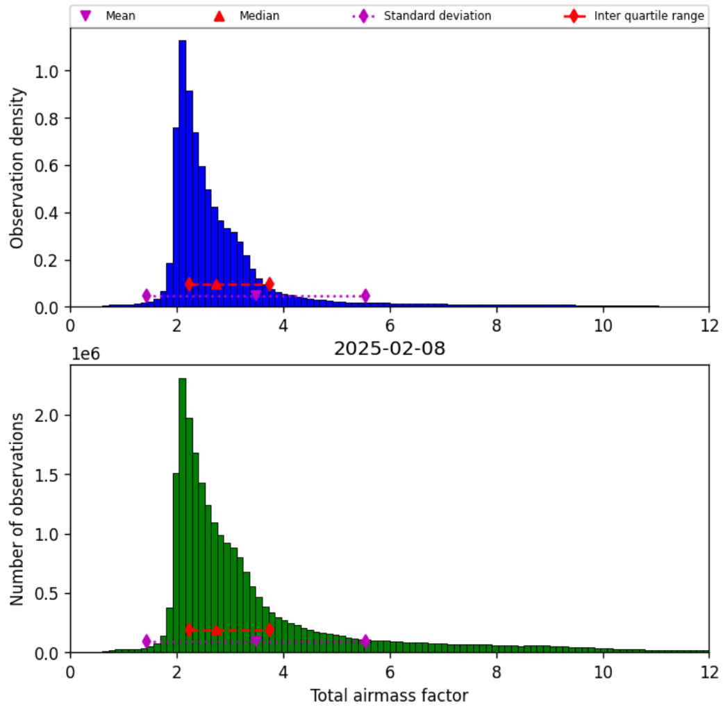
Figure 30: Histogram of “Total airmass factor” for 2025-02-08 to 2025-02-09
