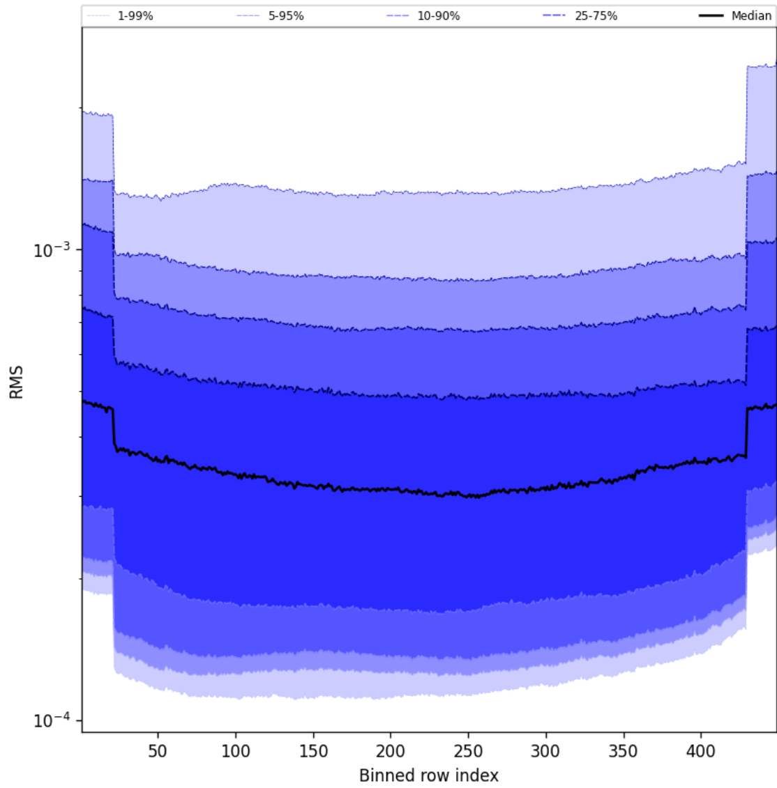
Figure 58: Along track statistics of “RMS” for 2025-02-08 to 2025-02-09
