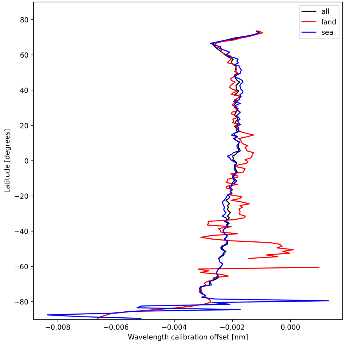
Figure 16: Zonal average of “Wavelength calibration offset” for 2025-02-08 to 2025-02-09.
