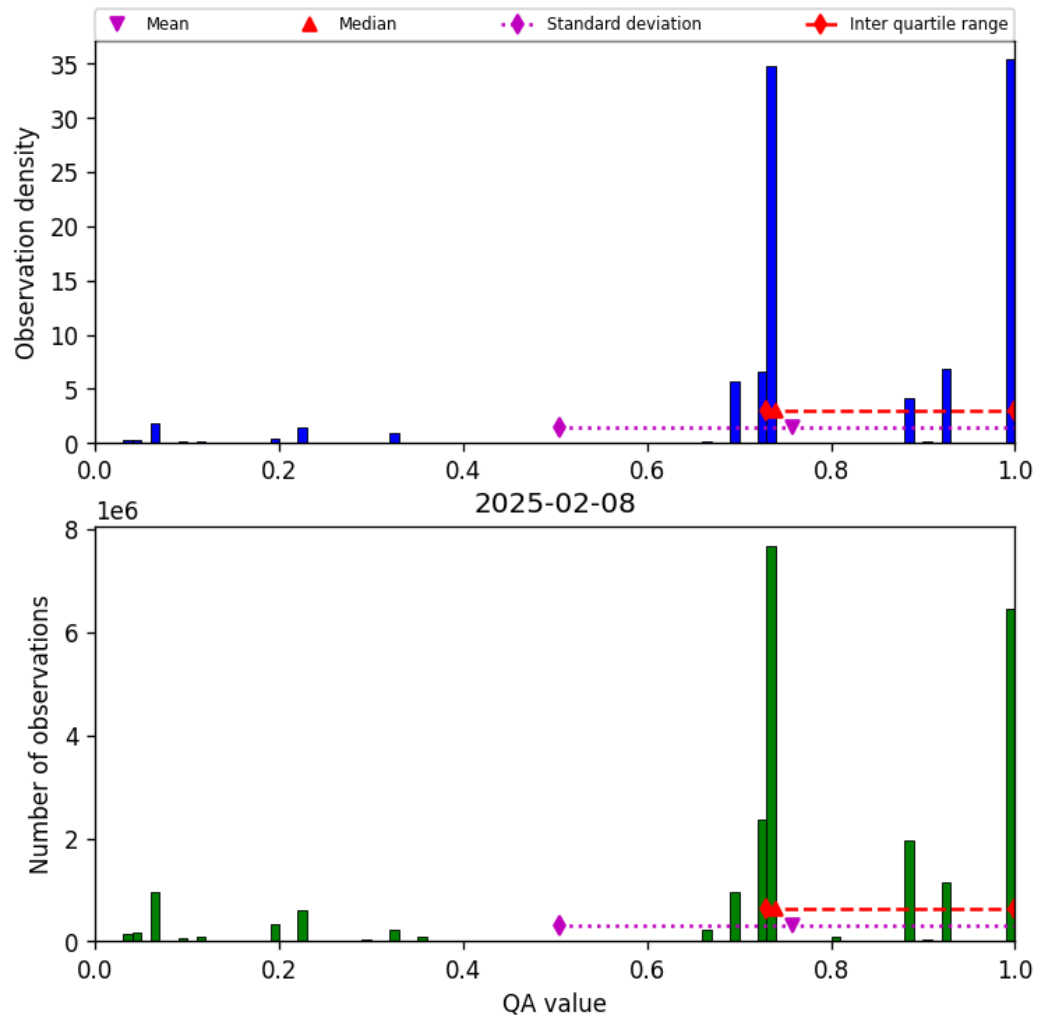
Figure 26: Histogram of “QA value” for 2025-02-08 to 2025-02-09
