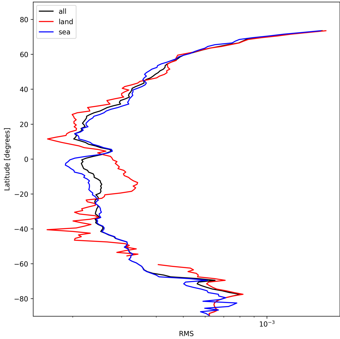
Figure 24: Zonal average of “RMS” for 2025-02-08 to 2025-02-09.
