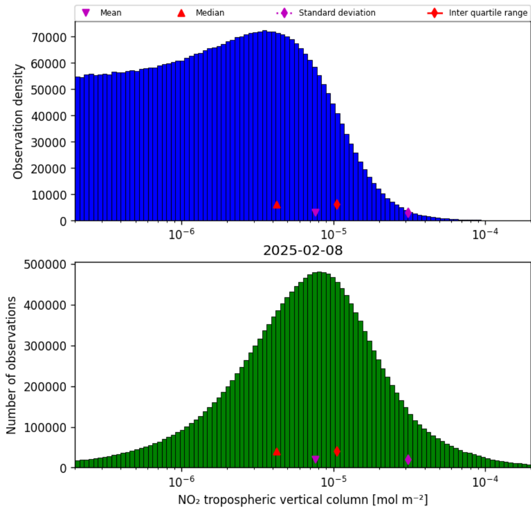
Figure 27: Histogram of “NO 2 tropospheric vertical column” for 2025-02-08 to 2025-02-09
