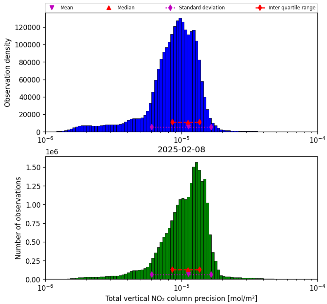
Figure 37: Histogram of “Total vertical NO 2 column precision” for 2025-02-08 to 2025-02-09
