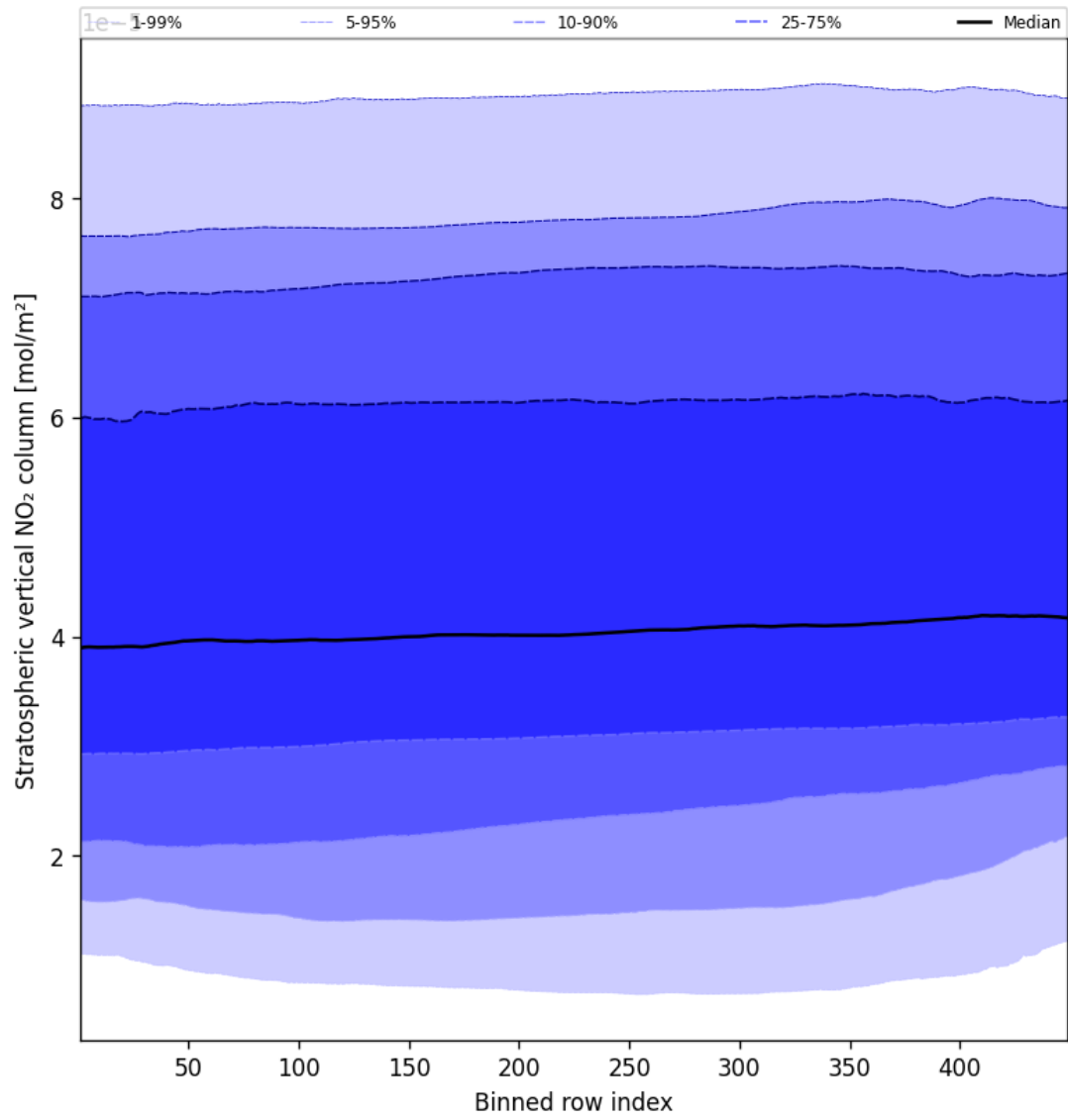
Figure 51: Along track statistics of “Stratospheric vertical NO 2 column” for 2025-02-08 to 2025-02-09
