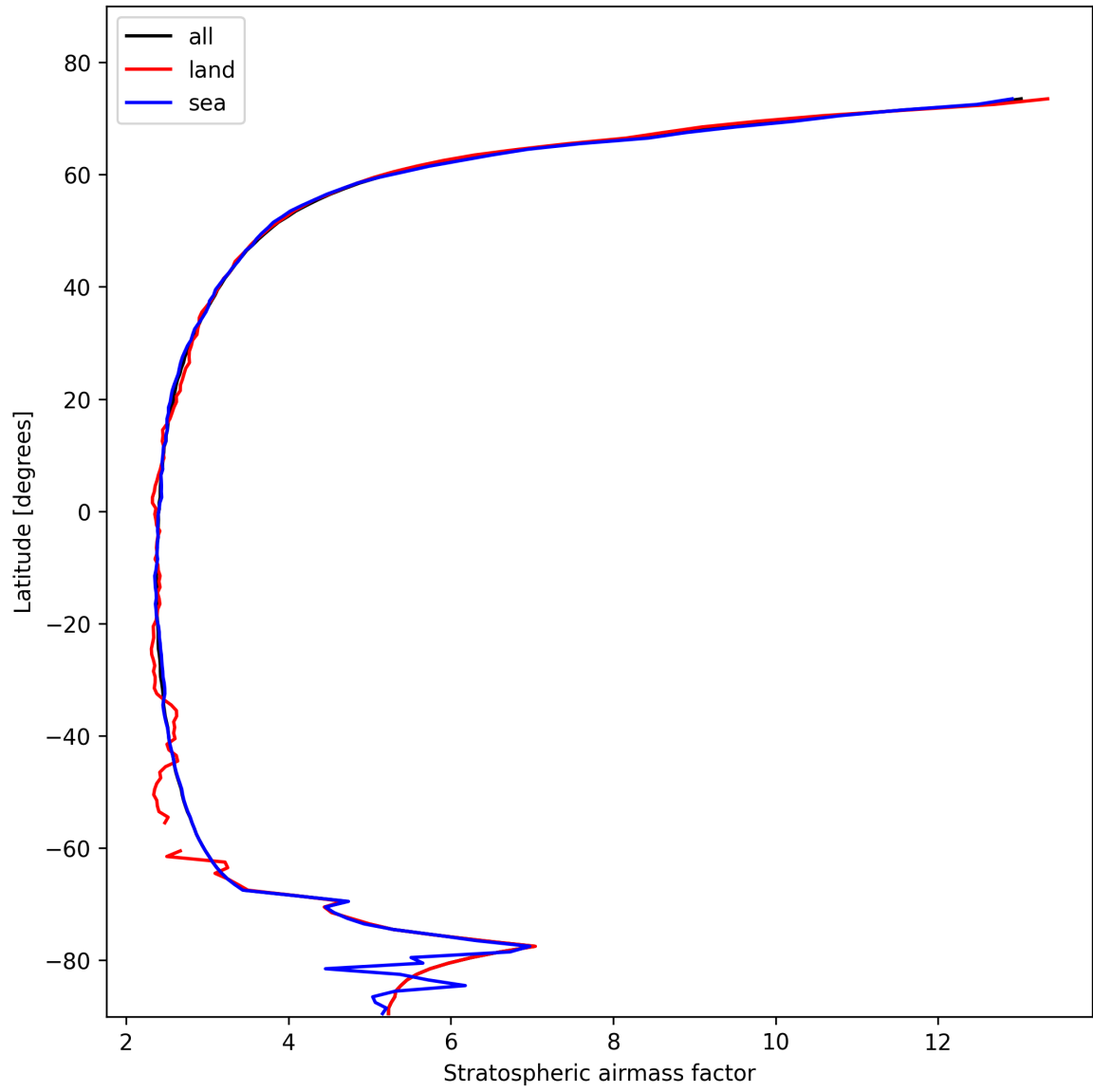
Figure 25: Zonal average of “Stratospheric air mass factor” for 2025-02-08 to 2025-02-09.
