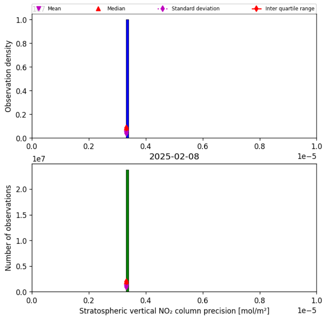
Figure 35: Histogram of “Stratospheric vertical NO 2 column precision” for 2025-02-08 to 2025-02-09
