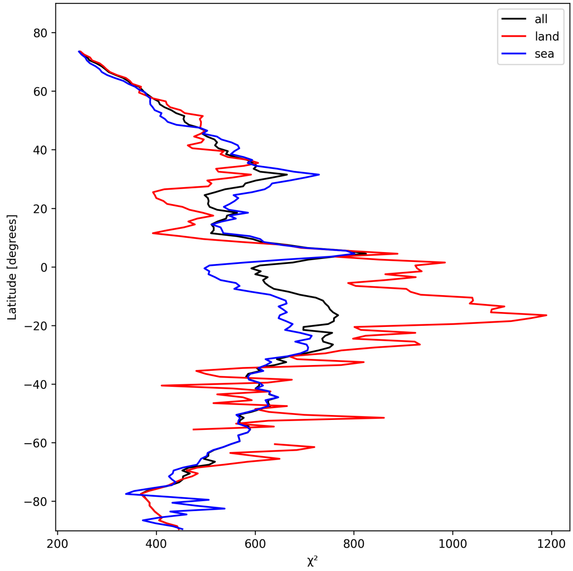
Figure 23: Zonal average of “ \chi^2 ” for 2025-02-08 to 2025-02-09.
