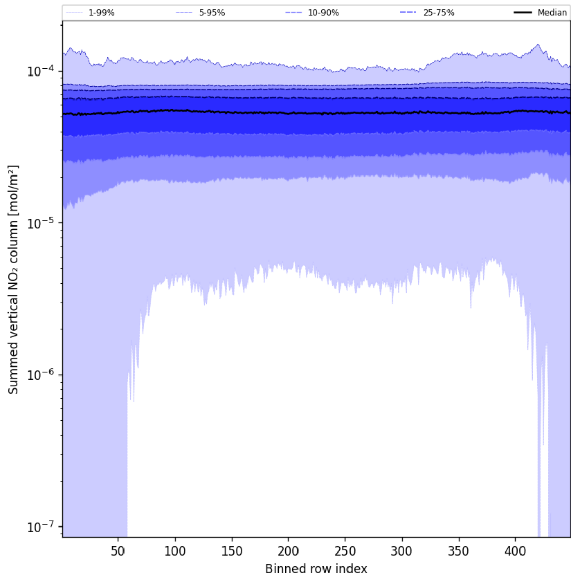
Figure 55: Along track statistics of “Summed vertical NO 2 column” for 2025-02-08 to 2025-02-09
