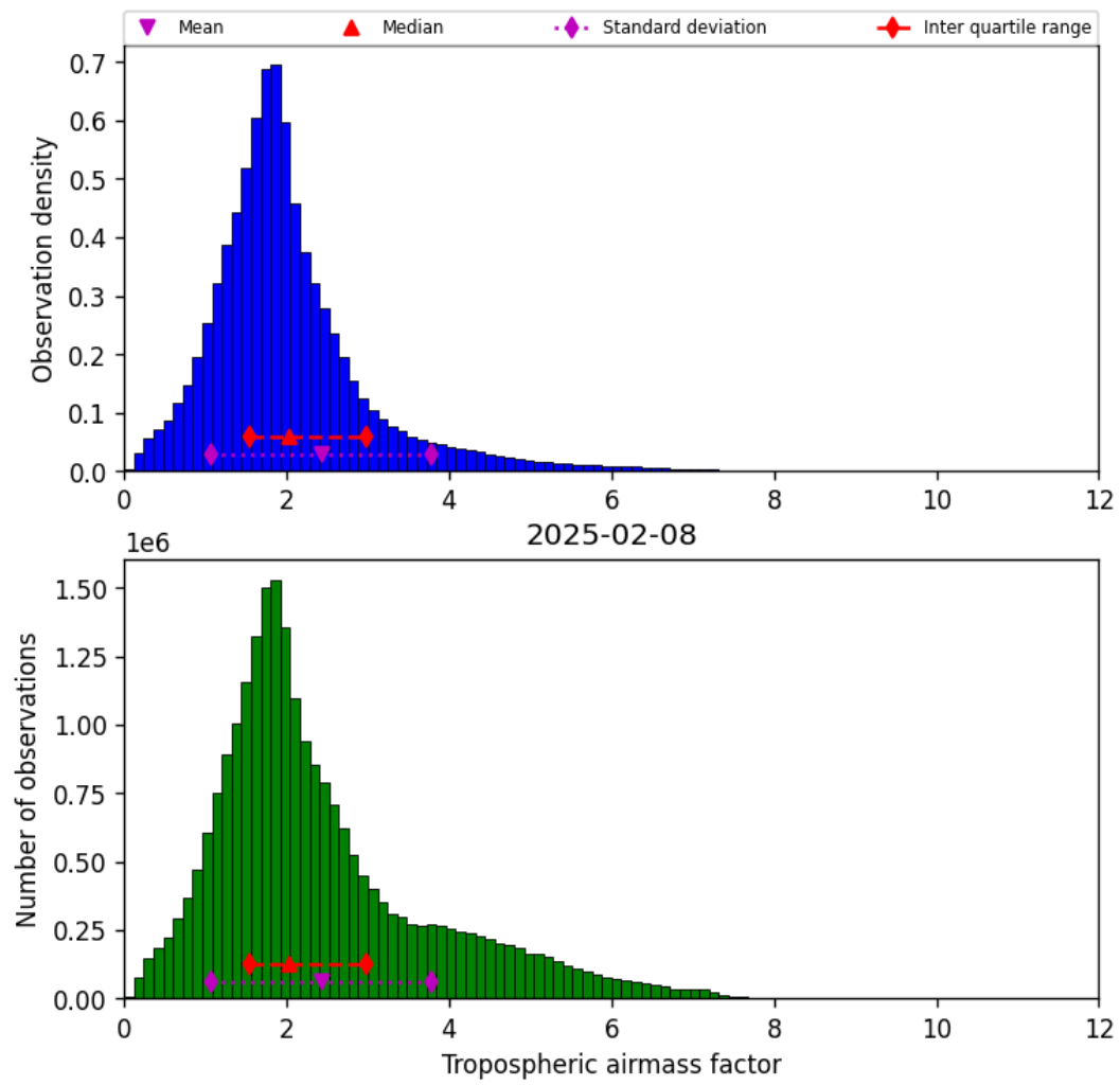
Figure 29: Histogram of “Tropospheric airmass factor” for 2025-02-08 to 2025-02-09
