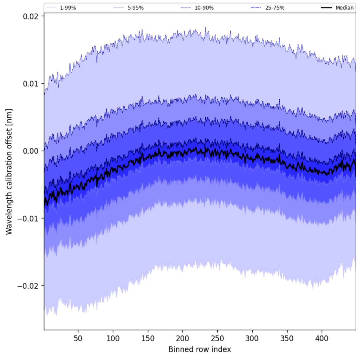
Figure 50: Along track statistics of “Wavelength calibration offset” for 2025-02-08 to 2025-02-09
