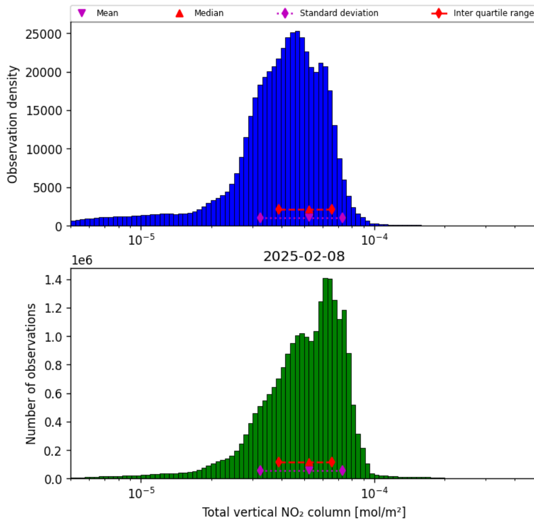
Figure 36: Histogram of “Total vertical NO 2 column” for 2025-02-08 to 2025-02-09
