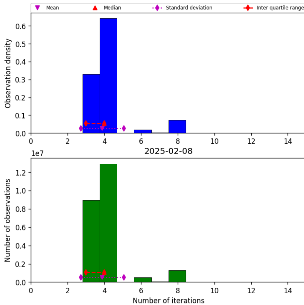
Figure 32: Histogram of “Number of iterations” for 2025-02-08 to 2025-02-09
