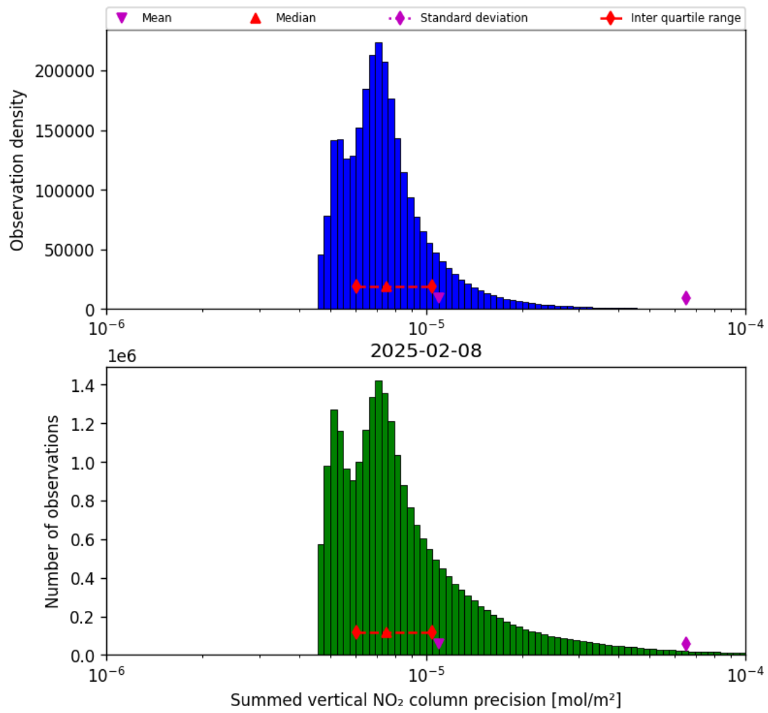
Figure 39: Histogram of “Summed vertical NO 2 column precision” for 2025-02-08 to 2025-02-09
