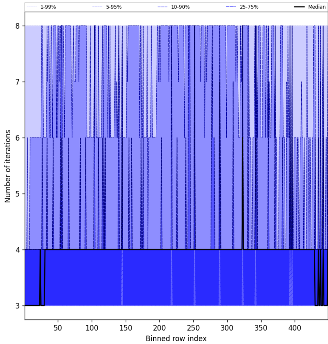
Figure 49: Along track statistics of “Number of iterations” for 2025-02-08 to 2025-02-09
