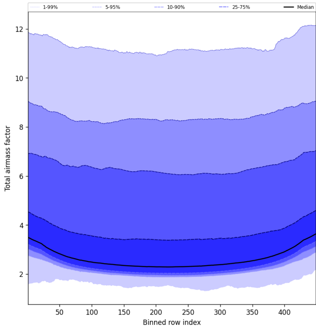
Figure 47: Along track statistics of “Total airmass factor” for 2025-02-08 to 2025-02-09
