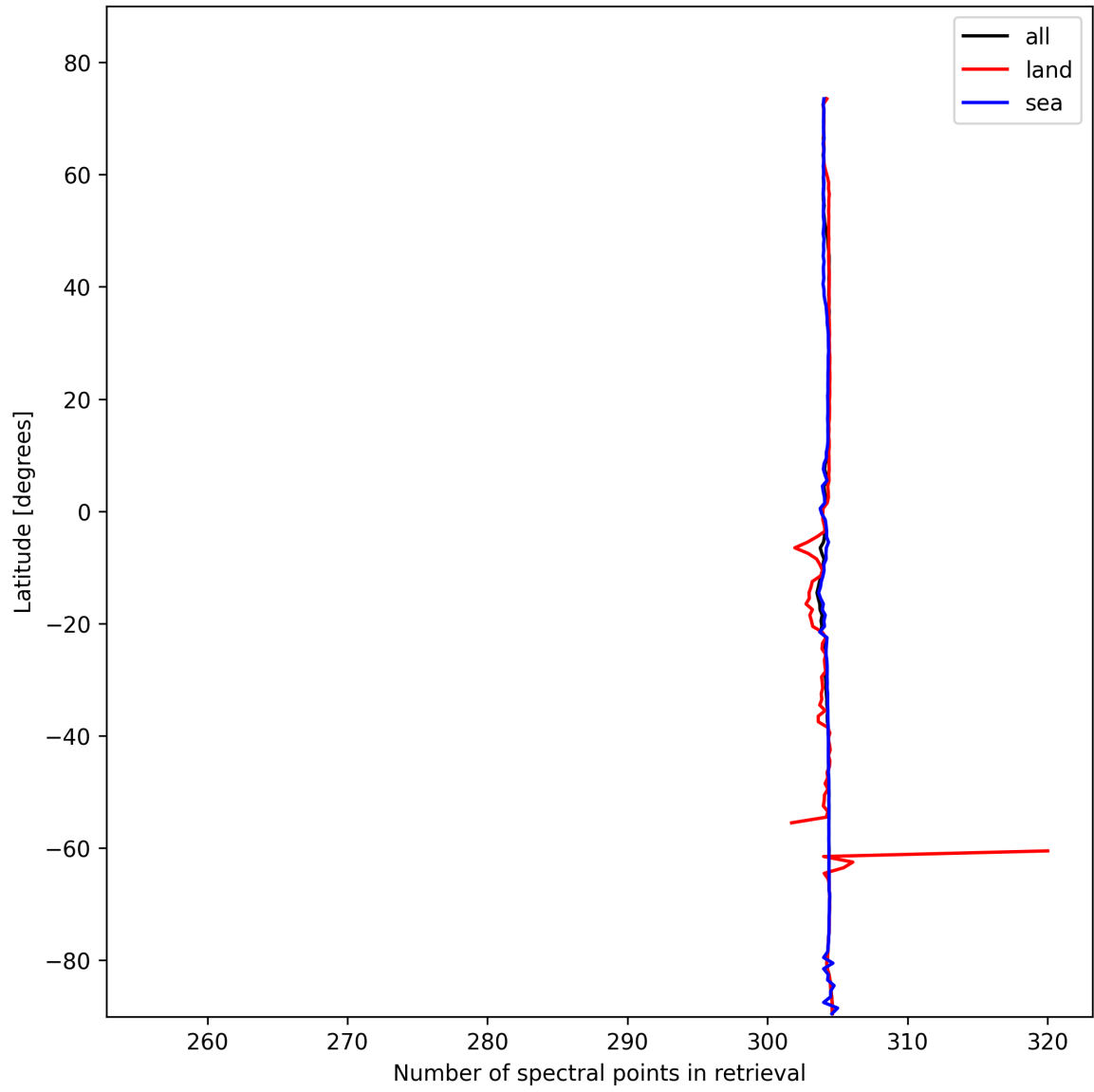
Figure 14: Zonal average of “Number of spectral points in retrieval” for 2025-02-08 to 2025-02-09.
