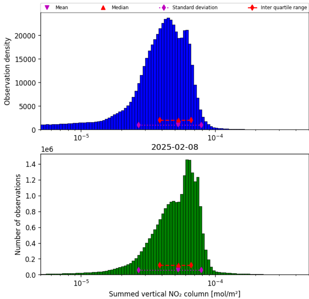
Figure 38: Histogram of “Summed vertical NO 2 column” for 2025-02-08 to 2025-02-09
