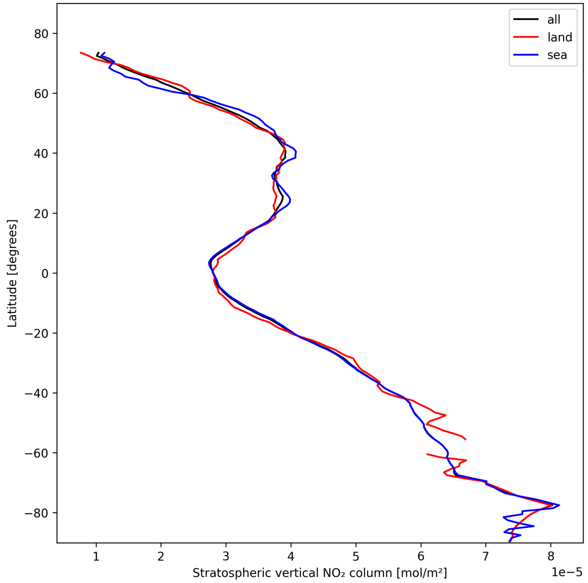
Figure 17: Zonal average of “Stratospheric vertical NO 2 column” for 2025-02-08 to 2025-02-09.
