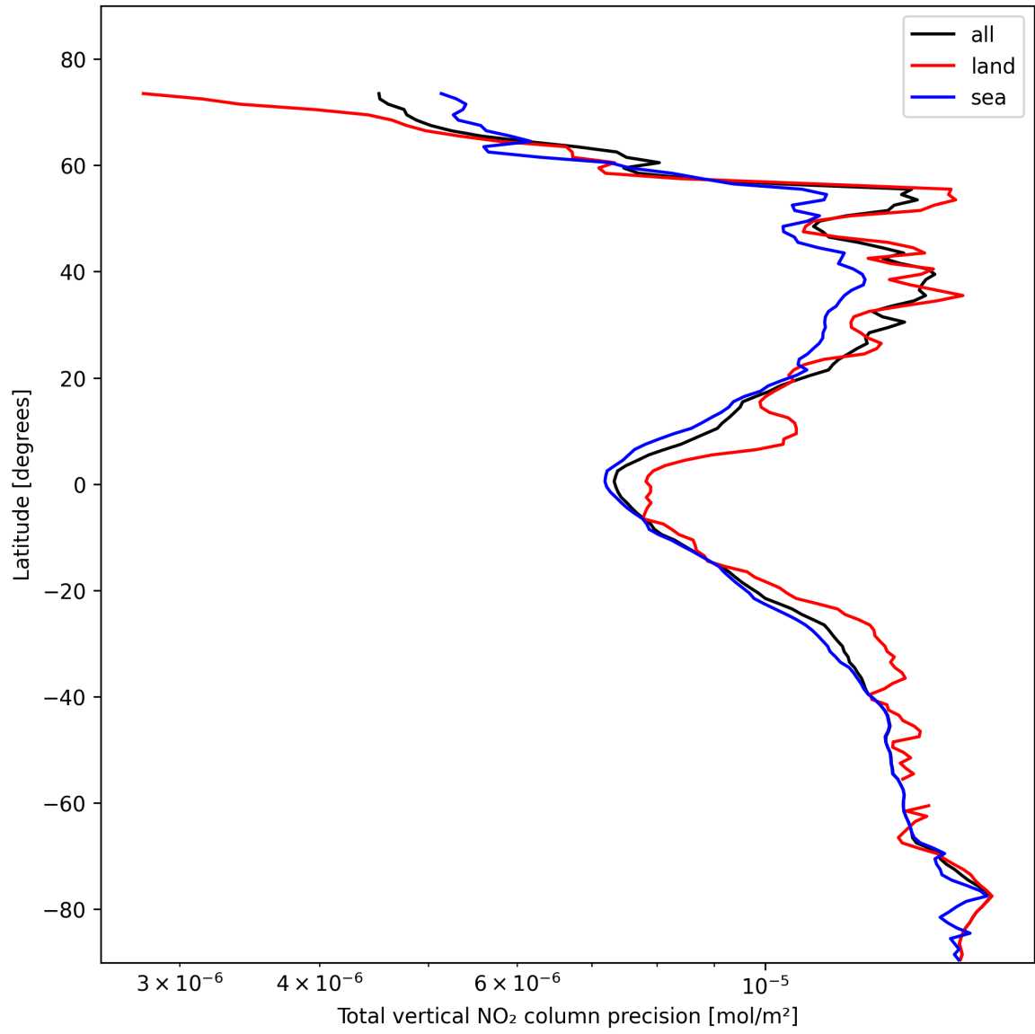
Figure 20: Zonal average of “Total vertical NO 2 column precision” for 2025-02-08 to 2025-02-09.
