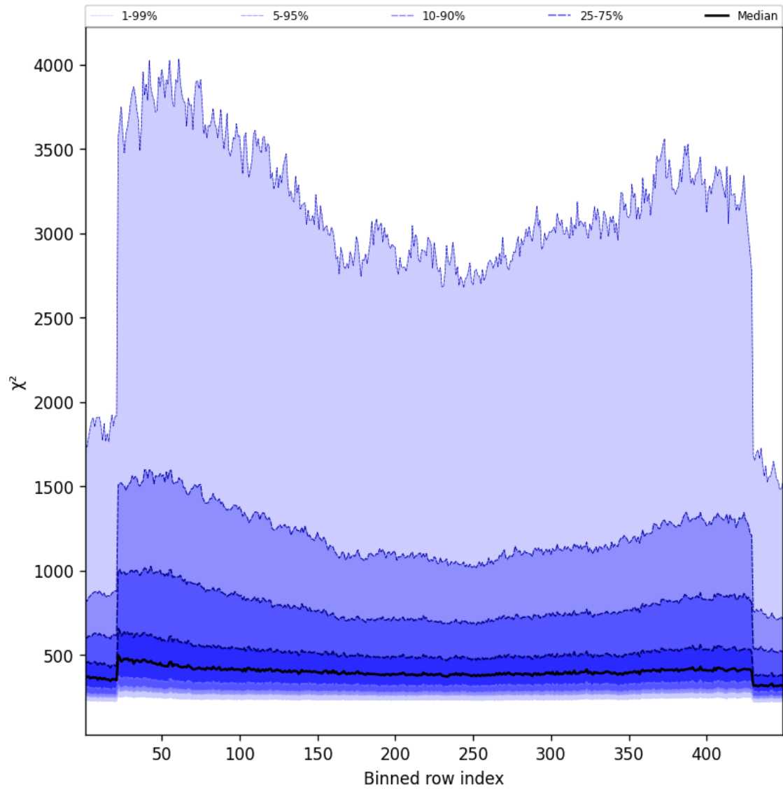
Figure 57: Along track statistics of “ \chi^2 ” for 2025-02-08 to 2025-02-09
