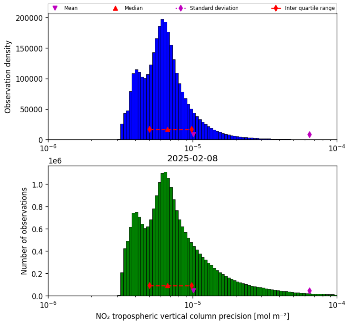
Figure 28: Histogram of “NO 2 tropospheric vertical column precision” for 2025-02-08 to 2025-02-09
