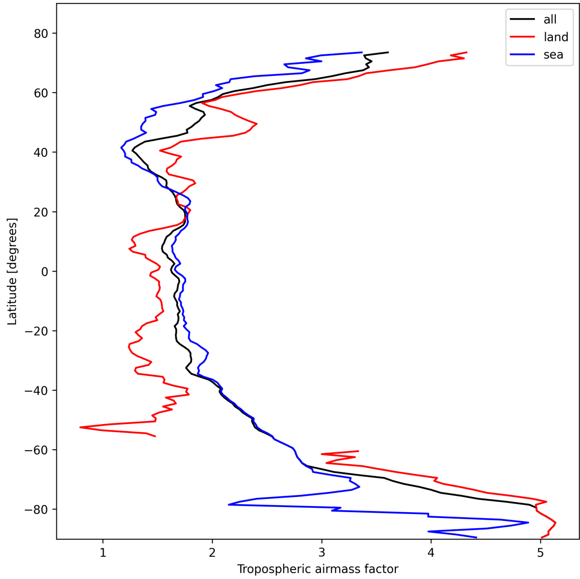
Figure 12: Zonal average of “Tropospheric airmass factor” for 2025-02-08 to 2025-02-09.
