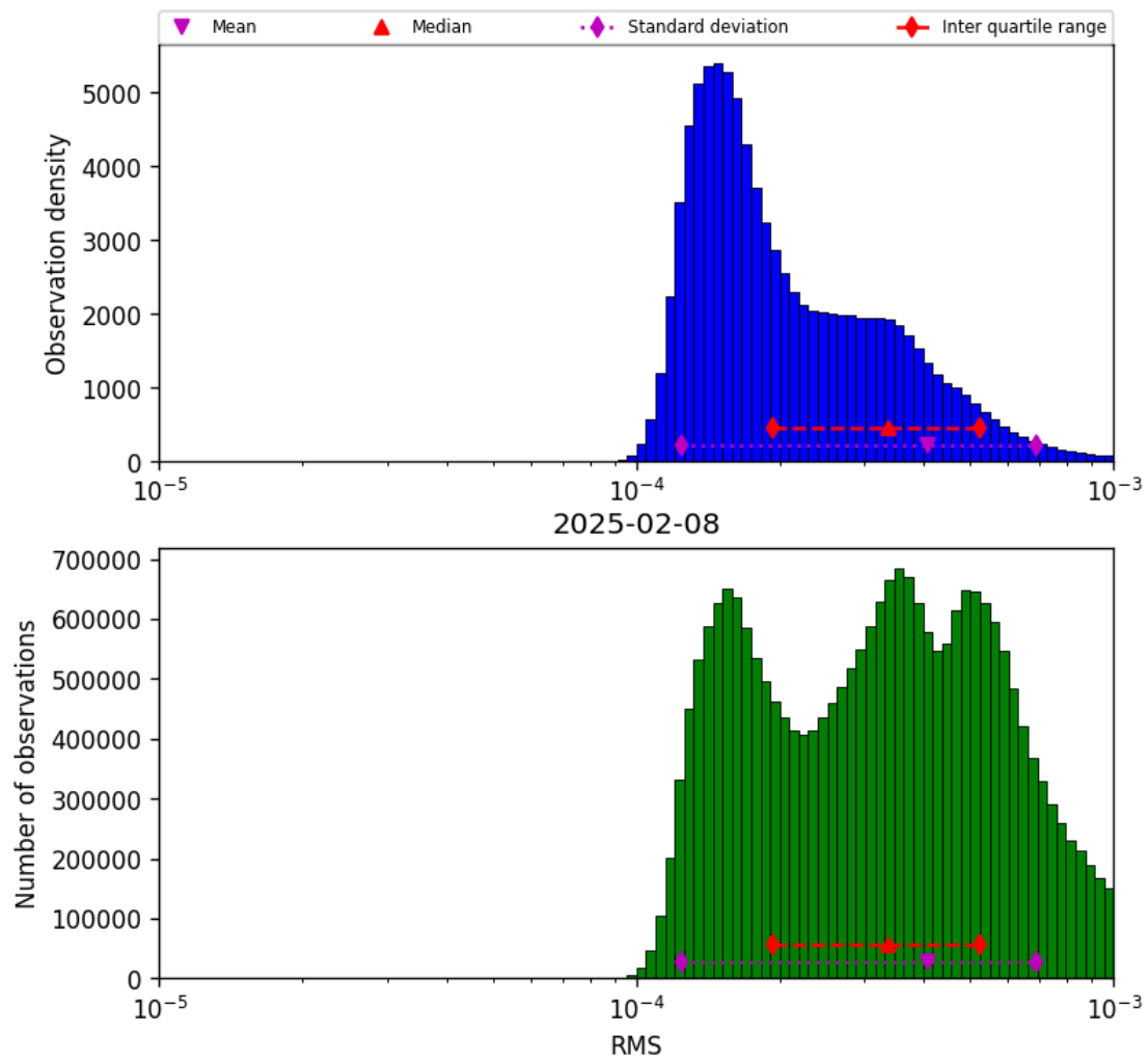
Figure 41: Histogram of “RMS” for 2025-02-08 to 2025-02-09
