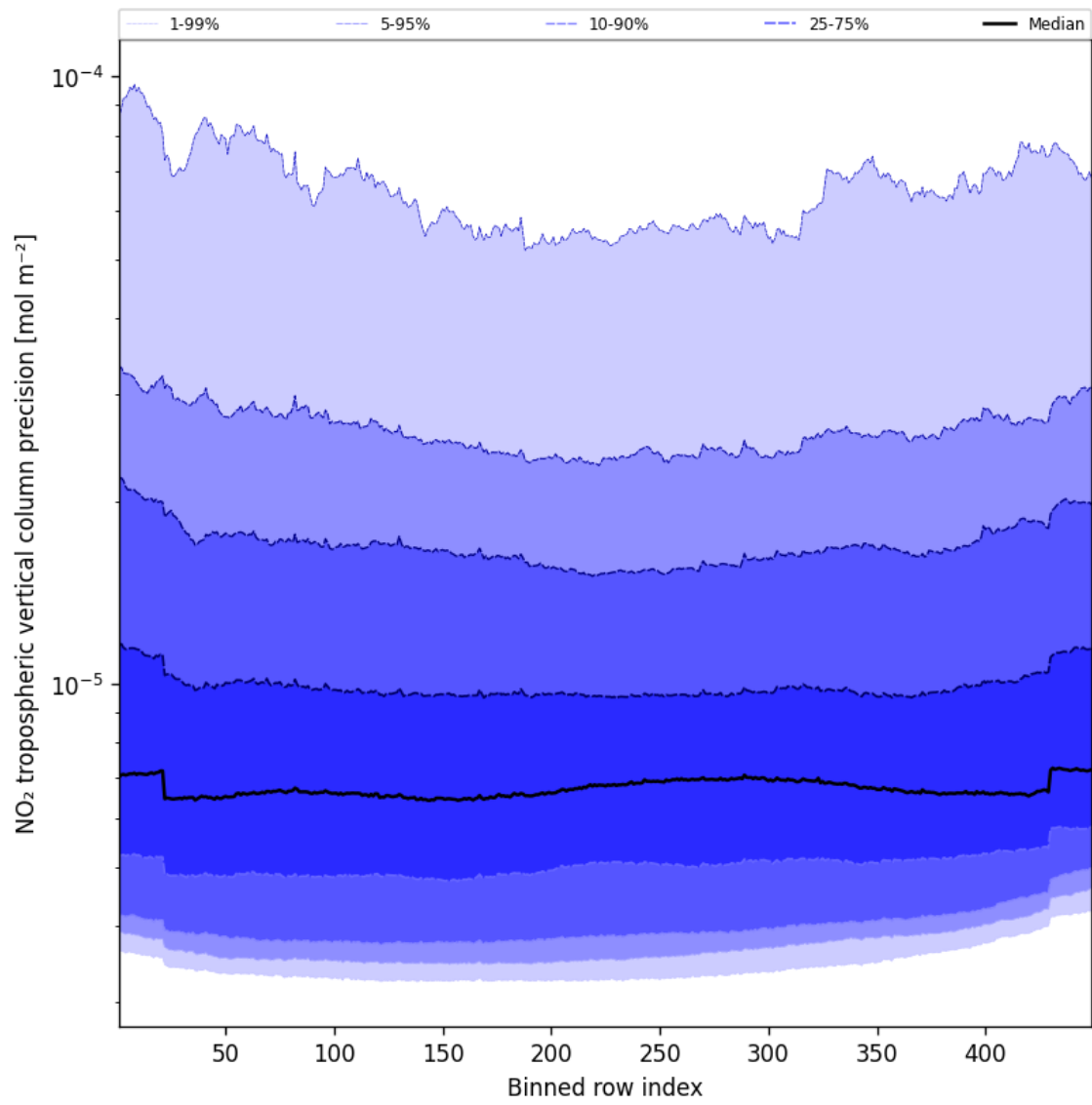
Figure 45: Along track statistics of “NO 2 tropospheric vertical column precision” for 2025-02-08 to 2025-02-09
