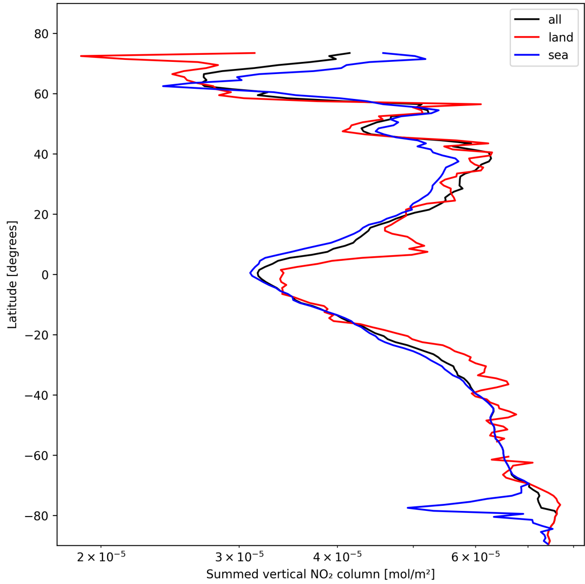
Figure 21: Zonal average of “Summed vertical NO 2 column” for 2025-02-08 to 2025-02-09.
