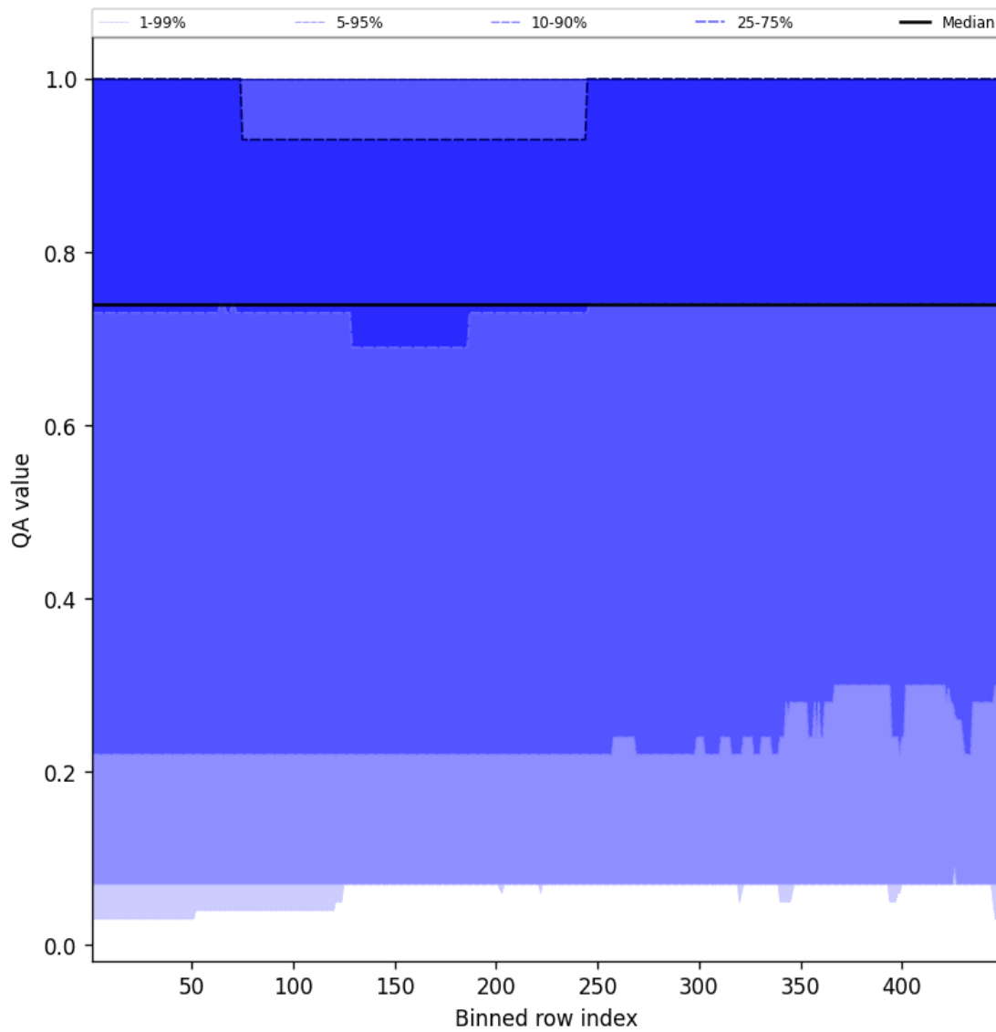
Figure 43: Along track statistics of “QA value” for 2025-02-08 to 2025-02-09
