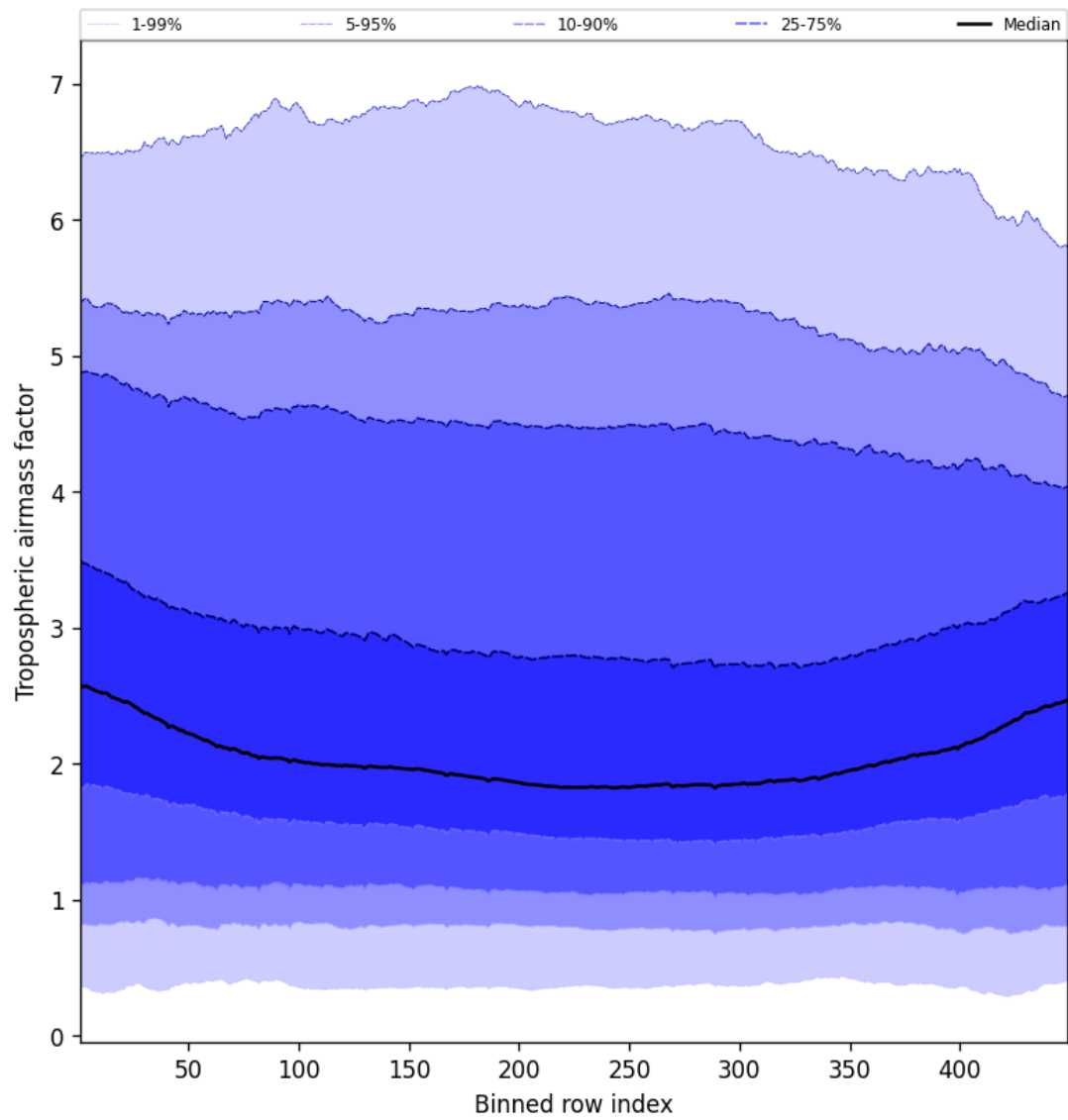
Figure 46: Along track statistics of “Tropospheric airmass factor” for 2025-02-08 to 2025-02-09
