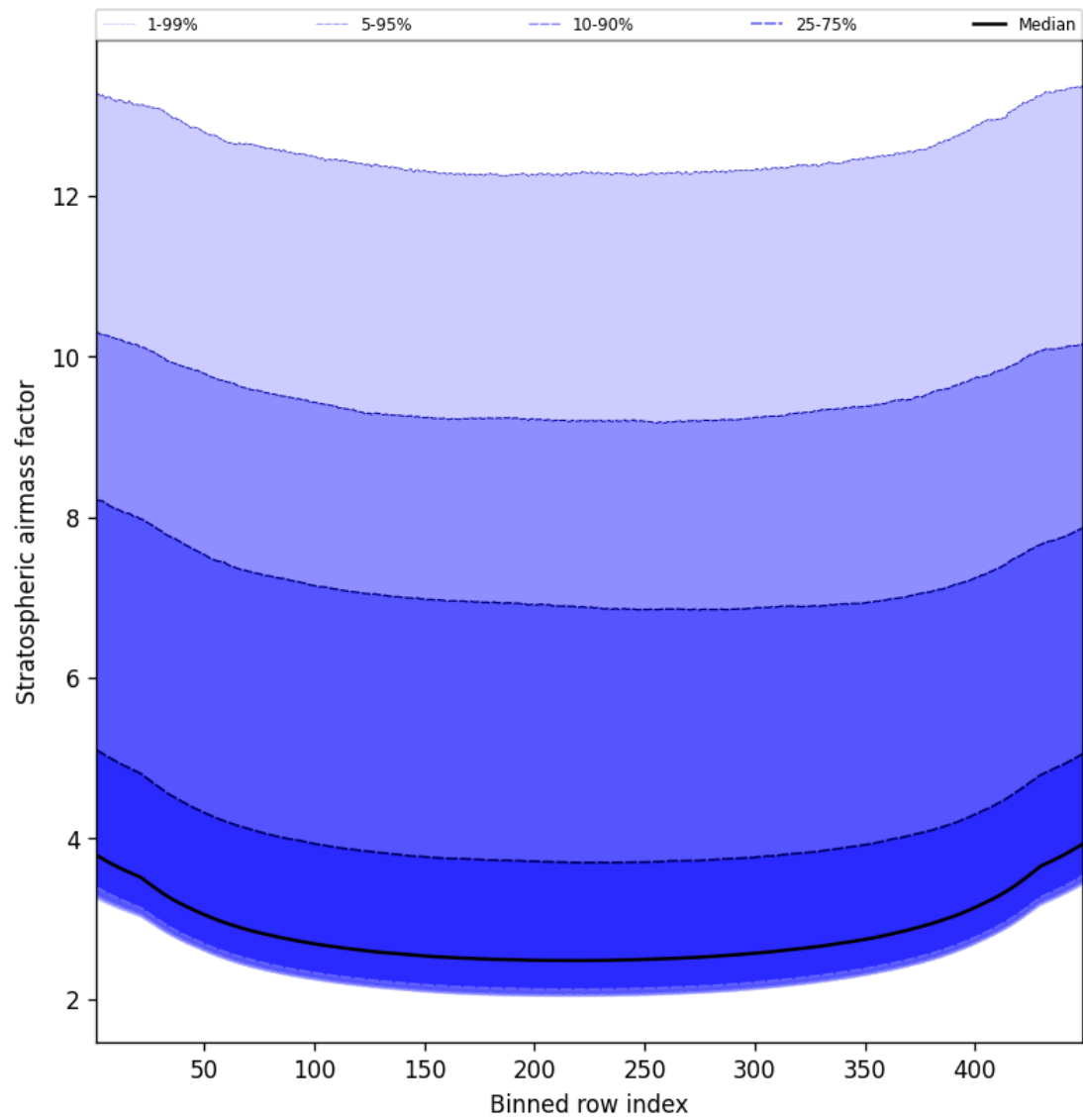
Figure 59: Along track statistics of “Stratospheric airmass factor” for 2025-02-08 to 2025-02-09
