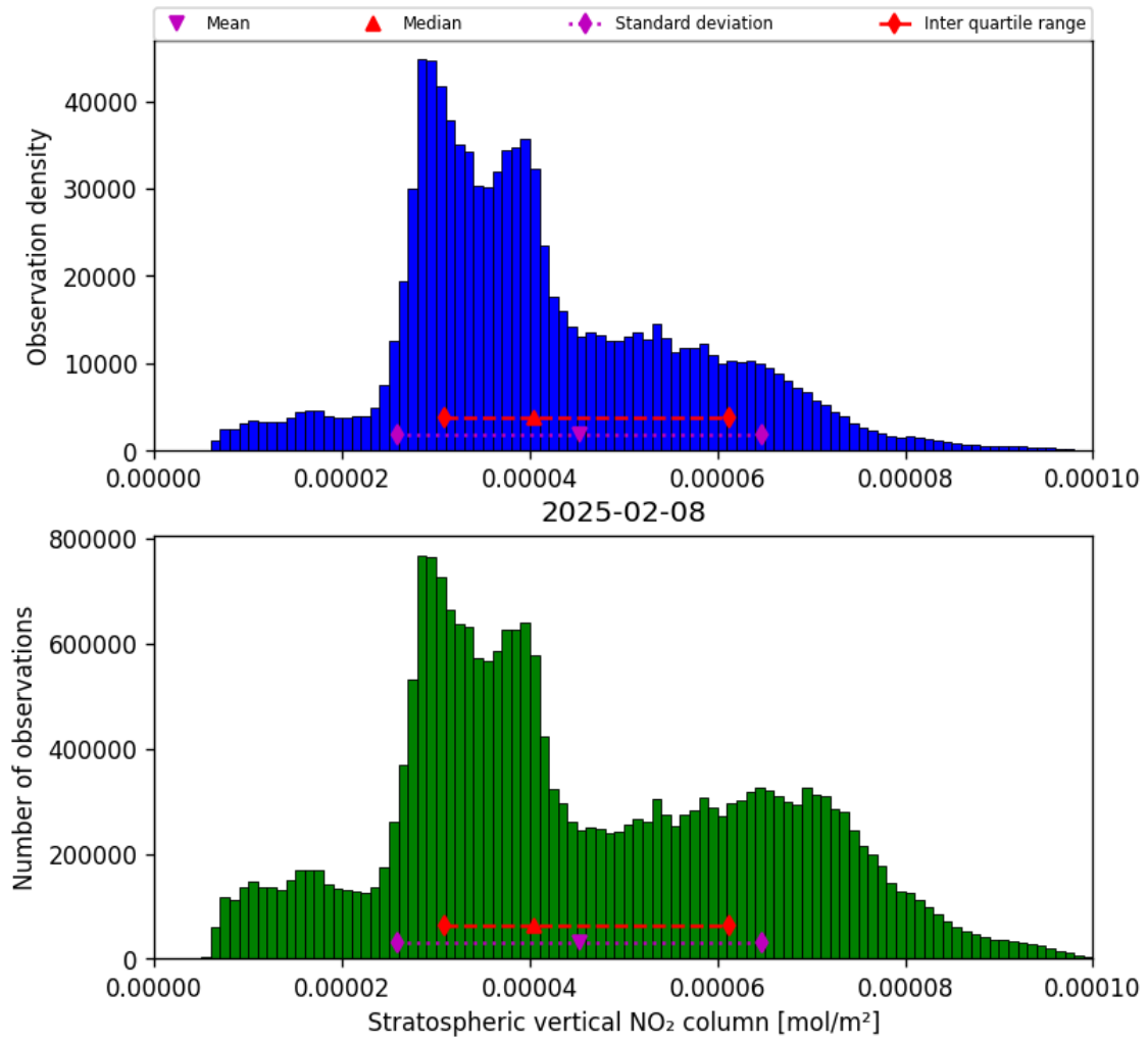
Figure 34: Histogram of “Stratospheric vertical NO 2 column” for 2025-02-08 to 2025-02-09
