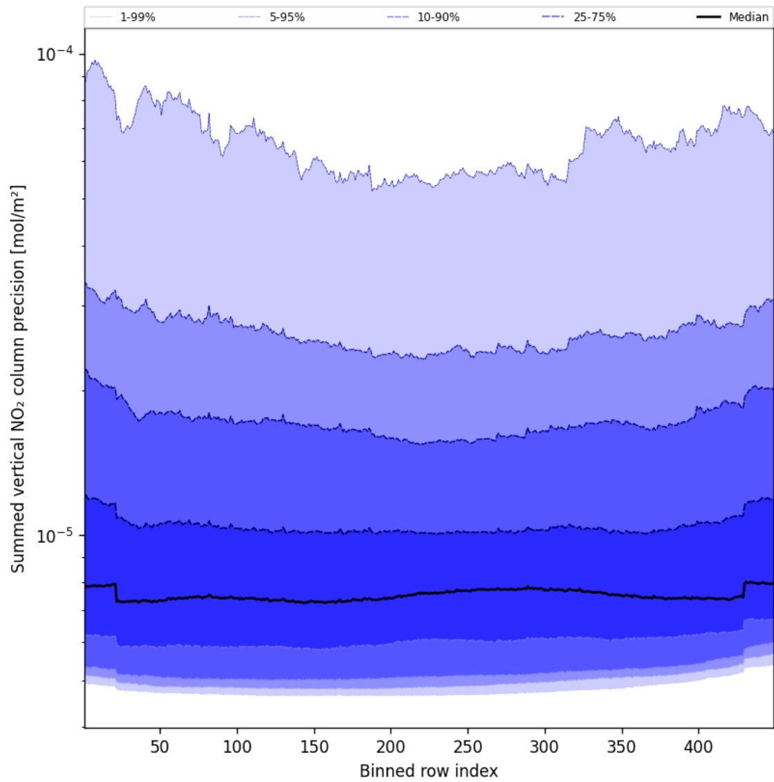
Figure 56: Along track statistics of “Summed vertical NO 2 column precision” for 2025-02-08 to 2025-02-09
