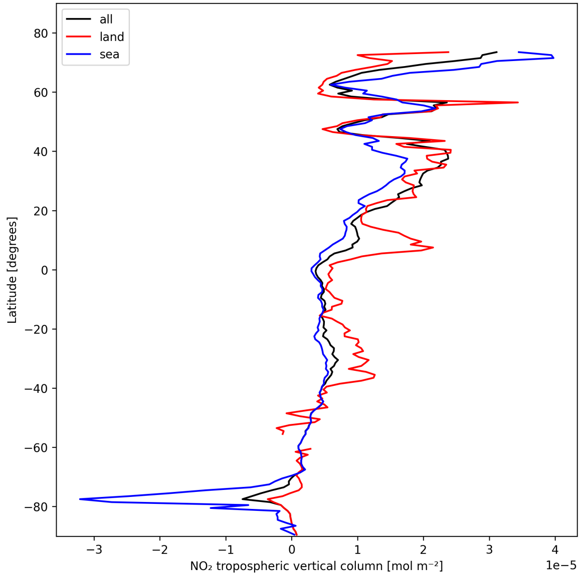
Figure 10: Zonal average of “NO 2 tropospheric vertical column” for 2025-02-08 to 2025-02-09.
