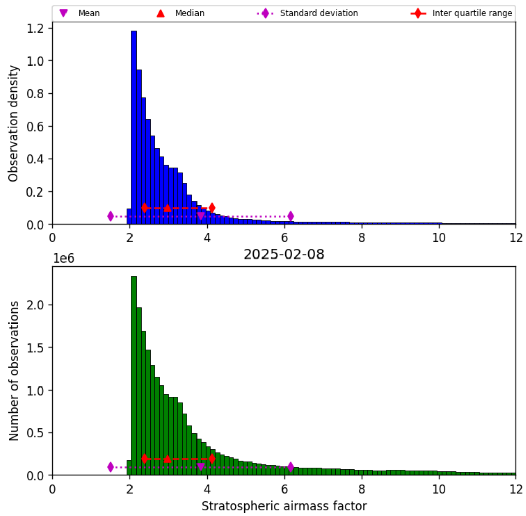
Figure 42: Histogram of “Stratospheric airmass factor” for 2025-02-08 to 2025-02-09
