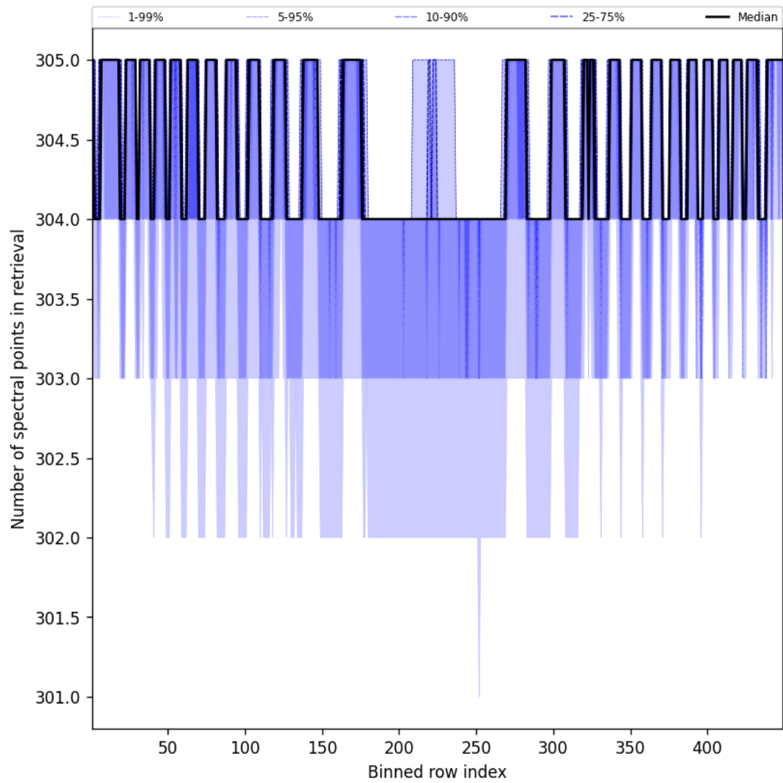
Figure 48: Along track statistics of “Number of spectral points in retrieval” for 2025-02-08 to 2025-02-09
