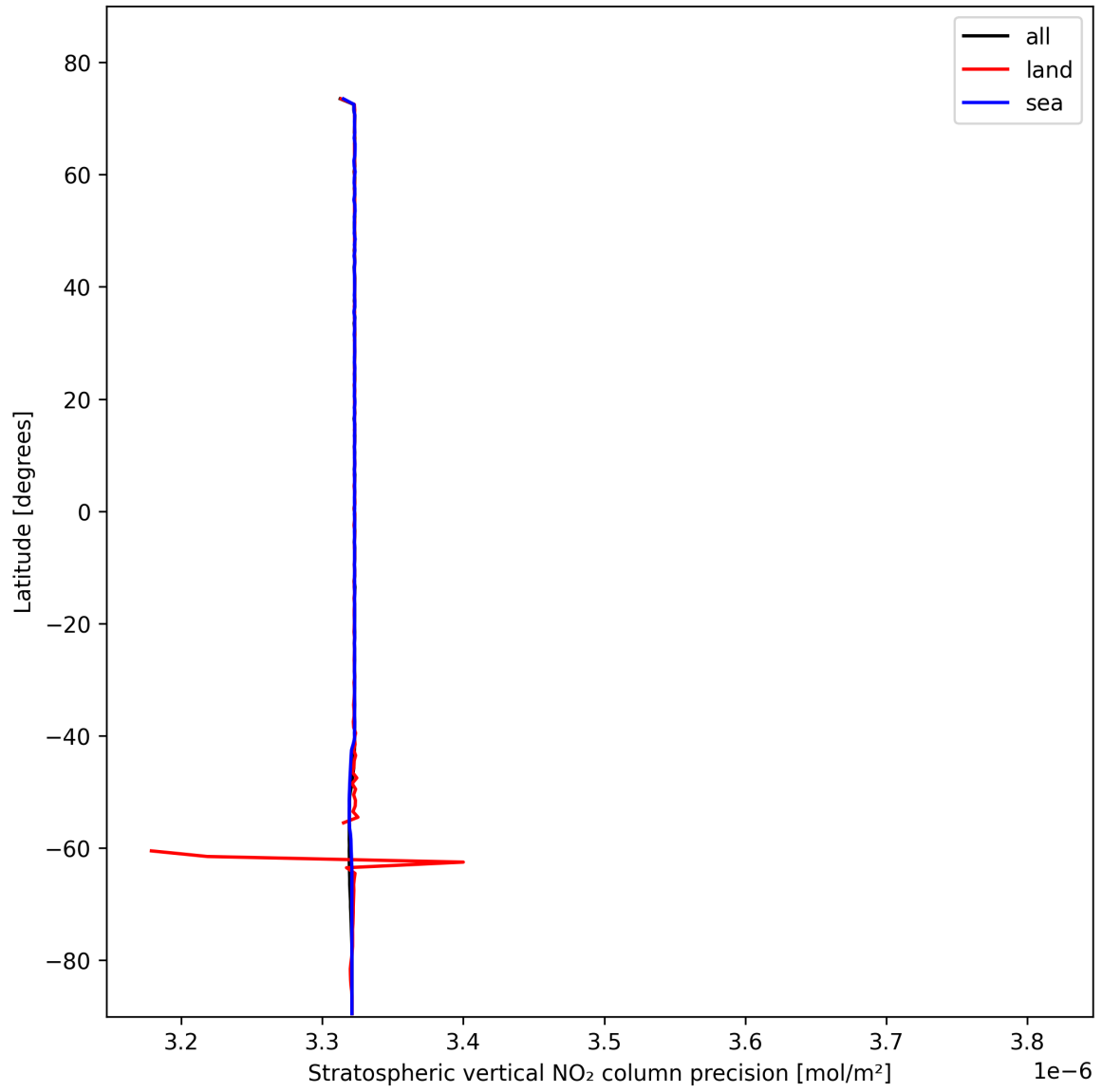
Figure 18: Zonal average of “Stratospheric vertical NO 2 column precision” for 2025-02-08 to 2025-02-09.
