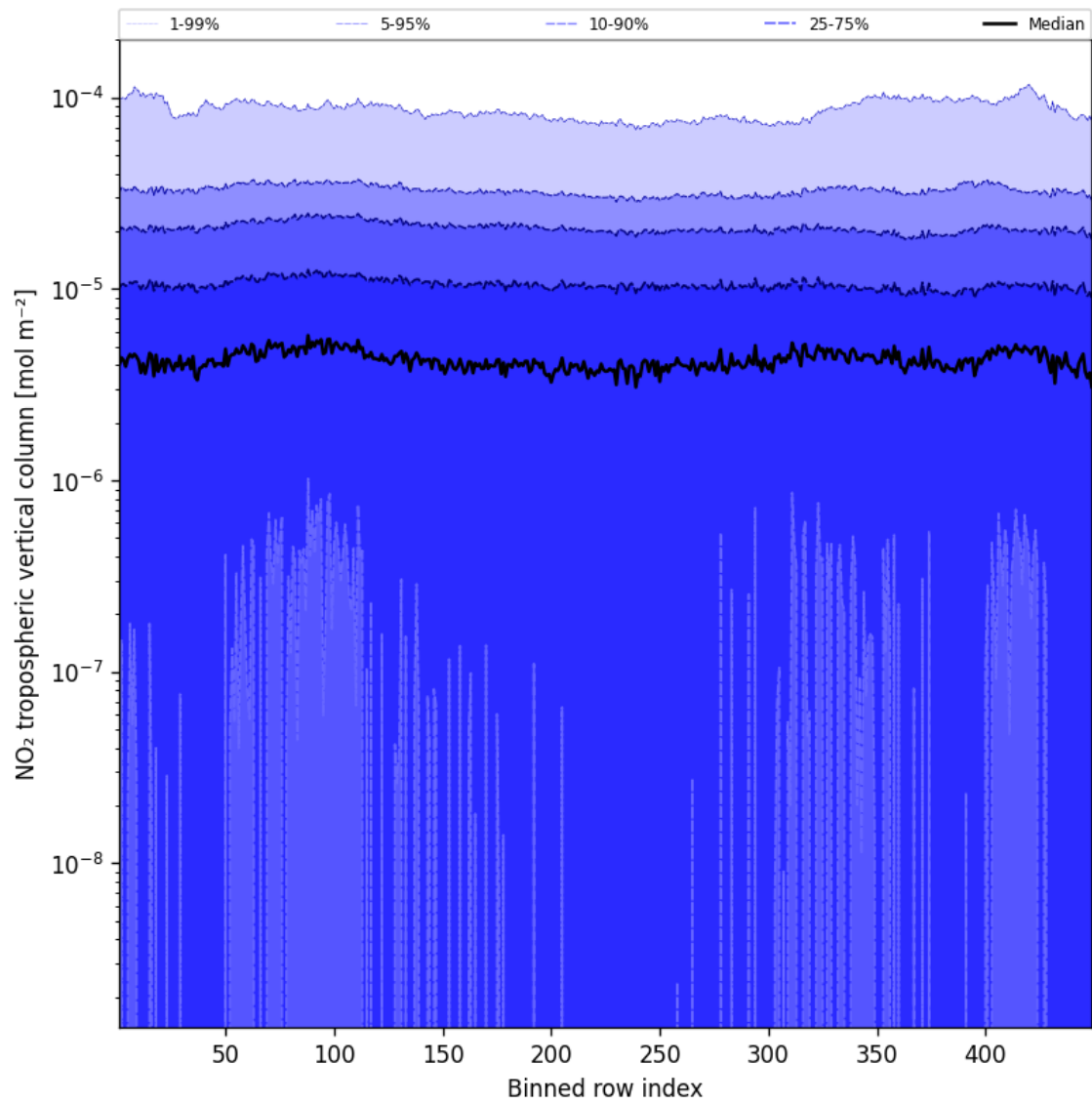
Figure 44: Along track statistics of “NO 2 tropospheric vertical column” for 2025-02-08 to 2025-02-09
