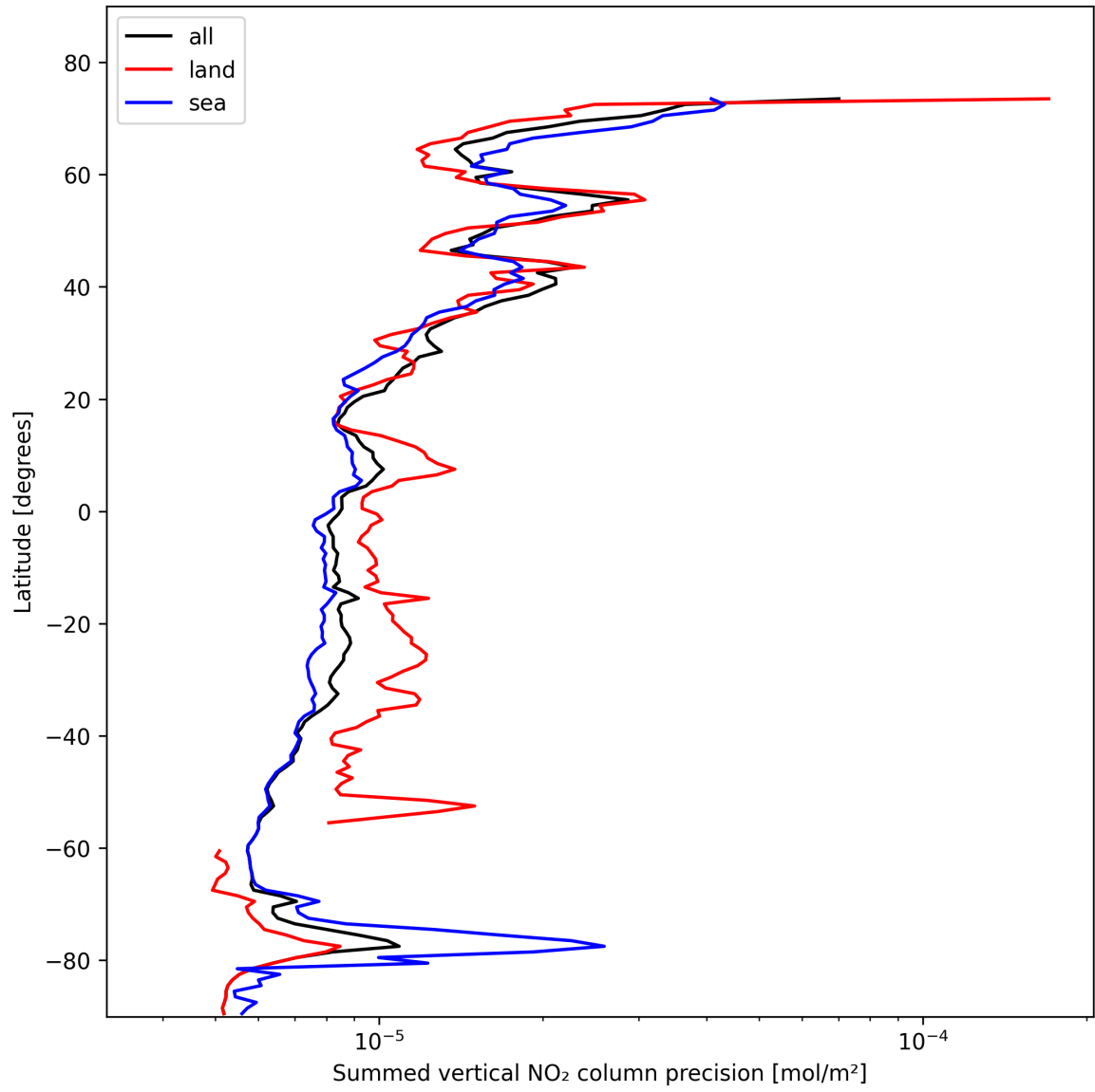
Figure 22: Zonal average of “Summed vertical NO 2 column precision” for 2025-02-08 to 2025-02-09.
