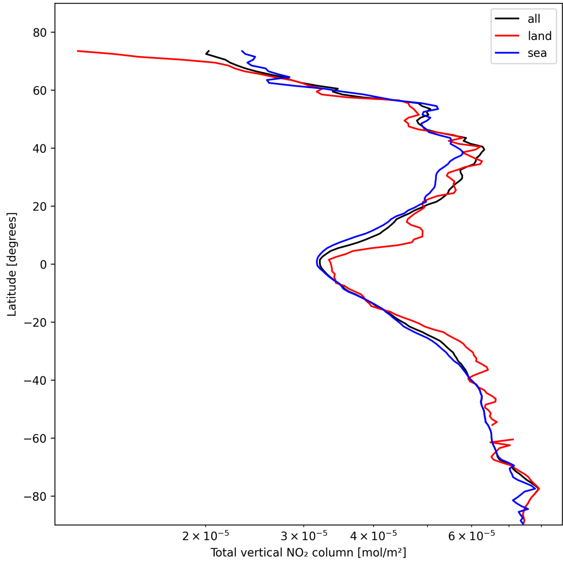
Figure 19: Zonal average of “Total vertical NO 2 column” for 2025-02-08 to 2025-02-09.
