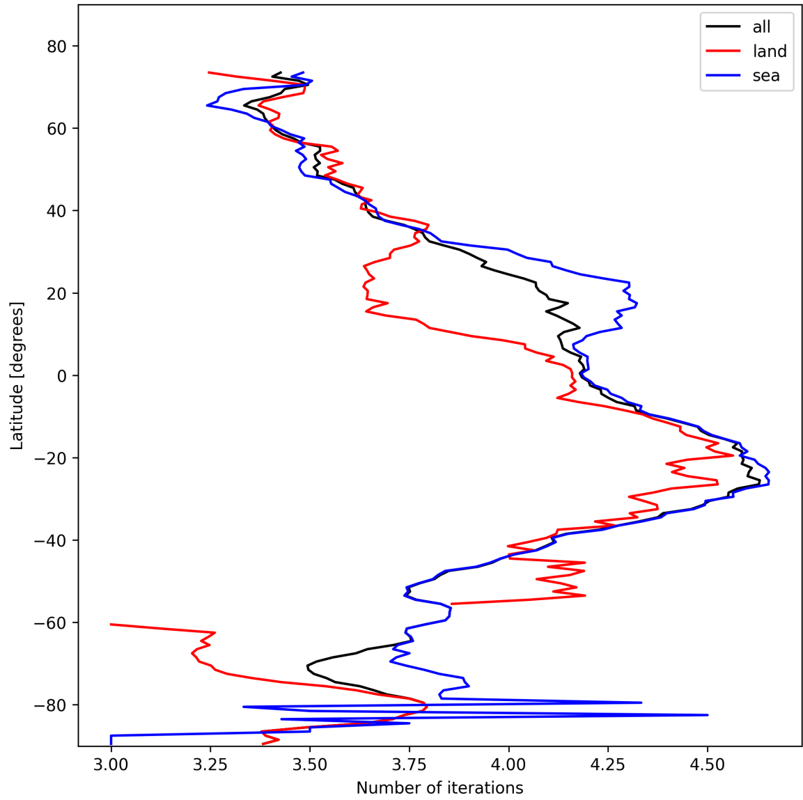
Figure 15: Zonal average of “Number of iterations” for 2025-02-08 to 2025-02-09.
