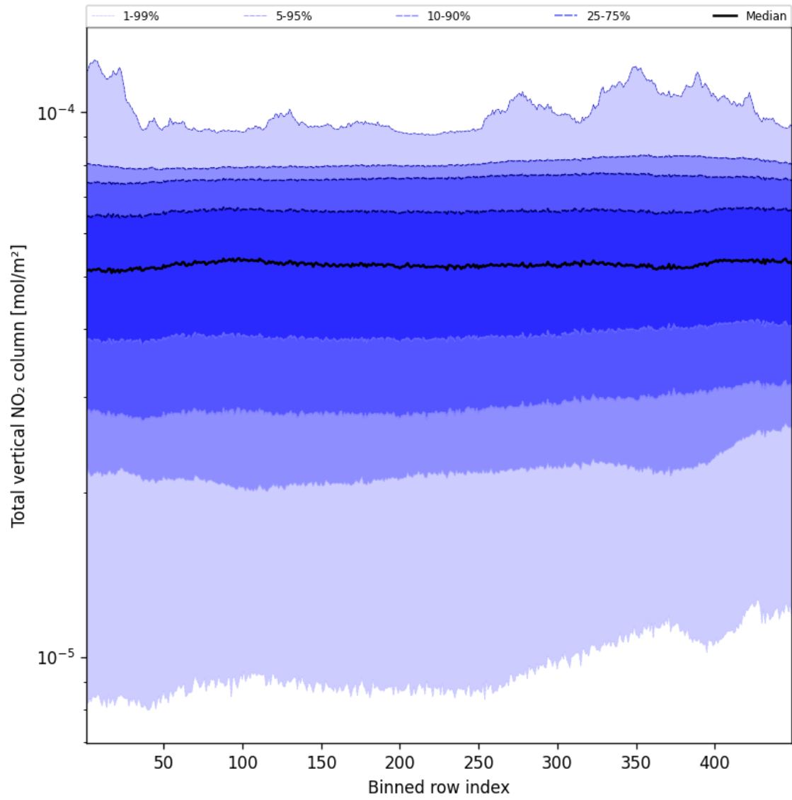
Figure 53: Along track statistics of “Total vertical NO 2 column” for 2025-02-08 to 2025-02-09
