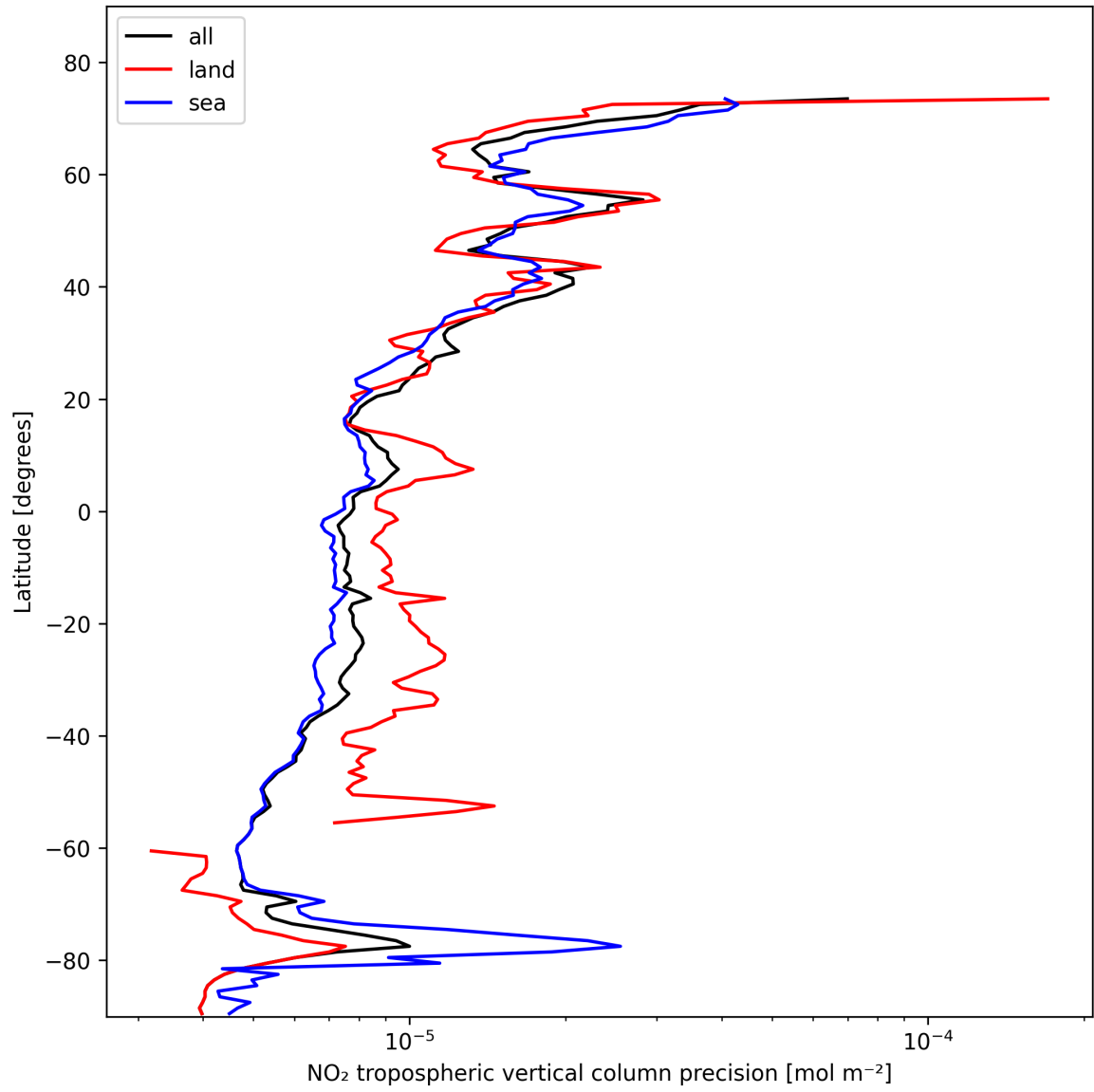
Figure 11: Zonal average of "NO 2 tropospheric vertical column precision" for 2025-02-08 to 2025-02-09.
