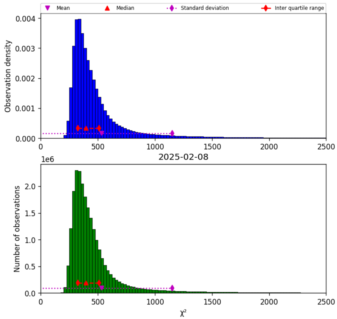
Figure 40: Histogram of “ \chi^2 ” for 2025-02-08 to 2025-02-09
