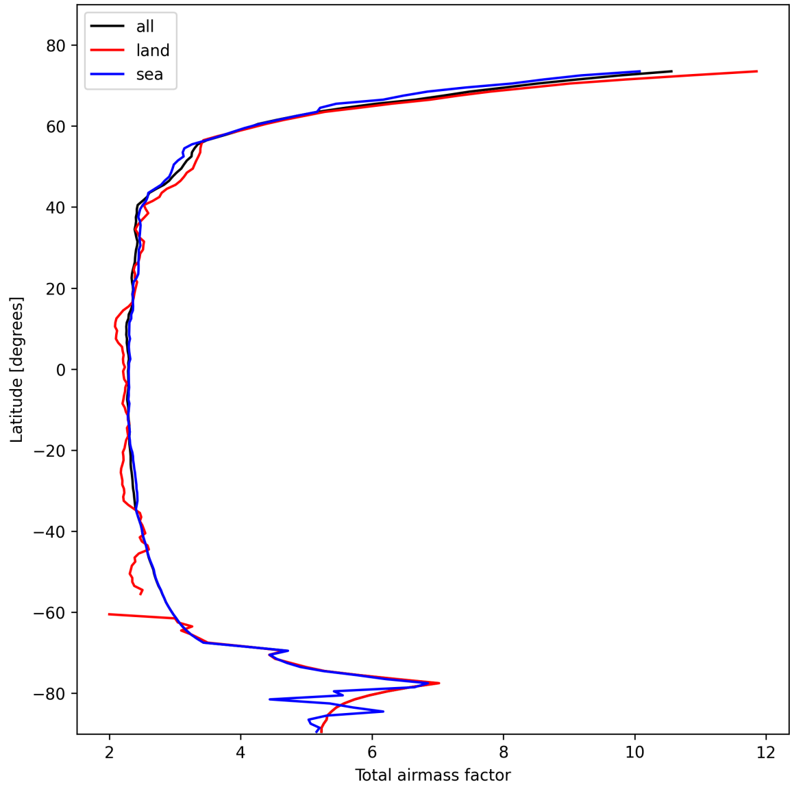
Figure 13: Zonal average of “Total airmass factor” for 2025-02-08 to 2025-02-09.
