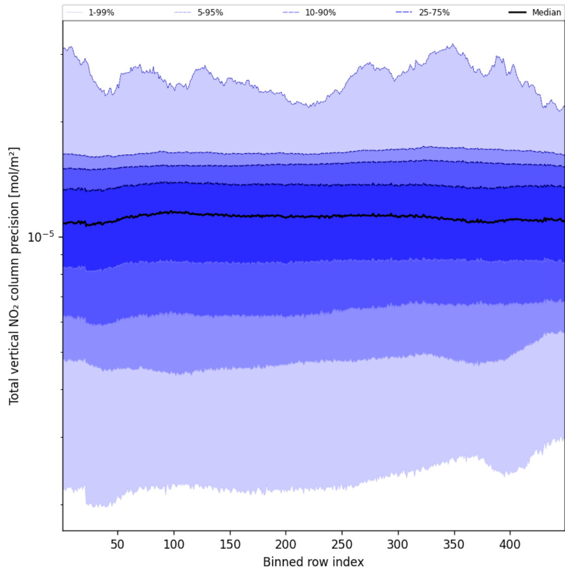
Figure 54: Along track statistics of “Total vertical NO 2 column precision” for 2025-02-08 to 2025-02-09
